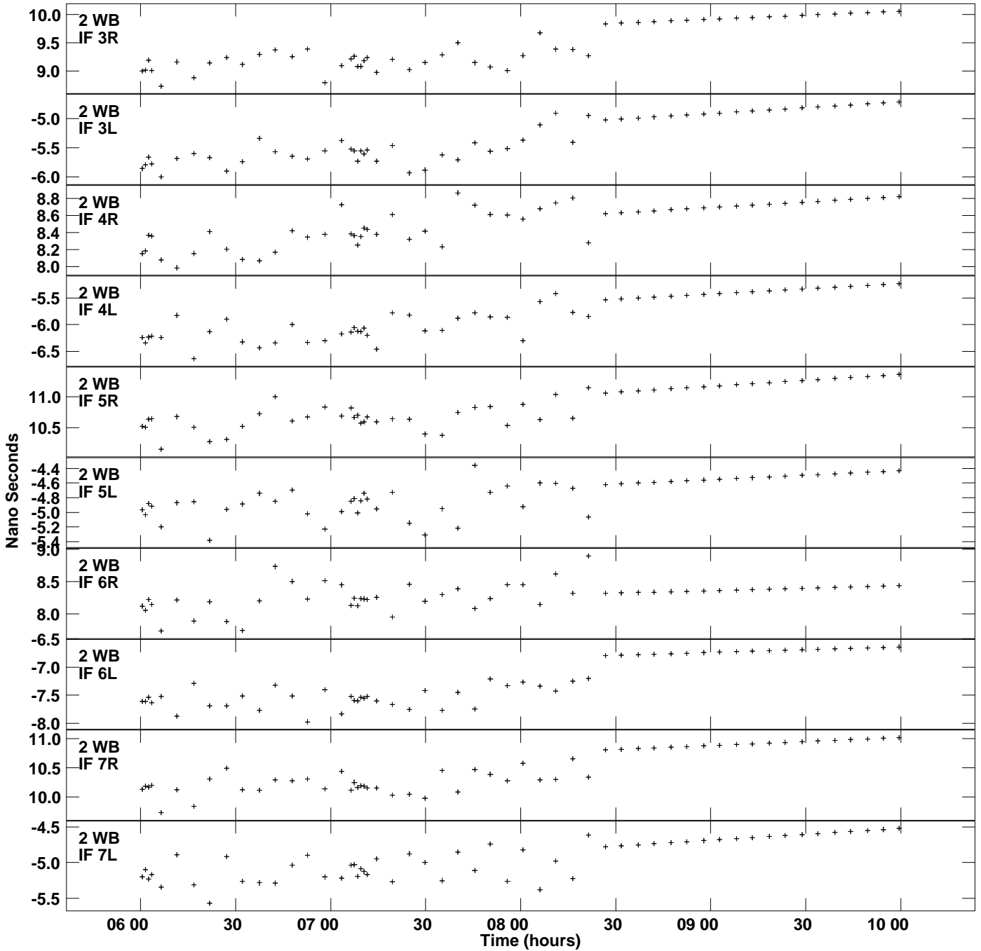
Plot file version 3 created 20-MAR-2014 14:47:07 Delay vs UTC time for ER030B.UVDATA.1 SN 2 Rpol & Lpol IF 1 - 8
