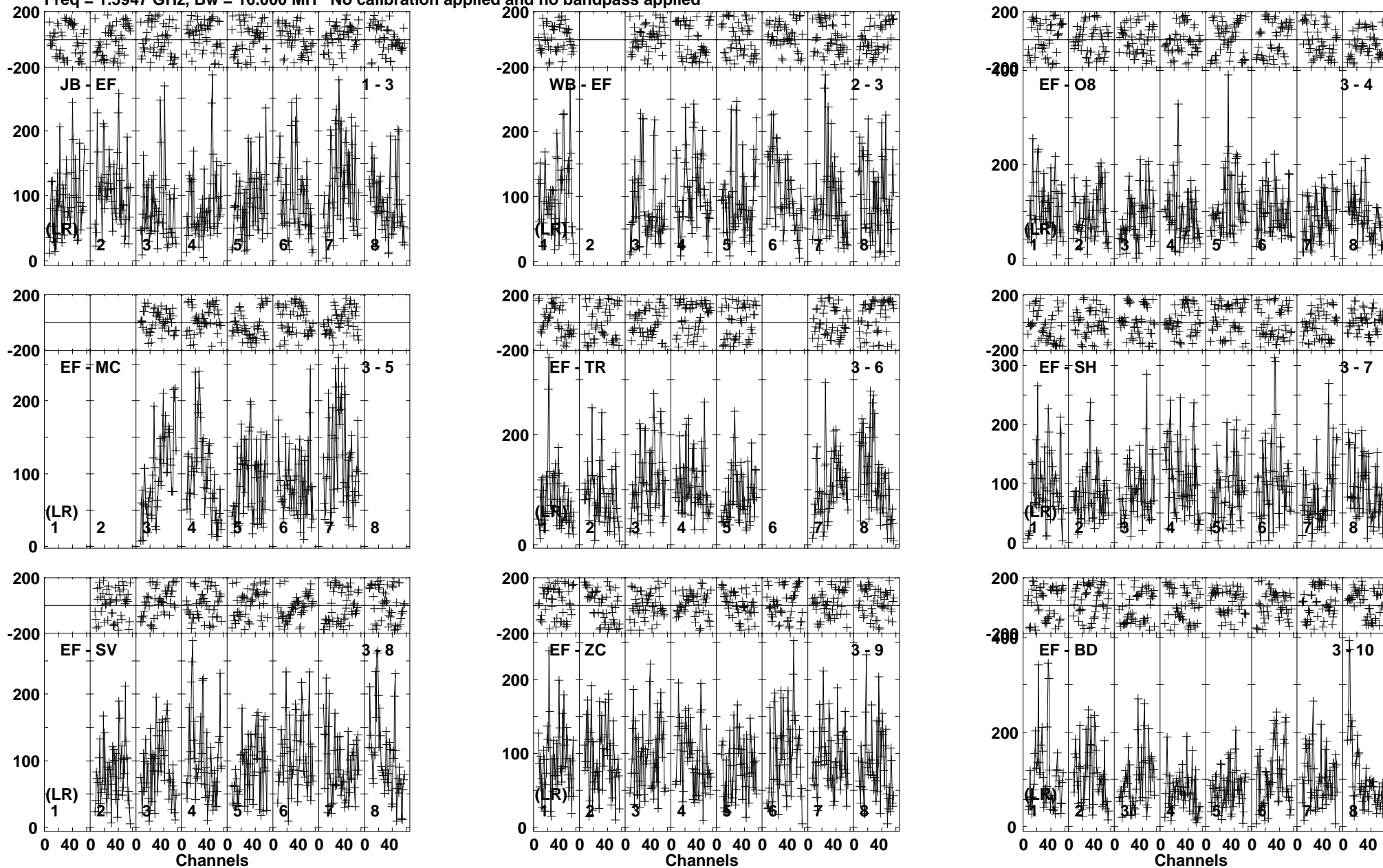
Lower frame: Micro Ampl Jy Top frame: Phas deg Vector averaged cross-power spectrum Baseline: JB (01) - EF (03) Timerange: 00/18:30:04 to 00/18:33:38
