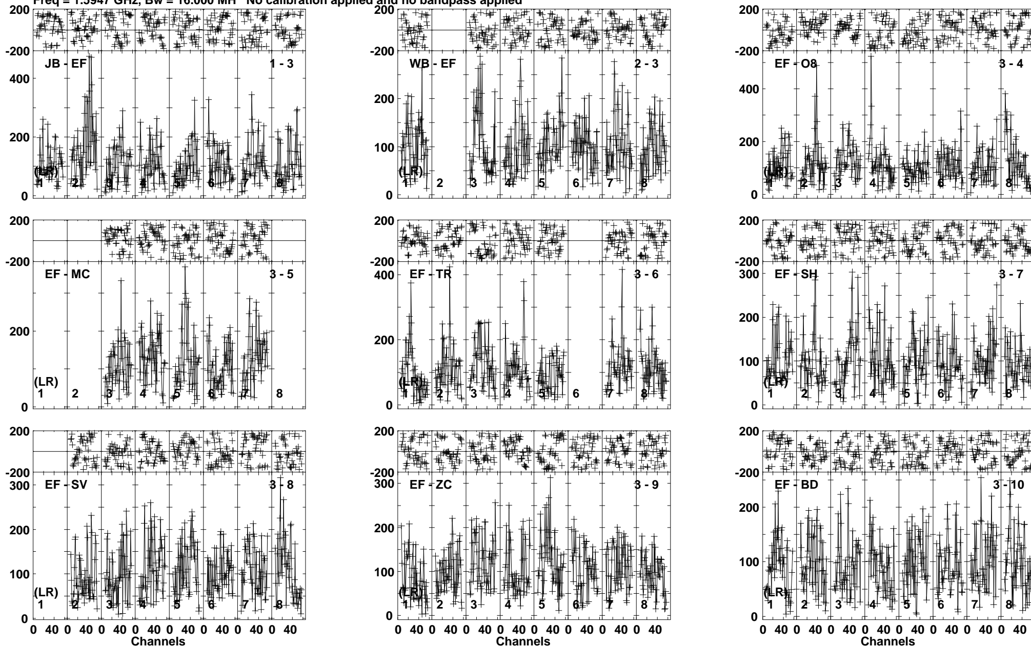
Lower frame: Micro Ampl Jy Top frame: Phas deg Vector averaged cross-power spectrum Baseline: JB (01) - EF (03) Timerange: 00/19:17:46 to 00/19:21:18
