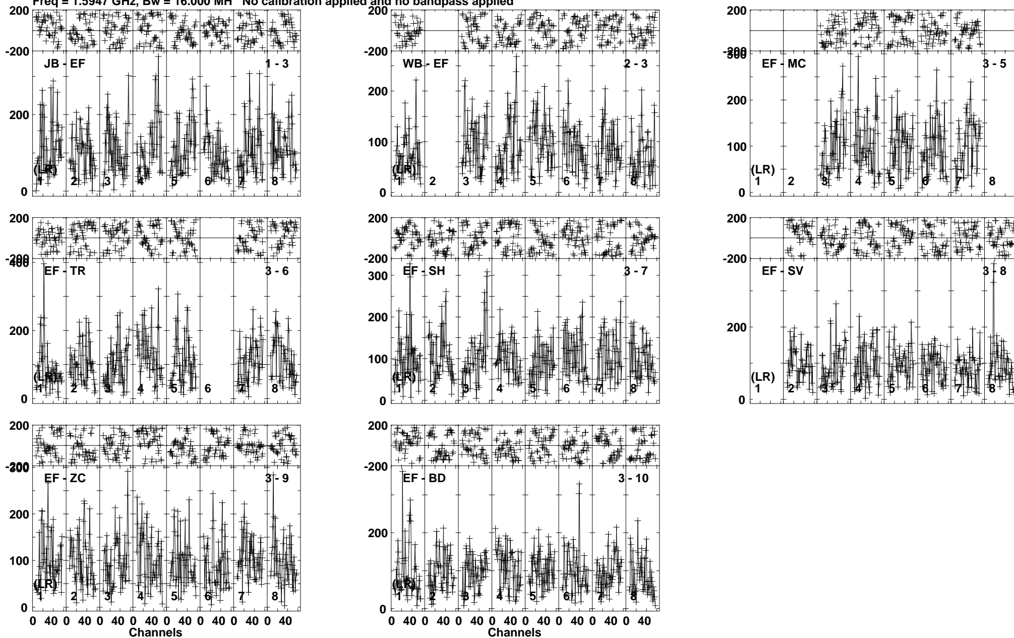
Lower frame: Micro Ampl Jy Top frame: Phas deg Vector averaged cross-power spectrum Baseline: JB (01) - EF (03) Timerange: 00/17:54:03 to 00/17:57:39
