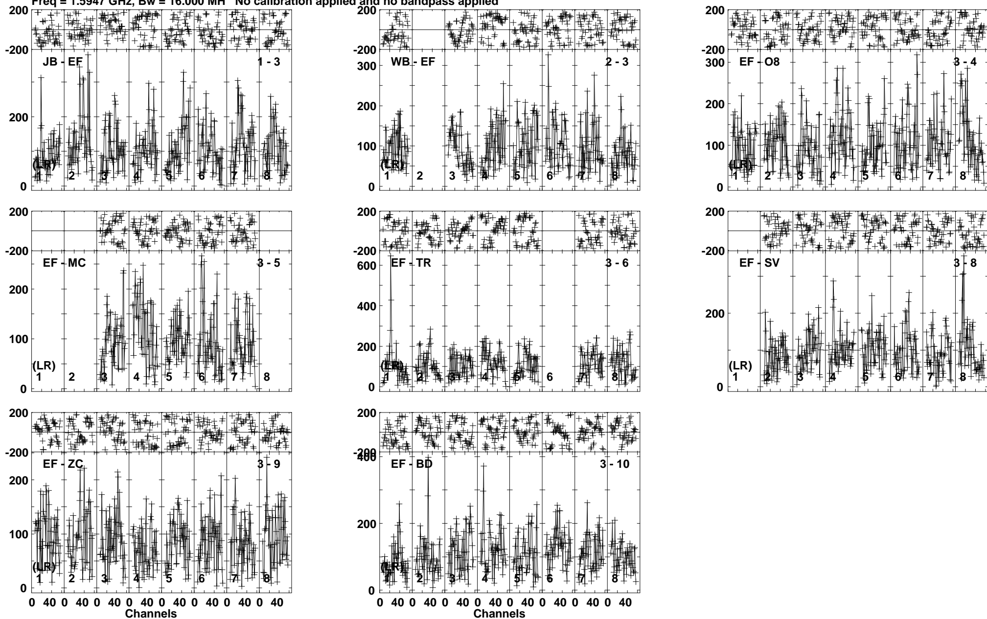
Lower frame: Micro Ampl Jy Top frame: Phas deg Vector averaged cross-power spectrum Baseline: JB (01) - EF (03) Timerange: 00/20:35:54 to 00/20:39:18
