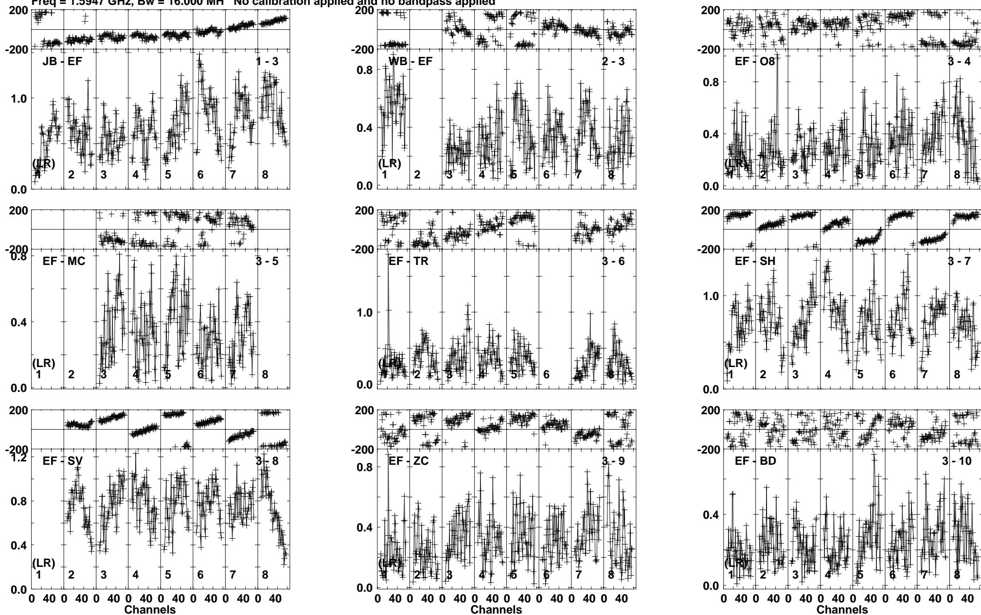
Lower frame: Milli Ampl Jy Top frame: Phas deg Vector averaged cross-power spectrum Baseline: JB (01) - EF (03) Timerange: 00/18:44:26 to 00/18:45:38
