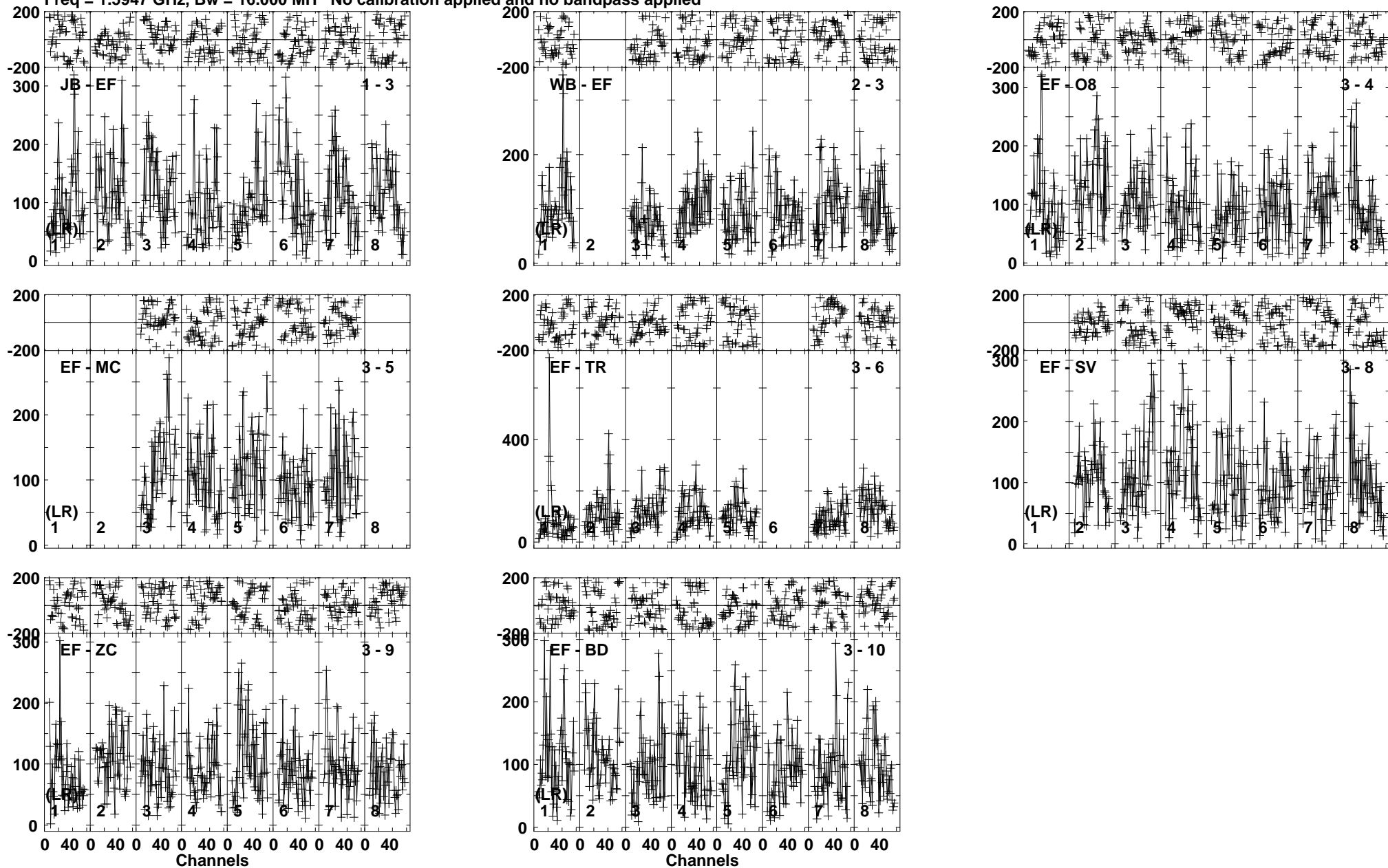
Lower frame: Micro Ampl Jy Top frame: Phas deg Vector averaged cross-power spectrum Baseline: JB (01) - EF (03) Timerange: 00/21:21:22 to 00/21:24:44
