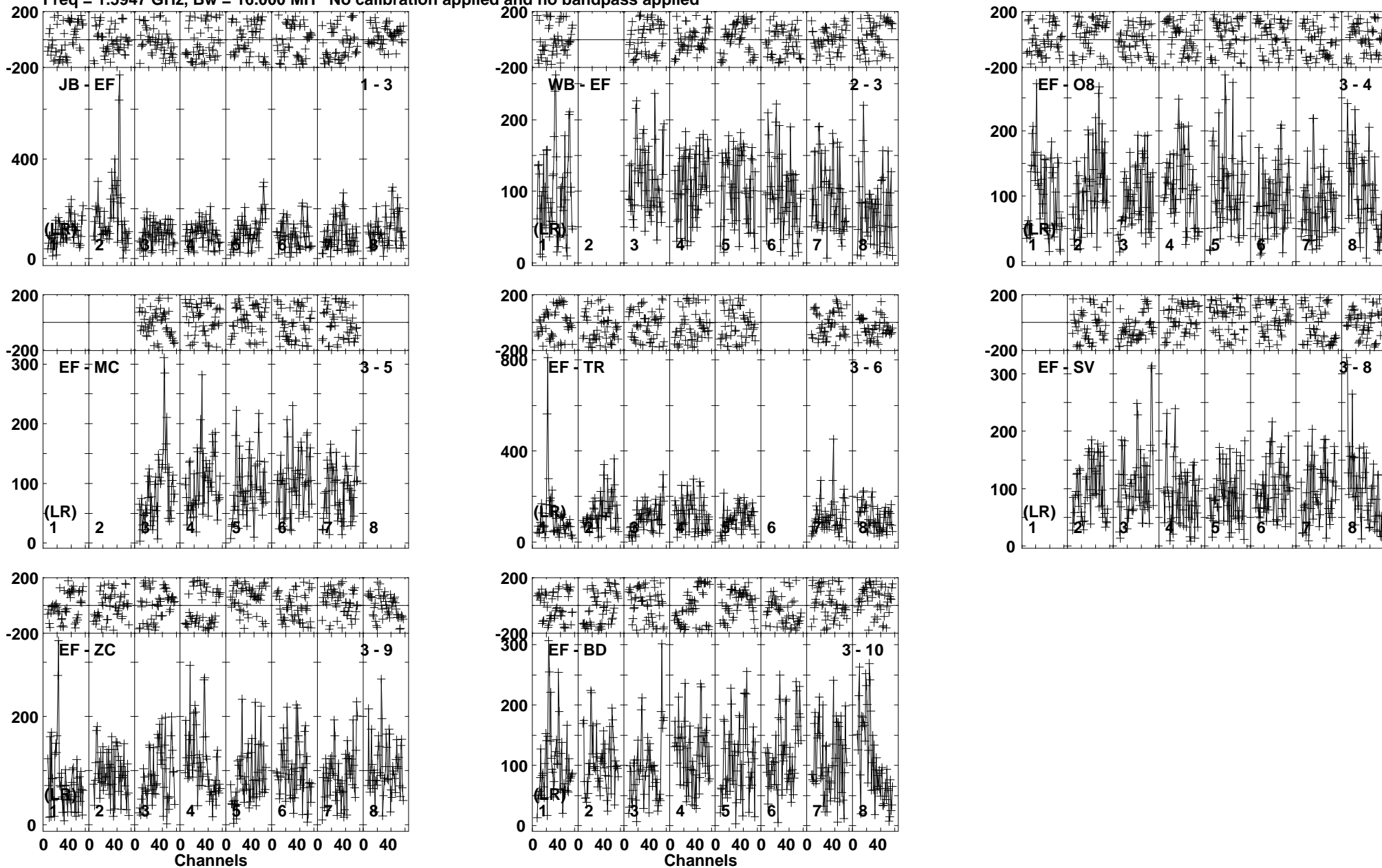
Lower frame: Micro Ampl Jy Top frame: Phas deg Vector average cross-power spectrum Baseline: JB (01) - EF (03) Timerange: 00/21:01:02 to 00/21:04:24
