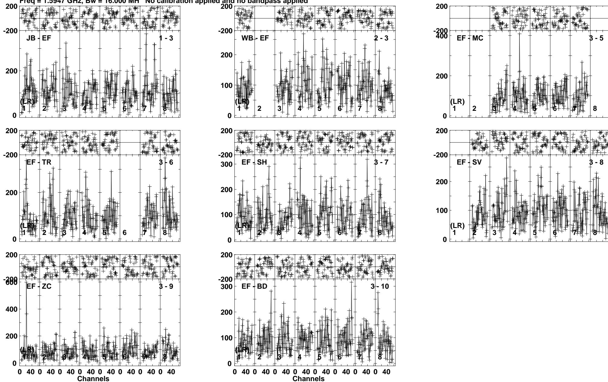
Lower frame: Micro Ampl Jy Top frame: Phas deg Vector average cross-power spectrum Baseline: JB (01) - EF (03) Timerange: 00/15:15:46 to 00/15:19:18
