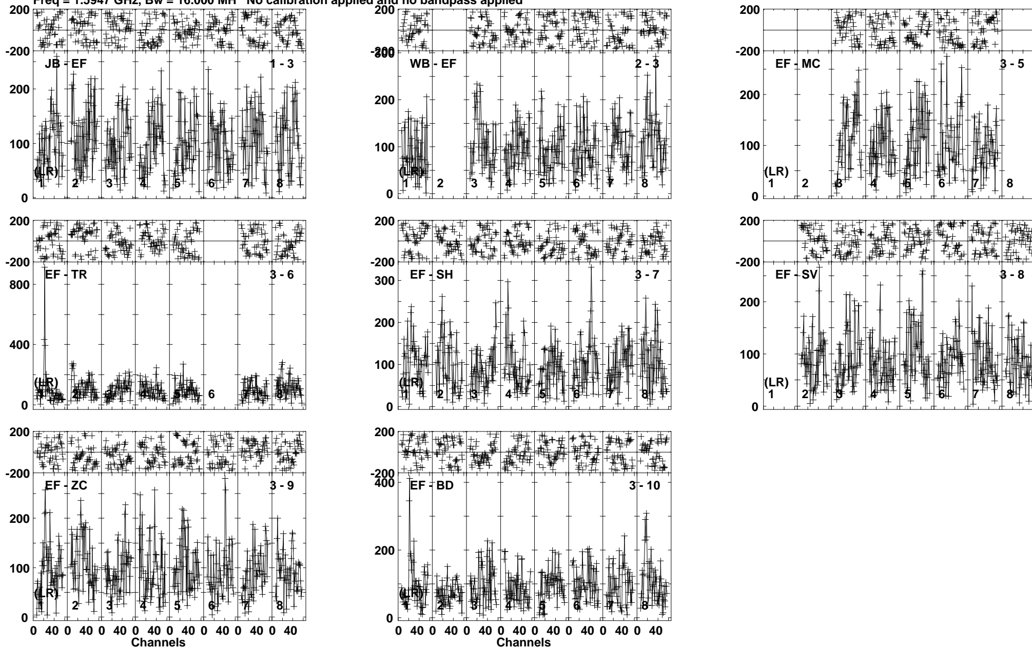
Lower frame: Micro Ampl Jy Top frame: Phas deg Vector average cross-power spectrum Baseline: JB (01) - EF (03) Timerange: 00/15:53:24 to 00/15:56:58
