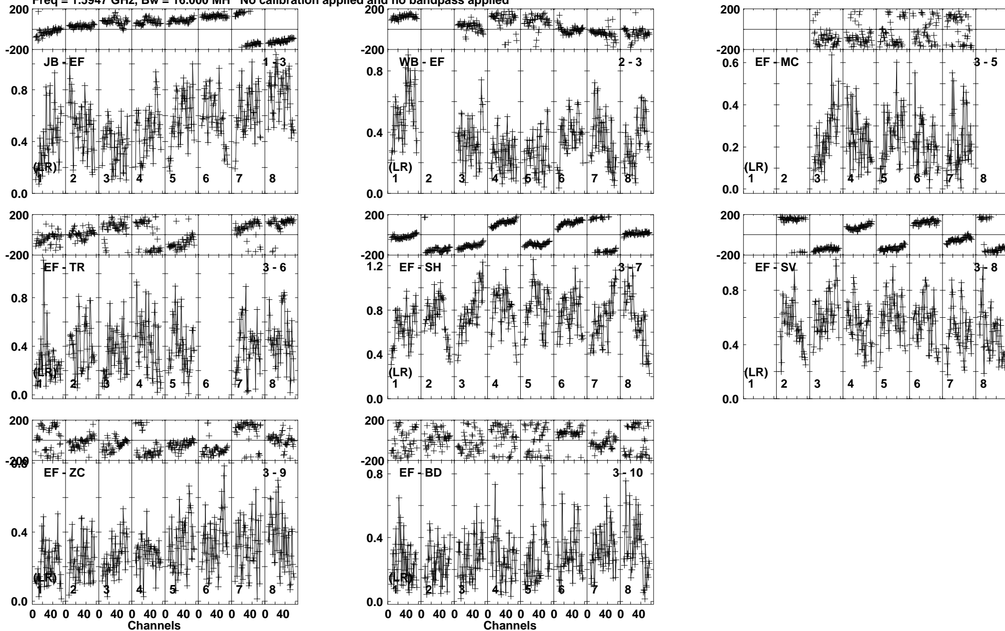
Lower frame: Milli Ampl Jy Top frame: Phas deg Vector averaged cross-power spectrum Baseline: JB (01) - EF (03) Timerange: 00/15:46:26 to 00/15:47:38
