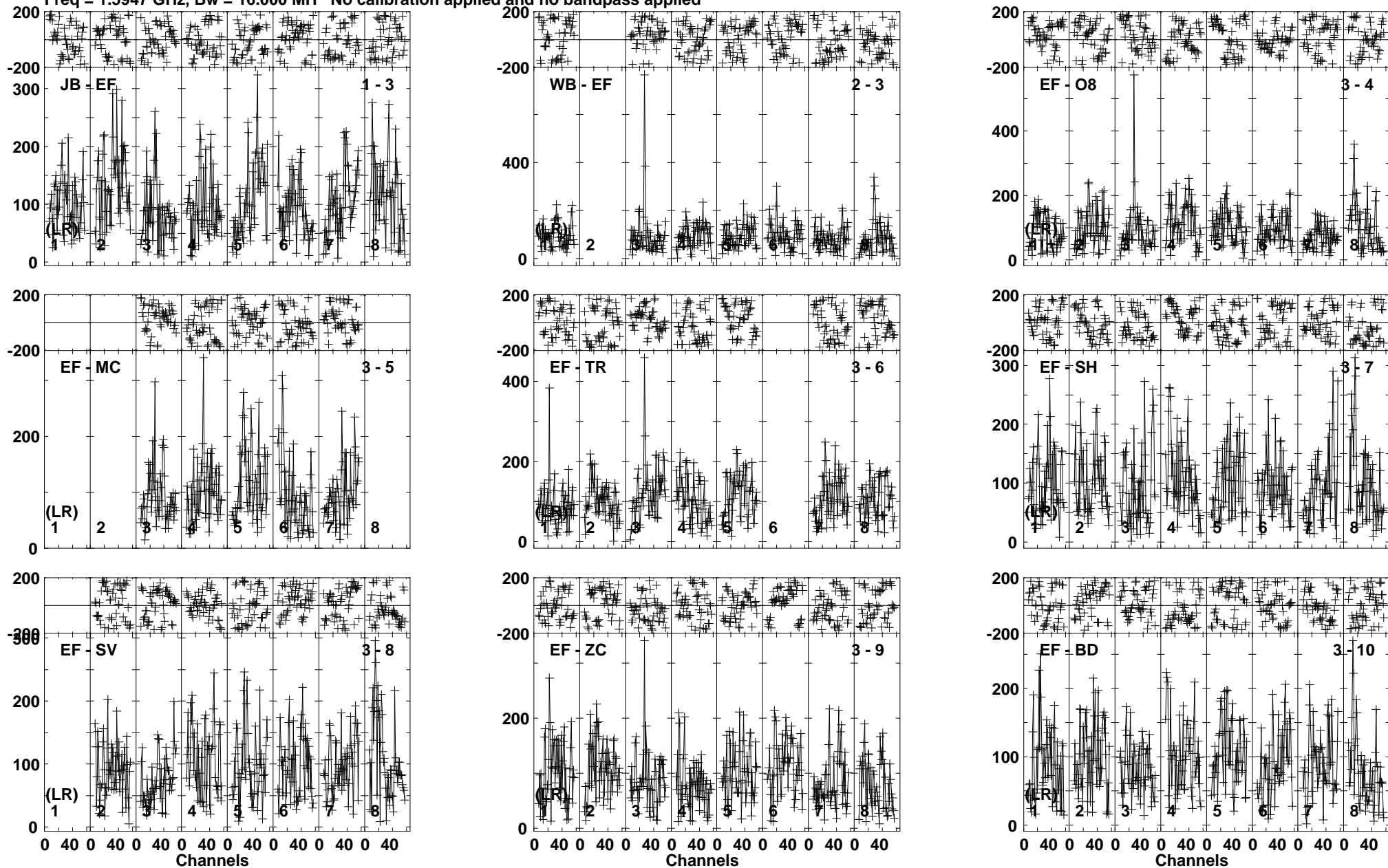
Lower frame: Micro Ampl Jy Top frame: Phas deg Vector averaged cross-power spectrum Baseline: JB (01) - EF (03) Timerange: 00/18:15:26 to 00/18:18:58
