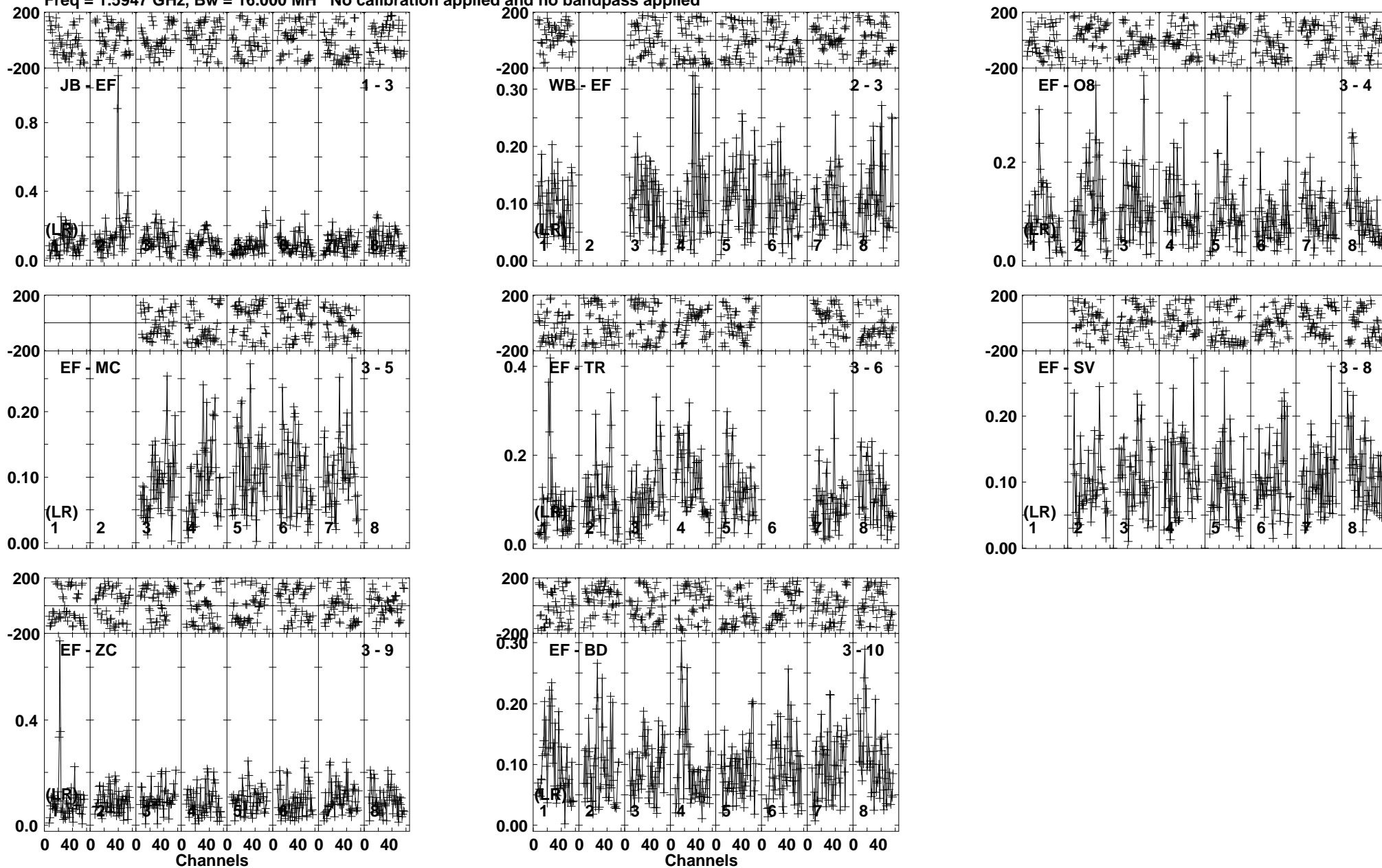
Lower frame: Milli Ampl Jy Top frame: Phas deg Vector average cross-power spectrum Baseline: JB (01) - EF (03) Timerange: 00/21:57:14 to 00/22:00:38
