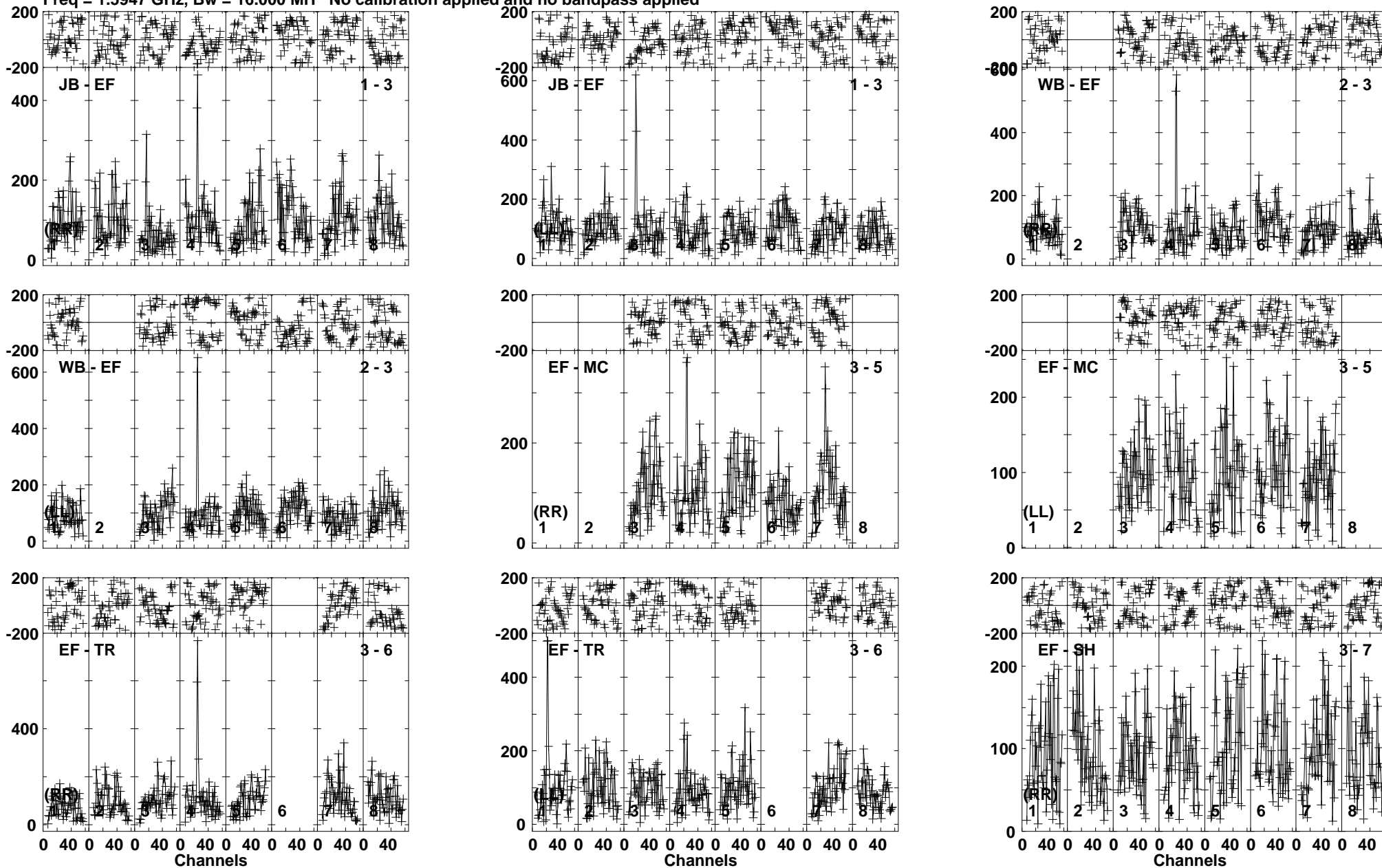
Lower frame: Micro Ampl Jy Top frame: Phas deg Vector averaged cross-power spectrum Baseline: JB (01) - EF (03) Timerange: 00/17:17:04 to 00/17:20:38
