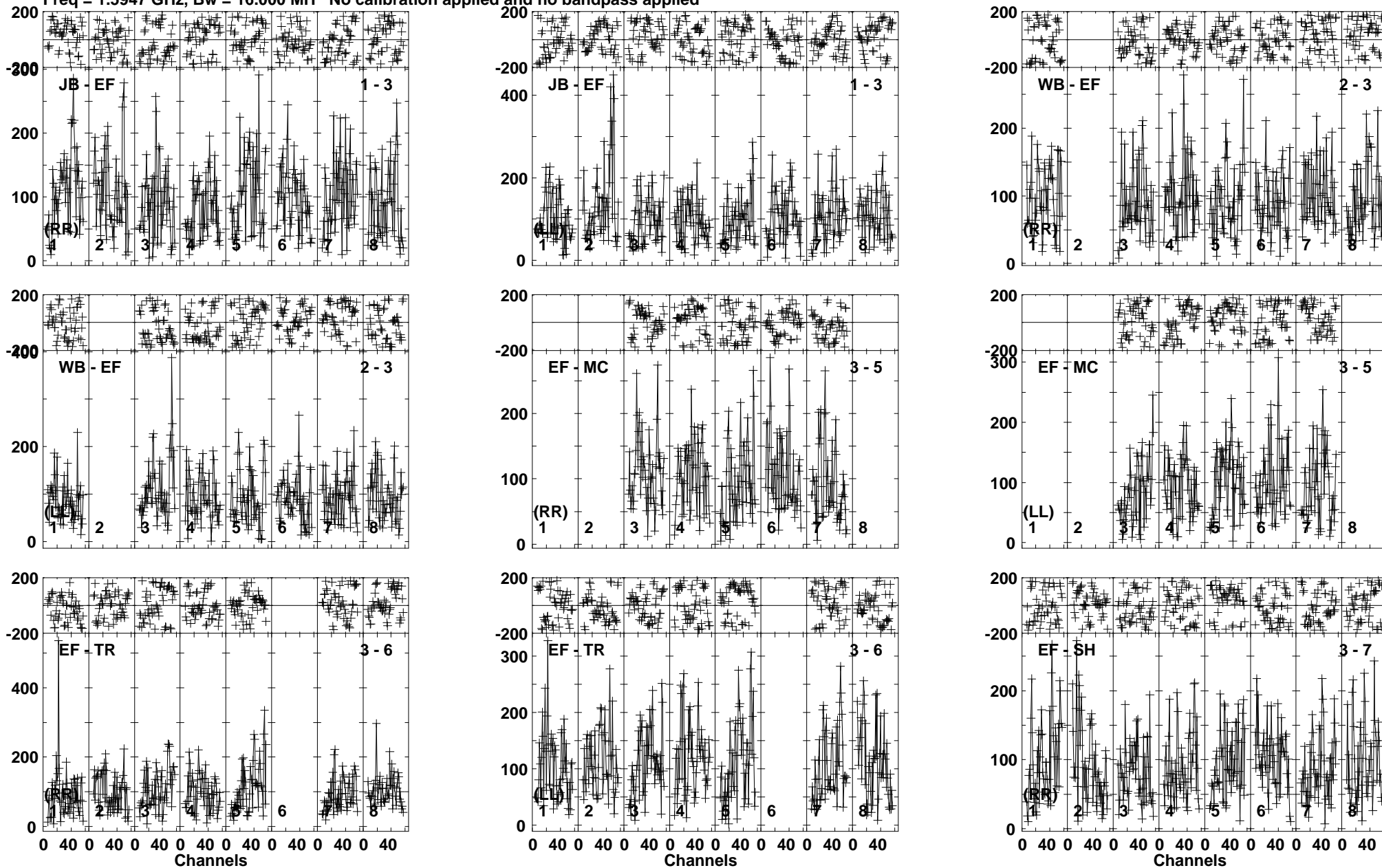
Lower frame: Micro Ampl Jy Top frame: Phas deg Vector averaged cross-power spectrum Baseline: JB (01) - EF (03) Timerange: 00/17:00:46 to 00/17:04:18
