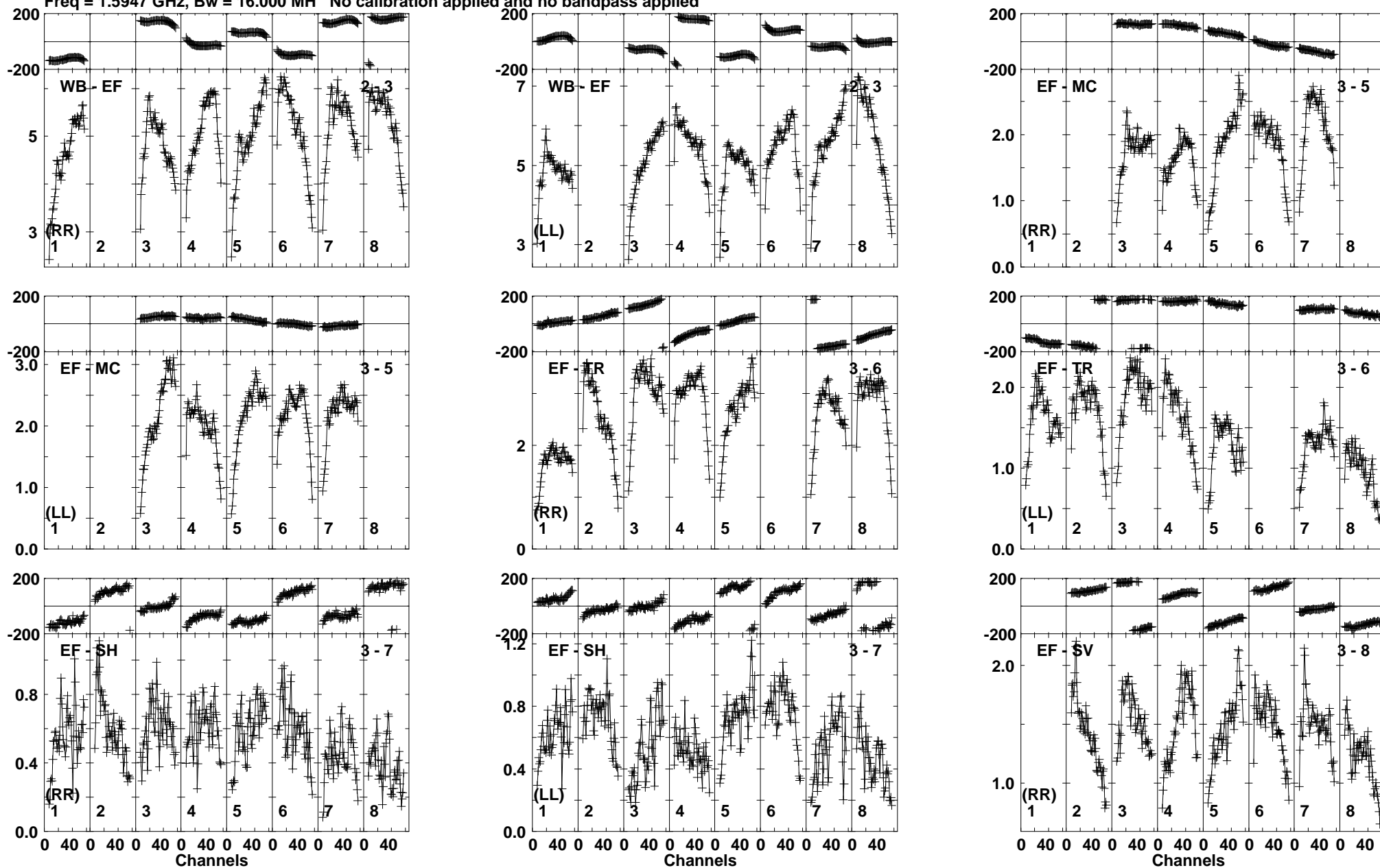
Lower frame: Milli Ampl Jy Top frame: Phas deg Vector averaged cross-power spectrum Baseline: WB (02) - EF (03) Timerange: 00/16:54:21 to 00/16:55:39
