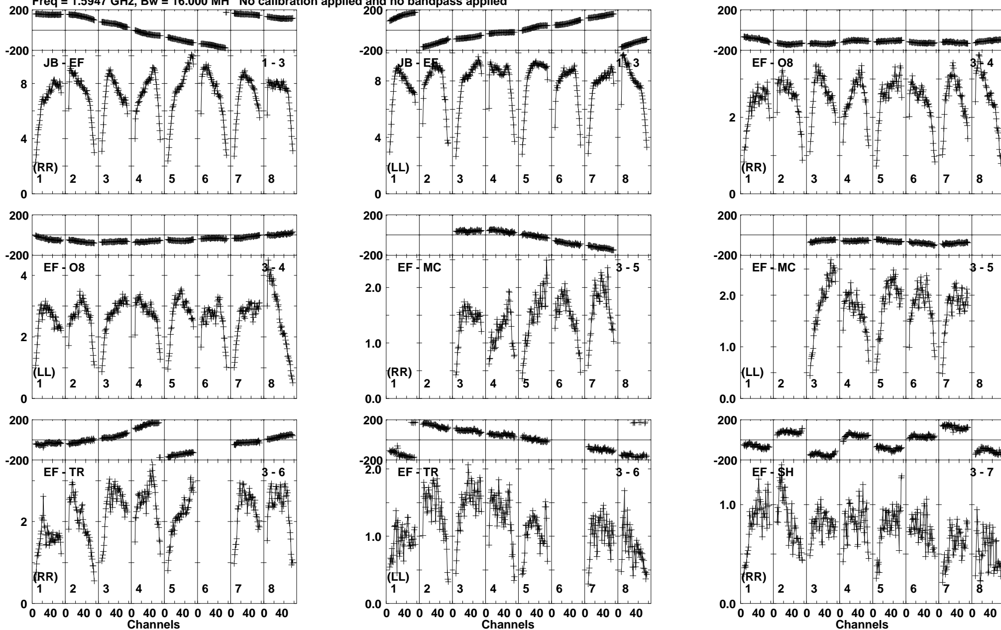
Lower frame: Milli Ampl Jy Top frame: Phas deg Vector averaged cross-power spectrum Baseline: JB (01) - EF (03) Timerange: 00:12:36:06 to 00:12:37:18
