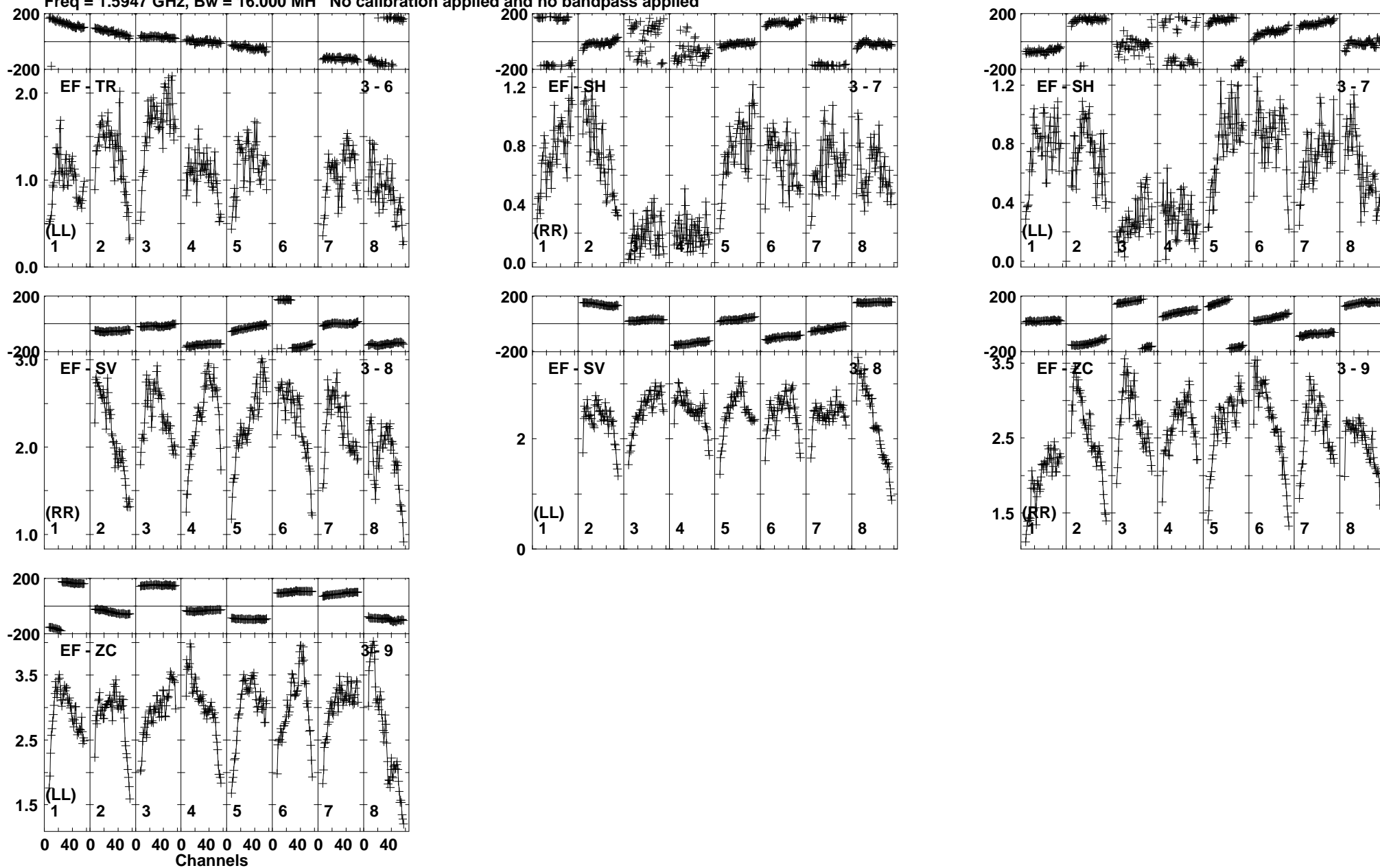
Lower frame: Milli Ampl Jy Top frame: Phas deg Vector averaged cross-power spectrum Baseline: EF (03) - TR (06) Timerange: 00/13:40:06 to 00/13:41:18
