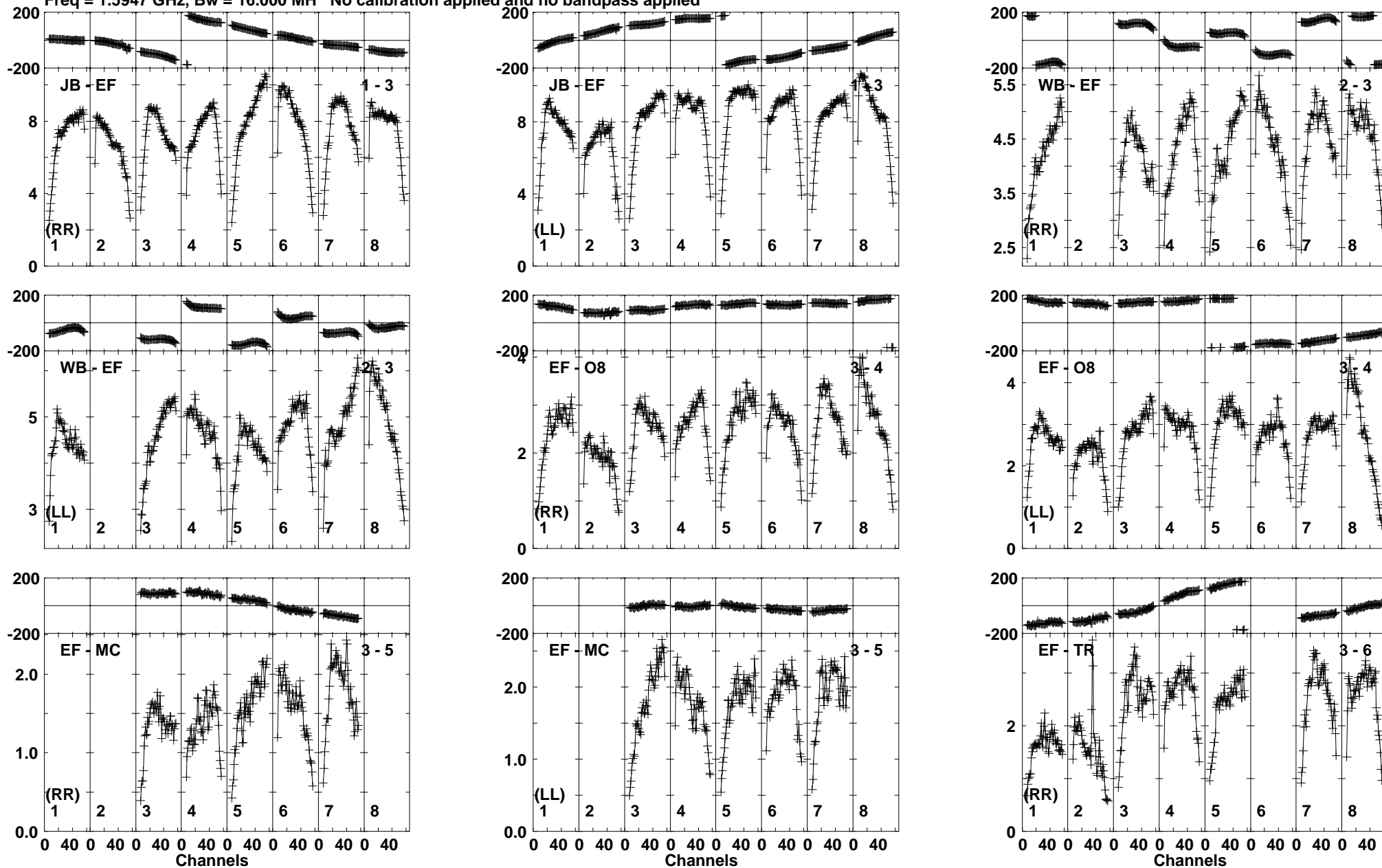
Lower frame: Milli Ampl Jy Top frame: Phas deg Vector averaged cross-power spectrum Baseline: JB (01) - EF (03) Timerange: 00/13:29:26 to 00/13:30:38
