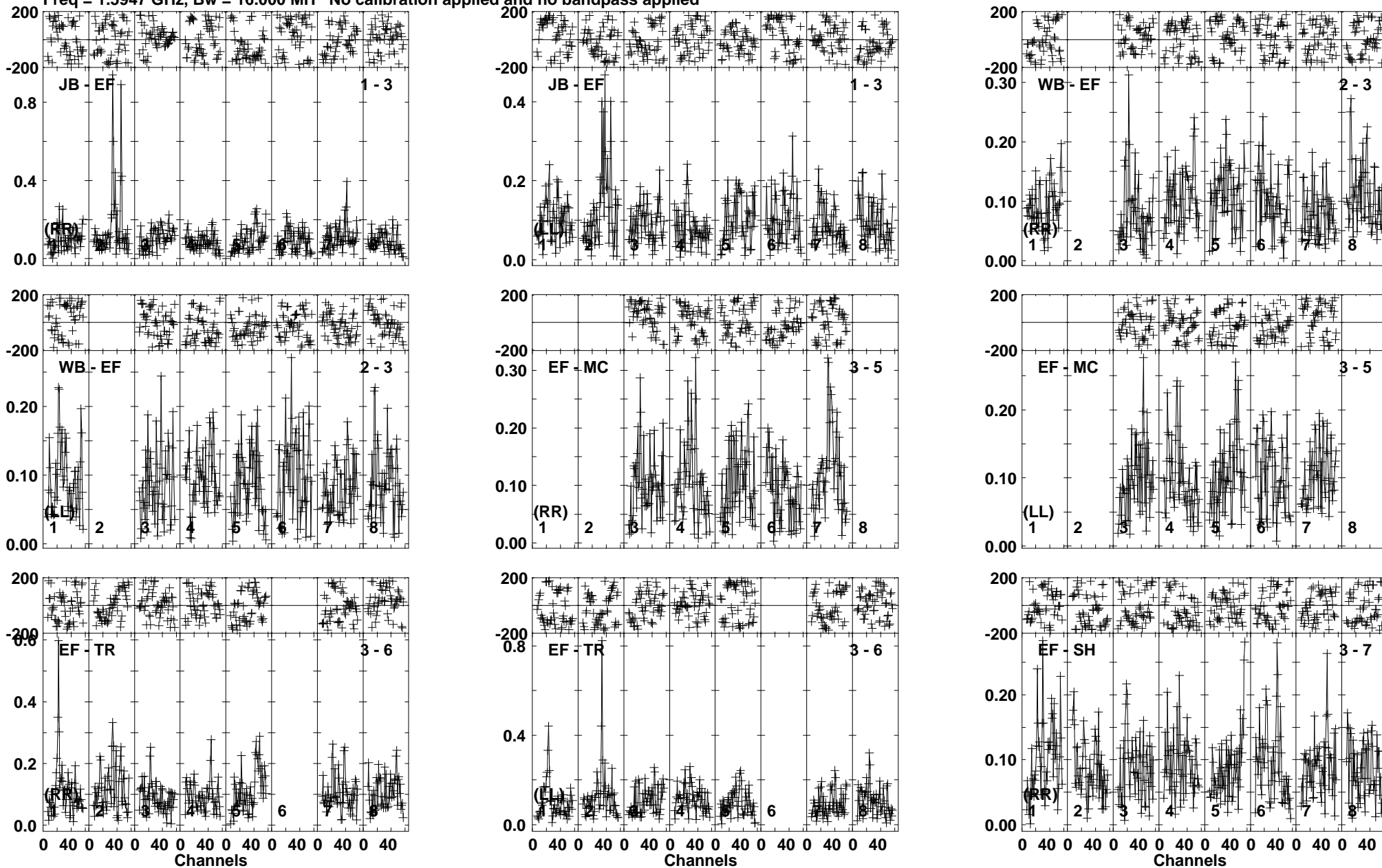
Lower frame: Milli Ampl Jy Top frame: Phas deg Vector averaged cross-power spectrum Baseline: JB (01) - EF (03) Timerange: 00/16:04:04 to 00/16:07:38
