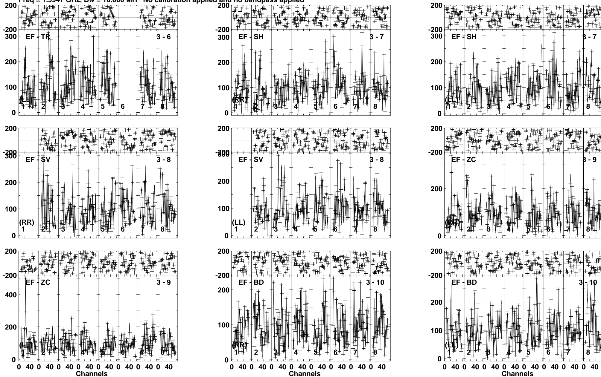
Lower frame: Micro Ampl Jy Top frame: Phas deg Vector averaged cross-power spectrum Baseline: EF (03) - TR (06) Timerange: 00/18:30:04 to 00/18:33:38
