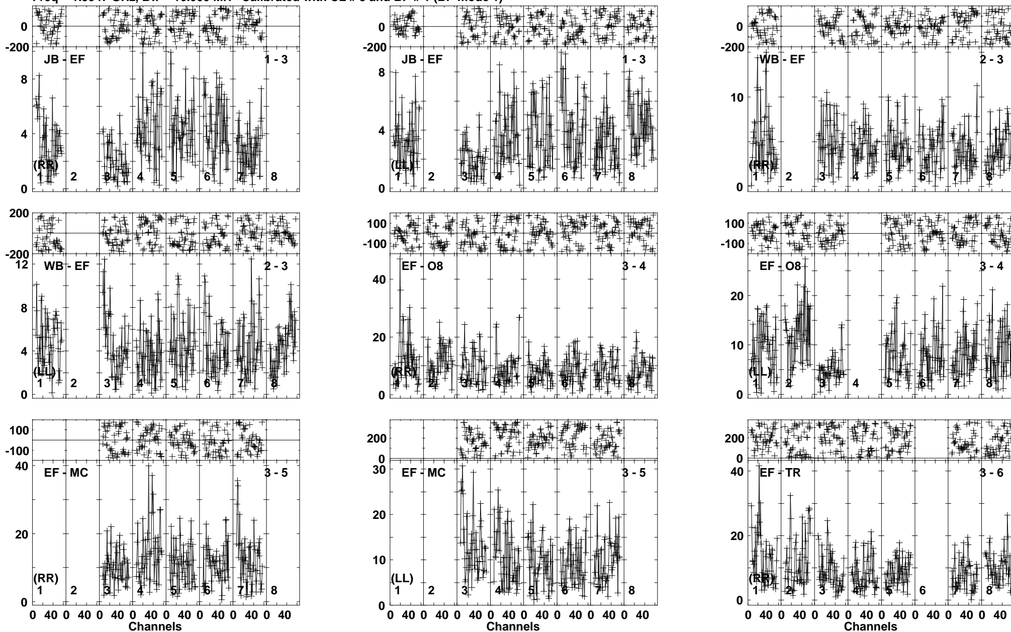
Lower frame: Milli Ampl Jy Top frame: Phas deg Vector averaged cross-power spectrum Baseline: JB (01) - EF (03) Timerange: 00/19:12:44 to 00/19:16:18
