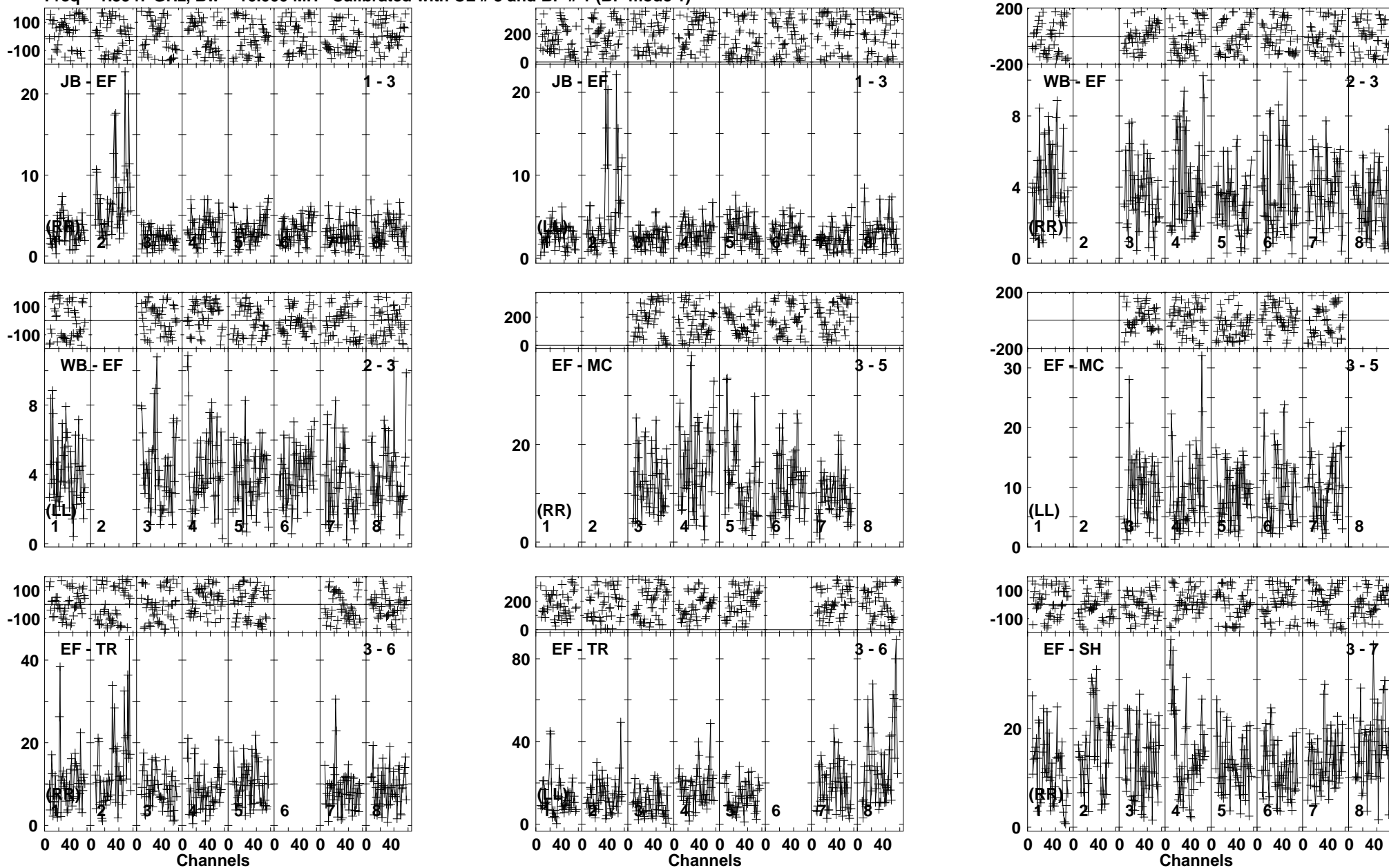
Lower frame: Milli Ampl Jy Top frame: Phas deg Vector averaged cross-power spectrum Baseline: JB (01) - EF (03) Timerange: 00/16:39:26 to 00/16:42:58
