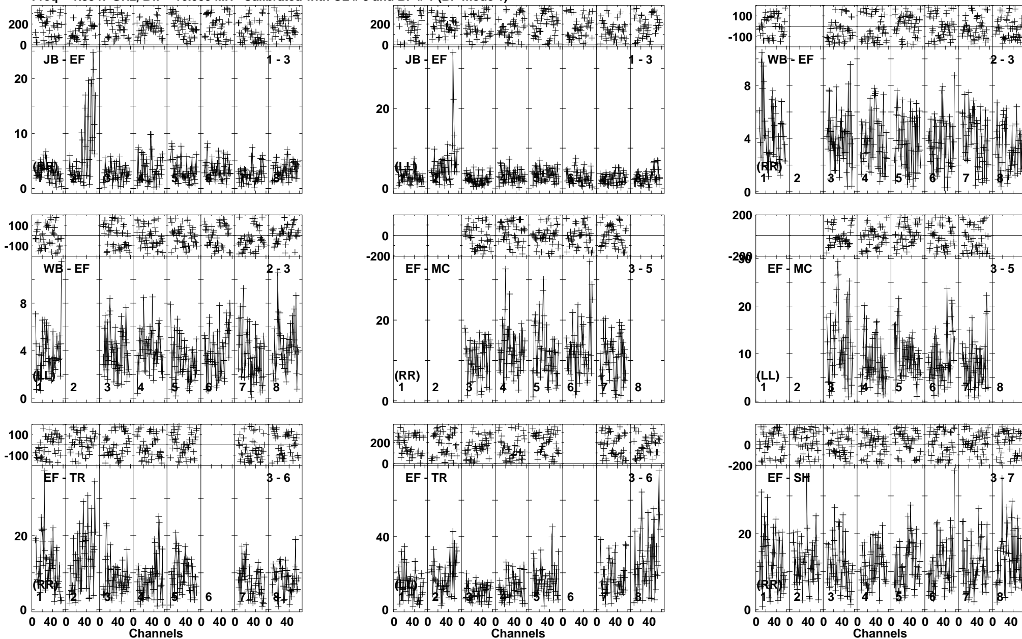
Lower frame: Milli Ampl Jy Top frame: Phas deg Vector averaged cross-power spectrum Baseline: JB (01) - EF (03) Timerange: 00/16:09:06 to 00/16:12:38
