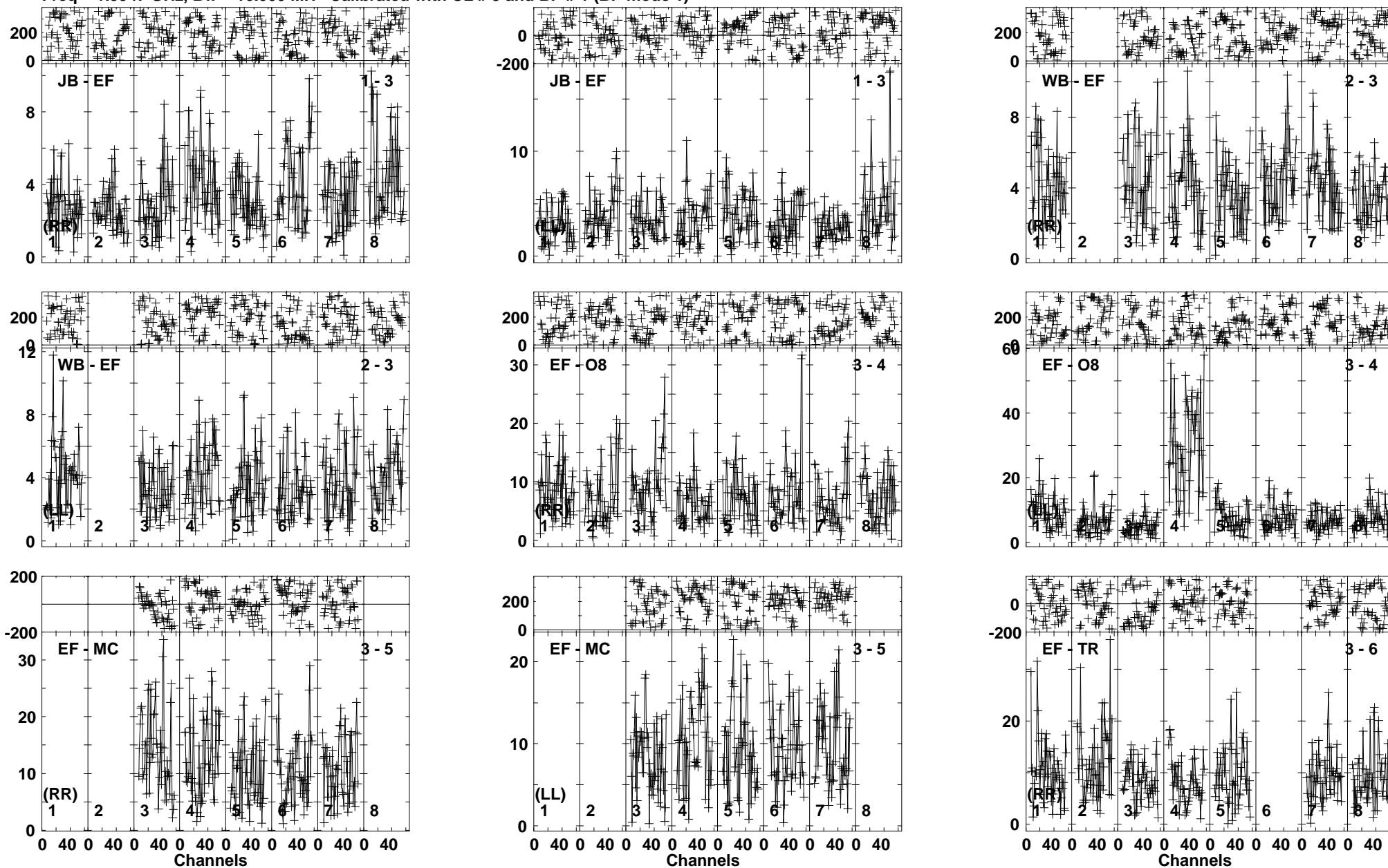
Lower frame: Milli Ampl Jy Top frame: Phas deg Vector averaged cross-power spectrum Baseline: JB (01) - EF (03) Timerange: 00/19:49:47 to 00/19:53:19
