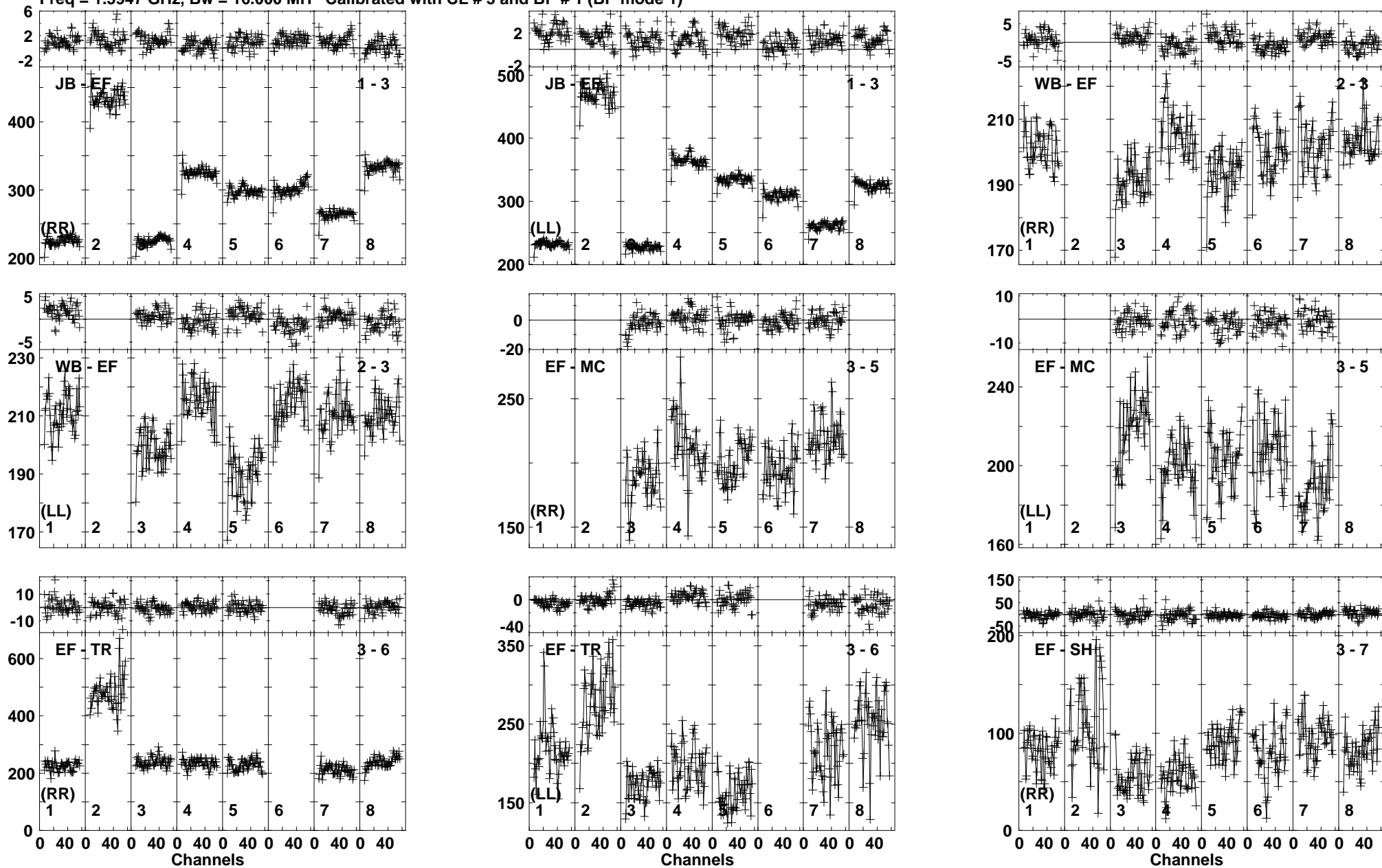
Lower frame: Milli Ampl Jy Top frame: Phas deg Vector averaged cross-power spectrum Baseline: JB (01) - EF (03) Timerange: 00/17:10:06 to 00/17:11:18
