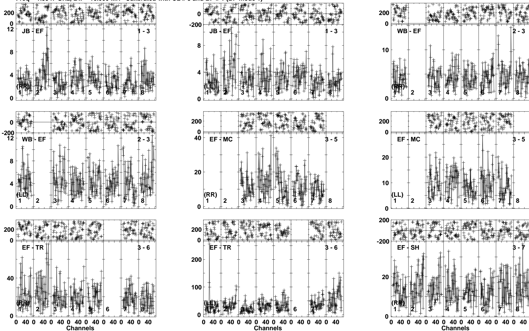
Lower frame: Milli Ampl Jy Top frame: Phas deg Vector averaged cross-power spectrum Baseline: JB (01) - EF (03) Timerange: 00/14:38:44 to 00/14:42:18
