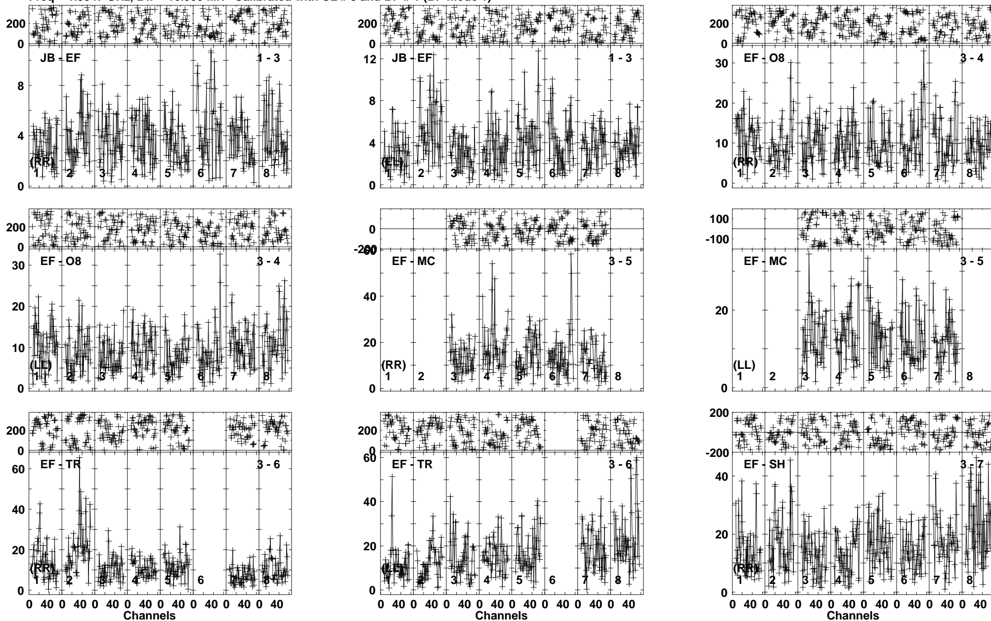
Lower frame: Milli Ampl Jy Top frame: Phas deg Vector averaged cross-power spectrum Baseline: JB (01) - EF (03) Timerange: 00/12:37:26 to 00/12:40:58
