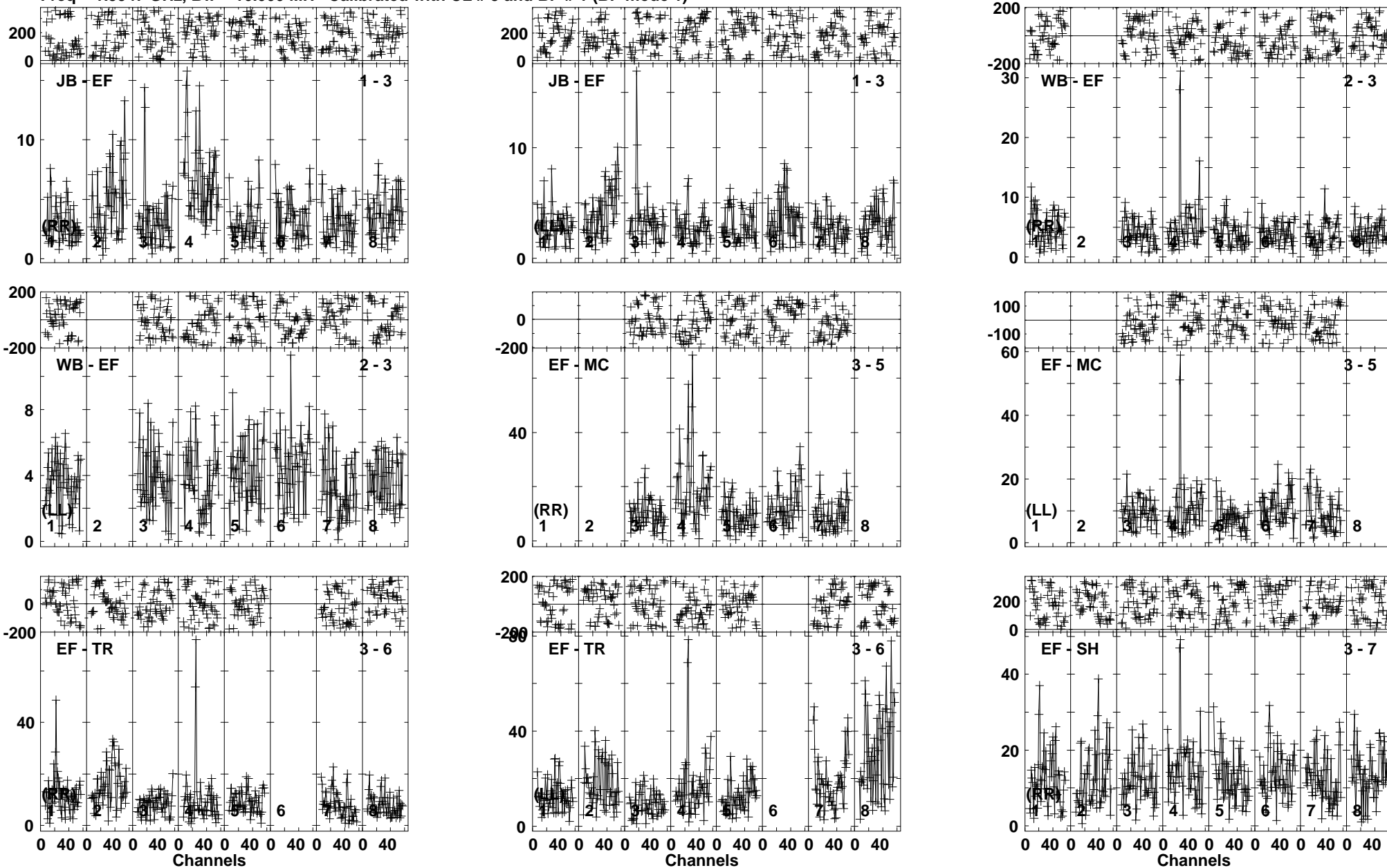
Lower frame: Milli Ampl Jy Top frame: Phas deg Vector averaged cross-power spectrum Baseline: JB (01) - EF (03) Timerange: 00/17:17:04 to 00/17:20:38
