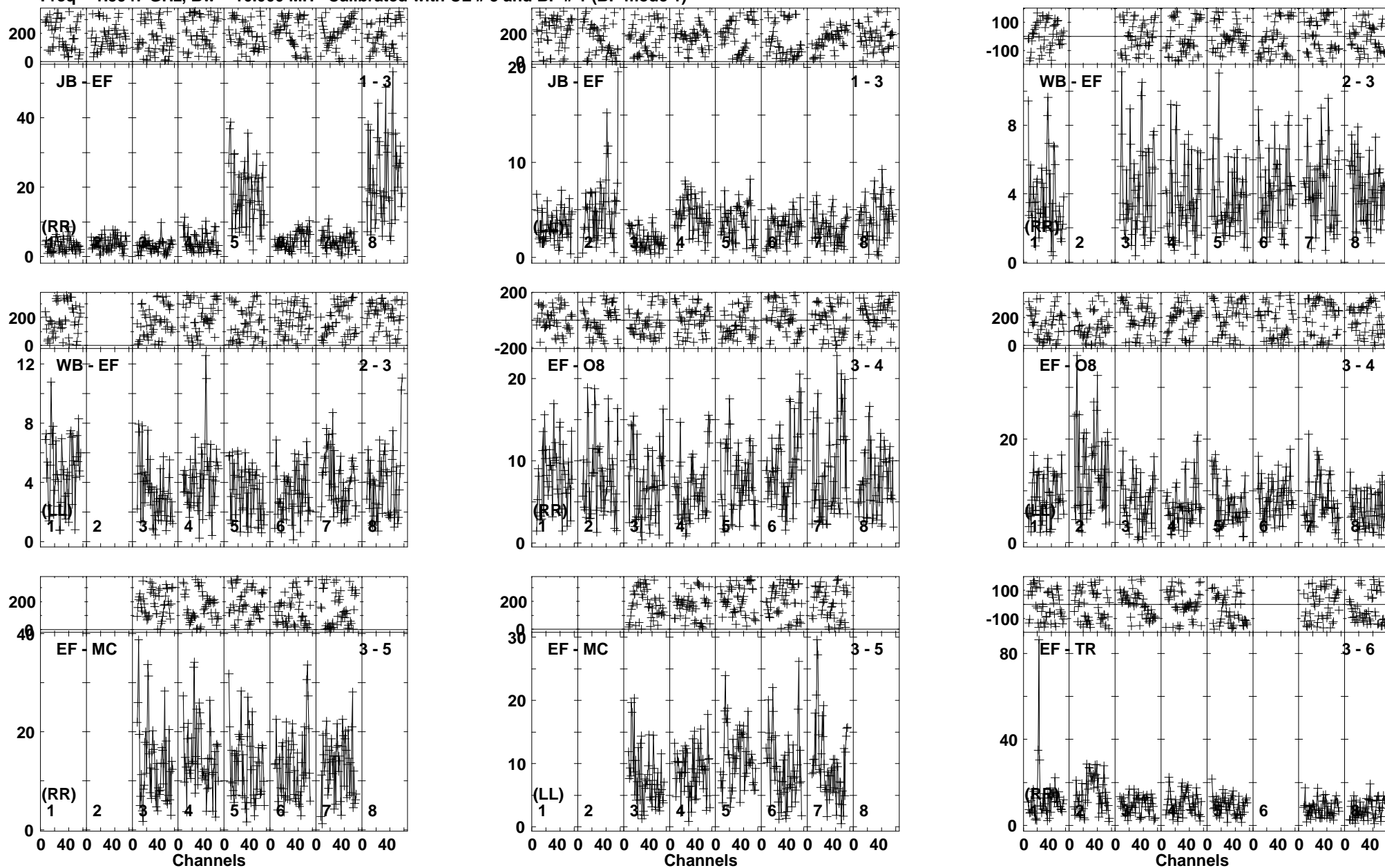
Lower frame: Milli Ampl Jy Top frame: Phas deg Vector averaged cross-power spectrum Baseline: JB (01) - EF (03) Timerange: 00/20:30:32 to 00/20:33:54
