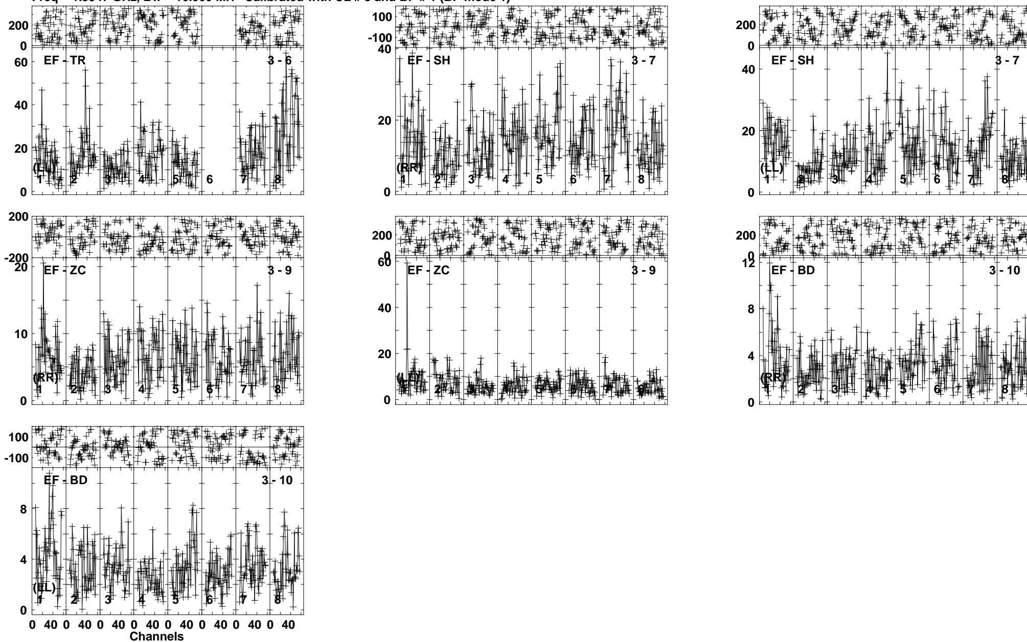
Lower frame: Milli Ampl Jy Top frame: Phas deg Vector averaged cross-power spectrum Baseline: EF (03) - TR (06) Timerange: 00:18:45:46 to 00:18:49:18
