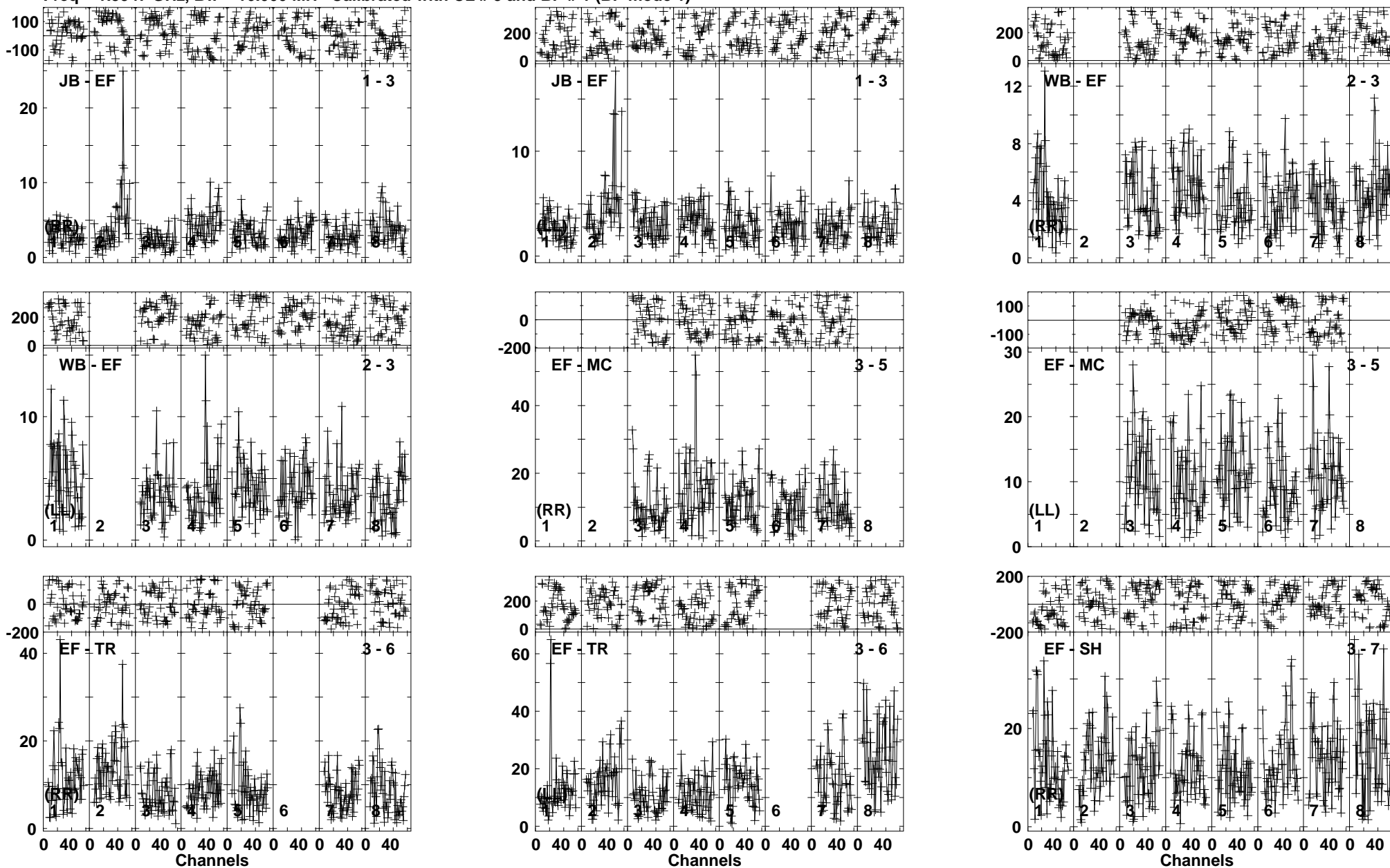
Lower frame: Milli Ampl Jy Top frame: Phas deg Vector averaged cross-power spectrum Baseline: JB (01) - EF (03) Timerange: 00/15:53:24 to 00/15:56:58
