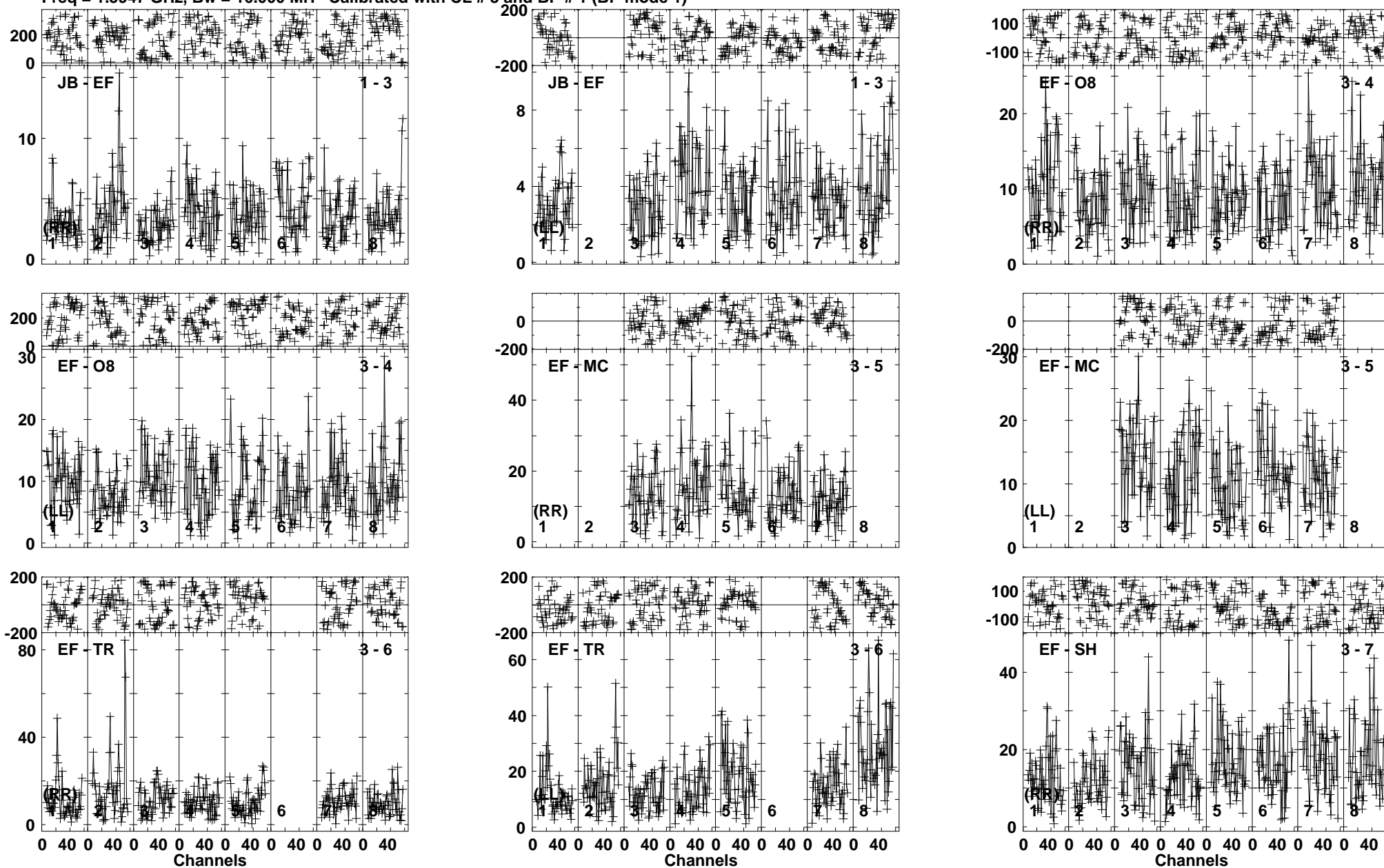
Lower frame: Milli Ampl Jy Top frame: Phas deg Vector averaged cross-power spectrum Baseline: JB (01) - EF (03) Timerange: 00:12:53:44 to 00:12:57:18
