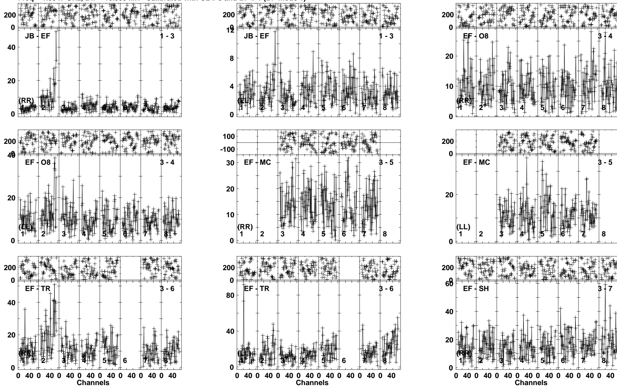
Lower frame: Milli Ampl Jy Top frame: Phas deg Vector averaged cross-power spectrum Baseline: JB (01) - EF (03) Timerange: 00/12:48:06 to 00/12:51:38
