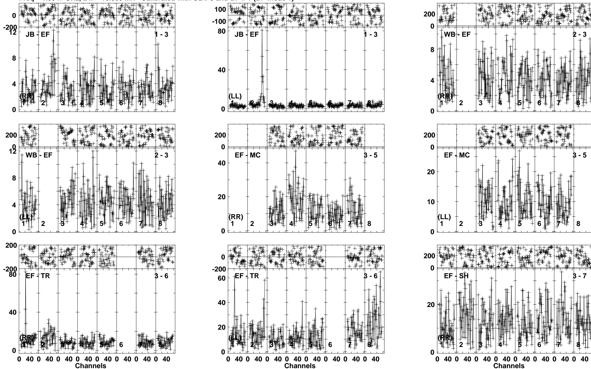
Lower frame: Milli Ampl Jy Top frame: Phas deg Vector averaged cross-power spectrum Baseline: JB (01) - EF (03) Timerange: 00/15:32:04 to 00/15:35:38
