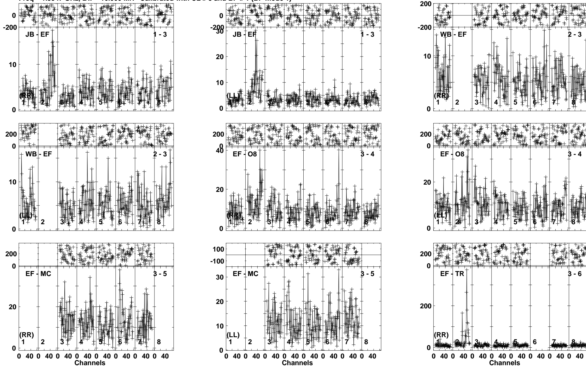
Lower frame: Milli Ampl Jy Top frame: Phas deg Vector averaged cross-power spectrum Baseline: JB (01) - EF (03) Timerange: 00/13:20:04 to 00/13:23:38
