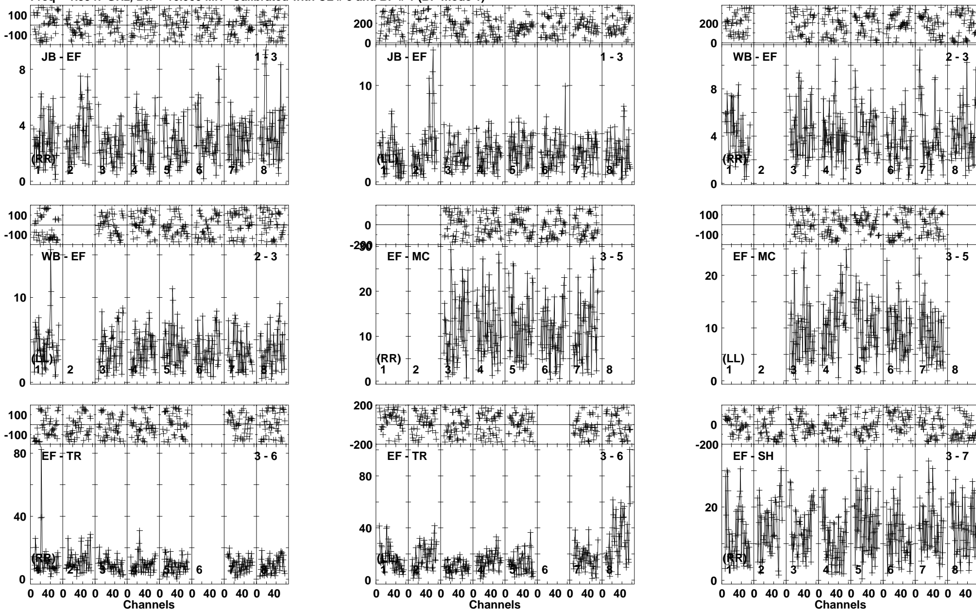
Lower frame: Milli Ampl Jy Top frame: Phas deg Vector averaged cross-power spectrum Baseline: JB (01) - EF (03) Timerange: 00/17:27:44 to 00/17:31:18
