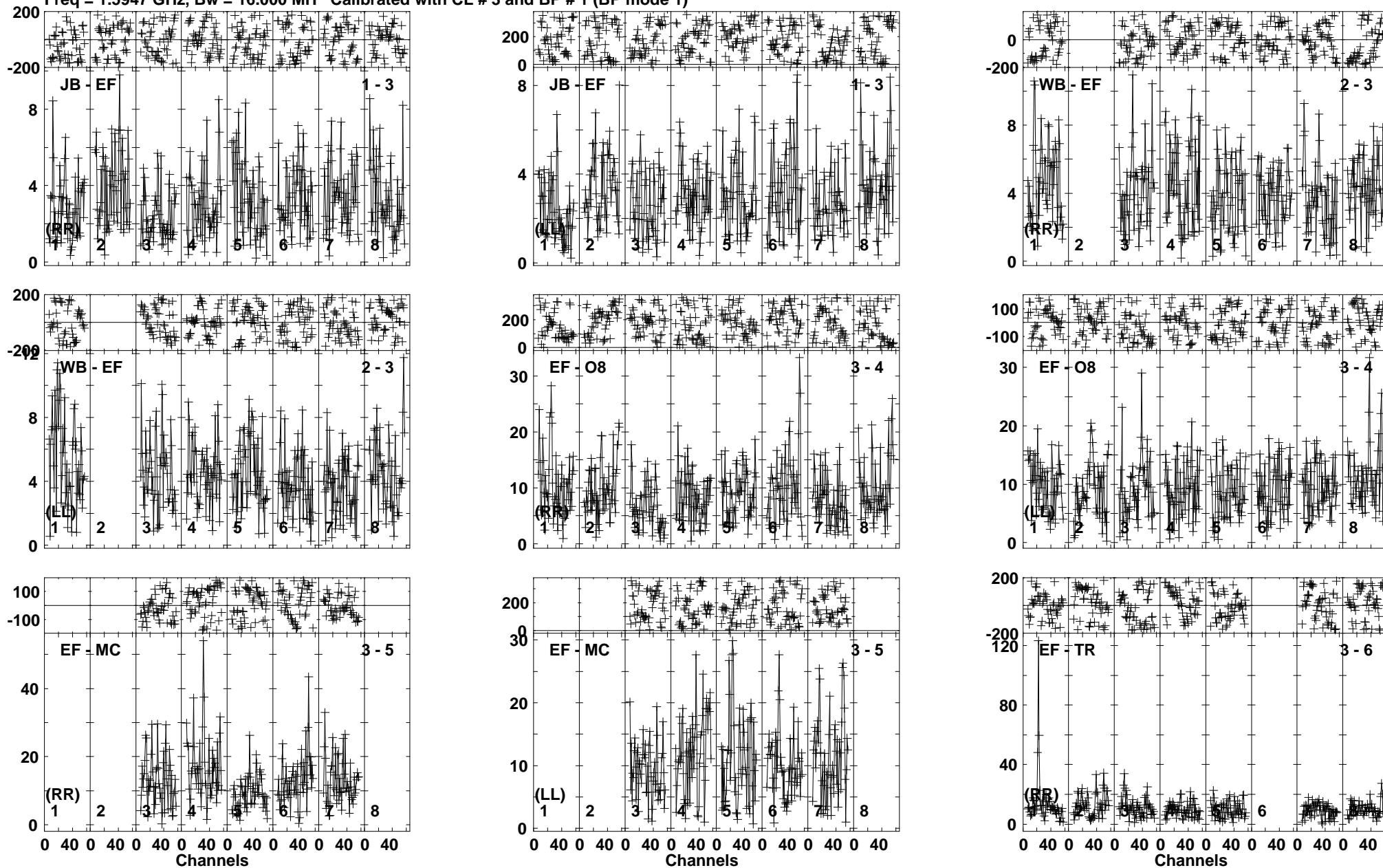
Lower frame: Milli Ampl Jy Top frame: Phas deg Vector averaged cross-power spectrum Baseline: JB (01) - EF (03) Timerange: 00/13:52:03 to 00/13:55:39
