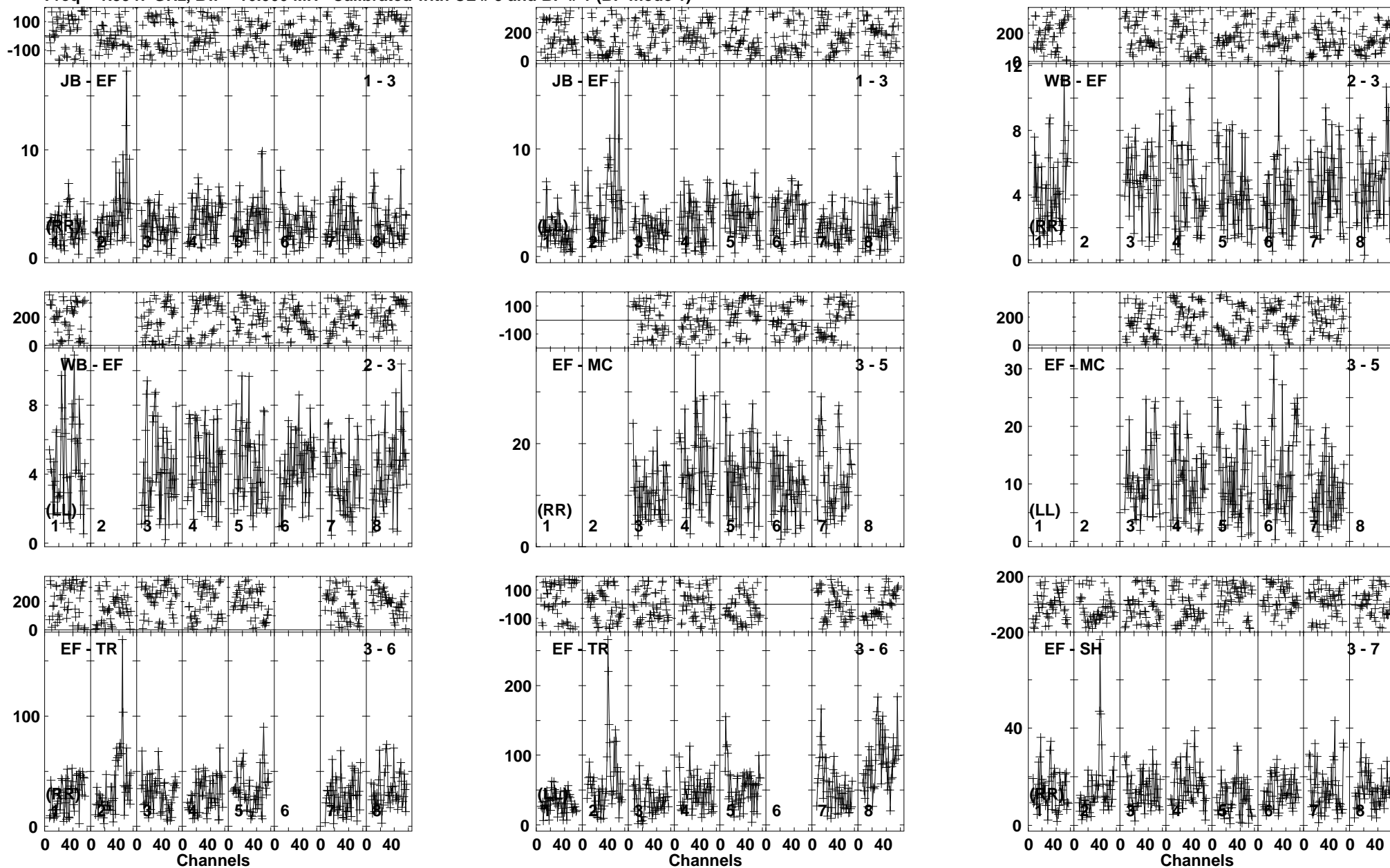
Lower frame: Milli Ampl Jy Top frame: Phas deg Vector averaged cross-power spectrum Baseline: JB (01) - EF (03) Timerange: 00/14:43:46 to 00/14:47:18
