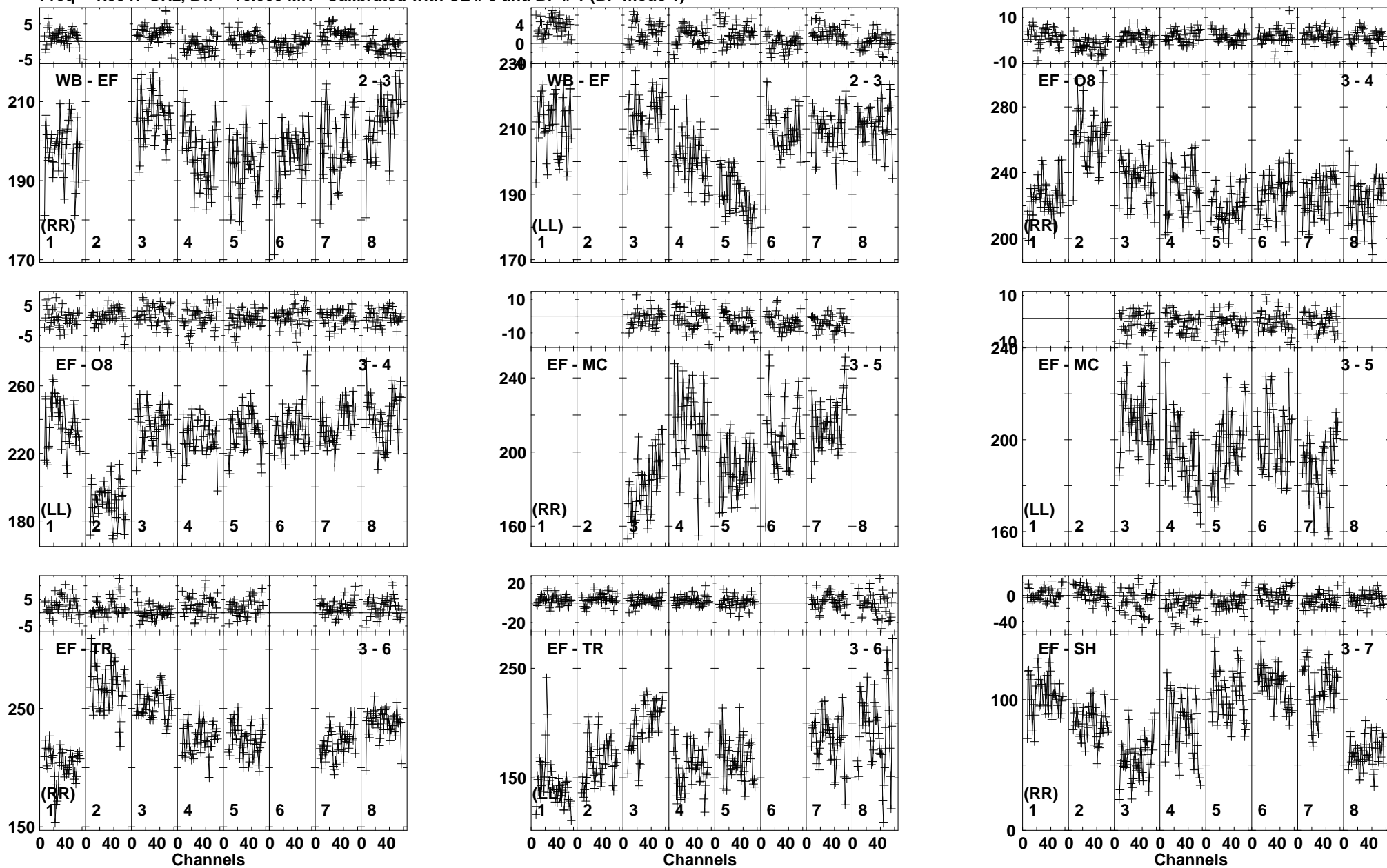
Lower frame: Milli Ampl Jy Top frame: Phas deg Vector averaged cross-power spectrum Baseline: WB (02) - EF (03) Timerange: 00/13:35:01 to 00/13:36:19
