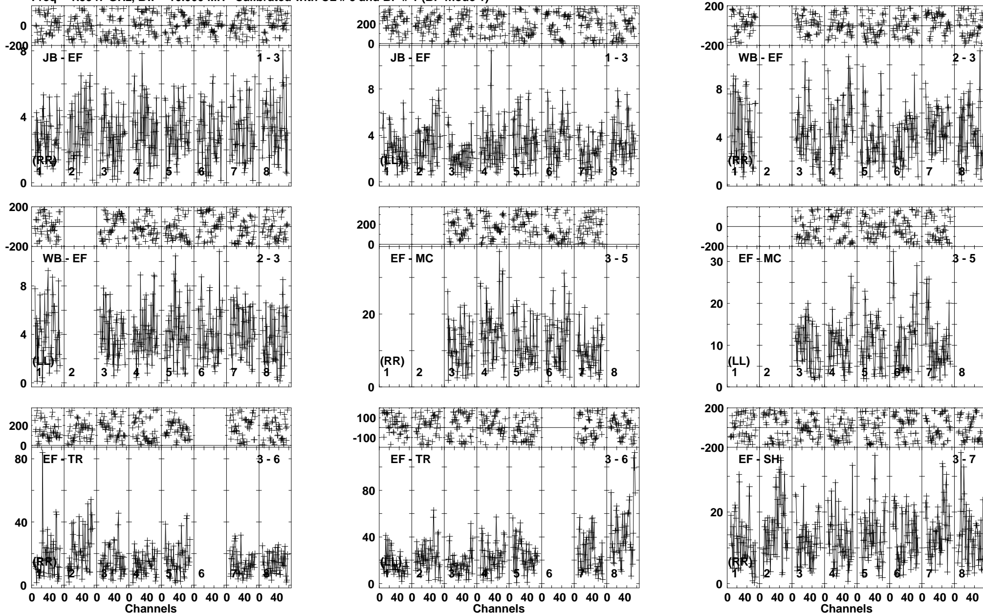
Lower frame: Milli Ampl Jy Top frame: Phas deg Vector averaged cross-power spectrum Baseline: JB (01) - EF (03) Timerange: 00/14:49:22 to 00/14:52:58
