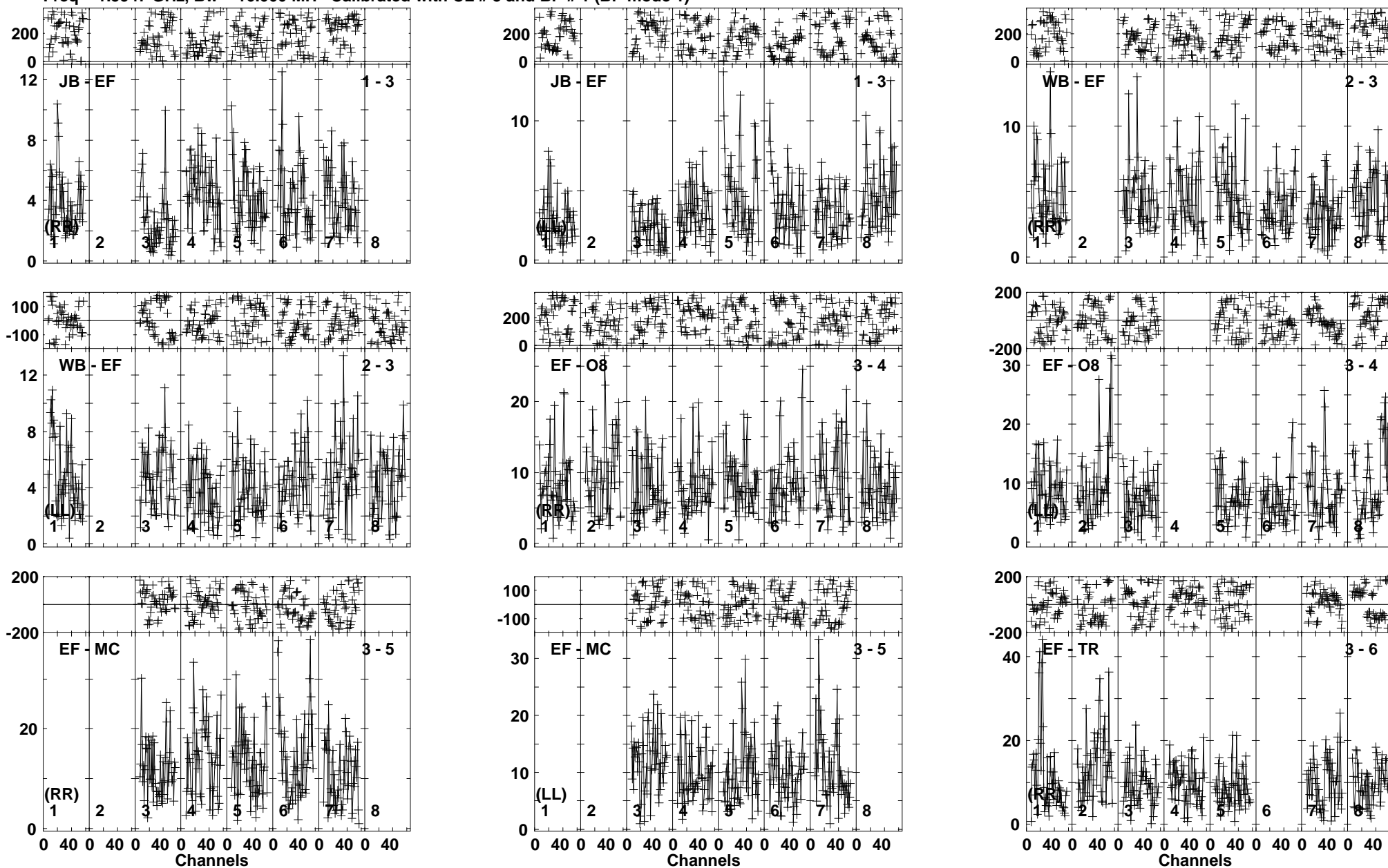
Lower frame: Milli Ampl Jy Top frame: Phas deg Vector averaged cross-power spectrum Baseline: JB (01) - EF (03) Timerange: 00/19:17:46 to 00/19:21:18
