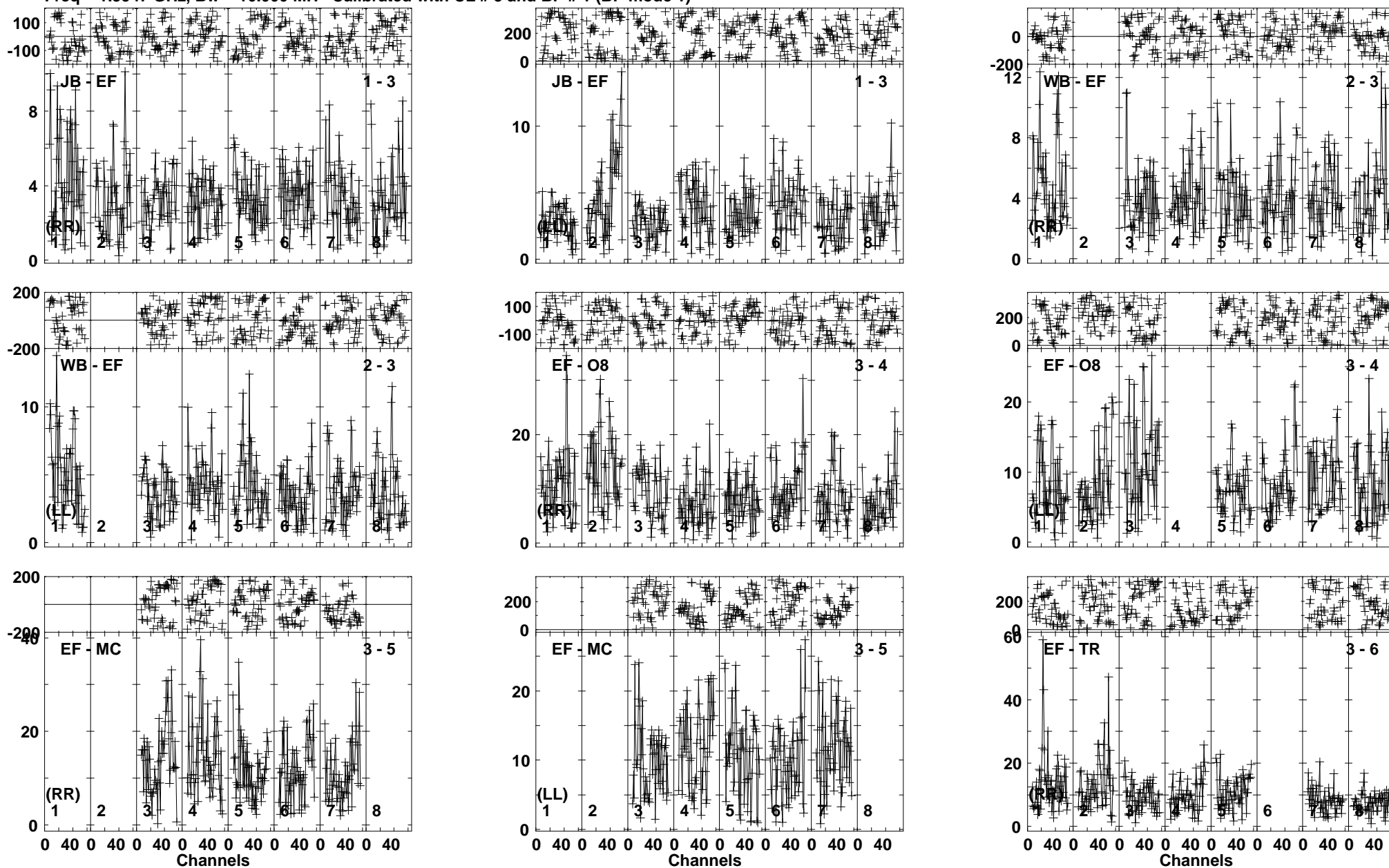
Lower frame: Milli Ampl Jy Top frame: Phas deg Vector averaged cross-power spectrum Baseline: JB (01) - EF (03) Timerange: 00/18:56:26 to 00/18:59:58
