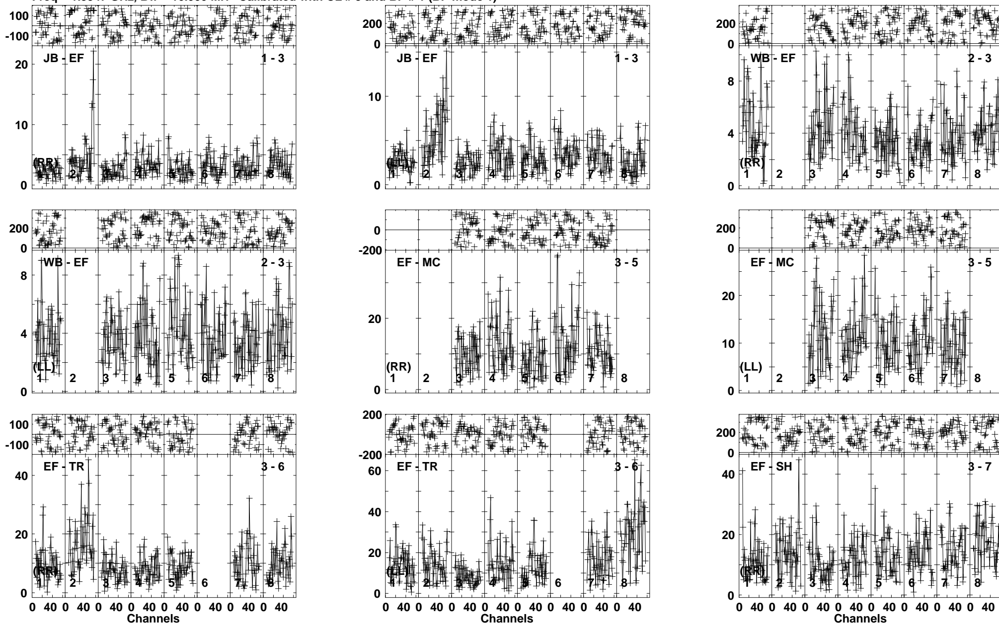
Lower frame: Milli Ampl Jy Top frame: Phas deg Vector averaged cross-power spectrum Baseline: JB (01) - EF (03) Timerange: 00/17:11:26 to 00/17:14:58
