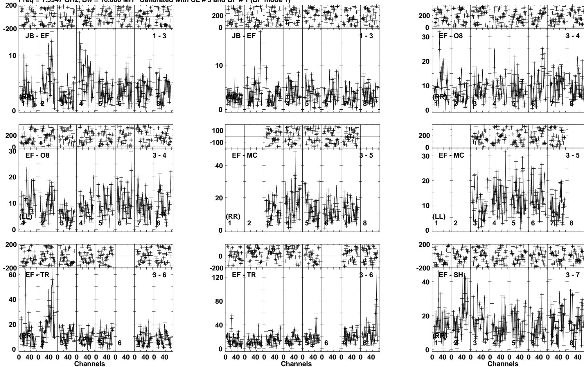
Lower frame: Milli Ampl Jy Top frame: Phas deg Vector averaged cross-power spectrum Baseline: JB (01) - EF (03) Timerange: 00/13:04:24 to 00/13:07:58
