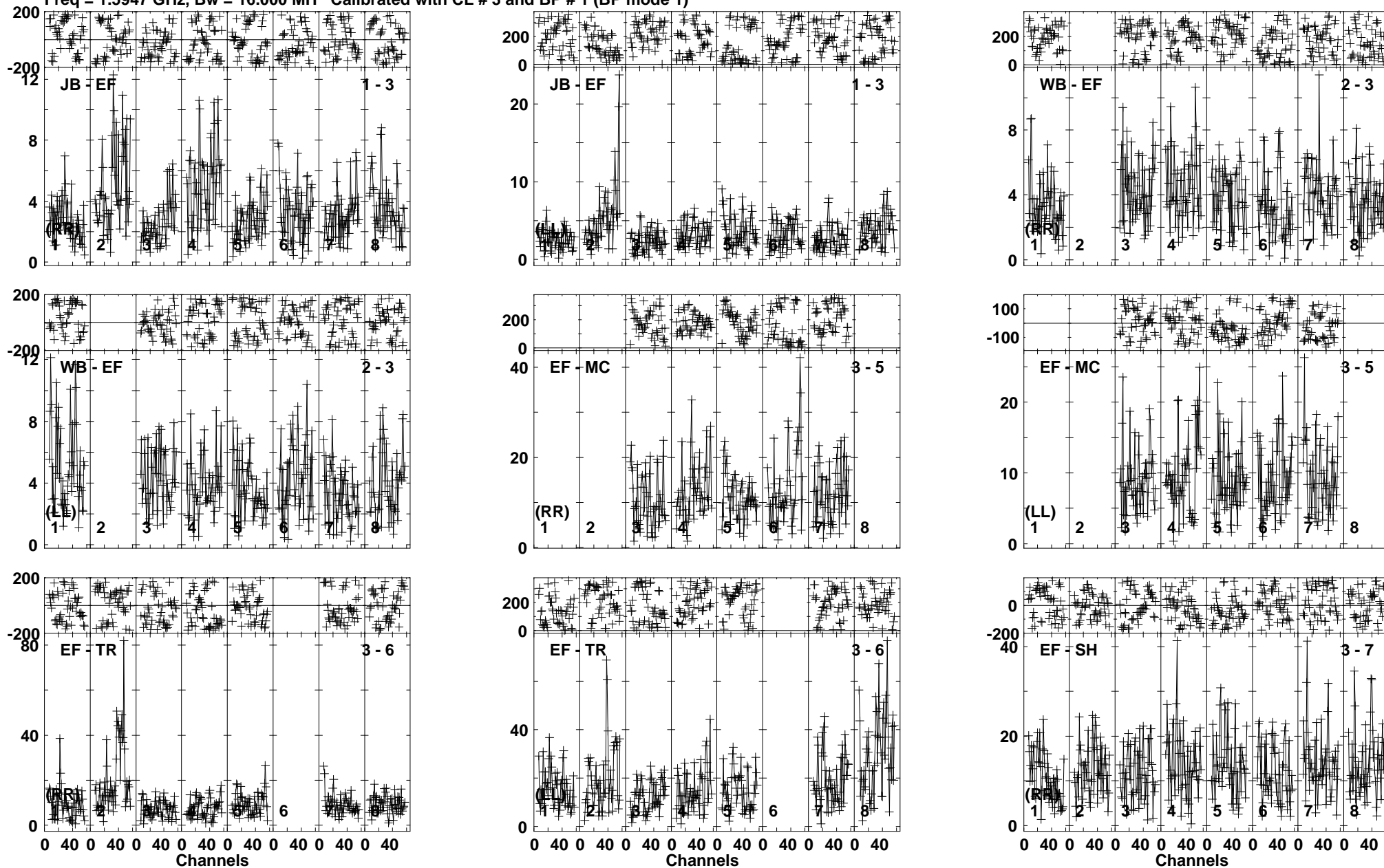
Lower frame: Milli Ampl Jy Top frame: Phas deg Vector averaged cross-power spectrum Baseline: JB (01) - EF (03) Timerange: 00/17:22:06 to 00/17:25:38
