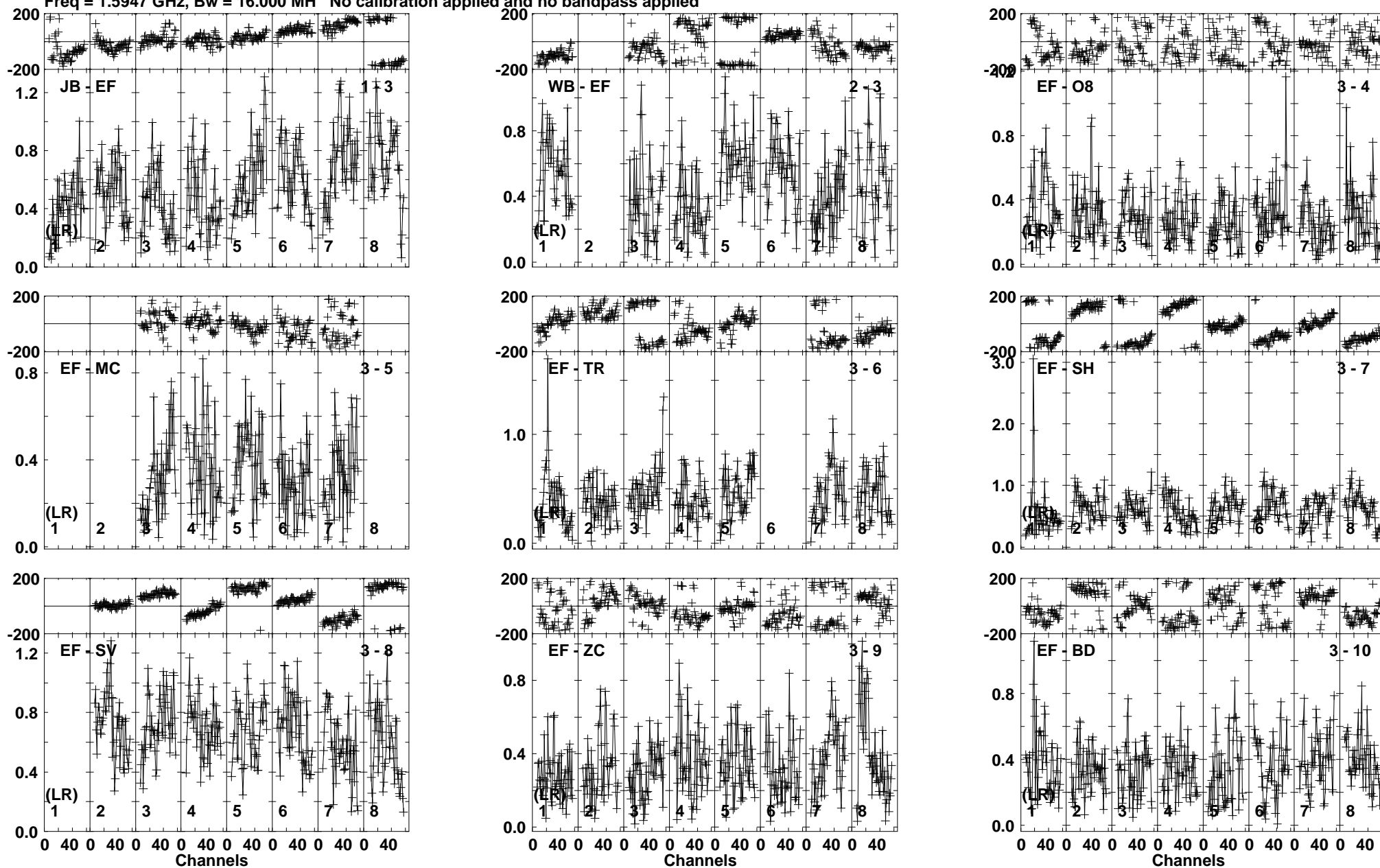
Lower frame: Milli Ampl Jy Top frame: Phas deg Vector averaged cross-power spectrum Baseline: JB (01) - EF (03) Timerange: 00:19:27:06 to 00:19:28:18
