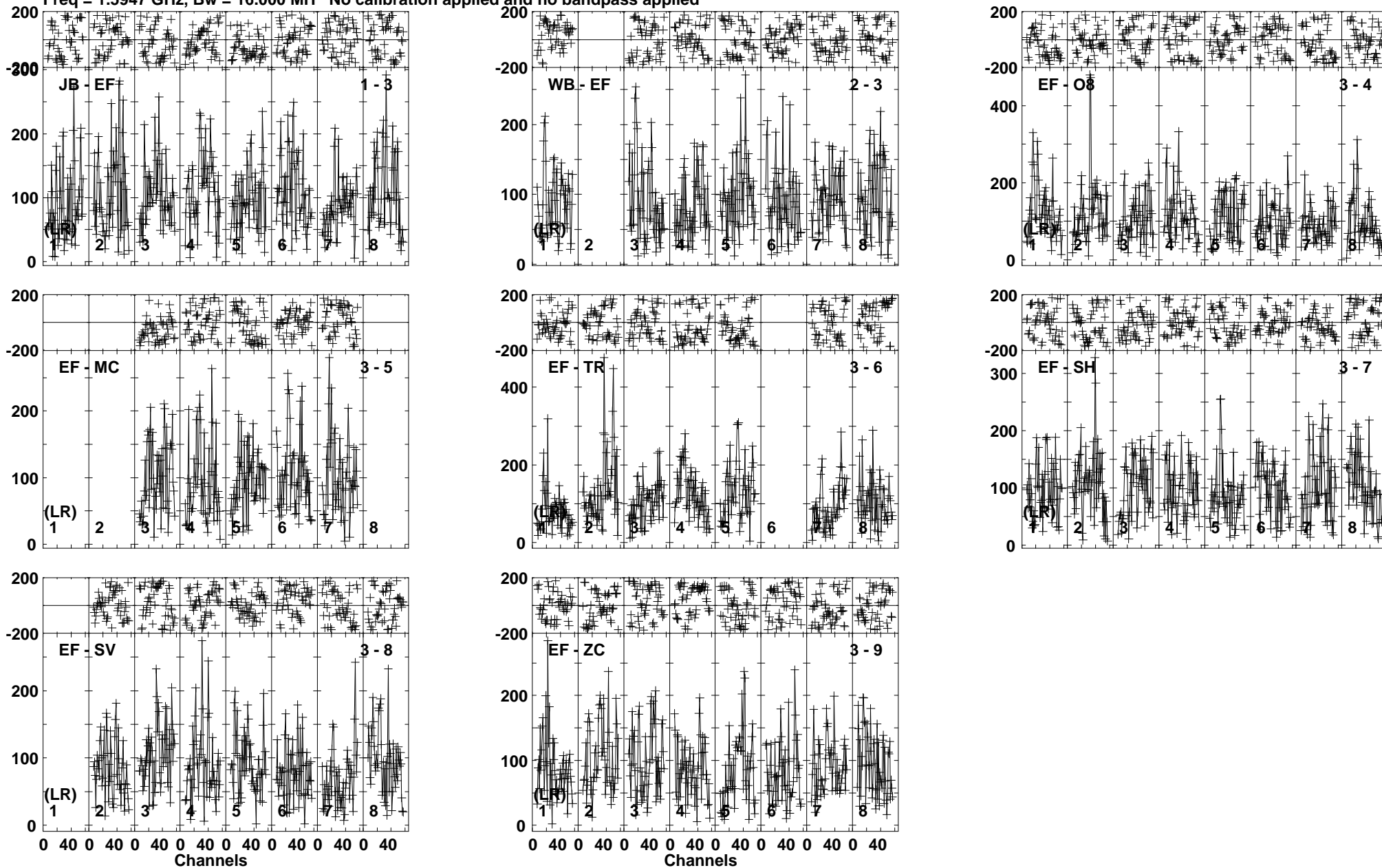
Lower frame: Micro Ampl Jy Top frame: Phas deg Vector averaged cross-power spectrum Baseline: JB (01) - EF (03) Timerange: 00/13:47:04 to 00/13:50:38
