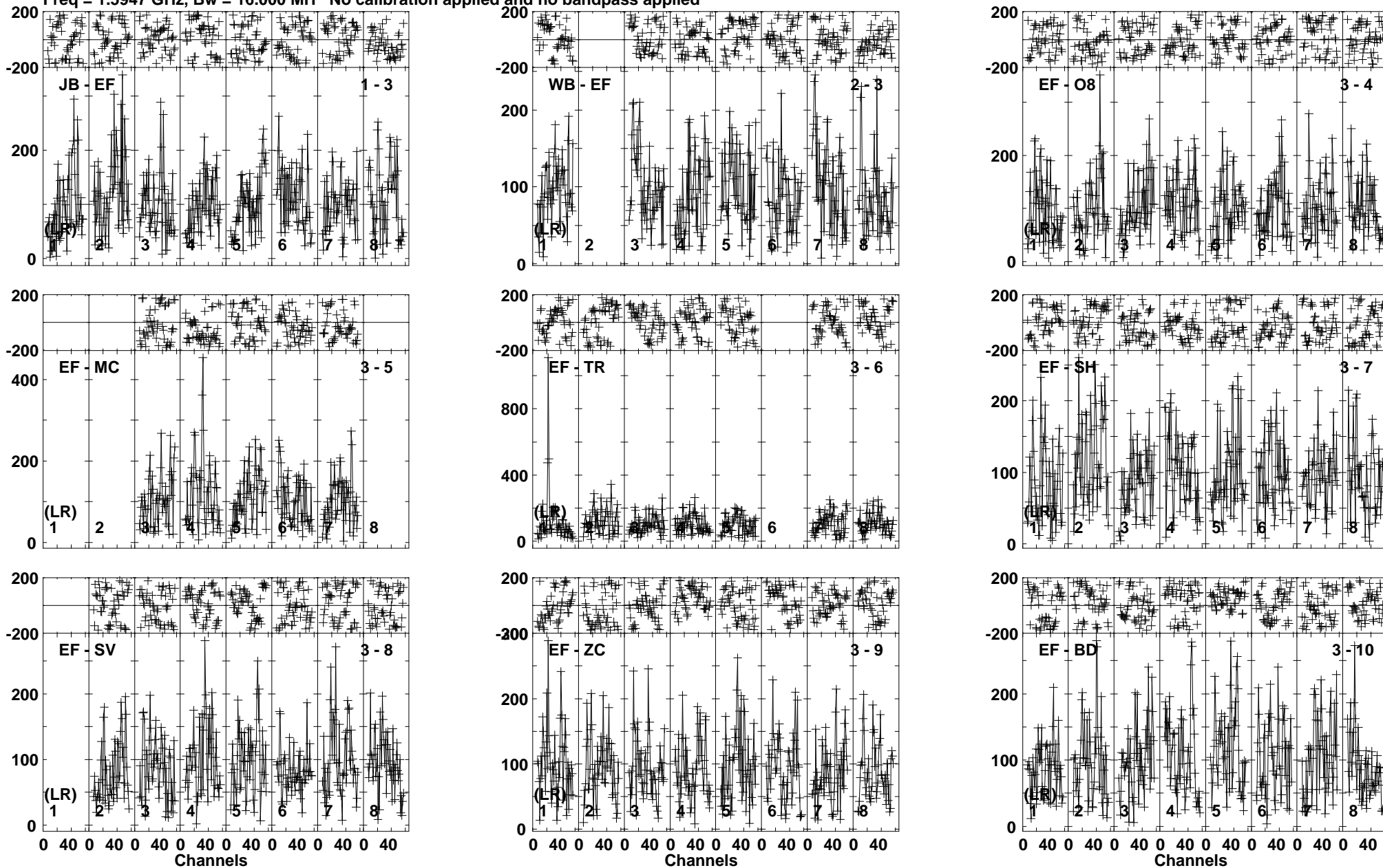
Lower frame: Micro Ampl Jy Top frame: Phas deg Vector averaged cross-power spectrum Baseline: JB (01) - EF (03) Timerange: 00/18:35:06 to 00/18:38:38
