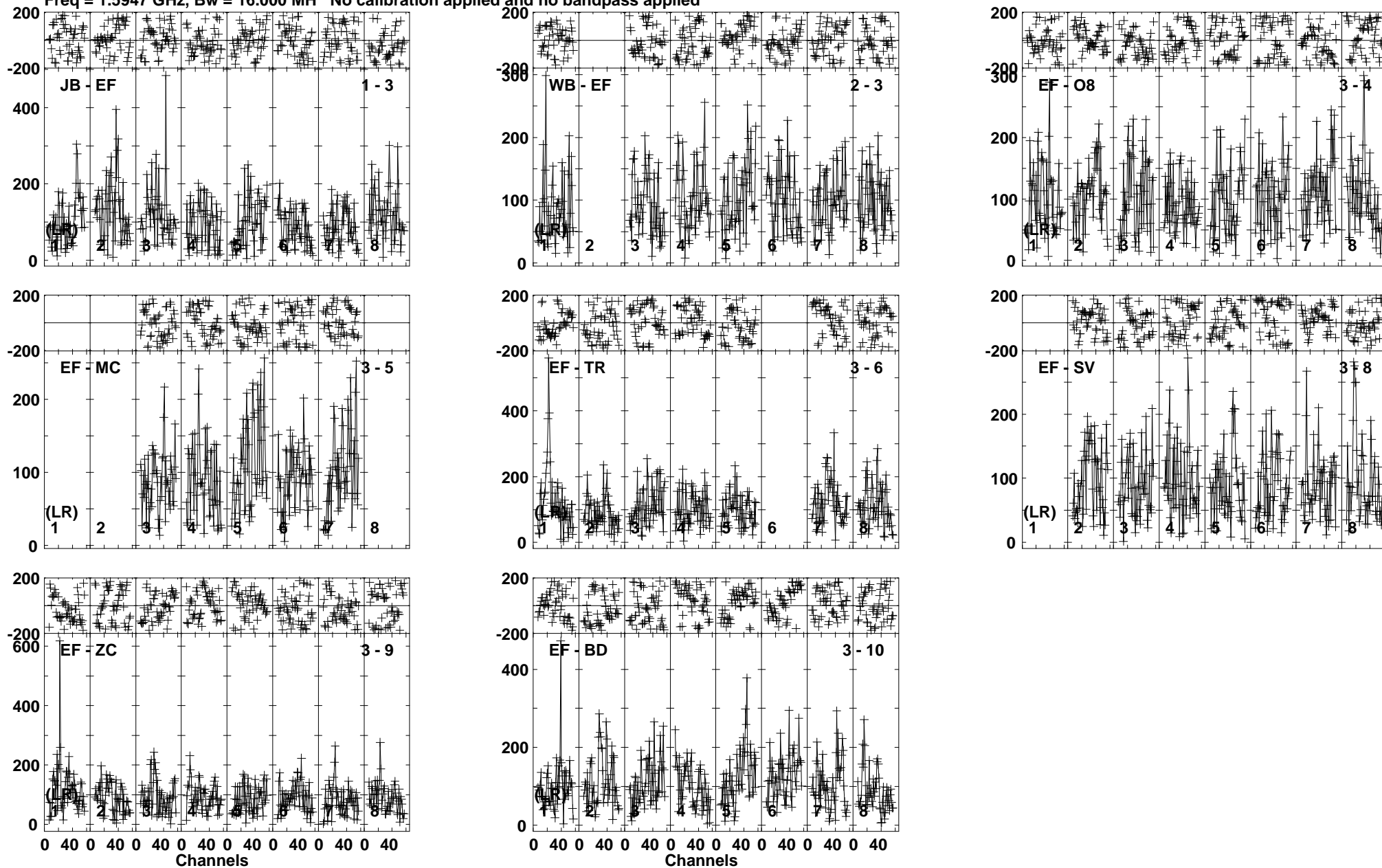
Lower frame: Micro Ampl Jy Top frame: Phas deg Vector averaged cross-power spectrum Baseline: JB (01) - EF (03) Timerange: 00/20:25:44 to 00/20:29:08
