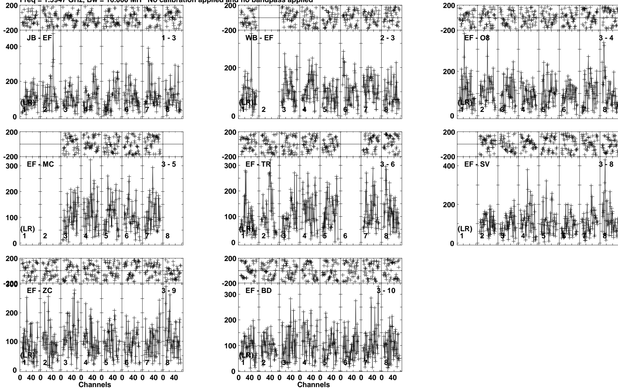
Lower frame: Micro Ampl Jy Top frame: Phas deg Vector averaged cross-power spectrum Baseline: JB (01) - EF (03) Timerange: 00/21:31:32 to 00/21:34:54
