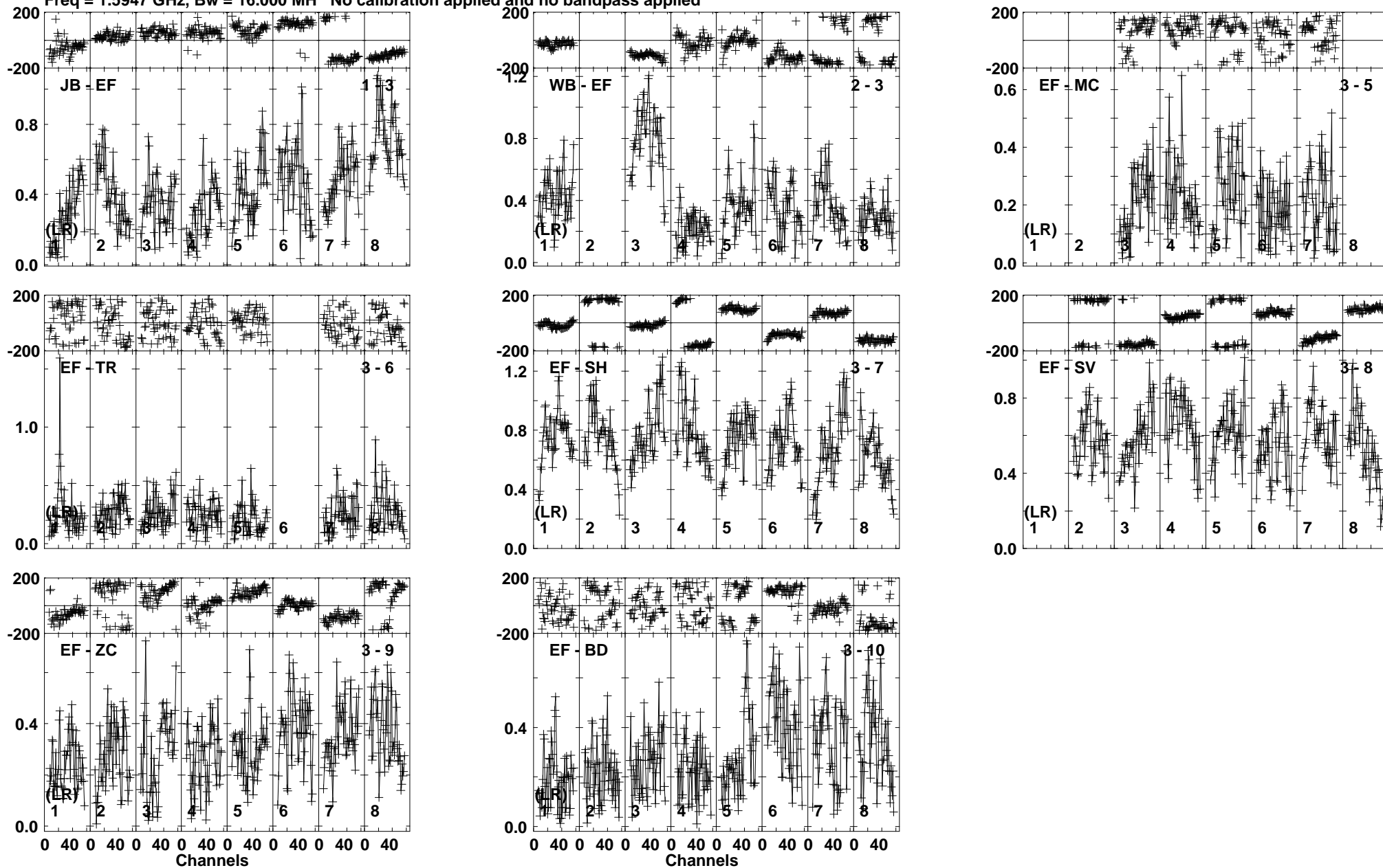
Lower frame: Milli Ampl Jy Top frame: Phas deg Vector averaged cross-power spectrum Baseline: JB (01) - EF (03) Timerange: 00/14:31:45 to 00/14:32:59
