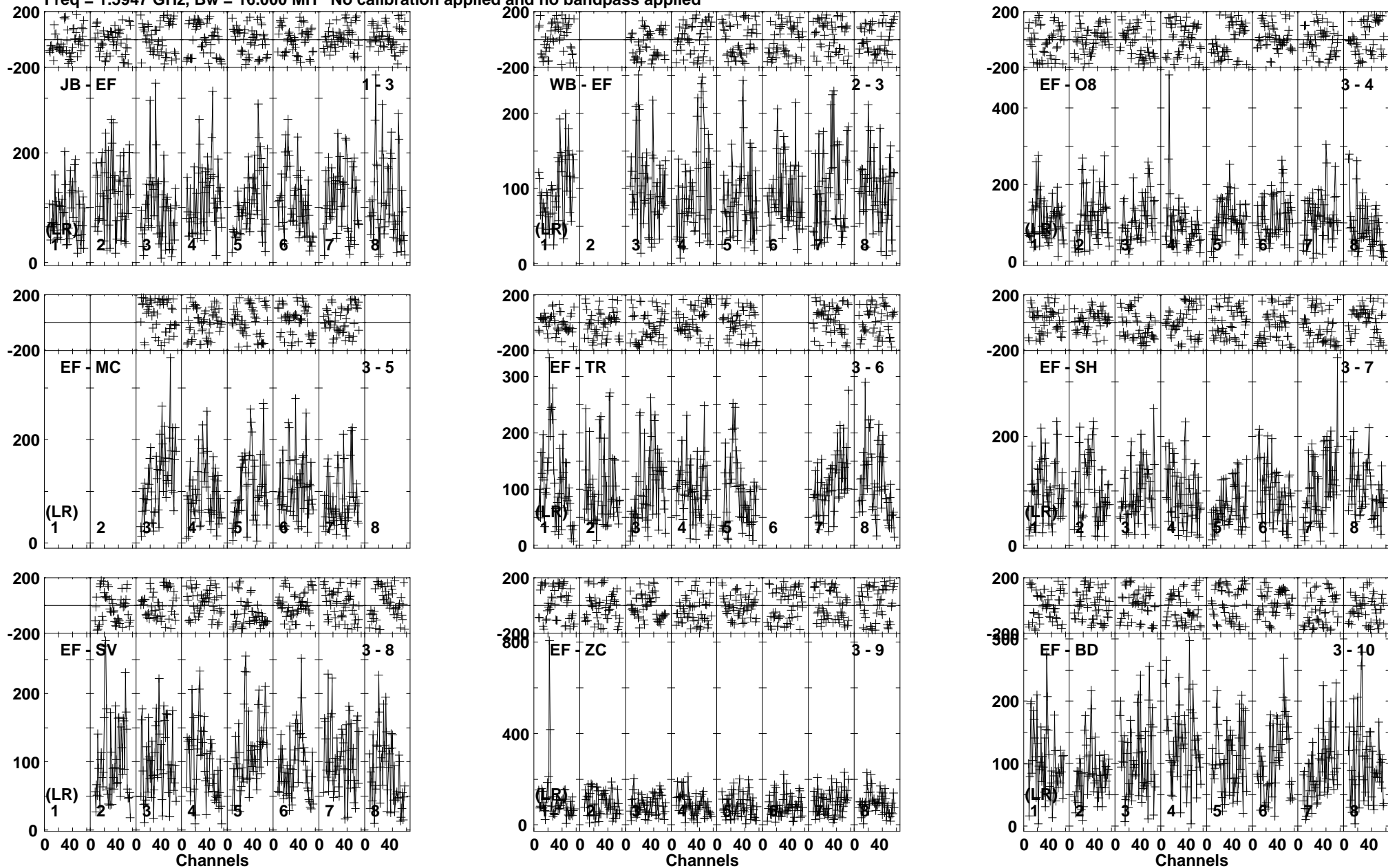
Lower frame: Micro Ampl Jy Top frame: Phas deg Vector averaged cross-power spectrum Baseline: JB (01) - EF (03) Timerange: 00/18:56:26 to 00/18:59:58
