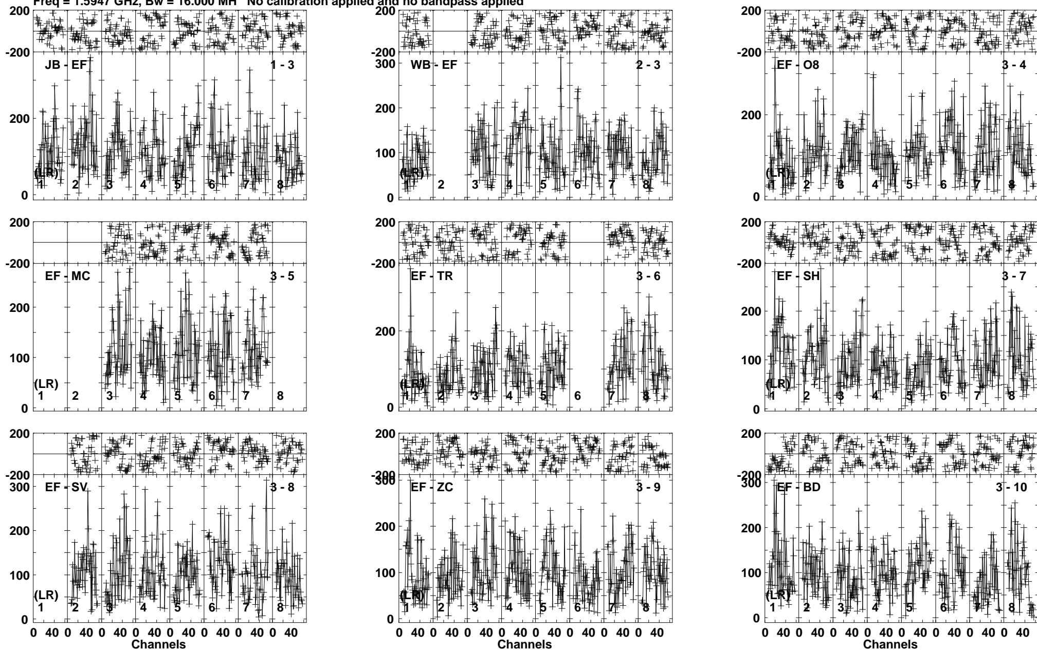
Lower frame: Micro Ampl Jy Top frame: Phas deg Vector averaged cross-power spectrum Baseline: JB (01) - EF (03) Timerange: 00/19:02:04 to 00/19:05:38
