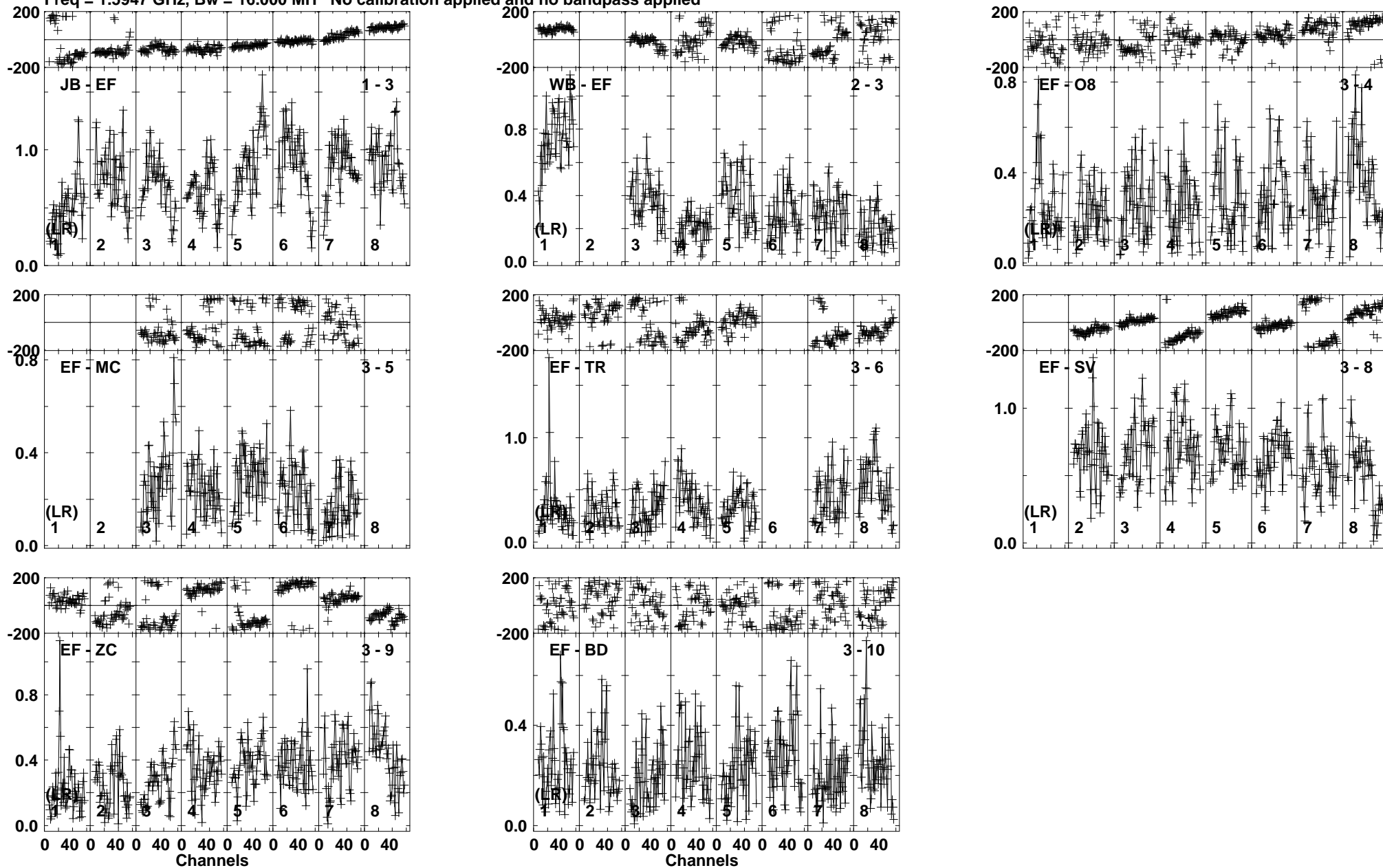
Lower frame: Milli Ampl Jy Top frame: Phas deg Vector averaged cross-power spectrum Baseline: JB (01) - EF (03) Timerange: 00/20:29:16 to 00/20:30:24
