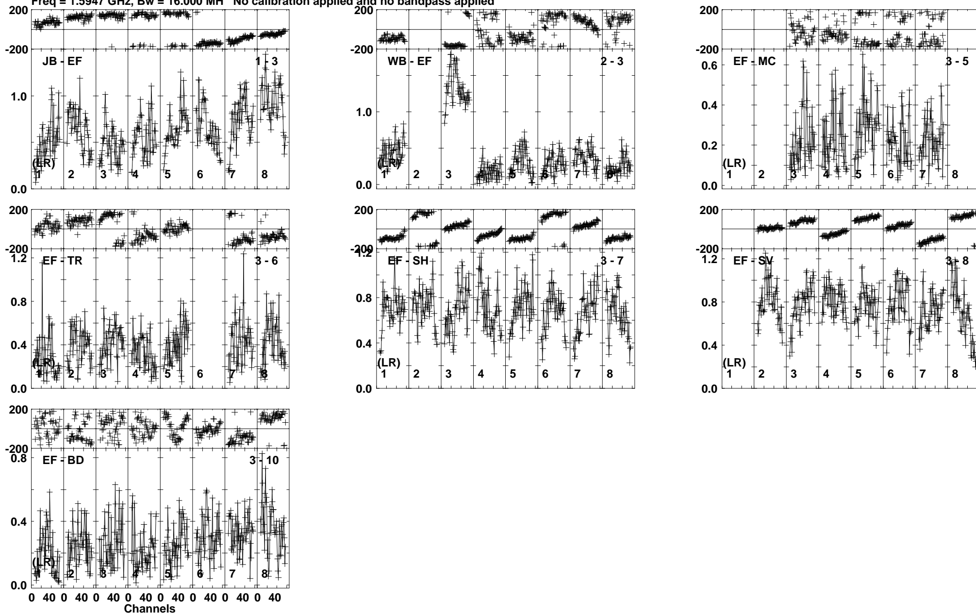
Lower frame: Milli Ampl Jy Top frame: Phas deg Vector averaged cross-power spectrum Baseline: JB (01) - EF (03) Timerange: 00/17:42:06 to 00/17:43:18
