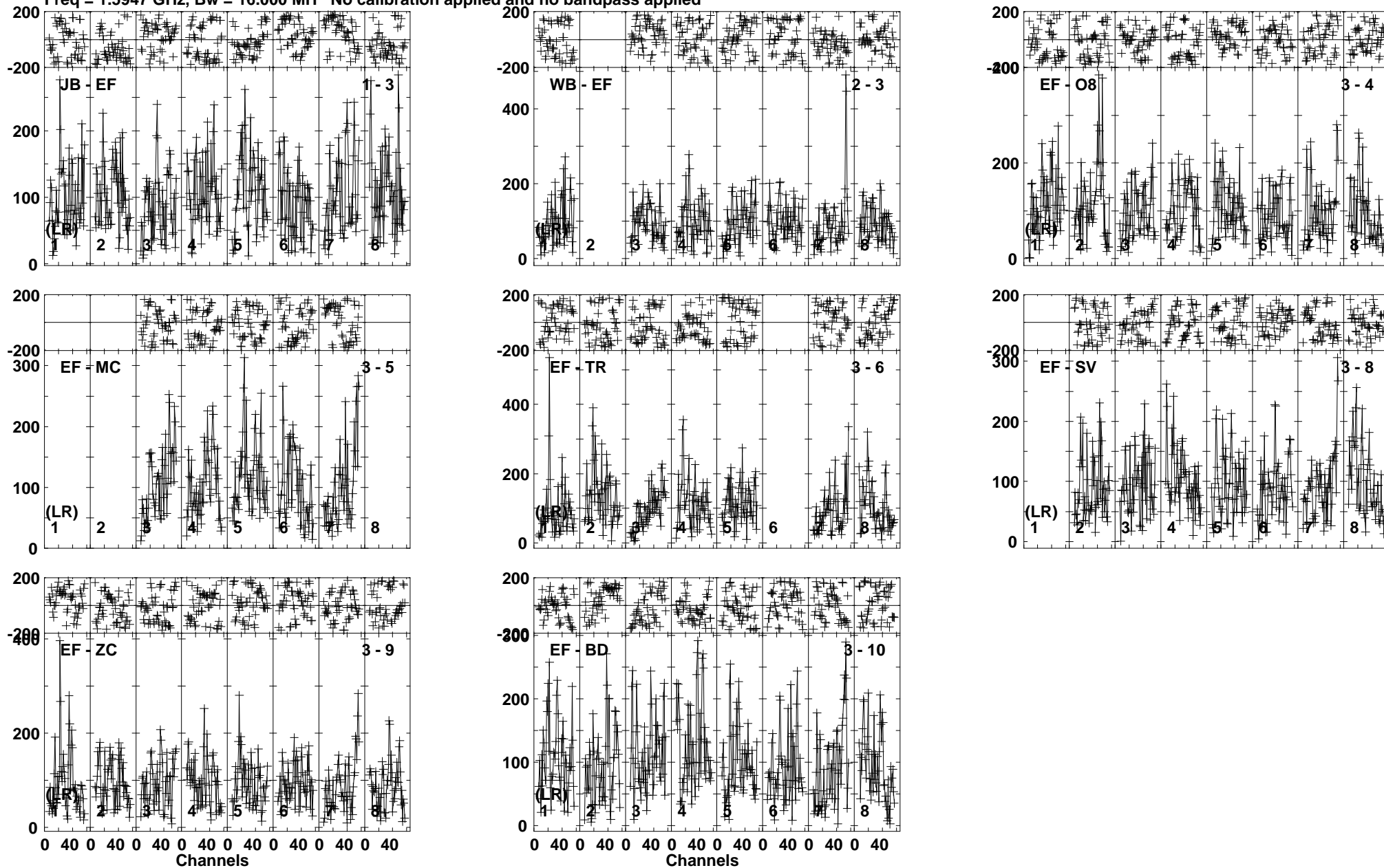
Lower frame: Micro Ampl Jy Top frame: Phas deg Vector averaged cross-power spectrum Baseline: JB (01) - EF (03) Timerange: 00:19:44:44 to 00:19:48:18
