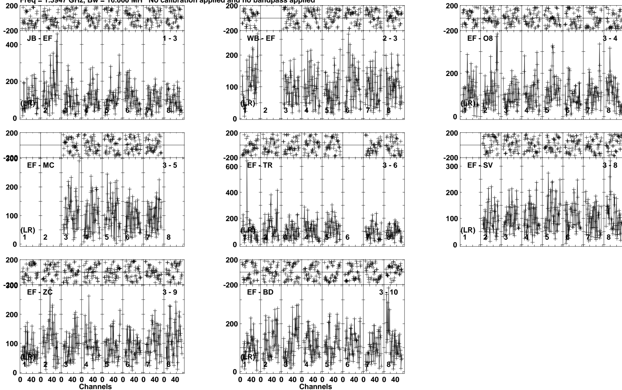
Lower frame: Micro Ampl Jy Top frame: Phas deg Vector averaged cross-power spectrum Baseline: JB (01) - EF (03) Timerange: 00/21:11:12 to 00/21:14:34
