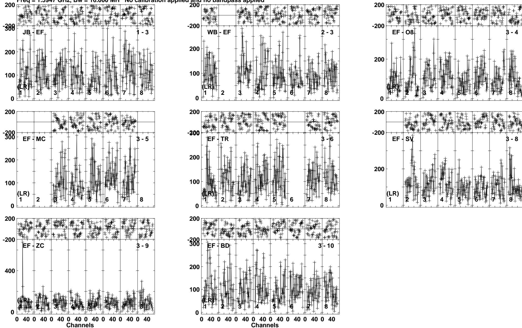
Lower frame: Micro Ampl Jy Top frame: Phas deg Vector averaged cross-power spectrum Baseline: JB (01) - EF (03) Timerange: 00/20:40:42 to 00/20:44:04
