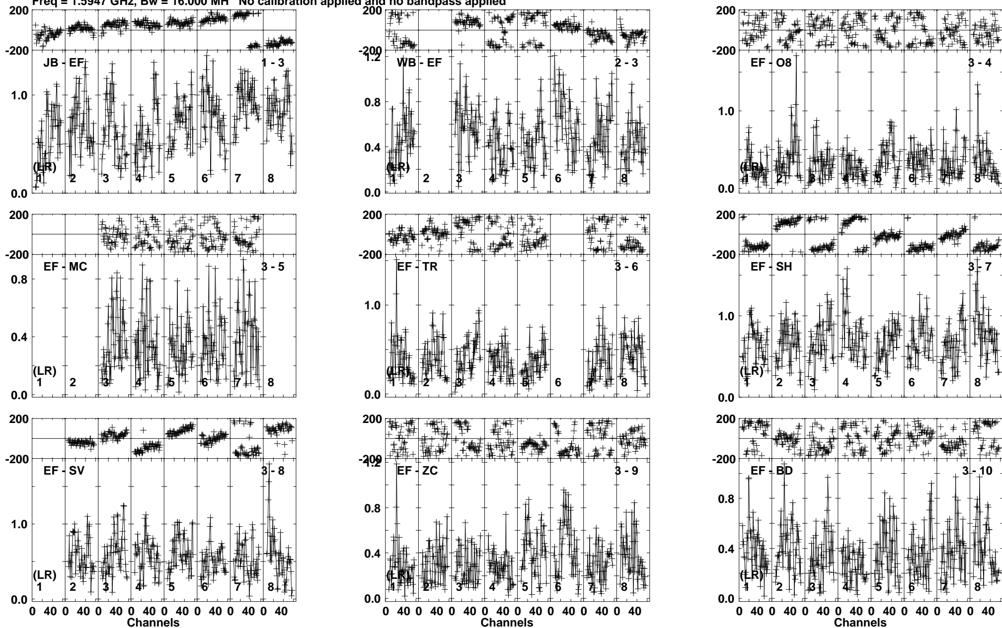
Lower frame: Milli Ampl Jy Top frame: Phas deg Vector averaged cross-power spectrum Baseline: JB (01) - EF (03) Timerange: 00/19:16:26 to 00/19:17:38
