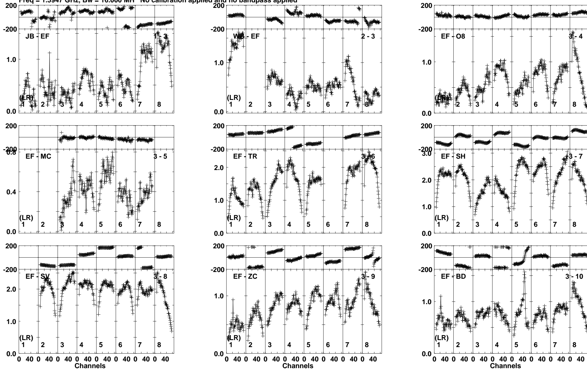
Lower frame: Milli Ampl Jy Top frame: Phas deg Vector averaged cross-power spectrum Baseline: JB (01) - EF (03) Timerange: 00:12:25:03 to 00:12:28:59
