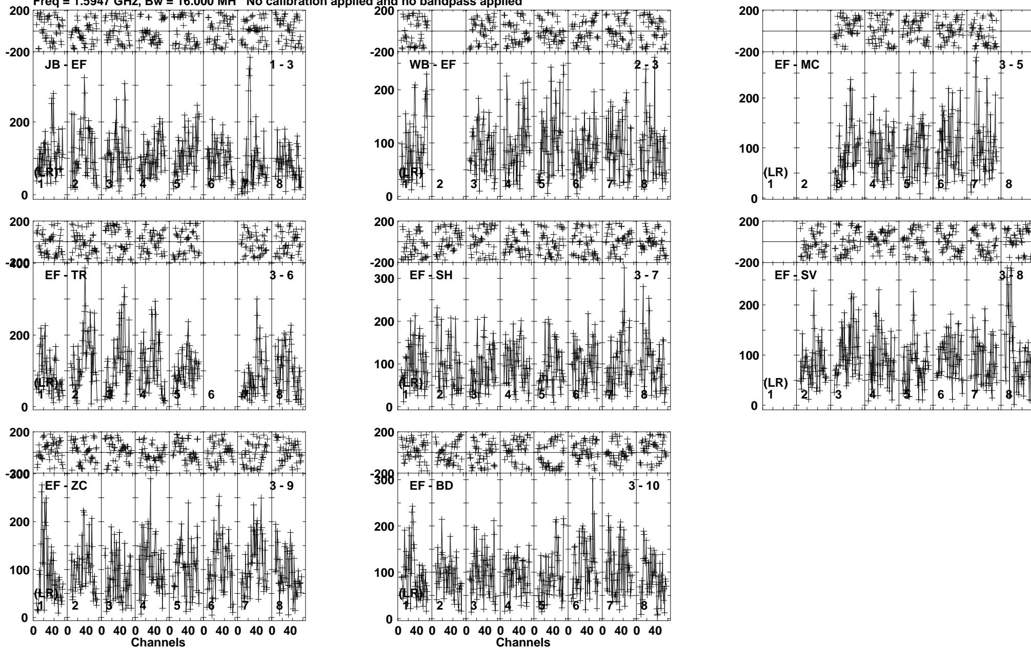
Lower frame: Micro Ampl Jy Top frame: Phas deg Vector averaged cross-power spectrum Baseline: JB (01) - EF (03) Timerange: 00/15:58:26 to 00/16:01:58
