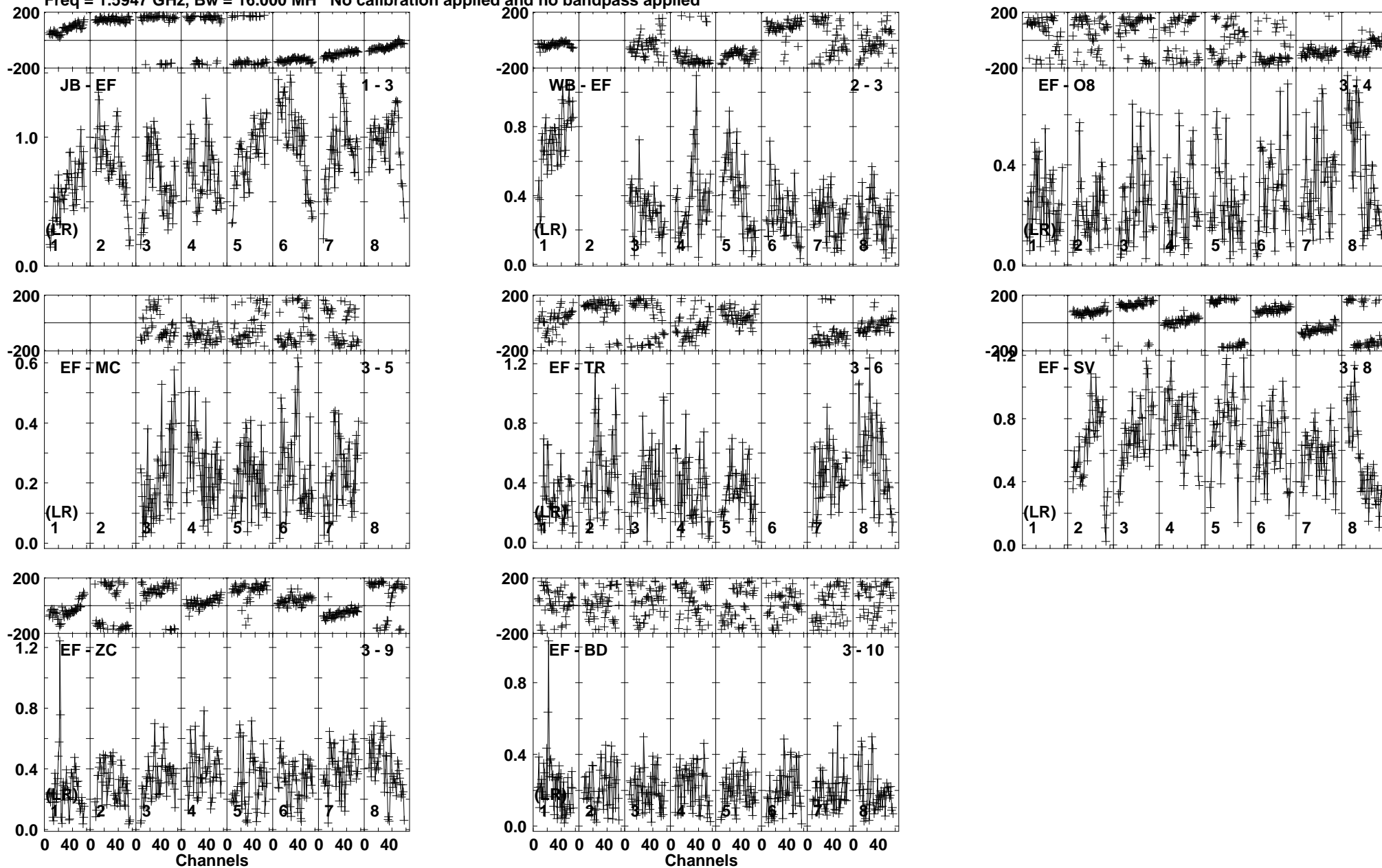
Lower frame: Milli Ampl Jy Top frame: Phas deg Vector averaged cross-power spectrum Baseline: JB (01) - EF (03) Timerange: 00/21:09:57 to 00/21:11:03
