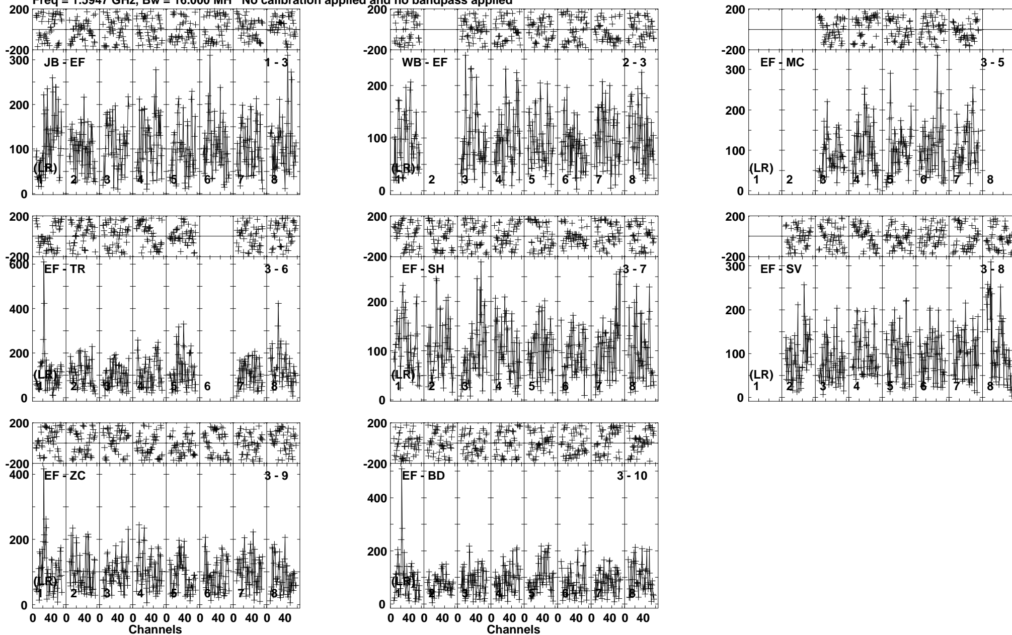
Lower frame: Micro Ampl Jy Top frame: Phas deg Vector averaged cross-power spectrum Baseline: JB (01) - EF (03) Timerange: 00/15:10:44 to 00/15:14:18
