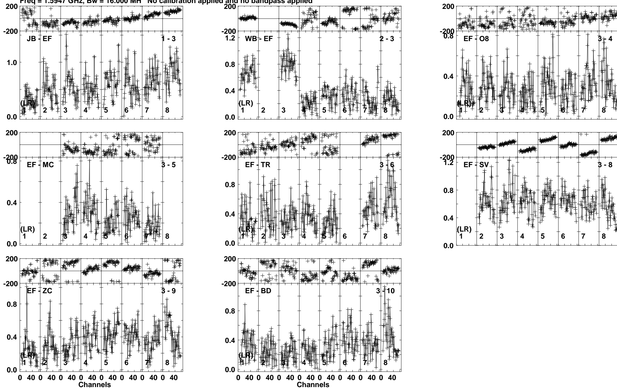
Lower frame: Milli Ampl Jy Top frame: Phas deg Vector averaged cross-power spectrum Baseline: JB (01) - EF (03) Timerange: 00:19:59:07 to 00:20:00:19
