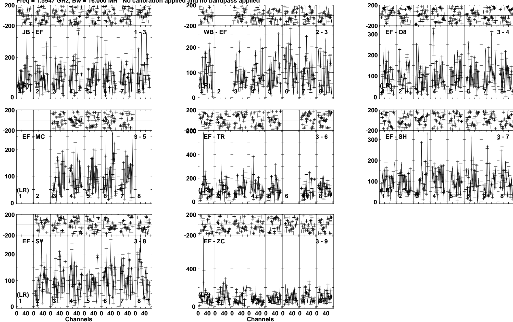
Lower frame: Micro Ampl Jy Top frame: Phas deg Vector averaged cross-power spectrum Baseline: JB (01) - EF (03) Timerange: 00/13:41:26 to 00/13:44:58
