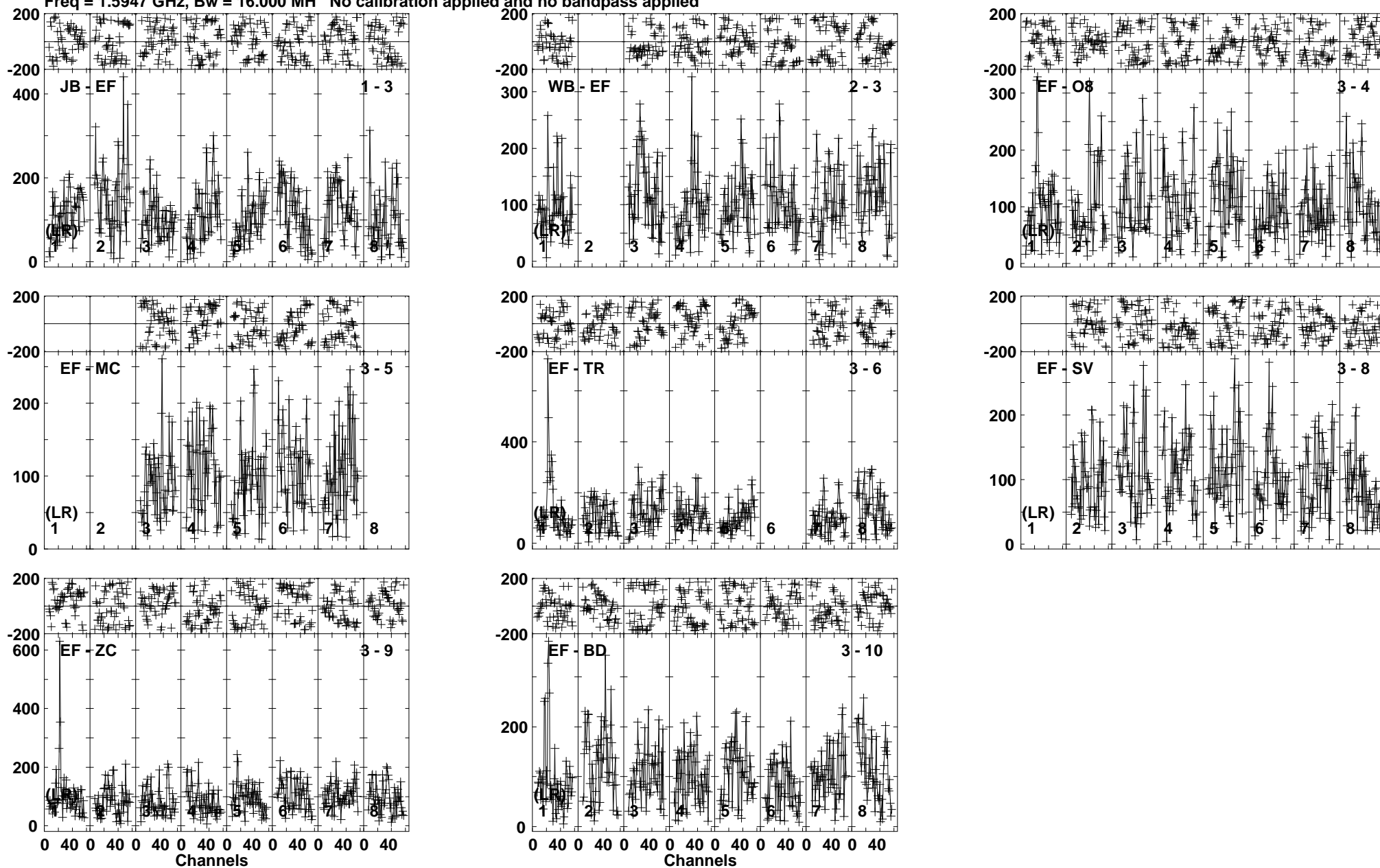
Lower frame: Micro Ampl Jy Top frame: Phas deg Vector average cross-power spectrum Baseline: JB (01) - EF (03) Timerange: 00/21:57:14 to 00/22:00:38
