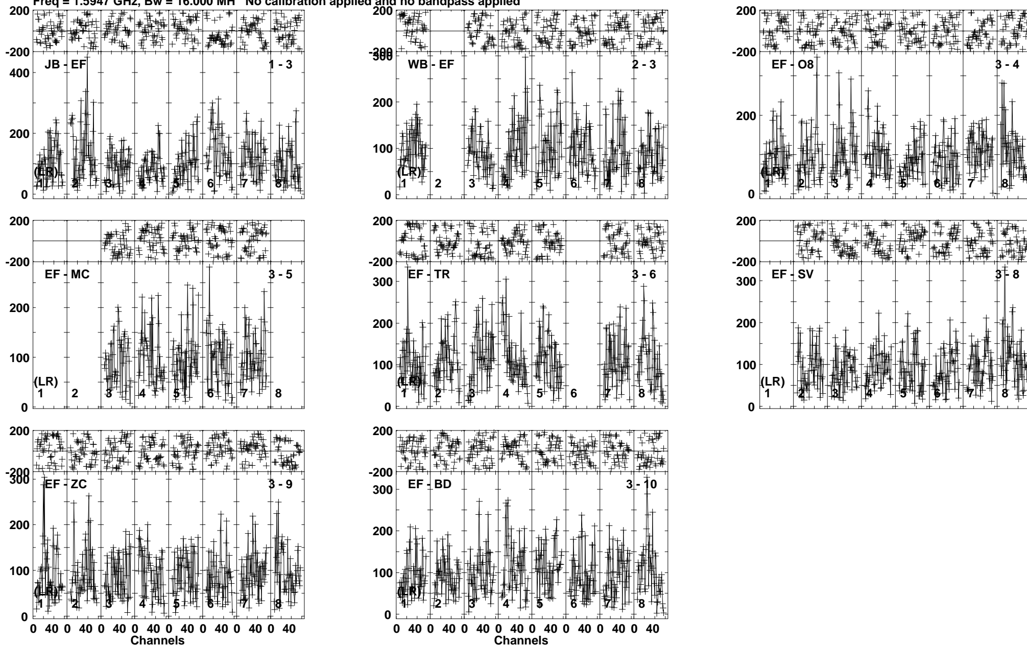
Lower frame: Micro Ampl Jy Top frame: Phas deg Vector average cross-power spectrum Baseline: JB (01) - EF (03) Timerange: 00/20:35:54 to 00/20:39:18
