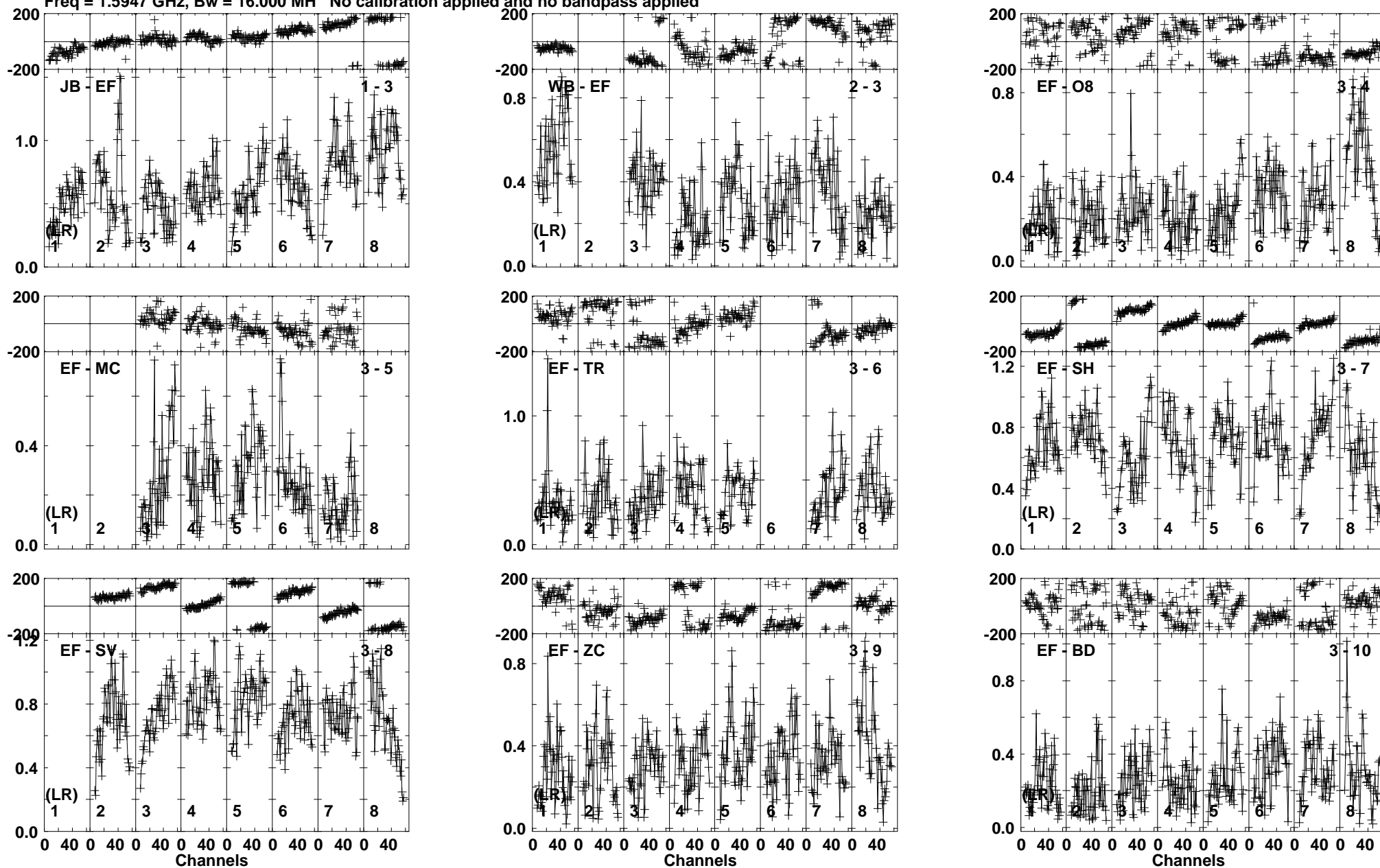
Lower frame: Milli Ampl Jy Top frame: Phas deg Vector averaged cross-power spectrum Baseline: JB (01) - EF (03) Timerange: 00/18:03:26 to 00/18:04:38
