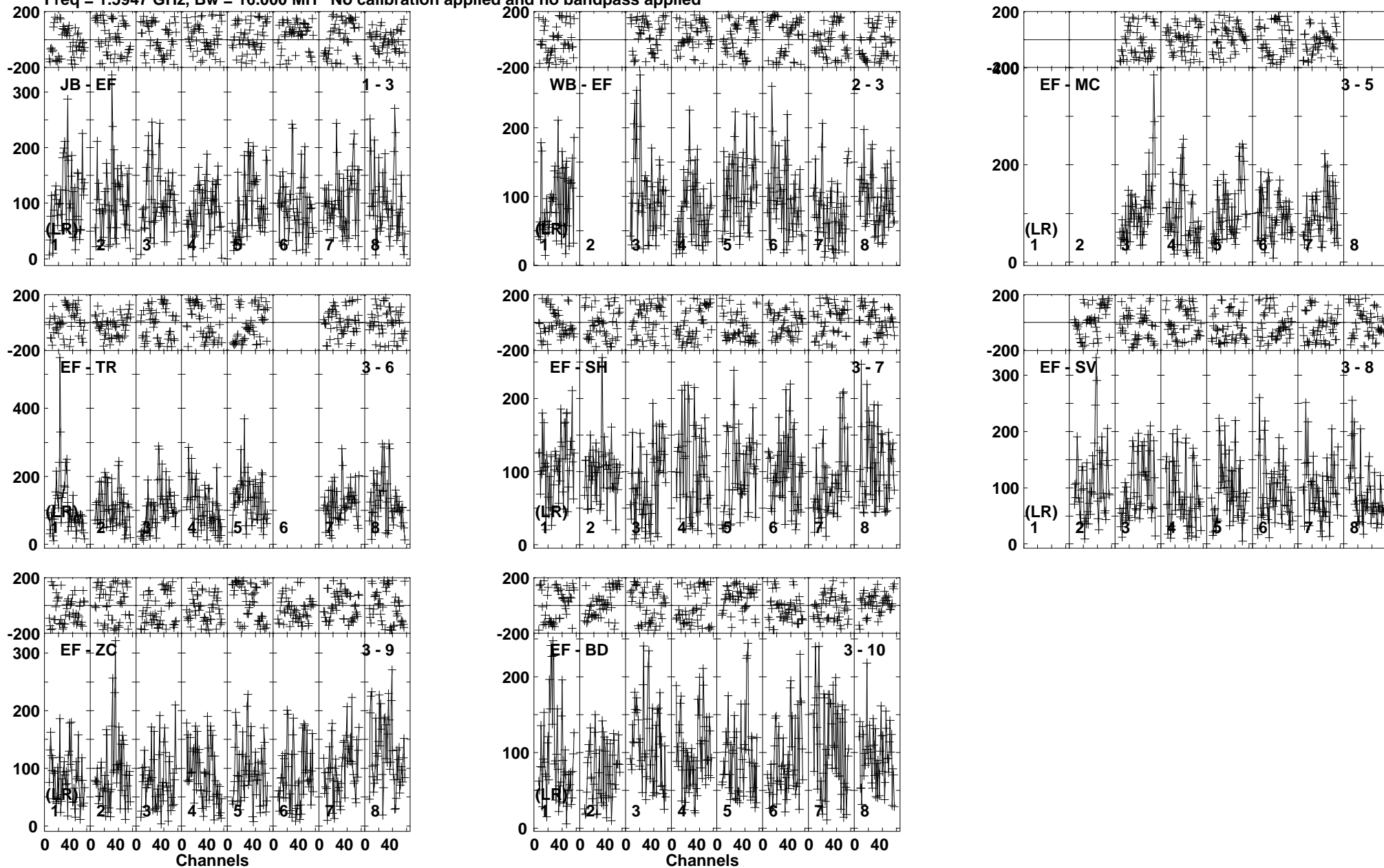
Lower frame: Micro Ampl Jy Top frame: Phas deg Vector averaged cross-power spectrum Baseline: JB (01) - EF (03) Timerange: 00/14:33:06 to 00/14:36:38
