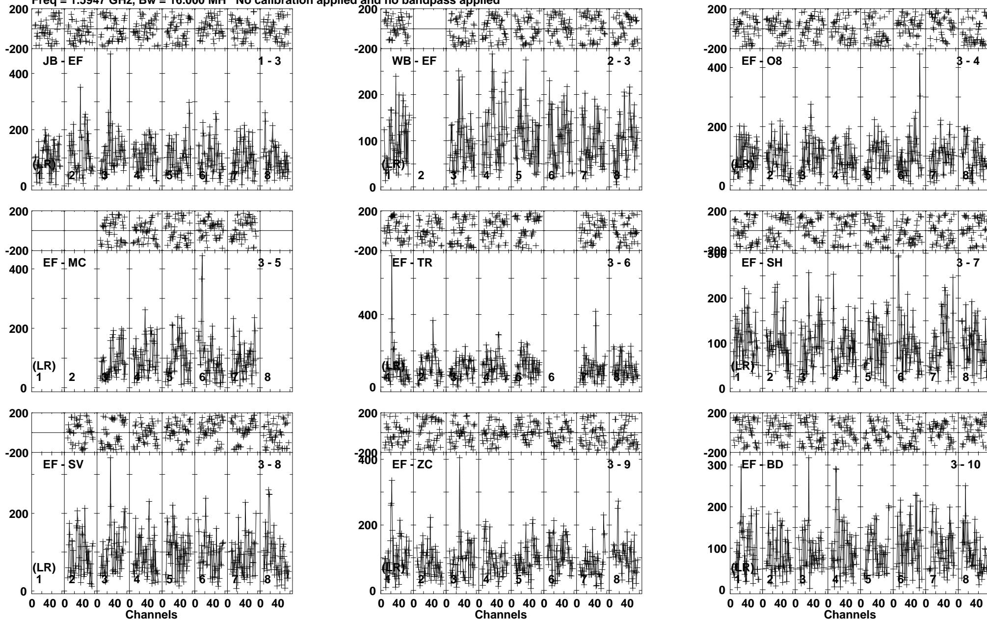
Lower frame: Micro Ampl Jy Top frame: Phas deg Vector averaged cross-power spectrum Baseline: JB (01) - EF (03) Timerange: 00/18:04:46 to 00/18:08:18
