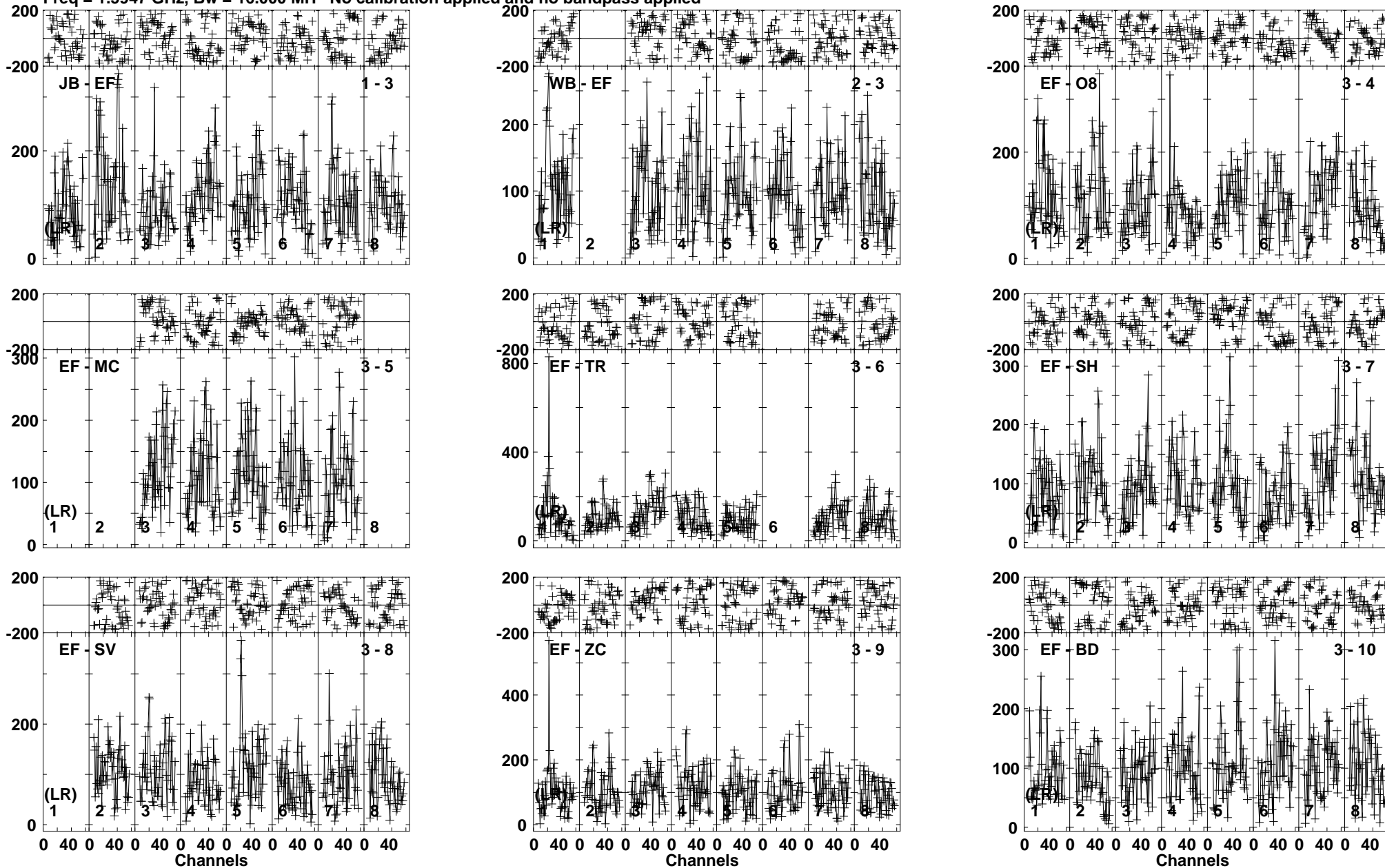
Lower frame: Micro Ampl Jy Top frame: Phas deg Vector averaged cross-power spectrum Baseline: JB (01) - EF (03) Timerange: 00/19:07:06 to 00/19:10:38
