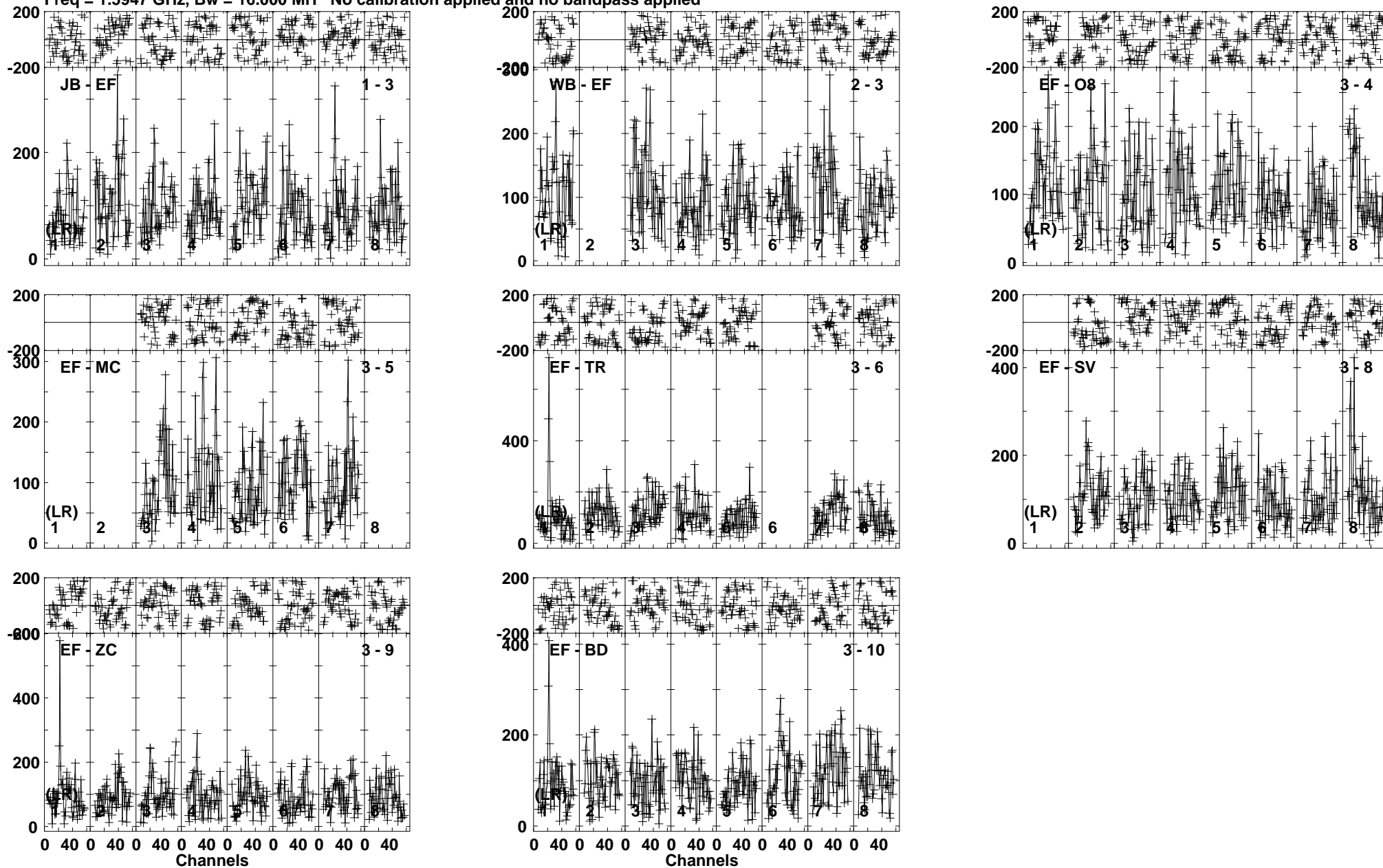
Lower frame: Micro Ampl Jy Top frame: Phas deg Vector average cross-power spectrum Baseline: JB (01) - EF (03) Timerange: 00/20:56:14 to 00/20:59:38
