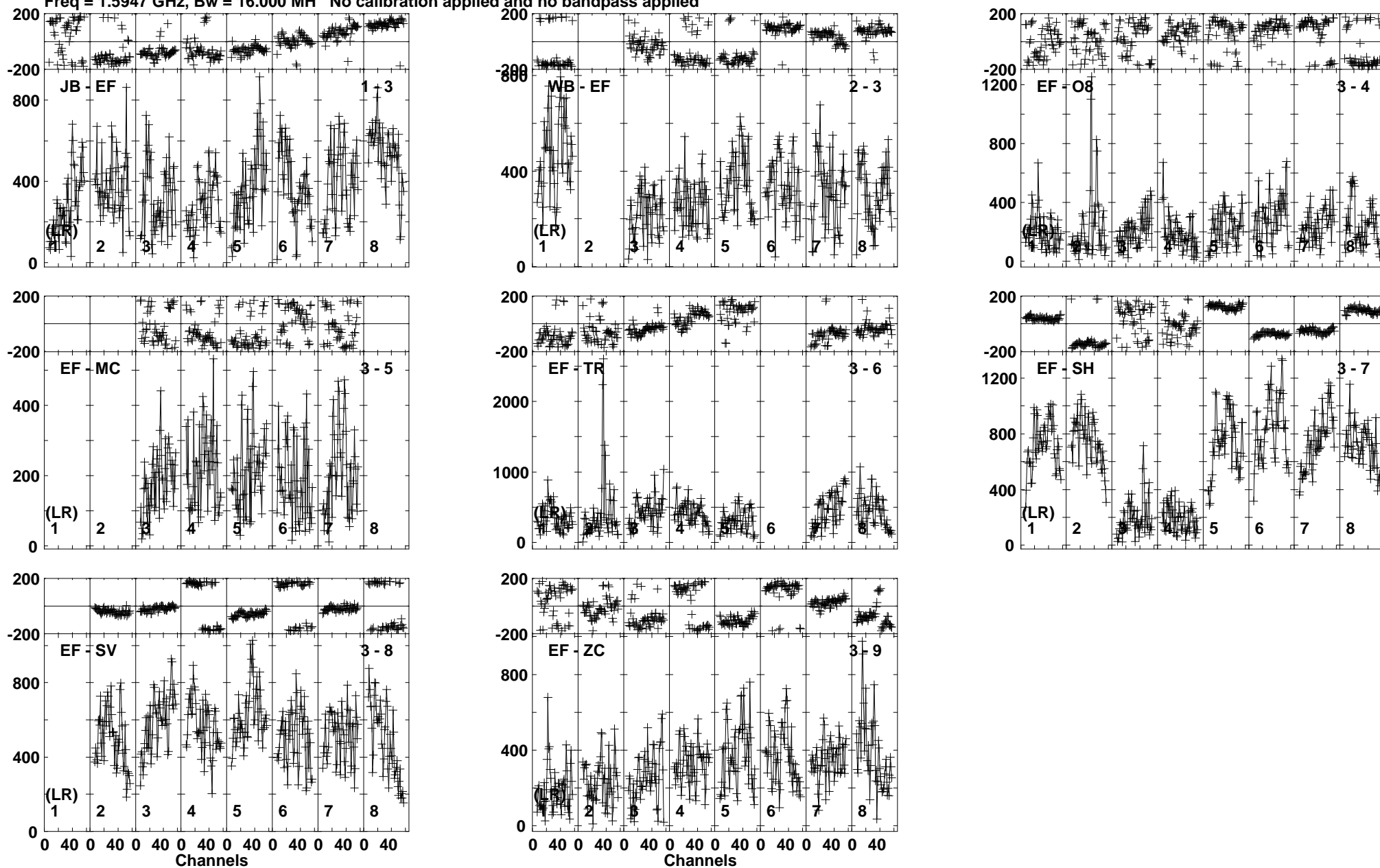
Lower frame: Micro Ampl Jy Top frame: Phas deg Vector averaged cross-power spectrum Baseline: JB (01) - EF (03) Timerange: 00/13:29:26 to 00/13:30:38
