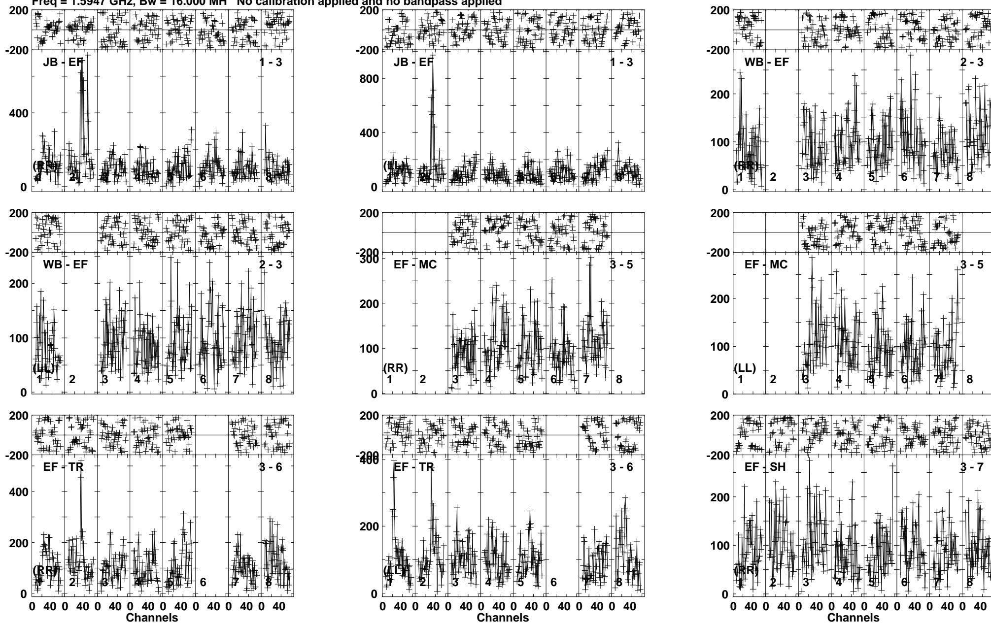
Lower frame: Micro Ampl Jy Top frame: Phas deg Vector averaged cross-power spectrum Baseline: JB (01) - EF (03) Timerange: 00/16:04:04 to 00/16:07:38
