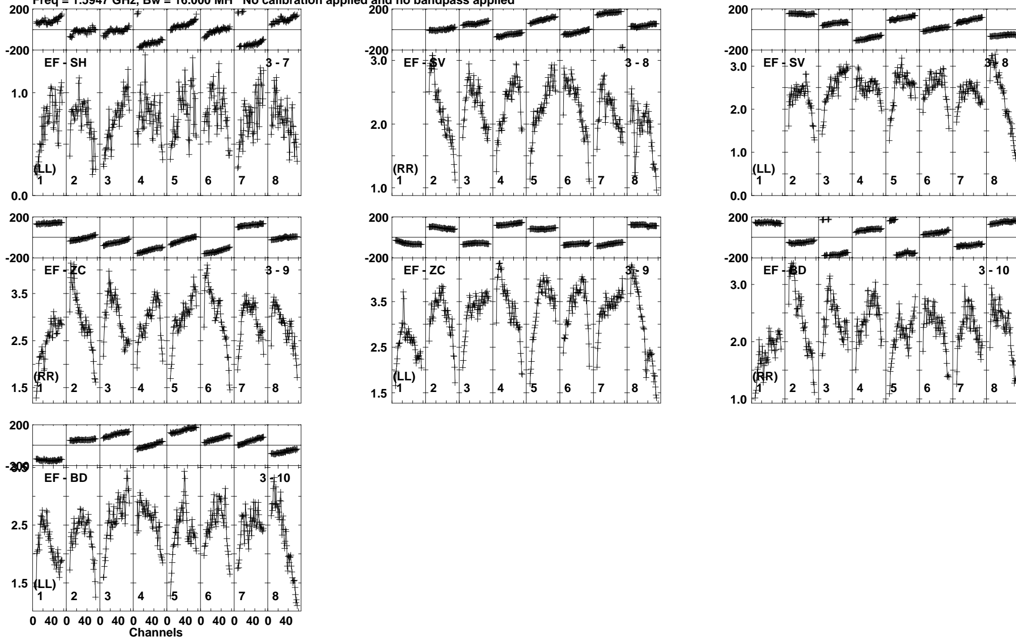
Lower frame: Milli Ampl Jy Top frame: Phas deg Vector averaged cross-power spectrum Baseline: EF (03) - SH (07) Timerange: 00/15:35:46 to 00/15:36:58
