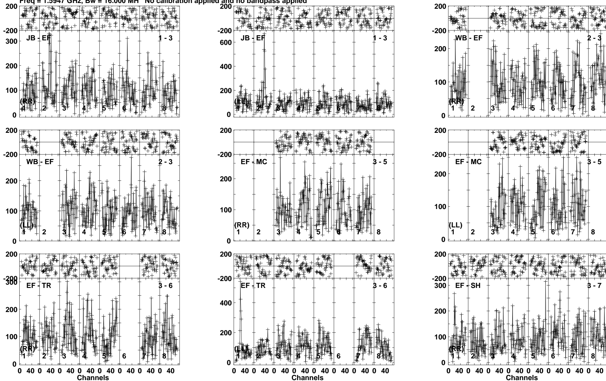
Lower frame: Micro Ampl Jy Top frame: Phas deg Vector averaged cross-power spectrum Baseline: JB (01) - EF (03) Timerange: 00/15:42:44 to 00/15:46:18
