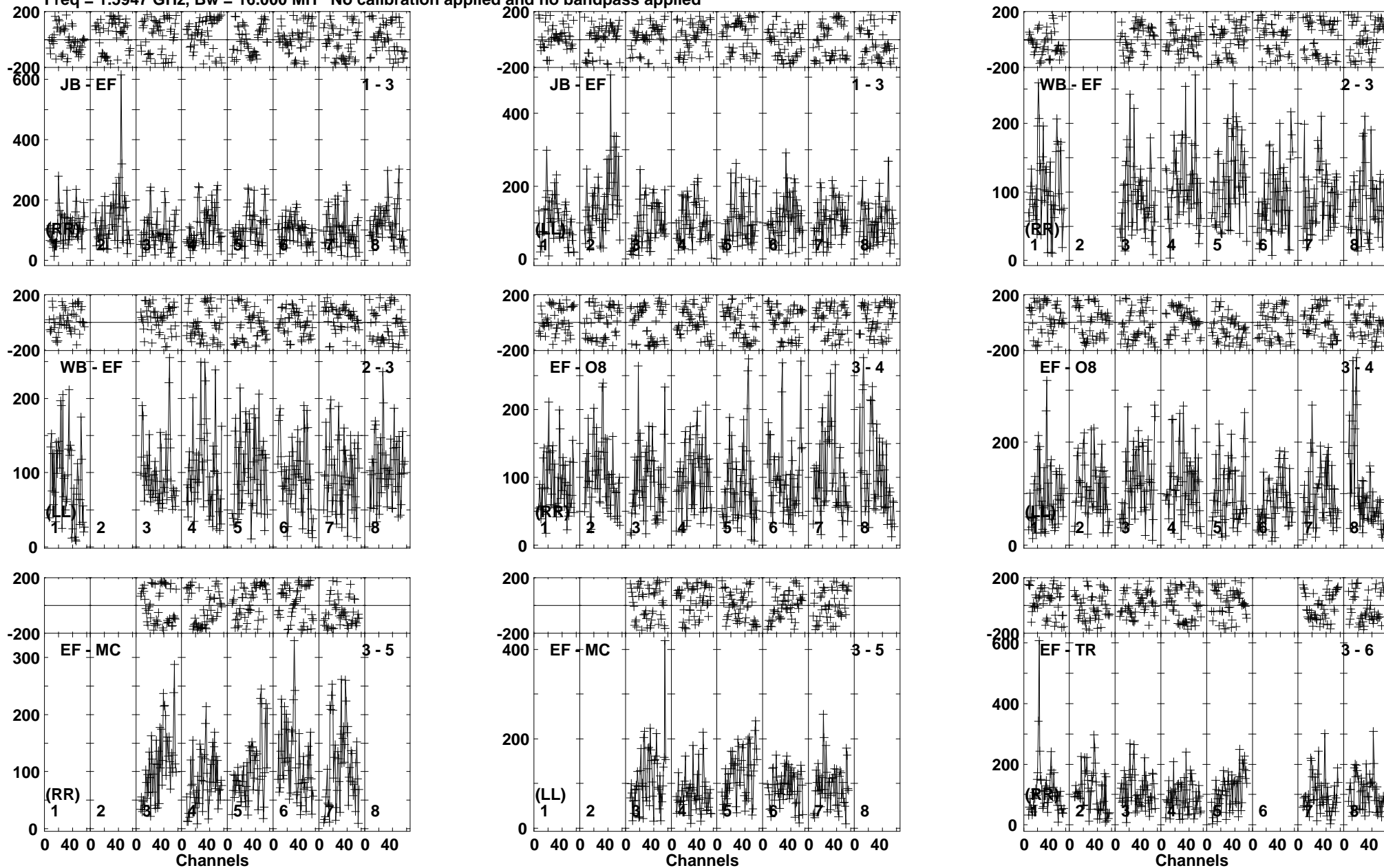
Lower frame: Micro Ampl Jy Top frame: Phas deg Vector averaged cross-power spectrum Baseline: JB (01) - EF (03) Timerange: 00/20:11:06 to 00/20:14:38
