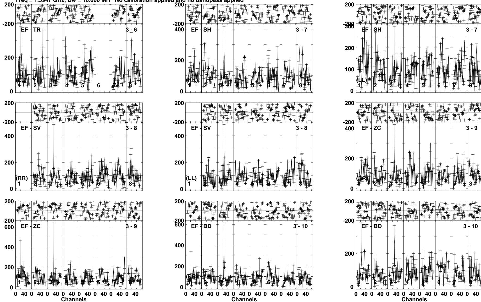
Lower frame: Micro Ampl Jy Top frame: Phas deg Vector averaged cross-power spectrum Baseline: EF (03) - TR (06) Timerange: 00/18:10:24 to 00/18:13:58
