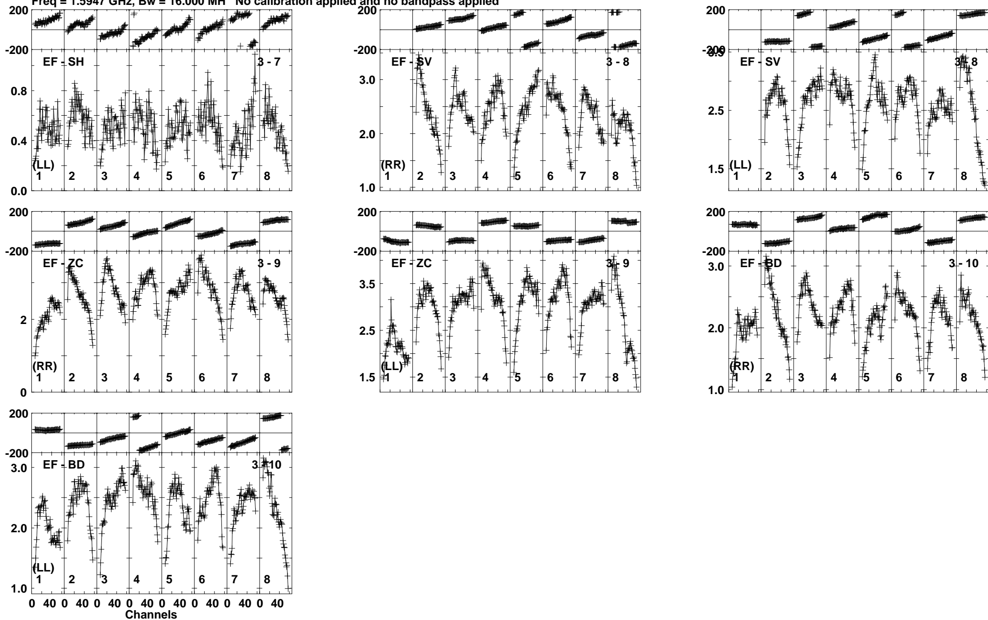
Lower frame: Milli Ampl Jy Top frame: Phas deg Vector averaged cross-power spectrum Baseline: EF (03) - SH (07) Timerange: 00:19:43:23 to 00:19:44:39
