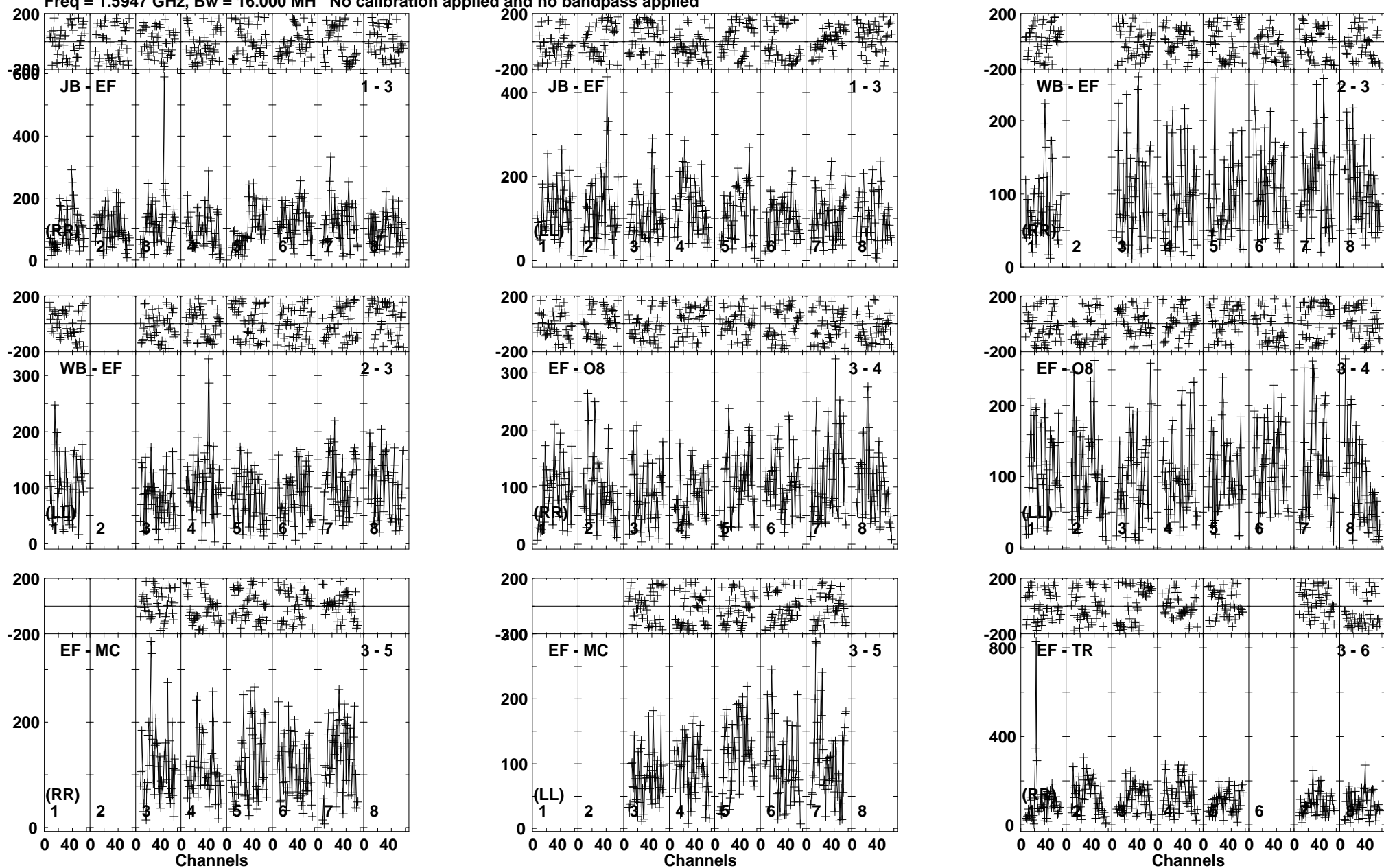
Lower frame: Micro Ampl Jy Top frame: Phas deg Vector averaged cross-power spectrum Baseline: JB (01) - EF (03) Timerange: 00/20:30:32 to 00/20:33:54
