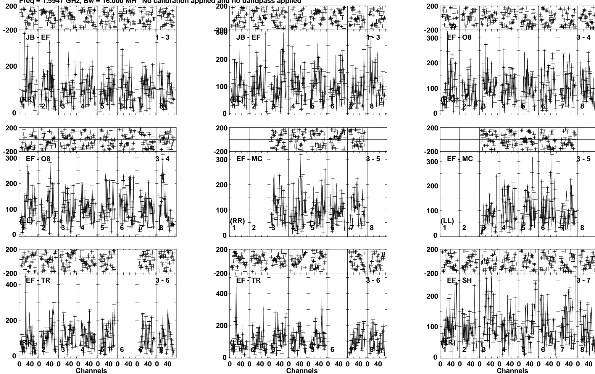
Lower frame: Micro Ampl Jy Top frame: Phas deg Vector averaged cross-power spectrum Baseline: JB (01) - EF (03) Timerange: 00/13:04:24 to 00/13:07:58
