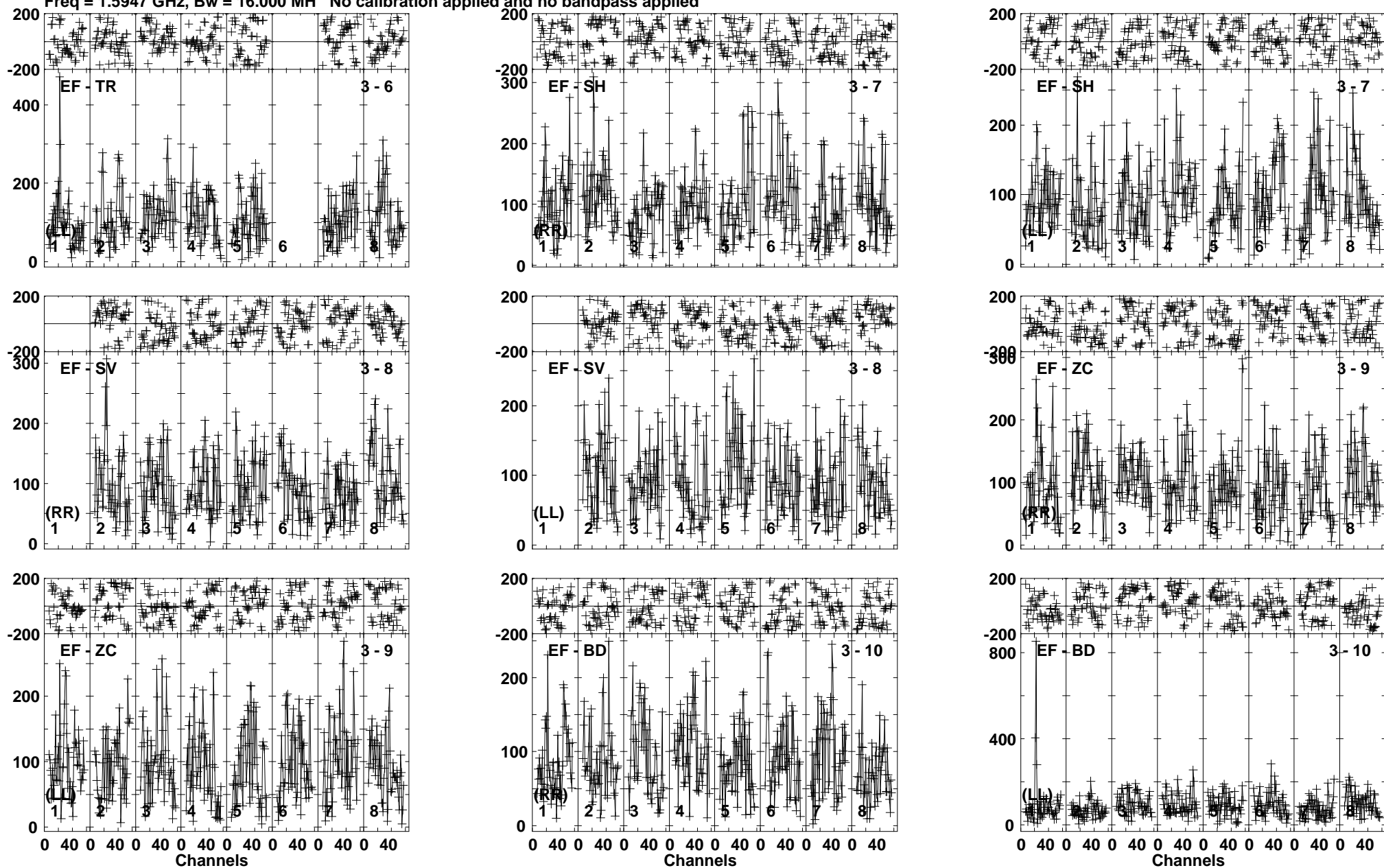
Lower frame: Micro Ampl Jy Top frame: Phas deg Vector averaged cross-power spectrum Baseline: EF (03) - TR (06) Timerange: 00/13:57:43 to 00/14:01:19
