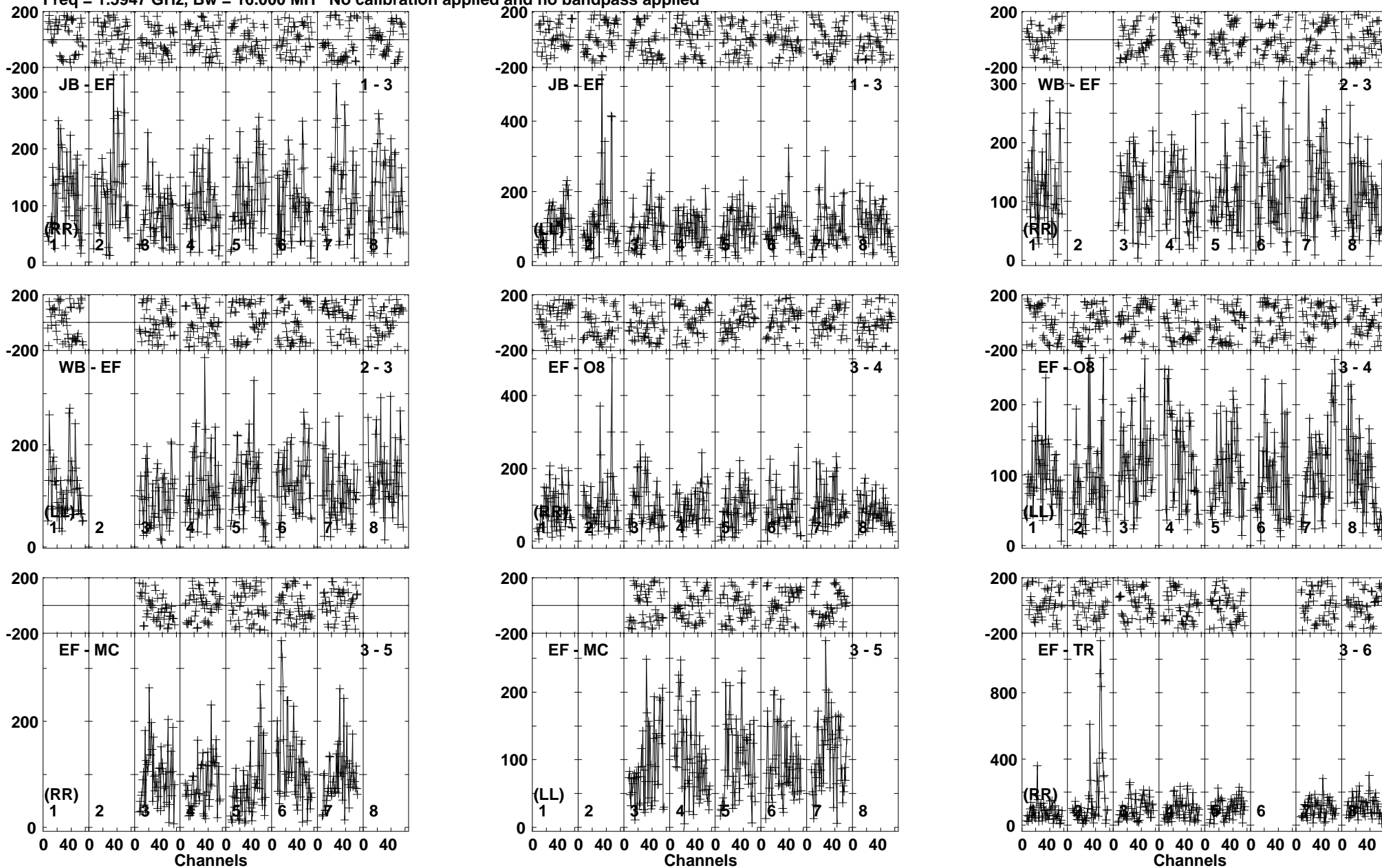
Lower frame: Micro Ampl Jy Top frame: Phas deg Vector averaged cross-power spectrum Baseline: JB (01) - EF (03) Timerange: 00/13:20:04 to 00/13:23:38
