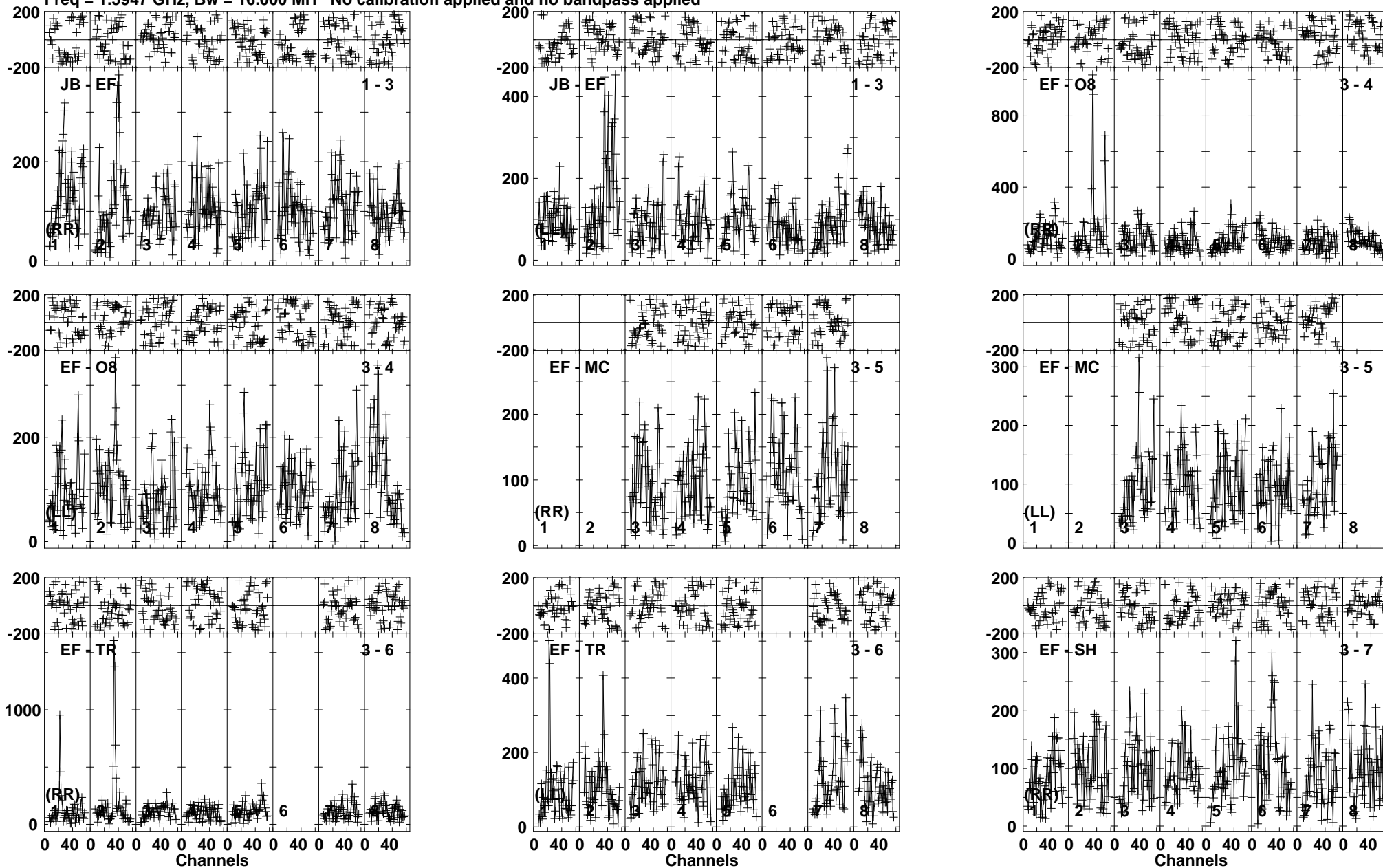
Lower frame: Micro Ampl Jy Top frame: Phas deg Vector averaged cross-power spectrum Baseline: JB (01) - EF (03) Timerange: 00:12:43:04 to 00:12:46:38
