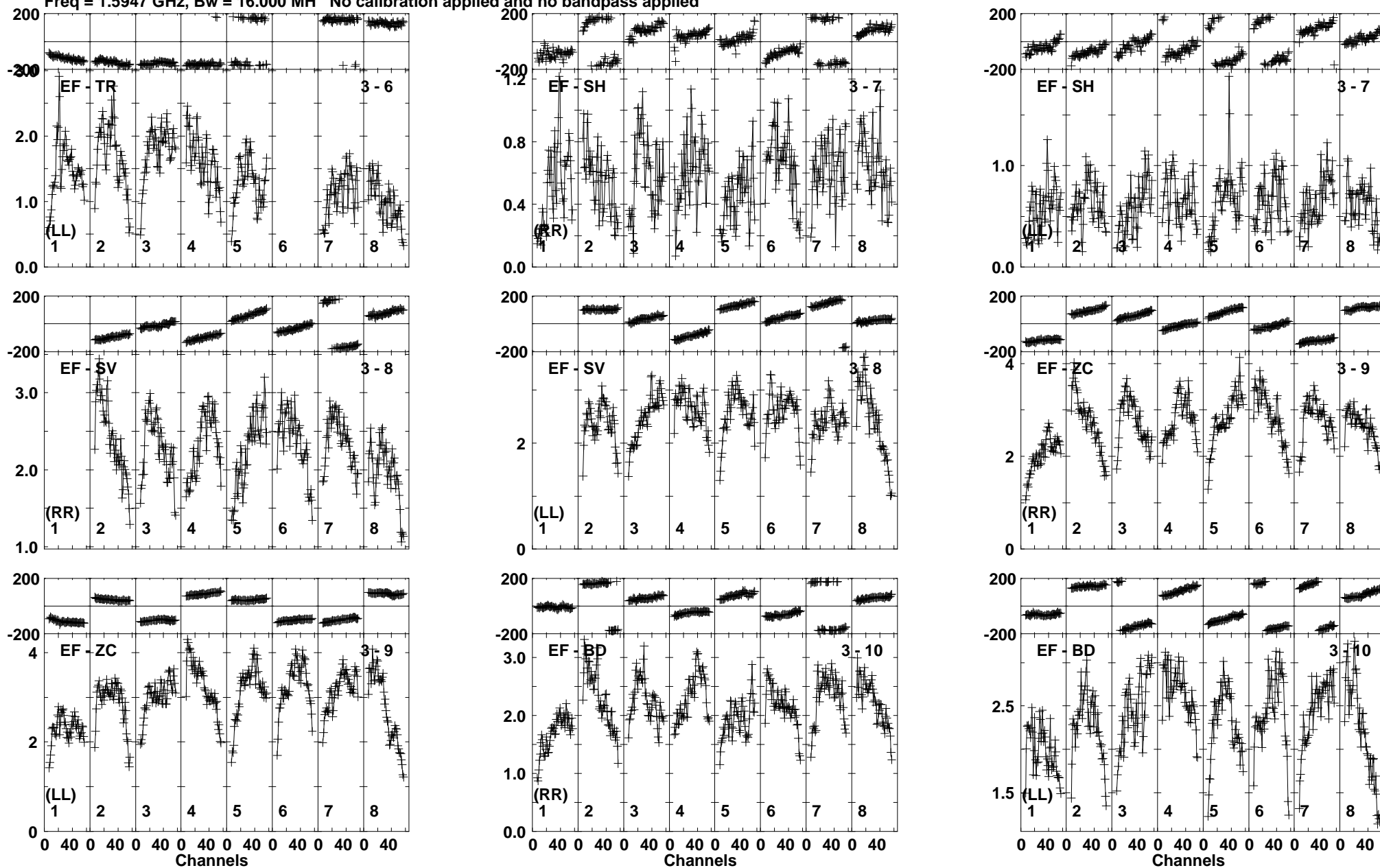
Lower frame: Milli Ampl Jy Top frame: Phas deg Vector averaged cross-power spectrum Baseline: EF (03) - TR (06) Timerange: 00:19:37:46 to 00:19:38:58
