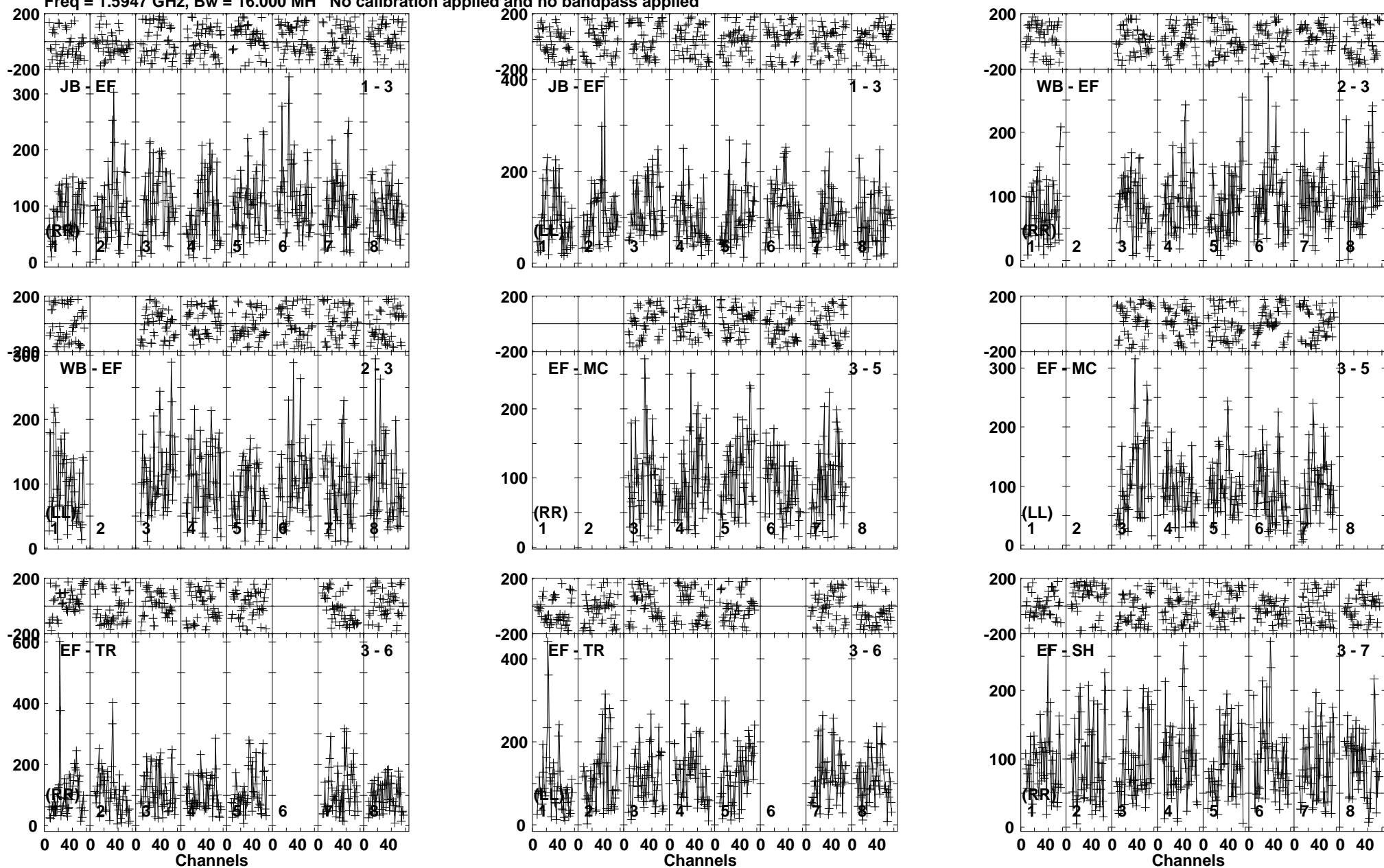
Lower frame: Micro Ampl Jy Top frame: Phas deg Vector averaged cross-power spectrum Baseline: JB (01) - EF (03) Timerange: 00/16:34:24 to 00/16:37:58
