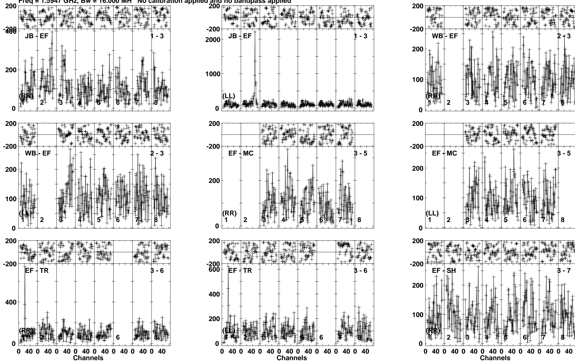
Lower frame: Micro Ampl Jy Top frame: Phas deg Vector averaged cross-power spectrum Baseline: JB (01) - EF (03) Timerange: 00/15:32:04 to 00/15:35:38
