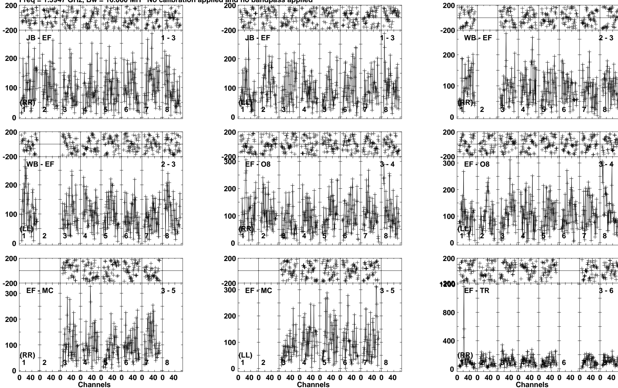
Lower frame: Micro Ampl Jy Top frame: Phas deg Vector averaged cross-power spectrum Baseline: JB (01) - EF (03) Timerange: 00/13:52:03 to 00/13:55:39
