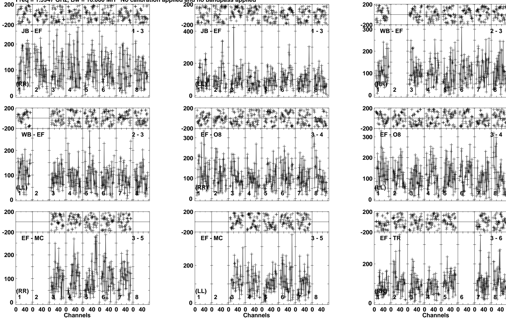
Lower frame: Micro Ampl Jy Top frame: Phas deg Vector averaged cross-power spectrum Baseline: JB (01) - EF (03) Timerange: 00/13:36:24 to 00/13:39:58
