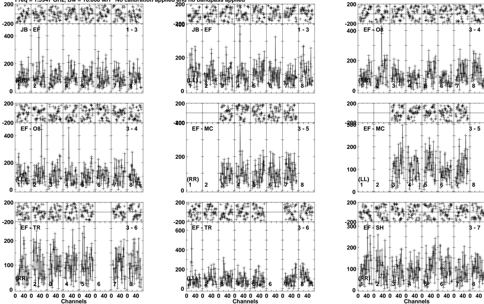
Lower frame: Micro Ampl Jy Top frame: Phas deg Vector averaged cross-power spectrum Baseline: JB (01) - EF (03) Timerange: 00/13:15:04 to 00/13:18:38
