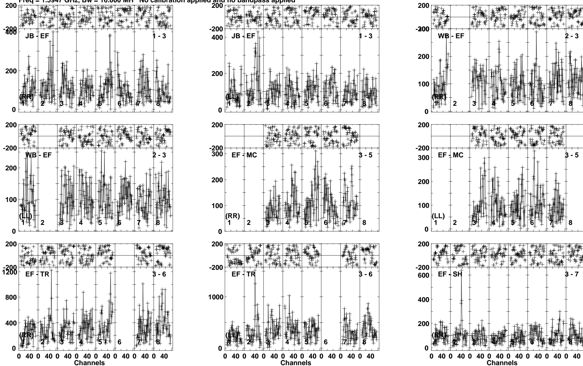
Lower frame: Micro Ampl Jy Top frame: Phas deg Vector averaged cross-power spectrum Baseline: JB (01) - EF (03) Timerange: 00/14:43:46 to 00/14:47:18
