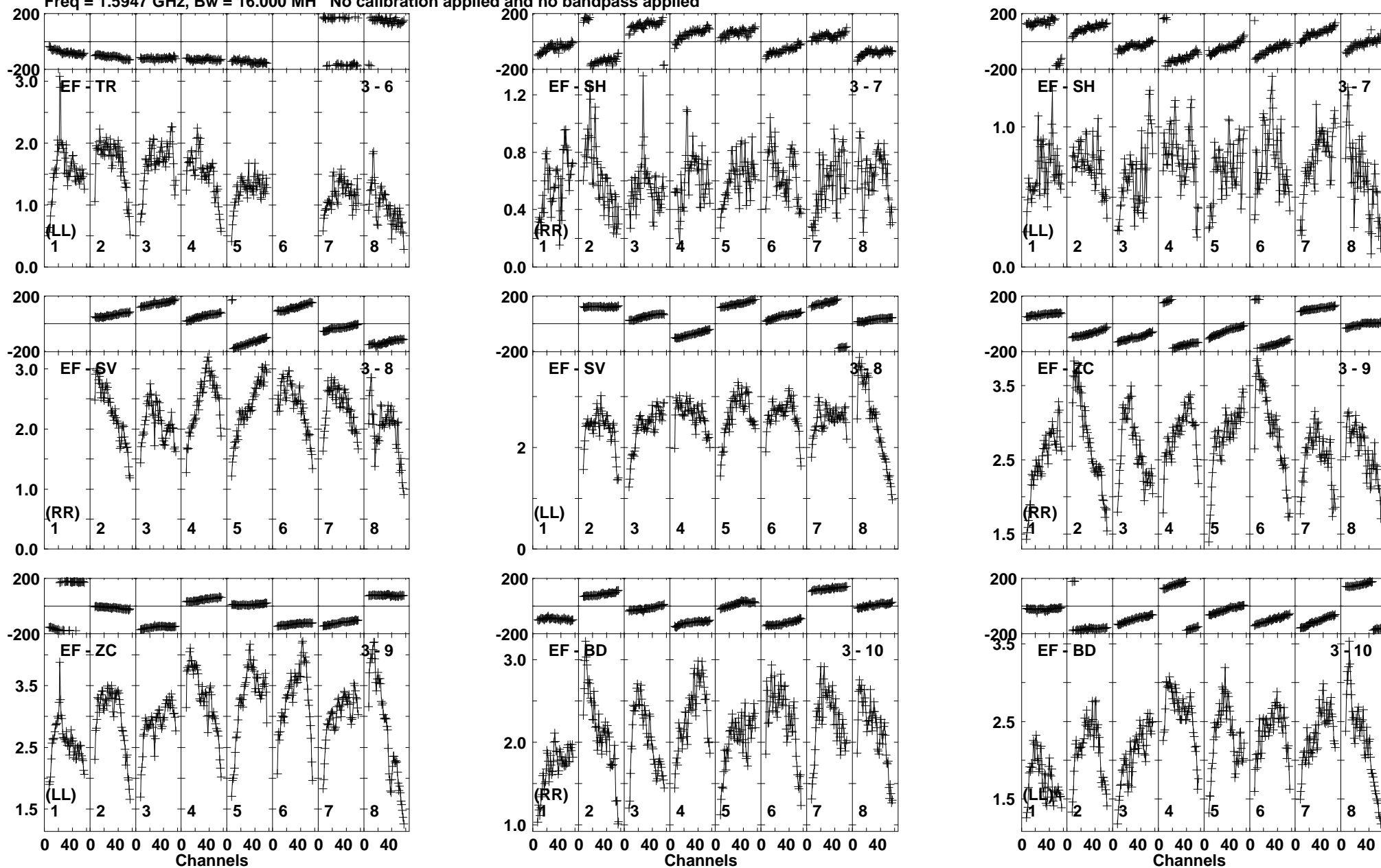
Lower frame: Milli Ampl Jy Top frame: Phas deg Vector averaged cross-power spectrum Baseline: EF (03) - TR (06) Timerange: 00:18:03:26 to 00:18:04:38
