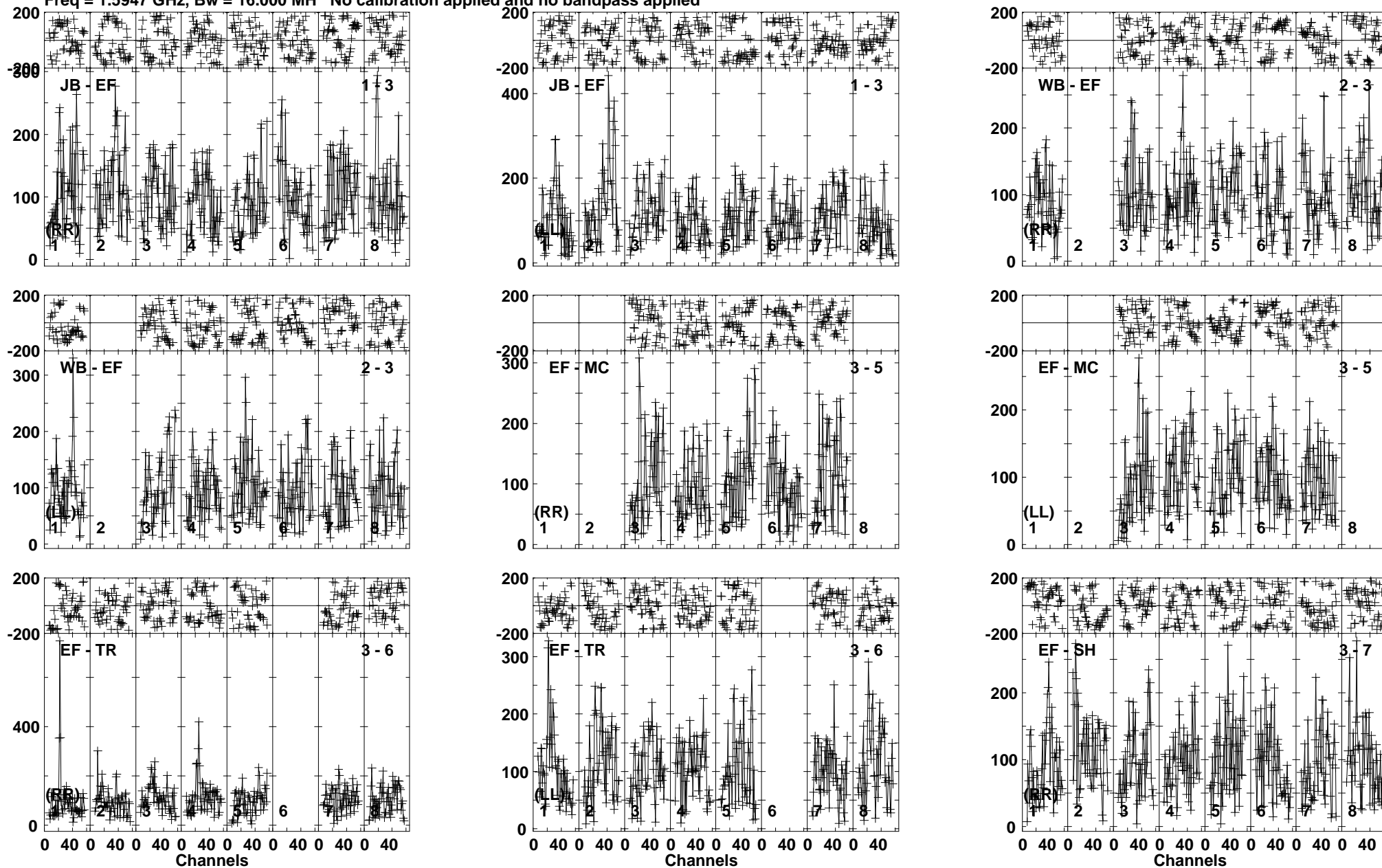
Lower frame: Micro Ampl Jy Top frame: Phas deg Vector averaged cross-power spectrum Baseline: JB (01) - EF (03) Timerange: 00/17:27:44 to 00/17:31:18
