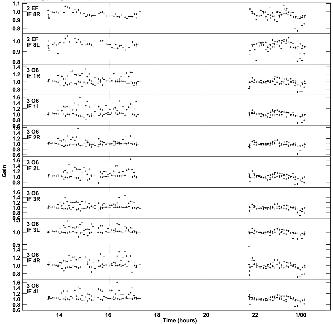
Plot file version 4 created 04-DEC-2015 15:48:42 Gain amp vs UTC time for J1102+2757.MULTI.1 SN 4 Rpol & Lpol IF 1 - 8
