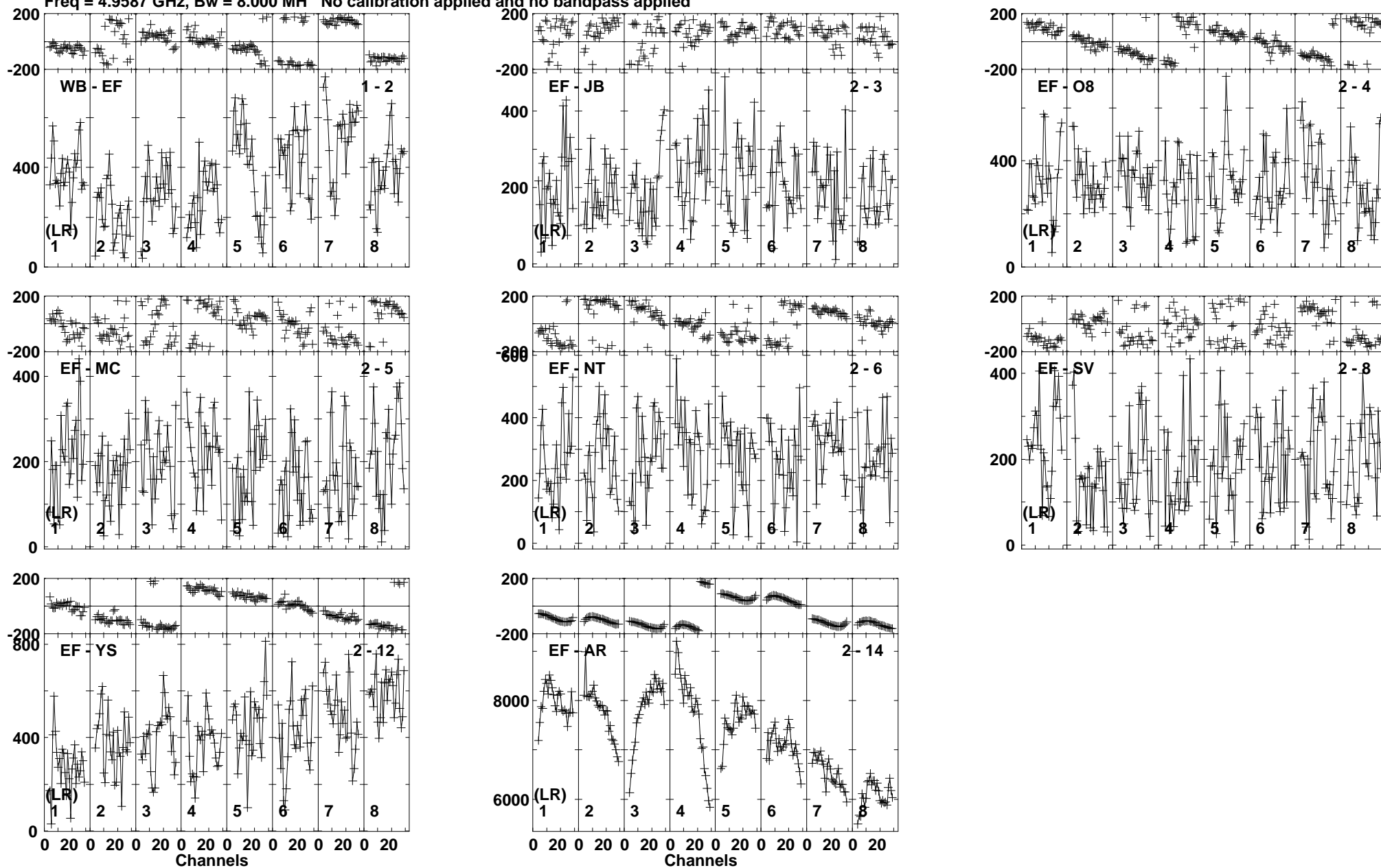
Lower frame: Micro Ampl Jy Top frame: Phas deg Vector averaged cross-power spectrum Baseline: WB (01) - EF (02) Timerange: 00/22:30:42 to 00/22:32:42
