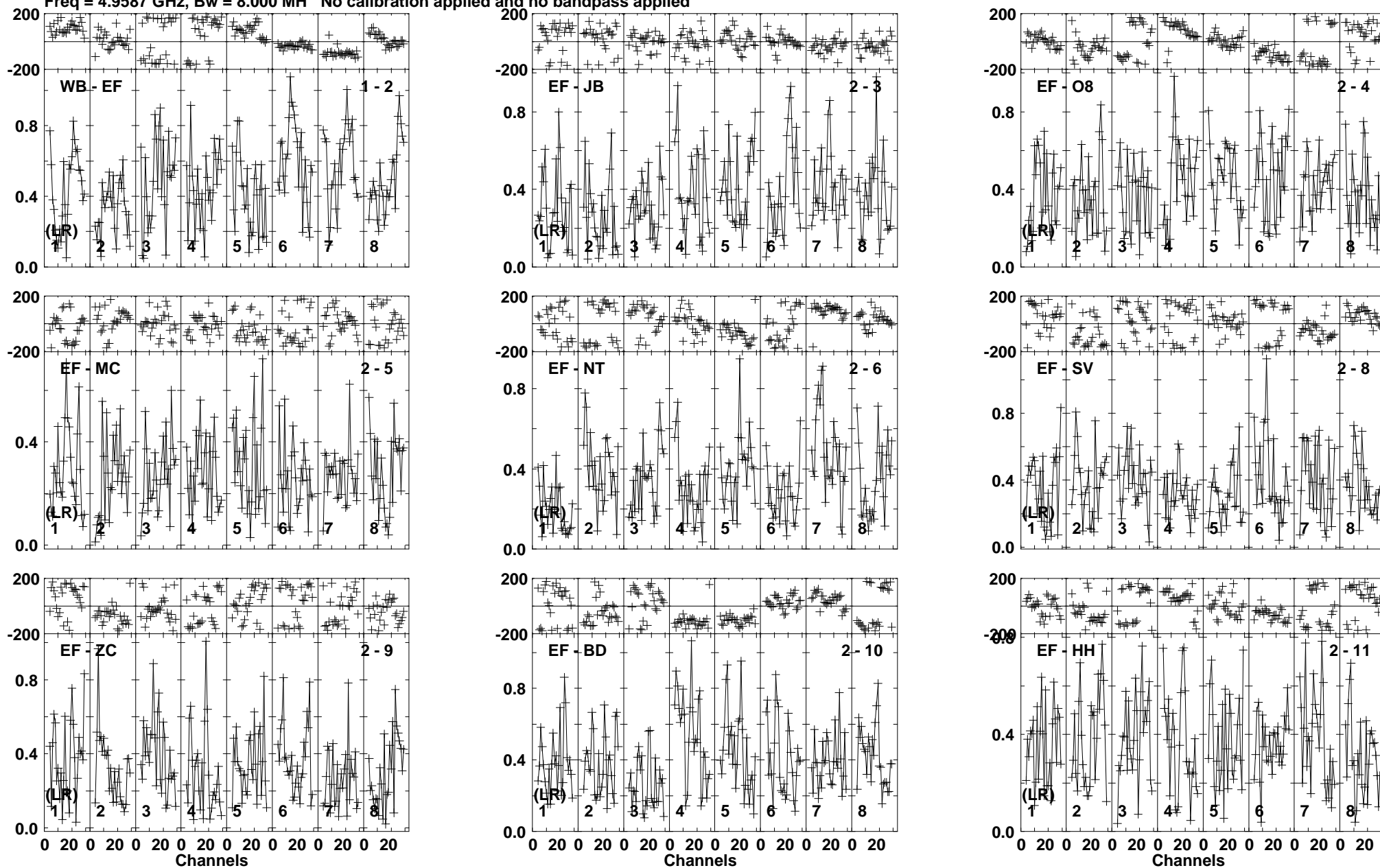
Lower frame: Milli Ampl Jy Top frame: Phas deg Vector averaged cross-power spectrum Baseline: WB (01) - EF (02) Timerange: 00/16:21:17 to 00/16:22:13
