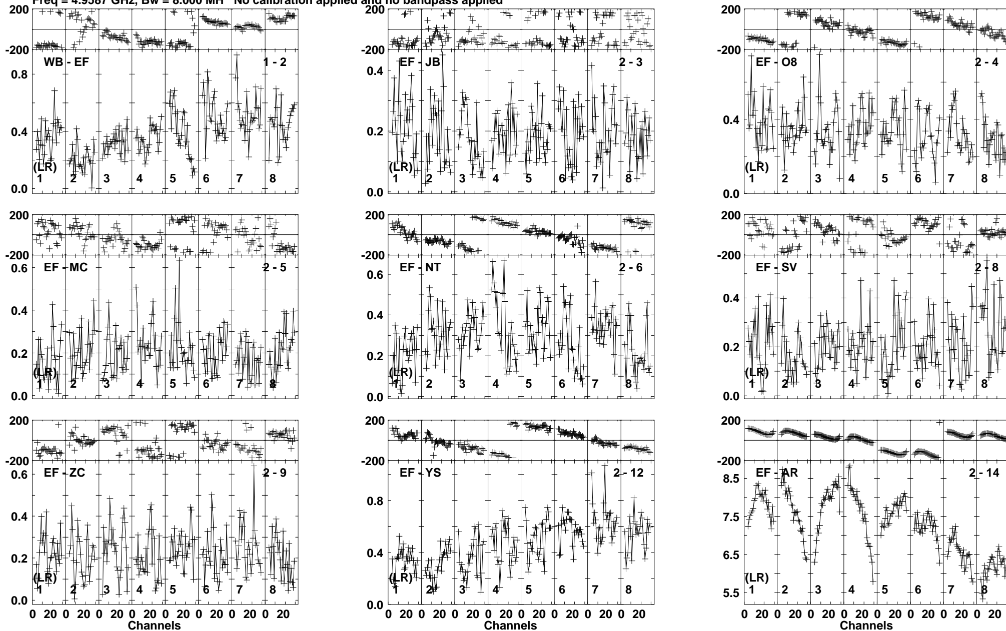
Lower frame: Milli Ampl Jy Top frame: Phas deg Vector averaged cross-power spectrum Baseline: WB (01) - EF (02) Timerange: 00:21:50:56 to 00:21:53:02
