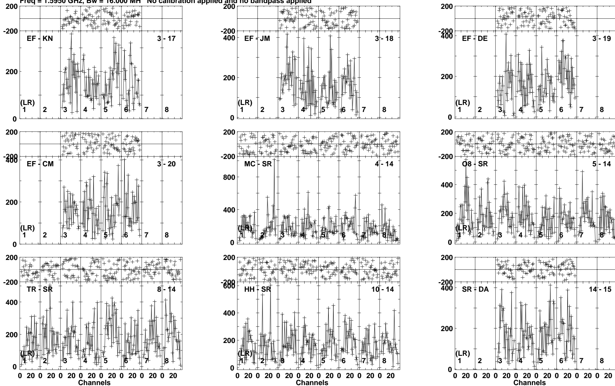
Lower frame: Micro Ampl Jy Top frame: Phas deg Vector averaged cross-power spectrum Baseline: EF (03) - KN (17) Timerange: 01/01:58:31 to 01/01:59:59
