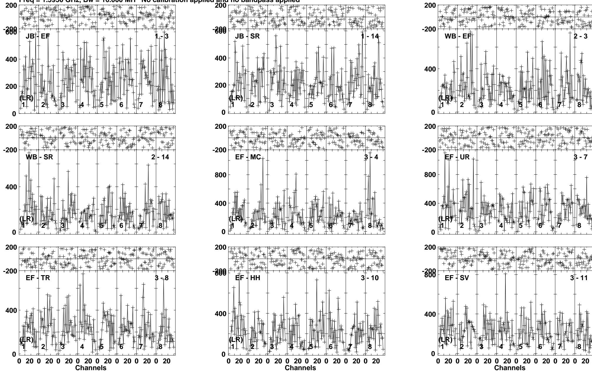
Lower frame: Micro Ampl Jy Top frame: Phas deg Vector averaged cross-power spectrum Baseline: JB (01) - EF (03) Timerange: 00/21:20:12 to 00/21:21:56
