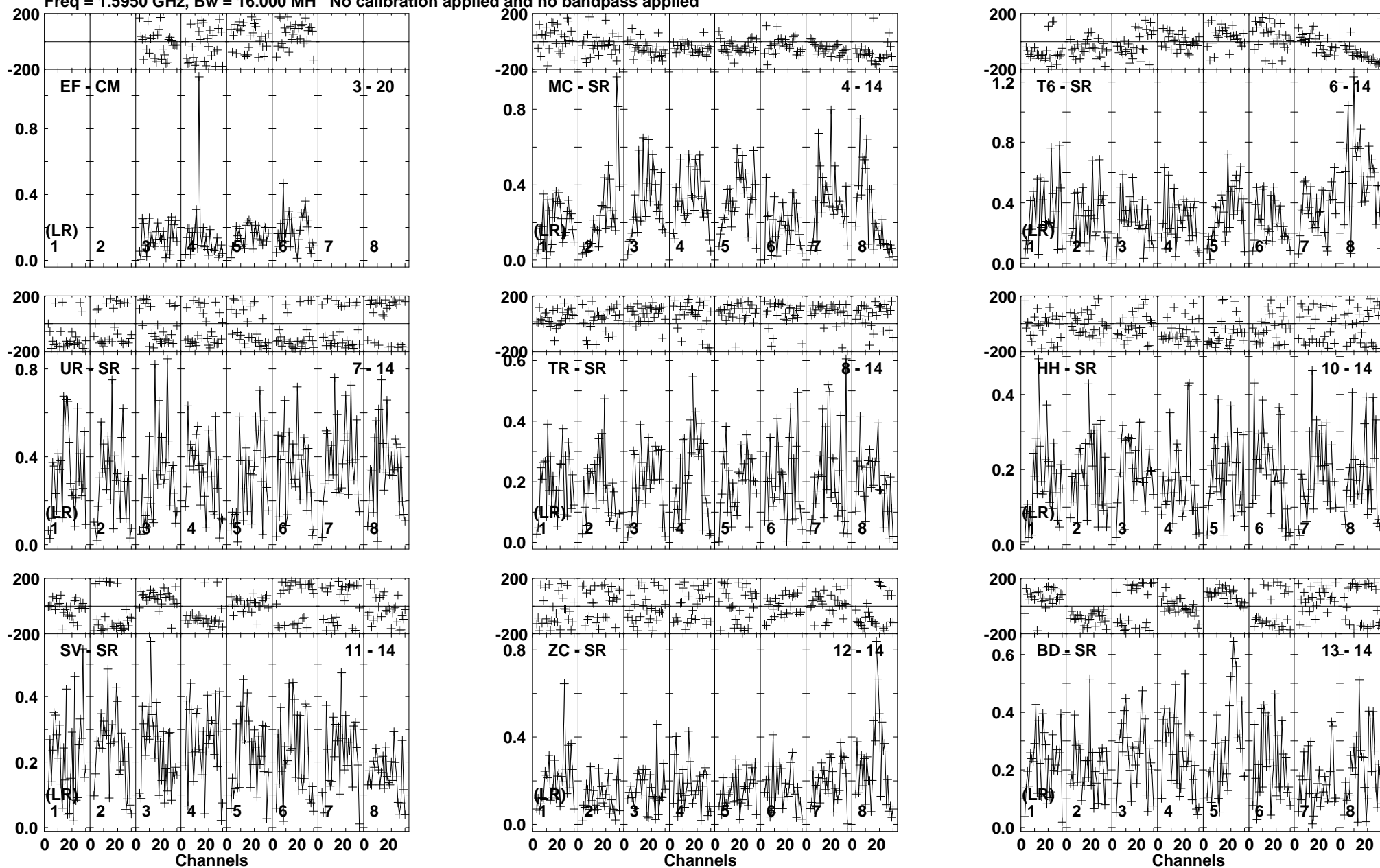
Lower frame: Milli Ampl Jy Top frame: Phas deg Vector averaged cross-power spectrum Baseline: EF (03) - CM (20) Timerange: 00/20:17:41 to 00/20:19:08
