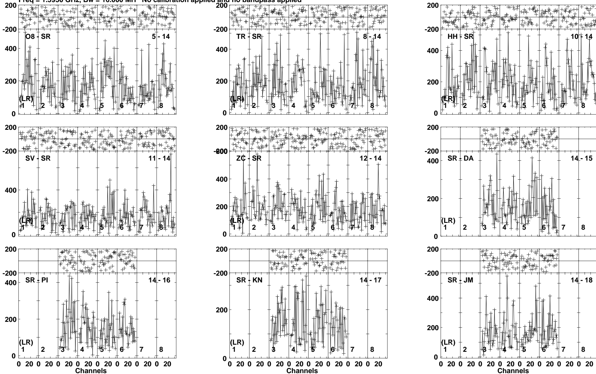
Lower frame: Micro Ampl Jy Top frame: Phas deg Vector averaged cross-power spectrum Baseline: O8 (05) - SR (14) Timerange: 00/23:22:12 to 00/23:23:57
