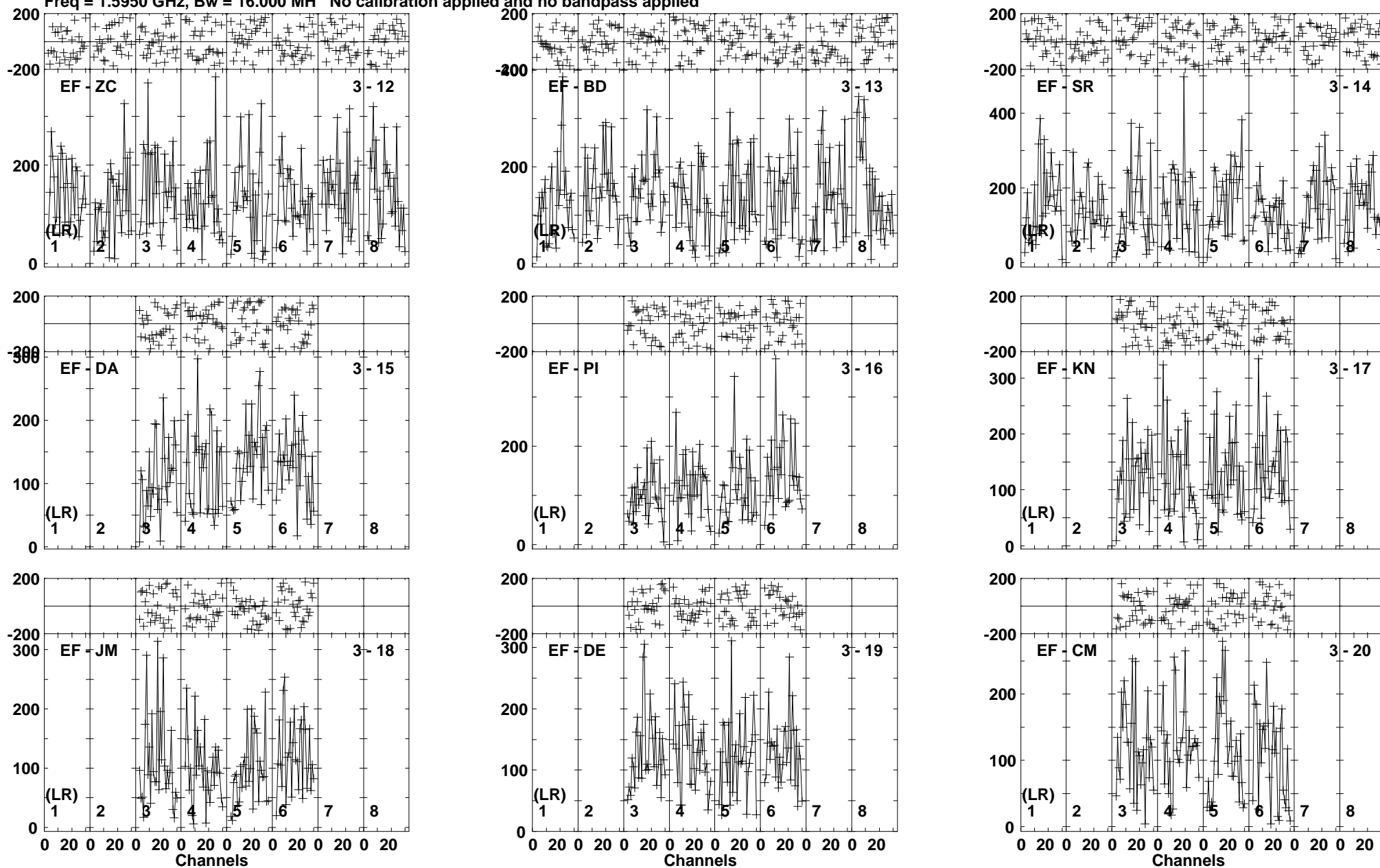
Lower frame: Micro Ampl Jy Top frame: Phas deg Vector averaged cross-power spectrum Baseline: EF (03) - ZC (12) Timerange: 00/20:29:32 to 00/20:37:29
