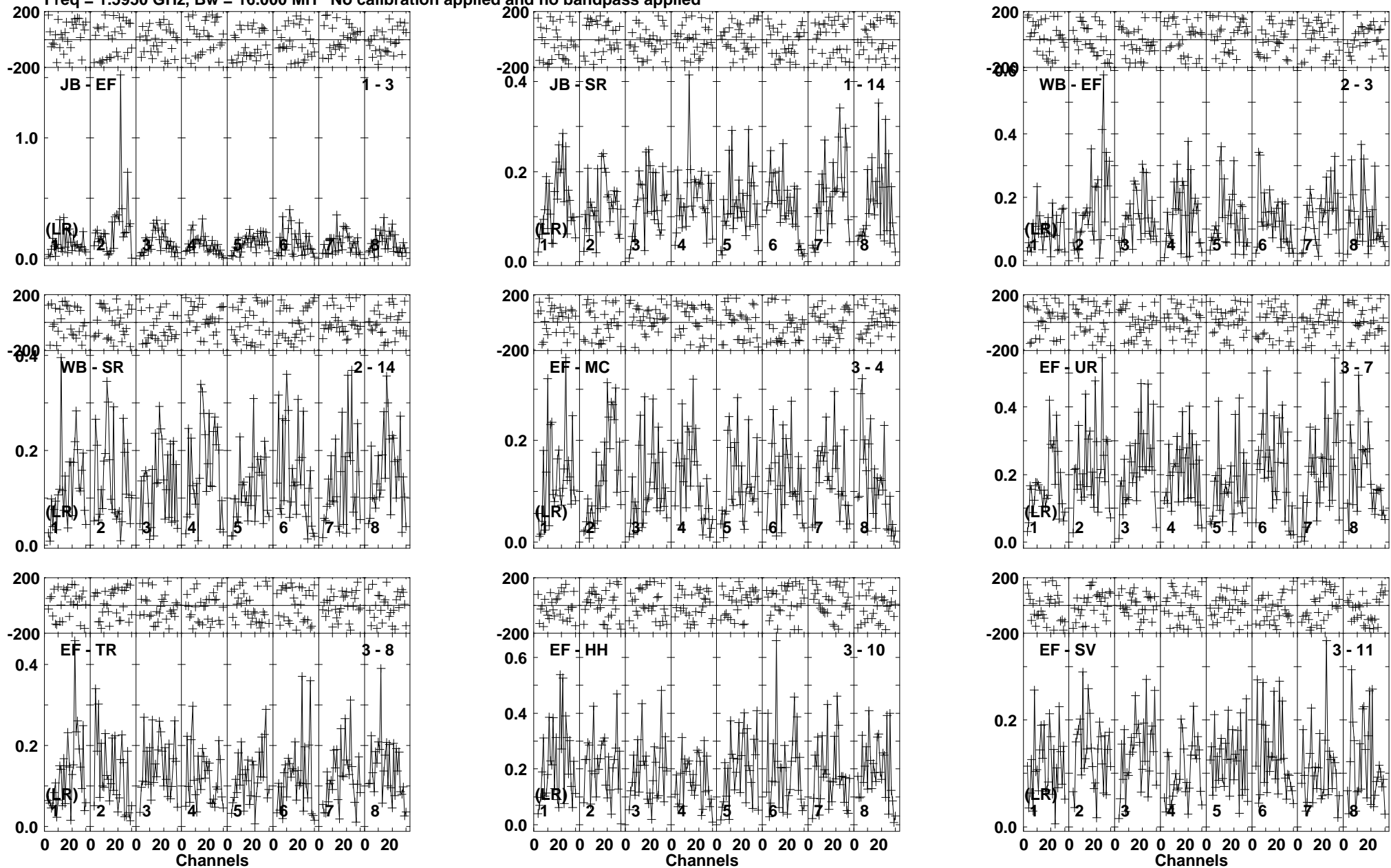
Lower frame: Milli Ampl Jy Top frame: Phas deg Vector averaged cross-power spectrum Baseline: JB (01) - EF (03) Timerange: 00/20:29:32 to 00/20:37:29
