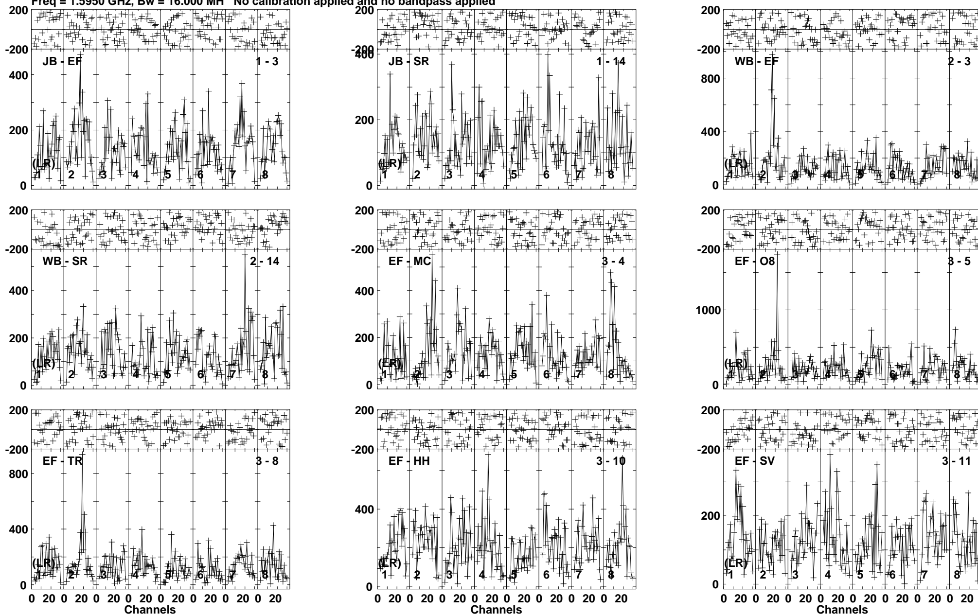
Lower frame: Micro Ampl Jy Top frame: Phas deg Vector averaged cross-power spectrum Baseline: JB (01) - EF (03) Timerange: 01/01:00:02 to 01/01:07:58
