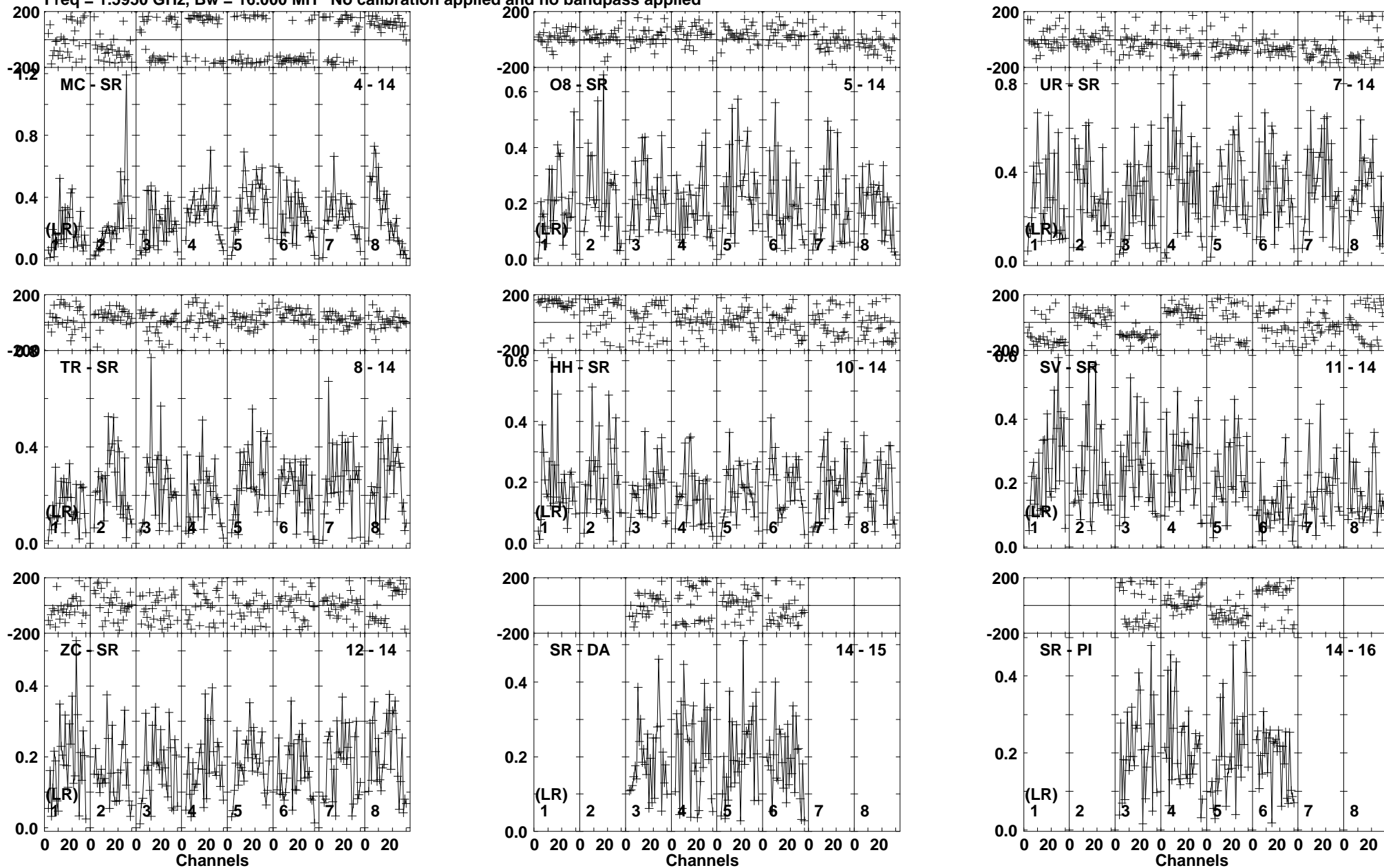
Lower frame: Milli Ampl Jy Top frame: Phas deg Vector averaged cross-power spectrum Baseline: MC (04) - SR (14) Timerange: 00/22:19:41 to 00/22:21:09
