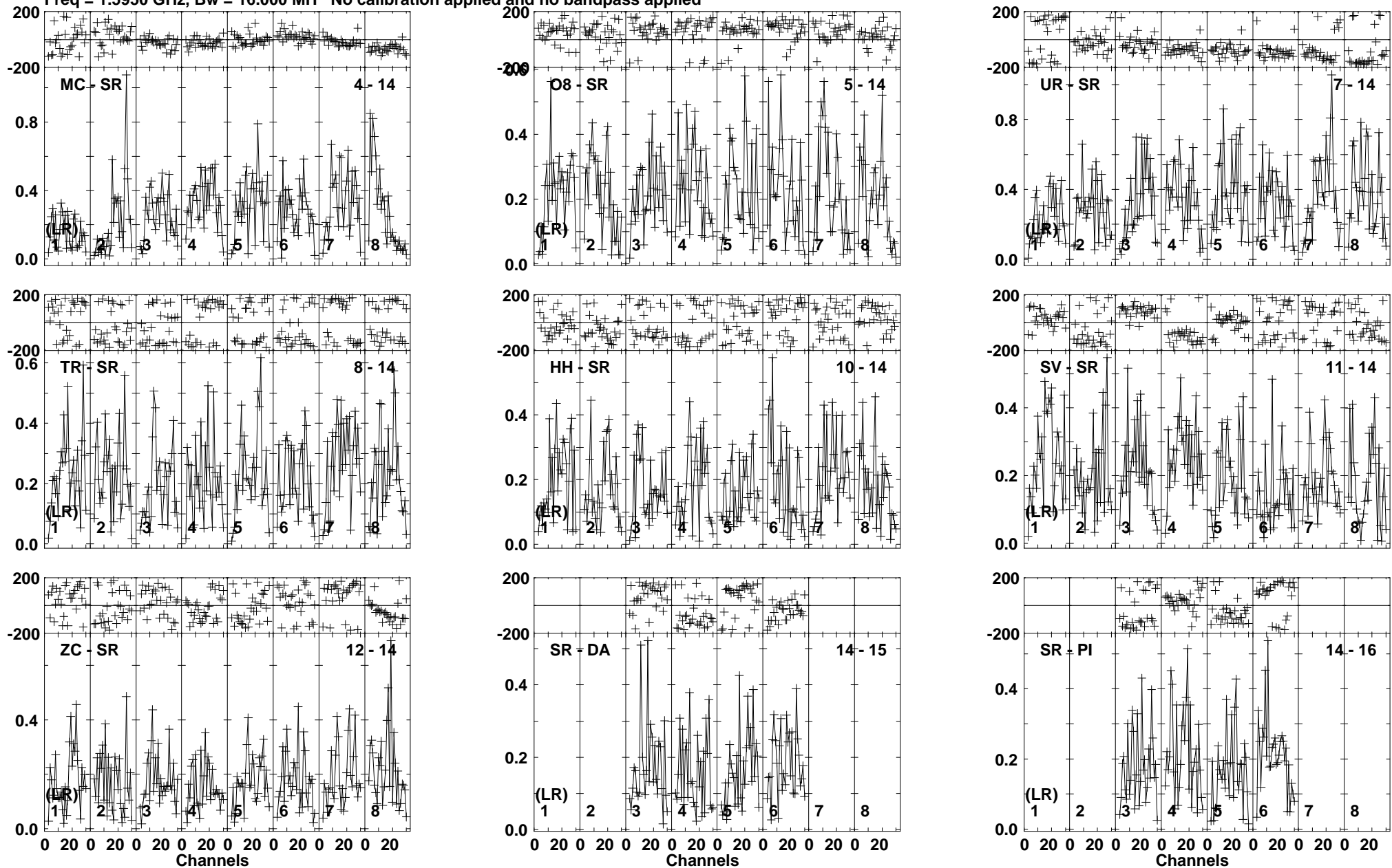
Lower frame: Milli Ampl Jy Top frame: Phas deg Vector averaged cross-power spectrum Baseline: MC (04) - SR (14) Timerange: 00/21:49:11 to 00/21:50:39
