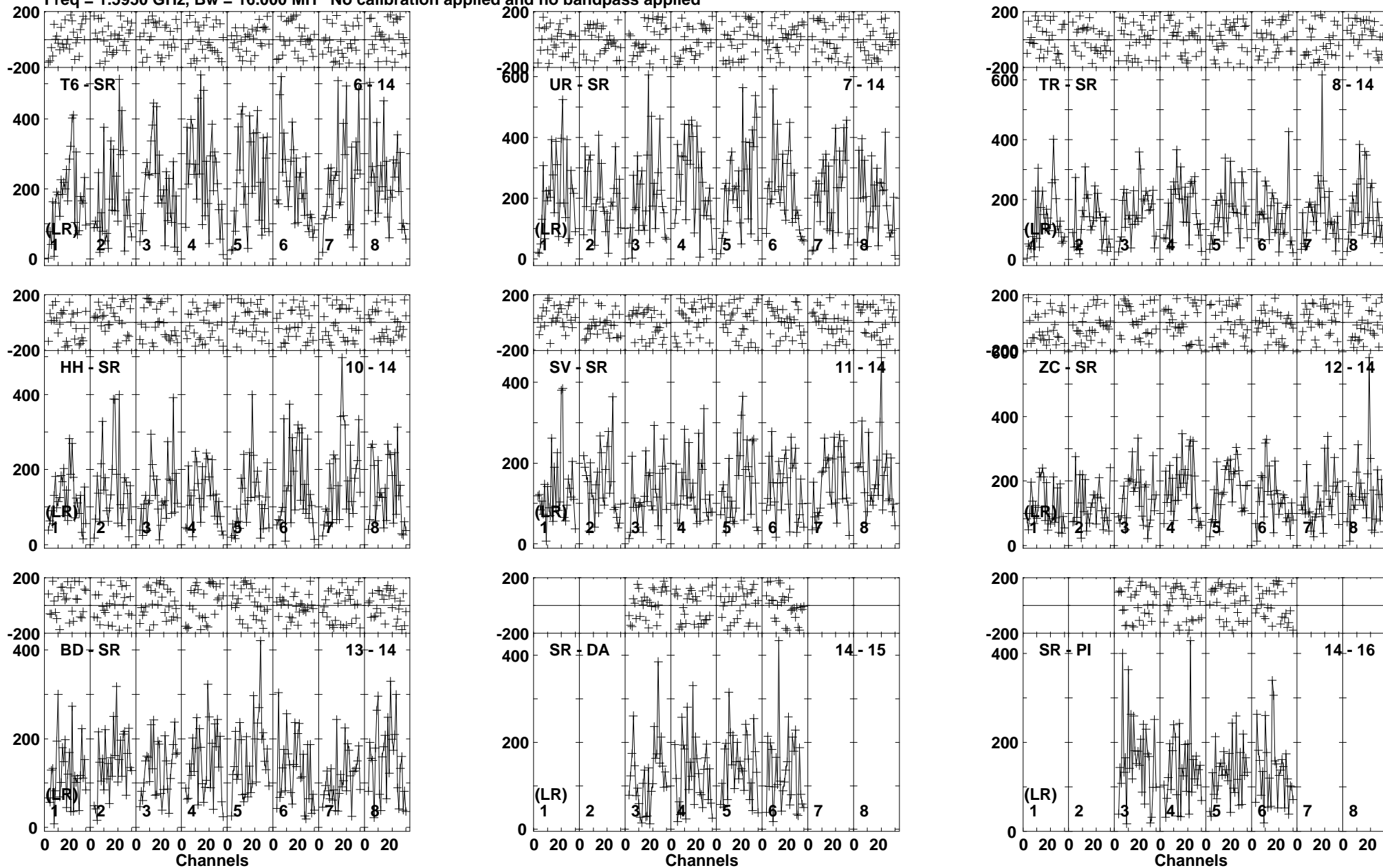
Lower frame: Micro Ampl Jy Top frame: Phas deg Vector averaged cross-power spectrum Baseline: T6 (06) - SR (14) Timerange: 00/18:56:02 to 00/18:57:59
