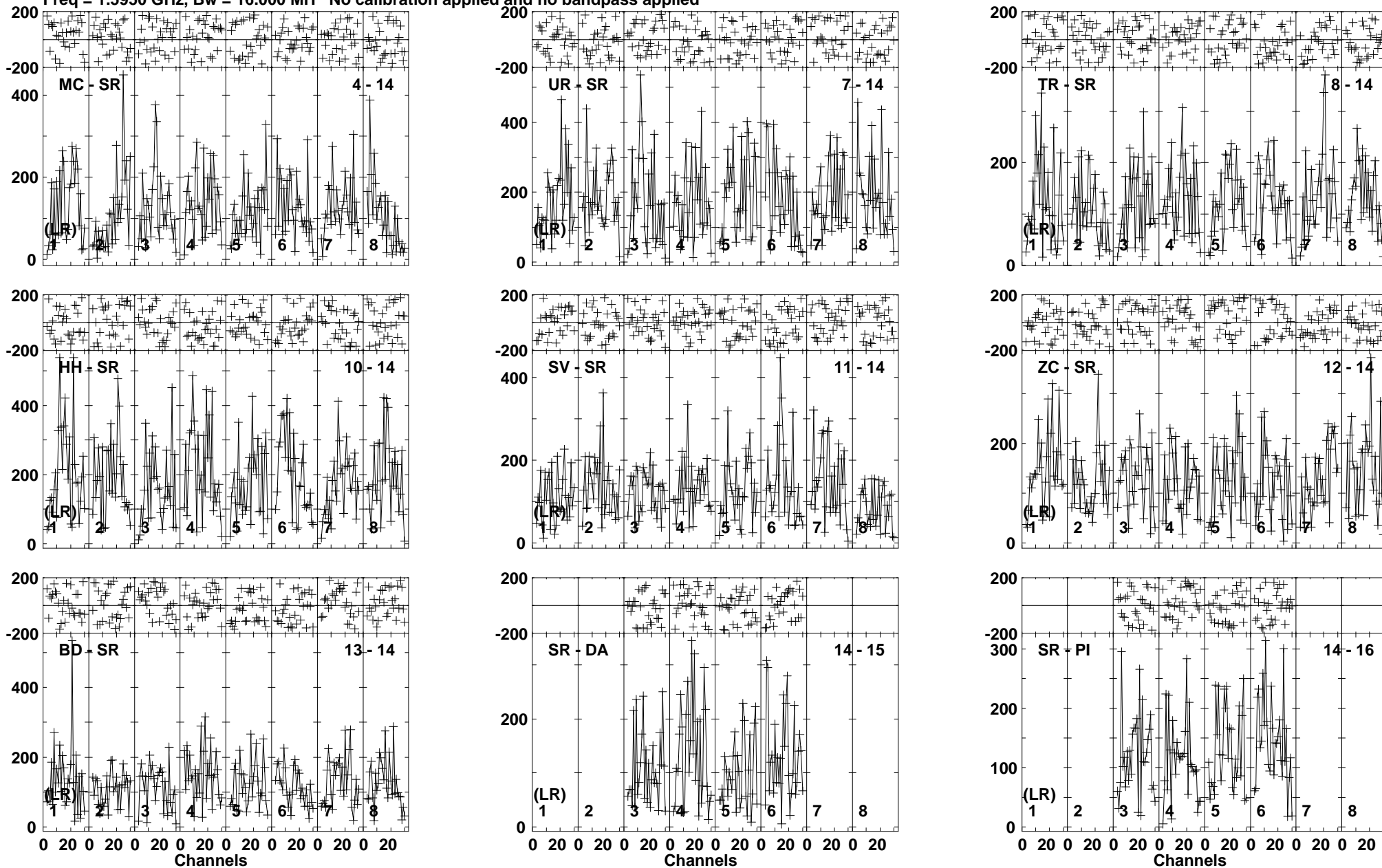
Lower frame: Micro Ampl Jy Top frame: Phas deg Vector averaged cross-power spectrum Baseline: MC (04) - SR (14) Timerange: 00/21:00:01 to 00/21:07:58
