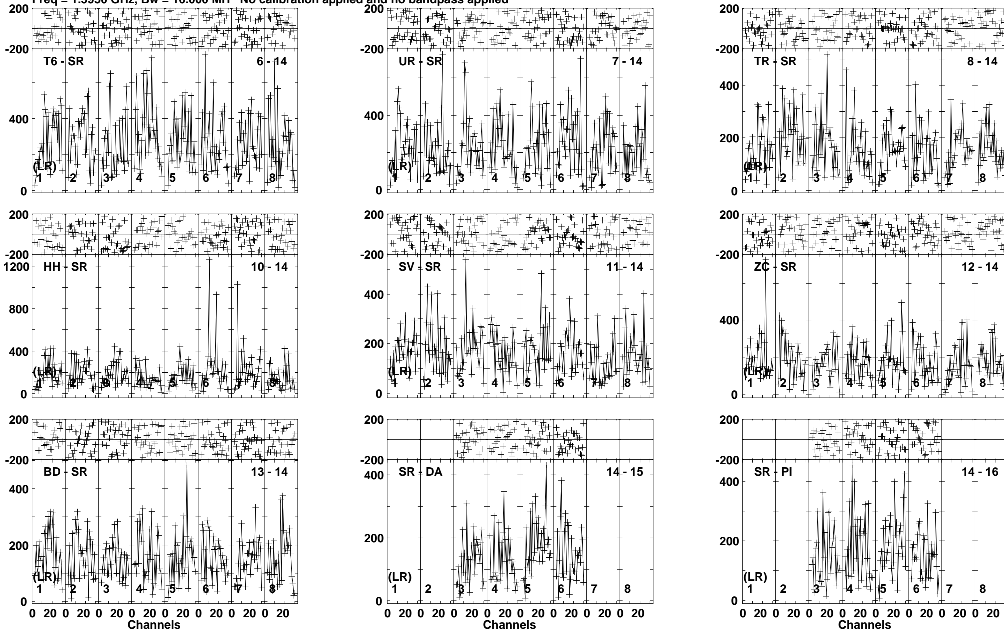
Lower frame: Micro Ampl Jy Top frame: Phas deg Vector averaged cross-power spectrum Baseline: T6 (06) - SR (14) Timerange: 00/17:24:41 to 00/17:26:09
