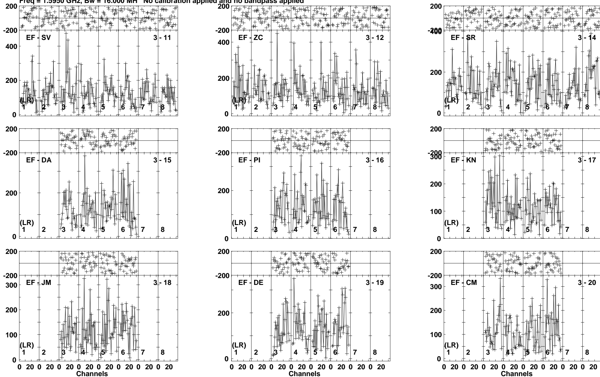
Lower frame: Micro Ampl Jy Top frame: Phas deg Vector averaged cross-power spectrum Baseline: EF (03) - SV (11) Timerange: 00/22:31:32 to 00/22:39:29
