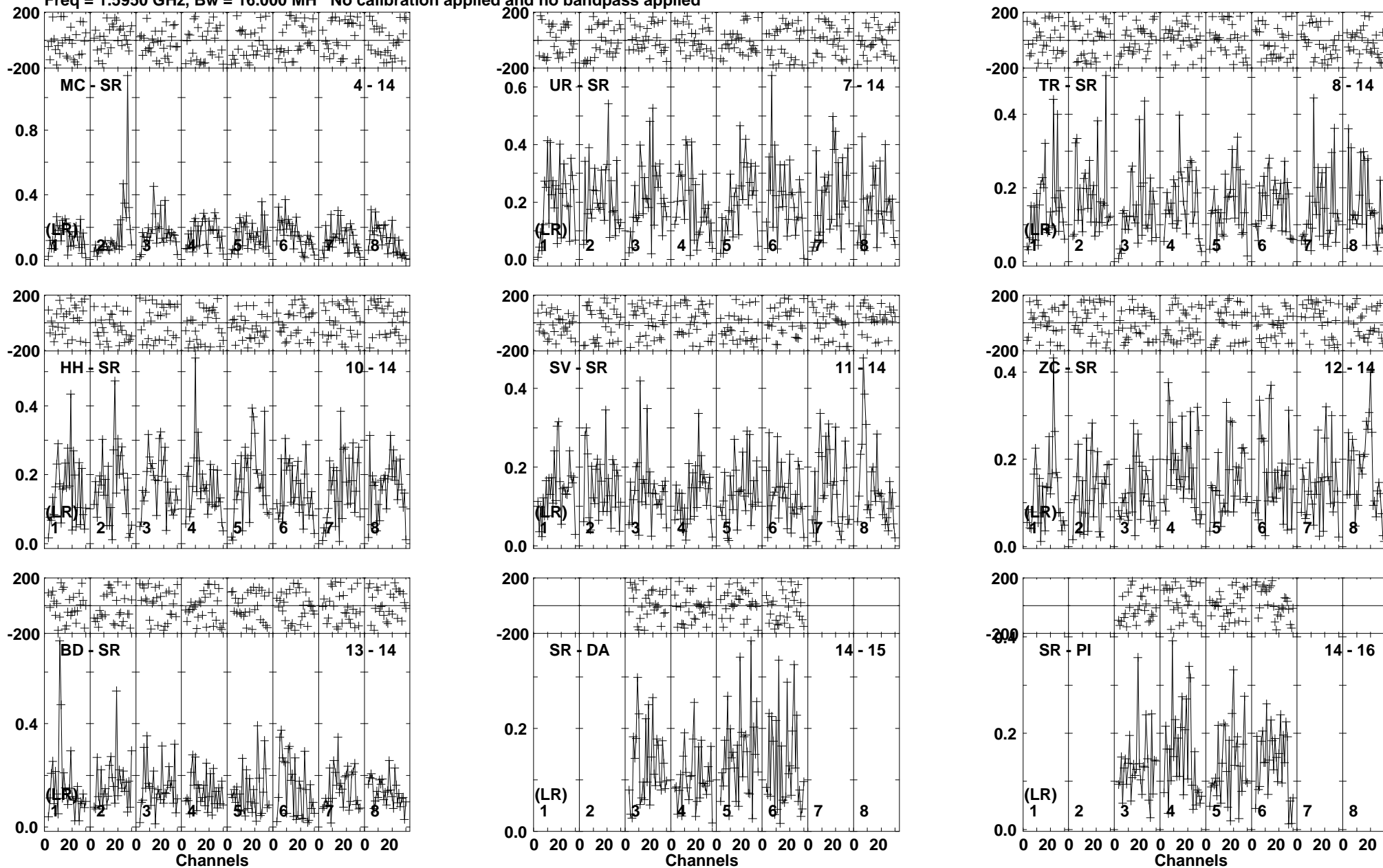
Lower frame: Milli Ampl Jy Top frame: Phas deg Vector averaged cross-power spectrum Baseline: MC (04) - SR (14) Timerange: 00/20:37:31 to 00/20:39:29
