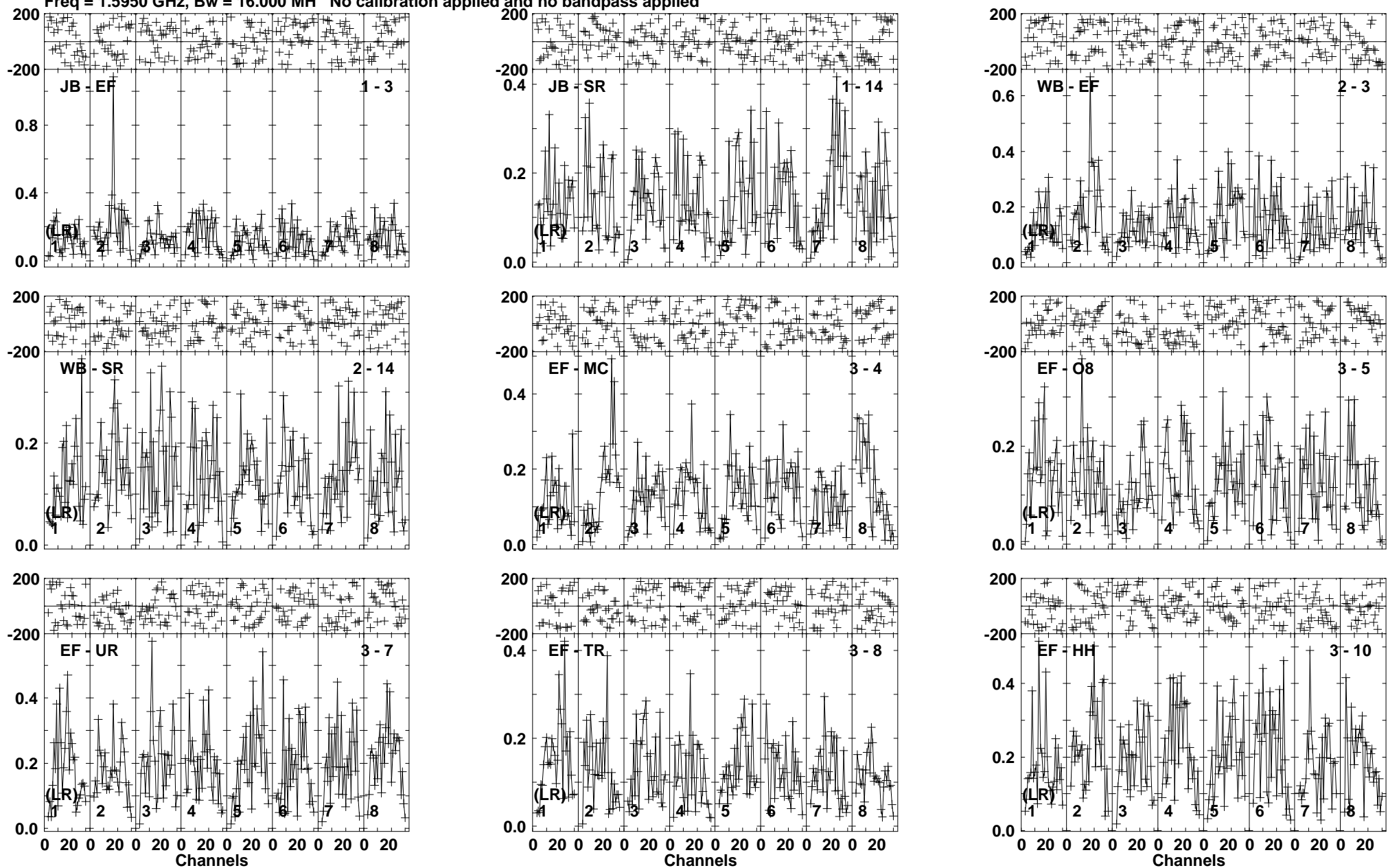
Lower frame: Milli Ampl Jy Top frame: Phas deg Vector averaged cross-power spectrum Baseline: JB (01) - EF (03) Timerange: 00:22:31:32 to 00:22:39:29
