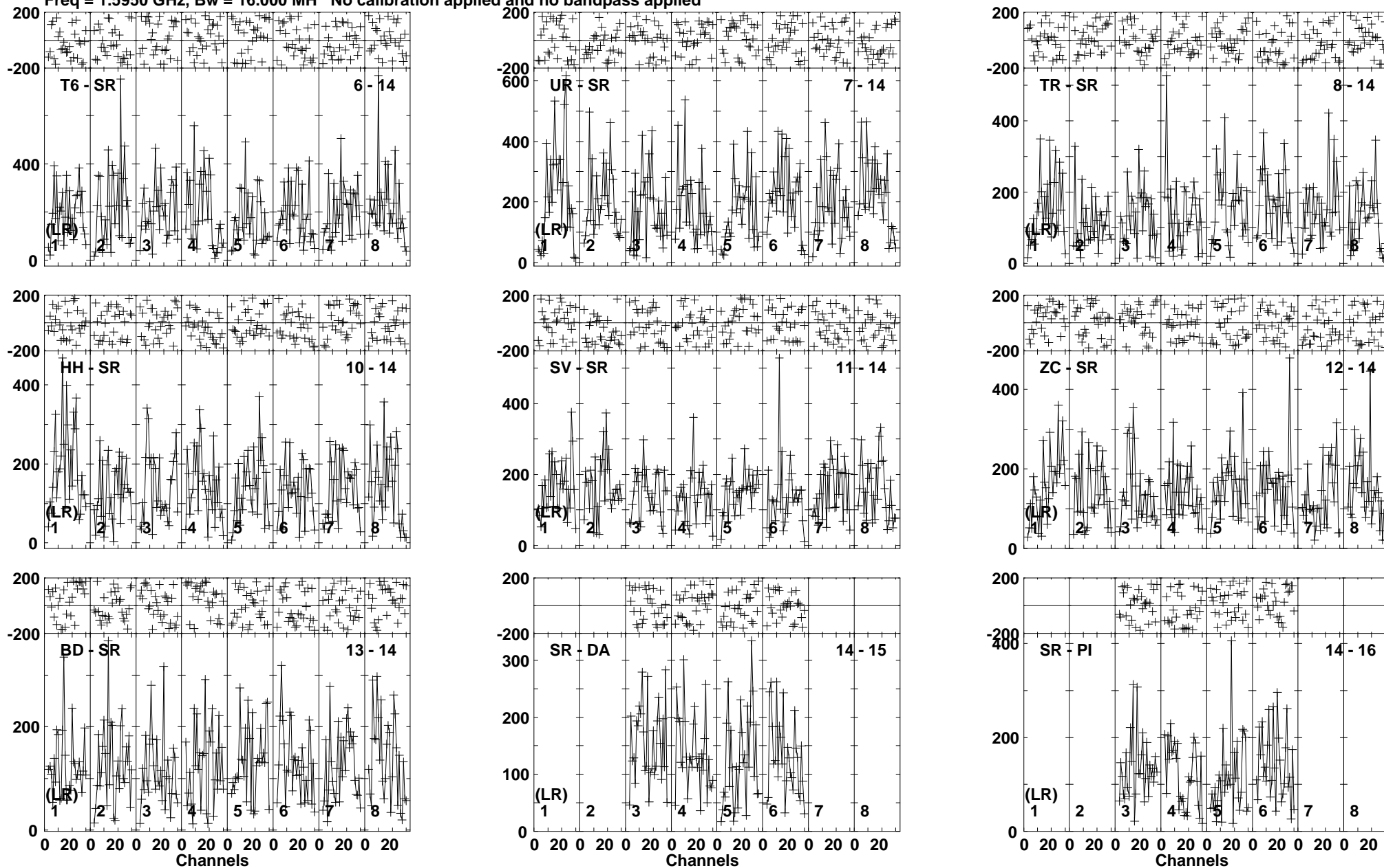
Lower frame: Micro Ampl Jy Top frame: Phas deg Vector averaged cross-power spectrum Baseline: T6 (06) - SR (14) Timerange: 00:19:57:01 to 00:19:58:59
