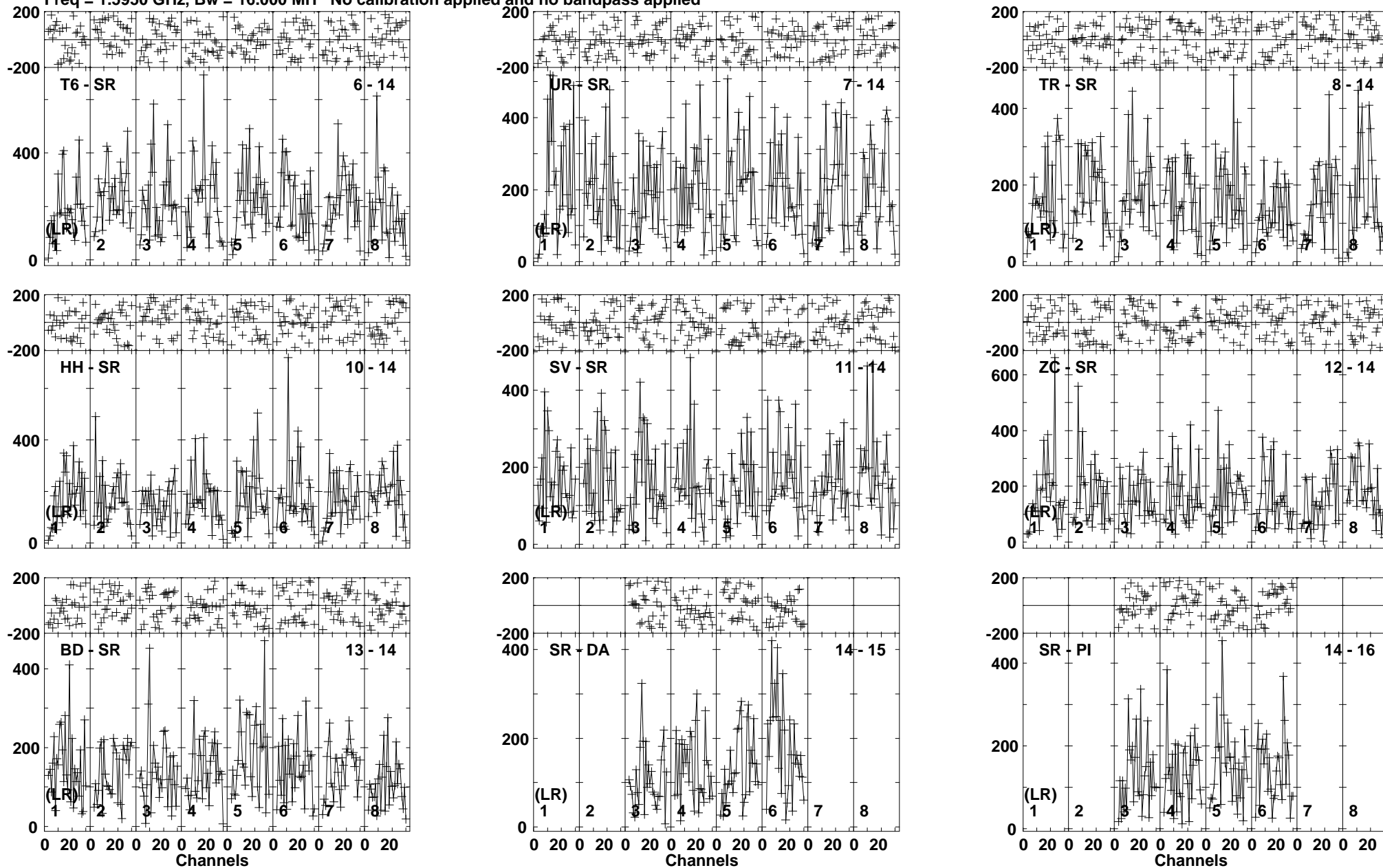
Lower frame: Micro Ampl Jy Top frame: Phas deg Vector averaged cross-power spectrum Baseline: T6 (06) - SR (14) Timerange: 00/17:44:12 to 00/17:46:09
