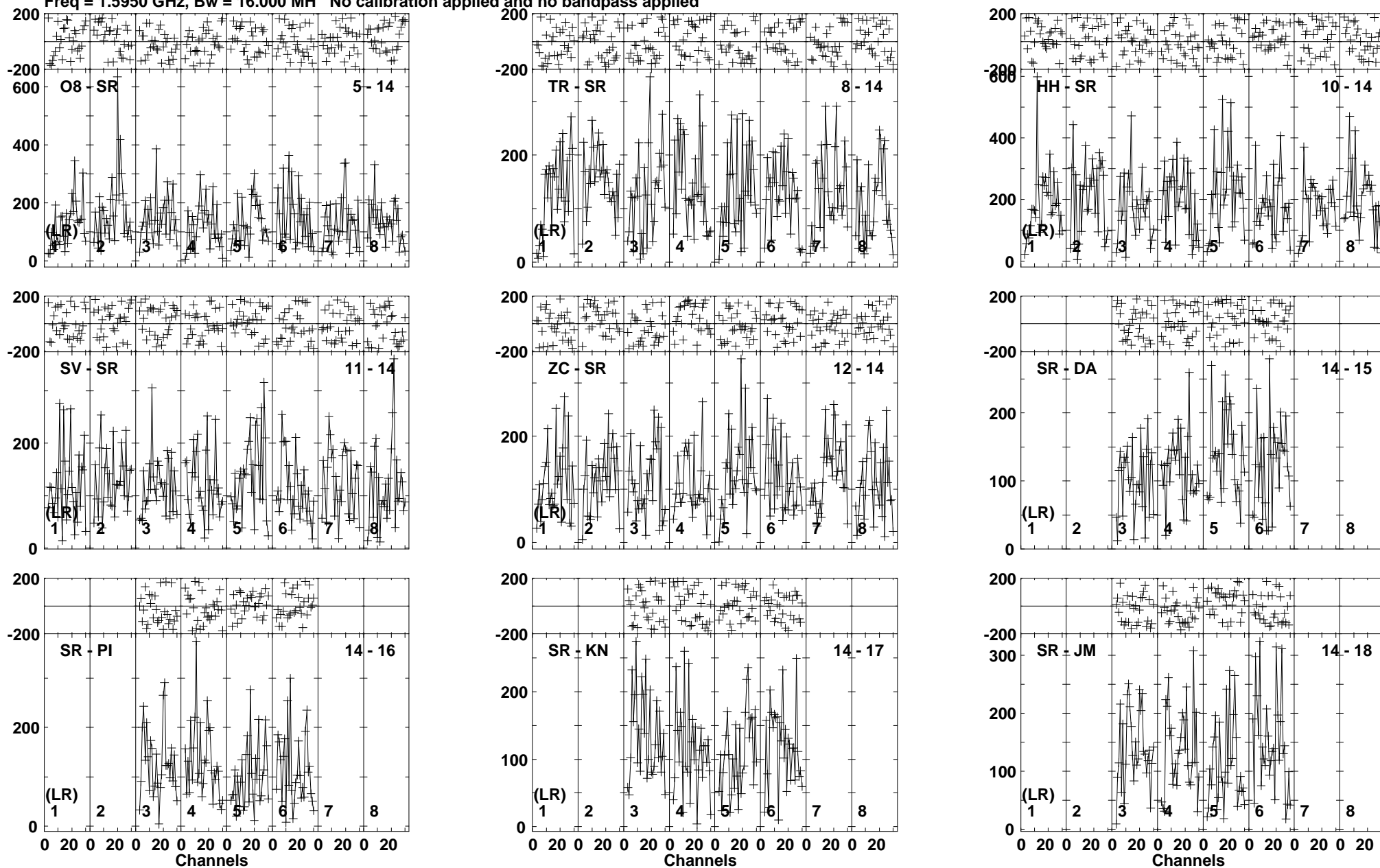
Lower frame: Micro Ampl Jy Top frame: Phas deg Vector average cross-power spectrum Baseline: O8 (05) - SR (14) Timerange: 01/00:03:02 to 01/00:10:58
