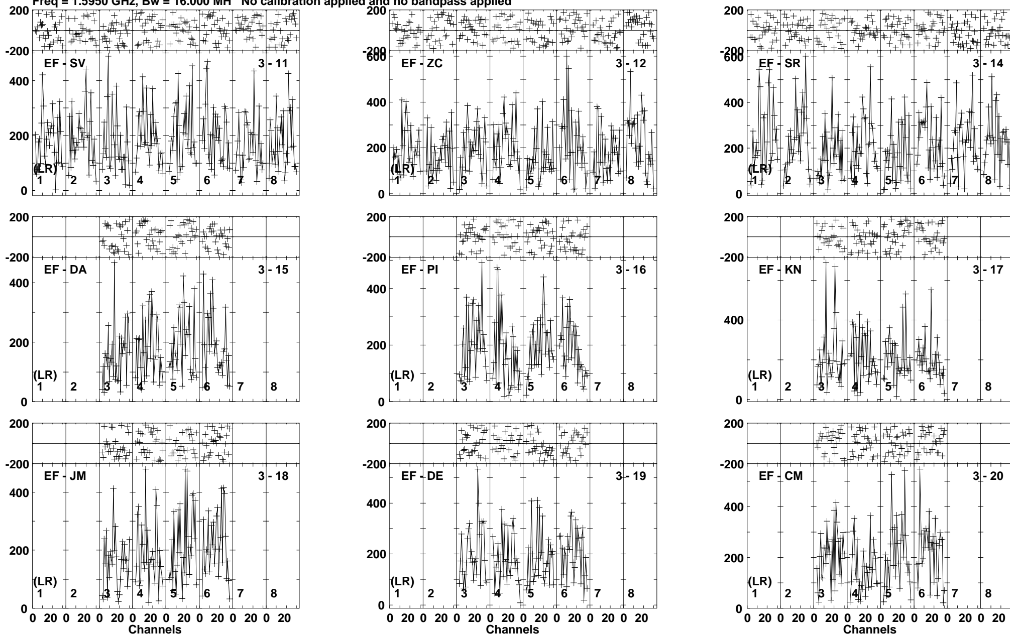
Lower frame: Micro Ampl Jy Top frame: Phas deg Vector averaged cross-power spectrum Baseline: EF (03) - SV (11) Timerange: 00/21:50:42 to 00/21:52:26
