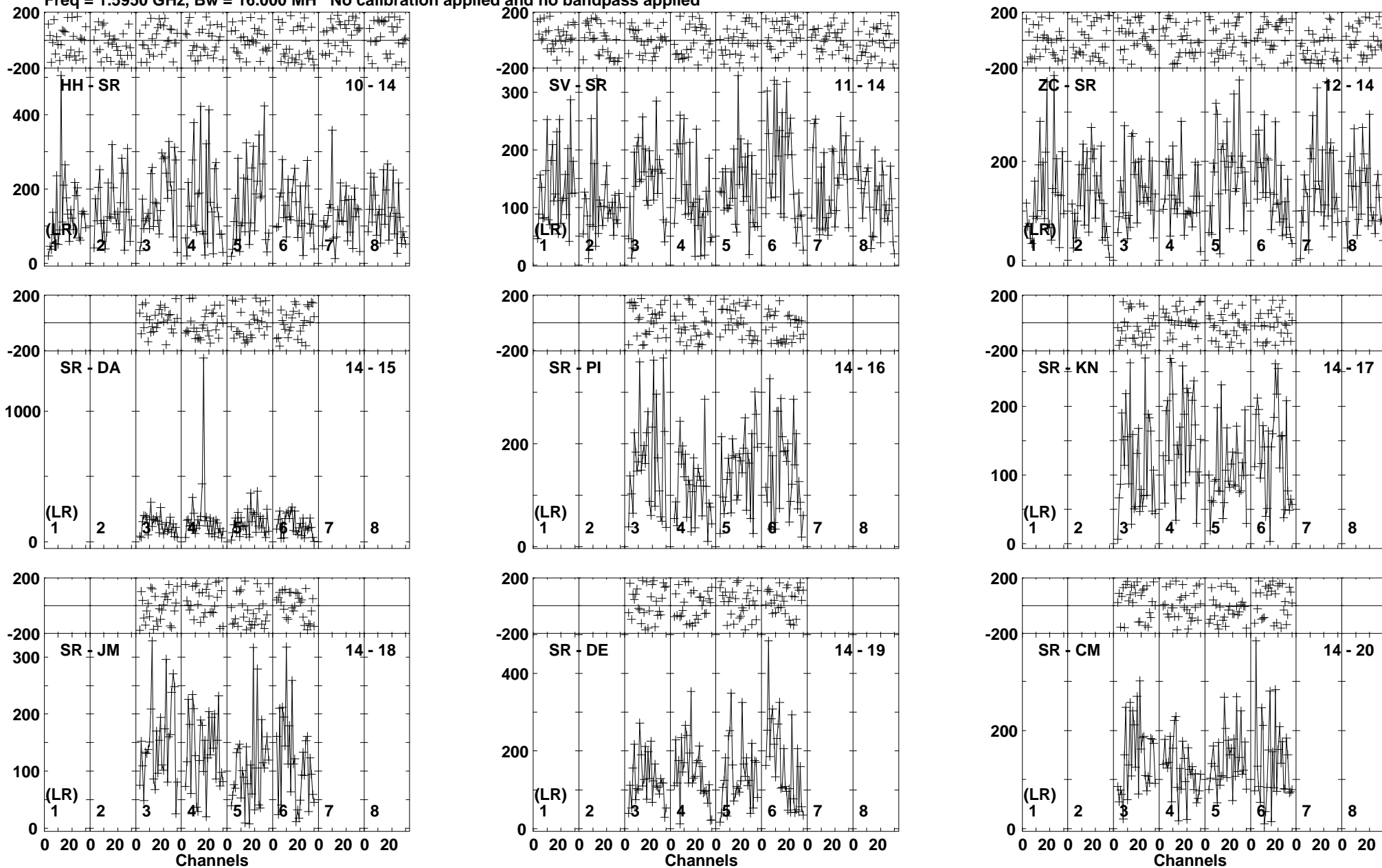
Lower frame: Micro Ampl Jy Top frame: Phas deg Vector averaged cross-power spectrum Baseline: HH (10) - SR (14) Timerange: 00/21:28:31 to 00/21:30:29
