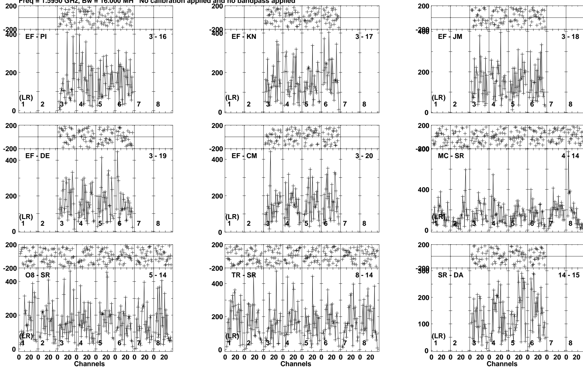
Lower frame: Micro Ampl Jy Top frame: Phas deg Vector averaged cross-power spectrum Baseline: EF (03) - PI (16) Timerange: 01/02:38:01 to 01/02:39:59
