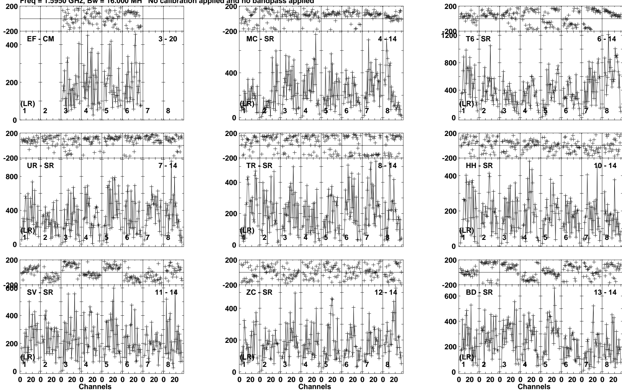
Lower frame: Micro Ampl Jy Top frame: Phas deg Vector averaged cross-power spectrum Baseline: EF (03) - CM (20) Timerange: 00/19:47:11 to 00/19:48:38
