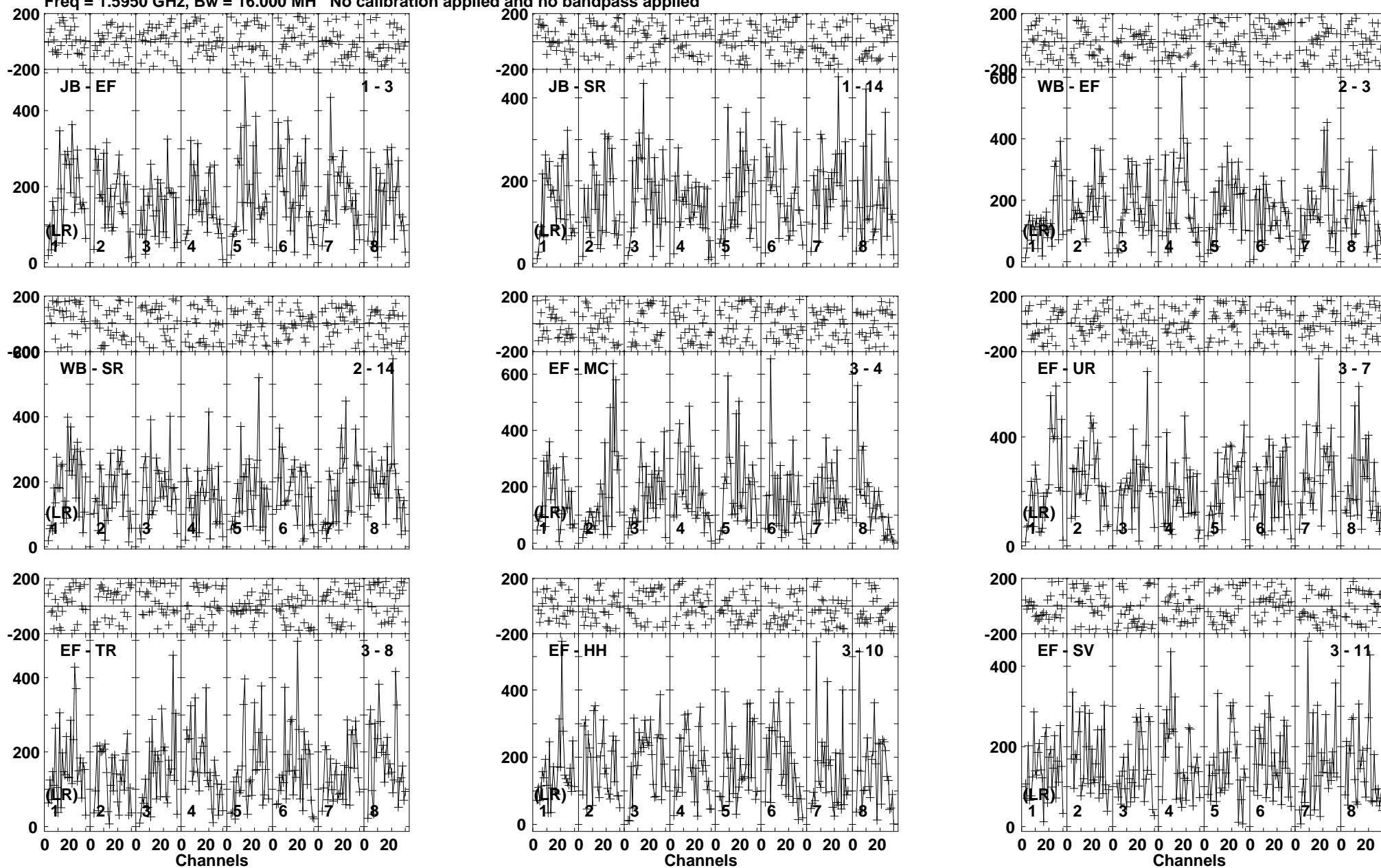
Lower frame: Micro Ampl Jy Top frame: Phas deg Vector averaged cross-power spectrum Baseline: JB (01) - EF (03) Timerange: 00/20:37:31 to 00/20:39:29
