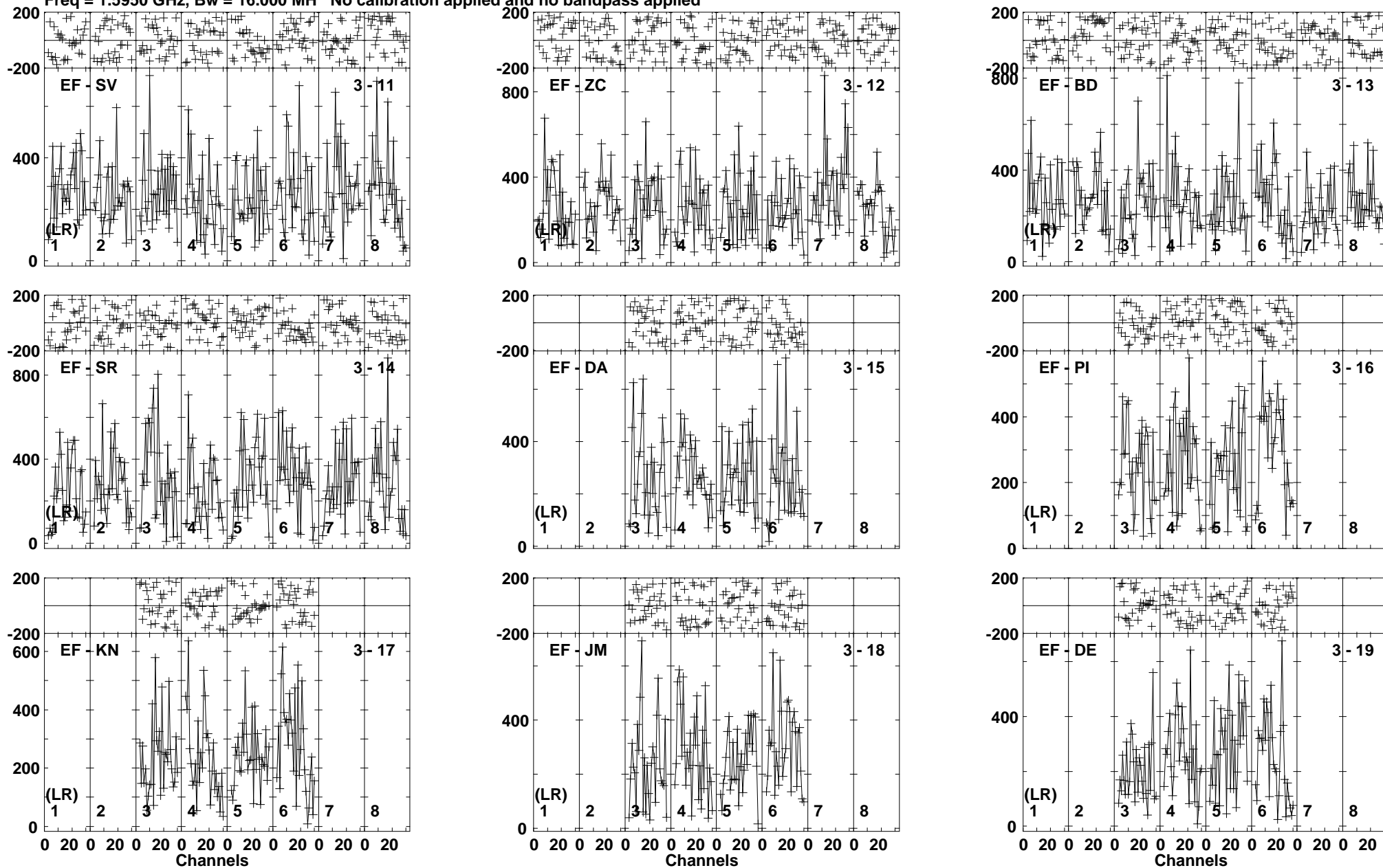
Lower frame: Micro Ampl Jy Top frame: Phas deg Vector averaged cross-power spectrum Baseline: EF (03) - SV (11) Timerange: 00/18:20:31 to 00/18:21:58
