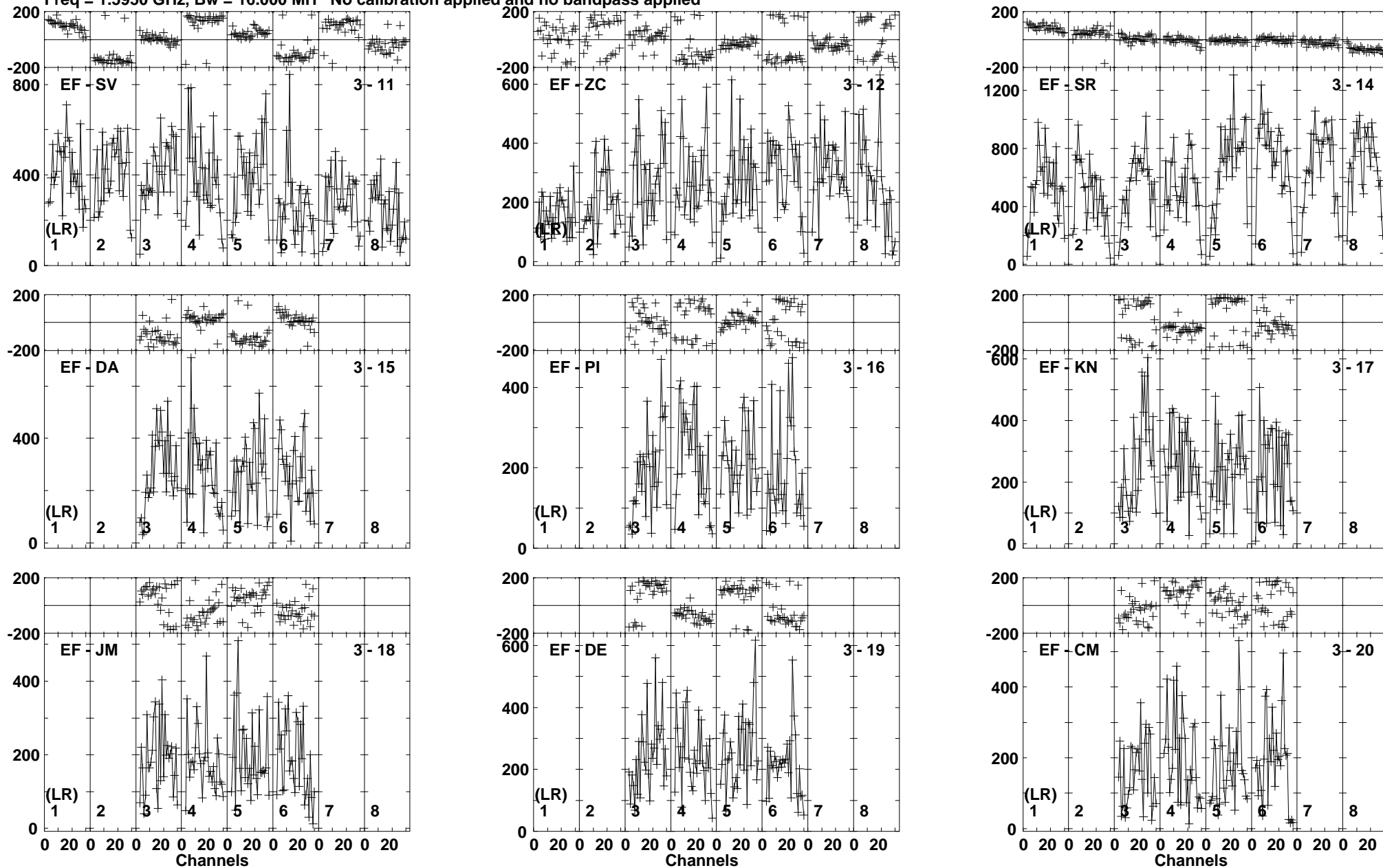
Lower frame: Micro Ampl Jy Top frame: Phas deg Vector averaged cross-power spectrum Baseline: EF (03) - SV (11) Timerange: 00/21:49:11 to 00/21:50:39
