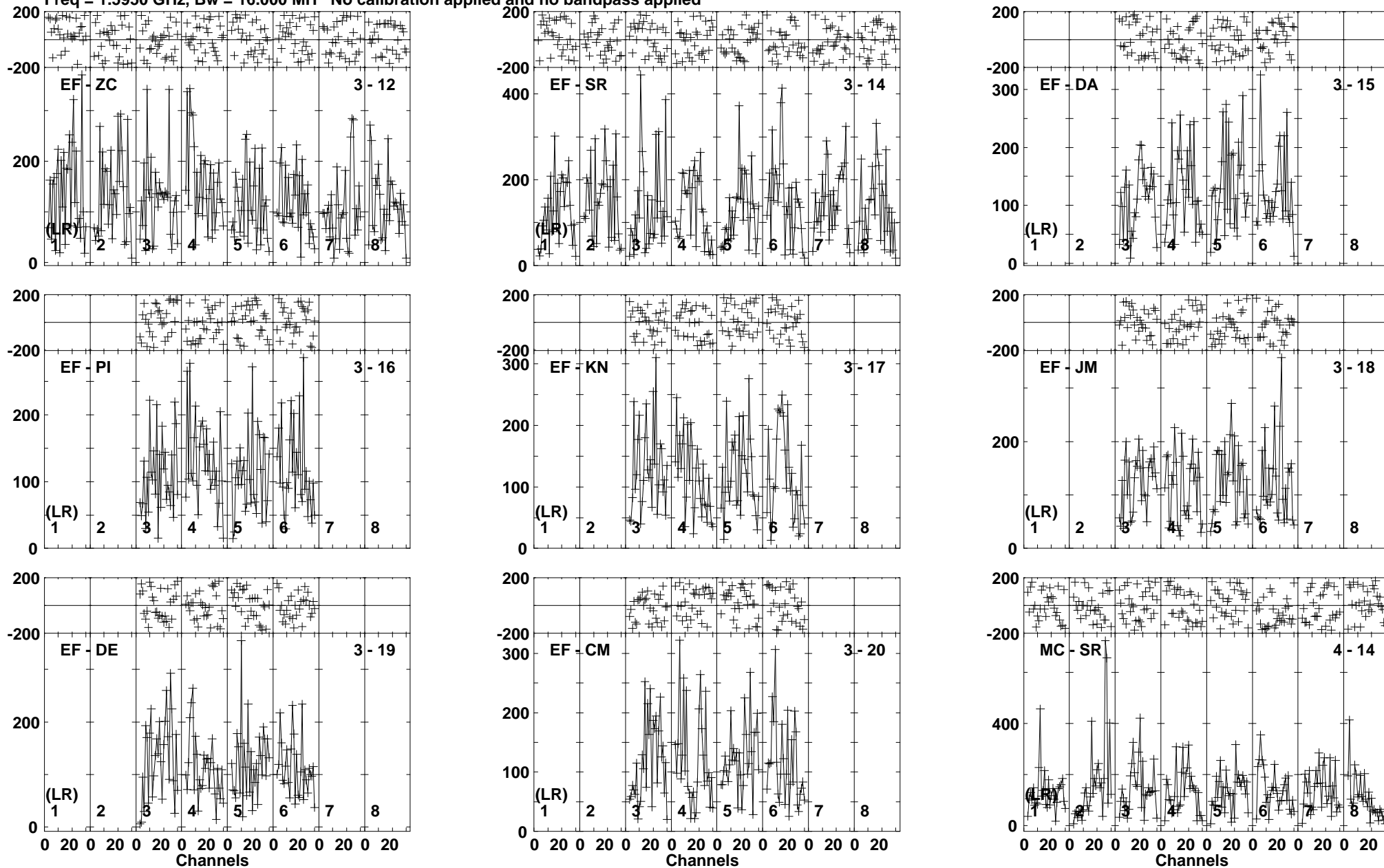
Lower frame: Micro Ampl Jy Top frame: Phas deg Vector averaged cross-power spectrum Baseline: EF (03) - ZC (12) Timerange: 00/23:42:32 to 00/23:50:29
