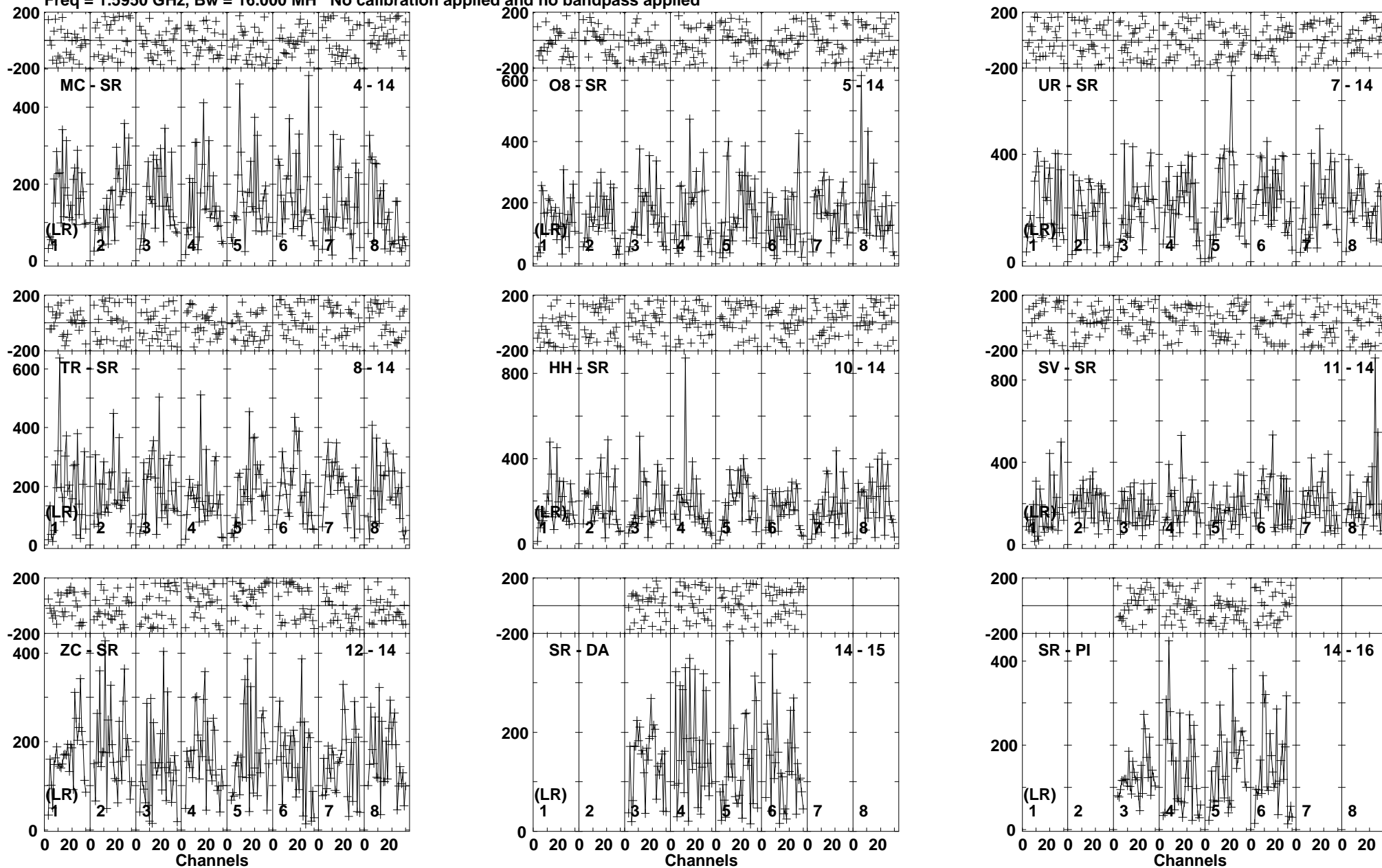
Lower frame: Micro Ampl Jy Top frame: Phas deg Vector averaged cross-power spectrum Baseline: MC (04) - SR (14) Timerange: 00/22:21:12 to 00/22:22:56
