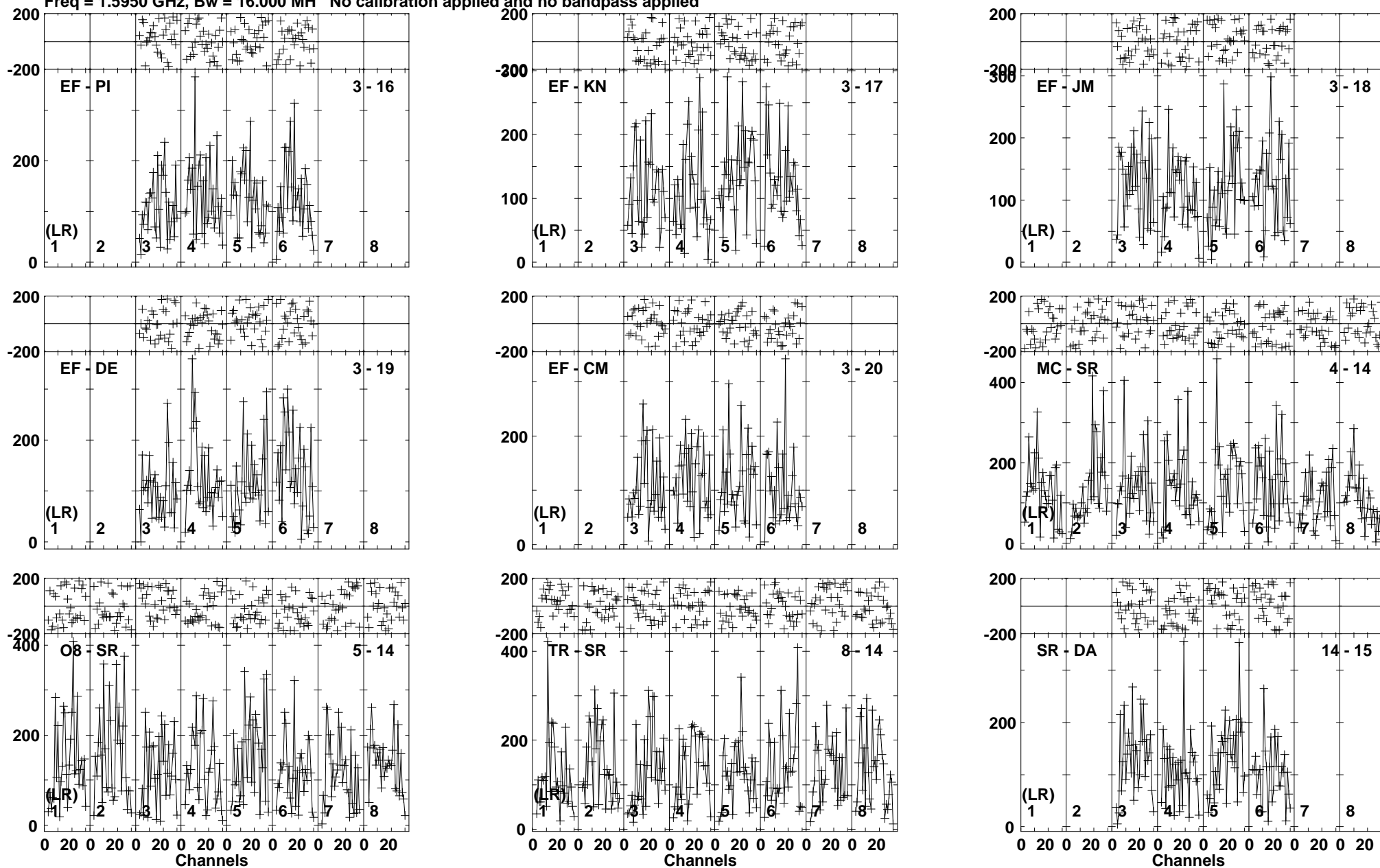
Lower frame: Micro Ampl Jy Top frame: Phas deg Vector averaged cross-power spectrum Baseline: EF (03) - PI (16) Timerange: 01/03:10:02 to 01/03:17:59
