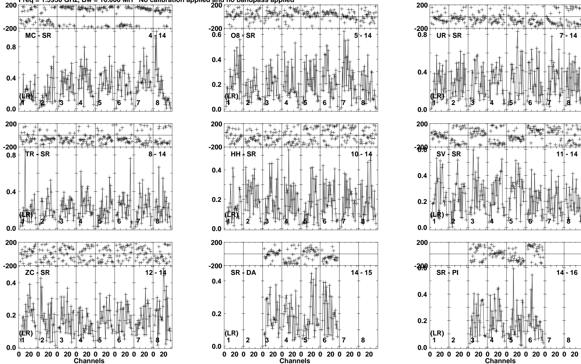
Lower frame: Milli Ampl Jy Top frame: Phas deg Vector averaged cross-power spectrum Baseline: MC (04) - SR (14) Timerange: 00:22:50:12 to 00:22:51:39
