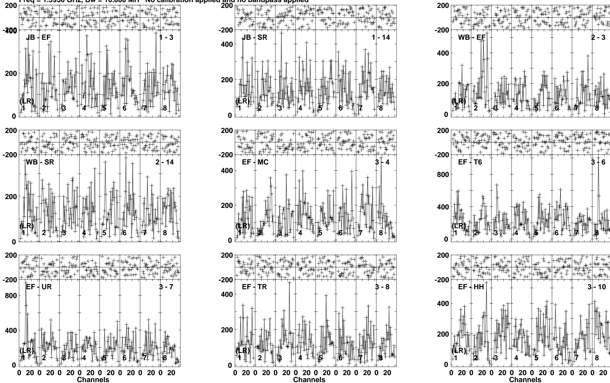
Lower frame: Micro Ampl Jy Top frame: Phas deg Vector averaged cross-power spectrum Baseline: JB (01) - EF (03) Timerange: 00/17:56:11 to 00/18:04:08
