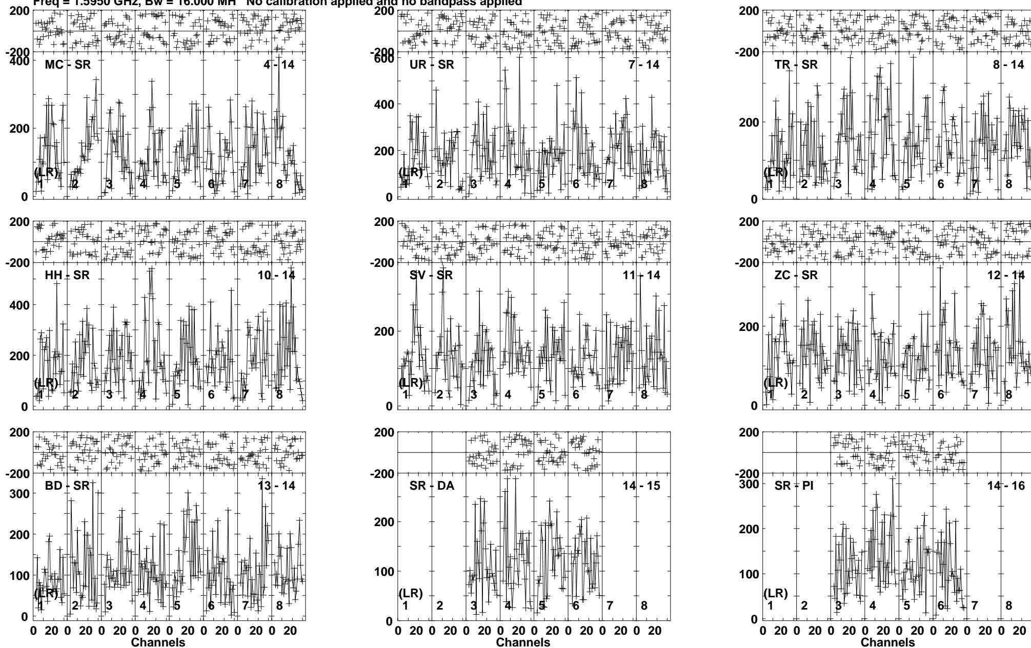
Lower frame: Micro Ampl Jy Top frame: Phas deg Vector averaged cross-power spectrum Baseline: MC (04) - SR (14) Timerange: 00/20:39:32 to 00/20:47:29
