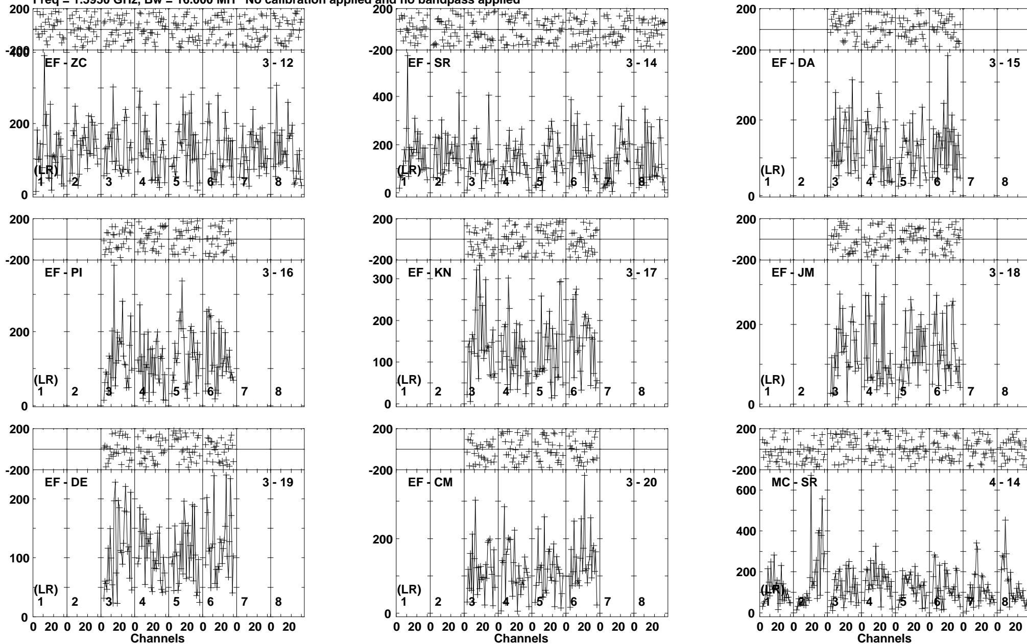
Lower frame: Micro Ampl Jy Top frame: Phas deg Vector averaged cross-power spectrum Baseline: EF (03) - ZC (12) Timerange: 00/23:32:32 to 00/23:40:29
