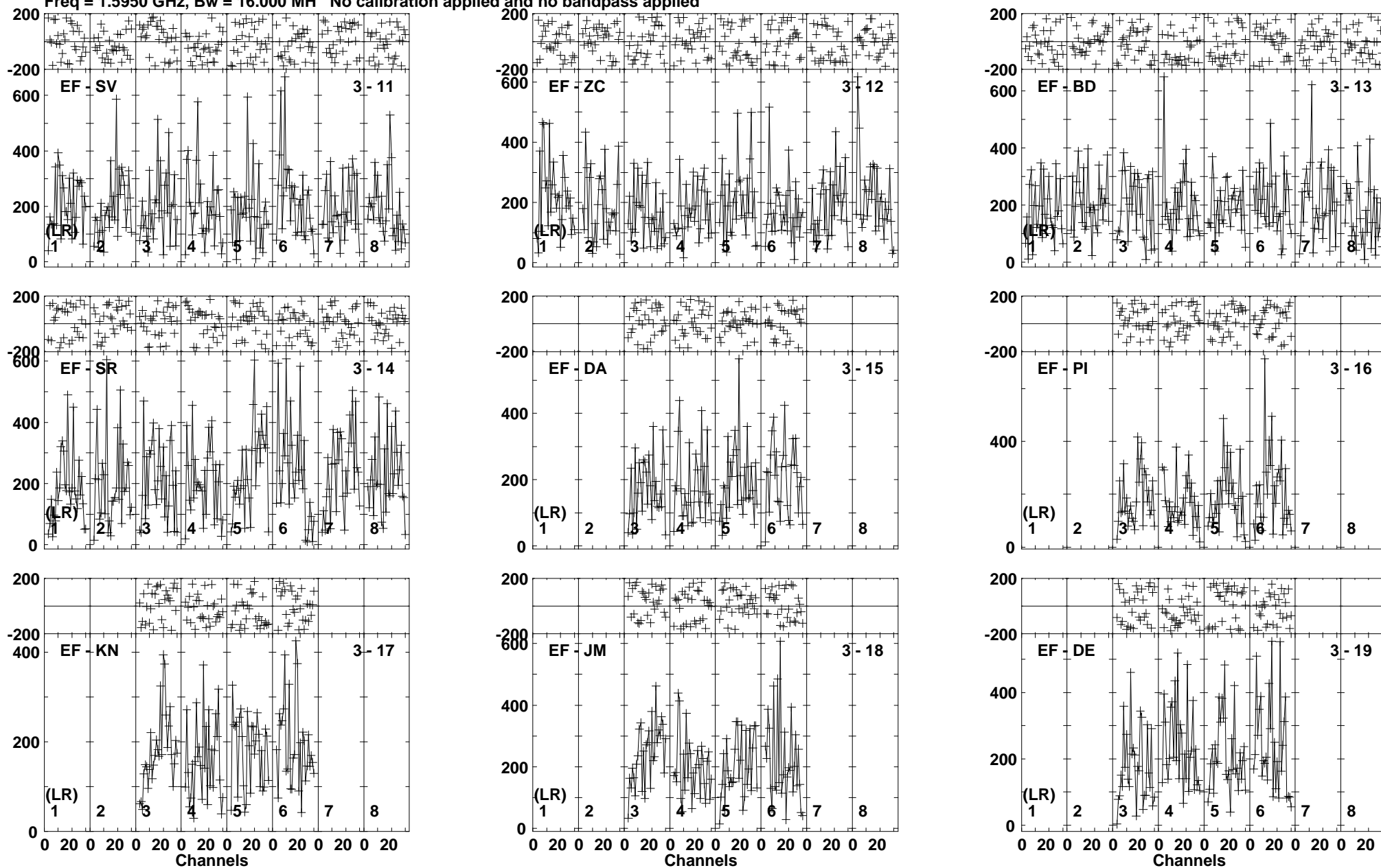
Lower frame: Micro Ampl Jy Top frame: Phas deg Vector averaged cross-power spectrum Baseline: EF (03) - SV (11) Timerange: 00/19:18:12 to 00/19:19:57
