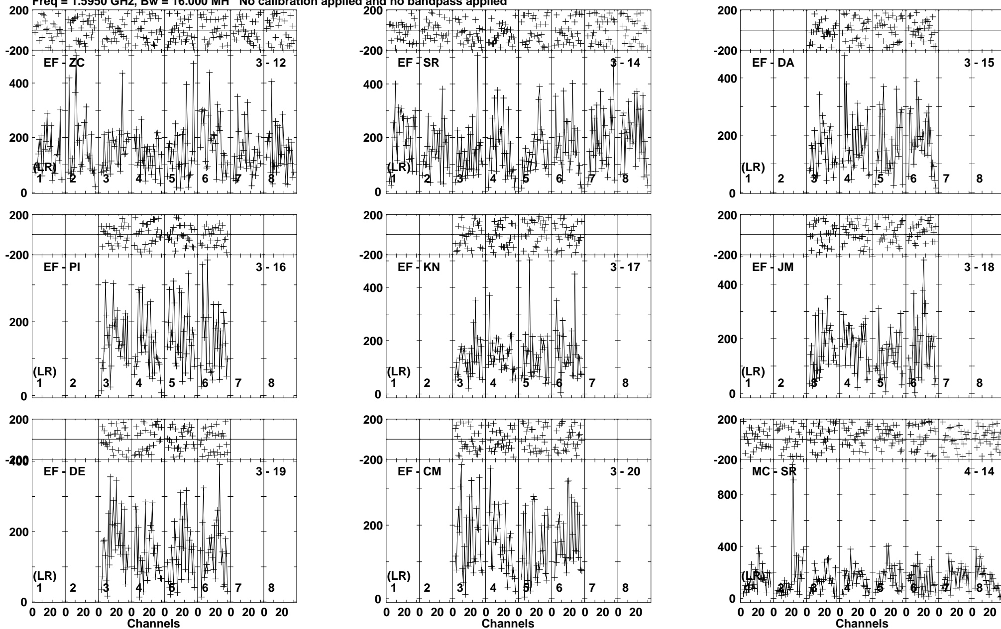
Lower frame: Micro Ampl Jy Top frame: Phas deg Vector averaged cross-power spectrum Baseline: EF (03) - ZC (12) Timerange: 01/00:11:01 to 01/00:12:59
