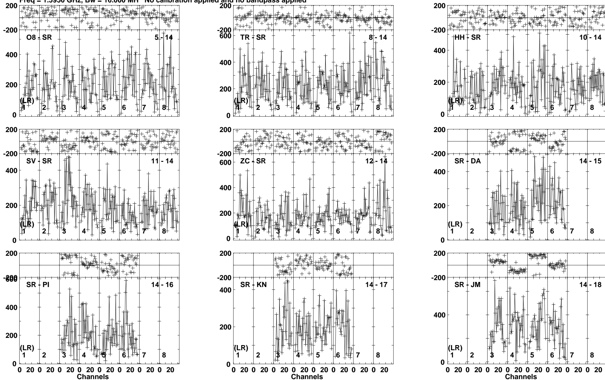
Lower frame: Micro Ampl Jy Top frame: Phas deg Vector averaged cross-power spectrum Baseline: O8 (05) - SR (14) Timerange: 00/23:20:42 to 00/23:22:08
