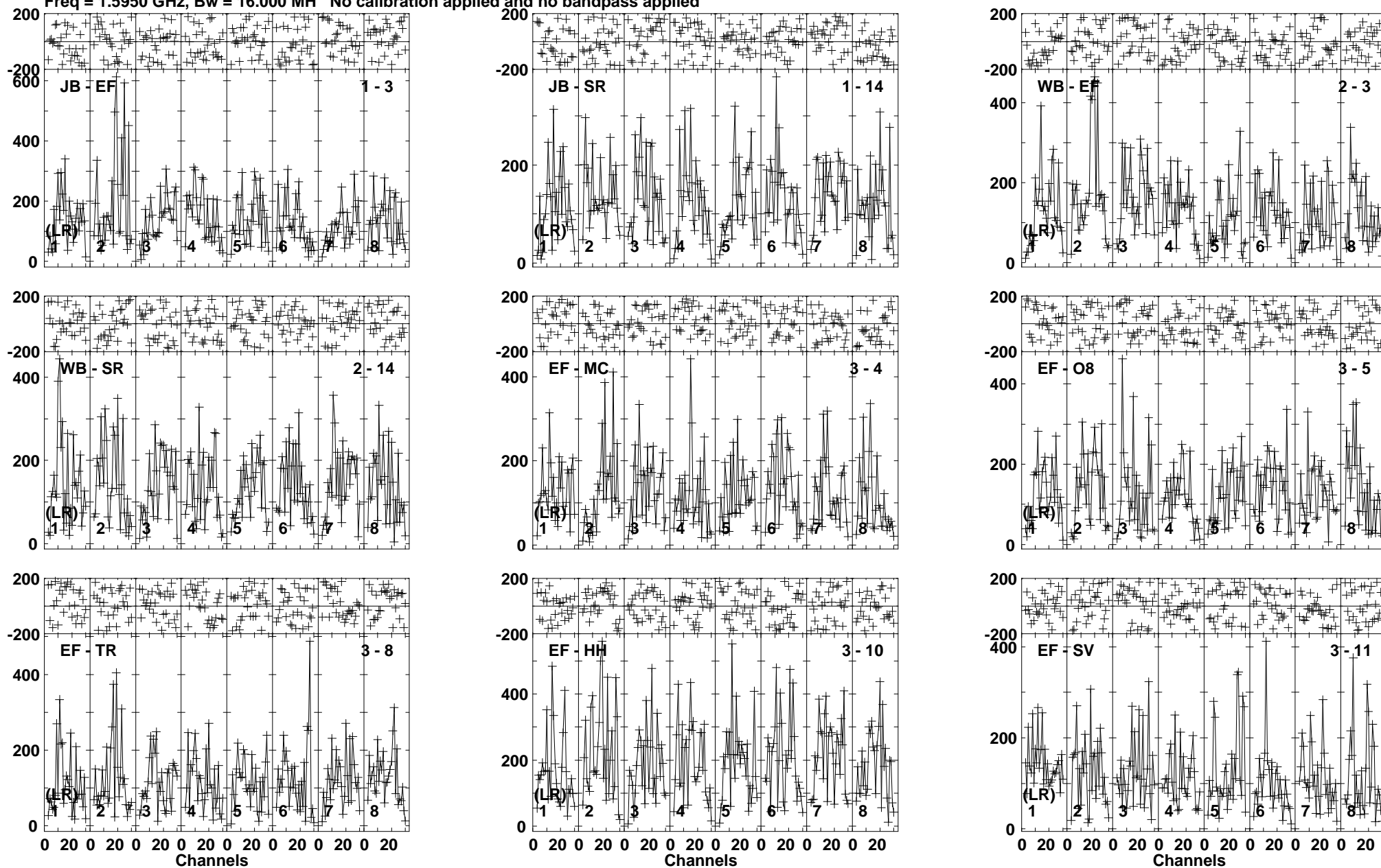
Lower frame: Micro Ampl Jy Top frame: Phas deg Vector averaged cross-power spectrum Baseline: JB (01) - EF (03) Timerange: 00/23:02:01 to 00/23:09:58
