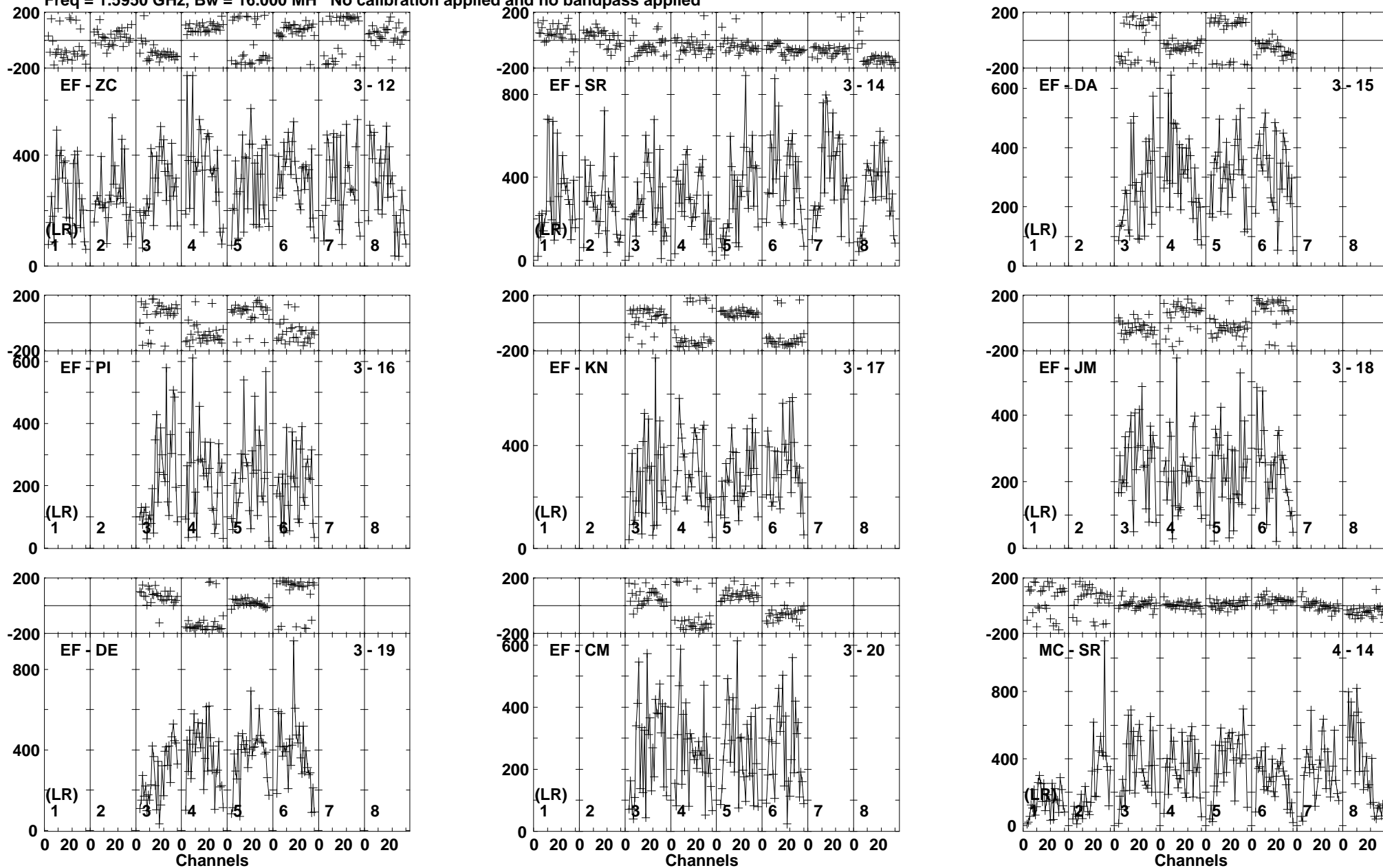
Lower frame: Micro Ampl Jy Top frame: Phas deg Vector averaged cross-power spectrum Baseline: EF (03) - ZC (12) Timerange: 00/23:51:11 to 00/23:52:39
