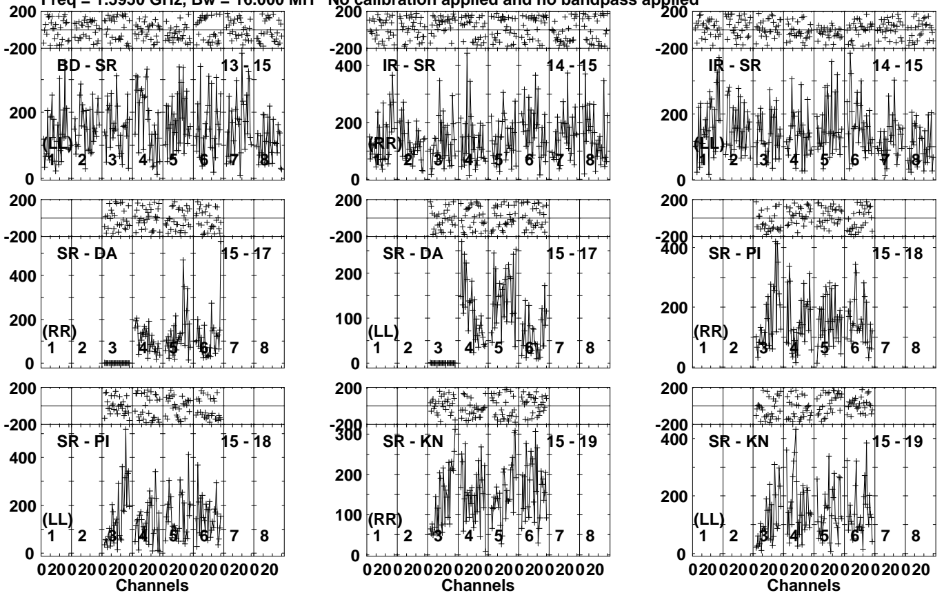
Lower frame: Micro Ampl Jy Top frame: Phas deg Vector averaged cross-power spectrum Several baselines displayed Timerange: 00/03:14:12 to 00/03:16:08
