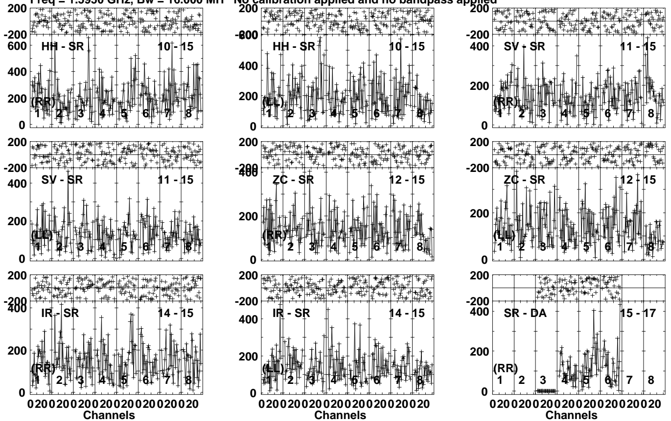
Lower frame: Micro Ampl Jy Top frame: Phas deg Vector averaged cross-power spectrum Several baselines displayed Timerange: 00/05:50:32 to 00/05:56:28
