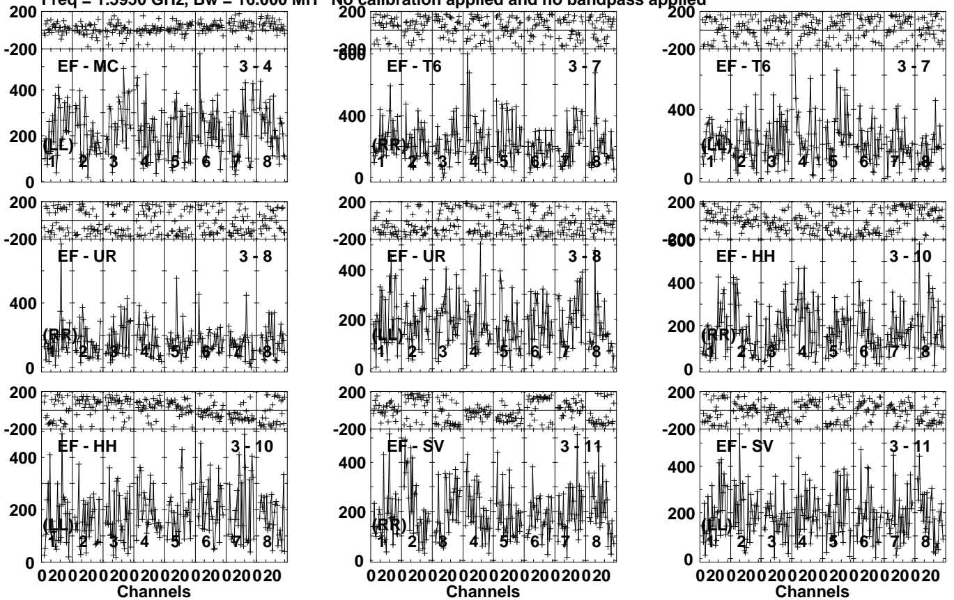
Lower frame: Micro Ampl Jy Top frame: Phas deg Vector averaged cross-power spectrum Several baselines displayed Timerange: 00/03:36:42 to 00/03:38:09
