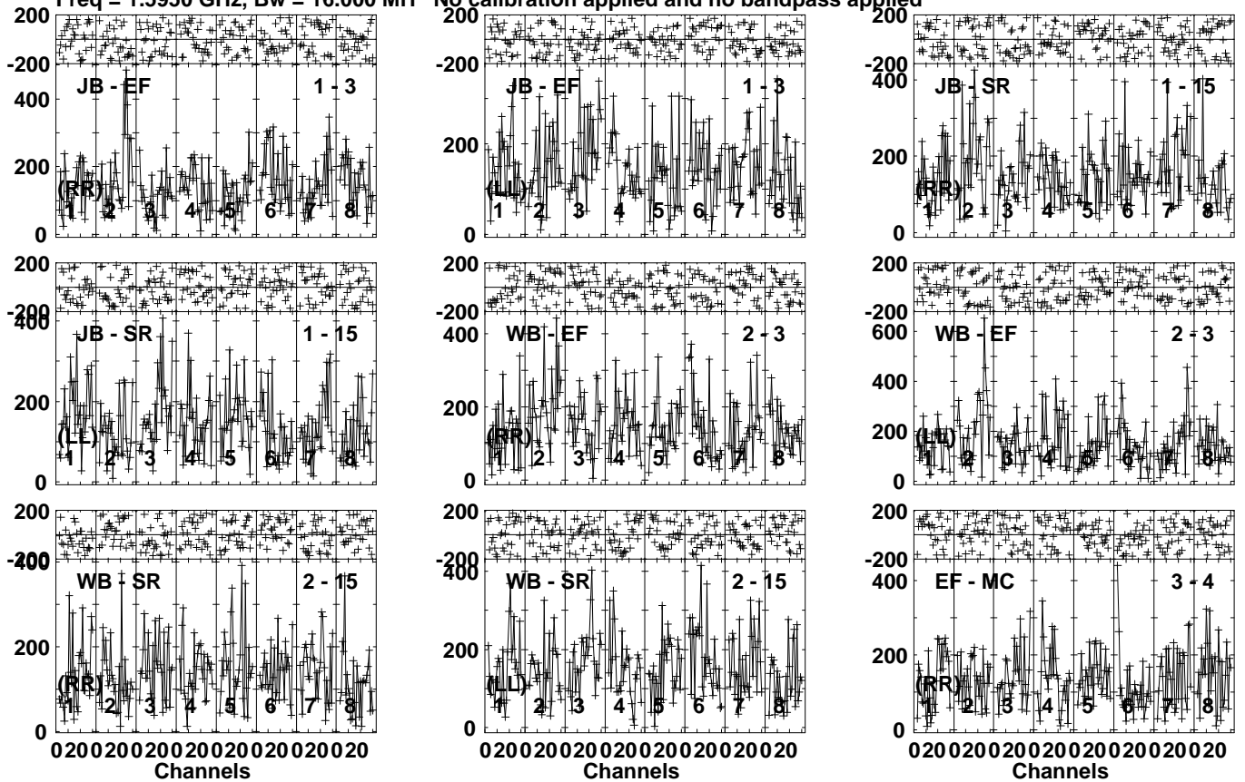
Lower frame: Micro Ampl Jy Top frame: Phas deg Vector averaged cross-power spectrum Several baselines displayed Timerange: 00/10:22:02 to 00/10:27:58
