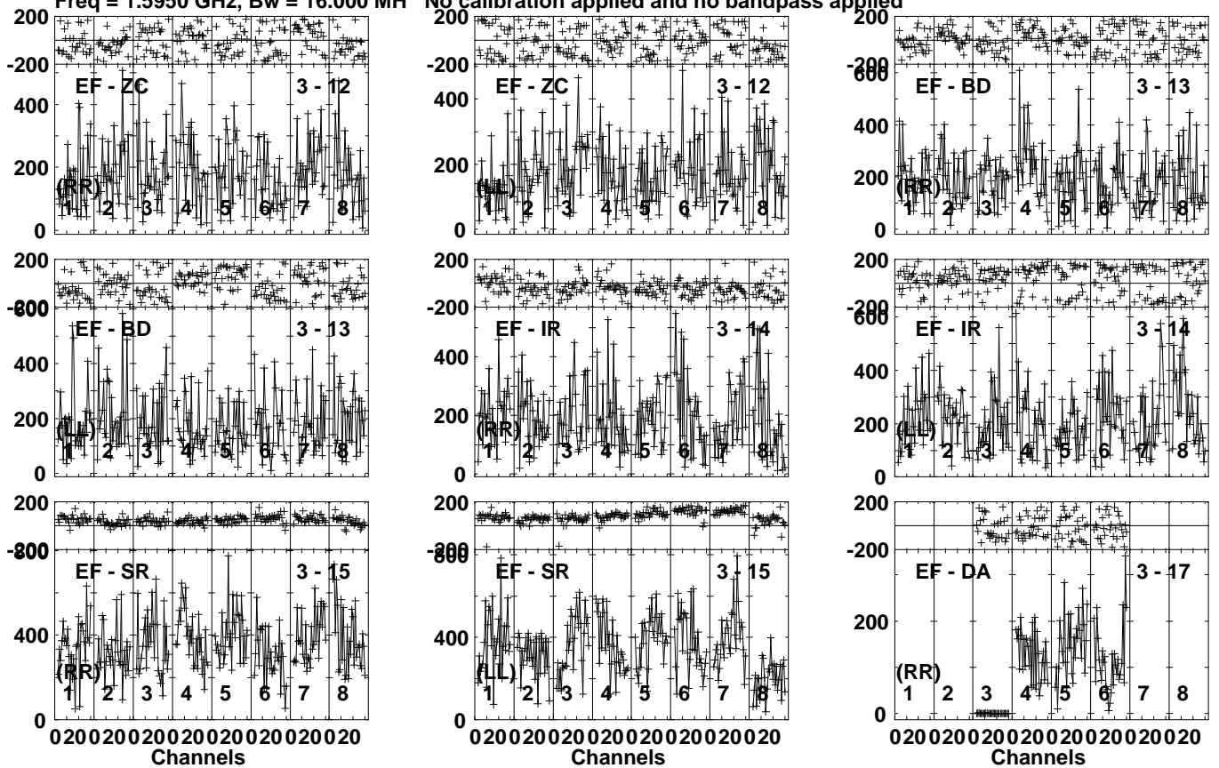
Lower frame: Micro Ampl Jy Top frame: Phas deg Vector averaged cross-power spectrum Several baselines displayed Timerange: 00/03:06:41 to 00/03:08:09
