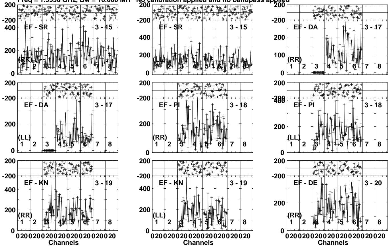
Lower frame: Micro Ampl Jy Top frame: Phas deg Vector averaged cross-power spectrum Several baselines displayed Timerange: 00/09:22:02 to 00/09:27:58
