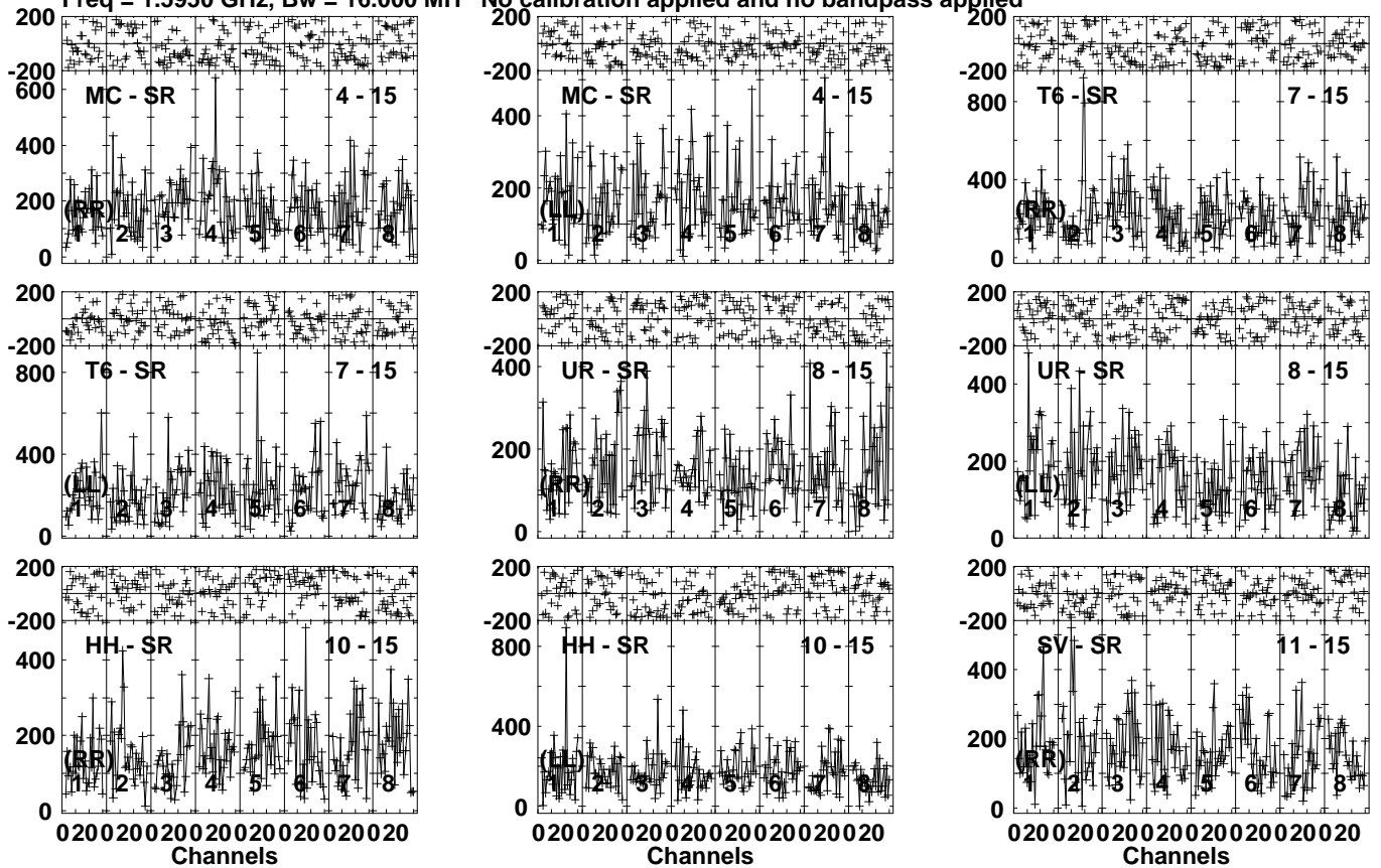
Lower frame: Micro Ampl Jy Top frame: Phas deg Vector averaged cross-power spectrum Several baselines displayed Timerange: 00/02:54:41 to 00/02:56:08
