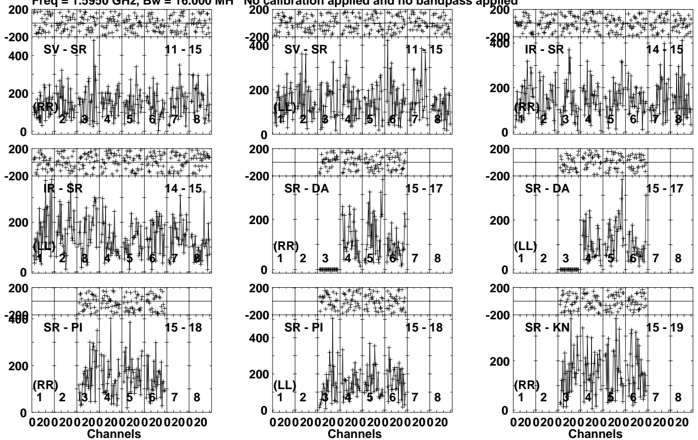
Lower frame: Micro Ampl Jy Top frame: Phas deg Vector averaged cross-power spectrum Several baselines displayed Timerange: 00/09:52:01 to 00/09:57:58
