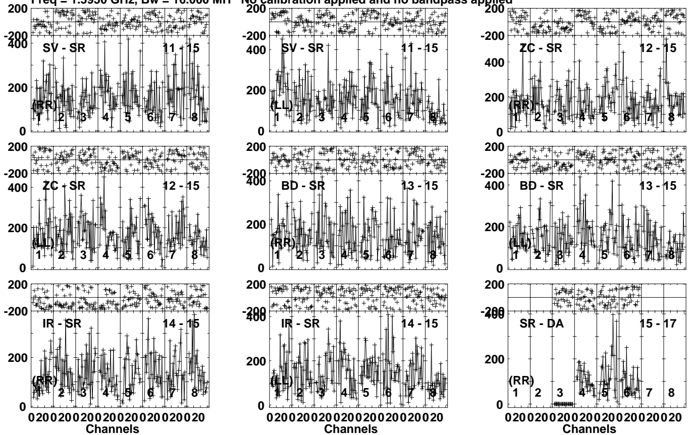
Lower frame: Micro Ampl Jy Top frame: Phas deg Vector averaged cross-power spectrum Several baselines displayed Timerange: 00/04:44:12 to 00/04:46:08
