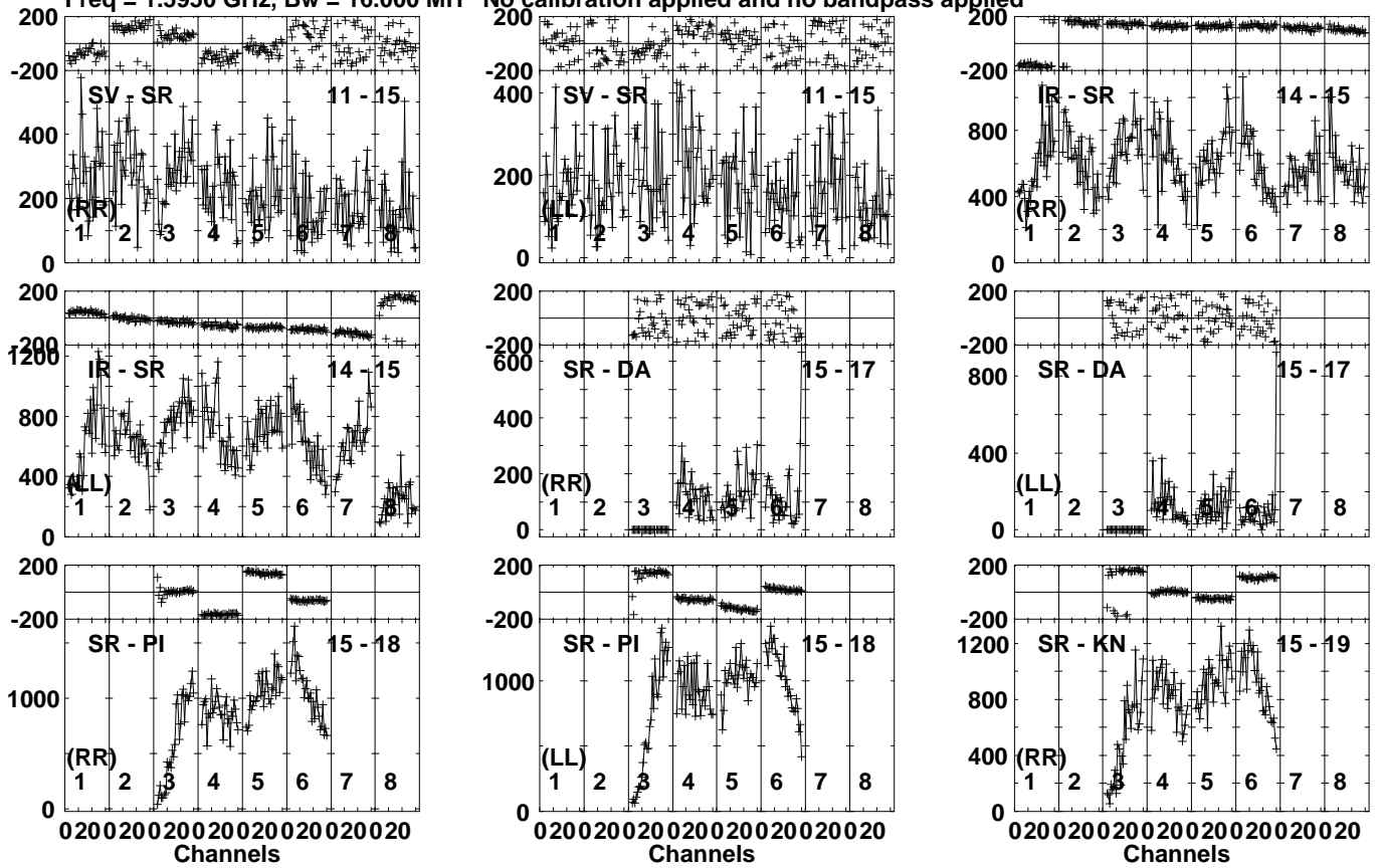
Lower frame: Micro Ampl Jy Top frame: Phas deg Vector averaged cross-power spectrum Several baselines displayed Timerange: 00/09:48:41 to 00/09:50:09
