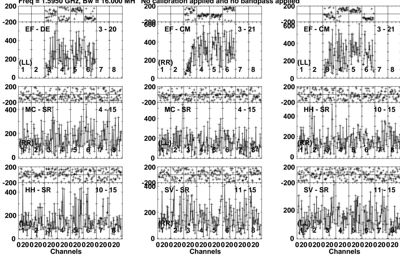
Lower frame: Micro Ampl Jy Top frame: Phas deg Vector averaged cross-power spectrum Several baselines displayed Timerange: 00/07:38:31 to 00/07:40:29
