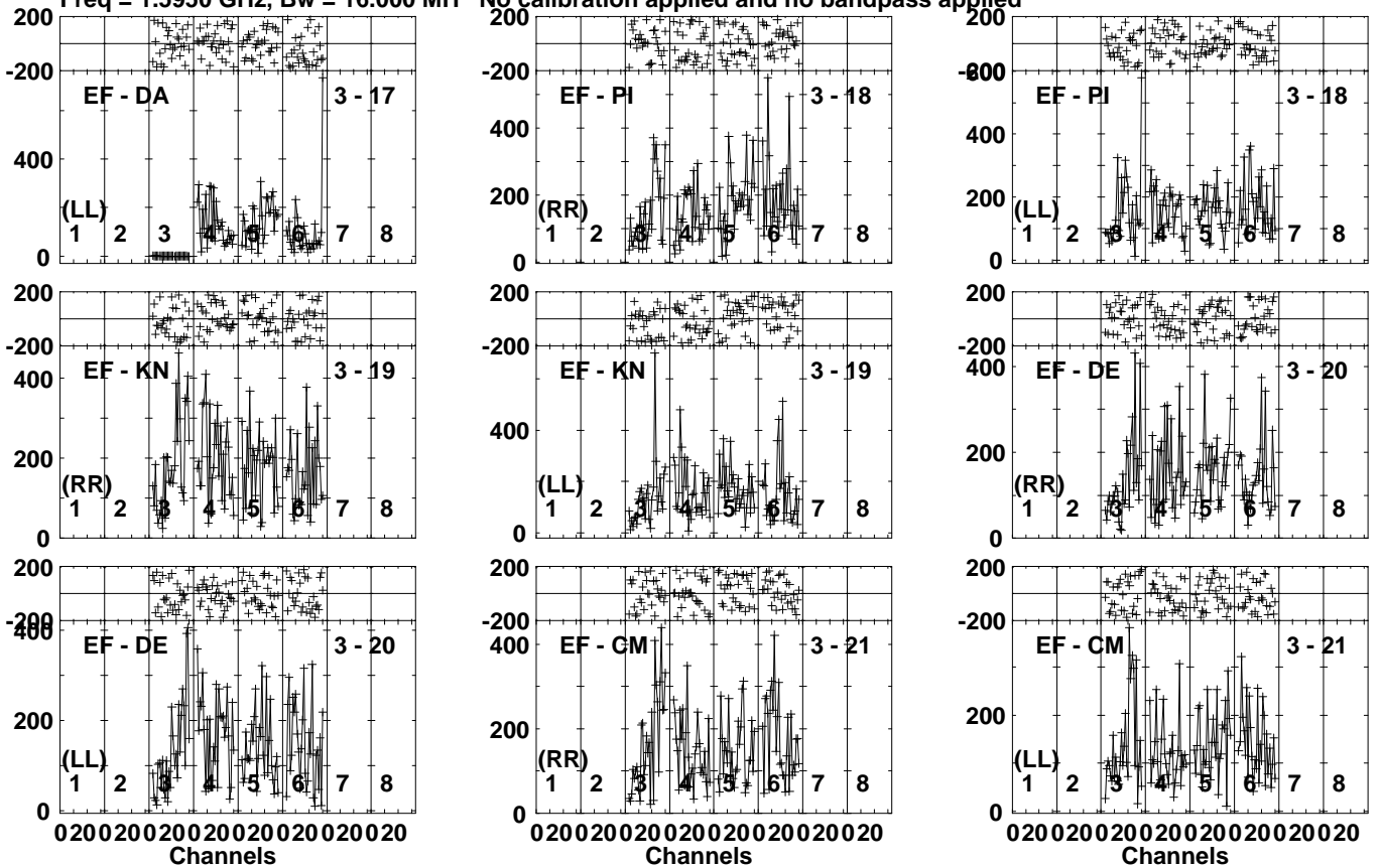
Lower frame: Micro Ampl Jy Top frame: Phas deg Vector averaged cross-power spectrum Several baselines displayed Timerange: 00/03:08:11 to 00/03:14:08
