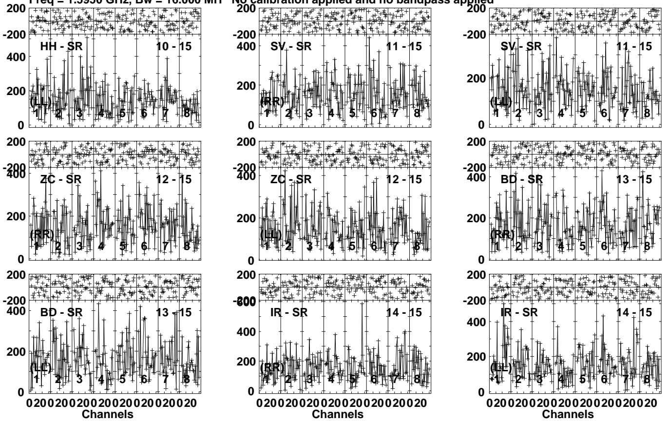
Lower frame: Micro Ampl Jy Top frame: Phas deg Vector averaged cross-power spectrum Several baselines displayed Timerange: 00/01:06:42 to 00/01:08:09
