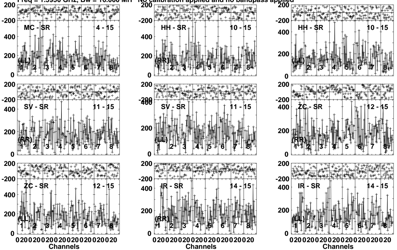
Lower frame: Micro Ampl Jy Top frame: Phas deg Vector averaged cross-power spectrum Several baselines displayed Timerange: 00/09:28:31 to 00/09:29:58
