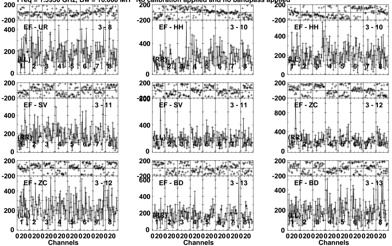
Lower frame: Micro Ampl Jy Top frame: Phas deg Vector averaged cross-power spectrum Several baselines displayed Timerange: 00/03:44:12 to 00/03:46:09
