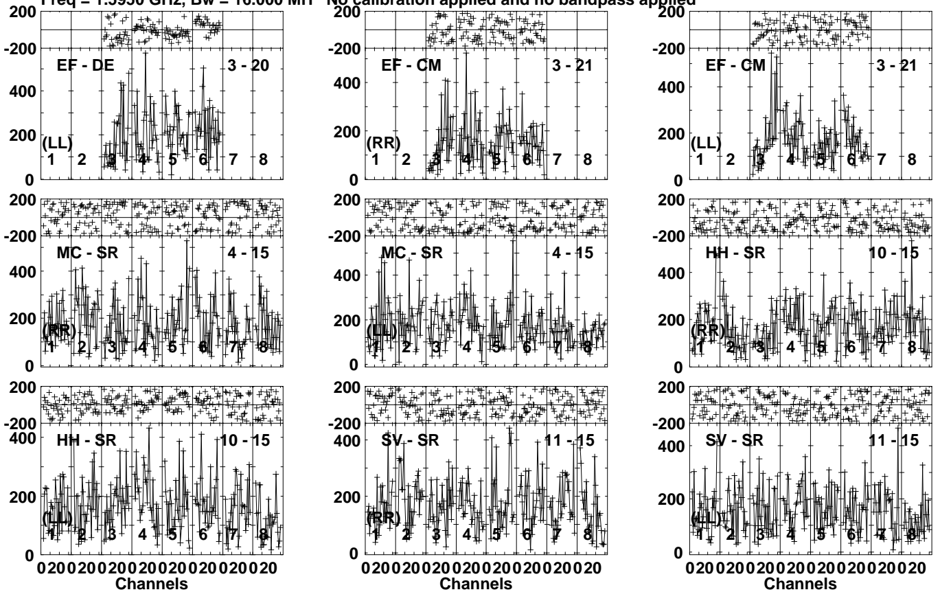
Lower frame: Micro Ampl Jy Top frame: Phas deg Vector averaged cross-power spectrum Several baselines displayed Timerange: 00/08:37:31 to 00/08:38:59
