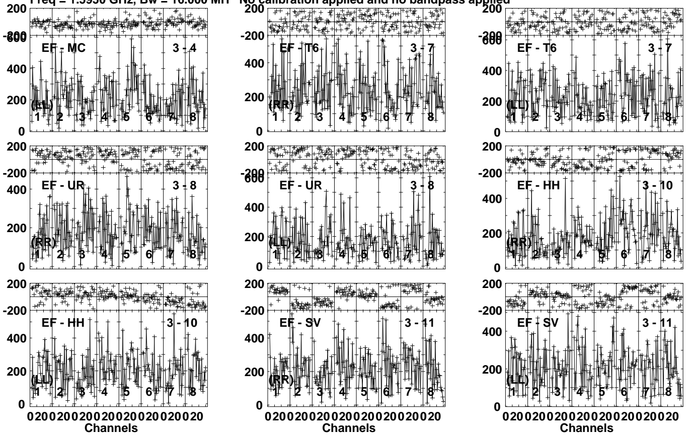
Lower frame: Micro Ampl Jy Top frame: Phas deg Vector averaged cross-power spectrum Several baselines displayed Timerange: 00/04:36:41 to 00/04:38:09
