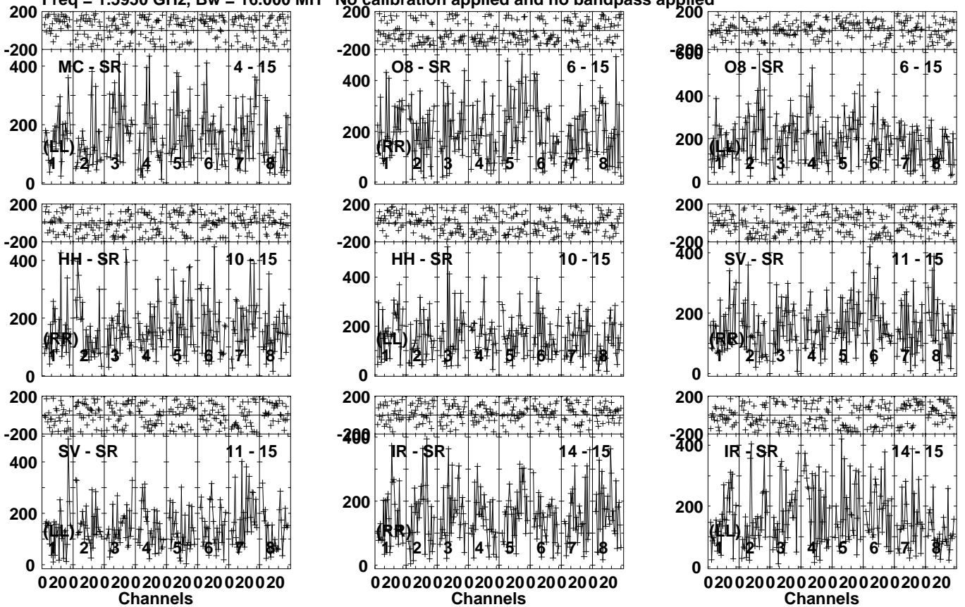
Lower frame: Micro Ampl Jy Top frame: Phas deg Vector averaged cross-power spectrum Several baselines displayed Timerange: 00/09:58:31 to 00/09:59:58
