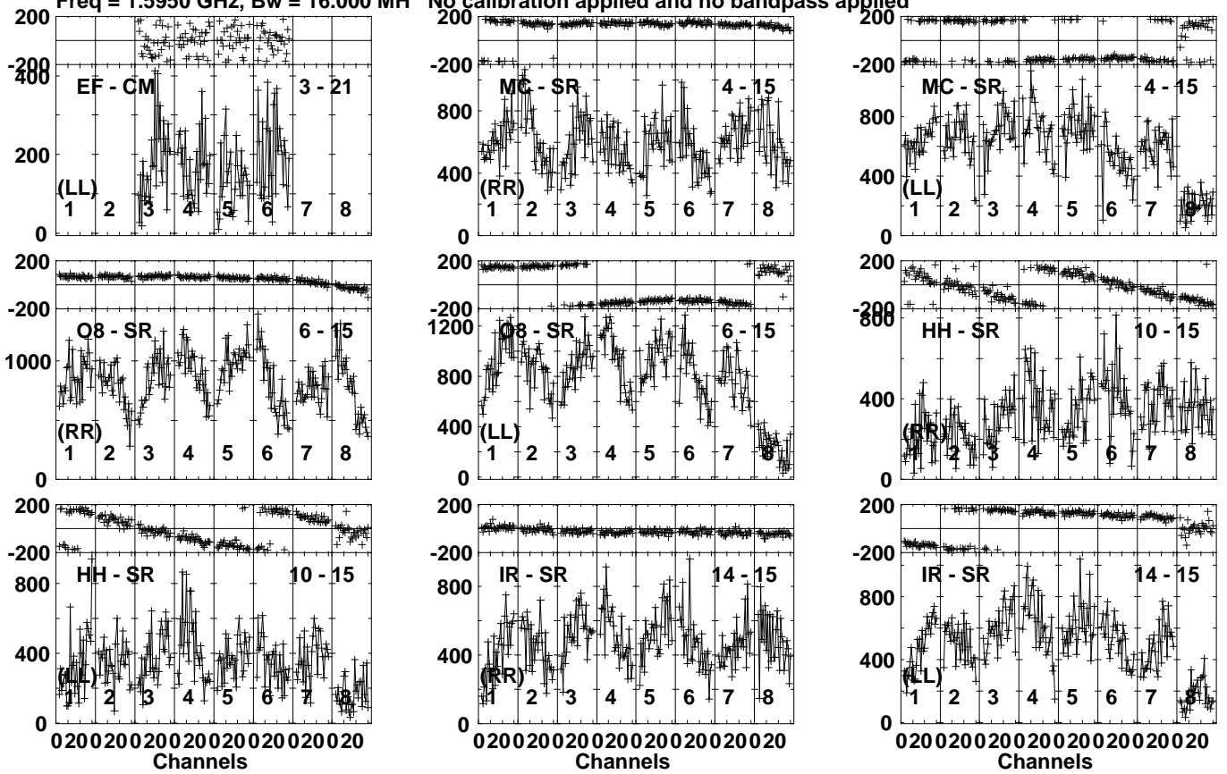
Lower frame: Micro Ampl Jy Top frame: Phas deg Vector averaged cross-power spectrum Several baselines displayed Timerange: 00/10:48:41 to 00/10:50:08
