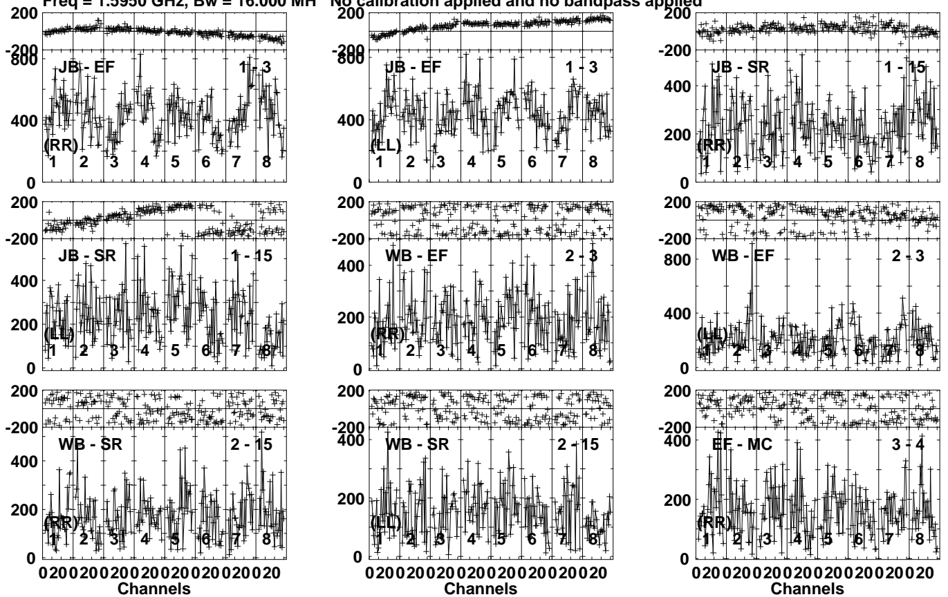
Lower frame: Micro Ampl Jy Top frame: Phas deg Vector averaged cross-power spectrum Several baselines displayed Timerange: 00/11:47:02 to 00/11:48:58
