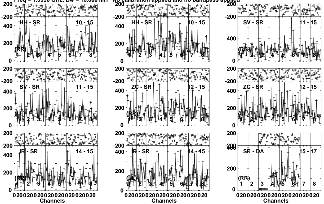
Lower frame: Micro Ampl Jy Top frame: Phas deg Vector averaged cross-power spectrum Several baselines displayed Timerange: 00/06:19:11 to 00/06:20:56
