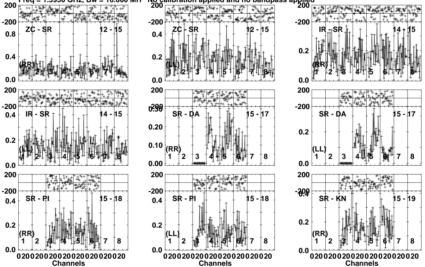
Lower frame: Milli Ampl Jy Top frame: Phas deg Vector averaged cross-power spectrum Several baselines displayed Timerange: 00/08:50:12 to 00/08:51:56
