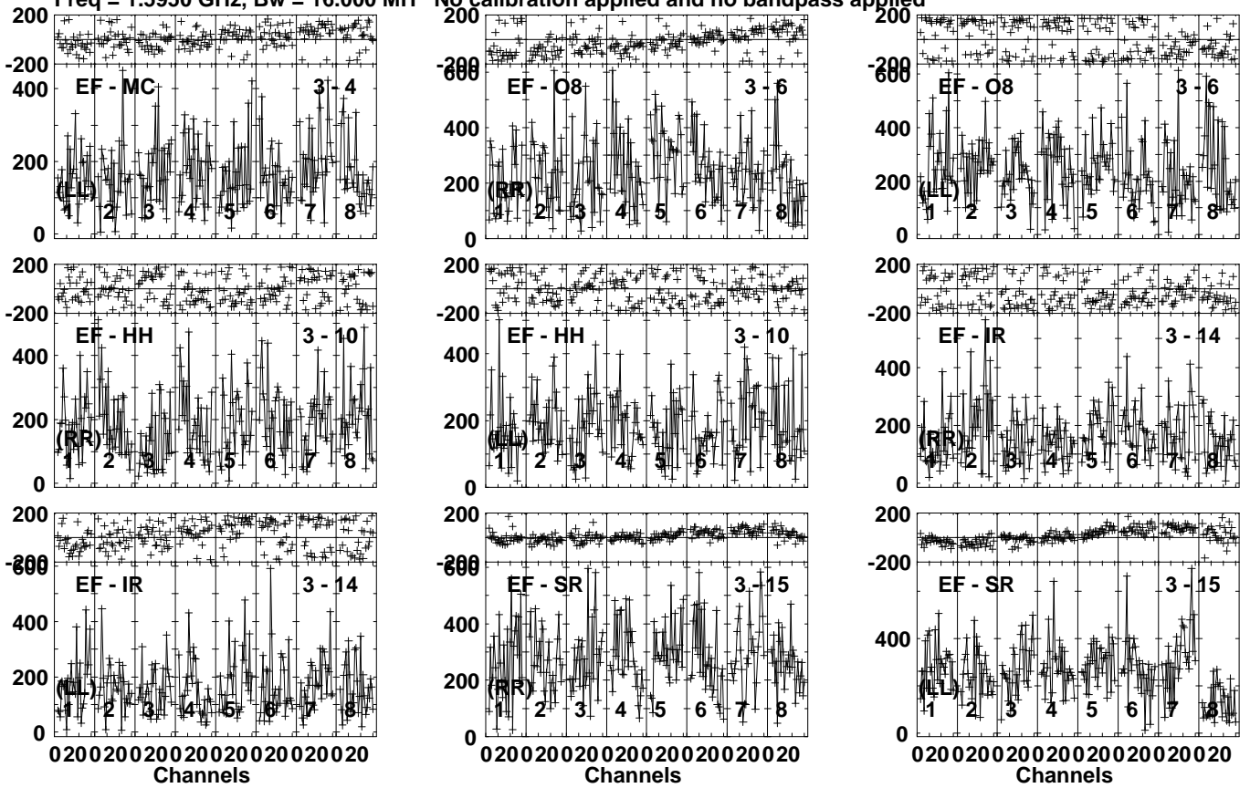
Lower frame: Micro Ampl Jy Top frame: Phas deg Vector averaged cross-power spectrum Several baselines displayed Timerange: 00/10:20:12 to 00/10:21:56
