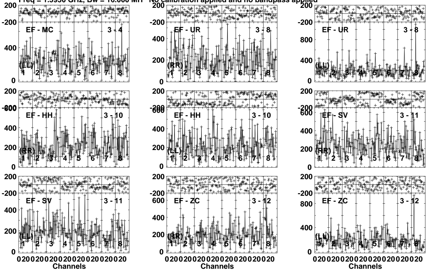
Lower frame: Micro Ampl Jy Top frame: Phas deg Vector averaged cross-power spectrum Several baselines displayed Timerange: 00/06:49:42 to 00/06:51:27
