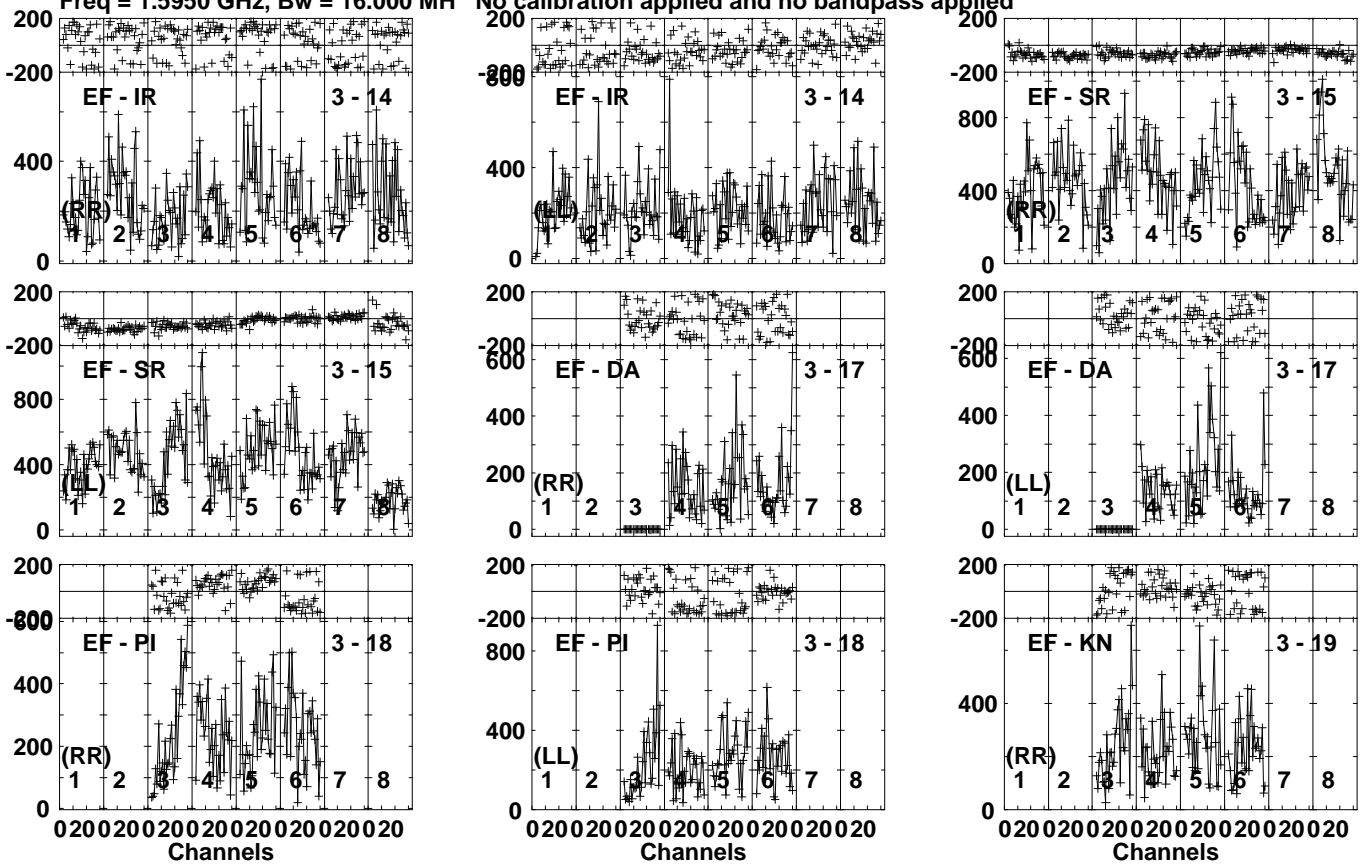
Lower frame: Micro Ampl Jy Top frame: Phas deg Vector averaged cross-power spectrum Several baselines displayed Timerange: 00/05:48:41 to 00/05:50:26
