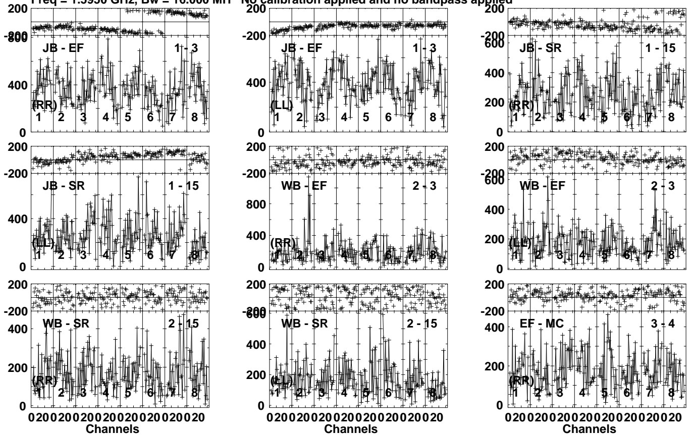
Lower frame: Micro Ampl Jy Top frame: Phas deg Vector averaged cross-power spectrum Several baselines displayed Timerange: 00/01:54:41 to 00/01:56:08
