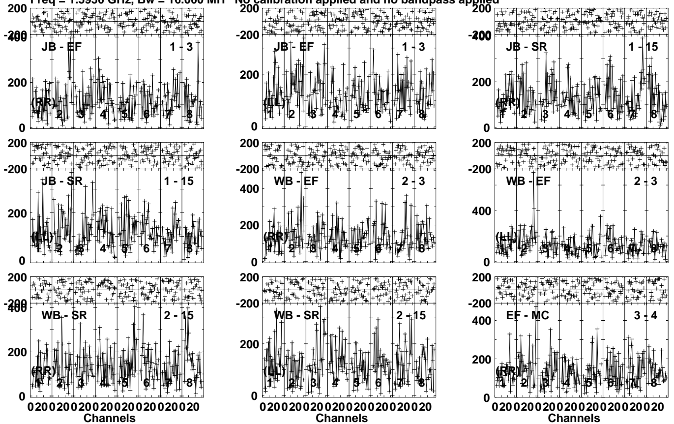
Lower frame: Micro Ampl Jy Top frame: Phas deg Vector averaged cross-power spectrum Several baselines displayed Timerange: 00/05:39:01 to 00/05:46:29
