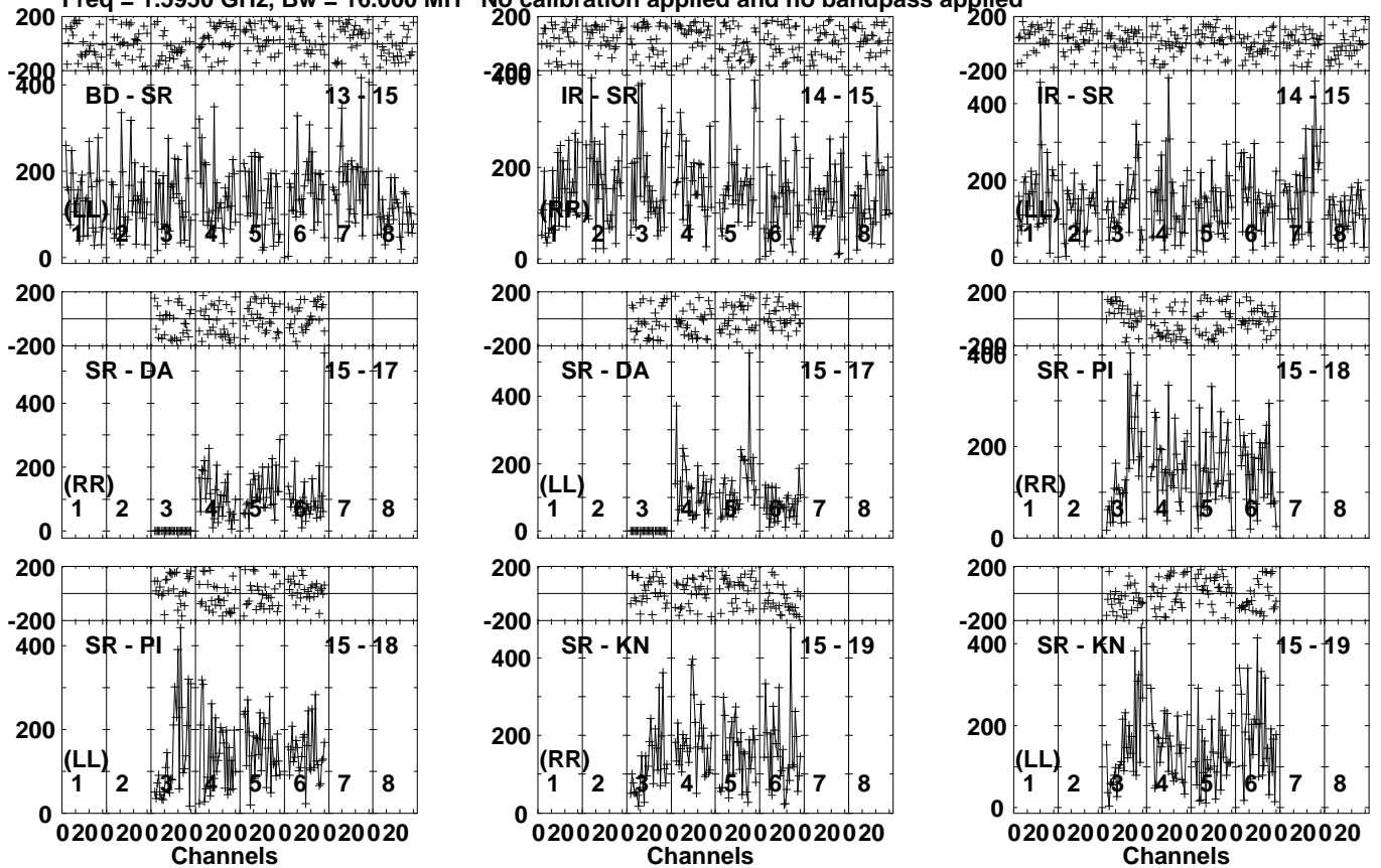
Lower frame: Micro Ampl Jy Top frame: Phas deg Vector averaged cross-power spectrum Several baselines displayed Timerange: 00/02:44:12 to 00/02:46:08
