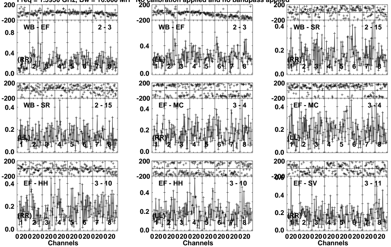
Lower frame: Milli Ampl Jy Top frame: Phas deg Vector averaged cross-power spectrum Several baselines displayed Timerange: 00/07:59:02 to 00/08:00:59
