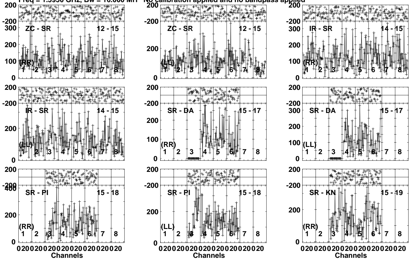
Lower frame: Micro Ampl Jy Top frame: Phas deg Vector averaged cross-power spectrum Several baselines displayed Timerange: 00/09:00:02 to 00/09:07:58
