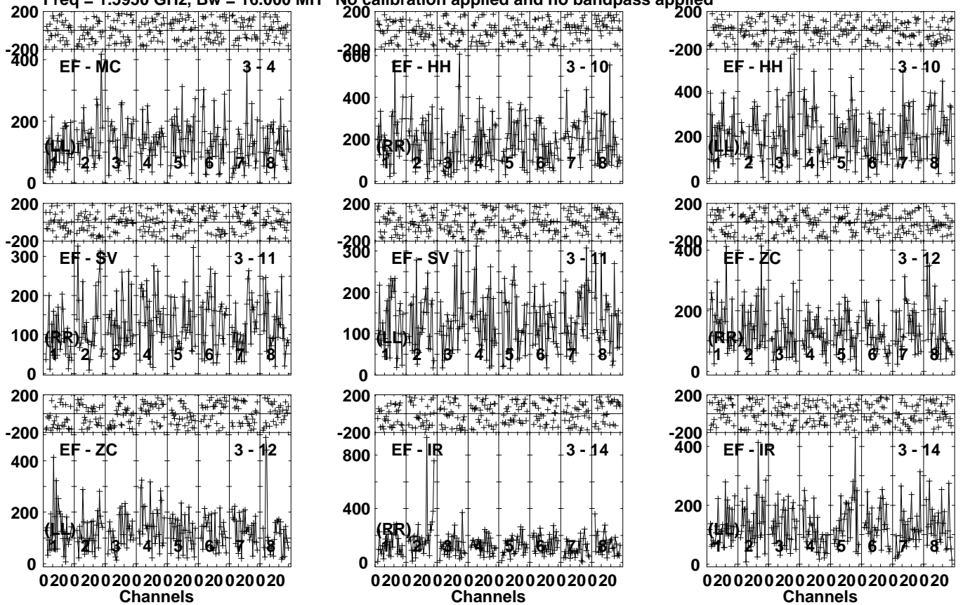
Lower frame: Micro Ampl Jy Top frame: Phas deg Vector averaged cross-power spectrum Several baselines displayed Timerange: 00/08:39:01 to 00/08:45:59
