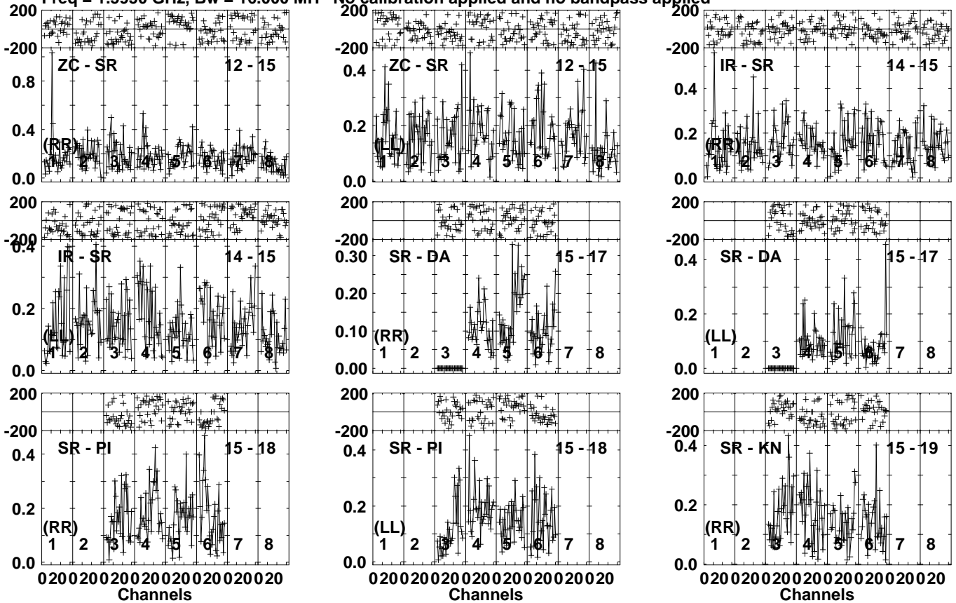
Lower frame: Milli Ampl Jy Top frame: Phas deg Vector averaged cross-power spectrum Several baselines displayed Timerange: 00/07:50:41 to 00/07:52:27
