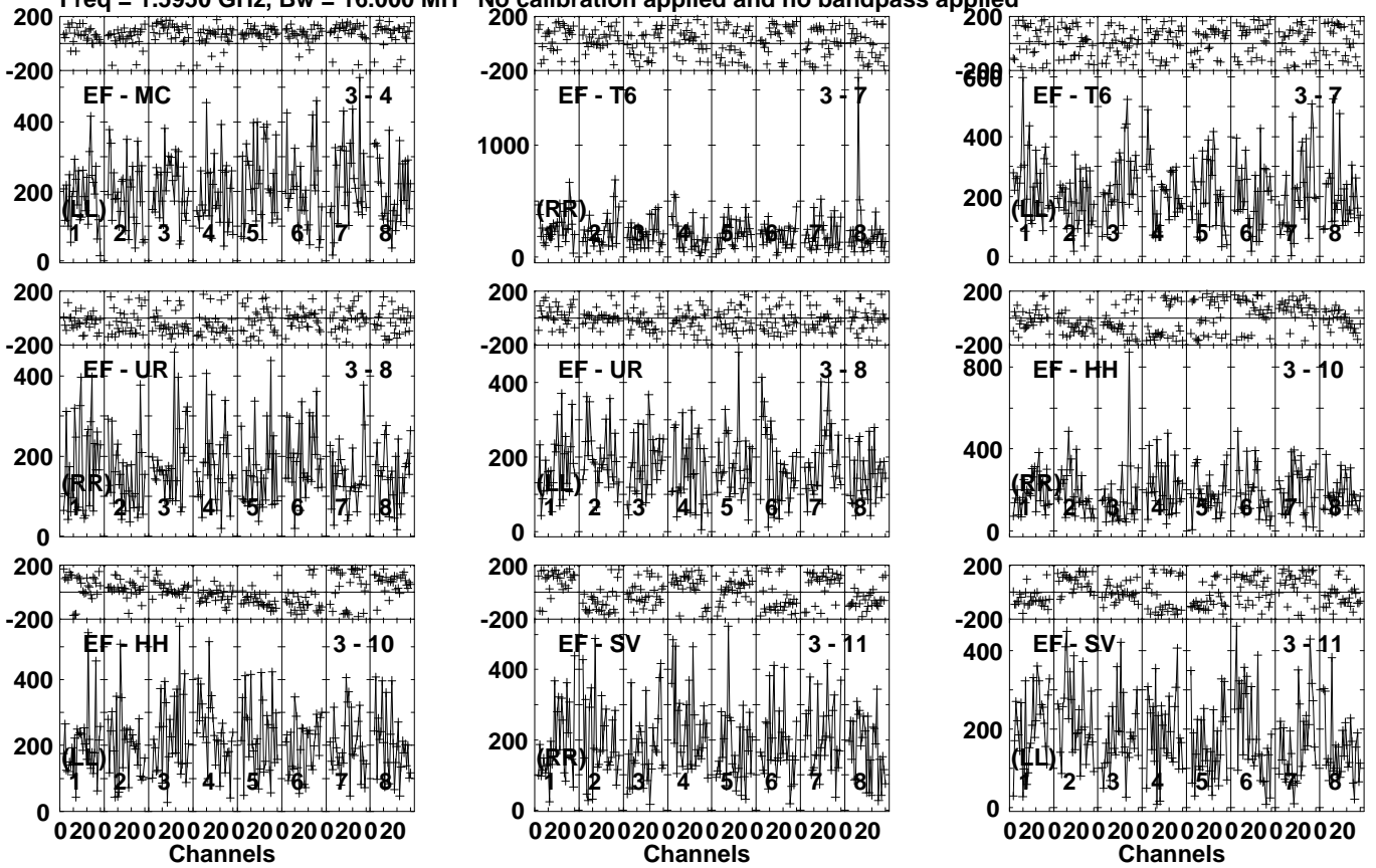
Lower frame: Micro Ampl Jy Top frame: Phas deg Vector averaged cross-power spectrum Several baselines displayed Timerange: 00/03:24:41 to 00/03:26:08
