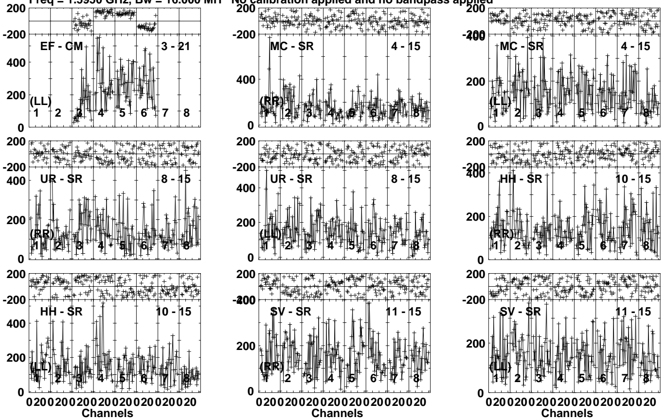
Lower frame: Micro Ampl Jy Top frame: Phas deg Vector averaged cross-power spectrum Several baselines displayed Timerange: 00/05:57:02 to 00/05:58:59
