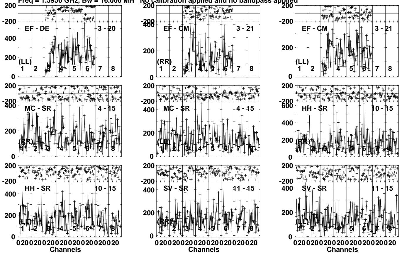
Lower frame: Micro Ampl Jy Top frame: Phas deg Vector averaged cross-power spectrum Several baselines displayed Timerange: 00/08:46:01 to 00/08:47:59
