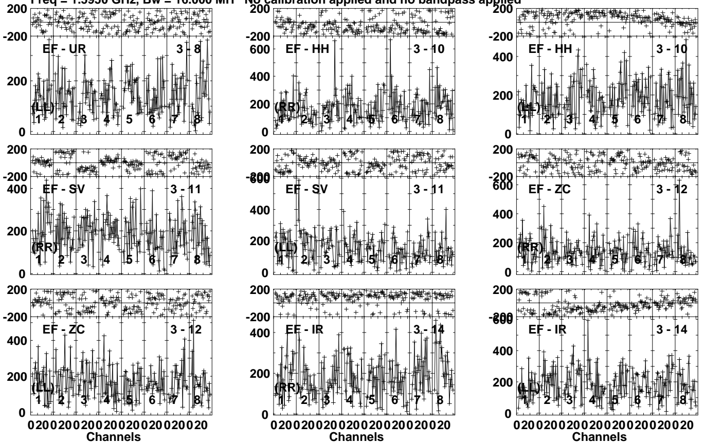
Lower frame: Micro Ampl Jy Top frame: Phas deg Vector averaged cross-power spectrum Several baselines displayed Timerange: 00/06:58:01 to 00/06:59:59
