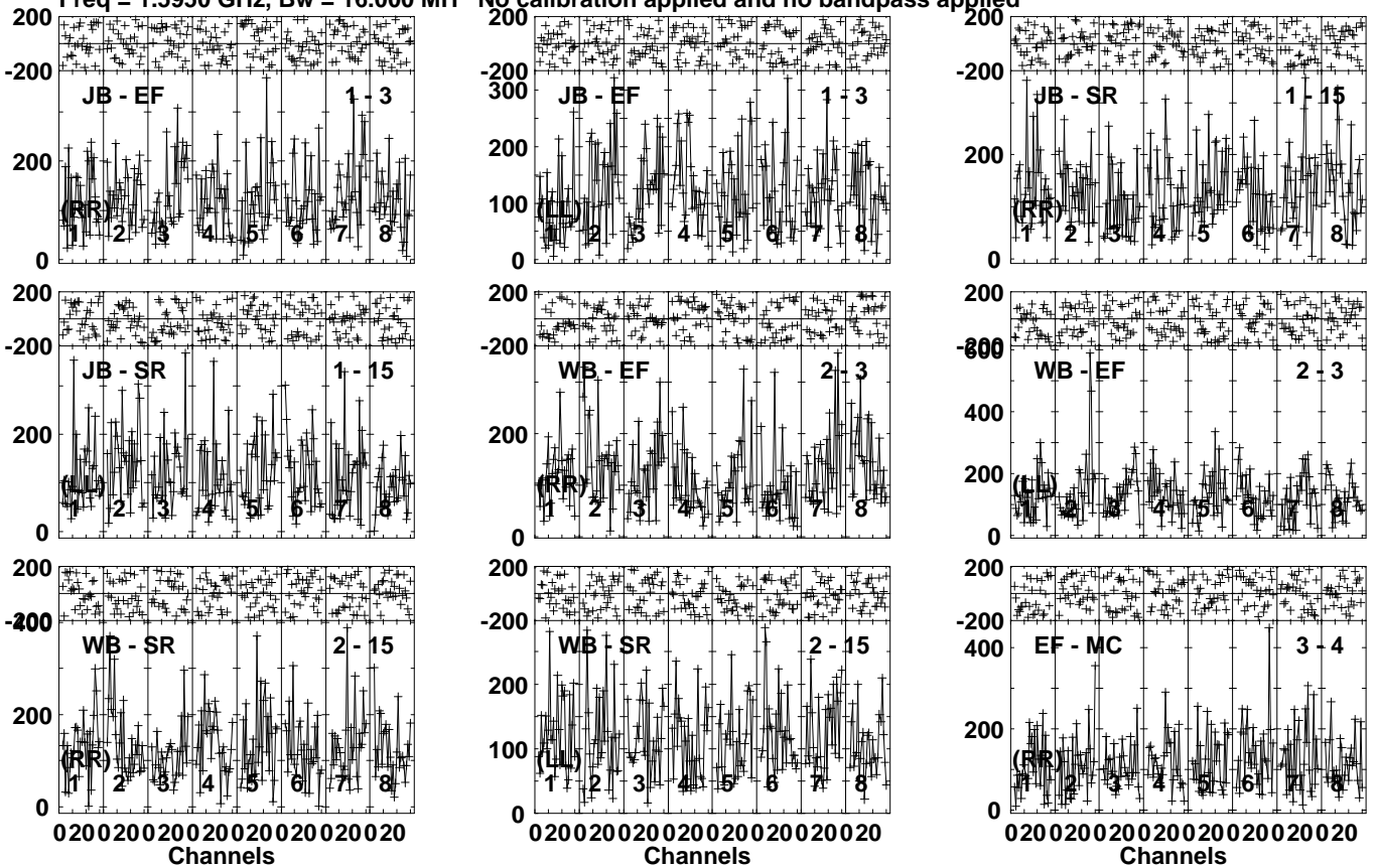
Lower frame: Micro Ampl Jy Top frame: Phas deg Vector averaged cross-power spectrum Several baselines displayed Timerange: 00/06:39:32 to 00/06:47:29
