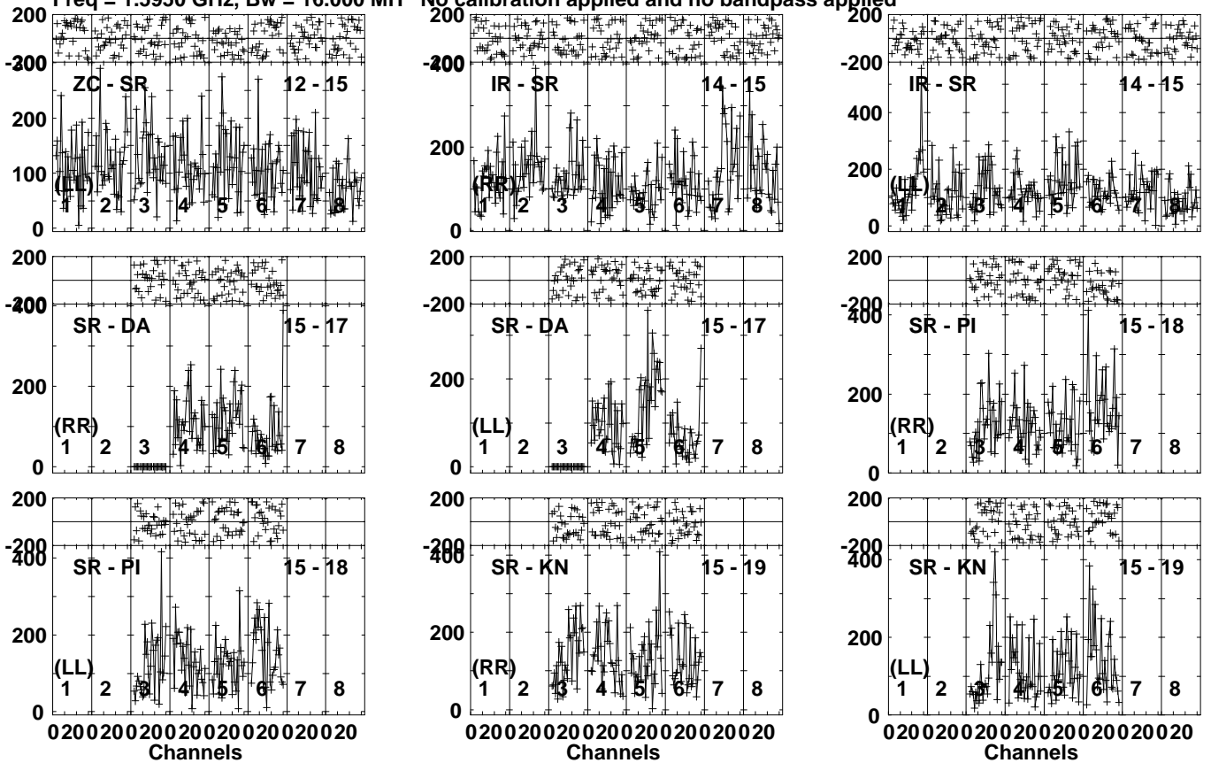
Lower frame: Micro Ampl Jy Top frame: Phas deg Vector averaged cross-power spectrum Several baselines displayed Timerange: 00/07:00:02 to 00/07:07:58
