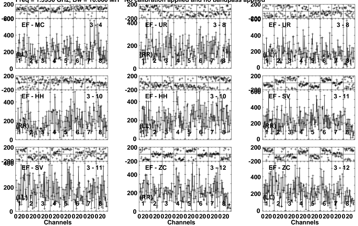
Lower frame: Micro Ampl Jy Top frame: Phas deg Vector averaged cross-power spectrum Several baselines displayed Timerange: 00/05:37:02 to 00/05:38:58
