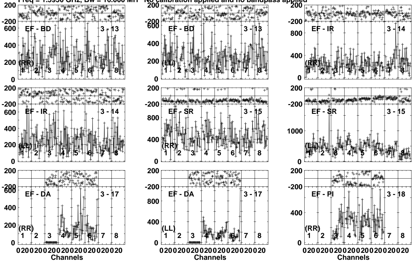
Lower frame: Micro Ampl Jy Top frame: Phas deg Vector averaged cross-power spectrum Several baselines displayed Timerange: 00/05:21:31 to 00/05:22:58
