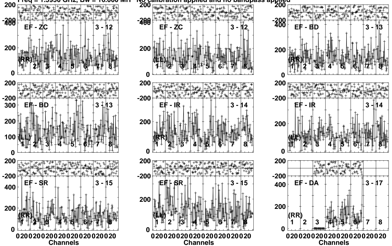
Lower frame: Micro Ampl Jy Top frame: Phas deg Vector averaged cross-power spectrum Several baselines displayed Timerange: 00/01:56:11 to 00/02:04:09
