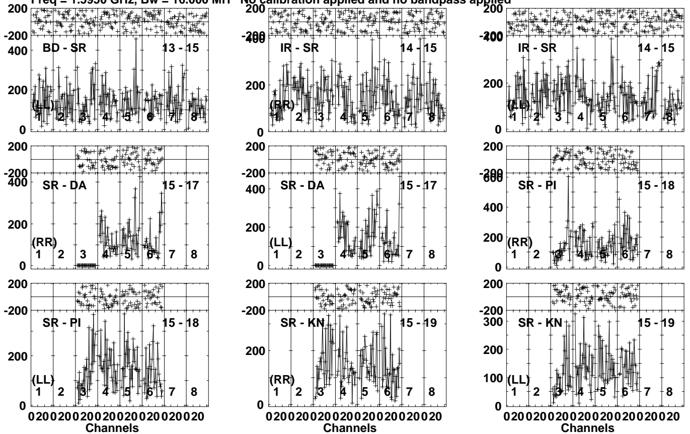
Lower frame: Micro Ampl Jy Top frame: Phas deg Vector averaged cross-power spectrum Several baselines displayed Timerange: 00/05:23:01 to 00/05:28:59
