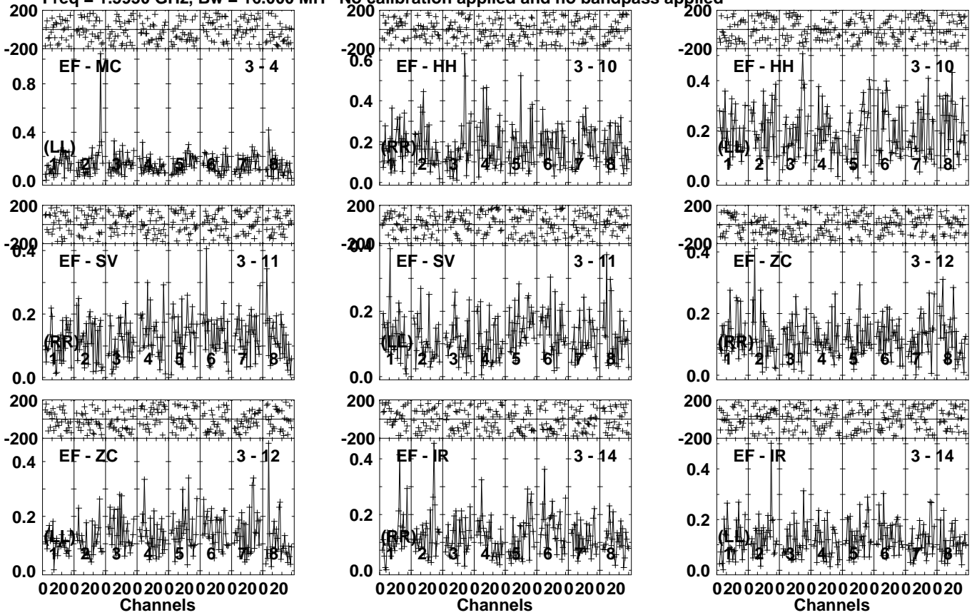
Lower frame: Milli Ampl Jy Top frame: Phas deg Vector averaged cross-power spectrum Several baselines displayed Timerange: 00/09:10:02 to 00/09:17:59
