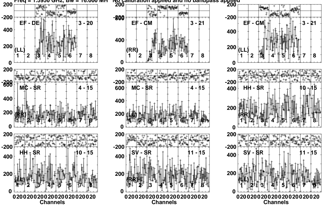
Lower frame: Micro Ampl Jy Top frame: Phas deg Vector averaged cross-power spectrum Several baselines displayed Timerange: 00/07:50:41 to 00/07:52:27
