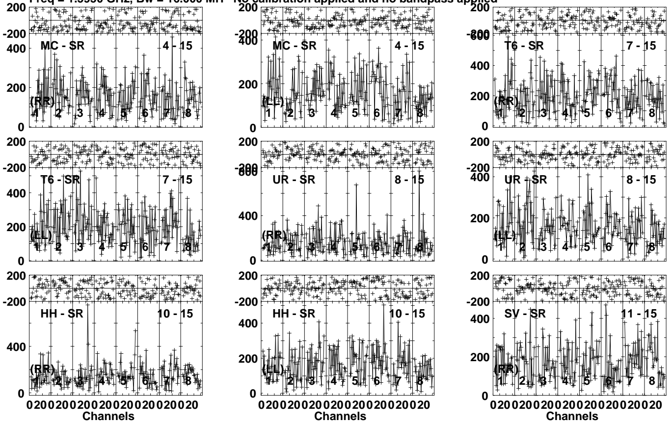
Lower frame: Micro Ampl Jy Top frame: Phas deg Vector averaged cross-power spectrum Several baselines displayed Timerange: 00/04:06:41 to 00/04:08:09
