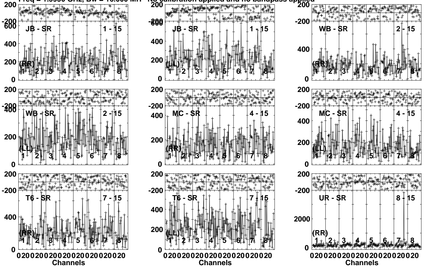
Lower frame: Micro Ampl Jy Top frame: Phas deg Vector averaged cross-power spectrum Several baselines displayed Timerange: 00/01:24:41 to 00/01:26:08
