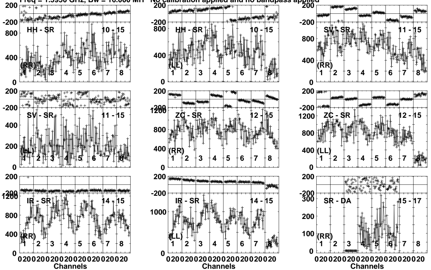
Lower frame: Micro Ampl Jy Top frame: Phas deg Vector averaged cross-power spectrum Several baselines displayed Timerange: 00/06:17:42 to 00/06:19:09
