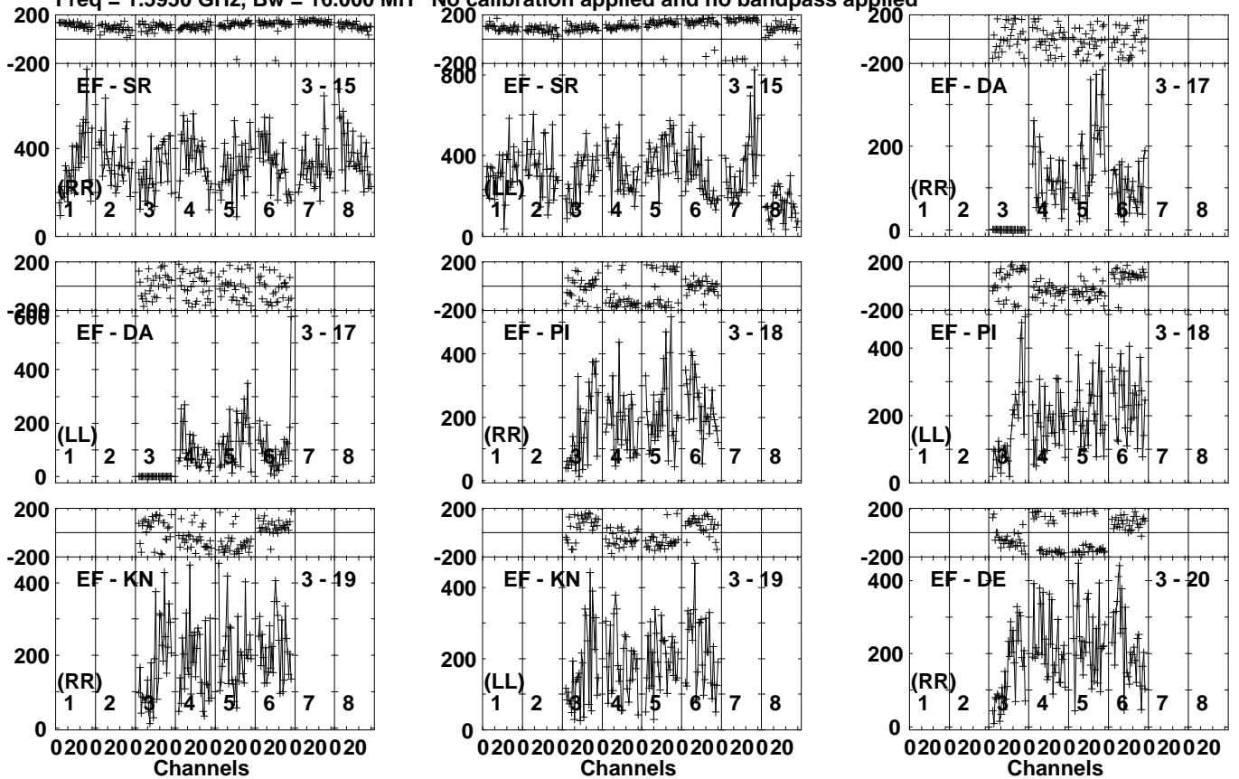
Lower frame: Micro Ampl Jy Top frame: Phas deg Vector averaged cross-power spectrum Several baselines displayed Timerange: 00/09:38:01 to 00/09:39:59
