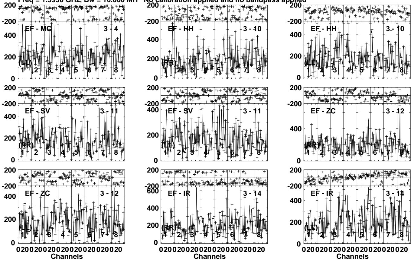
Lower frame: Micro Ampl Jy Top frame: Phas deg Vector averaged cross-power spectrum Several baselines displayed Timerange: 00/08:09:01 to 00/08:10:59
