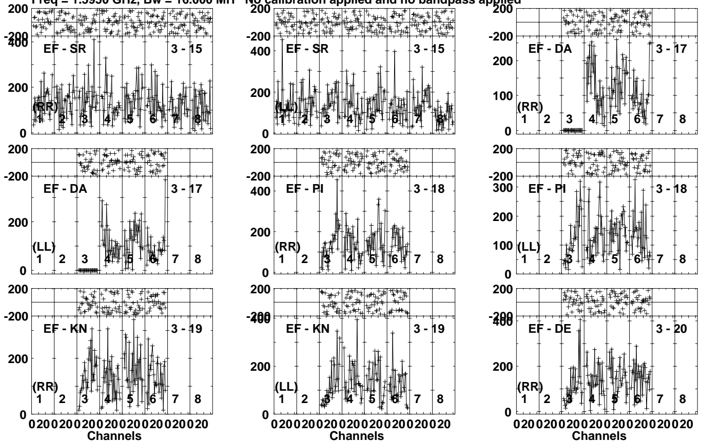
Lower frame: Micro Ampl Jy Top frame: Phas deg Vector averaged cross-power spectrum Several baselines displayed Timerange: 00/08:11:02 to 00/08:18:58
