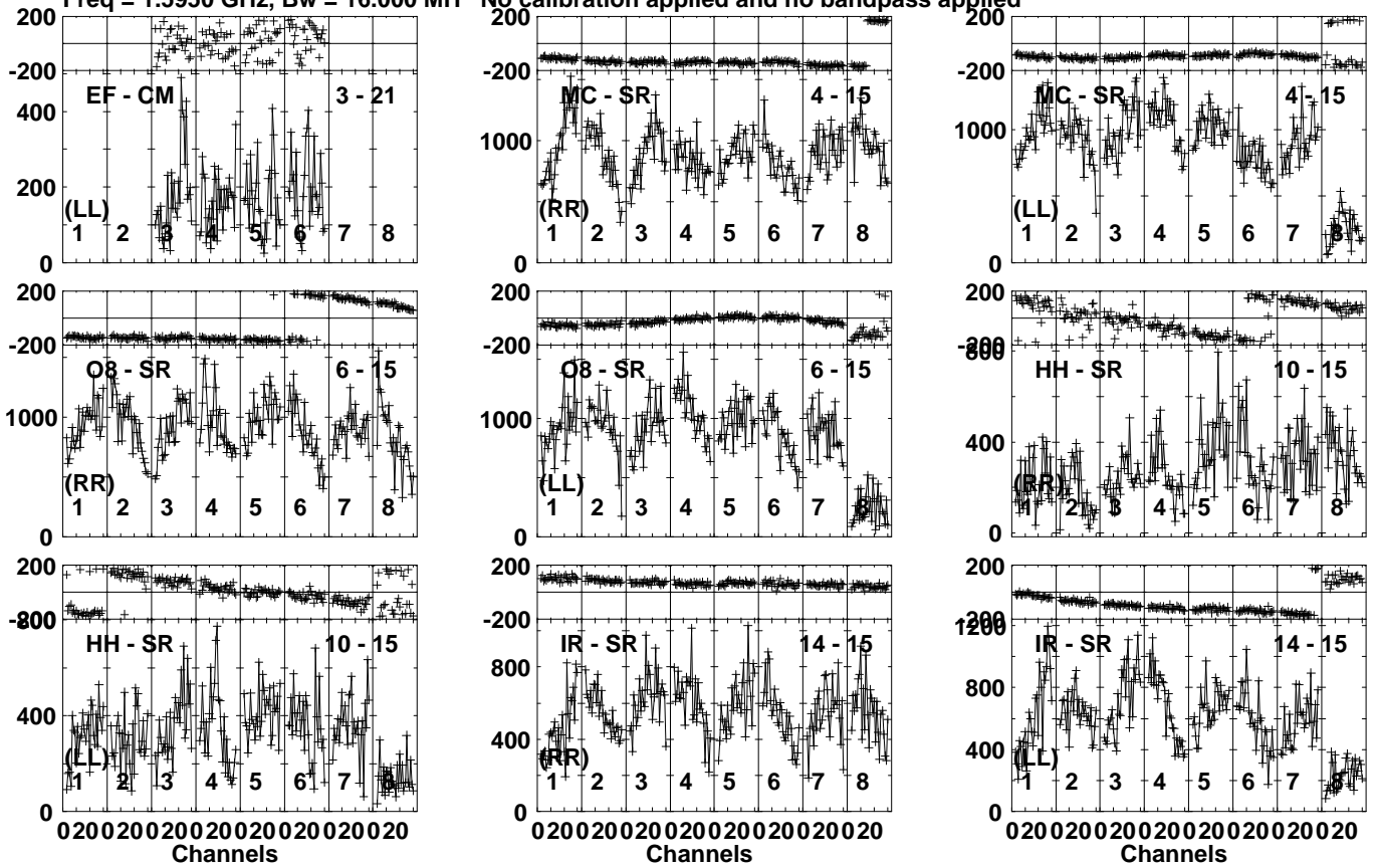
Lower frame: Micro Ampl Jy Top frame: Phas deg Vector averaged cross-power spectrum Several baselines displayed Timerange: 00/10:18:41 to 00/10:20:08
