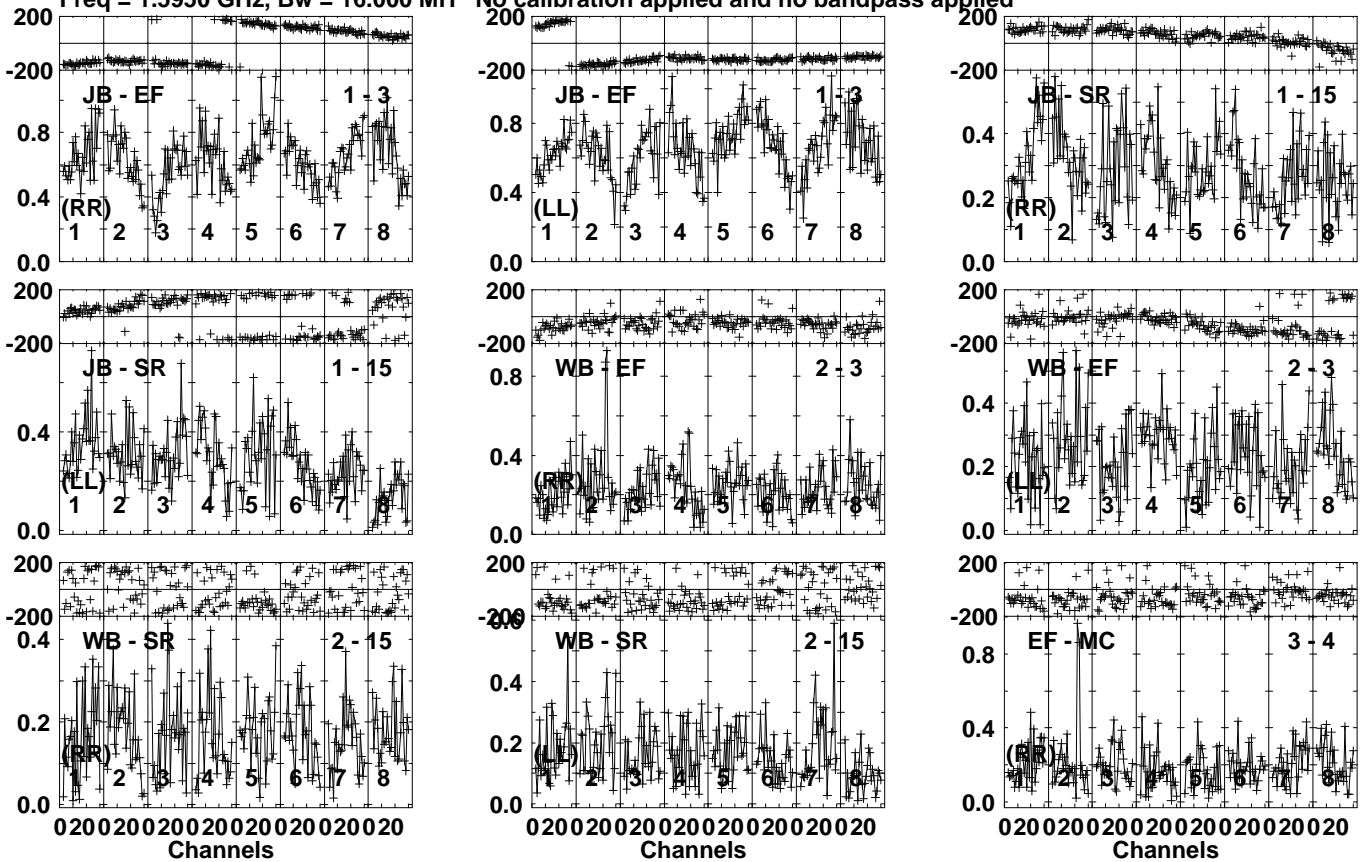
Lower frame: Milli Ampl Jy Top frame: Phas deg Vector averaged cross-power spectrum Several baselines displayed Timerange: 00/07:08:01 to 00/07:09:59
