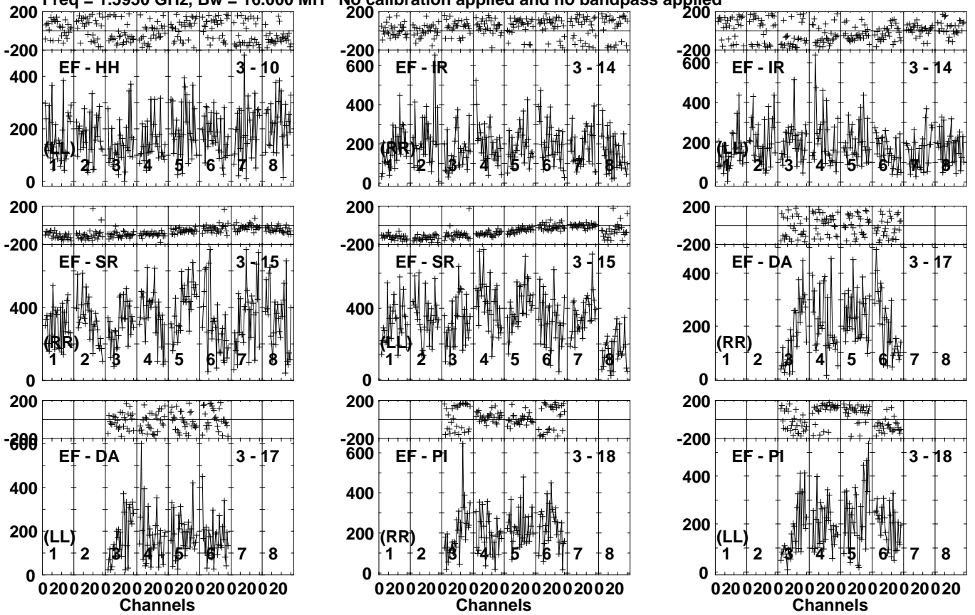
Lower frame: Micro Ampl Jy Top frame: Phas deg Vector averaged cross-power spectrum Several baselines displayed Timerange: 00/10:28:31 to 00/10:29:59
