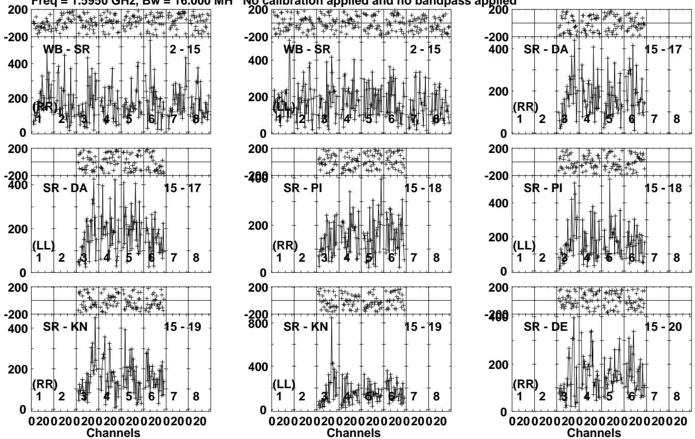
Lower frame: Micro Ampl Jy Top frame: Phas deg Vector averaged cross-power spectrum Several baselines displayed Timerange: 00/12:08:01 to 00/12:09:29
