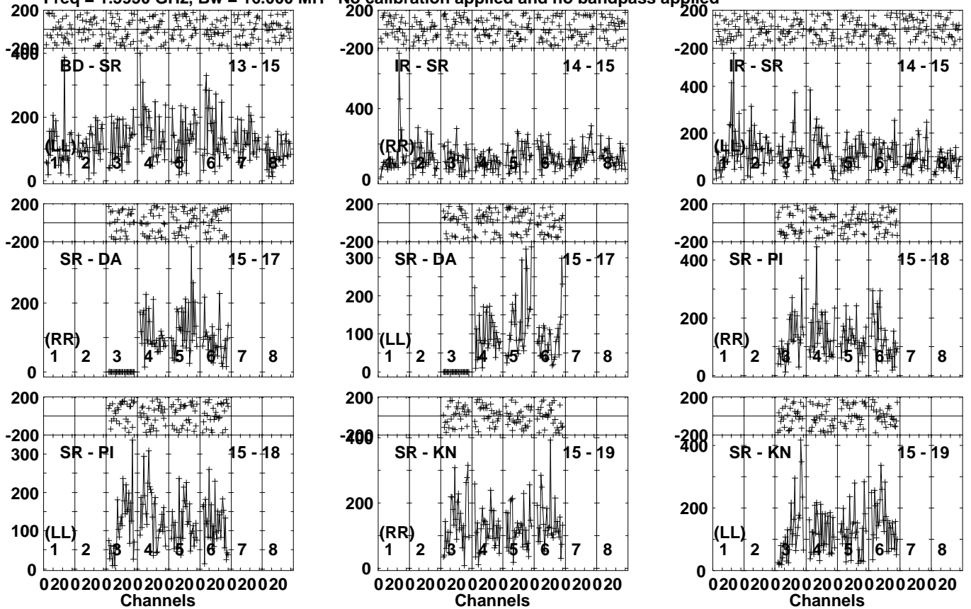
Lower frame: Micro Ampl Jy Top frame: Phas deg Vector averaged cross-power spectrum Several baselines displayed Timerange: 00/04:56:11 to 00/05:04:08
