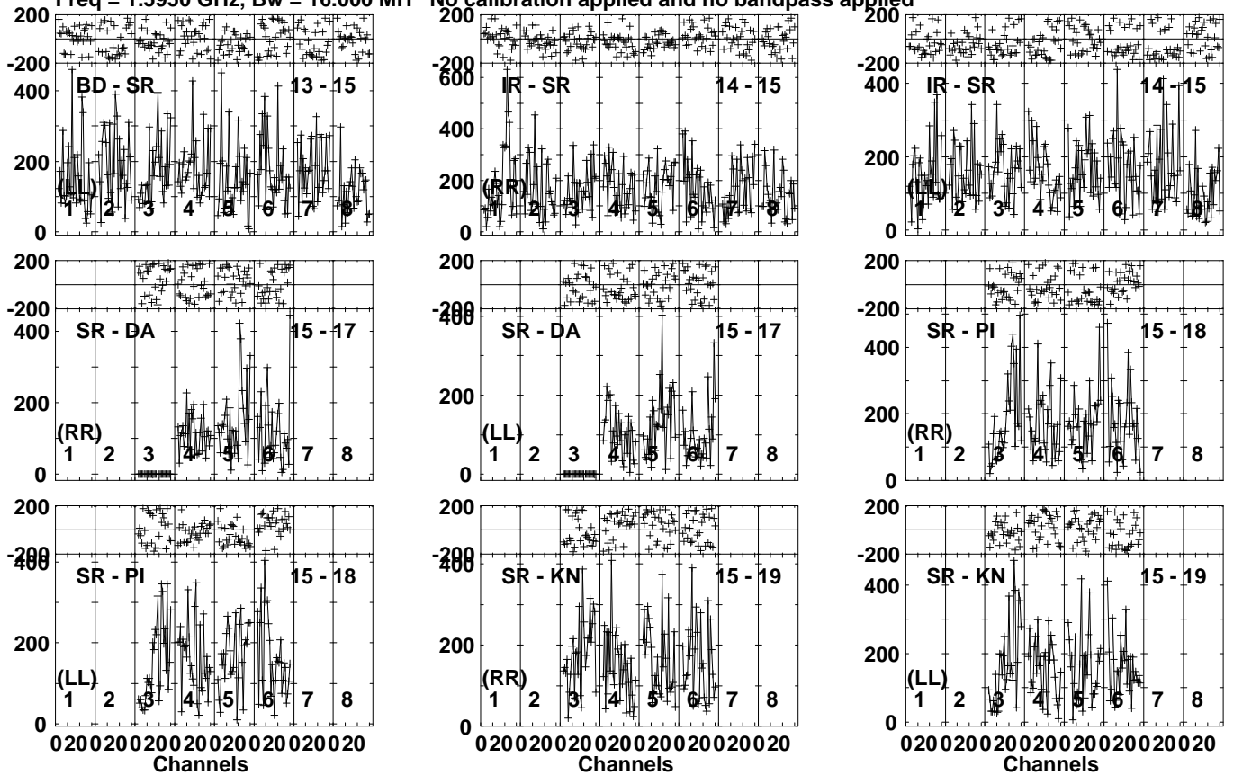
Lower frame: Micro Ampl Jy Top frame: Phas deg Vector averaged cross-power spectrum Several baselines displayed Timerange: 00/04:54:41 to 00/04:56:09
