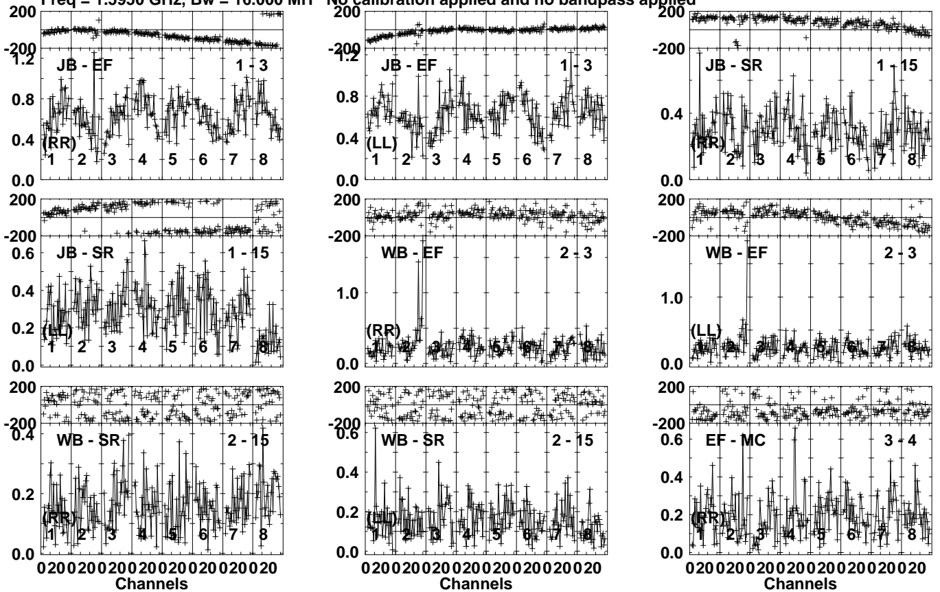
Lower frame: Milli Ampl Jy Top frame: Phas deg Vector averaged cross-power spectrum Several baselines displayed Timerange: 00/07:38:31 to 00/07:40:29
