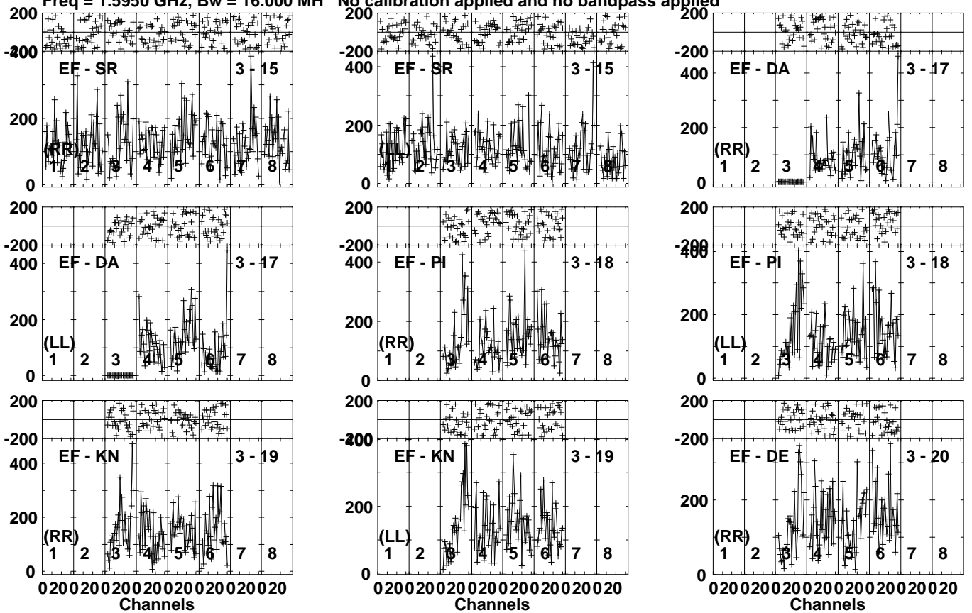
Lower frame: Micro Ampl Jy Top frame: Phas deg Vector averaged cross-power spectrum Several baselines displayed Timerange: 00/07:30:32 to 00/07:38:29
