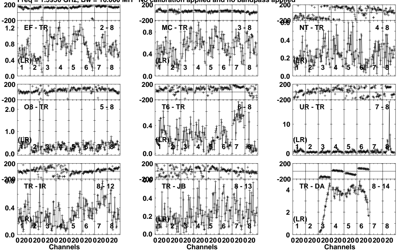
Lower frame: Giga Amp Jy Top frame: Phas deg Vector averaged cross-power spectrum Several baselines displayed Timerange: 00/06:56:56 to 00/06:59:18
