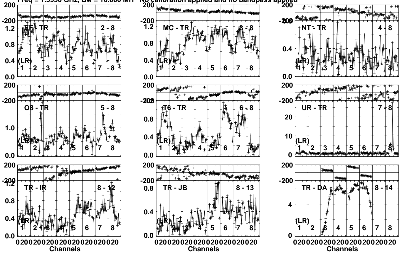
Lower frame: Giga Ampl Jy Top frame: Phas deg Vector averaged cross-power spectrum Several baselines displayed Timerange: 00/07:42:51 to 00/07:45:13
