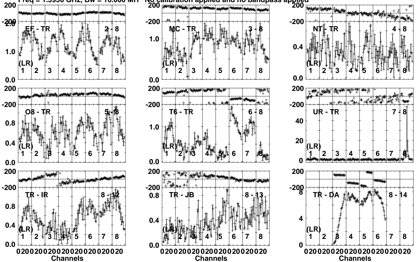
Lower frame: Giga Ampl Jy Top frame: Phas deg Vector averaged cross-power spectrum Several baselines displayed Timerange: 00/07:11:26 to 00/07:13:48
