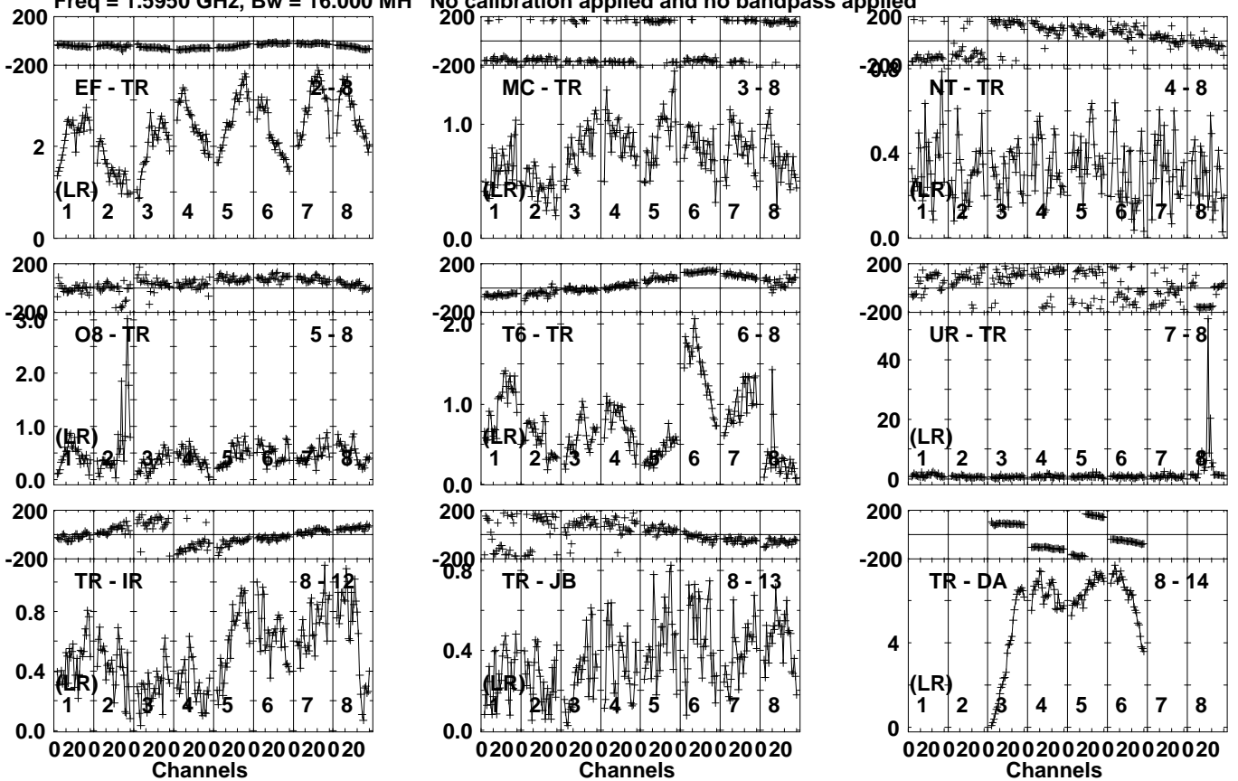
Lower frame: Giga Amp Jy Top frame: Phas deg Vector averaged cross-power spectrum Several baselines displayed Timerange: 00/07:13:51 to 00/07:16:13
