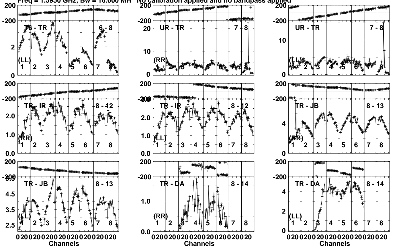
Lower frame: Giga Ampl Jy Top frame: Phas deg Vector averaged cross-power spectrum Several baselines displayed Timerange: 00/06:32:46 to 00/06:35:08
