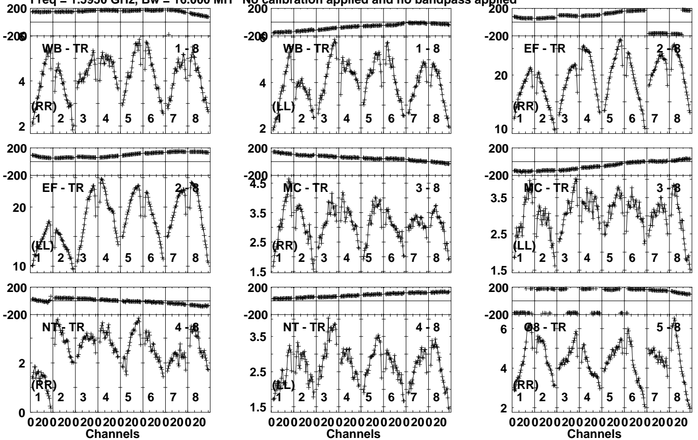
Lower frame: Giga Ampl Jy Top frame: Phas deg Vector averaged cross-power spectrum Several baselines displayed Timerange: 00/04:48:51 to 00/04:51:13
