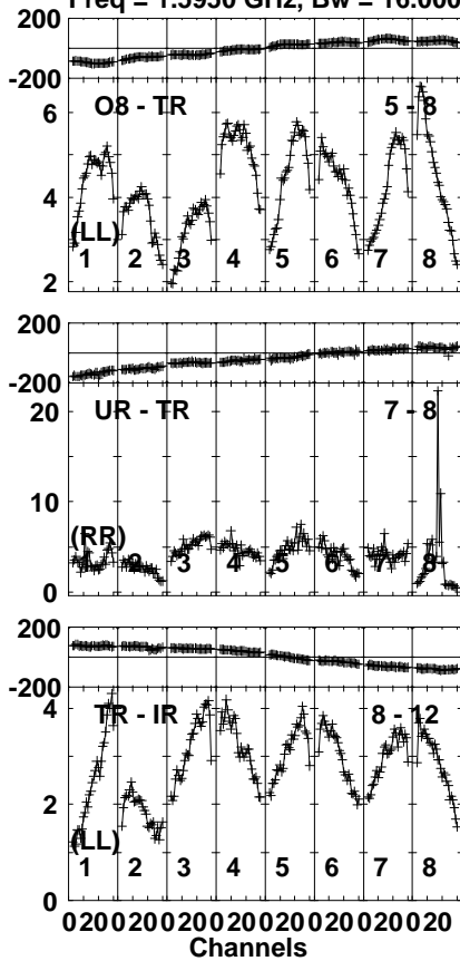
Lower frame: Giga Ampl Jy Top frame: Phas deg Vector averaged cross-power spectrum Several baselines displayed Timerange: 00/05:42:01 to 00/05:44:23
