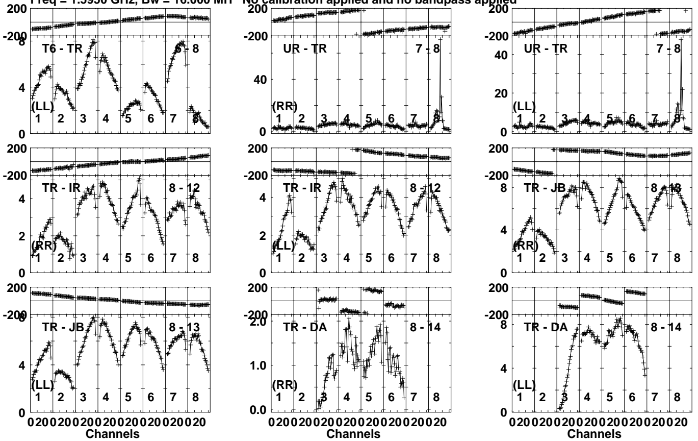
Lower frame: Giga Ampl Jy Top frame: Phas deg Vector averaged cross-power spectrum Several baselines displayed Timerange: 00/06:47:16 to 00/06:49:38
