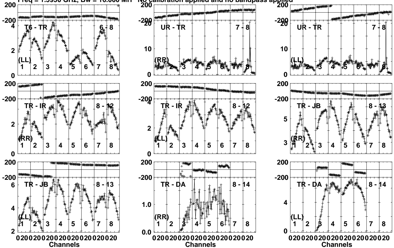
Lower frame: Giga Ampl Jy Top frame: Phas deg Vector averaged cross-power spectrum Several baselines displayed Timerange: 00/05:58:56 to 00/06:01:18
