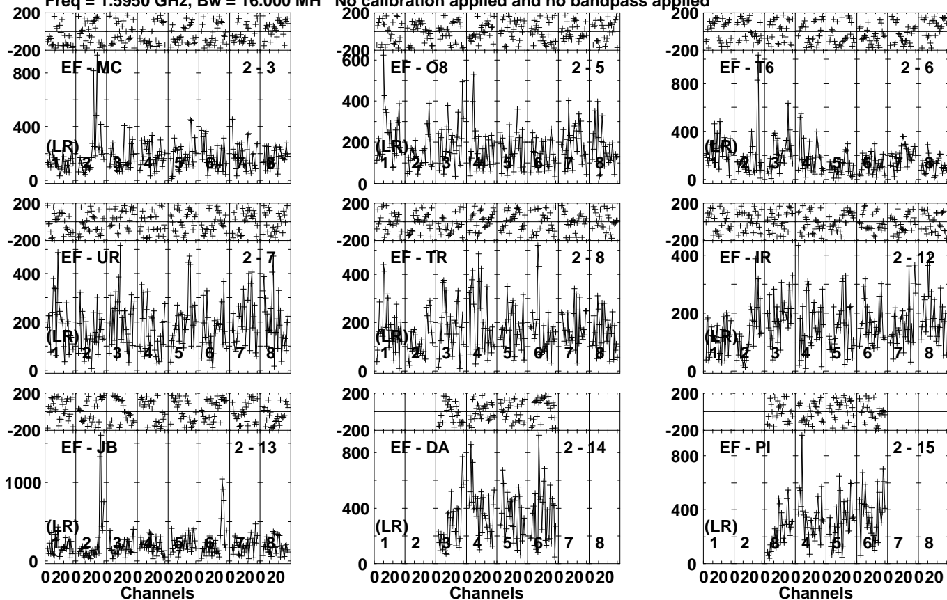
Lower frame: Mega Ampl Jy Top frame: Phas deg Vector averaged cross-power spectrum Several baselines displayed Timerange: 00/06:56:56 to 00/06:59:18
