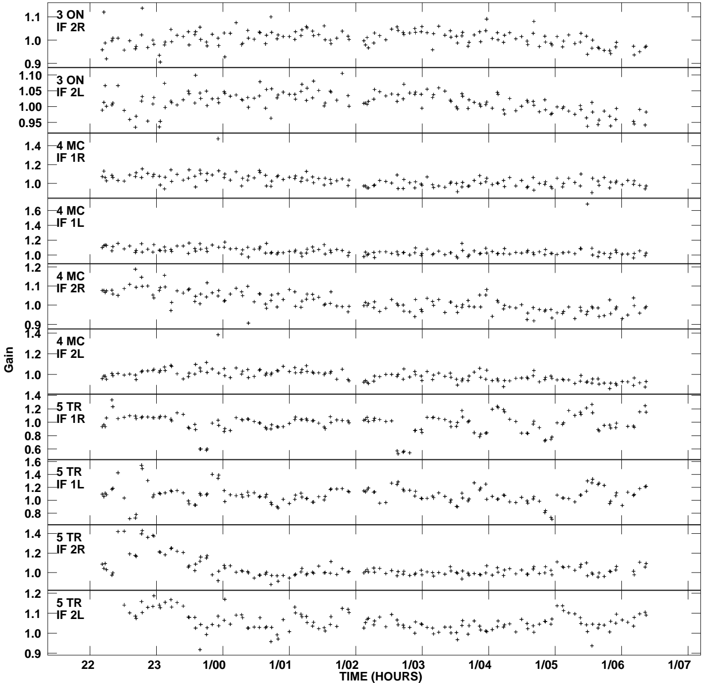
Plot file version 2 created 10-AUG-2010 16:57:24 Gain amp vs UTC time for J2052+1619.MULTI.1 SN 2 Rpol & Lpol IF 1 - 2
