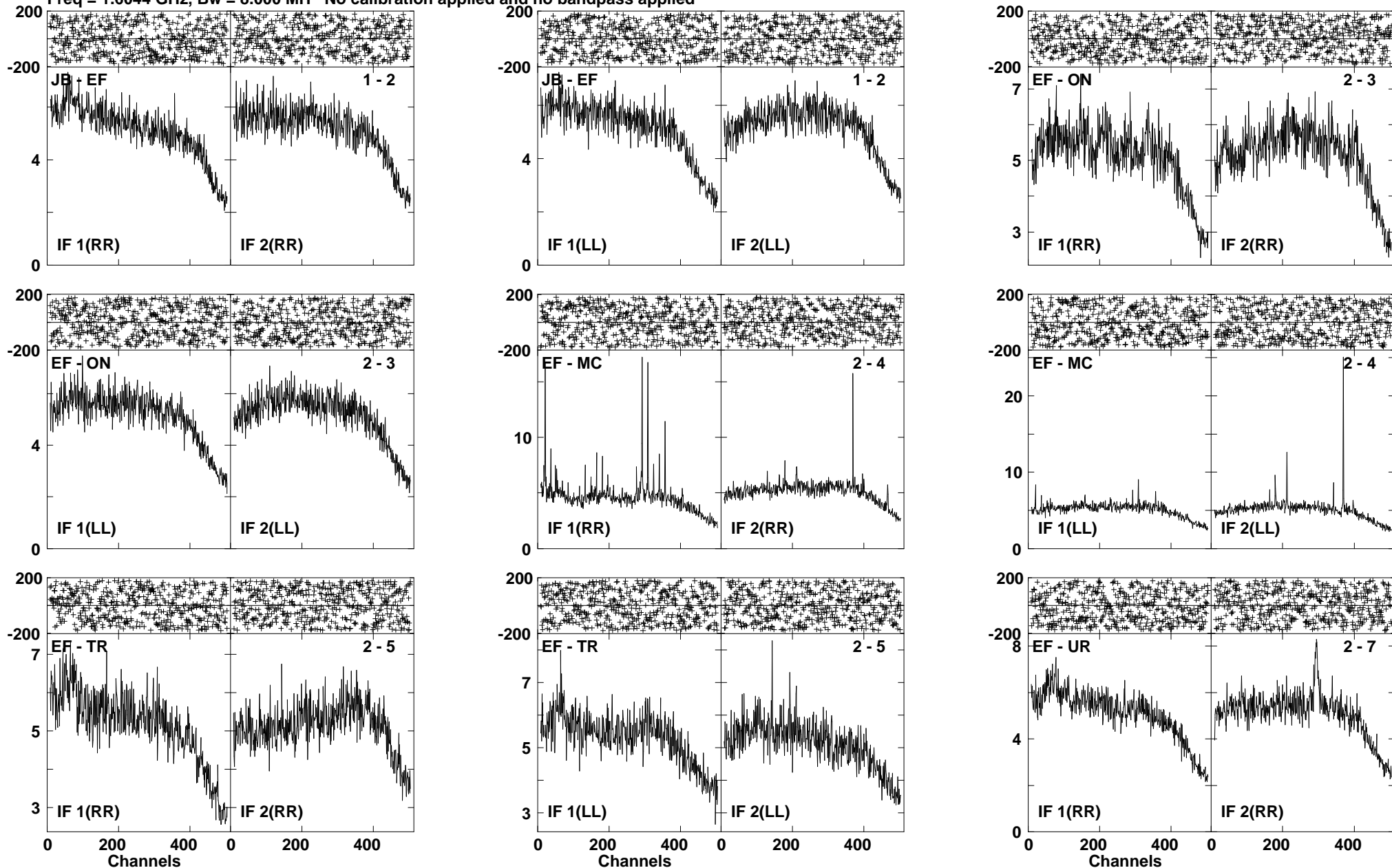
Lower frame: Milli Ampl Jy Top frame: Phas deg Scalar averaged cross-power spectrum Several baselines displayed Timerange: 01/03:21:16 to 01/03:24:44
