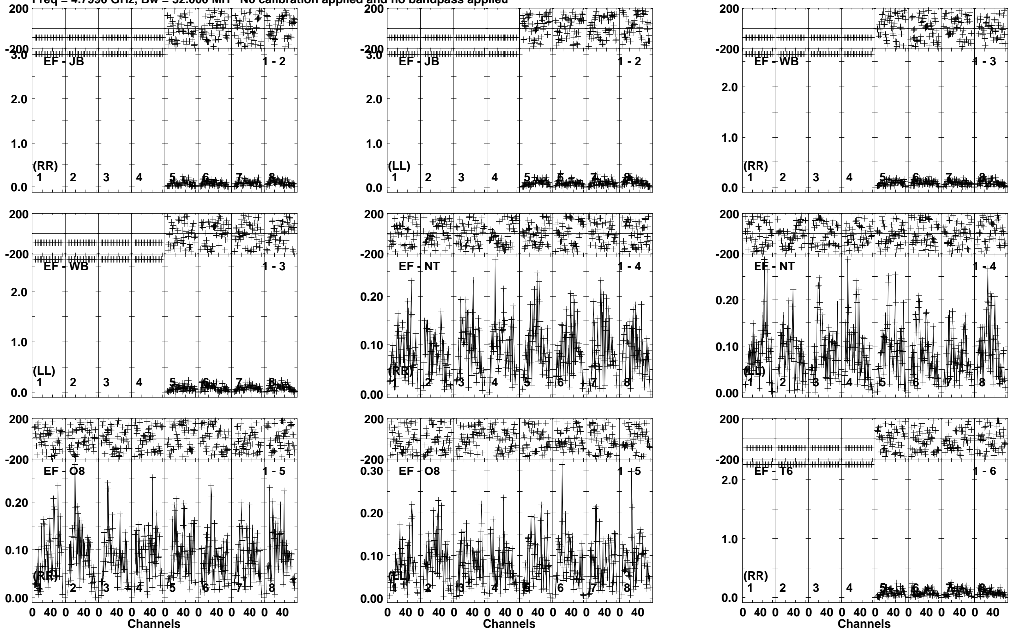
Lower frame: Milli Ampl Jy Top frame: Phas deg Vector averaged cross-power spectrum Baseline: EF (01) - JB (02) Timerange: 00/18:10:31 to 00/18:13:59
