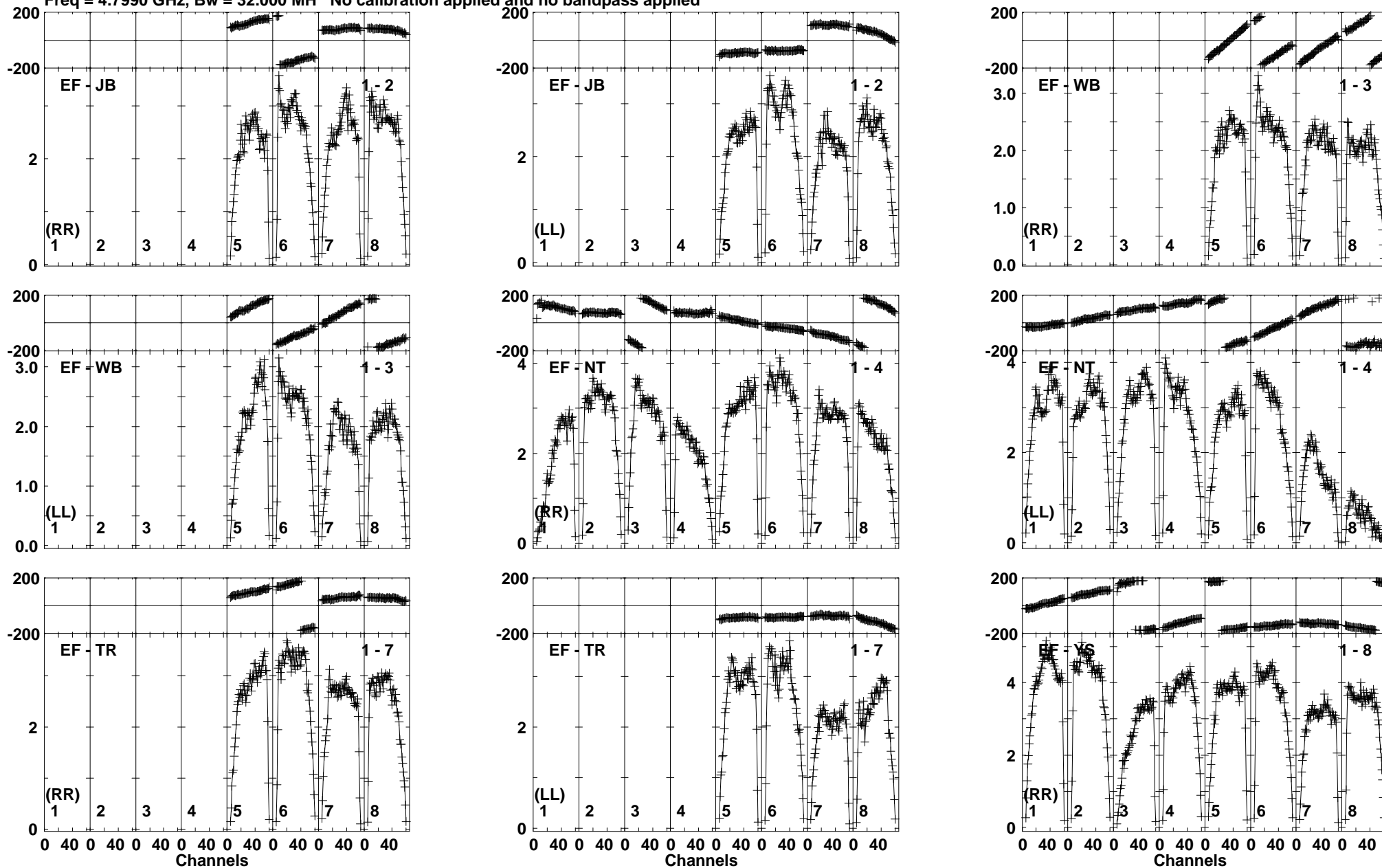
Lower frame: Milli Ampl Jy Top frame: Phas deg Vector averaged cross-power spectrum Baseline: EF (01) - JB (02) Timerange: 00:22:29:01 to 00:22:29:59
