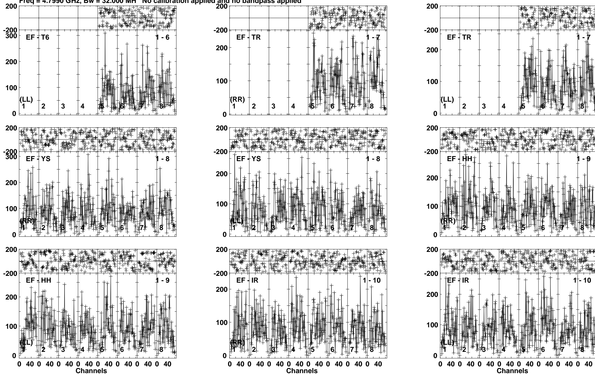
Lower frame: Micro Ampl Jy Top frame: Phas deg Vector averaged cross-power spectrum Baseline: EF (01) - T6 (06) Timerange: 00:18:35:31 to 00:18:38:59
