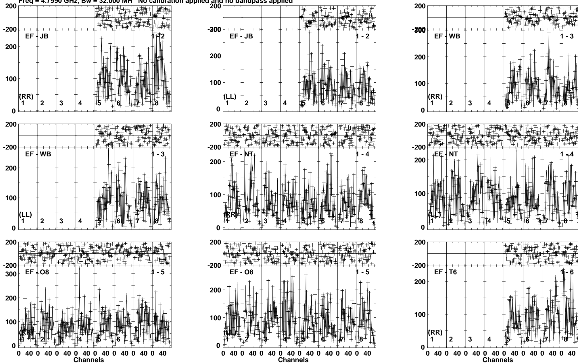
Lower frame: Micro Ampl Jy Top frame: Phas deg Vector averaged cross-power spectrum Baseline: EF (01) - JB (02) Timerange: 00/16:21:01 to 00/16:24:29
