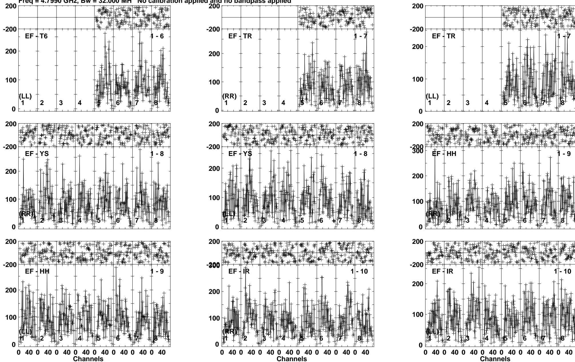
Lower frame: Micro Ampl Jy Top frame: Phas deg Vector averaged cross-power spectrum Baseline: EF (01) - T6 (06) Timerange: 00/18:20:31 to 00/18:23:59
