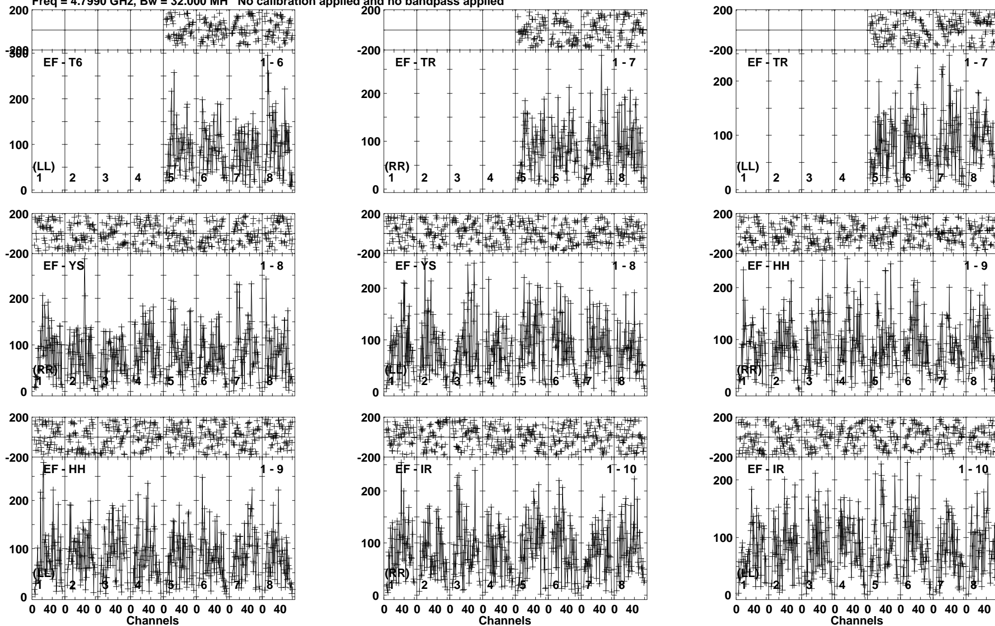
Lower frame: Micro Ampl Jy Top frame: Phas deg Vector averaged cross-power spectrum Baseline: EF (01) - T6 (06) Timerange: 00/19:30:31 to 00/19:33:59
