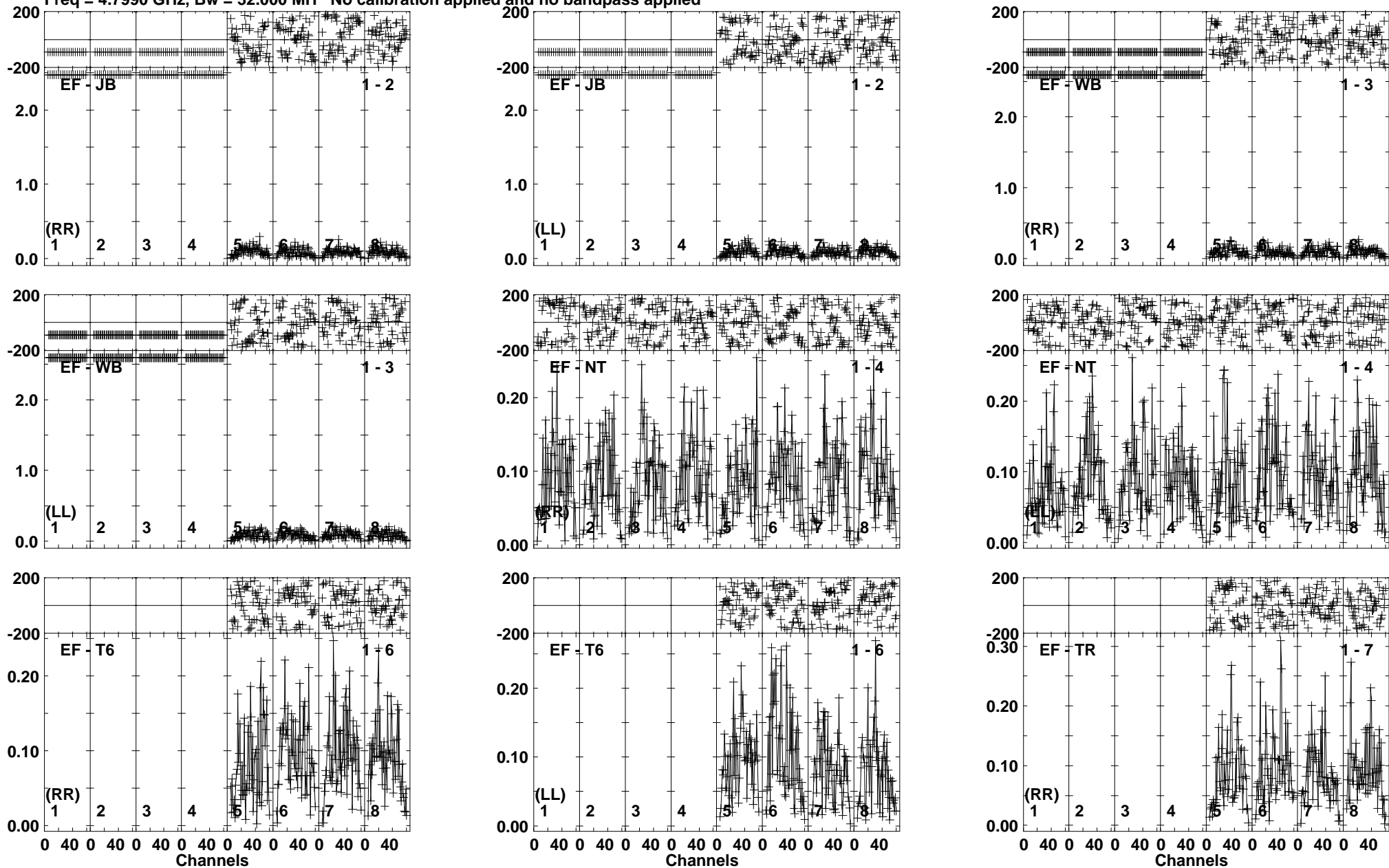
Lower frame: Milli Ampl Jy Top frame: Phas deg Vector averaged cross-power spectrum Baseline: EF (01) - JB (02) Timerange: 00/22:09:31 to 00/22:12:59
