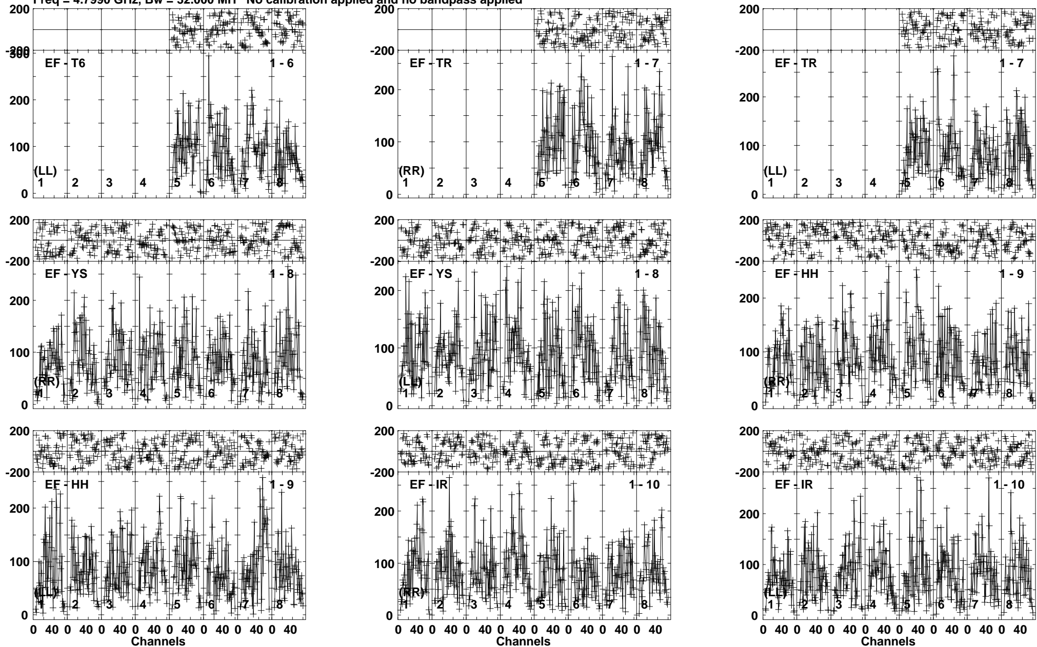
Lower frame: Micro Ampl Jy Top frame: Phas deg Vector averaged cross-power spectrum Baseline: EF (01) - T6 (06) Timerange: 00/16:41:01 to 00/16:44:29
