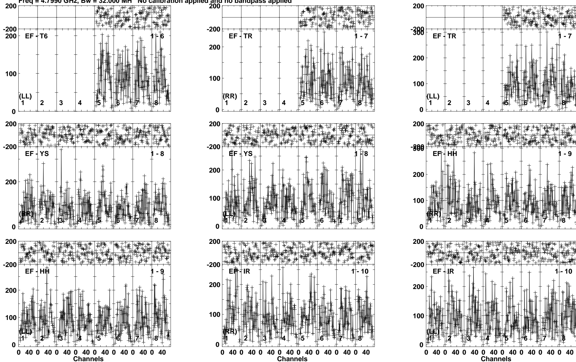
Lower frame: Micro Ampl Jy Top frame: Phas deg Vector averaged cross-power spectrum Baseline: EF (01) - T6 (06) Timerange: 00/20:27:51 to 00/20:31:19
