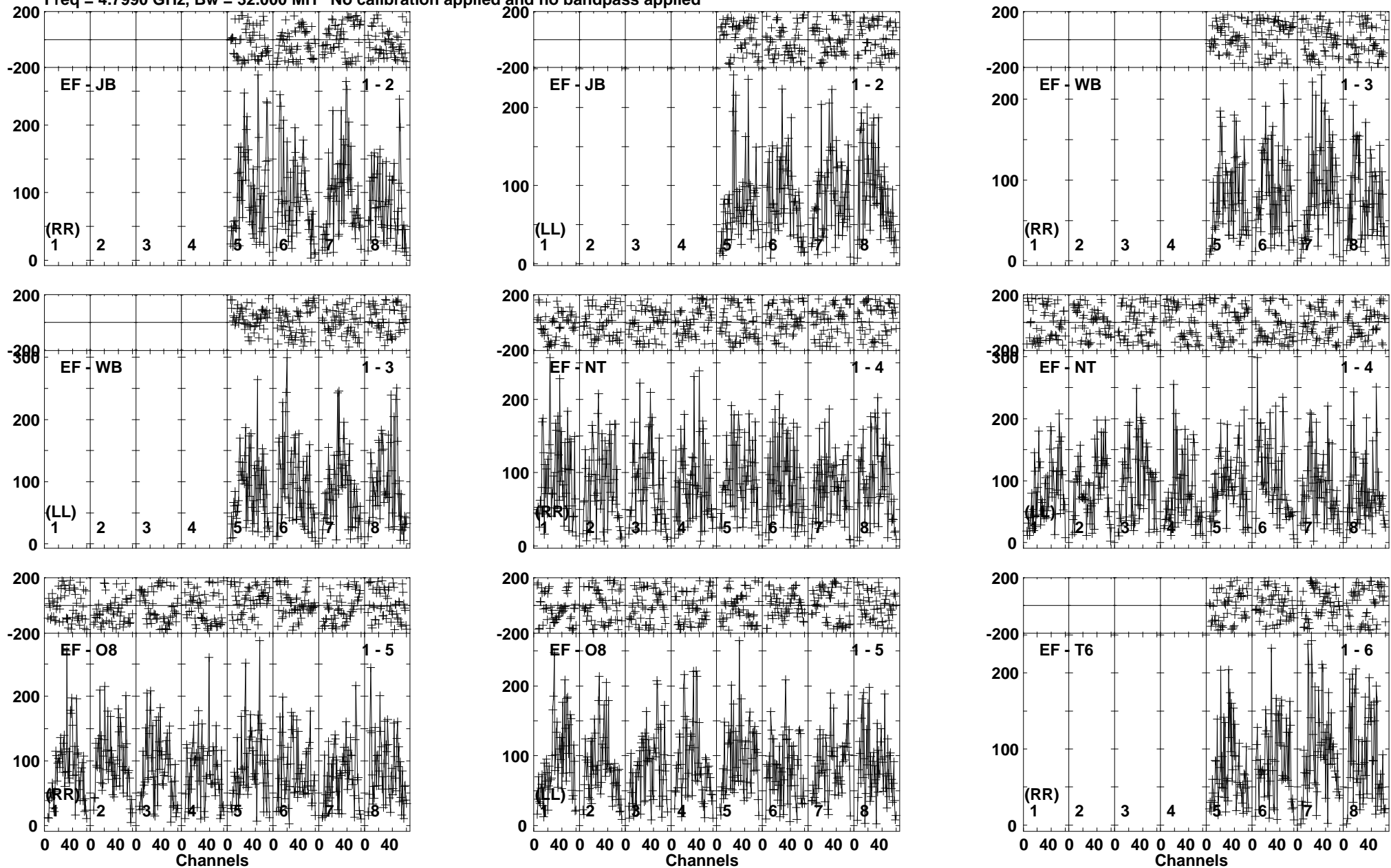
Lower frame: Micro Ampl Jy Top frame: Phas deg Vector averaged cross-power spectrum Baseline: EF (01) - JB (02) Timerange: 00/20:22:51 to 00/20:26:19
