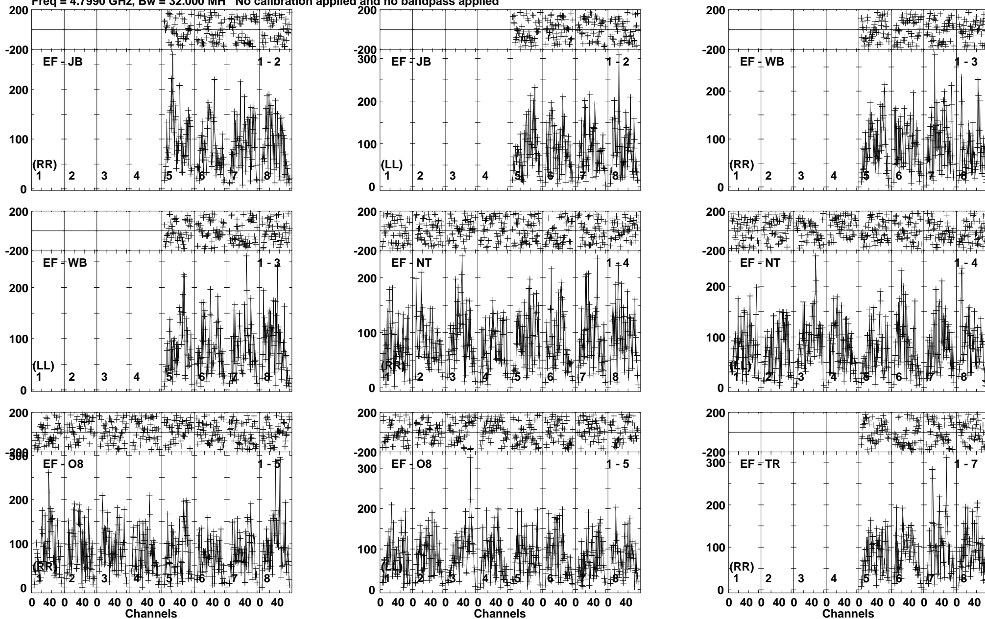
Lower frame: Micro Ampl Jy Top frame: Phas deg Vector averaged cross-power spectrum Baseline: EF (01) - JB (02) Timerange: 00/15:31:32 to 00/15:34:58
