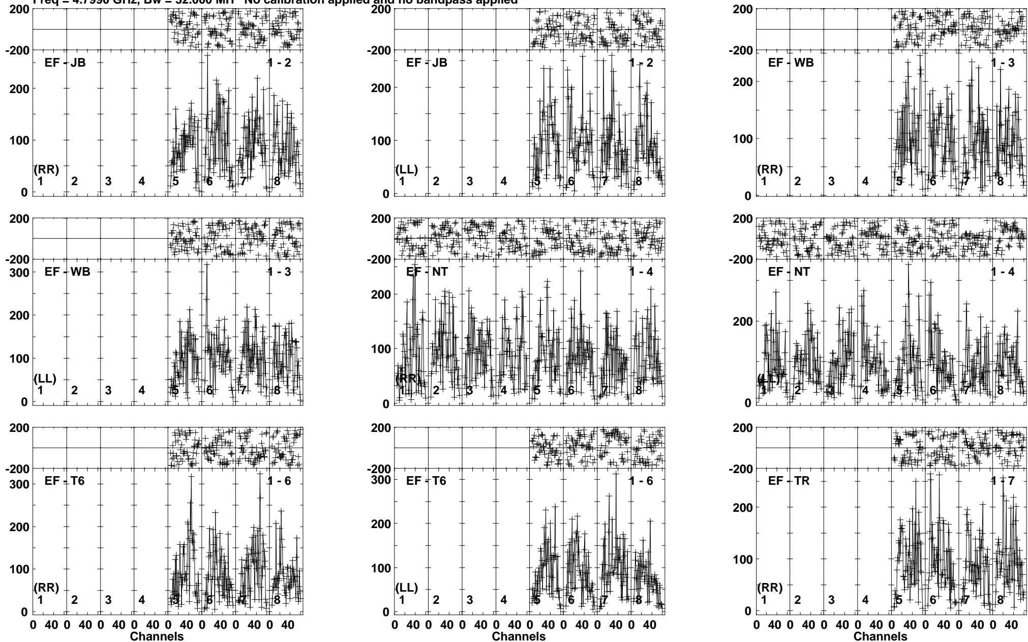
Lower frame: Micro Ampl Jy Top frame: Phas deg Vector averaged cross-power spectrum Baseline: EF (01) - JB (02) Timerange: 00/21:23:51 to 00/21:27:19
