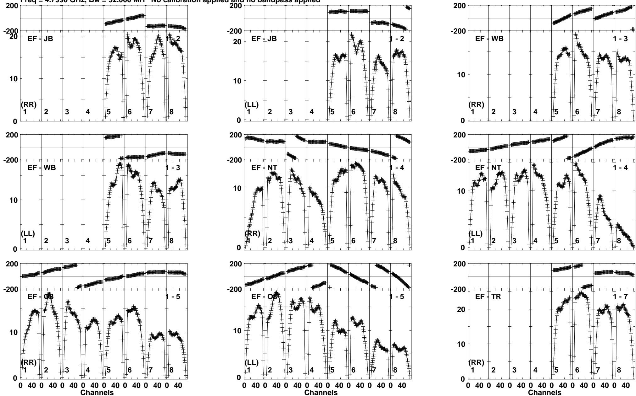
Lower frame: Milli Ampl Jy Top frame: Phas deg Vector averaged cross-power spectrum Baseline: EF (01) - JB (02) Timerange: 00/14:00:32 to 00/14:01:28
