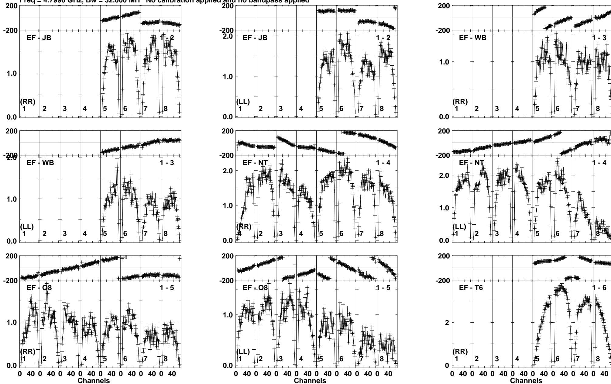
Lower frame: Milli Ampl Jy Top frame: Phas deg Vector averaged cross-power spectrum Baseline: EF (01) - JB (02) Timerange: 00:16:10:01 to 00:16:10:59
