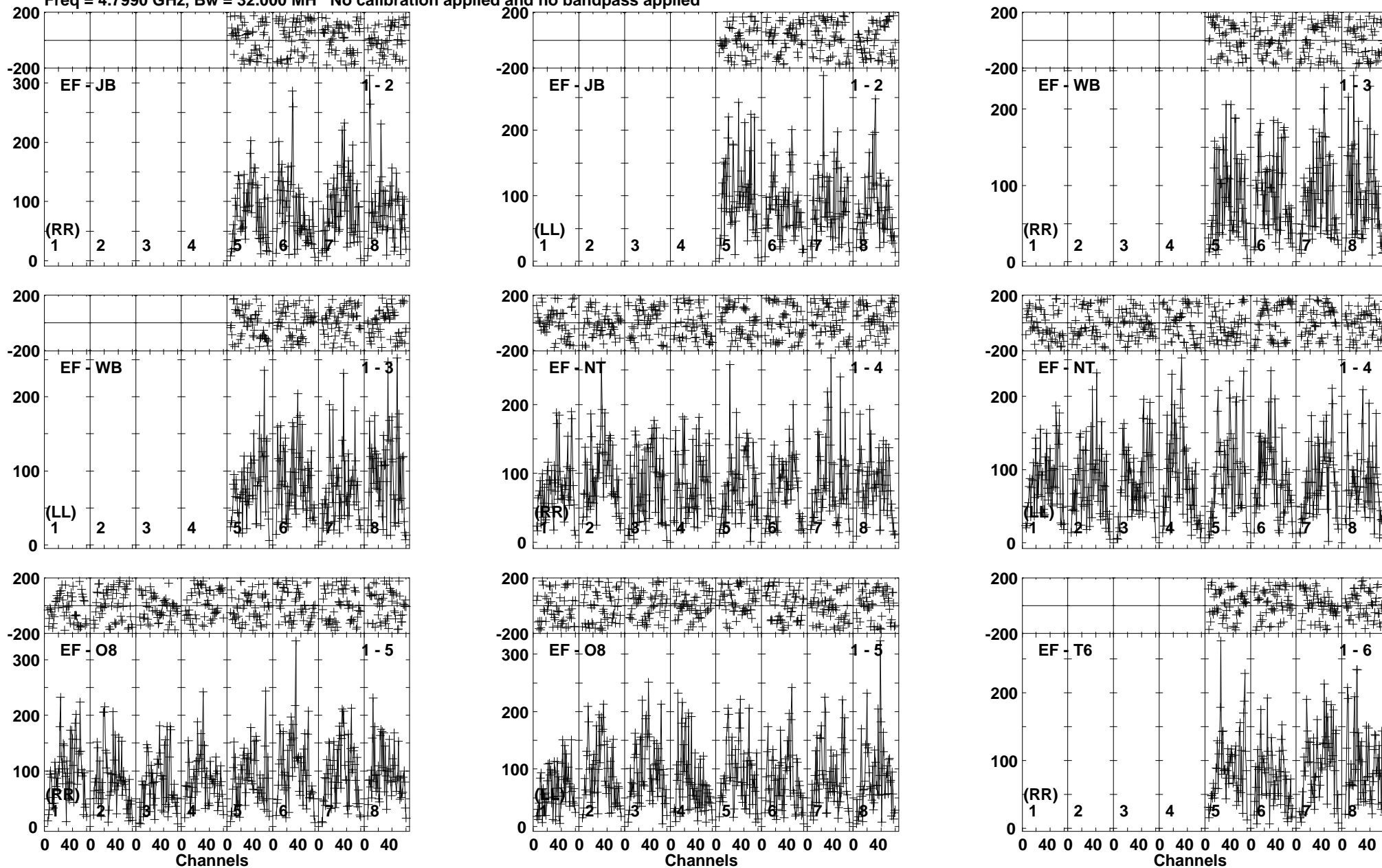
Lower frame: Micro Ampl Jy Top frame: Phas deg Vector averaged cross-power spectrum Baseline: EF (01) - JB (02) Timerange: 00/20:10:31 to 00/20:13:59
