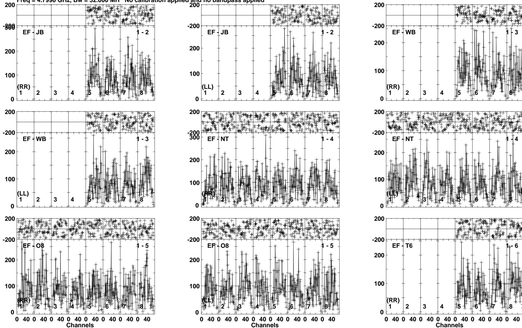
Lower frame: Micro Ampl Jy Top frame: Phas deg Vector averaged cross-power spectrum Baseline: EF (01) - JB (02) Timerange: 00/17:46:01 to 00/17:49:29
