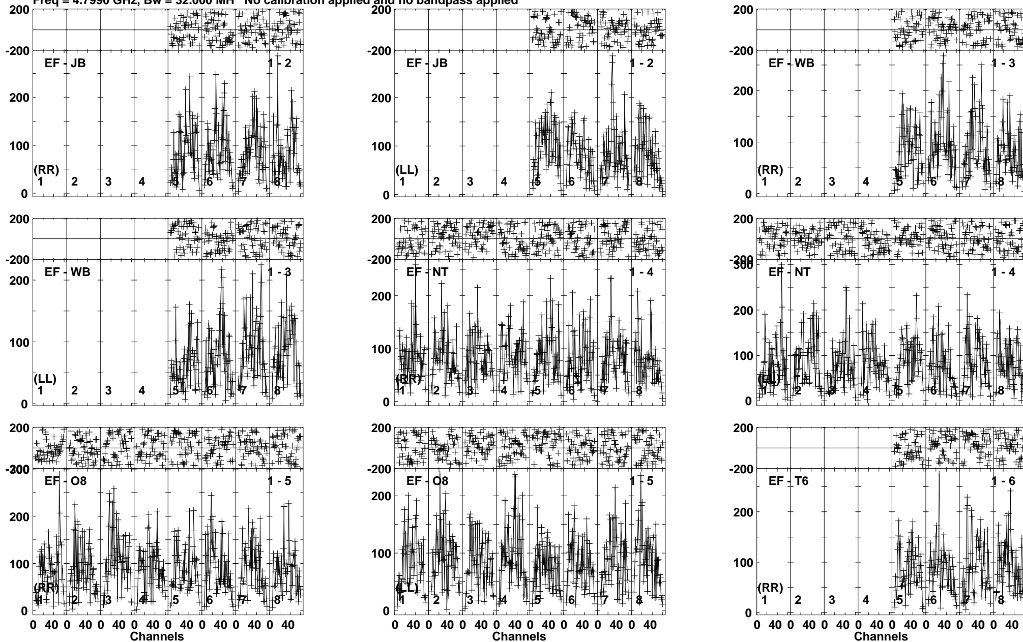
Lower frame: Micro Ampl Jy Top frame: Phas deg Vector averaged cross-power spectrum Baseline: EF (01) - JB (02) Timerange: 00/18:20:31 to 00/18:23:59
