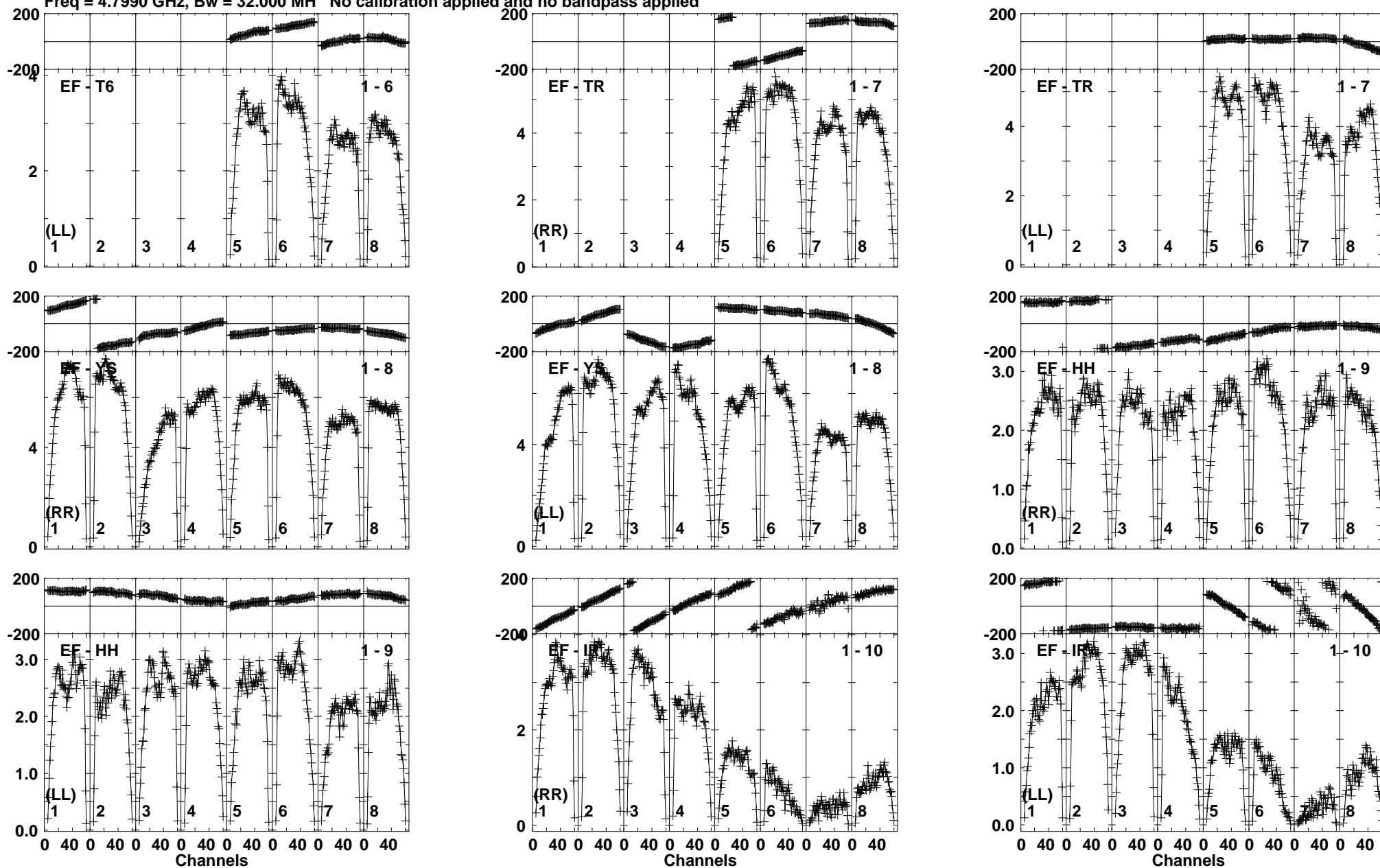
Lower frame: Milli Ampl Jy Top frame: Phas deg Vector averaged cross-power spectrum Baseline: EF (01) - T6 (06) Timerange: 00/19:19:01 to 00/19:20:29
