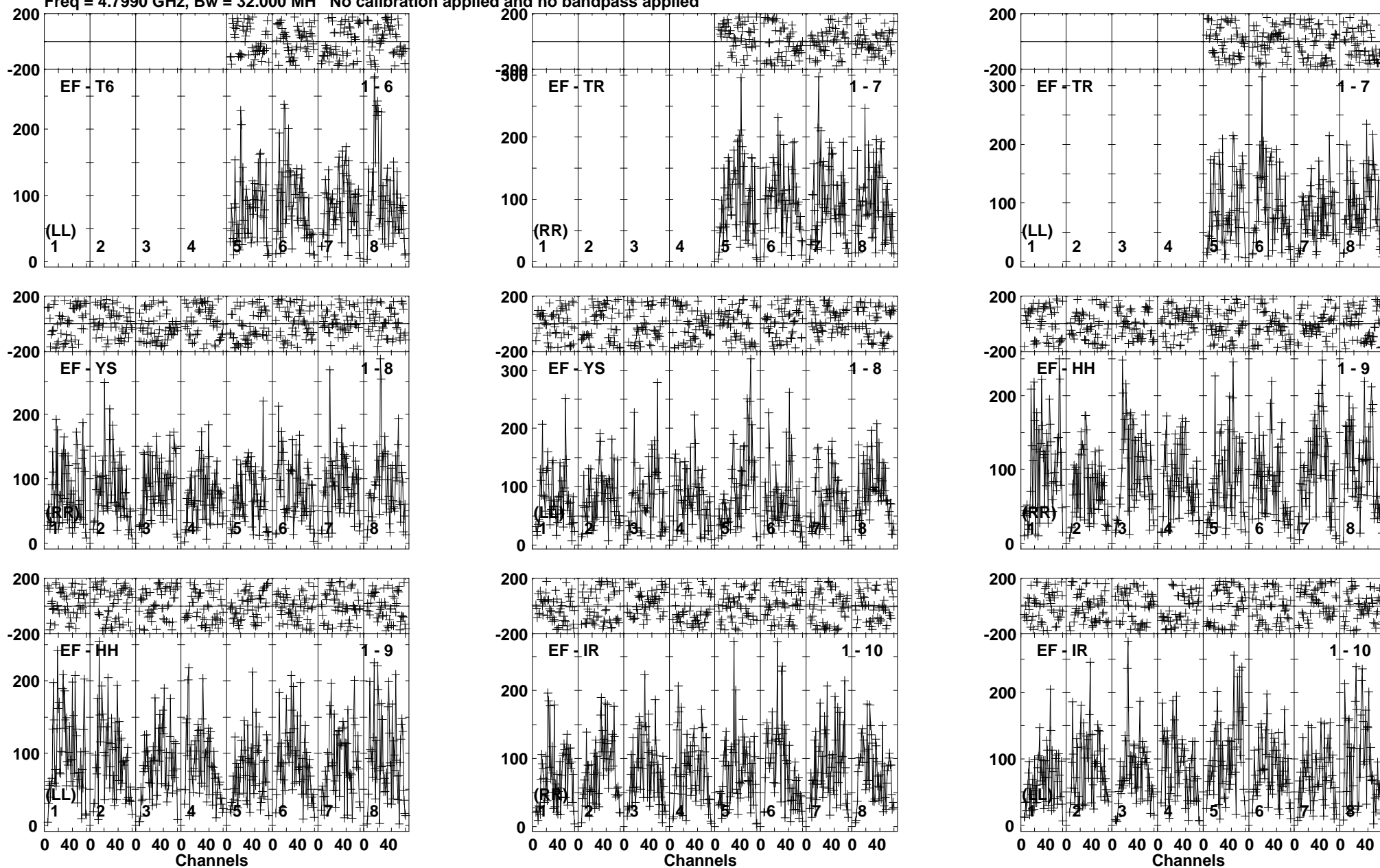
Lower frame: Micro Ampl Jy Top frame: Phas deg Vector averaged cross-power spectrum Baseline: EF (01) - T6 (06) Timerange: 00/19:35:31 to 00/19:38:59
