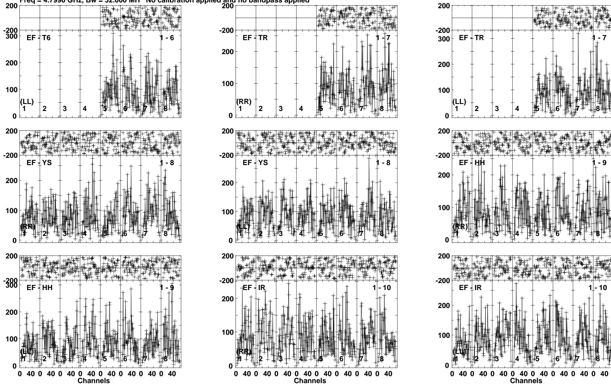
Lower frame: Micro Ampl Jy Top frame: Phas deg Vector averaged cross-power spectrum Baseline: EF (01) - T6 (06) Timerange: 00/16:21:01 to 00/16:24:29
