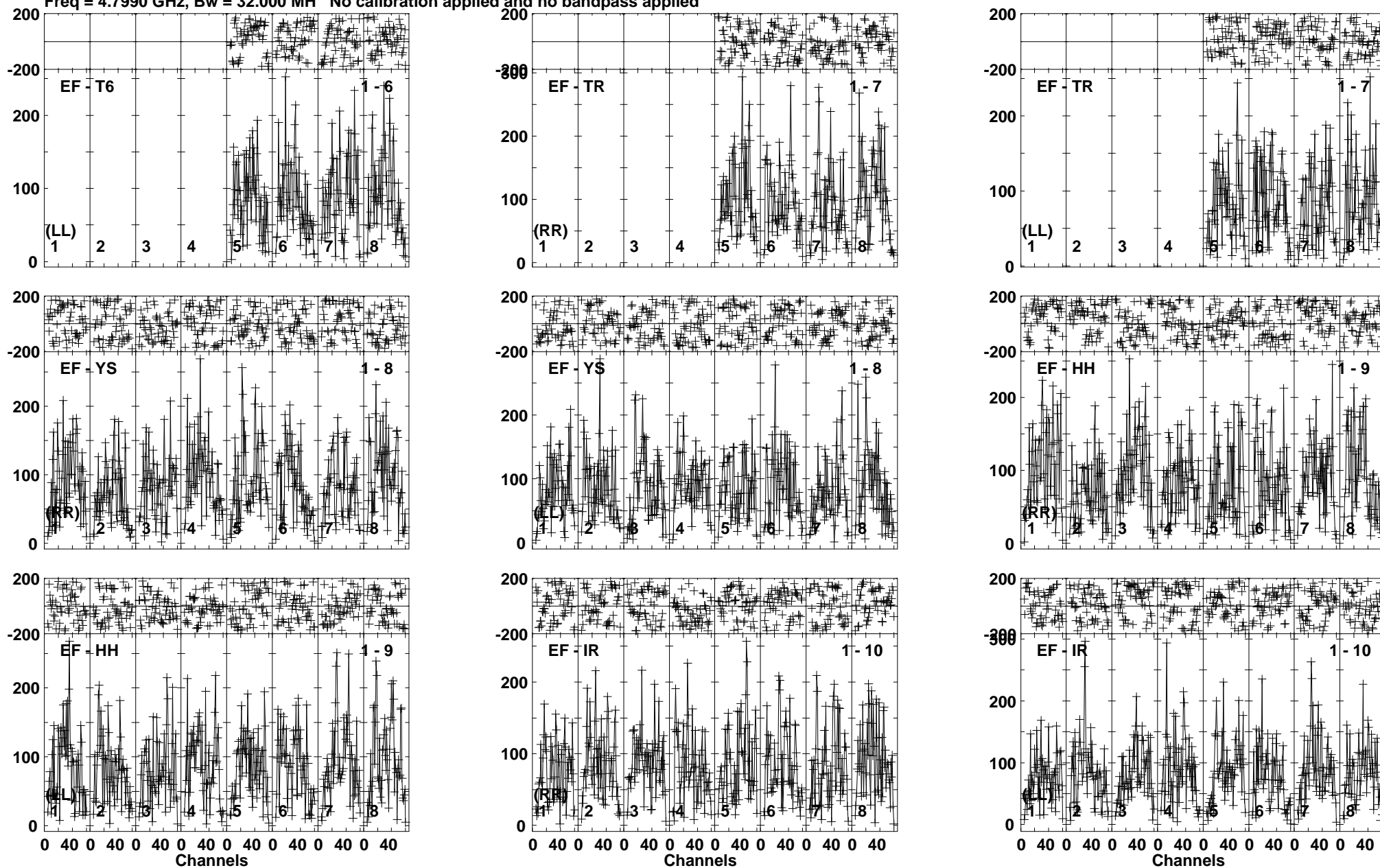
Lower frame: Micro Ampl Jy Top frame: Phas deg Vector averaged cross-power spectrum Baseline: EF (01) - T6 (06) Timerange: 00/16:06:01 to 00/16:09:29
