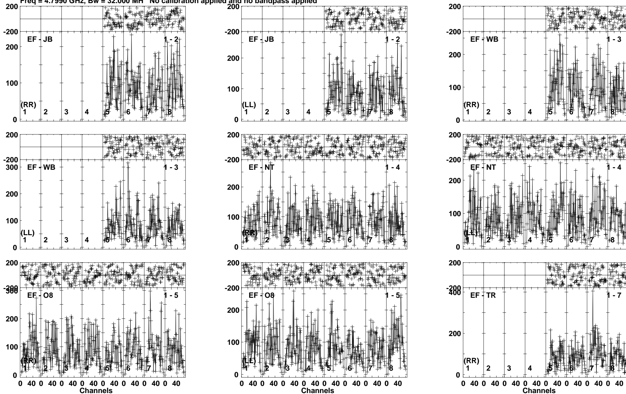
Lower frame: Micro Ampl Jy Top frame: Phas deg Vector averaged cross-power spectrum Baseline: EF (01) - JB (02) Timerange: 00/14:31:32 to 00/14:34:58
