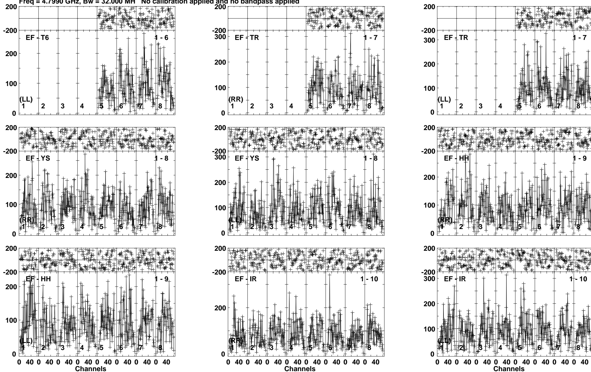
Lower frame: Micro Ampl Jy Top frame: Phas deg Vector averaged cross-power spectrum Baseline: EF (01) - T6 (06) Timerange: 00/20:38:01 to 00/20:41:29
