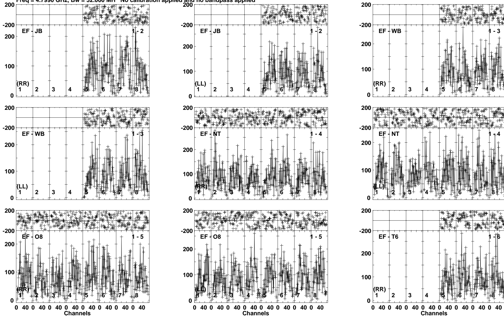
Lower frame: Micro Ampl Jy Top frame: Phas deg Vector averaged cross-power spectrum Baseline: EF (01) - JB (02) Timerange: 00:17:01:01 to 00:17:04:29
