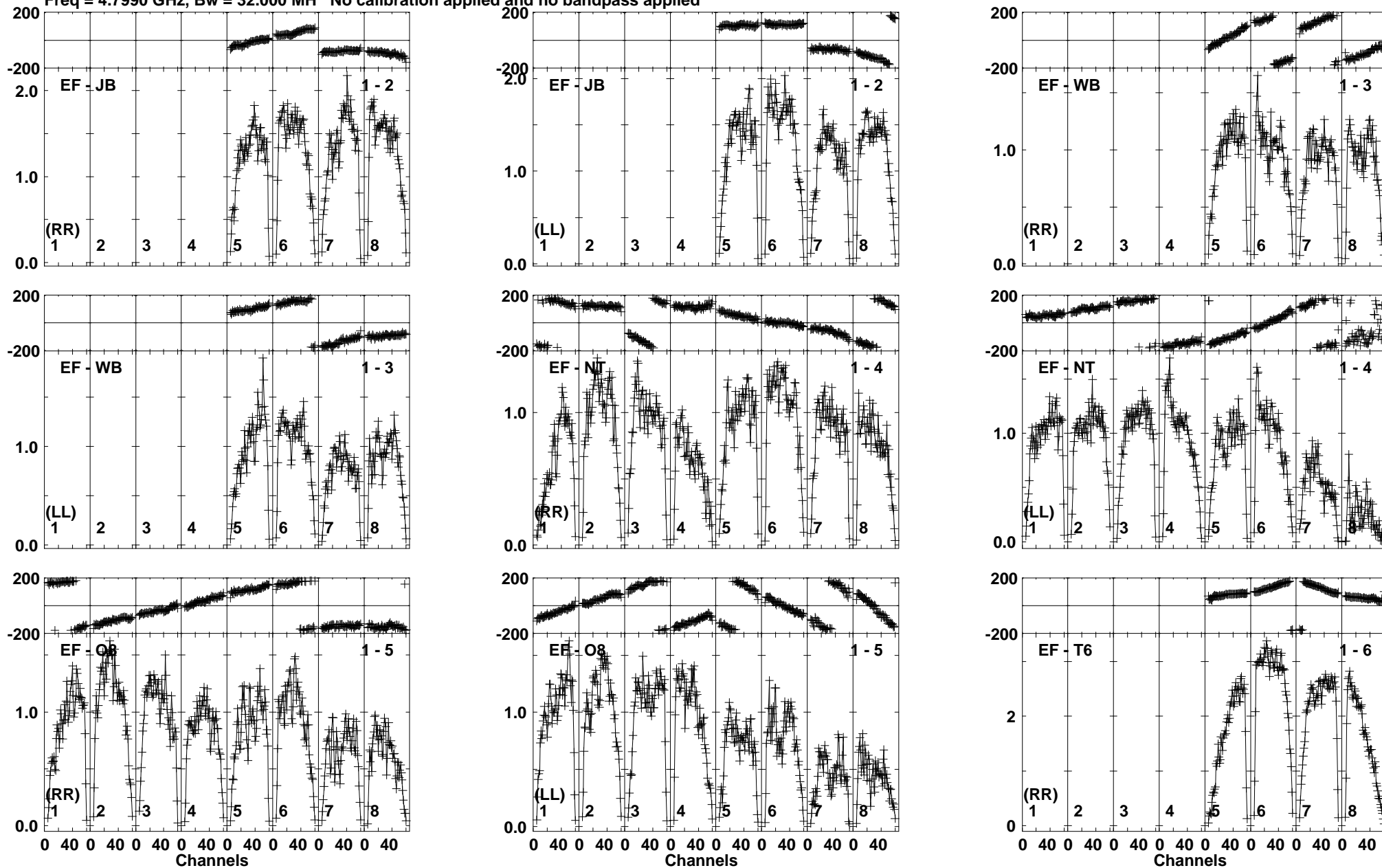
Lower frame: Milli Ampl Jy Top frame: Phas deg Vector averaged cross-power spectrum Baseline: EF (01) - JB (02) Timerange: 00/16:14:31 to 00/16:15:59
