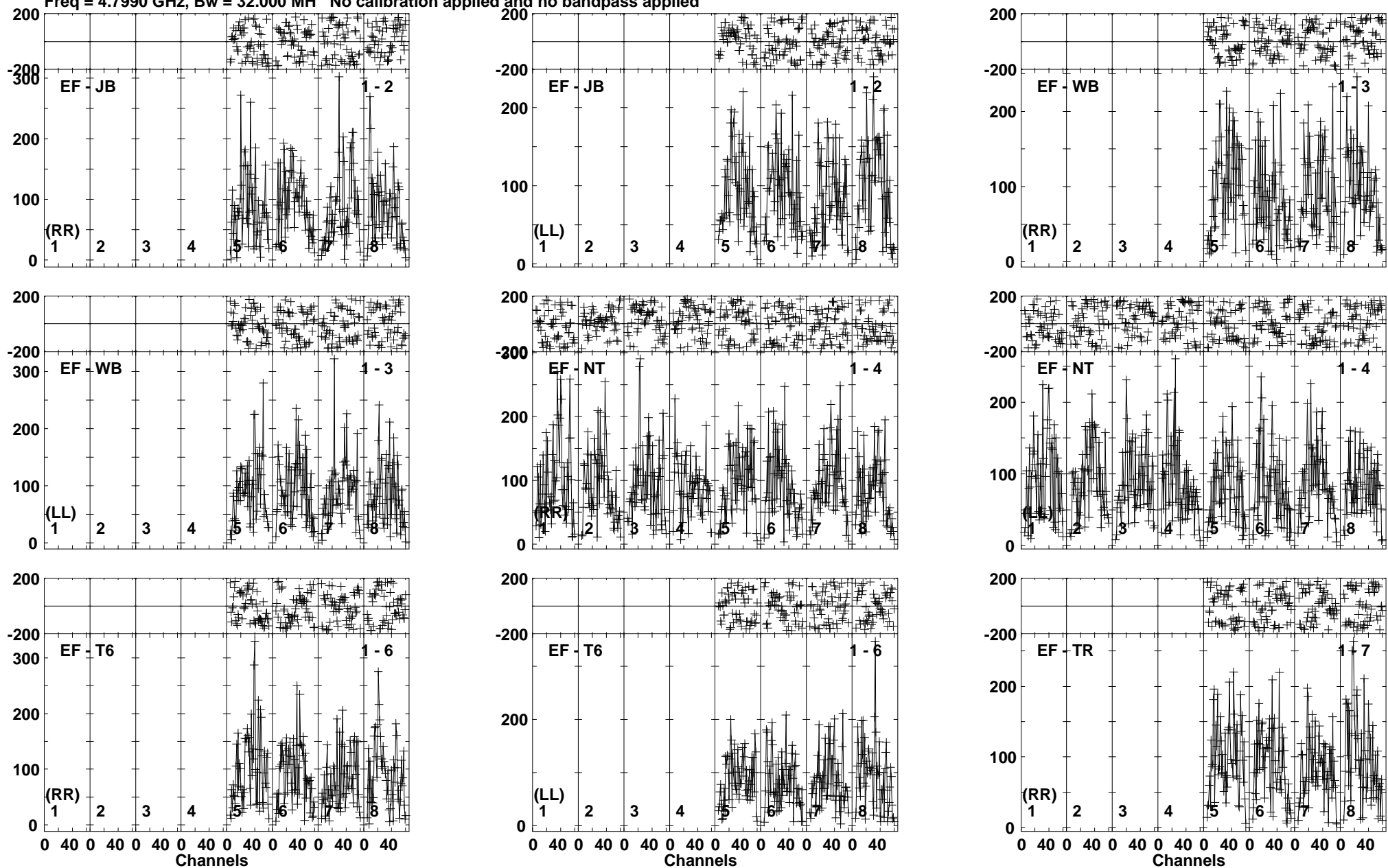
Lower frame: Micro Ampl Jy Top frame: Phas deg Vector averaged cross-power spectrum Baseline: EF (01) - JB (02) Timerange: 00/21:03:31 to 00/21:06:59
