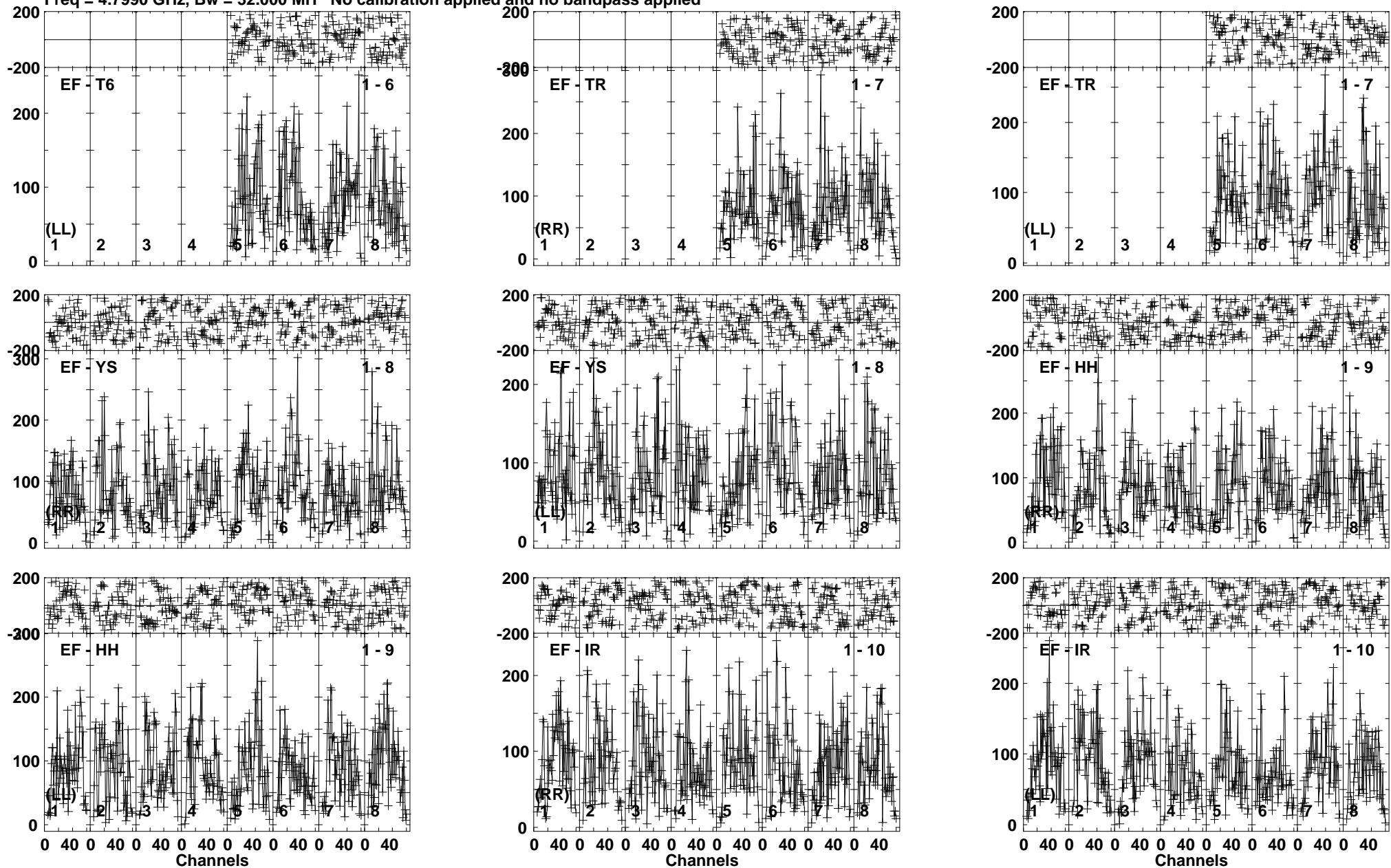
Lower frame: Micro Ampl Jy Top frame: Phas deg Vector averaged cross-power spectrum Baseline: EF (01) - T6 (06) Timerange: 00/18:25:31 to 00/18:28:59
