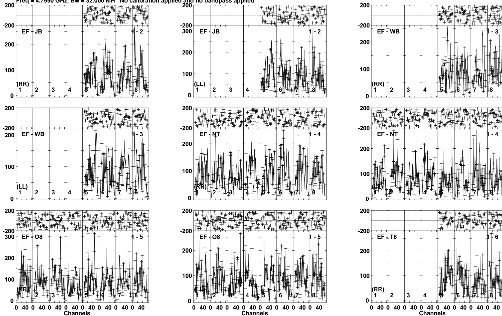
Lower frame: Micro Ampl Jy Top frame: Phas deg Vector averaged cross-power spectrum Baseline: EF (01) - JB (02) Timerange: 00/17:36:01 to 00/17:39:29
