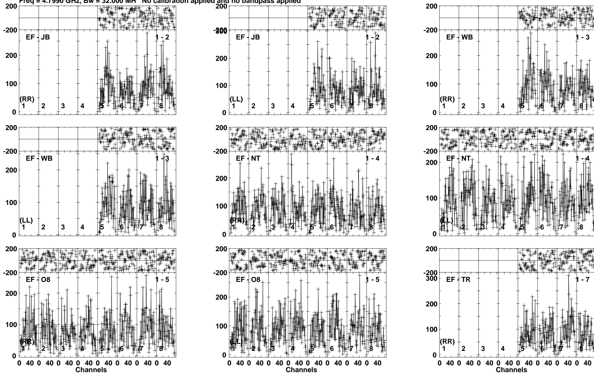
Lower frame: Micro Ampl Jy Top frame: Phas deg Vector averaged cross-power spectrum Baseline: EF (01) - JB (02) Timerange: 00/13:46:32 to 00/13:49:58
