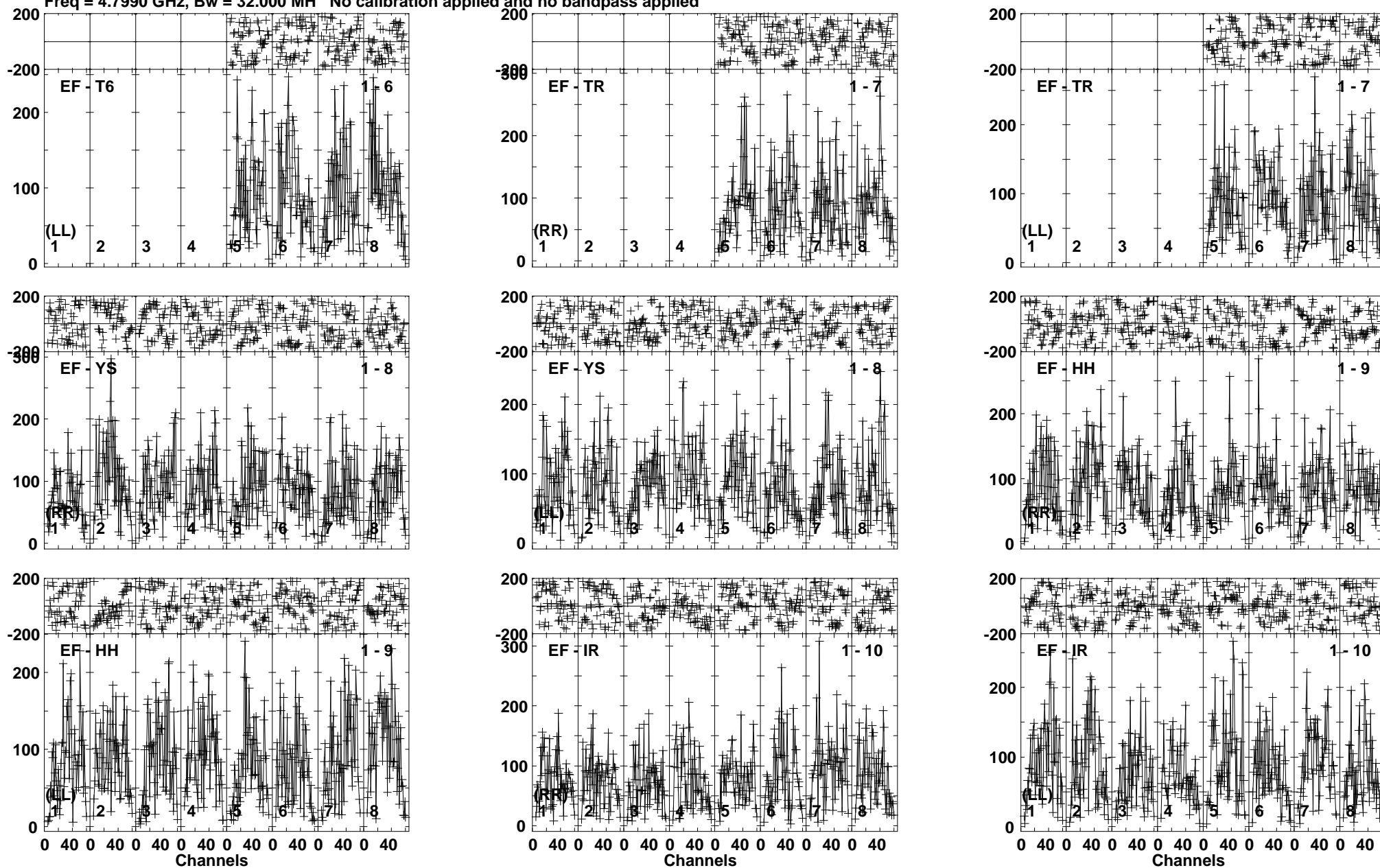
Lower frame: Micro Ampl Jy Top frame: Phas deg Vector averaged cross-power spectrum Baseline: EF (01) - T6 (06) Timerange: 00/16:26:01 to 00/16:29:29
