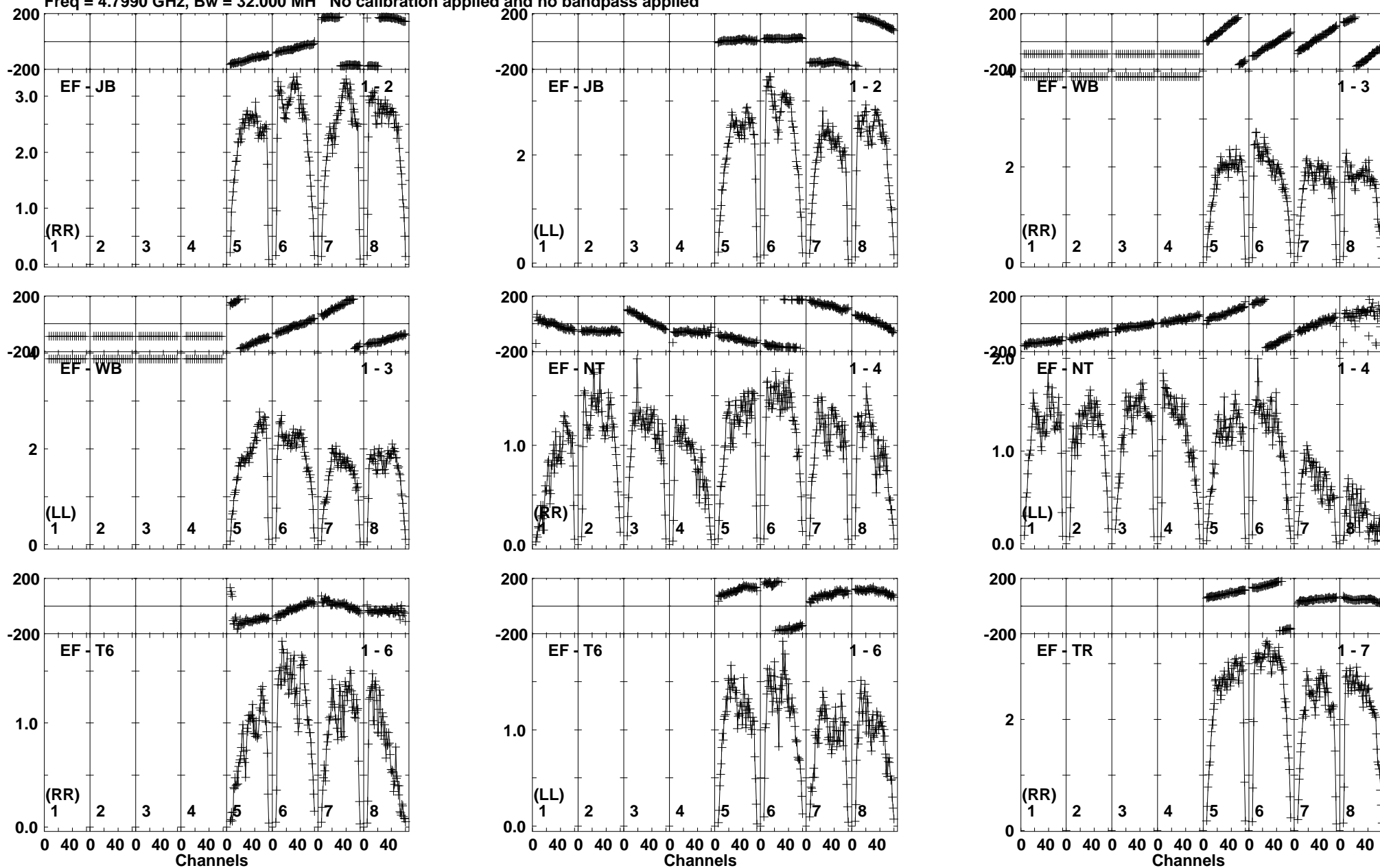
Lower frame: Milli Ampl Jy Top frame: Phas deg Vector averaged cross-power spectrum Baseline: EF (01) - JB (02) Timerange: 00/21:22:51 to 00/21:23:49
