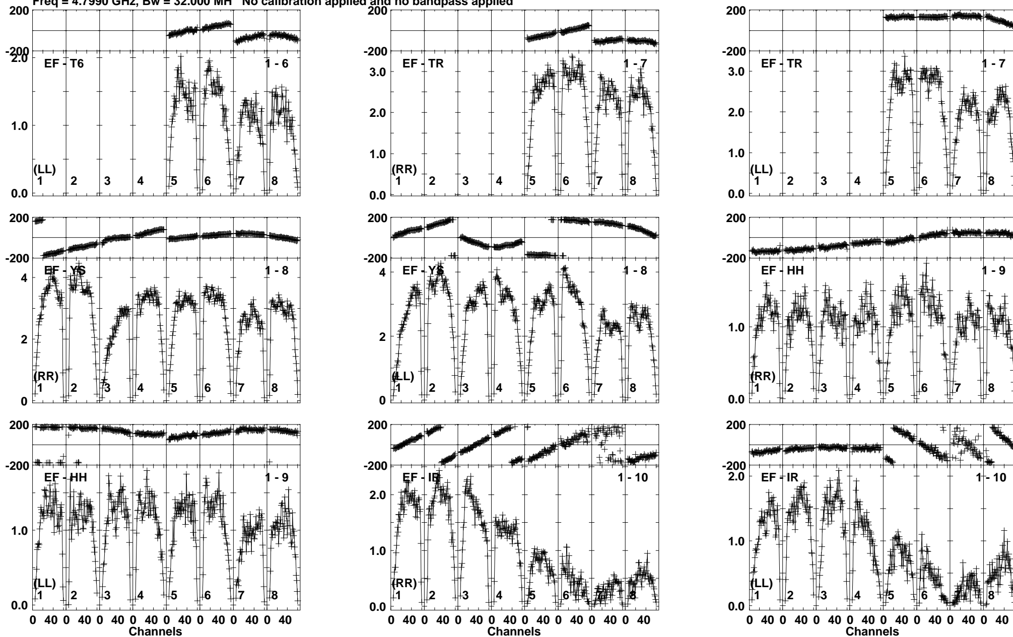
Lower frame: Milli Ampl Jy Top frame: Phas deg Vector averaged cross-power spectrum Baseline: EF (01) - T6 (06) Timerange: 00/20:26:21 to 00/20:27:49
