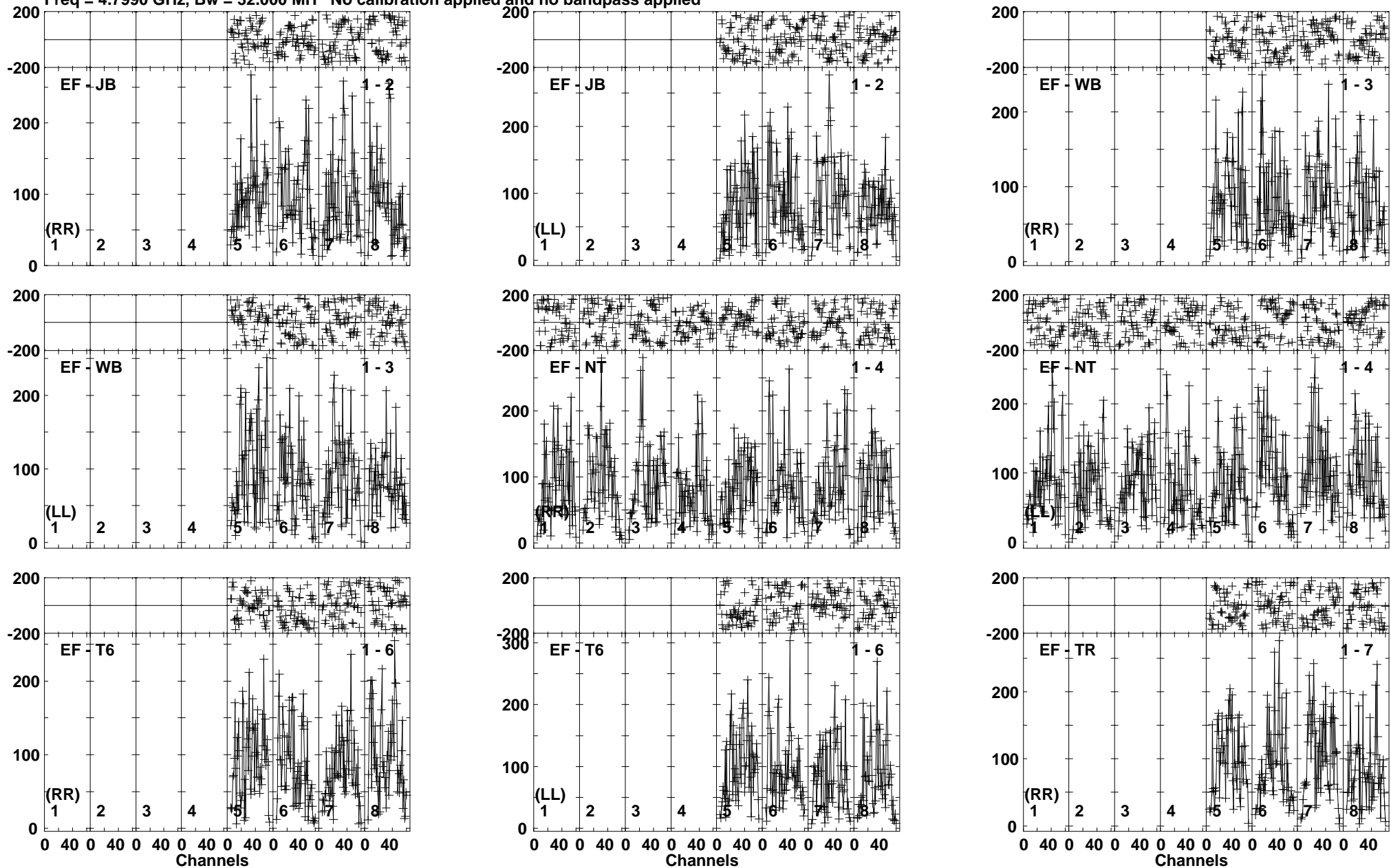
Lower frame: Micro Ampl Jy Top frame: Phas deg Vector averaged cross-power spectrum Baseline: EF (01) - JB (02) Timerange: 00/21:08:31 to 00/21:11:59
