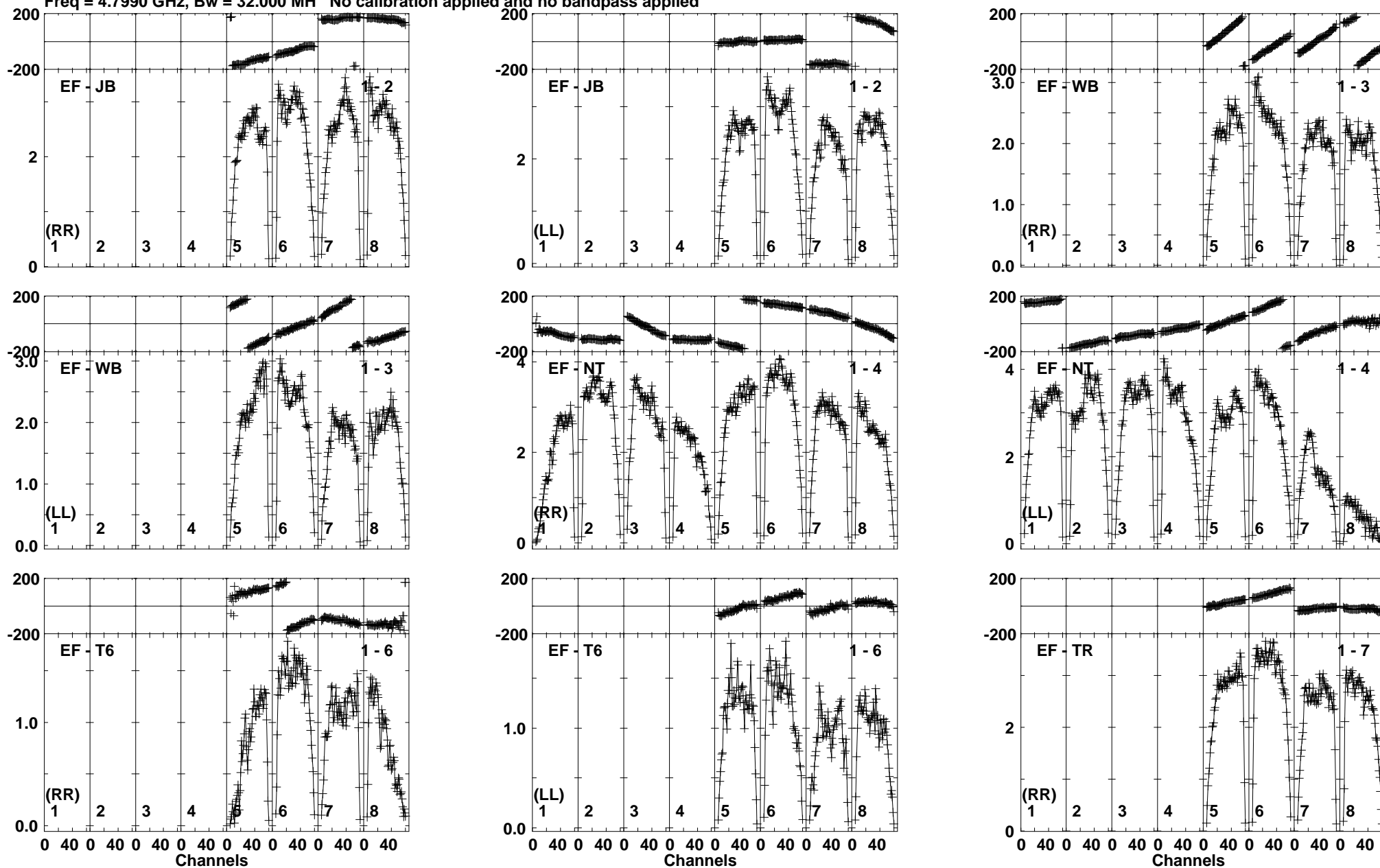
Lower frame: Milli Ampl Jy Top frame: Phas deg Vector averaged cross-power spectrum Baseline: EF (01) - JB (02) Timerange: 00/22:03:31 to 00/22:04:29
