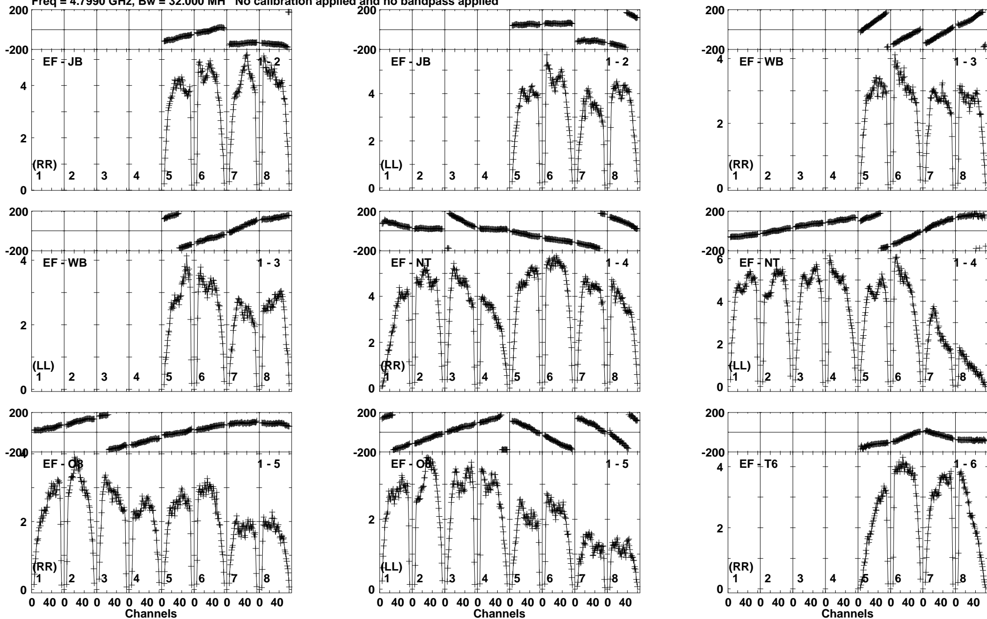
Lower frame: Milli Ampl Jy Top frame: Phas deg Vector averaged cross-power spectrum Baseline: EF (01) - JB (02) Timerange: 00/19:29:01 to 00/19:30:29
