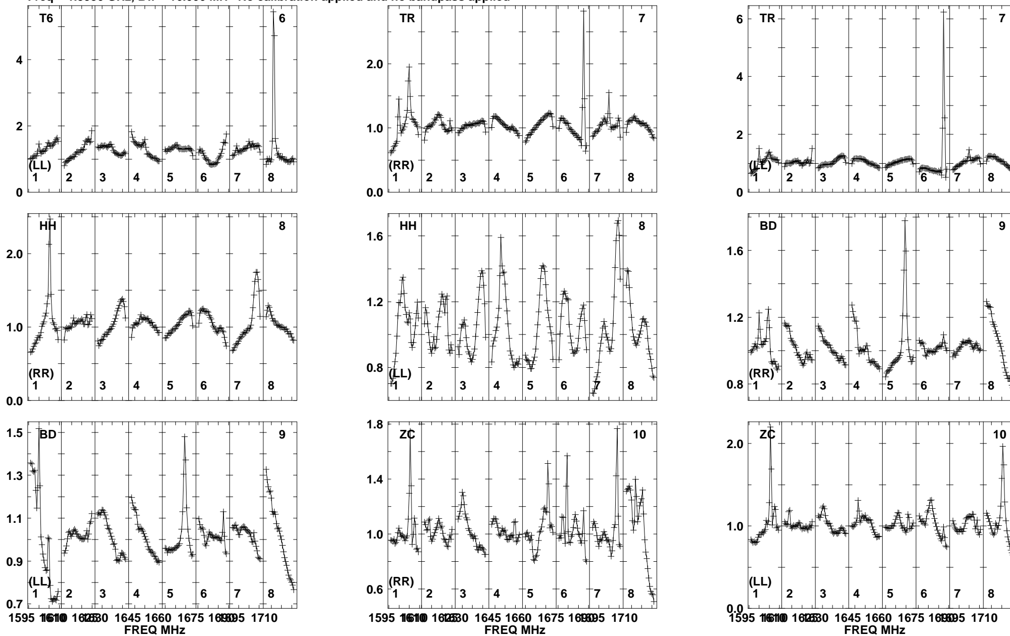
Lower frame: Real Jy Total-power spectrum Antenna: T6 (06) Timerange: 01/03:08:21 to 01/03:14:15
