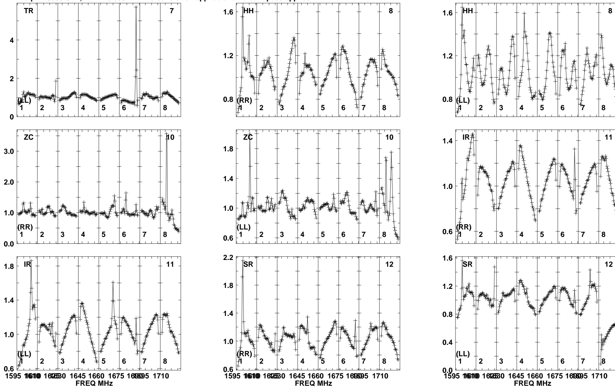
Lower frame: Real Jy Total-power spectrum Antenna: TR (07) Timerange: 01/06:22:30 to 01/06:24:00
