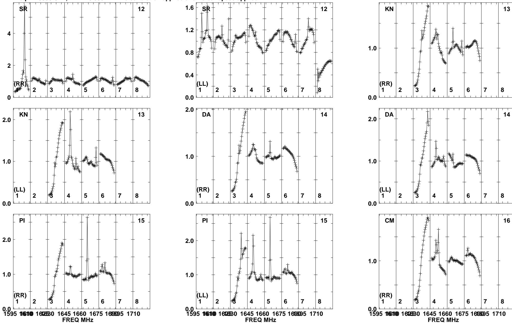
Lower frame: Real Jy Total-power spectrum Antenna: SR (12) Timerange: 01/05:20:01 to 01/05:21:40
