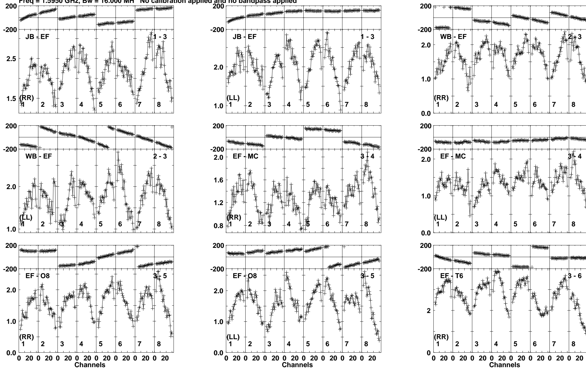
Lower frame: Milli Ampl Jy Top frame: Phas deg Vector averaged cross-power spectrum Baseline: JB (01) - EF (03) Timerange: 01/00:40:21 to 01/00:41:20
