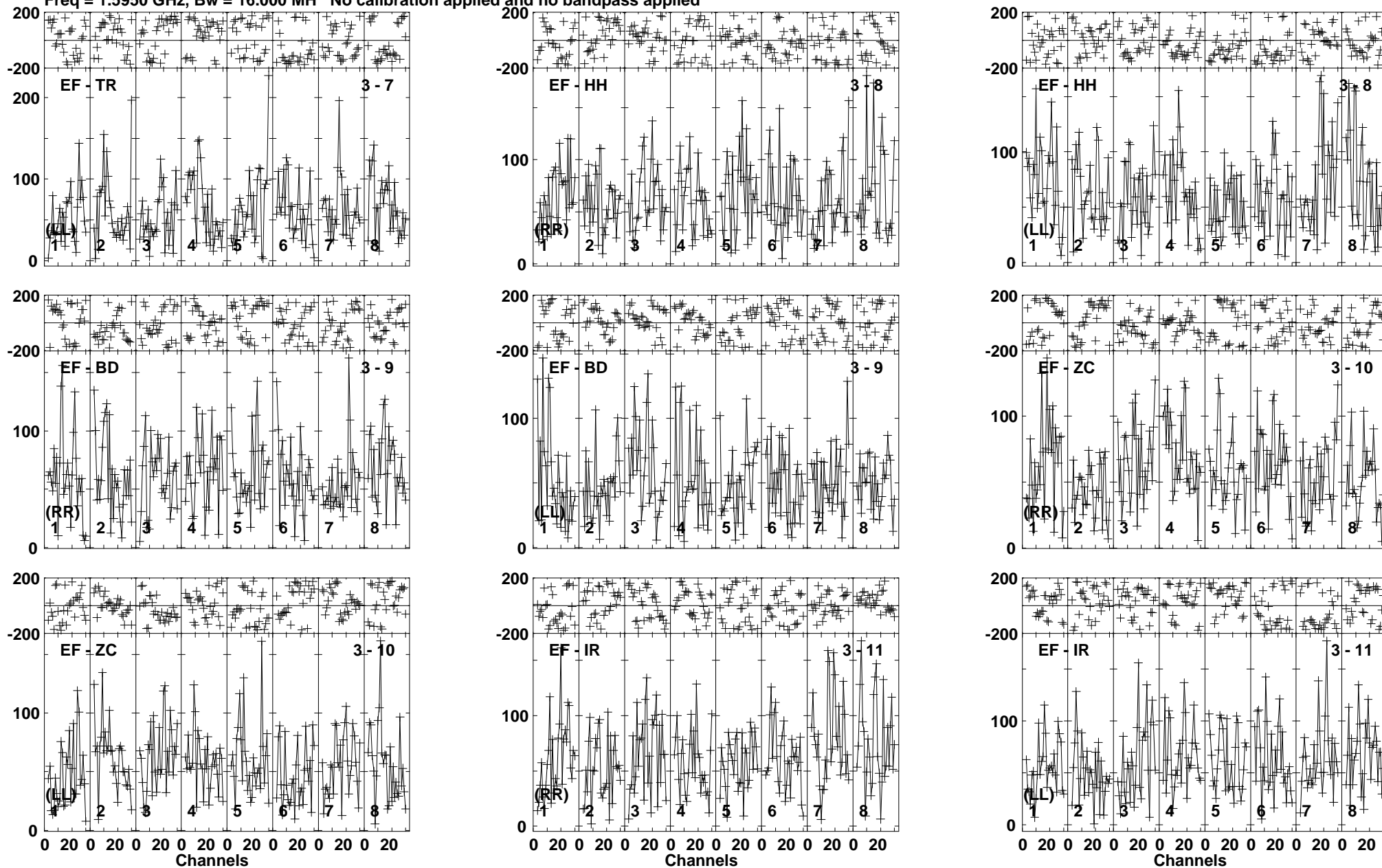
Lower frame: Micro Ampl Jy Top frame: Phas deg Vector averaged cross-power spectrum Baseline: EF (03) - TR (07) Timerange: 01/03:57:20 to 01/04:03:14
