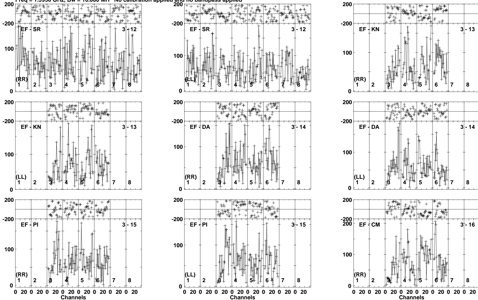
Lower frame: Micro Ampl Jy Top frame: Phas deg Vector averaged cross-power spectrum Baseline: EF (03) - SR (12) Timerange: 01/07:34:06 to 01/07:39:54
