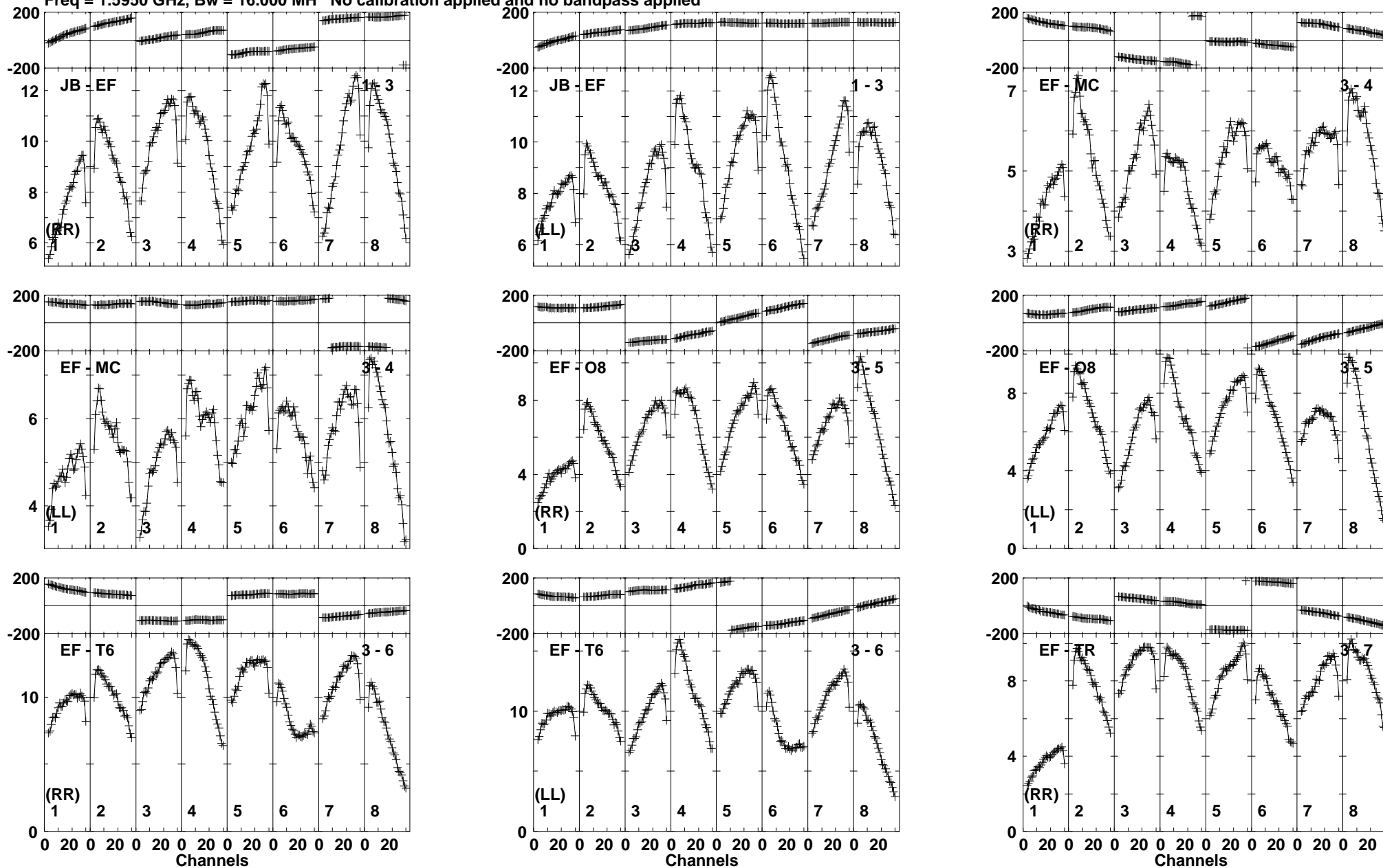
Lower frame: Milli Ampl Jy Top frame: Phas deg Vector averaged cross-power spectrum Baseline: JB (01) - EF (03) Timerange: 01/03:53:46 to 01/03:55:25
