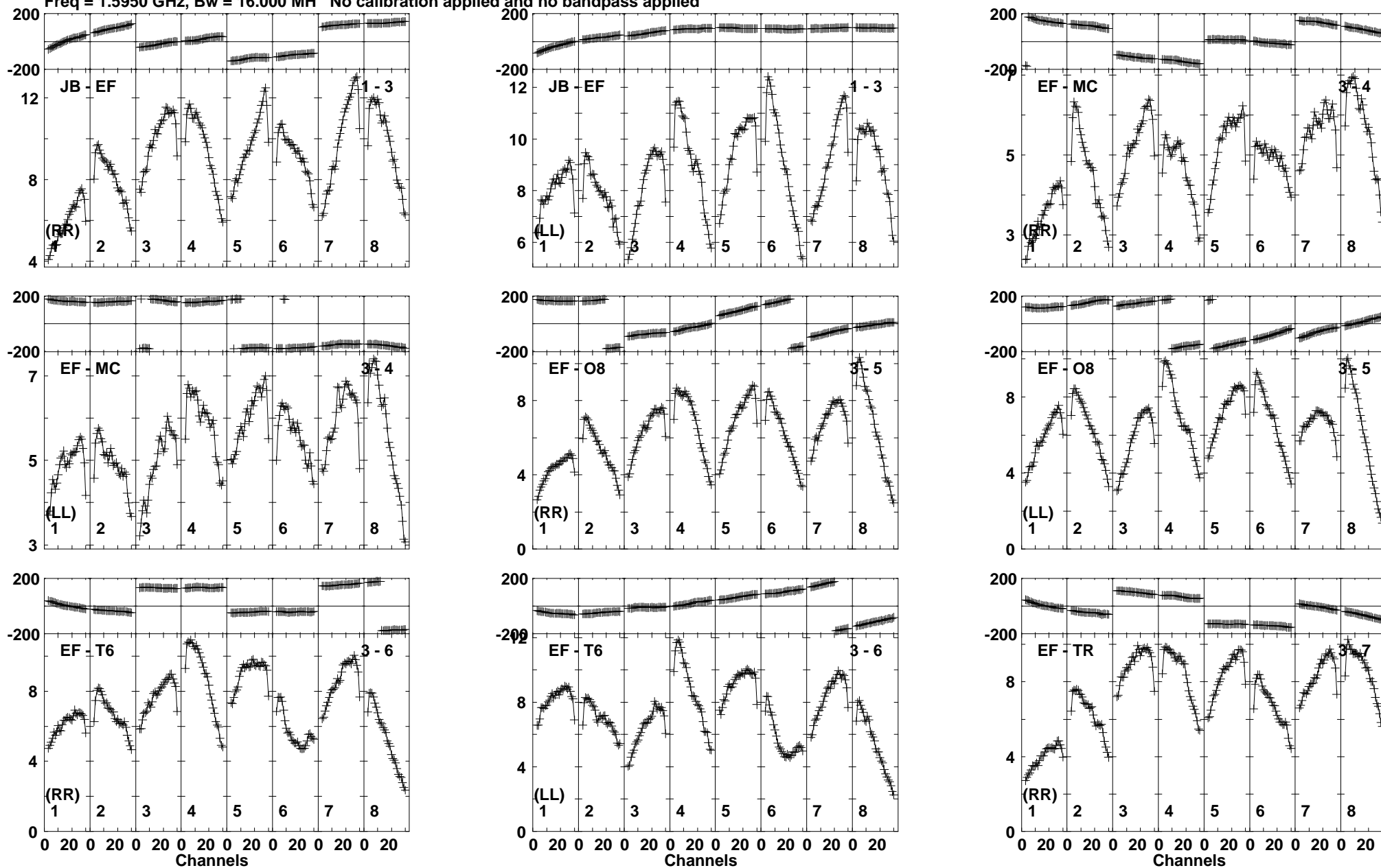
Lower frame: Milli Ampl Jy Top frame: Phas deg Vector averaged cross-power spectrum Baseline: JB (01) - EF (03) Timerange: 01/03:46:50 to 01/03:47:49
