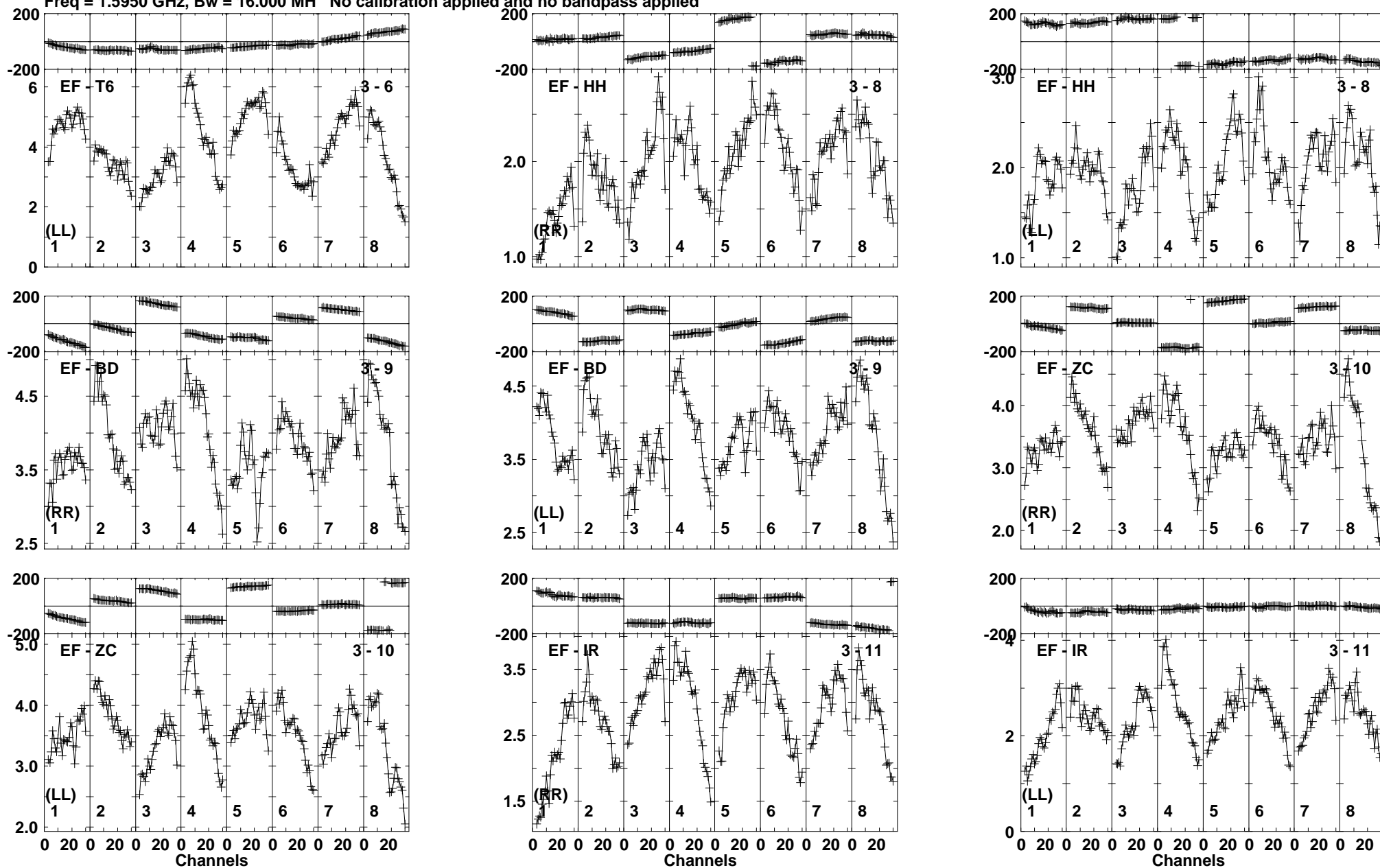
Lower frame: Milli Ampl Jy Top frame: Phas deg Vector averaged cross-power spectrum Baseline: EF (03) - T6 (06) Timerange: 00/22:17:41 to 00/22:18:39
