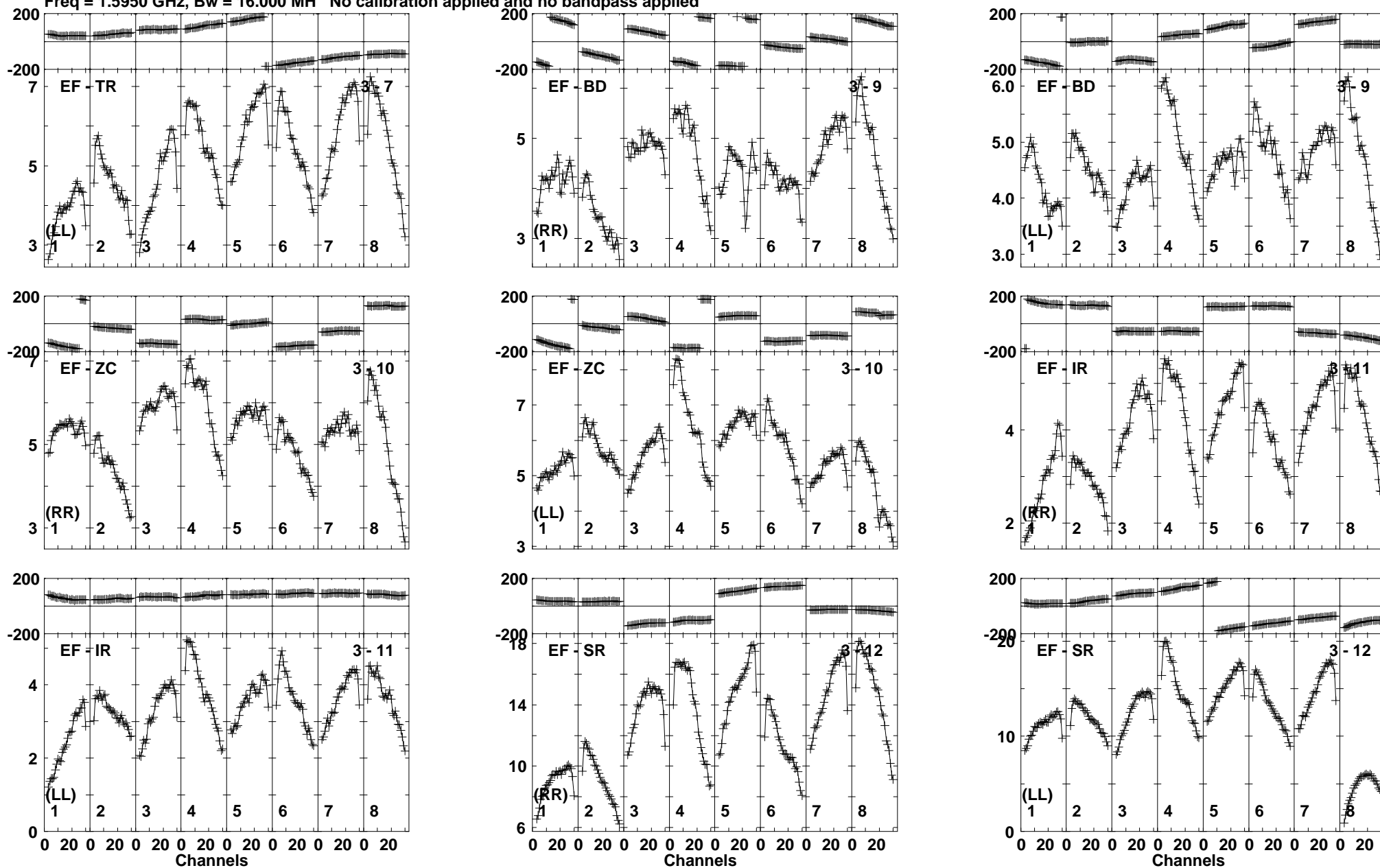
Lower frame: Milli Ampl Jy Top frame: Phas deg Vector averaged cross-power spectrum Baseline: EF (03) - TR (07) Timerange: 01/04:49:01 to 01/04:50:00
