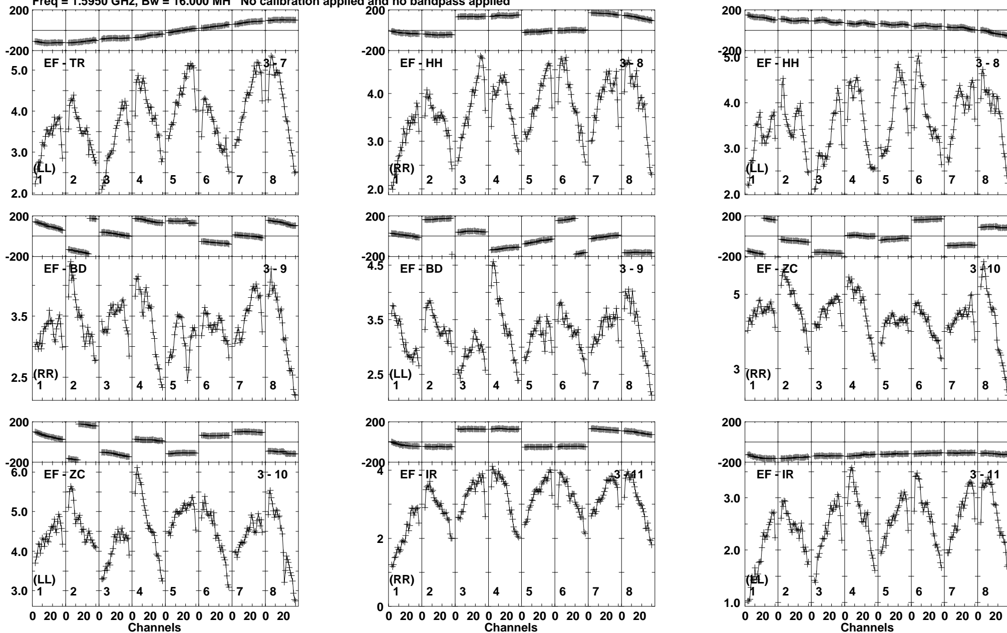
Lower frame: Milli Ampl Jy Top frame: Phas deg Vector averaged cross-power spectrum Baseline: EF (03) - TR (07) Timerange: 01/03:34:35 to 01/03:36:14
