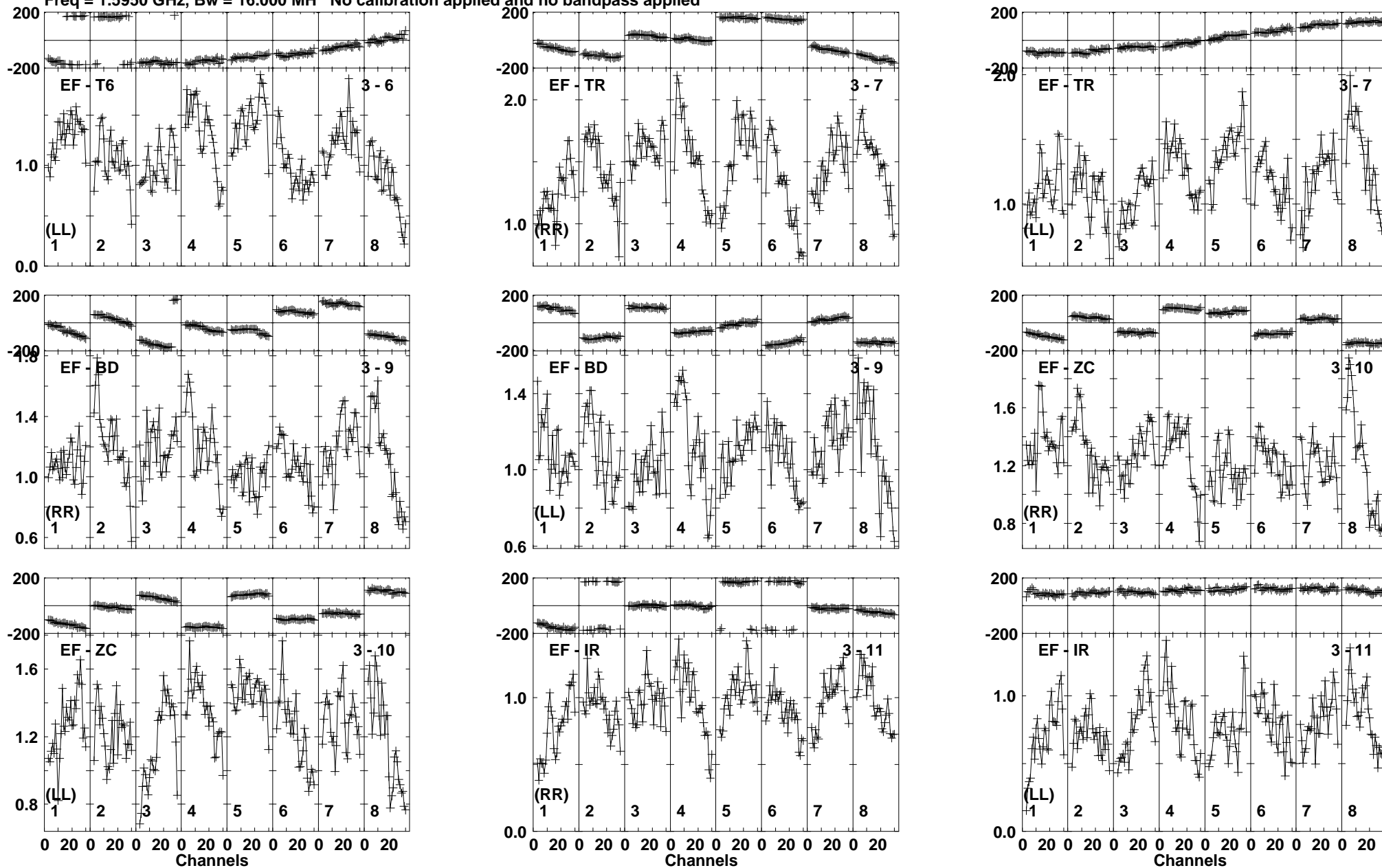
Lower frame: Milli Ampl Jy Top frame: Phas deg Vector averaged cross-power spectrum Baseline: EF (03) - T6 (06) Timerange: 01/00:30:10 to 01/00:31:09
