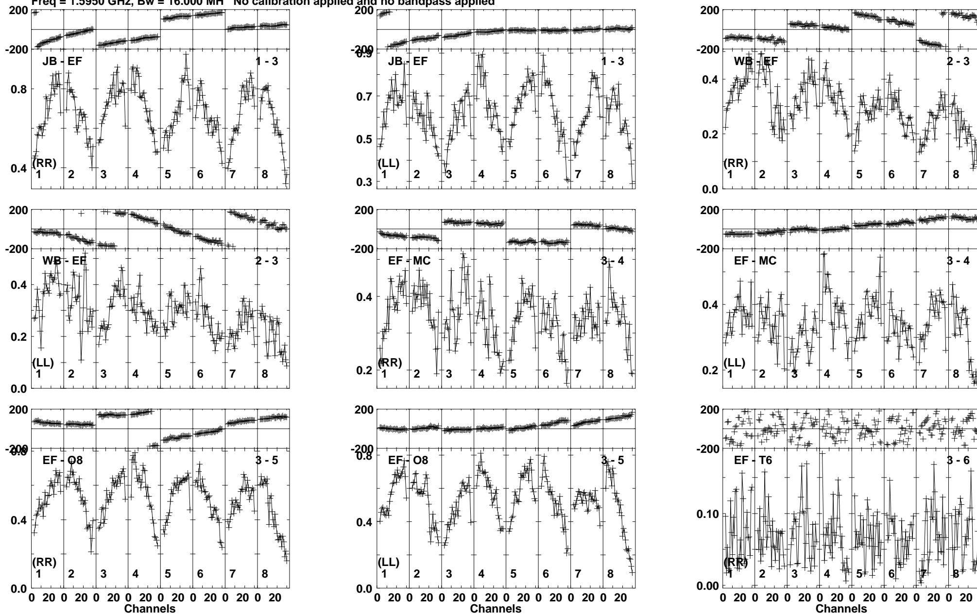
Lower frame: Milli Ampl Jy Top frame: Phas deg Vector averaged cross-power spectrum Baseline: JB (01) - EF (03) Timerange: 00:22:49:31 to 00:22:55:29
