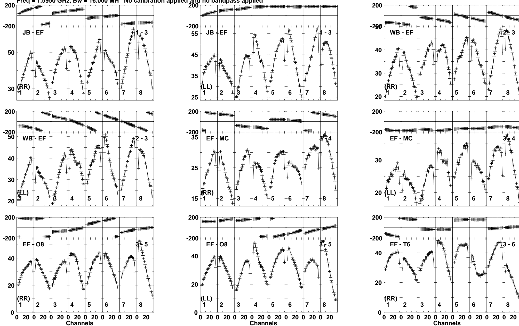
Lower frame: Milli Ampl Jy Top frame: Phas deg Vector averaged cross-power spectrum Baseline: JB (01) - EF (03) Timerange: 01/02:02:15 to 01/02:06:14
