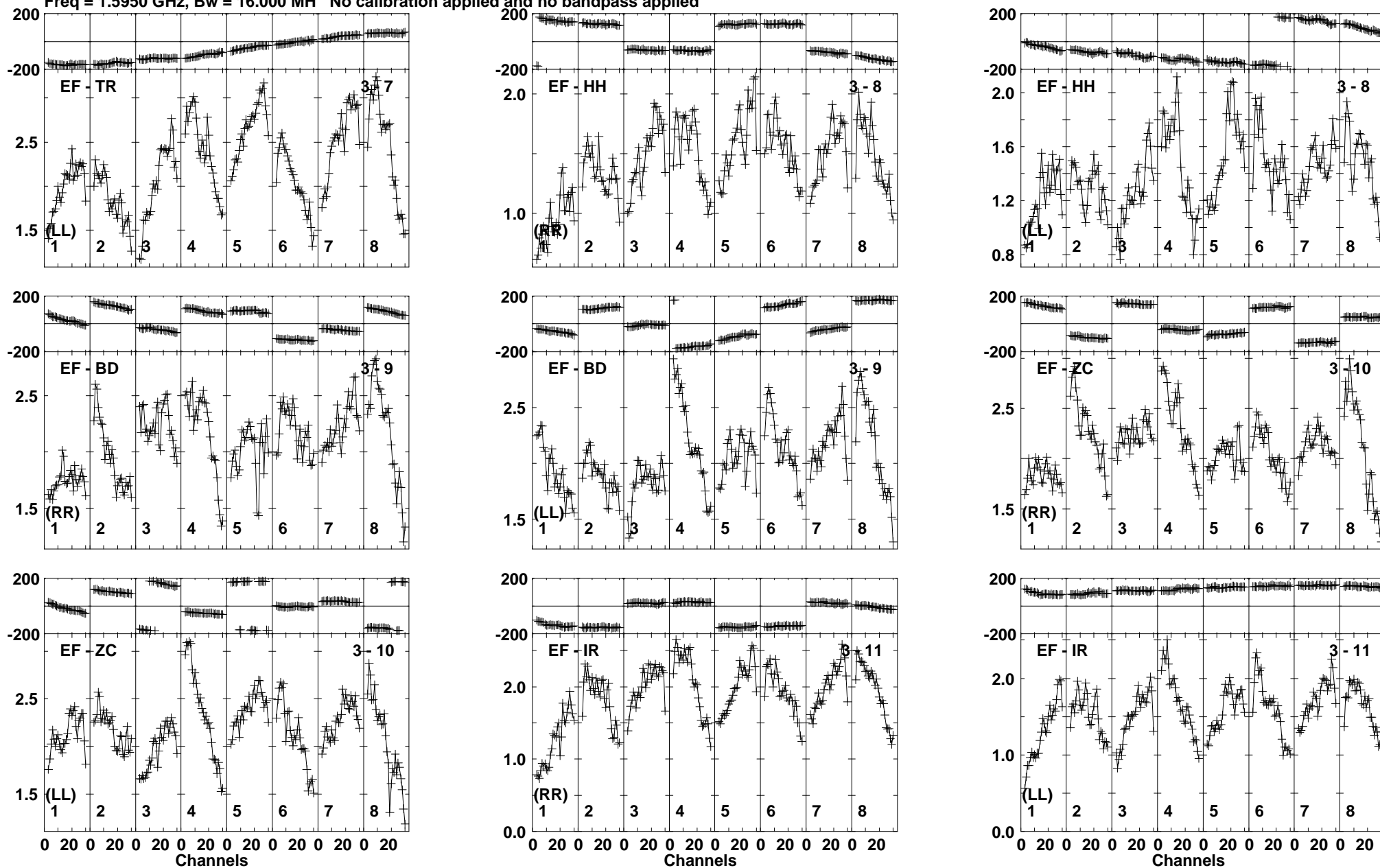
Lower frame: Milli Ampl Jy Top frame: Phas deg Vector averaged cross-power spectrum Baseline: EF (03) - TR (07) Timerange: 01/03:14:16 to 01/03:15:45
