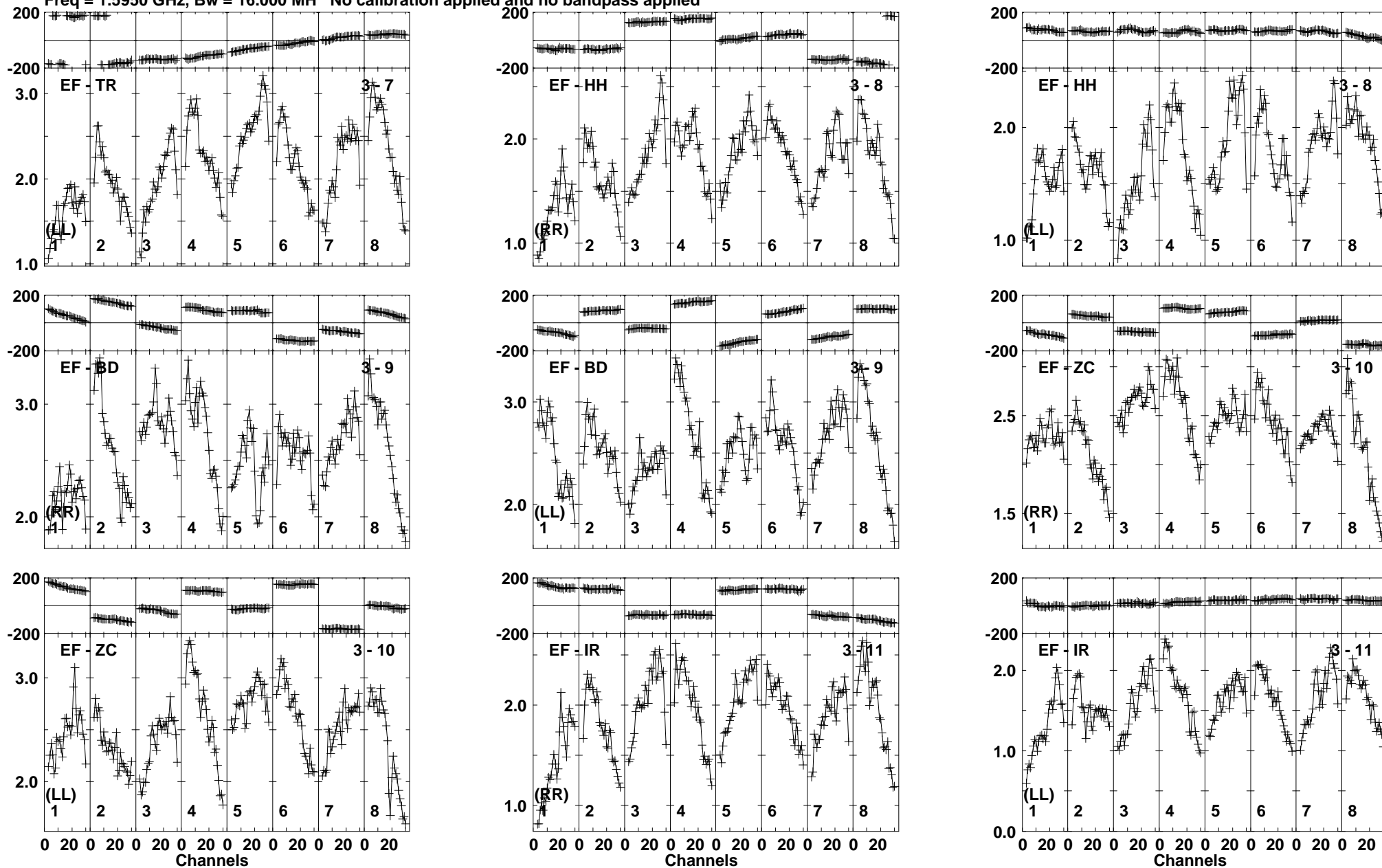
Lower frame: Milli Ampl Jy Top frame: Phas deg Vector averaged cross-power spectrum Baseline: EF (03) - TR (07) Timerange: 01/04:12:35 to 01/04:14:14
