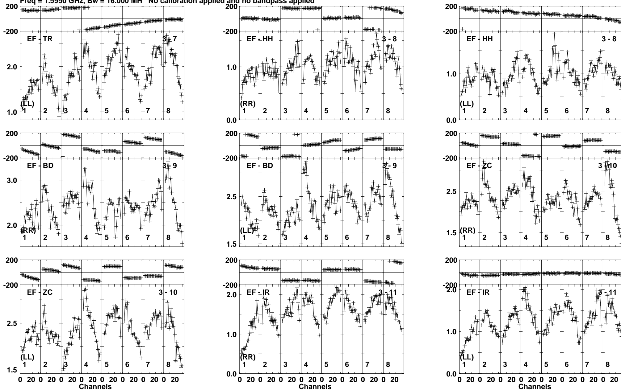
Lower frame: Milli Ampl Jy Top frame: Phas deg Vector averaged cross-power spectrum Baseline: EF (03) - TR (07) Timerange: 01/02:56:56 to 01/02:57:54
