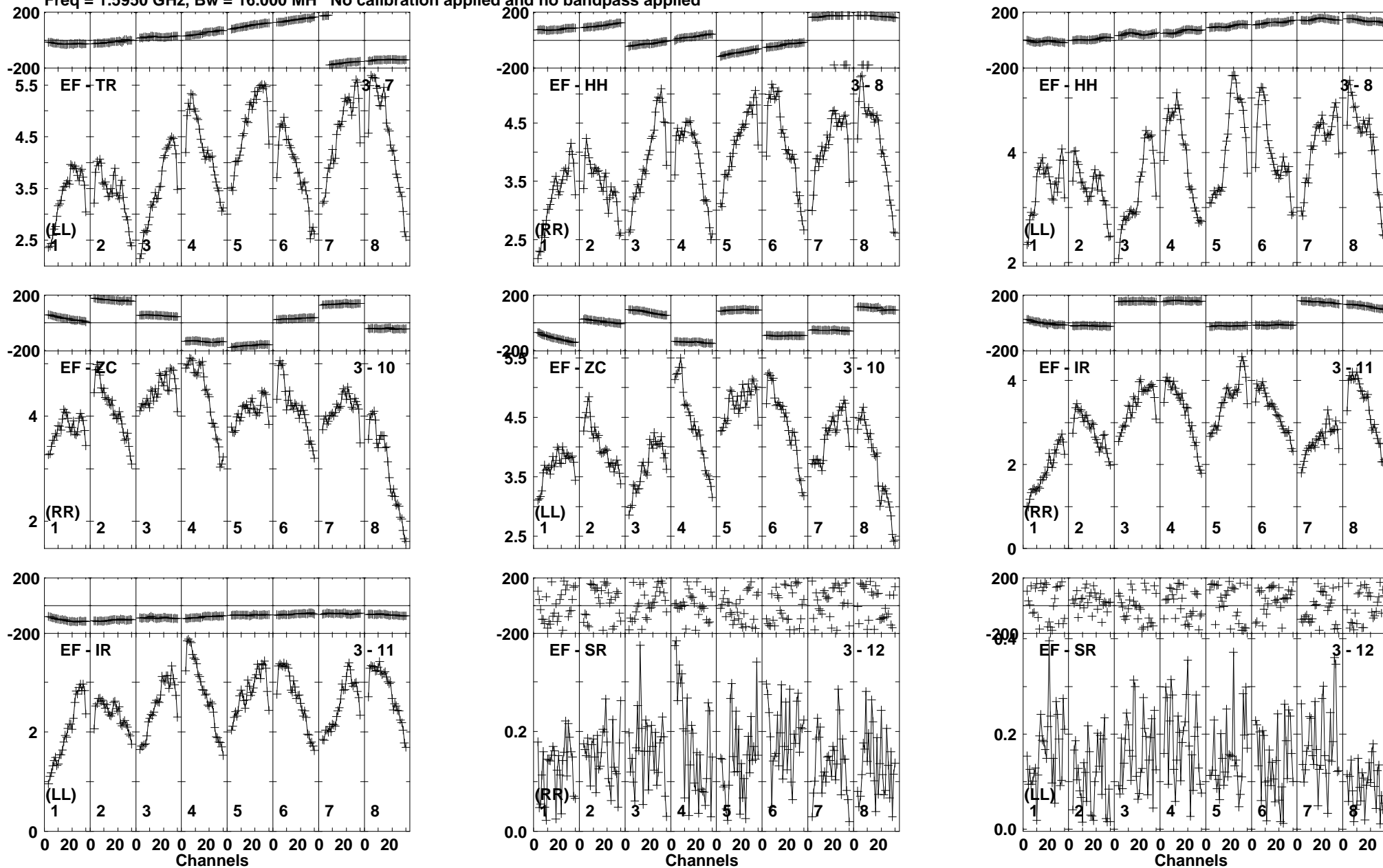
Lower frame: Milli Ampl Jy Top frame: Phas deg Vector averaged cross-power spectrum Baseline: EF (03) - TR (07) Timerange: 01/08:18:50 to 01/08:20:29
