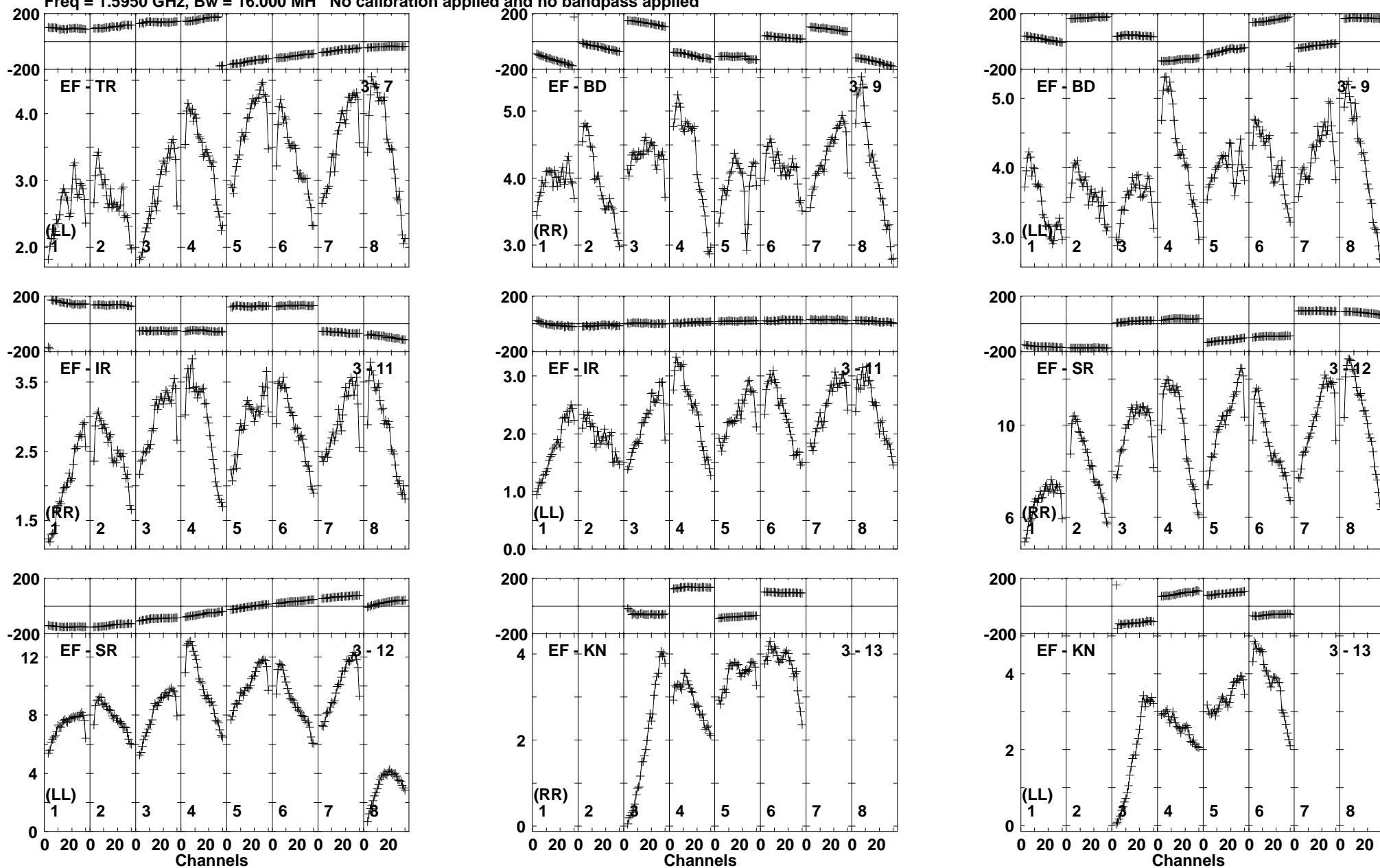
Lower frame: Milli Ampl Jy Top frame: Phas deg Vector averaged cross-power spectrum Baseline: EF (03) - TR (07) Timerange: 01/04:44:51 to 01/04:46:30
