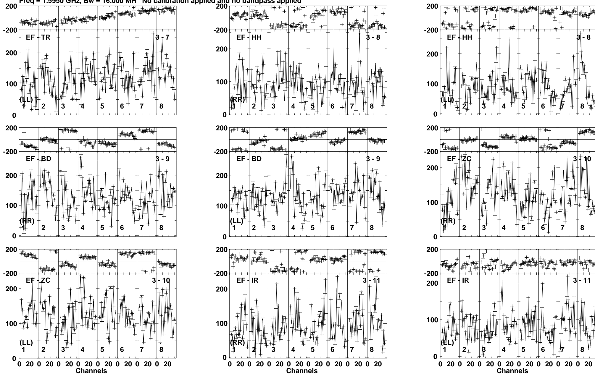
Lower frame: Micro Ampl Jy Top frame: Phas deg Vector averaged cross-power spectrum Baseline: EF (03) - TR (07) Timerange: 01/03:38:11 to 01/03:44:05
