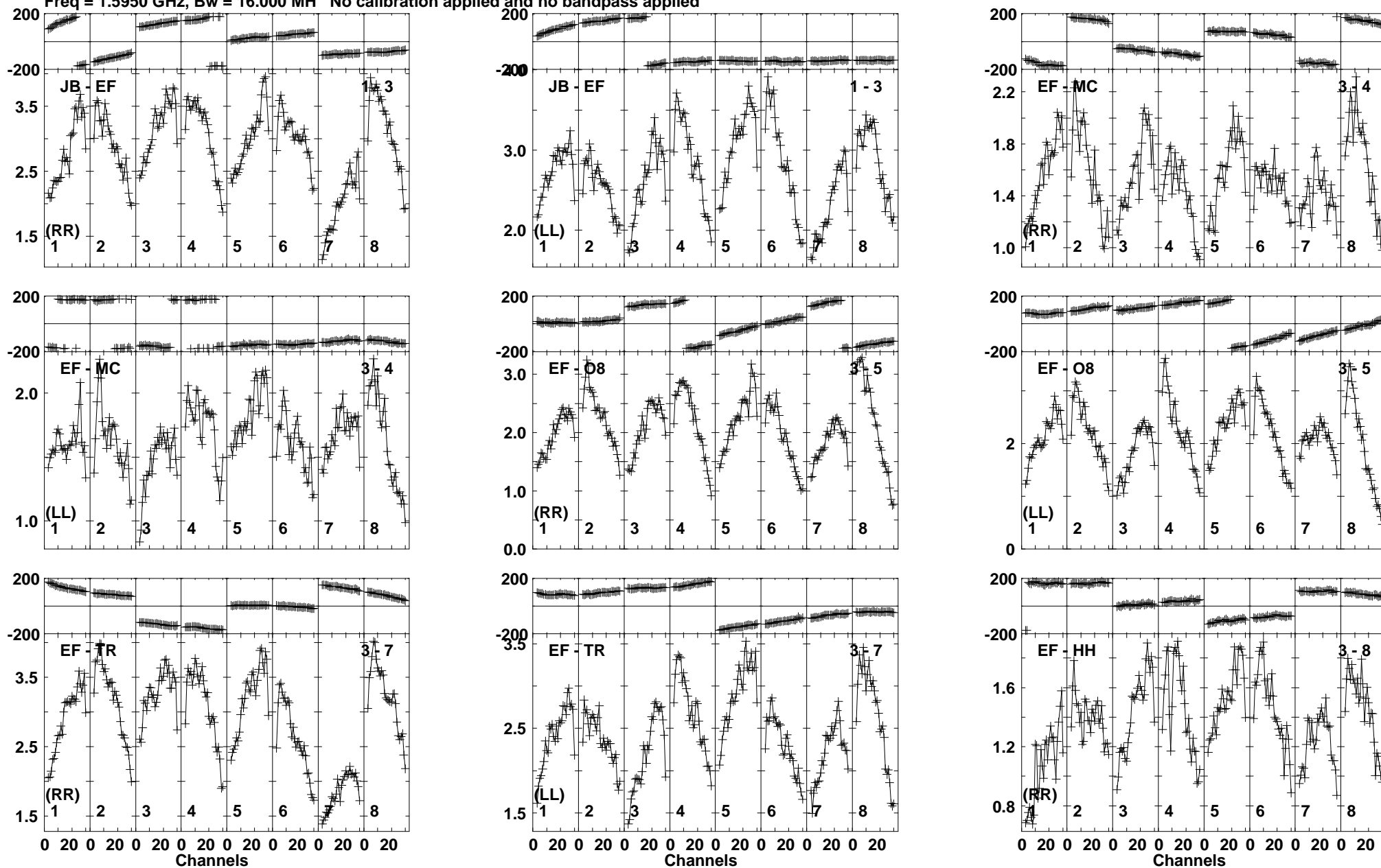
Lower frame: Milli Amp Jy Top frame: Phas deg Vector averaged cross-power spectrum Baseline: JB (01) - EF (03) Timerange: 01/06:15:35 to 01/06:16:34
