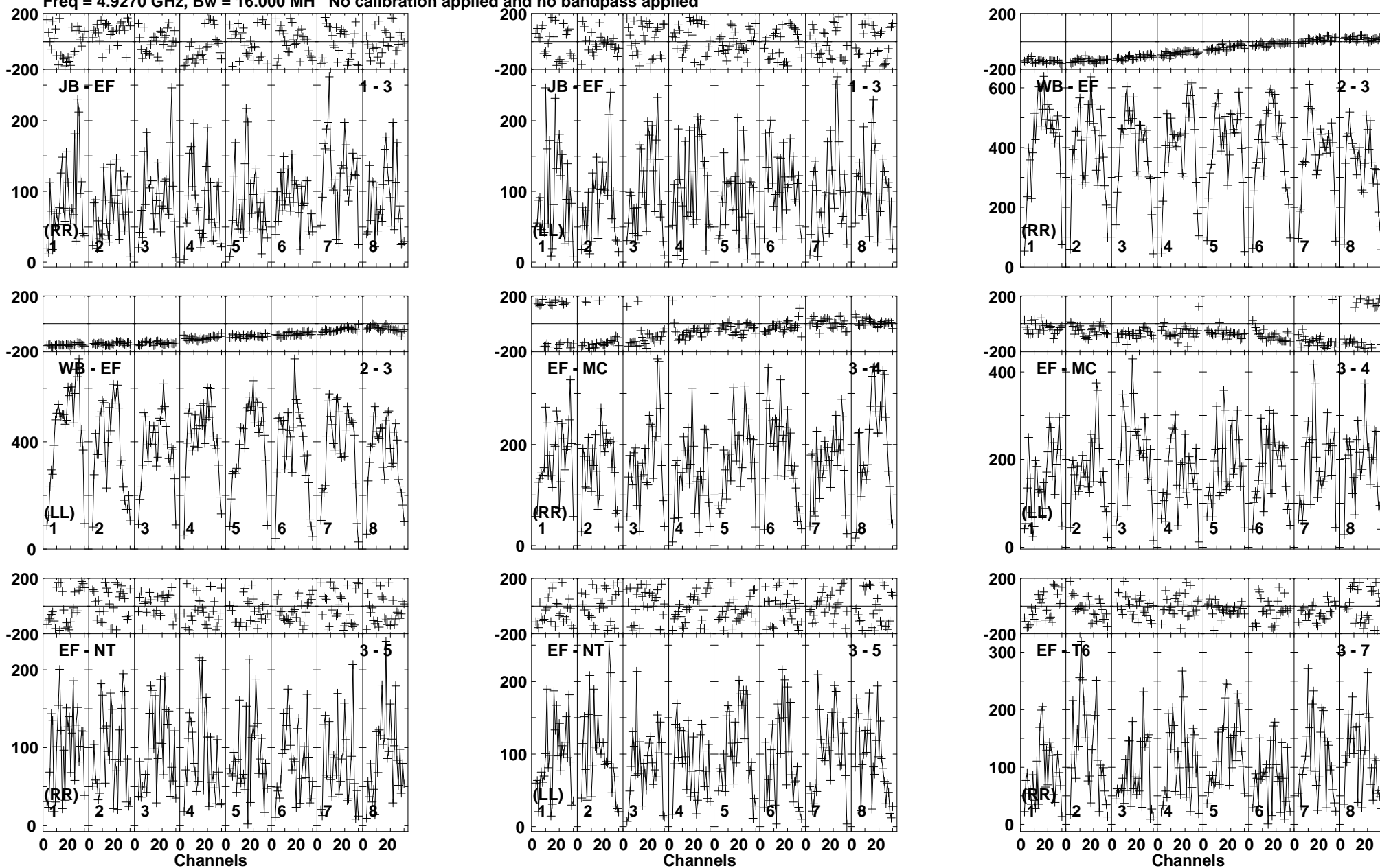
Lower frame: Micro Ampl Jy Top frame: Phas deg Vector averaged cross-power spectrum Baseline: JB (01) - EF (03) Timerange: 00/11:01:31 to 00/11:04:29
