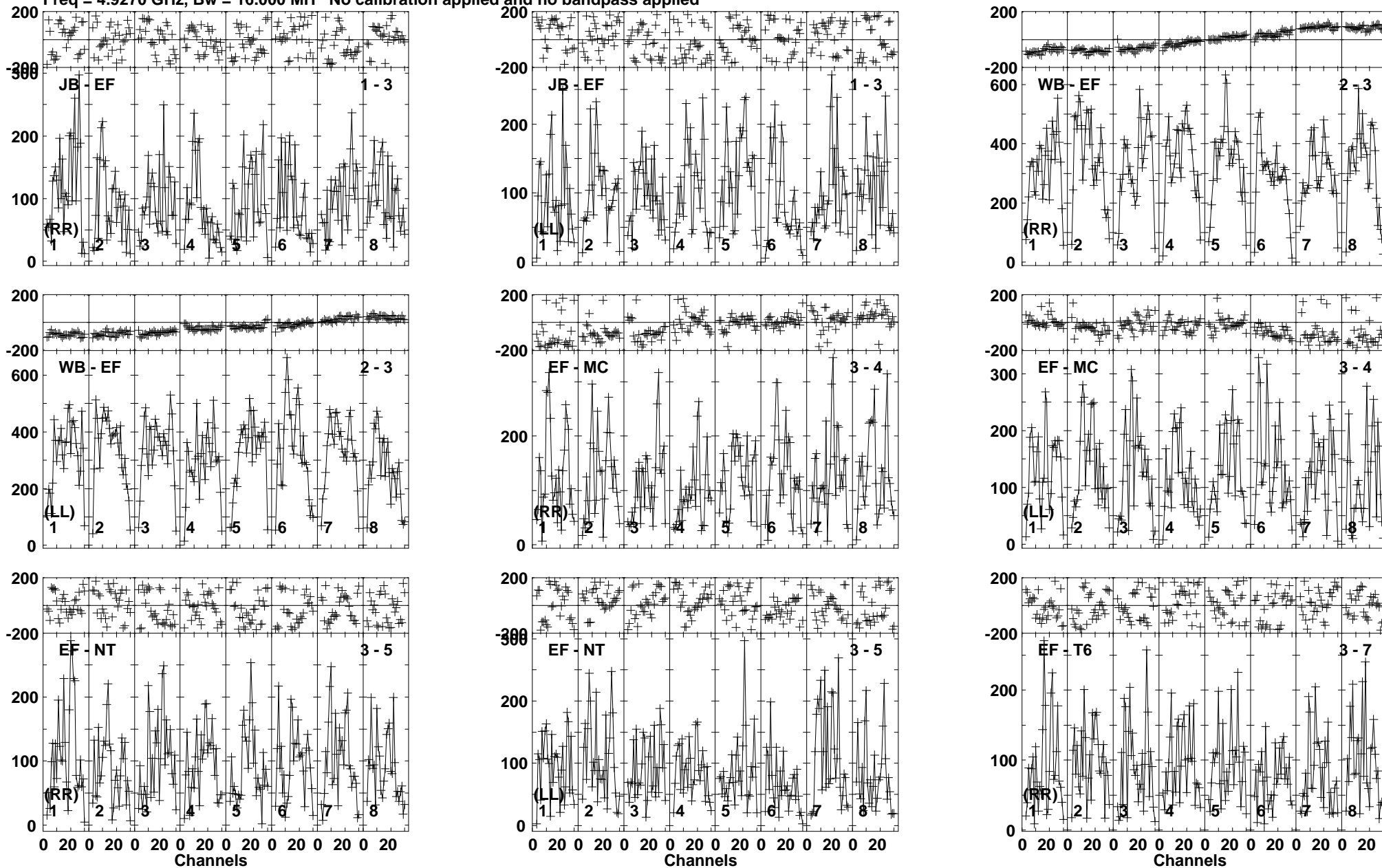
Lower frame: Micro Ampl Jy Top frame: Phas deg Vector averaged cross-power spectrum Baseline: JB (01) - EF (03) Timerange: 00/10:50:31 to 00/10:53:29
