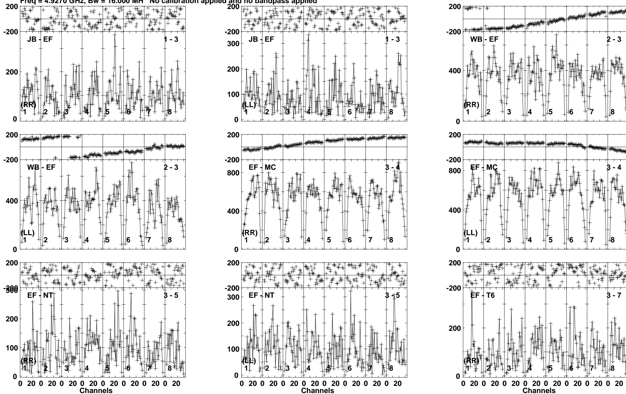
Lower frame: Micro Ampl Jy Top frame: Phas deg Vector averaged cross-power spectrum Baseline: JB (01) - EF (03) Timerange: 00/08:27:31 to 00/08:30:29
