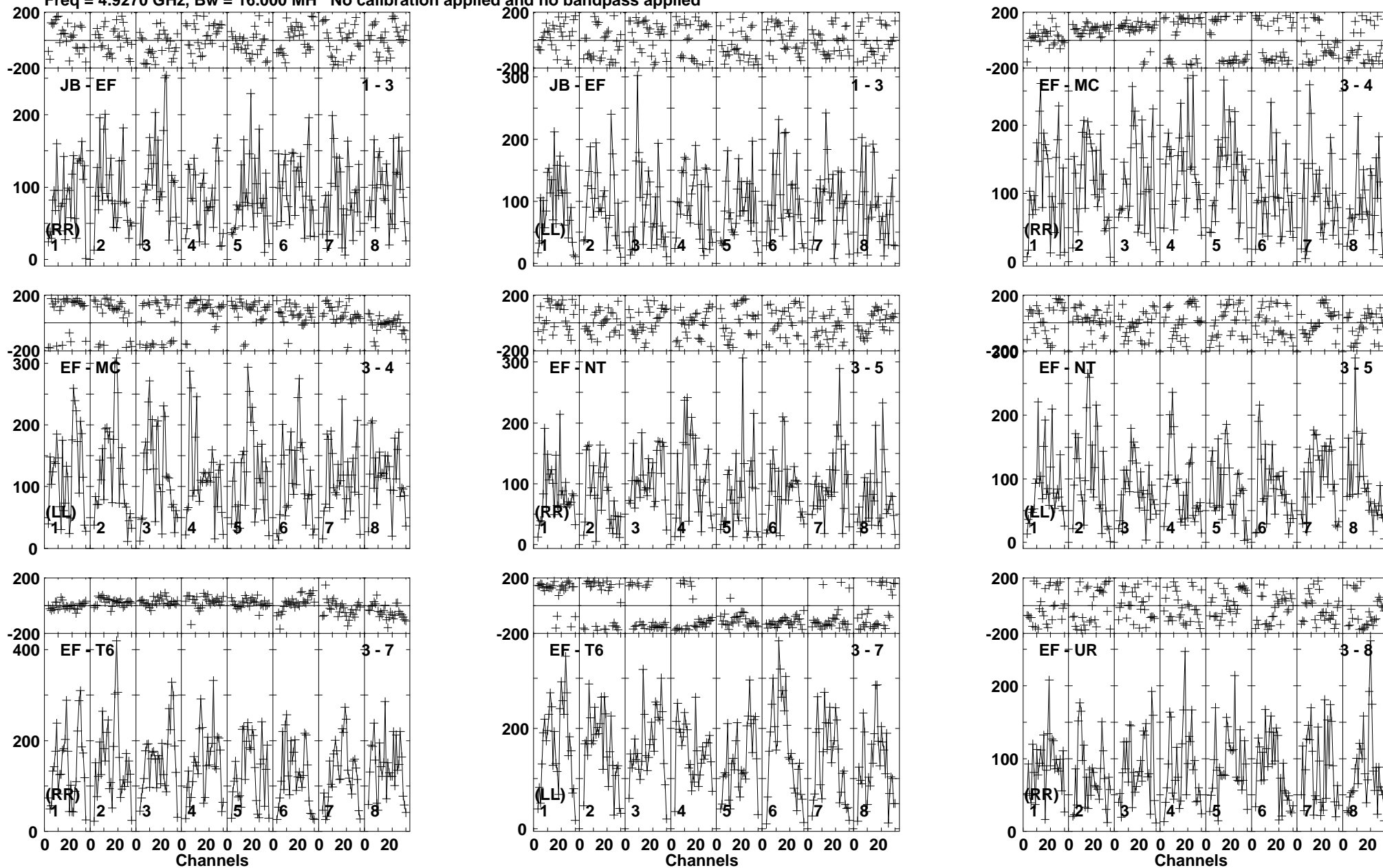
Lower frame: Micro Ampl Jy Top frame: Phas deg Vector averaged cross-power spectrum Baseline: JB (01) - EF (03) Timerange: 00/06:35:01 to 00/06:37:59
