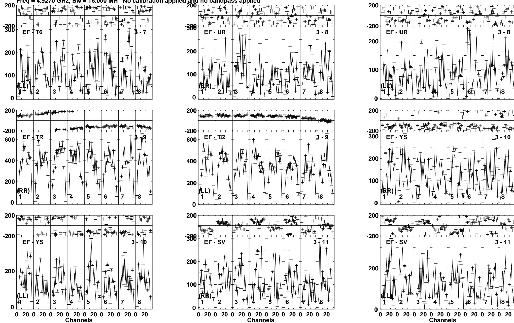
Lower frame: Micro Ampl Jy Top frame: Phas deg Vector averaged cross-power spectrum Baseline: EF (03) - T6 (07) Timerange: 00/10:17:31 to 00/10:20:29
