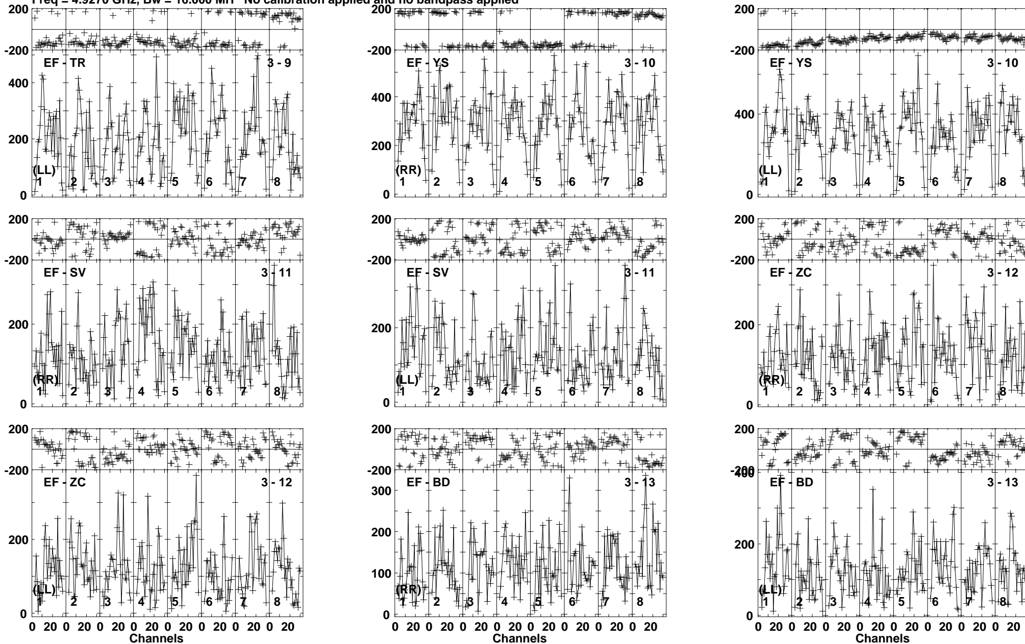
Lower frame: Micro Ampl Jy Top frame: Phas deg Vector averaged cross-power spectrum Baseline: EF (03) - TR (09) Timerange: 00/13:54:31 to 00/13:57:29
