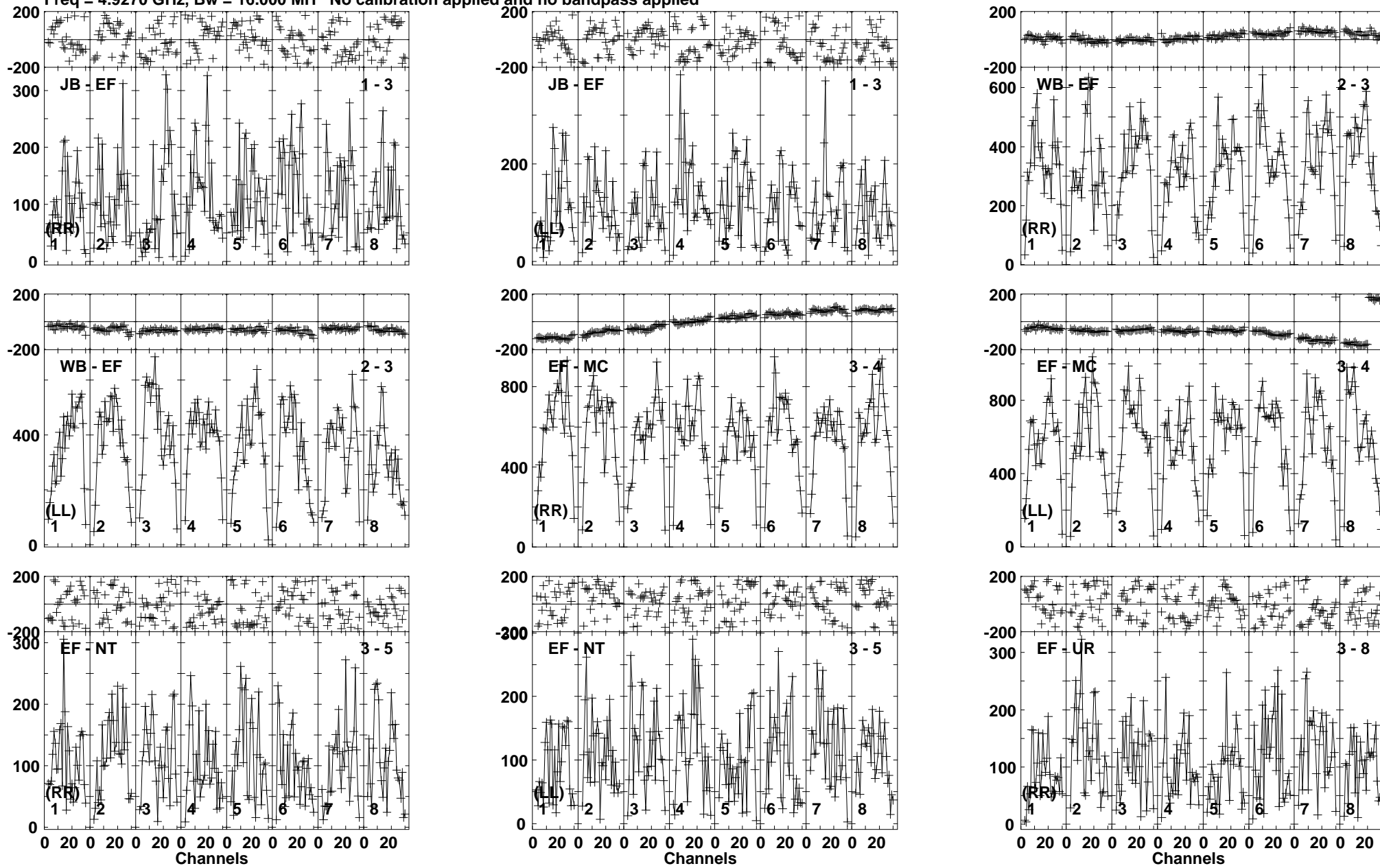
Lower frame: Micro Ampl Jy Top frame: Phas deg Vector averaged cross-power spectrum Baseline: JB (01) - EF (03) Timerange: 00/13:38:01 to 00/13:40:59
