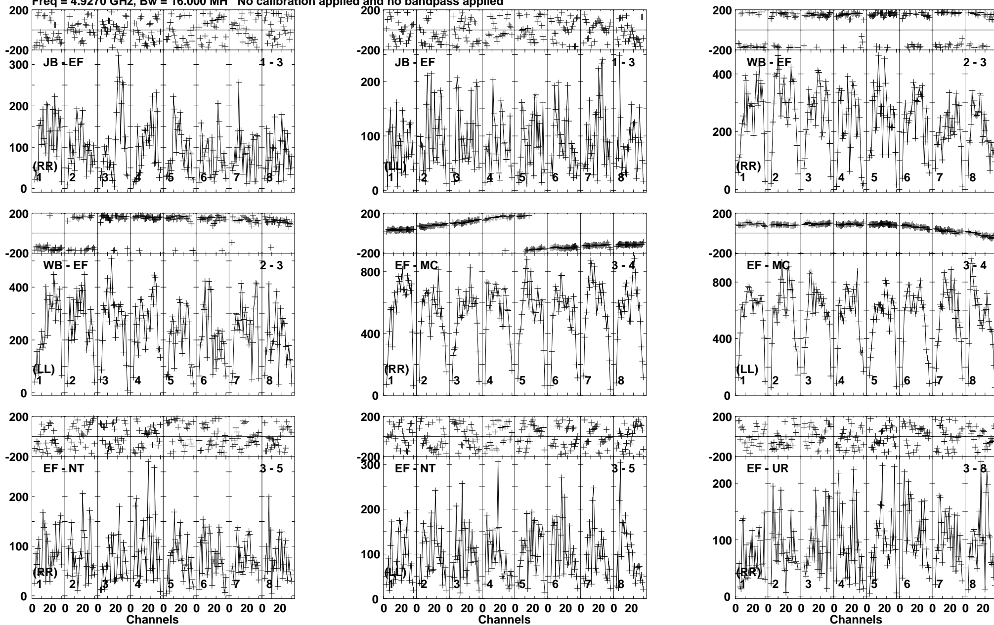
Lower frame: Micro Ampl Jy Top frame: Phas deg Vector averaged cross-power spectrum Baseline: JB (01) - EF (03) Timerange: 00/14:38:31 to 00/14:41:29
