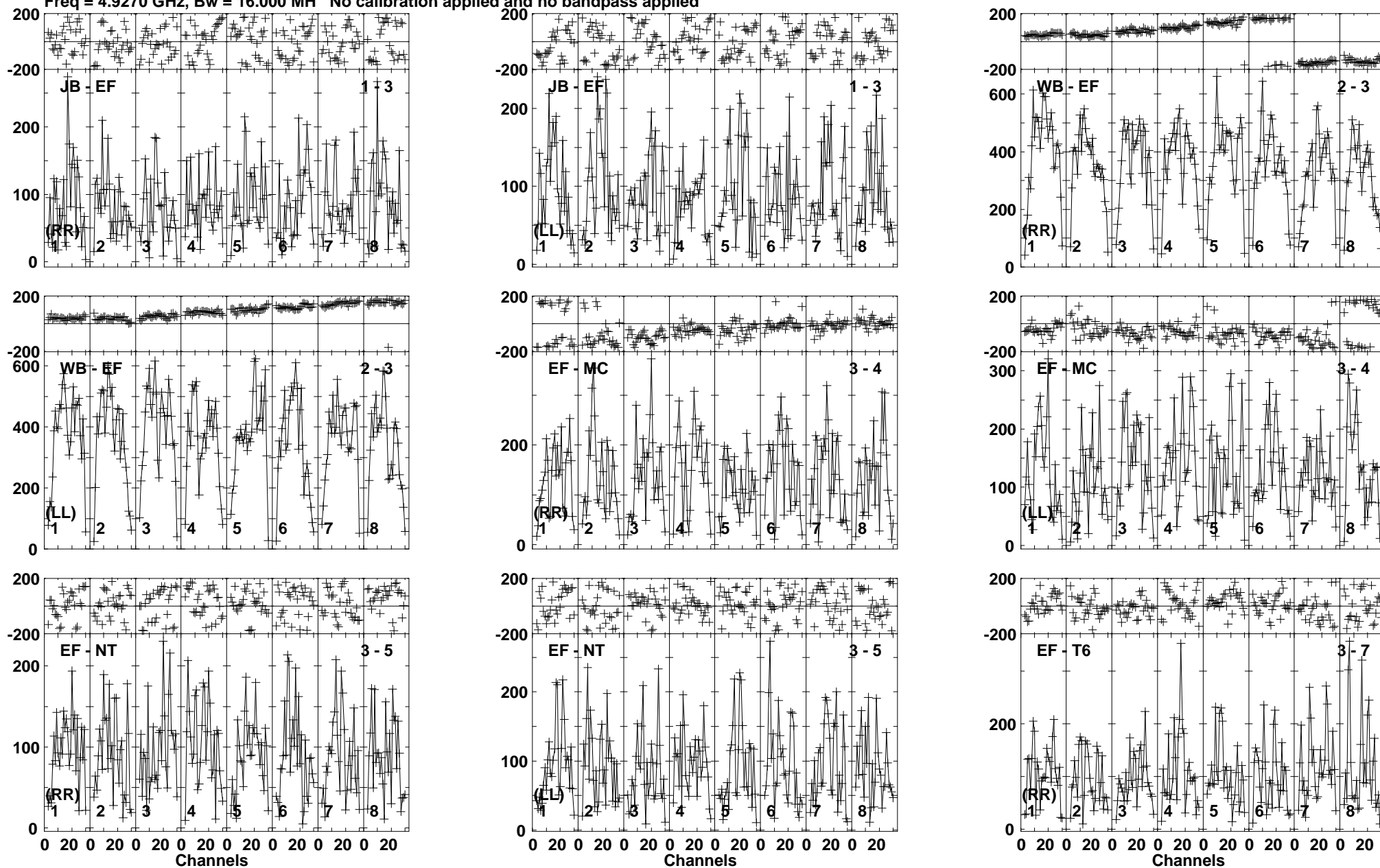
Lower frame: Micro Ampl Jy Top frame: Phas deg Vector averaged cross-power spectrum Baseline: JB (01) - EF (03) Timerange: 00/10:56:01 to 00/10:58:59
