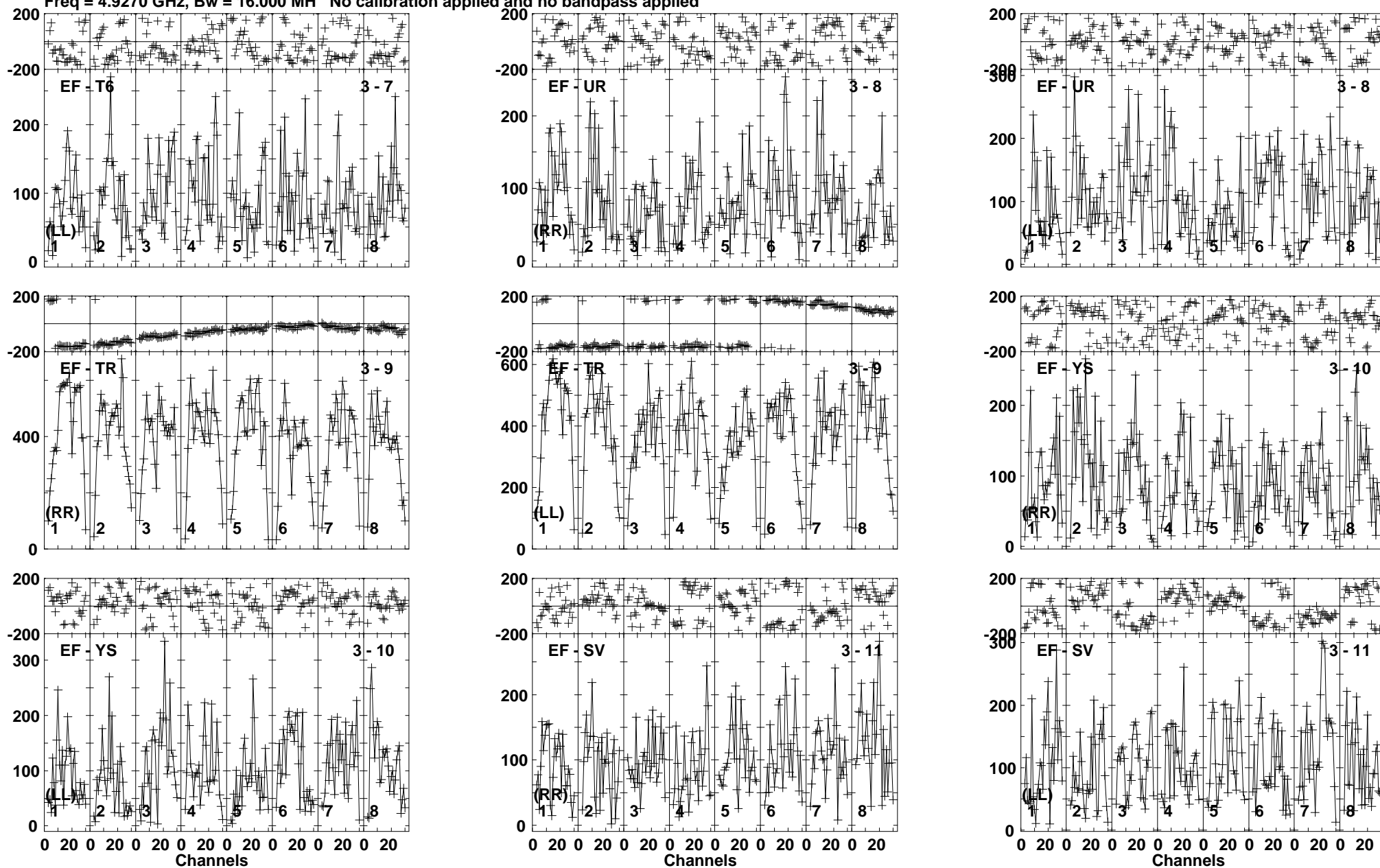
Lower frame: Micro Ampl Jy Top frame: Phas deg Vector averaged cross-power spectrum Baseline: EF (03) - T6 (07) Timerange: 00/09:39:01 to 00/09:41:59
