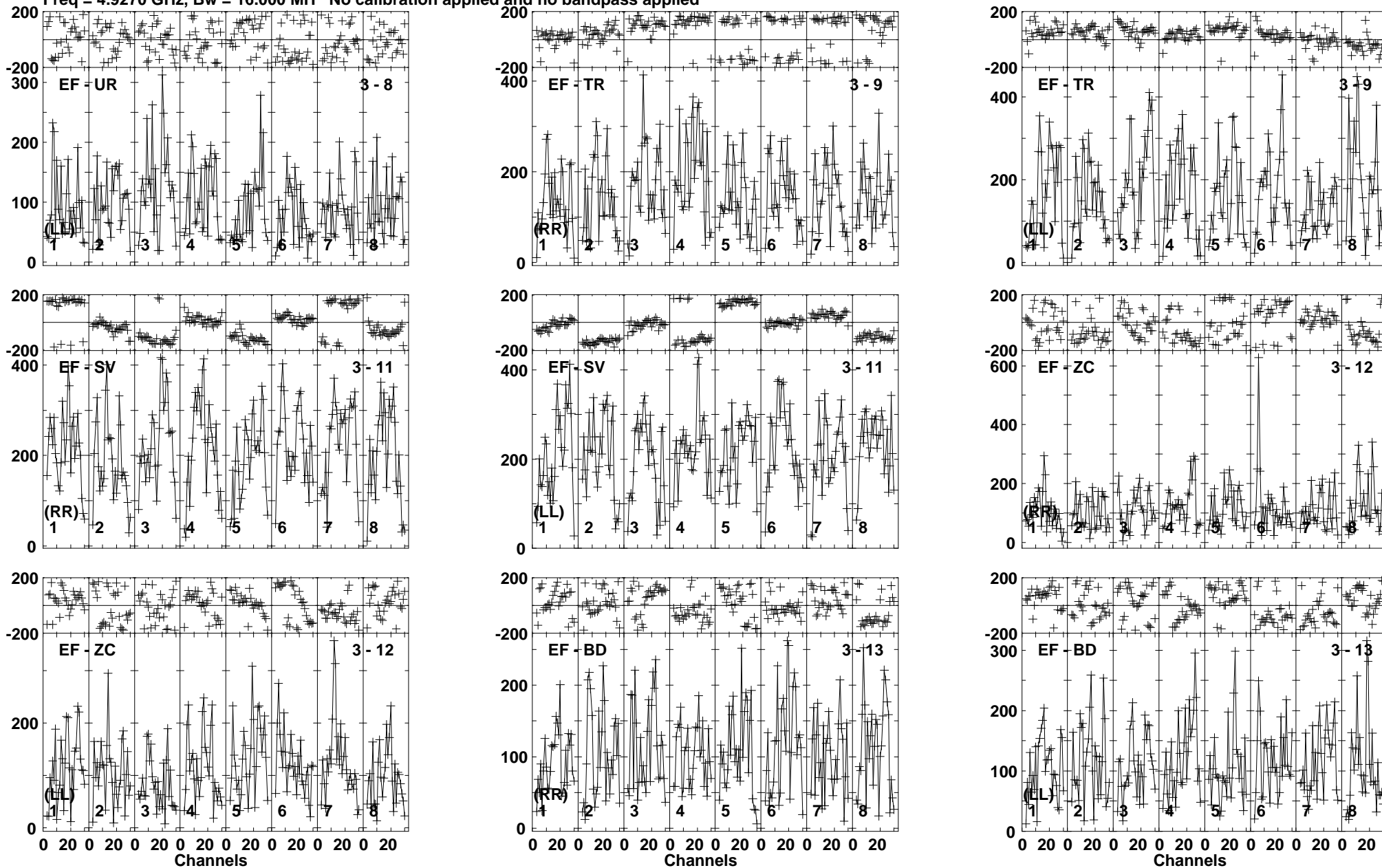
Lower frame: Micro Ampl Jy Top frame: Phas deg Vector averaged cross-power spectrum Baseline: EF (03) - UR (08) Timerange: 00/14:05:31 to 00/14:08:29
