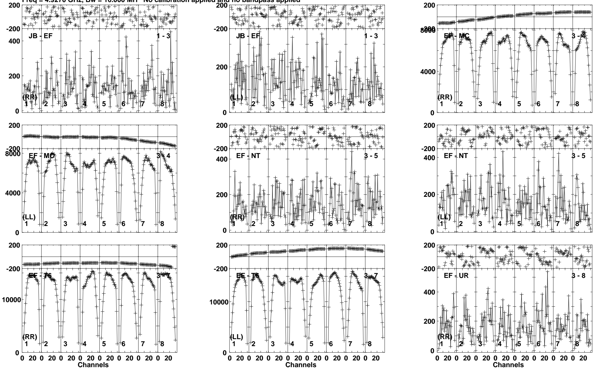
Lower frame: Micro Ampl Jy Top frame: Phas deg Vector averaged cross-power spectrum Baseline: JB (01) - EF (03) Timerange: 00/06:33:01 to 00/06:34:29
