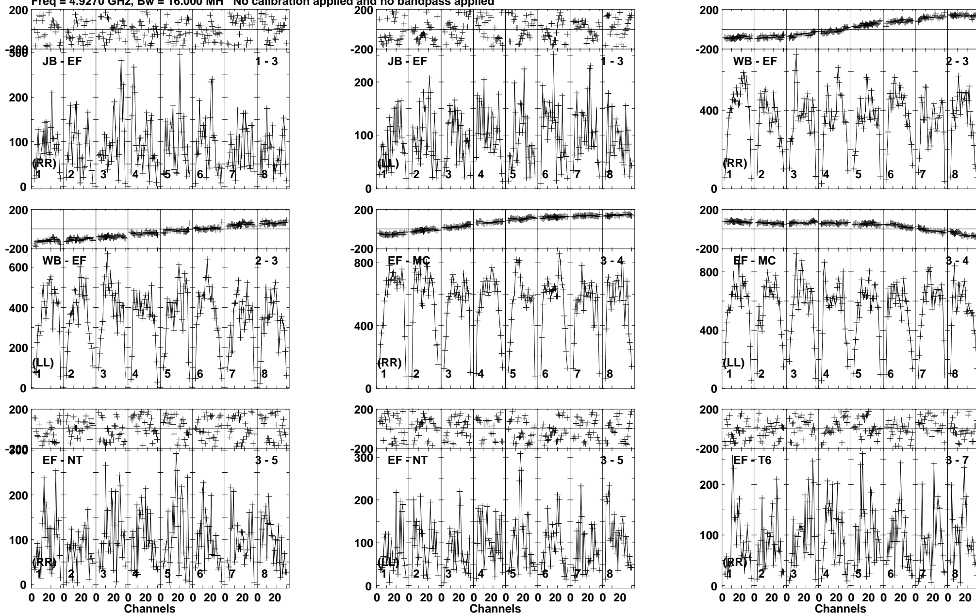
Lower frame: Micro Ampl Jy Top frame: Phas deg Vector averaged cross-power spectrum Baseline: JB (01) - EF (03) Timerange: 00/09:33:31 to 00/09:36:29
