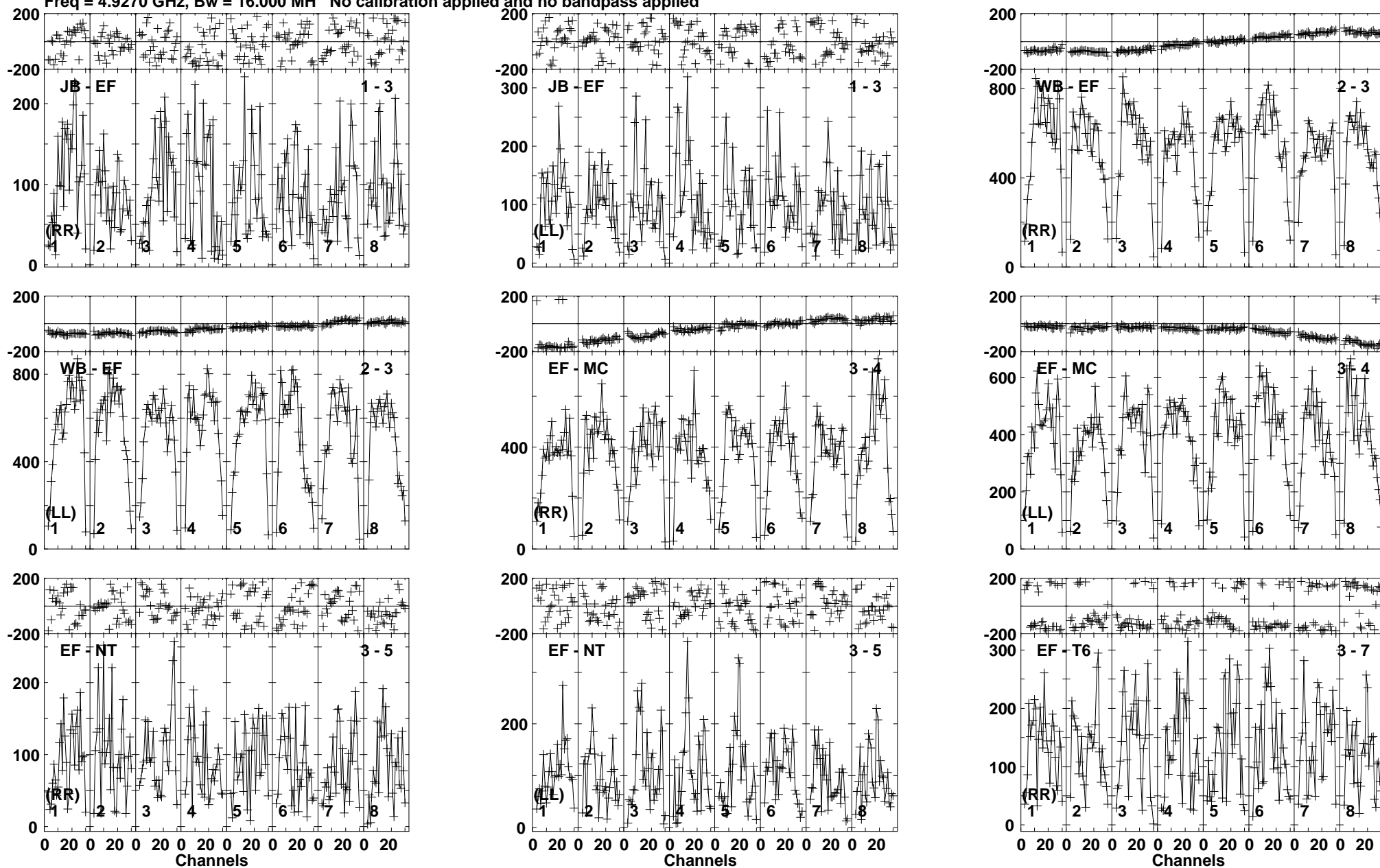
Lower frame: Micro Ampl Jy Top frame: Phas deg Vector averaged cross-power spectrum Baseline: JB (01) - EF (03) Timerange: 00/11:29:01 to 00/11:31:59
