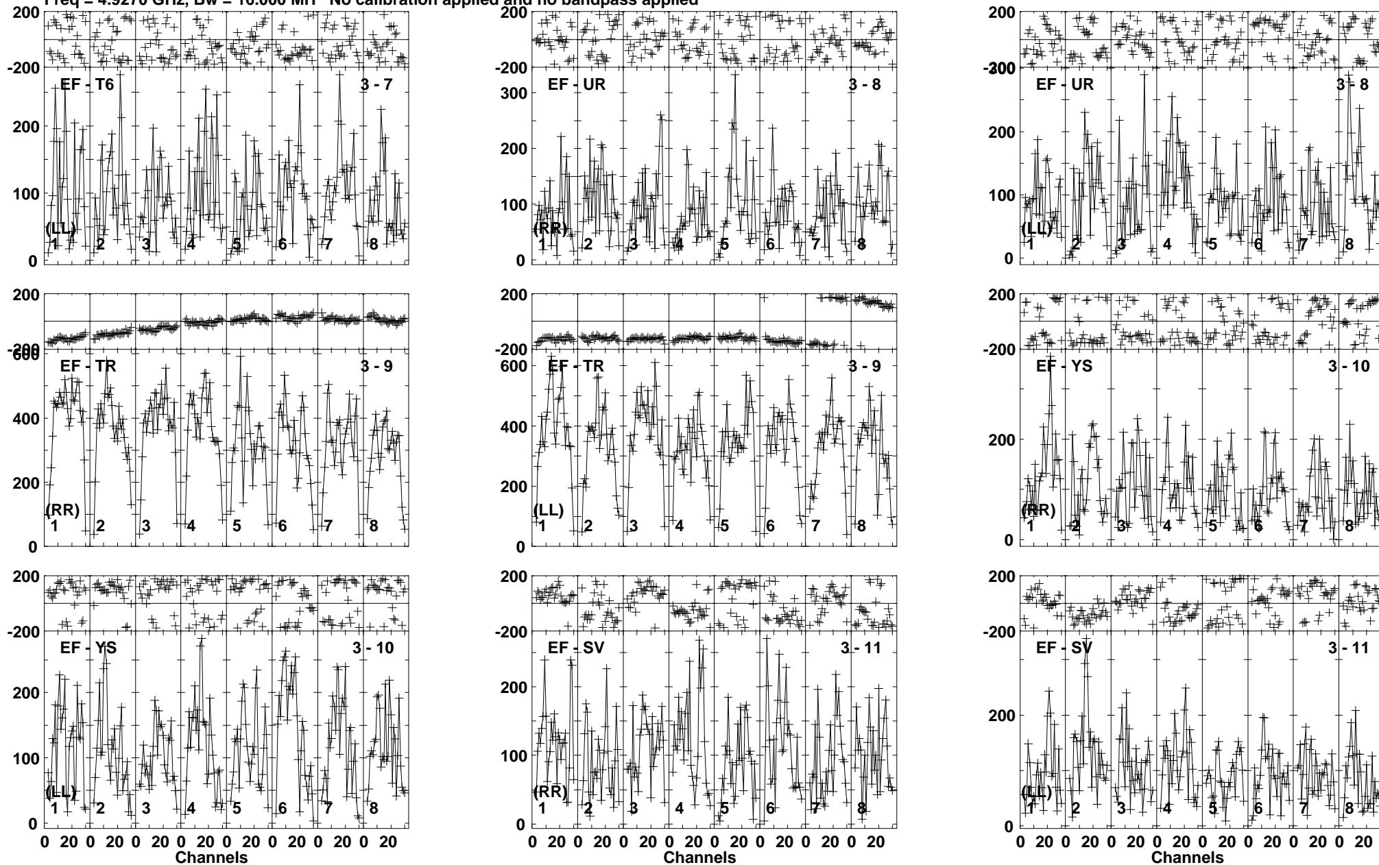
Lower frame: Micro Ampl Jy Top frame: Phas deg Vector averaged cross-power spectrum Baseline: EF (03) - T6 (07) Timerange: 00/10/06:31 to 00/10/09:29
