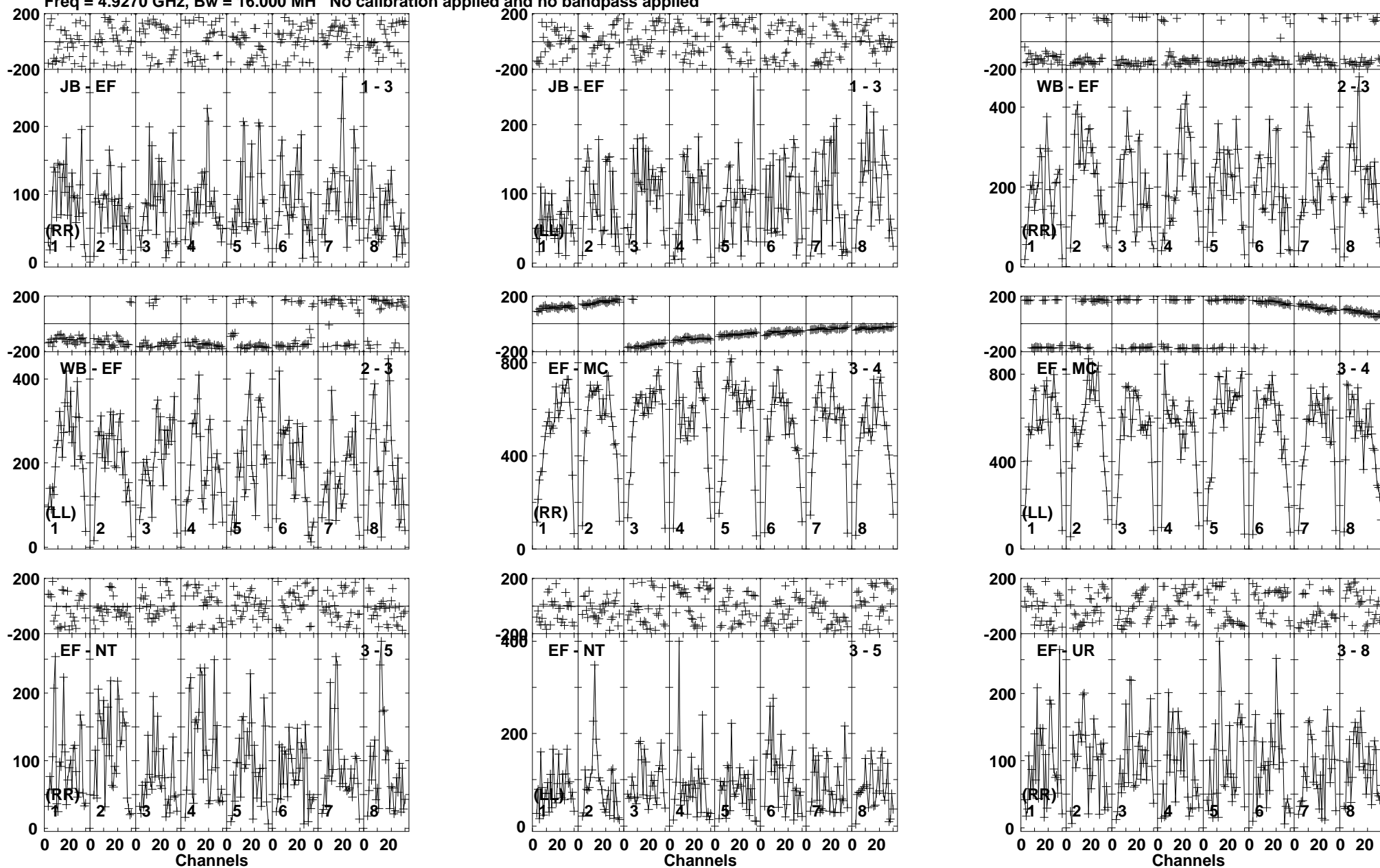
Lower frame: Micro Ampl Jy Top frame: Phas deg Vector averaged cross-power spectrum Baseline: JB (01) - EF (03) Timerange: 00/14:55:01 to 00/14:57:59
