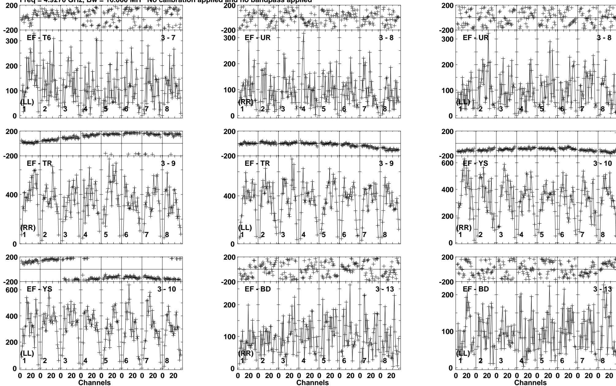
Lower frame: Micro Ampl Jy Top frame: Phas deg Vector averaged cross-power spectrum Baseline: EF (03) - T6 (07) Timerange: 00/11:45:31 to 00/11:48:29
