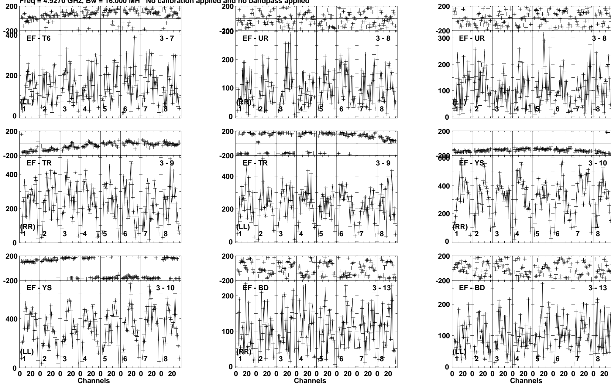
Lower frame: Micro Ampl Jy Top frame: Phas deg Vector averaged cross-power spectrum Baseline: EF (03) - T6 (07) Timerange: 00/12:18:31 to 00/12:21:29
