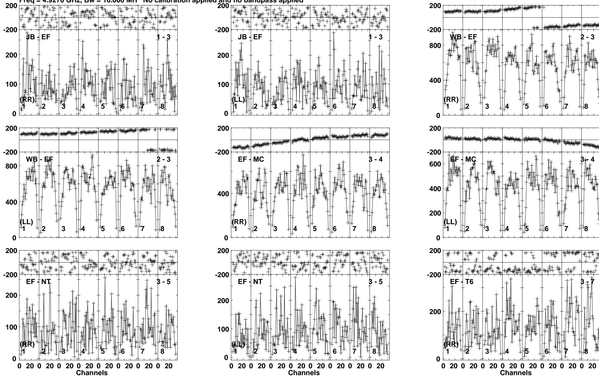
Lower frame: Micro Ampl Jy Top frame: Phas deg Vector averaged cross-power spectrum Baseline: JB (01) - EF (03) Timerange: 00/11:34:31 to 00/11:37:29
