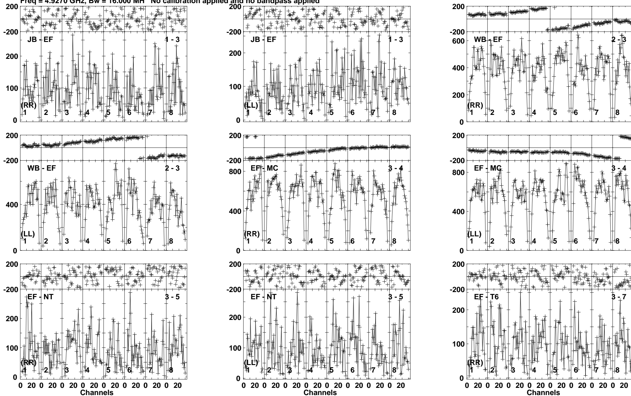
Lower frame: Micro Ampl Jy Top frame: Phas deg Vector averaged cross-power spectrum Baseline: JB (01) - EF (03) Timerange: 00/09:11:31 to 00/09:14:29
