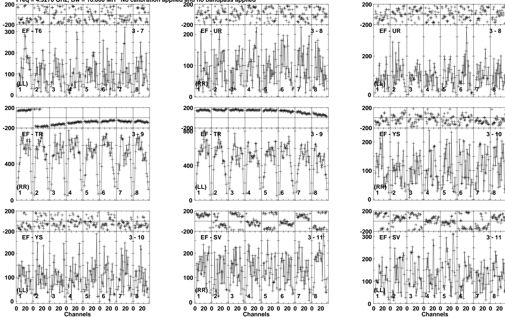
Lower frame: Micro Ampl Jy Top frame: Phas deg Vector averaged cross-power spectrum Baseline: EF (03) - T6 (07) Timerange: 00/09:00:31 to 00/09:03:29
