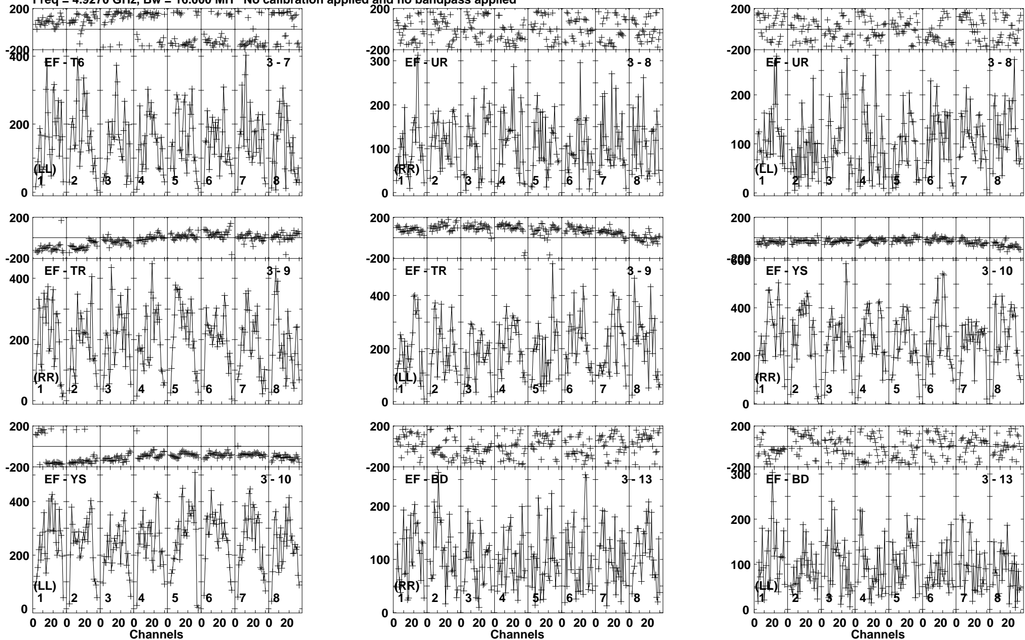
Lower frame: Micro Ampl Jy Top frame: Phas deg Vector averaged cross-power spectrum Baseline: EF (03) - T6 (07) Timerange: 00/12:29:31 to 00/12:32:29
