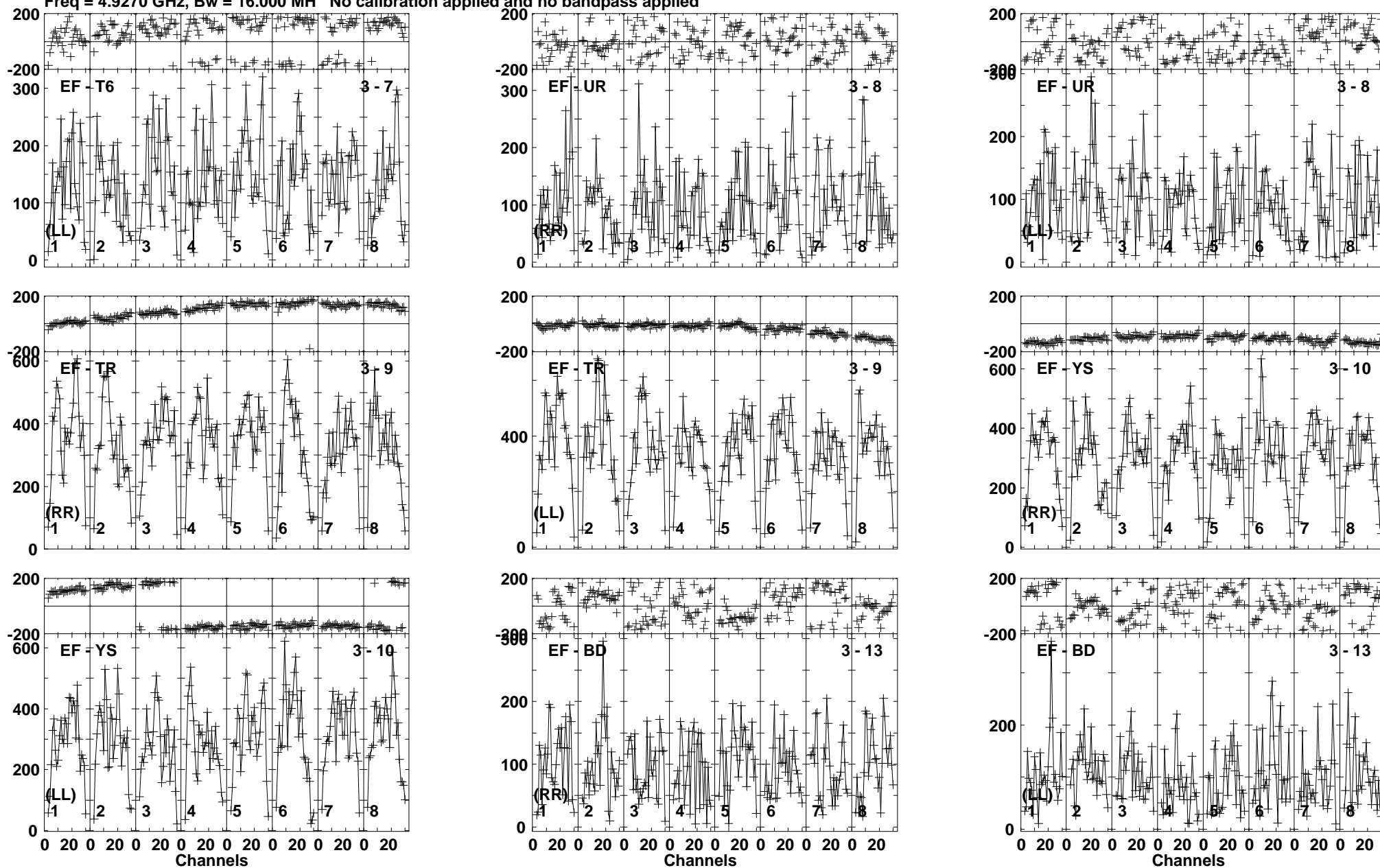
Lower frame: Micro Ampl Jy Top frame: Phas deg Vector averaged cross-power spectrum Baseline: EF (03) - T6 (07) Timerange: 00/11:34:31 to 00/11:37:29
