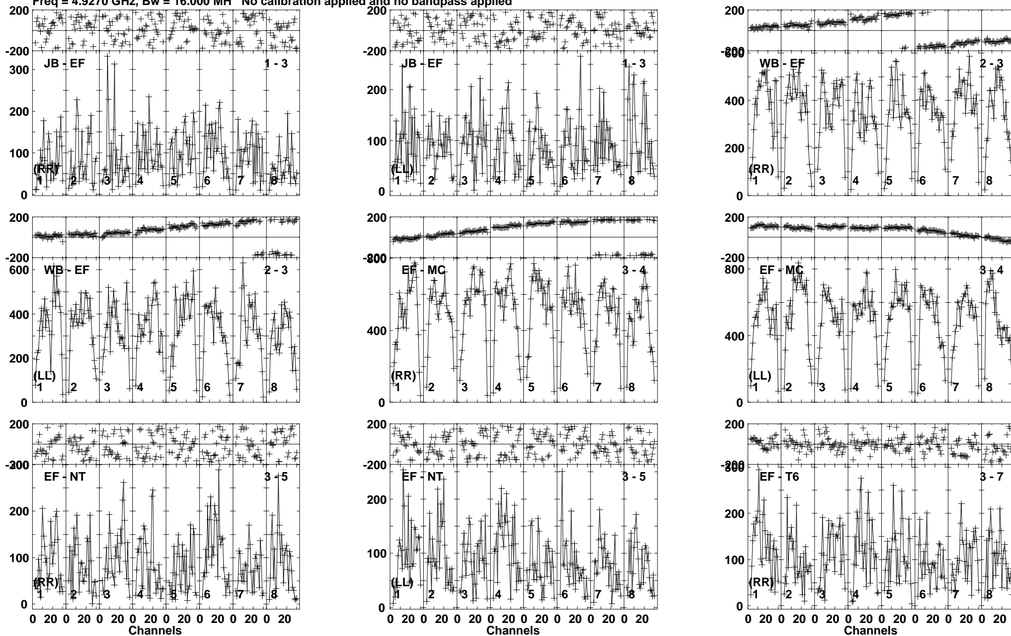
Lower frame: Micro Ampl Jy Top frame: Phas deg Vector averaged cross-power spectrum Baseline: JB (01) - EF (03) Timerange: 00/09:50:01 to 00/09:52:59
