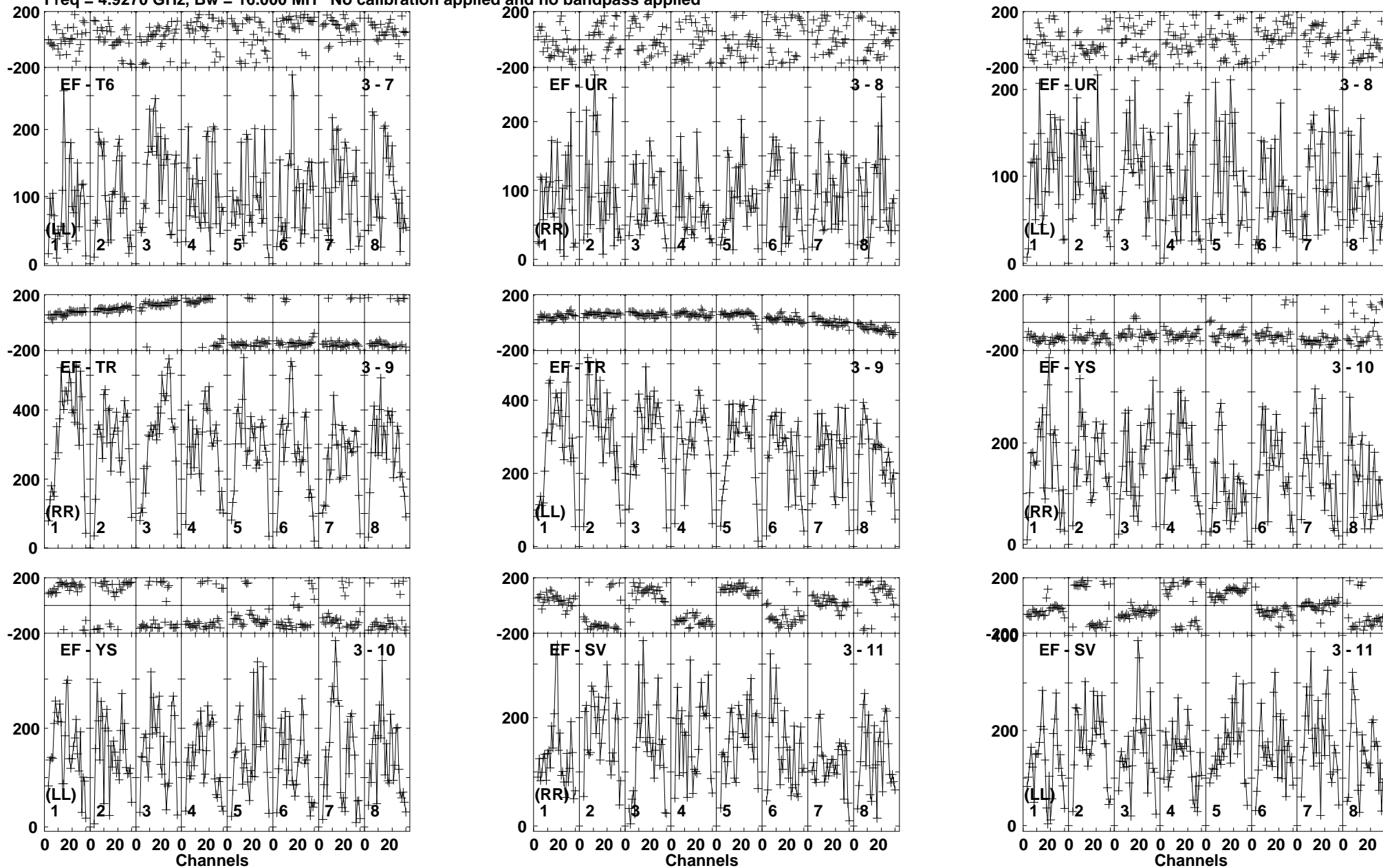
Lower frame: Micro Ampl Jy Top frame: Phas deg Vector averaged cross-power spectrum Baseline: EF (03) - T6 (07) Timerange: 00/10:28:31 to 00/10:31:29
