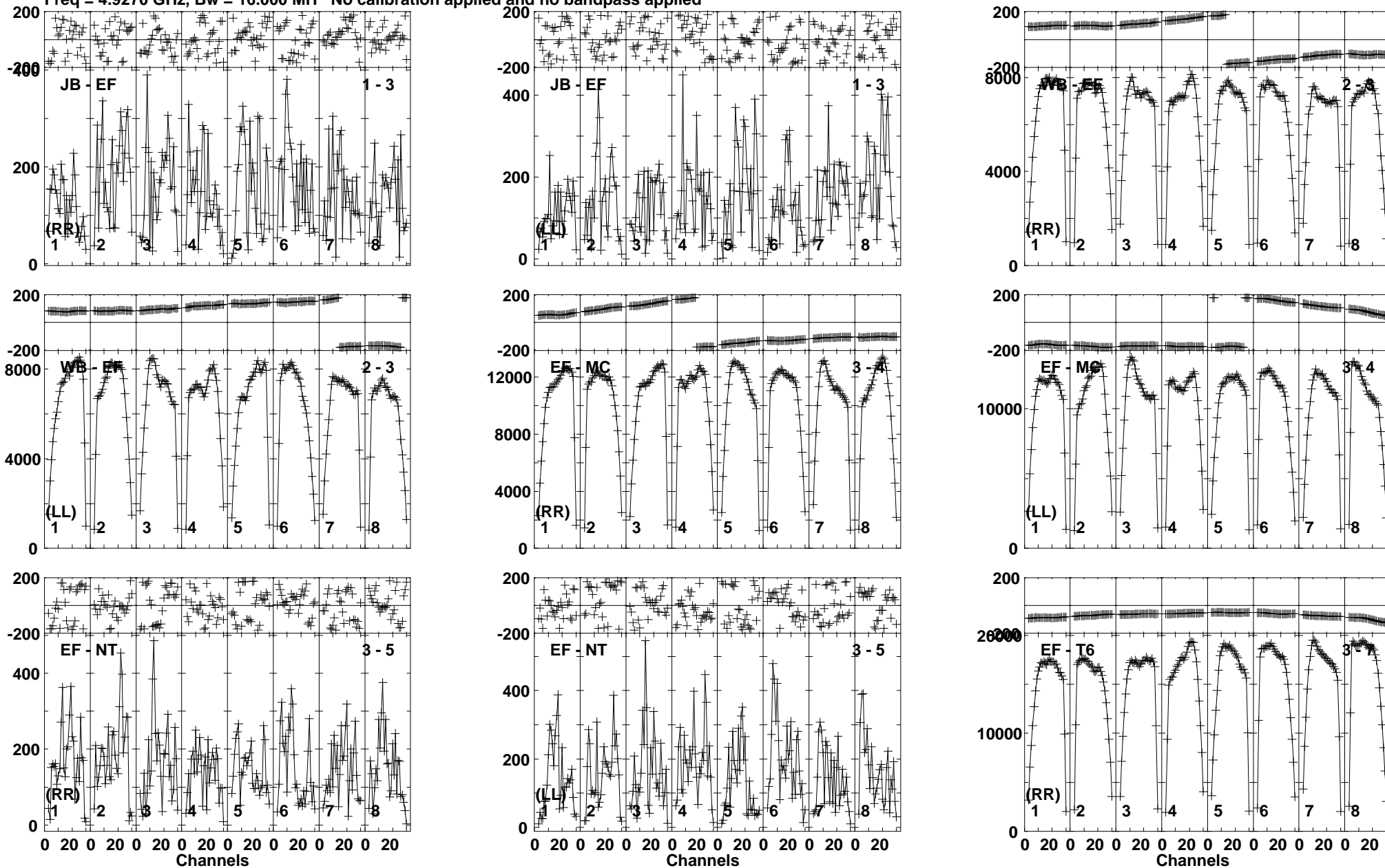
Lower frame: Micro Ampl Jy Top frame: Phas deg Vector averaged cross-power spectrum Baseline: JB (01) - EF (03) Timerange: 00/11:05:01 to 00/11:06:29
