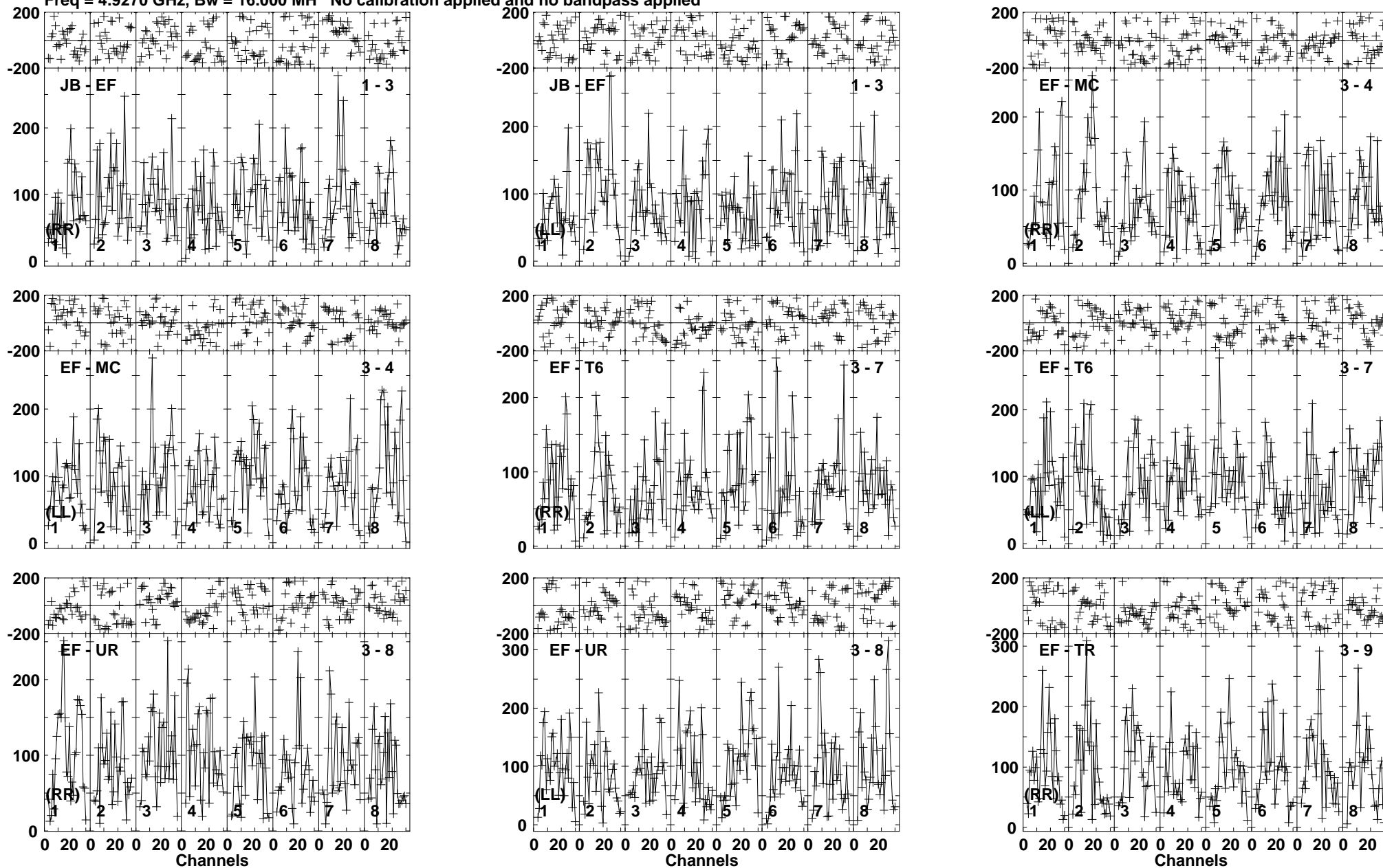
Lower frame: Micro Ampl Jy Top frame: Phas deg Vector averaged cross-power spectrum Baseline: JB (01) - EF (03) Timerange: 00/06:07:31 to 00/06:10:29
