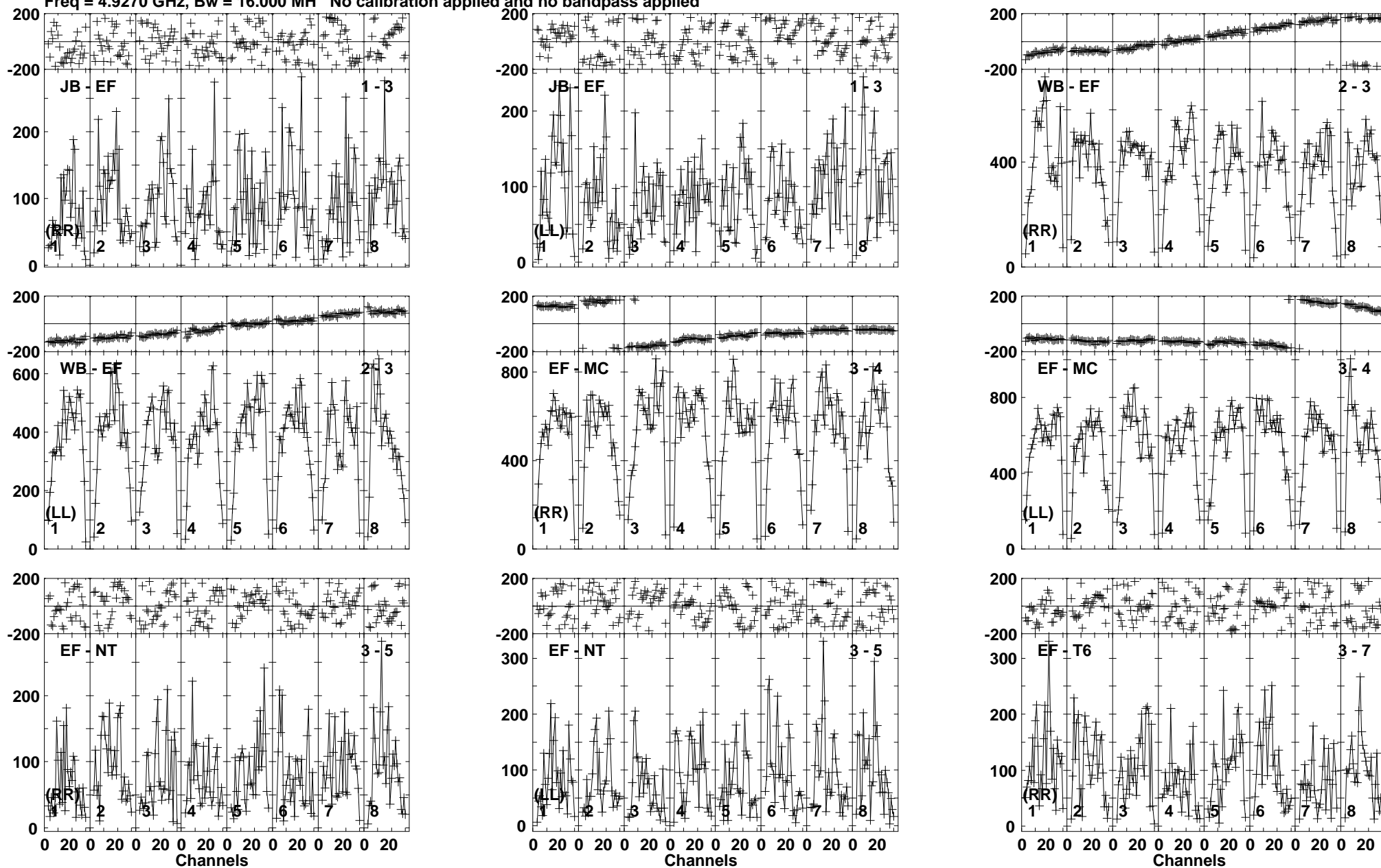
Lower frame: Micro Ampl Jy Top frame: Phas deg Vector averaged cross-power spectrum Baseline: JB (01) - EF (03) Timerange: 00/09:06:01 to 00/09:08:59
