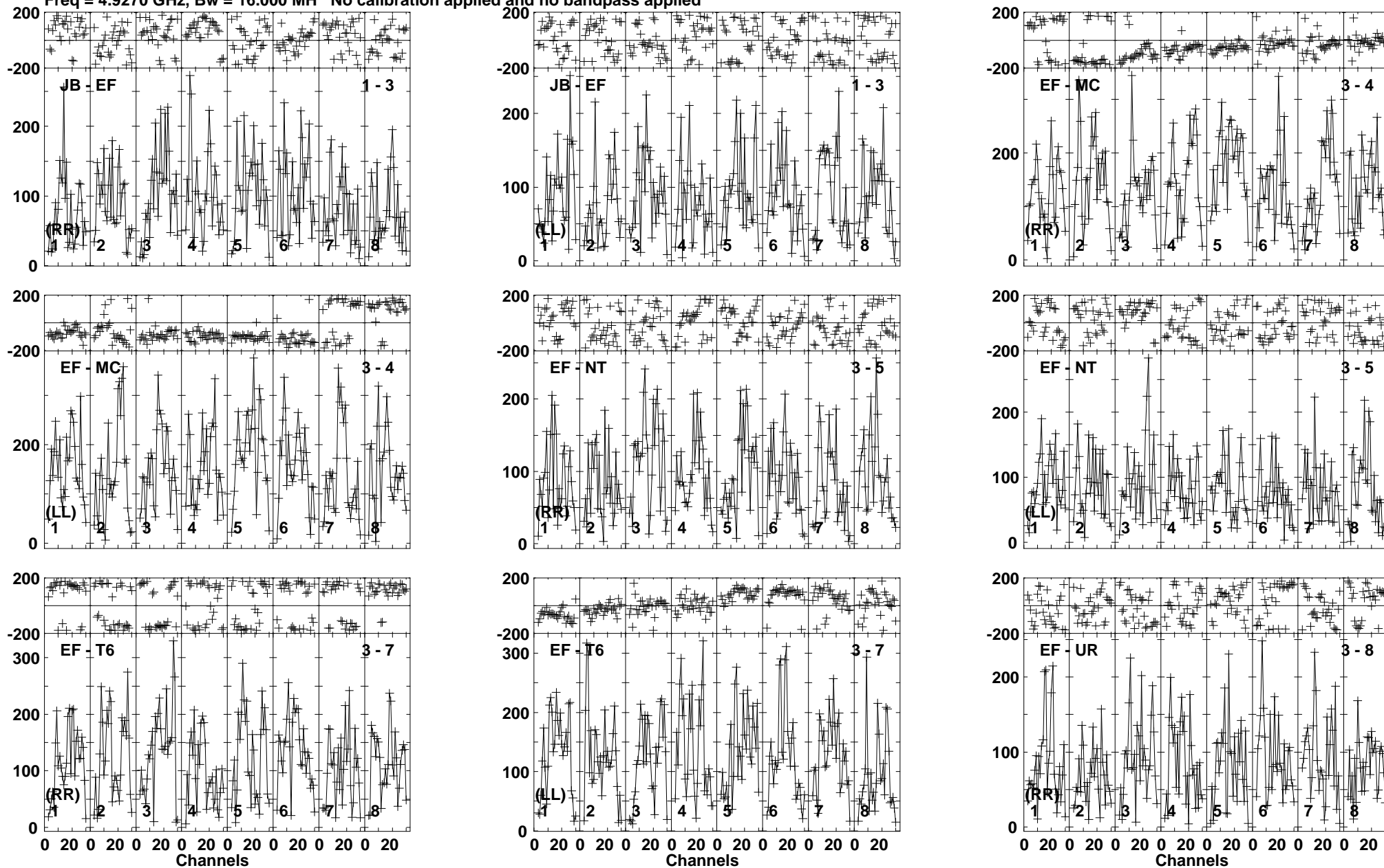
Lower frame: Micro Ampl Jy Top frame: Phas deg Vector averaged cross-power spectrum Baseline: JB (01) - EF (03) Timerange: 00/06:57:01 to 00/06:59:59
