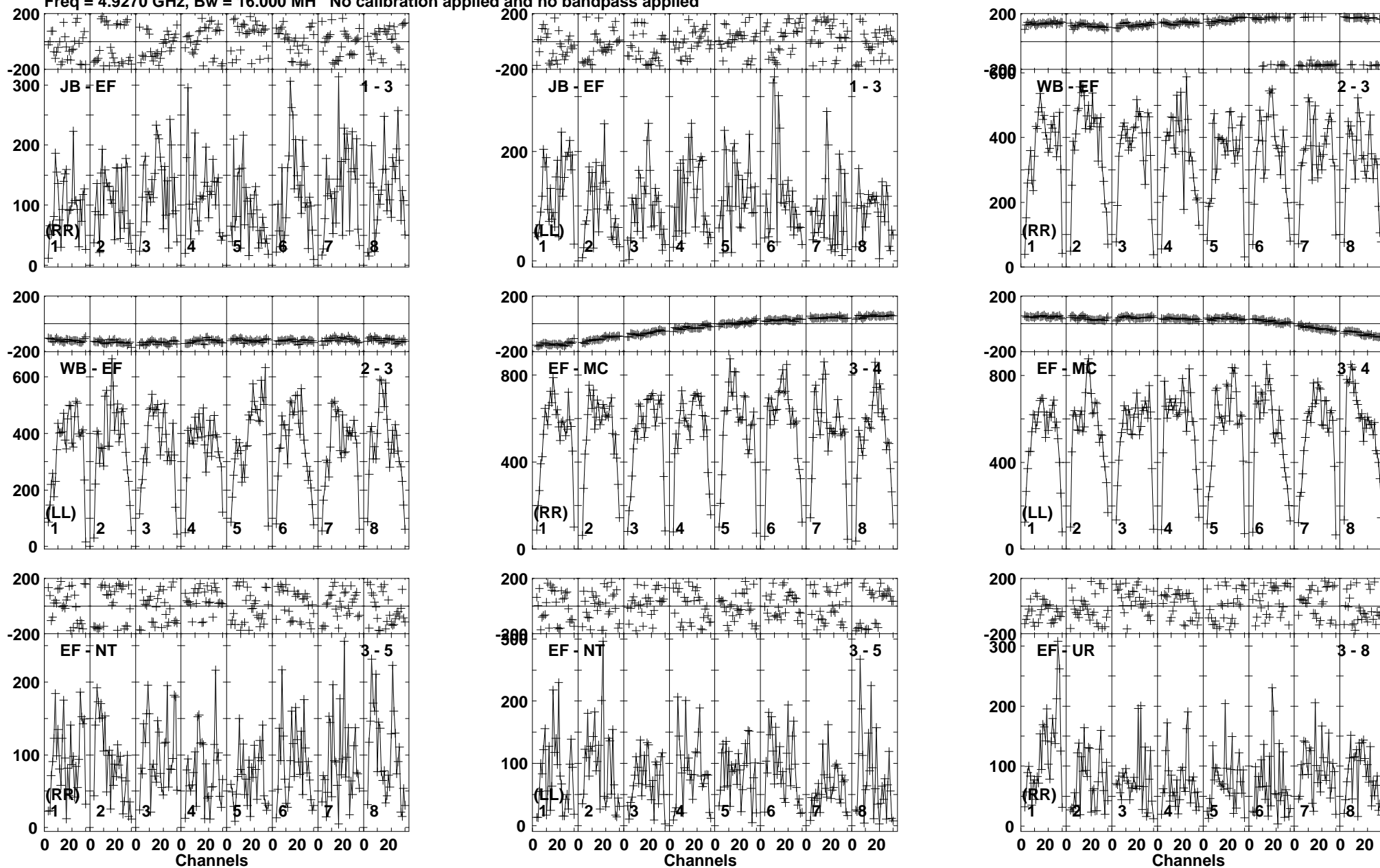
Lower frame: Micro Ampl Jy Top frame: Phas deg Vector averaged cross-power spectrum Baseline: JB (01) - EF (03) Timerange: 00/13:08:01 to 00/13:10:59
