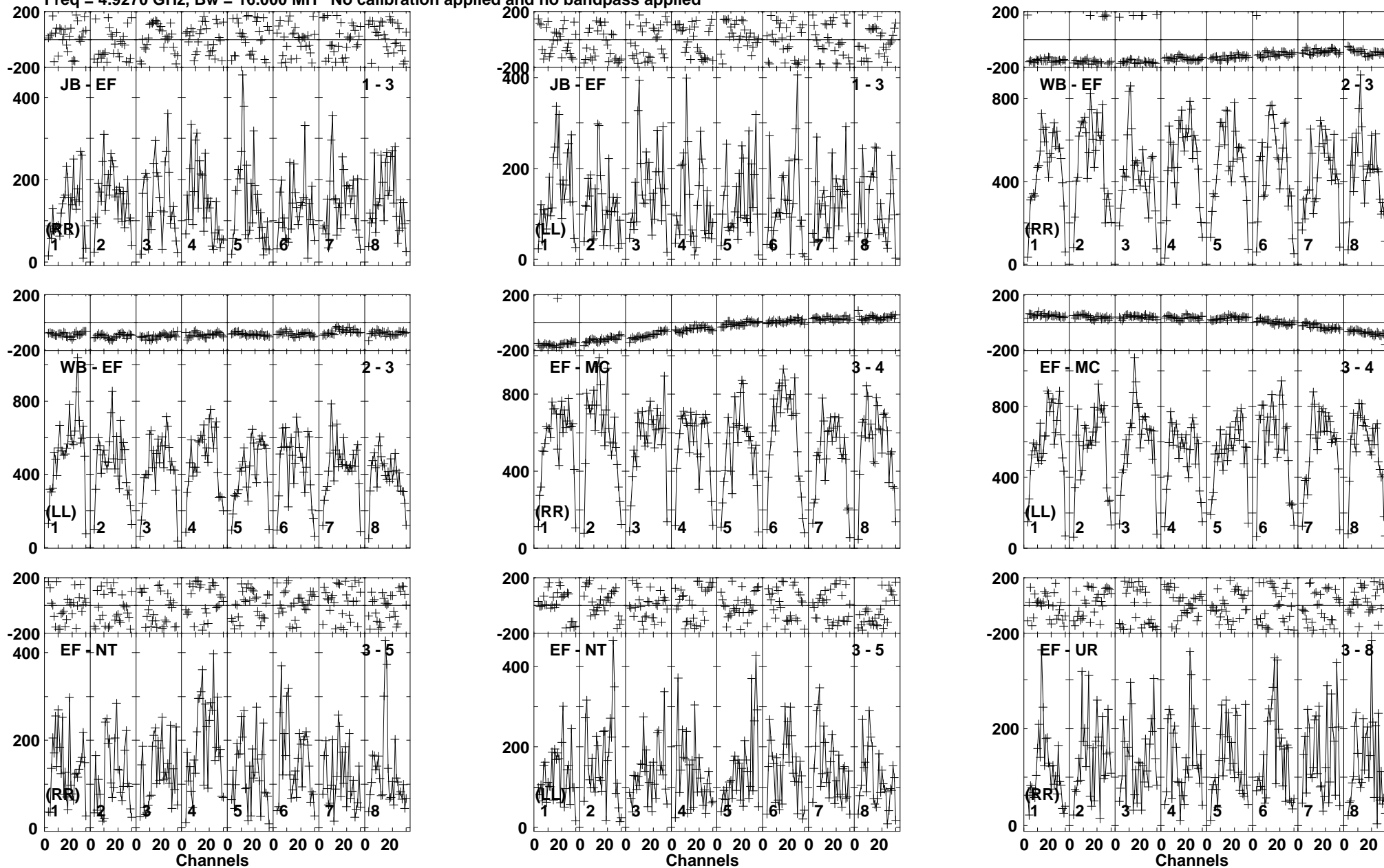
Lower frame: Micro Ampl Jy Top frame: Phas deg Vector averaged cross-power spectrum Baseline: JB (01) - EF (03) Timerange: 00/12:57:01 to 00/12:59:59
