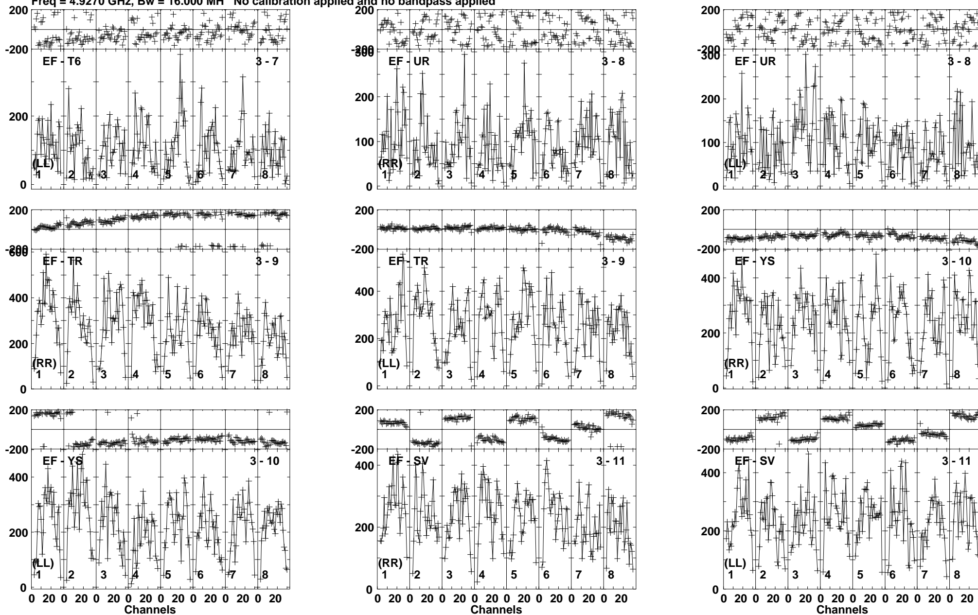
Lower frame: Micro Ampl Jy Top frame: Phas deg Vector averaged cross-power spectrum Baseline: EF (03) - T6 (07) Timerange: 00/10:56:01 to 00/10:58:59
