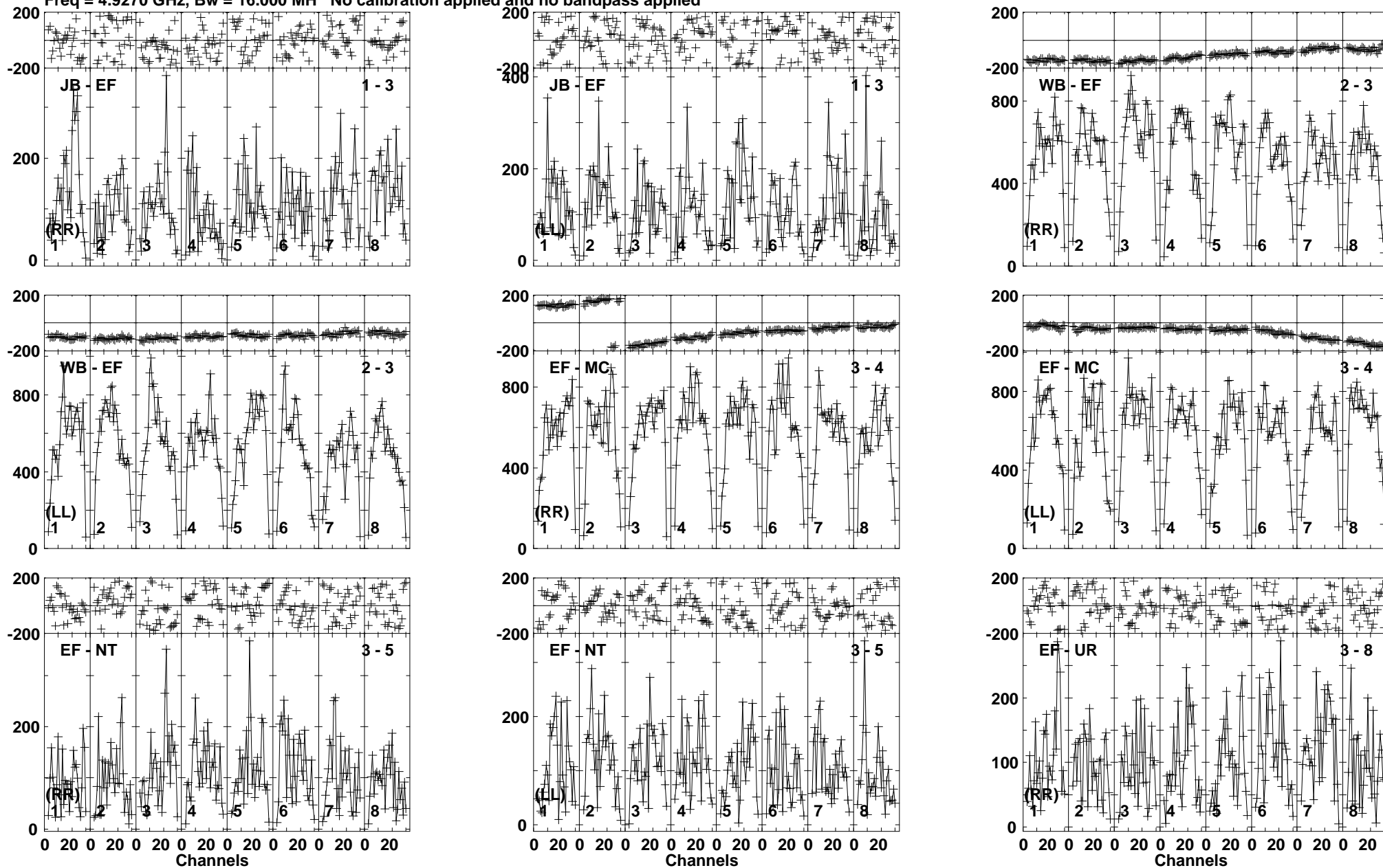
Lower frame: Micro Ampl Jy Top frame: Phas deg Vector averaged cross-power spectrum Baseline: JB (01) - EF (03) Timerange: 00:12:40:31 to 00:12:43:29
