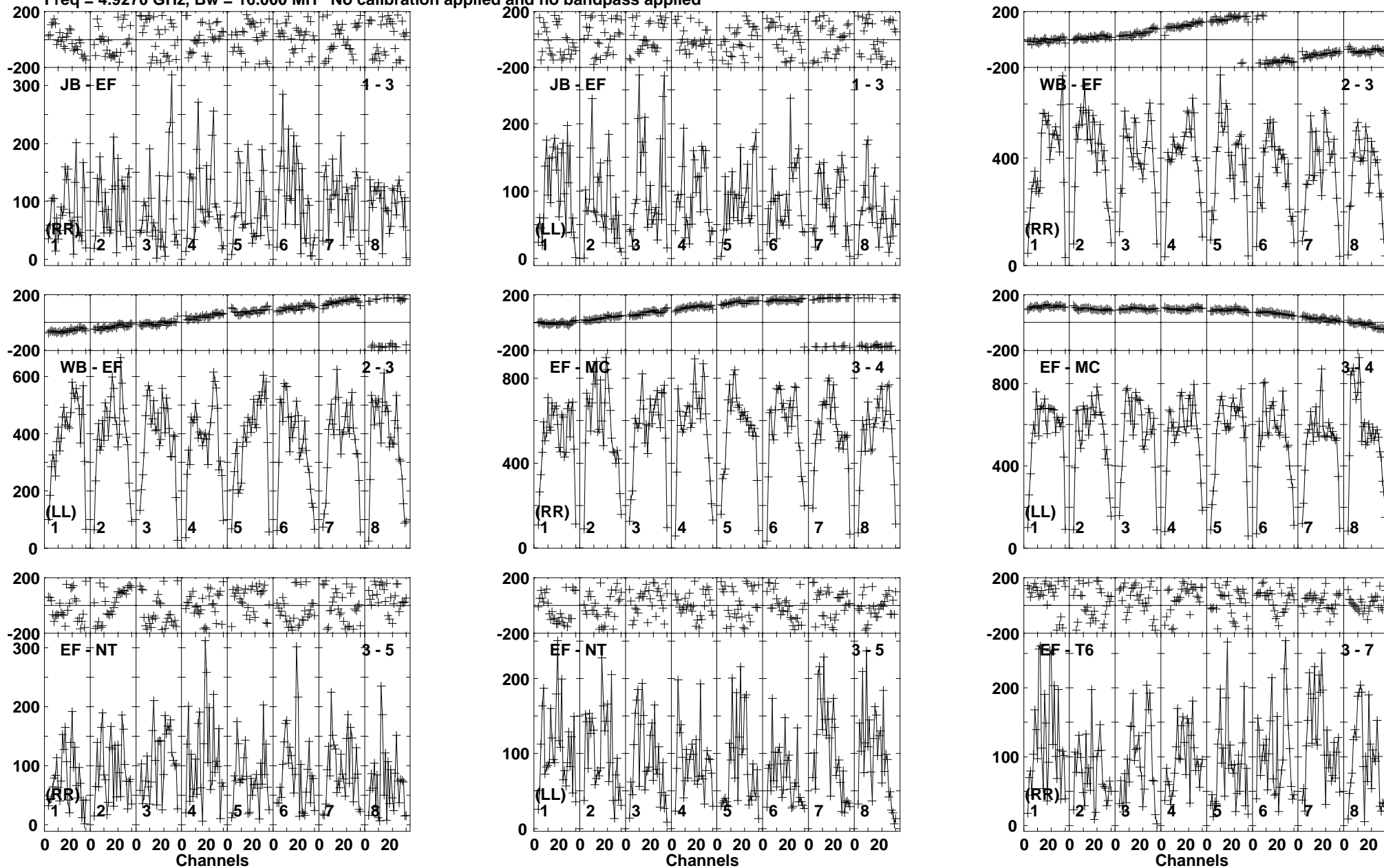
Lower frame: Micro Ampl Jy Top frame: Phas deg Vector averaged cross-power spectrum Baseline: JB (01) - EF (03) Timerange: 00/08:33:01 to 00/08:35:59
