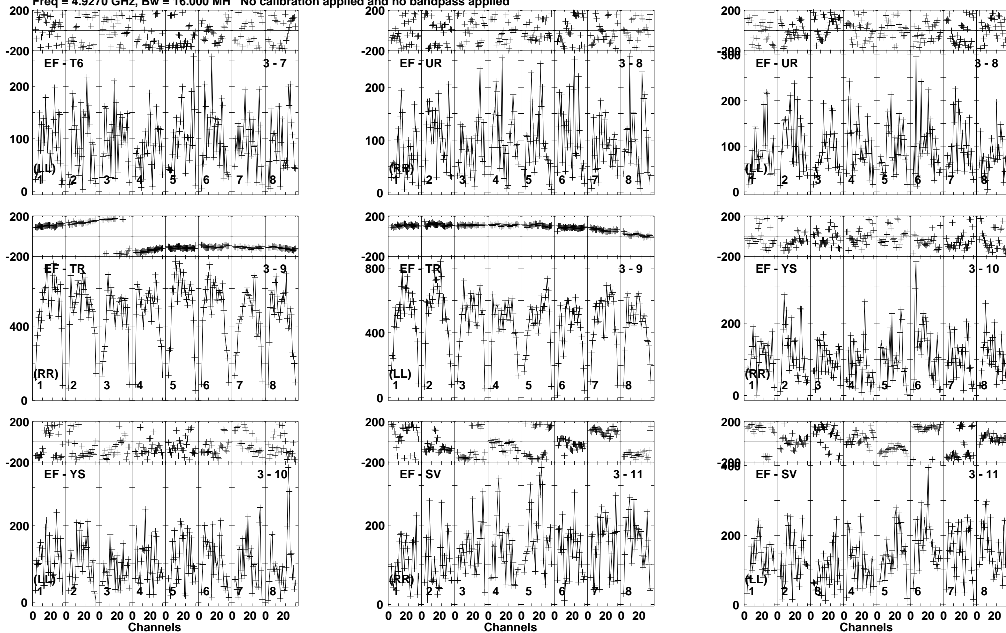
Lower frame: Micro Ampl Jy Top frame: Phas deg Vector averaged cross-power spectrum Baseline: EF (03) - T6 (07) Timerange: 00/08:55:01 to 00/08:57:59
