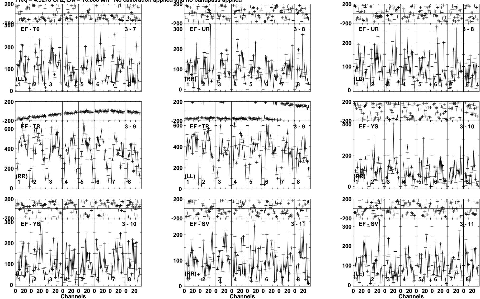
Lower frame: Micro Ampl Jy Top frame: Phas deg Vector averaged cross-power spectrum Baseline: EF (03) - T6 (07) Timerange: 00/09:50:01 to 00/09:52:59
