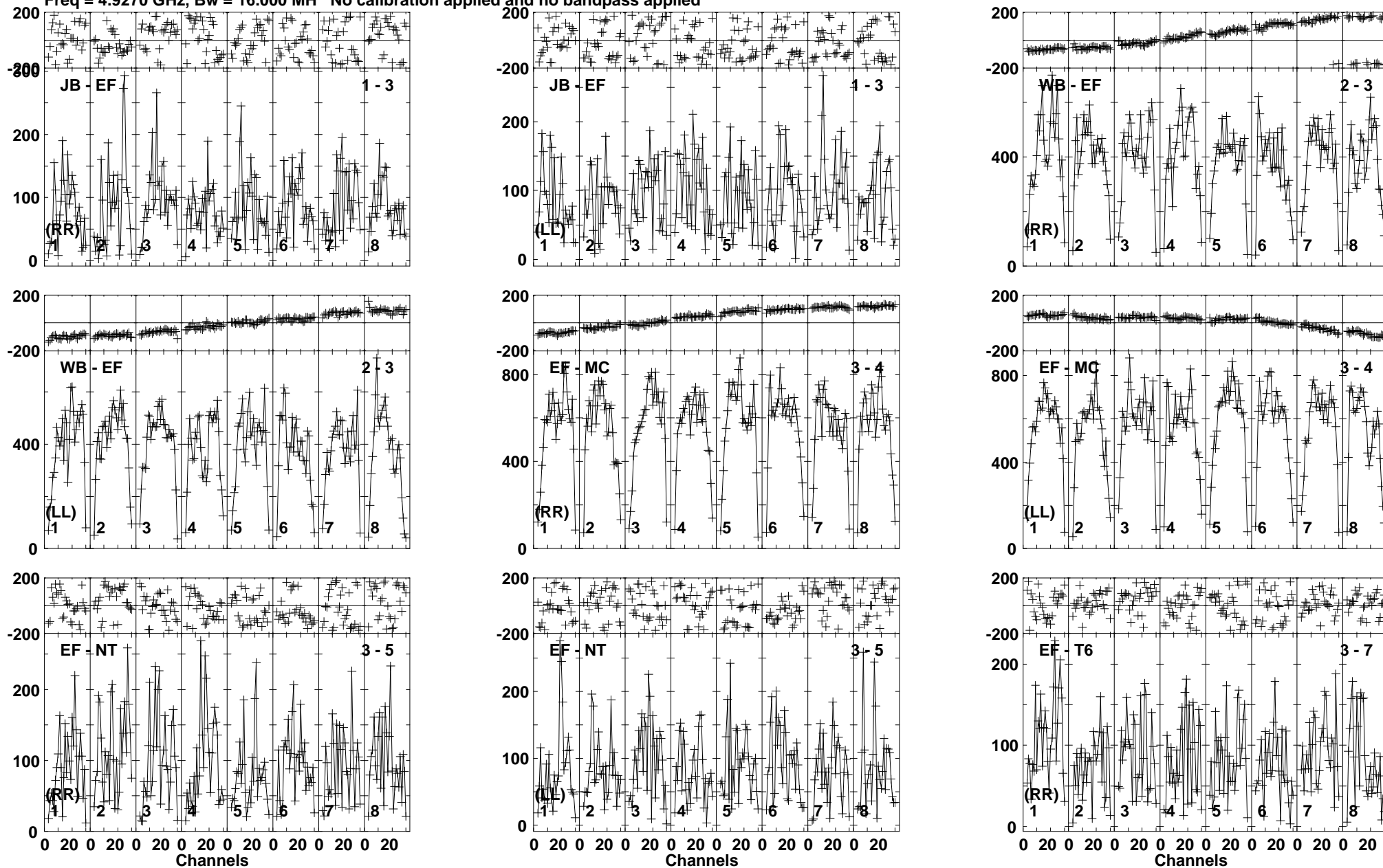
Lower frame: Micro Ampl Jy Top frame: Phas deg Vector averaged cross-power spectrum Baseline: JB (01) - EF (03) Timerange: 00/09:22:31 to 00/09:25:29
