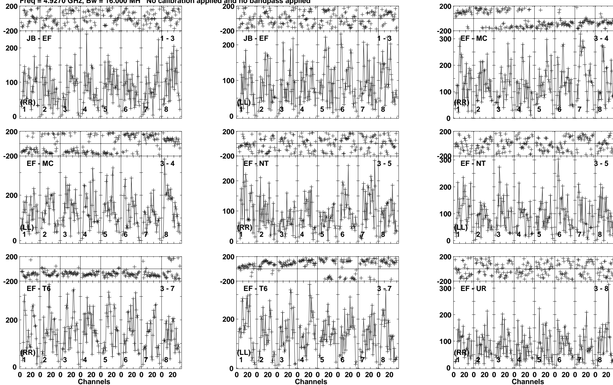
Lower frame: Micro Ampl Jy Top frame: Phas deg Vector averaged cross-power spectrum Baseline: JB (01) - EF (03) Timerange: 00/06:46:01 to 00/06:48:59
