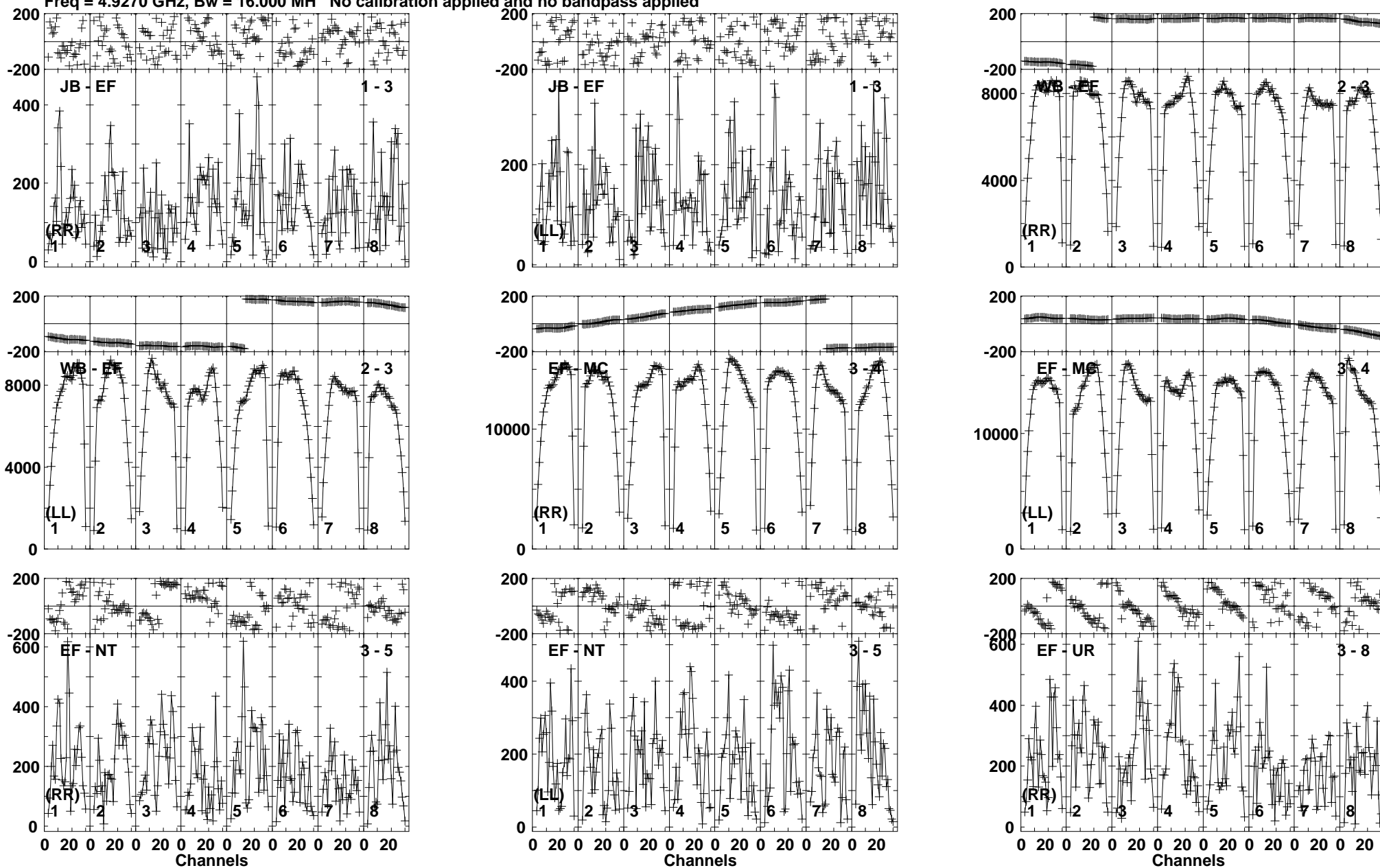
Lower frame: Micro Ampl Jy Top frame: Phas deg Vector averaged cross-power spectrum Baseline: JB (01) - EF (03) Timerange: 00/15:26:01 to 00/15:27:29
