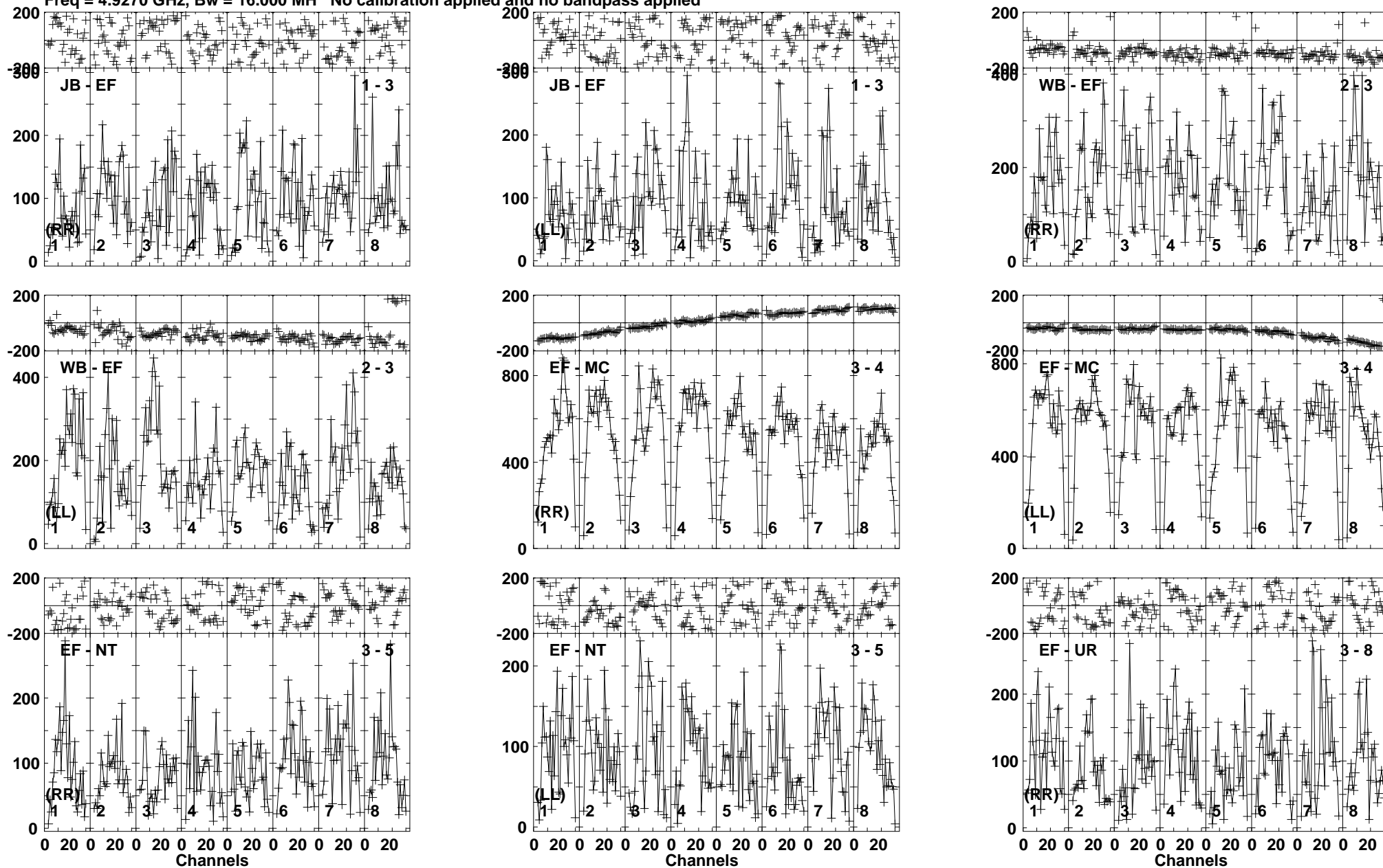
Lower frame: Micro Ampl Jy Top frame: Phas deg Vector averaged cross-power spectrum Baseline: JB (01) - EF (03) Timerange: 00/15:22:31 to 00/15:25:29
