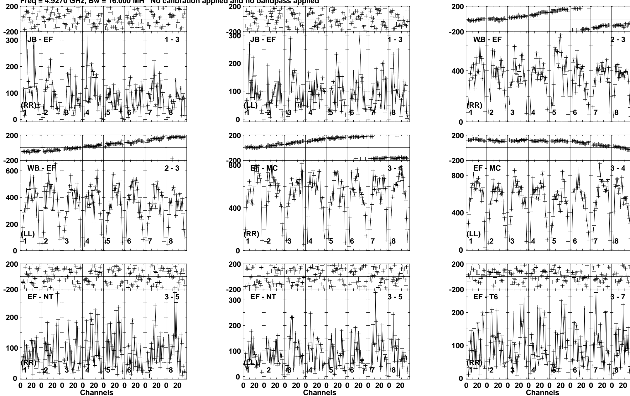
Lower frame: Micro Ampl Jy Top frame: Phas deg Vector averaged cross-power spectrum Baseline: JB (01) - EF (03) Timerange: 00/08:44:01 to 00/08:46:59
