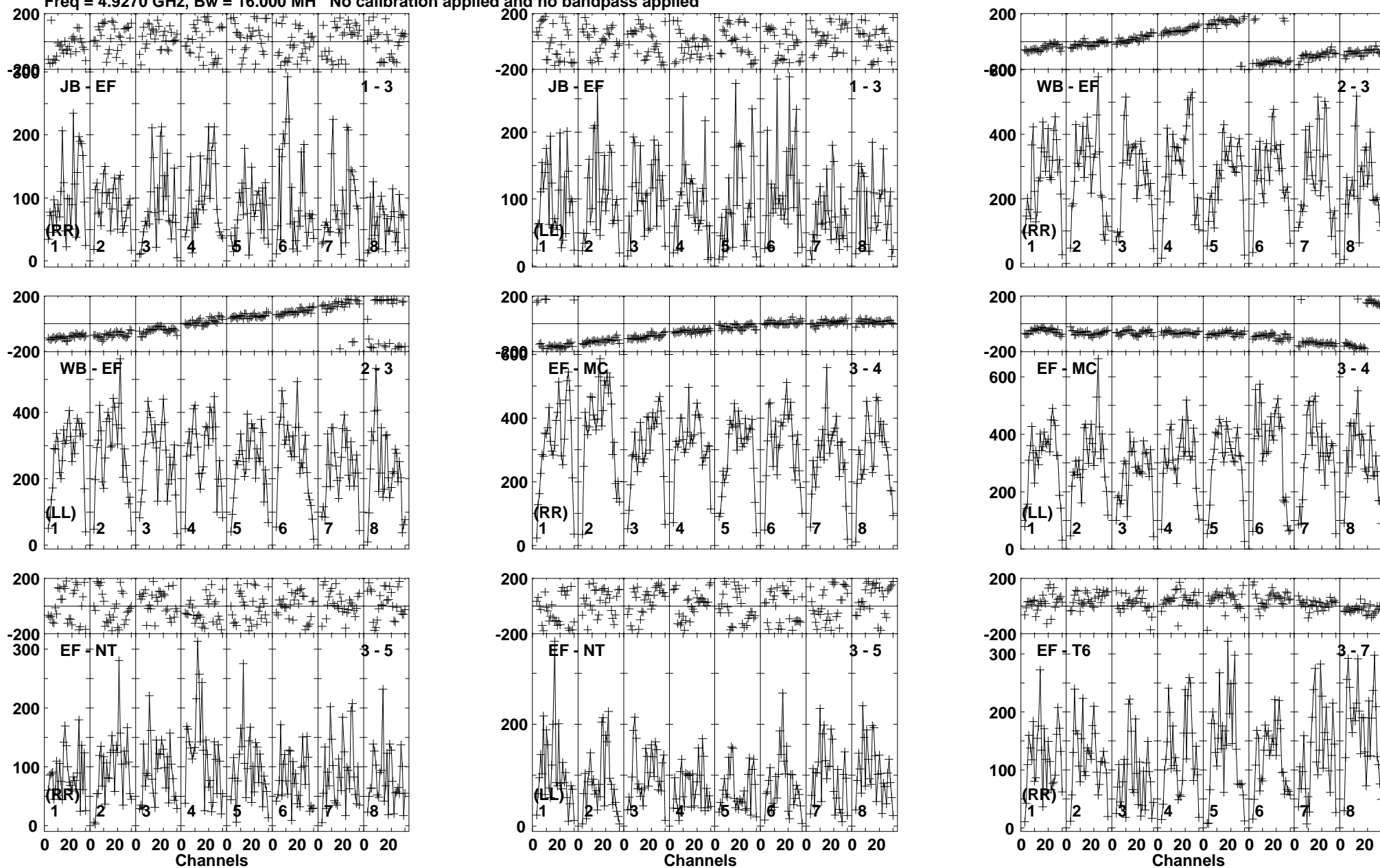
Lower frame: Micro Ampl Jy Top frame: Phas deg Vector averaged cross-power spectrum Baseline: JB (01) - EF (03) Timerange: 00/07:35:31 to 00/07:38:29
