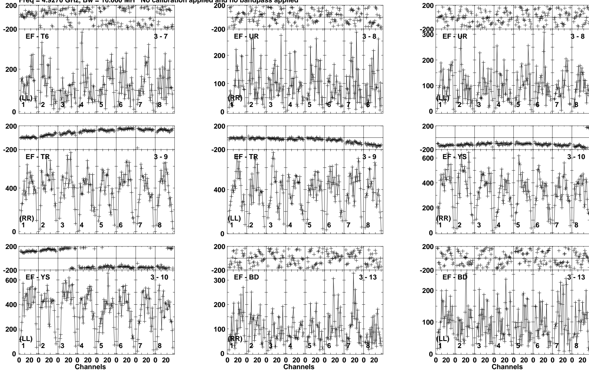
Lower frame: Micro Ampl Jy Top frame: Phas deg Vector averaged cross-power spectrum Baseline: EF (03) - T6 (07) Timerange: 00/11:56:31 to 00/11:59:29
