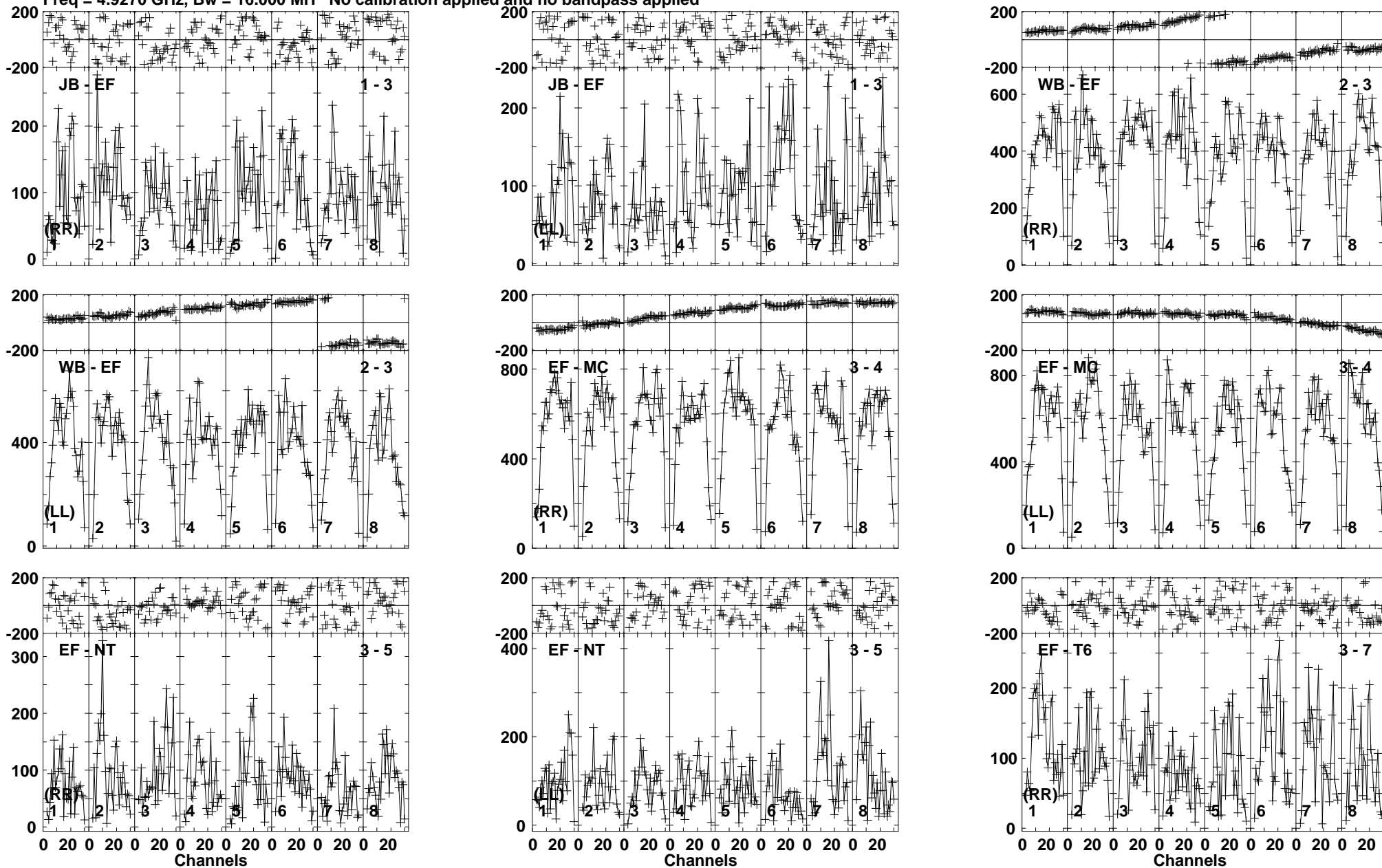
Lower frame: Micro Ampl Jy Top frame: Phas deg Vector averaged cross-power spectrum Baseline: JB (01) - EF (03) Timerange: 00/09:39:01 to 00/09:41:59
