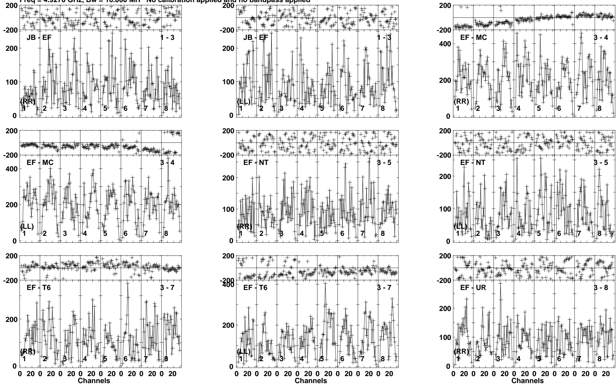
Lower frame: Micro Ampl Jy Top frame: Phas deg Vector averaged cross-power spectrum Baseline: JB (01) - EF (03) Timerange: 00/07:13:31 to 00/07:16:29
