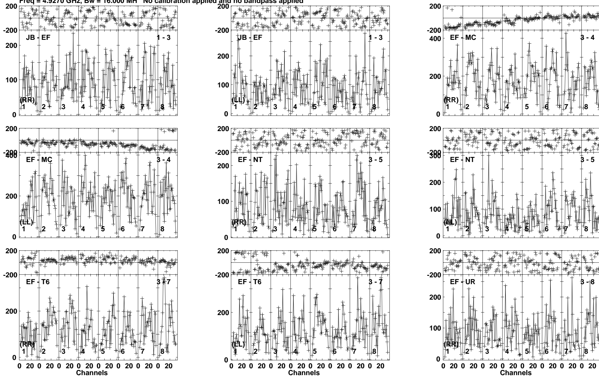
Lower frame: Micro Ampl Jy Top frame: Phas deg Vector averaged cross-power spectrum Baseline: JB (01) - EF (03) Timerange: 00/07:08:01 to 00/07:10:59
