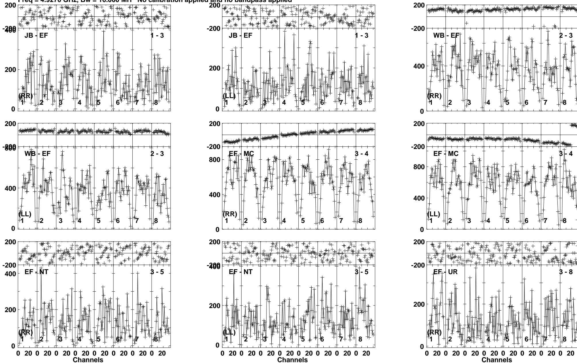
Lower frame: Micro Ampl Jy Top frame: Phas deg Vector averaged cross-power spectrum Baseline: JB (01) - EF (03) Timerange: 00/13:43:31 to 00/13:46:29
