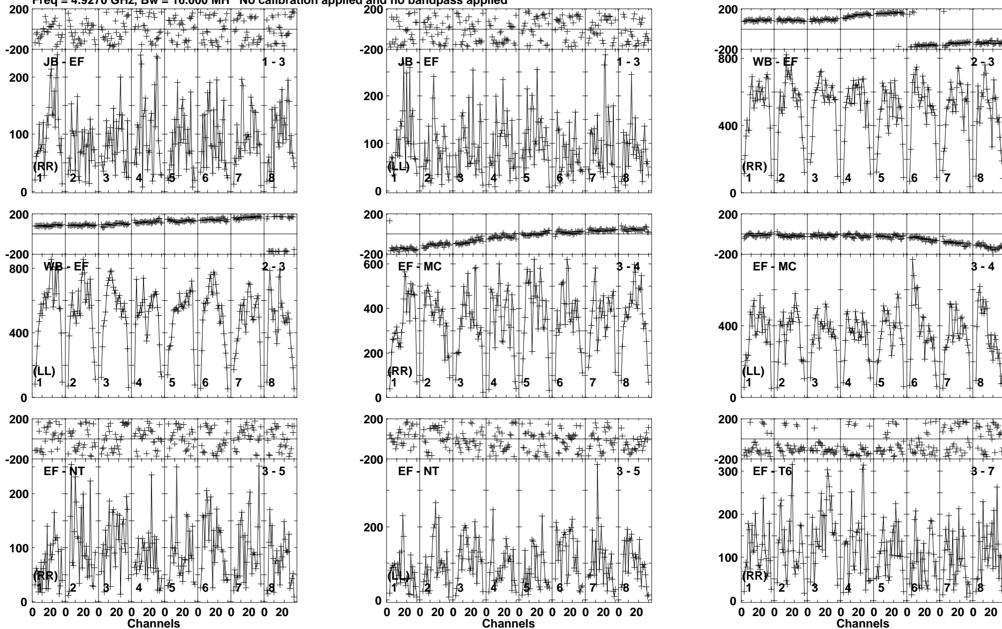
Lower frame: Micro Ampl Jy Top frame: Phas deg Vector averaged cross-power spectrum Baseline: JB (01) - EF (03) Timerange: 00/11:23:31 to 00/11:26:29
