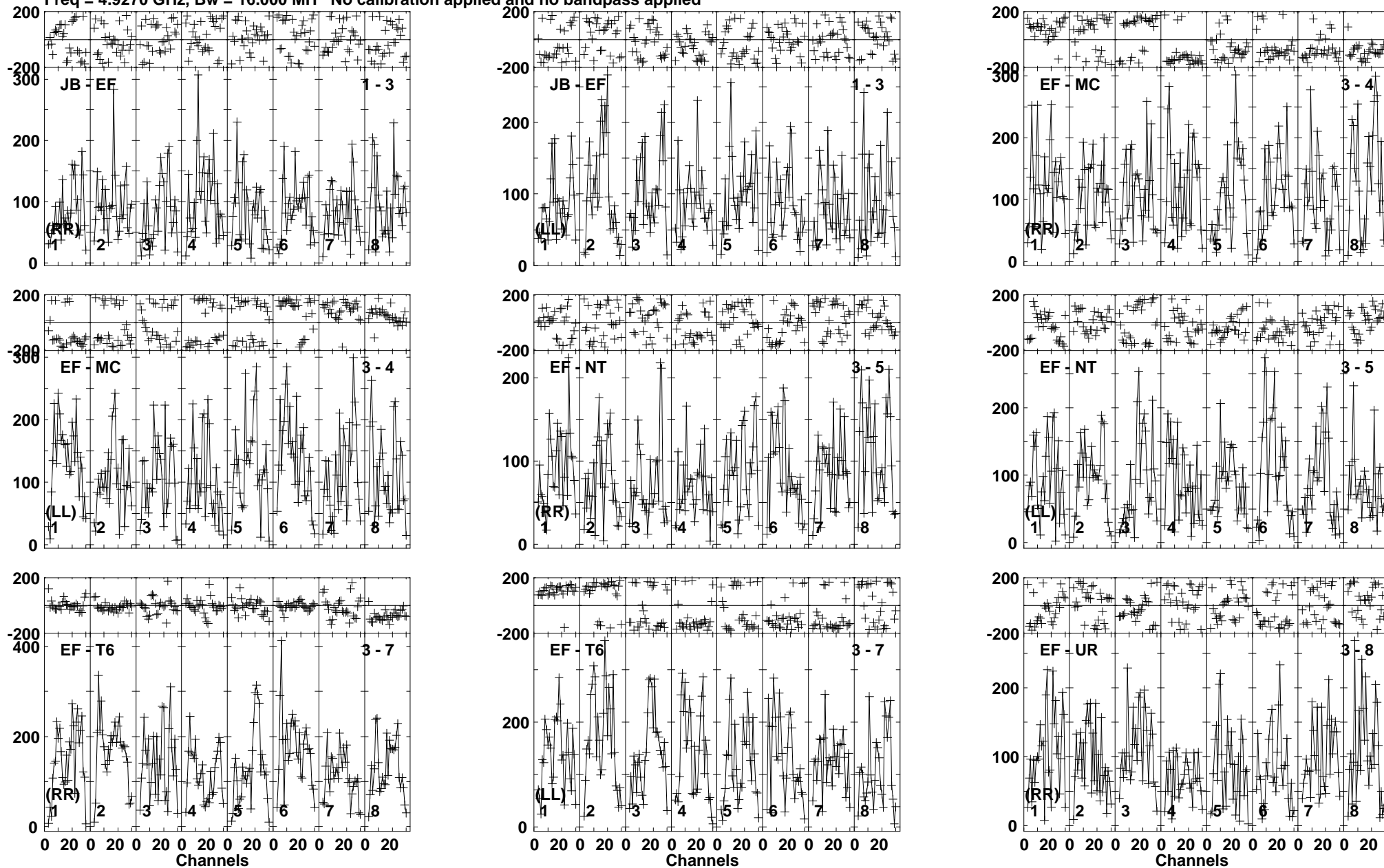
Lower frame: Micro Ampl Jy Top frame: Phas deg Vector averaged cross-power spectrum Baseline: JB (01) - EF (03) Timerange: 00/06:40:31 to 00/06:43:29
