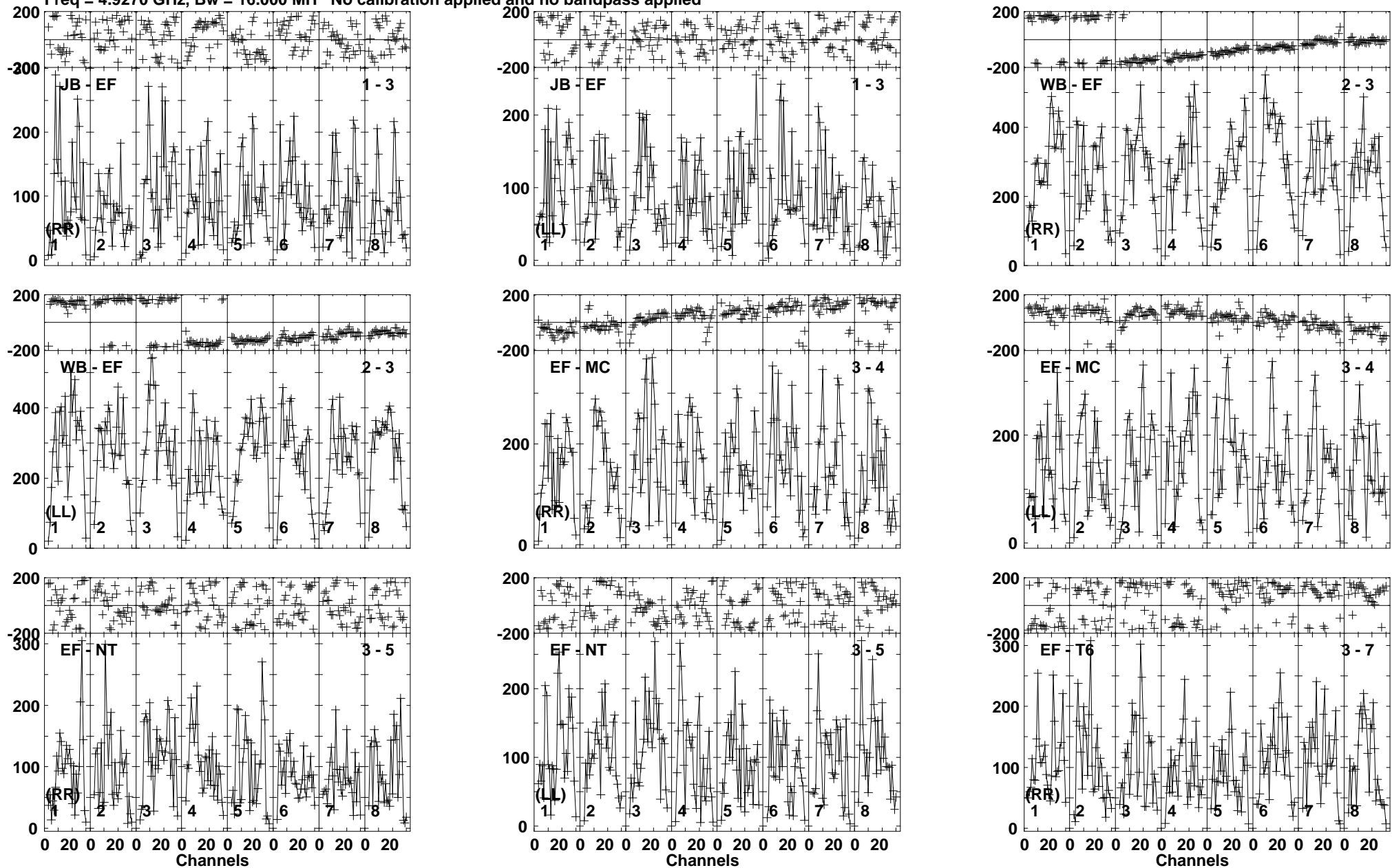
Lower frame: Micro Ampl Jy Top frame: Phas deg Vector averaged cross-power spectrum Baseline: JB (01) - EF (03) Timerange: 00/10:34:01 to 00/10:36:59
