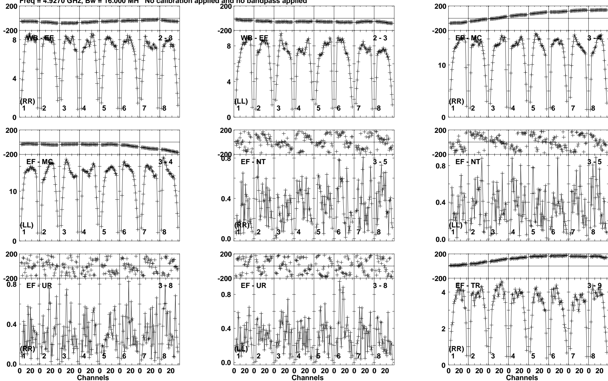
Lower frame: Milli Ampl Jy Top frame: Phas deg Vector averaged cross-power spectrum Baseline: WB (02) - EF (03) Timerange: 00/13:58:01 to 00/13:59:29
