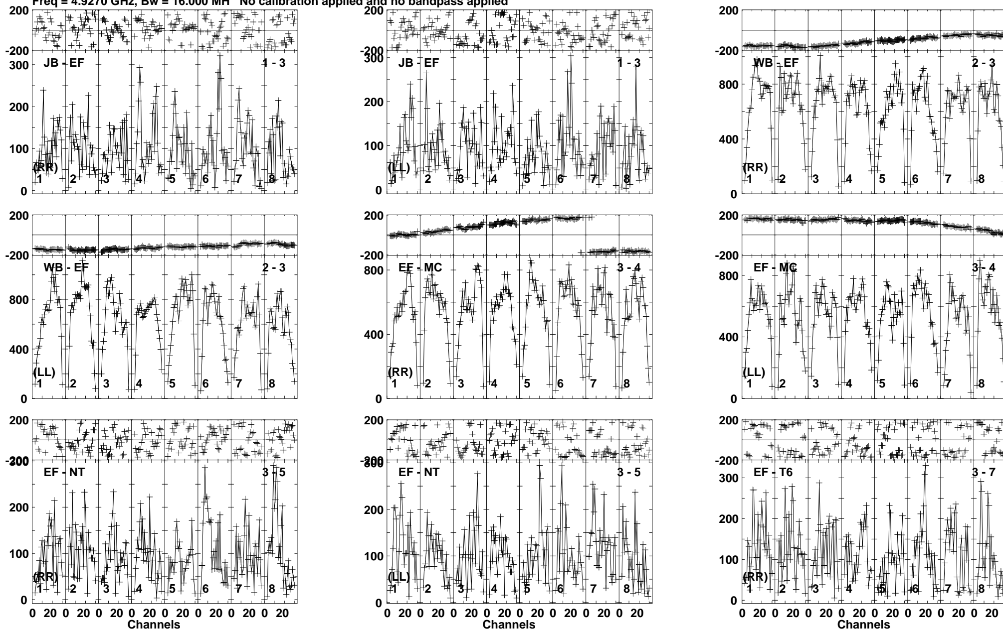
Lower frame: Micro Ampl Jy Top frame: Phas deg Vector averaged cross-power spectrum Baseline: JB (01) - EF (03) Timerange: 00:12:02:01 to 00:12:04:59
