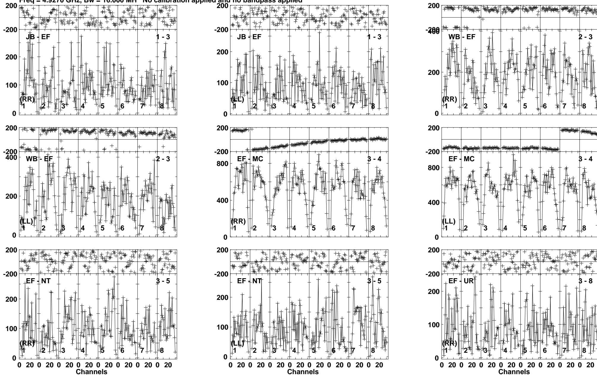
Lower frame: Micro Ampl Jy Top frame: Phas deg Vector averaged cross-power spectrum Baseline: JB (01) - EF (03) Timerange: 00/15:06:01 to 00/15:08:59
