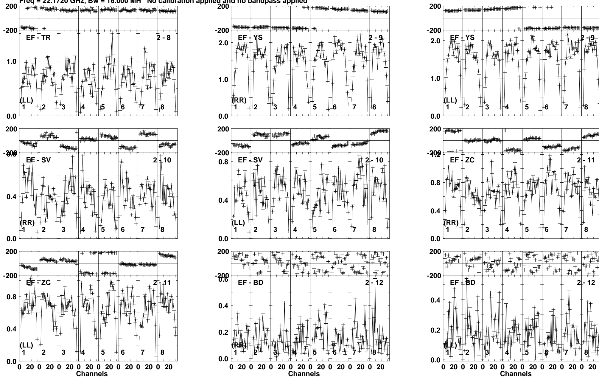
Lower frame: Milli Ampl Jy Top frame: Phas deg Vector averaged cross-power spectrum Baseline: EF (02) - TR (08) Timerange: 00/07:09:31 to 00/07:10:29
