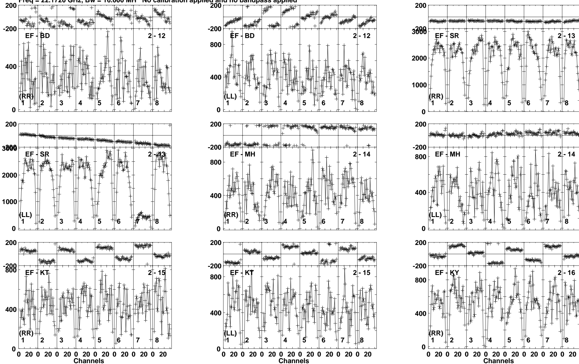
Lower frame: Micro Ampl Jy Top frame: Phas deg Vector averaged cross-power spectrum Baseline: EF (02) - BD (12) Timerange: 00/10:12:51 to 00/10:13:49
