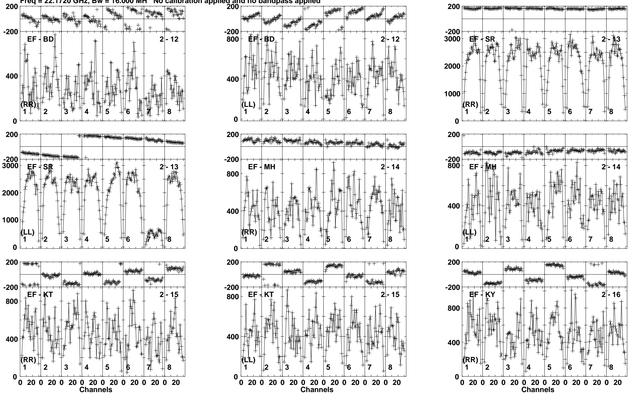
Lower frame: Micro Ampl Jy Top frame: Phas deg Vector averaged cross-power spectrum Baseline: EF (02) - BD (12) Timerange: 00/10:19:31 to 00/10:20:29
