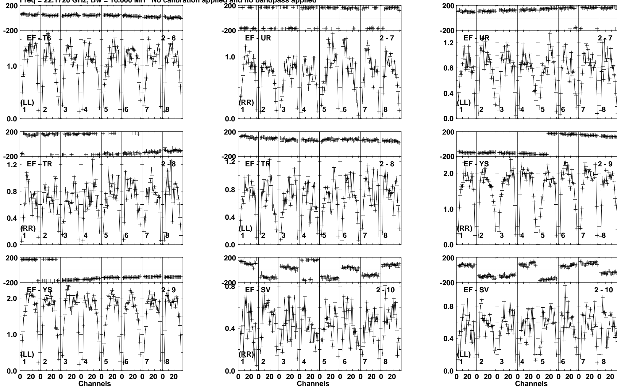
Lower frame: Milli Ampl Jy Top frame: Phas deg Vector averaged cross-power spectrum Baseline: EF (02) - T6 (06) Timerange: 00/08:12:51 to 00/08:13:49
