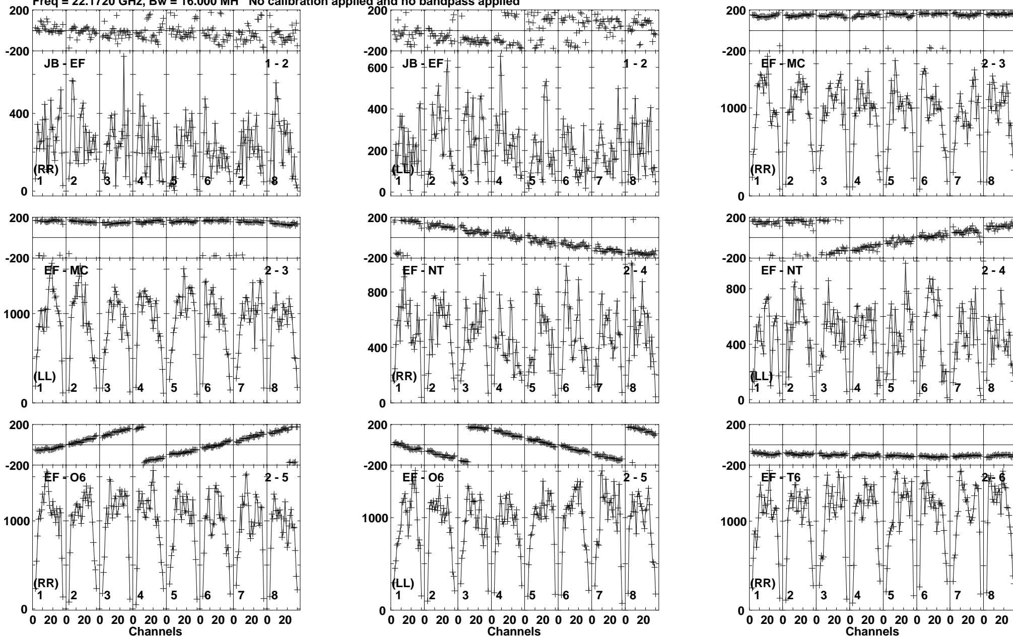
Lower frame: Micro Ampl Jy Top frame: Phas deg Vector averaged cross-power spectrum Baseline: JB (01) - EF (02) Timerange: 00/09:22:51 to 00/09:23:49
