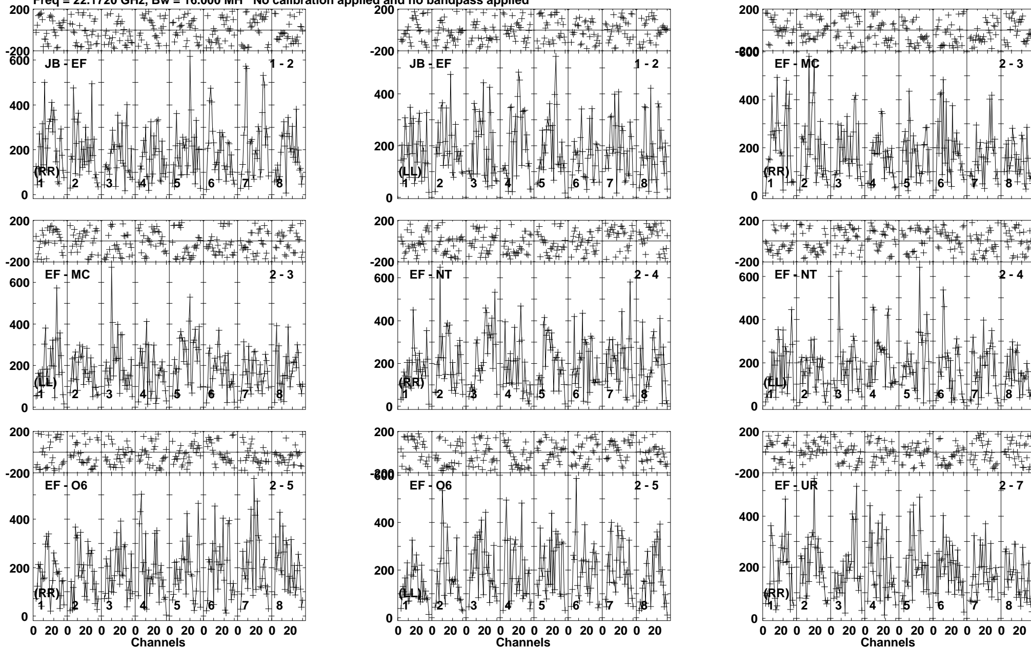
Lower frame: Micro Ampl Jy Top frame: Phas deg Vector averaged cross-power spectrum Baseline: JB (01) - EF (02) Timerange: 00/14:14:01 to 00/14:14:59
