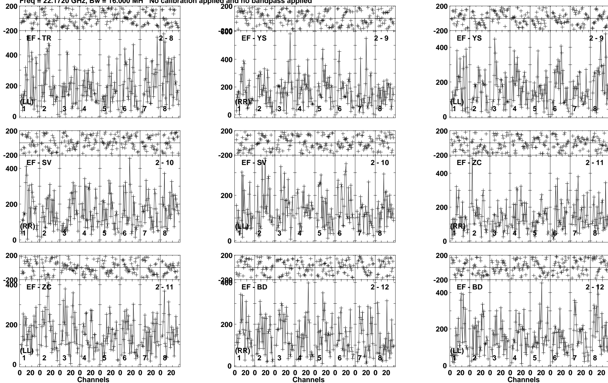
Lower frame: Micro Ampl Jy Top frame: Phas deg Vector averaged cross-power spectrum Baseline: EF (02) - TR (08) Timerange: 00/04:25:01 to 00/04:25:59
