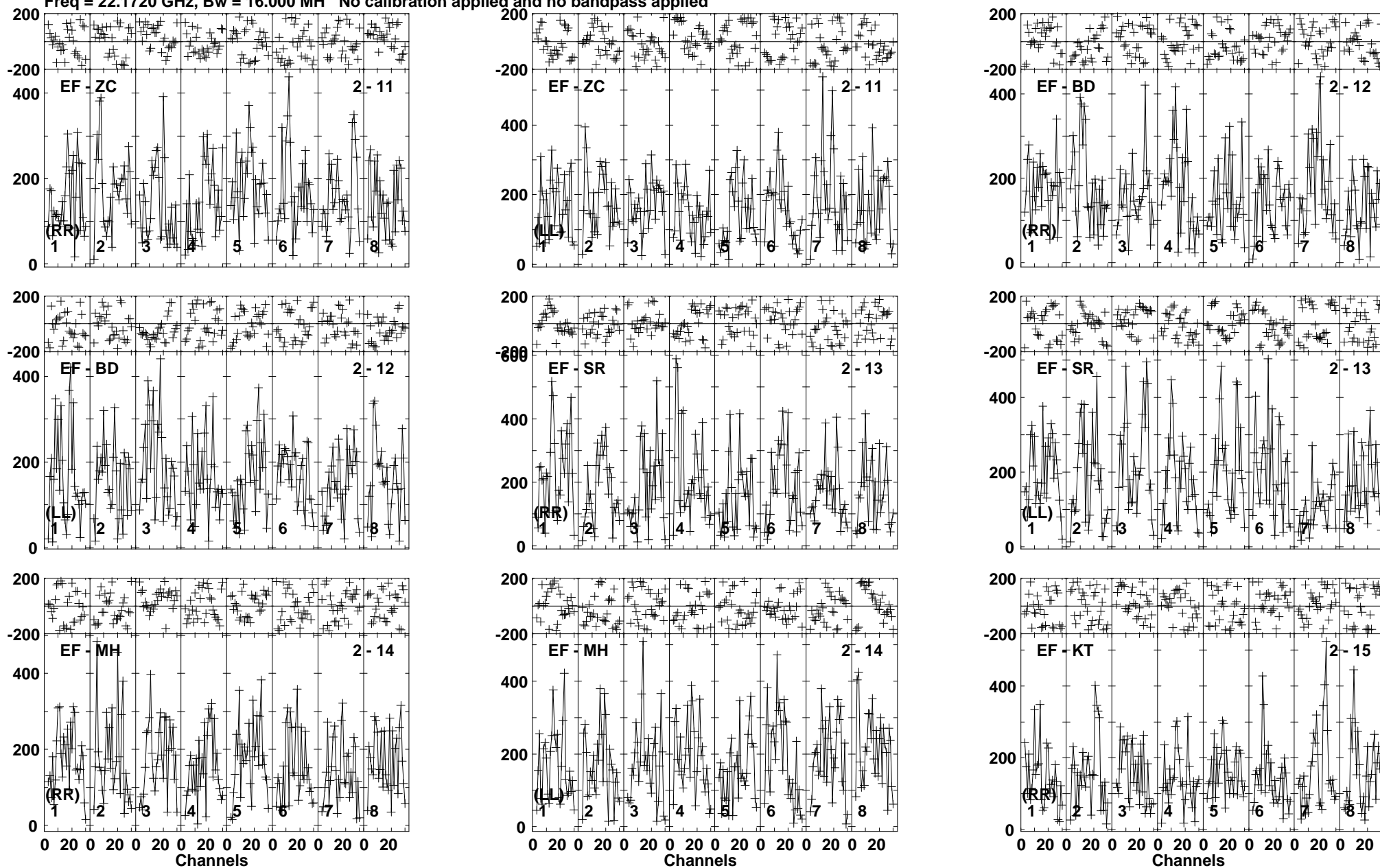
Lower frame: Micro Ampl Jy Top frame: Phas deg Vector averaged cross-power spectrum Baseline: EF (02) - ZC (11) Timerange: 00/08:07:51 to 00/08:08:49
