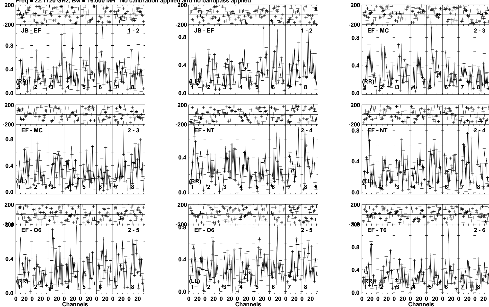
Lower frame: Milli Ampl Jy Top frame: Phas deg Vector averaged cross-power spectrum Baseline: JB (01) - EF (02) Timerange: 00/11:01:11 to 00/11:02:09
