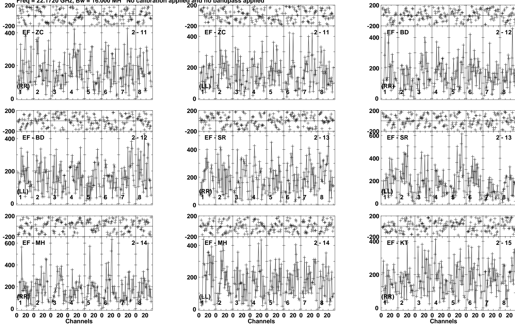
Lower frame: Micro Ampl Jy Top frame: Phas deg Vector averaged cross-power spectrum Baseline: EF (02) - ZC (11) Timerange: 00/08:54:31 to 00/08:55:29
