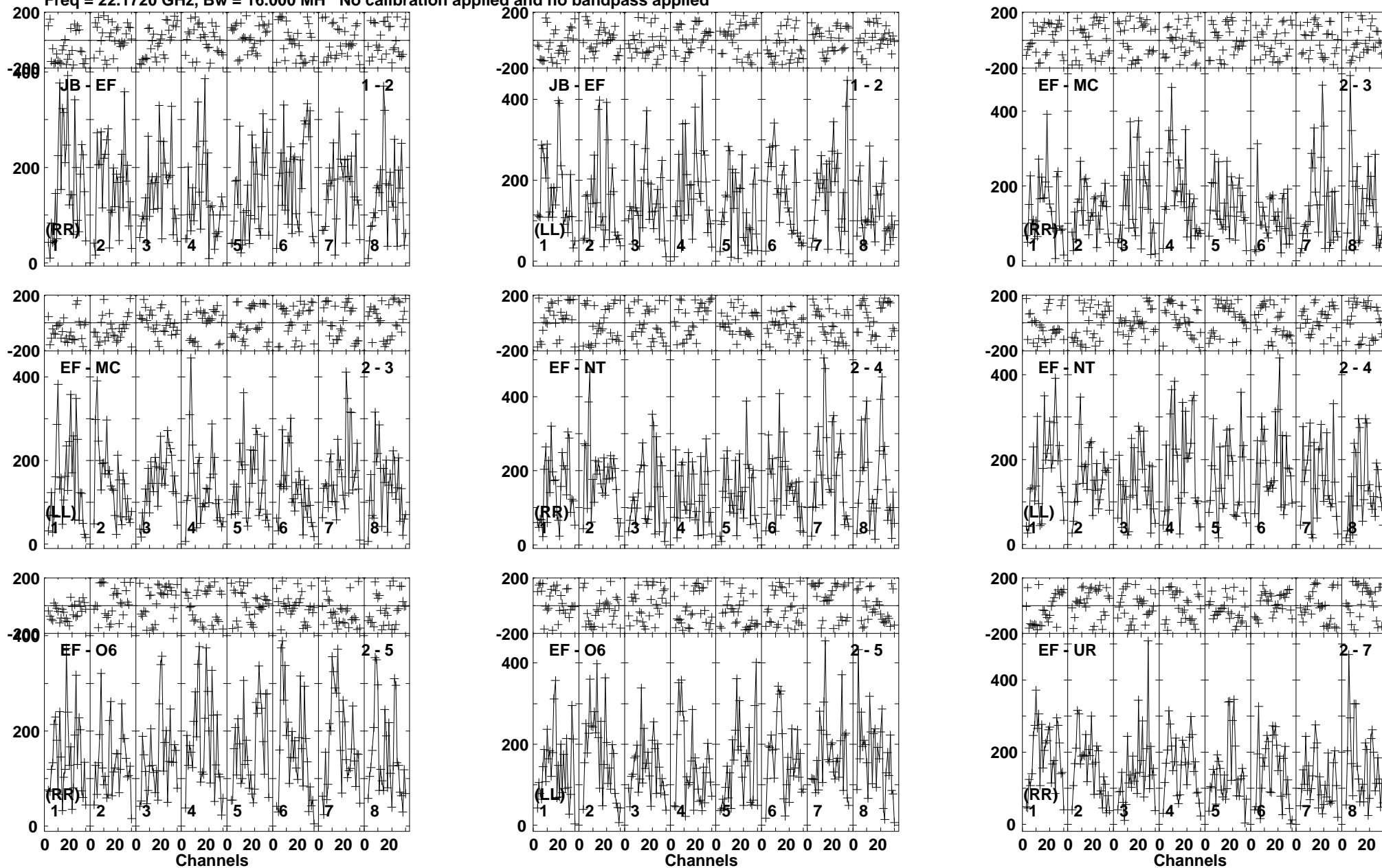
Lower frame: Micro Ampl Jy Top frame: Phas deg Vector averaged cross-power spectrum Baseline: JB (01) - EF (02) Timerange: 00/14:42:21 to 00/14:43:19
