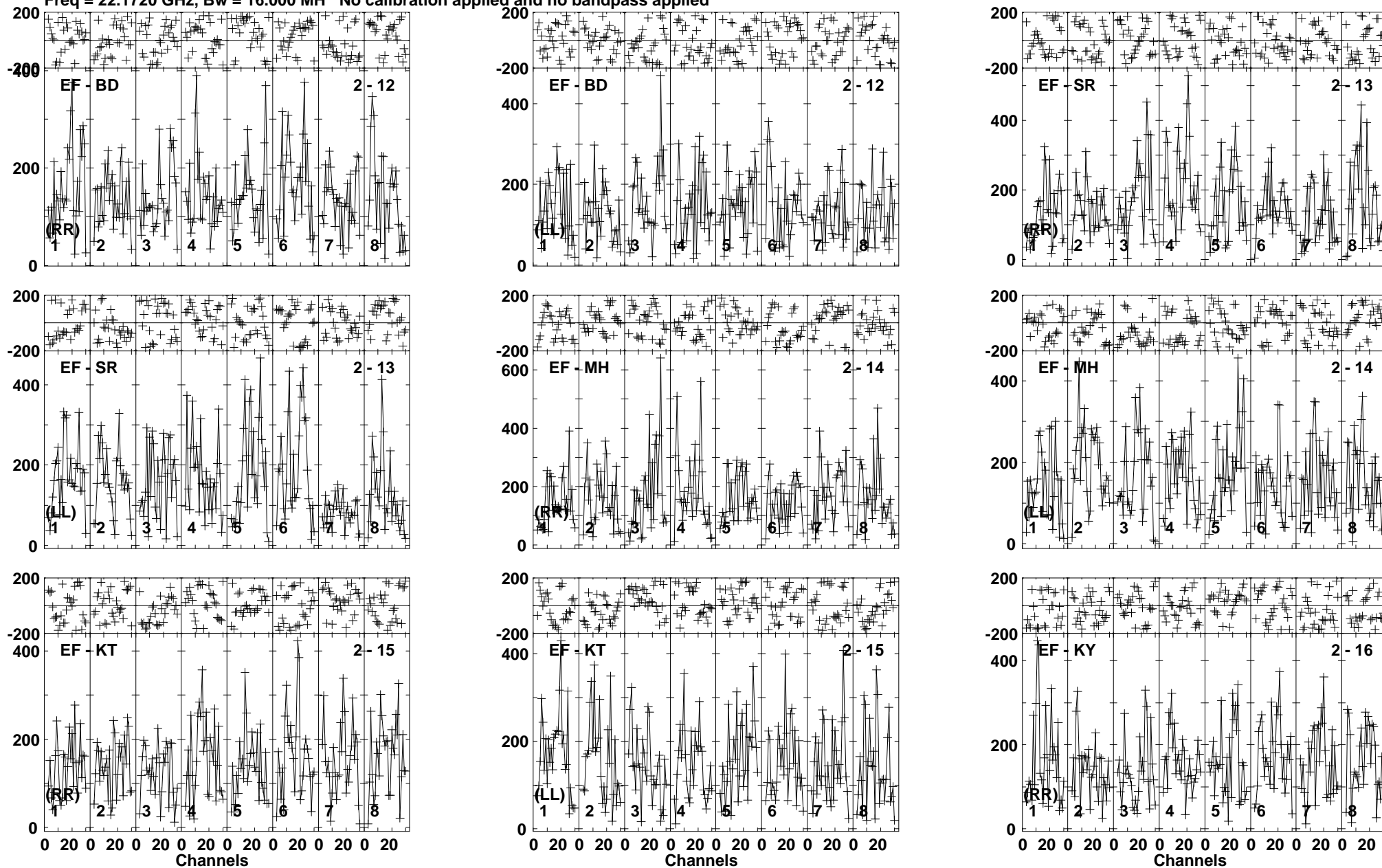
Lower frame: Micro Ampl Jy Top frame: Phas deg Vector averaged cross-power spectrum Baseline: EF (02) - BD (12) Timerange: 00/04:11:41 to 00/04:12:39
