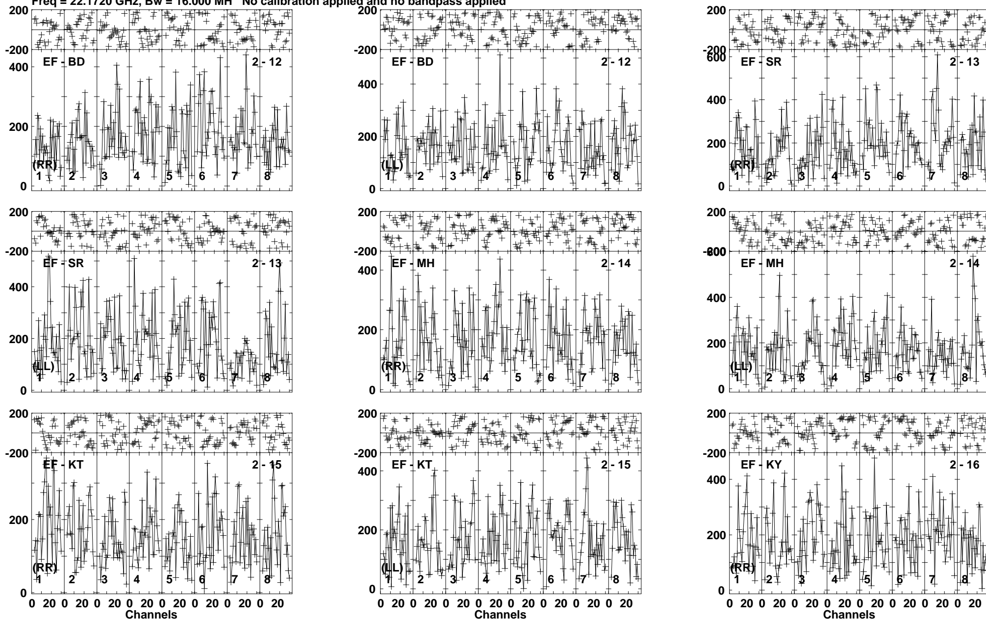
Lower frame: Micro Ampl Jy Top frame: Phas deg Vector averaged cross-power spectrum Baseline: EF (02) - BD (12) Timerange: 00/07:37:51 to 00/07:38:49
