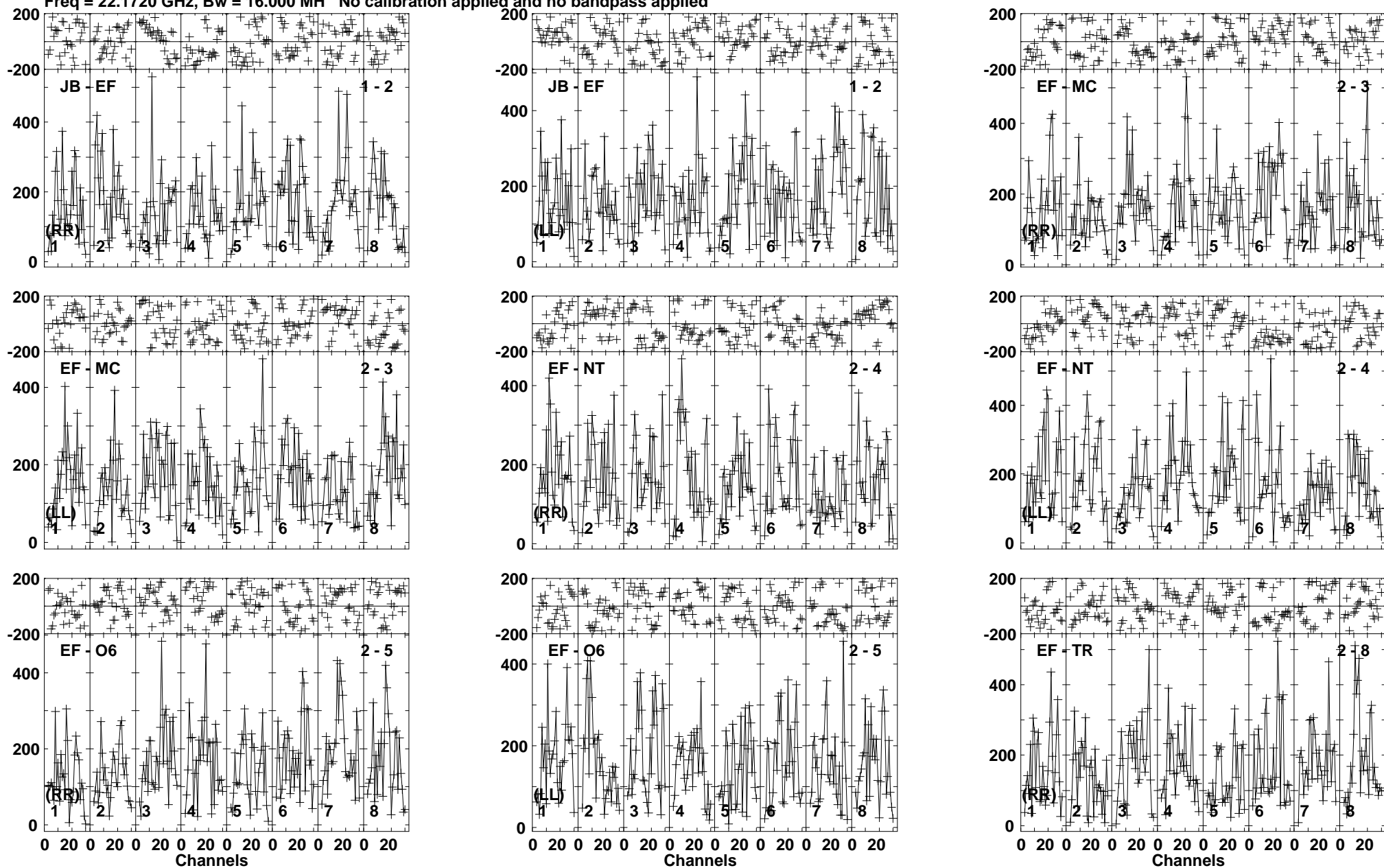
Lower frame: Micro Ampl Jy Top frame: Phas deg Vector averaged cross-power spectrum Baseline: JB (01) - EF (02) Timerange: 00/06:25:01 to 00/06:25:59
