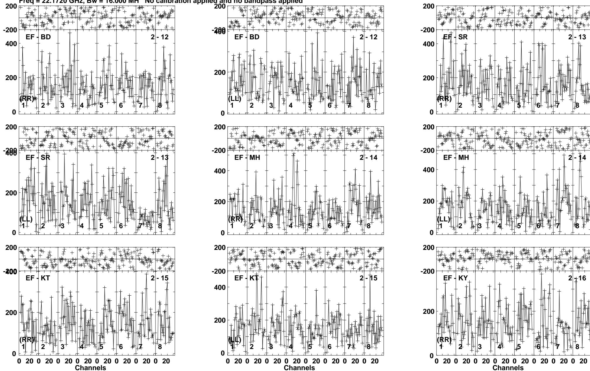
Lower frame: Micro Ampl Jy Top frame: Phas deg Vector averaged cross-power spectrum Baseline: EF (02) - BD (12) Timerange: 00/04:08:21 to 00/04:09:19
