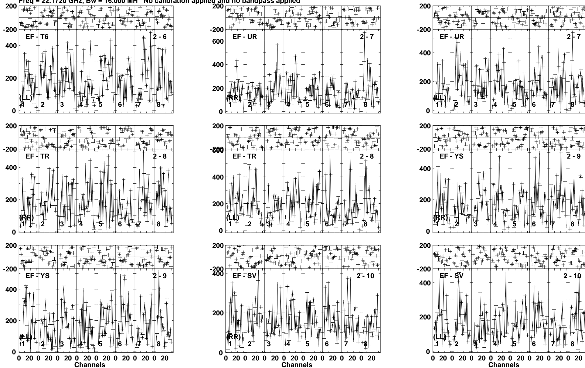
Lower frame: Micro Ampl Jy Top frame: Phas deg Vector averaged cross-power spectrum Baseline: EF (02) - T6 (06) Timerange: 00/09:01:11 to 00/09:02:09
