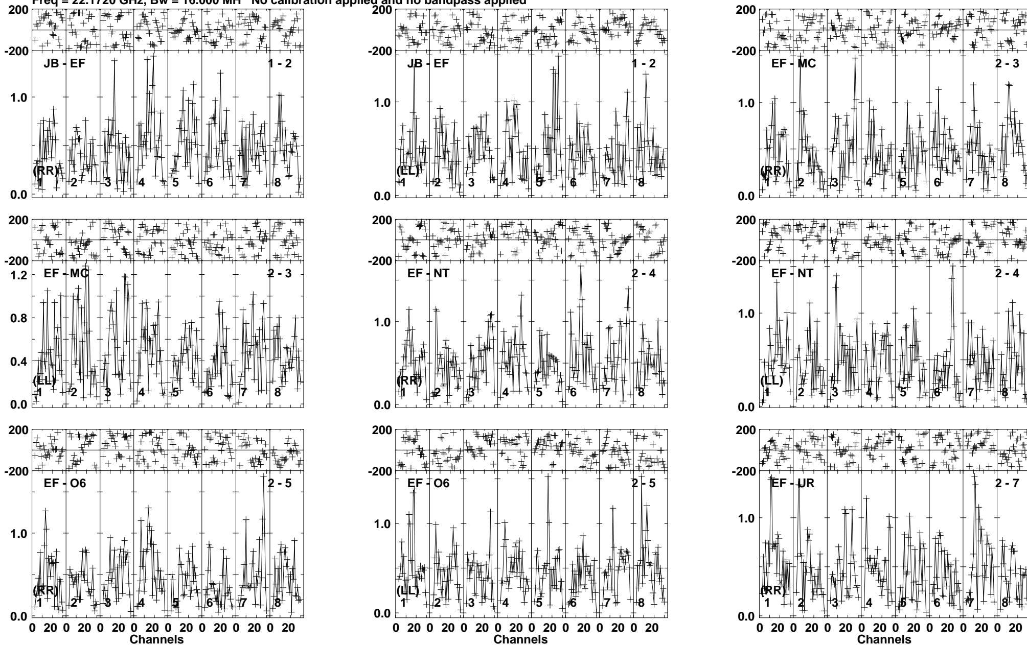
Lower frame: Milli Ampl Jy Top frame: Phas deg Vector averaged cross-power spectrum Baseline: JB (01) - EF (02) Timerange: 00/13:17:21 to 00/13:18:19
