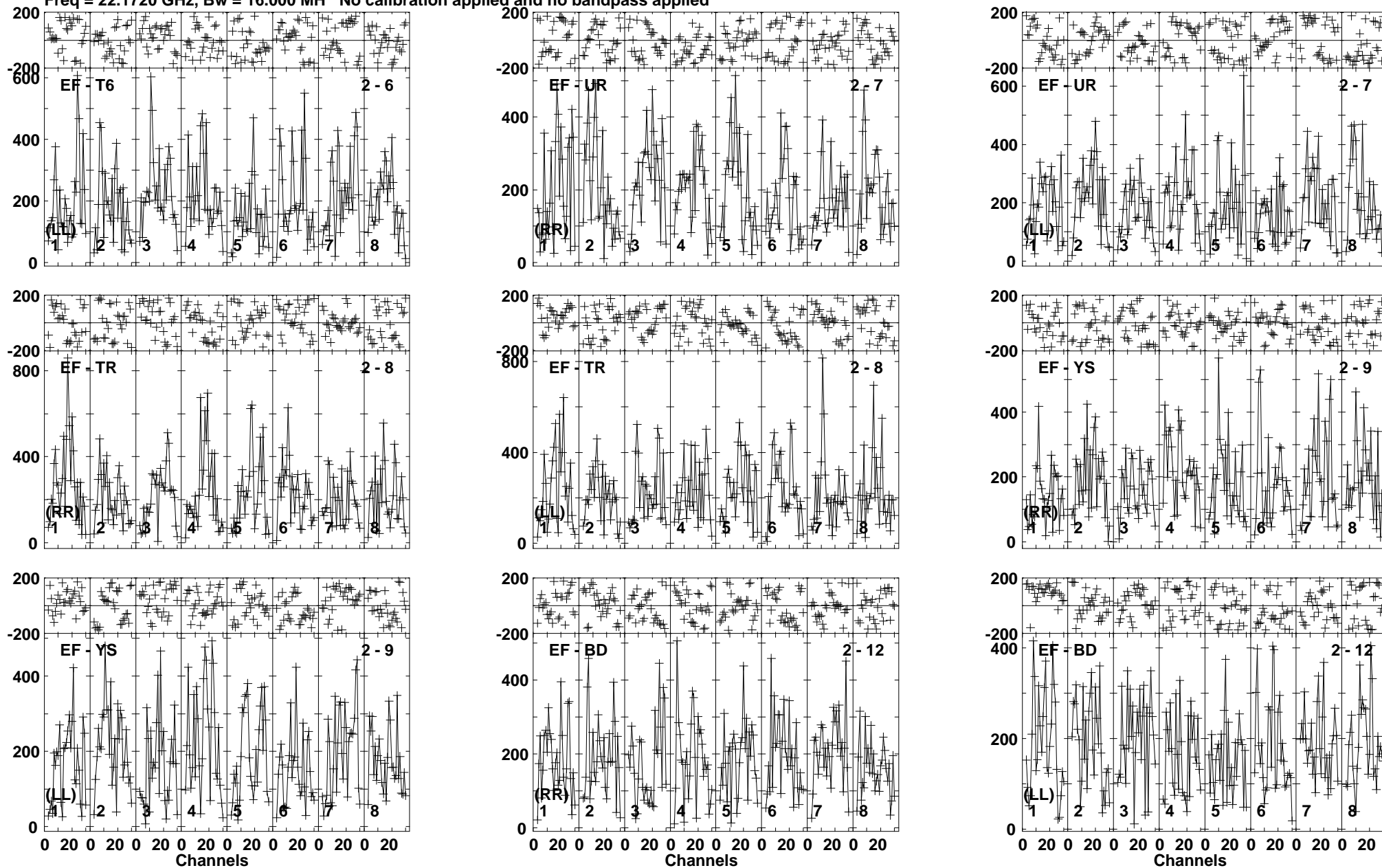
Lower frame: Micro Ampl Jy Top frame: Phas deg Vector averaged cross-power spectrum Baseline: EF (02) - T6 (06) Timerange: 00/10:17:51 to 00/10:18:49
