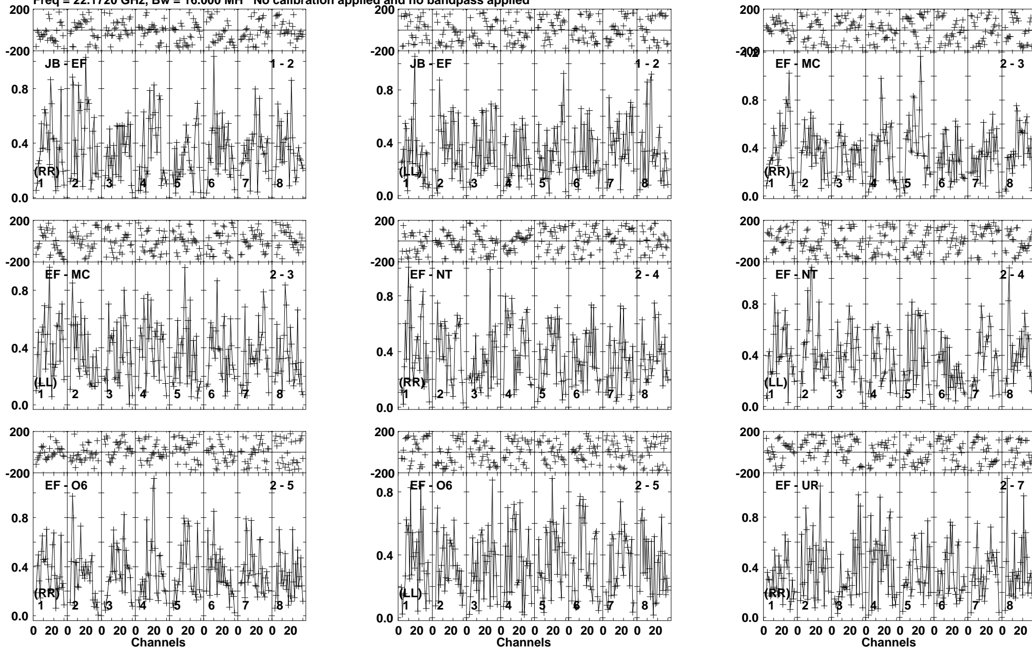
Lower frame: Milli Ampl Jy Top frame: Phas deg Vector averaged cross-power spectrum Baseline: JB (01) - EF (02) Timerange: 00/13:20:41 to 00/13:21:39
