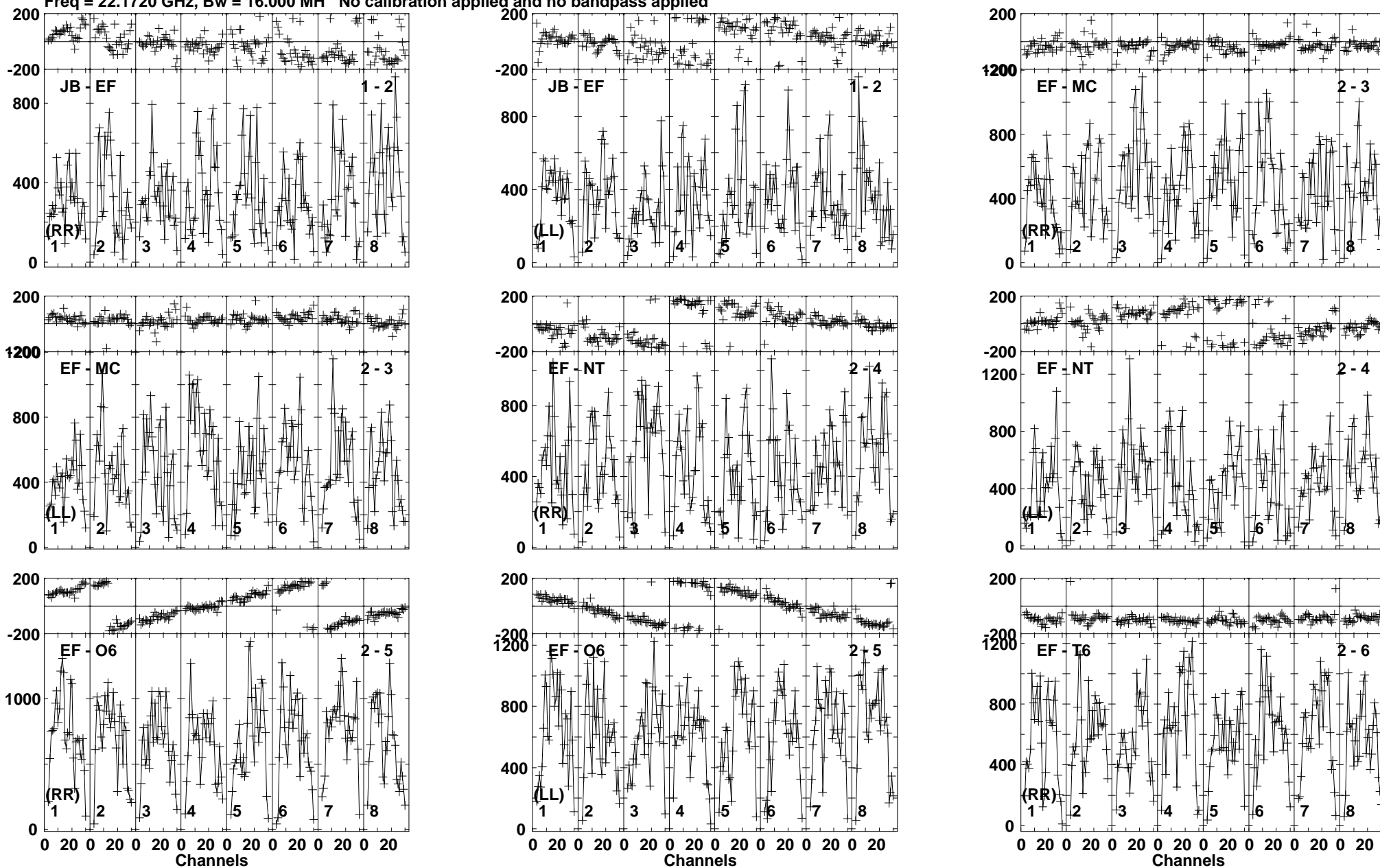
Lower frame: Micro Ampl Jy Top frame: Phas deg Vector averaged cross-power spectrum Baseline: JB (01) - EF (02) Timerange: 00/11:26:11 to 00/11:27:09
