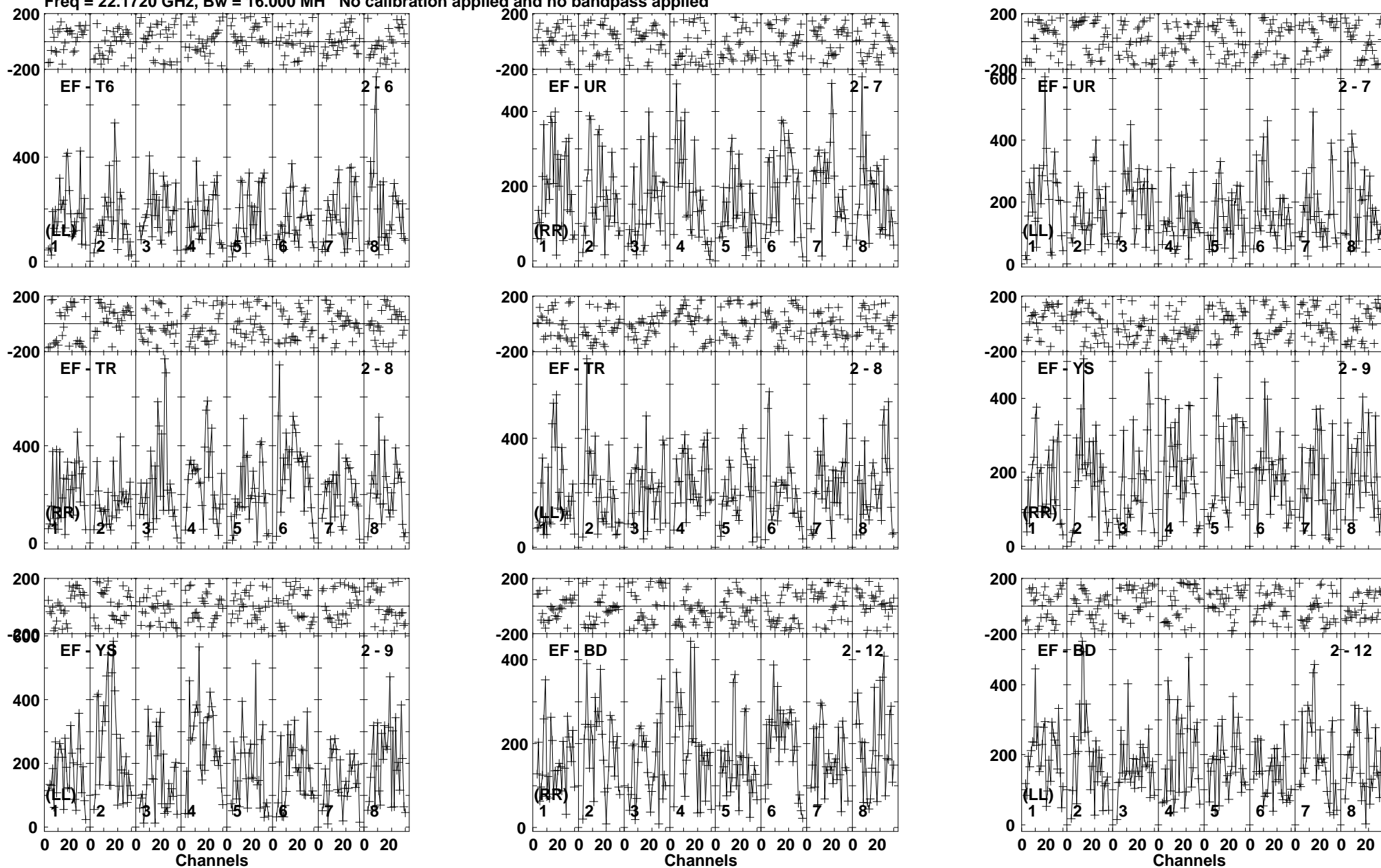
Lower frame: Micro Ampl Jy Top frame: Phas deg Vector averaged cross-power spectrum Baseline: EF (02) - T6 (06) Timerange: 00/10:21:11 to 00/10:22:09
