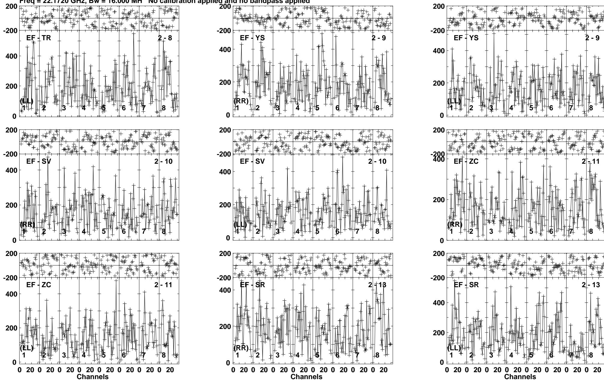
Lower frame: Micro Ampl Jy Top frame: Phas deg Vector averaged cross-power spectrum Baseline: EF (02) - TR (08) Timerange: 00/06:28:21 to 00/06:29:19
