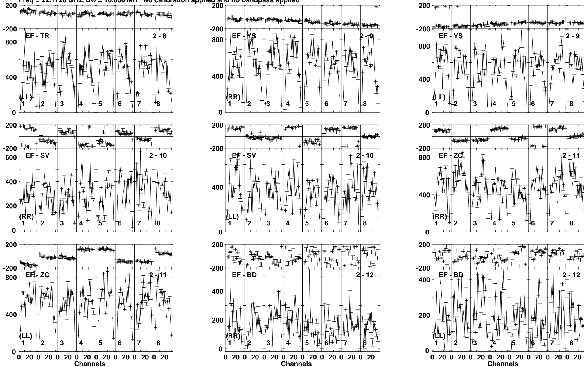
Lower frame: Micro Ampl Jy Top frame: Phas deg Vector averaged cross-power spectrum Baseline: EF (02) - TR (08) Timerange: 00/04:26:41 to 00/04:27:39
