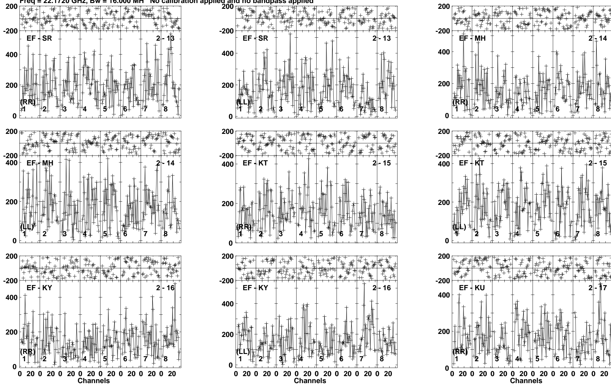
Lower frame: Micro Ampl Jy Top frame: Phas deg Vector averaged cross-power spectrum Baseline: EF (02) - SR (13) Timerange: 00/07:24:31 to 00/07:25:29
