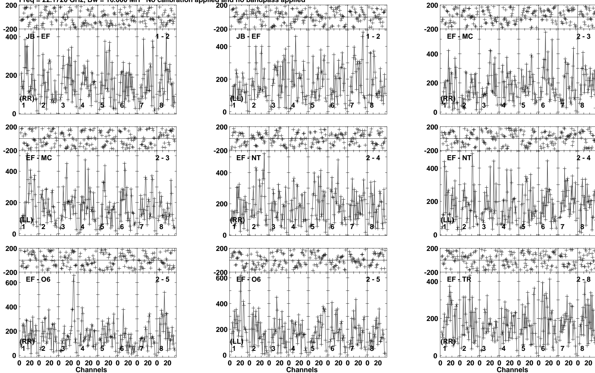
Lower frame: Micro Ampl Jy Top frame: Phas deg Vector averaged cross-power spectrum Baseline: JB (01) - EF (02) Timerange: 00/05:25:01 to 00/05:25:59
