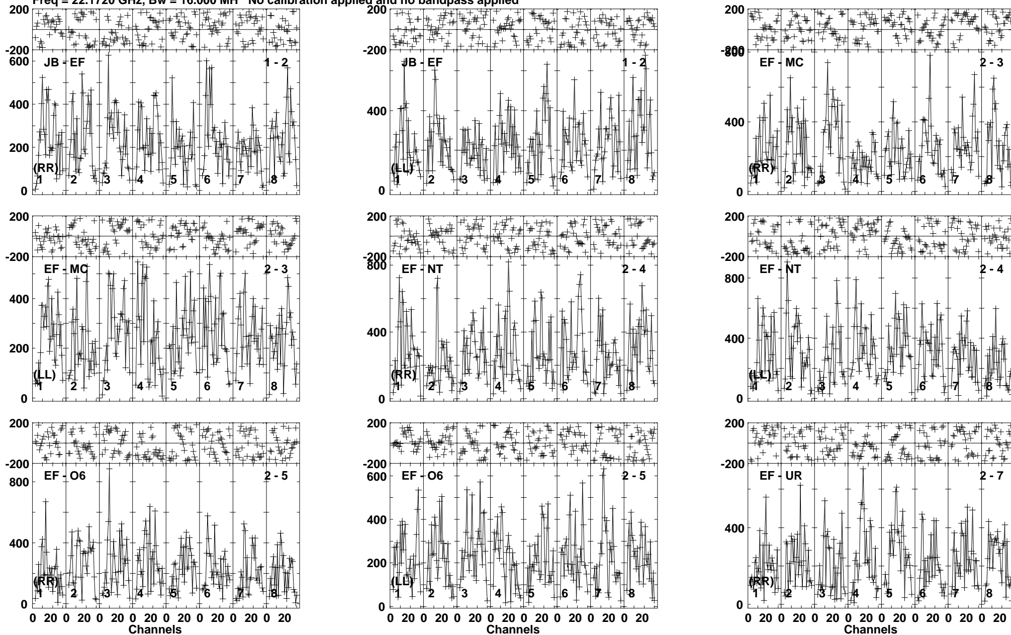
Lower frame: Micro Ampl Jy Top frame: Phas deg Vector averaged cross-power spectrum Baseline: JB (01) - EF (02) Timerange: 00/13:37:21 to 00/13:38:19
