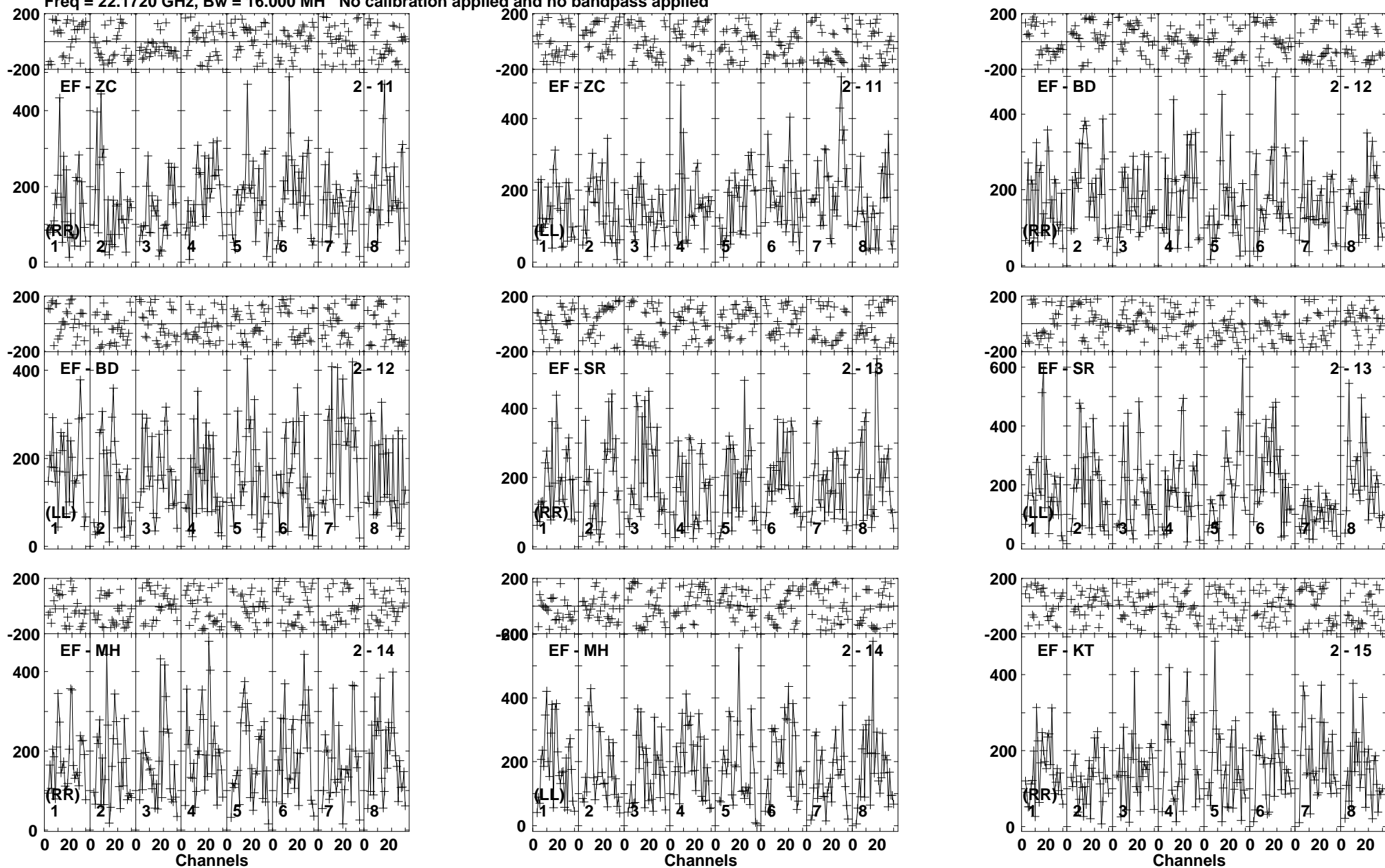
Lower frame: Micro Ampl Jy Top frame: Phas deg Vector averaged cross-power spectrum Baseline: EF (02) - ZC (11) Timerange: 00/09:31:11 to 00/09:32:09
