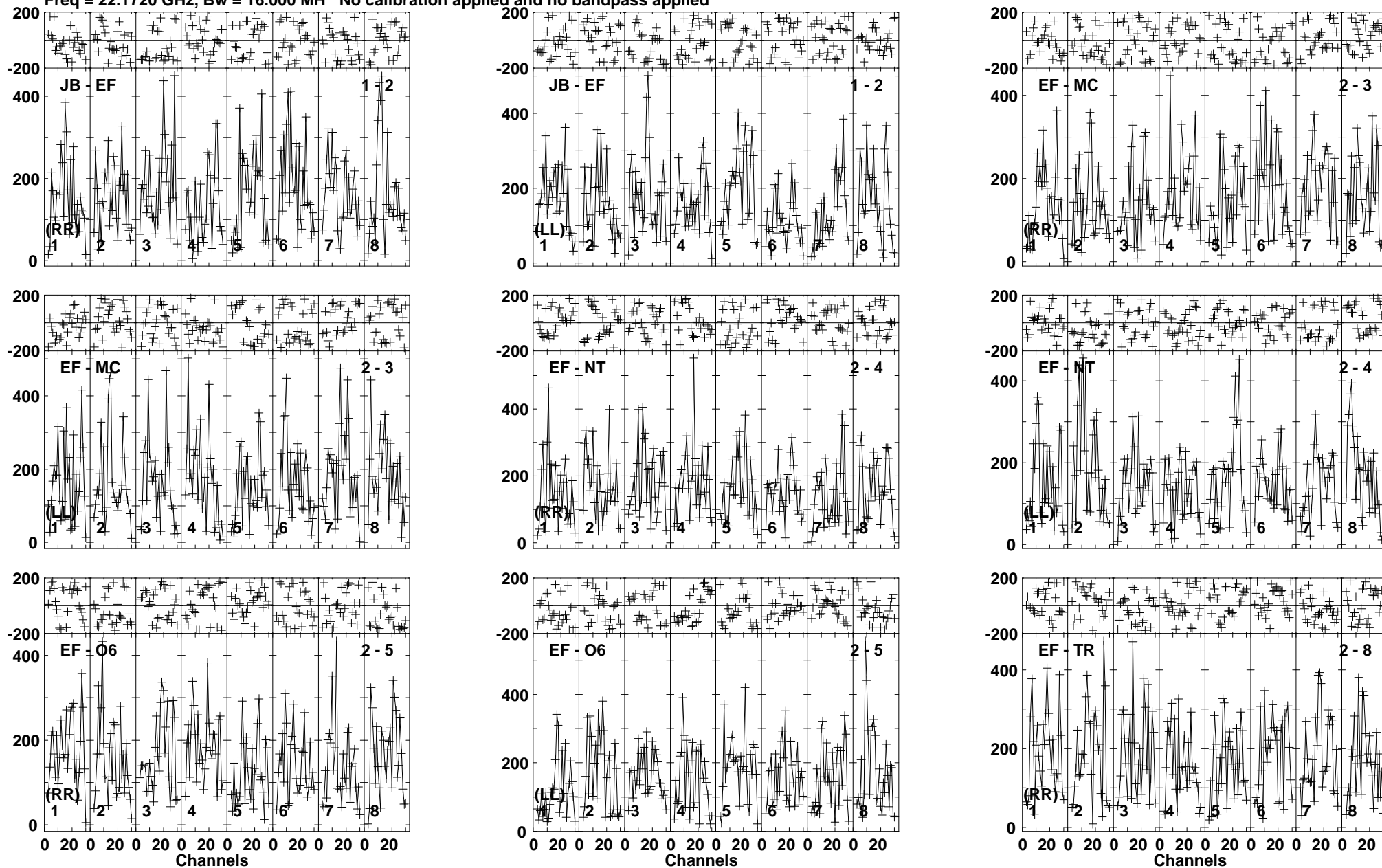
Lower frame: Micro Ampl Jy Top frame: Phas deg Vector average cross-power spectrum Baseline: JB (01) - EF (02) Timerange: 00/05:35:01 to 00/05:35:59
