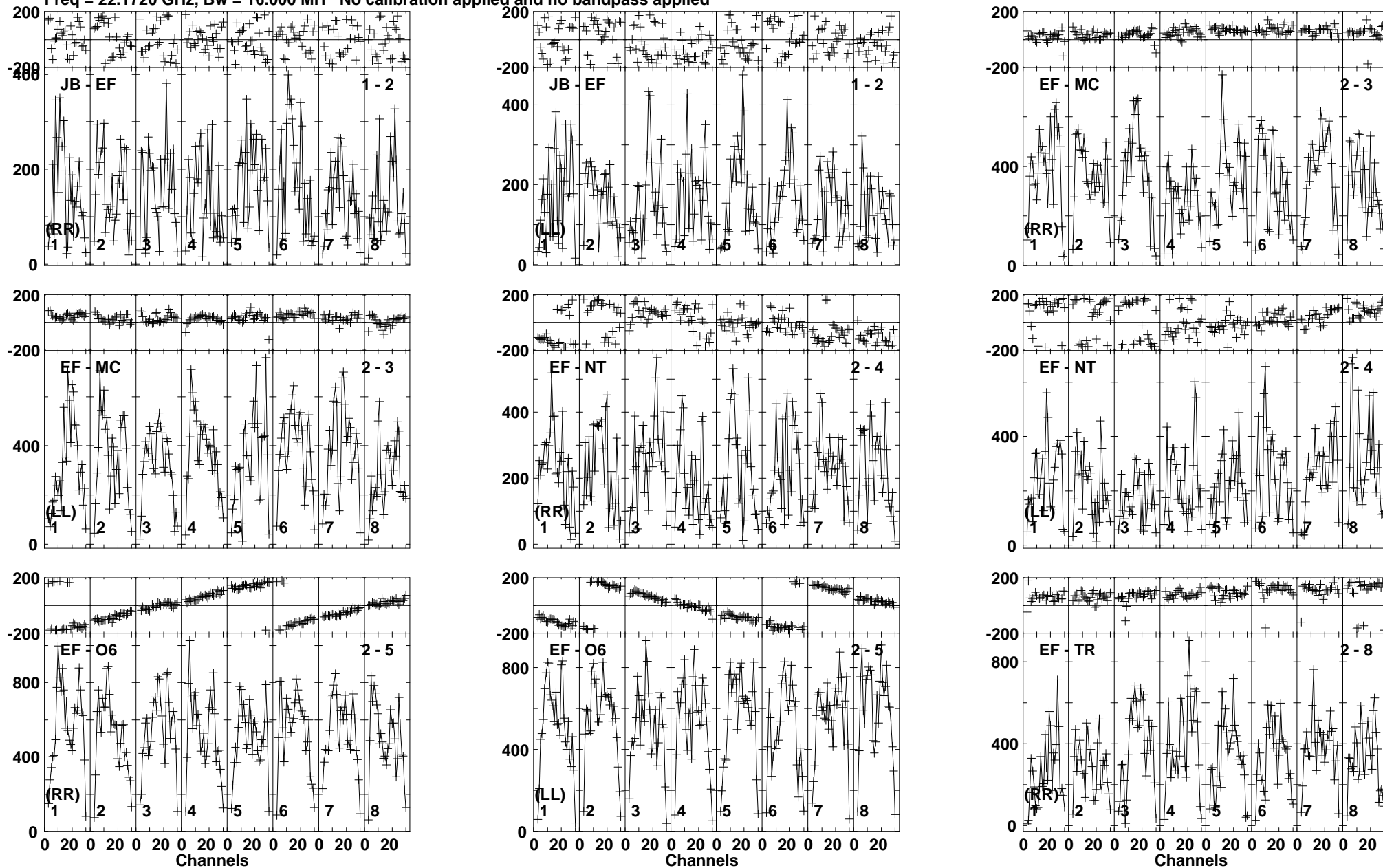
Lower frame: Micro Ampl Jy Top frame: Phas deg Vector averaged cross-power spectrum Baseline: JB (01) - EF (02) Timerange: 00/04:23:21 to 00/04:24:19
