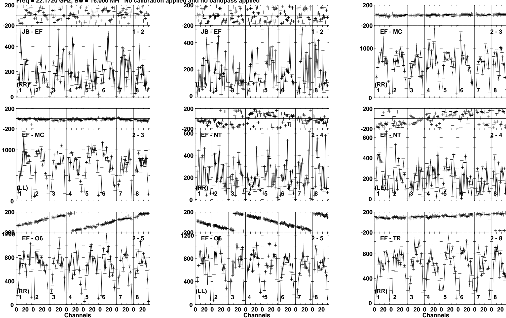
Lower frame: Micro Ampl Jy Top frame: Phas deg Vector averaged cross-power spectrum Baseline: JB (01) - EF (02) Timerange: 00/06:26:41 to 00/06:27:39
