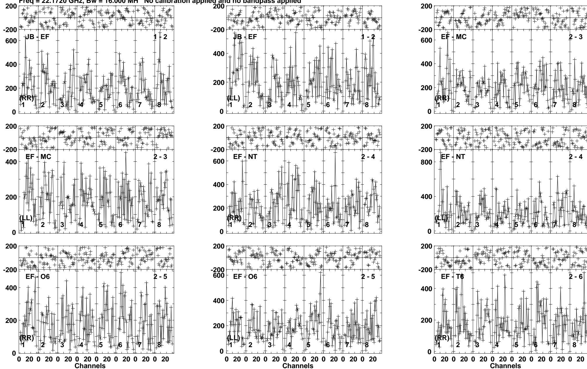
Lower frame: Micro Ampl Jy Top frame: Phas deg Vector averaged cross-power spectrum Baseline: JB (01) - EF (02) Timerange: 00/10:14:31 to 00/10:15:29
