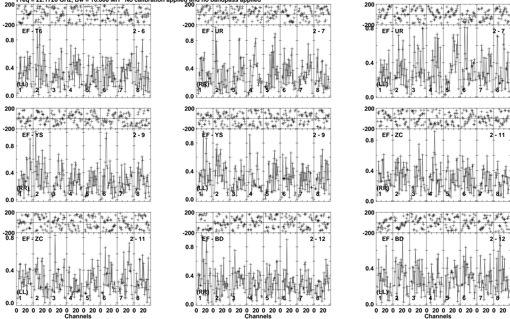
Lower frame: Milli Ampl Jy Top frame: Phas deg Vector averaged cross-power spectrum Baseline: EF (02) - T6 (06) Timerange: 00/11:04:31 to 00/11:05:29
