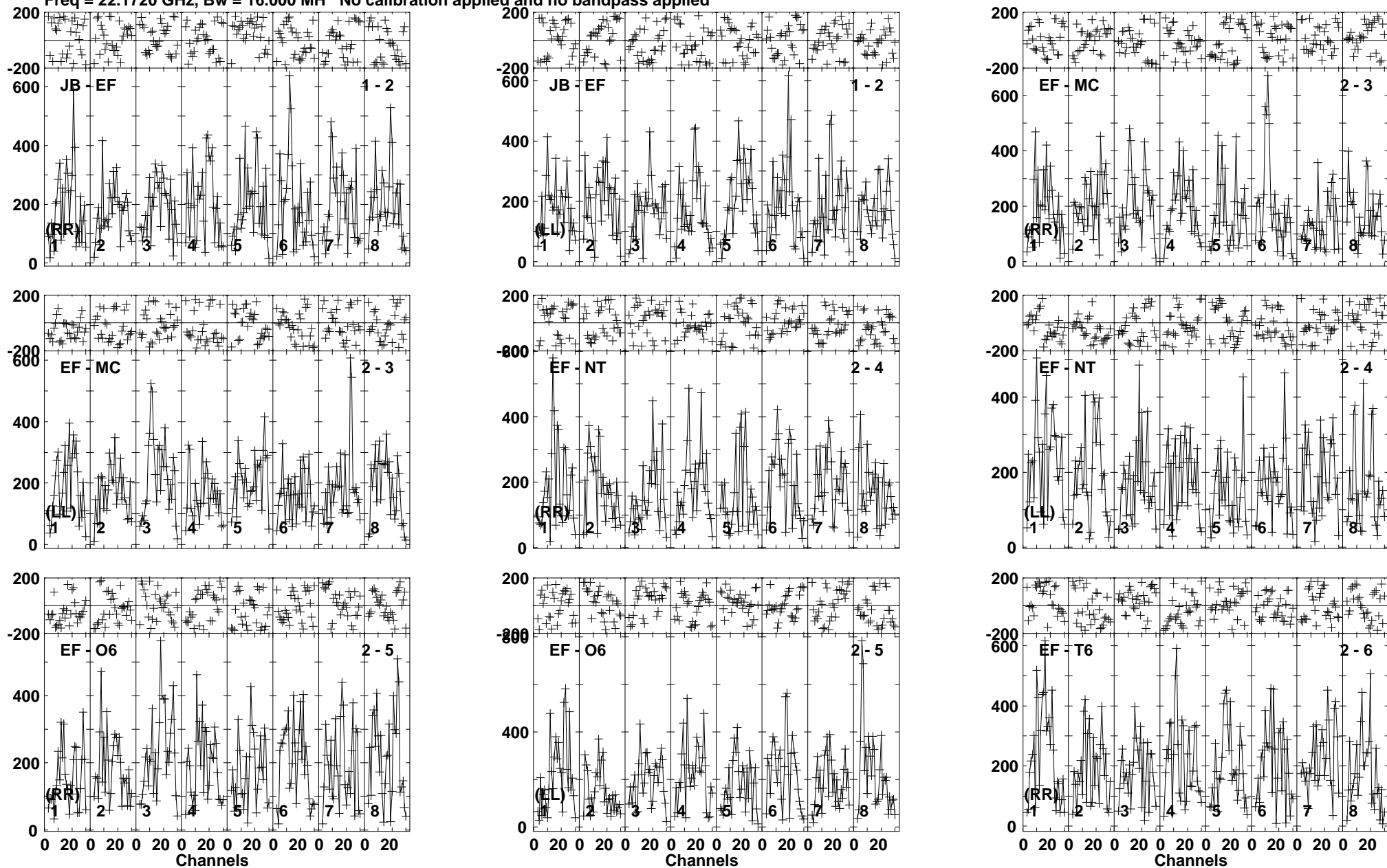
Lower frame: Micro Ampl Jy Top frame: Phas deg Vector averaged cross-power spectrum Baseline: JB (01) - EF (02) Timerange: 00/10:34:31 to 00/10:35:29
