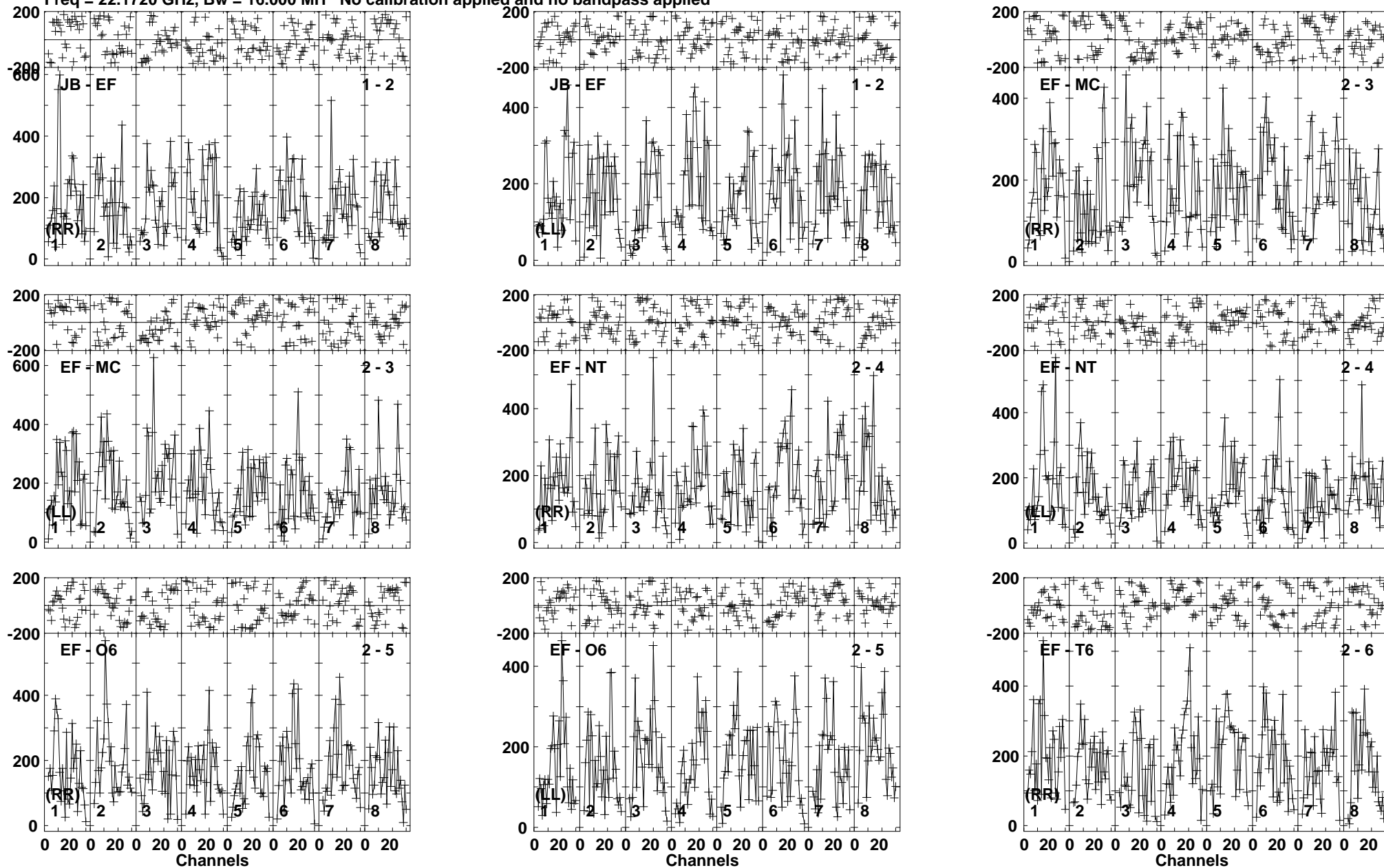
Lower frame: Micro Ampl Jy Top frame: Phas deg Vector averaged cross-power spectrum Baseline: JB (01) - EF (02) Timerange: 00/08:31:11 to 00/08:32:09
