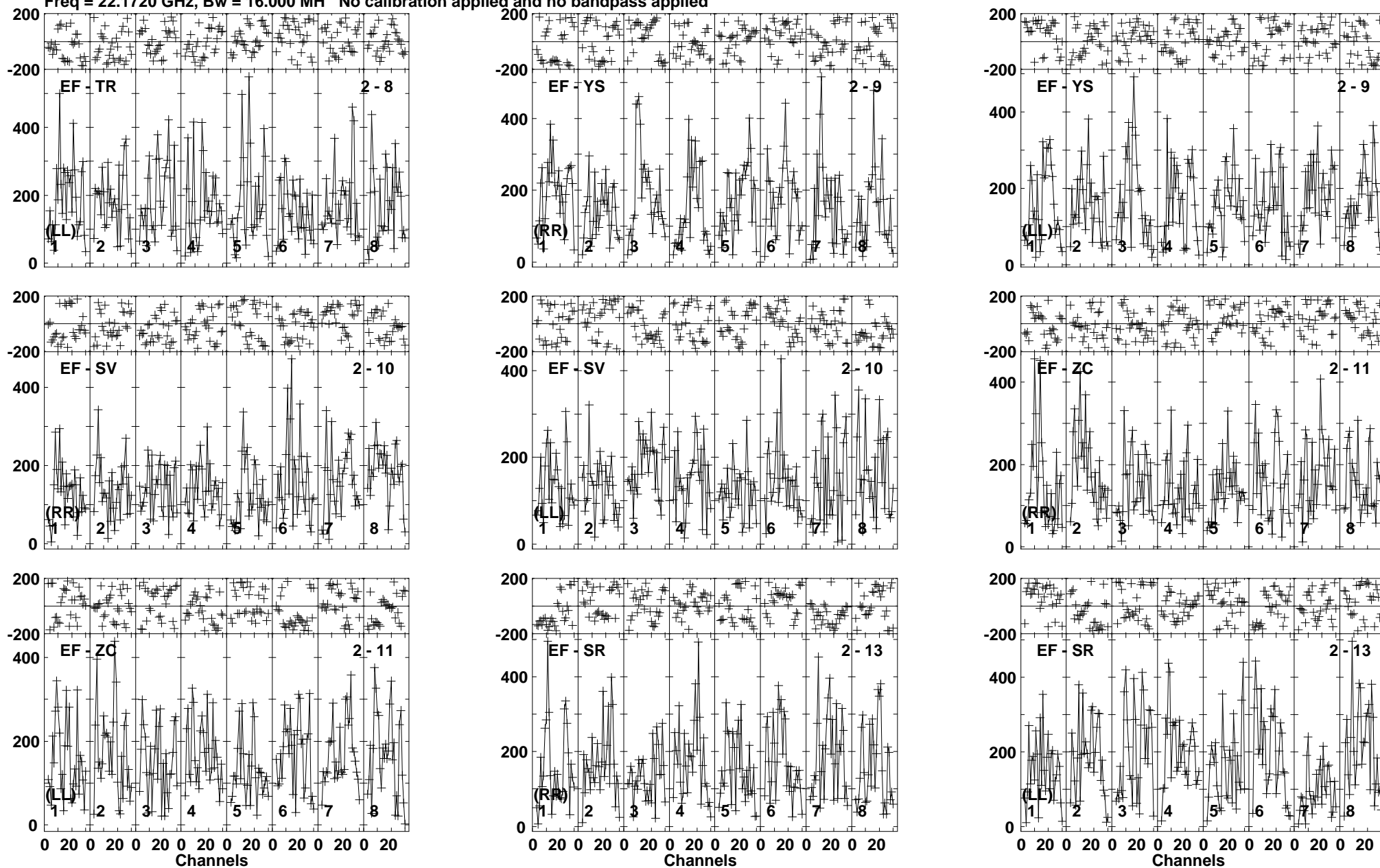
Lower frame: Micro Ampl Jy Top frame: Phas deg Vector averaged cross-power spectrum Baseline: EF (02) - TR (08) Timerange: 00/05:11:41 to 00/05:12:39
