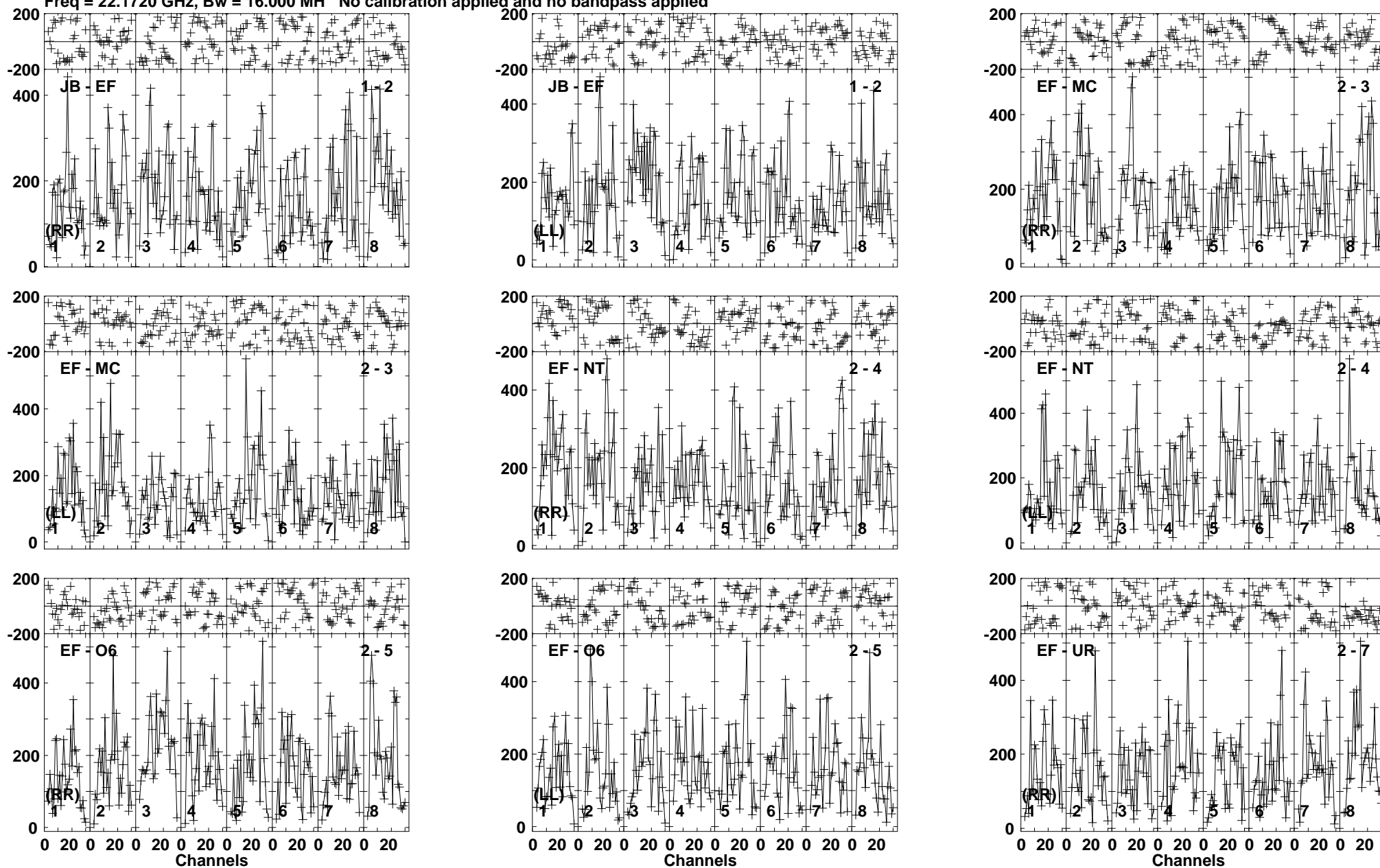
Lower frame: Micro Ampl Jy Top frame: Phas deg Vector averaged cross-power spectrum Baseline: JB (01) - EF (02) Timerange: 00/14:34:01 to 00/14:34:59
