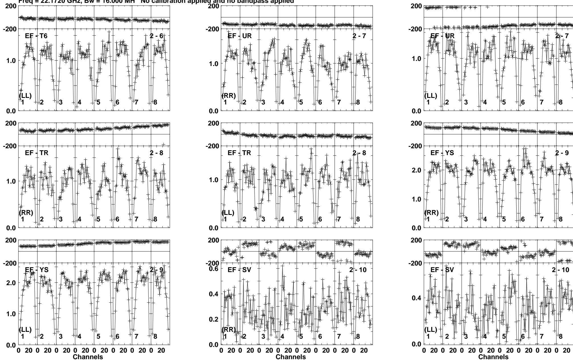
Lower frame: Milli Ampl Jy Top frame: Phas deg Vector averaged cross-power spectrum Baseline: EF (02) - T6 (06) Timerange: 00/08:59:31 to 00/09:00:29
