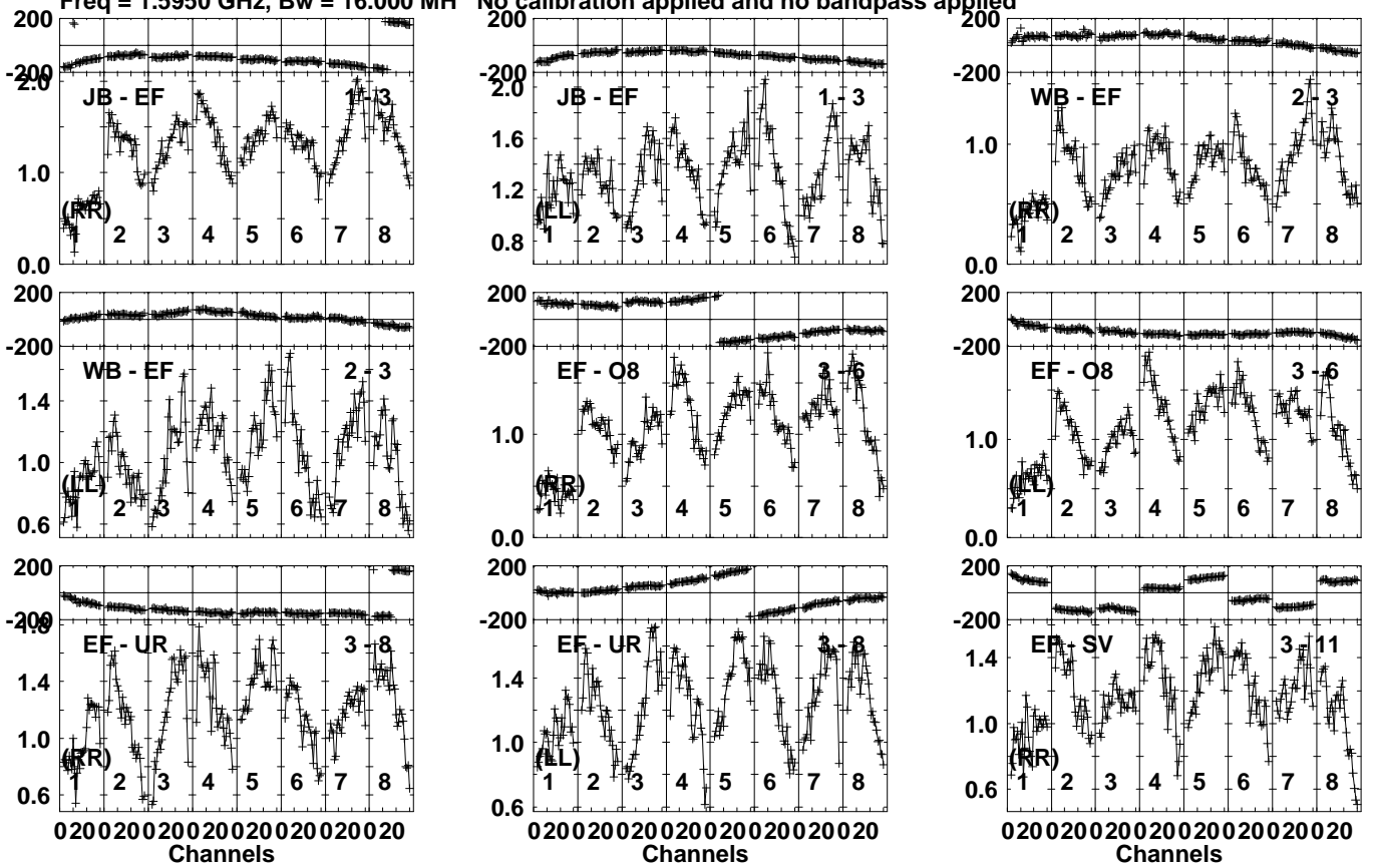
Lower frame: Milli Ampl Jy Top frame: Phas deg Vector averaged cross-power spectrum Several baselines displayed Timerange: 00/14:55:58 to 00/14:57:20
