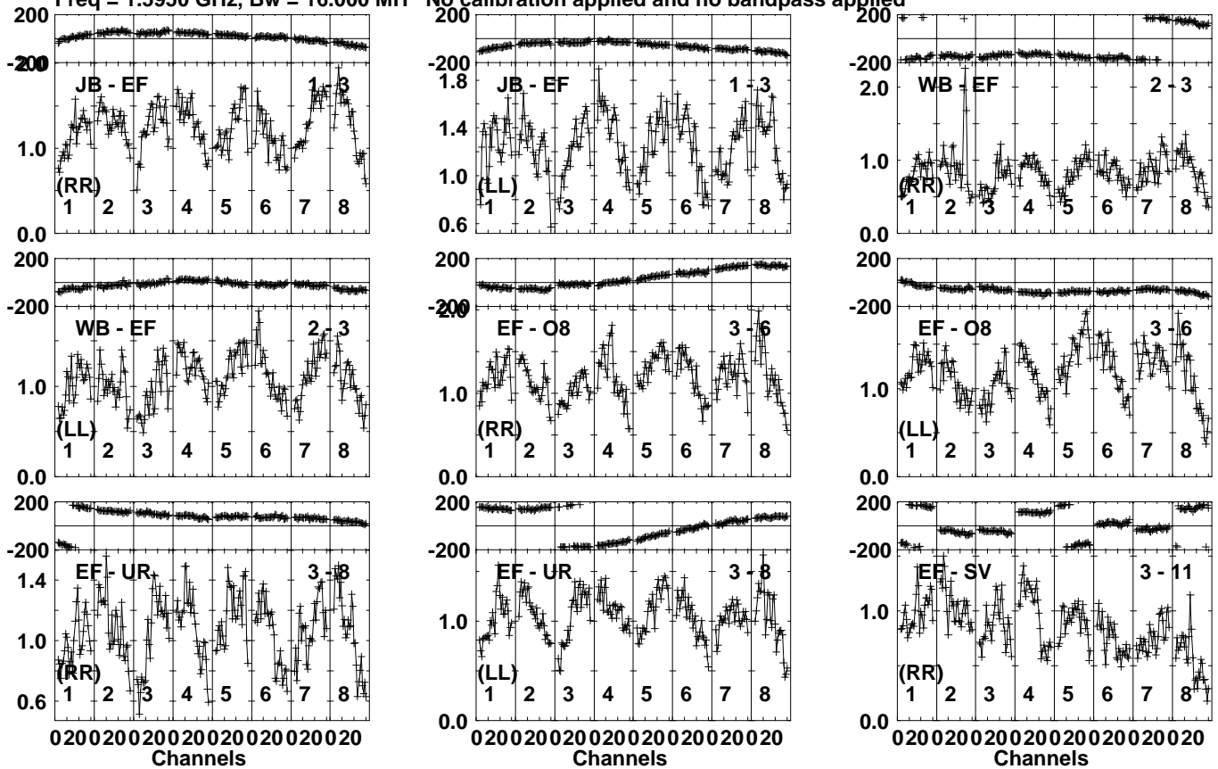
Lower frame: Milli Ampl Jy Top frame: Phas deg Vector averaged cross-power spectrum Several baselines displayed Timerange: 00/19:29:09 to 00/19:30:31
