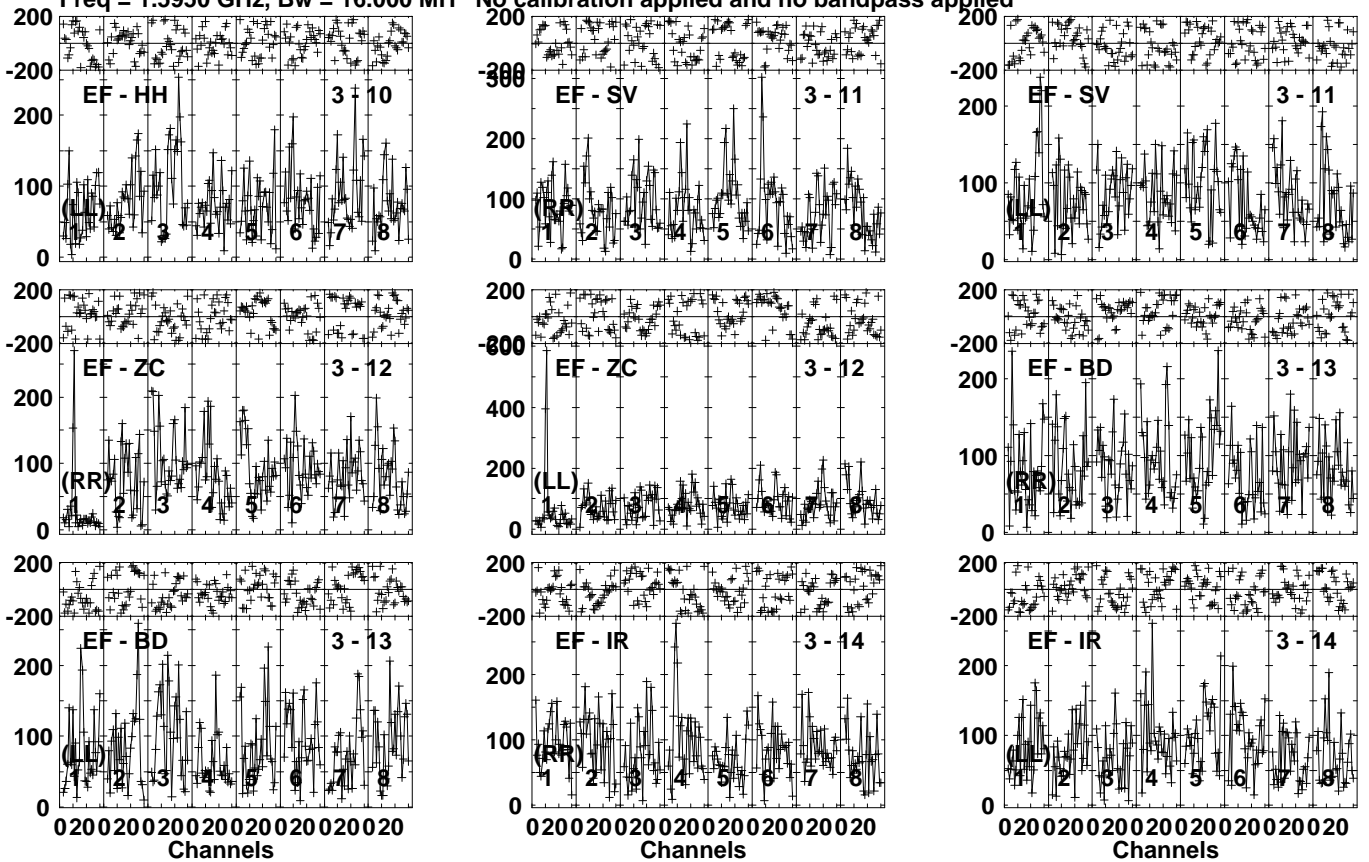
Lower frame: Micro Ampl Jy Top frame: Phas deg Vector averaged cross-power spectrum Several baselines displayed Timerange: 00/19:51:27 to 00/19:54:55
