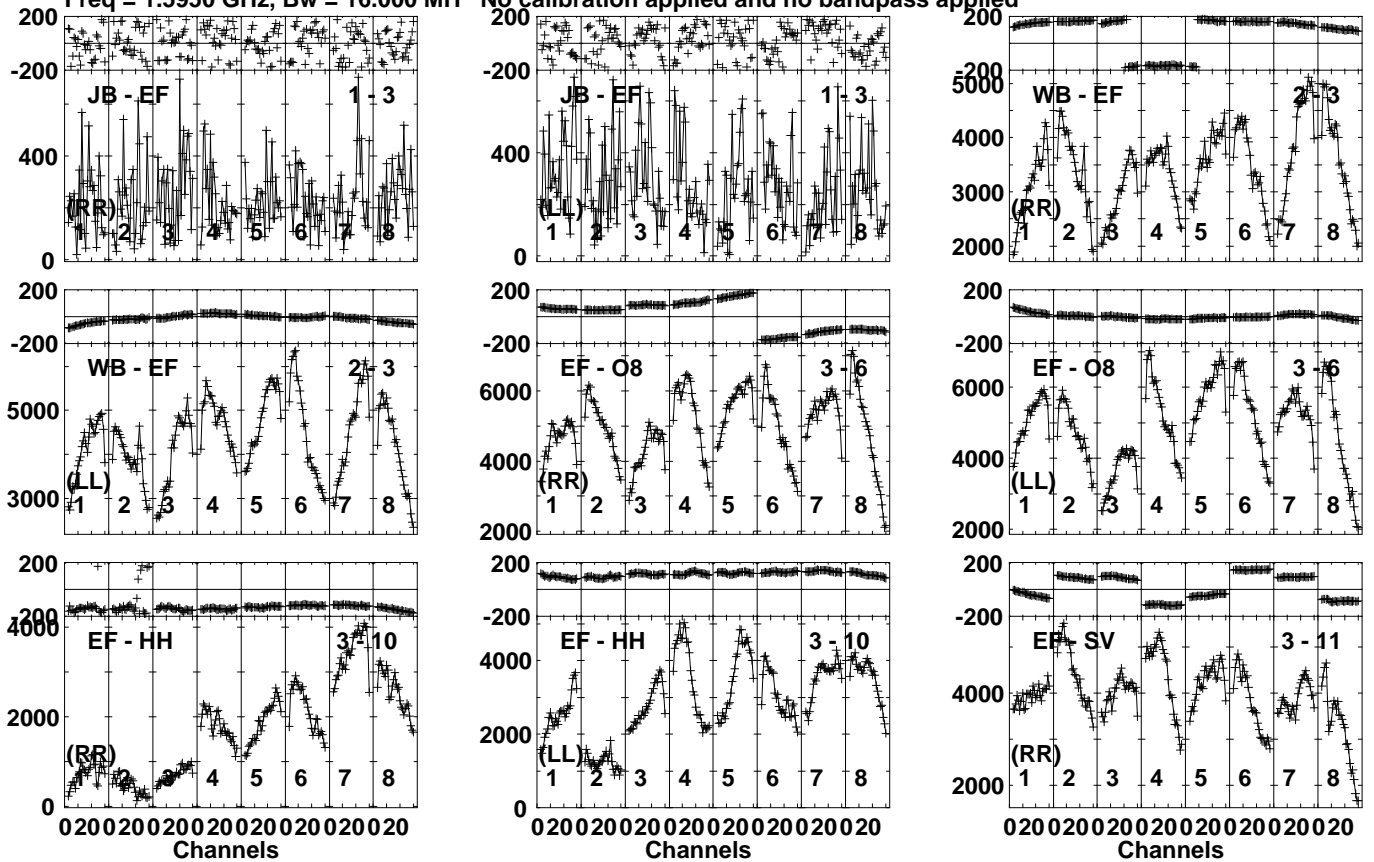
Lower frame: Micro Ampl Jy Top frame: Phas deg Vector averaged cross-power spectrum Several baselines displayed Timerange: 00/21:57:16 to 00/21:58:44
