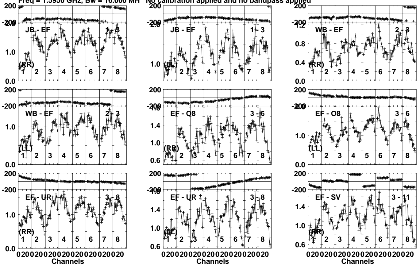
Lower frame: Milli Ampl Jy Top frame: Phas deg Vector averaged cross-power spectrum Several baselines displayed Timerange: 00/14:30:01 to 00/14:31:05
