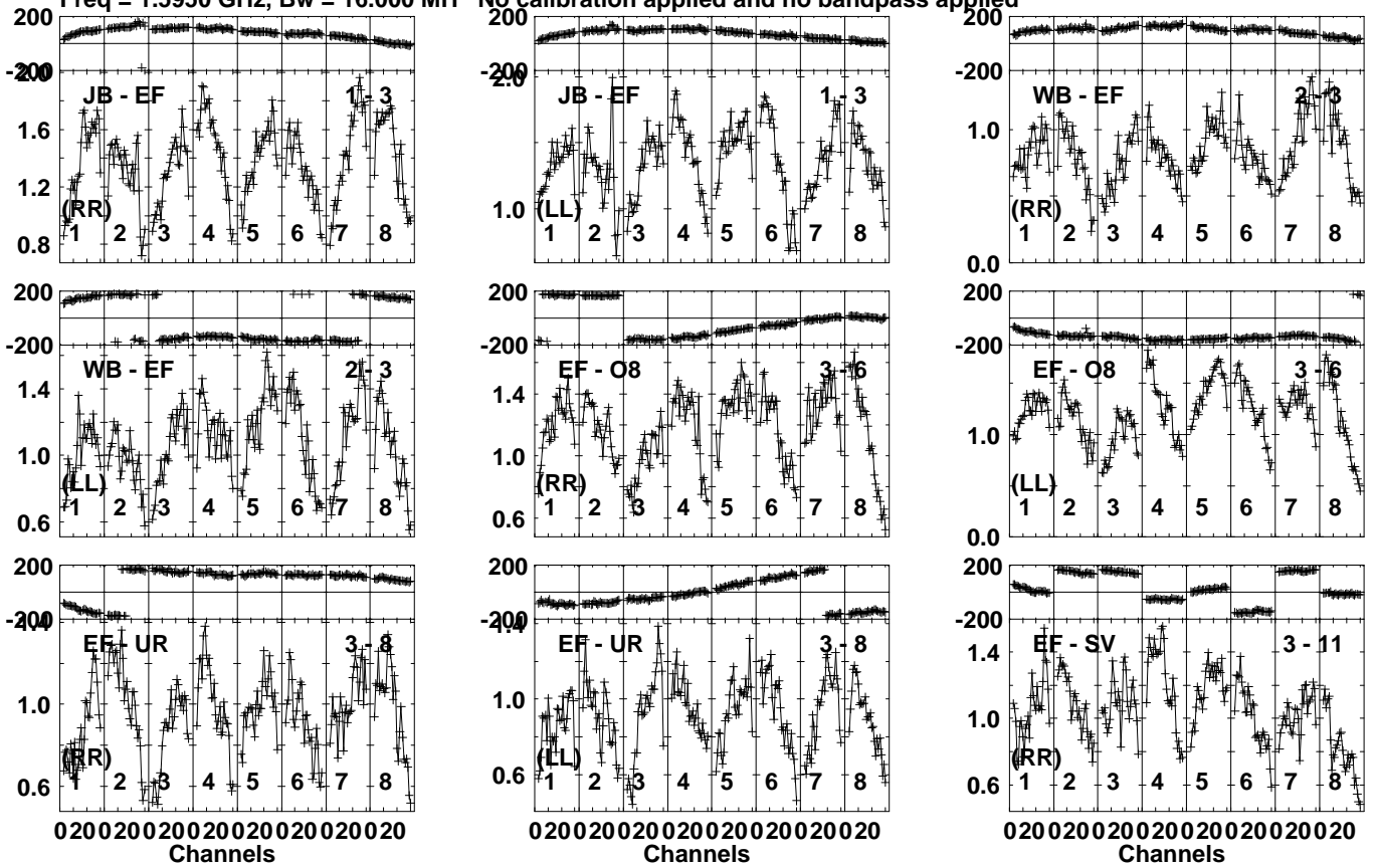
Lower frame: Milli Ampl Jy Top frame: Phas deg Vector averaged cross-power spectrum Several baselines displayed Timerange: 00/20:54:32 to 00/20:55:54
