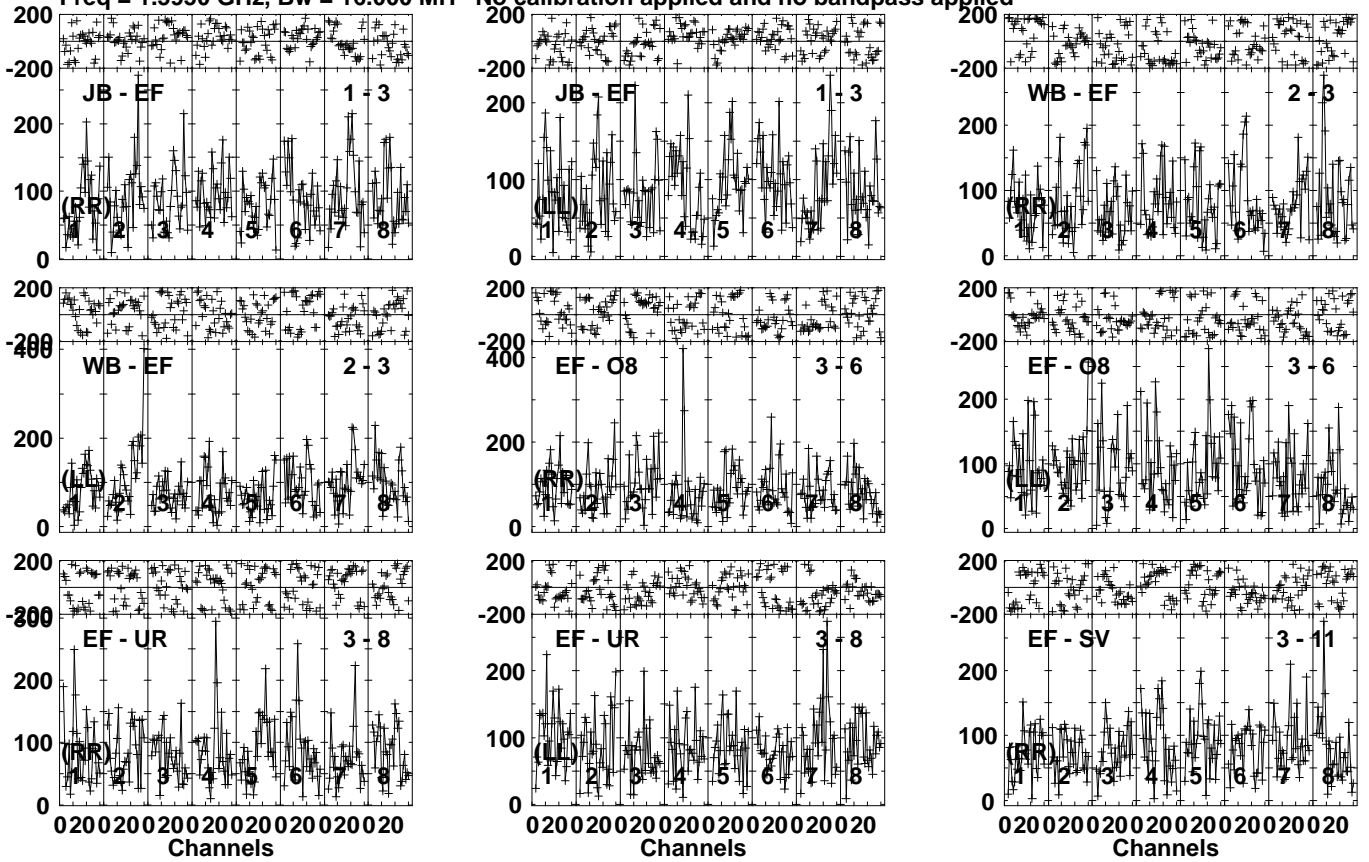
Lower frame: Micro Ampl Jy Top frame: Phas deg Vector averaged cross-power spectrum Several baselines displayed Timerange: 00/15:23:13 to 00/15:26:41
