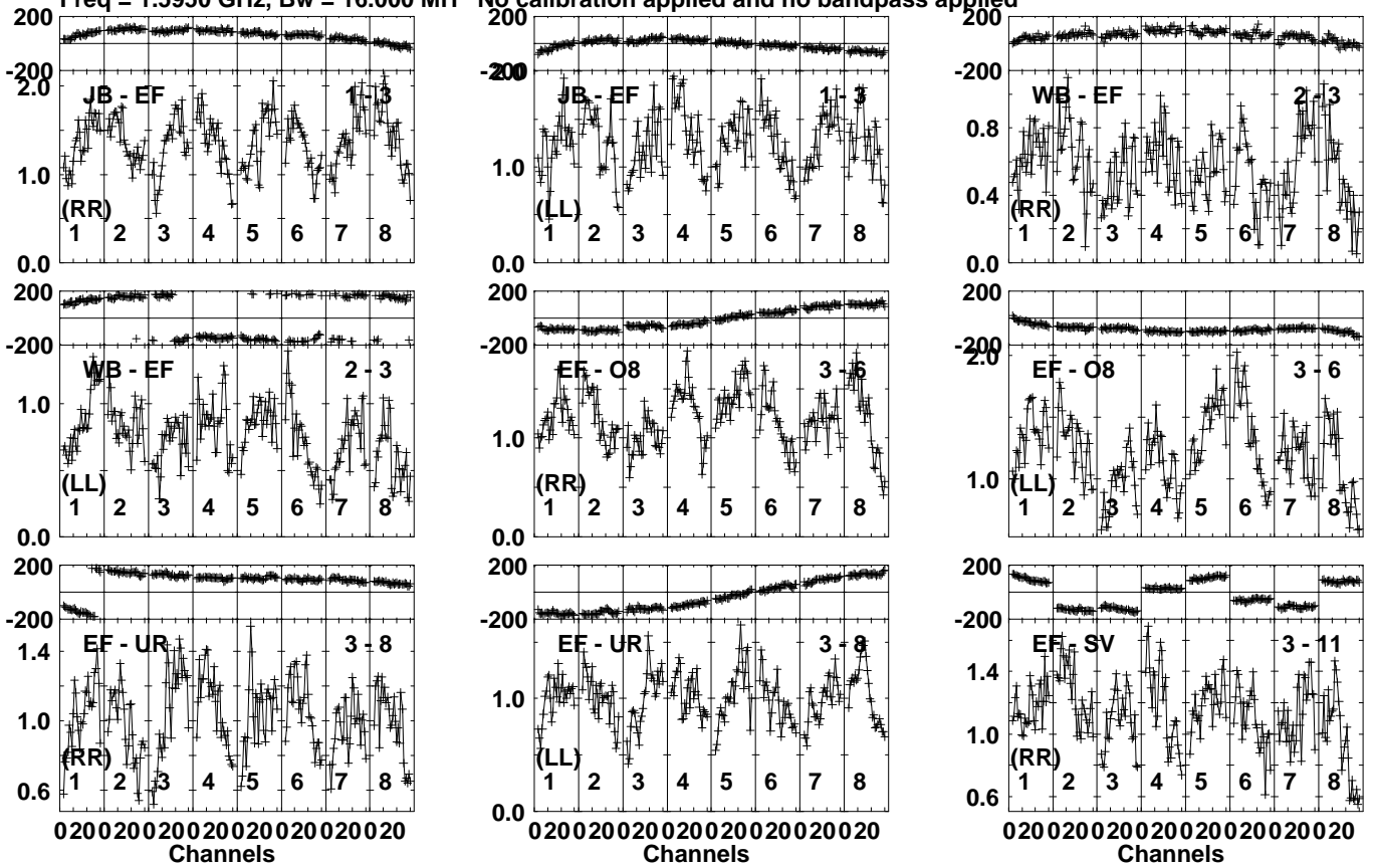
Lower frame: Milli Ampl Jy Top frame: Phas deg Vector averaged cross-power spectrum Several baselines displayed Timerange: 00/19:44:29 to 00/19:45:57
