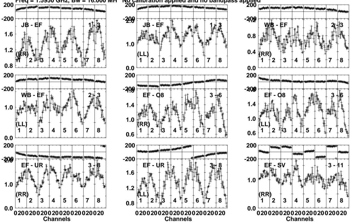
Lower frame: Milli Ampl Jy Top frame: Phas deg Vector averaged cross-power spectrum Several baselines displayed Timerange: 00/15:37:38 to 00/15:39:00
