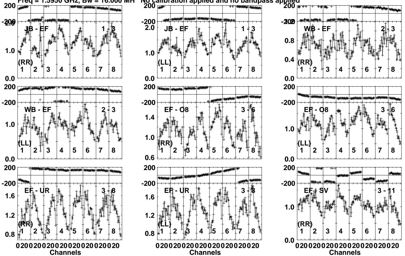
Lower frame: Milli Ampl Jy Top frame: Phas deg Vector averaged cross-power spectrum Several baselines displayed Timerange: 00/15:16:48 to 00/15:18:10
