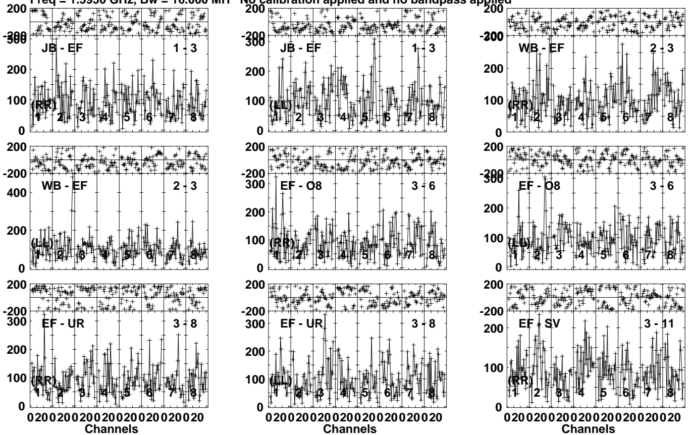
Lower frame: Micro Ampl Jy Top frame: Phas deg Vector averaged cross-power spectrum Several baselines displayed Timerange: 00/17:57:24 to 00/18:00:52
