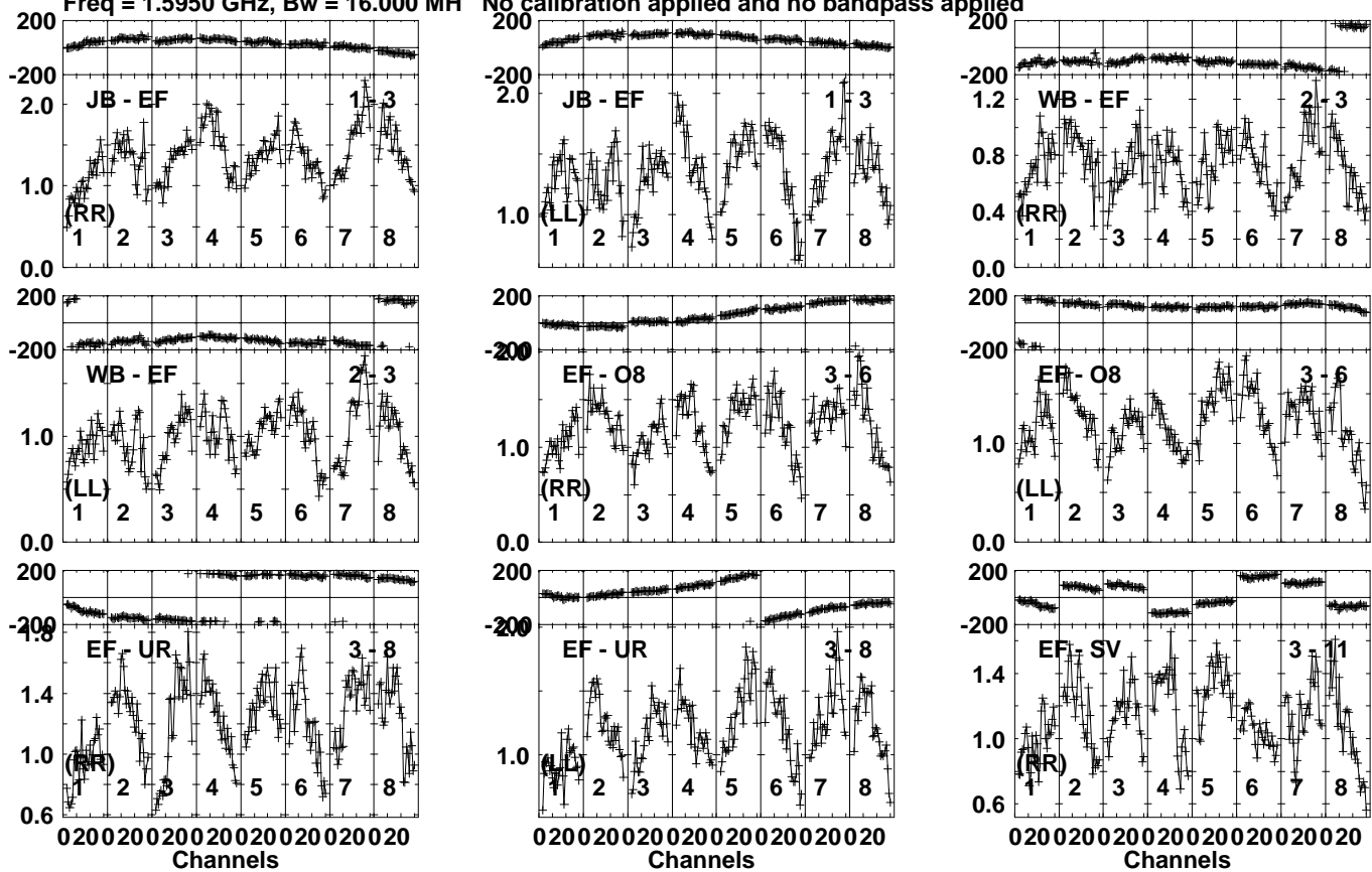
Lower frame: Milli Ampl Jy Top frame: Phas deg Vector averaged cross-power spectrum Several baselines displayed Timerange: 00/17:55:59 to 00/17:57:21
