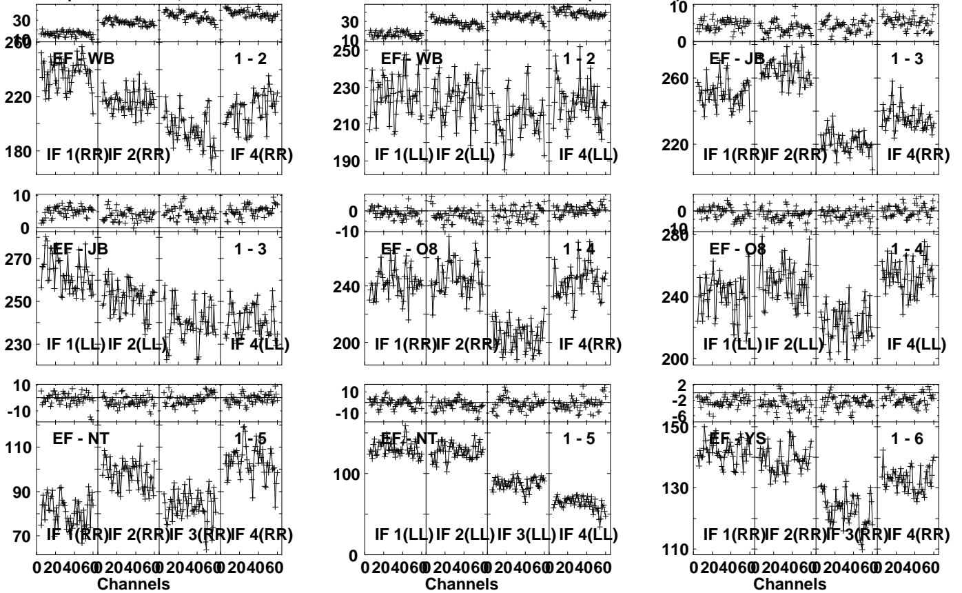
Lower frame: Milli Ampl Jy Top frame: Phas deg Vector averaged cross-power spectrum Several baselines displayed Timerange: 00:18:58:41 to 00:19:00:19
