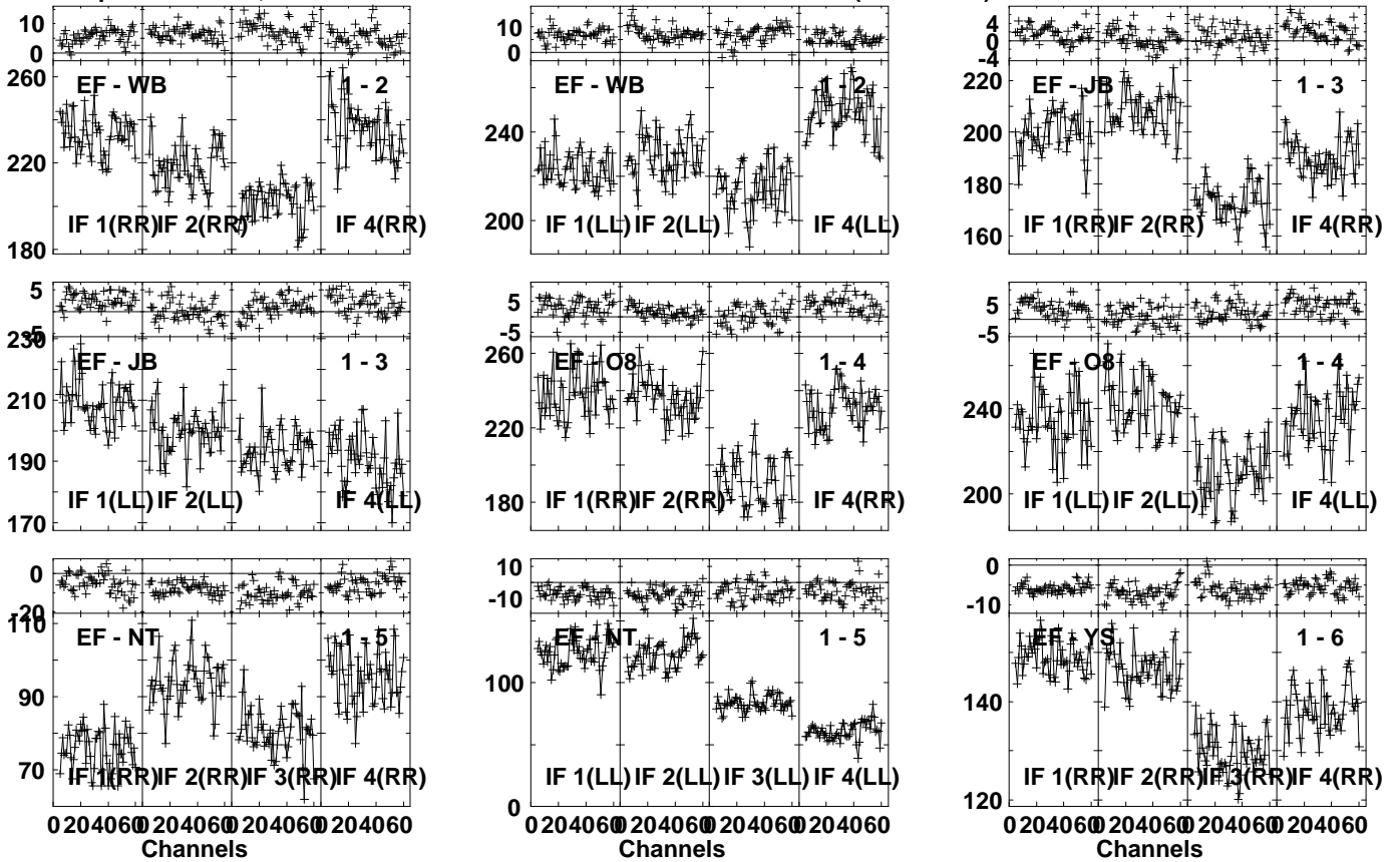
Lower frame: Milli Ampl Jy Top frame: Phas deg Vector averaged cross-power spectrum Several baselines displayed Timerange: 00/17:33:21 to 00/17:34:59
