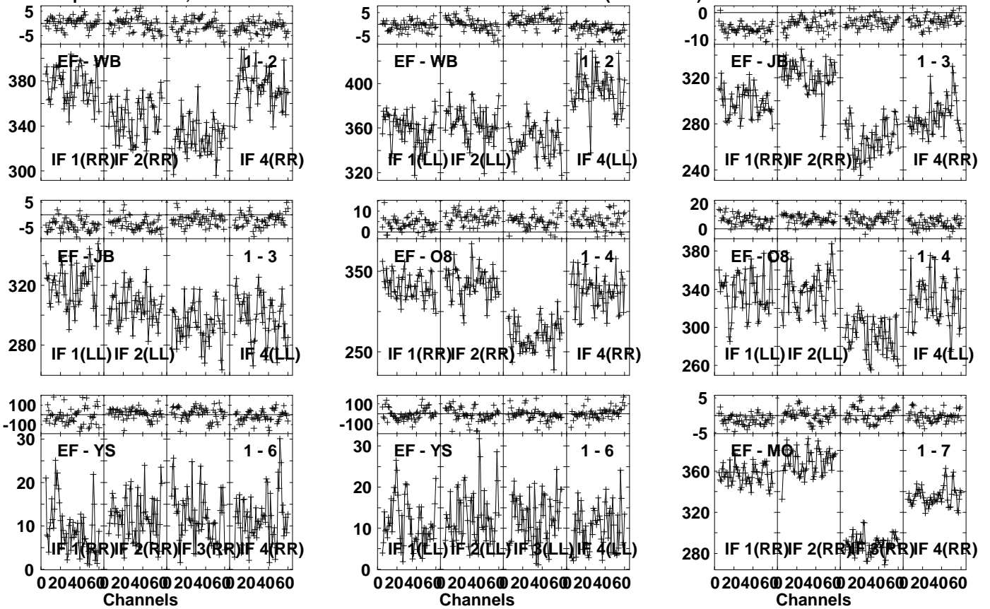
Lower frame: Milli Ampl Jy Top frame: Phas deg Vector averaged cross-power spectrum Several baselines displayed Timerange: 00/23:42:21 to 00/23:43:59
