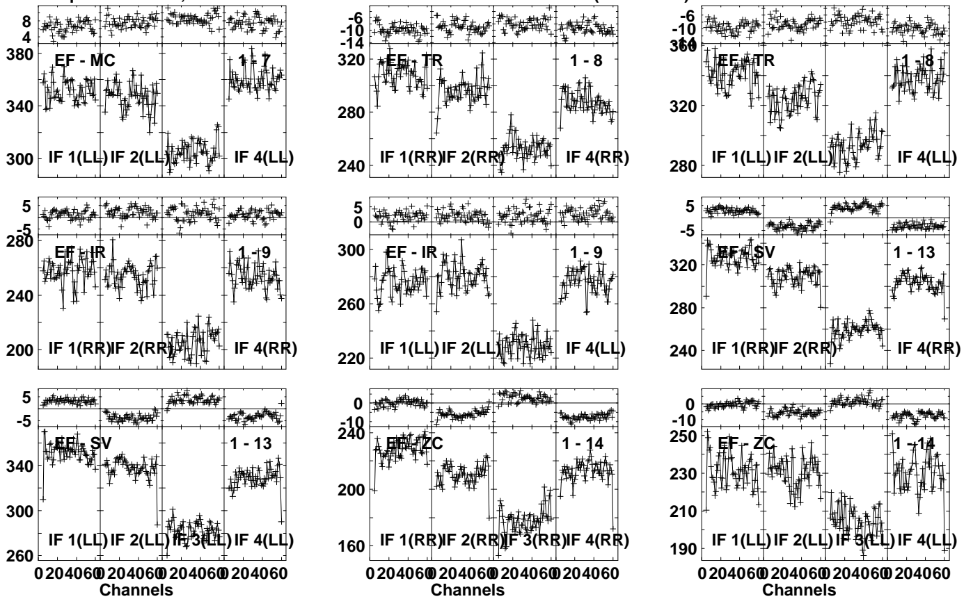
Lower frame: Milli Ampl Jy Top frame: Phas deg Vector averaged cross-power spectrum Several baselines displayed Timerange: 01/02:02:01 to 01/02:03:39
