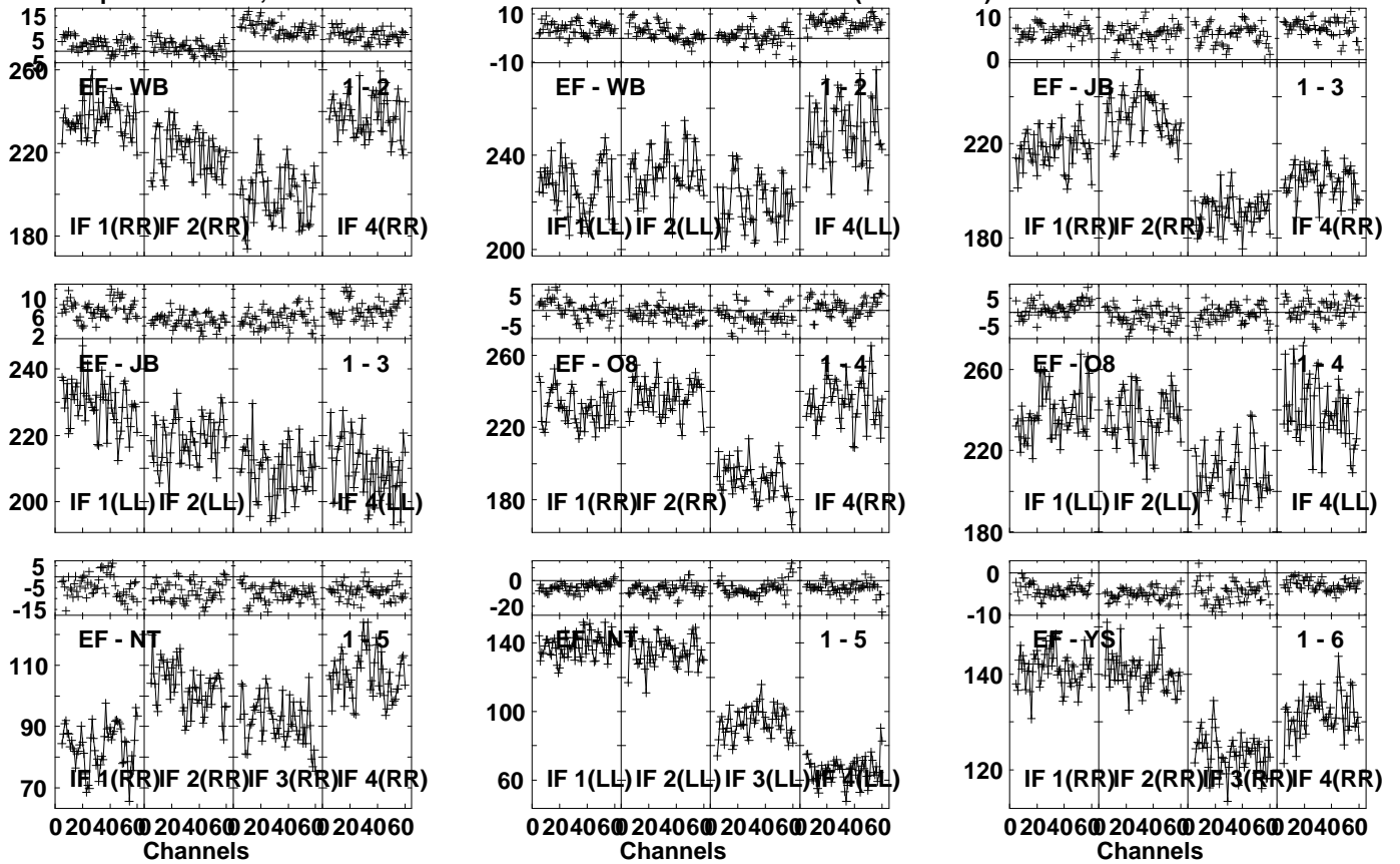
Lower frame: Milli Ampl Jy Top frame: Phas deg Vector averaged cross-power spectrum Several baselines displayed Timerange: 00/18:16:01 to 00/18:17:39
