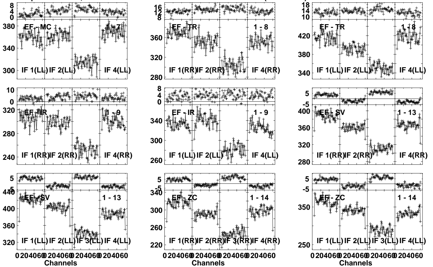
Lower frame: Milli Ampl Jy Top frame: Phas deg Vector averaged cross-power spectrum Several baselines displayed Timerange: 01/03:36:31 to 01/03:38:09
