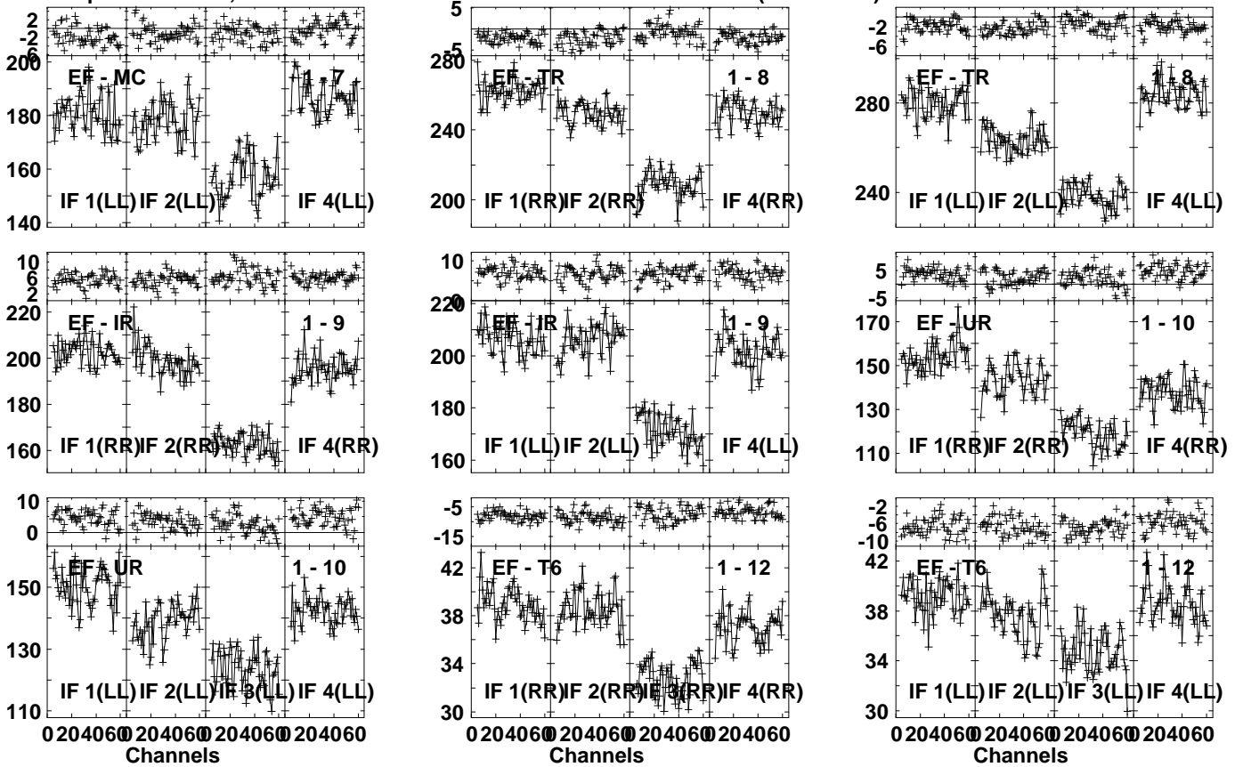
Lower frame: Milli Ampl Jy Top frame: Phas deg Vector averaged cross-power spectrum Several baselines displayed Timerange: 00:16:45:21 to 00:16:46:59
