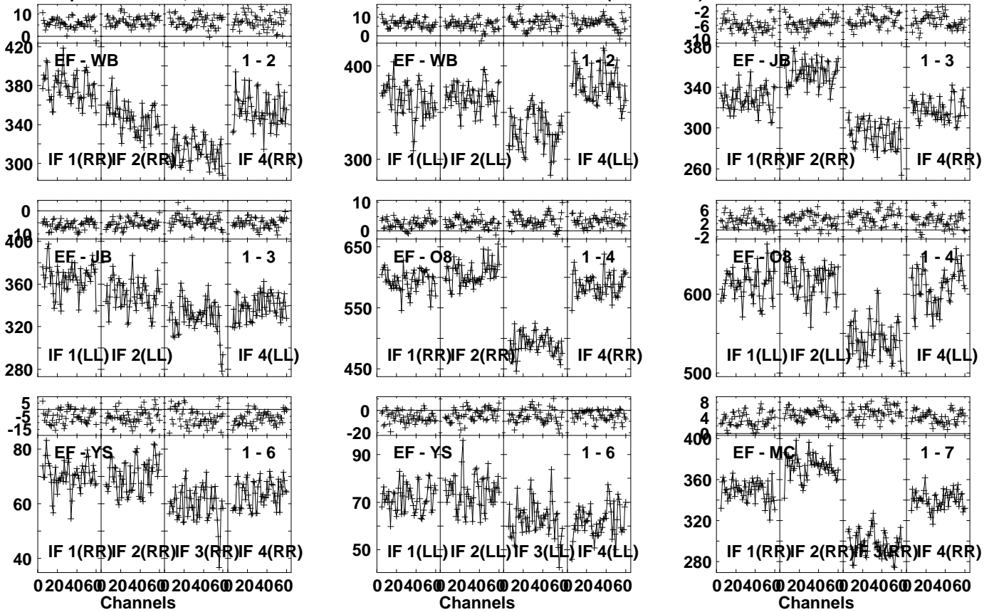
Lower frame: Milli Ampl Jy Top frame: Phas deg Vector averaged cross-power spectrum Several baselines displayed Timerange: 01/02:58:11 to 01/02:59:49
