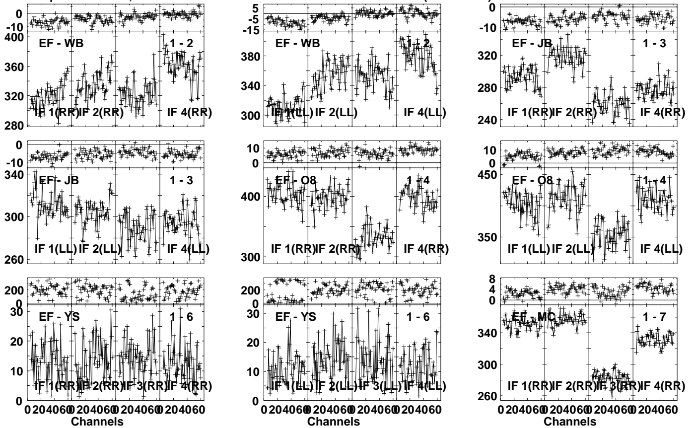
Lower frame: Milli Ampl Jy Top frame: Phas deg Vector averaged cross-power spectrum Several baselines displayed Timerange: 01/00:52:41 to 01/00:54:19
