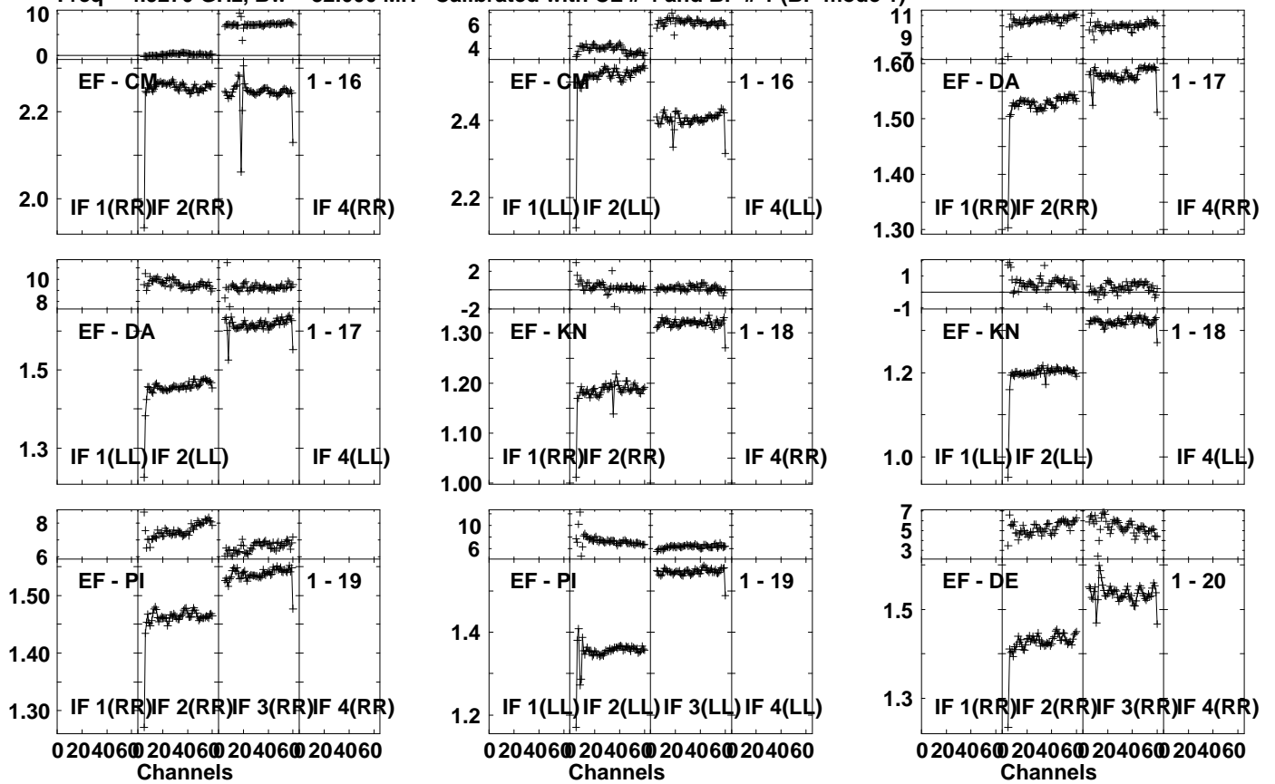
Lower frame: Ampl Jy Top frame: Phas deg Vector averaged cross-power spectrum Several baselines displayed Timerange: 00/16:07:01 to 00/16:11:59
