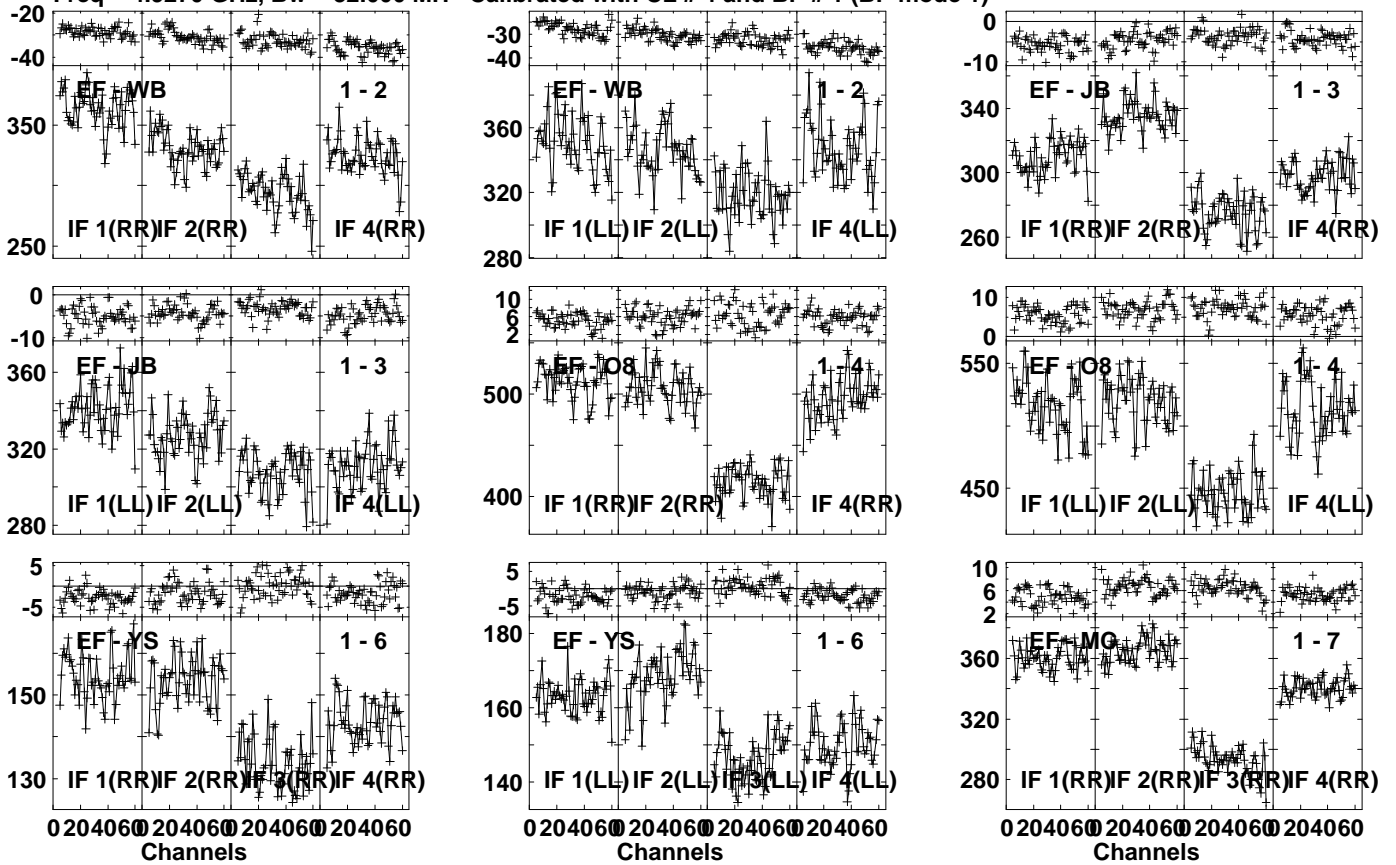
Lower frame: Milli Ampl Jy Top frame: Phas deg Vector averaged cross-power spectrum Several baselines displayed Timerange: 01/01:56:41 to 01/01:58:19
