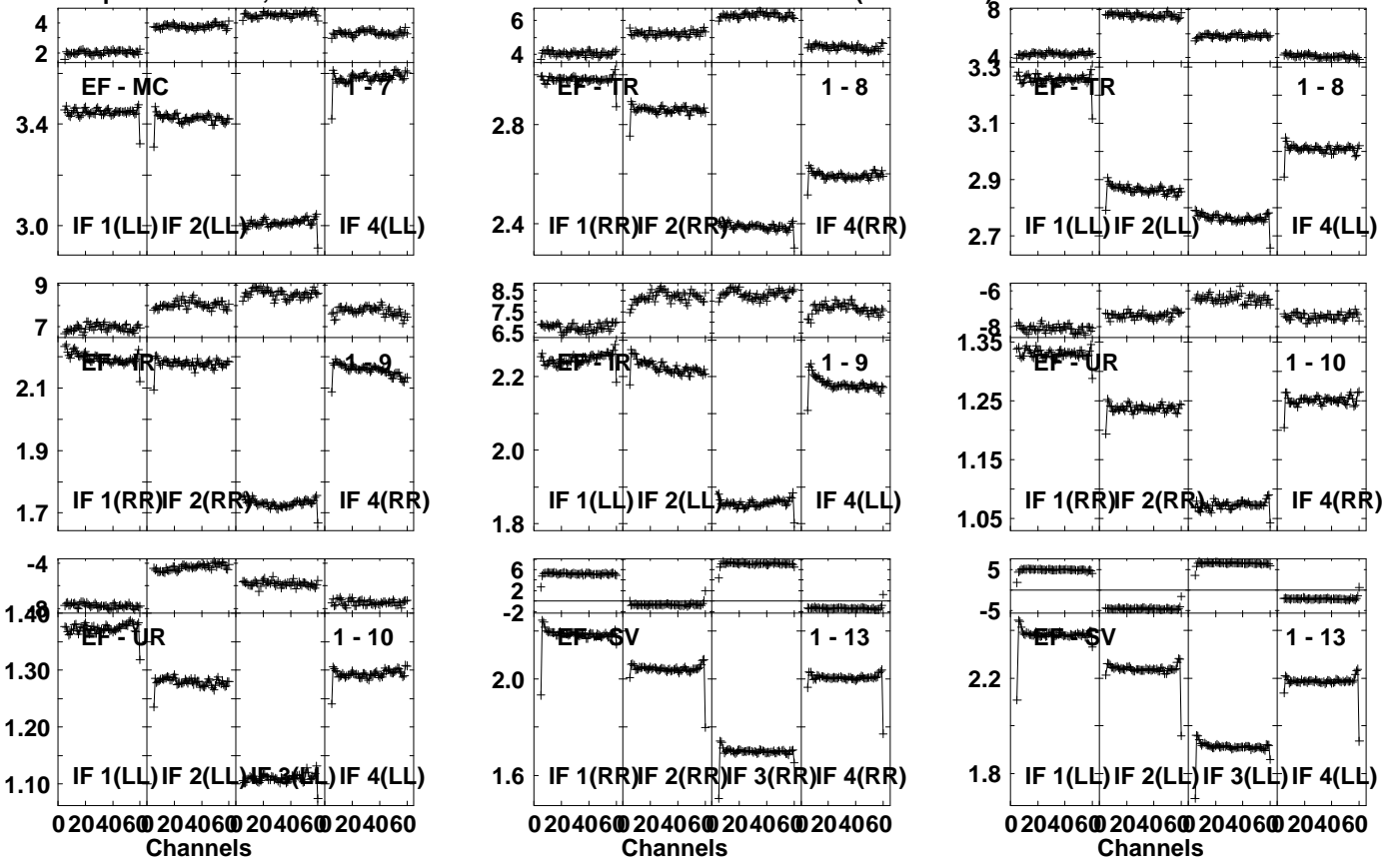
Lower frame: Ampl Jy Top frame: Phas deg Vector averaged cross-power spectrum Several baselines displayed Timerange: 00/22:48:41 to 00/22:53:39
