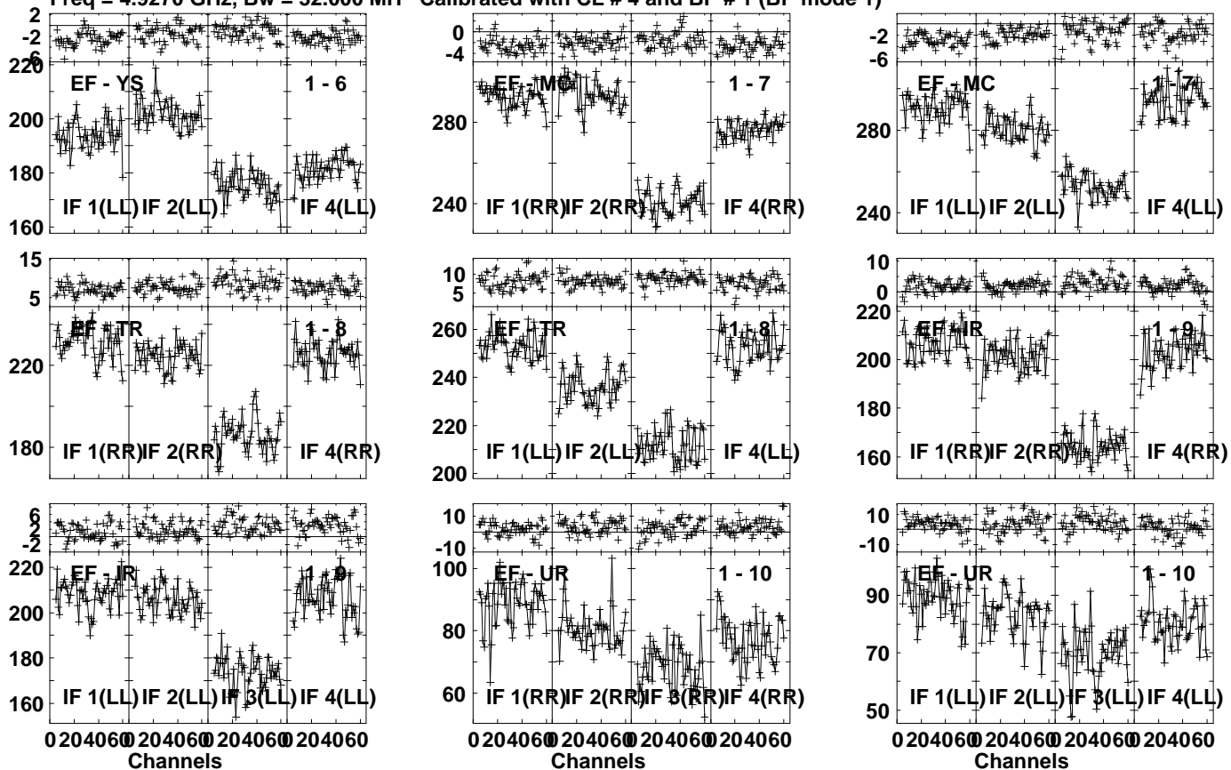
Lower frame: Milli Ampl Jy Top frame: Phas deg Vector averaged cross-power spectrum Several baselines displayed Timerange: 00:21:57:01 to 00:21:58:39
