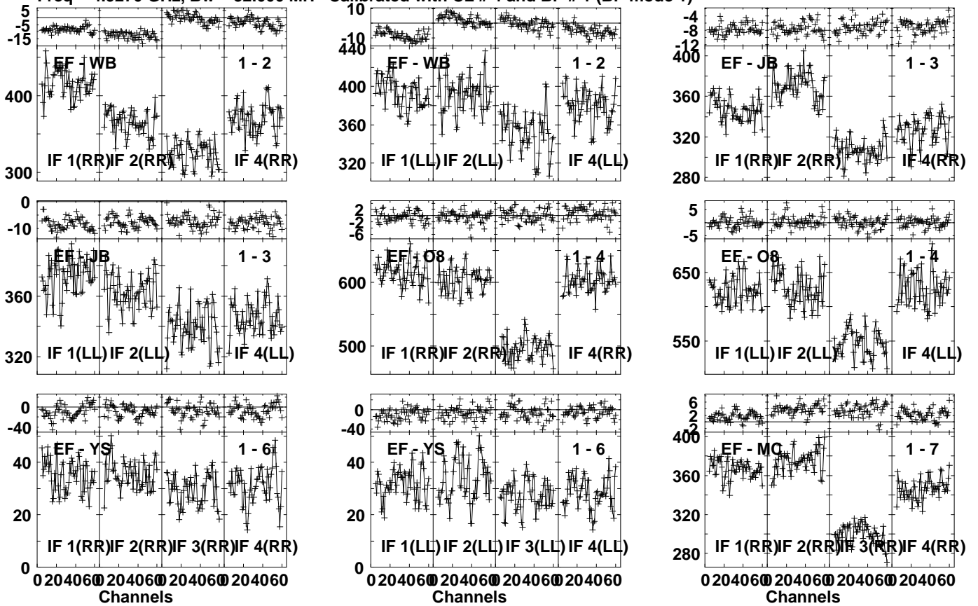
Lower frame: Milli Ampl Jy Top frame: Phas deg Vector averaged cross-power spectrum Several baselines displayed Timerange: 01/03:30:56 to 01/03:32:34
