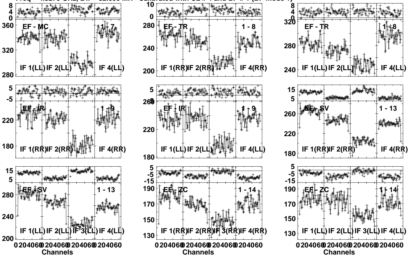
Lower frame: Milli Ampl Jy Top frame: Phas deg Vector averaged cross-power spectrum Several baselines displayed Timerange: 01/00:09:01 to 01/00:10:39
