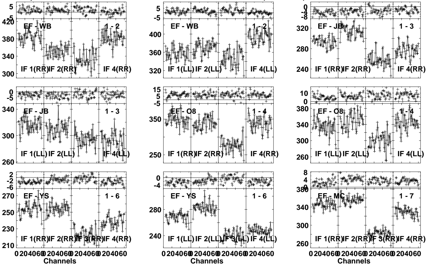
Lower frame: Milli Ampl Jy Top frame: Phas deg Vector averaged cross-power spectrum Several baselines displayed Timerange: 01/00:03:41 to 01/00:05:19
