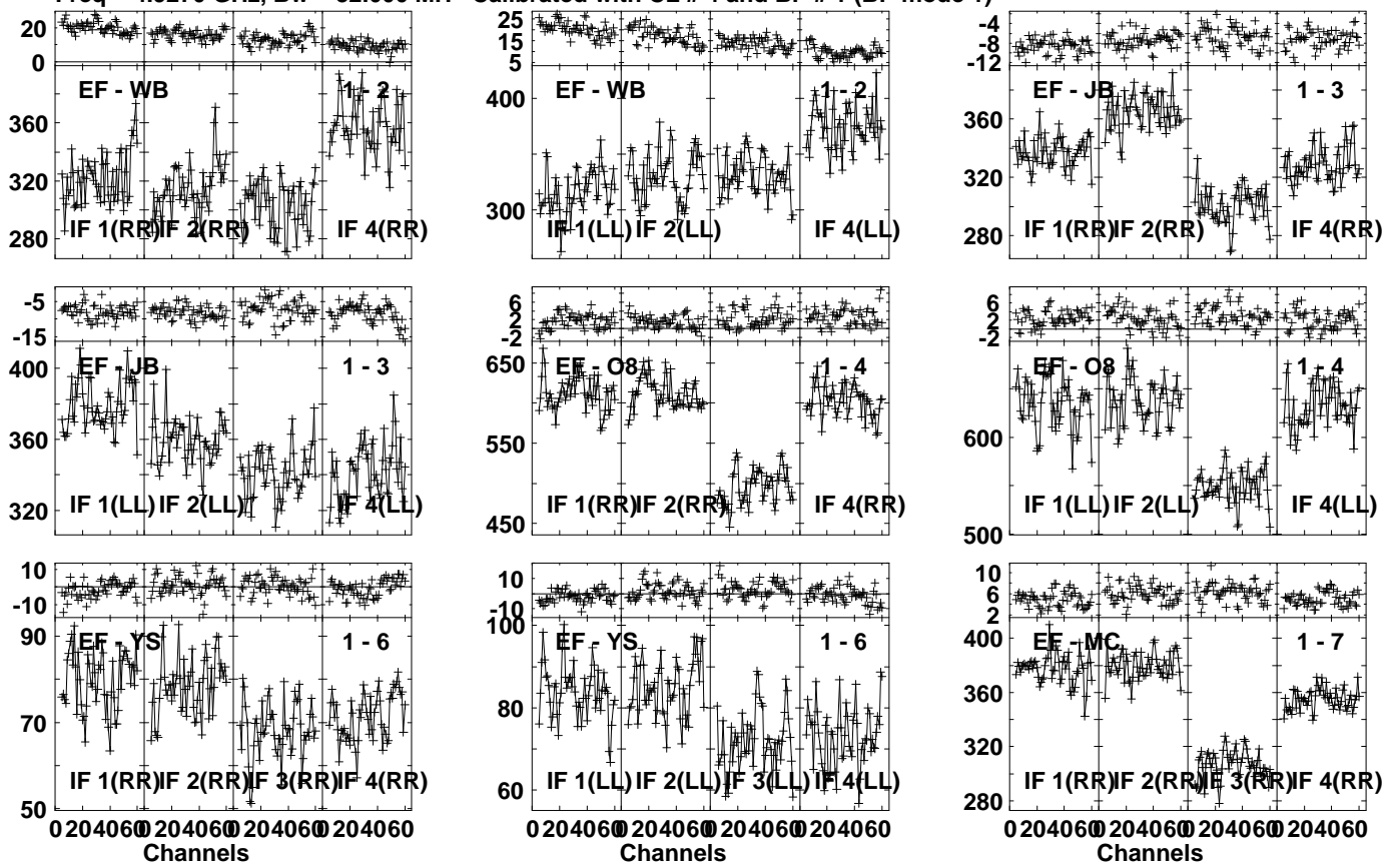
Lower frame: Milli Ampl Jy Top frame: Phas deg Vector averaged cross-power spectrum Several baselines displayed Timerange: 01/02:52:51 to 01/02:54:29
