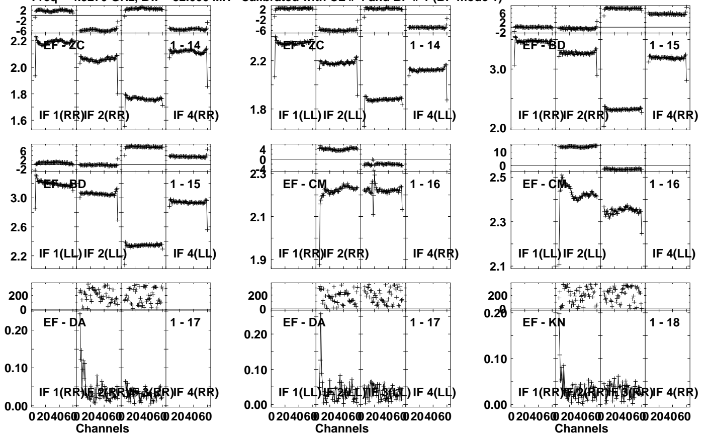
Lower frame: Ampl Jy Top frame: Phas deg Vector averaged cross-power spectrum Several baselines displayed Timerange: 01/00:36:01 to 01/00:41:59
