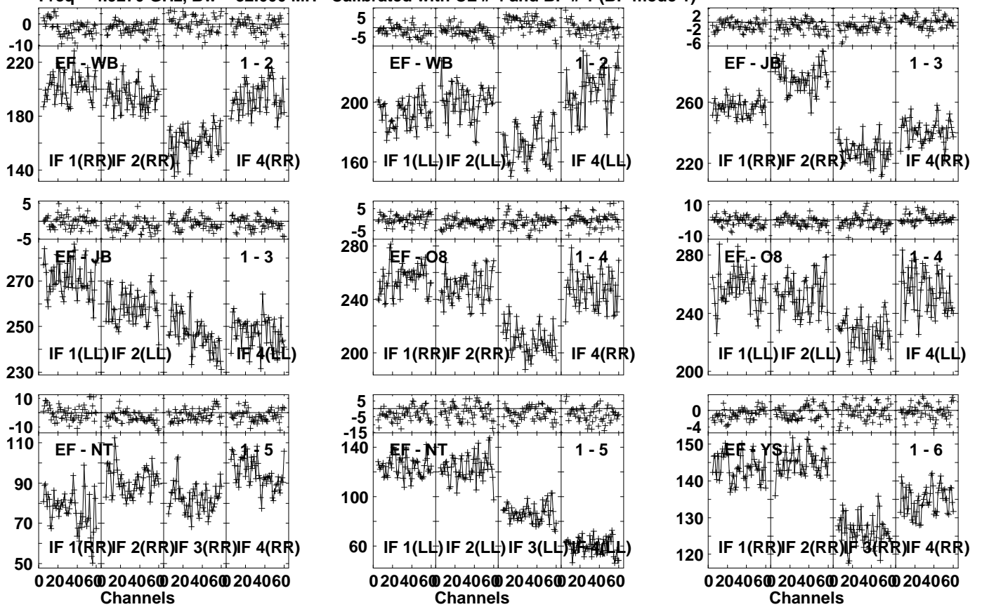
Lower frame: Milli Ampl Jy Top frame: Phas deg Vector averaged cross-power spectrum Several baselines displayed Timerange: 00/19:14:41 to 00/19:16:19
