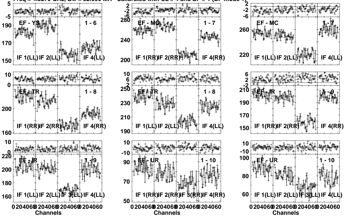
Lower frame: Milli Ampl Jy Top frame: Phas deg Vector averaged cross-power spectrum Several baselines displayed Timerange: 00/21:03:41 to 00/21:05:19
