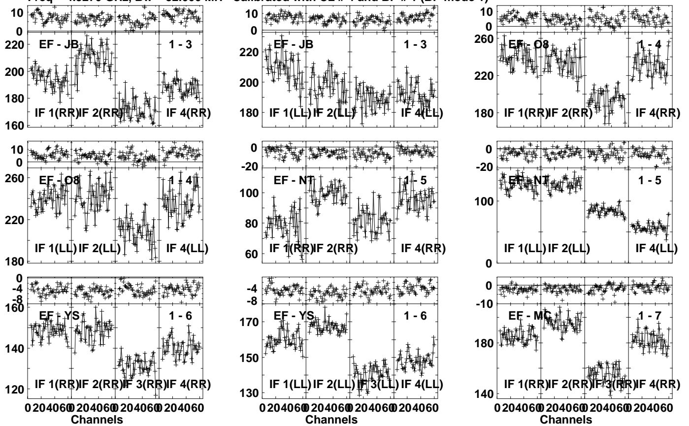
Lower frame: Milli Ampl Jy Top frame: Phas deg Vector averaged cross-power spectrum Several baselines displayed Timerange: 00/17:22:41 to 00/17:24:19
