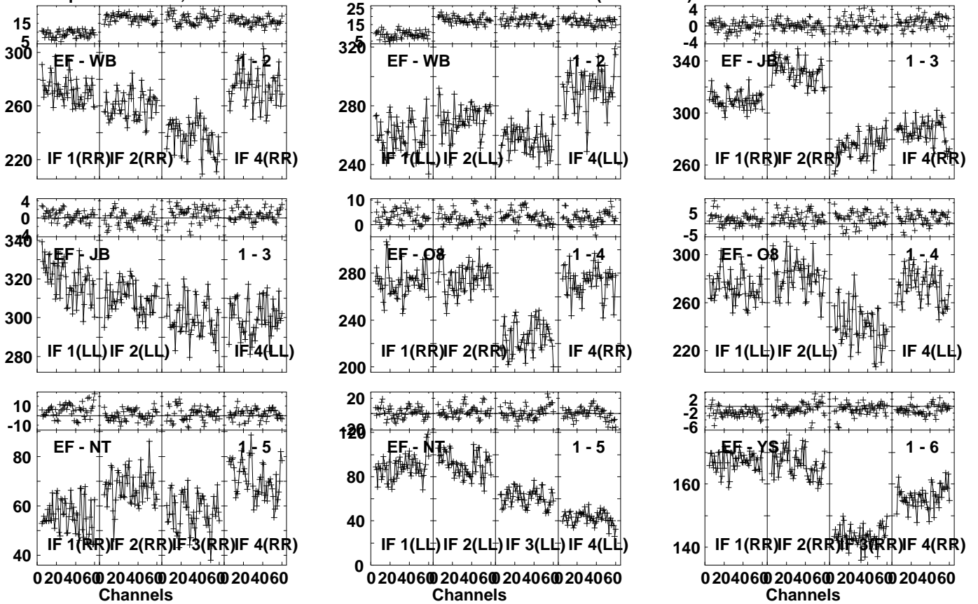
Lower frame: Milli Ampl Jy Top frame: Phas deg Vector averaged cross-power spectrum Several baselines displayed Timerange: 00/21:09:01 to 00/21:10:39
