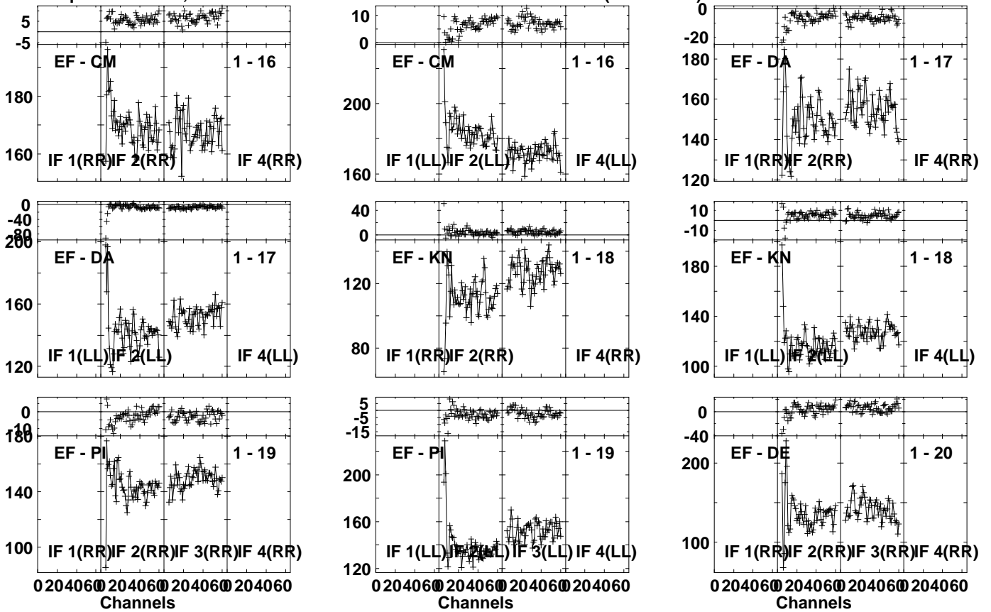
Lower frame: Milli Ampl Jy Top frame: Phas deg Vector averaged cross-power spectrum Several baselines displayed Timerange: 00/16:24:01 to 00/16:25:39
