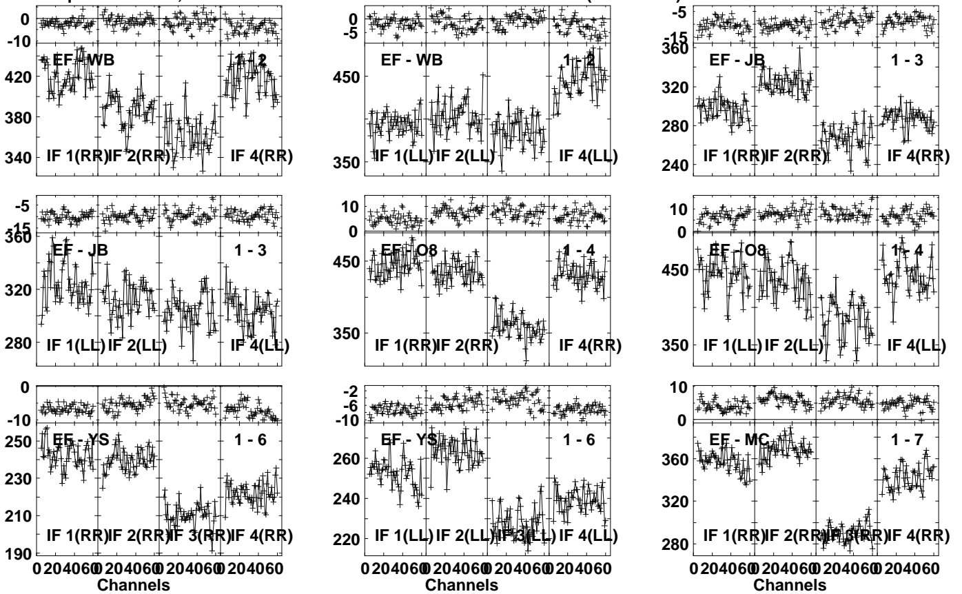
Lower frame: Milli Ampl Jy Top frame: Phas deg Vector averaged cross-power spectrum Several baselines displayed Timerange: 01/01:08:41 to 01/01:10:19
