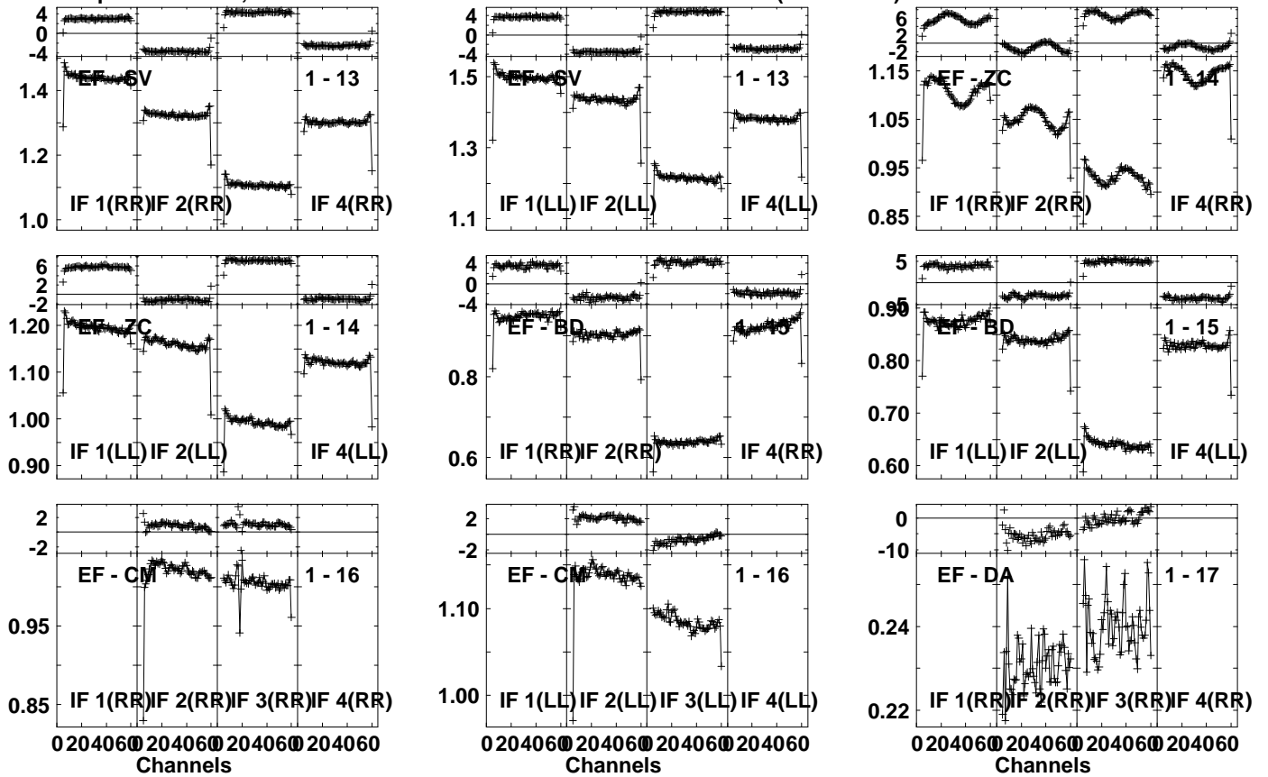
Lower frame: Ampl Jy Top frame: Phas deg Vector averaged cross-power spectrum Several baselines displayed Timerange: 00/20:12:41 to 00/20:17:39
