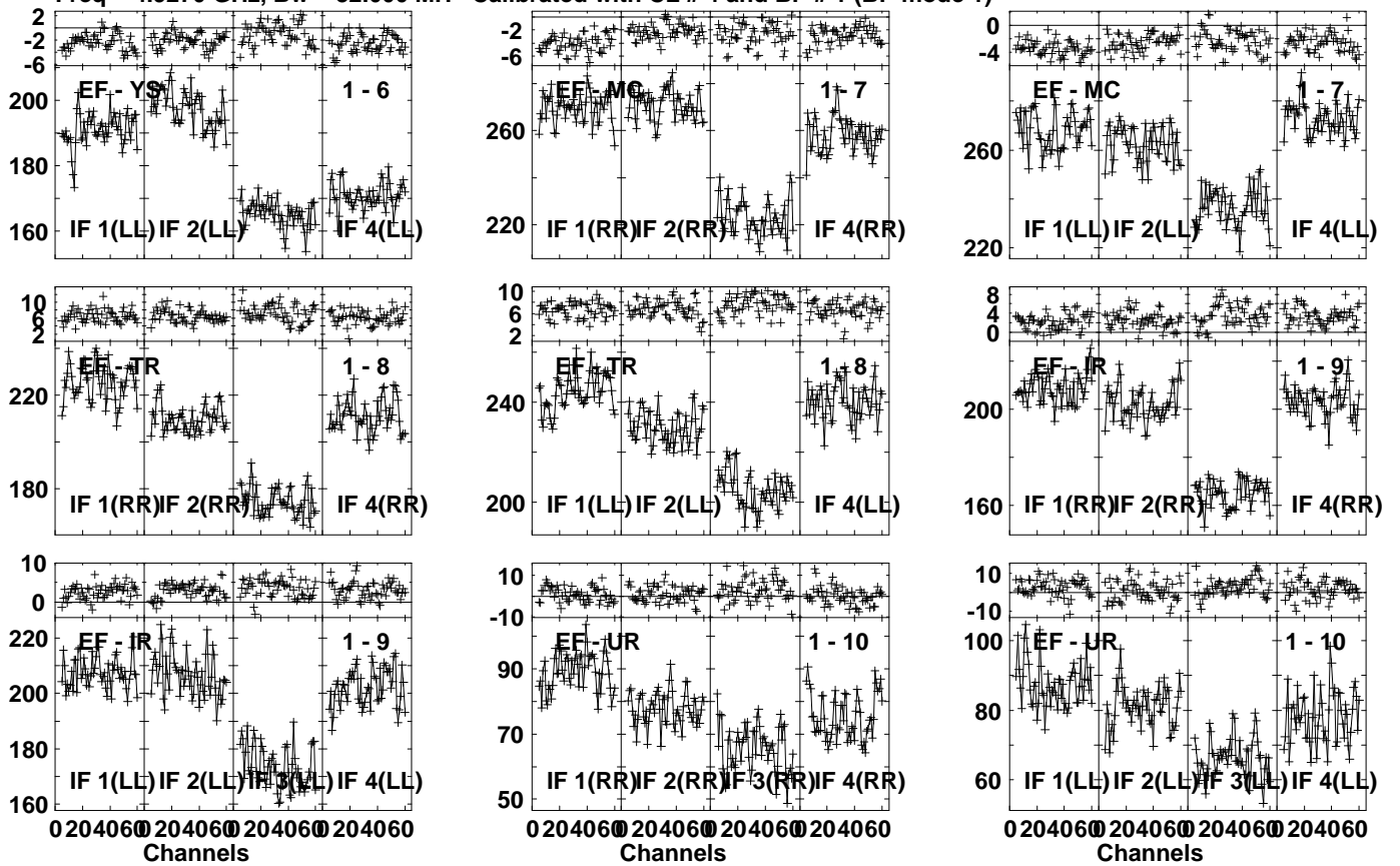
Lower frame: Milli Ampl Jy Top frame: Phas deg Vector averaged cross-power spectrum Several baselines displayed Timerange: 00/21:25:01 to 00/21:26:39
