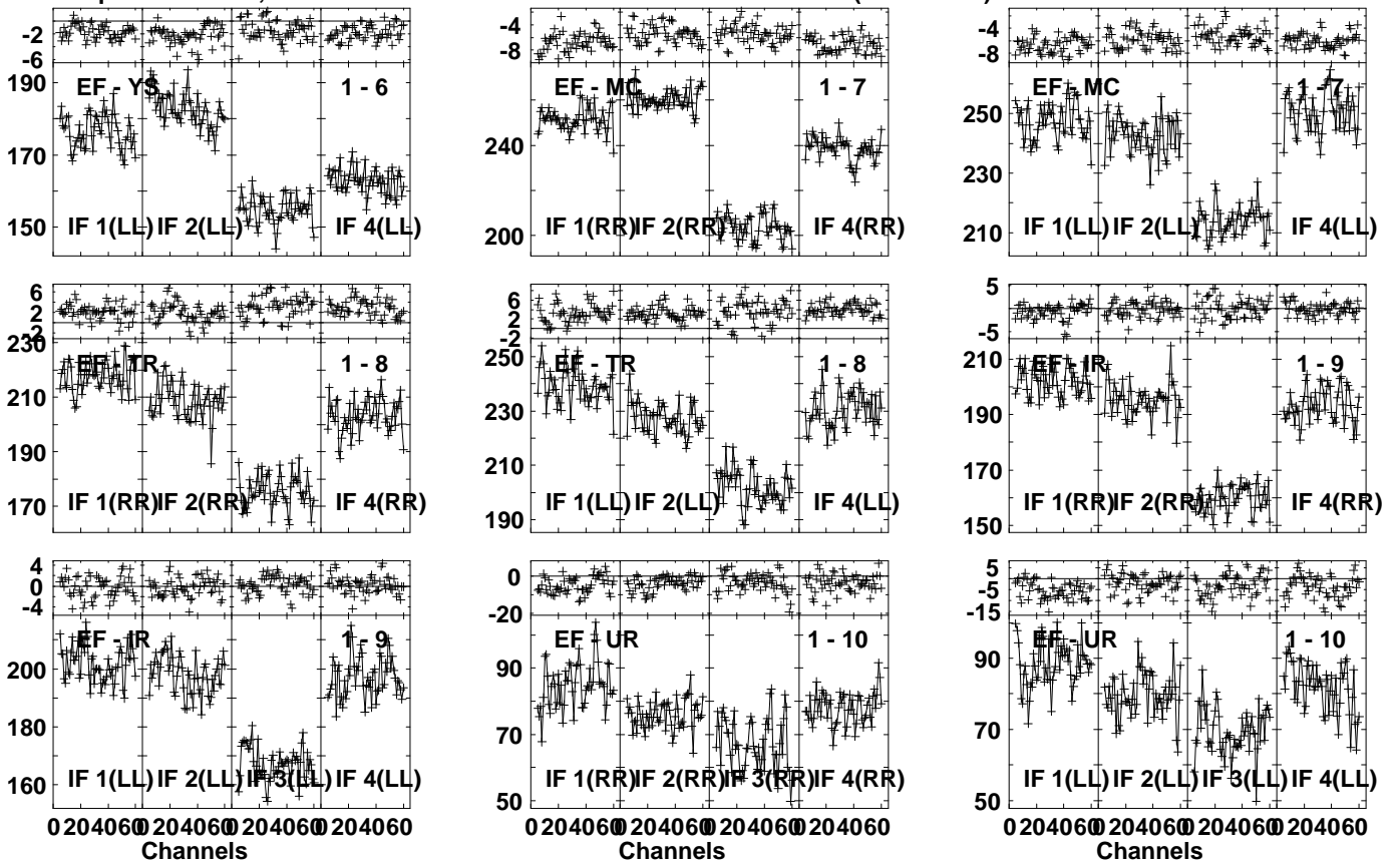
Lower frame: Milli Ampl Jy Top frame: Phas deg Vector averaged cross-power spectrum Several baselines displayed Timerange: 00/20:53:01 to 00/20:54:39
