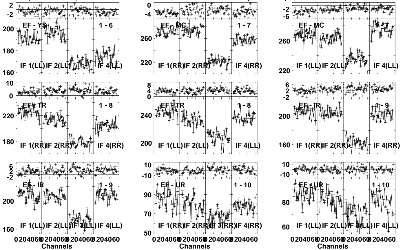
Lower frame: Milli Ampl Jy Top frame: Phas deg Vector averaged cross-power spectrum Several baselines displayed Timerange: 00:21:30:21 to 00:21:31:59
