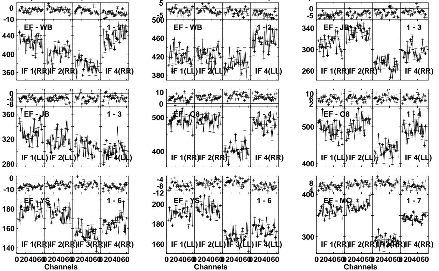
Lower frame: Milli Ampl Jy Top frame: Phas deg Vector averaged cross-power spectrum Several baselines displayed Timerange: 01/01:46:01 to 01/01:47:39
