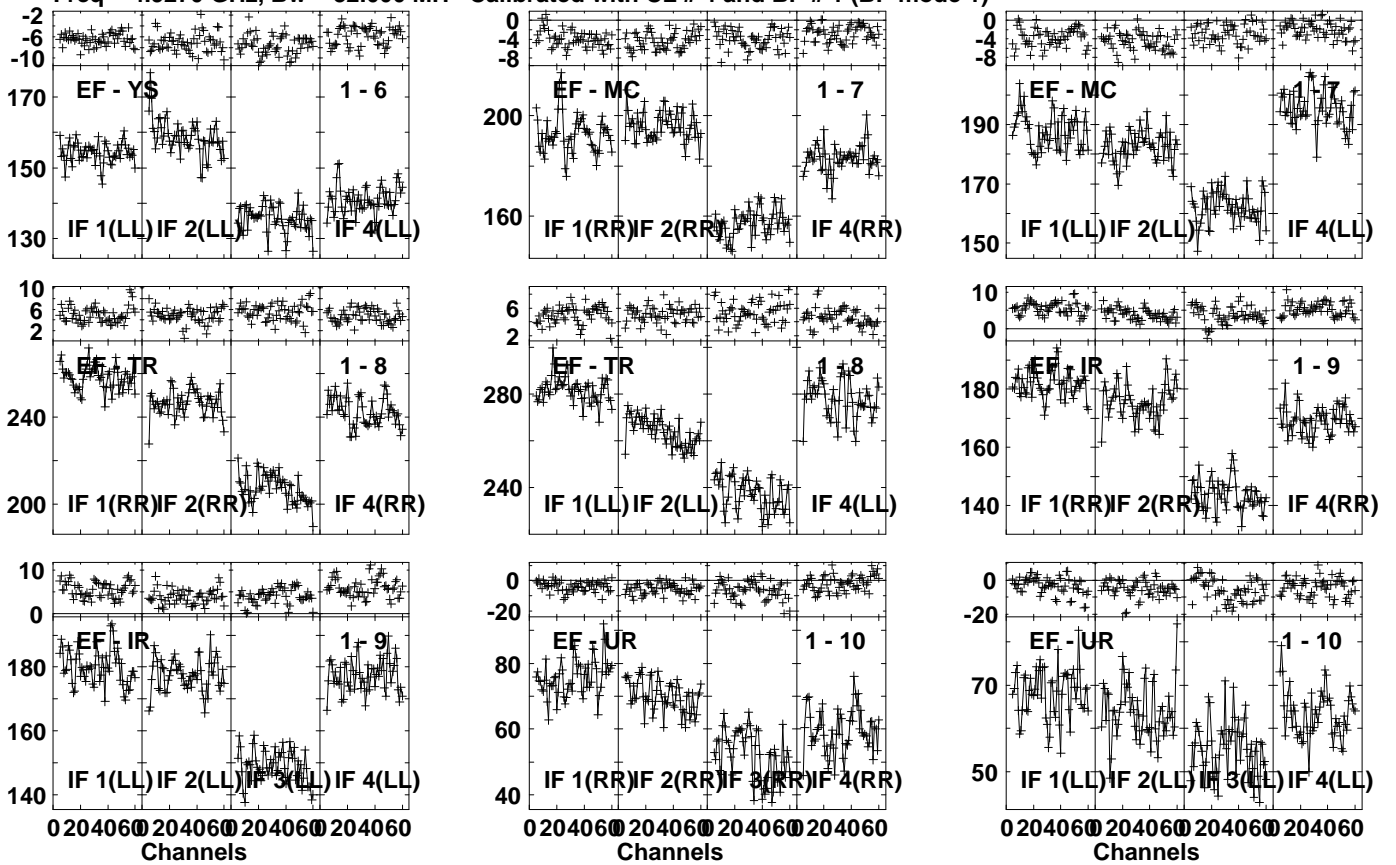
Lower frame: Milli Ampl Jy Top frame: Phas deg Vector averaged cross-power spectrum Several baselines displayed Timerange: 00/17:54:41 to 00/17:56:19
