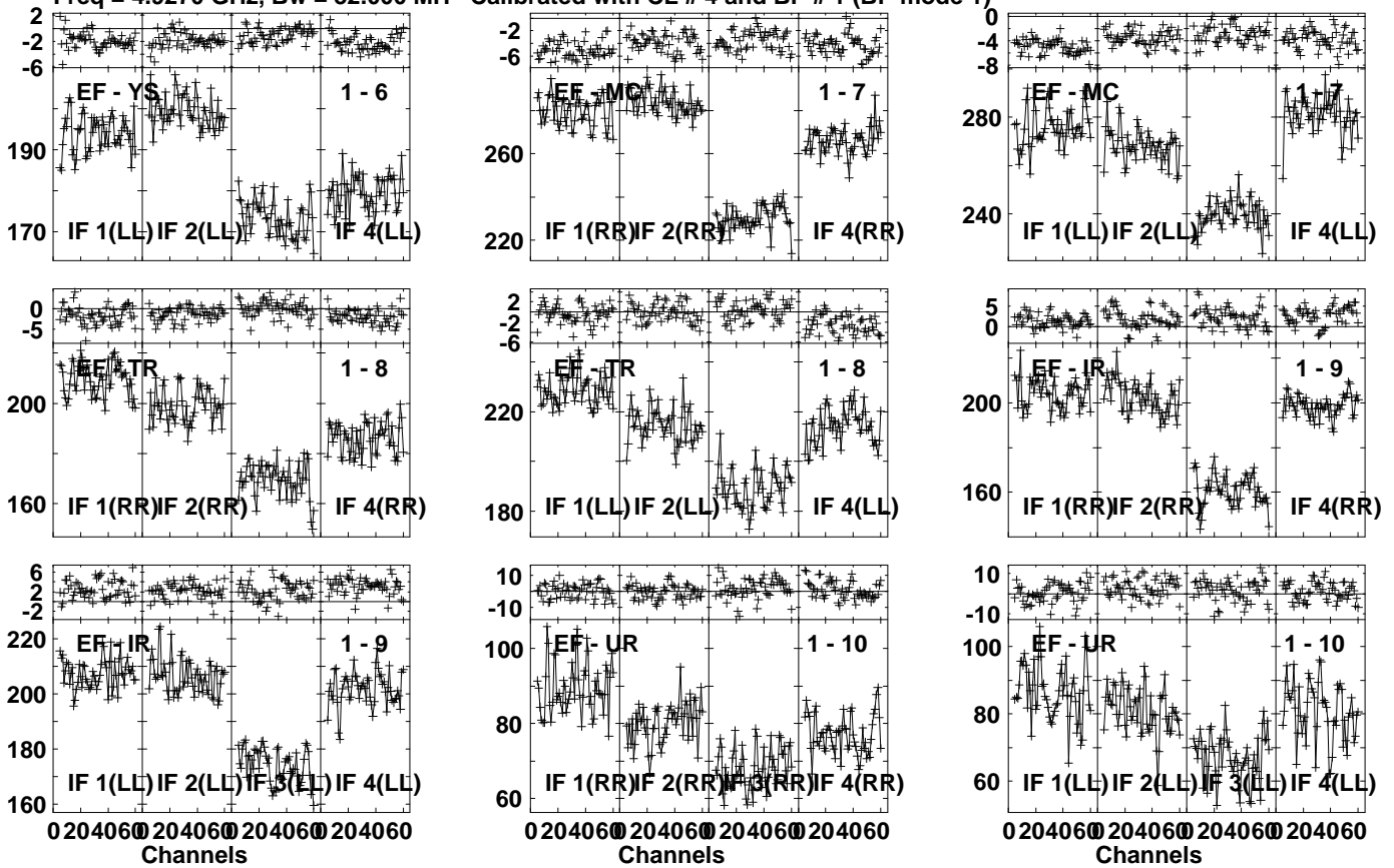
Lower frame: Milli Ampl Jy Top frame: Phas deg Vector averaged cross-power spectrum Several baselines displayed Timerange: 00/21:41:01 to 00/21:42:39
