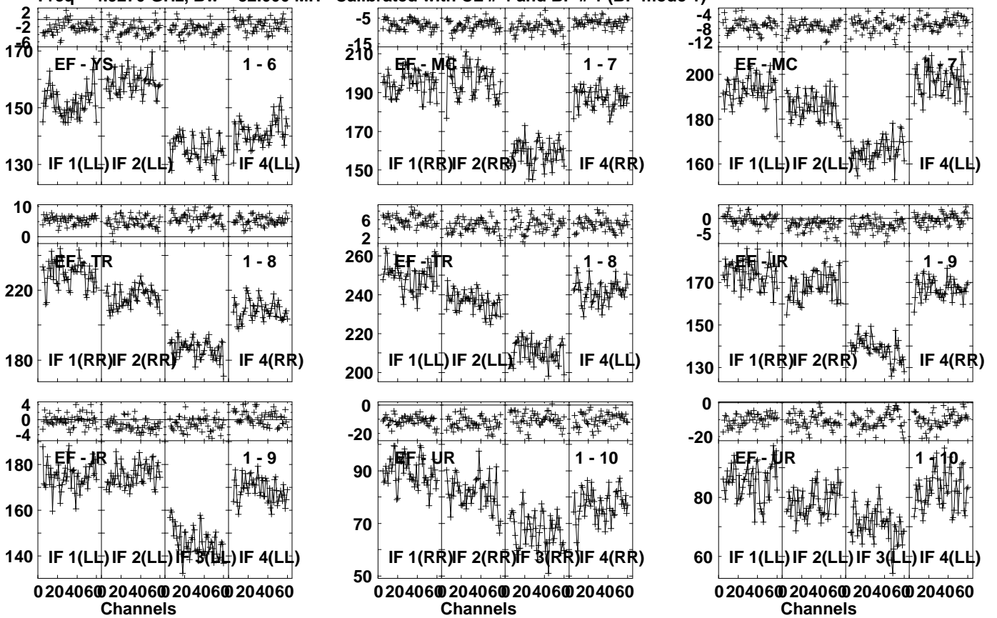
Lower frame: Milli Ampl Jy Top frame: Phas deg Vector averaged cross-power spectrum Several baselines displayed Timerange: 00/18:53:21 to 00/18:54:59
