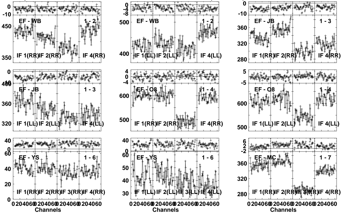
Lower frame: Milli Ampl Jy Top frame: Phas deg Vector averaged cross-power spectrum Several baselines displayed Timerange: 01/03:14:41 to 01/03:16:19
