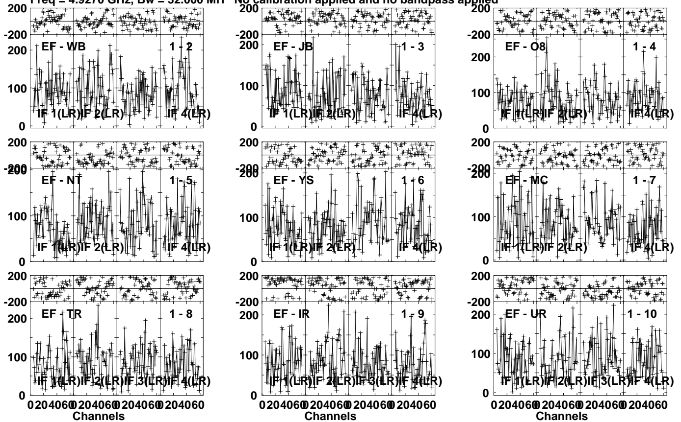
Lower frame: Micro Ampl Jy Top frame: Phas deg Vector averaged cross-power spectrum Several baselines displayed Timerange: 00/17:30:01 to 00/17:32:59
