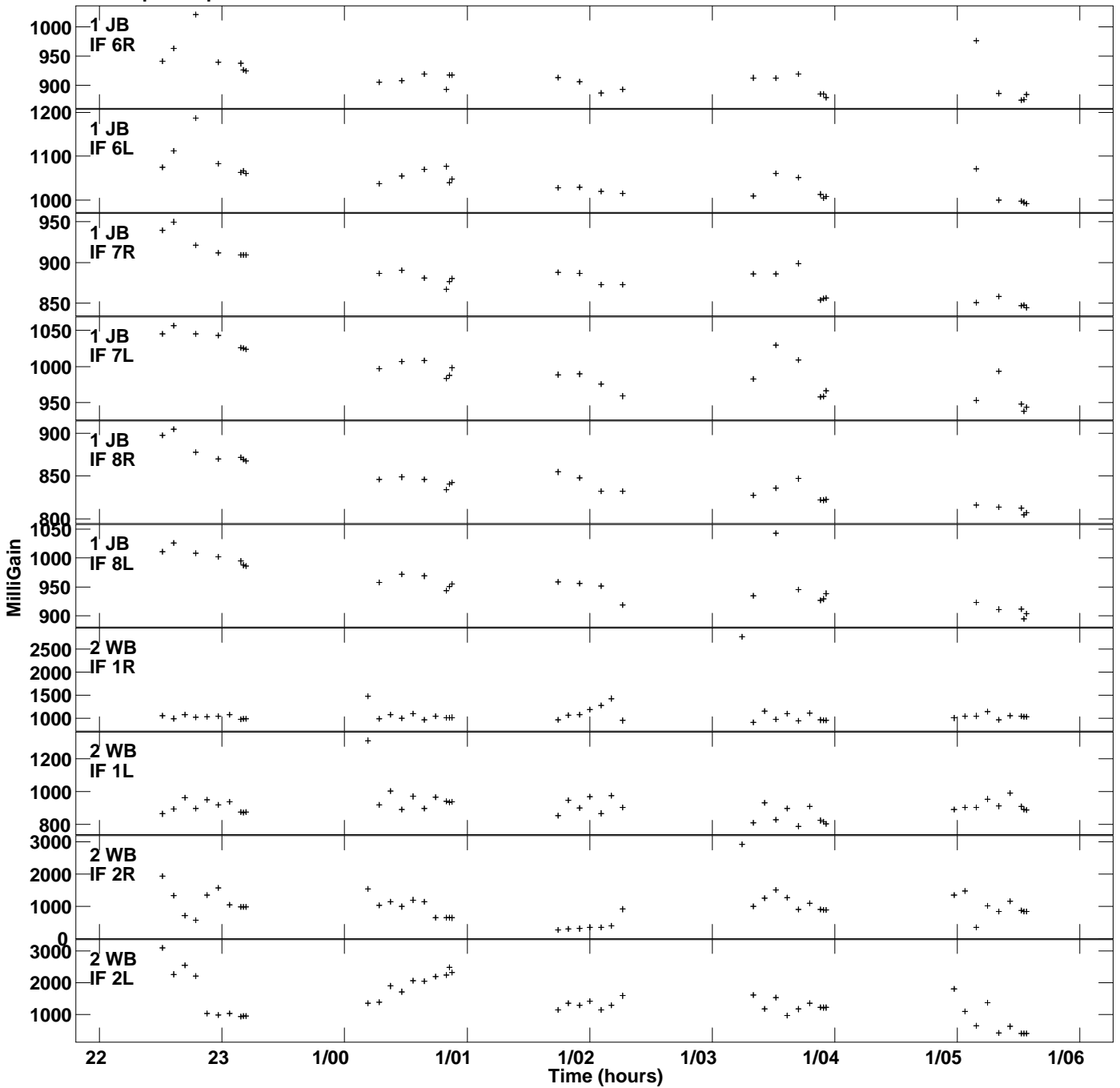
Plot file version 2 created 28-JUL-2021 18:08:06 Gain amp vs UTC time for J1329+3154.MULTI.1 SN 2 Rpol & Lpol IF 1 - 8
