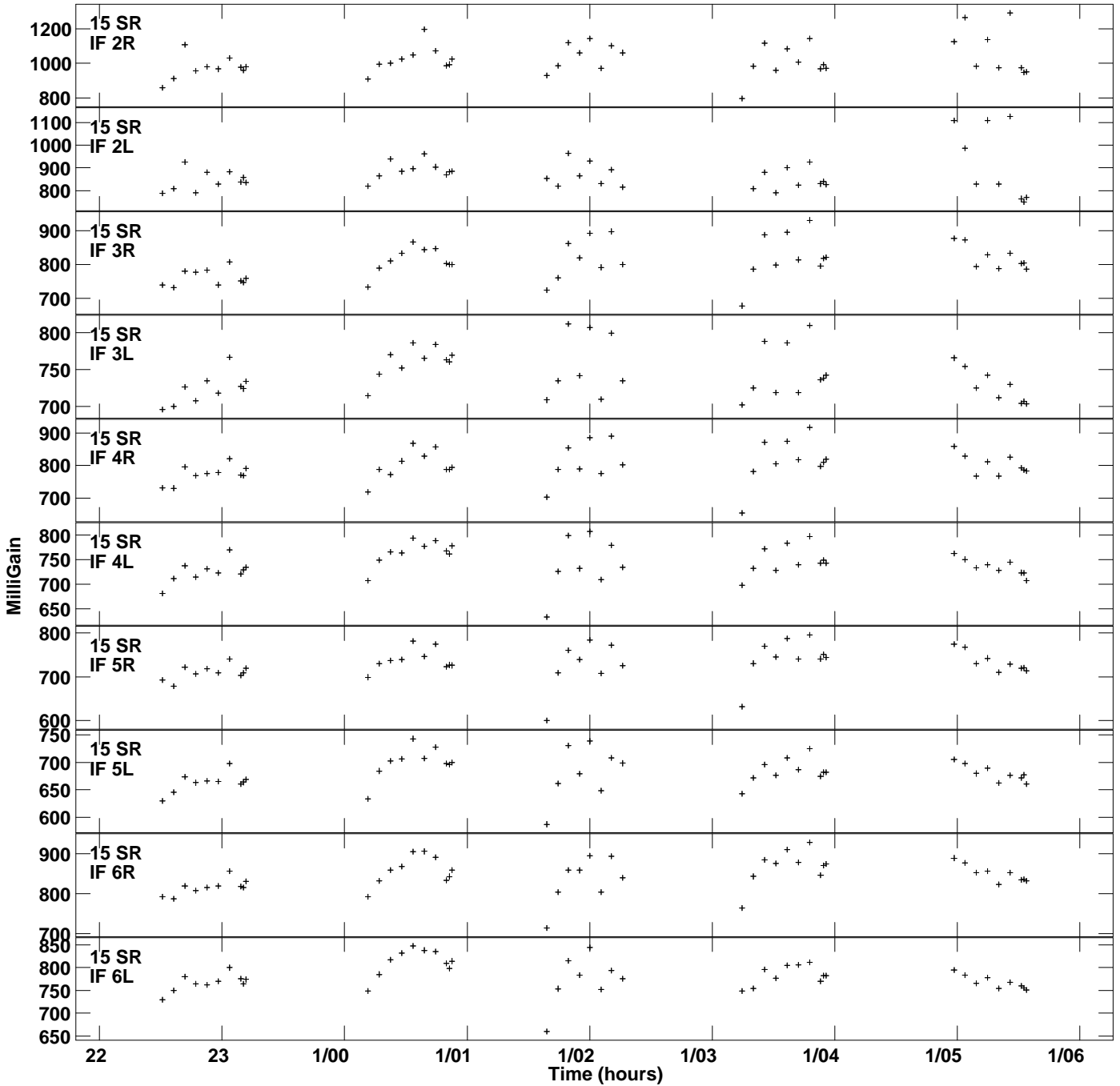
Plot file version 22 created 28-JUL-2021 18:08:07 Gain amp vs UTC time for J1329+3154.MULTI.1 SN 2 Rpol & Lpol IF 1 - 8
