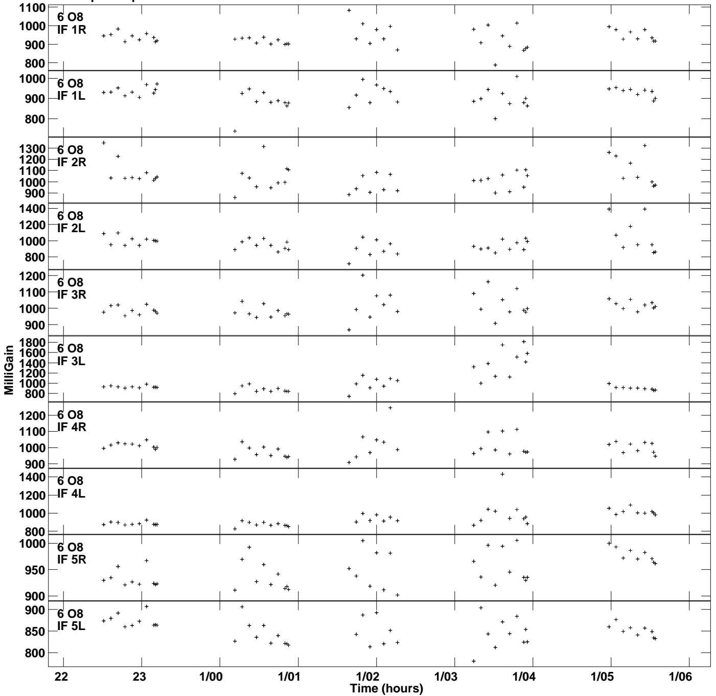
Plot file version 9 created 28-JUL-2021 18:08:07 Gain amp vs UTC time for J1329+3154.MULTI.1 SN 2 Rpol & Lpol IF 1 - 8
