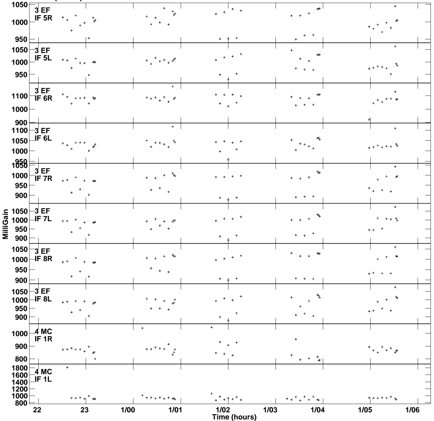
Plot file version 5 created 28-JUL-2021 18:08:06 Gain amp vs UTC time for J1329+3154.MULTI.1 SN 2 Rpol & Lpol IF 1 - 8
