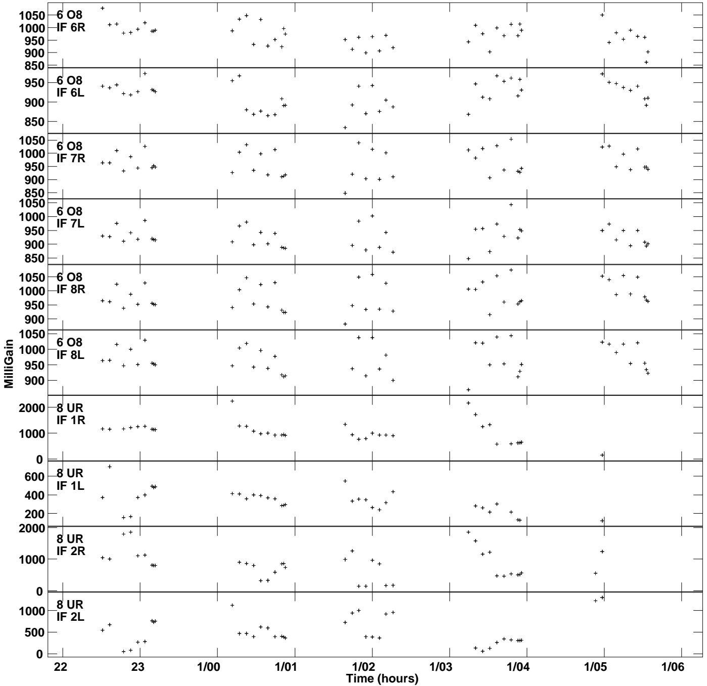
Plot file version 10 created 28-JUL-2021 18:08:07 Gain amp vs UTC time for J1329+3154.MULTI.1 SN 2 Rpol & Lpol IF 1 - 8
