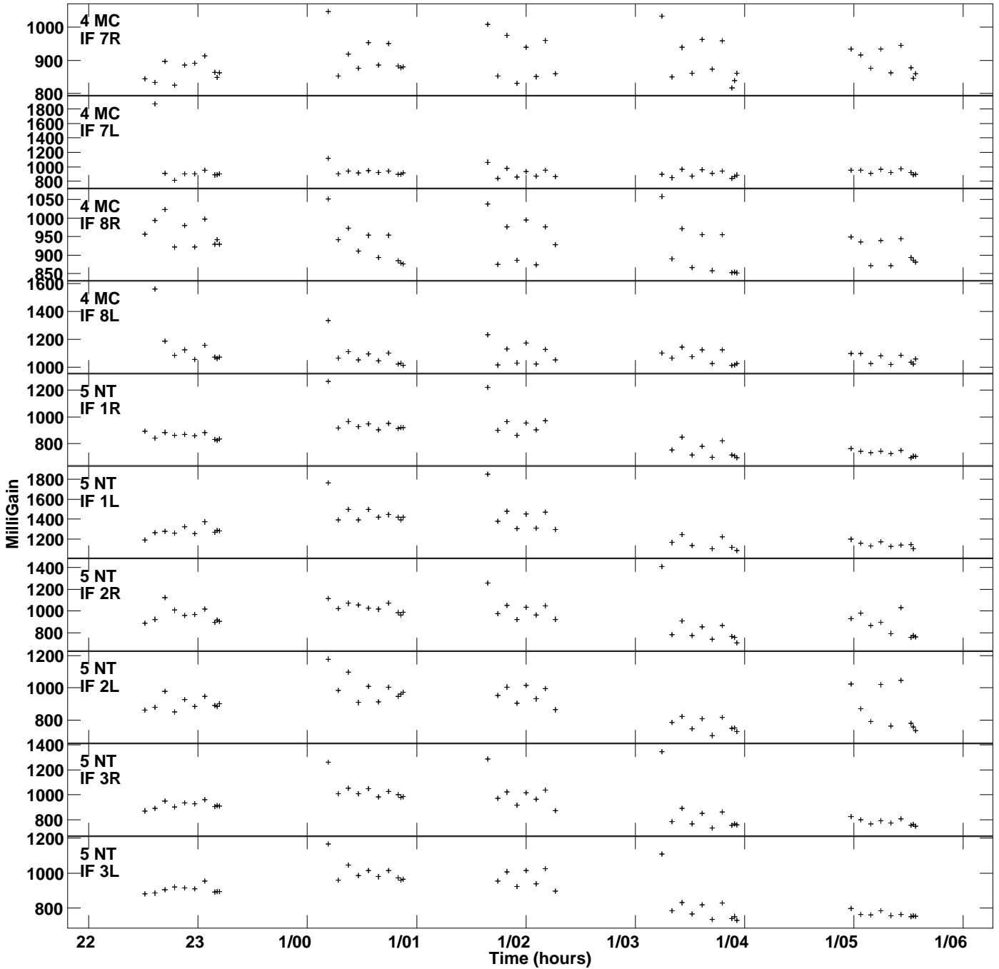
Plot file version 7 created 28-JUL-2021 18:08:06 Gain amp vs UTC time for J1329+3154.MULTI.1 SN 2 Rpol & Lpol IF 1 - 8
