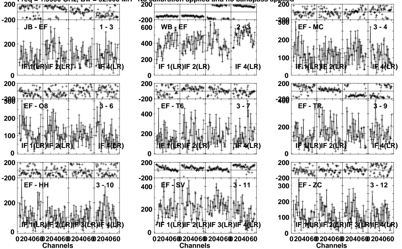
Lower frame: Micro Ampl Jy Top frame: Phas deg Vector averaged cross-power spectrum Several baselines displayed Timerange: 00/18:22:21 to 00/18:24:19
