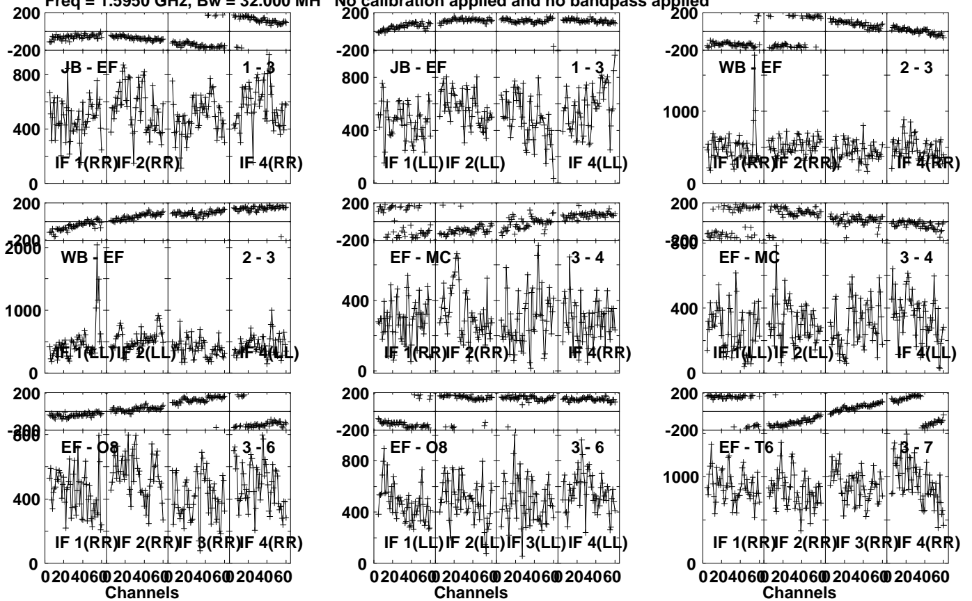
Lower frame: Micro Ampl Jy Top frame: Phas deg Vector averaged cross-power spectrum Several baselines displayed Timerange: 00/21:28:11 to 00/21:29:39
