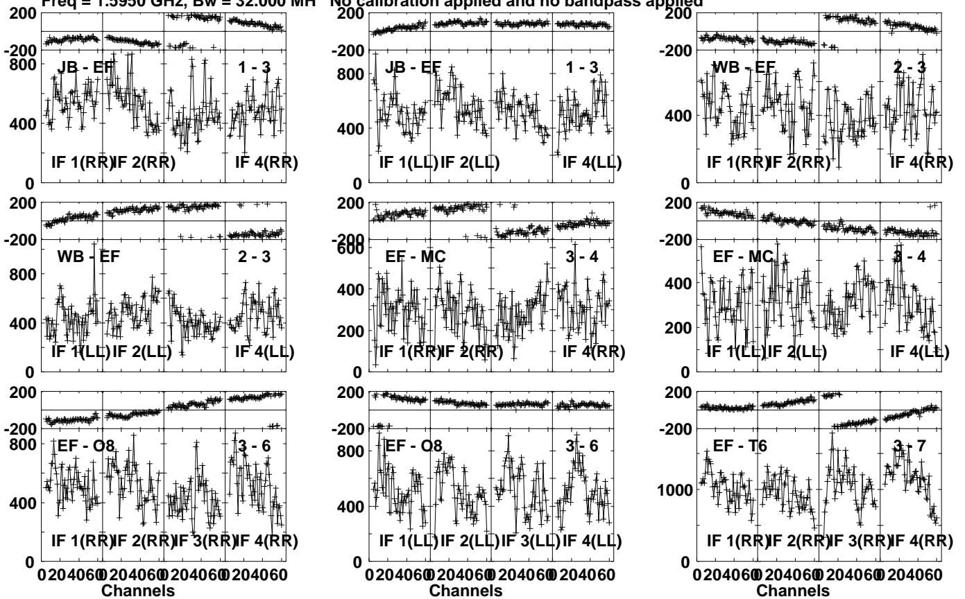
Lower frame: Micro Ampl Jy Top frame: Phas deg Vector averaged cross-power spectrum Several baselines displayed Timerange: 00/20:48:41 to 00/20:50:09
