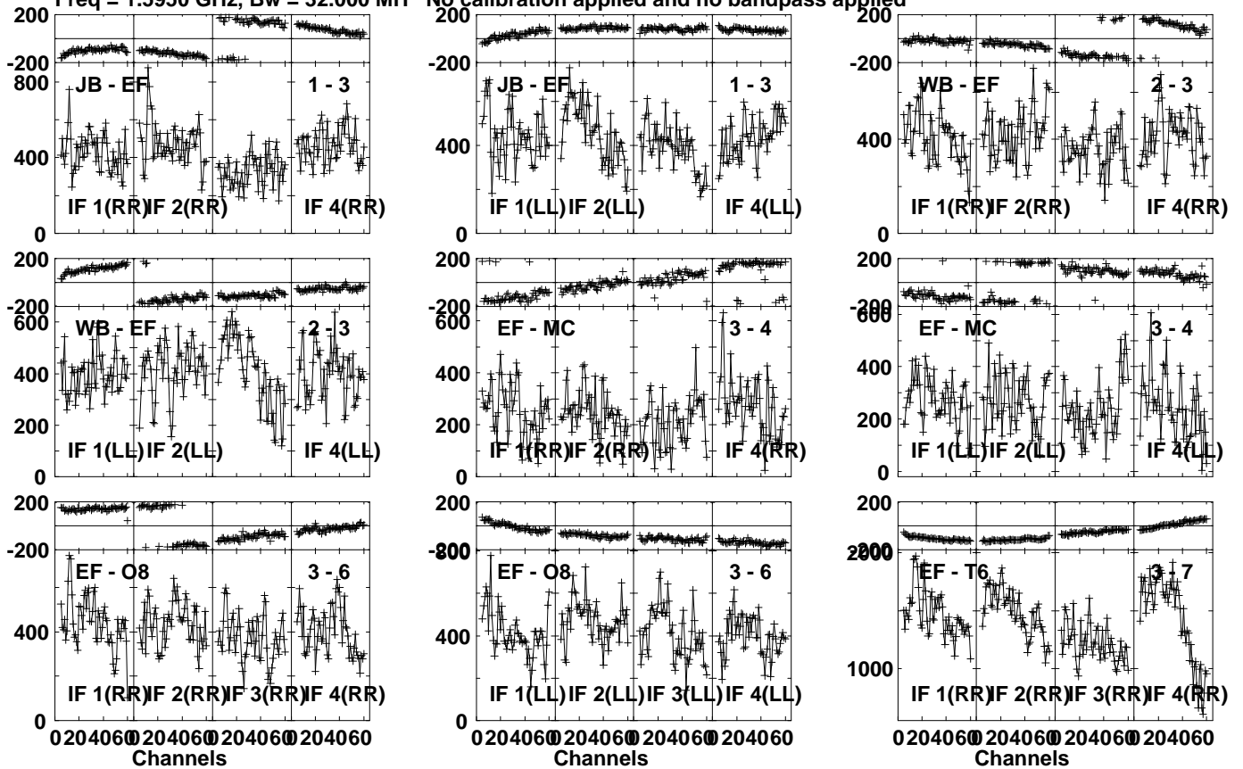
Lower frame: Micro Ampl Jy Top frame: Phas deg Vector averaged cross-power spectrum Several baselines displayed Timerange: 00/18:15:21 to 00/18:16:49
