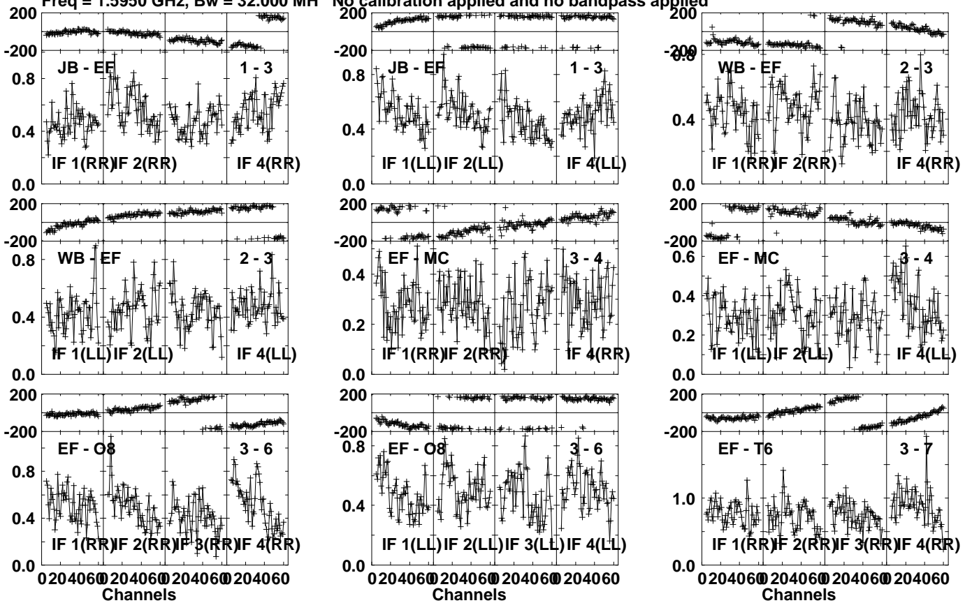
Lower frame: Milli Ampl Jy Top frame: Phas deg Vector averaged cross-power spectrum Several baselines displayed Timerange: 00/21:24:11 to 00/21:25:39
