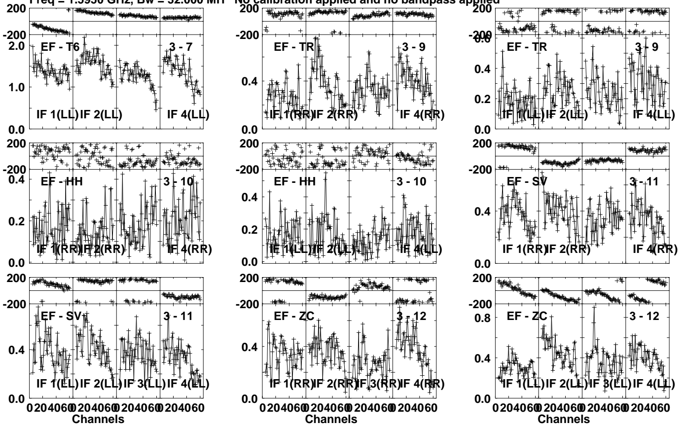
Lower frame: Milli Ampl Jy Top frame: Phas deg Vector averaged cross-power spectrum Several baselines displayed Timerange: 00/17:59:21 to 00/18:00:49
