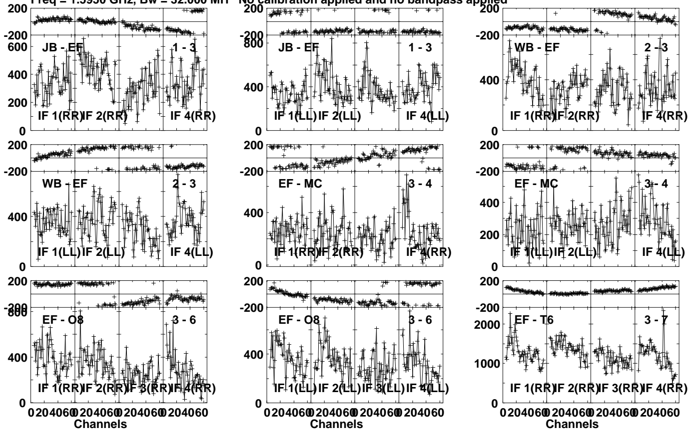
Lower frame: Micro Ampl Jy Top frame: Phas deg Vector averaged cross-power spectrum Several baselines displayed Timerange: 00/17:19:51 to 00/17:21:19
