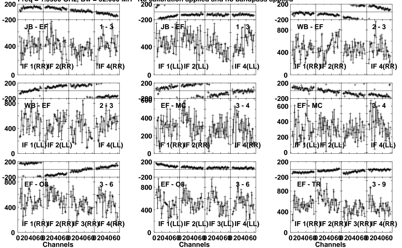
Lower frame: Micro Ampl Jy Top frame: Phas deg Vector averaged cross-power spectrum Several baselines displayed Timerange: 00/22:53:41 to 00/22:55:09
