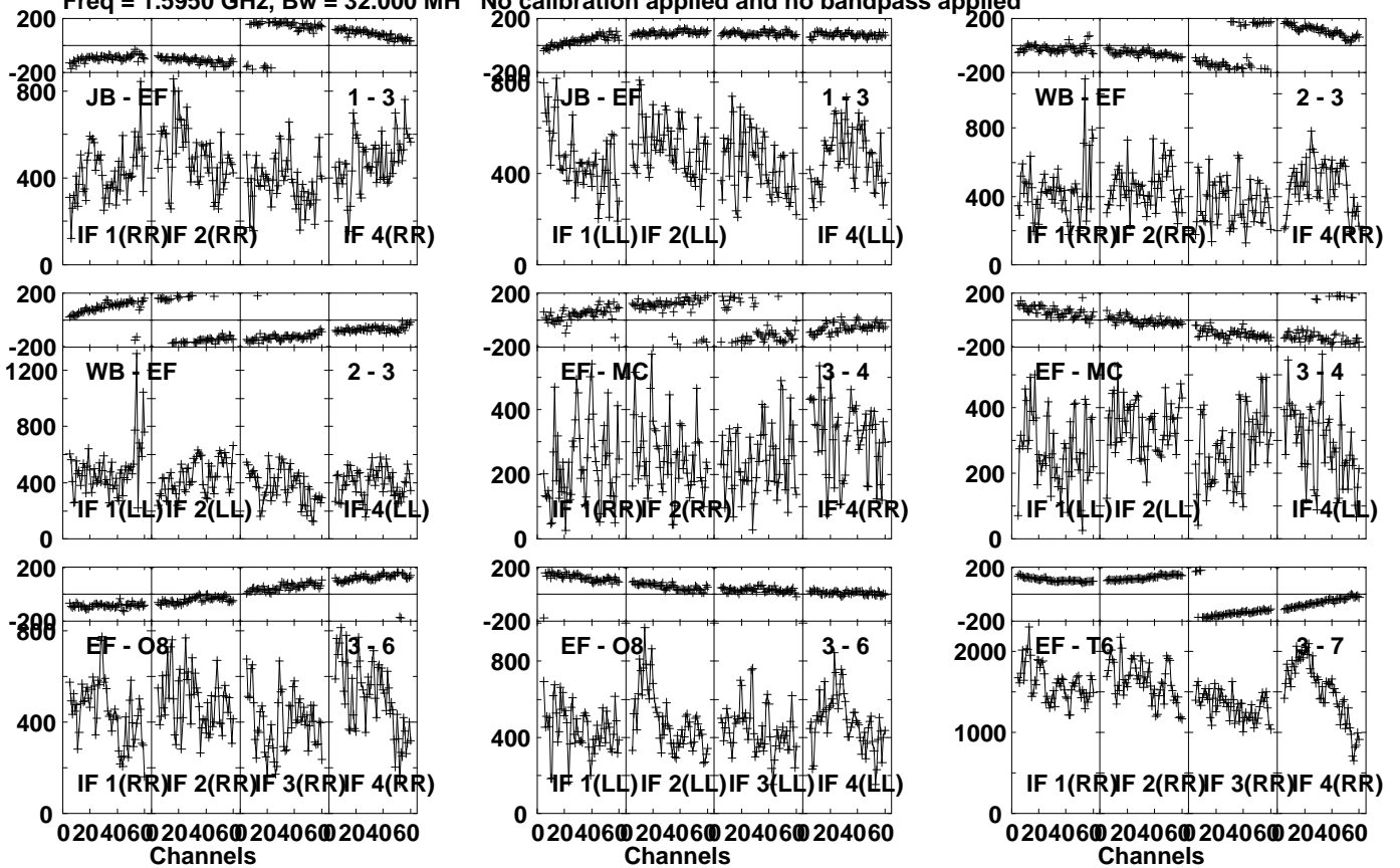
Lower frame: Micro Ampl Jy Top frame: Phas deg Vector averaged cross-power spectrum Several baselines displayed Timerange: 00/19:14:21 to 00/19:15:49
