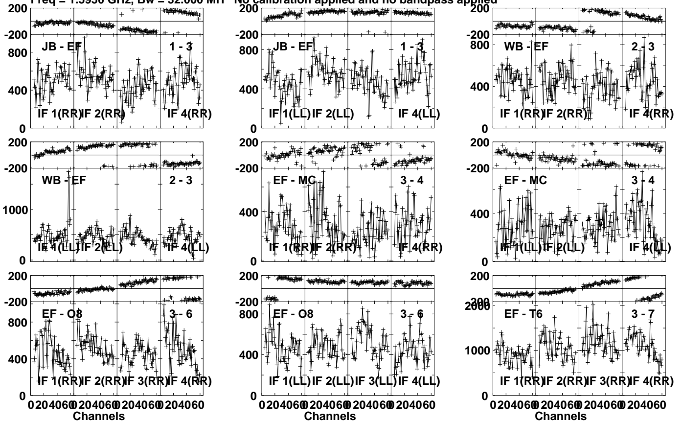
Lower frame: Micro Ampl Jy Top frame: Phas deg Vector averaged cross-power spectrum Several baselines displayed Timerange: 00:20:38:11 to 00:20:39:39
