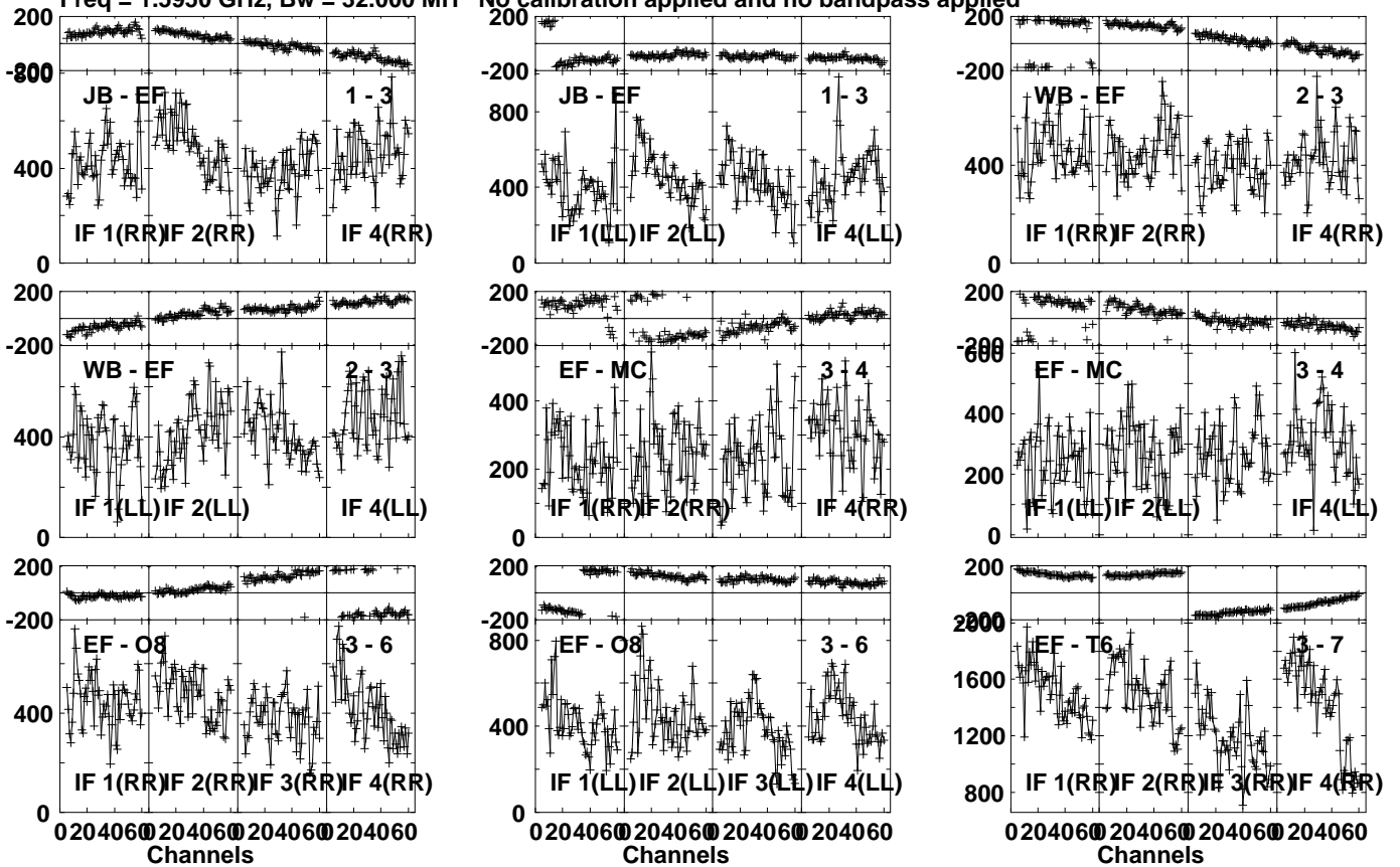
Lower frame: Micro Ampl Jy Top frame: Phas deg Vector averaged cross-power spectrum Several baselines displayed Timerange: 00:18:40:21 to 00:18:41:49
