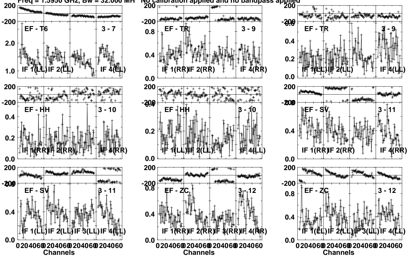
Lower frame: Milli Ampl Jy Top frame: Phas deg Vector averaged cross-power spectrum Several baselines displayed Timerange: 00:18:20:21 to 00:18:21:49
