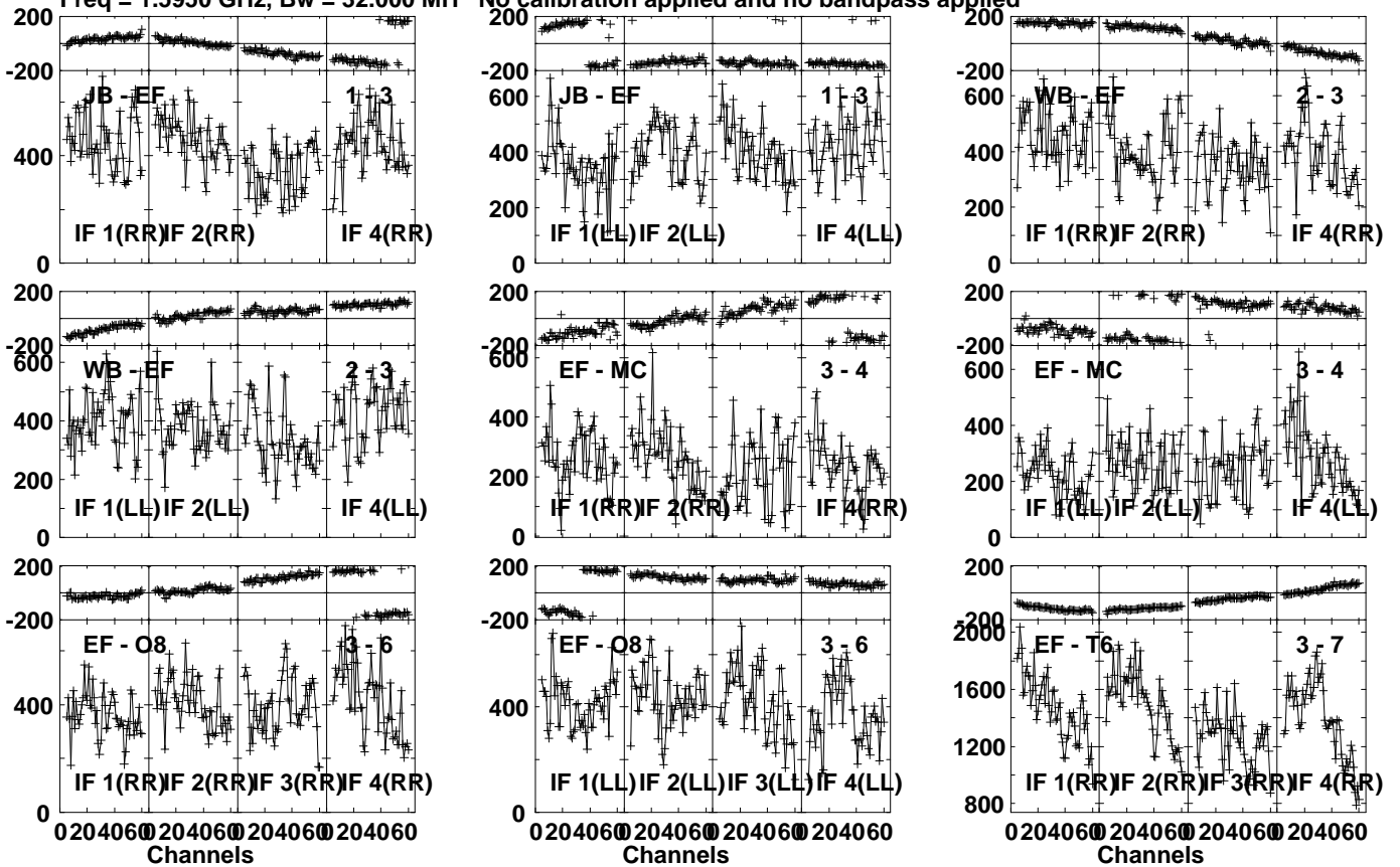
Lower frame: Micro Ampl Jy Top frame: Phas deg Vector averaged cross-power spectrum Several baselines displayed Timerange: 00:18:29:51 to 00:18:31:19
