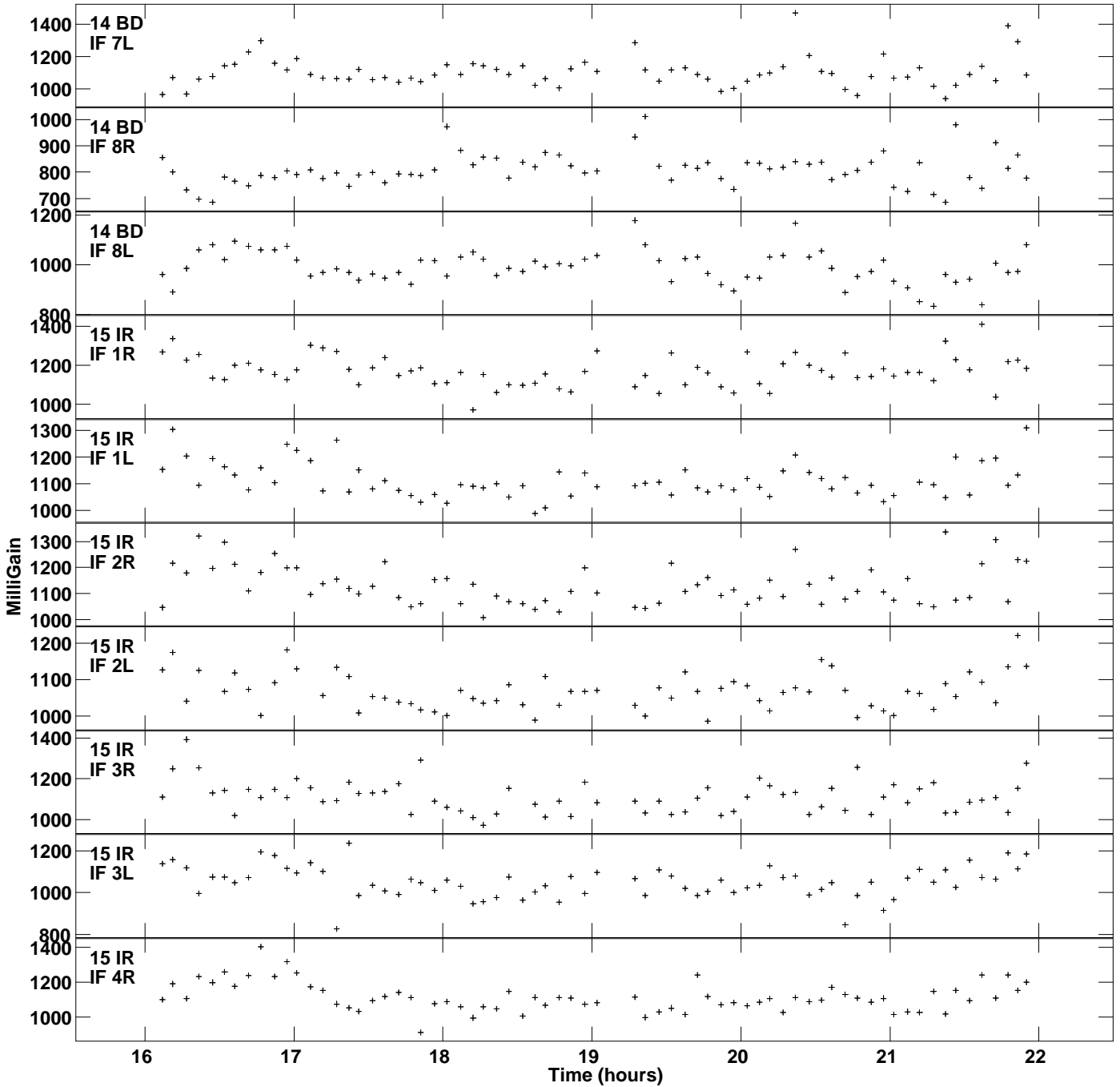
Plot file version 22 created 10-NOV-2021 21:01:56 Gain amp vs UTC time for J1547+2052.MULTI.1 SN 2 Rpol & Lpol IF 1 - 8
