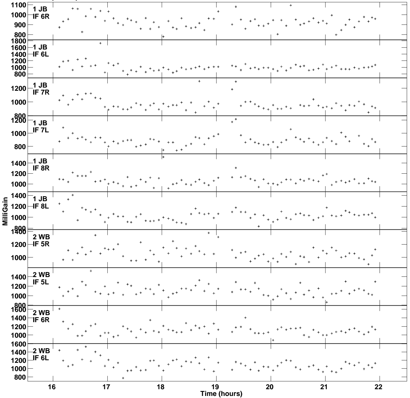
Plot file version 2 created 10-NOV-2021 21:01:56 Gain amp vs UTC time for J1547+2052.MULTI.1 SN 2 Rpol & Lpol IF 1 - 8
