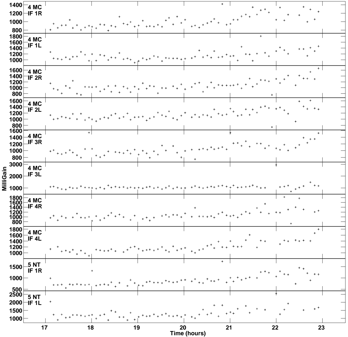
Plot file version 3 created 03-SEP-2021 14:45:48 Gain amp vs UTC time for J1553+5253.MULTI.1 SN 2 Rpol & Lpol IF 1 - 4
