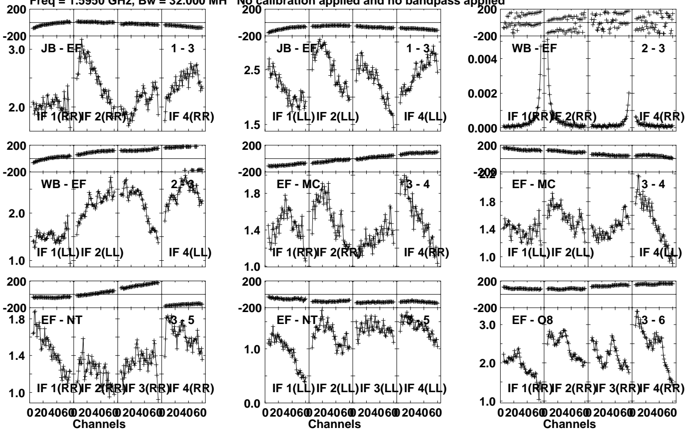
Lower frame: Milli Ampl Jy Top frame: Phas deg Vector averaged cross-power spectrum Several baselines displayed Timerange: 00/18:22:51 to 00/18:24:49
