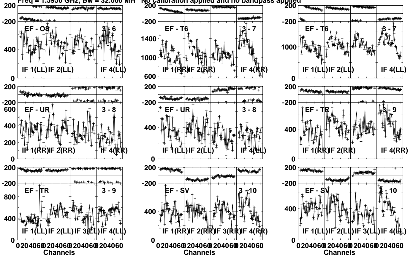
Lower frame: Micro Ampl Jy Top frame: Phas deg Vector averaged cross-power spectrum Several baselines displayed Timerange: 00/17:20:21 to 00/17:21:49
