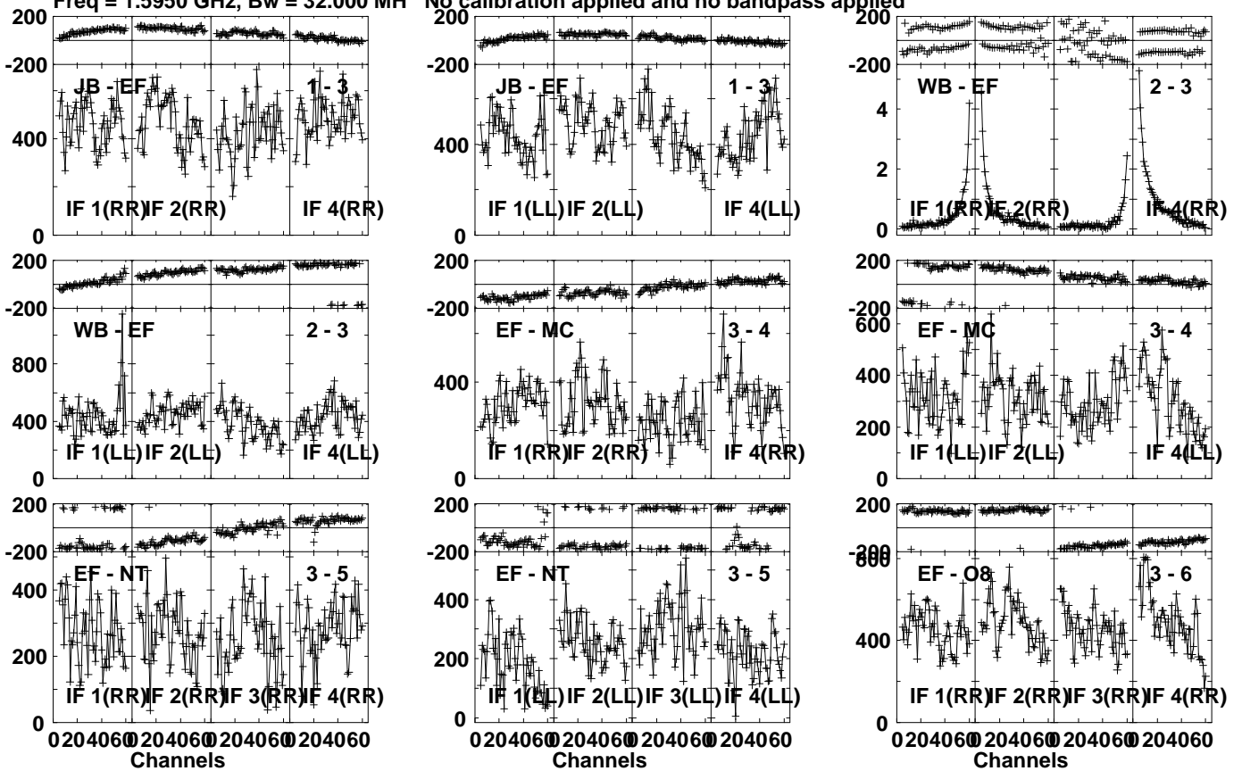
Lower frame: Micro Ampl Jy Top frame: Phas deg Vector averaged cross-power spectrum Several baselines displayed Timerange: 00/21:09:11 to 00/21:10:39
