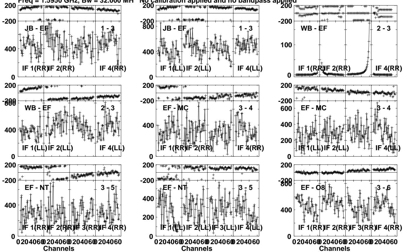
Lower frame: Micro Ampl Jy Top frame: Phas deg Vector averaged cross-power spectrum Several baselines displayed Timerange: 00/22:04:11 to 00/22:05:39
