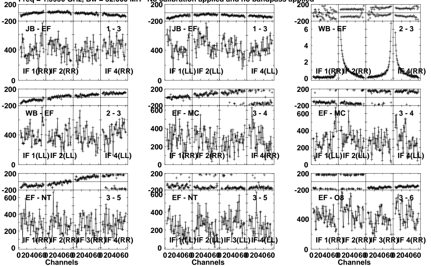
Lower frame: Micro Ampl Jy Top frame: Phas deg Vector averaged cross-power spectrum Several baselines displayed Timerange: 00/17:30:51 to 00/17:32:19
