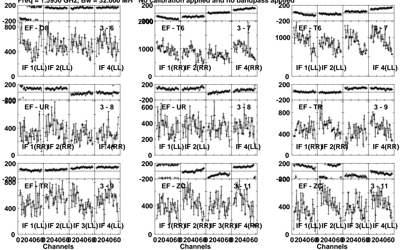
Lower frame: Micro Ampl Jy Top frame: Phas deg Vector averaged cross-power spectrum Several baselines displayed Timerange: 00/20:49:11 to 00/20:50:39
