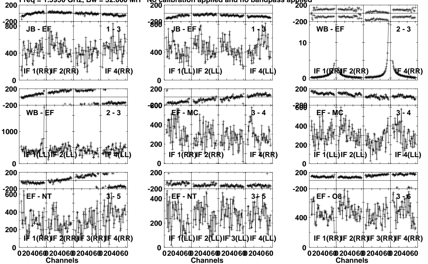
Lower frame: Micro Ampl Jy Top frame: Phas deg Vector averaged cross-power spectrum Several baselines displayed Timerange: 00/18:20:51 to 00/18:22:19
