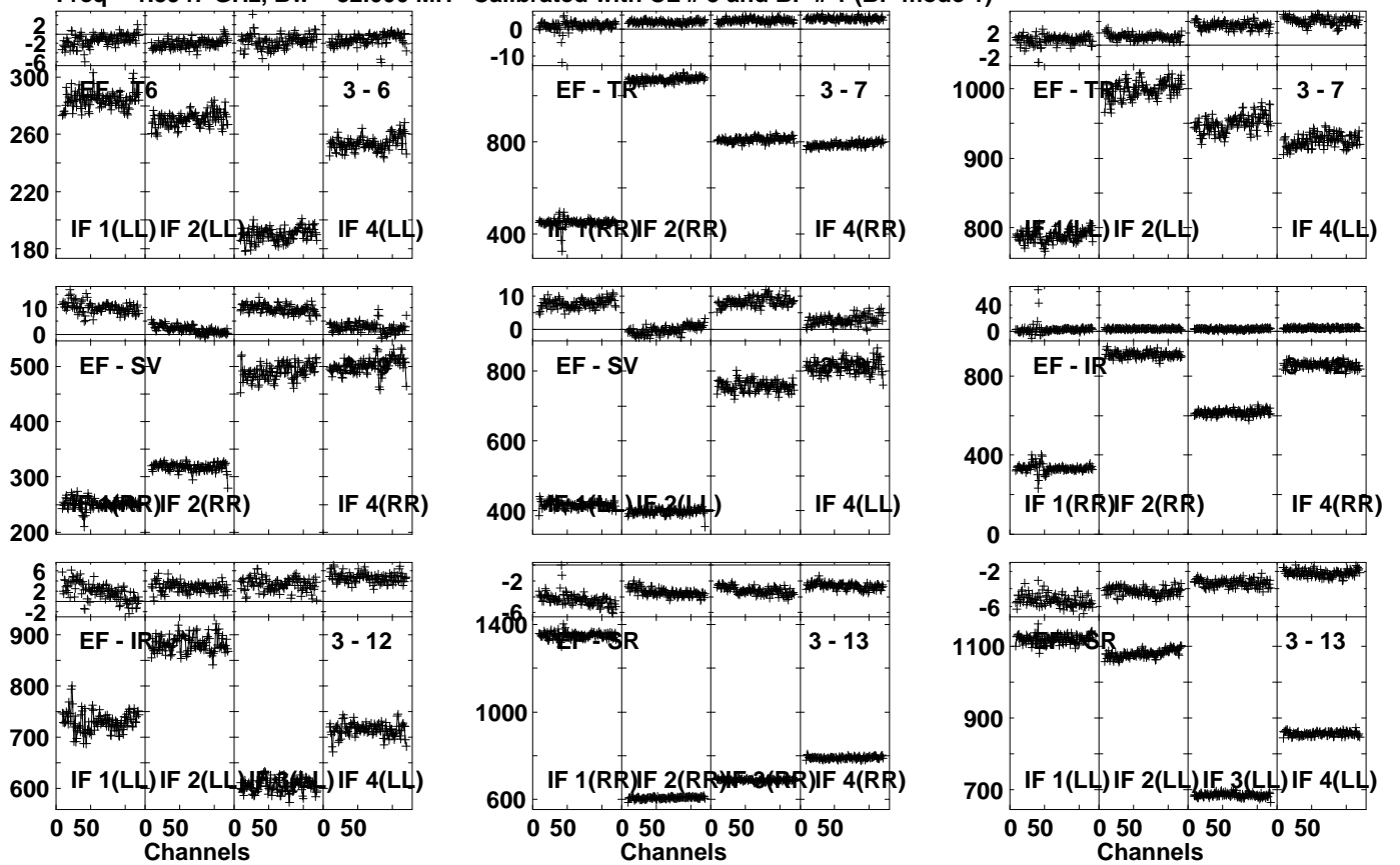
Lower frame: Milli Ampl Jy Top frame: Phas deg Vector averaged cross-power spectrum Several baselines displayed Timerange: 00/21:33:31 to 00/21:34:59
