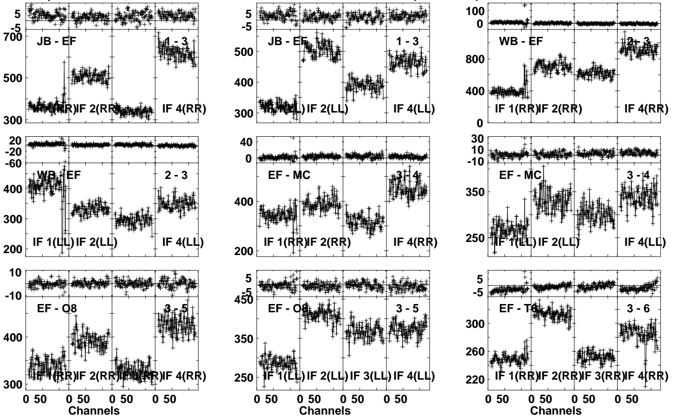
Lower frame: Milli Ampl Jy Top frame: Phas deg Vector averaged cross-power spectrum Several baselines displayed Timerange: 00/14:30:01 to 00/14:31:29
