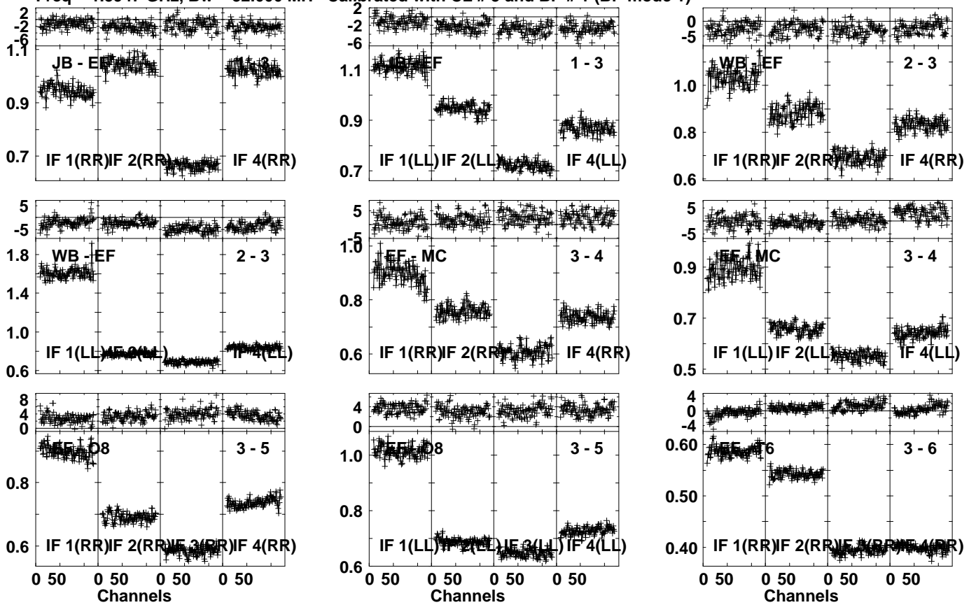
Lower frame: Ampl Jy Top frame: Phas deg Vector averaged cross-power spectrum Several baselines displayed Timerange: 01/00:08:01 to 01/00:09:29
