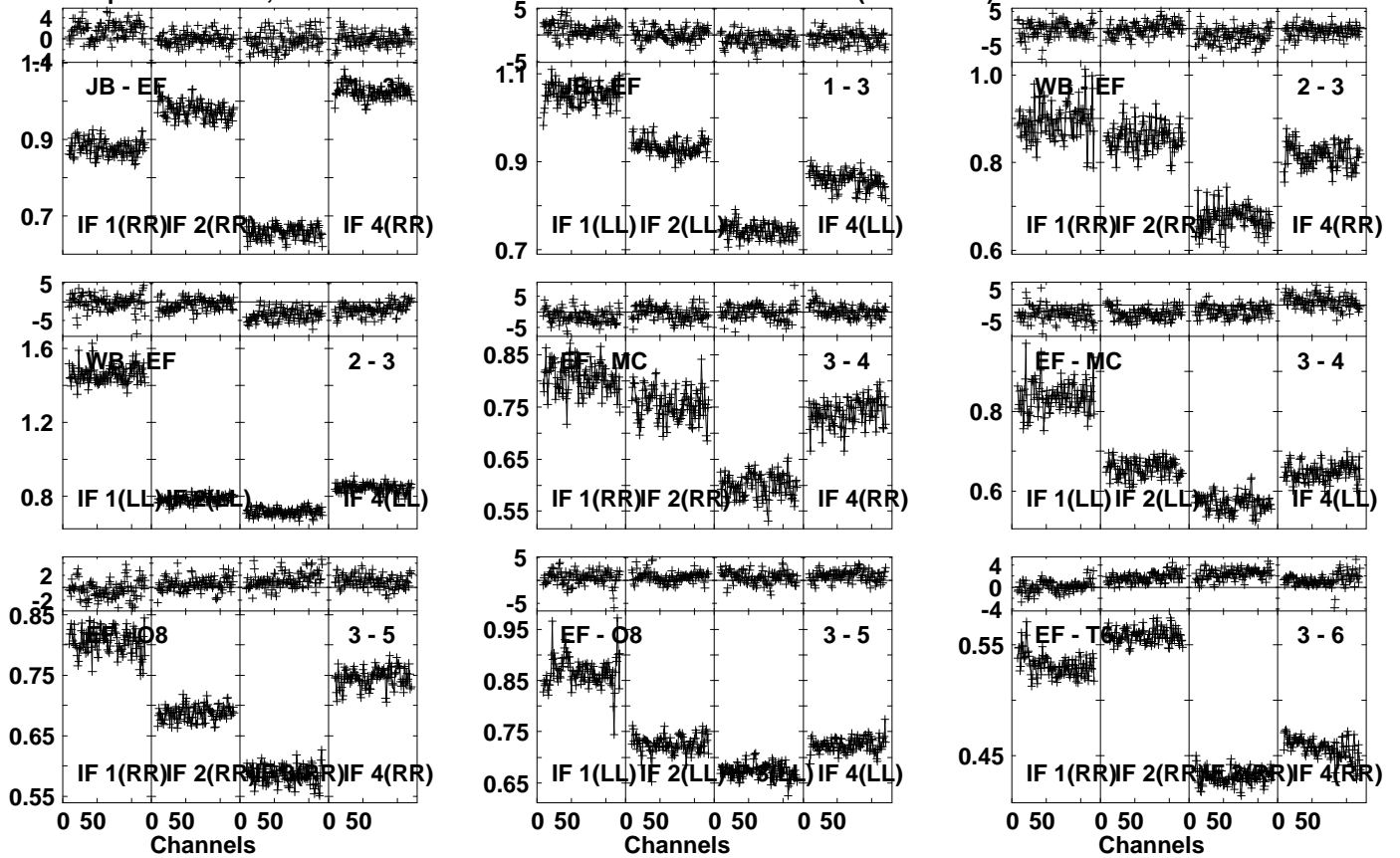
Lower frame: Ampl Jy Top frame: Phas deg Vector averaged cross-power spectrum Several baselines displayed Timerange: 01/00:03:31 to 01/00:04:29
