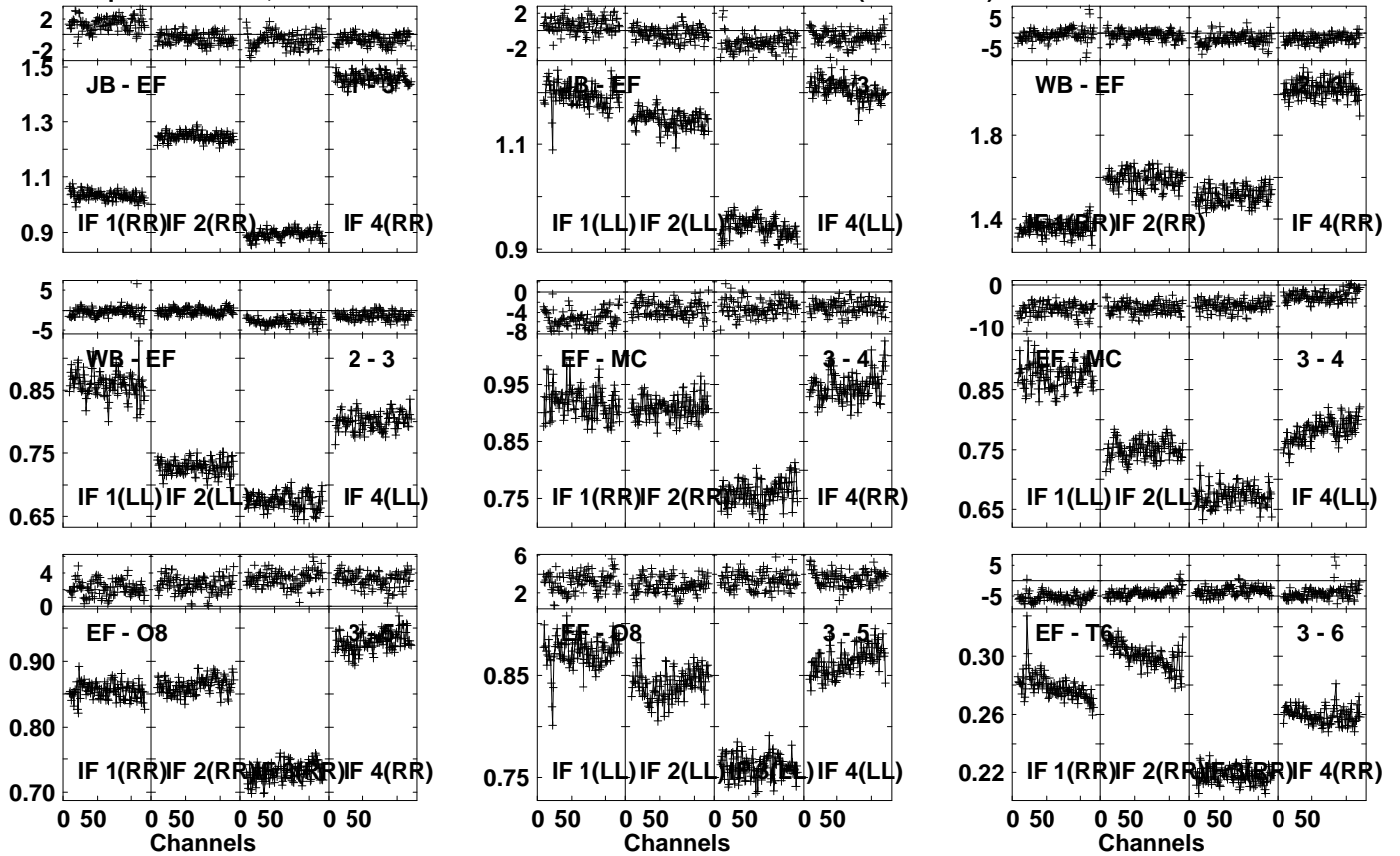
Lower frame: Ampl Jy Top frame: Phas deg Vector averaged cross-power spectrum Several baselines displayed Timerange: 00/22:34:01 to 00/22:34:59
