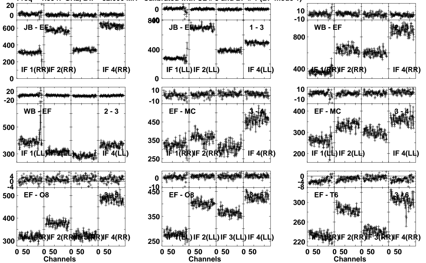
Lower frame: Milli Ampl Jy Top frame: Phas deg Vector averaged cross-power spectrum Several baselines displayed Timerange: 00/14:35:01 to 00/14:36:29
