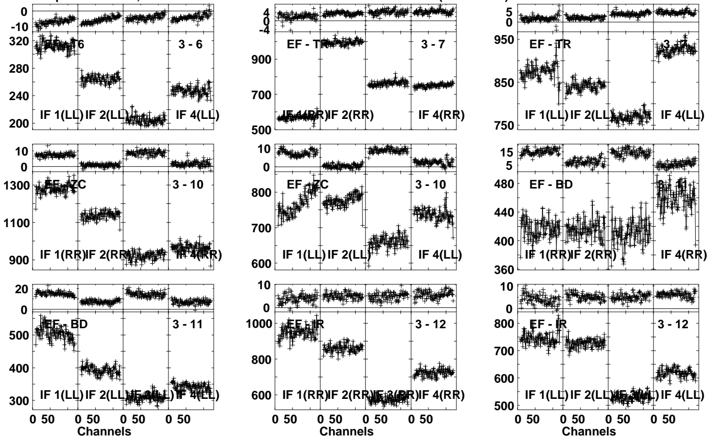
Lower frame: Milli Ampl Jy Top frame: Phas deg Vector averaged cross-power spectrum Several baselines displayed Timerange: 00/23:04:01 to 00/23:04:59
