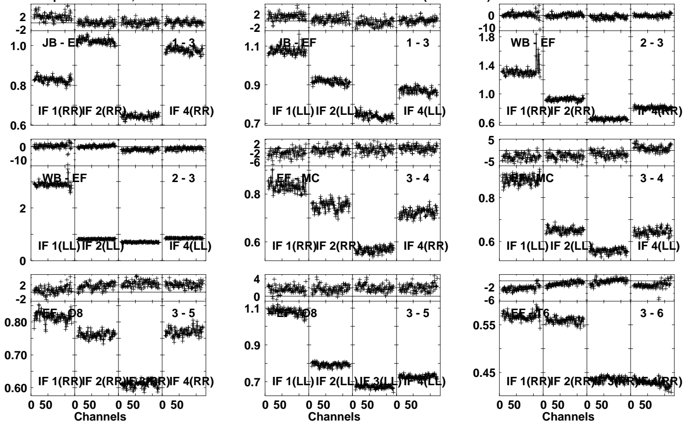
Lower frame: Ampl Jy Top frame: Phas deg Vector averaged cross-power spectrum Several baselines displayed Timerange: 00/23:33:01 to 00/23:34:29
