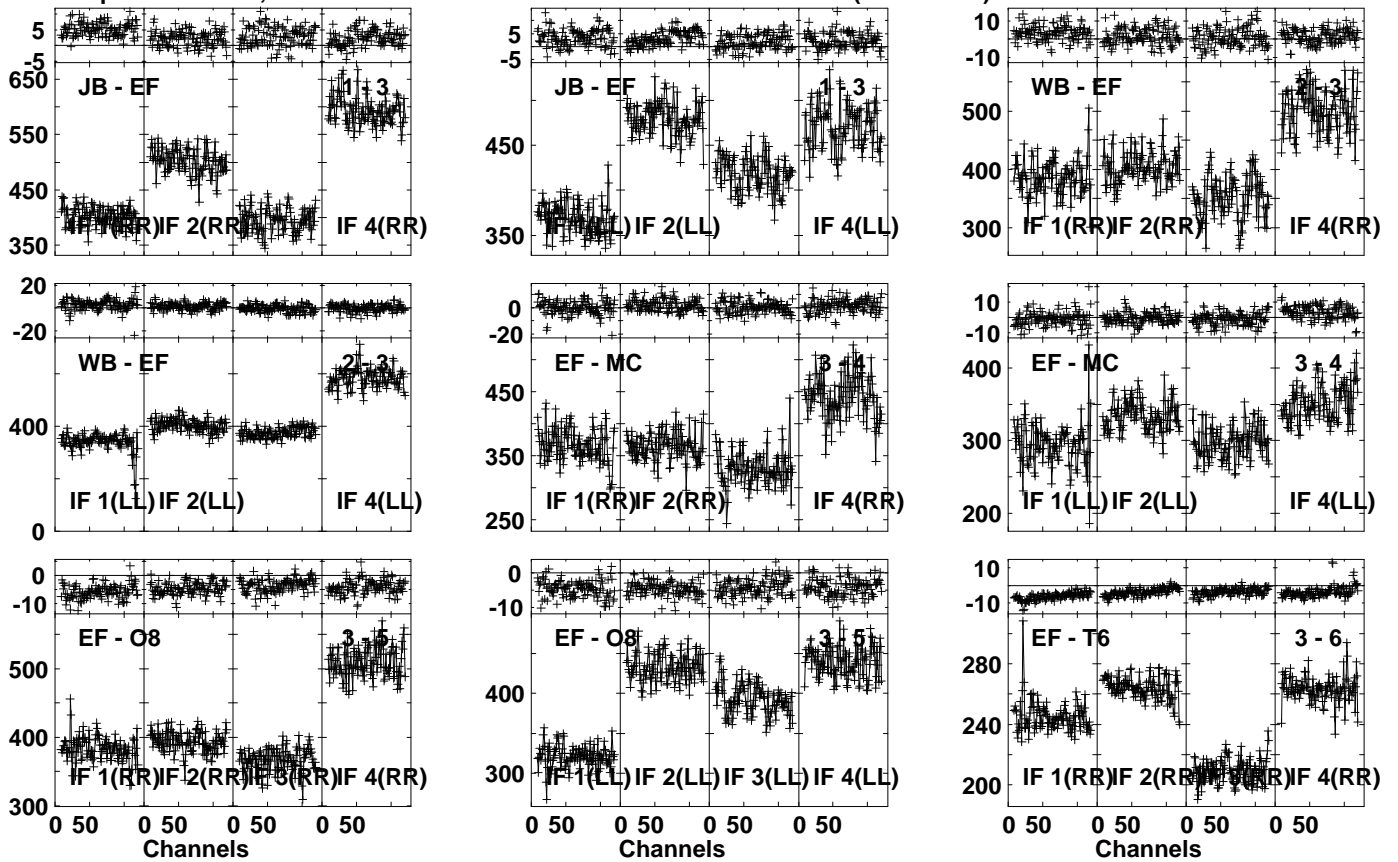
Lower frame: Milli Ampl Jy Top frame: Phas deg Vector averaged cross-power spectrum Several baselines displayed Timerange: 00/16:10:31 to 00/16:11:29
