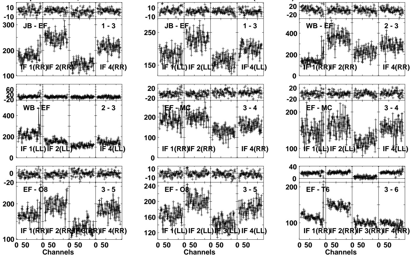
Lower frame: Milli Ampl Jy Top frame: Phas deg Vector averaged cross-power spectrum Several baselines displayed Timerange: 01/11:13:32 to 01/11:14:58
