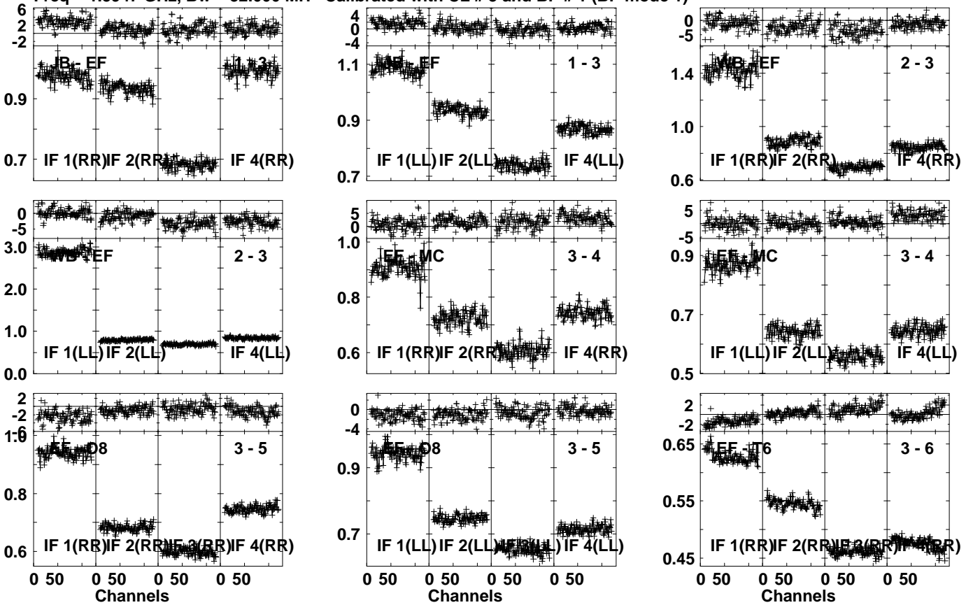
Lower frame: Ampl Jy Top frame: Phas deg Vector averaged cross-power spectrum Several baselines displayed Timerange: 00/23:38:01 to 00/23:39:29
