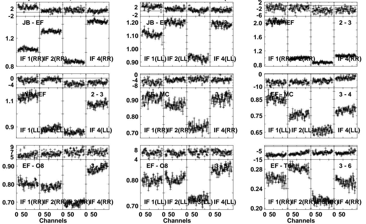
Lower frame: Ampl Jy Top frame: Phas deg Vector averaged cross-power spectrum Several baselines displayed Timerange: 00:22:48:31 to 00:22:49:59
