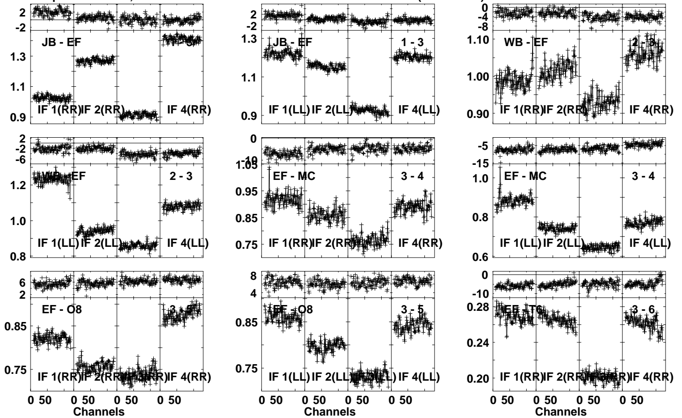
Lower frame: Ampl Jy Top frame: Phas deg Vector averaged cross-power spectrum Several baselines displayed Timerange: 00/22:28:31 to 00/22:29:59
