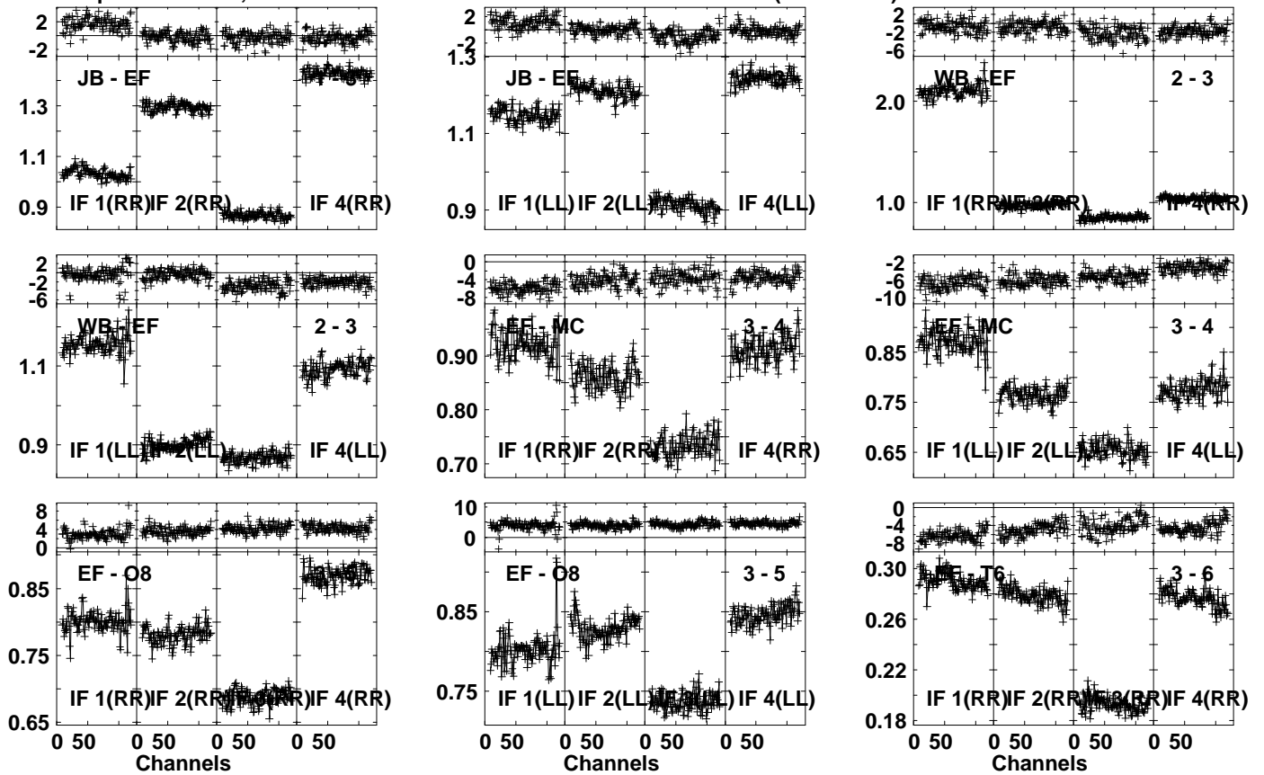
Lower frame: Ampl Jy Top frame: Phas deg Vector averaged cross-power spectrum Several baselines displayed Timerange: 00/22:44:01 to 00/22:44:59
