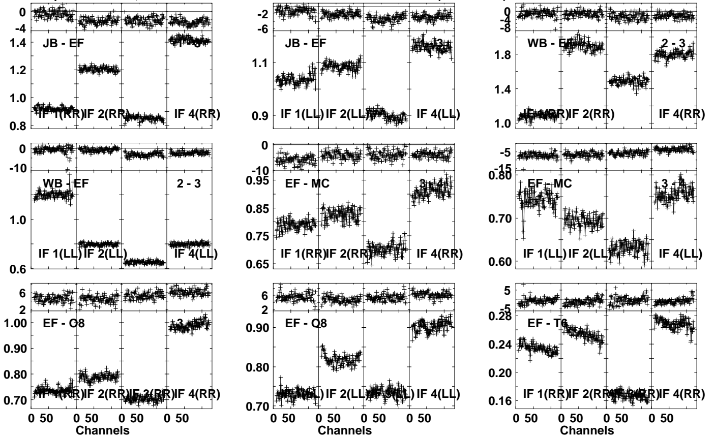
Lower frame: Ampl Jy Top frame: Phas deg Vector averaged cross-power spectrum Several baselines displayed Timerange: 00/21:58:31 to 00/21:59:59
