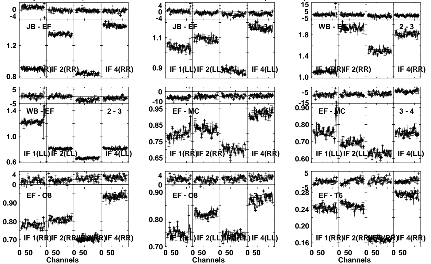
Lower frame: Ampl Jy Top frame: Phas deg Vector averaged cross-power spectrum Several baselines displayed Timerange: 00/21:54:01 to 00/21:54:59
