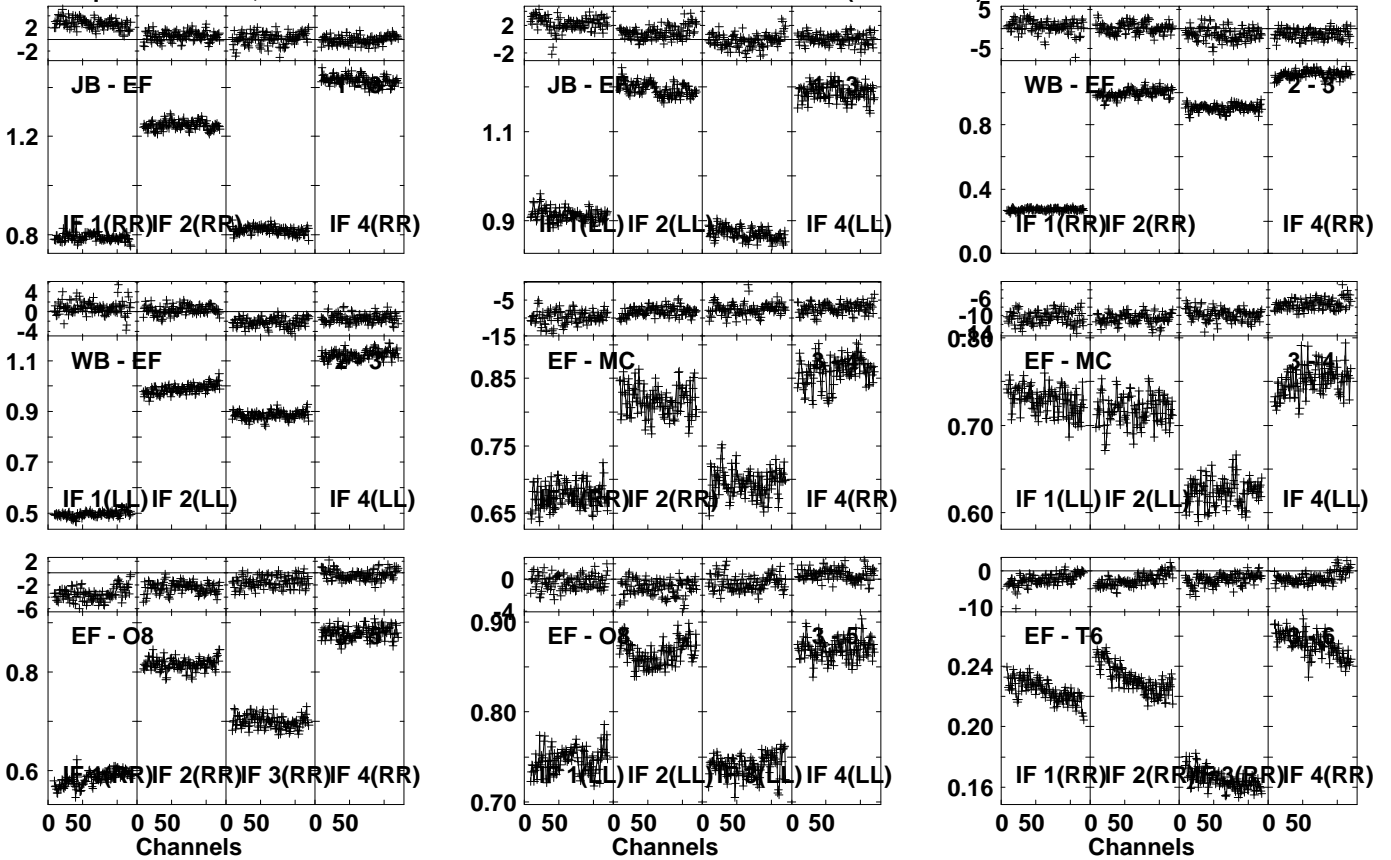
Lower frame: Ampl Jy Top frame: Phas deg Vector averaged cross-power spectrum Several baselines displayed Timerange: 00/21:38:31 to 00/21:39:59
