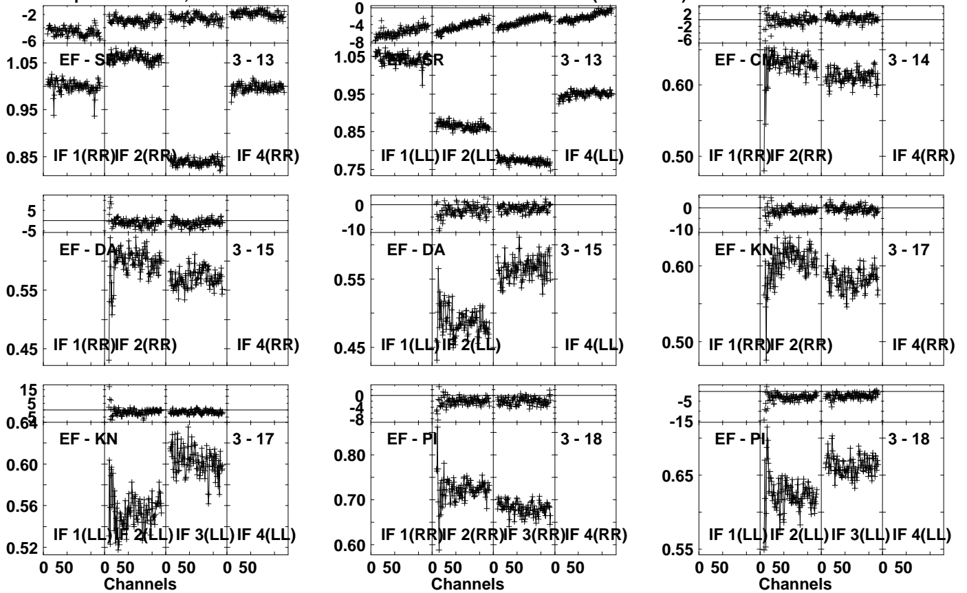
Lower frame: Ampl Jy Top frame: Phas deg Vector averaged cross-power spectrum Several baselines displayed Timerange: 01/00:58:01 to 01/00:59:29
