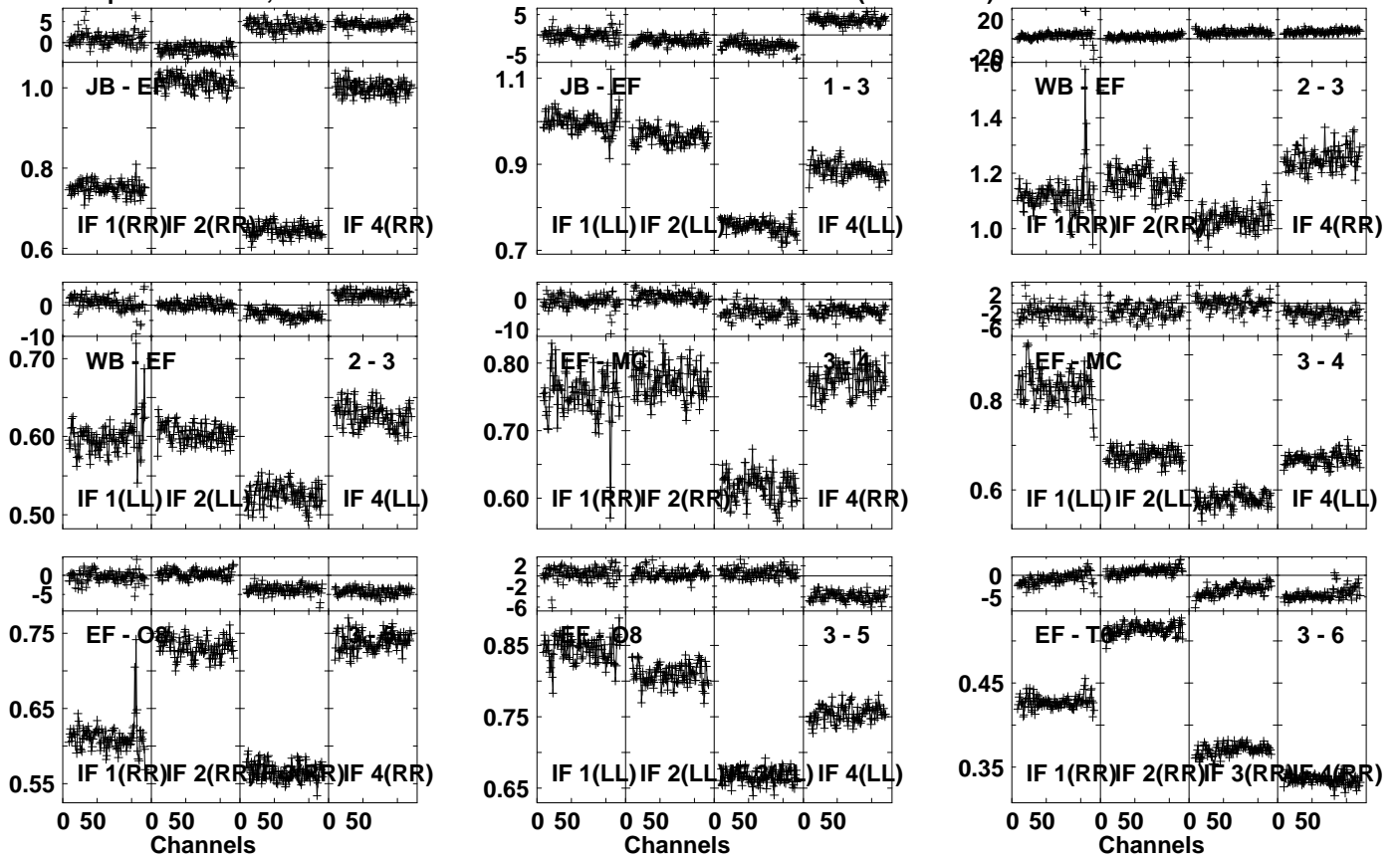
Lower frame: Ampl Jy Top frame: Phas deg Vector averaged cross-power spectrum Several baselines displayed Timerange: 01/01:18:01 to 01/01:19:29
