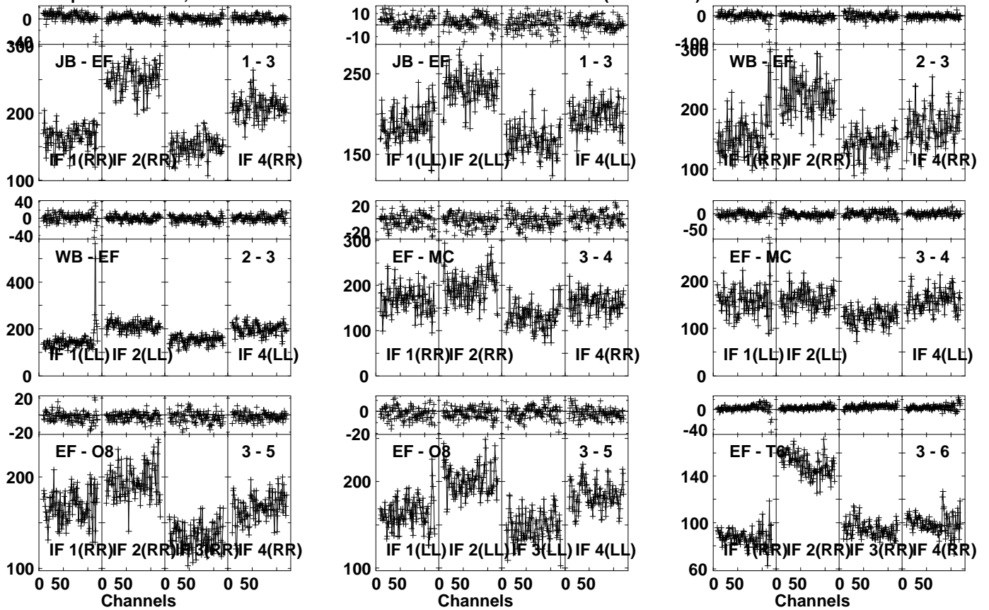
Lower frame: Milli Ampl Jy Top frame: Phas deg Vector averaged cross-power spectrum Several baselines displayed Timerange: 01/11:23:32 to 01/11:24:58
