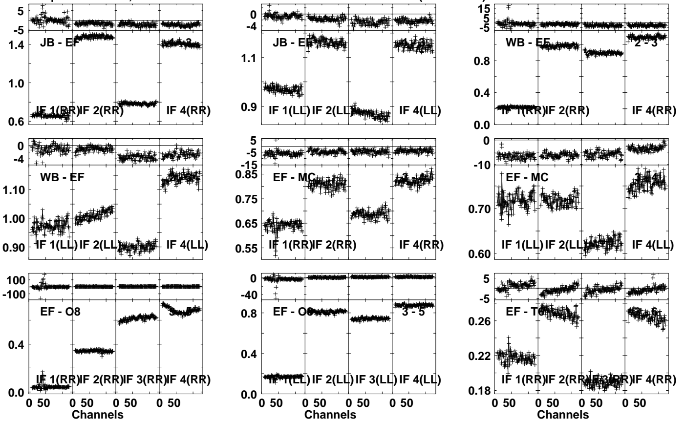
Lower frame: Ampl Jy Top frame: Phas deg Vector averaged cross-power spectrum Several baselines displayed Timerange: 00/21:33:31 to 00/21:34:59
