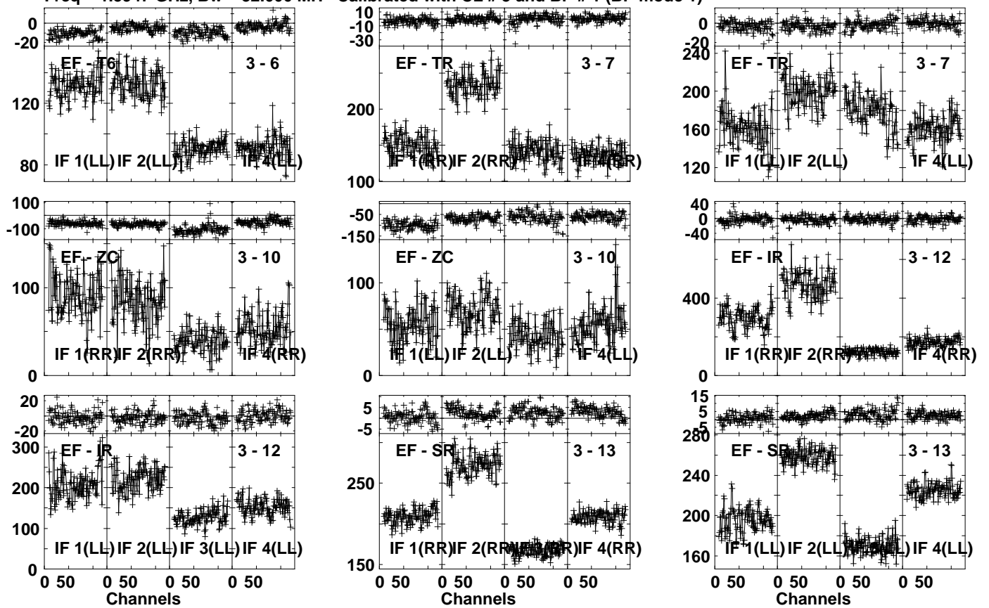
Lower frame: Milli Ampl Jy Top frame: Phas deg Vector averaged cross-power spectrum Several baselines displayed Timerange: 01/11:19:02 to 01/11:19:58
