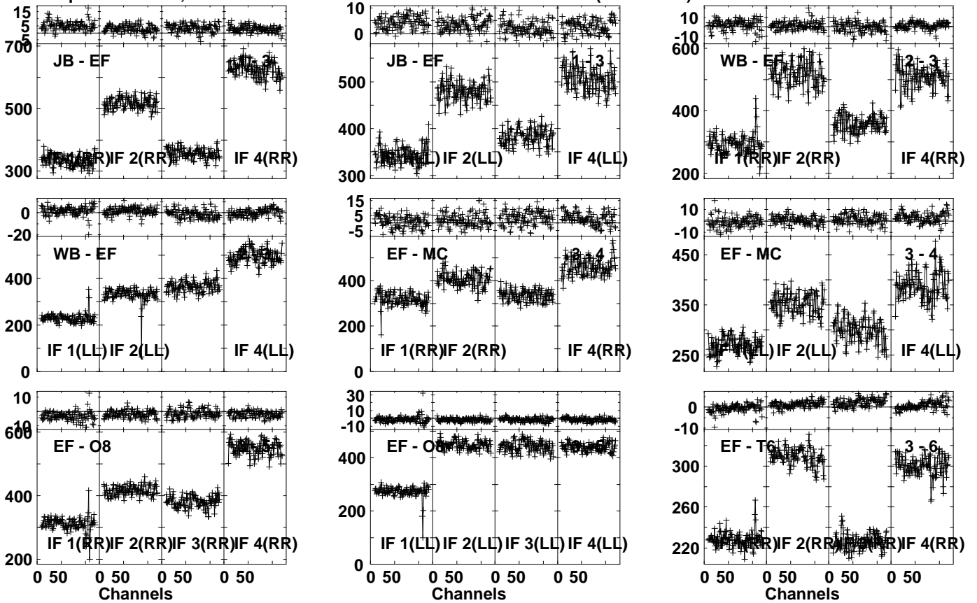
Lower frame: Milli Ampl Jy Top frame: Phas deg Vector averaged cross-power spectrum Several baselines displayed Timerange: 00/15:40:31 to 00/15:41:29
