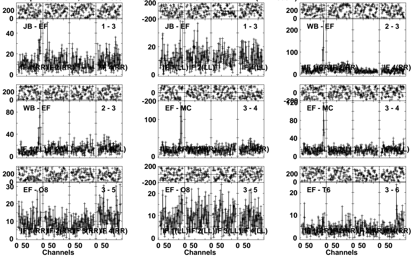
Lower frame: Milli Ampl Jy Top frame: Phas deg Vector averaged cross-power spectrum Several baselines displayed Timerange: 00/14:56:31 to 00/14:59:59
