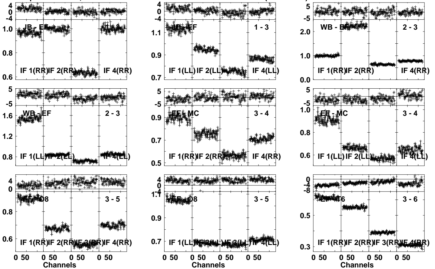
Lower frame: Ampl Jy Top frame: Phas deg Vector averaged cross-power spectrum Several baselines displayed Timerange: 00/23:58:01 to 00/23:59:29
