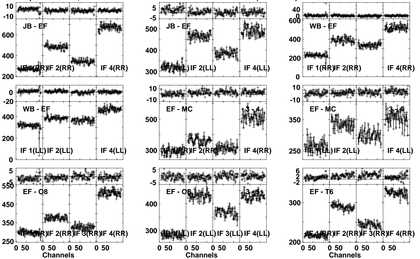
Lower frame: Milli Ampl Jy Top frame: Phas deg Vector averaged cross-power spectrum Several baselines displayed Timerange: 00/14:45:01 to 00/14:46:29
