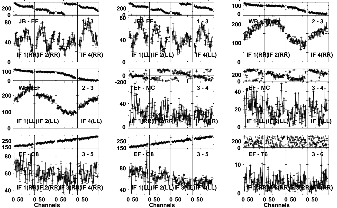
Lower frame: Milli Ampl Jy Top frame: Phas deg Vector averaged cross-power spectrum Several baselines displayed Timerange: 00/22:25:01 to 00/22:28:29
