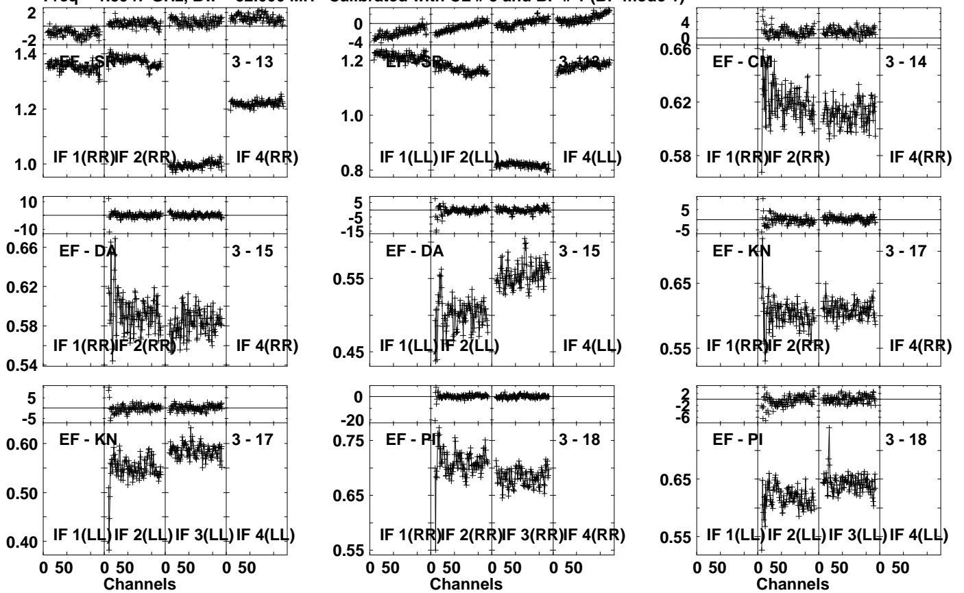
Lower frame: Ampl Jy Top frame: Phas deg Vector averaged cross-power spectrum Several baselines displayed Timerange: 01/01:03:31 to 01/01:04:29
