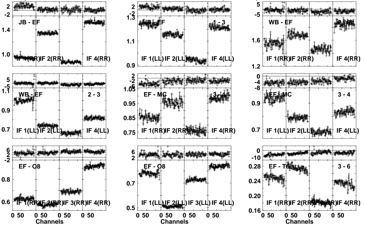
Lower frame: Ampl Jy Top frame: Phas deg Vector averaged cross-power spectrum Several baselines displayed Timerange: 00/23:14:01 to 00/23:14:59
