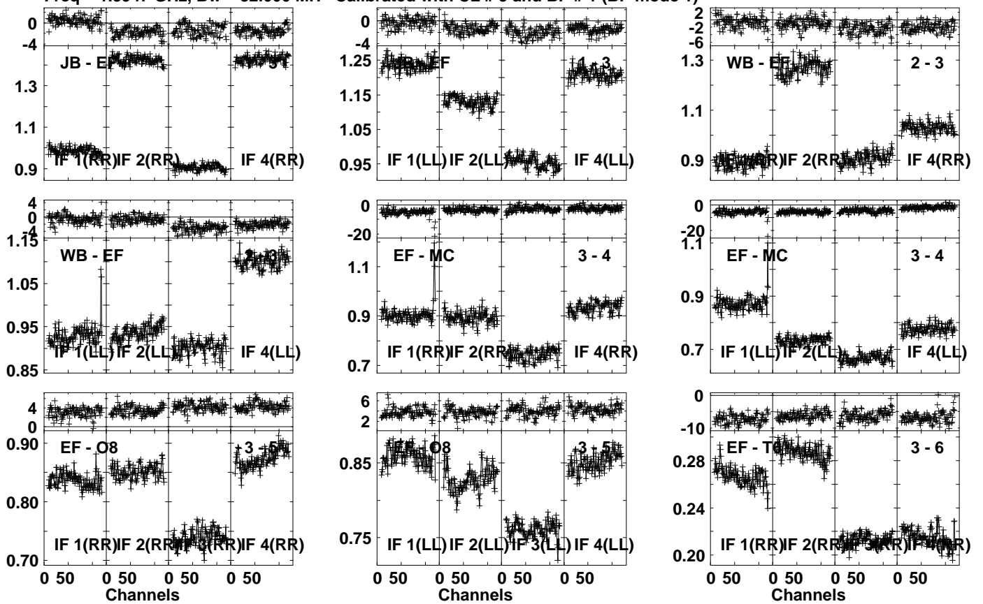
Lower frame: Ampl Jy Top frame: Phas deg Vector averaged cross-power spectrum Several baselines displayed Timerange: 00/22:14:01 to 00/22:14:59
