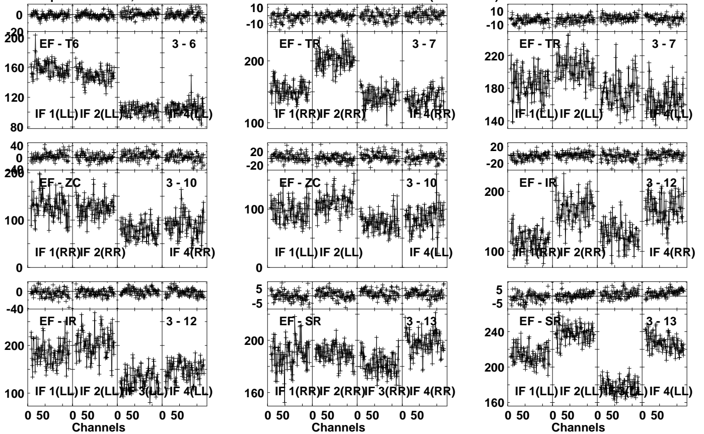
Lower frame: Milli Ampl Jy Top frame: Phas deg Vector averaged cross-power spectrum Several baselines displayed Timerange: 01/11:29:02 to 01/11:29:58
