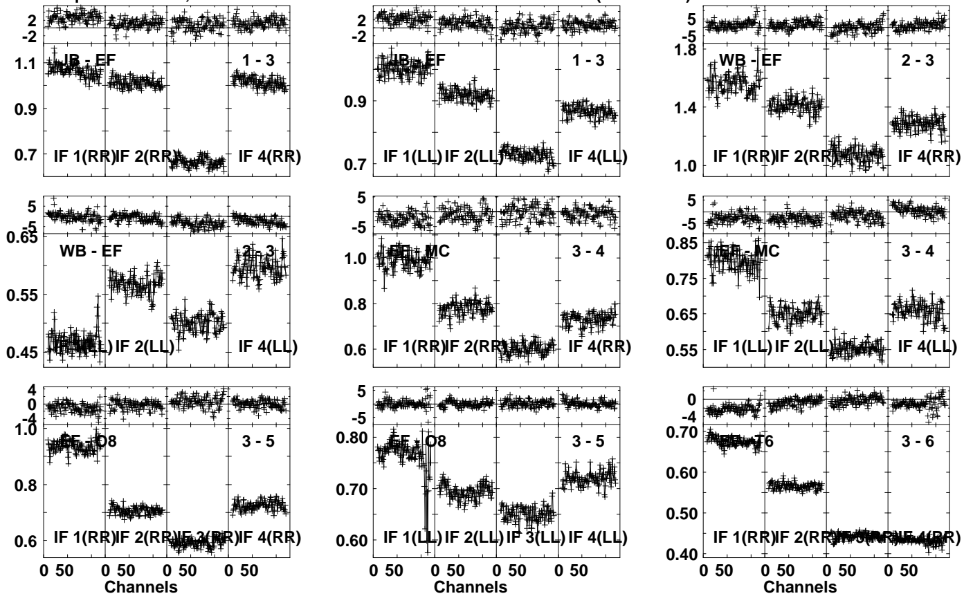
Lower frame: Ampl Jy Top frame: Phas deg Vector averaged cross-power spectrum Several baselines displayed Timerange: 01/00:23:31 to 01/00:24:29
