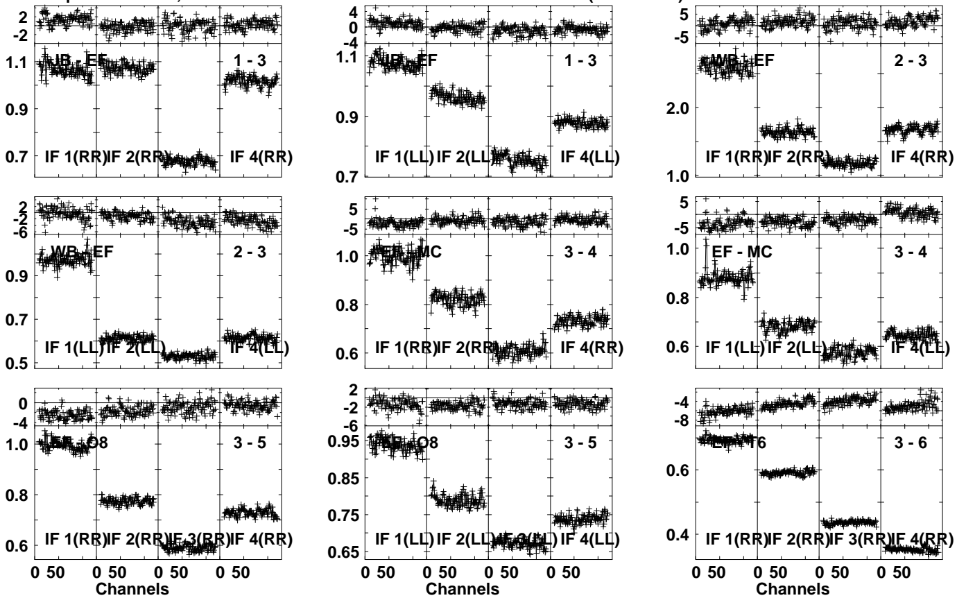
Lower frame: Ampl Jy Top frame: Phas deg Vector averaged cross-power spectrum Several baselines displayed Timerange: 01/00:48:01 to 01/00:49:29
