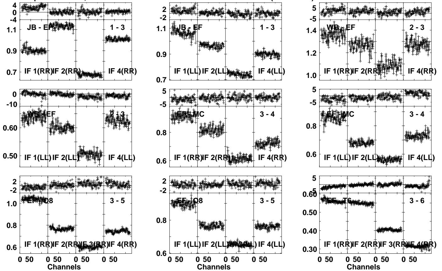
Lower frame: Ampl Jy Top frame: Phas deg Vector averaged cross-power spectrum Several baselines displayed Timerange: 01/01:13:31 to 01/01:14:29
