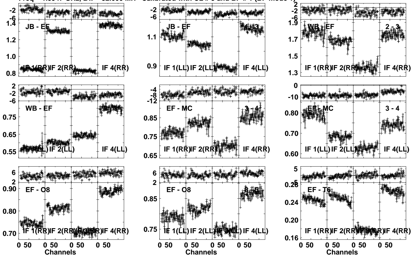
Lower frame: Ampl Jy Top frame: Phas deg Vector averaged cross-power spectrum Several baselines displayed Timerange: 00/21:48:31 to 00/21:49:59
