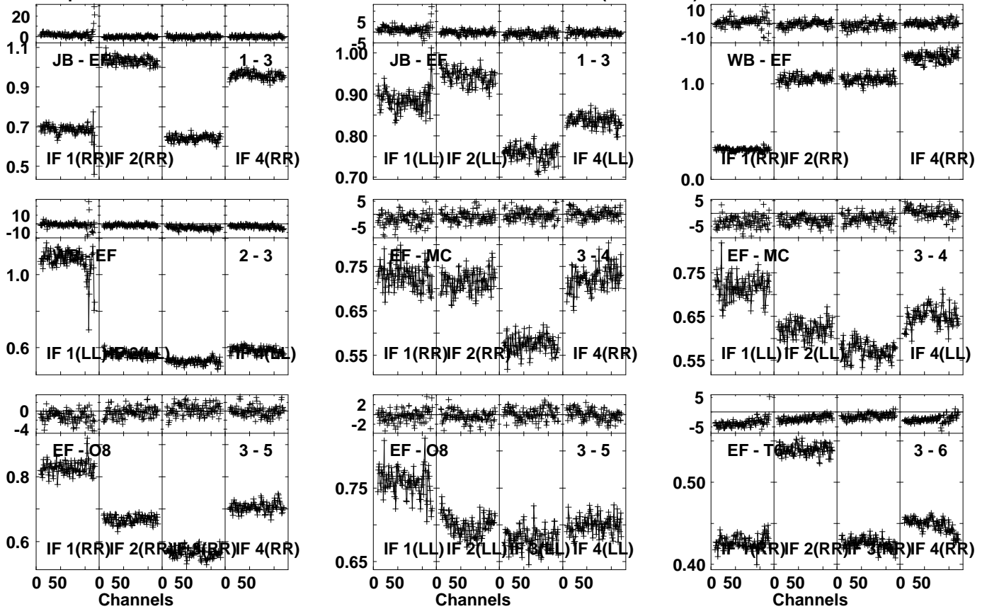
Lower frame: Ampl Jy Top frame: Phas deg Vector averaged cross-power spectrum Several baselines displayed Timerange: 00/23:43:31 to 00/23:44:29
