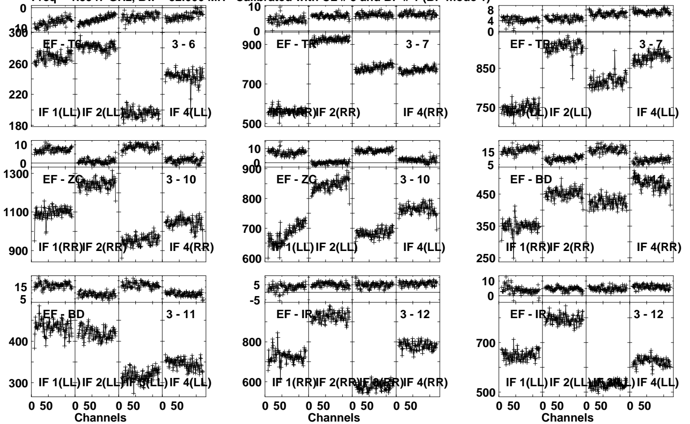
Lower frame: Milli Ampl Jy Top frame: Phas deg Vector averaged cross-power spectrum Several baselines displayed Timerange: 00/22:54:01 to 00/22:54:59
