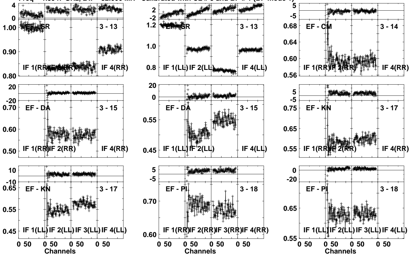
Lower frame: Ampl Jy Top frame: Phas deg Vector averaged cross-power spectrum Several baselines displayed Timerange: 01/00:18:01 to 01/00:19:29
