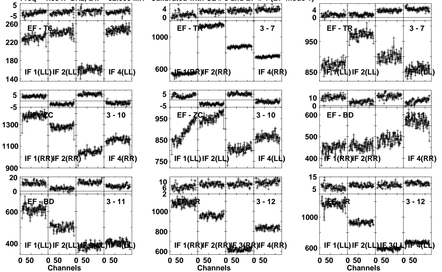
Lower frame: Milli Ampl Jy Top frame: Phas deg Vector averaged cross-power spectrum Several baselines displayed Timerange: 00/22:04:01 to 00/22:04:59
