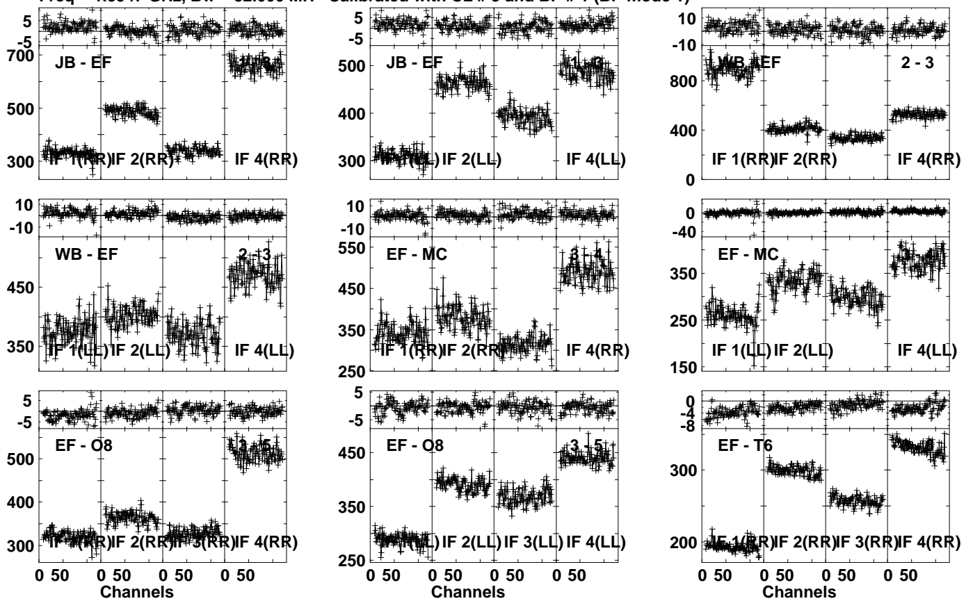
Lower frame: Milli Ampl Jy Top frame: Phas deg Vector averaged cross-power spectrum Several baselines displayed Timerange: 00/15:00:31 to 00/15:01:29
