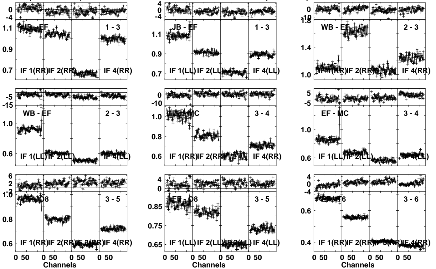
Lower frame: Ampl Jy Top frame: Phas deg Vector averaged cross-power spectrum Several baselines displayed Timerange: 01/00:33:31 to 01/00:34:29
