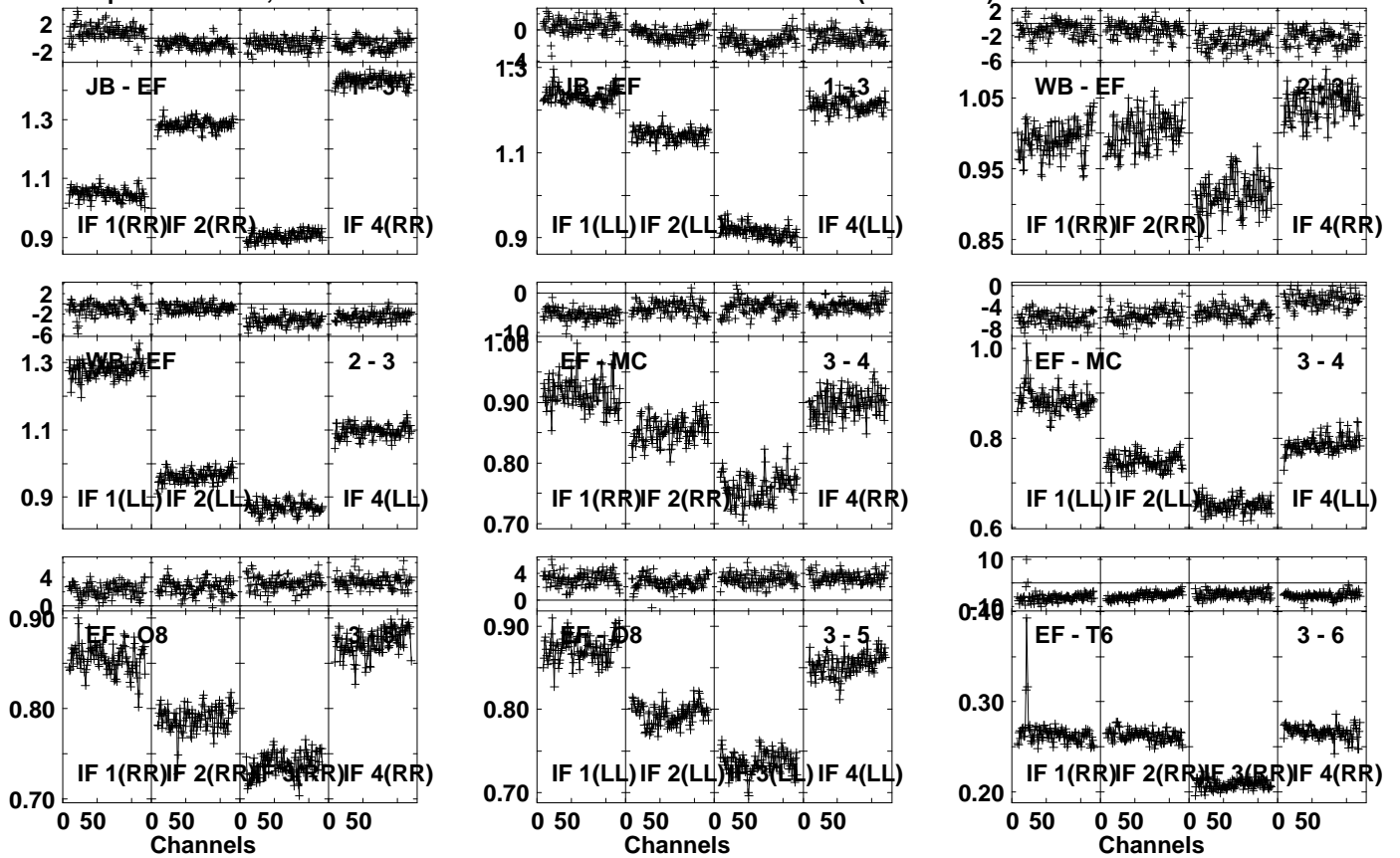
Lower frame: Ampl Jy Top frame: Phas deg Vector averaged cross-power spectrum Several baselines displayed Timerange: 00/22:24:01 to 00/22:24:59
