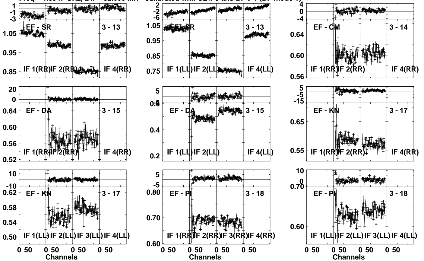
Lower frame: Ampl Jy Top frame: Phas deg Vector averaged cross-power spectrum Several baselines displayed Timerange: 01/00:53:31 to 01/00:54:29
