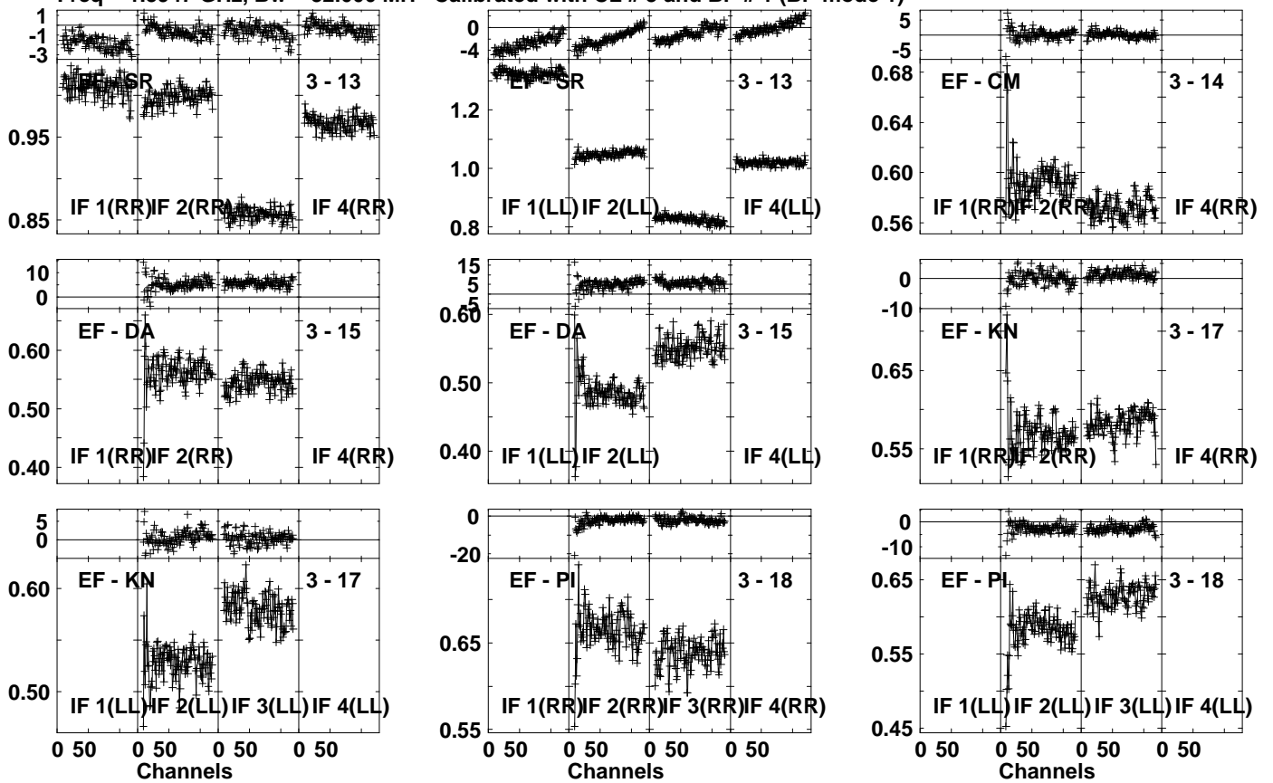
Lower frame: Ampl Jy Top frame: Phas deg Vector averaged cross-power spectrum Several baselines displayed Timerange: 00/23:48:01 to 00/23:49:29
