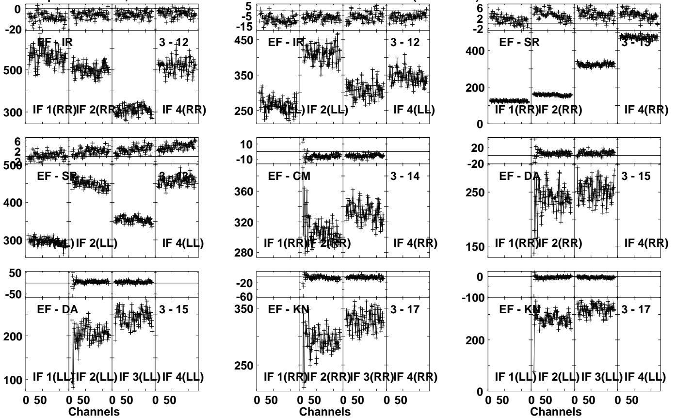
Lower frame: Milli Ampl Jy Top frame: Phas deg Vector averaged cross-power spectrum Several baselines displayed Timerange: 00/16:15:01 to 00/16:16:29
