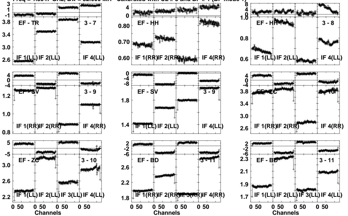
Lower frame: Ampl Jy Top frame: Phas deg Vector averaged cross-power spectrum Several baselines displayed Timerange: 00/16:23:31 to 00/16:26:59
