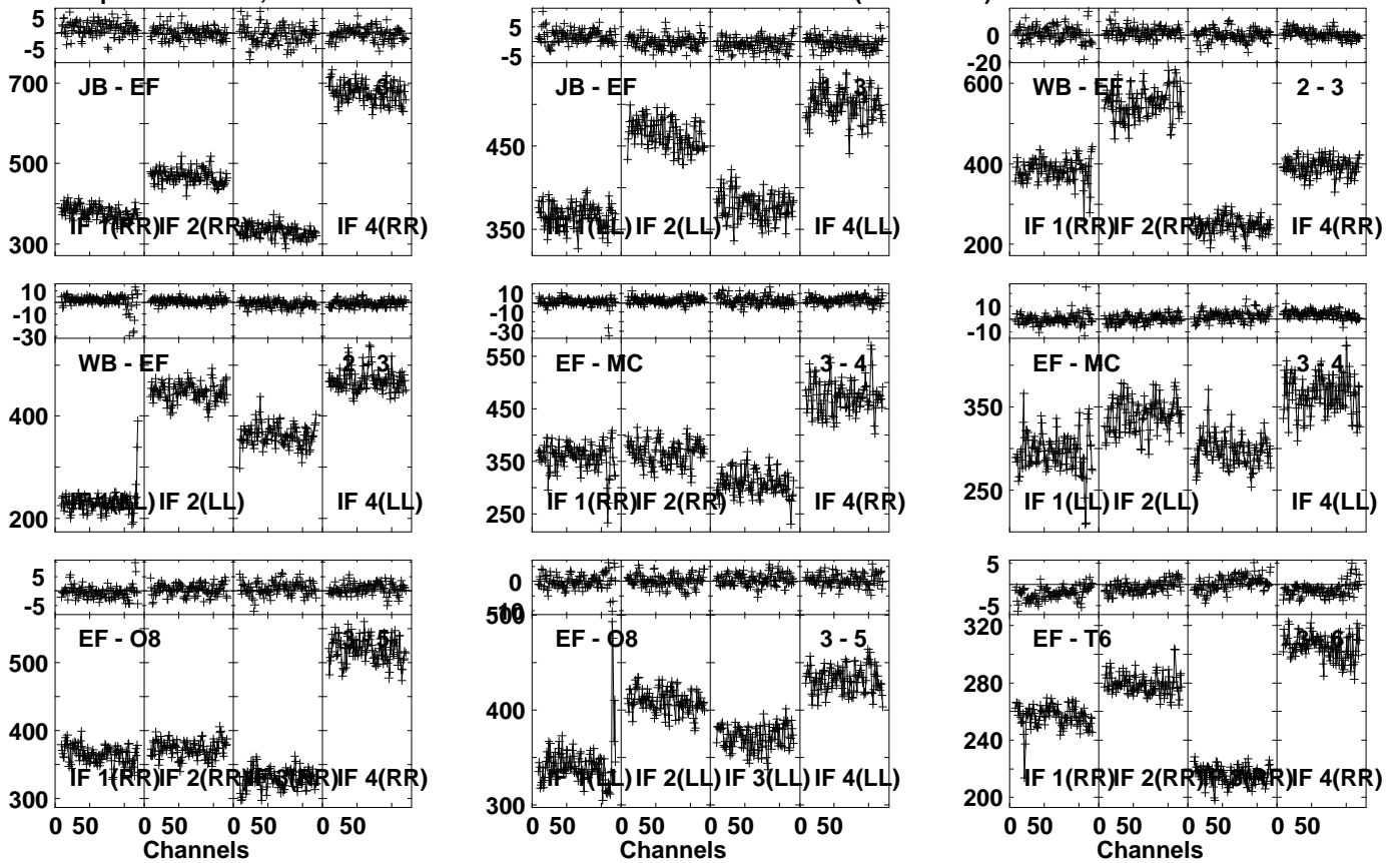
Lower frame: Milli Ampl Jy Top frame: Phas deg Vector averaged cross-power spectrum Several baselines displayed Timerange: 00/14:50:31 to 00/14:51:29
