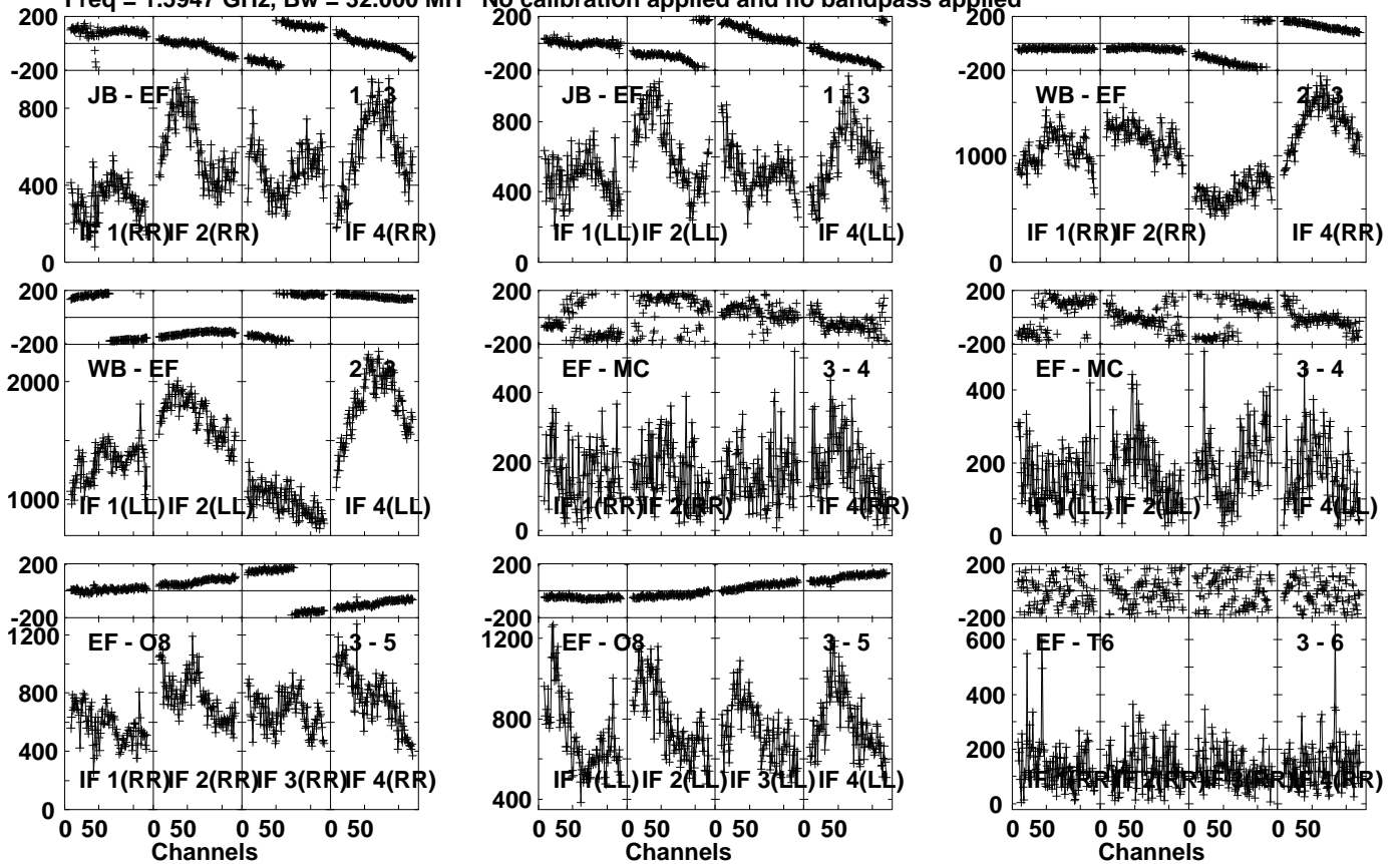
Lower frame: Micro Ampl Jy Top frame: Phas deg Vector averaged cross-power spectrum Several baselines displayed Timerange: 00/22:55:01 to 00/22:58:29
