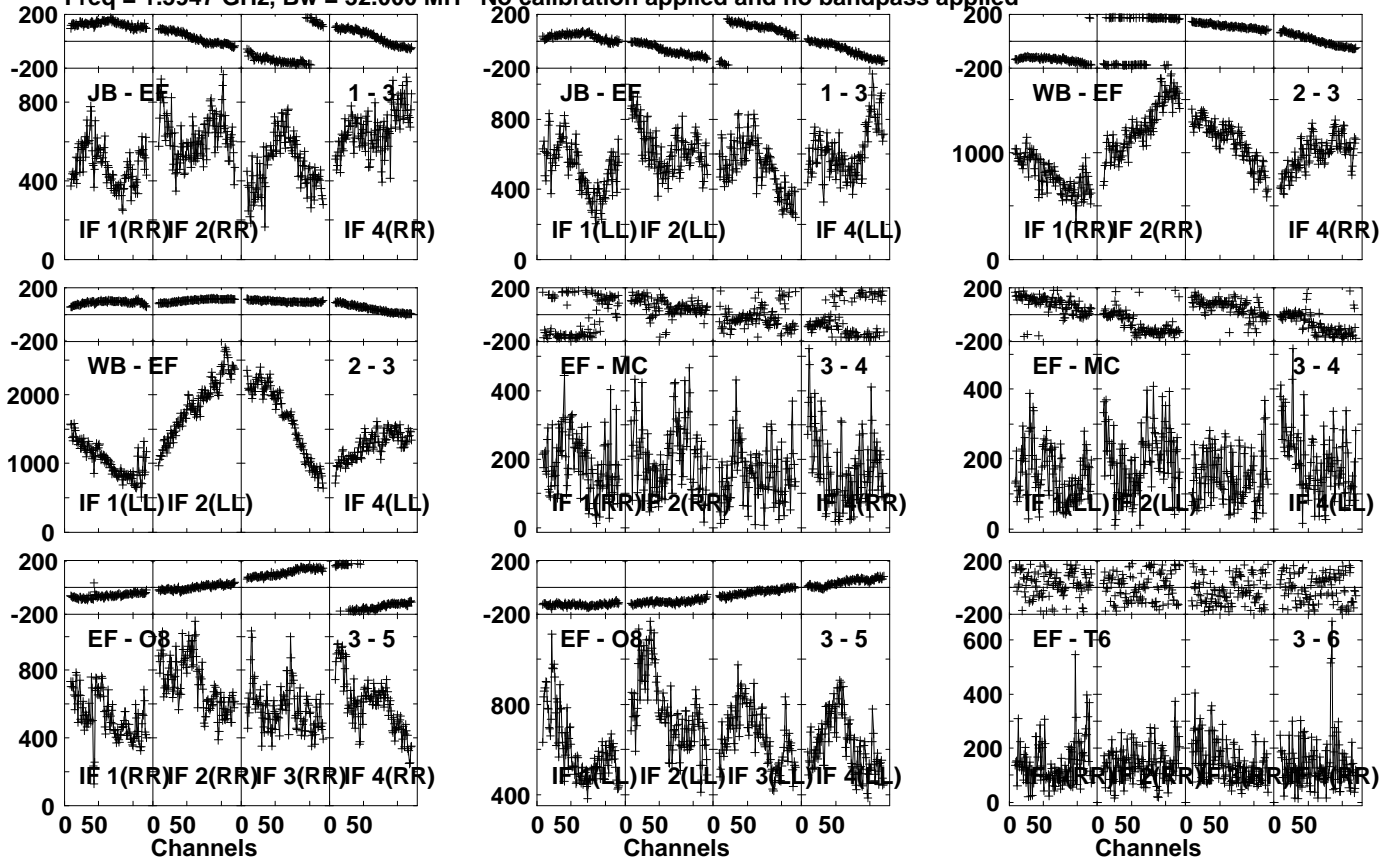
Lower frame: Micro Ampl Jy Top frame: Phas deg Vector averaged cross-power spectrum Several baselines displayed Timerange: 00/23:05:01 to 00/23:08:29
