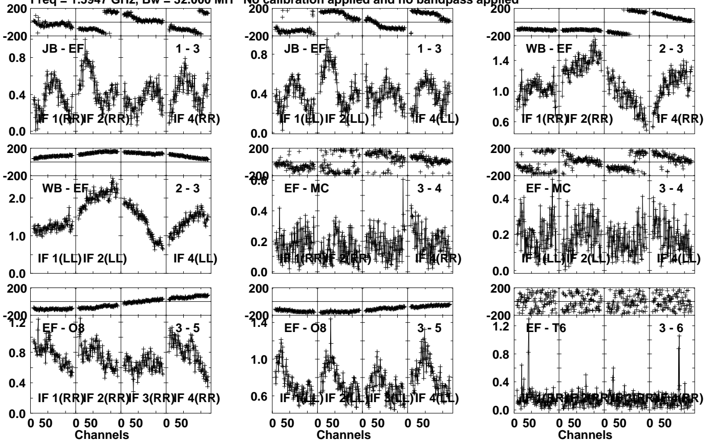
Lower frame: Milli Ampl Jy Top frame: Phas deg Vector averaged cross-power spectrum Several baselines displayed Timerange: 00/22:10:01 to 00/22:13:29
