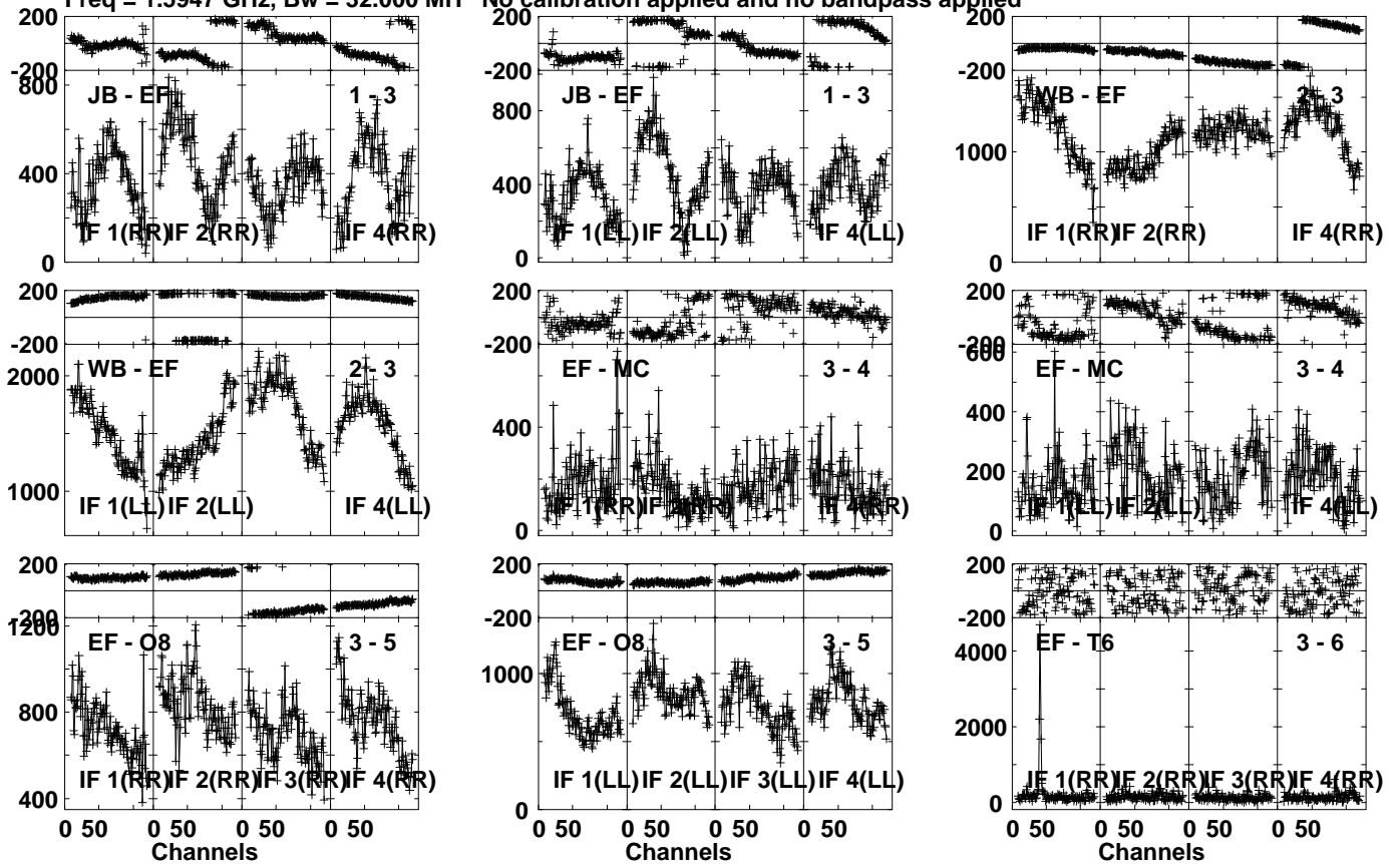
Lower frame: Micro Ampl Jy Top frame: Phas deg Vector averaged cross-power spectrum Several baselines displayed Timerange: 00/22:05:01 to 00/22:08:29
