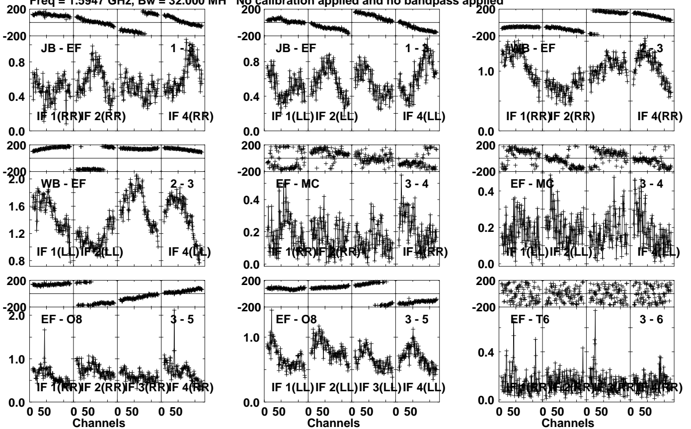
Lower frame: Milli Ampl Jy Top frame: Phas deg Vector averaged cross-power spectrum Several baselines displayed Timerange: 00/23:00:01 to 00/23:03:29
