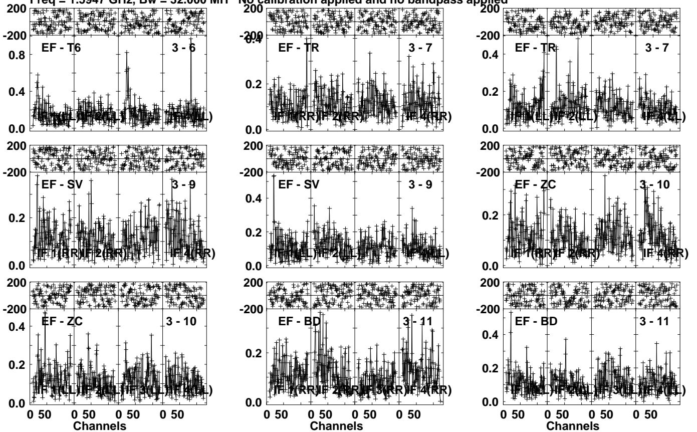
Lower frame: Milli Ampl Jy Top frame: Phas deg Vector averaged cross-power spectrum Several baselines displayed Timerange: 00/16:11:31 to 00/16:14:59
