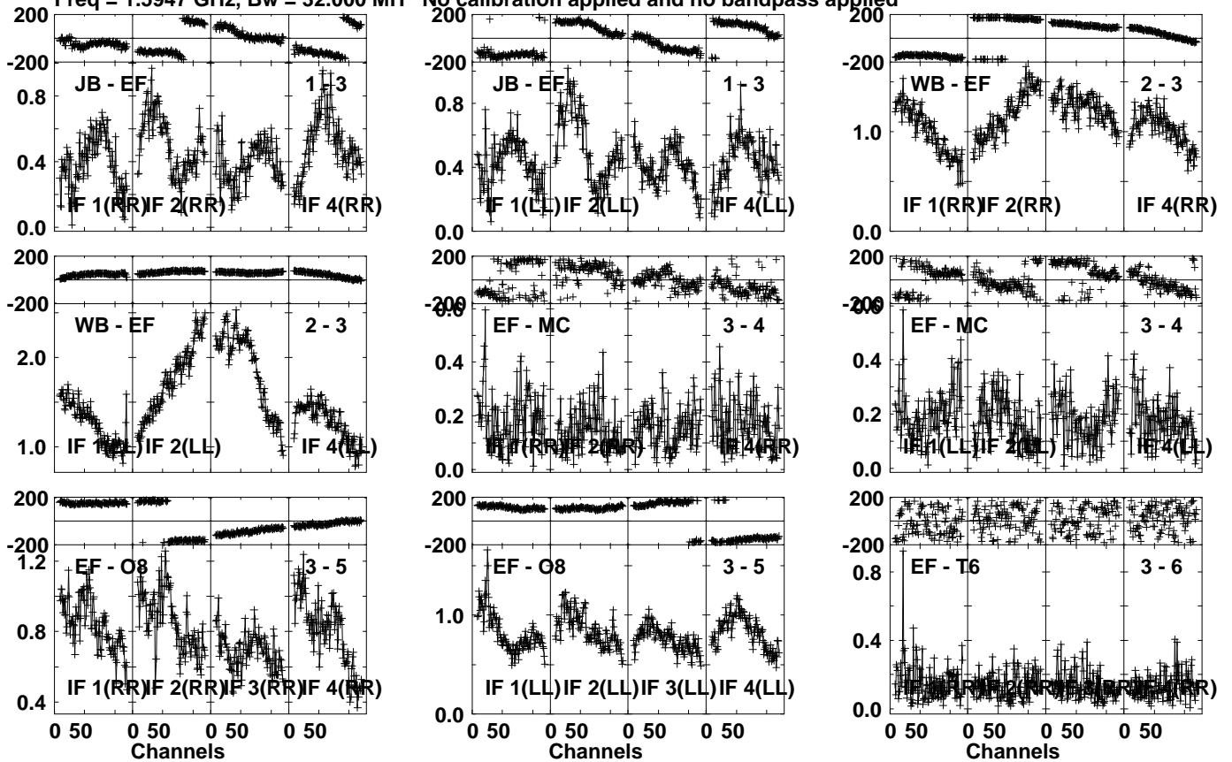
Lower frame: Milli Ampl Jy Top frame: Phas deg Vector averaged cross-power spectrum Several baselines displayed Timerange: 00/22:20:01 to 00/22:23:29
