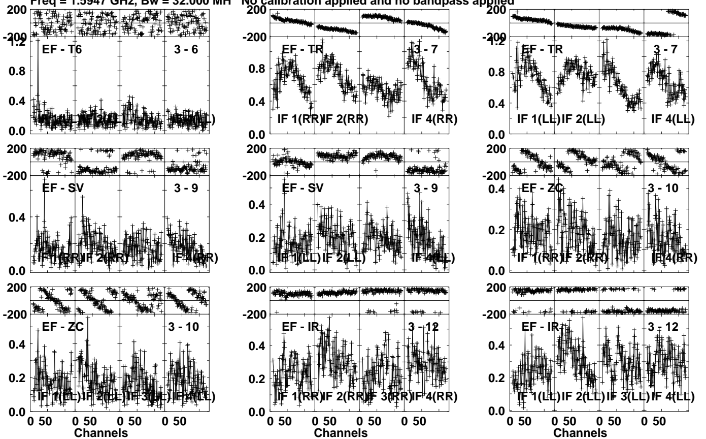
Lower frame: Milli Ampl Jy Top frame: Phas deg Vector averaged cross-power spectrum Several baselines displayed Timerange: 00/21:40:01 to 00/21:43:29
