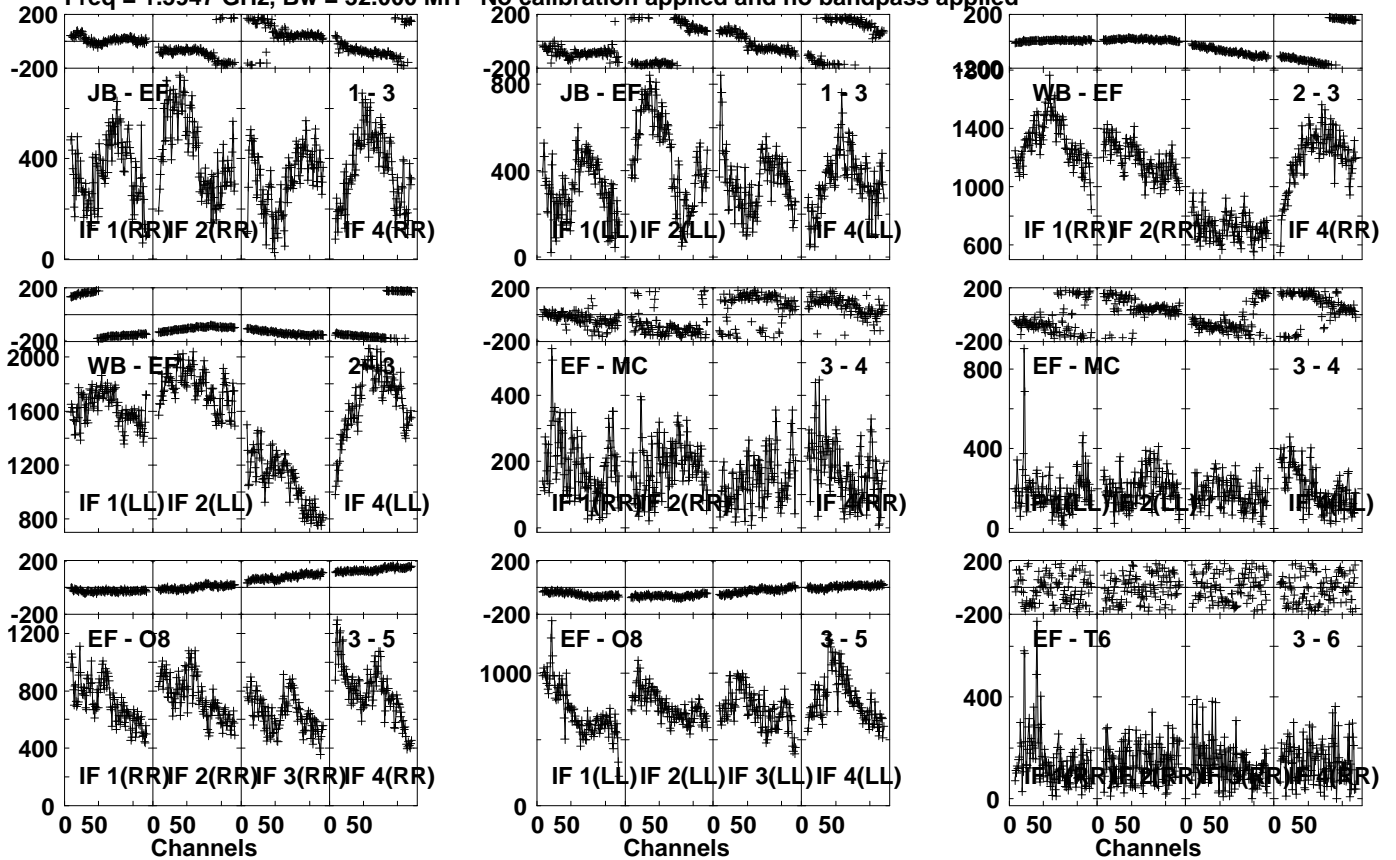
Lower frame: Micro Ampl Jy Top frame: Phas deg Vector averaged cross-power spectrum Several baselines displayed Timerange: 00/22:00:01 to 00/22:03:29
