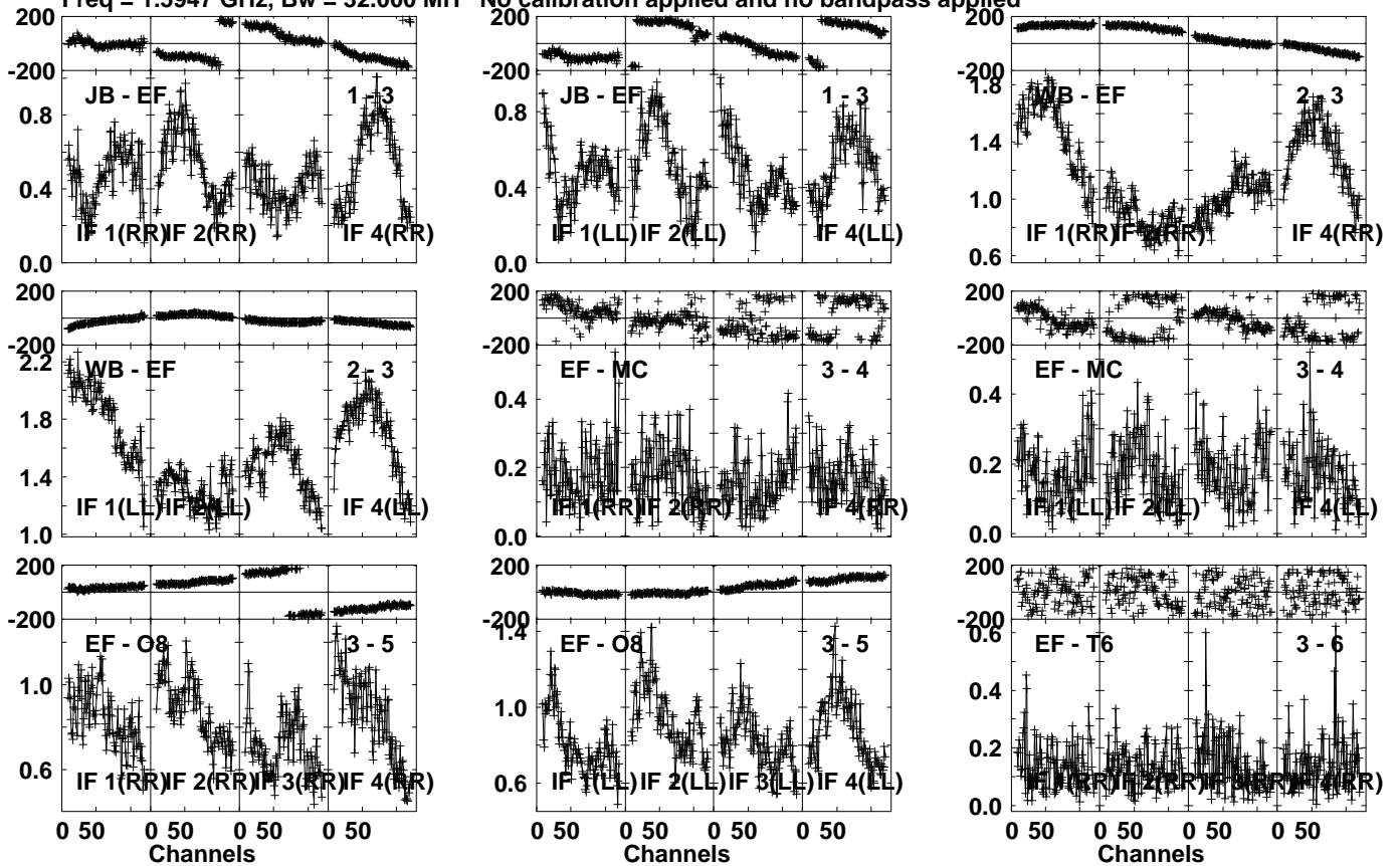
Lower frame: Milli Ampl Jy Top frame: Phas deg Vector averaged cross-power spectrum Several baselines displayed Timerange: 00/22:30:01 to 00/22:33:29
