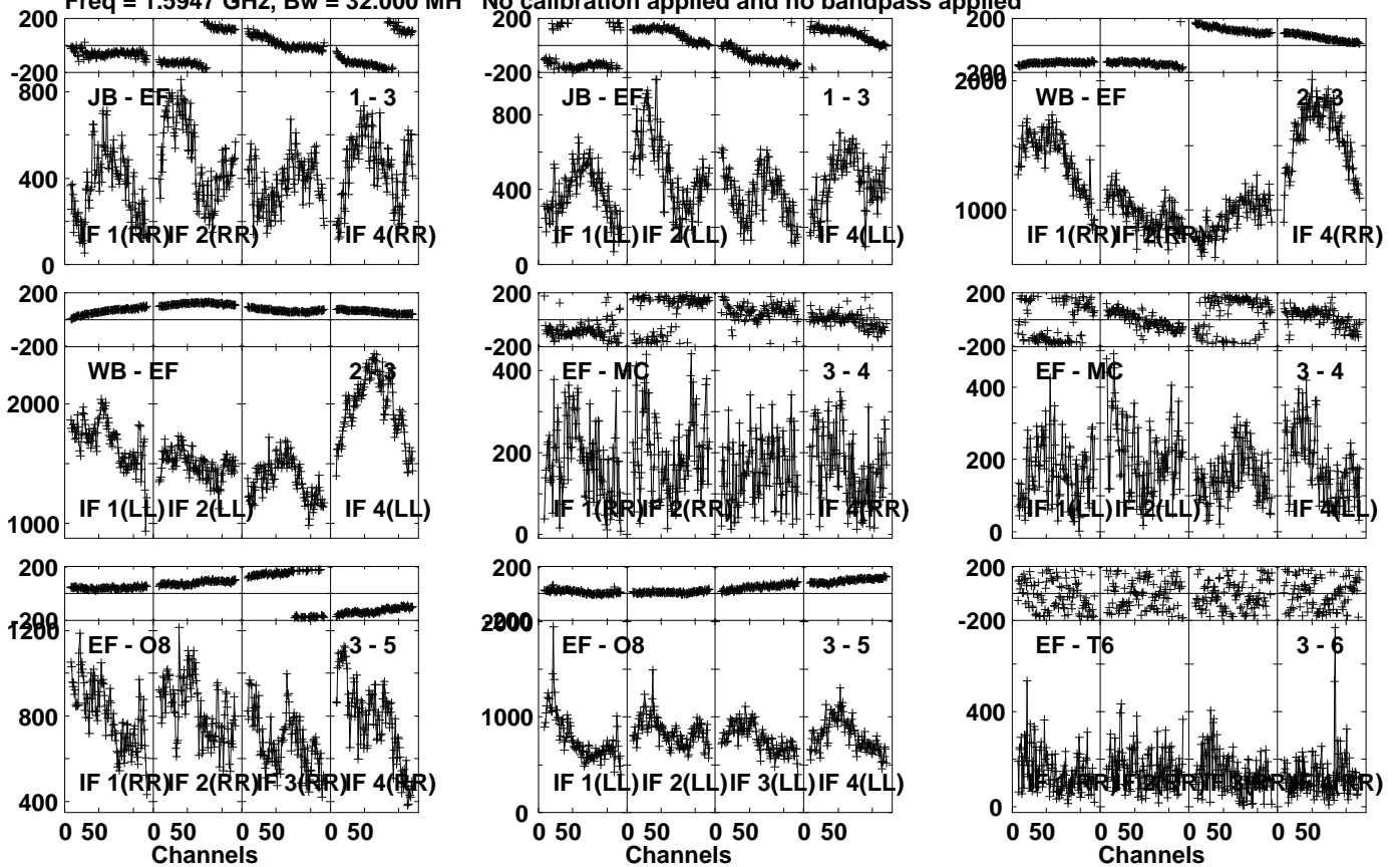
Lower frame: Micro Ampl Jy Top frame: Phas deg Vector averaged cross-power spectrum Several baselines displayed Timerange: 00/22:15:01 to 00/22:18:29
