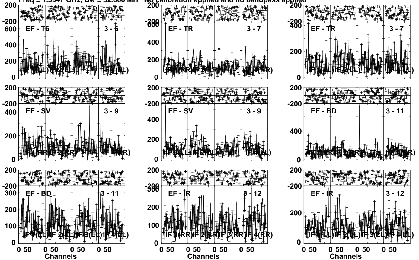
Lower frame: Micro Ampl Jy Top frame: Phas deg Vector averaged cross-power spectrum Several baselines displayed Timerange: 00/15:11:31 to 00/15:14:59
