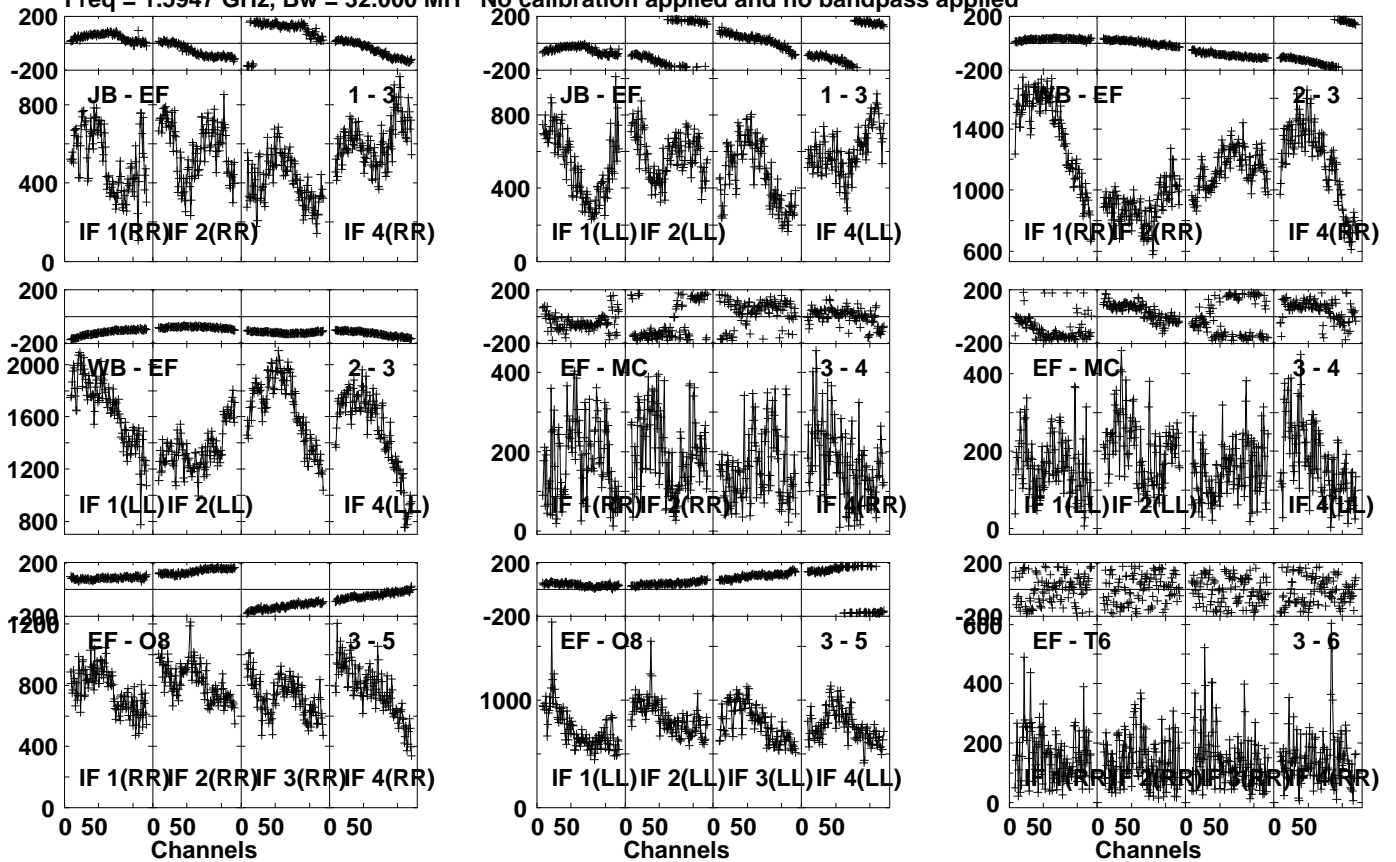
Lower frame: Micro Ampl Jy Top frame: Phas deg Vector averaged cross-power spectrum Several baselines displayed Timerange: 00/22:45:01 to 00/22:48:29
