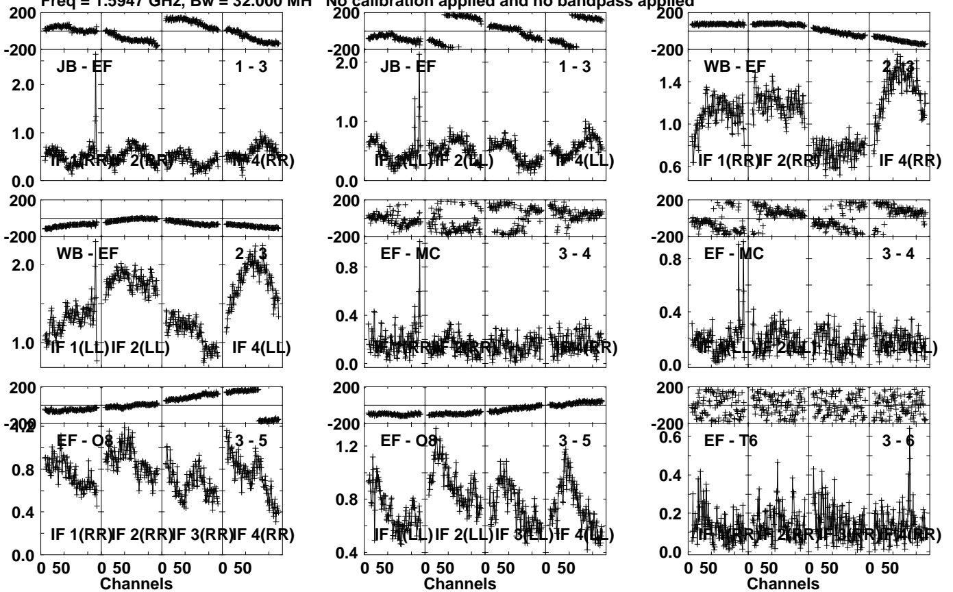
Lower frame: Milli Ampl Jy Top frame: Phas deg Vector averaged cross-power spectrum Several baselines displayed Timerange: 00/22:40:01 to 00/22:43:29
