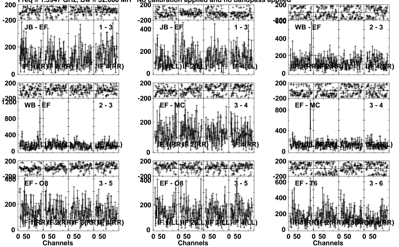
Lower frame: Micro Ampl Jy Top frame: Phas deg Vector averaged cross-power spectrum Several baselines displayed Timerange: 01/00:59:31 to 01/01:02:59
