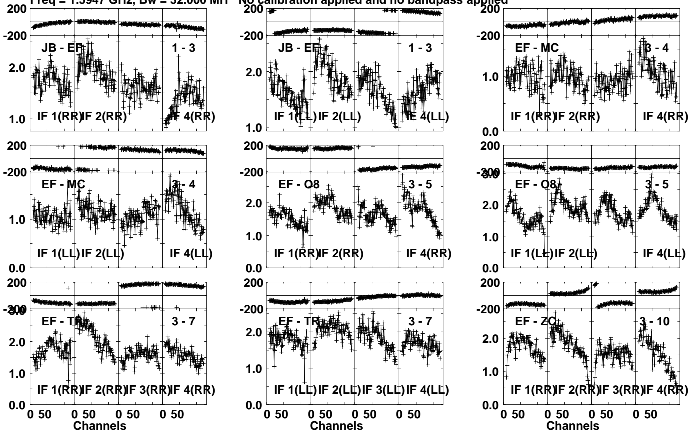
Lower frame: Milli Ampl Jy Top frame: Phas deg Vector averaged cross-power spectrum Several baselines displayed Timerange: 01/09:49:01 to 01/09:49:59
