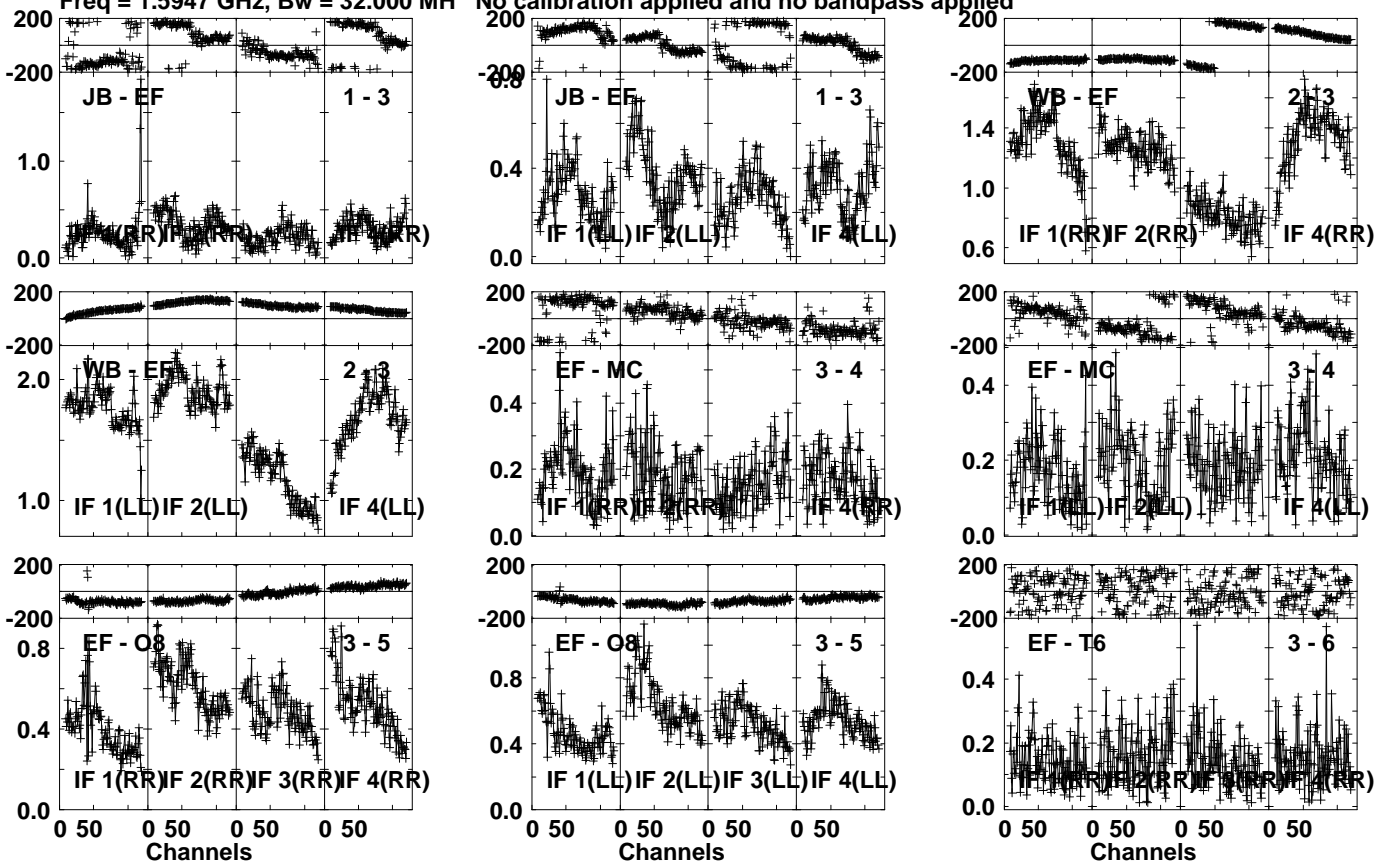
Lower frame: Milli Ampl Jy Top frame: Phas deg Vector averaged cross-power spectrum Several baselines displayed Timerange: 00/21:35:01 to 00/21:38:29
