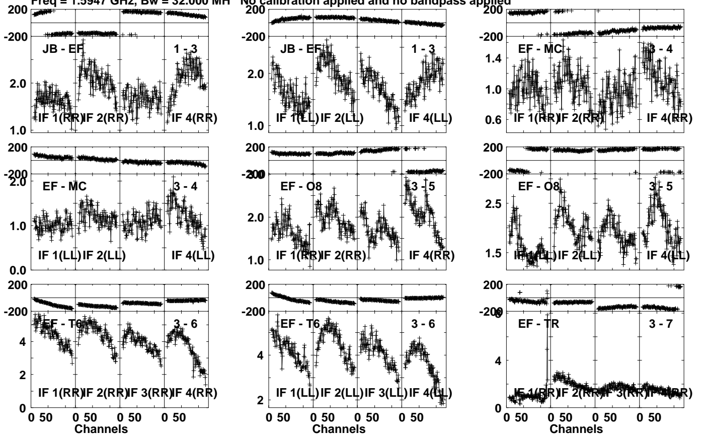
Lower frame: Milli Ampl Jy Top frame: Phas deg Vector averaged cross-power spectrum Several baselines displayed Timerange: 01/10:39:02 to 01/10:39:58
