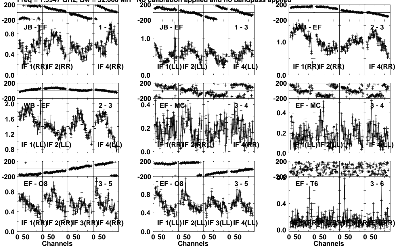
Lower frame: Milli Ampl Jy Top frame: Phas deg Vector averaged cross-power spectrum Several baselines displayed Timerange: 00/23:15:01 to 00/23:18:29
