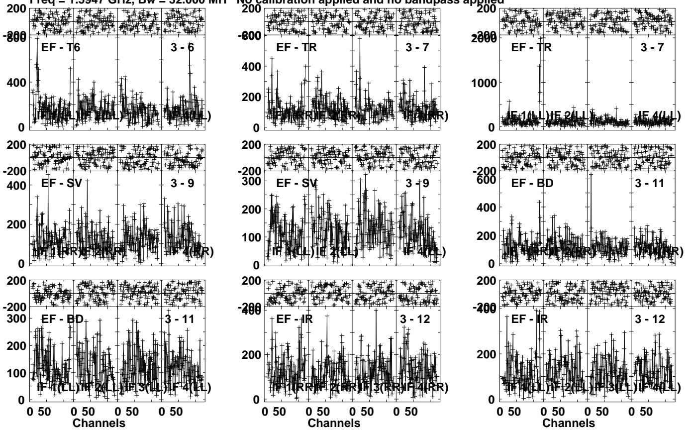
Lower frame: Micro Ampl Jy Top frame: Phas deg Vector averaged cross-power spectrum Several baselines displayed Timerange: 00/15:46:31 to 00/15:49:59
