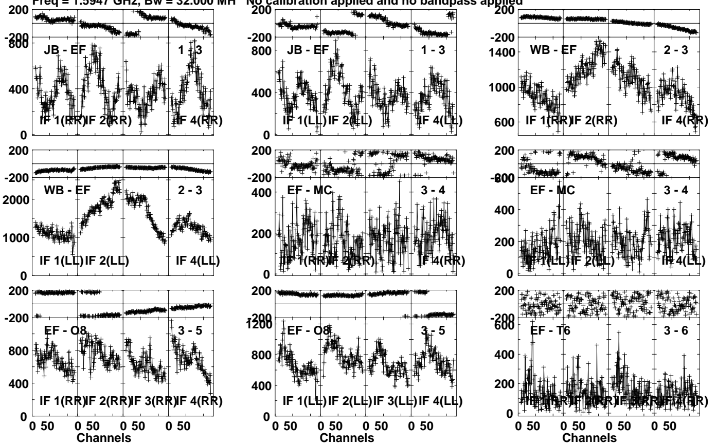
Lower frame: Micro Ampl Jy Top frame: Phas deg Vector averaged cross-power spectrum Several baselines displayed Timerange: 00/21:55:01 to 00/21:58:29
