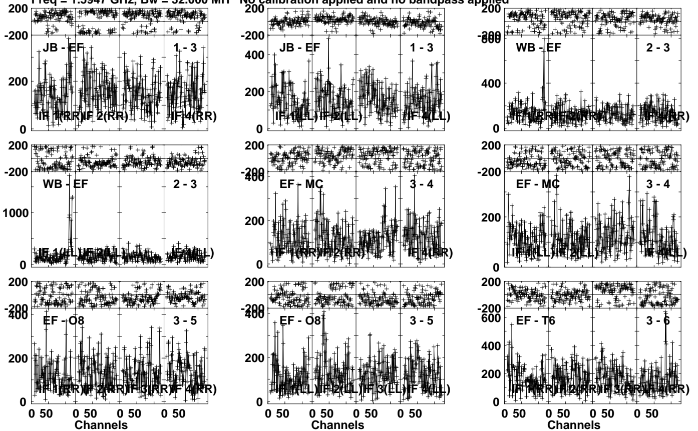
Lower frame: Micro Ampl Jy Top frame: Phas deg Vector averaged cross-power spectrum Several baselines displayed Timerange: 00/23:49:31 to 00/23:52:59
