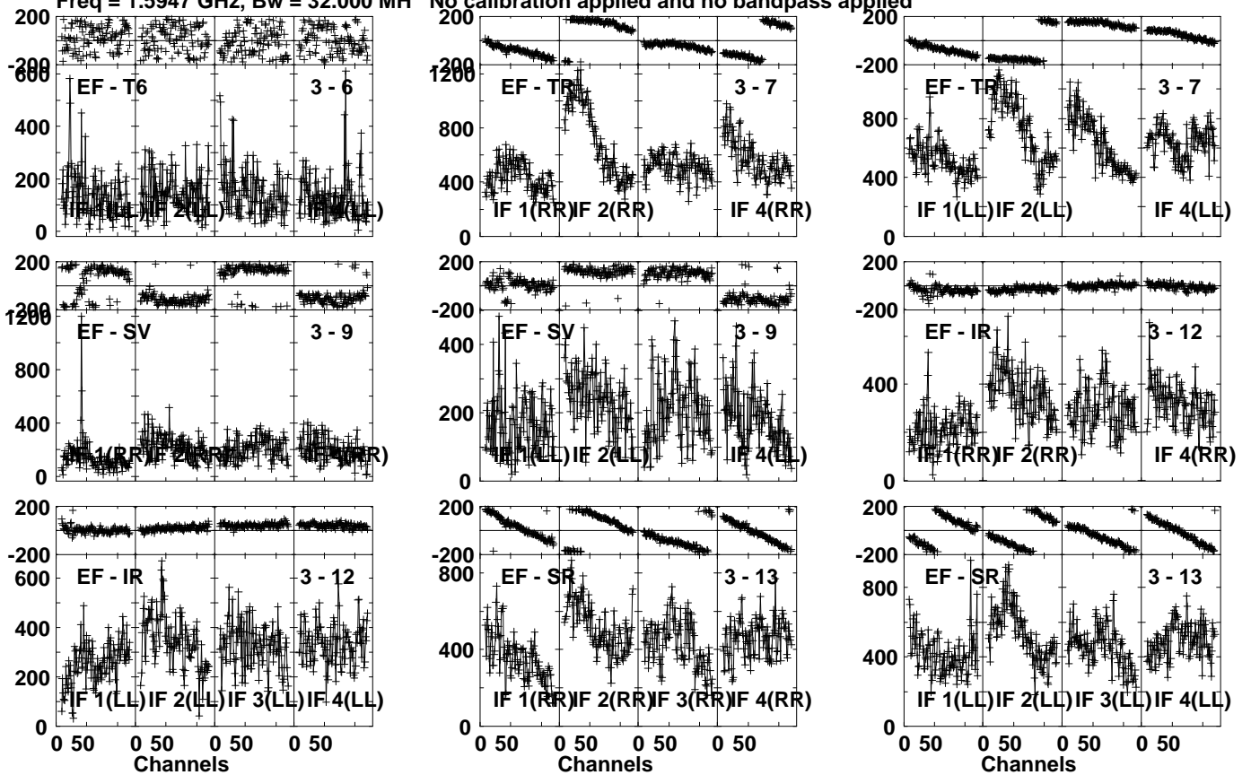
Lower frame: Micro Ampl Jy Top frame: Phas deg Vector averaged cross-power spectrum Several baselines displayed Timerange: 00/21:35:01 to 00/21:38:29
