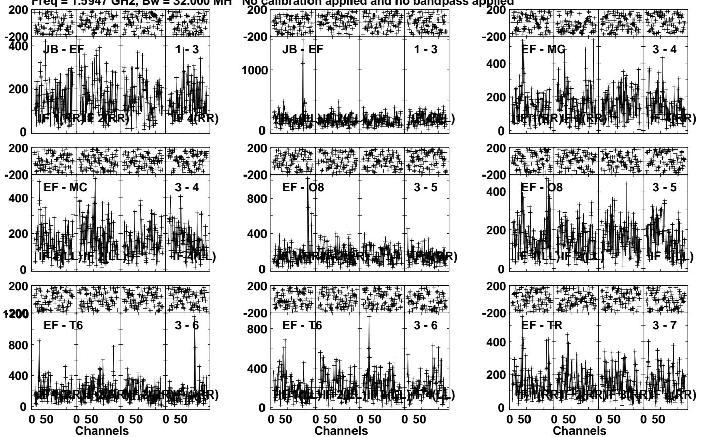
Lower frame: Micro Ampl Jy Top frame: Phas deg Vector averaged cross-power spectrum Several baselines displayed Timerange: 01/10:40:02 to 01/10:43:28
