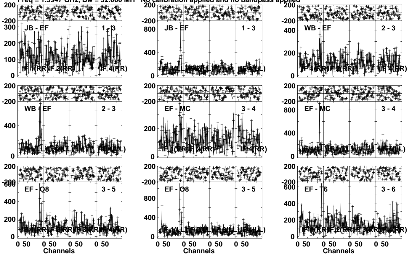
Lower frame: Micro Ampl Jy Top frame: Phas deg Vector averaged cross-power spectrum Several baselines displayed Timerange: 00/14:31:31 to 00/14:34:59
