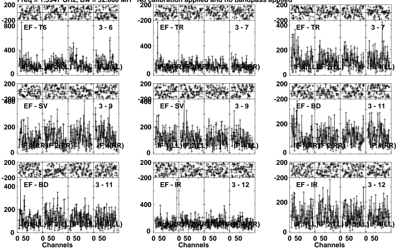
Lower frame: Micro Ampl Jy Top frame: Phas deg Vector averaged cross-power spectrum Several baselines displayed Timerange: 00/15:21:31 to 00/15:24:59
