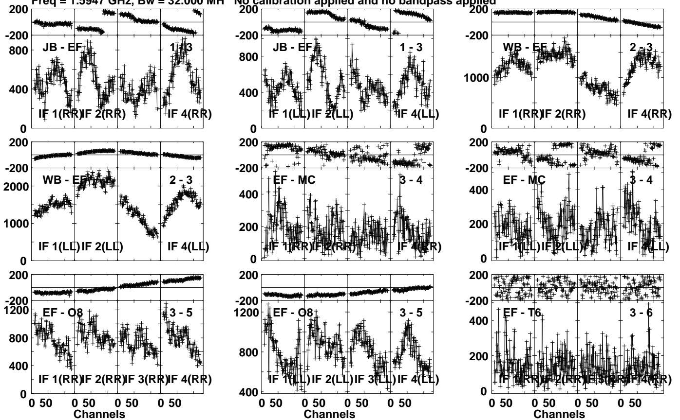
Lower frame: Micro Ampl Jy Top frame: Phas deg Vector averaged cross-power spectrum Several baselines displayed Timerange: 00/22:25:01 to 00/22:28:29
