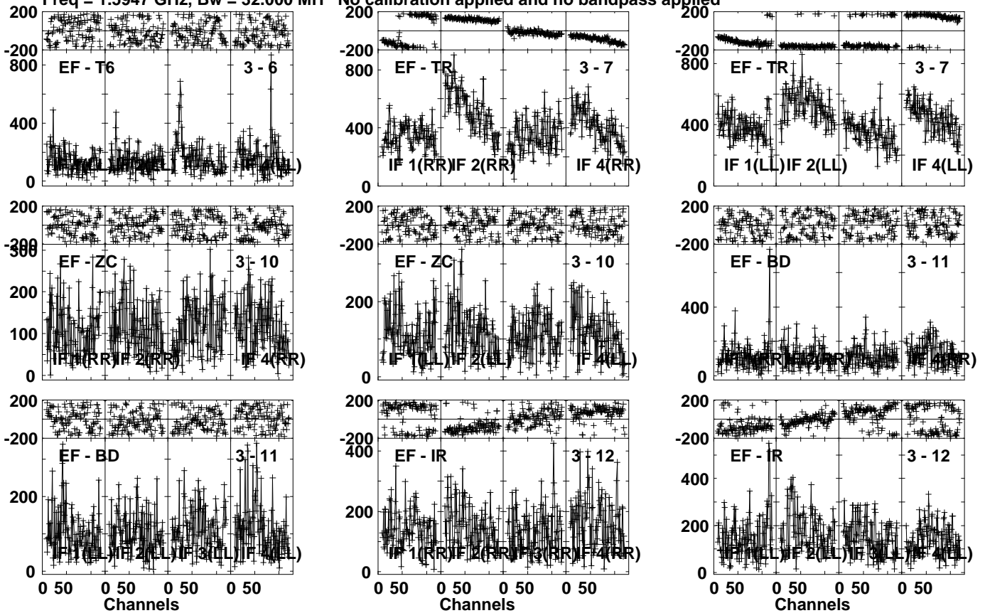
Lower frame: Micro Ampl Jy Top frame: Phas deg Vector averaged cross-power spectrum Several baselines displayed Timerange: 00/23:15:01 to 00/23:18:29
