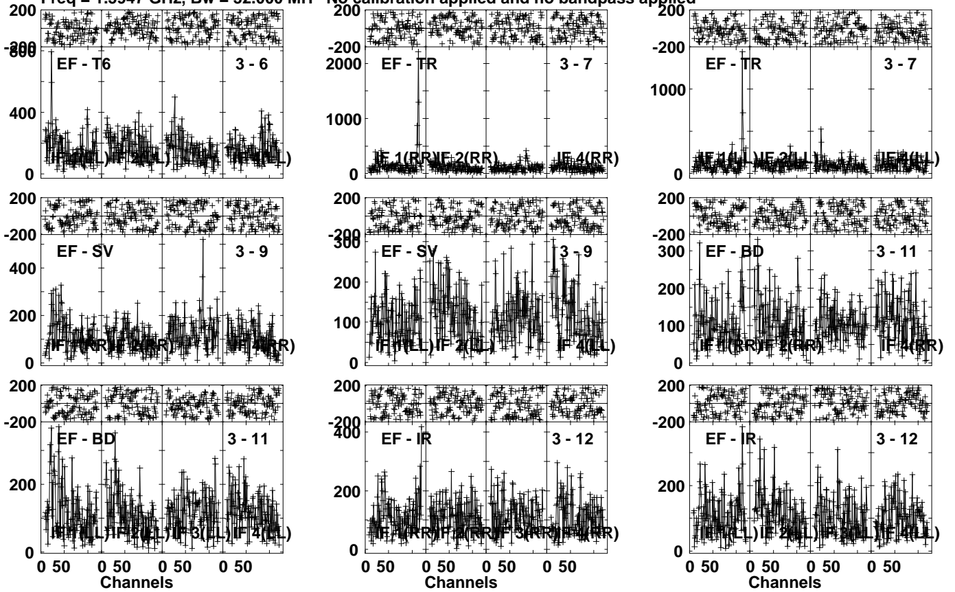
Lower frame: Micro Ampl Jy Top frame: Phas deg Vector averaged cross-power spectrum Several baselines displayed Timerange: 00/15:26:31 to 00/15:29:59
