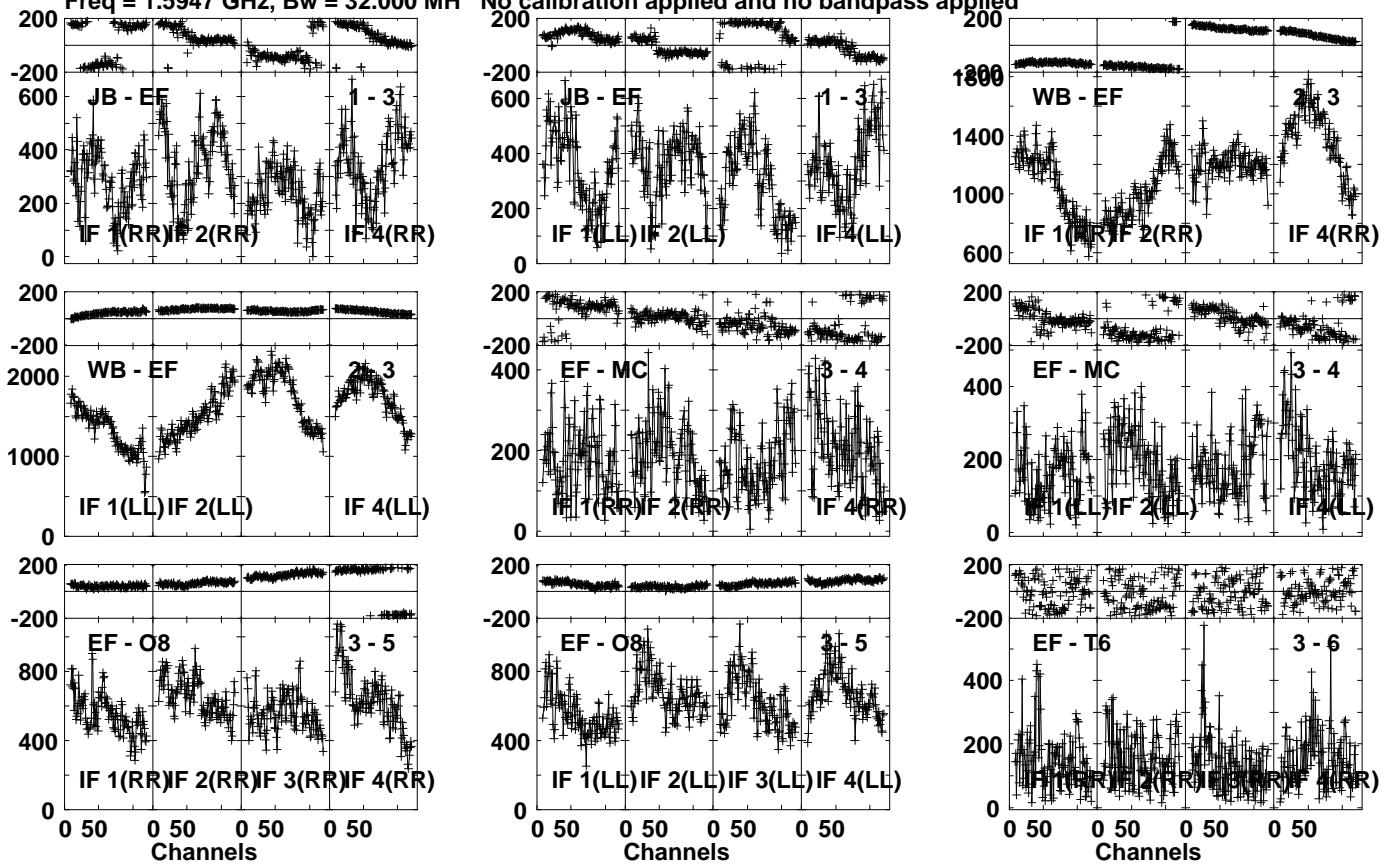
Lower frame: Micro Ampl Jy Top frame: Phas deg Vector averaged cross-power spectrum Several baselines displayed Timerange: 00/21:40:01 to 00/21:43:29
