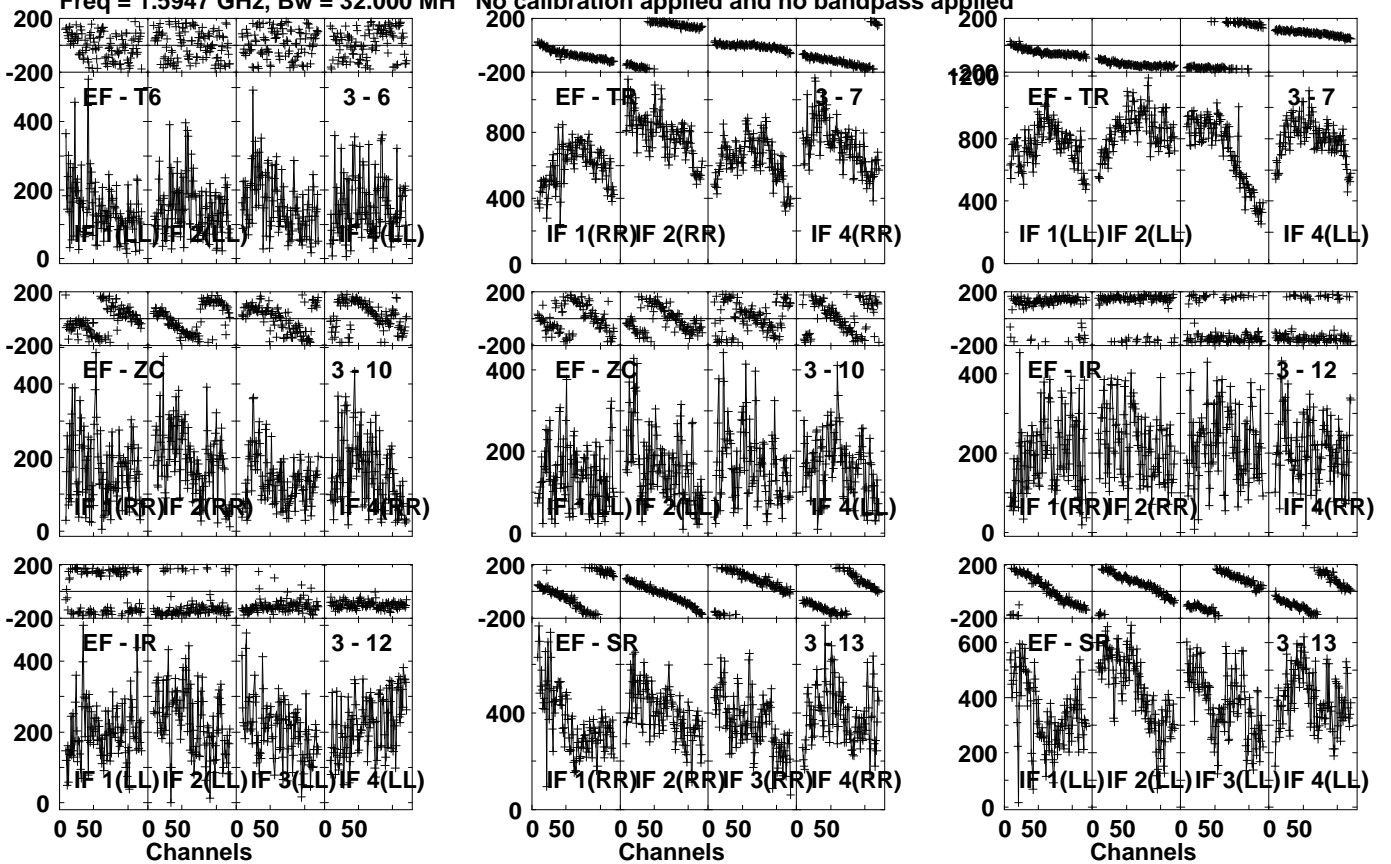
Lower frame: Micro Ampl Jy Top frame: Phas deg Vector averaged cross-power spectrum Several baselines displayed Timerange: 00/21:50:01 to 00/21:53:29
