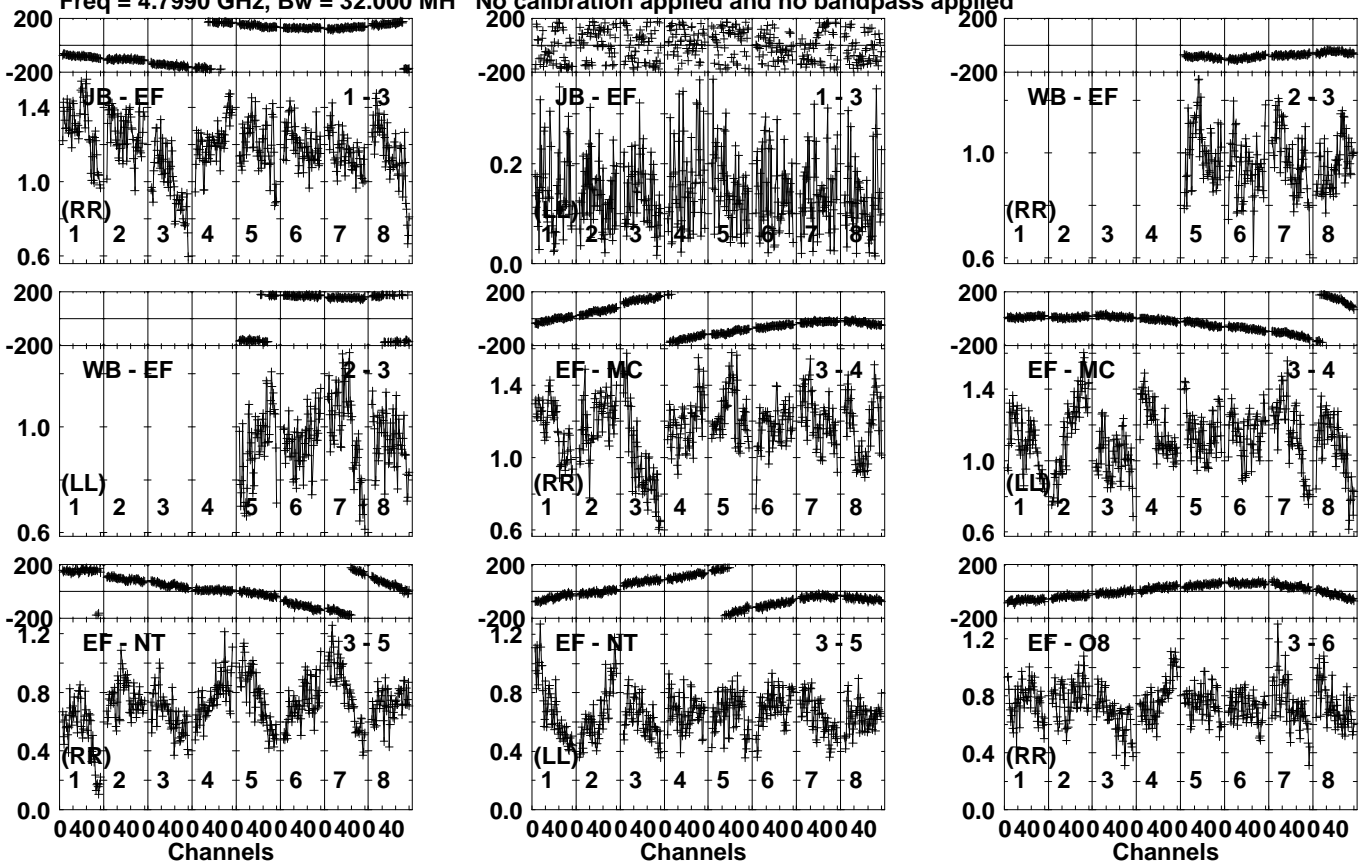
Lower frame: Milli Ampl Jy Top frame: Phas deg Vector averaged cross-power spectrum Several baselines displayed Timerange: 00/20:30:01 to 00/20:31:59
