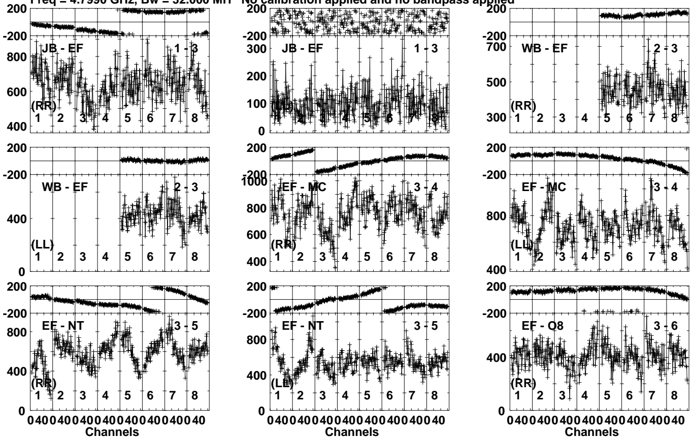
Lower frame: Micro Ampl Jy Top frame: Phas deg Vector averaged cross-power spectrum Several baselines displayed Timerange: 00/20:06:03 to 00/20:08:59
