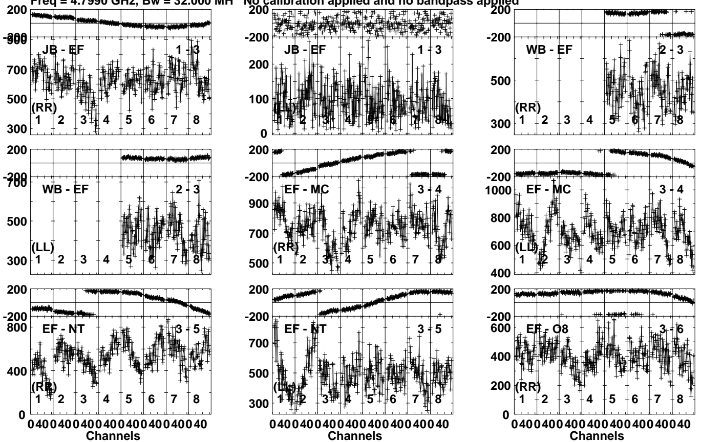
Lower frame: Micro Ampl Jy Top frame: Phas deg Vector averaged cross-power spectrum Several baselines displayed Timerange: 00/19:39:31 to 00/19:42:29
