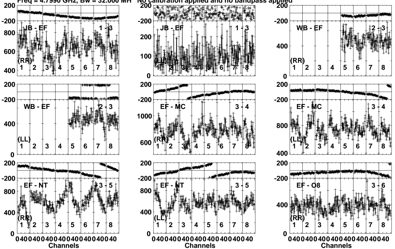
Lower frame: Micro Ampl Jy Top frame: Phas deg Vector averaged cross-power spectrum Several baselines displayed Timerange: 00/20:42:31 to 00/20:45:29
