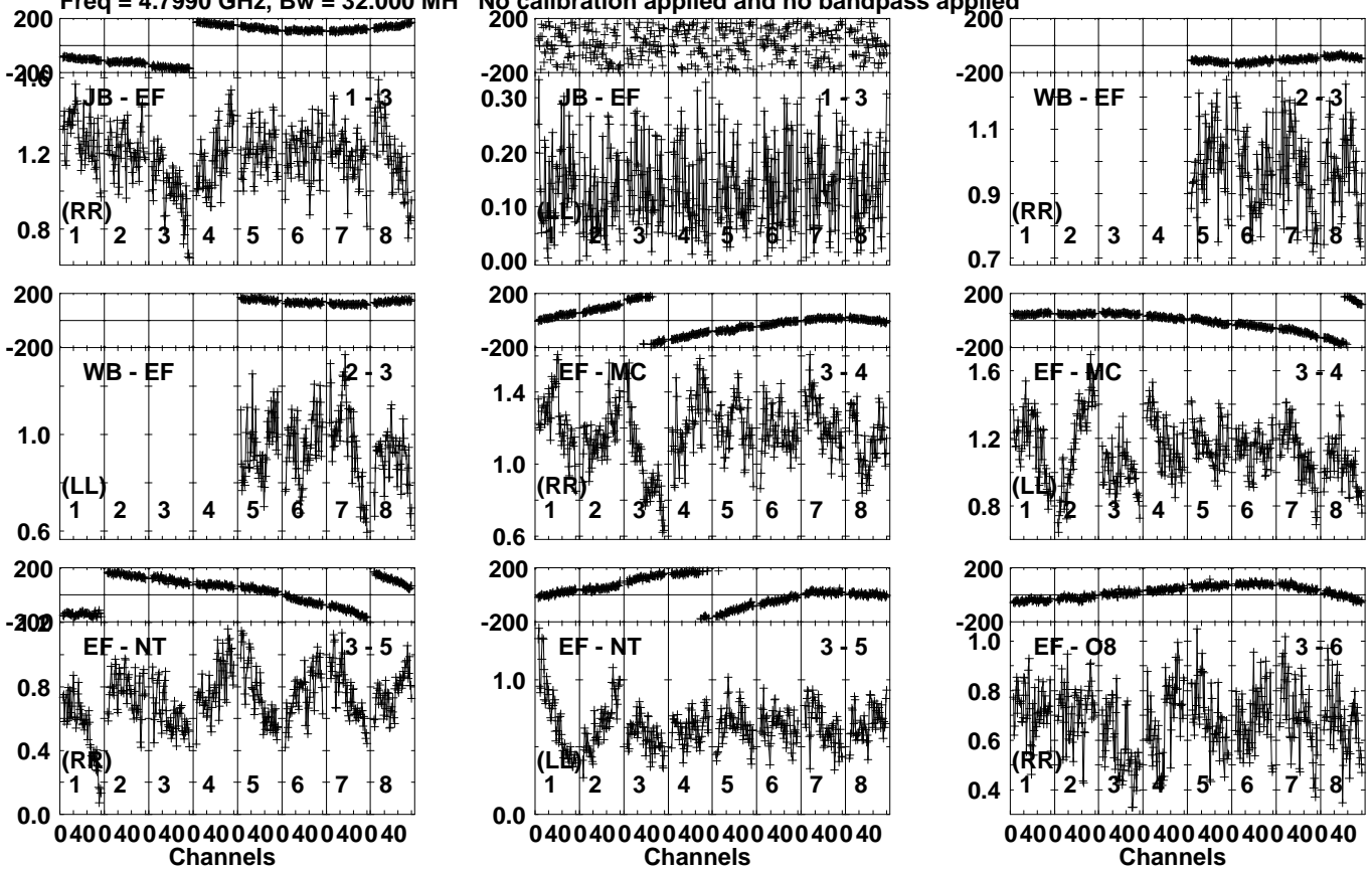
Lower frame: Milli Ampl Jy Top frame: Phas deg Vector averaged cross-power spectrum Several baselines displayed Timerange: 00/20:40:31 to 00/20:42:29
