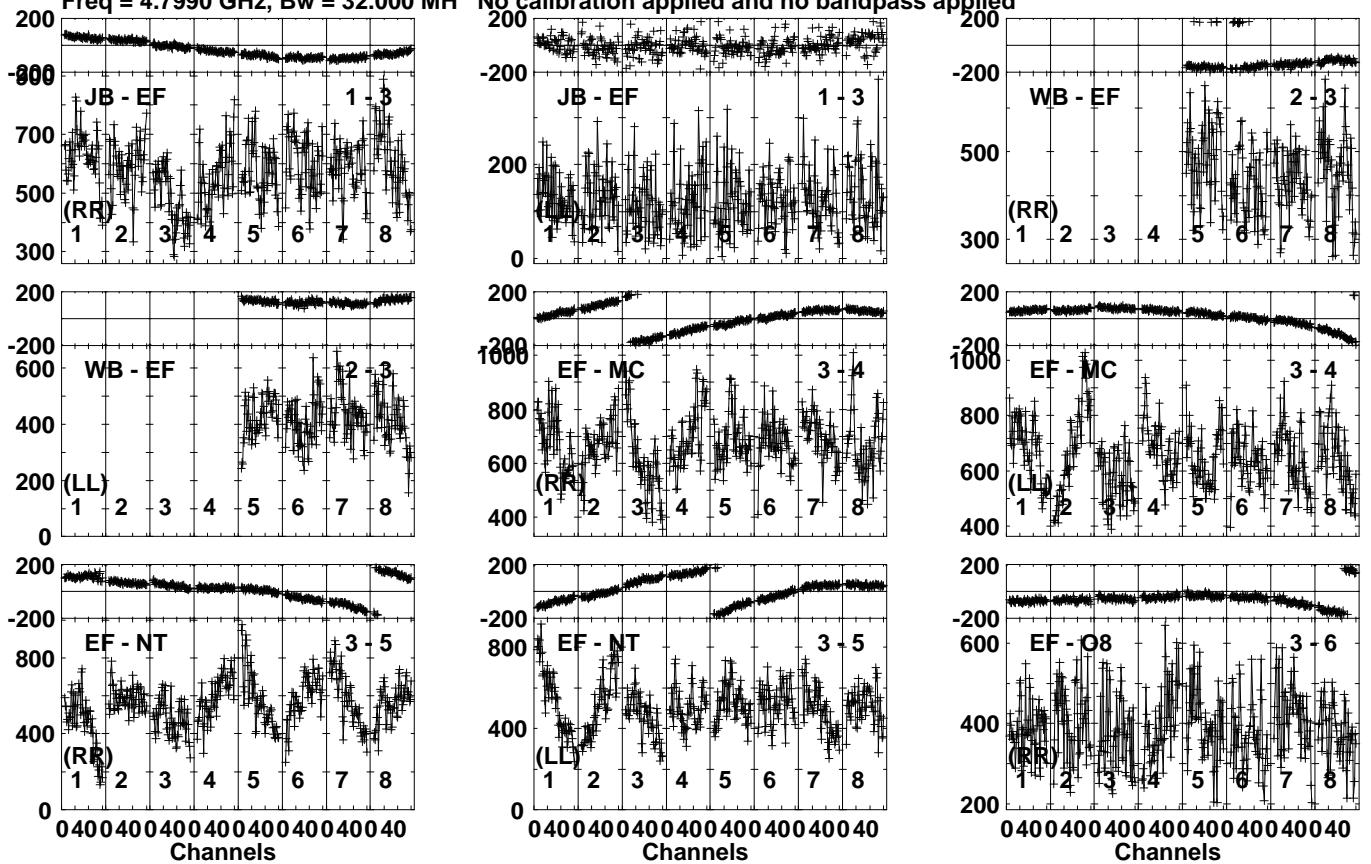
Lower frame: Micro Ampl Jy Top frame: Phas deg Vector averaged cross-power spectrum Several baselines displayed Timerange: 00:18:45:31 to 00:18:48:29
