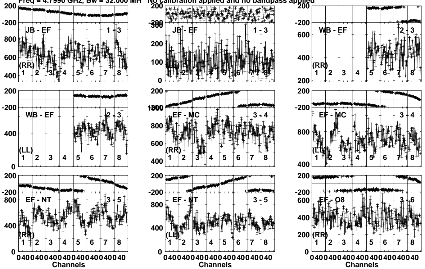
Lower frame: Micro Ampl Jy Top frame: Phas deg Vector averaged cross-power spectrum Several baselines displayed Timerange: 00:19:34:33 to 00:19:37:29
