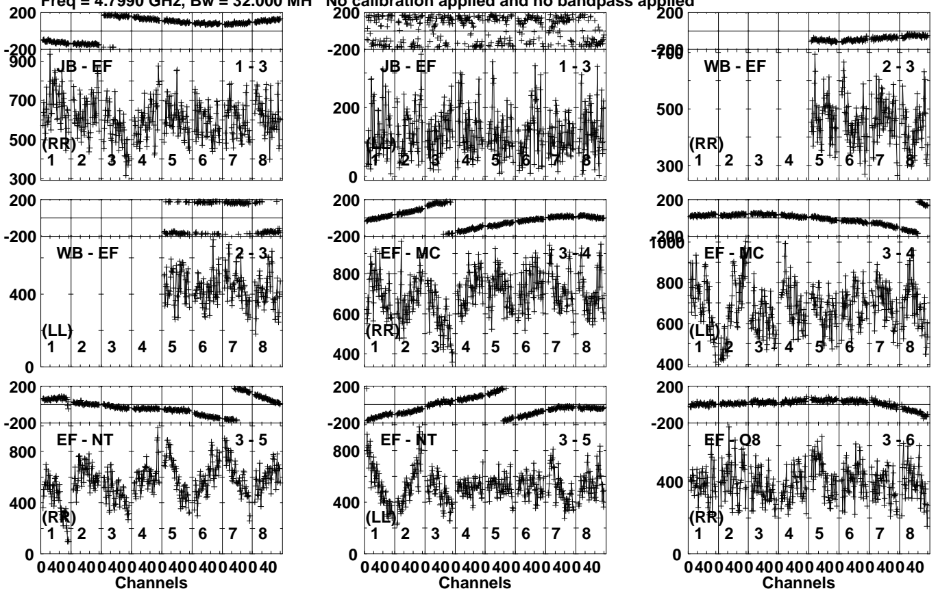
Lower frame: Micro Ampl Jy Top frame: Phas deg Vector averaged cross-power spectrum Several baselines displayed Timerange: 00/19:13:33 to 00/19:16:29
