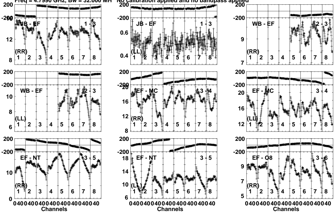
Lower frame: Milli Ampl Jy Top frame: Phas deg Vector averaged cross-power spectrum Several baselines displayed Timerange: 00/20:54:01 to 00/20:58:59
