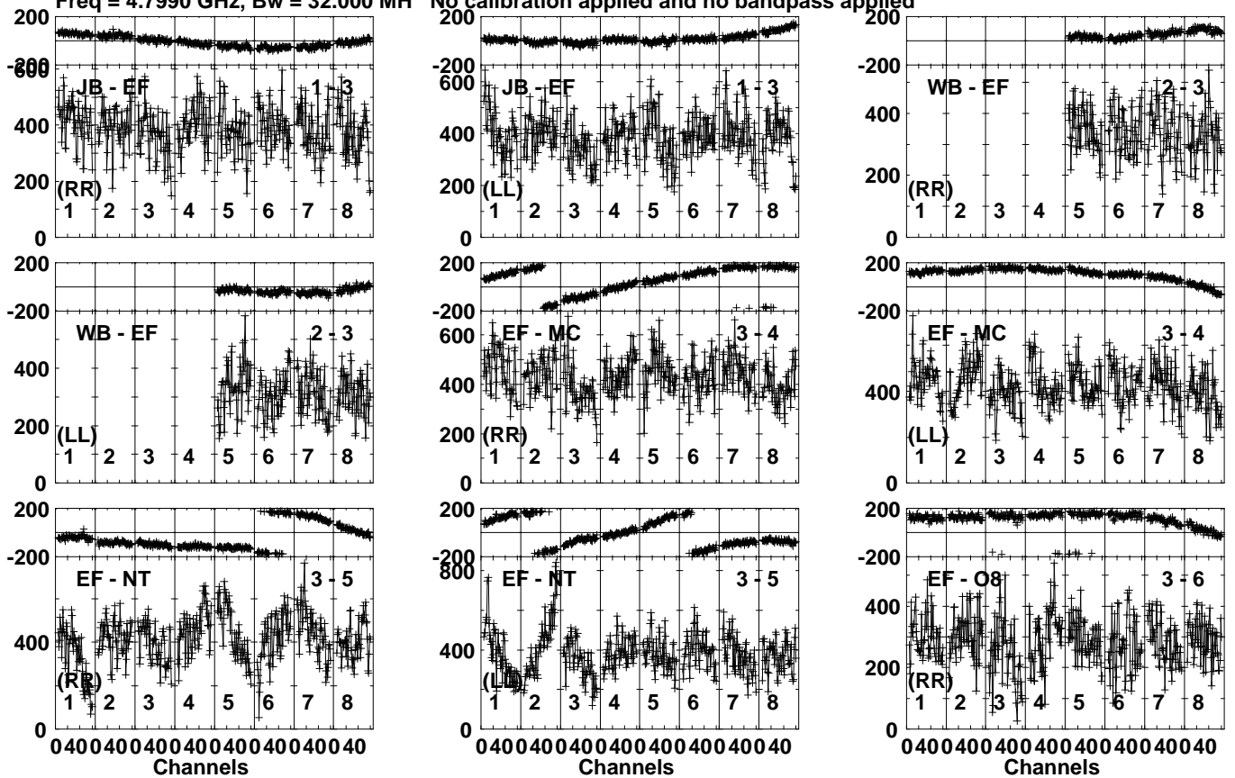
Lower frame: Micro Ampl Jy Top frame: Phas deg Vector averaged cross-power spectrum Several baselines displayed Timerange: 00/17:16:33 to 00/17:19:29
