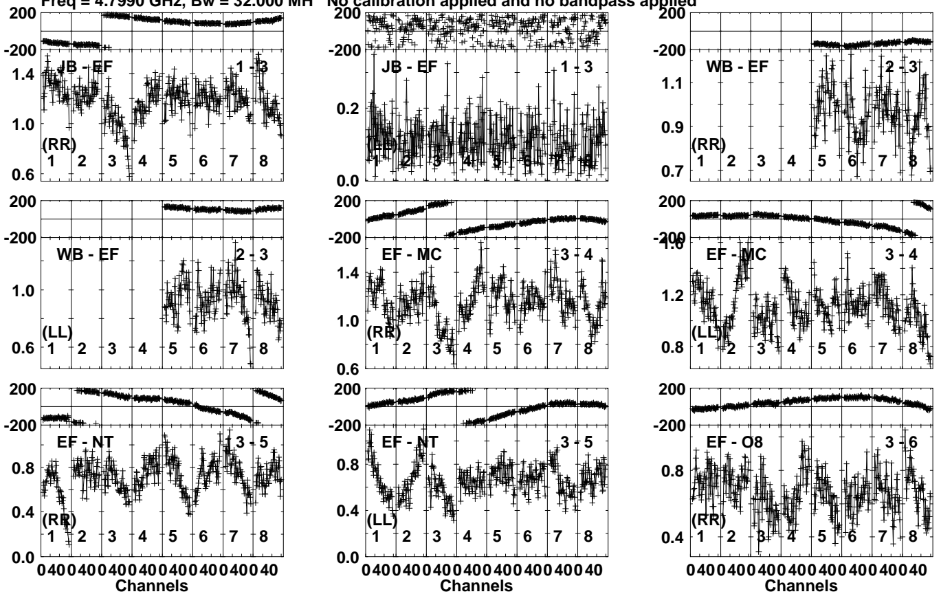
Lower frame: Milli Ampl Jy Top frame: Phas deg Vector averaged cross-power spectrum Several baselines displayed Timerange: 00/20:46:01 to 00/20:47:59
