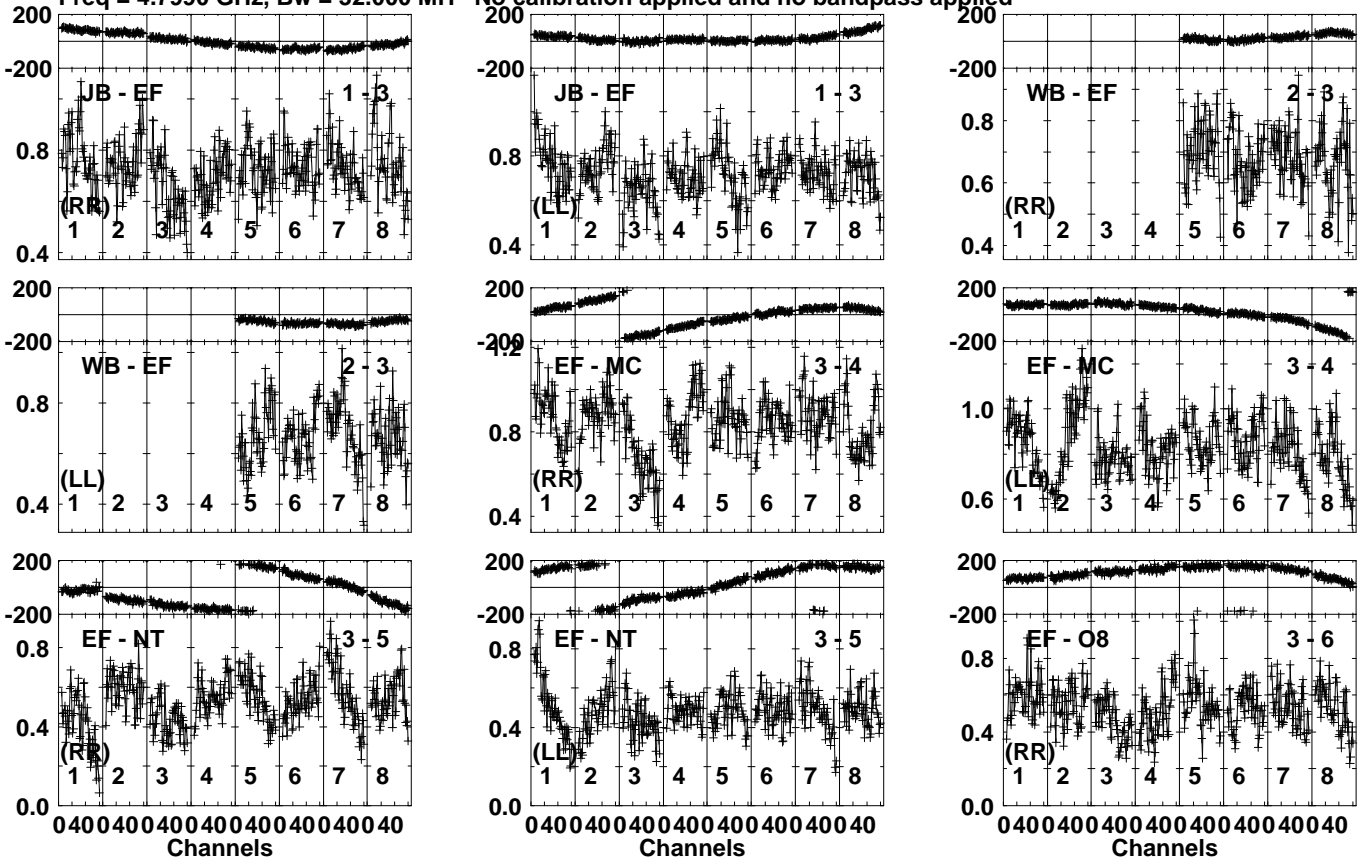
Lower frame: Milli Ampl Jy Top frame: Phas deg Vector averaged cross-power spectrum Several baselines displayed Timerange: 00/17:14:31 to 00/17:16:29
