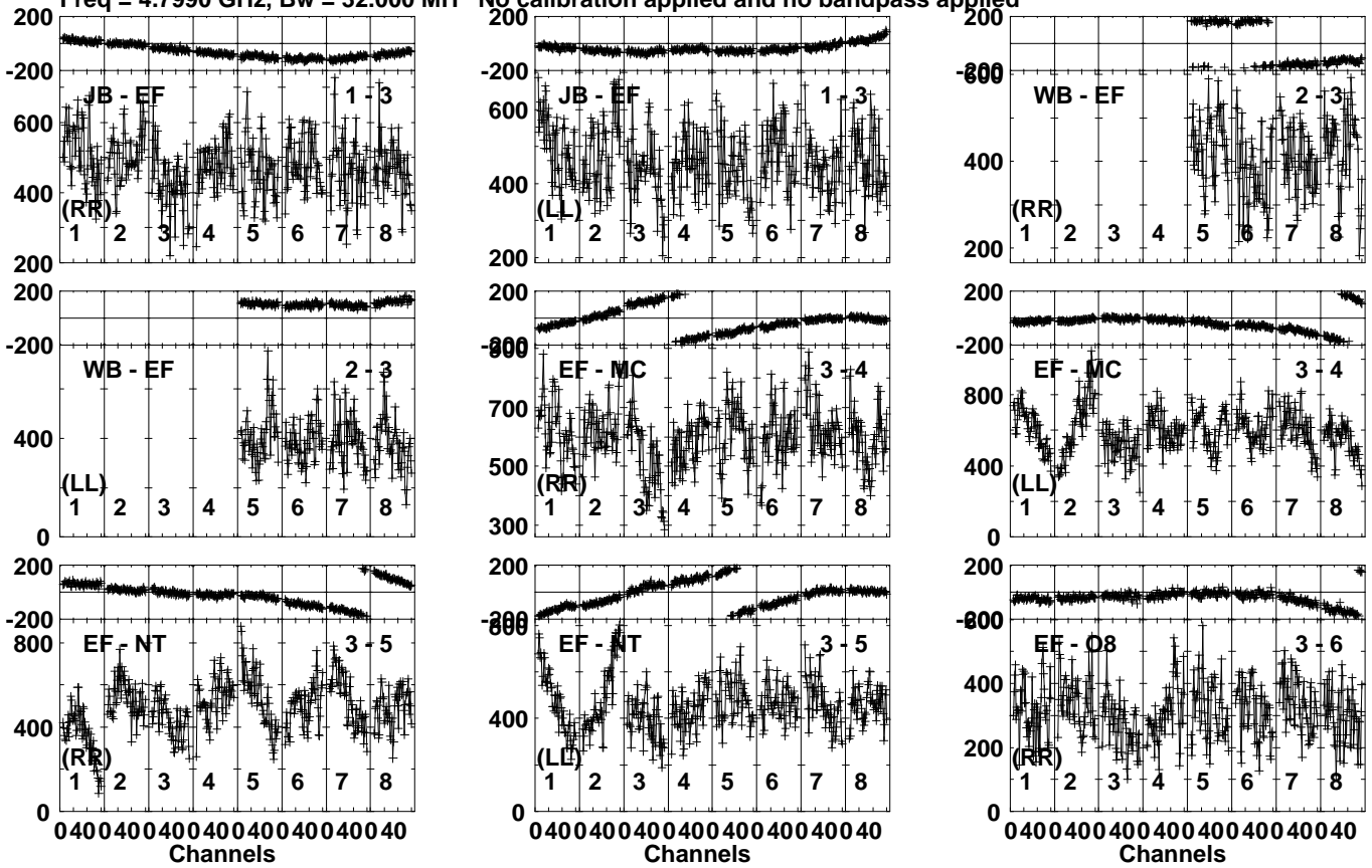
Lower frame: Micro Ampl Jy Top frame: Phas deg Vector averaged cross-power spectrum Several baselines displayed Timerange: 00/17:48:03 to 00/17:50:59
