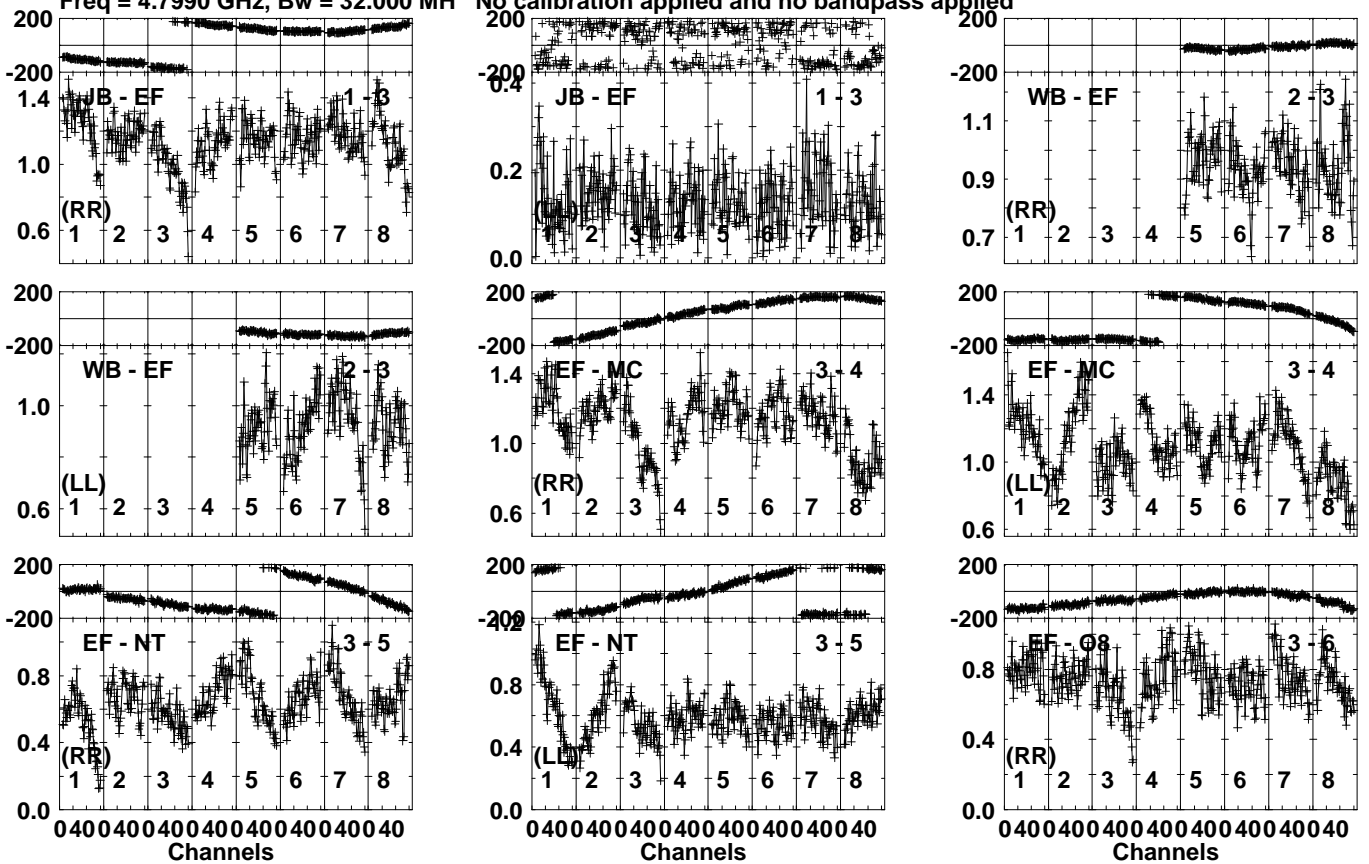
Lower frame: Milli Ampl Jy Top frame: Phas deg Vector averaged cross-power spectrum Several baselines displayed Timerange: 00/19:53:31 to 00/19:55:29
