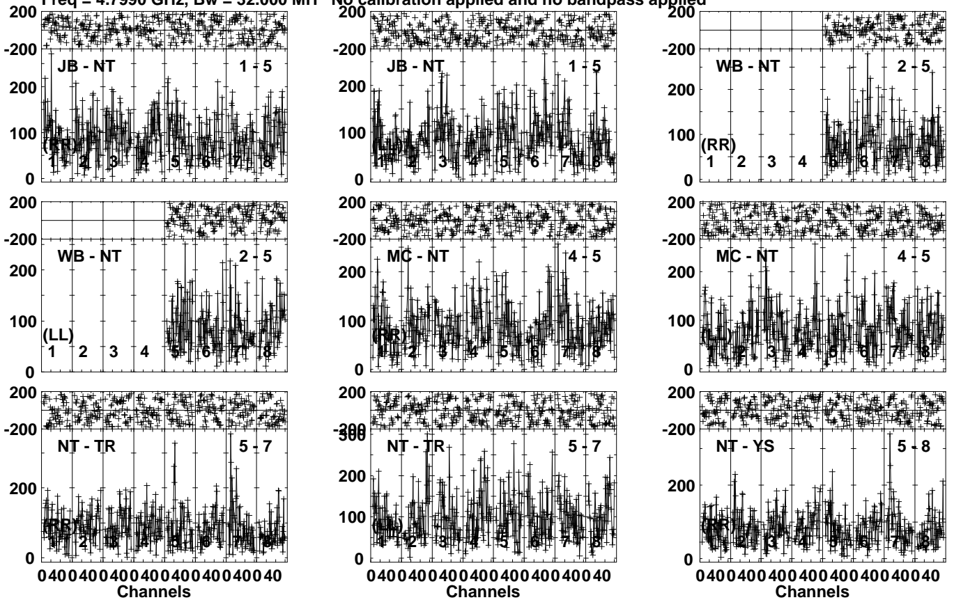
Lower frame: Micro Ampl Jy Top frame: Phas deg Vector averaged cross-power spectrum Several baselines displayed Timerange: 00/04:24:01 to 00/04:26:59
