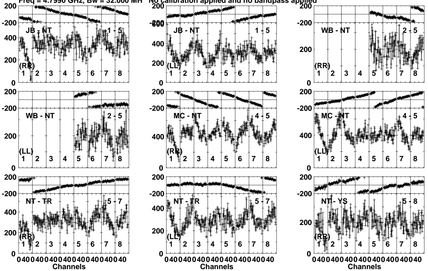
Lower frame: Micro Ampl Jy Top frame: Phas deg Vector averaged cross-power spectrum Several baselines displayed Timerange: 00/02:06:01 to 00/02:10:59
