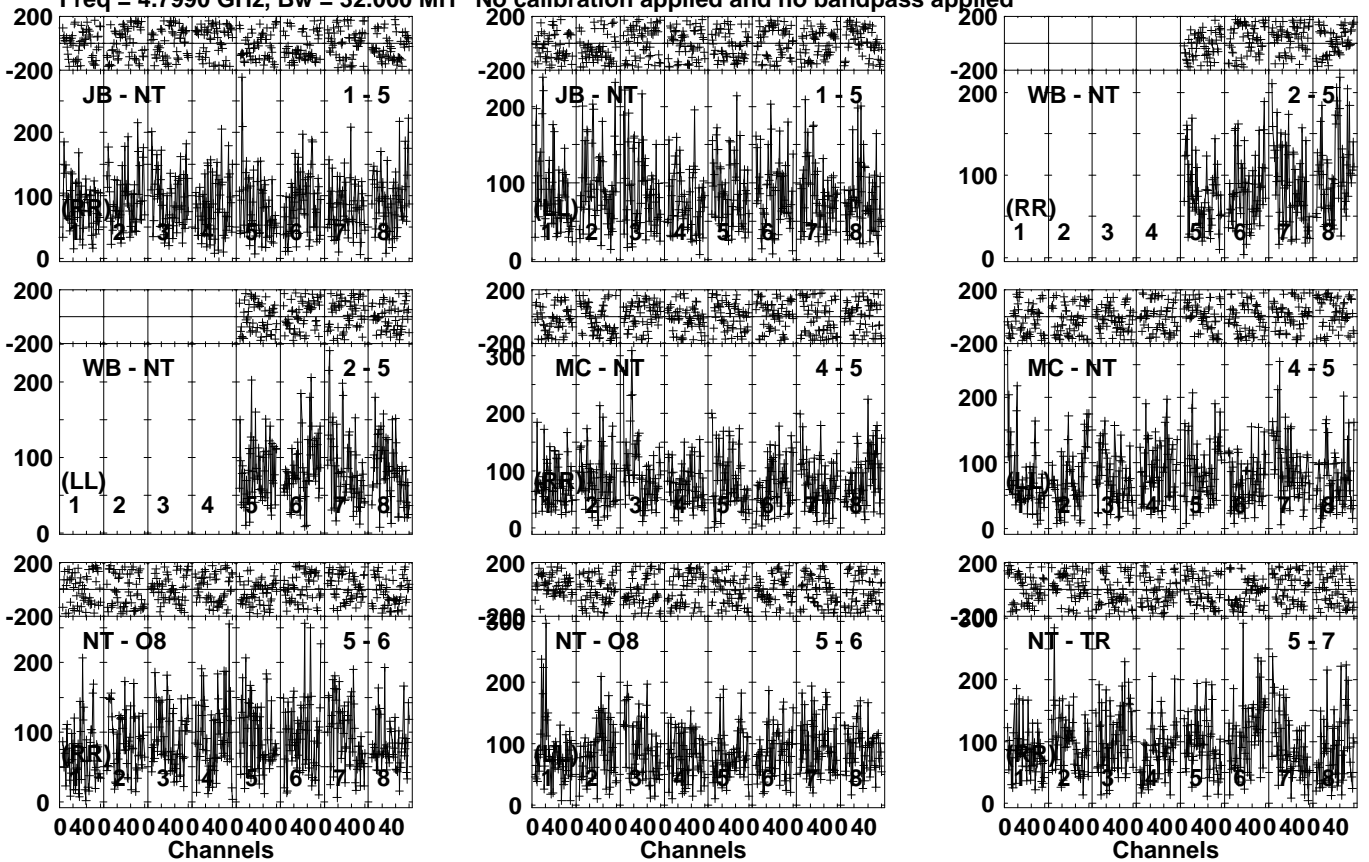
Lower frame: Micro Ampl Jy Top frame: Phas deg Vector averaged cross-power spectrum Several baselines displayed Timerange: 00/05:27:03 to 00/05:29:59
