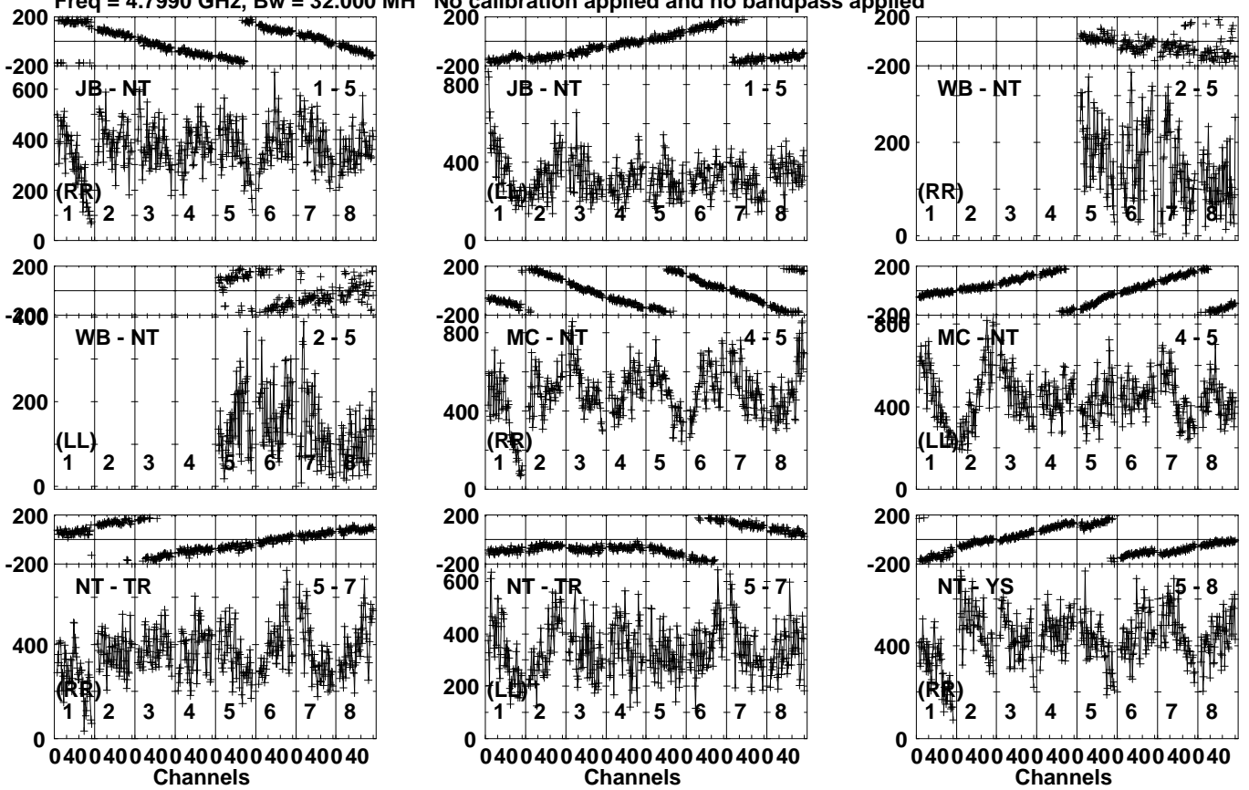
Lower frame: Micro Ampl Jy Top frame: Phas deg Vector averaged cross-power spectrum Several baselines displayed Timerange: 00/04:22:01 to 00/04:23:59
