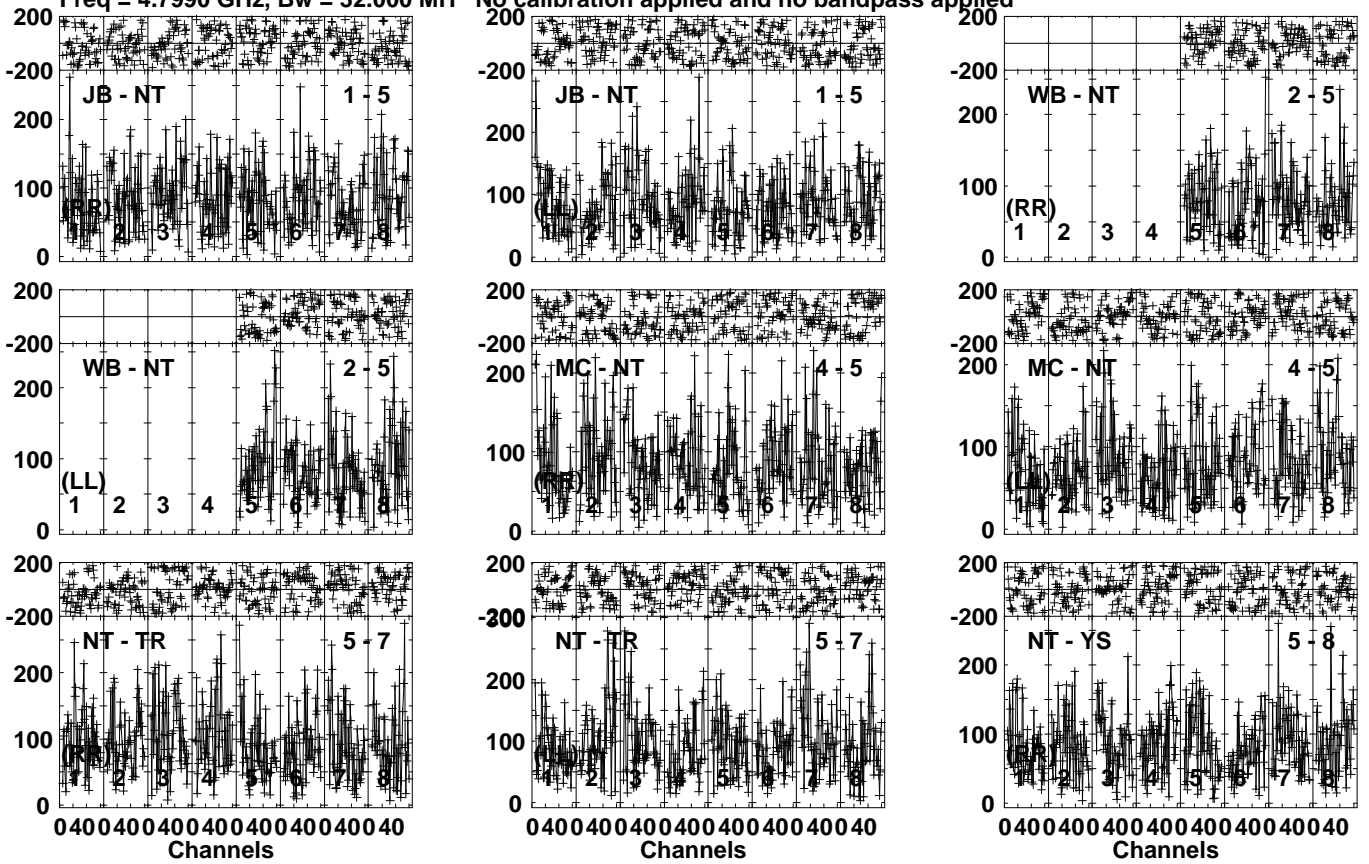
Lower frame: Micro Ampl Jy Top frame: Phas deg Vector averaged cross-power spectrum Several baselines displayed Timerange: 00/04:08:01 to 00/04:10:59
