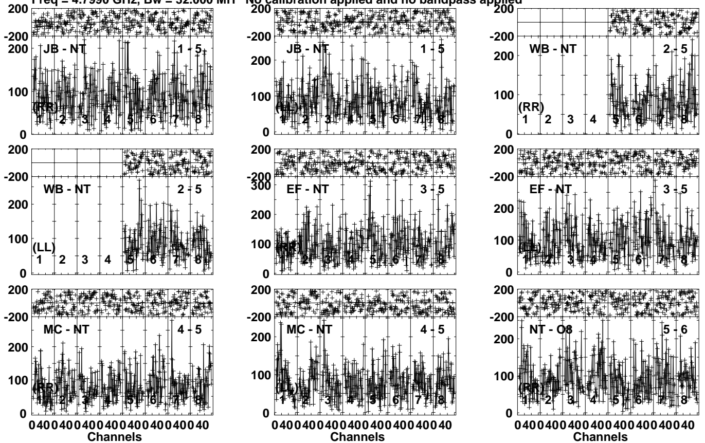
Lower frame: Micro Ampl Jy Top frame: Phas deg Vector averaged cross-power spectrum Several baselines displayed Timerange: 00/05:37:31 to 00/05:40:29
