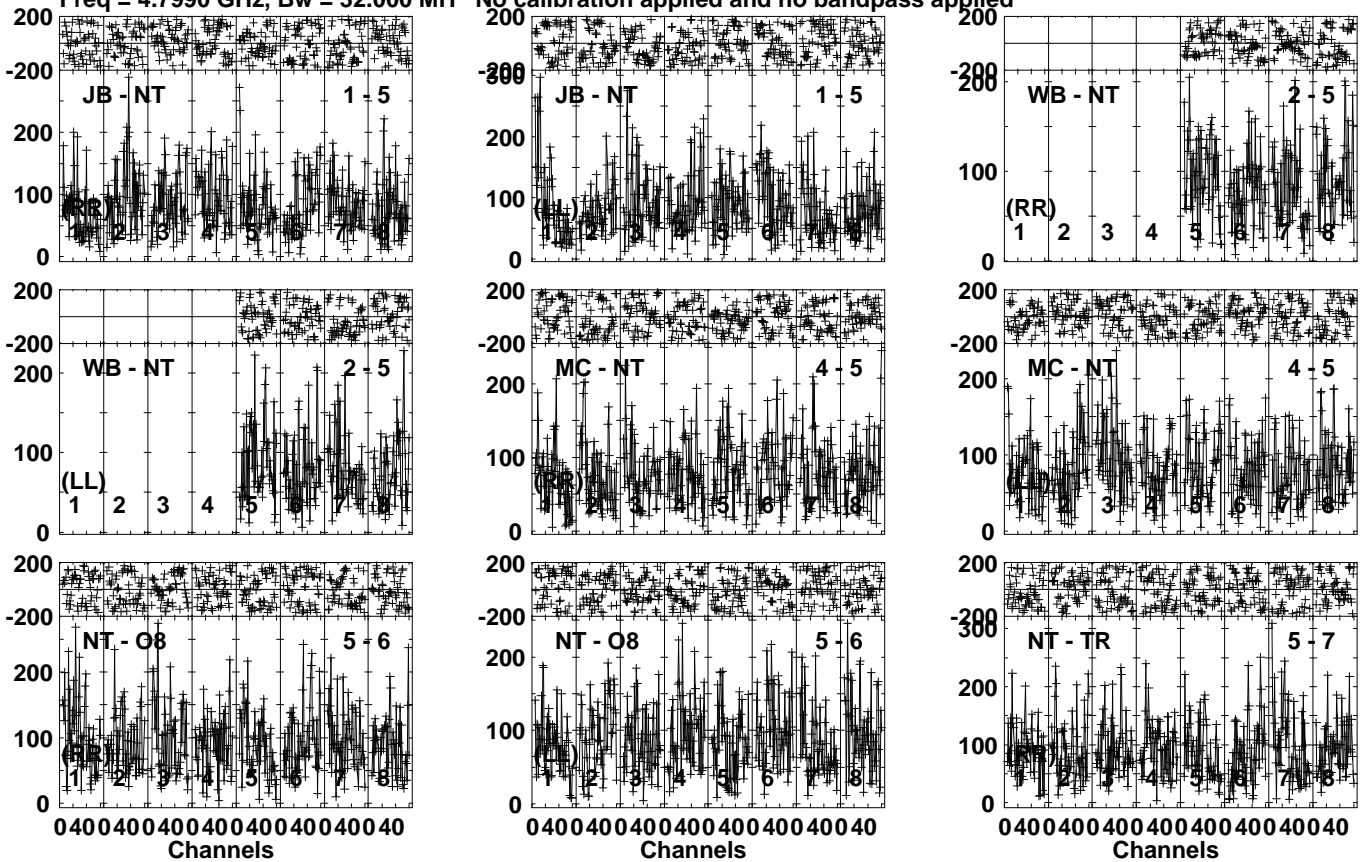
Lower frame: Micro Ampl Jy Top frame: Phas deg Vector averaged cross-power spectrum Several baselines displayed Timerange: 00/05:06:03 to 00/05:08:59
