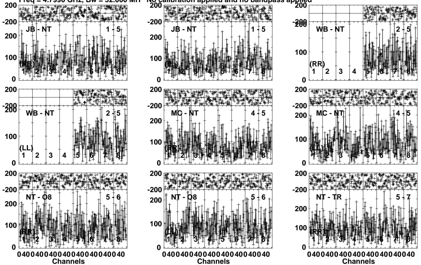
Lower frame: Micro Ampl Jy Top frame: Phas deg Vector averaged cross-power spectrum Several baselines displayed Timerange: 00/04:39:31 to 00/04:42:29
