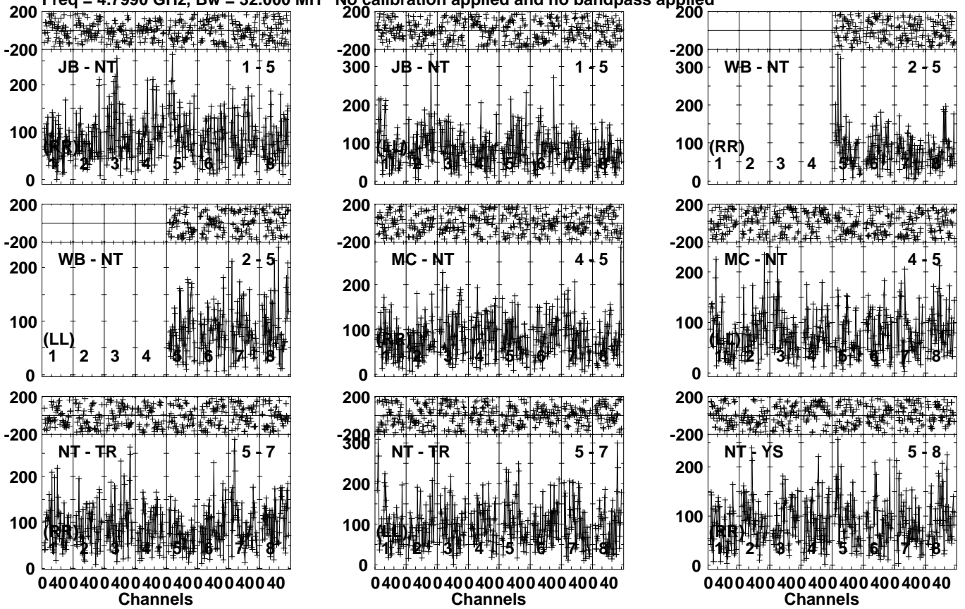
Lower frame: Micro Ampl Jy Top frame: Phas deg Vector averaged cross-power spectrum Several baselines displayed Timerange: 00/04:13:33 to 00/04:16:29
