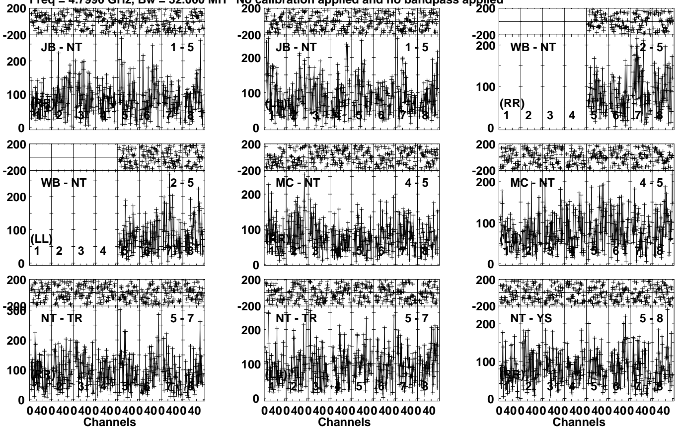
Lower frame: Micro Ampl Jy Top frame: Phas deg Vector averaged cross-power spectrum Several baselines displayed Timerange: 00/02:48:01 to 00/02:50:59
