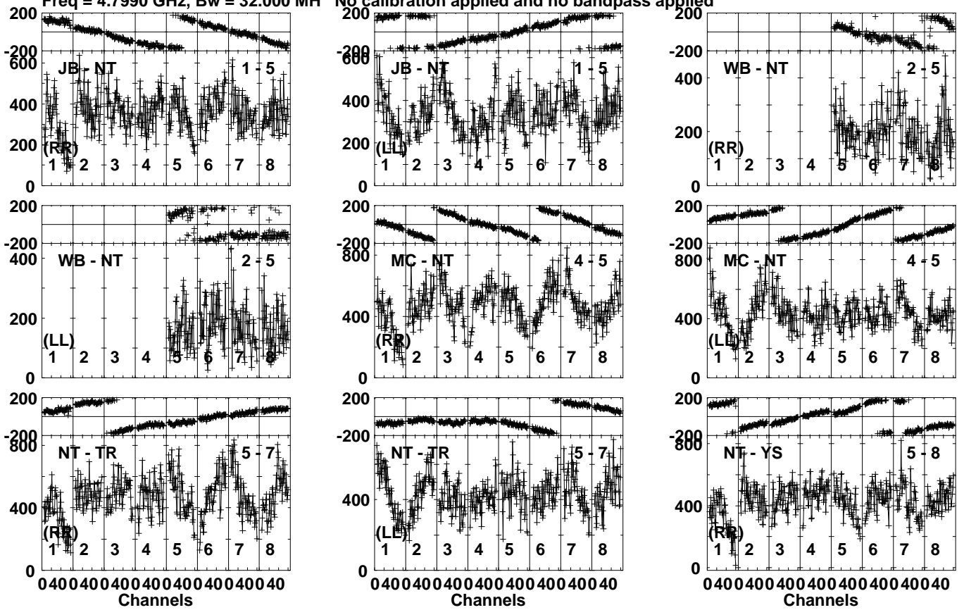
Lower frame: Micro Ampl Jy Top frame: Phas deg Vector averaged cross-power spectrum Several baselines displayed Timerange: 00/03:28:01 to 00/03:29:59
