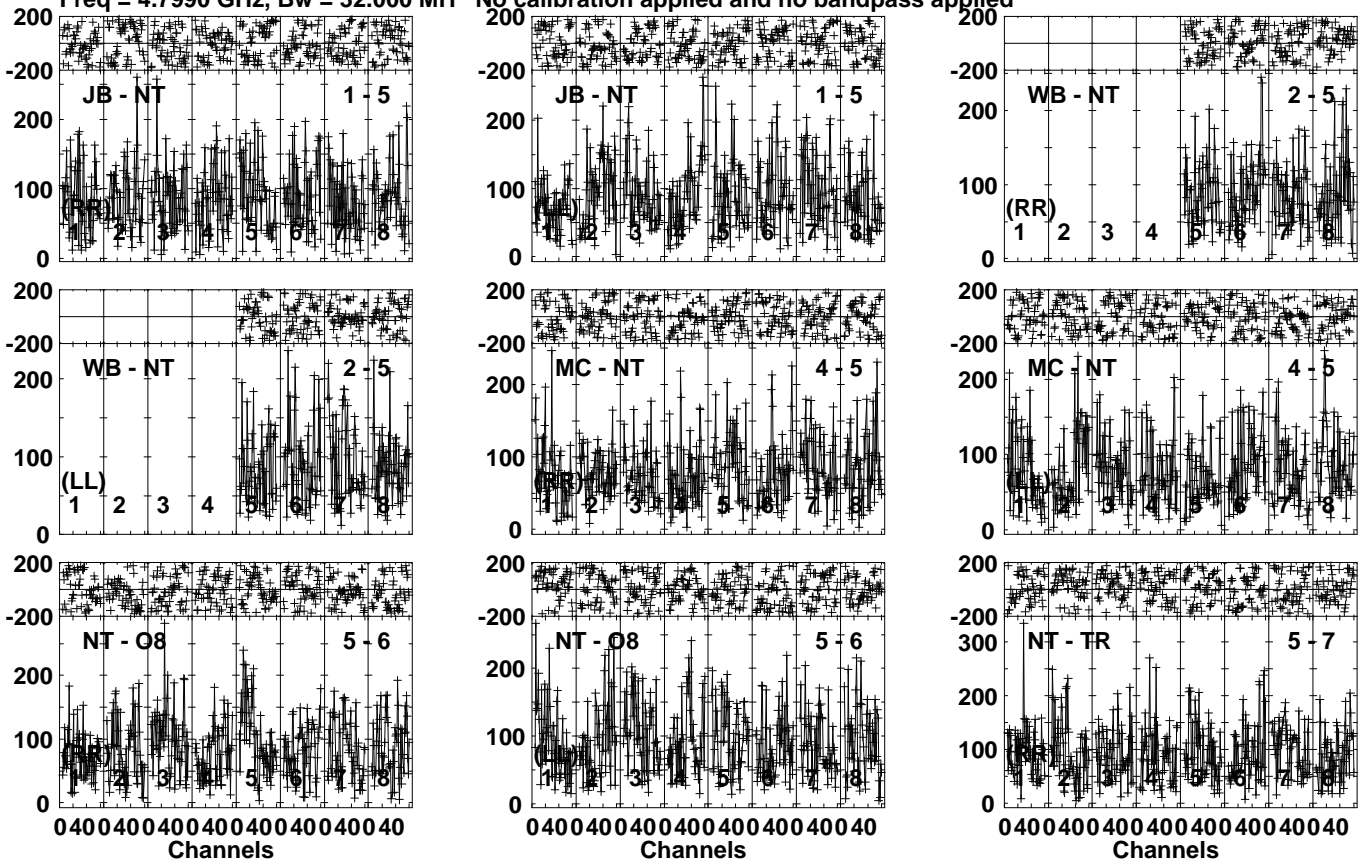
Lower frame: Micro Ampl Jy Top frame: Phas deg Vector averaged cross-power spectrum Several baselines displayed Timerange: 00/04:34:31 to 00/04:37:29
