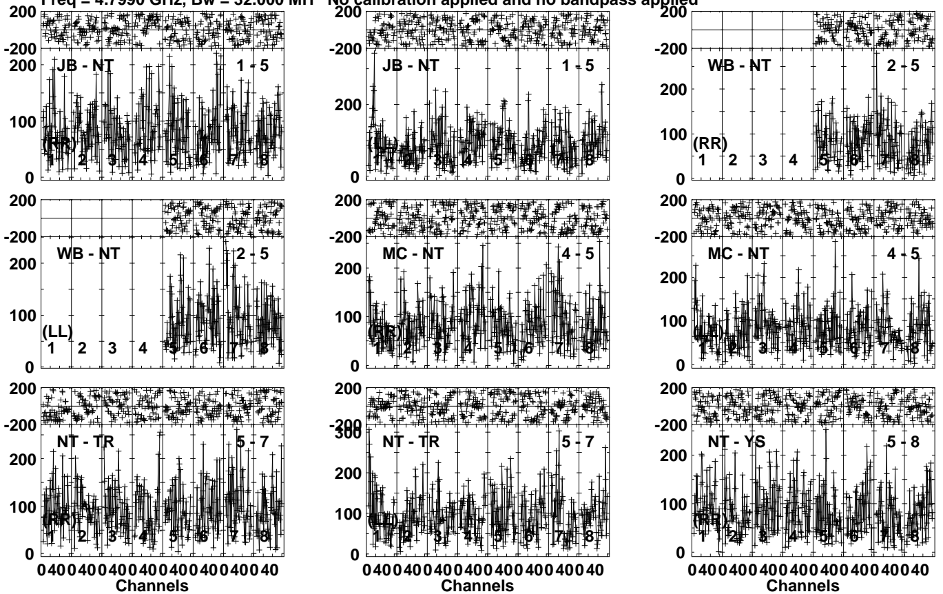
Lower frame: Micro Ampl Jy Top frame: Phas deg Vector averaged cross-power spectrum Several baselines displayed Timerange: 00/02:11:01 to 00/02:13:59
