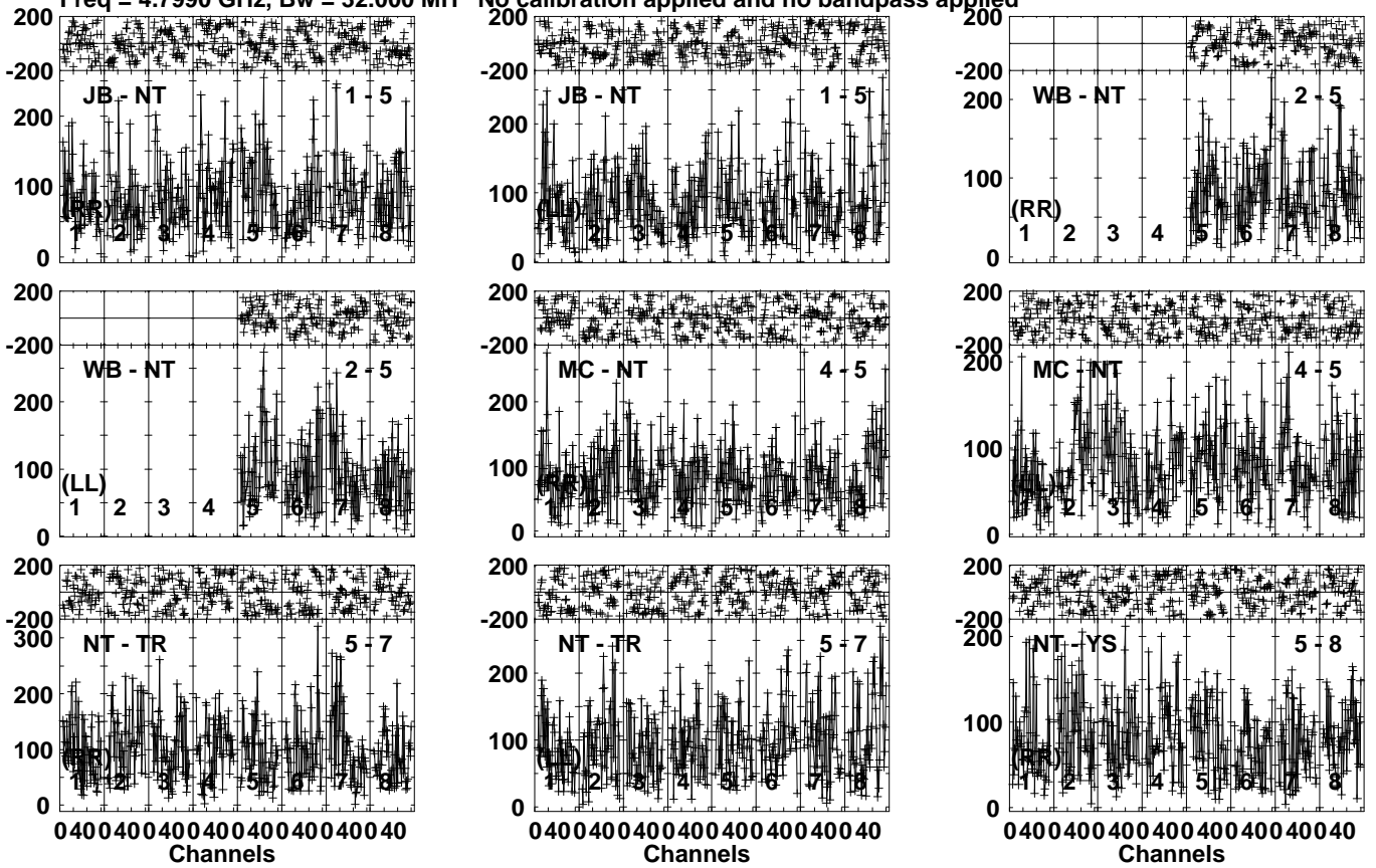
Lower frame: Micro Ampl Jy Top frame: Phas deg Vector averaged cross-power spectrum Several baselines displayed Timerange: 00/02:42:31 to 00/02:45:29
