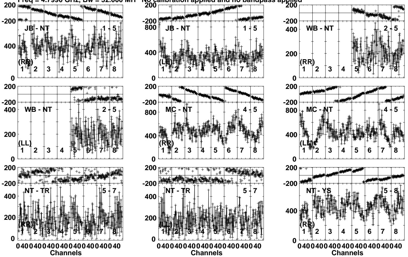
Lower frame: Micro Ampl Jy Top frame: Phas deg Vector averaged cross-power spectrum Several baselines displayed Timerange: 00/03:54:01 to 00/03:55:59
