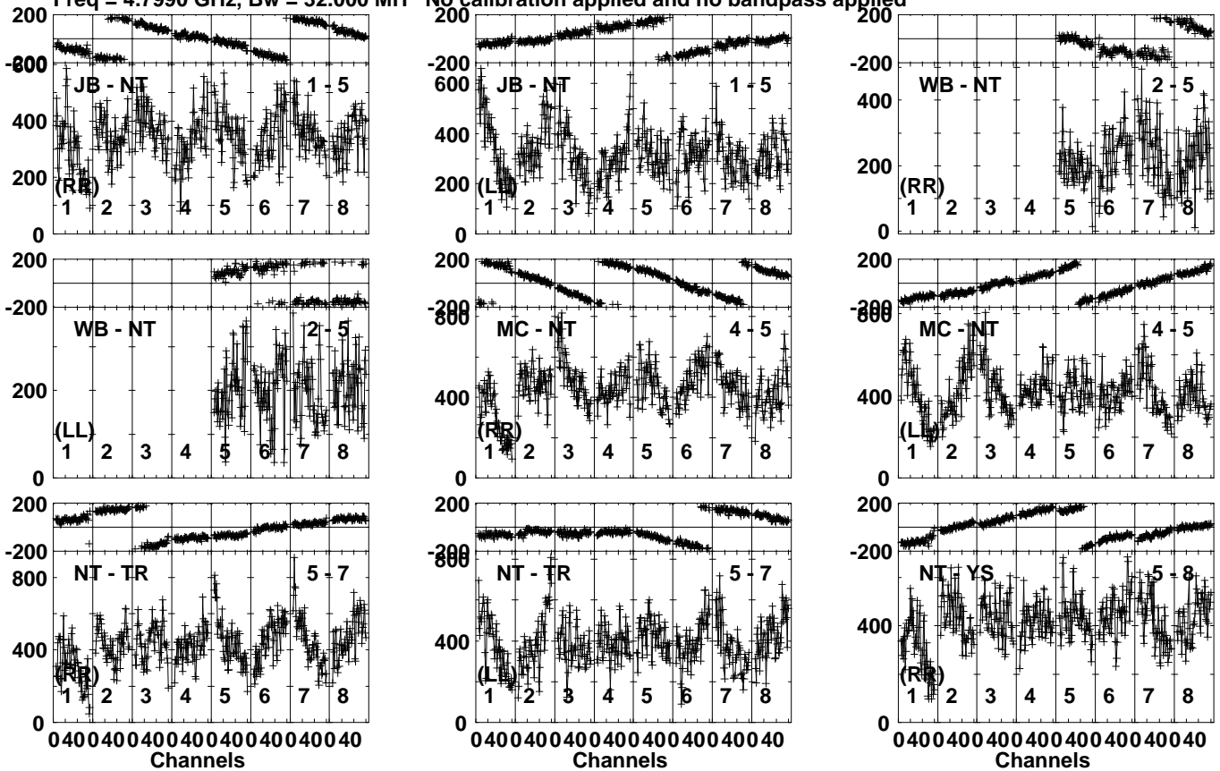
Lower frame: Micro Ampl Jy Top frame: Phas deg Vector averaged cross-power spectrum Several baselines displayed Timerange: 00/02:14:31 to 00/02:16:29
