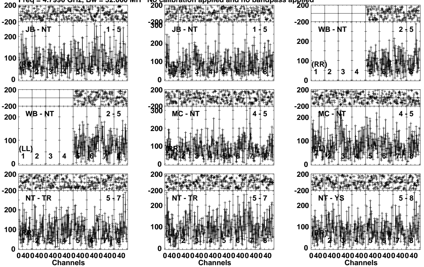
Lower frame: Micro Ampl Jy Top frame: Phas deg Vector averaged cross-power spectrum Several baselines displayed Timerange: 00/02:58:33 to 00/03:01:29
