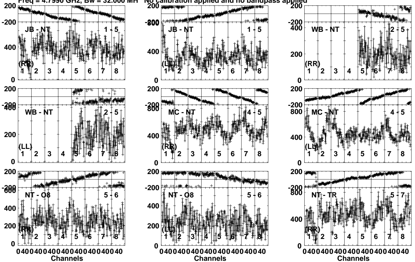
Lower frame: Micro Ampl Jy Top frame: Phas deg Vector averaged cross-power spectrum Several baselines displayed Timerange: 00/04:37:31 to 00/04:39:29
