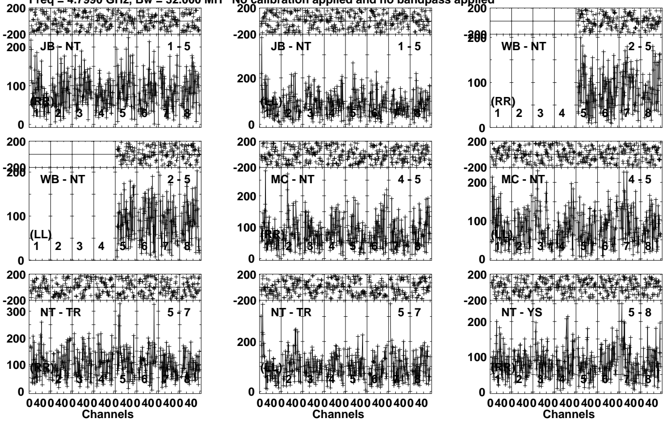
Lower frame: Micro Ampl Jy Top frame: Phas deg Vector averaged cross-power spectrum Several baselines displayed Timerange: 00/02:53:01 to 00/02:55:59
