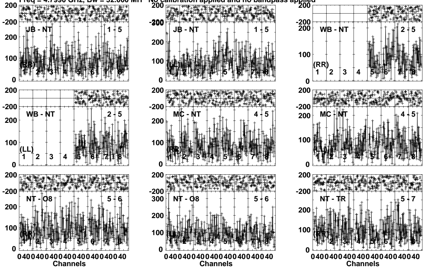
Lower frame: Micro Ampl Jy Top frame: Phas deg Vector averaged cross-power spectrum Several baselines displayed Timerange: 00/05:16:31 to 00/05:19:29
