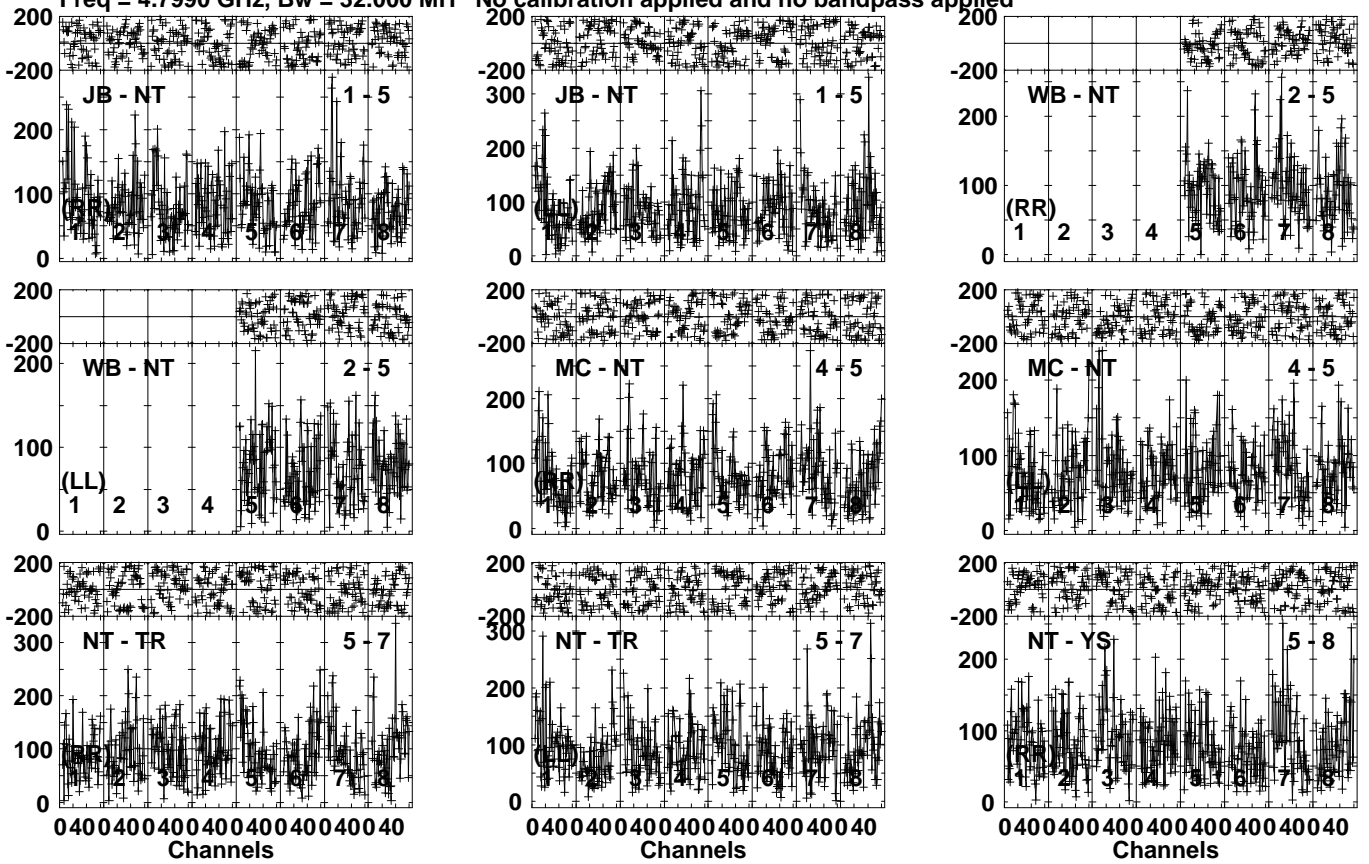
Lower frame: Micro Ampl Jy Top frame: Phas deg Vector averaged cross-power spectrum Several baselines displayed Timerange: 00/03:45:31 to 00/03:48:29
