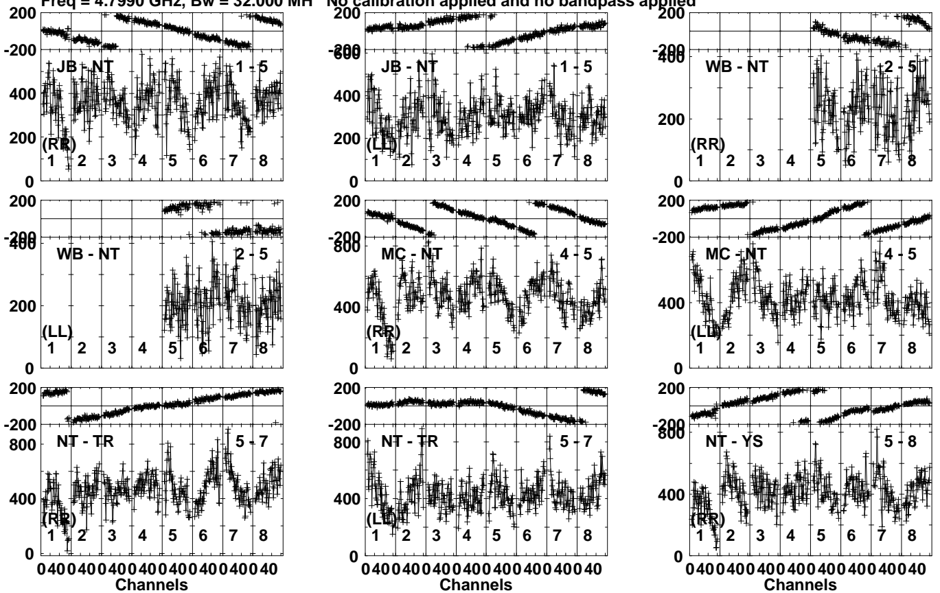
Lower frame: Micro Ampl Jy Top frame: Phas deg Vector averaged cross-power spectrum Several baselines displayed Timerange: 00/02:56:31 to 00/02:58:29
