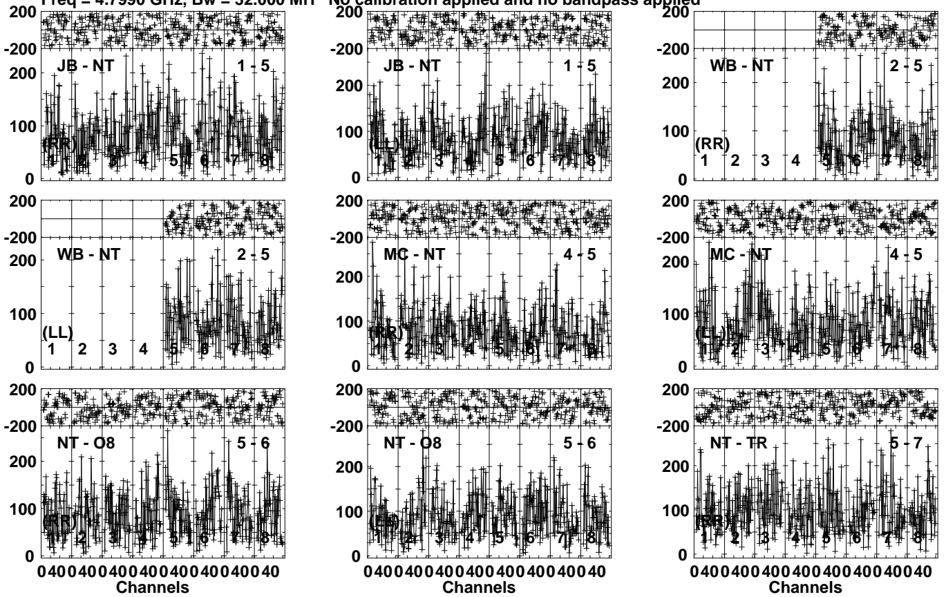
Lower frame: Micro Ampl Jy Top frame: Phas deg Vector averaged cross-power spectrum Several baselines displayed Timerange: 00/05:32:01 to 00/05:34:59
