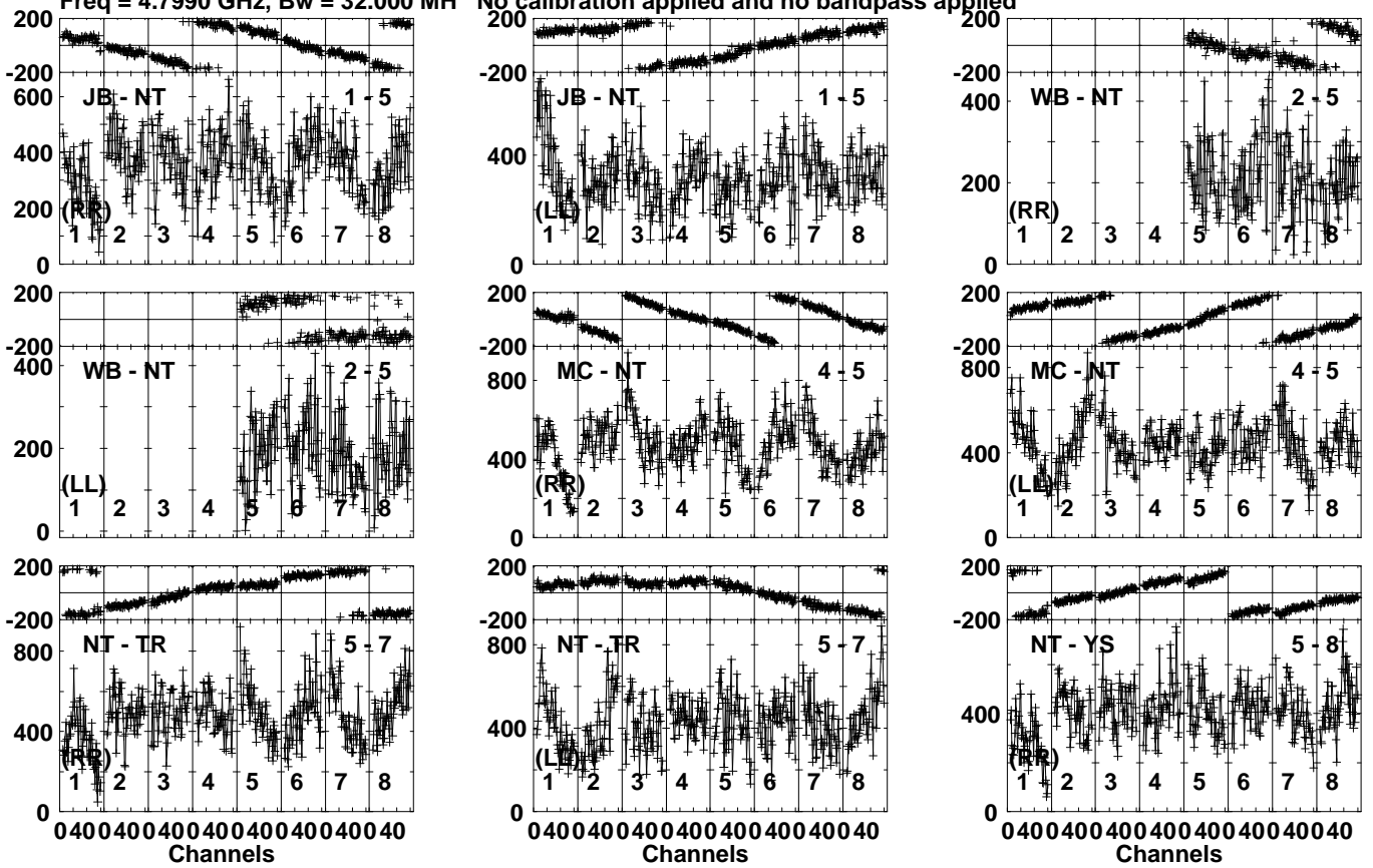
Lower frame: Micro Ampl Jy Top frame: Phas deg Vector averaged cross-power spectrum Several baselines displayed Timerange: 00/03:12:01 to 00/03:13:59
