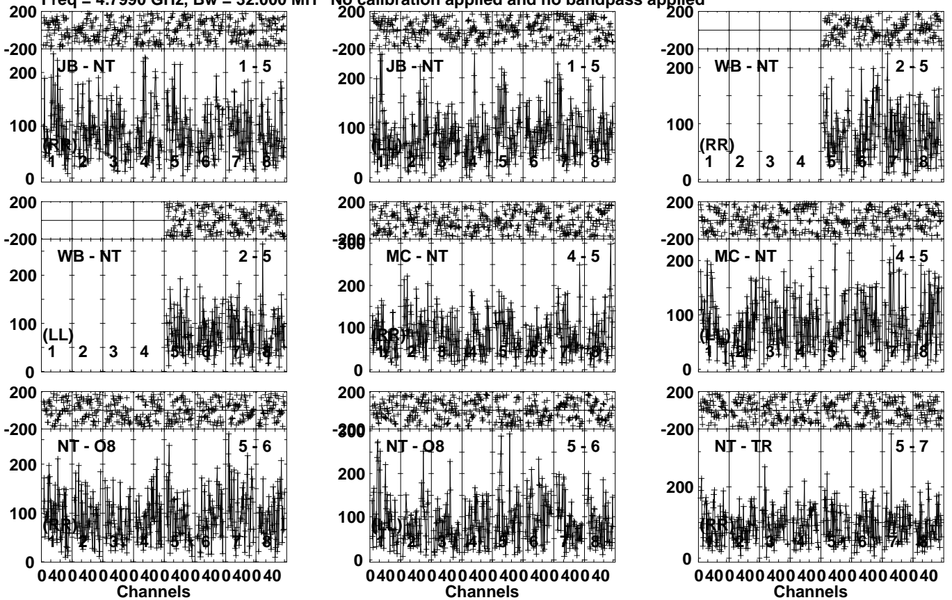
Lower frame: Micro Ampl Jy Top frame: Phas deg Vector averaged cross-power spectrum Several baselines displayed Timerange: 00/05:11:01 to 00/05:13:59
