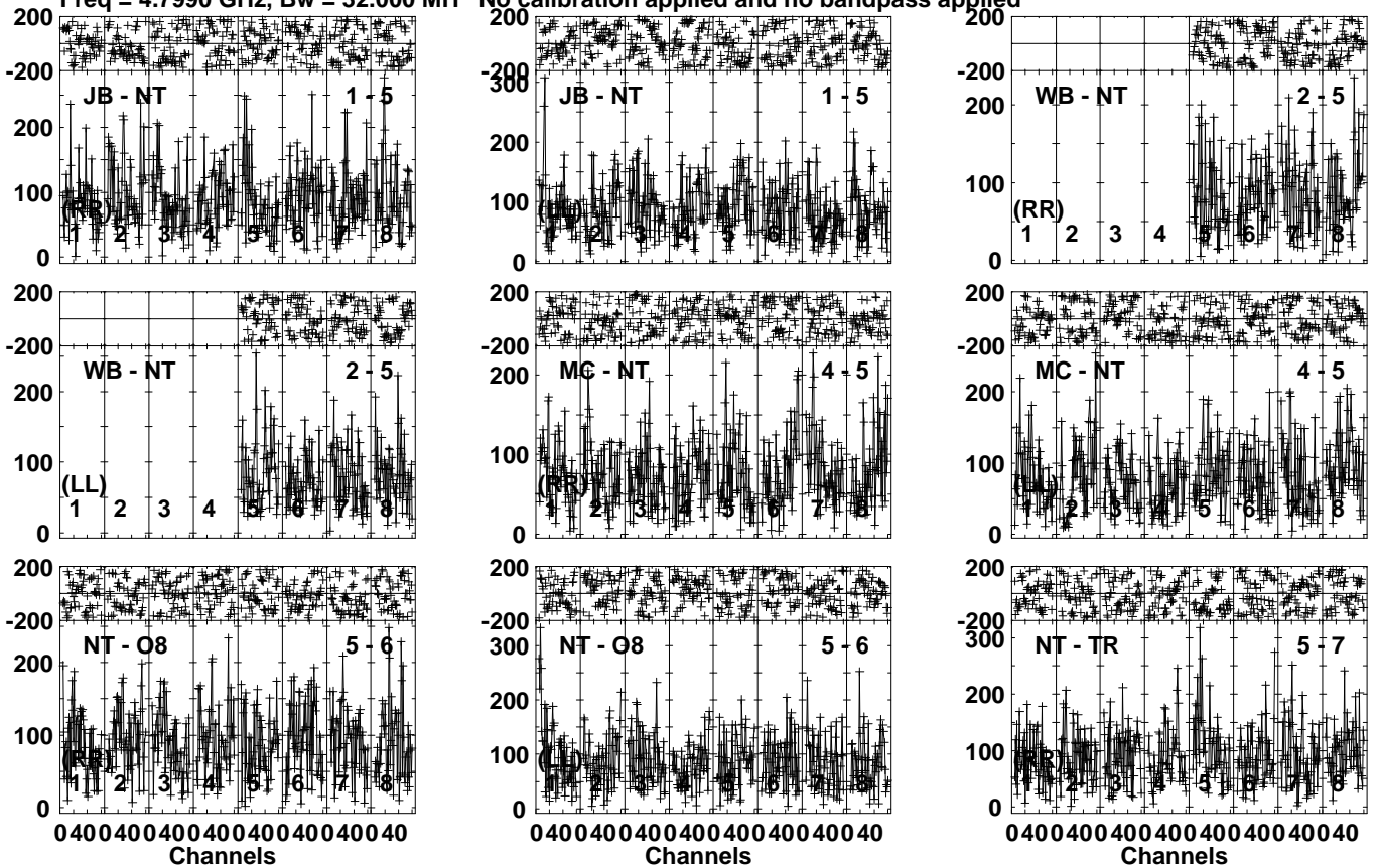
Lower frame: Micro Ampl Jy Top frame: Phas deg Vector averaged cross-power spectrum Several baselines displayed Timerange: 00/04:45:03 to 00/04:47:59
