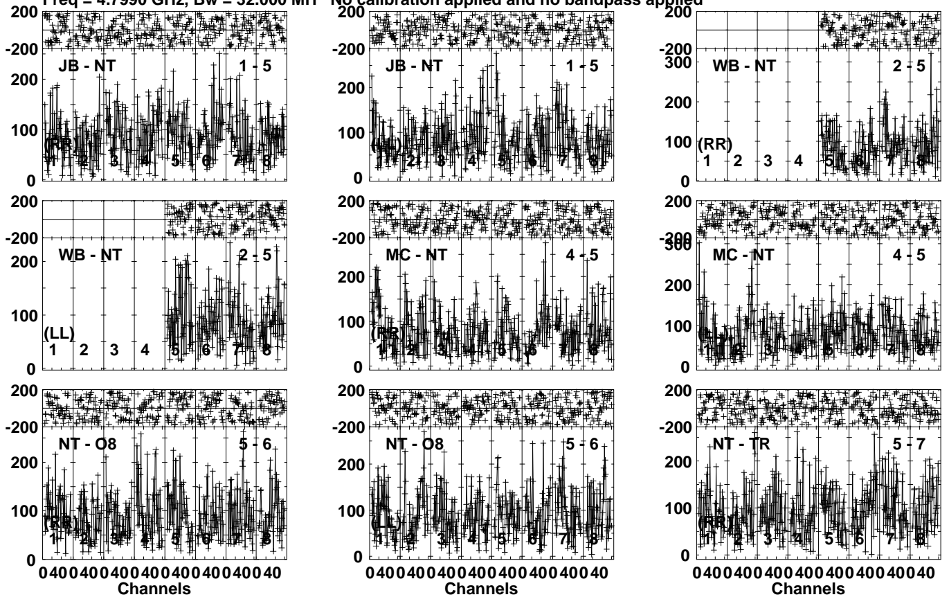
Lower frame: Micro Ampl Jy Top frame: Phas deg Vector averaged cross-power spectrum Several baselines displayed Timerange: 00/05:00:31 to 00/05:03:29
