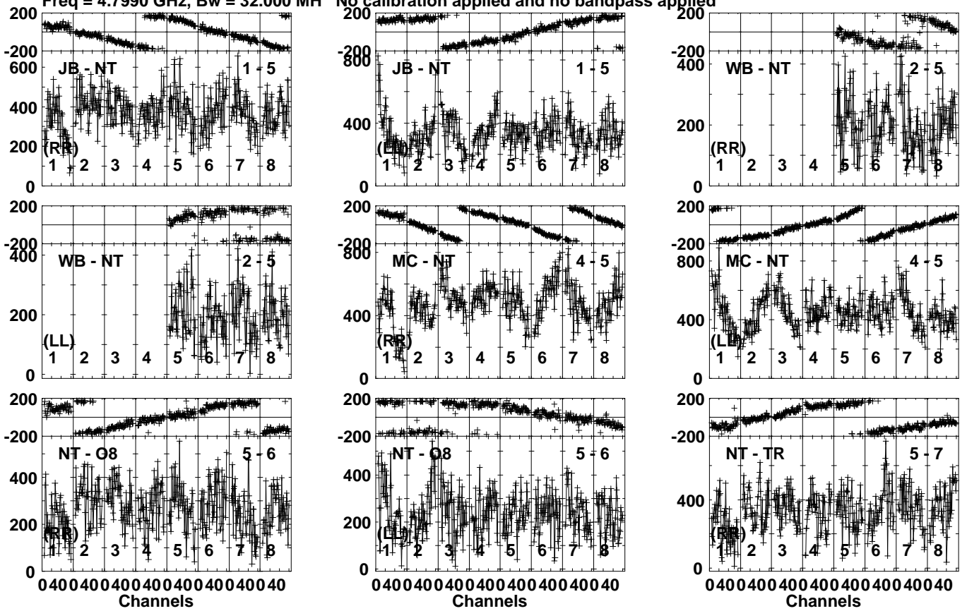
Lower frame: Micro Ampl Jy Top frame: Phas deg Vector averaged cross-power spectrum Several baselines displayed Timerange: 00/04:58:31 to 00/05:00:29
