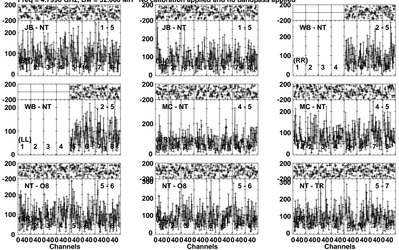
Lower frame: Micro Ampl Jy Top frame: Phas deg Vector averaged cross-power spectrum Several baselines displayed Timerange: 00/04:55:33 to 00/04:58:29
