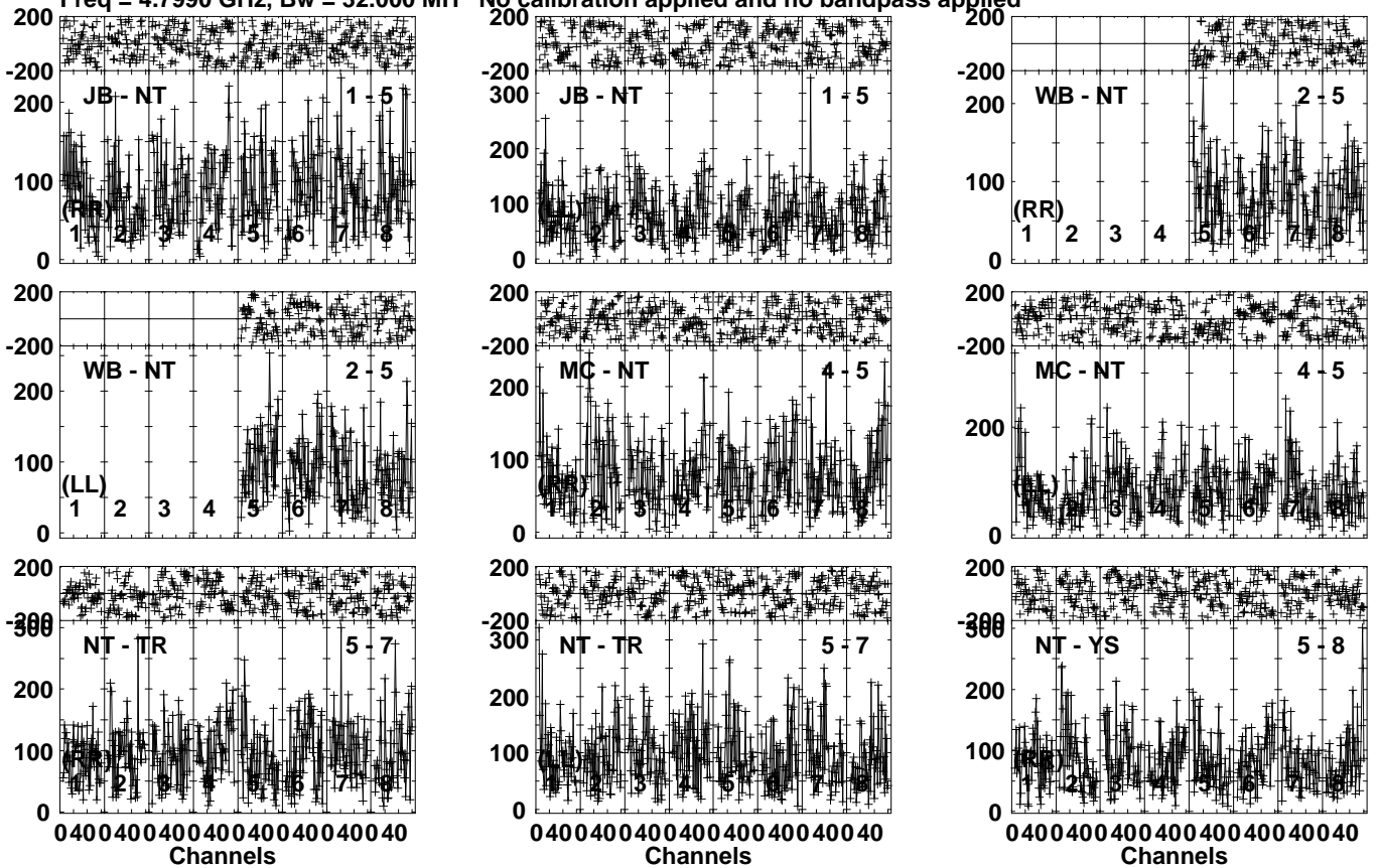
Lower frame: Micro Ampl Jy Top frame: Phas deg Vector averaged cross-power spectrum Several baselines displayed Timerange: 00/03:35:01 to 00/03:37:59
