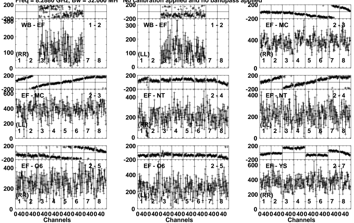
Lower frame: Micro Ampl Jy Top frame: Phas deg Vector averaged cross-power spectrum Several baselines displayed Timerange: 00/16:21:31 to 00/16:24:29
