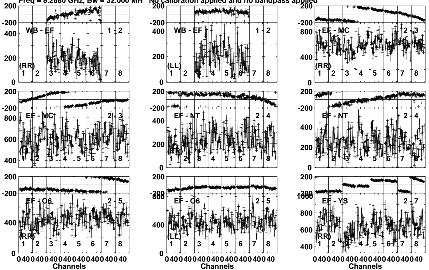
Lower frame: Micro Ampl Jy Top frame: Phas deg Vector averaged cross-power spectrum Several baselines displayed Timerange: 00/16:25:01 to 00/16:26:59
