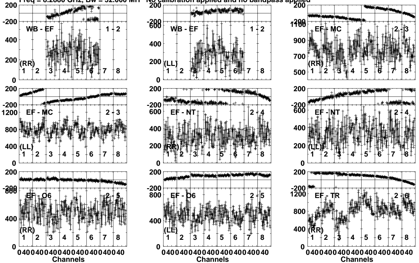
Lower frame: Micro Ampl Jy Top frame: Phas deg Vector averaged cross-power spectrum Several baselines displayed Timerange: 00/19:39:31 to 00/19:41:29
