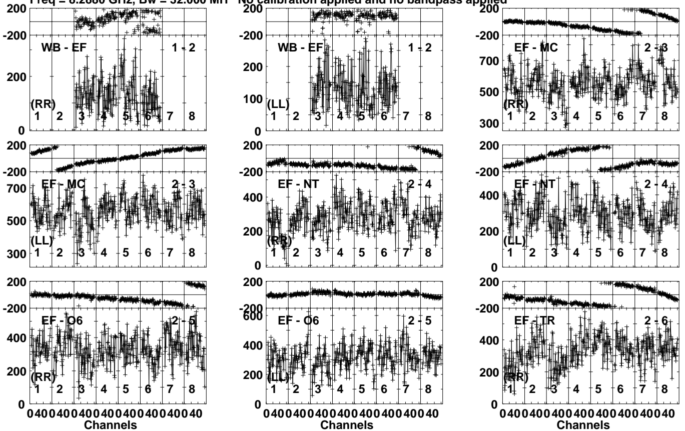
Lower frame: Micro Ampl Jy Top frame: Phas deg Vector averaged cross-power spectrum Several baselines displayed Timerange: 00/18:59:31 to 00/19:02:29
