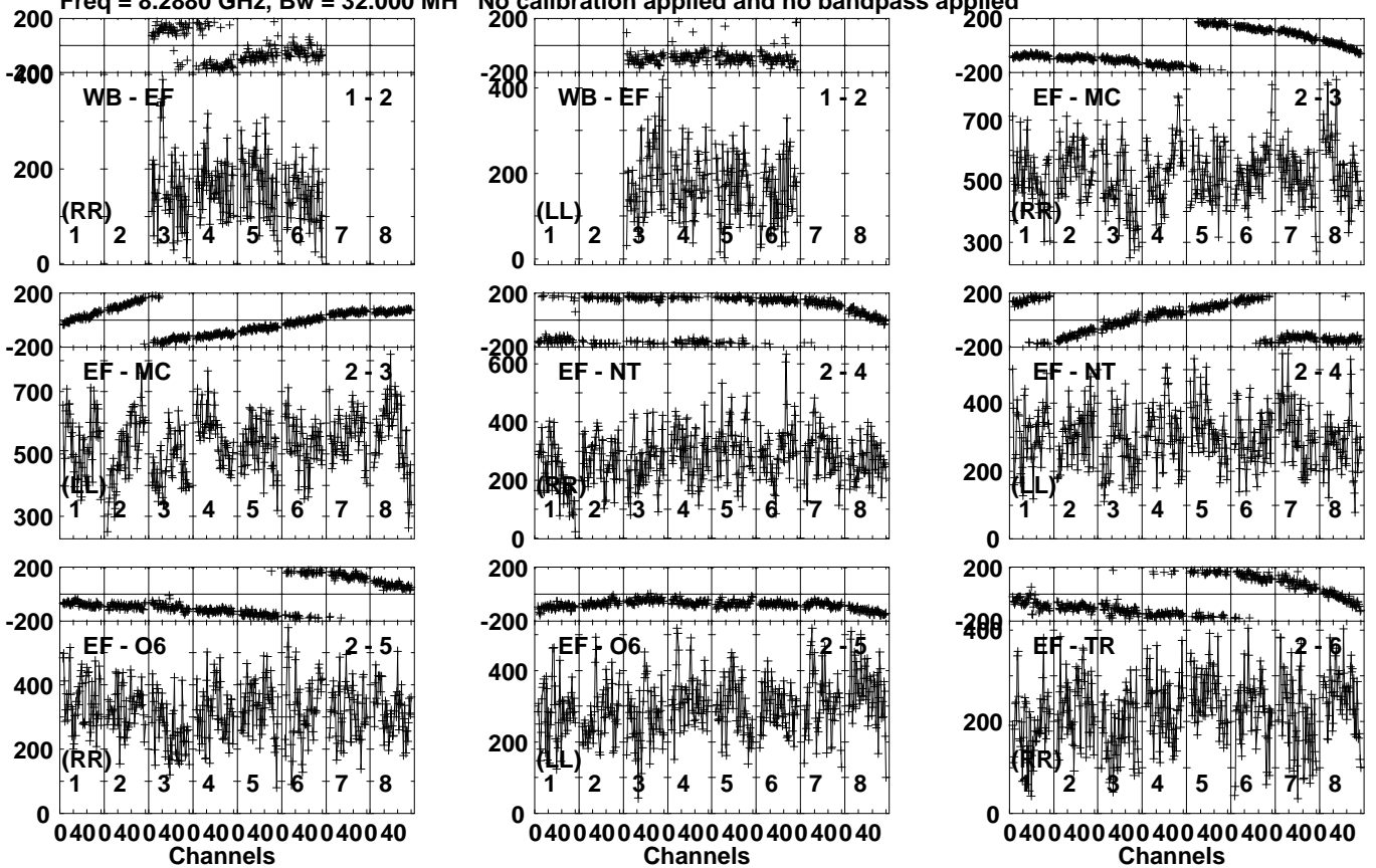
Lower frame: Micro Ampl Jy Top frame: Phas deg Vector averaged cross-power spectrum Several baselines displayed Timerange: 00/18:12:33 to 00/18:15:29
