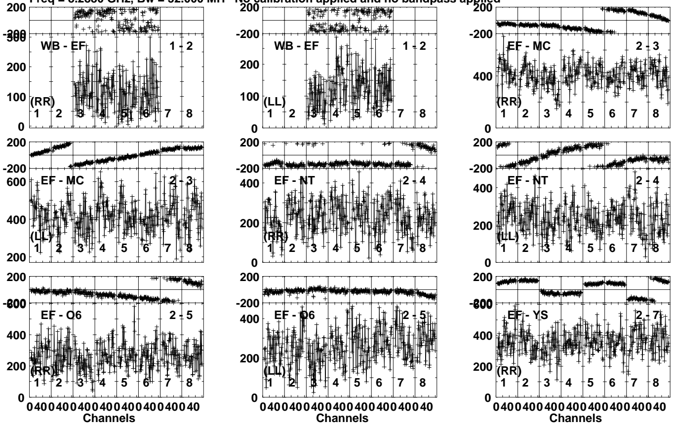
Lower frame: Micro Ampl Jy Top frame: Phas deg Vector averaged cross-power spectrum Several baselines displayed Timerange: 00/16:32:01 to 00/16:34:59
