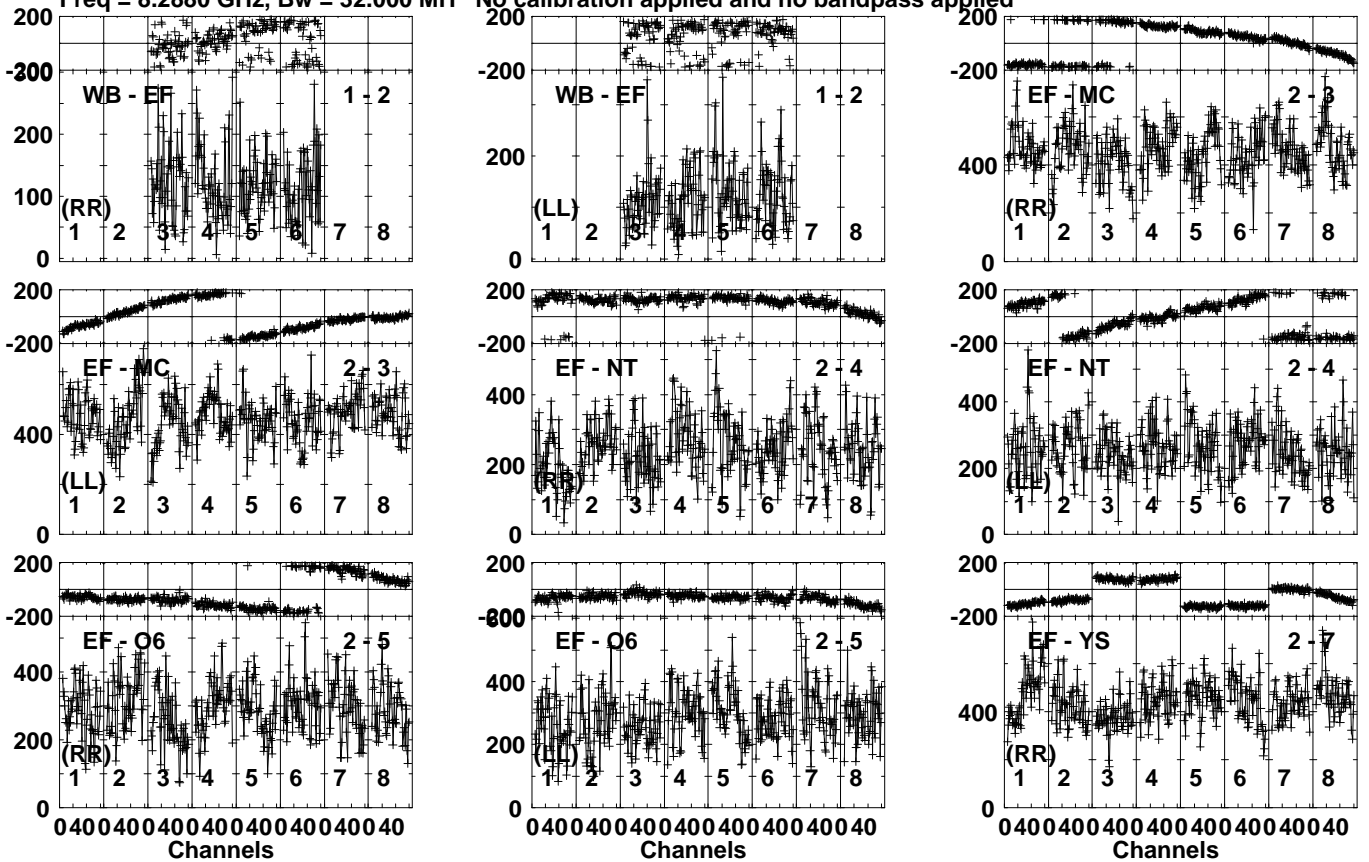
Lower frame: Micro Ampl Jy Top frame: Phas deg Vector averaged cross-power spectrum Several baselines displayed Timerange: 00/17:09:03 to 00/17:11:59
