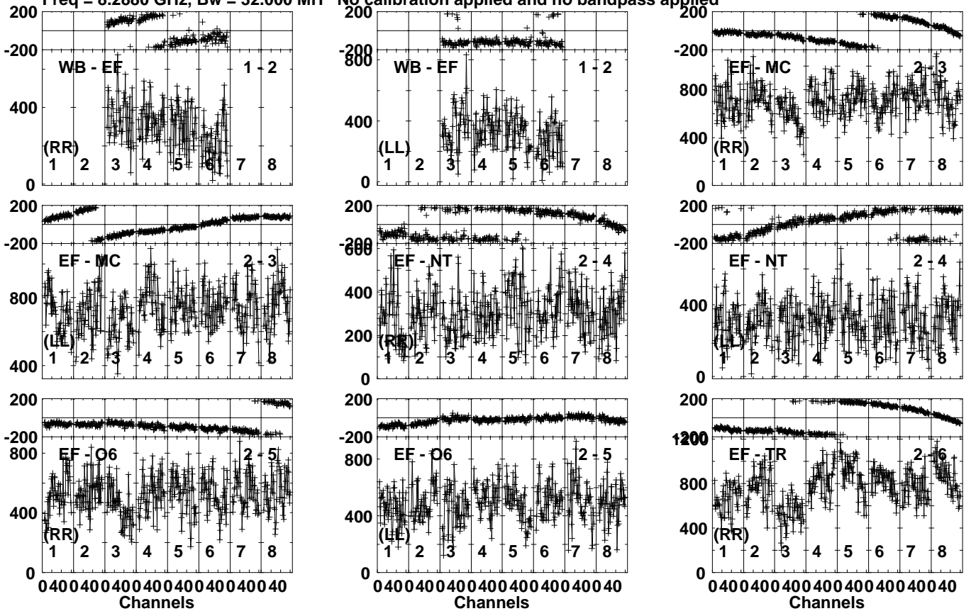
Lower frame: Micro Ampl Jy Top frame: Phas deg Vector averaged cross-power spectrum Several baselines displayed Timerange: 00/17:54:01 to 00/17:55:59
