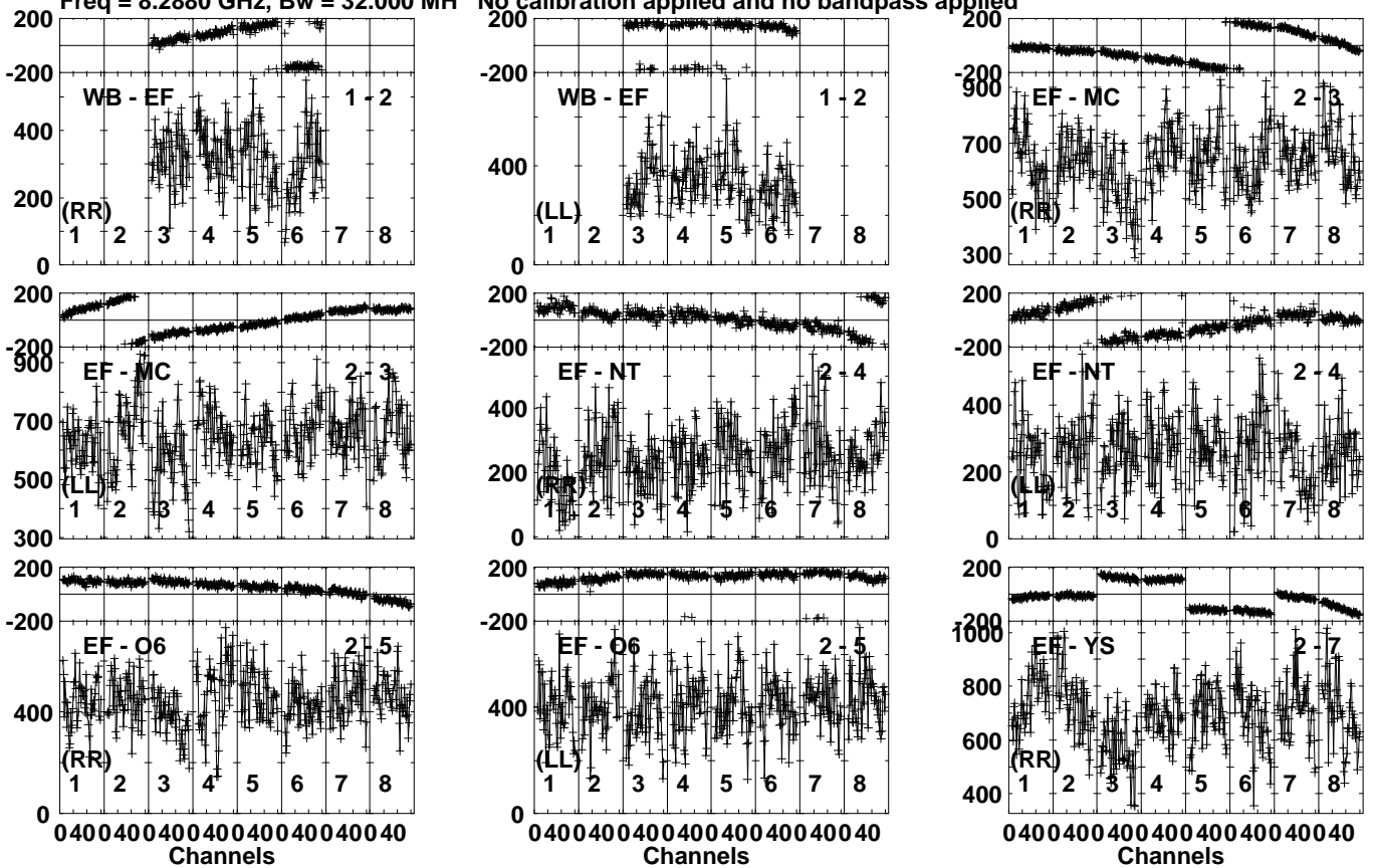
Lower frame: Micro Ampl Jy Top frame: Phas deg Vector averaged cross-power spectrum Several baselines displayed Timerange: 00/16:46:01 to 00/16:47:59
