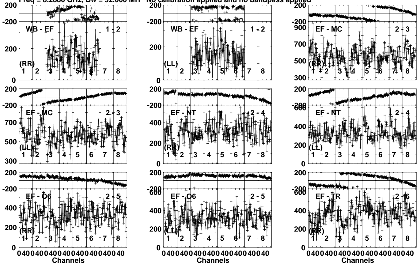
Lower frame: Micro Ampl Jy Top frame: Phas deg Vector averaged cross-power spectrum Several baselines displayed Timerange: 00/19:05:03 to 00/19:07:59
