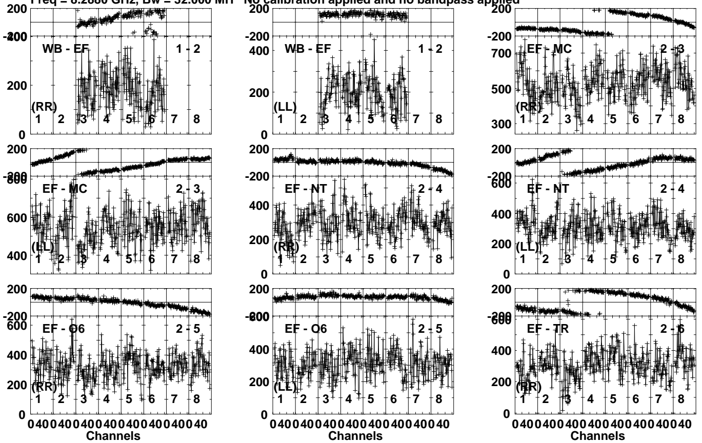
Lower frame: Micro Ampl Jy Top frame: Phas deg Vector averaged cross-power spectrum Several baselines displayed Timerange: 00/18:17:31 to 00/18:20:29
