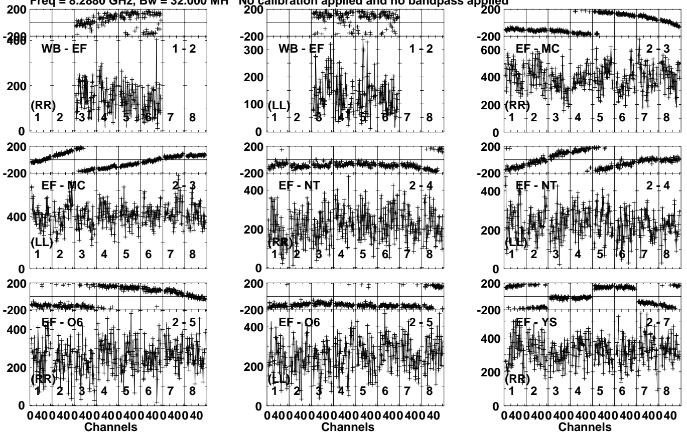
Lower frame: Micro Ampl Jy Top frame: Phas deg Vector averaged cross-power spectrum Several baselines displayed Timerange: 00/16:27:03 to 00/16:29:59
