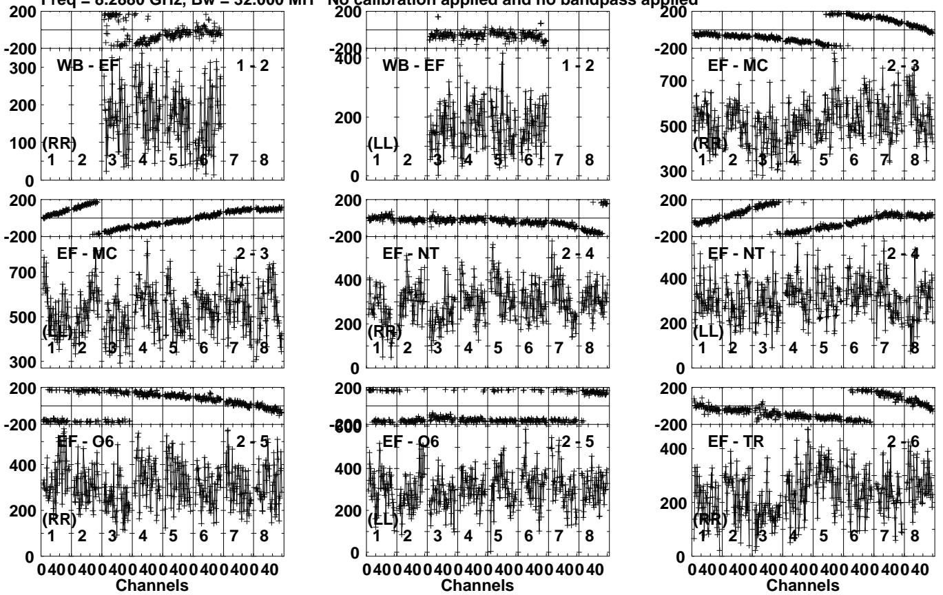
Lower frame: Micro Ampl Jy Top frame: Phas deg Vector averaged cross-power spectrum Several baselines displayed Timerange: 00/18:07:01 to 00/18:09:59
