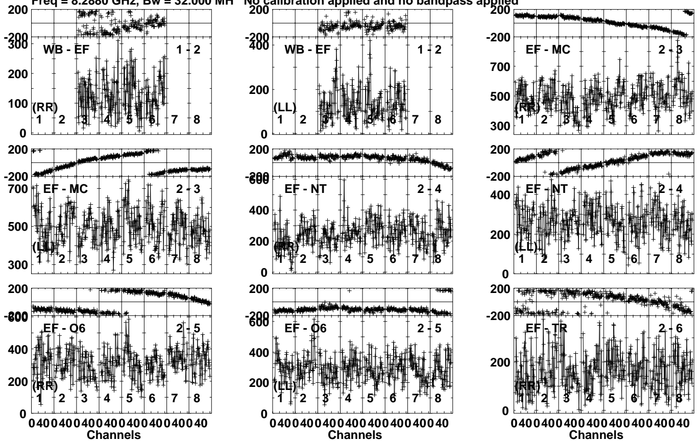
Lower frame: Micro Ampl Jy Top frame: Phas deg Vector averaged cross-power spectrum Several baselines displayed Timerange: 00/17:40:33 to 00/17:43:29
