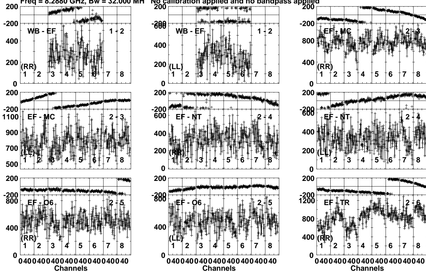
Lower frame: Micro Ampl Jy Top frame: Phas deg Vector averaged cross-power spectrum Several baselines displayed Timerange: 00/19:08:01 to 00/19:09:59
