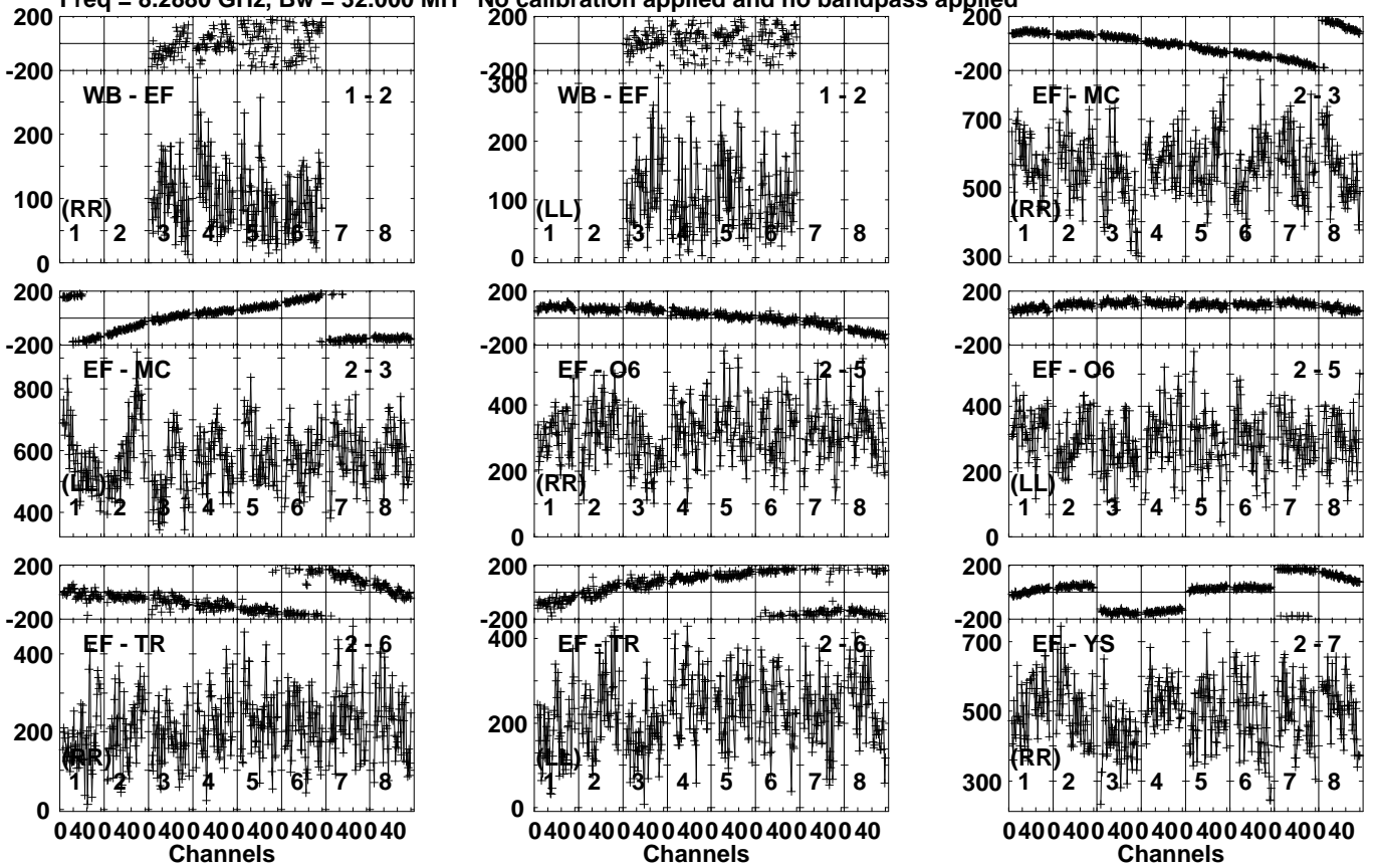
Lower frame: Micro Ampl Jy Top frame: Phas deg Vector averaged cross-power spectrum Several baselines displayed Timerange: 00/19:26:03 to 00/19:28:59
