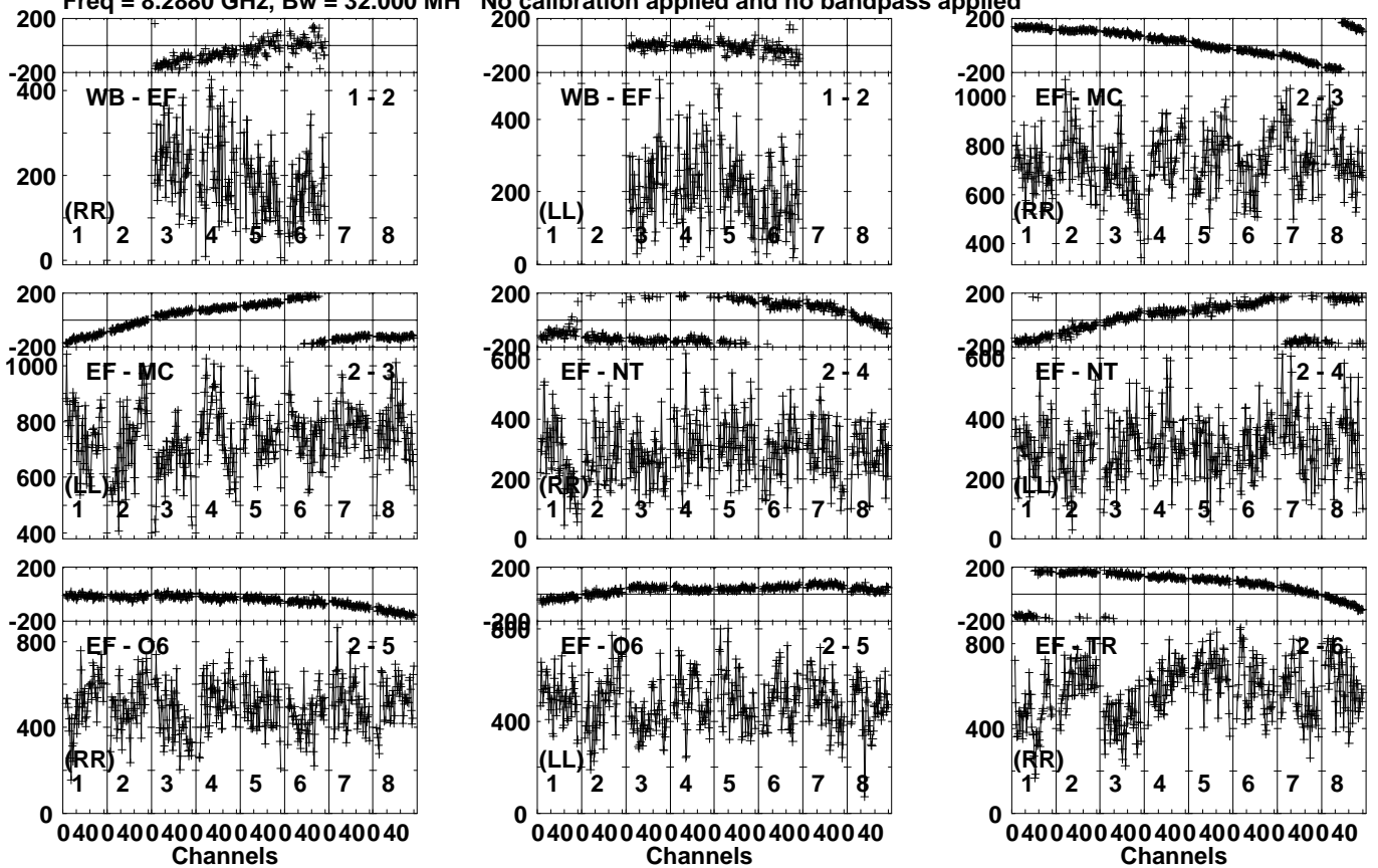
Lower frame: Micro Ampl Jy Top frame: Phas deg Vector averaged cross-power spectrum Several baselines displayed Timerange: 00/18:21:01 to 00/18:22:59
