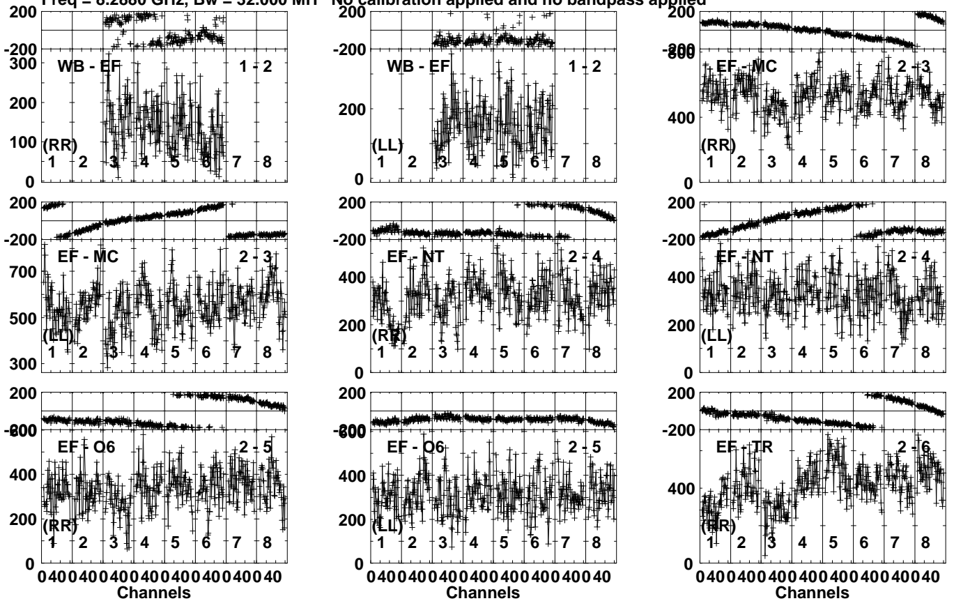
Lower frame: Micro Ampl Jy Top frame: Phas deg Vector averaged cross-power spectrum Several baselines displayed Timerange: 00/18:49:01 to 00/18:51:59
