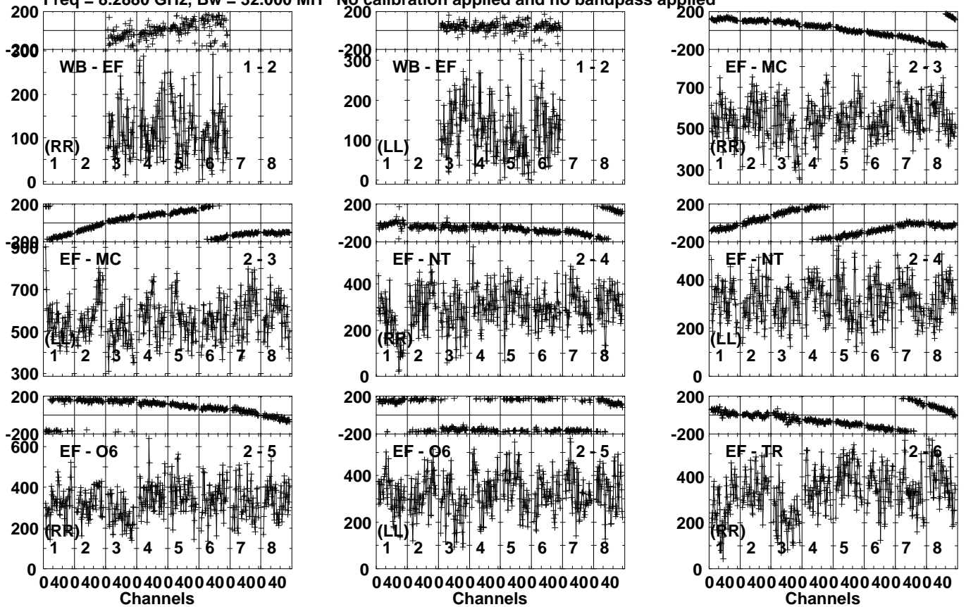
Lower frame: Micro Ampl Jy Top frame: Phas deg Vector averaged cross-power spectrum Several baselines displayed Timerange: 00:18:44:03 to 00:18:46:59
