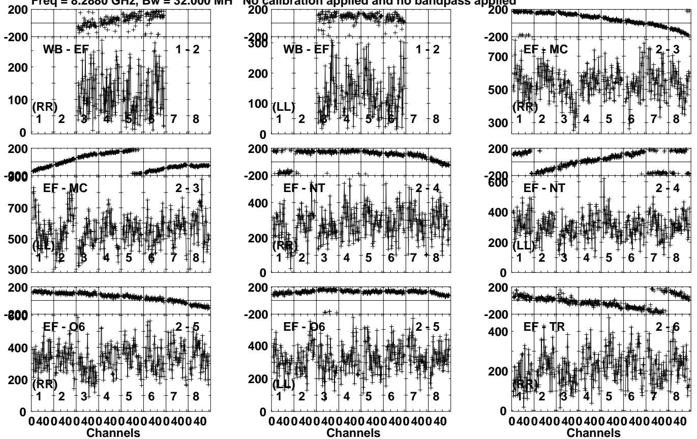
Lower frame: Micro Ampl Jy Top frame: Phas deg Vector averaged cross-power spectrum Several baselines displayed Timerange: 00/18:38:31 to 00/18:41:29
