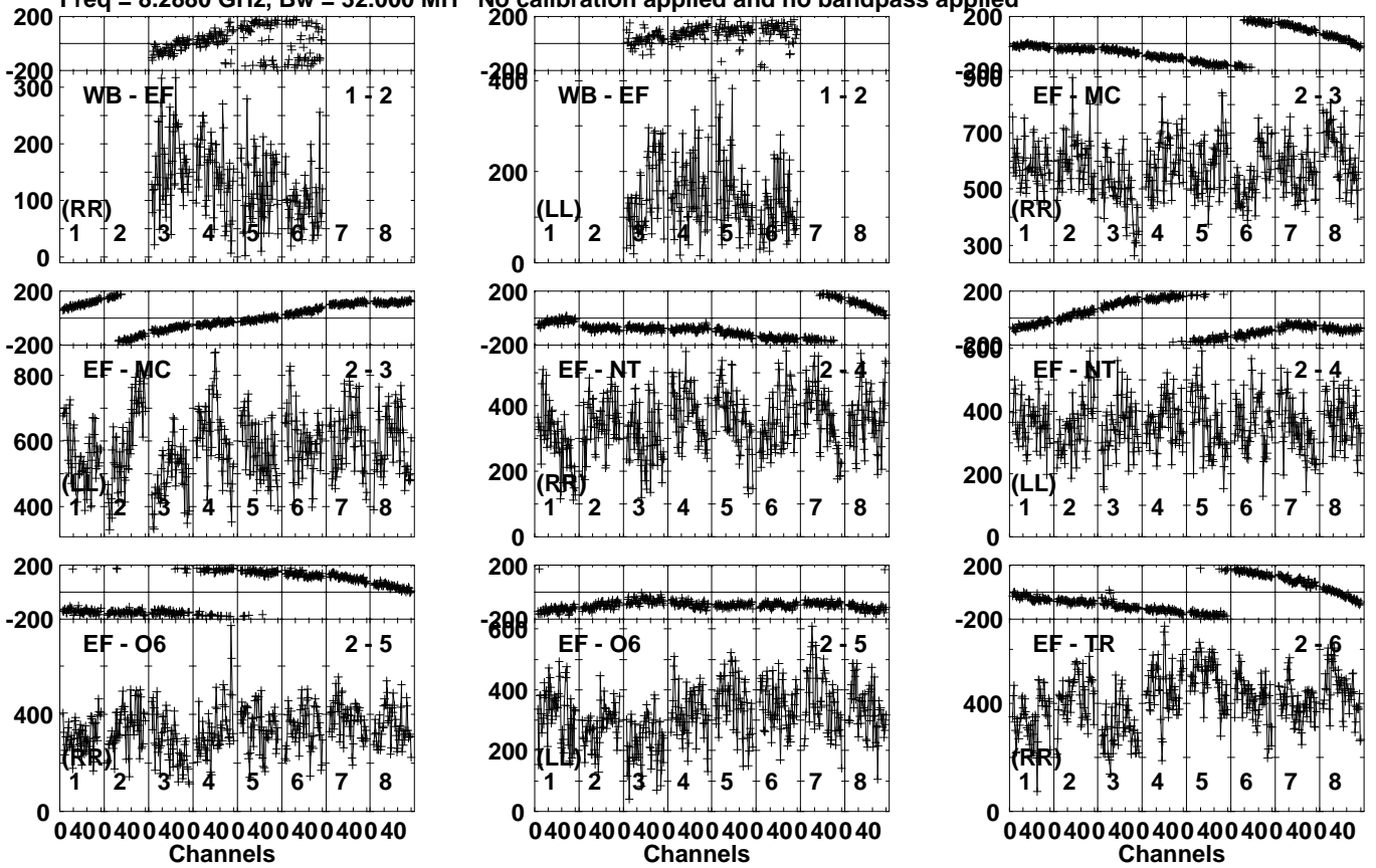
Lower frame: Micro Ampl Jy Top frame: Phas deg Vector averaged cross-power spectrum Several baselines displayed Timerange: 00/19:47:03 to 00/19:49:59
