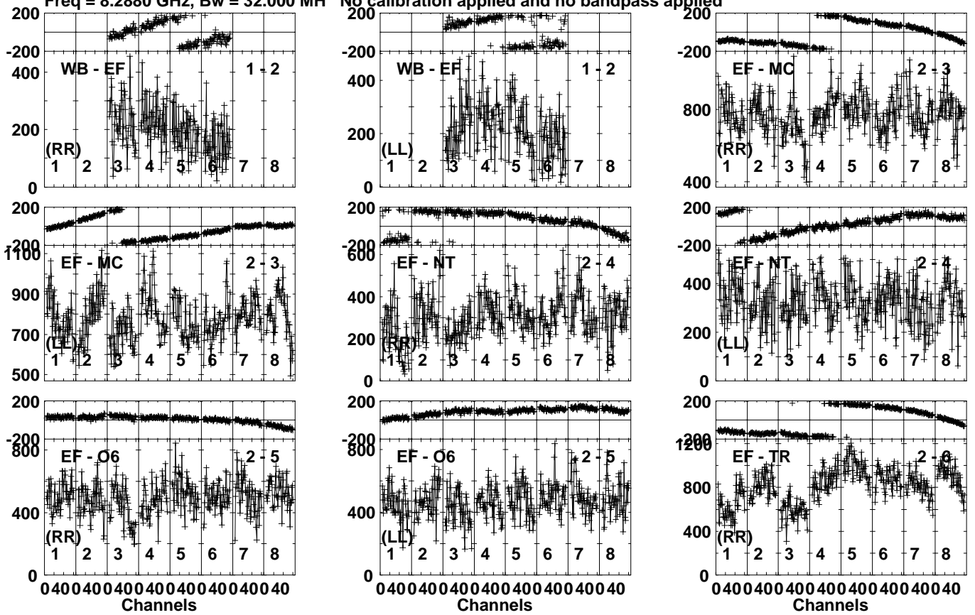
Lower frame: Micro Ampl Jy Top frame: Phas deg Vector averaged cross-power spectrum Several baselines displayed Timerange: 00/19:13:31 to 00/19:15:29
