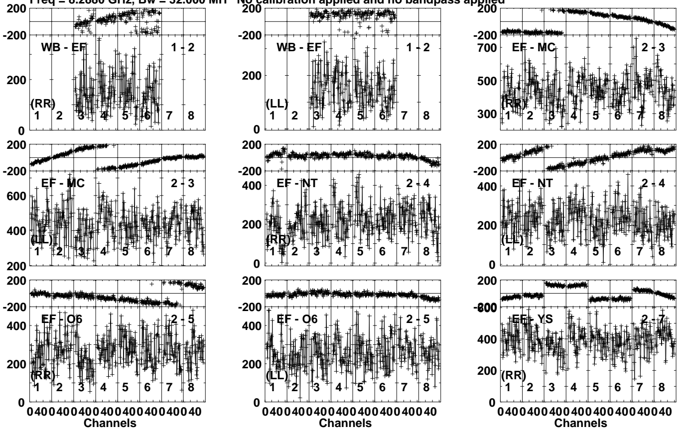
Lower frame: Micro Ampl Jy Top frame: Phas deg Vector averaged cross-power spectrum Several baselines displayed Timerange: 00/16:42:31 to 00/16:45:29
