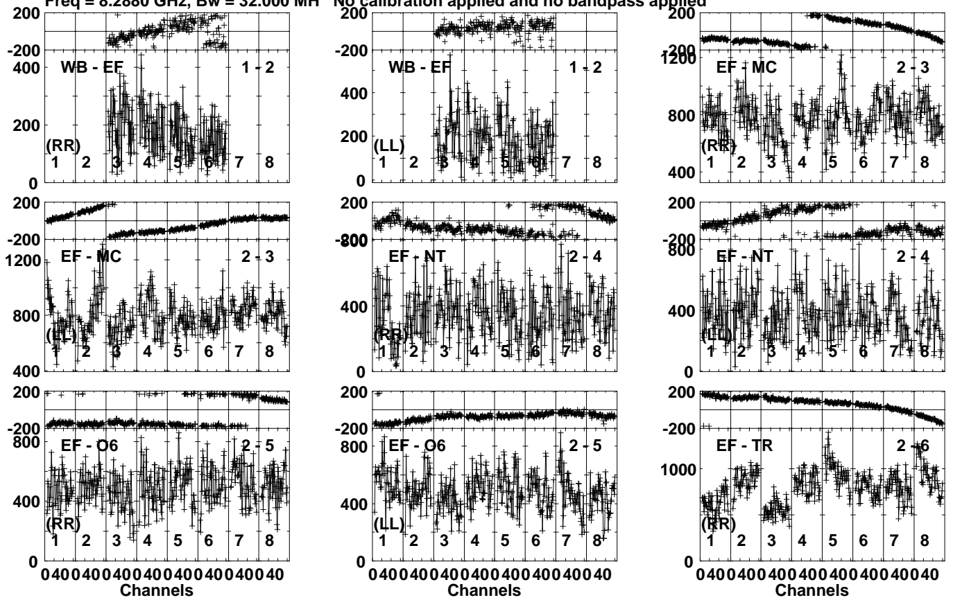
Lower frame: Micro Ampl Jy Top frame: Phas deg Vector averaged cross-power spectrum Several baselines displayed Timerange: 00/19:29:01 to 00/19:30:59
