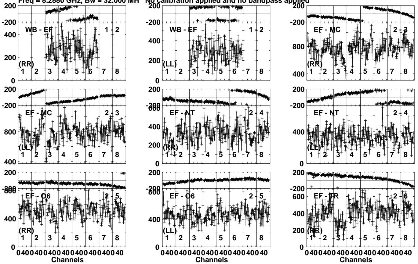
Lower frame: Micro Ampl Jy Top frame: Phas deg Vector averaged cross-power spectrum Several baselines displayed Timerange: 00/19:34:31 to 00/19:36:29
