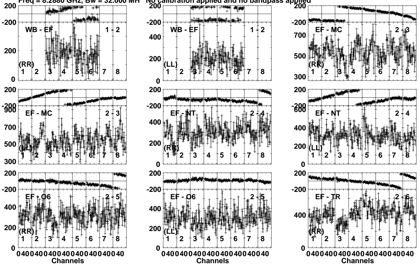
Lower frame: Micro Ampl Jy Top frame: Phas deg Vector averaged cross-power spectrum Several baselines displayed Timerange: 00/18:33:33 to 00/18:36:29
