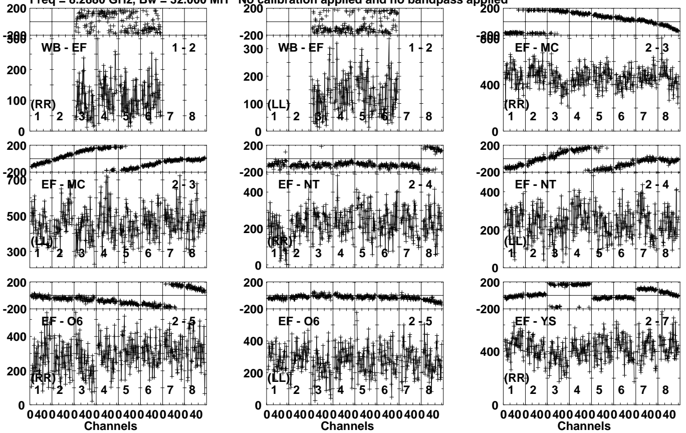
Lower frame: Micro Ampl Jy Top frame: Phas deg Vector averaged cross-power spectrum Several baselines displayed Timerange: 00/17:03:31 to 00/17:06:29
