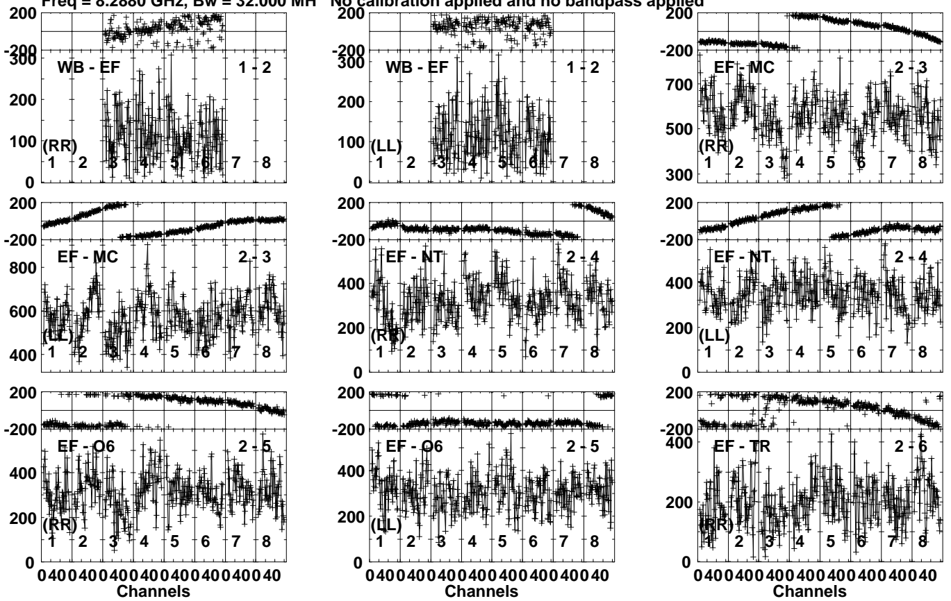
Lower frame: Micro Ampl Jy Top frame: Phas deg Vector averaged cross-power spectrum Several baselines displayed Timerange: 00/19:10:01 to 00/19:12:59
