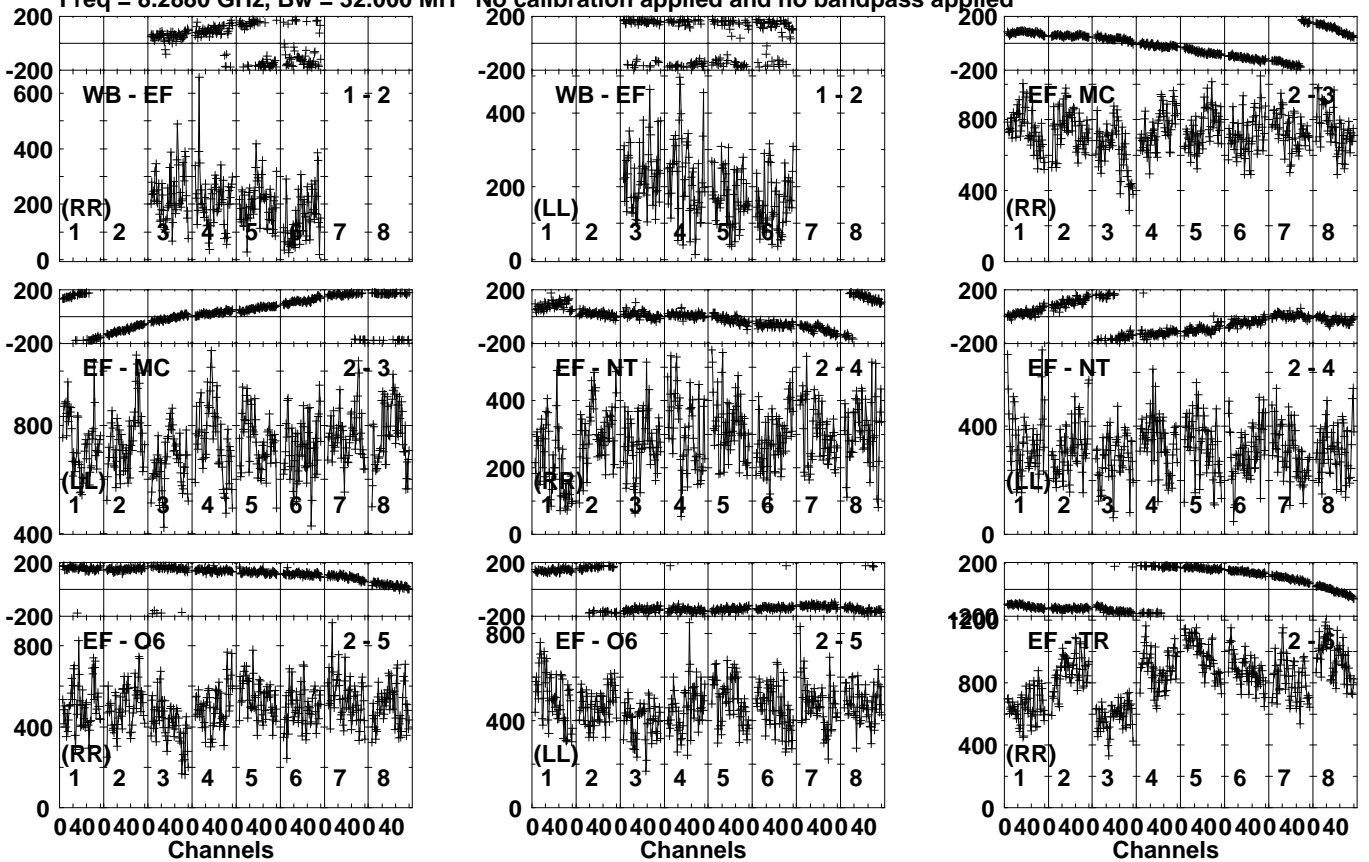
Lower frame: Micro Ampl Jy Top frame: Phas deg Vector averaged cross-power spectrum Several baselines displayed Timerange: 00:18:10:31 to 00:18:12:29
