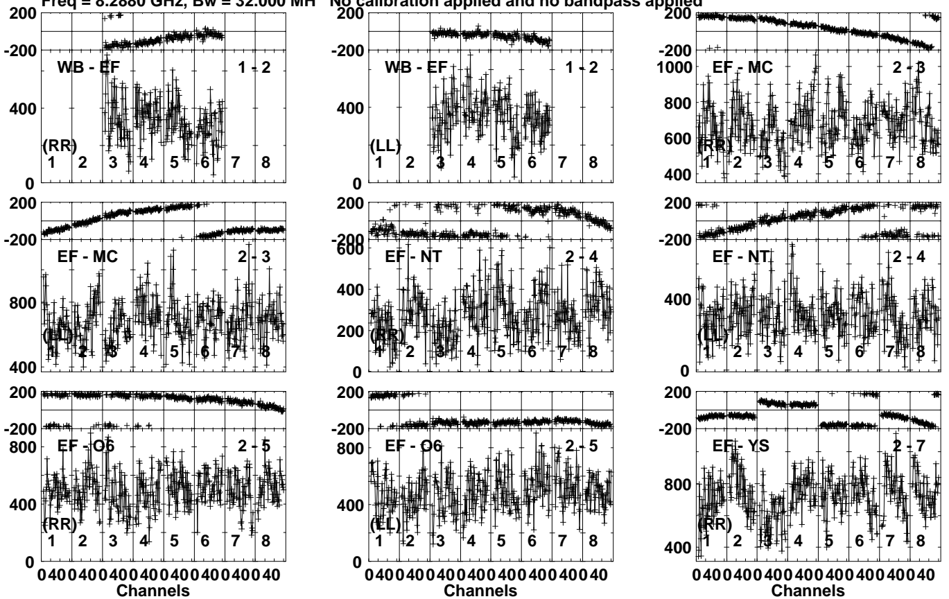
Lower frame: Micro Ampl Jy Top frame: Phas deg Vector averaged cross-power spectrum Several baselines displayed Timerange: 00/17:12:01 to 00/17:13:59
