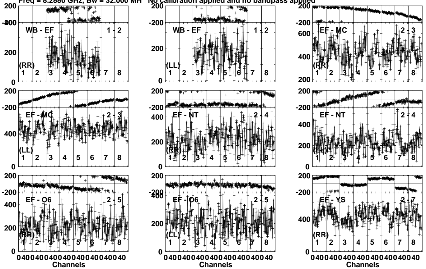
Lower frame: Micro Ampl Jy Top frame: Phas deg Vector averaged cross-power spectrum Several baselines displayed Timerange: 00/16:48:03 to 00/16:50:59
