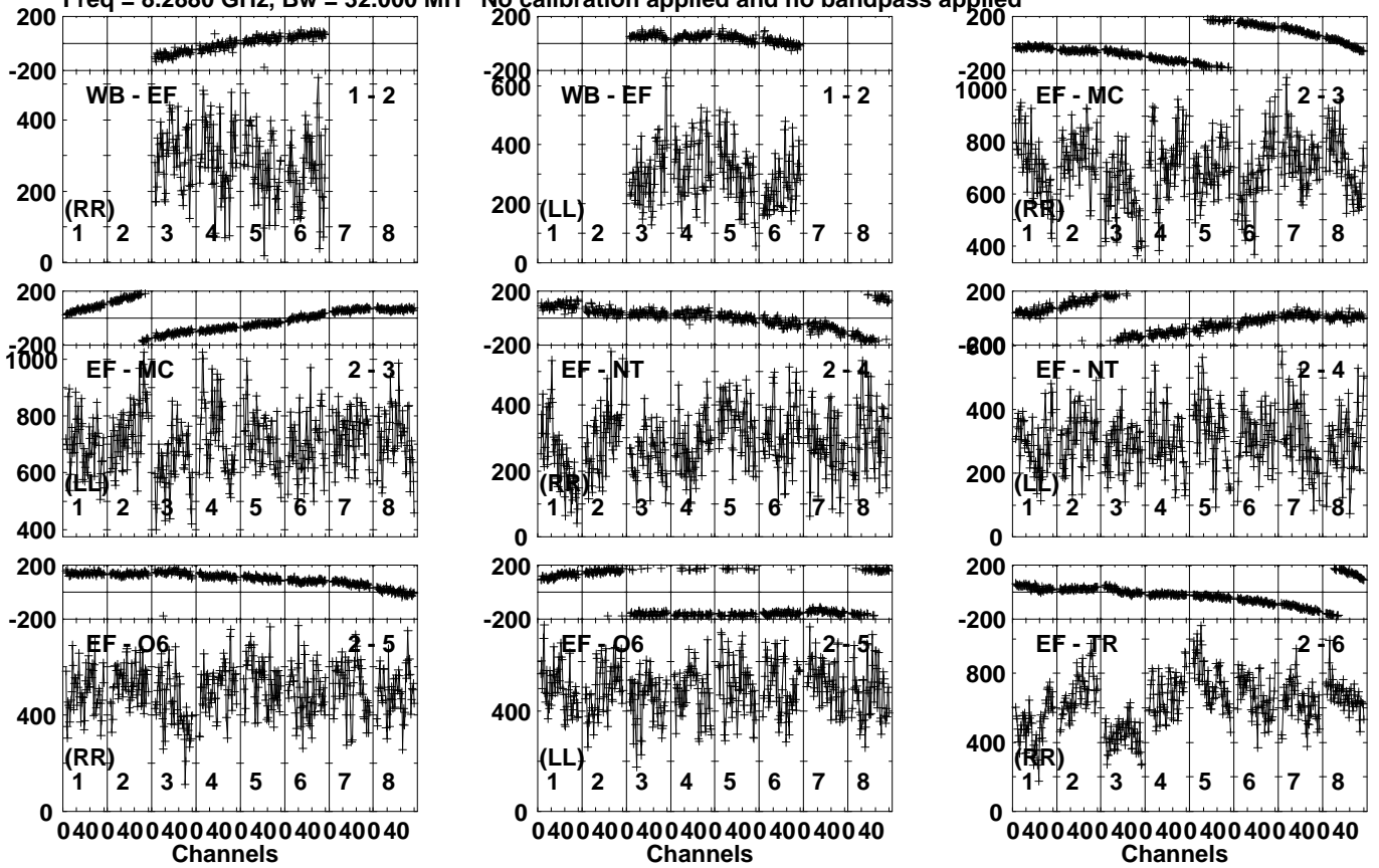
Lower frame: Micro Ampl Jy Top frame: Phas deg Vector averaged cross-power spectrum Several baselines displayed Timerange: 00/17:38:31 to 00/17:40:29
