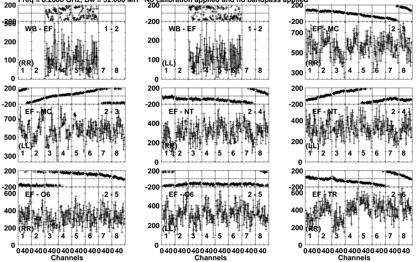
Lower frame: Micro Ampl Jy Top frame: Phas deg Vector averaged cross-power spectrum Several baselines displayed Timerange: 00/19:31:01 to 00/19:33:59
