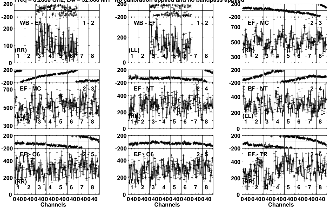
Lower frame: Micro Ampl Jy Top frame: Phas deg Vector averaged cross-power spectrum Several baselines displayed Timerange: 00/17:45:31 to 00/17:48:29
