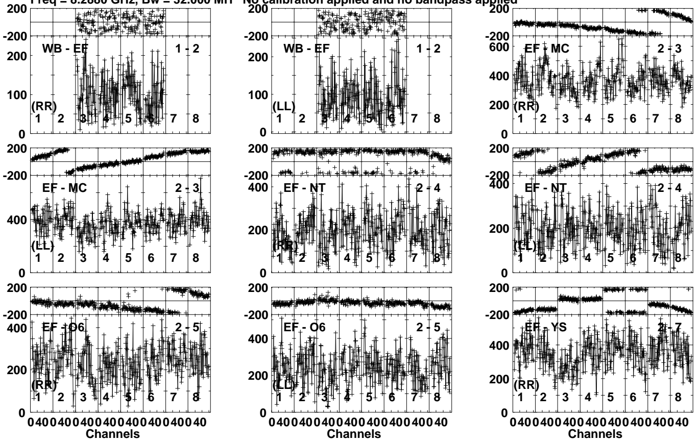
Lower frame: Micro Ampl Jy Top frame: Phas deg Vector averaged cross-power spectrum Several baselines displayed Timerange: 00/16:16:33 to 00/16:19:29
