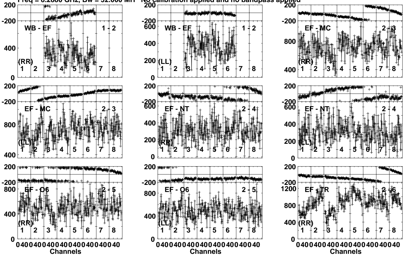
Lower frame: Micro Ampl Jy Top frame: Phas deg Vector averaged cross-power spectrum Several baselines displayed Timerange: 00/17:43:31 to 00/17:45:29
