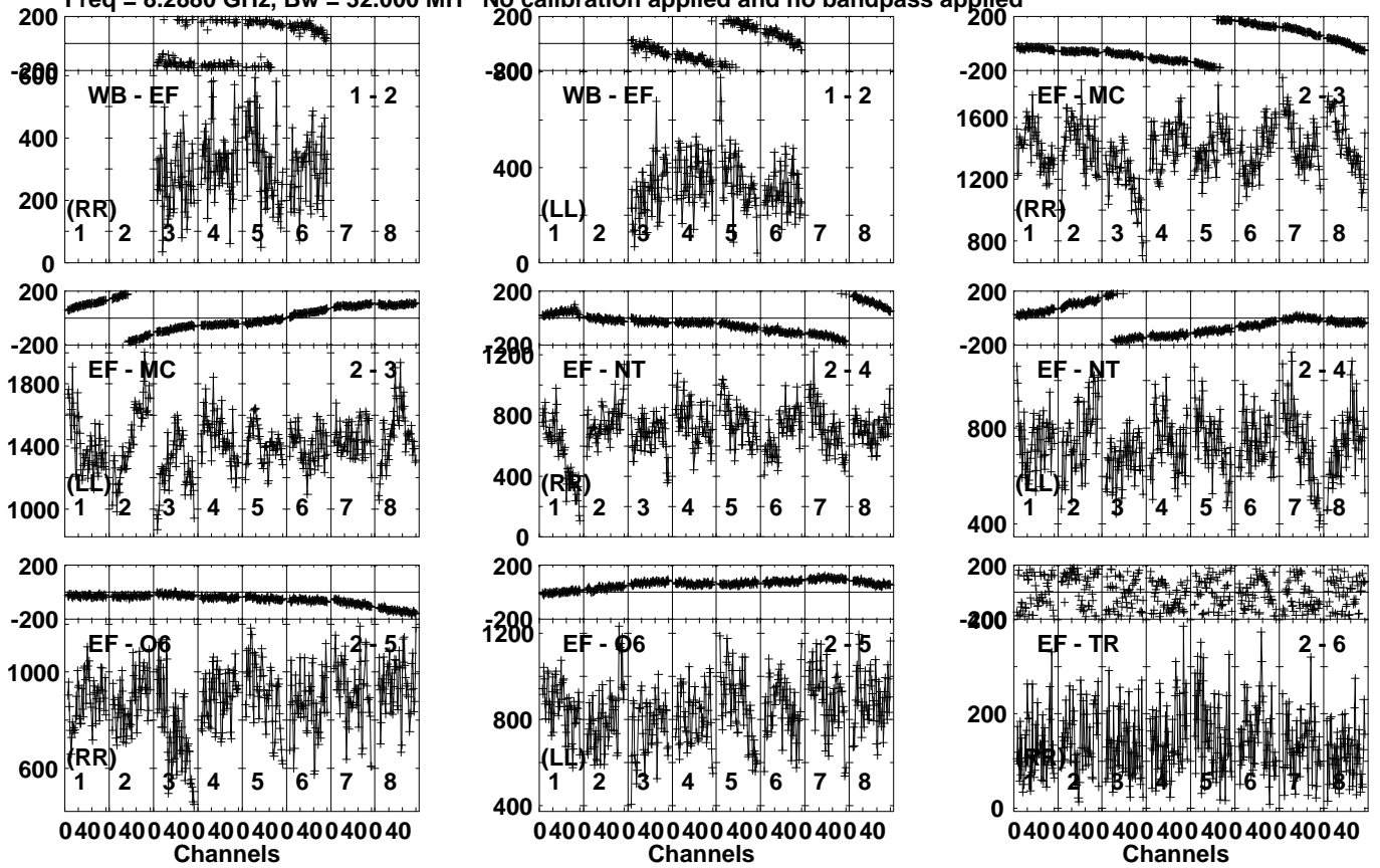
Lower frame: Micro Ampl Jy Top frame: Phas deg Vector averaged cross-power spectrum Several baselines displayed Timerange: 00/01:21:31 to 00/01:23:29
