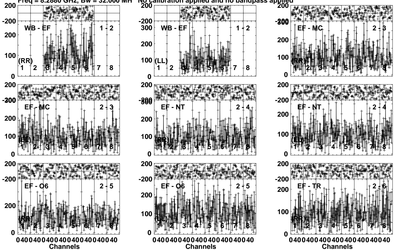
Lower frame: Micro Ampl Jy Top frame: Phas deg Vector averaged cross-power spectrum Several baselines displayed Timerange: 00/04:01:31 to 00/04:04:29
