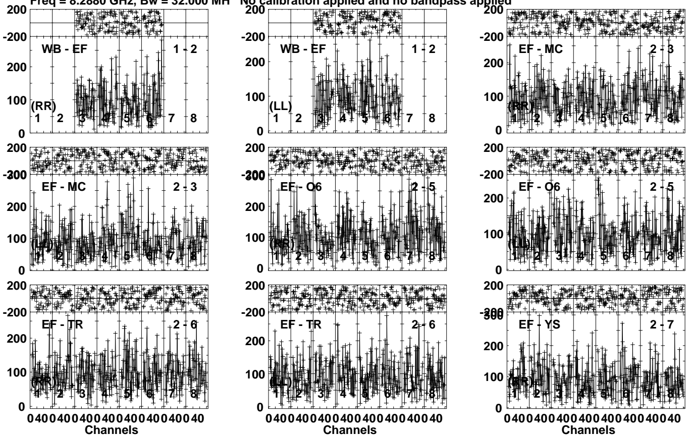
Lower frame: Micro Ampl Jy Top frame: Phas deg Vector averaged cross-power spectrum Several baselines displayed Timerange: 00/03:09:01 to 00/03:11:59
