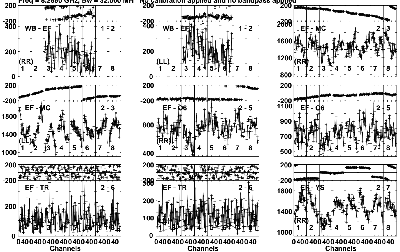
Lower frame: Micro Ampl Jy Top frame: Phas deg Vector averaged cross-power spectrum Several baselines displayed Timerange: 00/03:23:01 to 00/03:24:59
