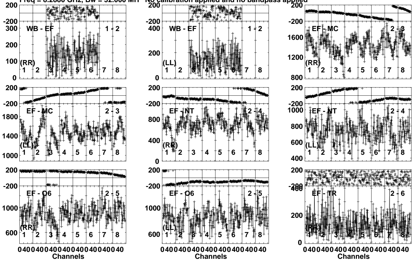
Lower frame: Micro Ampl Jy Top frame: Phas deg Vector averaged cross-power spectrum Several baselines displayed Timerange: 00/01:42:31 to 00/01:44:29
