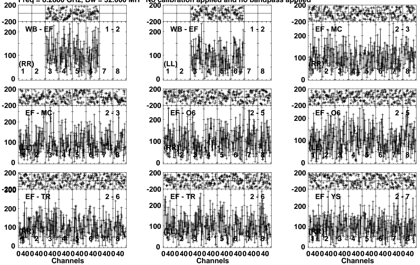
Lower frame: Micro Ampl Jy Top frame: Phas deg Vector averaged cross-power spectrum Several baselines displayed Timerange: 00/03:14:33 to 00/03:17:29
