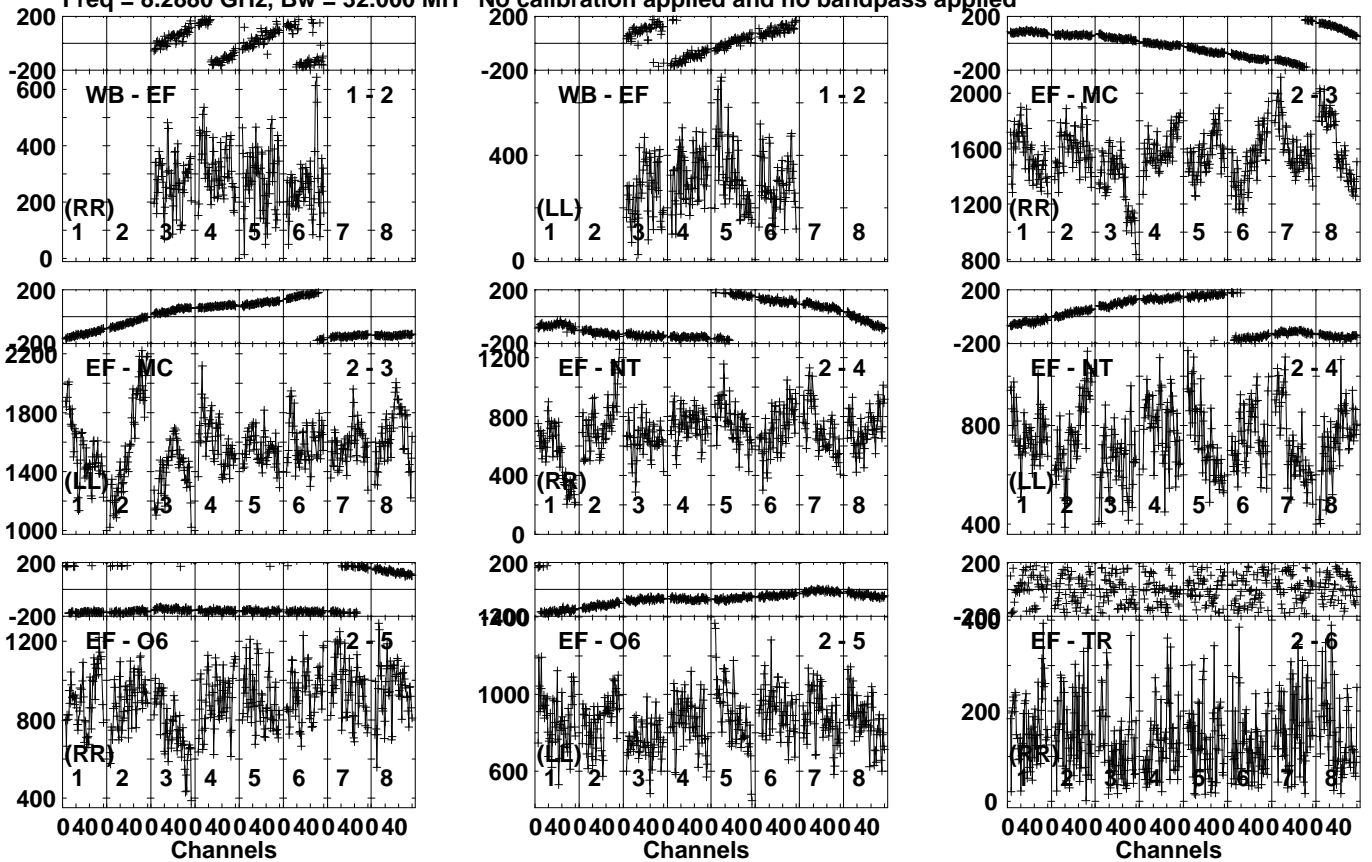
Lower frame: Micro Ampl Jy Top frame: Phas deg Vector averaged cross-power spectrum Several baselines displayed Timerange: 00/04:20:31 to 00/04:22:29
