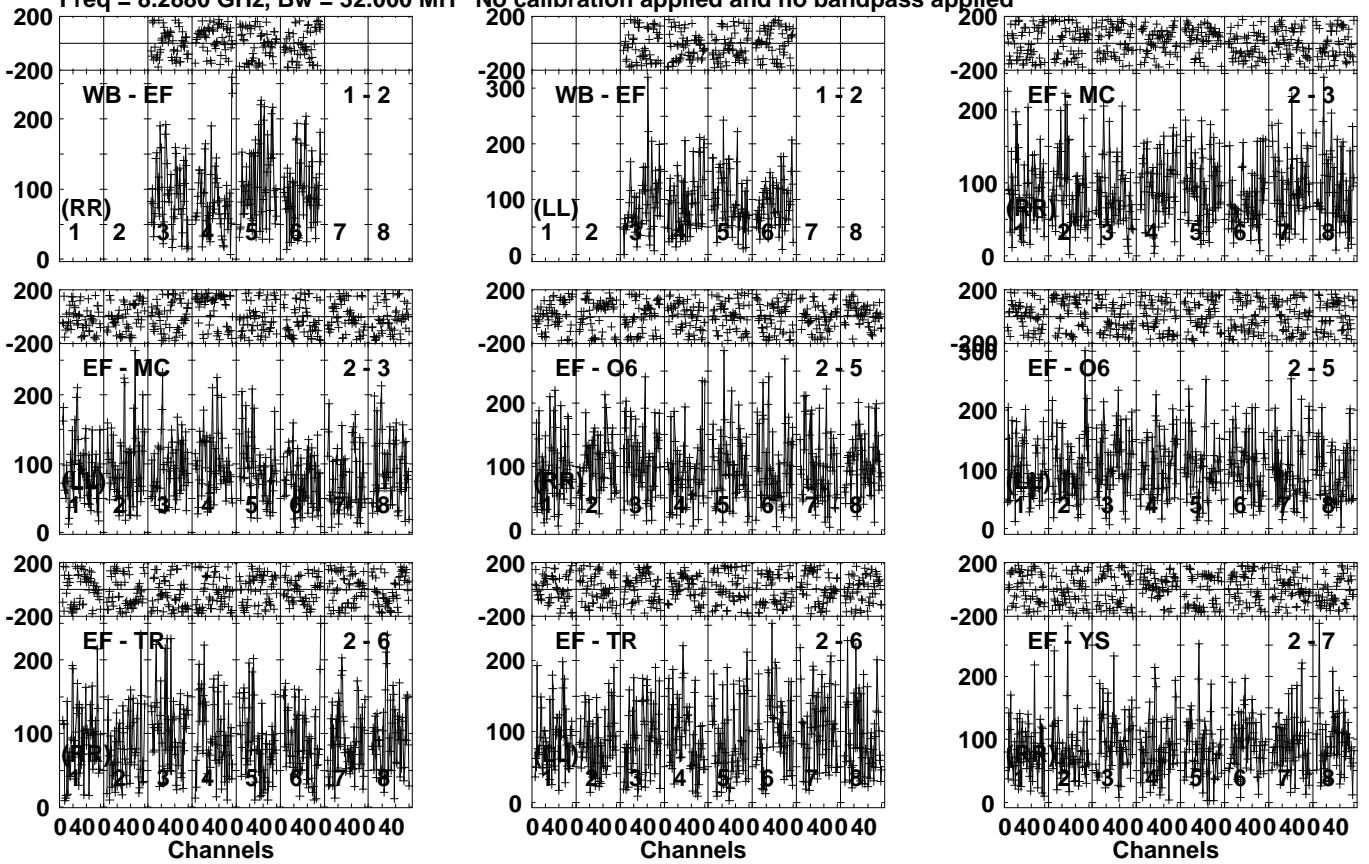
Lower frame: Micro Ampl Jy Top frame: Phas deg Vector averaged cross-power spectrum Several baselines displayed Timerange: 00/03:19:31 to 00/03:22:29
