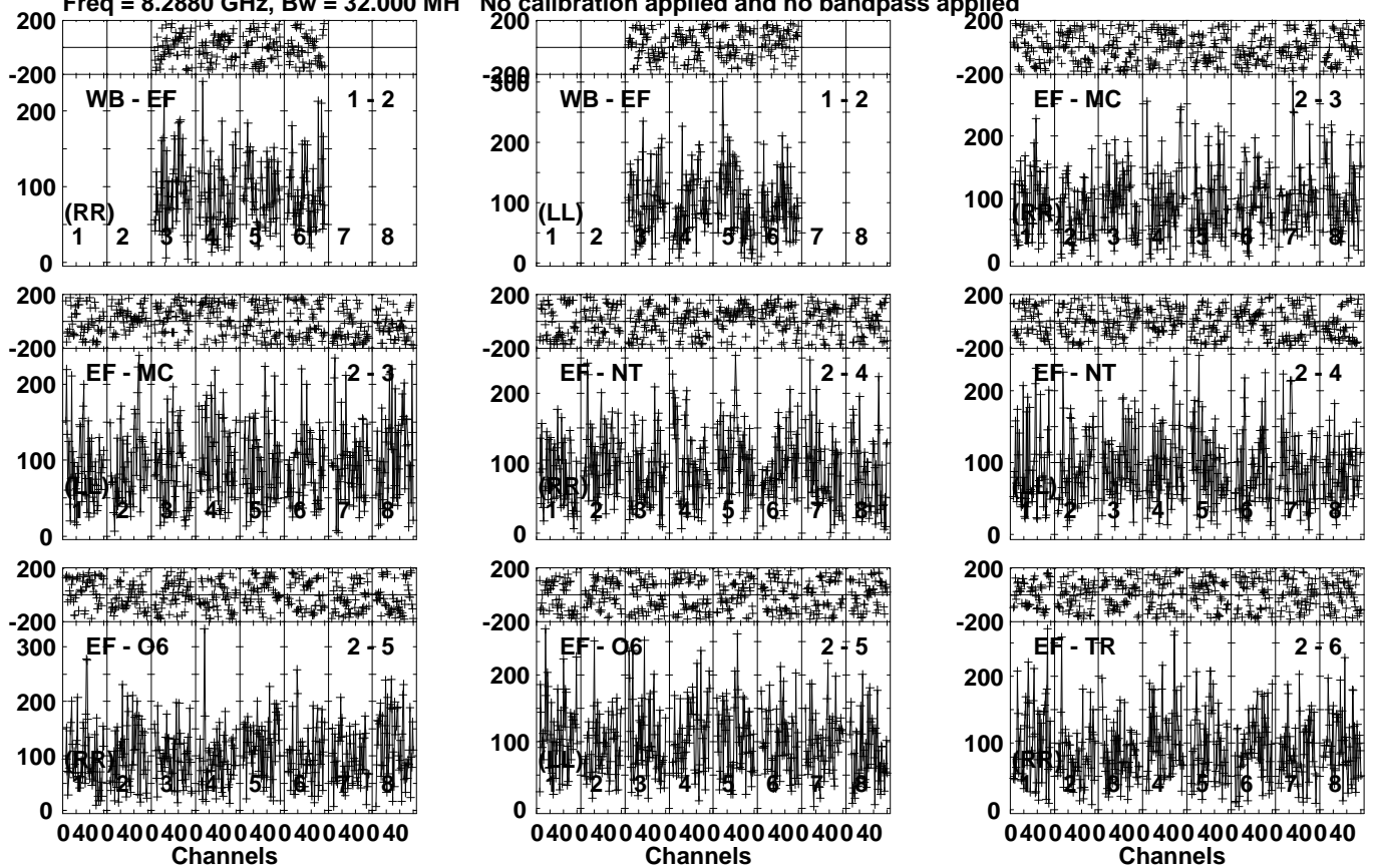
Lower frame: Micro Ampl Jy Top frame: Phas deg Vector averaged cross-power spectrum Several baselines displayed Timerange: 00/01:55:01 to 00/01:57:59
