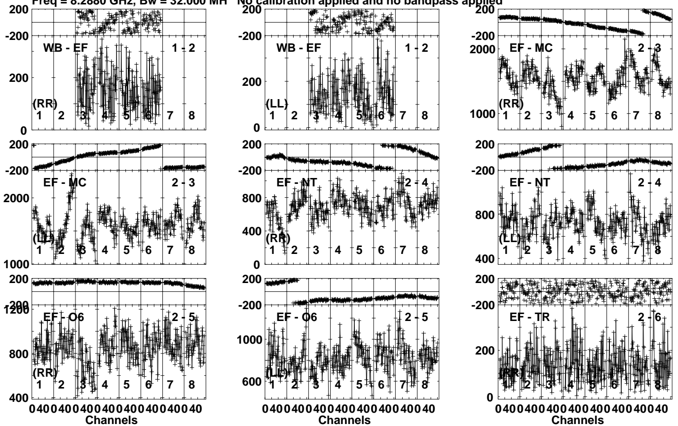
Lower frame: Micro Ampl Jy Top frame: Phas deg Vector averaged cross-power spectrum Several baselines displayed Timerange: 00/04:41:31 to 00/04:43:29
