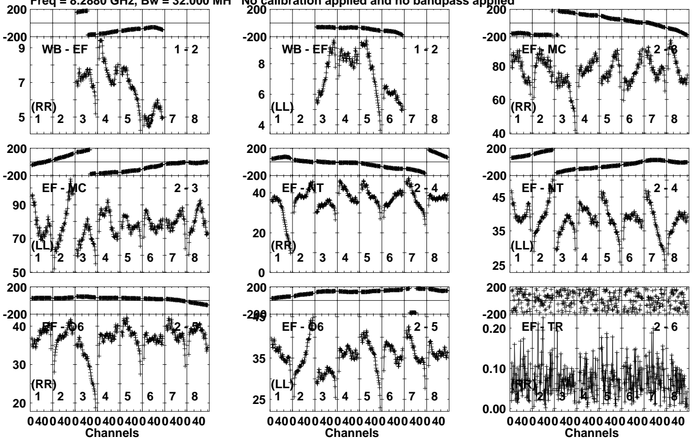
Lower frame: Milli Ampl Jy Top frame: Phas deg Vector averaged cross-power spectrum Several baselines displayed Timerange: 00/02:58:01 to 00/03:02:59
