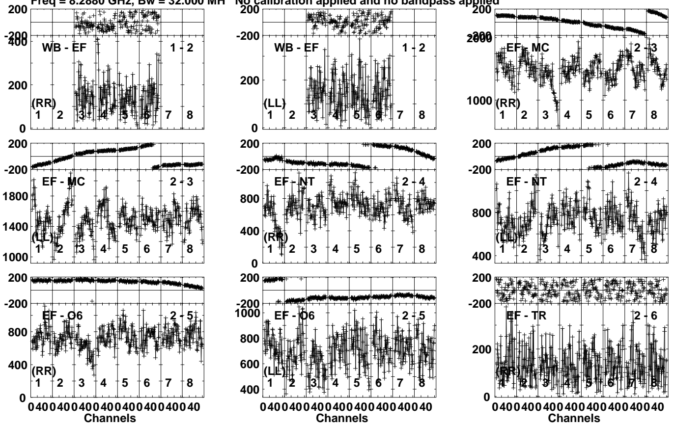
Lower frame: Micro Ampl Jy Top frame: Phas deg Vector averaged cross-power spectrum Several baselines displayed Timerange: 00/02:35:01 to 00/02:36:59
