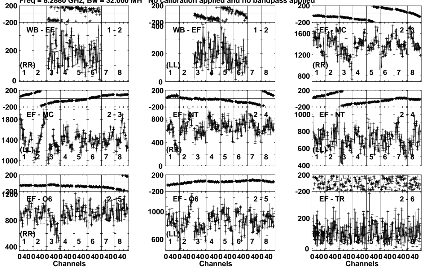
Lower frame: Micro Ampl Jy Top frame: Phas deg Vector averaged cross-power spectrum Several baselines displayed Timerange: 00/01:16:31 to 00/01:18:29
