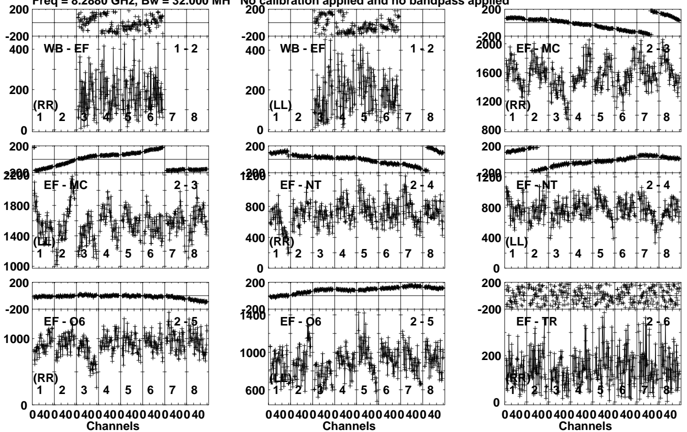
Lower frame: Micro Ampl Jy Top frame: Phas deg Vector averaged cross-power spectrum Several baselines displayed Timerange: 00/04:10:01 to 00/04:11:59
