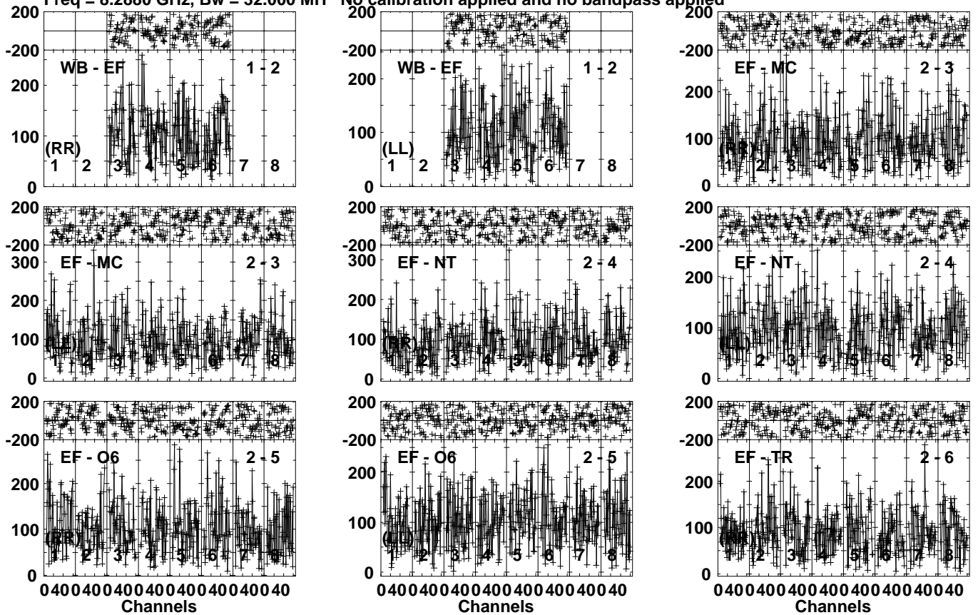
Lower frame: Micro Ampl Jy Top frame: Phas deg Vector averaged cross-power spectrum Several baselines displayed Timerange: 00/04:12:01 to 00/04:14:59
