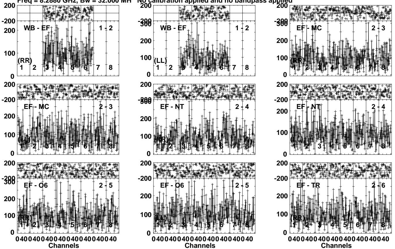
Lower frame: Micro Ampl Jy Top frame: Phas deg Vector averaged cross-power spectrum Several baselines displayed Timerange: 00/03:30:01 to 00/03:32:59
