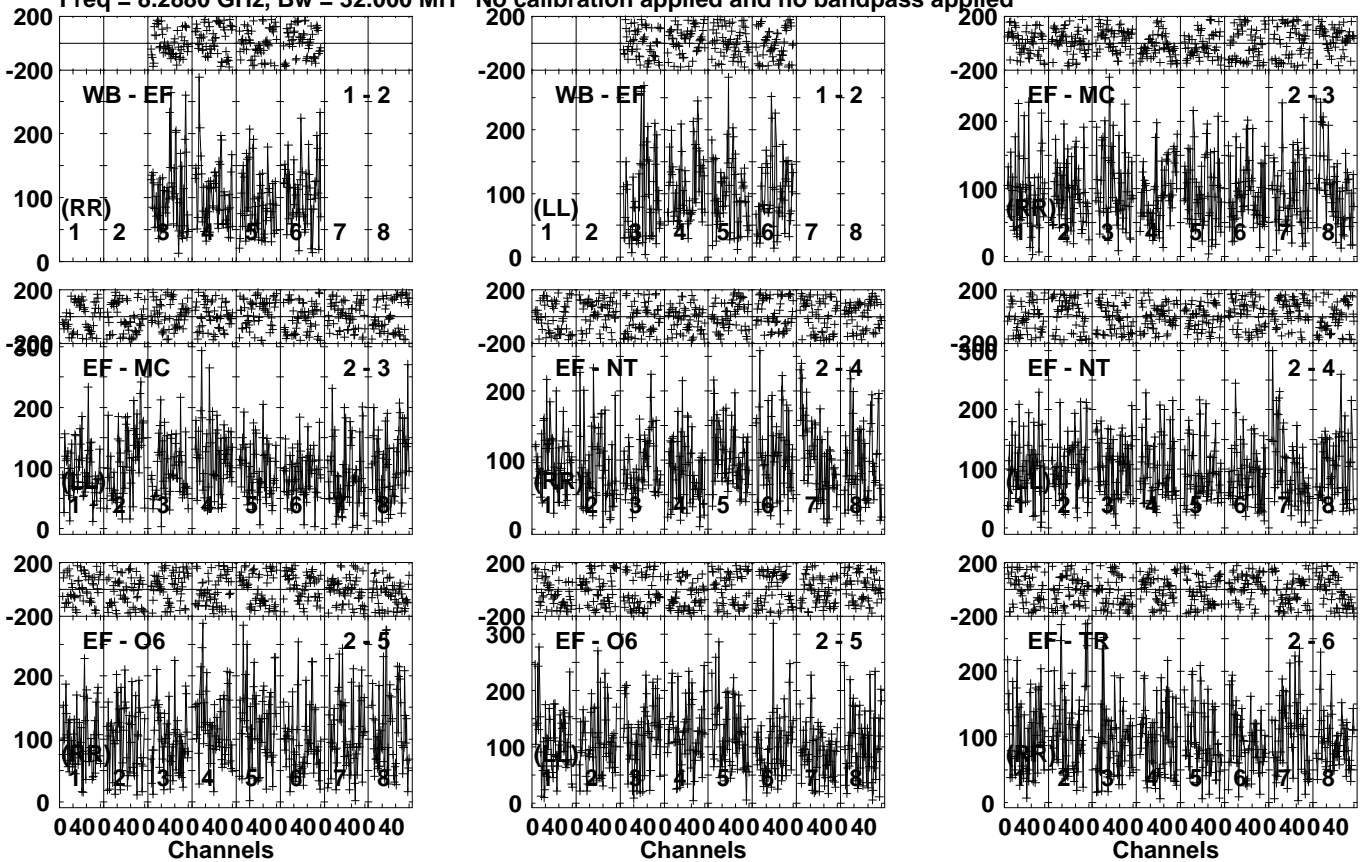
Lower frame: Micro Ampl Jy Top frame: Phas deg Vector averaged cross-power spectrum Several baselines displayed Timerange: 00/04:22:31 to 00/04:25:29
