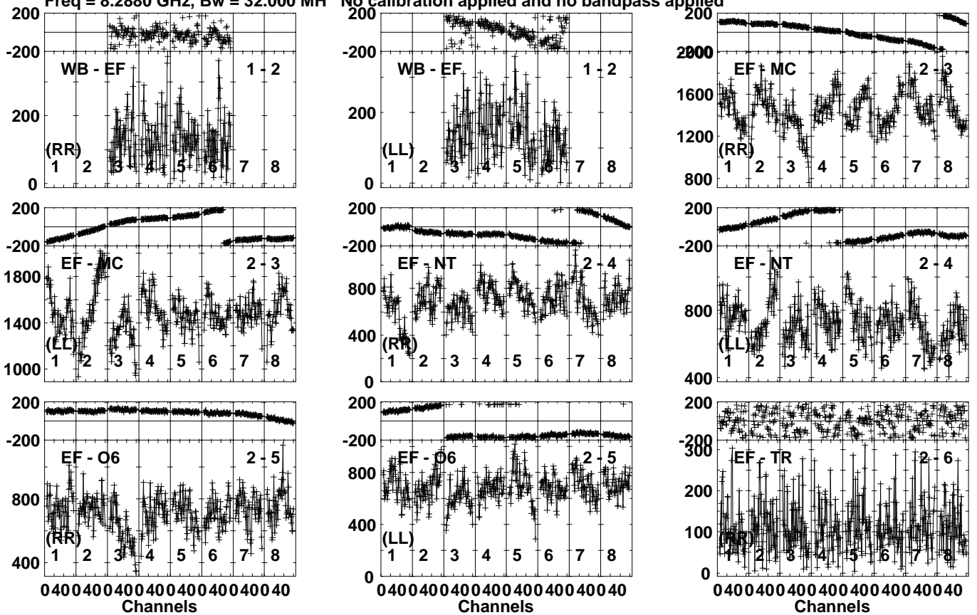
Lower frame: Micro Ampl Jy Top frame: Phas deg Vector averaged cross-power spectrum Several baselines displayed Timerange: 00/02:30:01 to 00/02:31:59
