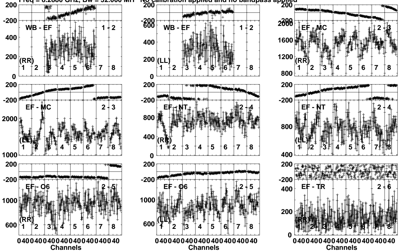
Lower frame: Micro Ampl Jy Top frame: Phas deg Vector averaged cross-power spectrum Several baselines displayed Timerange: 00/03:59:31 to 00/04:01:29
