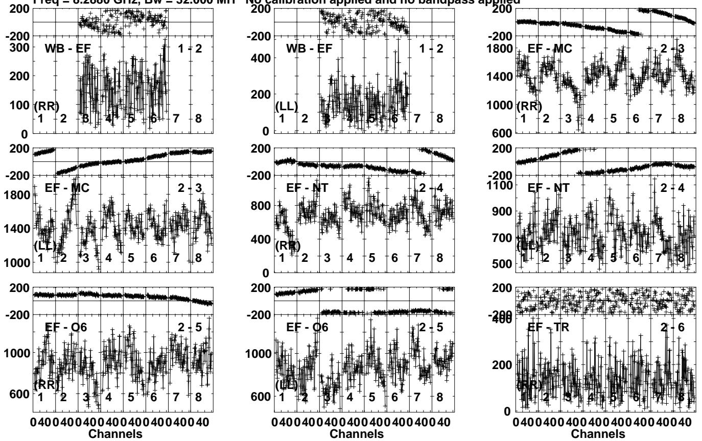
Lower frame: Micro Ampl Jy Top frame: Phas deg Vector averaged cross-power spectrum Several baselines displayed Timerange: 00/01:32:01 to 00/01:33:59
