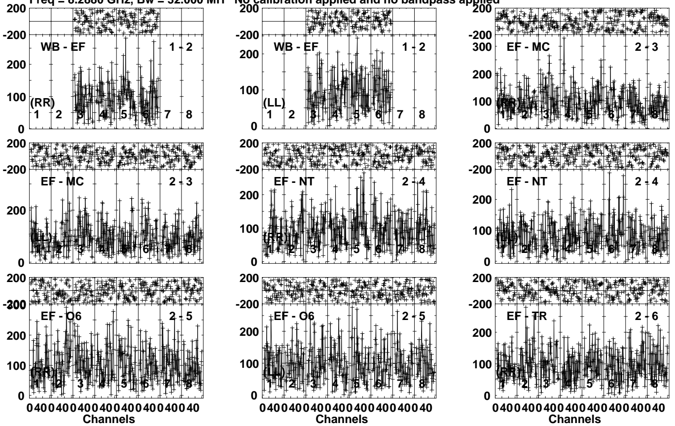
Lower frame: Micro Ampl Jy Top frame: Phas deg Vector averaged cross-power spectrum Several baselines displayed Timerange: 00/04:33:01 to 00/04:35:59
