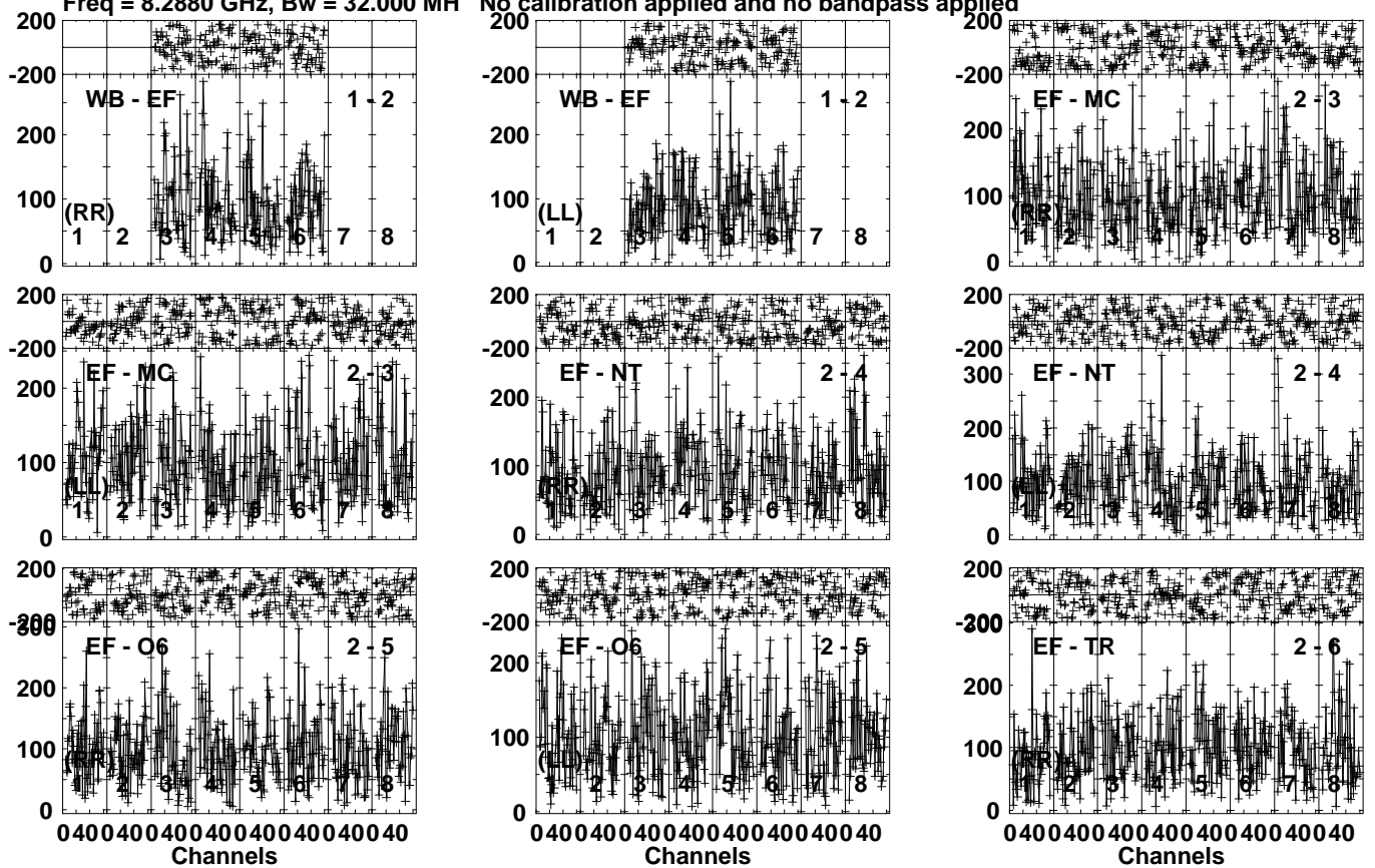
Lower frame: Micro Ampl Jy Top frame: Phas deg Vector averaged cross-power spectrum Several baselines displayed Timerange: 00/02:21:33 to 00/02:24:29
