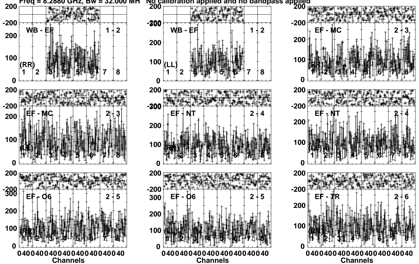
Lower frame: Micro Ampl Jy Top frame: Phas deg Vector averaged cross-power spectrum Several baselines displayed Timerange: 00/02:26:31 to 00/02:29:29
