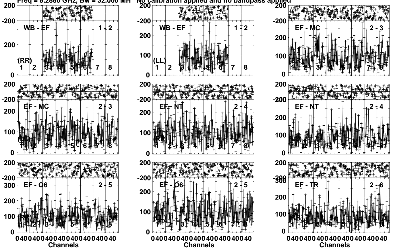
Lower frame: Micro Ampl Jy Top frame: Phas deg Vector averaged cross-power spectrum Several baselines displayed Timerange: 00/01:23:31 to 00/01:26:29
