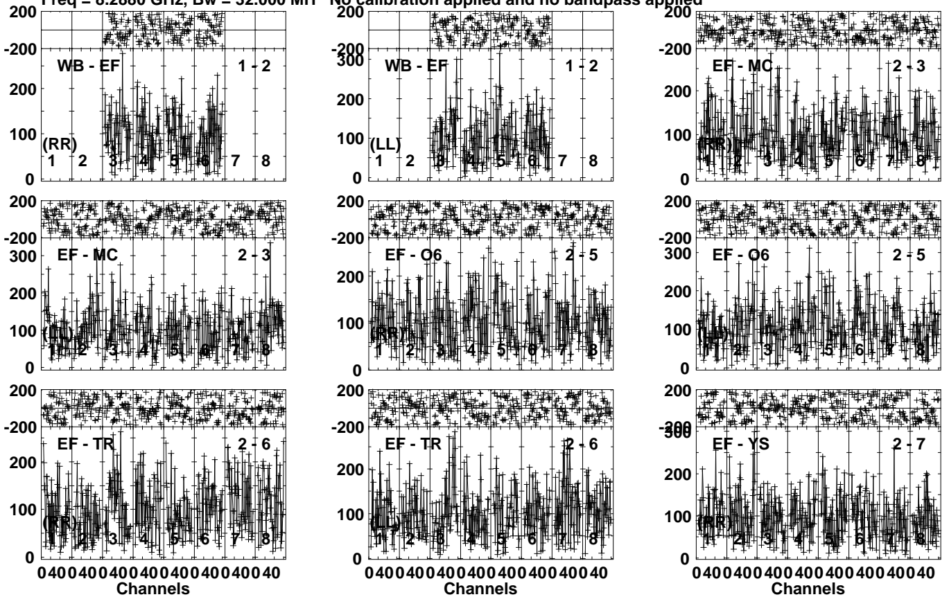
Lower frame: Micro Ampl Jy Top frame: Phas deg Vector averaged cross-power spectrum Several baselines displayed Timerange: 00/04:49:03 to 00/04:51:59
