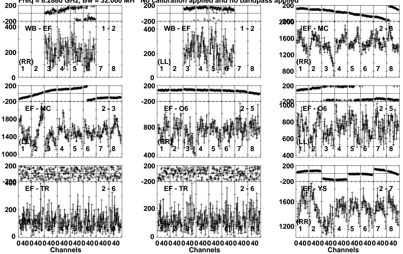
Lower frame: Micro Ampl Jy Top frame: Phas deg Vector averaged cross-power spectrum Several baselines displayed Timerange: 00/03:12:31 to 00/03:14:29
