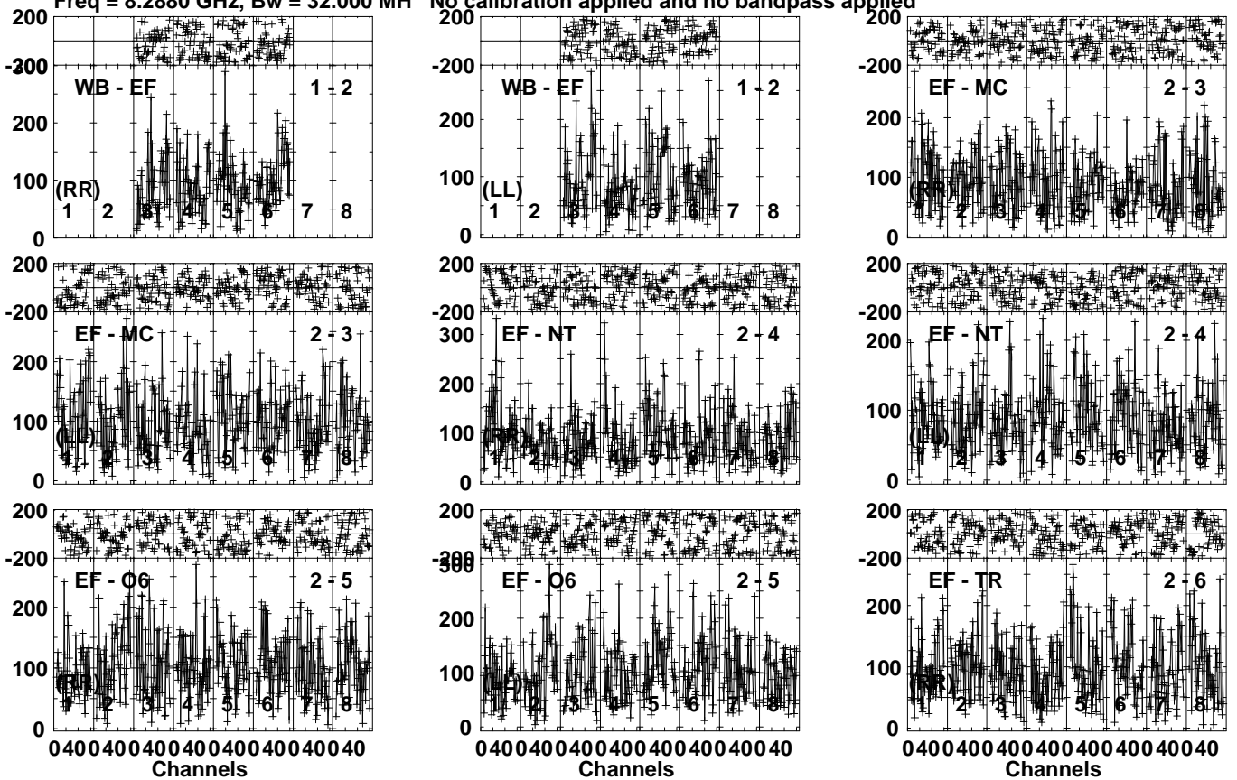
Lower frame: Micro Ampl Jy Top frame: Phas deg Vector averaged cross-power spectrum Several baselines displayed Timerange: 00/04:38:33 to 00/04:41:29
