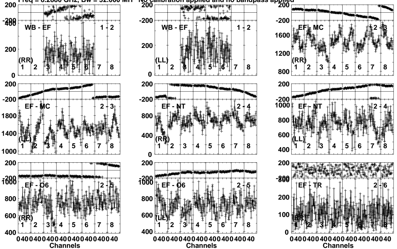
Lower frame: Micro Ampl Jy Top frame: Phas deg Vector averaged cross-power spectrum Several baselines displayed Timerange: 00/02:51:01 to 00/02:52:59
