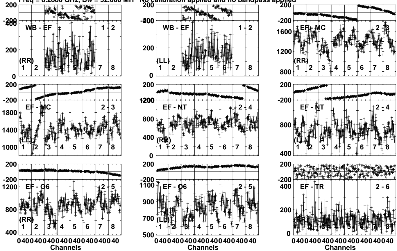
Lower frame: Micro Ampl Jy Top frame: Phas deg Vector averaged cross-power spectrum Several baselines displayed Timerange: 00/01:27:01 to 00/01:28:59
