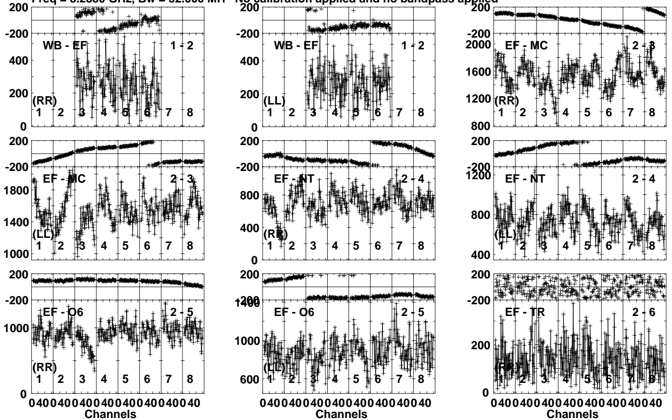
Lower frame: Micro Ampl Jy Top frame: Phas deg Vector averaged cross-power spectrum Several baselines displayed Timerange: 00/03:49:01 to 00/03:50:59
