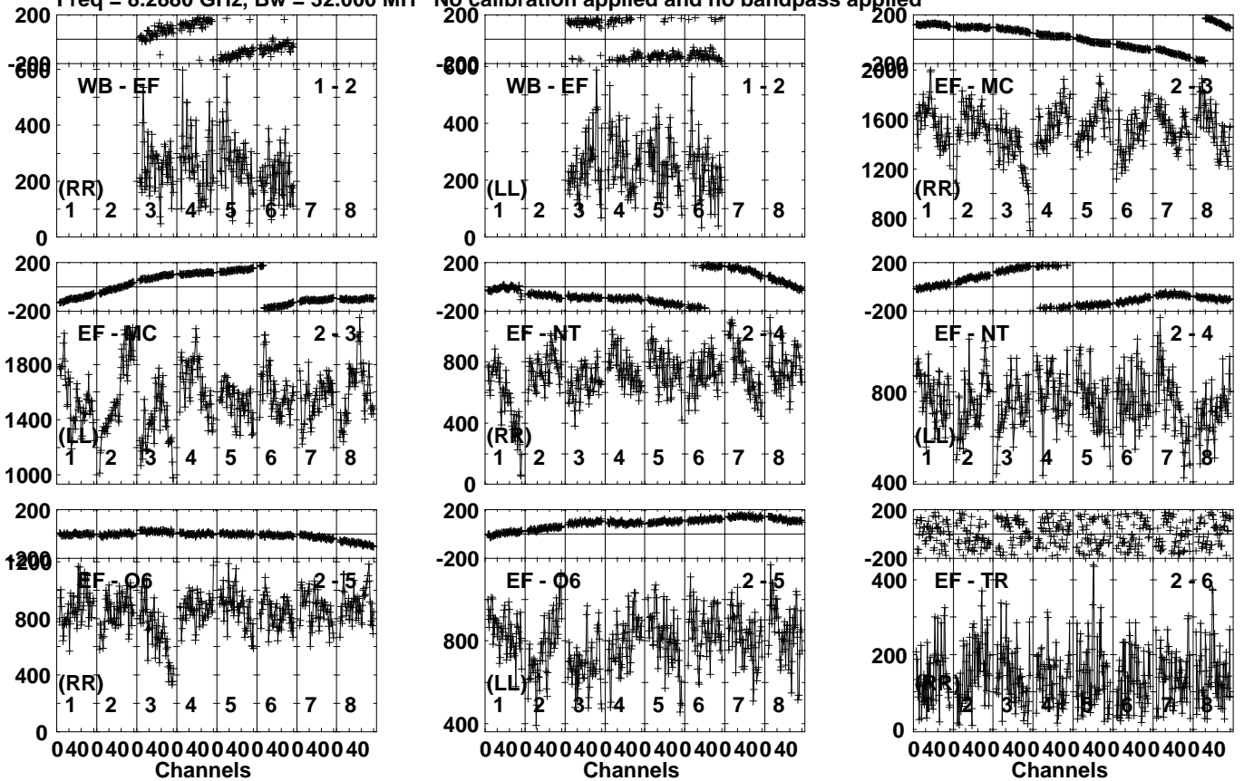
Lower frame: Micro Ampl Jy Top frame: Phas deg Vector averaged cross-power spectrum Several baselines displayed Timerange: 00/03:38:31 to 00/03:40:29
