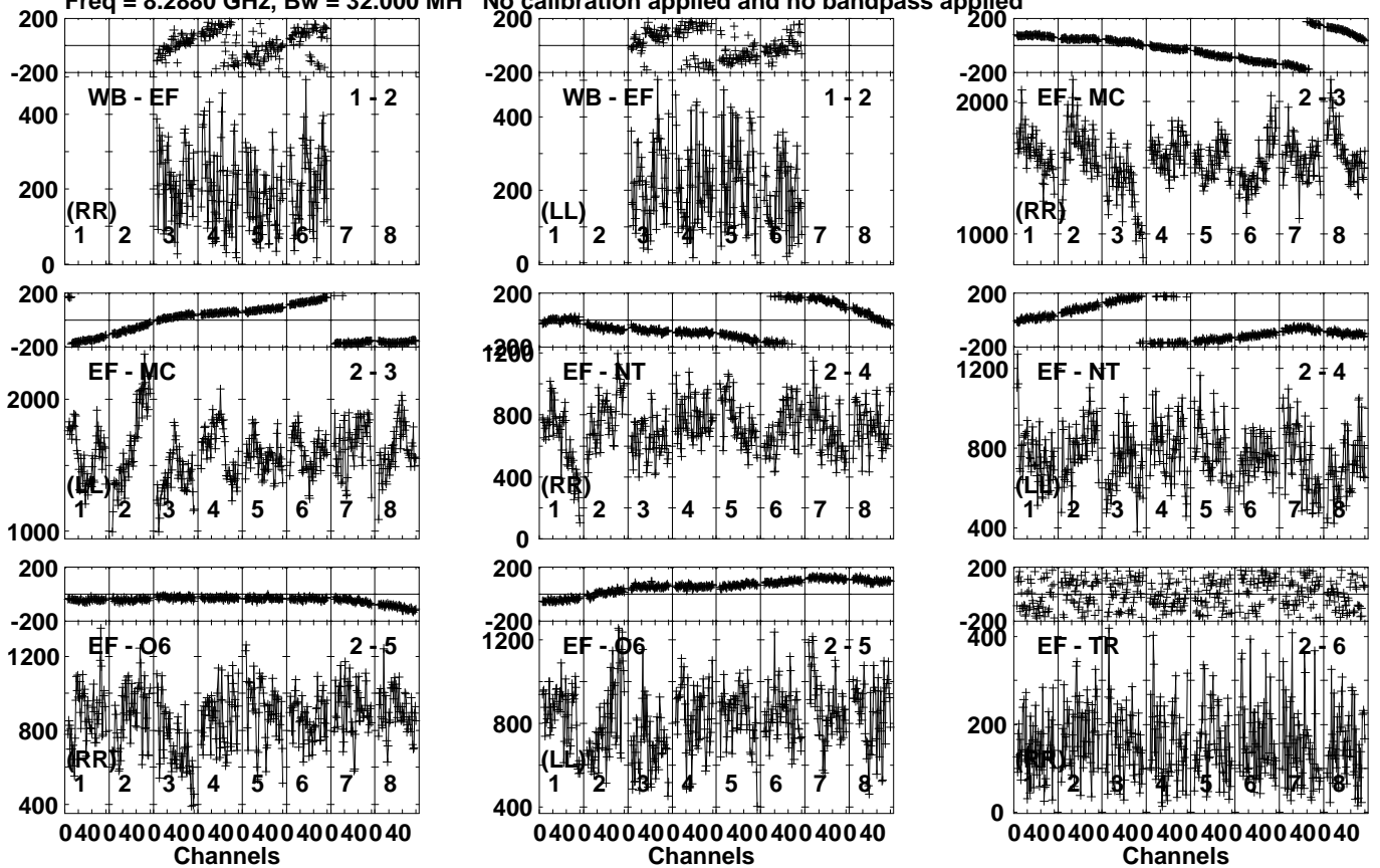
Lower frame: Micro Ampl Jy Top frame: Phas deg Vector averaged cross-power spectrum Several baselines displayed Timerange: 00/04:52:01 to 00/04:53:59
