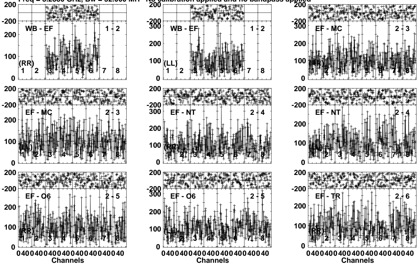
Lower frame: Micro Ampl Jy Top frame: Phas deg Vector averaged cross-power spectrum Several baselines displayed Timerange: 00/03:51:01 to 00/03:53:59
