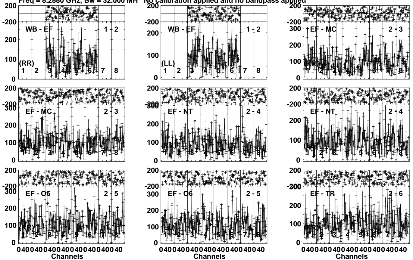
Lower frame: Micro Ampl Jy Top frame: Phas deg Vector averaged cross-power spectrum Several baselines displayed Timerange: 00/03:56:33 to 00/03:59:29
