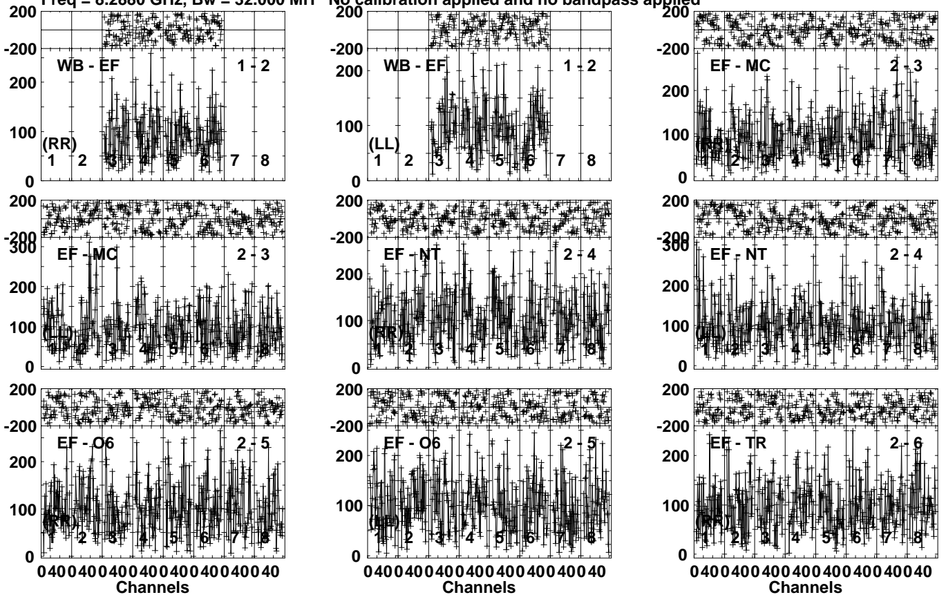
Lower frame: Micro Ampl Jy Top frame: Phas deg Vector averaged cross-power spectrum Several baselines displayed Timerange: 00/03:25:03 to 00/03:27:59
