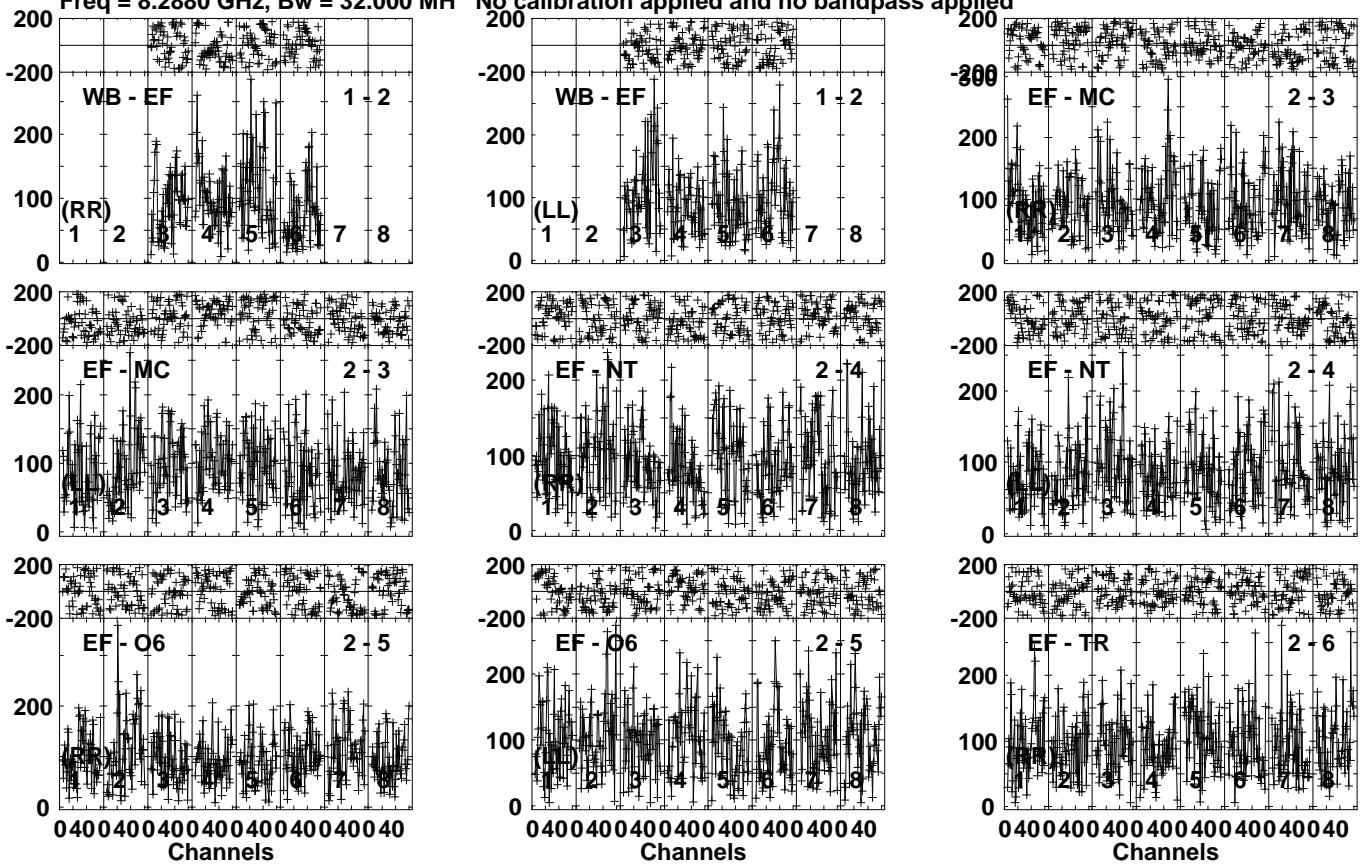
Lower frame: Micro Ampl Jy Top frame: Phas deg Vector averaged cross-power spectrum Several baselines displayed Timerange: 00/01:39:33 to 00/01:42:29
