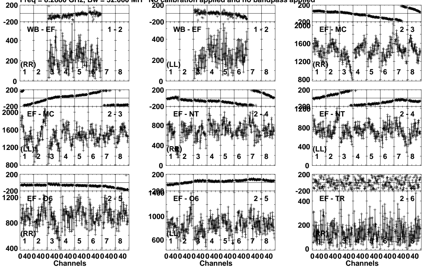
Lower frame: Micro Ampl Jy Top frame: Phas deg Vector averaged cross-power spectrum Several baselines displayed Timerange: 00/02:14:01 to 00/02:15:59
