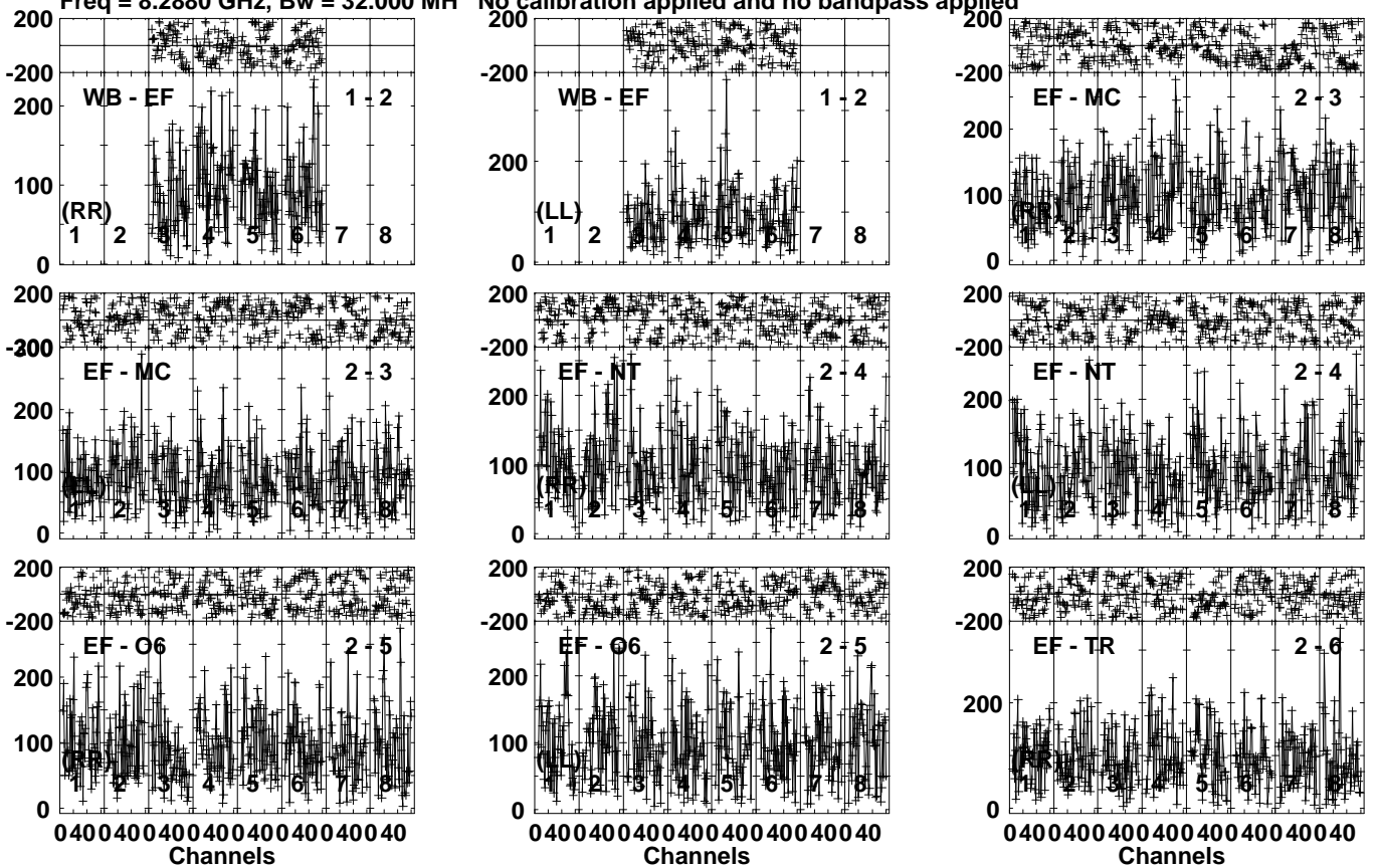
Lower frame: Micro Ampl Jy Top frame: Phas deg Vector averaged cross-power spectrum Several baselines displayed Timerange: 00/03:40:31 to 00/03:43:29
