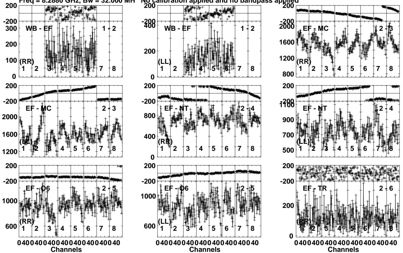
Lower frame: Micro Ampl Jy Top frame: Phas deg Vector averaged cross-power spectrum Several baselines displayed Timerange: 00/04:26:01 to 00/04:27:59
