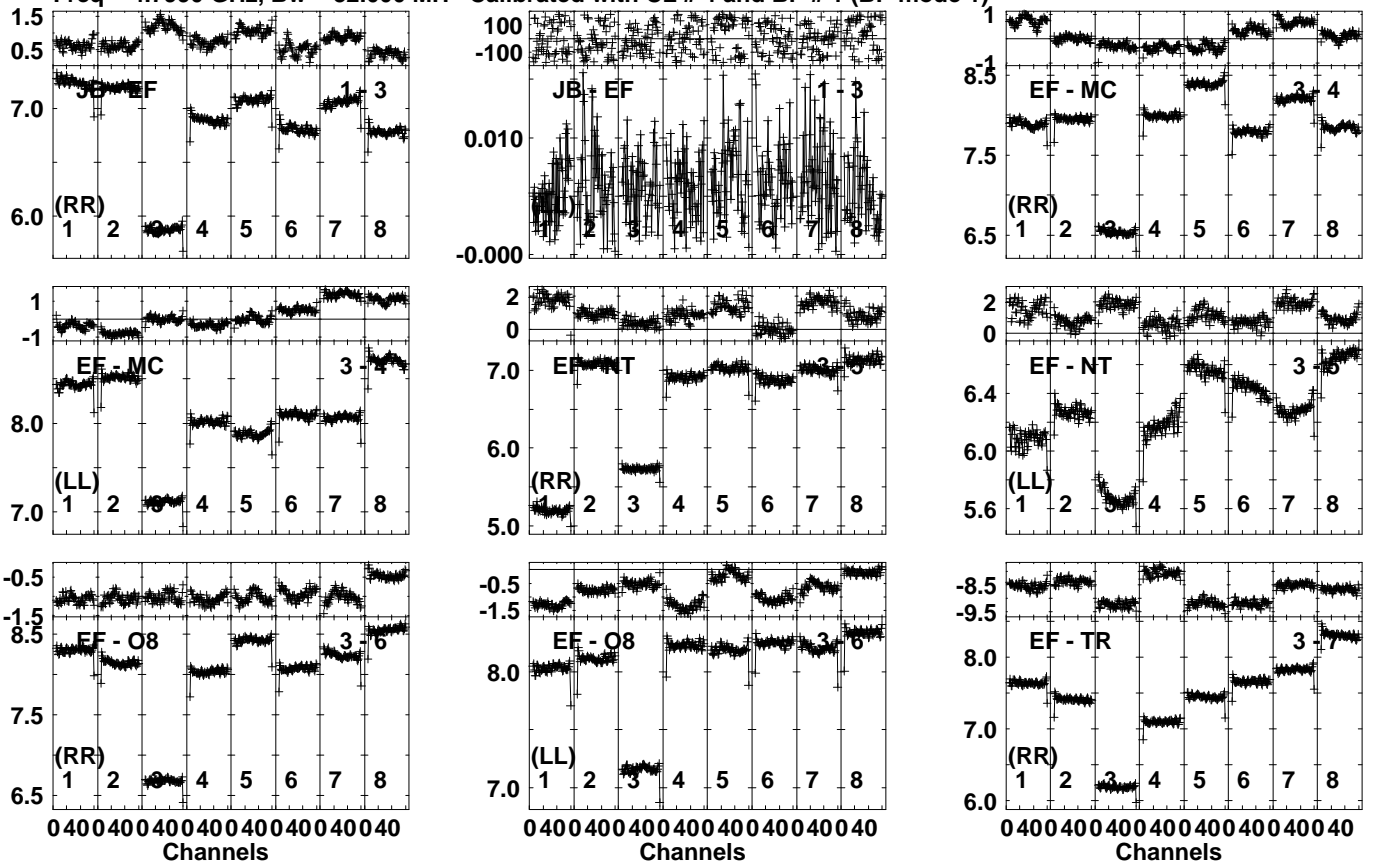
Lower frame: Ampl Jy Top frame: Phas deg Vector averaged cross-power spectrum Several baselines displayed Timerange: 00/16:30:01 to 00/16:34:59
