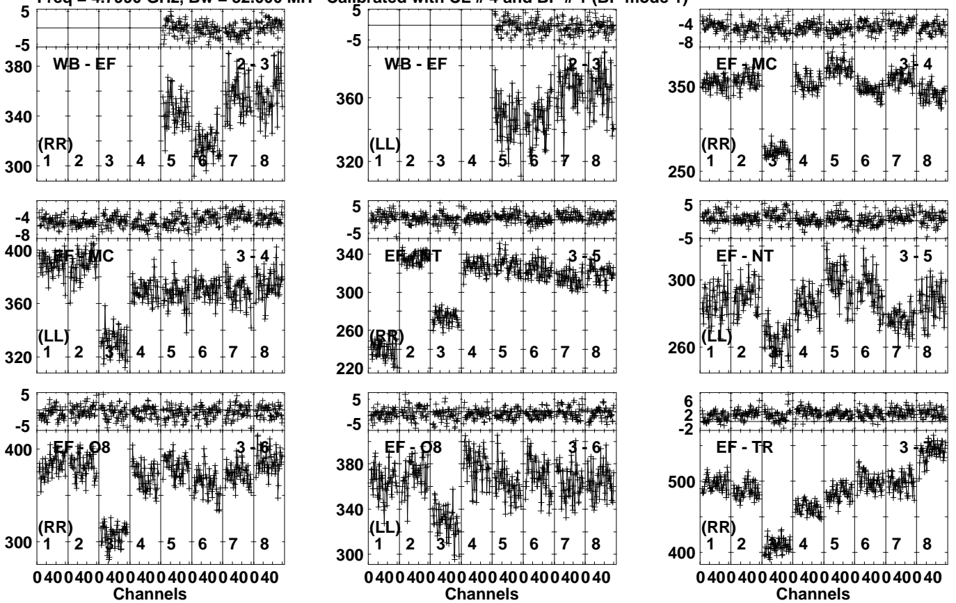
Lower frame: Milli Ampl Jy Top frame: Phas deg Vector averaged cross-power spectrum Several baselines displayed Timerange: 00:16:49:31 to 00:16:51:29
