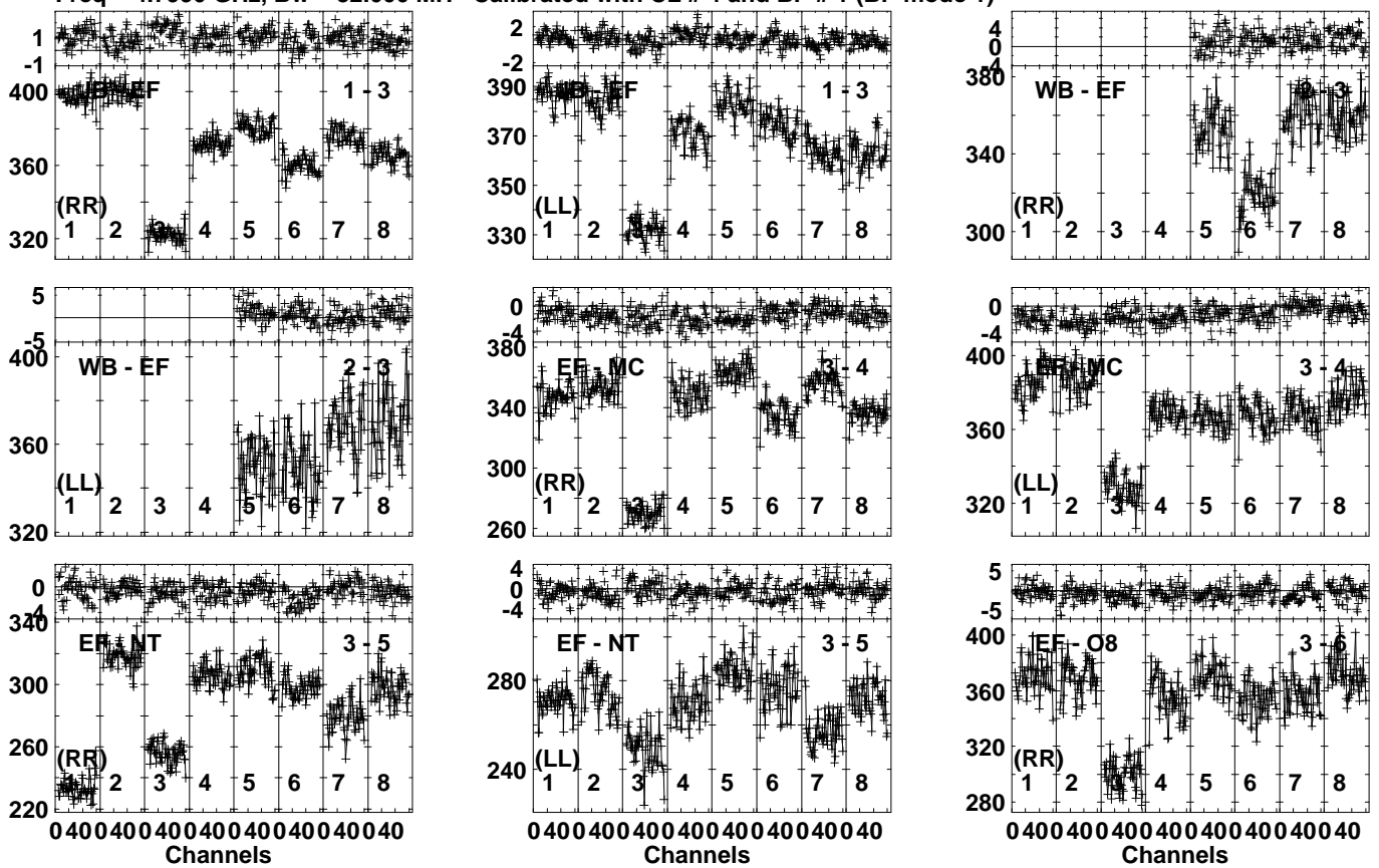
Lower frame: Milli Ampl Jy Top frame: Phas deg Vector averaged cross-power spectrum Several baselines displayed Timerange: 00:18:52:01 to 00:18:53:59
