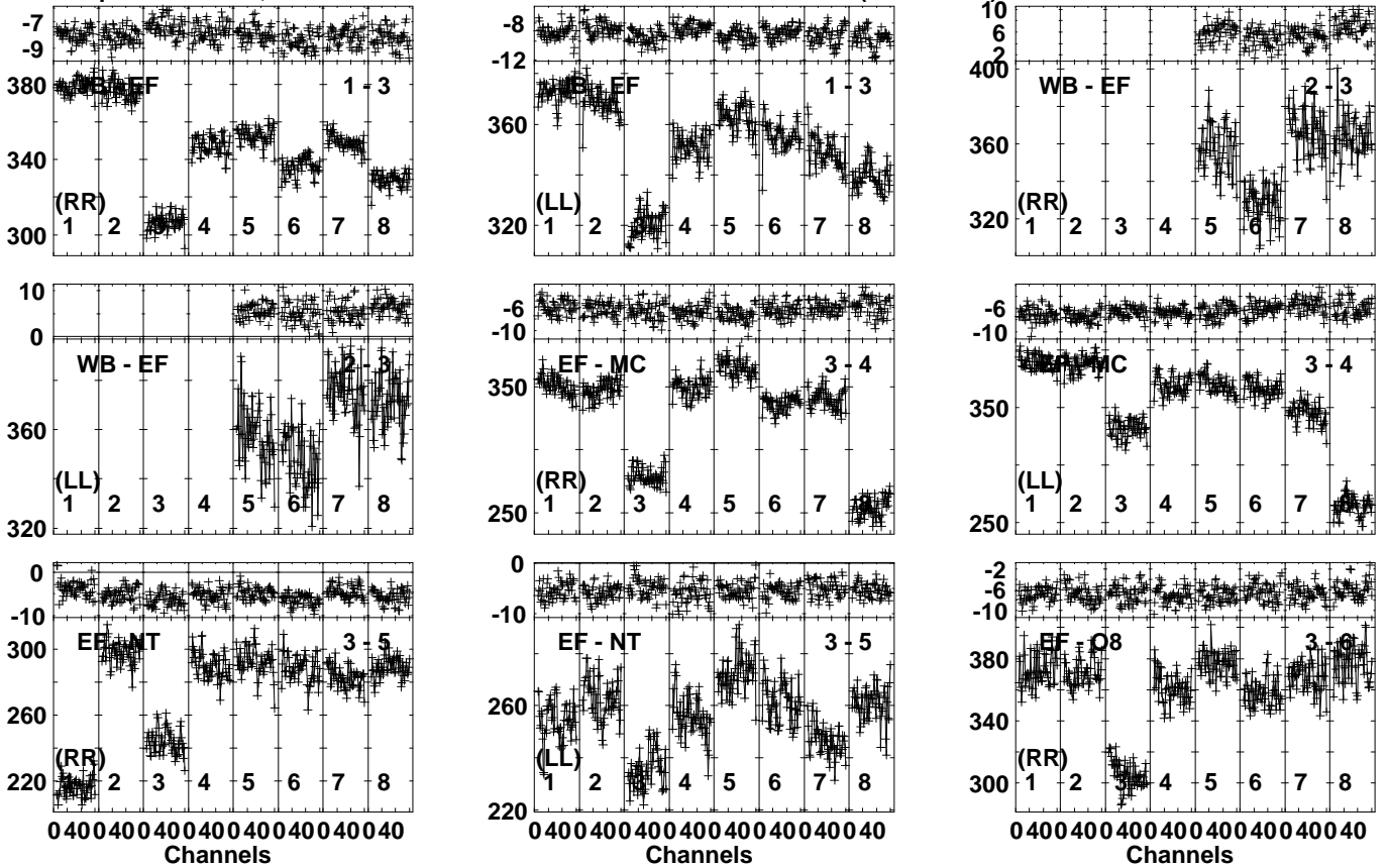
Lower frame: Milli Ampl Jy Top frame: Phas deg Vector averaged cross-power spectrum Several baselines displayed Timerange: 00/20:05:31 to 00/20:07:29
