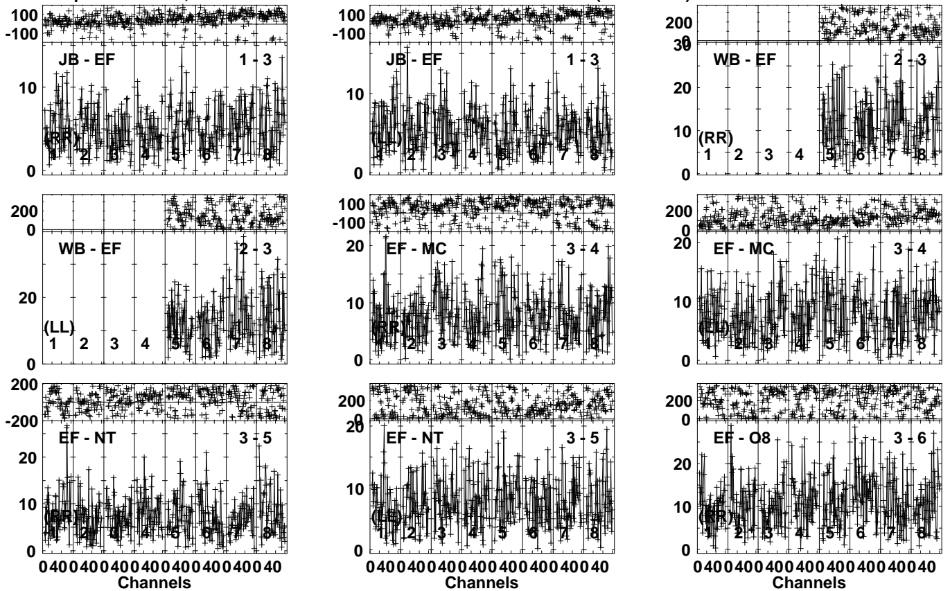
Lower frame: Milli Ampl Jy Top frame: Phas deg Vector averaged cross-power spectrum Several baselines displayed Timerange: 00/17:49:31 to 00/17:52:29
