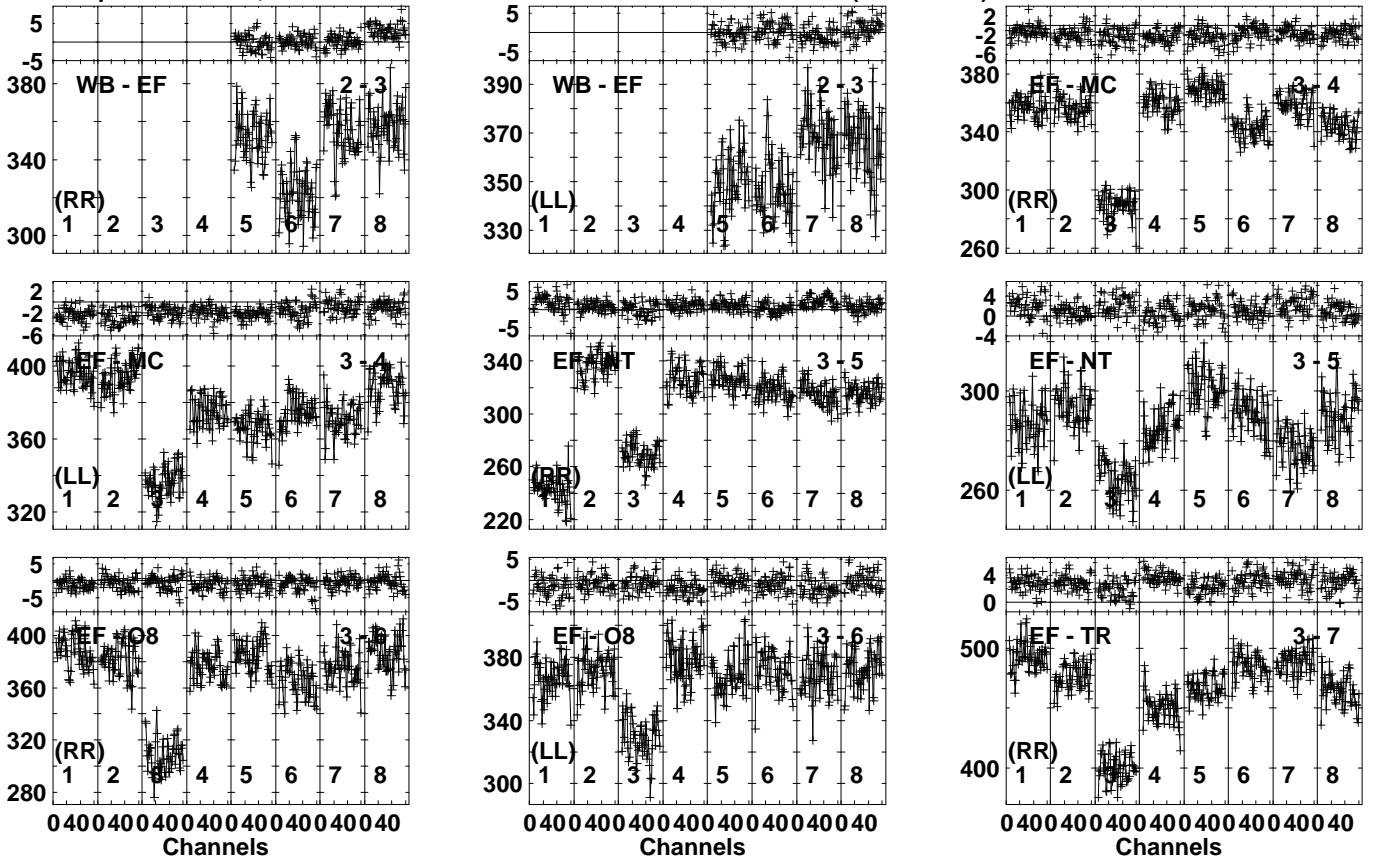
Lower frame: Milli Ampl Jy Top frame: Phas deg Vector averaged cross-power spectrum Several baselines displayed Timerange: 00/17:00:01 to 00/17:01:59
