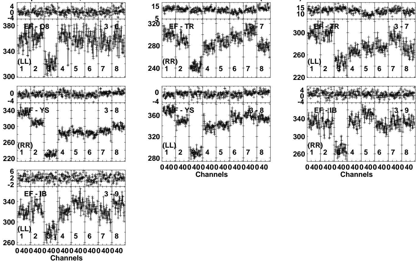
Lower frame: Milli Ampl Jy Top frame: Phas deg Vector averaged cross-power spectrum Several baselines displayed Timerange: 00:18:41:31 to 00:18:43:29
