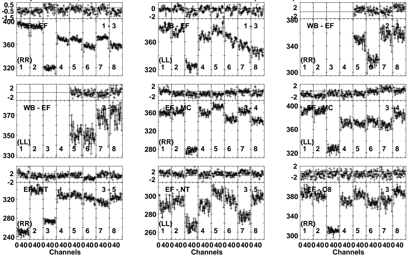
Lower frame: Milli Ampl Jy Top frame: Phas deg Vector averaged cross-power spectrum Several baselines displayed Timerange: 00/16:36:01 to 00/16:40:59
