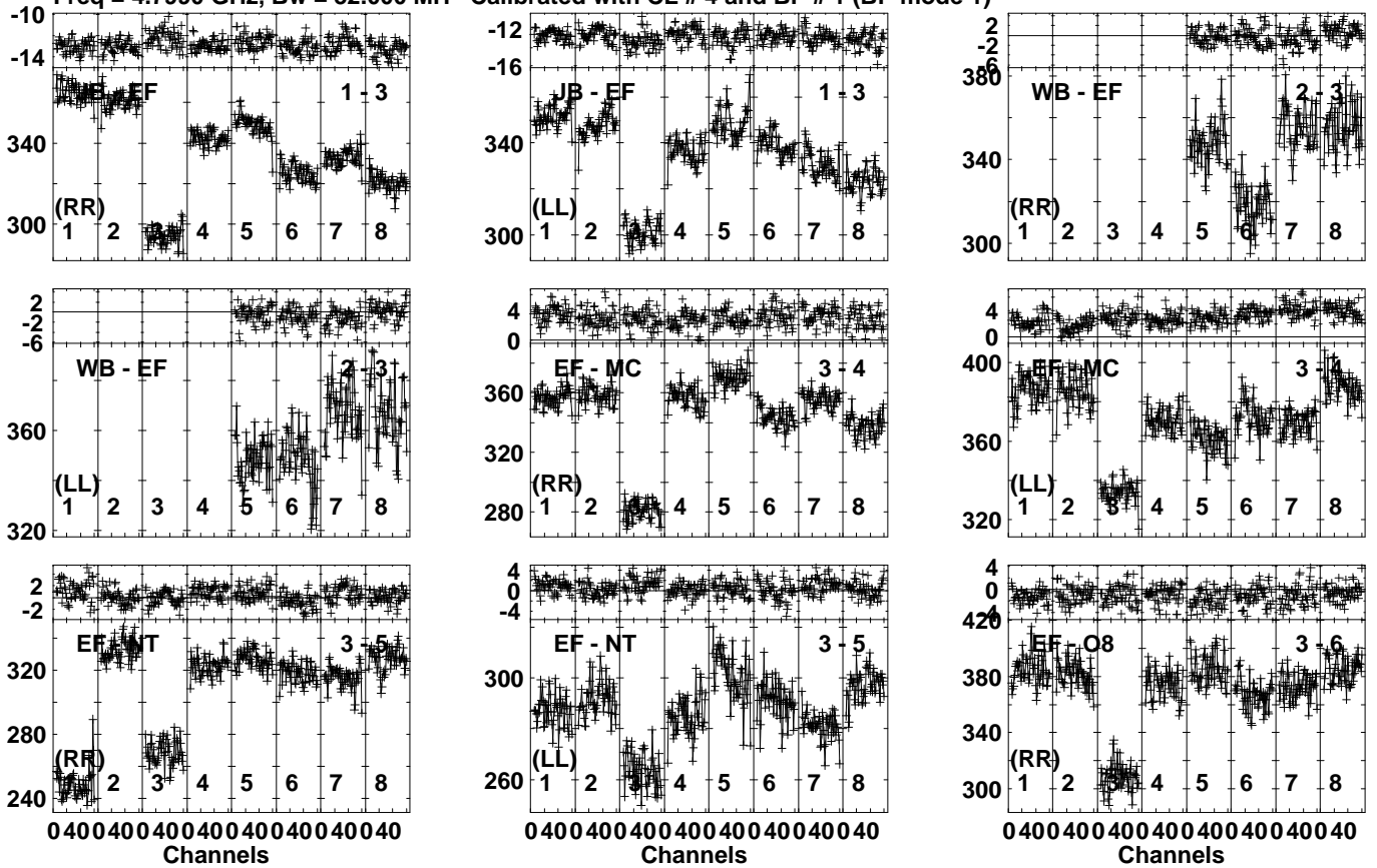
Lower frame: Milli Ampl Jy Top frame: Phas deg Vector averaged cross-power spectrum Several baselines displayed Timerange: 00/17:05:31 to 00/17:07:29
