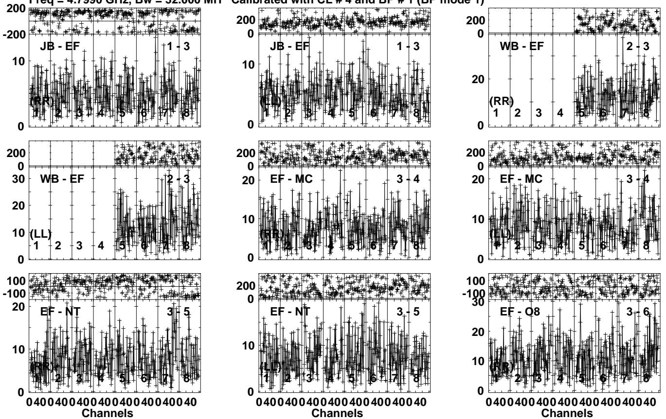
Lower frame: Milli Ampl Jy Top frame: Phas deg Vector averaged cross-power spectrum Several baselines displayed Timerange: 00/18:00:01 to 00/18:02:59
