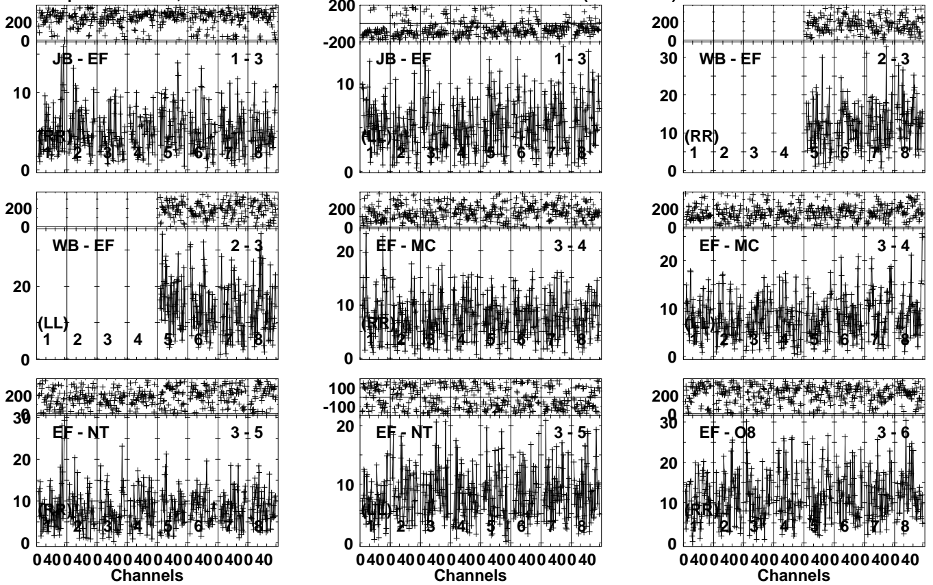
Lower frame: Milli Ampl Jy Top frame: Phas deg Vector averaged cross-power spectrum Several baselines displayed Timerange: 00/19:20:01 to 00/19:22:59
