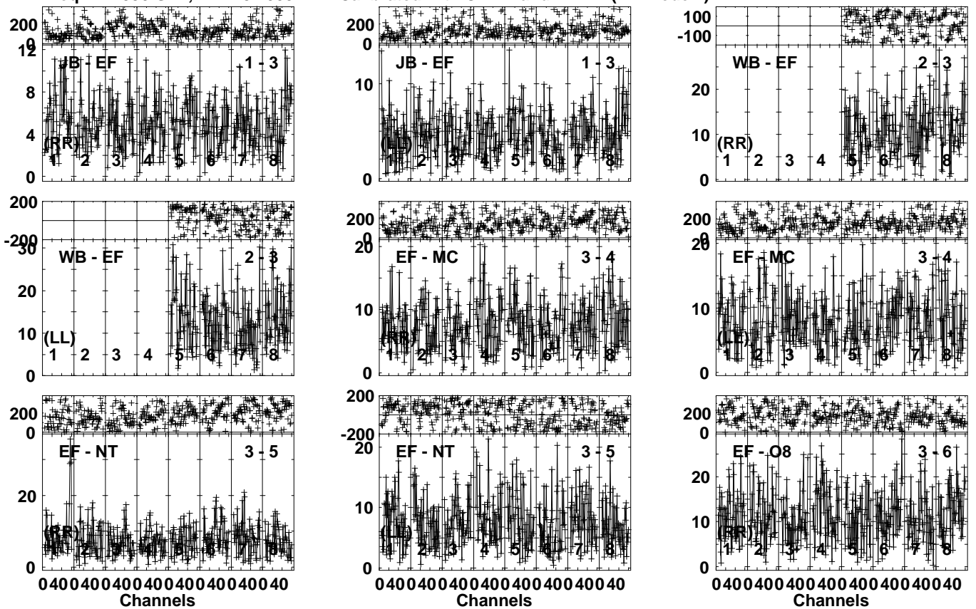
Lower frame: Milli Ampl Jy Top frame: Phas deg Vector averaged cross-power spectrum Several baselines displayed Timerange: 00/18:21:03 to 00/18:23:59
