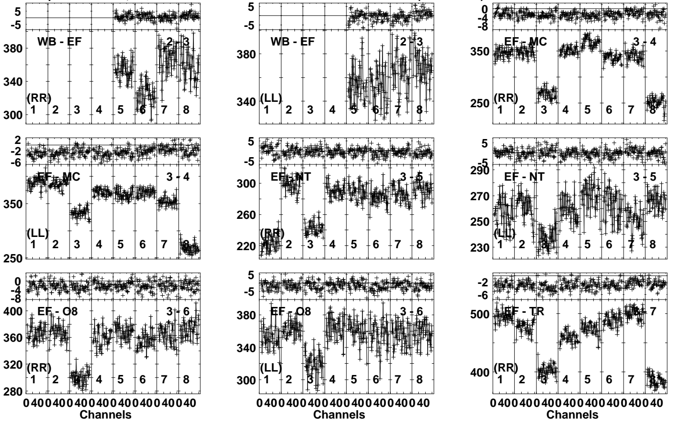
Lower frame: Milli Ampl Jy Top frame: Phas deg Vector averaged cross-power spectrum Several baselines displayed Timerange: 00/20:00:01 to 00/20:01:59
