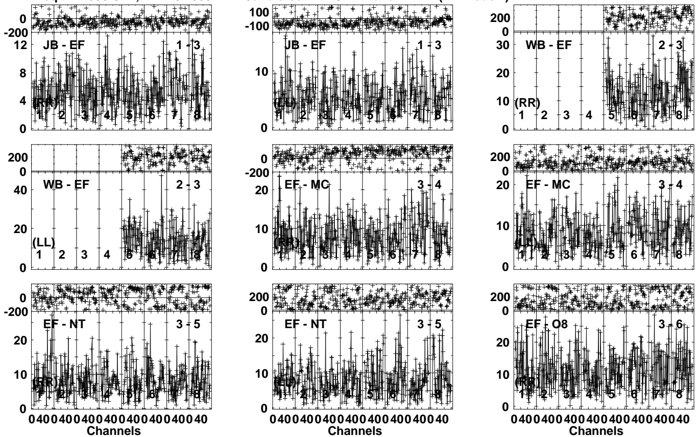
Lower frame: Milli Ampl Jy Top frame: Phas deg Vector averaged cross-power spectrum Several baselines displayed Timerange: 00/20:18:03 to 00/20:20:59
