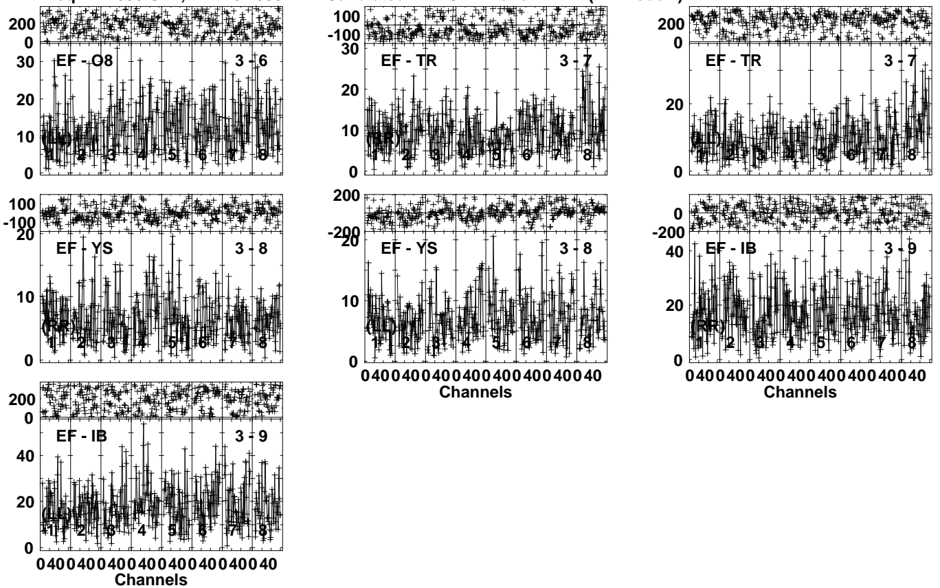
Lower frame: Milli Ampl Jy Top frame: Phas deg Vector averaged cross-power spectrum Several baselines displayed Timerange: 00/19:41:01 to 00/19:43:59
