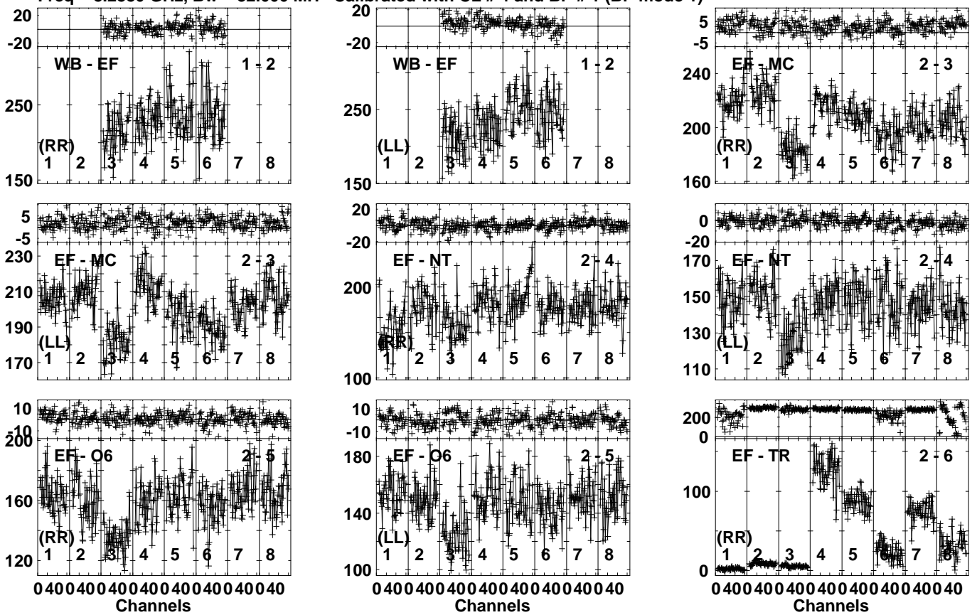
Lower frame: Milli Ampl Jy Top frame: Phas deg Vector averaged cross-power spectrum Several baselines displayed Timerange: 00:17:40:31 to 00:17:42:29
