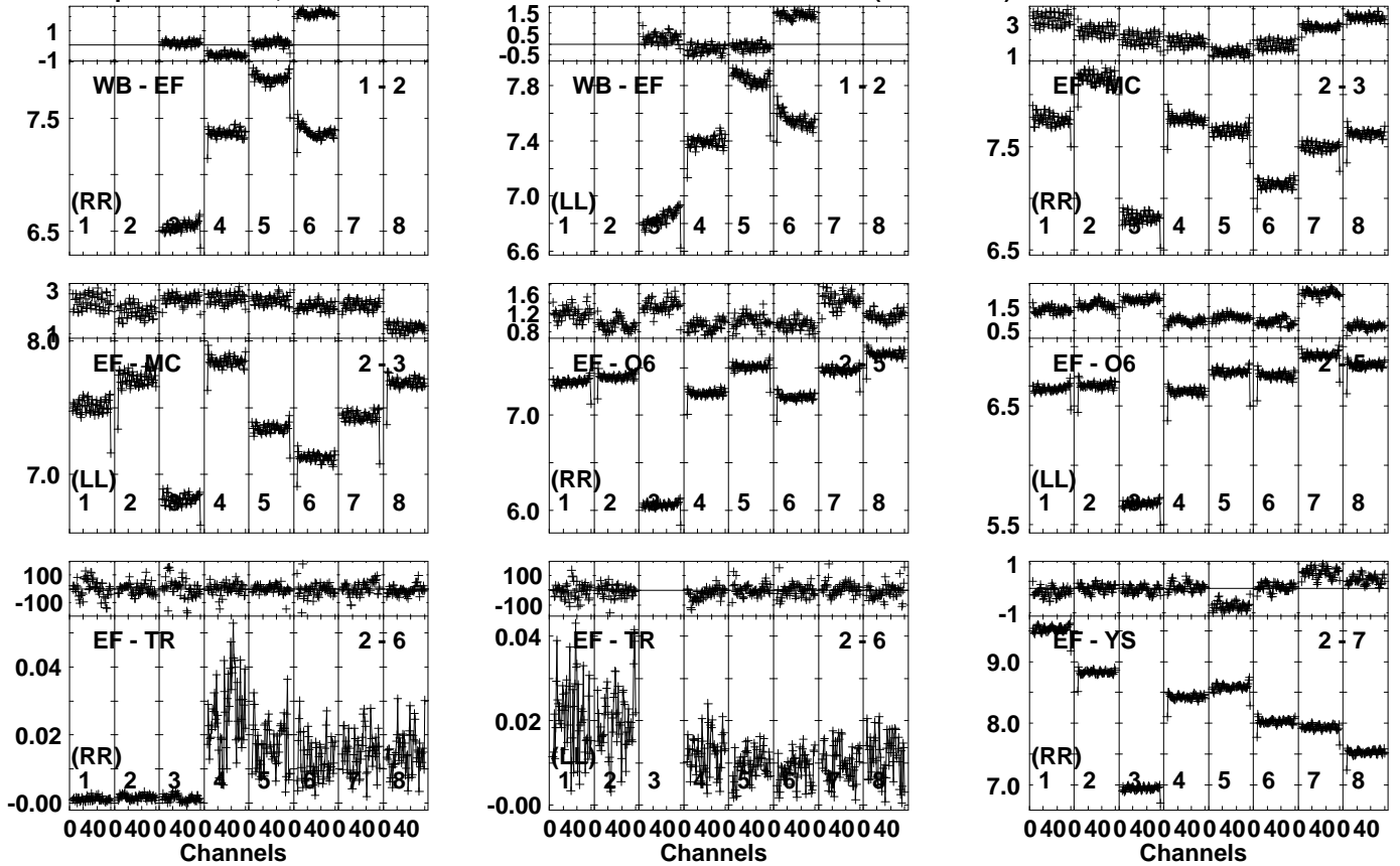
Lower frame: Ampl Jy Top frame: Phas deg Vector averaged cross-power spectrum Several baselines displayed Timerange: 00/20:54:01 to 00/20:59:59
