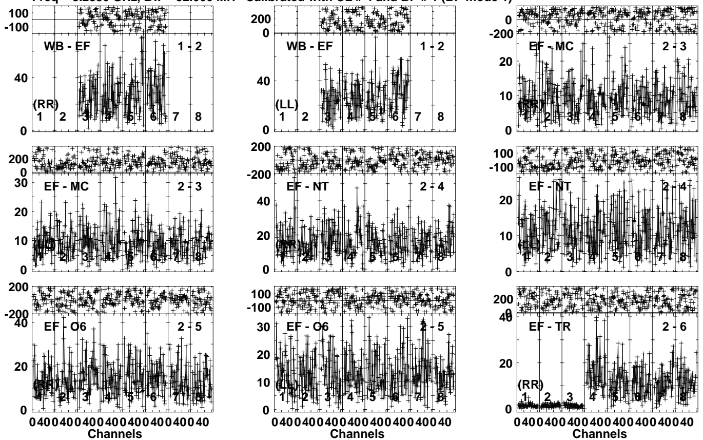
Lower frame: Milli Ampl Jy Top frame: Phas deg Vector averaged cross-power spectrum Several baselines displayed Timerange: 00/17:42:31 to 00/17:45:29
