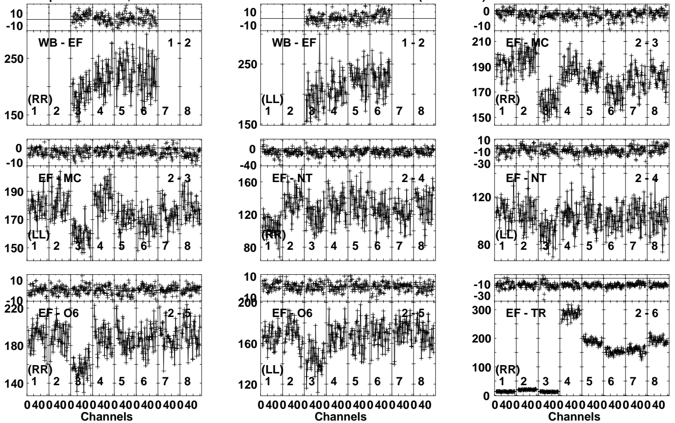
Lower frame: Milli Ampl Jy Top frame: Phas deg Vector averaged cross-power spectrum Several baselines displayed Timerange: 00:18:49:01 to 00:18:50:59
