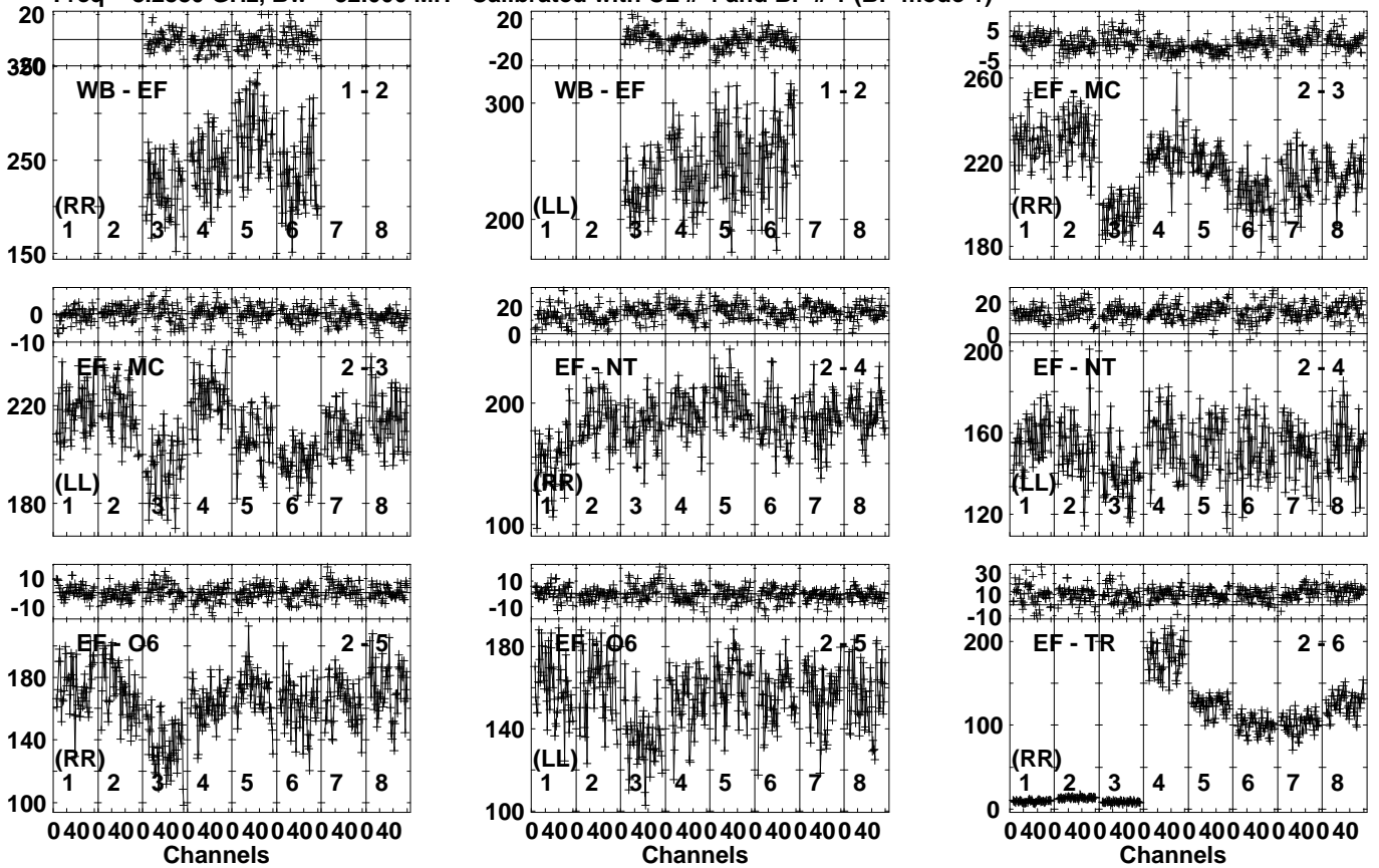
Lower frame: Milli Ampl Jy Top frame: Phas deg Vector averaged cross-power spectrum Several baselines displayed Timerange: 00:17:30:01 to 00:17:31:59
