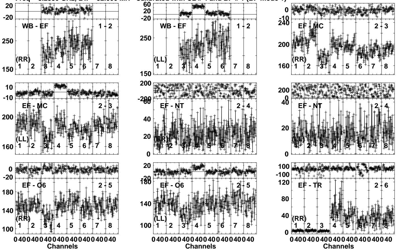
Lower frame: Milli Ampl Jy Top frame: Phas deg Vector averaged cross-power spectrum Several baselines displayed Timerange: 00/18:01:31 to 00/18:03:29
