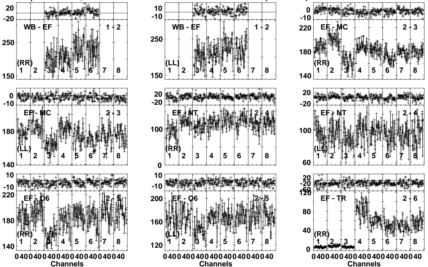
Lower frame: Milli Ampl Jy Top frame: Phas deg Vector averaged cross-power spectrum Several baselines displayed Timerange: 00/18:43:31 to 00/18:45:29
