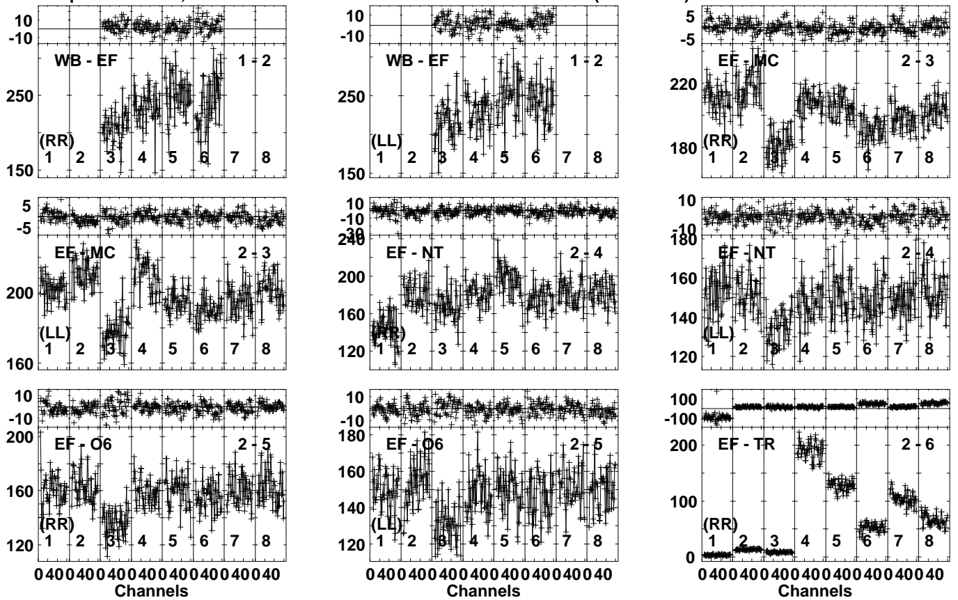
Lower frame: Milli Ampl Jy Top frame: Phas deg Vector averaged cross-power spectrum Several baselines displayed Timerange: 00/17:46:01 to 00/17:47:59
