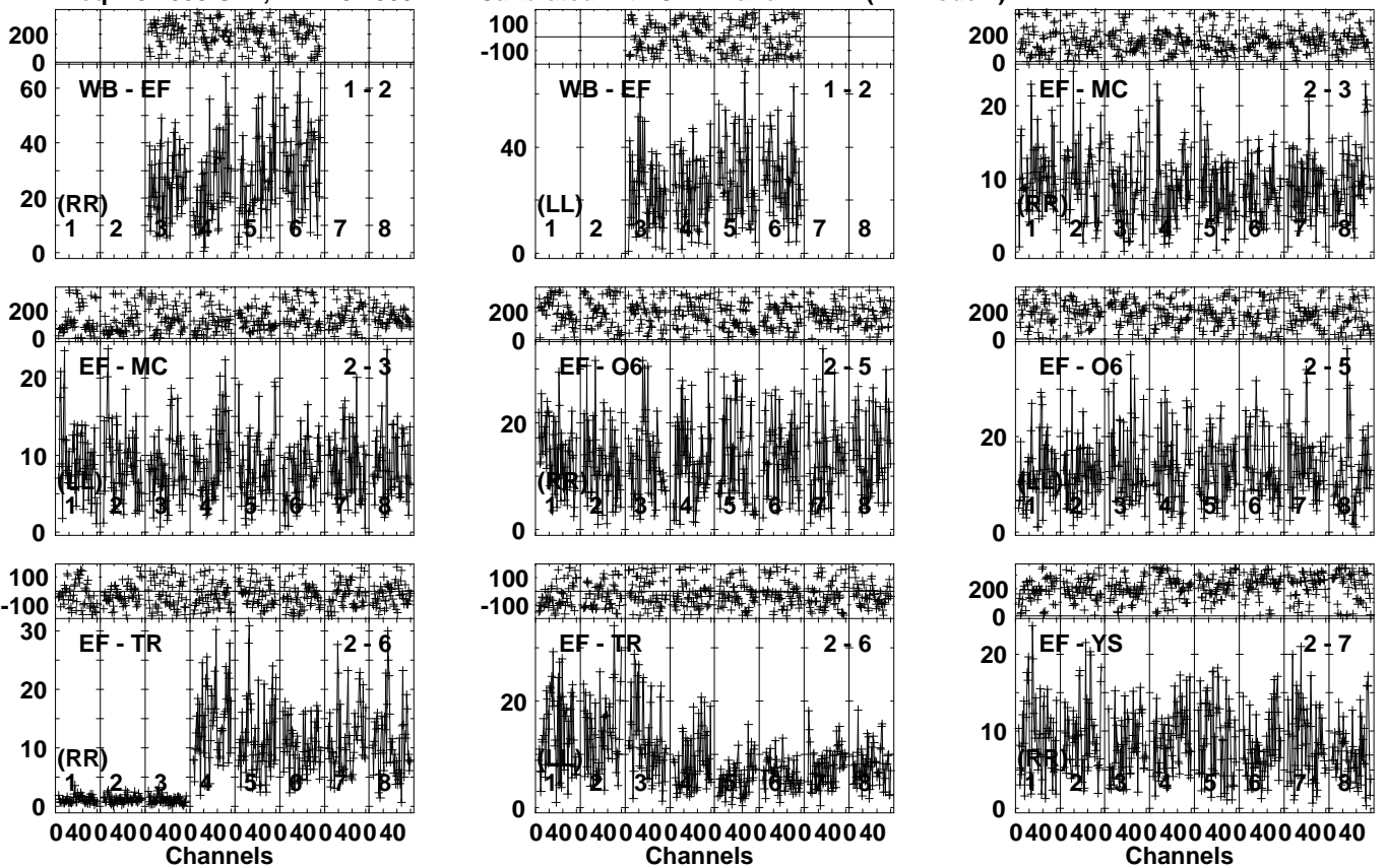
Lower frame: Milli Ampl Jy Top frame: Phas deg Vector averaged cross-power spectrum Several baselines displayed Timerange: 00/19:45:03 to 00/19:47:59
