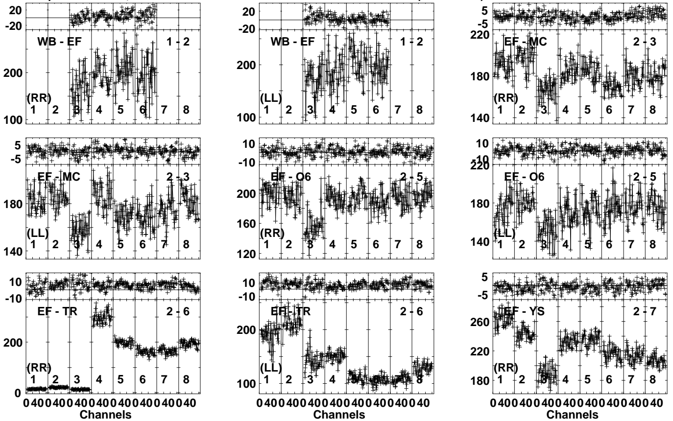
Lower frame: Milli Ampl Jy Top frame: Phas deg Vector averaged cross-power spectrum Several baselines displayed Timerange: 00:19:48:01 to 00:19:49:59
