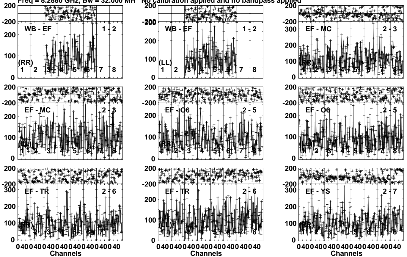
Lower frame: Micro Ampl Jy Top frame: Phas deg Vector averaged cross-power spectrum Several baselines displayed Timerange: 00/20:32:01 to 00/20:34:59
