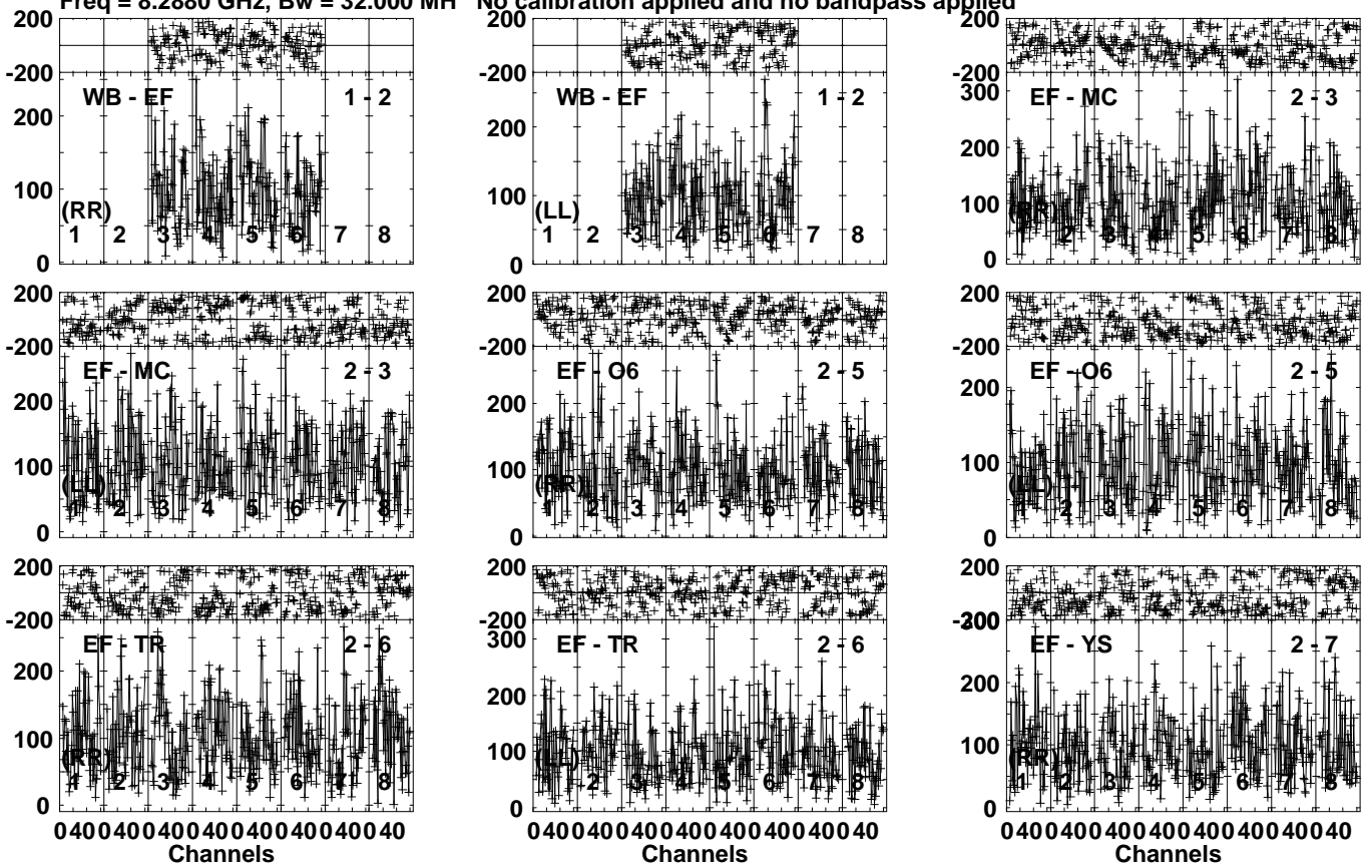
Lower frame: Micro Ampl Jy Top frame: Phas deg Vector averaged cross-power spectrum Several baselines displayed Timerange: 00/20:27:03 to 00/20:29:59
