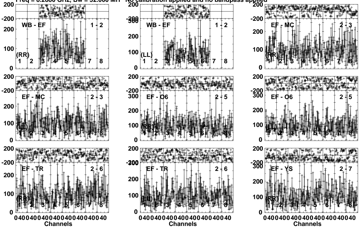
Lower frame: Micro Ampl Jy Top frame: Phas deg Vector averaged cross-power spectrum Several baselines displayed Timerange: 00/19:50:01 to 00/19:52:59
