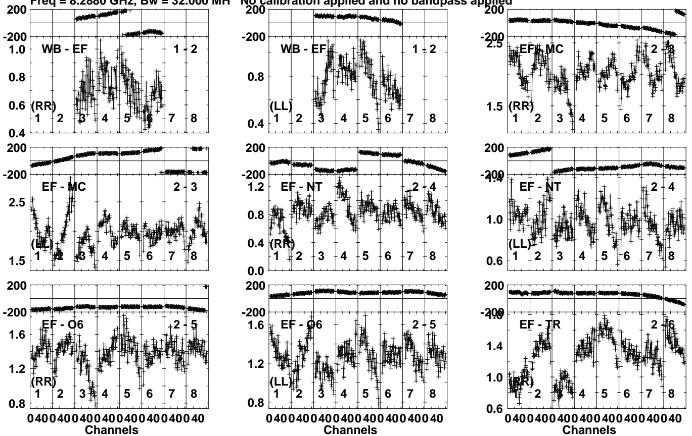
Lower frame: Milli Ampl Jy Top frame: Phas deg Vector averaged cross-power spectrum Several baselines displayed Timerange: 00/19:22:01 to 00/19:23:59
