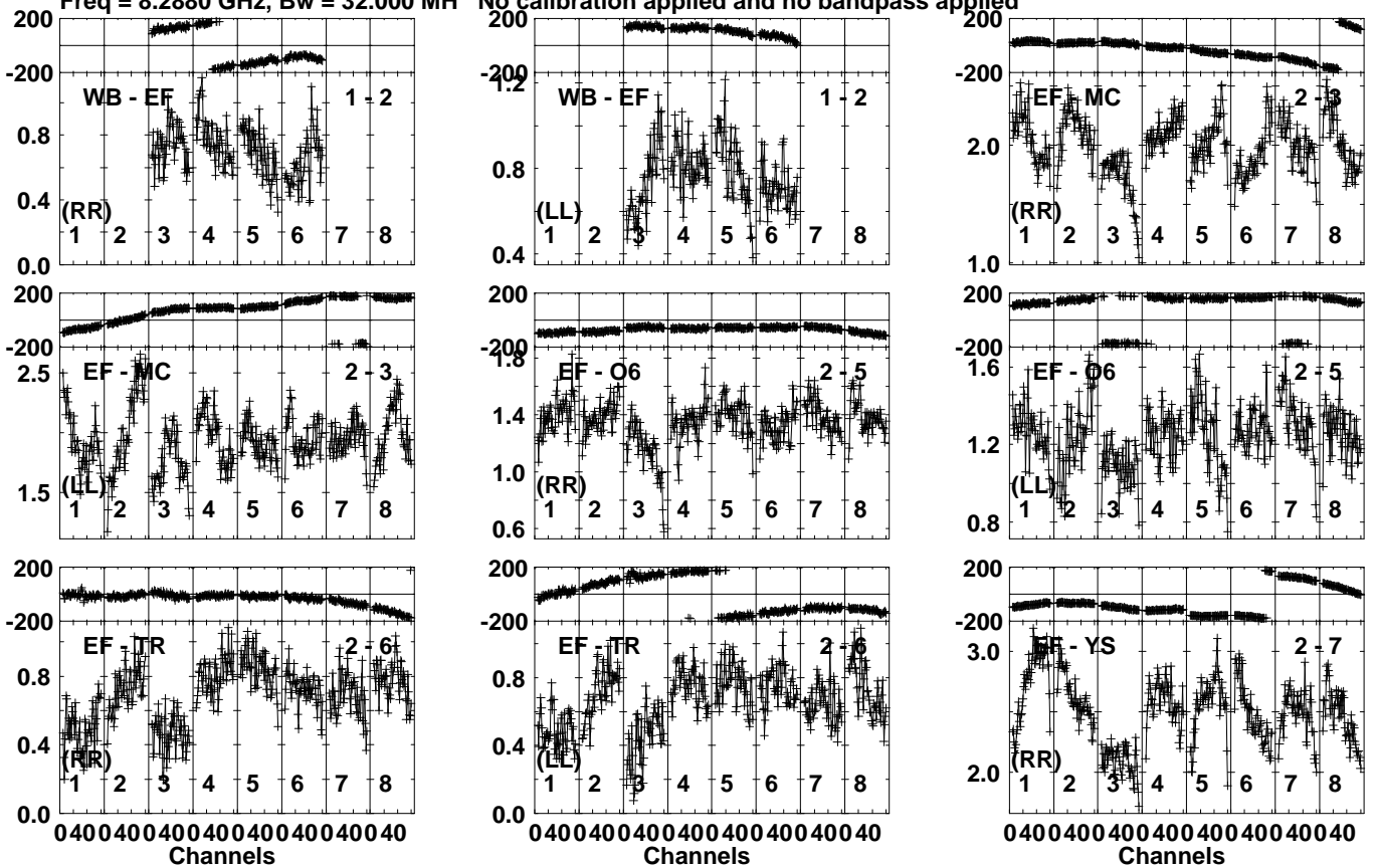
Lower frame: Milli Ampl Jy Top frame: Phas deg Vector averaged cross-power spectrum Several baselines displayed Timerange: 00/18:33:01 to 00/18:34:59
