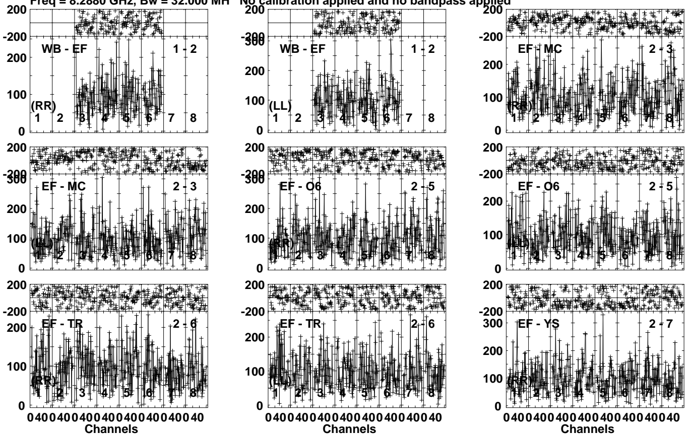
Lower frame: Micro Ampl Jy Top frame: Phas deg Vector averaged cross-power spectrum Several baselines displayed Timerange: 00/20:21:31 to 00/20:24:29
