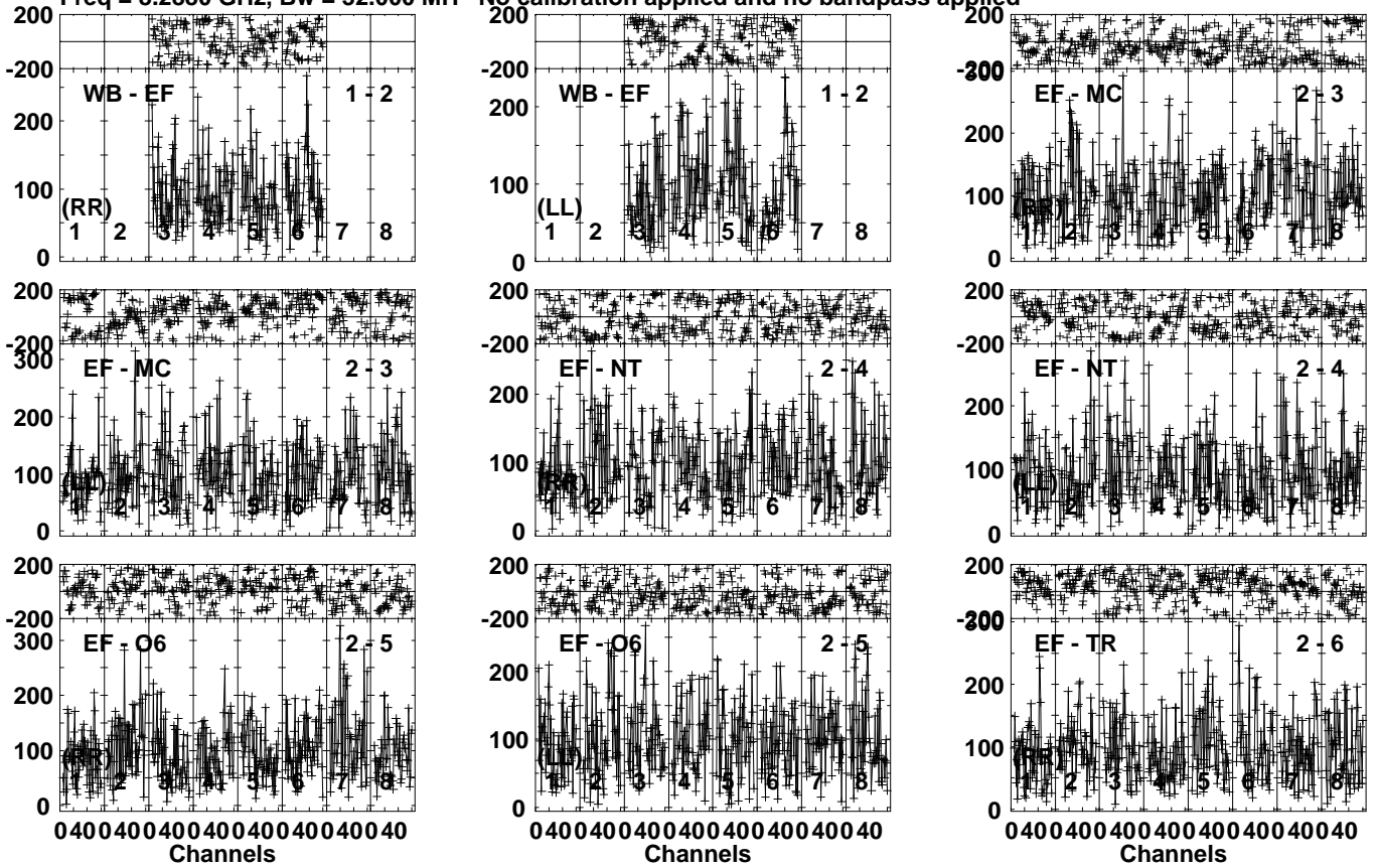
Lower frame: Micro Ampl Jy Top frame: Phas deg Vector averaged cross-power spectrum Several baselines displayed Timerange: 00/17:16:31 to 00/17:19:29
