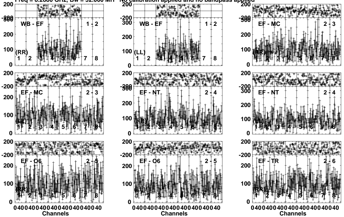
Lower frame: Micro Ampl Jy Top frame: Phas deg Vector averaged cross-power spectrum Several baselines displayed Timerange: 00/17:32:01 to 00/17:34:59
