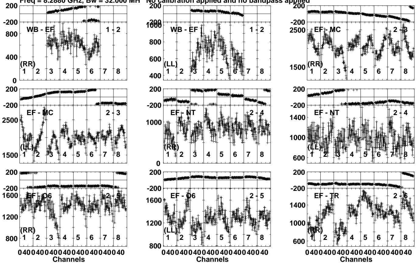
Lower frame: Micro Ampl Jy Top frame: Phas deg Vector averaged cross-power spectrum Several baselines displayed Timerange: 00/19:32:31 to 00/19:34:29
