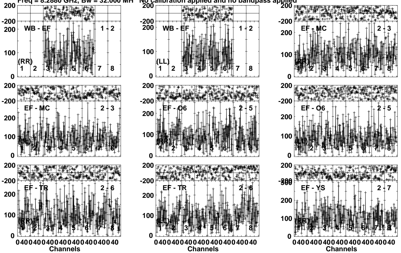
Lower frame: Micro Ampl Jy Top frame: Phas deg Vector averaged cross-power spectrum Several baselines displayed Timerange: 00/18:35:01 to 00/18:37:59
