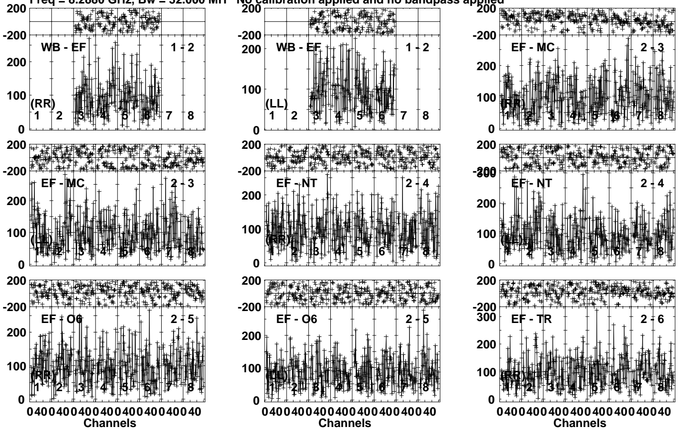
Lower frame: Micro Ampl Jy Top frame: Phas deg Vector averaged cross-power spectrum Several baselines displayed Timerange: 00/17:37:33 to 00/17:40:29
