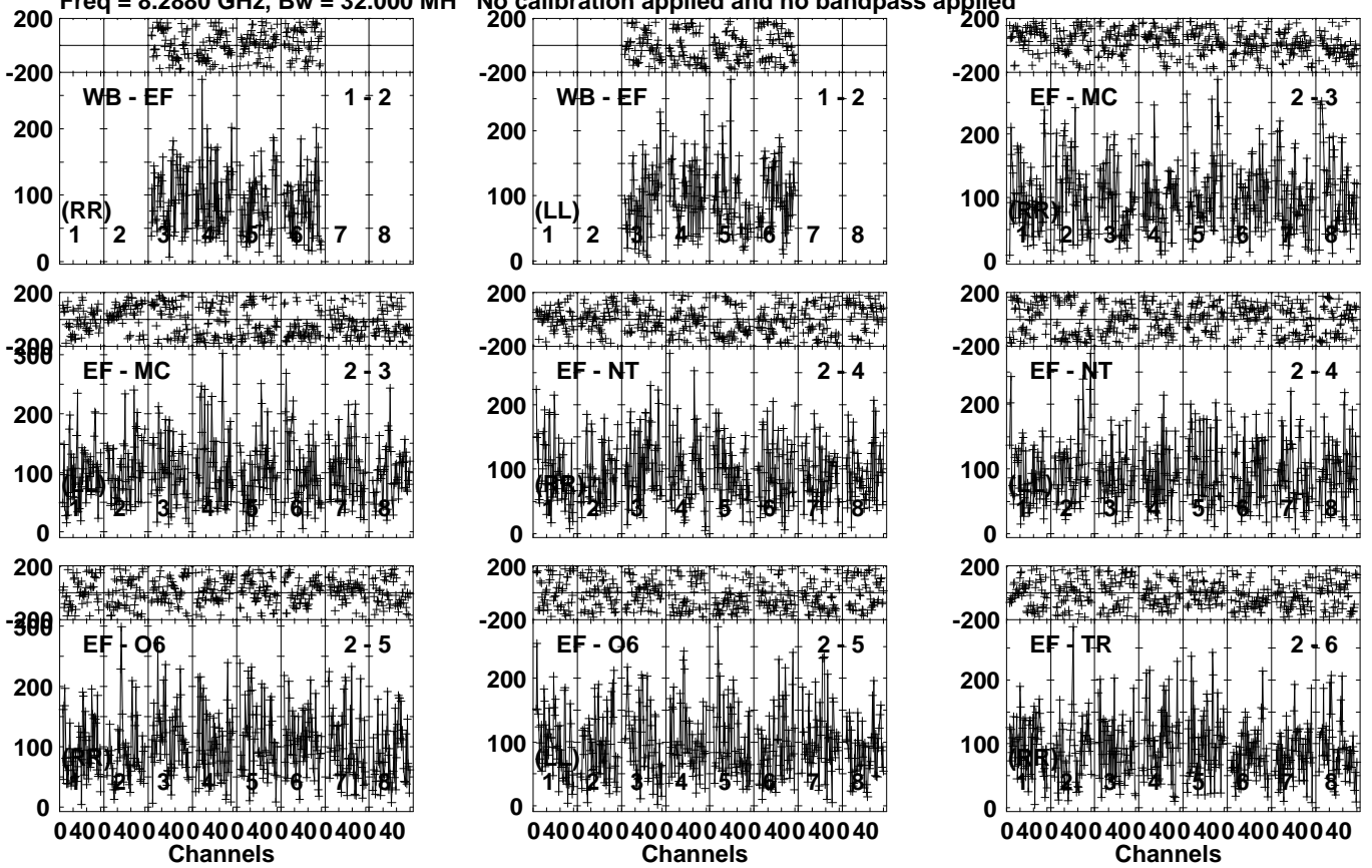
Lower frame: Micro Ampl Jy Top frame: Phas deg Vector averaged cross-power spectrum Several baselines displayed Timerange: 00/17:42:31 to 00/17:45:29
