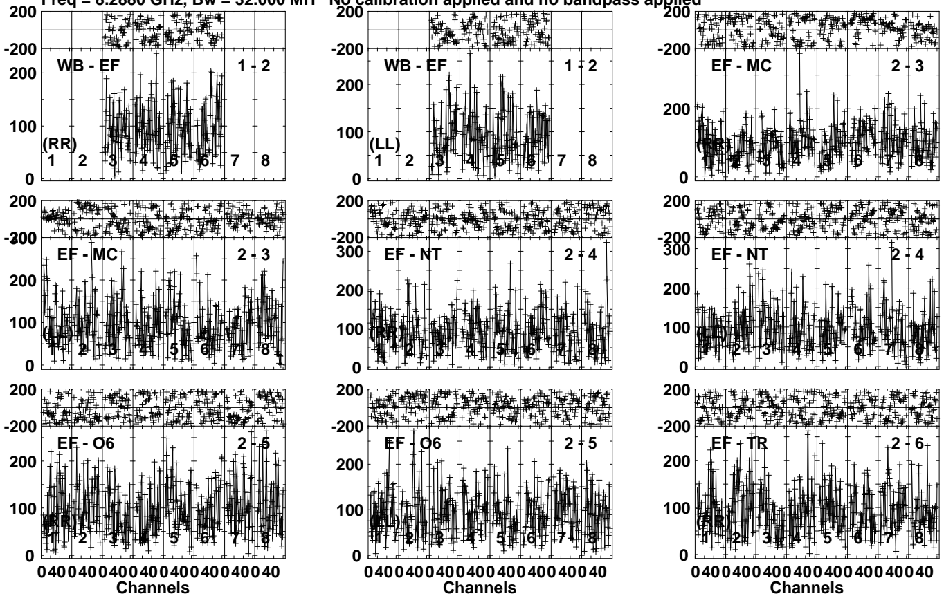
Lower frame: Micro Ampl Jy Top frame: Phas deg Vector averaged cross-power spectrum Several baselines displayed Timerange: 00/18:40:33 to 00/18:43:29
