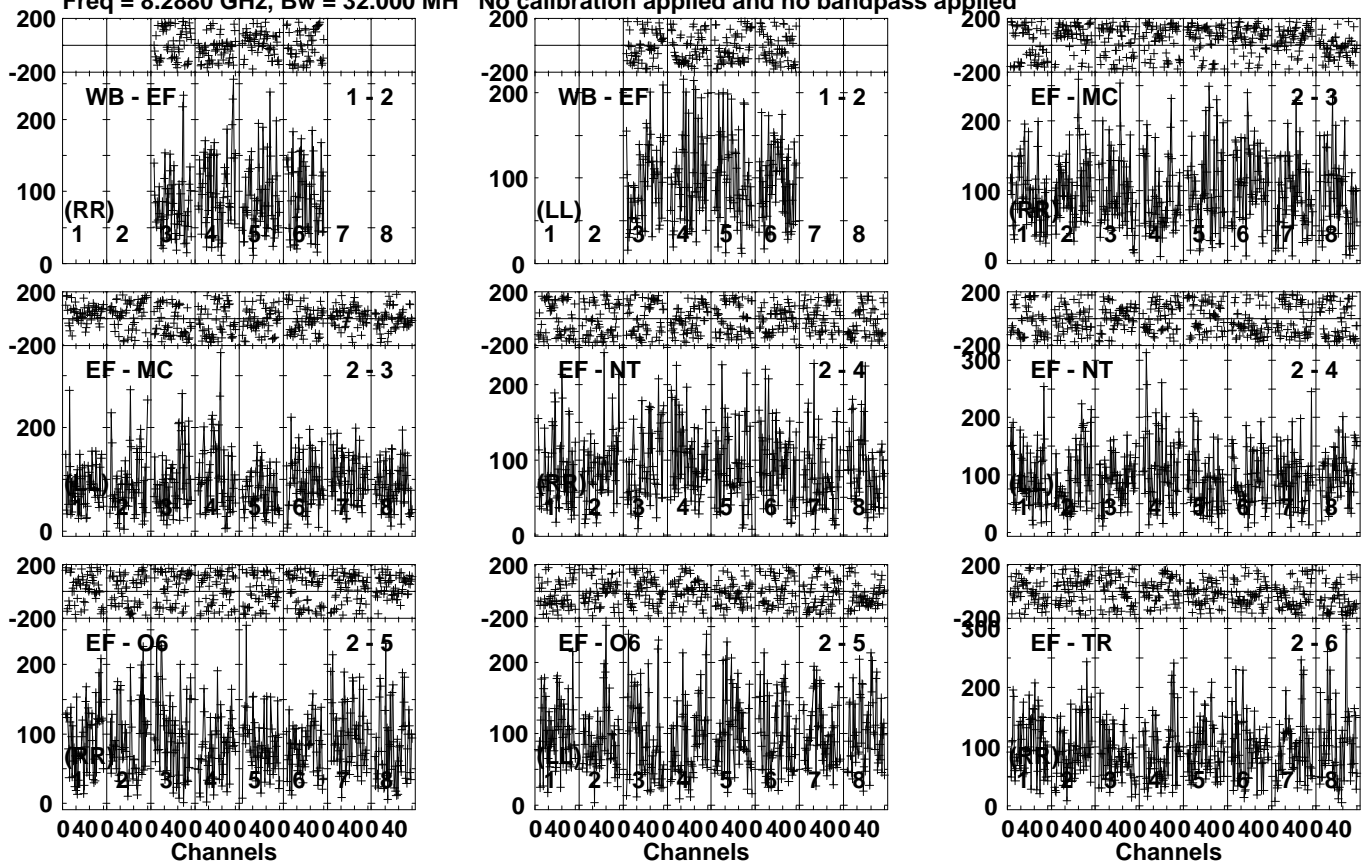
Lower frame: Micro Ampl Jy Top frame: Phas deg Vector averaged cross-power spectrum Several baselines displayed Timerange: 00/18:51:03 to 00/18:53:59
