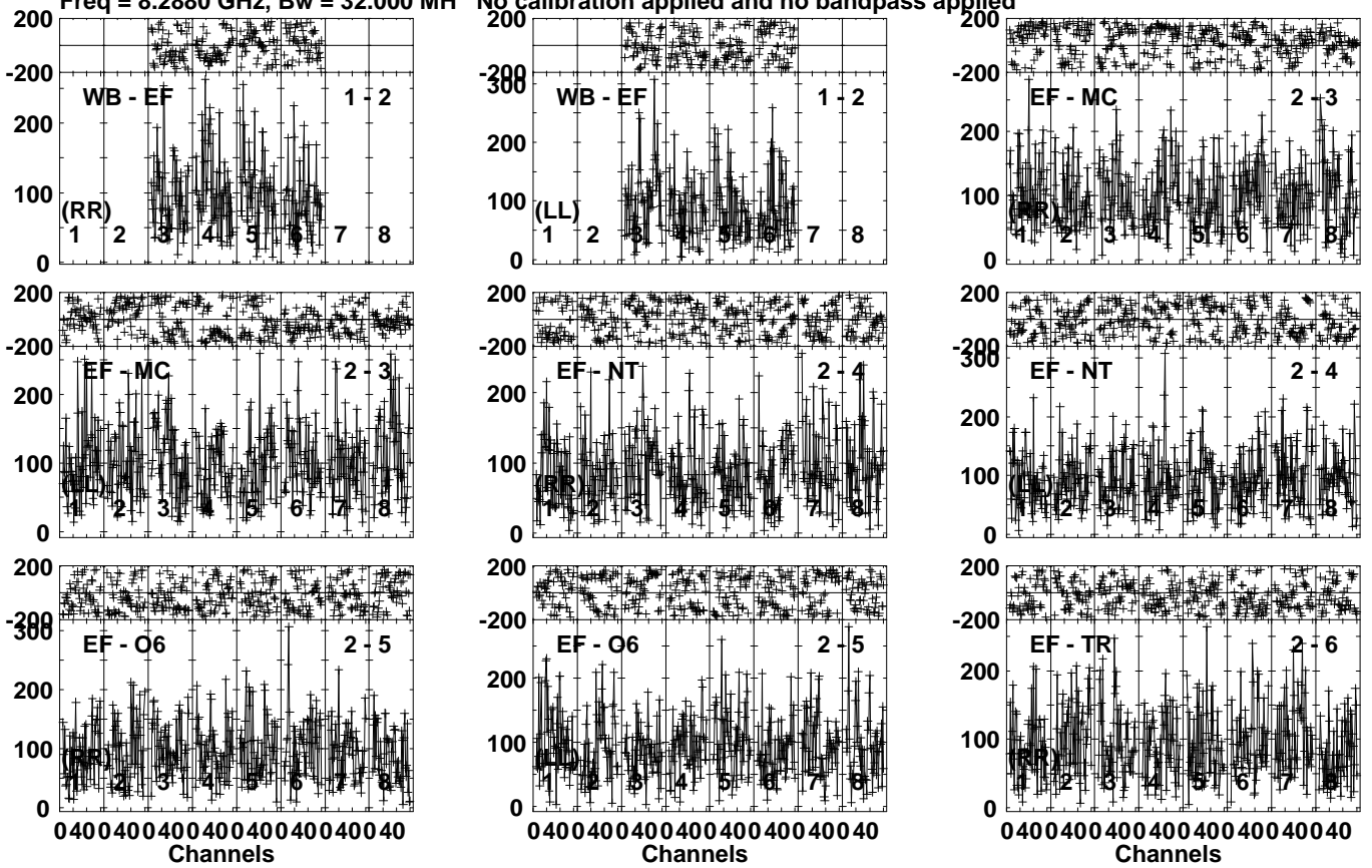
Lower frame: Micro Ampl Jy Top frame: Phas deg Vector averaged cross-power spectrum Several baselines displayed Timerange: 00/17:53:01 to 00/17:55:59
