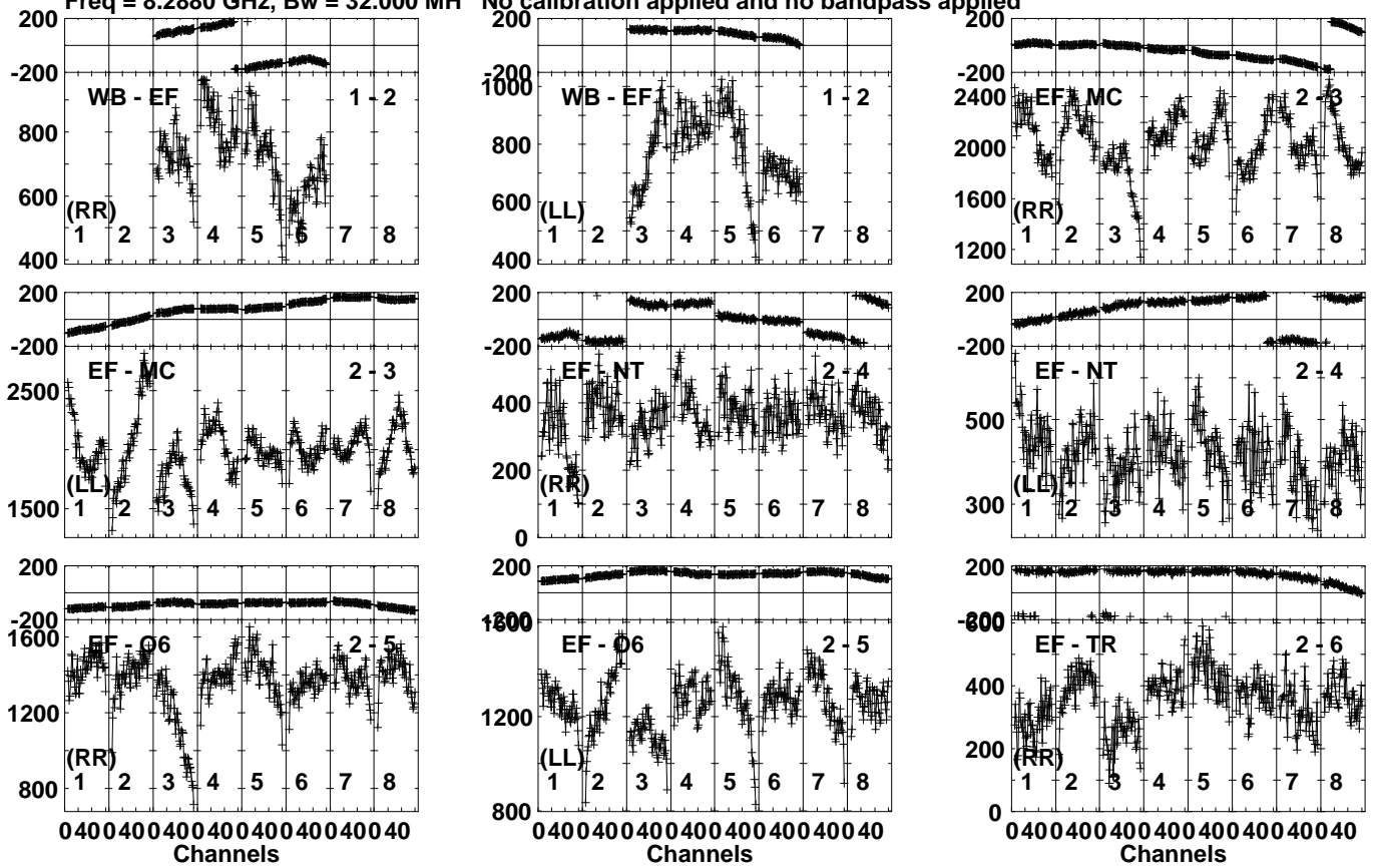
Lower frame: Micro Ampl Jy Top frame: Phas deg Vector averaged cross-power spectrum Several baselines displayed Timerange: 00/19:03:01 to 00/19:07:59
