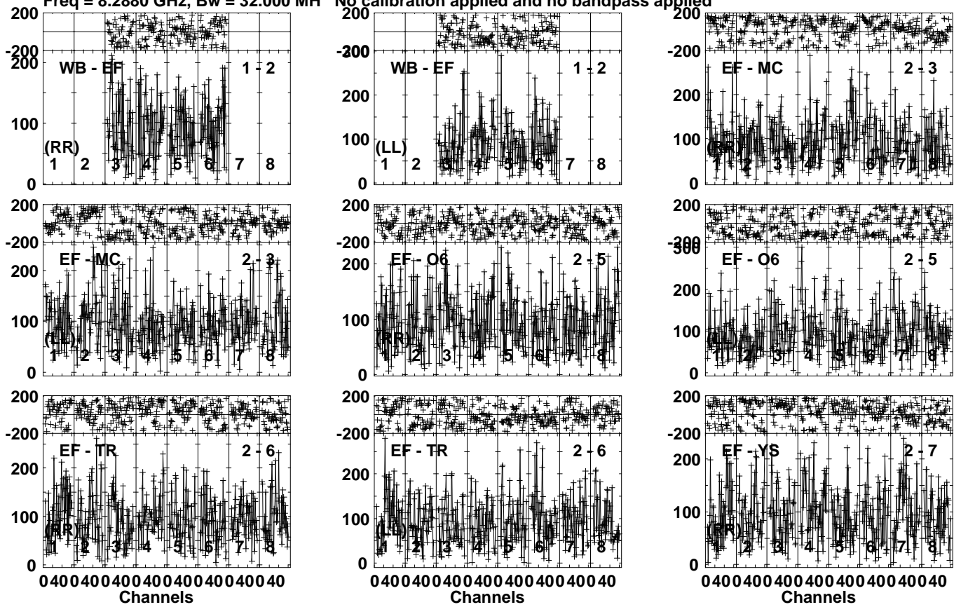
Lower frame: Micro Ampl Jy Top frame: Phas deg Vector averaged cross-power spectrum Several baselines displayed Timerange: 00/18:24:31 to 00/18:27:29
