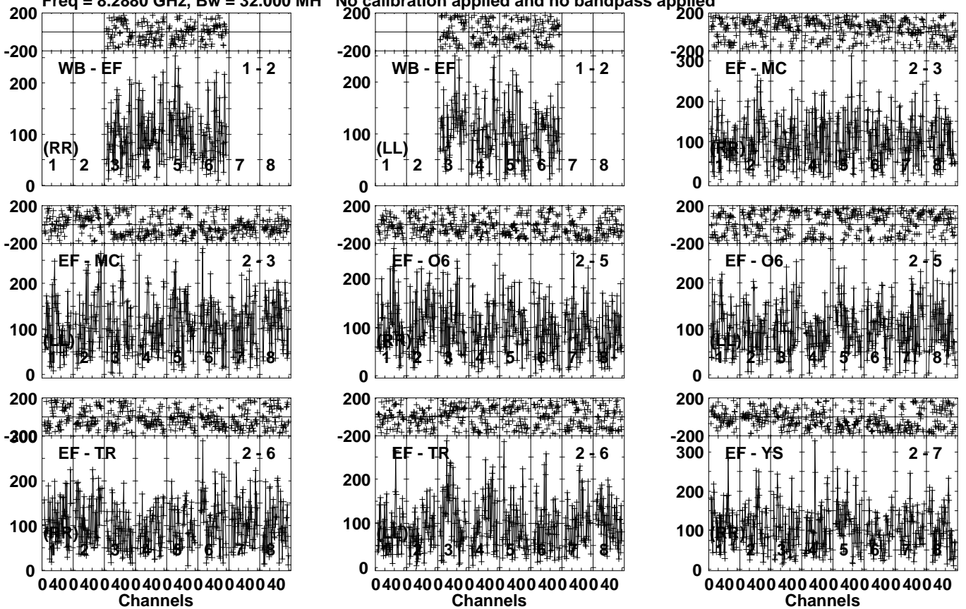
Lower frame: Micro Ampl Jy Top frame: Phas deg Vector averaged cross-power spectrum Several baselines displayed Timerange: 00/19:55:33 to 00/19:58:29
