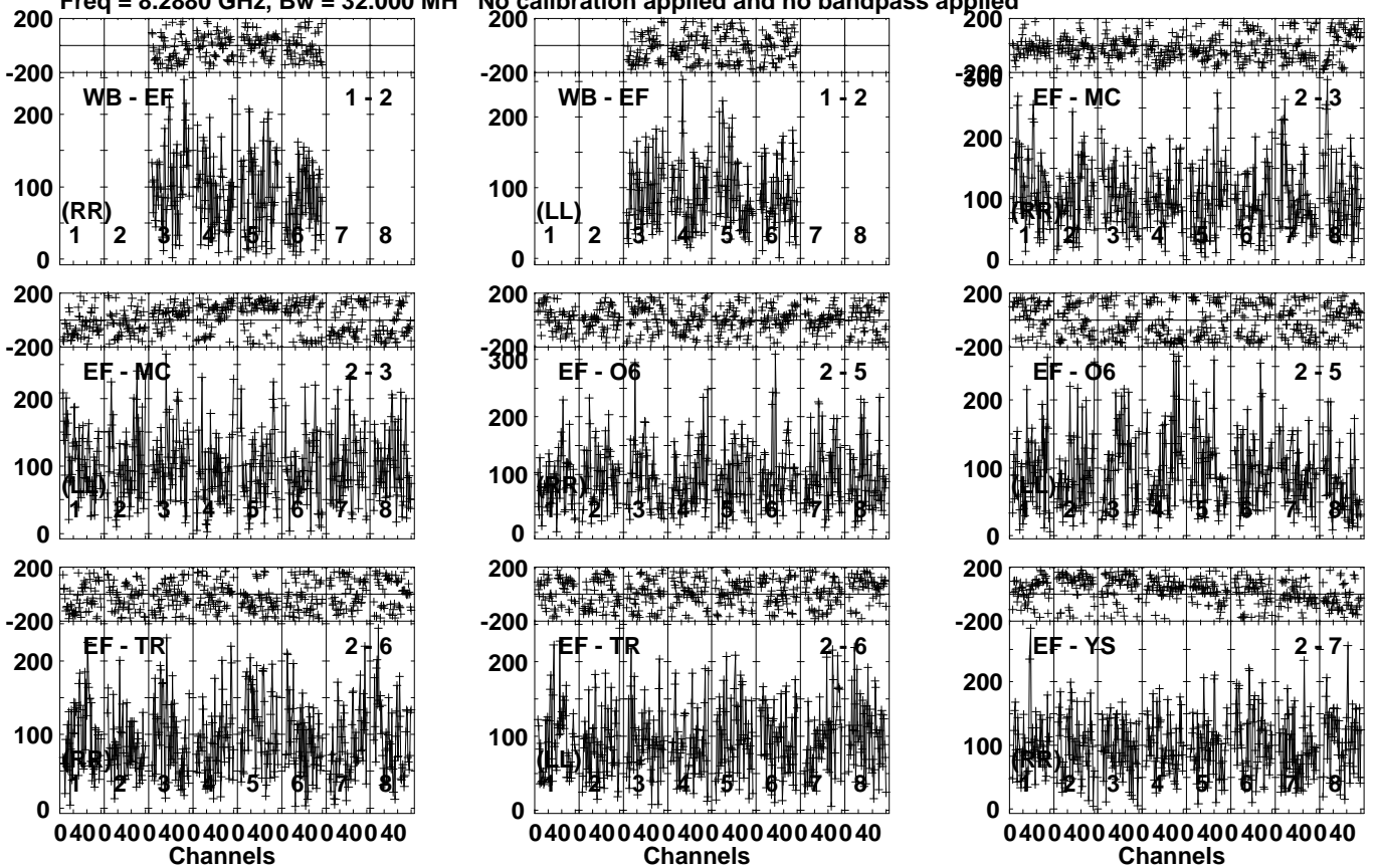
Lower frame: Micro Ampl Jy Top frame: Phas deg Vector averaged cross-power spectrum Several baselines displayed Timerange: 00/20:37:33 to 00/20:40:29
