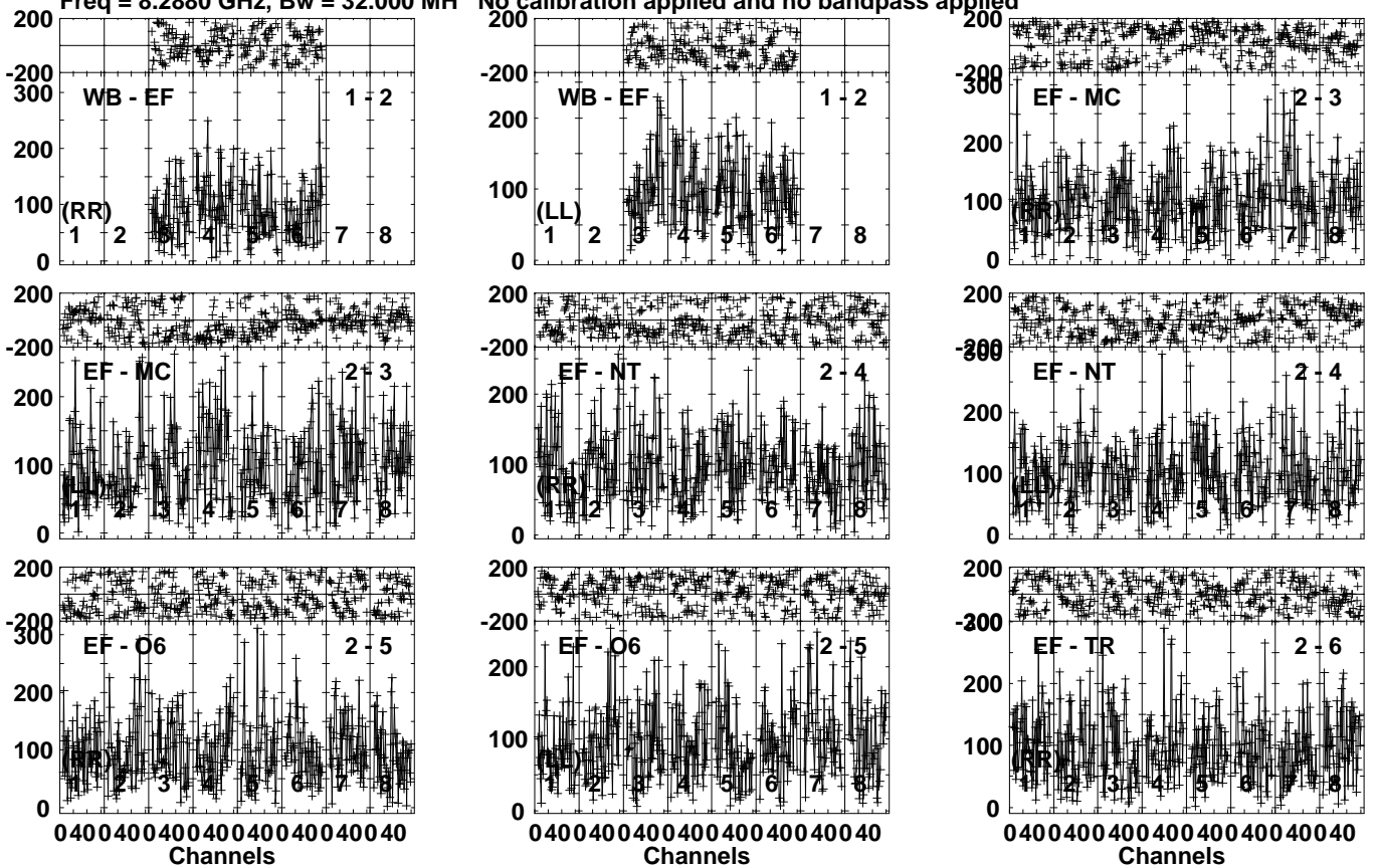
Lower frame: Micro Ampl Jy Top frame: Phas deg Vector averaged cross-power spectrum Several baselines displayed Timerange: 00/19:18:31 to 00/19:21:29
