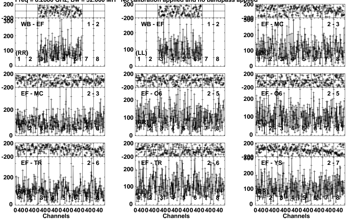
Lower frame: Micro Ampl Jy Top frame: Phas deg Vector averaged cross-power spectrum Several baselines displayed Timerange: 00/18:19:33 to 00/18:22:29
