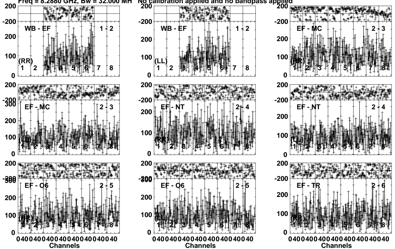
Lower frame: Micro Ampl Jy Top frame: Phas deg Vector averaged cross-power spectrum Several baselines displayed Timerange: 00/19:29:01 to 00/19:31:59
