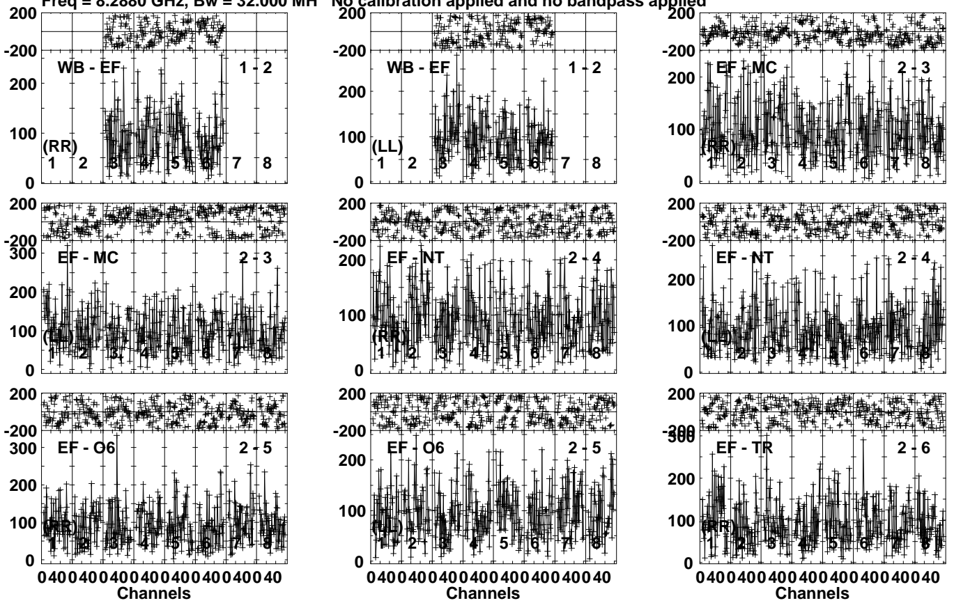
Lower frame: Micro Ampl Jy Top frame: Phas deg Vector averaged cross-power spectrum Several baselines displayed Timerange: 00/17:21:31 to 00/17:24:29
