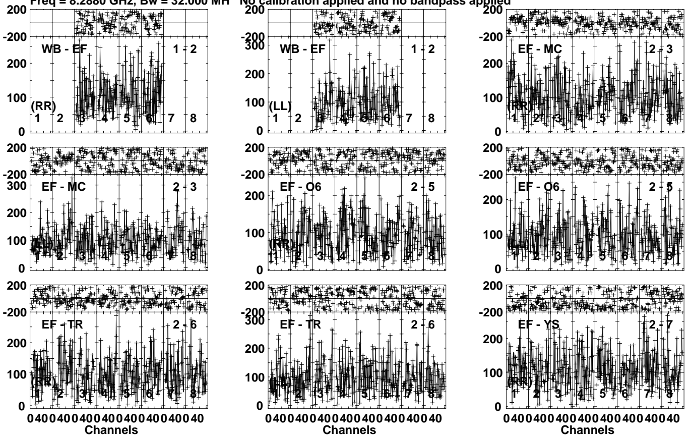
Lower frame: Micro Ampl Jy Top frame: Phas deg Vector averaged cross-power spectrum Several baselines displayed Timerange: 00/20:16:33 to 00/20:19:29
