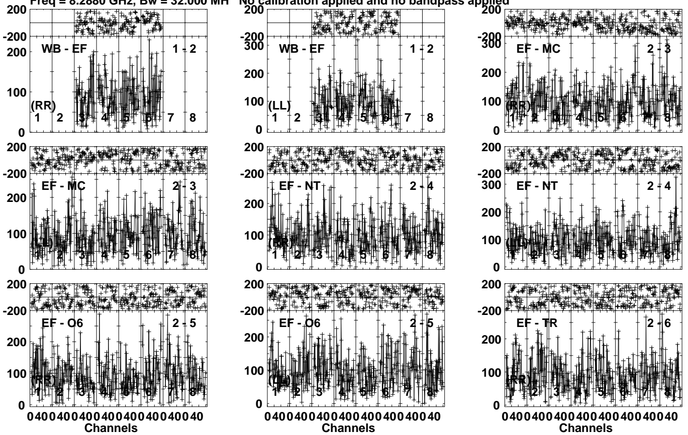
Lower frame: Micro Ampl Jy Top frame: Phas deg Vector averaged cross-power spectrum Several baselines displayed Timerange: 00/17:27:01 to 00/17:29:59
