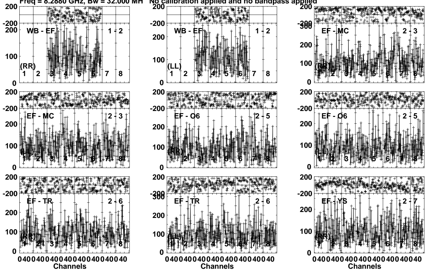
Lower frame: Micro Ampl Jy Top frame: Phas deg Vector averaged cross-power spectrum Several baselines displayed Timerange: 00/18:03:31 to 00/18:06:29
