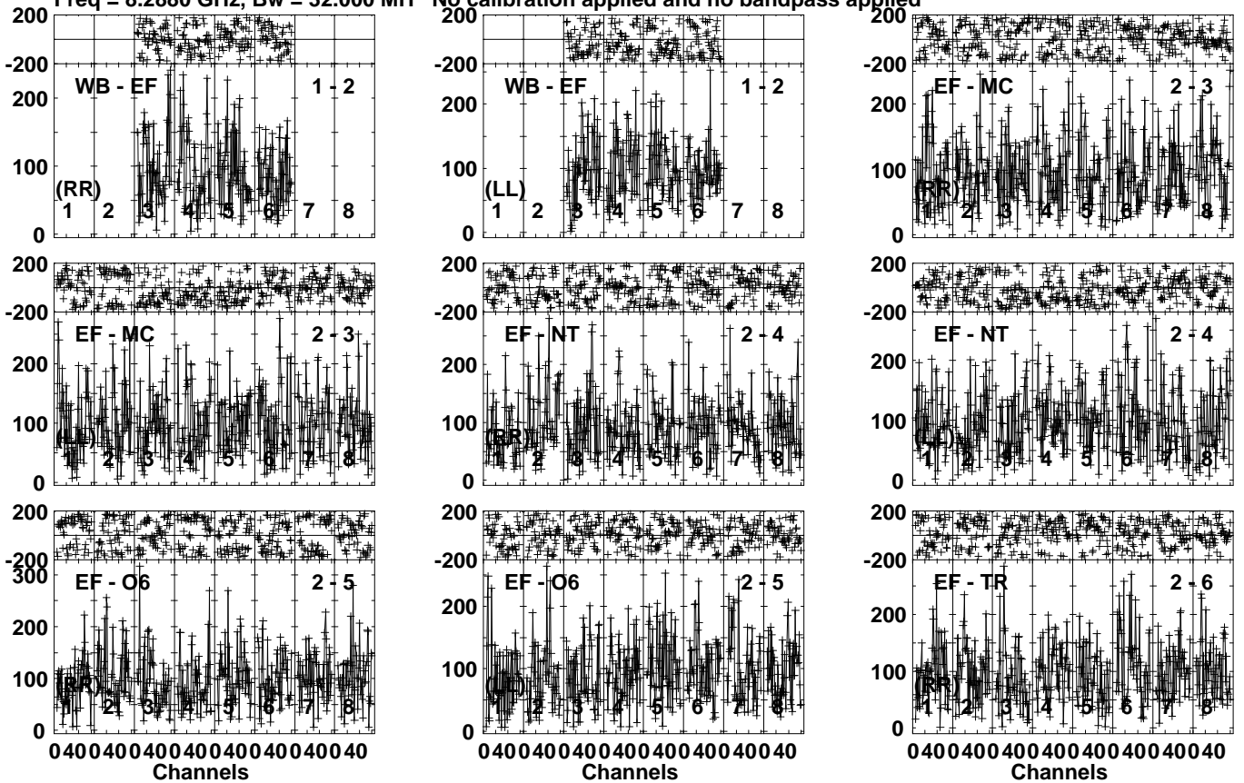
Lower frame: Micro Ampl Jy Top frame: Phas deg Vector averaged cross-power spectrum Several baselines displayed Timerange: 00/19:24:03 to 00/19:26:59
