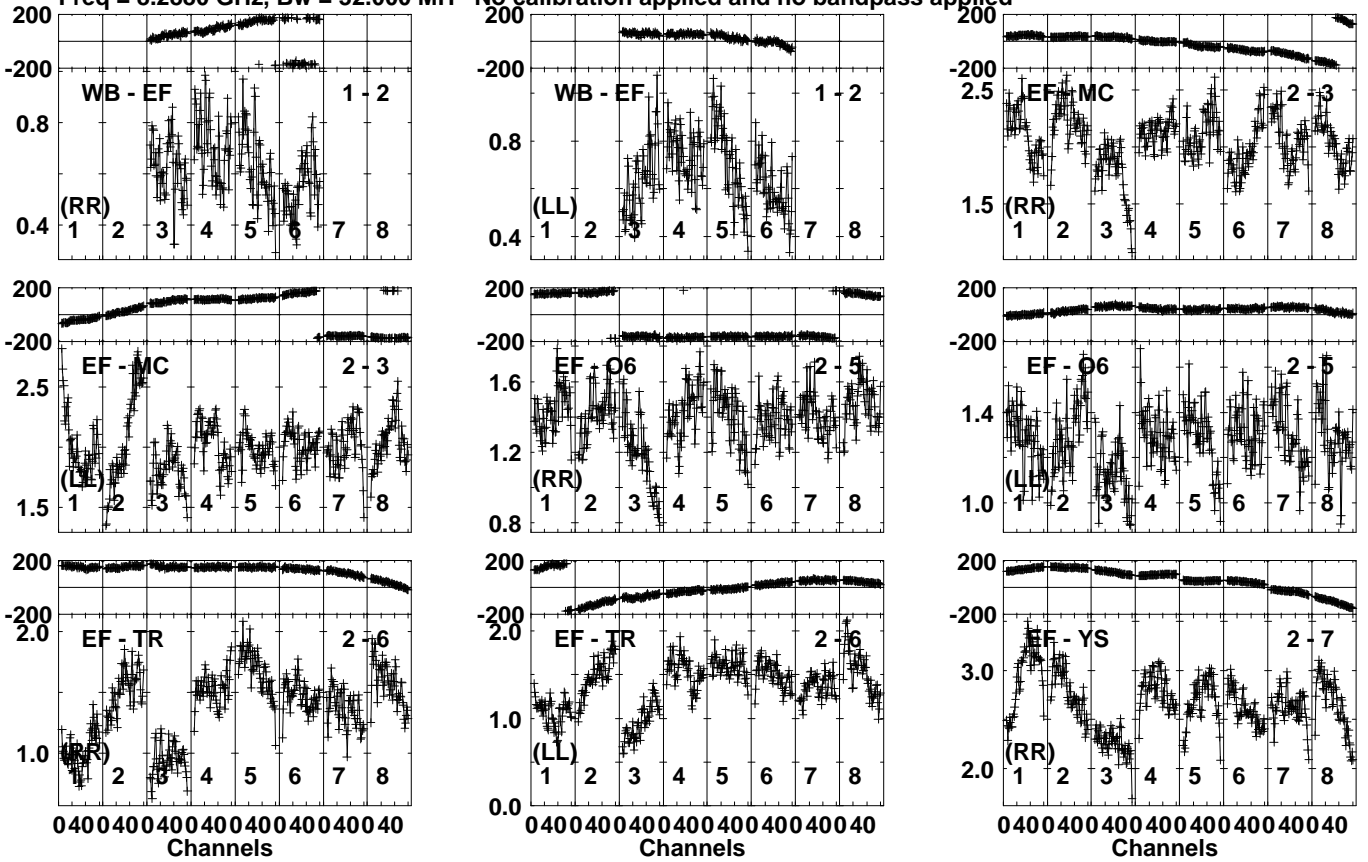
Lower frame: Milli Ampl Jy Top frame: Phas deg Vector averaged cross-power spectrum Several baselines displayed Timerange: 00/19:37:31 to 00/19:39:29
