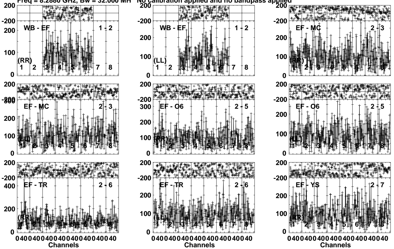
Lower frame: Micro Ampl Jy Top frame: Phas deg Vector averaged cross-power spectrum Several baselines displayed Timerange: 00/18:30:03 to 00/18:32:59
