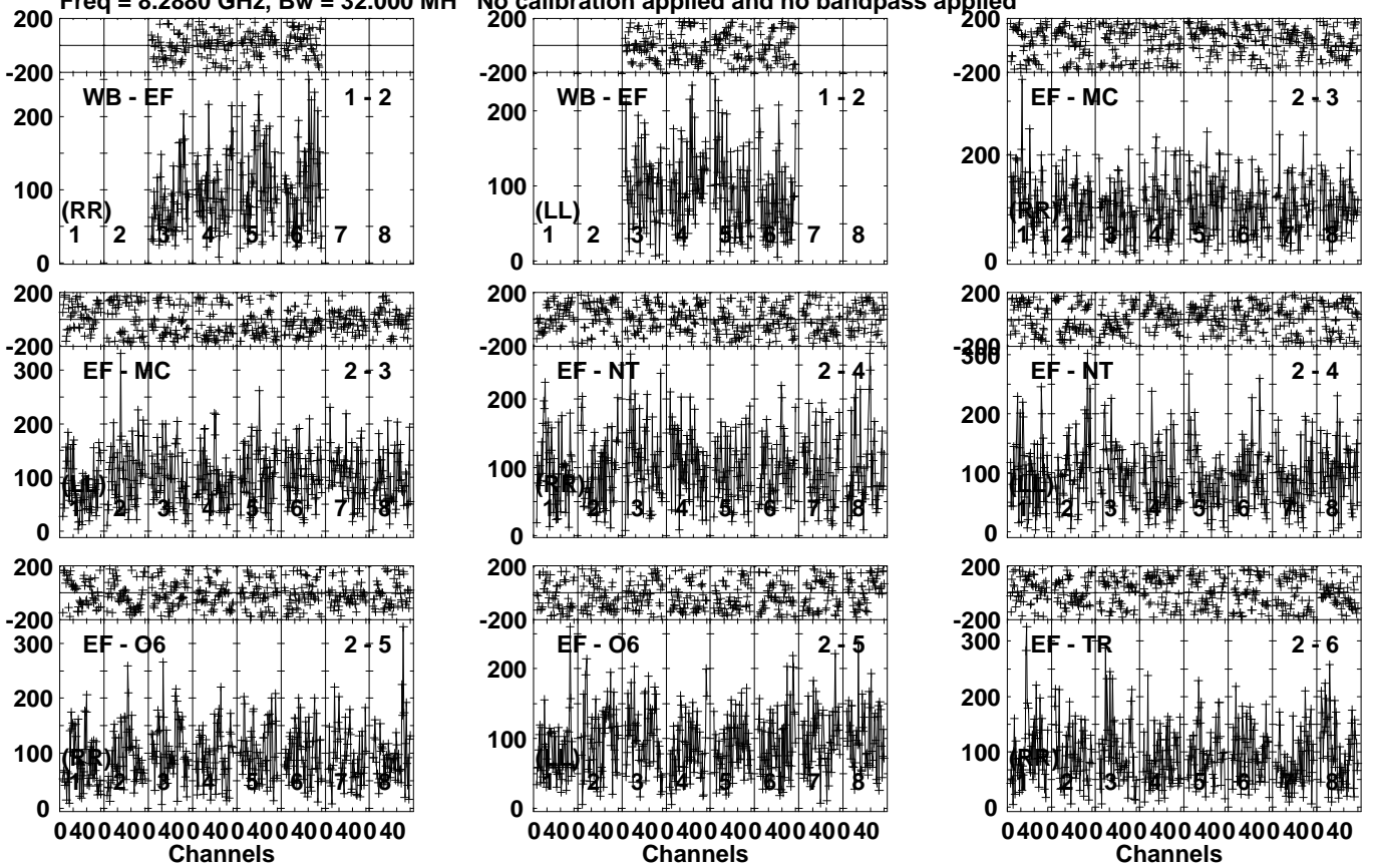
Lower frame: Micro Ampl Jy Top frame: Phas deg Vector averaged cross-power spectrum Several baselines displayed Timerange: 00/19:08:01 to 00/19:10:59
