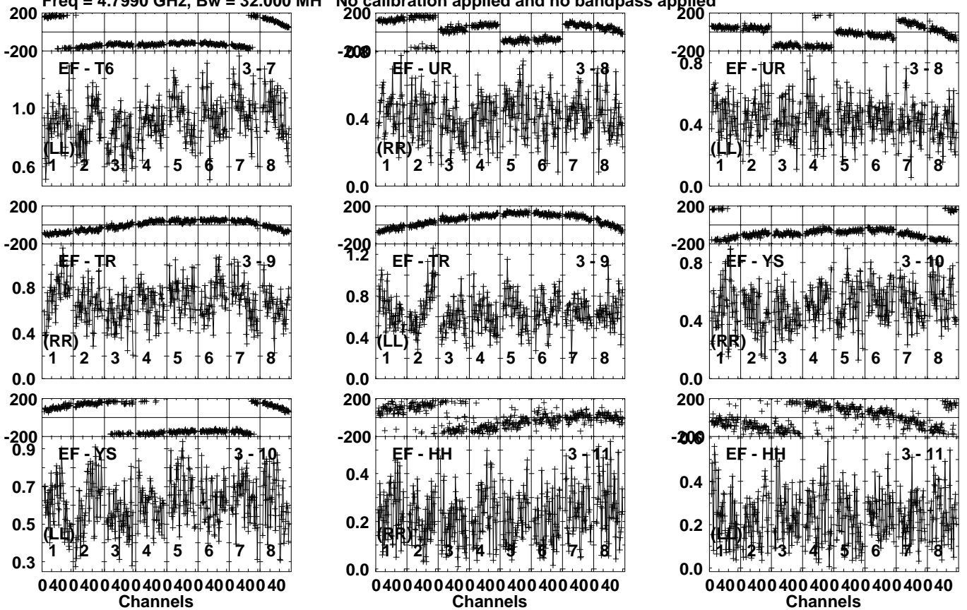
Lower frame: Milli Ampl Jy Top frame: Phas deg Vector averaged cross-power spectrum Several baselines displayed Timerange: 00/02:43:21 to 00/02:44:49
