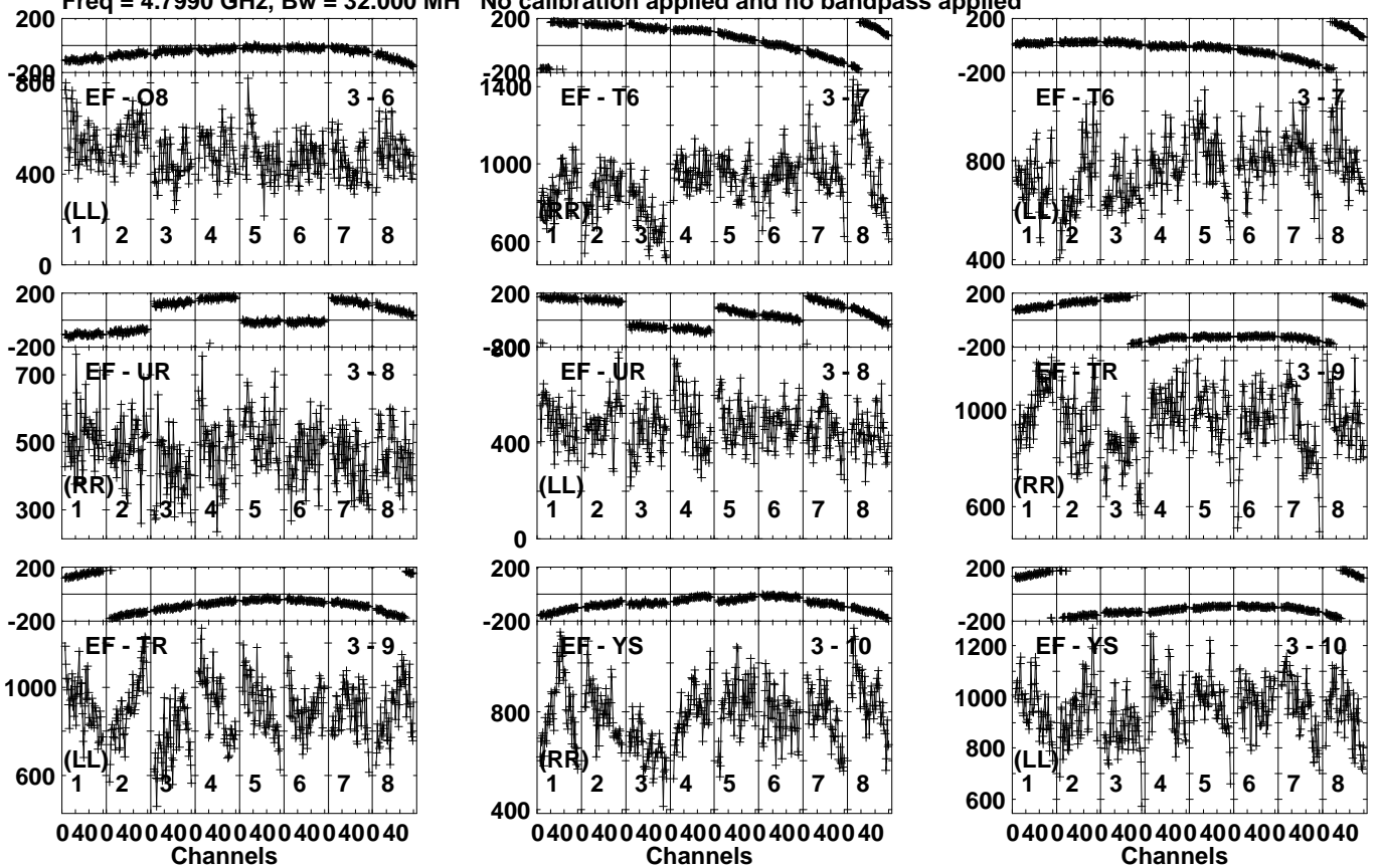
Lower frame: Micro Ampl Jy Top frame: Phas deg Vector averaged cross-power spectrum Several baselines displayed Timerange: 00/01:33:21 to 00/01:35:49
