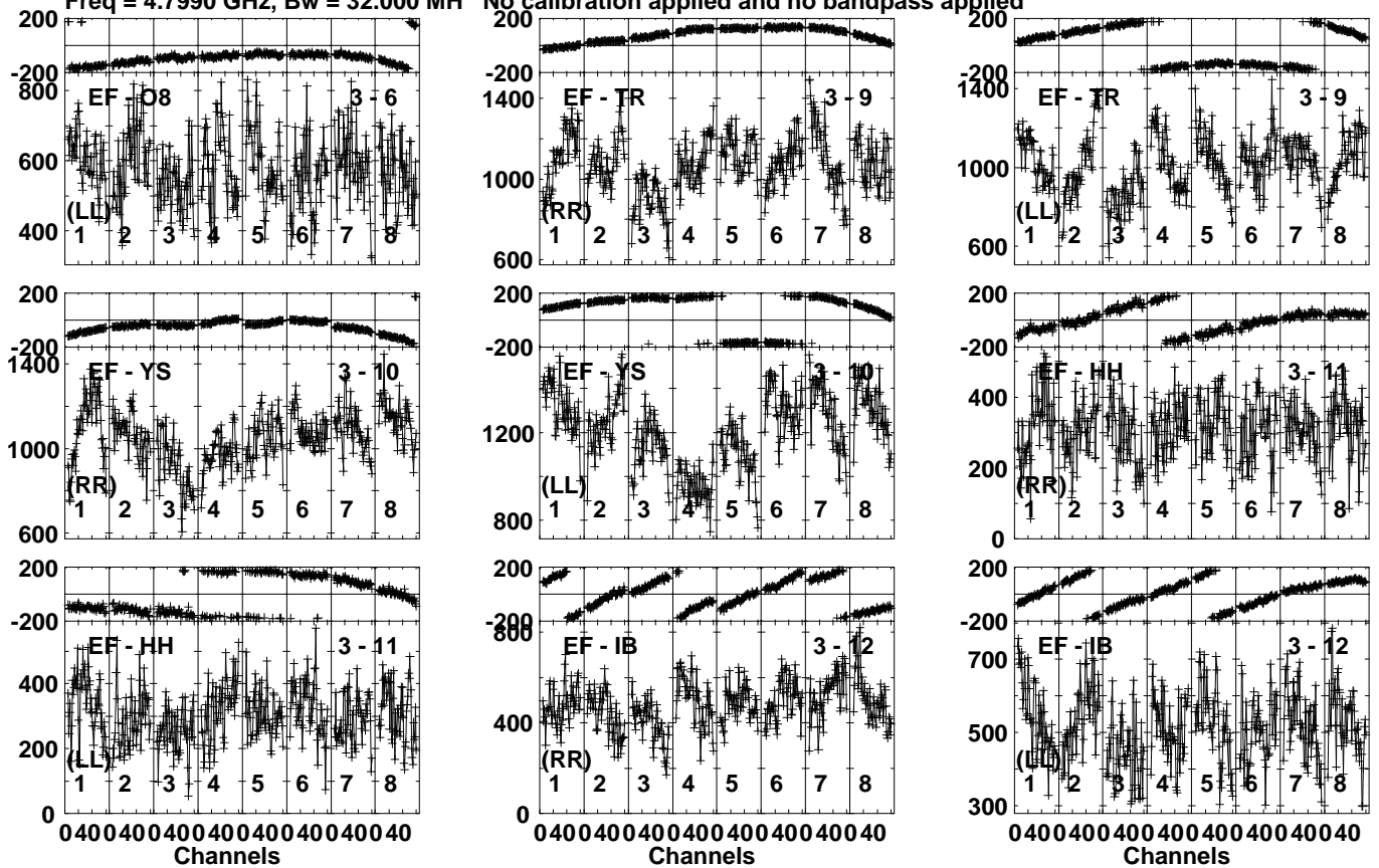
Lower frame: Micro Ampl Jy Top frame: Phas deg Vector averaged cross-power spectrum Several baselines displayed Timerange: 00/06:18:01 to 00/06:20:29
