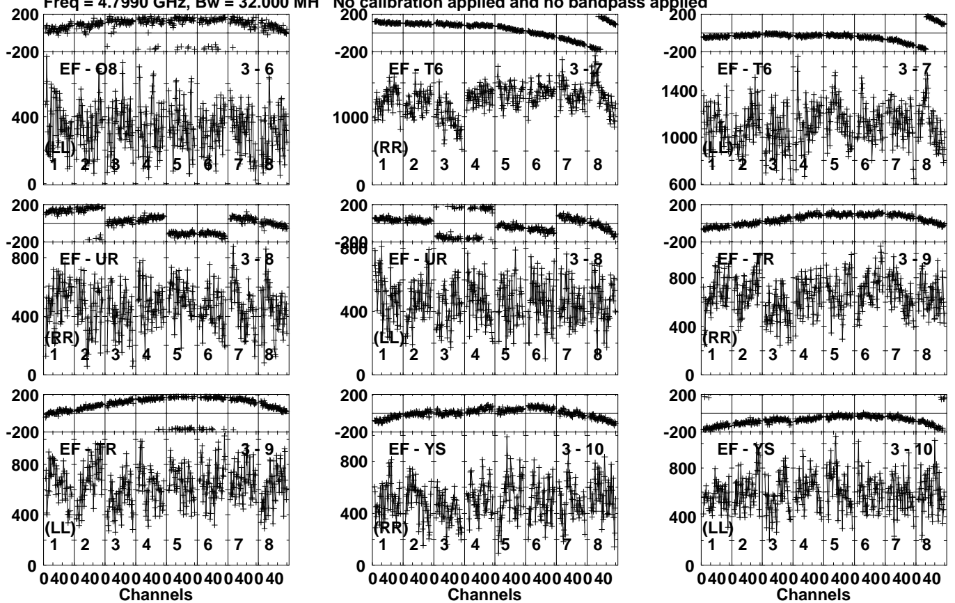
Lower frame: Micro Ampl Jy Top frame: Phas deg Vector averaged cross-power spectrum Several baselines displayed Timerange: 00/02:16:51 to 00/02:18:19
