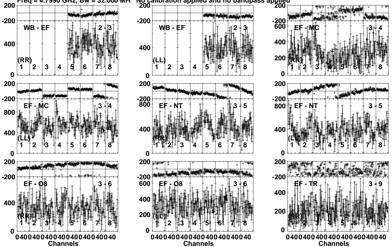
Lower frame: Micro Ampl Jy Top frame: Phas deg Vector averaged cross-power spectrum Several baselines displayed Timerange: 00/06:06:01 to 00/06:07:29
