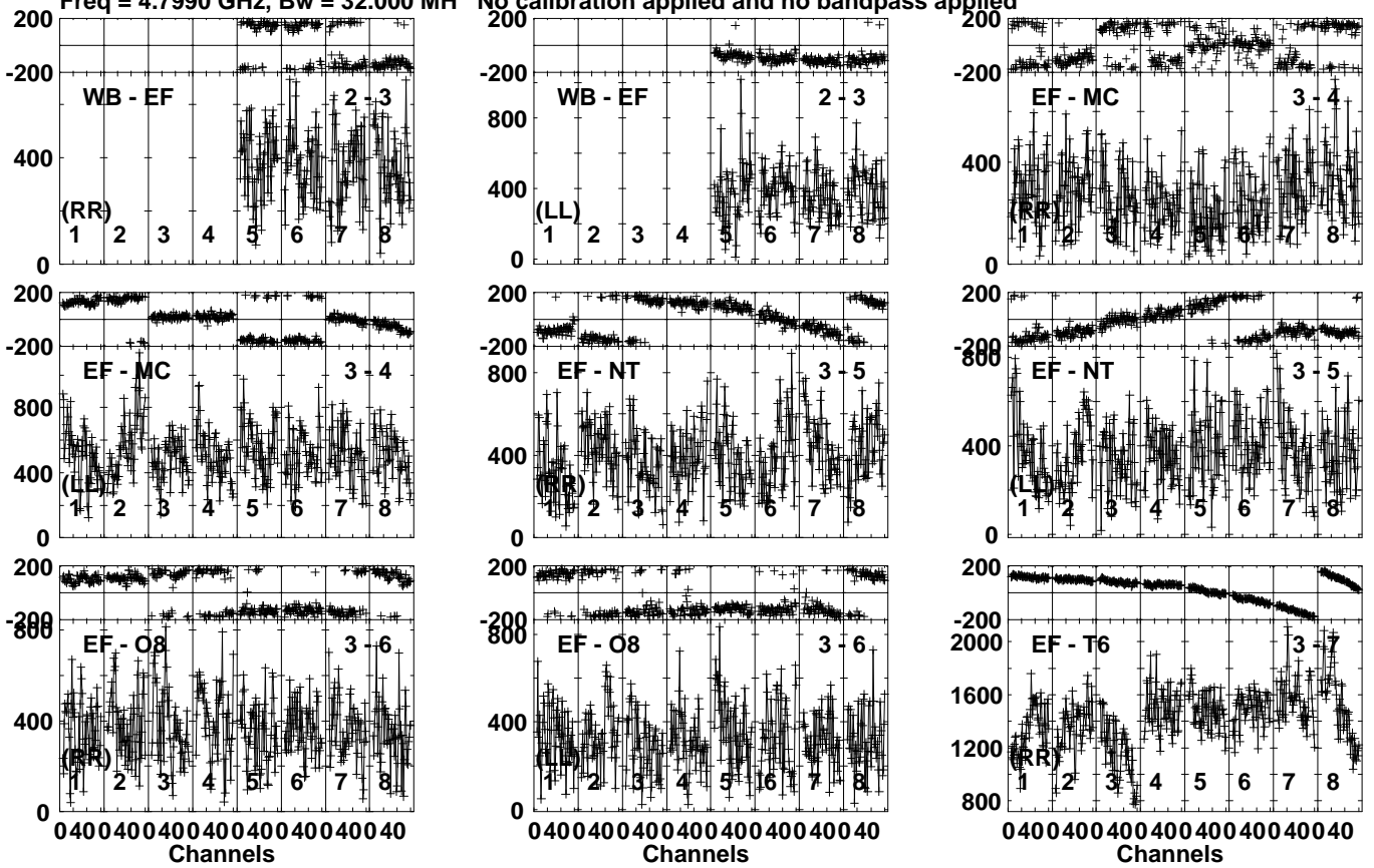
Lower frame: Micro Ampl Jy Top frame: Phas deg Vector averaged cross-power spectrum Several baselines displayed Timerange: 00/01:41:51 to 00/01:43:19
