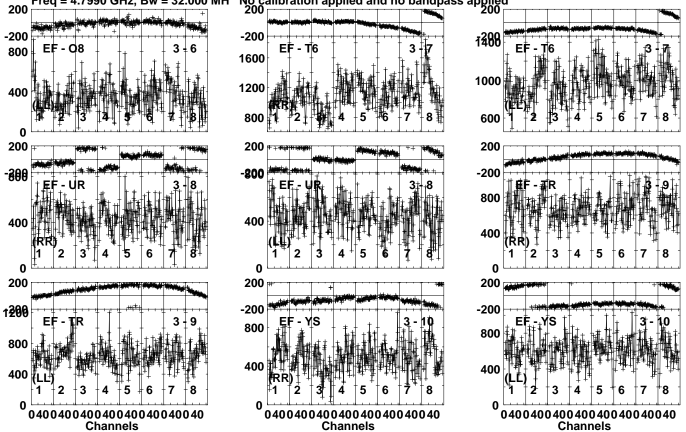
Lower frame: Micro Ampl Jy Top frame: Phas deg Vector averaged cross-power spectrum Several baselines displayed Timerange: 00/02:37:21 to 00/02:38:49
