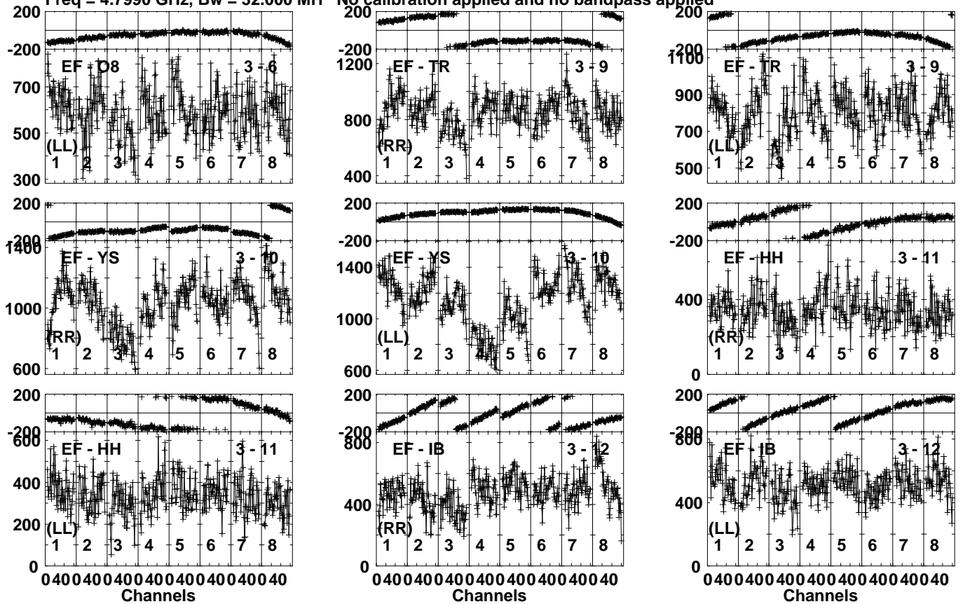
Lower frame: Micro Ampl Jy Top frame: Phas deg Vector averaged cross-power spectrum Several baselines displayed Timerange: 00/05:57:31 to 00/05:59:59
