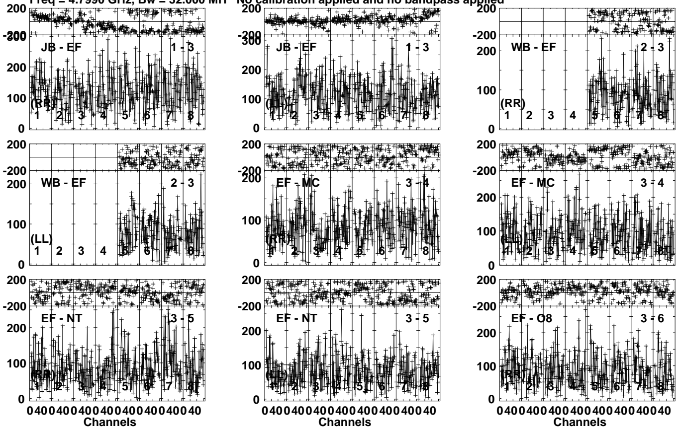
Lower frame: Micro Ampl Jy Top frame: Phas deg Vector averaged cross-power spectrum Several baselines displayed Timerange: 00/02:09:21 to 00/02:12:49
