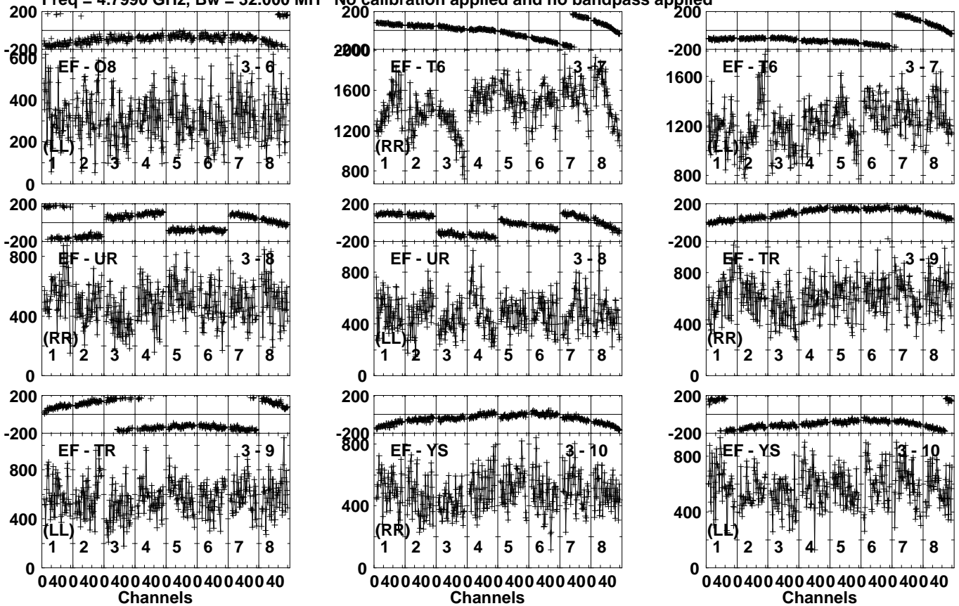
Lower frame: Micro Ampl Jy Top frame: Phas deg Vector averaged cross-power spectrum Several baselines displayed Timerange: 00/01:35:51 to 00/01:37:19
