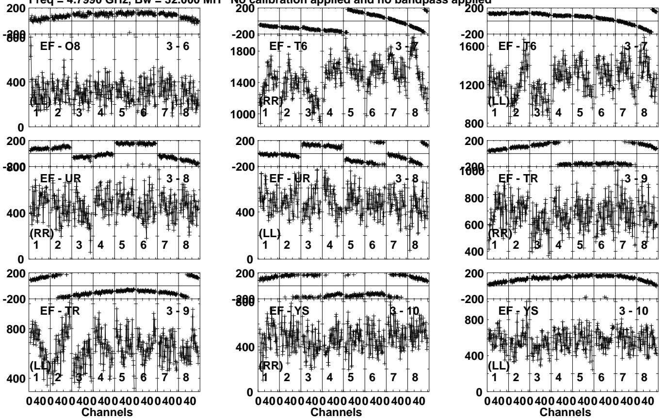
Lower frame: Micro Ampl Jy Top frame: Phas deg Vector averaged cross-power spectrum Several baselines displayed Timerange: 00/01:06:01 to 00/01:07:49
