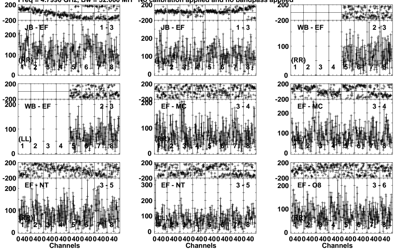
Lower frame: Micro Ampl Jy Top frame: Phas deg Vector averaged cross-power spectrum Several baselines displayed Timerange: 00/01:58:21 to 00/02:02:19
