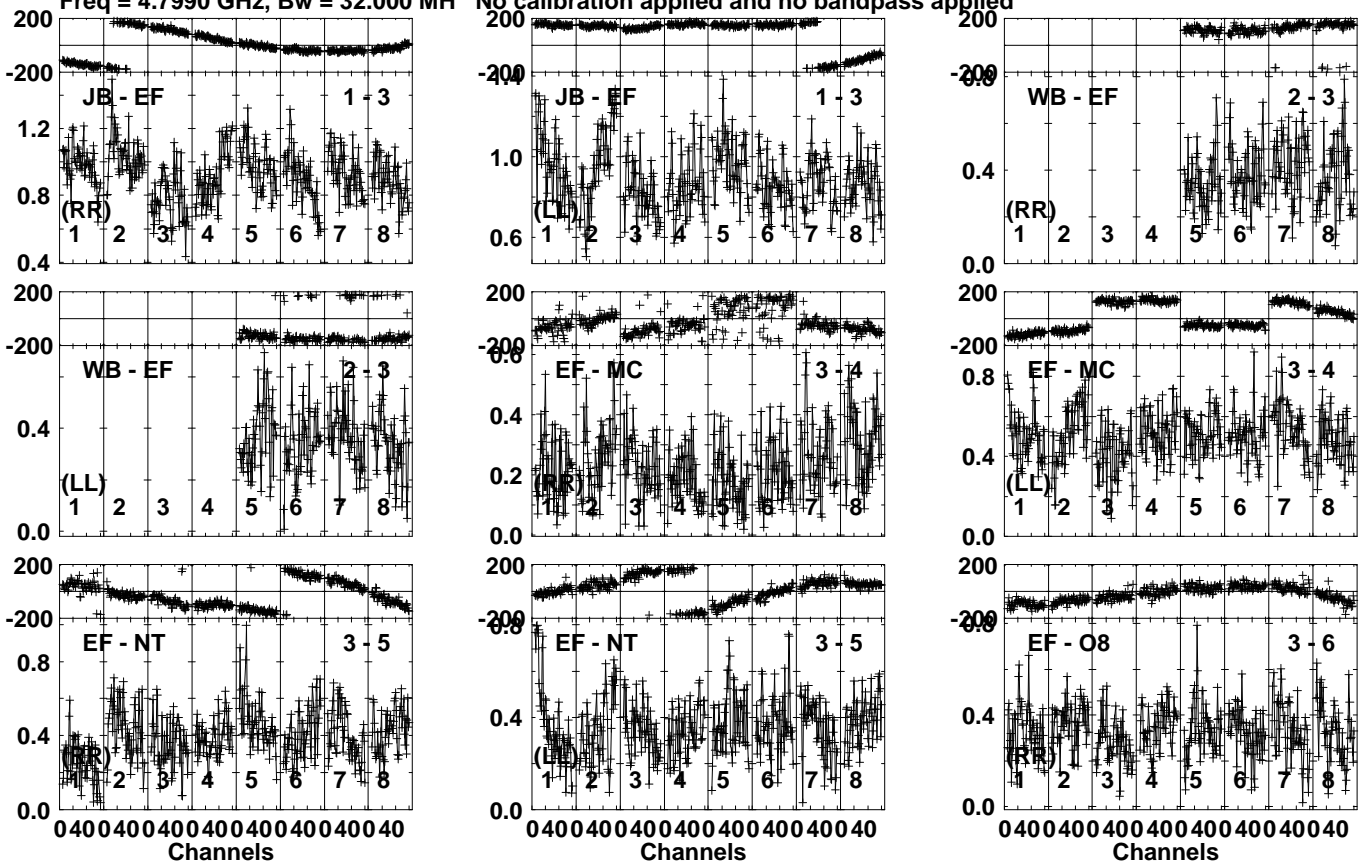
Lower frame: Milli Ampl Jy Top frame: Phas deg Vector averaged cross-power spectrum Several baselines displayed Timerange: 00/01:15:21 to 00/01:16:49
