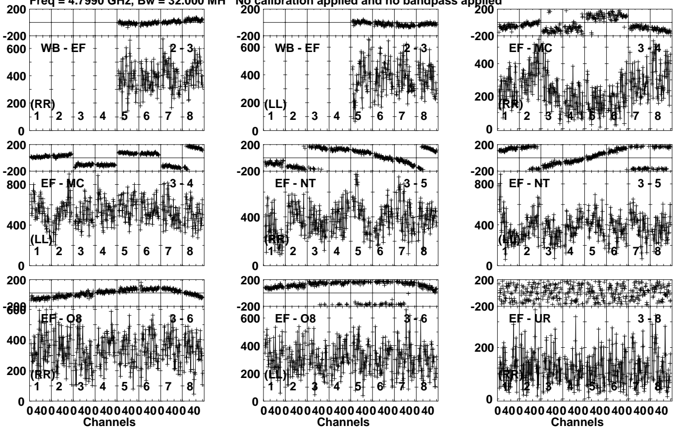
Lower frame: Micro Ampl Jy Top frame: Phas deg Vector averaged cross-power spectrum Several baselines displayed Timerange: 00/05:30:31 to 00/05:31:59
