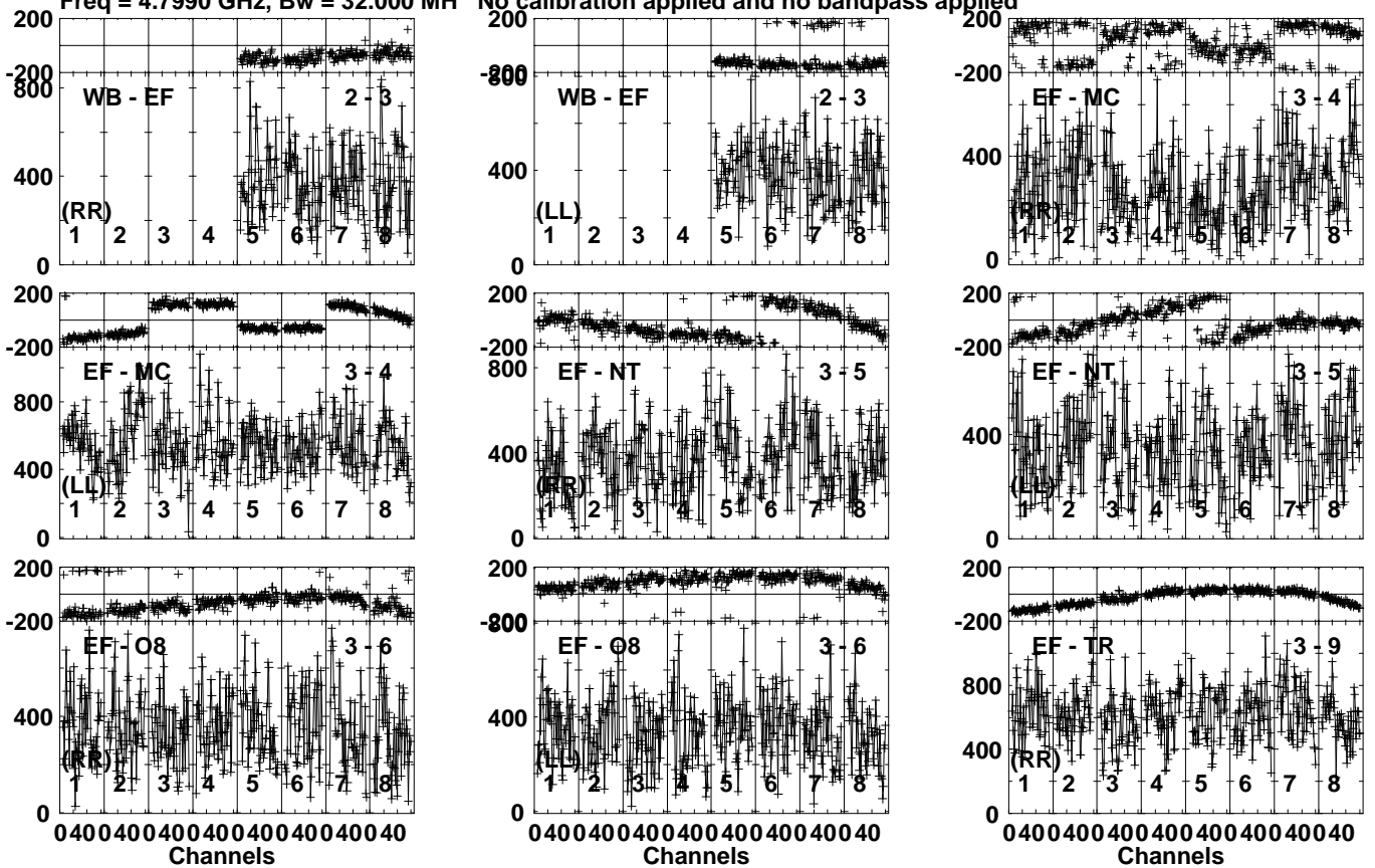
Lower frame: Micro Ampl Jy Top frame: Phas deg Vector averaged cross-power spectrum Several baselines displayed Timerange: 00/06:47:01 to 00/06:48:29
