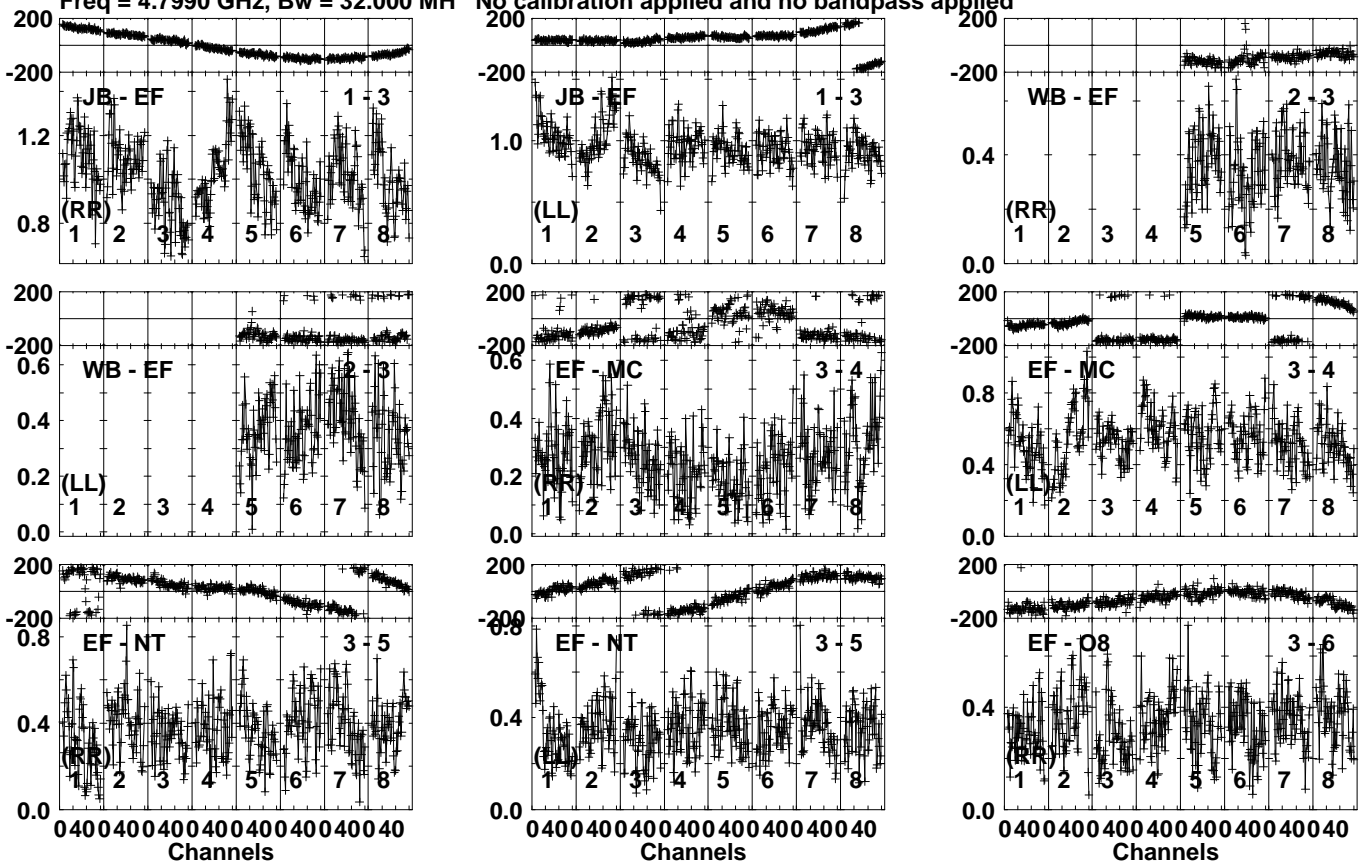
Lower frame: Milli Ampl Jy Top frame: Phas deg Vector averaged cross-power spectrum Several baselines displayed Timerange: 00/06:41:01 to 00/06:42:29
