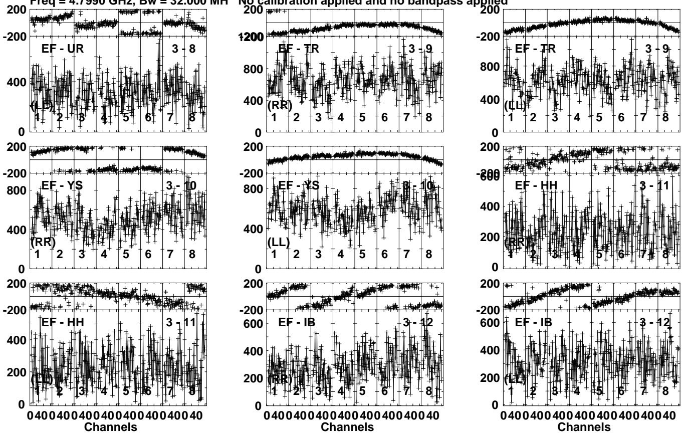
Lower frame: Micro Ampl Jy Top frame: Phas deg Vector averaged cross-power spectrum Several baselines displayed Timerange: 00/05:04:31 to 00/05:05:59
