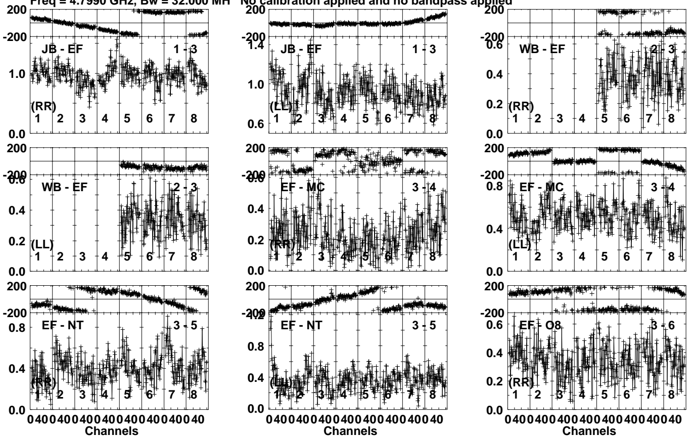
Lower frame: Milli Ampl Jy Top frame: Phas deg Vector averaged cross-power spectrum Several baselines displayed Timerange: 00/01:52:21 to 00/01:53:49
