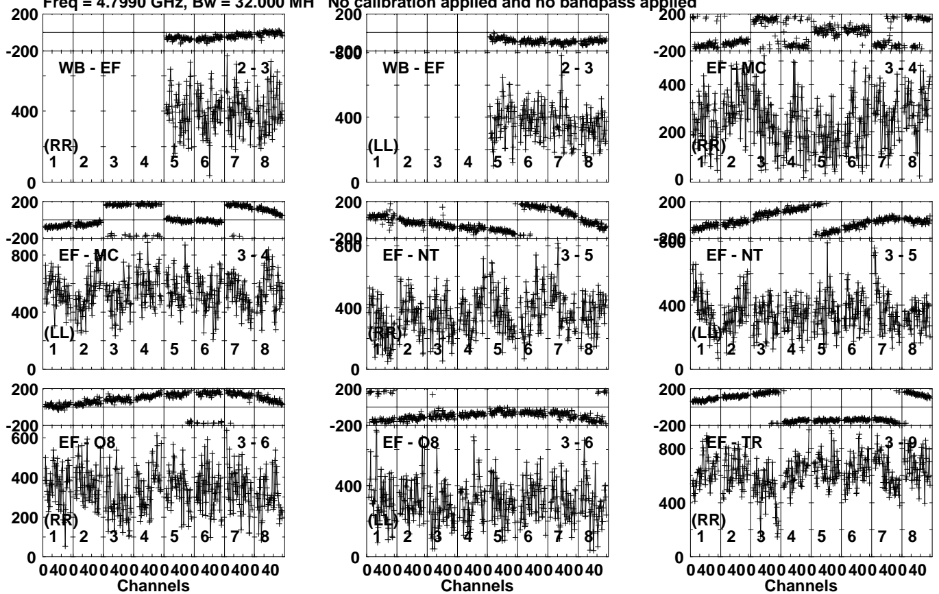
Lower frame: Micro Ampl Jy Top frame: Phas deg Vector averaged cross-power spectrum Several baselines displayed Timerange: 00/06:11:31 to 00/06:12:59
