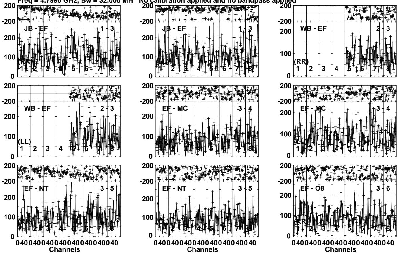
Lower frame: Micro Ampl Jy Top frame: Phas deg Vector averaged cross-power spectrum Several baselines displayed Timerange: 00/02:50:21 to 00/02:53:49
