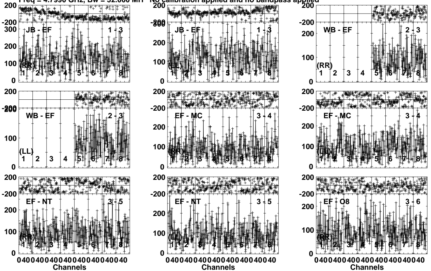
Lower frame: Micro Ampl Jy Top frame: Phas deg Vector averaged cross-power spectrum Several baselines displayed Timerange: 00/04:51:01 to 00/04:54:29
