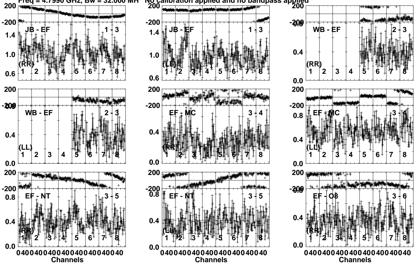
Lower frame: Milli Ampl Jy Top frame: Phas deg Vector averaged cross-power spectrum Several baselines displayed Timerange: 00/02:57:51 to 00/02:59:19
