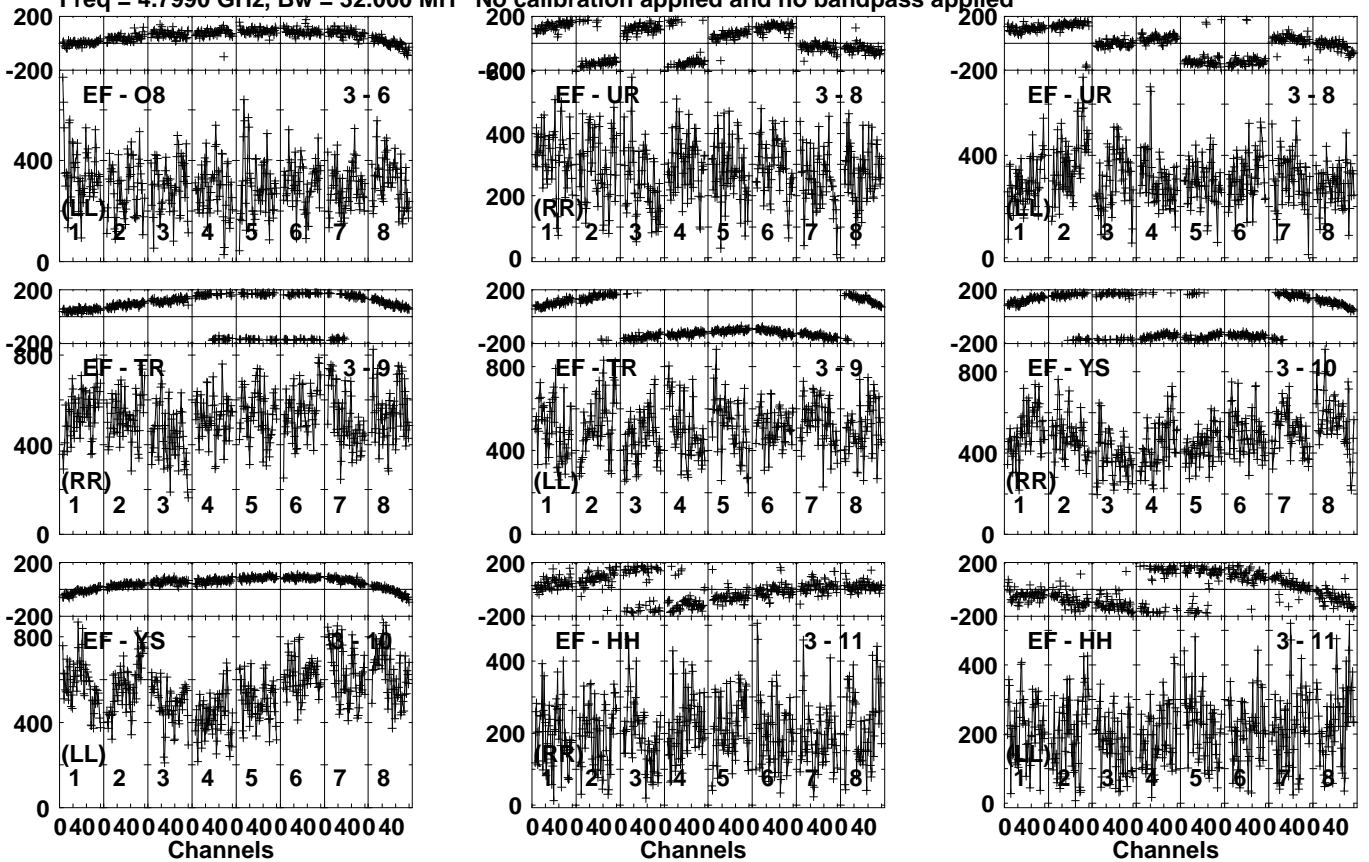
Lower frame: Micro Ampl Jy Top frame: Phas deg Vector averaged cross-power spectrum Several baselines displayed Timerange: 00/04:49:11 to 00/04:50:59
