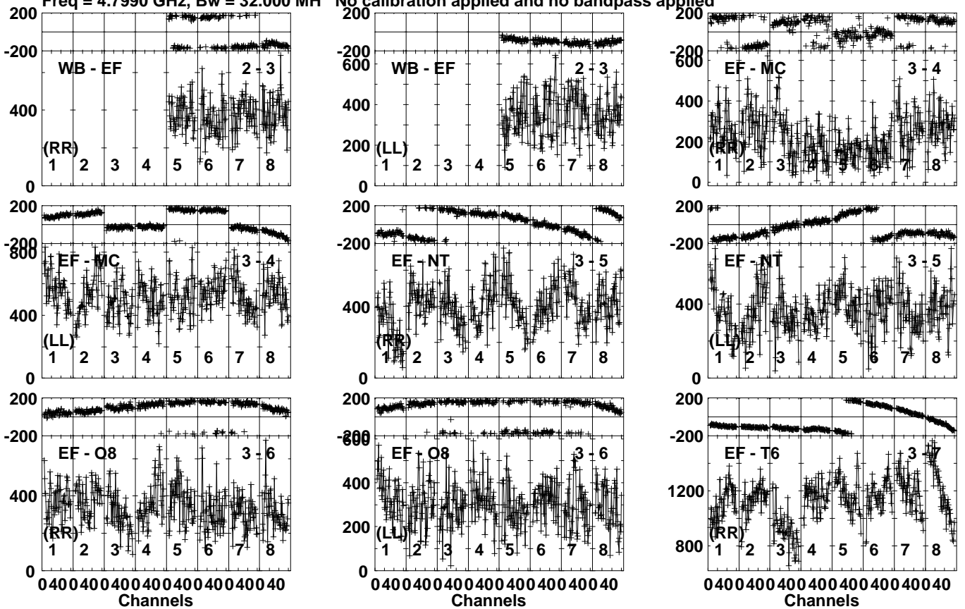
Lower frame: Micro Ampl Jy Top frame: Phas deg Vector averaged cross-power spectrum Several baselines displayed Timerange: 00/02:07:51 to 00/02:09:19
