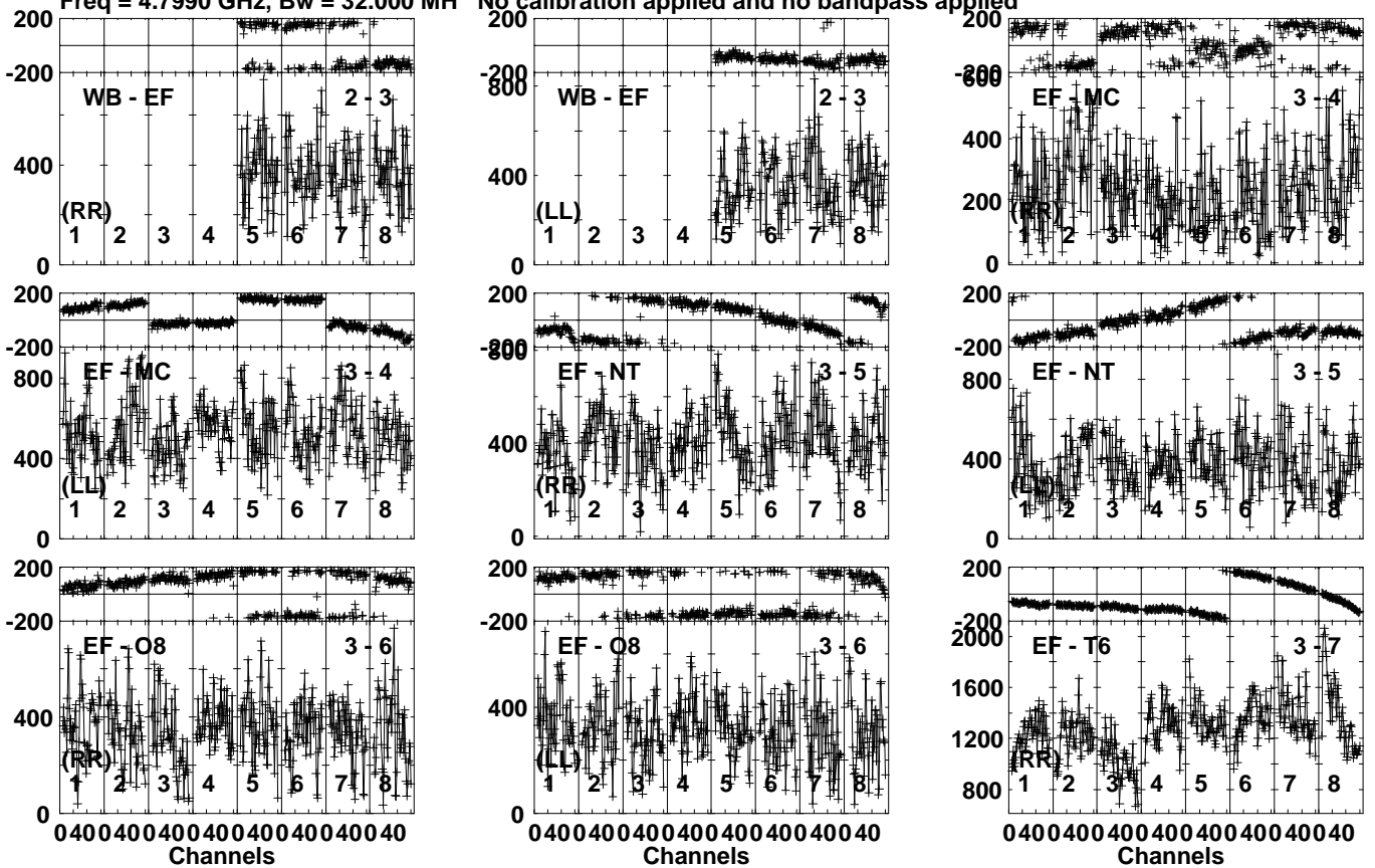
Lower frame: Micro Ampl Jy Top frame: Phas deg Vector averaged cross-power spectrum Several baselines displayed Timerange: 00/02:02:21 to 00/02:03:49
