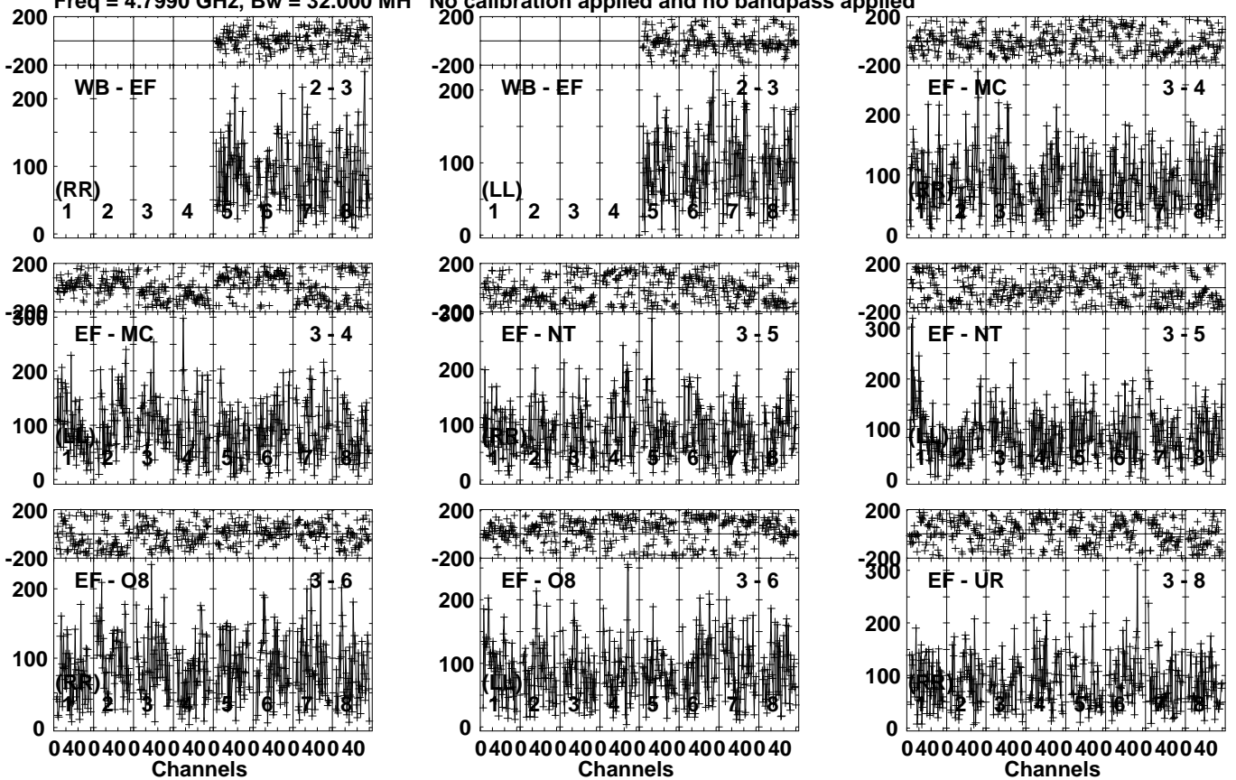
Lower frame: Micro Ampl Jy Top frame: Phas deg Vector averaged cross-power spectrum Several baselines displayed Timerange: 00/05:26:31 to 00/05:29:59
