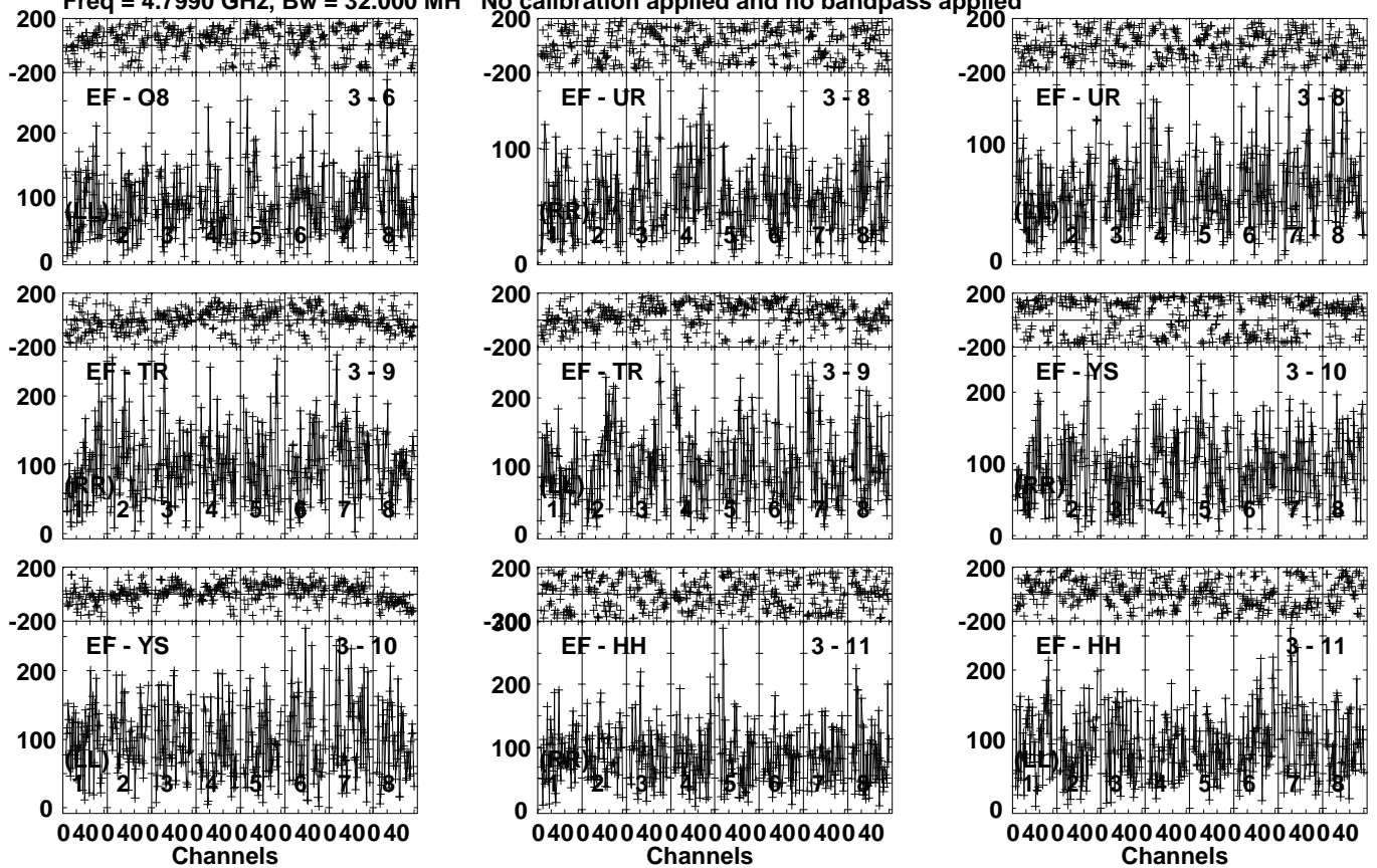
Lower frame: Micro Ampl Jy Top frame: Phas deg Vector averaged cross-power spectrum Several baselines displayed Timerange: 00/05:32:01 to 00/05:35:29
