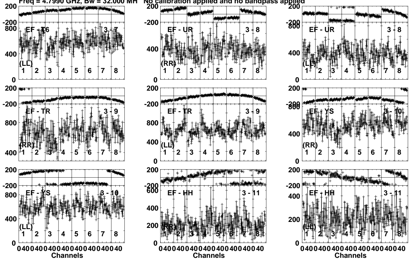
Lower frame: Micro Ampl Jy Top frame: Phas deg Vector averaged cross-power spectrum Several baselines displayed Timerange: 00/03:09:21 to 00/03:10:49
