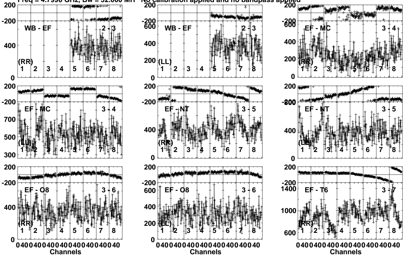
Lower frame: Micro Ampl Jy Top frame: Phas deg Vector averaged cross-power spectrum Several baselines displayed Timerange: 00/02:28:21 to 00/02:29:49
