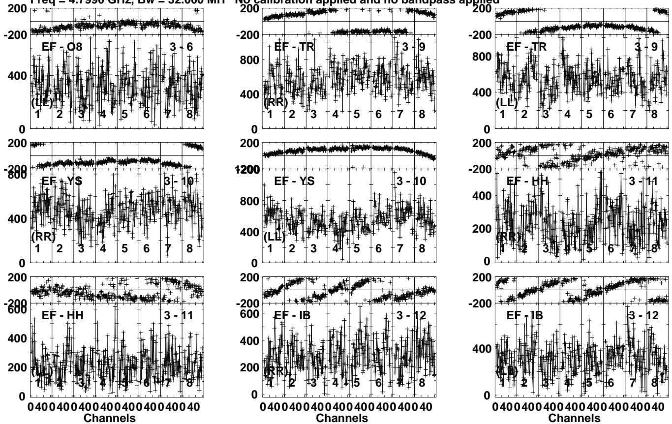
Lower frame: Micro Ampl Jy Top frame: Phas deg Vector averaged cross-power spectrum Several baselines displayed Timerange: 00/05:56:01 to 00/05:57:29
