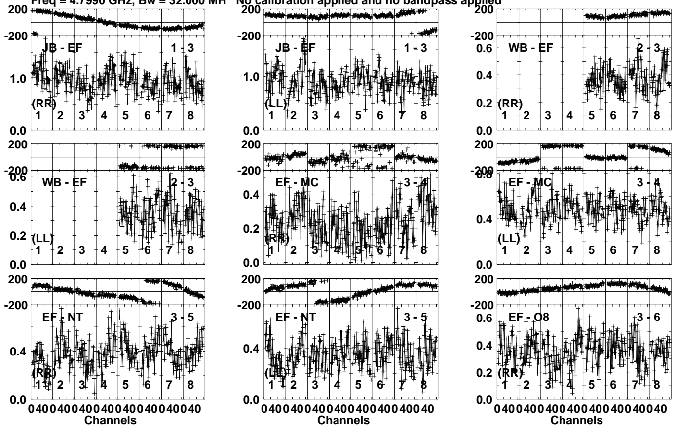
Lower frame: Milli Ampl Jy Top frame: Phas deg Vector averaged cross-power spectrum Several baselines displayed Timerange: 00/01:06:01 to 00/01:07:49
