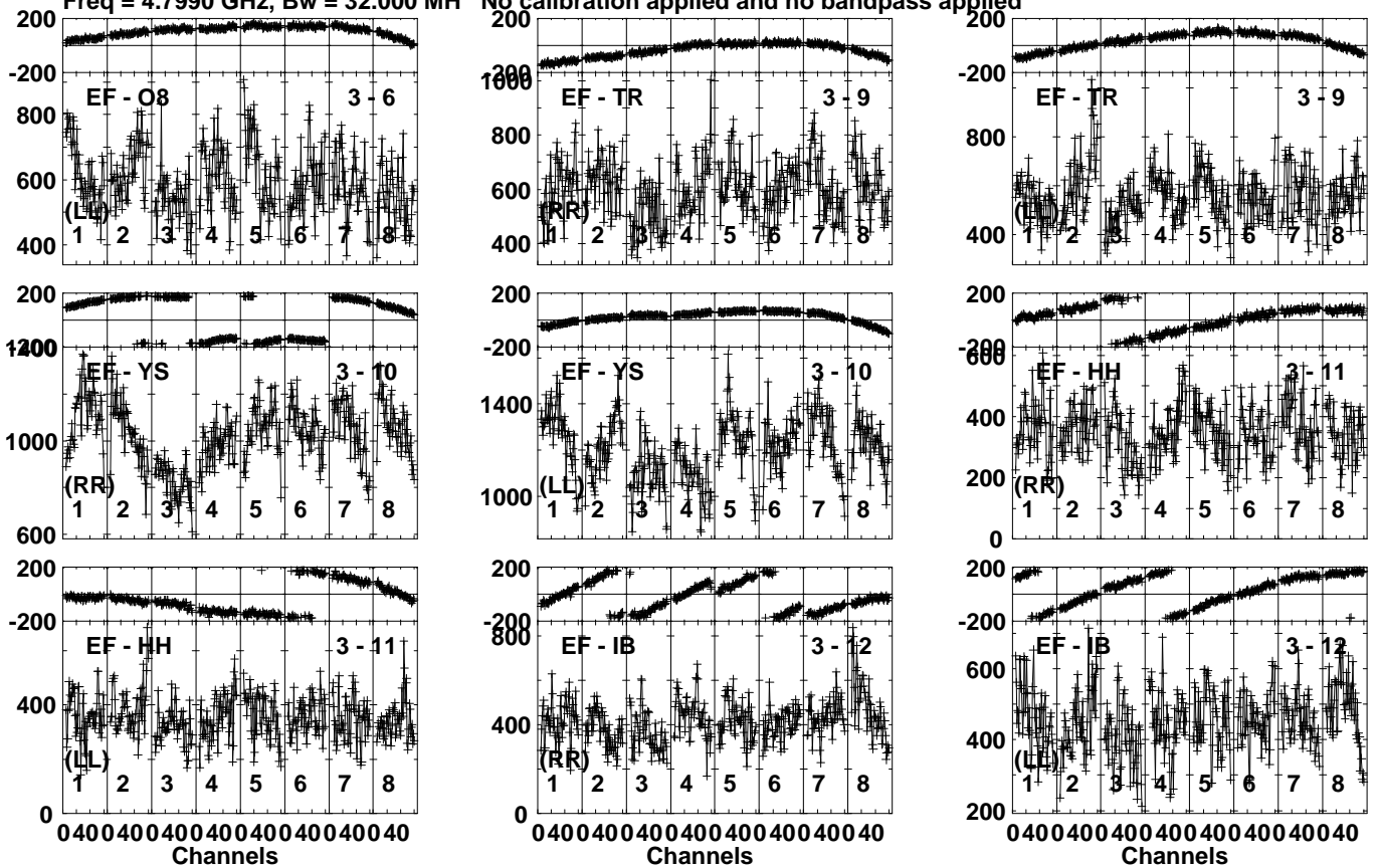
Lower frame: Micro Ampl Jy Top frame: Phas deg Vector averaged cross-power spectrum Several baselines displayed Timerange: 00/05:37:01 to 00/05:39:29
