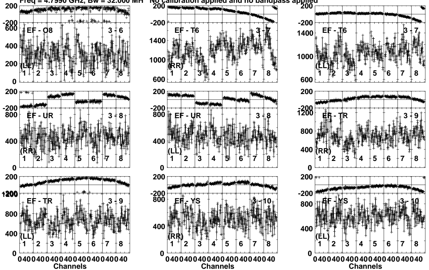
Lower frame: Micro Ampl Jy Top frame: Phas deg Vector averaged cross-power spectrum Several baselines displayed Timerange: 00/02:12:51 to 00/02:14:19
