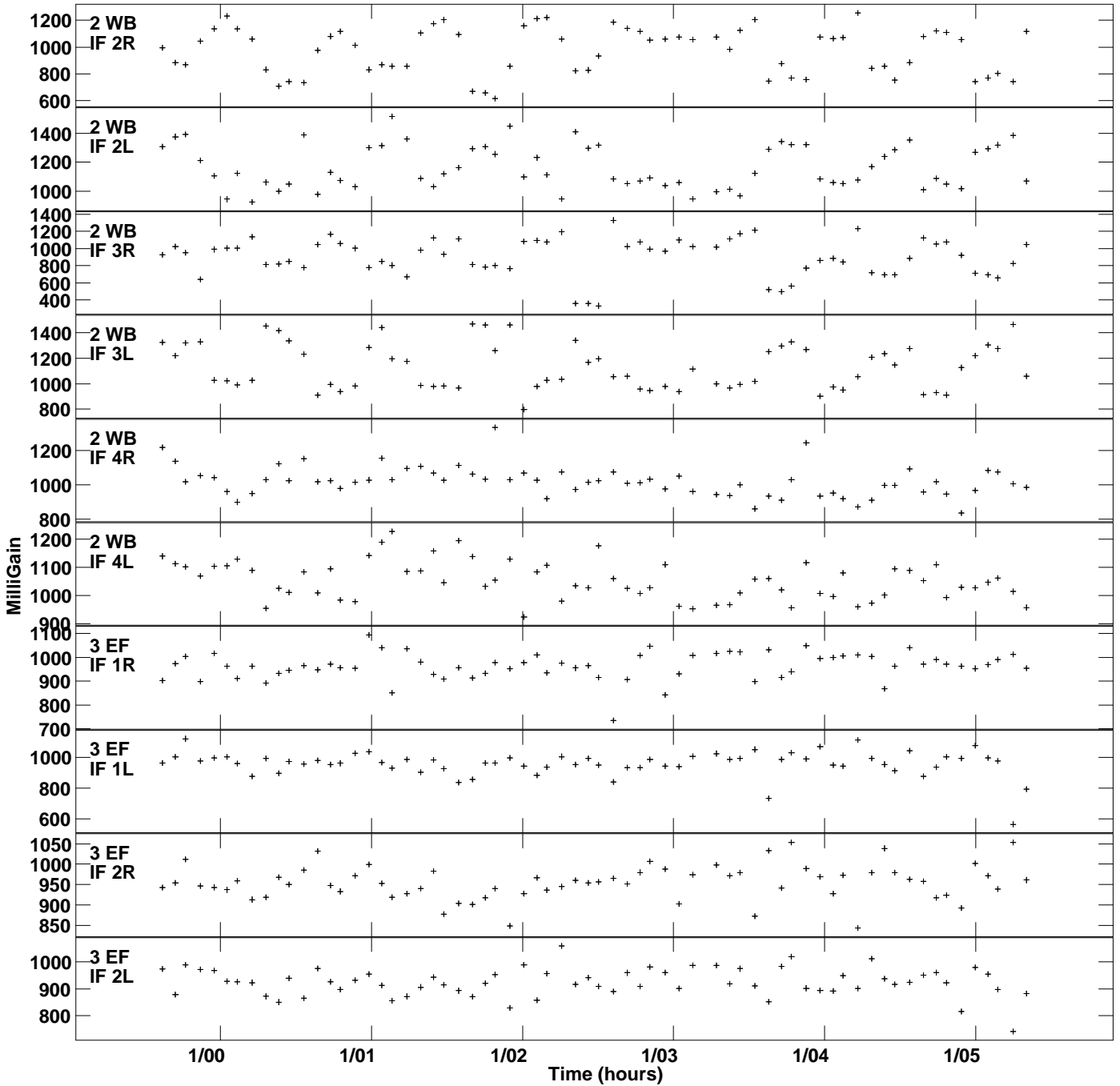
Plot file version 2 created 12-JUN-2023 14:52:35 Gain amp vs UTC time for J1547+2052.MULTI.1 SN 2 Rpol & Lpol IF 1 - 4
