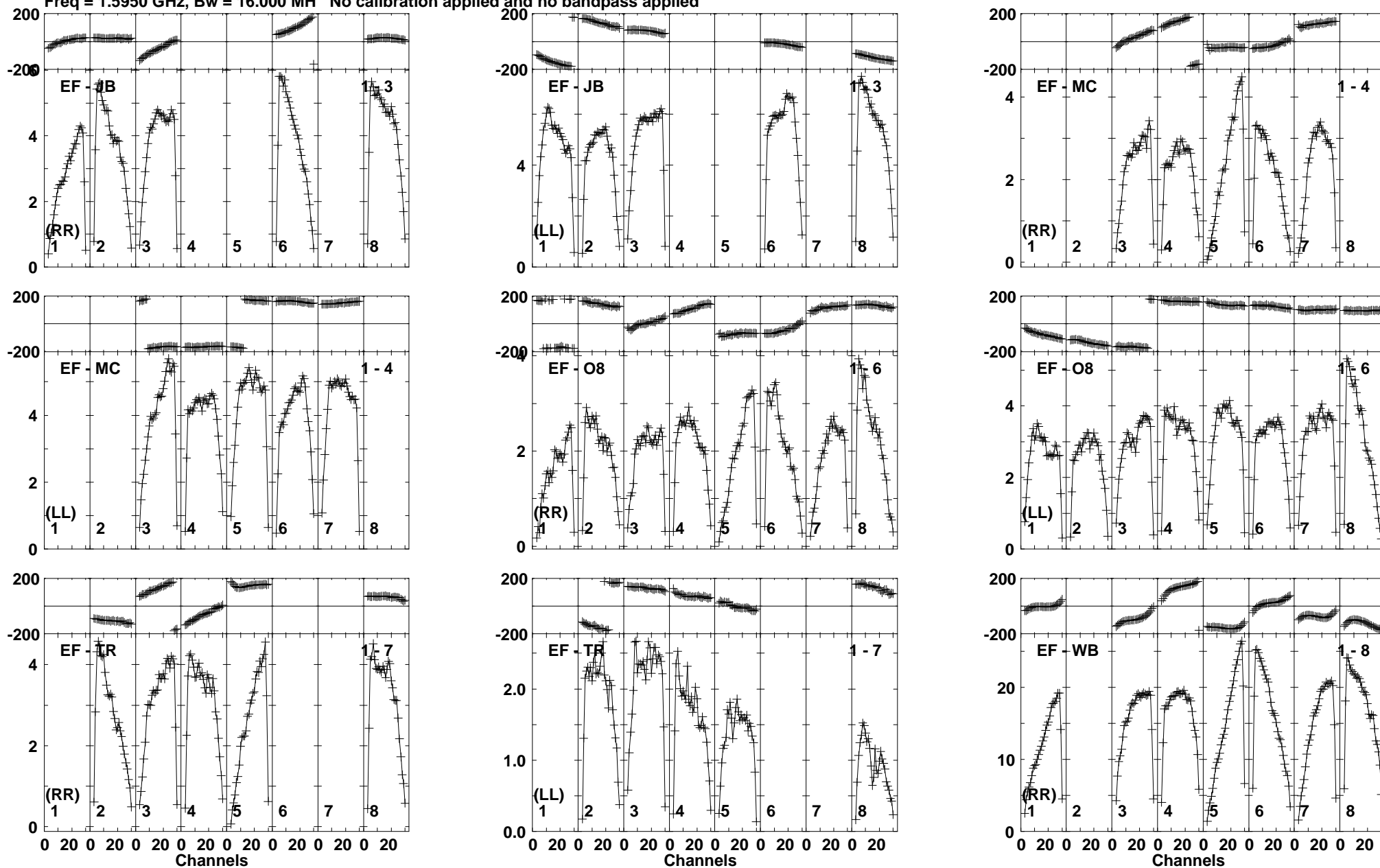
Lower frame: Milli Ampl Jy Top frame: Phas deg Vector averaged cross-power spectrum Baseline: EF (01) - JB (03) Timerange: 01/05:48:32 to 01/05:49:48
