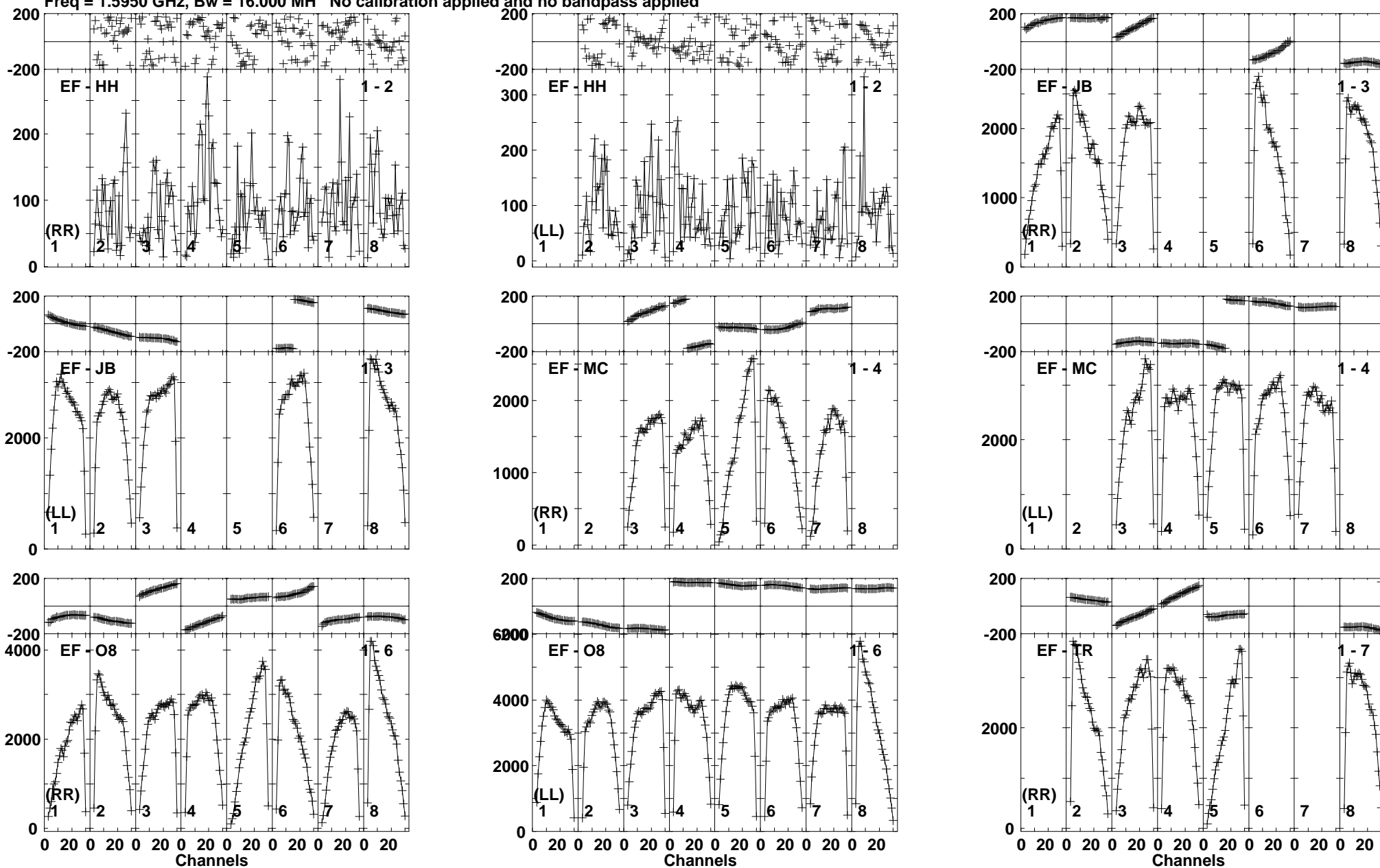
Lower frame: Micro Ampl Jy Top frame: Phas deg Vector averaged cross-power spectrum Baseline: EF (01) - HH (02) Timerange: 01/01:33:02 to 01/01:36:28
