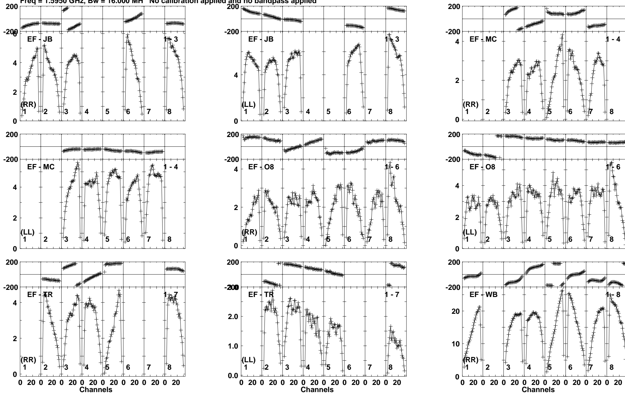
Lower frame: Milli Amp Jy Top frame: Phas deg Vector averaged cross-power spectrum Baseline: EF (01) - JB (03) Timerange: 01/05:38:32 to 01/05:39:48
