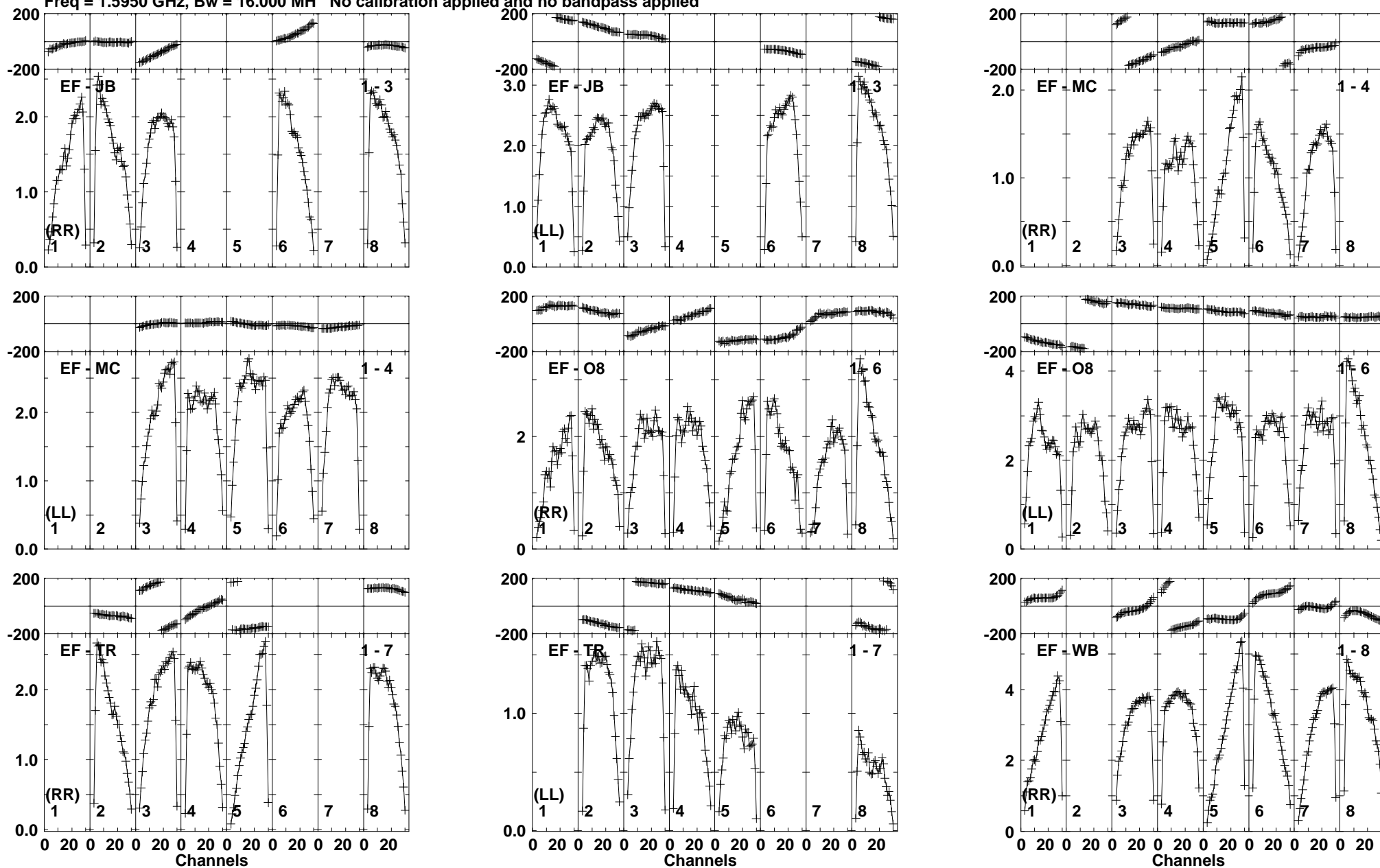
Lower frame: Milli Ampl Jy Top frame: Phas deg Vector averaged cross-power spectrum Baseline: EF (01) - JB (03) Timerange: 01/06:09:52 to 01/06:13:18
