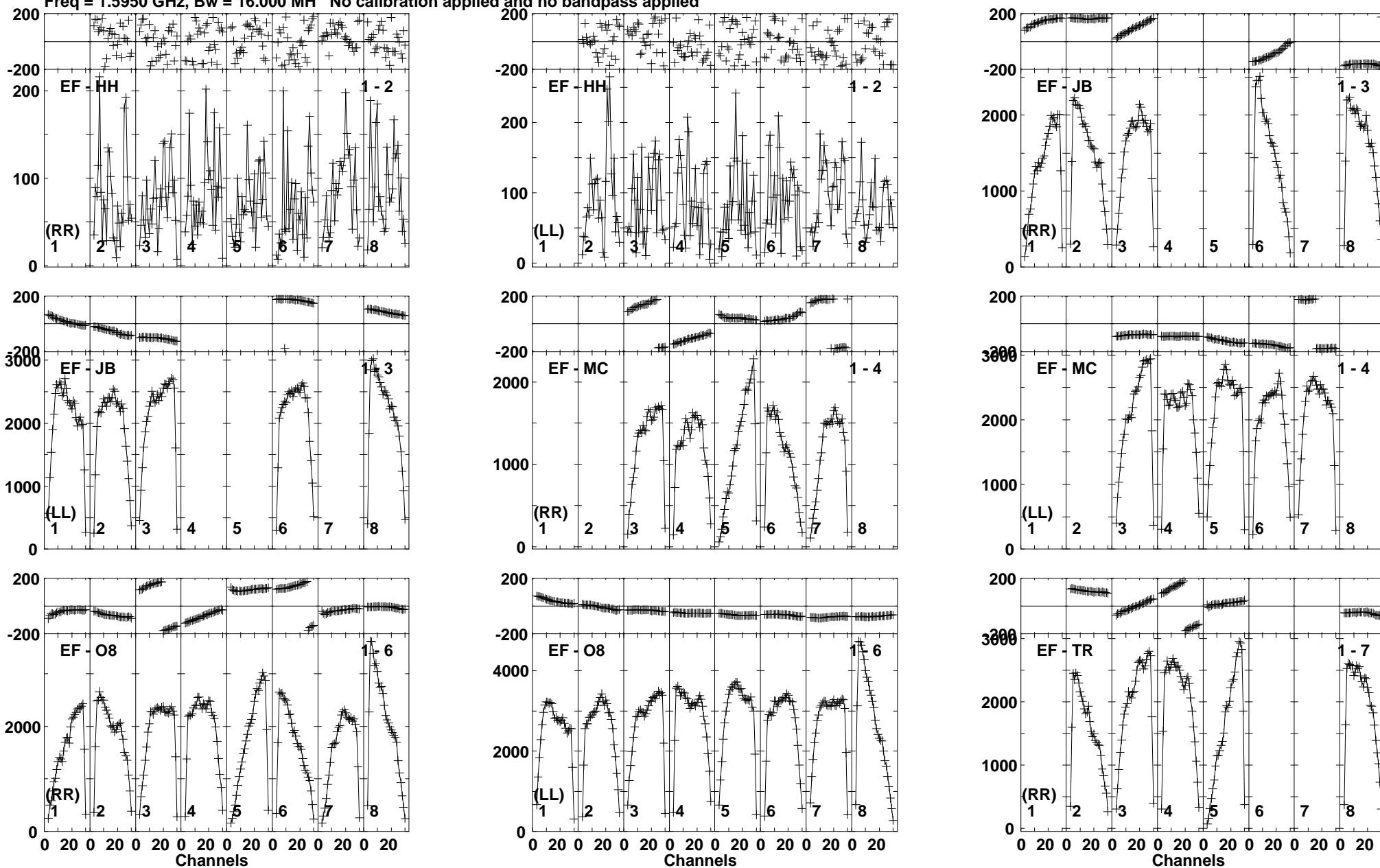
Lower frame: Micro Ampl Jy Top frame: Phas deg Vector averaged cross-power spectrum Baseline: EF (01) - HH (02) Timerange: 01/03:07:52 to 01/03:11:18
