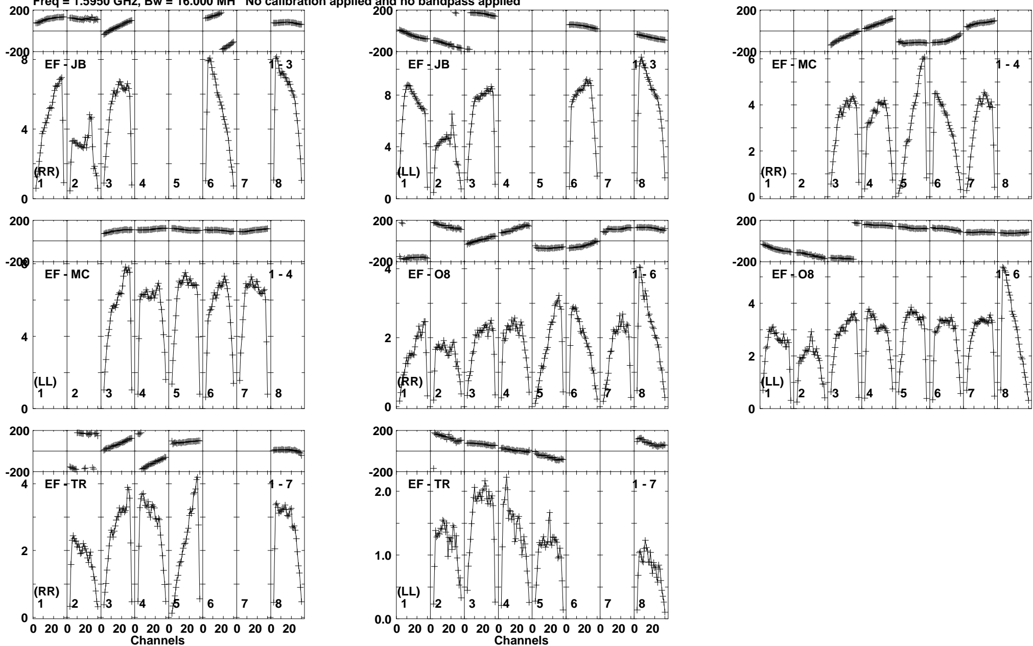
Lower frame: Milli Ampl Jy Top frame: Phas deg Vector averaged cross-power spectrum Baseline: EF (01) - JB (03) Timerange: 01/07:54:02 to 01/07:54:58
