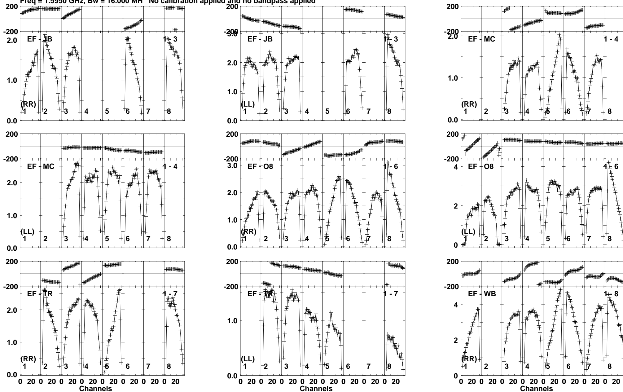
Lower frame: Milli Ampl Jy Top frame: Phas deg Vector averaged cross-power spectrum Baseline: EF (01) - JB (03) Timerange: 01/04:35:02 to 01/04:38:28
