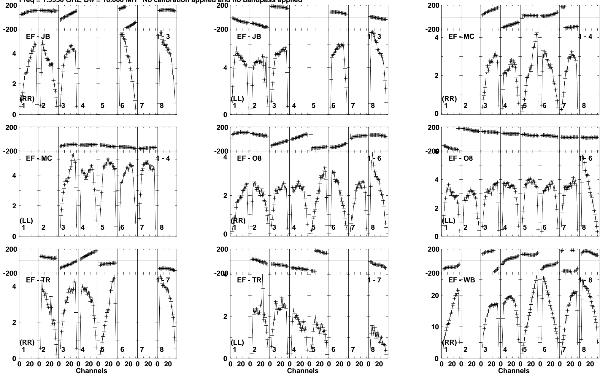
Lower frame: Milli Ampl Jy Top frame: Phas deg Vector averaged cross-power spectrum Baseline: EF (01) - JB (03) Timerange: 01/05:18:32 to 01/05:19:48
