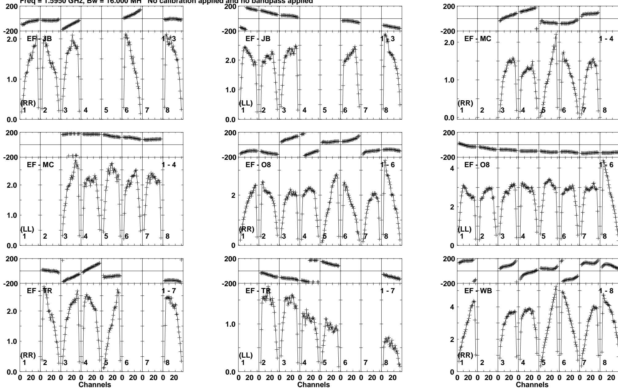
Lower frame: Milli Ampl Jy Top frame: Phas deg Vector averaged cross-power spectrum Baseline: EF (01) - JB (03) Timerange: 01/03:55:02 to 01/03:58:28
