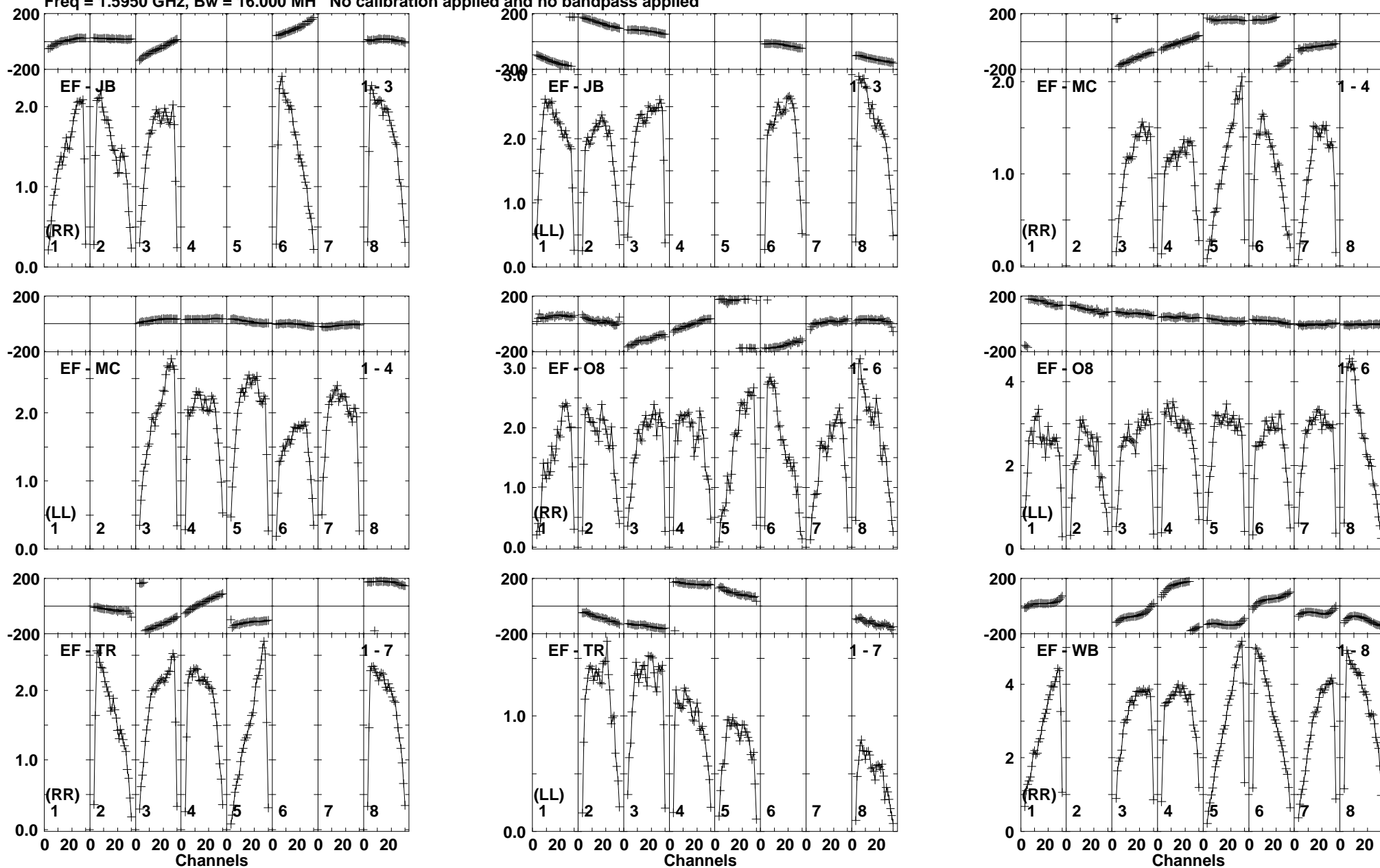
Lower frame: Milli Ampl Jy Top frame: Phas deg Vector averaged cross-power spectrum Baseline: EF (01) - JB (03) Timerange: 01/05:35:02 to 01/05:38:28
