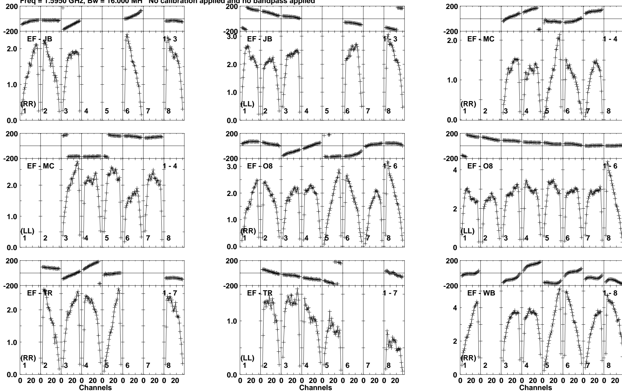
Lower frame: Milli Ampl Jy Top frame: Phas deg Vector averaged cross-power spectrum Baseline: EF (01) - JB (03) Timerange: 01/05:25:02 to 01/05:28:28
