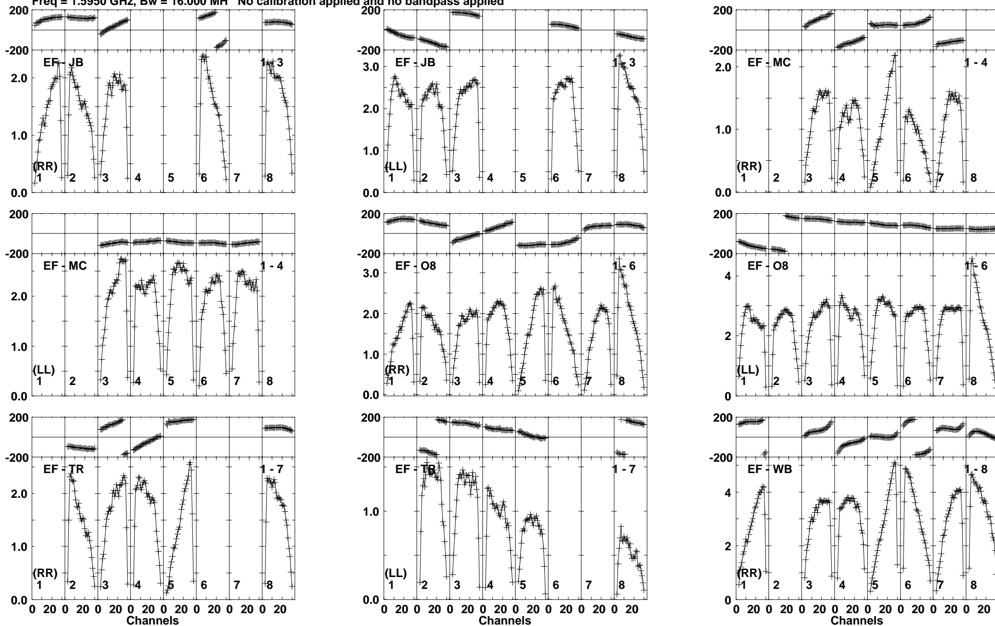
Lower frame: Milli Ampl Jy Top frame: Phas deg Vector averaged cross-power spectrum Baseline: EF (01) - JB (03) Timerange: 01/06:55:02 to 01/06:58:28
