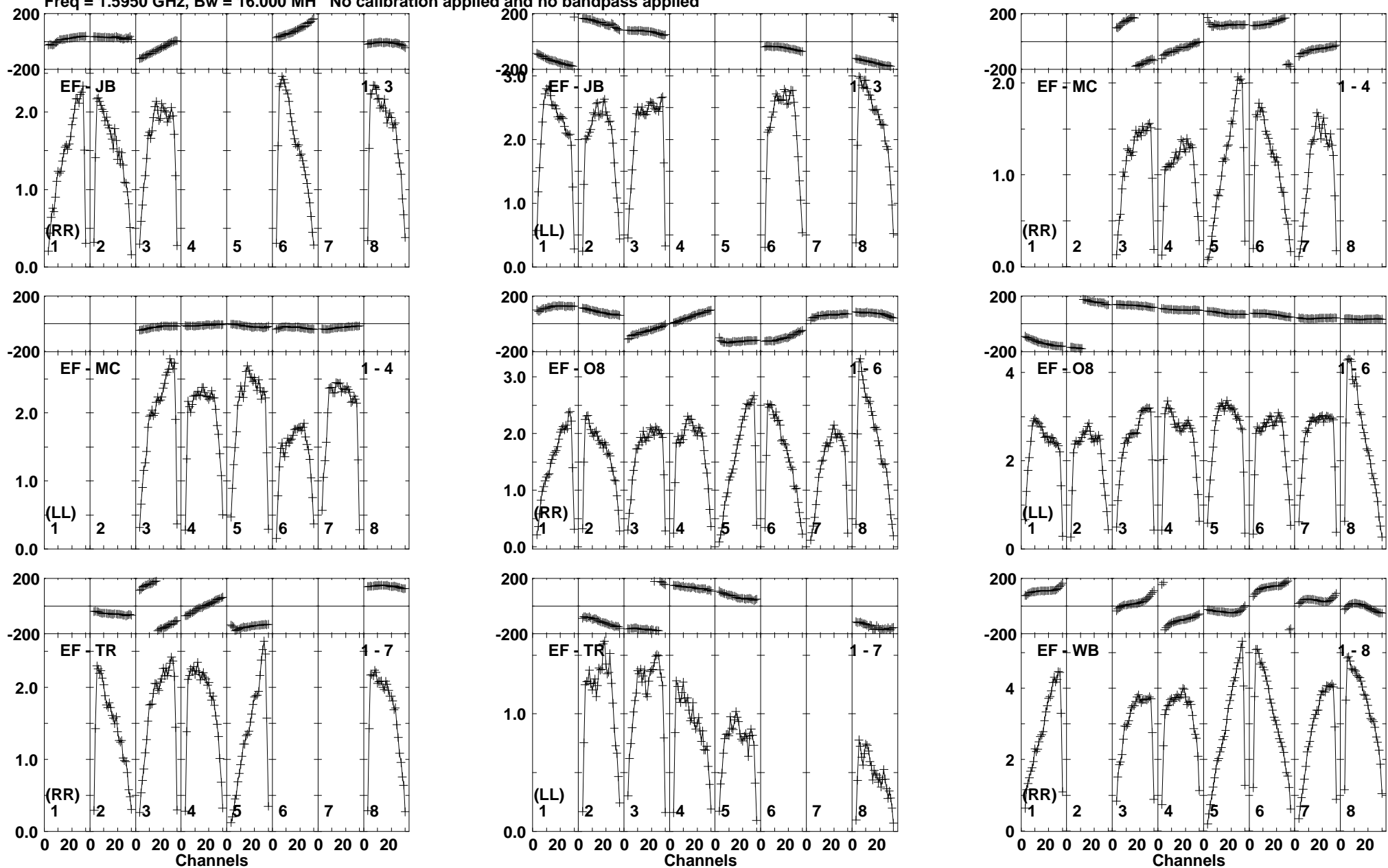
Lower frame: Milli Ampl Jy Top frame: Phas deg Vector averaged cross-power spectrum Baseline: EF (01) - JB (03) Timerange: 01/06:45:02 to 01/06:48:28
