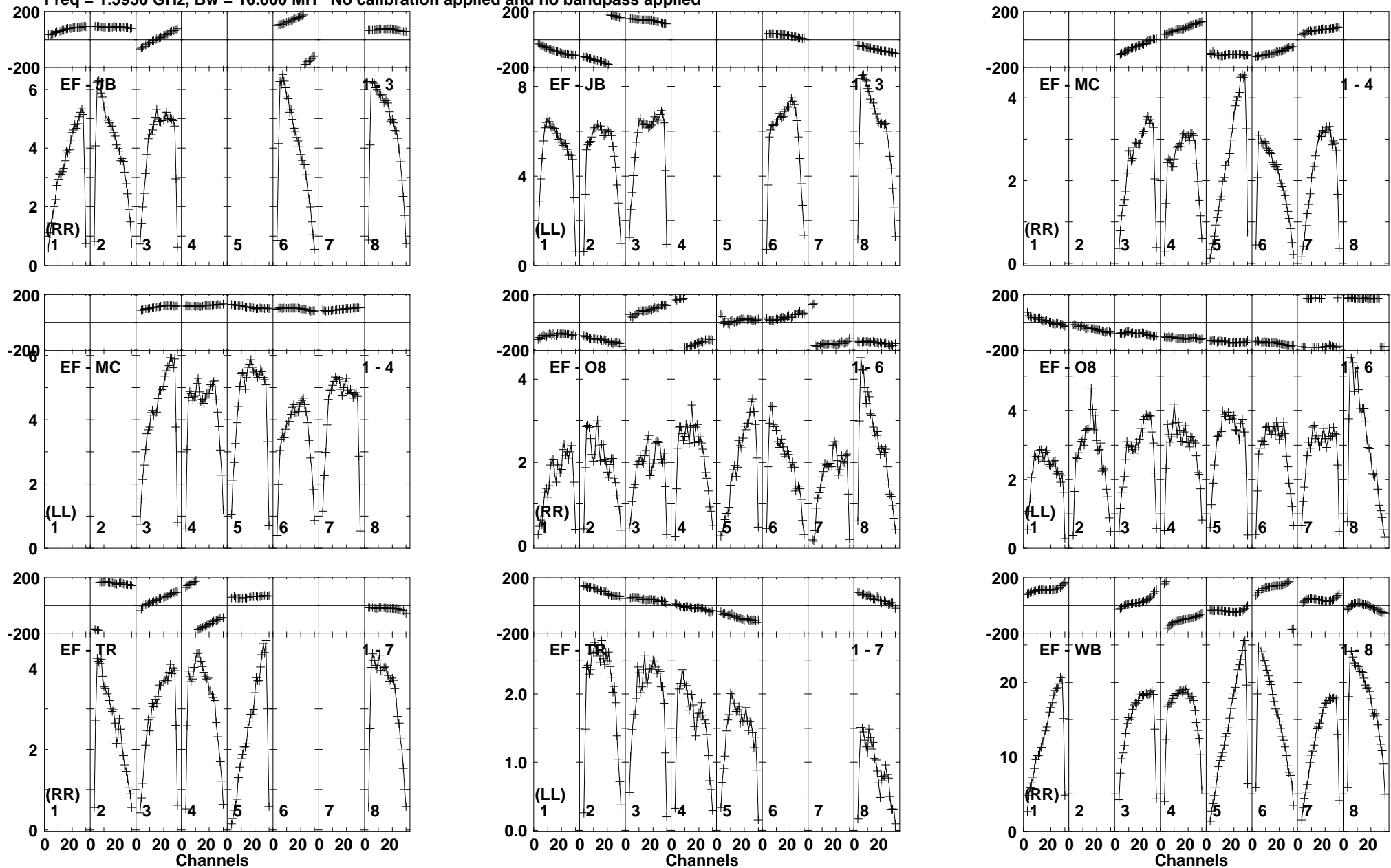
Lower frame: Milli Ampl Jy Top frame: Phas deg Vector averaged cross-power spectrum Baseline: EF (01) - JB (03) Timerange: 01/06:28:32 to 01/06:29:48
