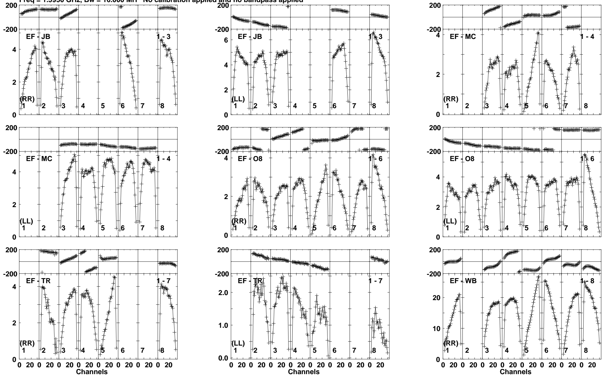
Lower frame: Milli Ampl Jy Top frame: Phas deg Vector averaged cross-power spectrum Baseline: EF (01) - JB (03) Timerange: 01/04:48:32 to 01/04:49:48
