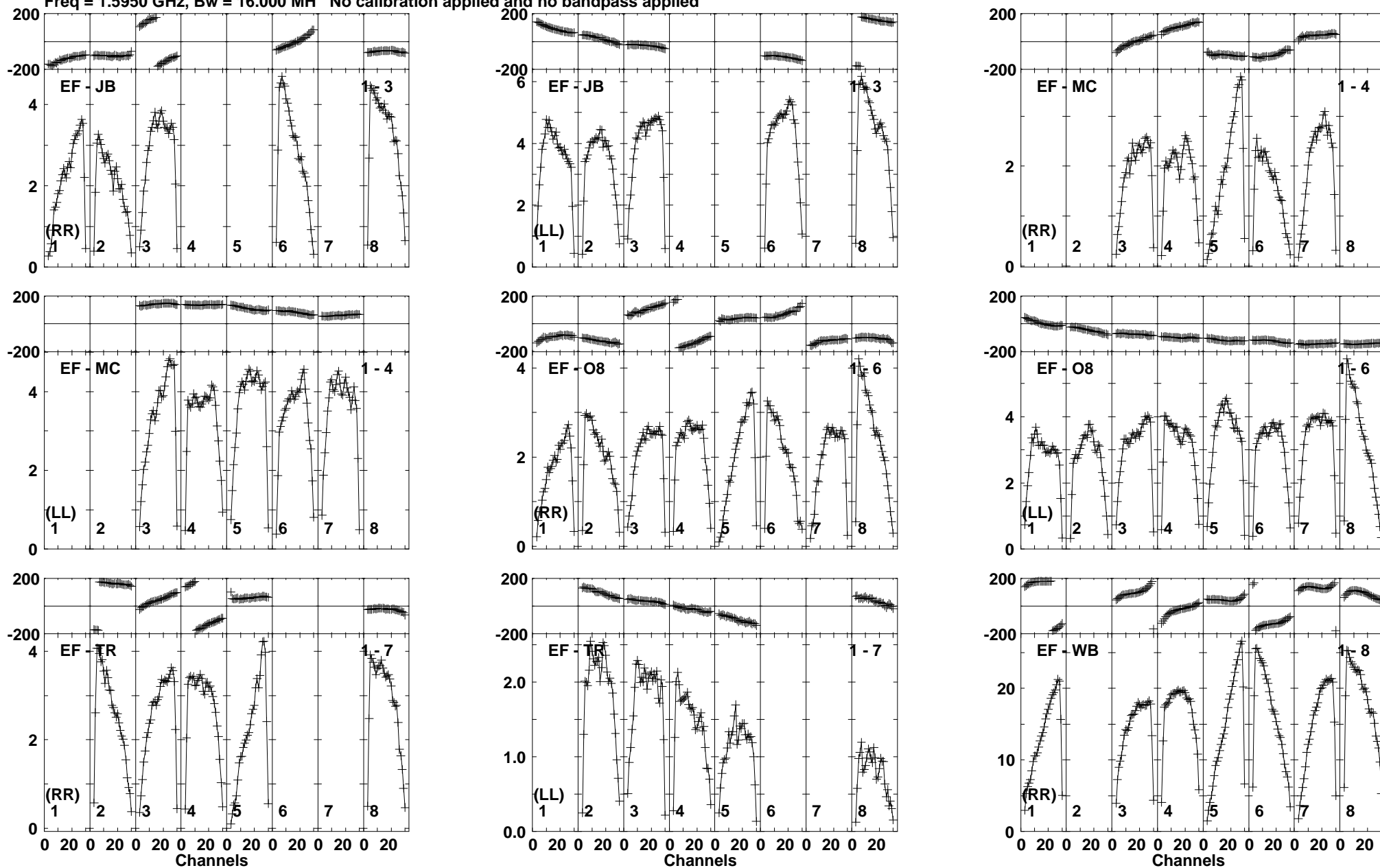
Lower frame: Milli Ampl Jy Top frame: Phas deg Vector averaged cross-power spectrum Baseline: EF (01) - JB (03) Timerange: 01/04:14:02 to 01/04:14:58
