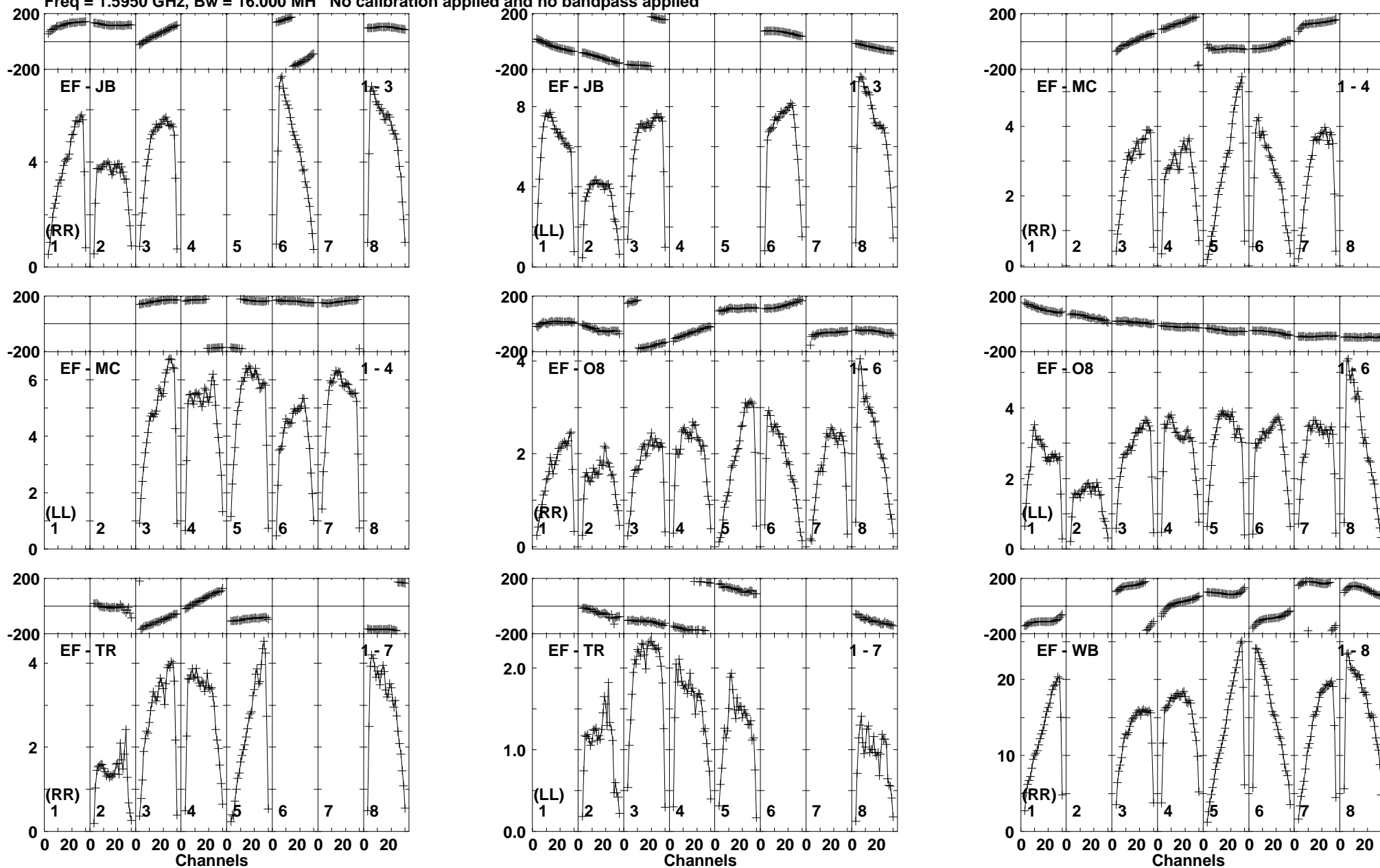
Lower frame: Milli Ampl Jy Top frame: Phas deg Vector averaged cross-power spectrum Baseline: EF (01) - JB (03) Timerange: 01/07:08:32 to 01/07:09:48
