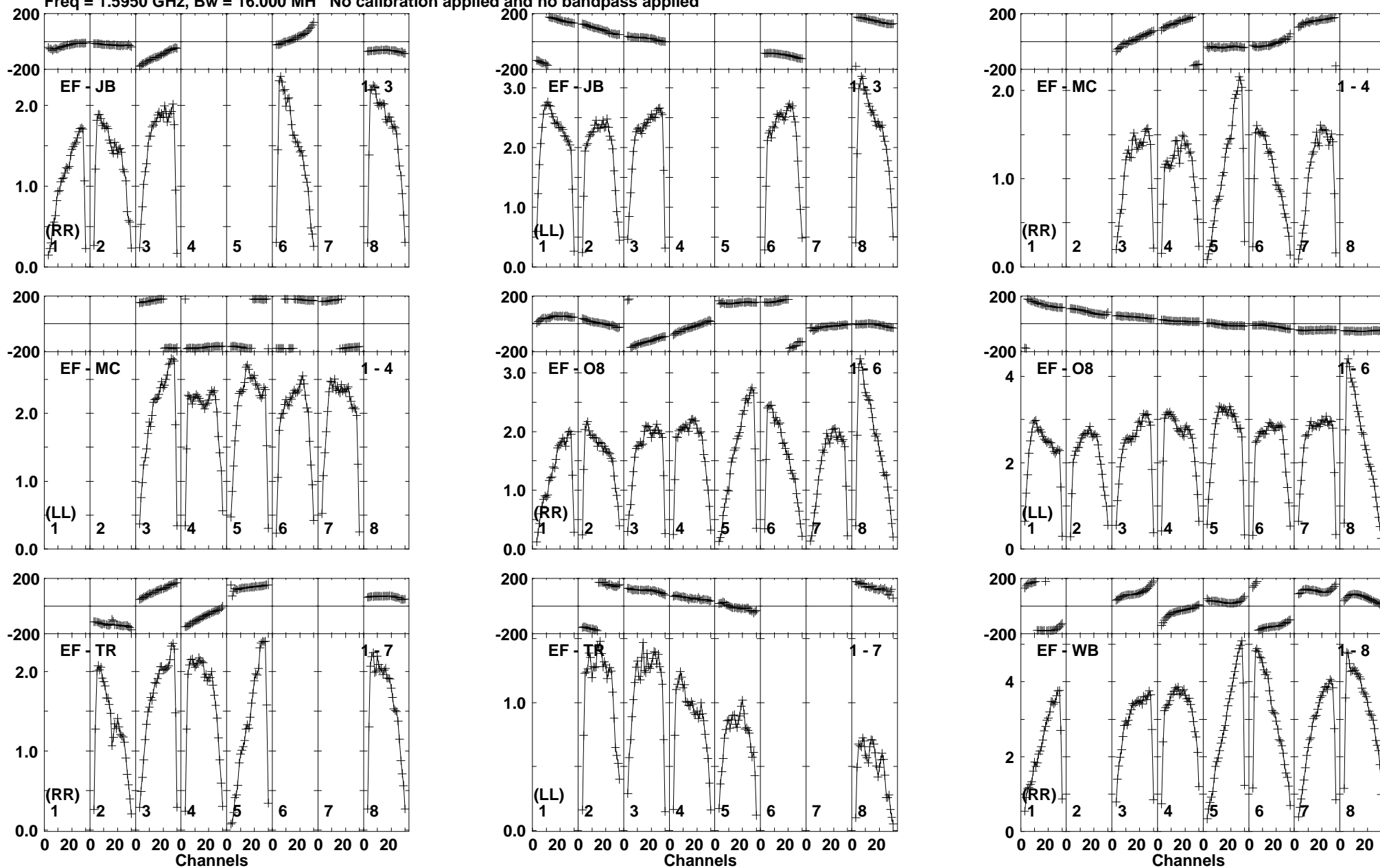
Lower frame: Milli Amply Jy Top frame: Phas deg Vector averaged cross-power spectrum Baseline: EF (01) - JB (03) Timerange: 01/07:19:52 to 01/07:23:18
