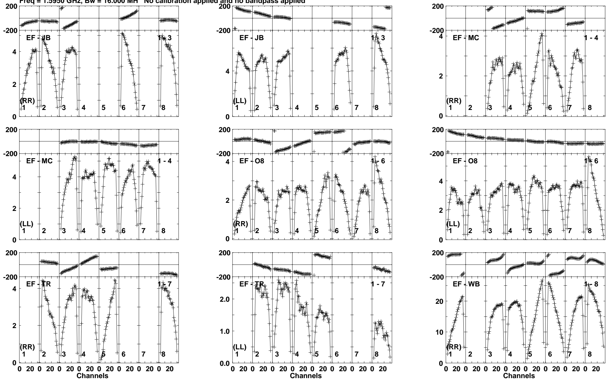
Lower frame: Milli Ampl Jy Top frame: Phas deg Vector averaged cross-power spectrum Baseline: EF (01) - JB (03) Timerange: 01/05:08:32 to 01/05:09:48
