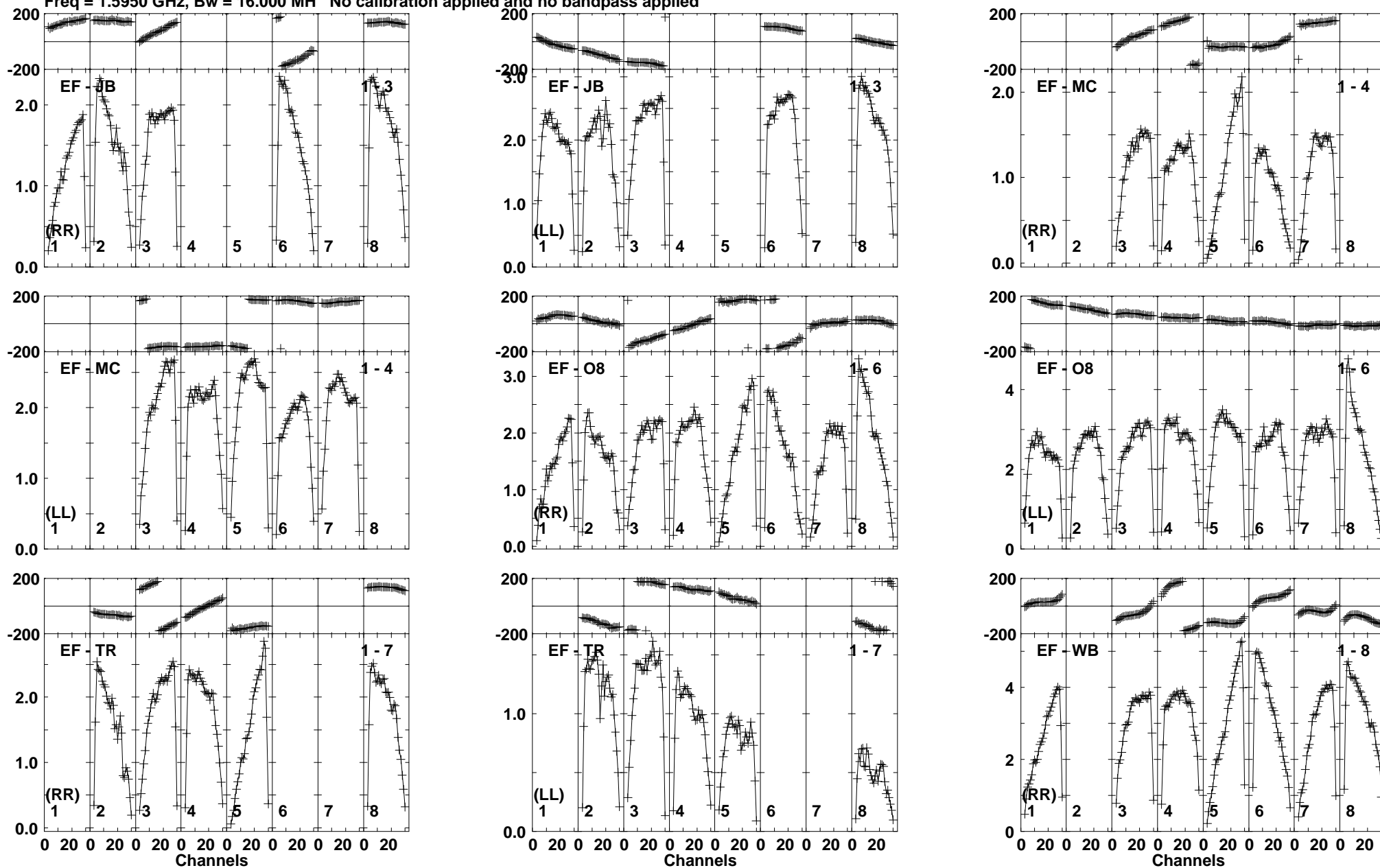
Lower frame: Milli Ampl Jy Top frame: Phas deg Vector averaged cross-power spectrum Baseline: EF (01) - JB (03) Timerange: 01/05:49:52 to 01/05:53:18
