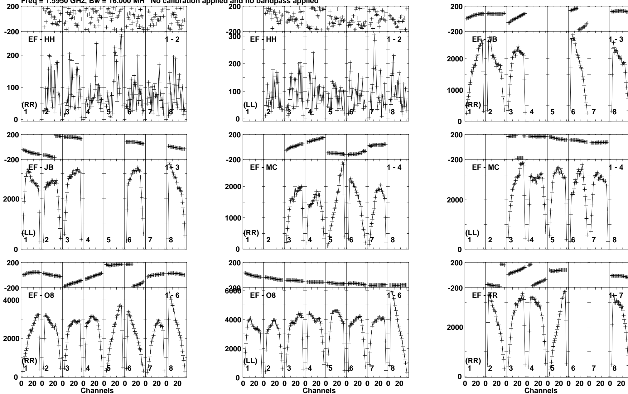
Lower frame: Micro Ampl Jy Top frame: Phas deg Vector averaged cross-power spectrum Baseline: EF (01) - HH (02) Timerange: 01/01:03:02 to 01/01:06:28
