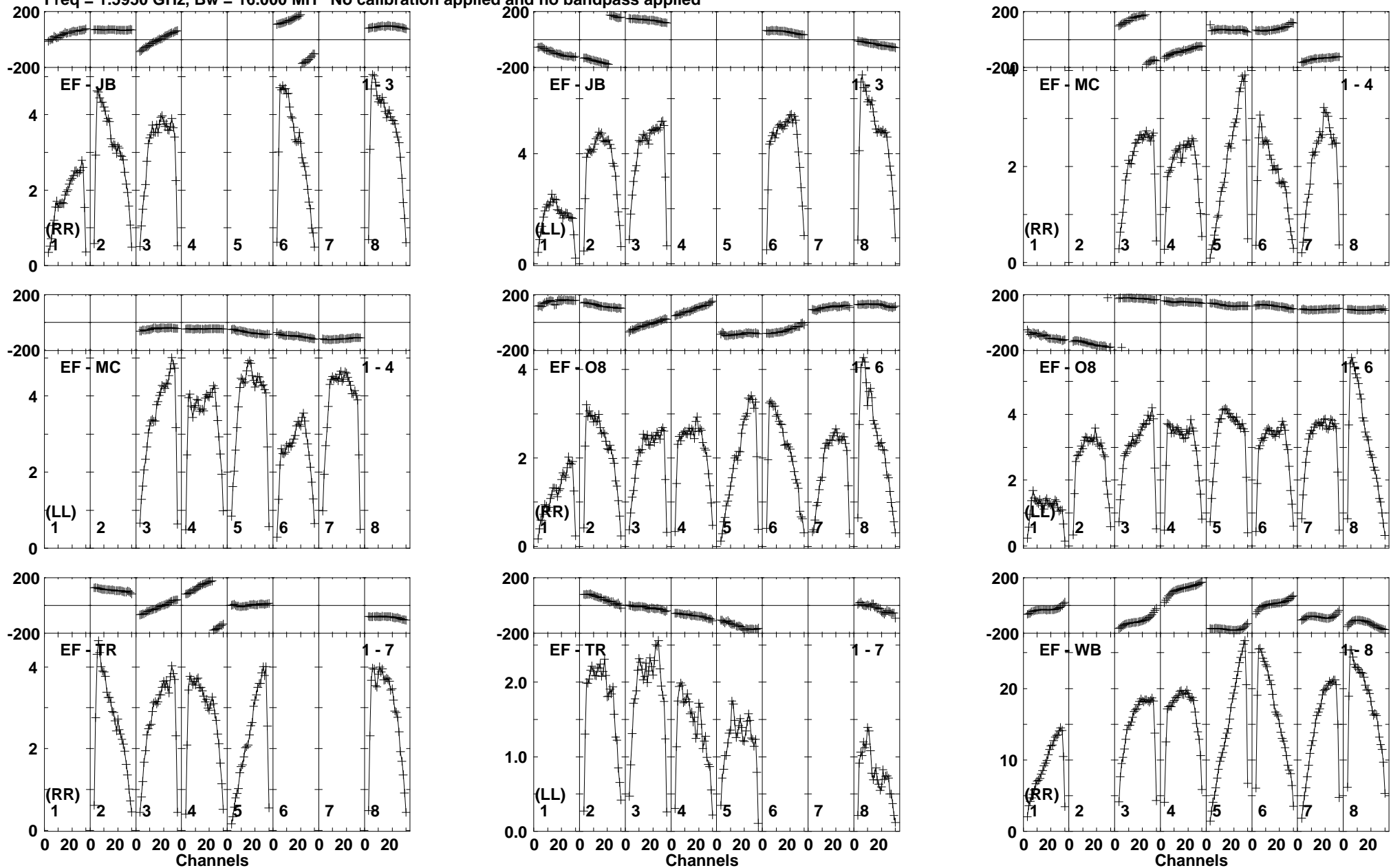
Lower frame: Milli Ampl Jy Top frame: Phas deg Vector averaged cross-power spectrum Baseline: EF (01) - JB (03) Timerange: 01/04:44:02 to 01/04:44:58
