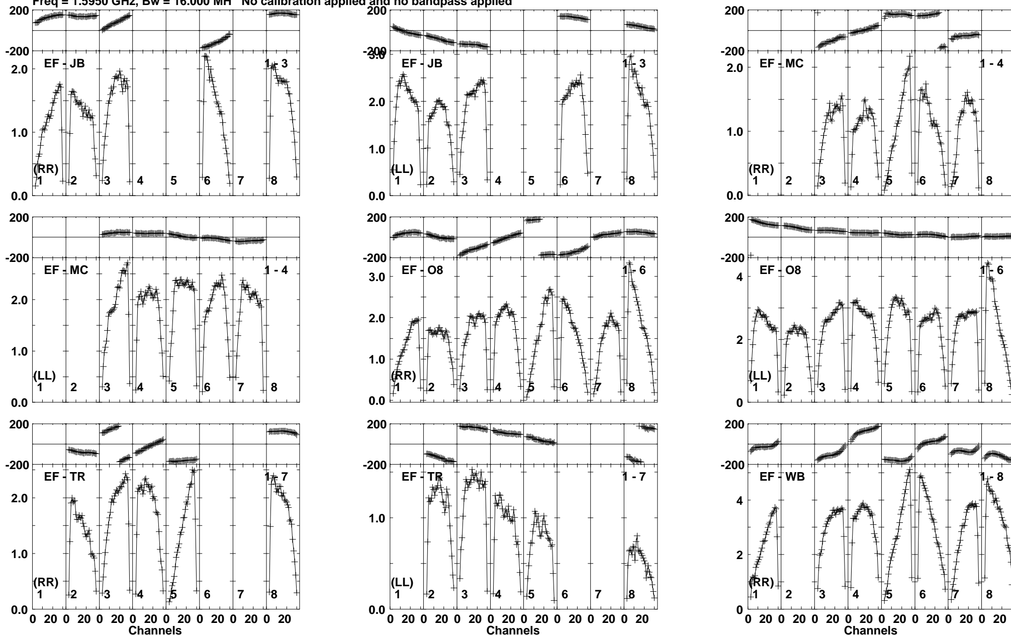
Lower frame: Milli Ampl Jy Top frame: Phas deg Vector averaged cross-power spectrum Baseline: EF (01) - JB (03) Timerange: 01/04:29:52 to 01/04:33:18
