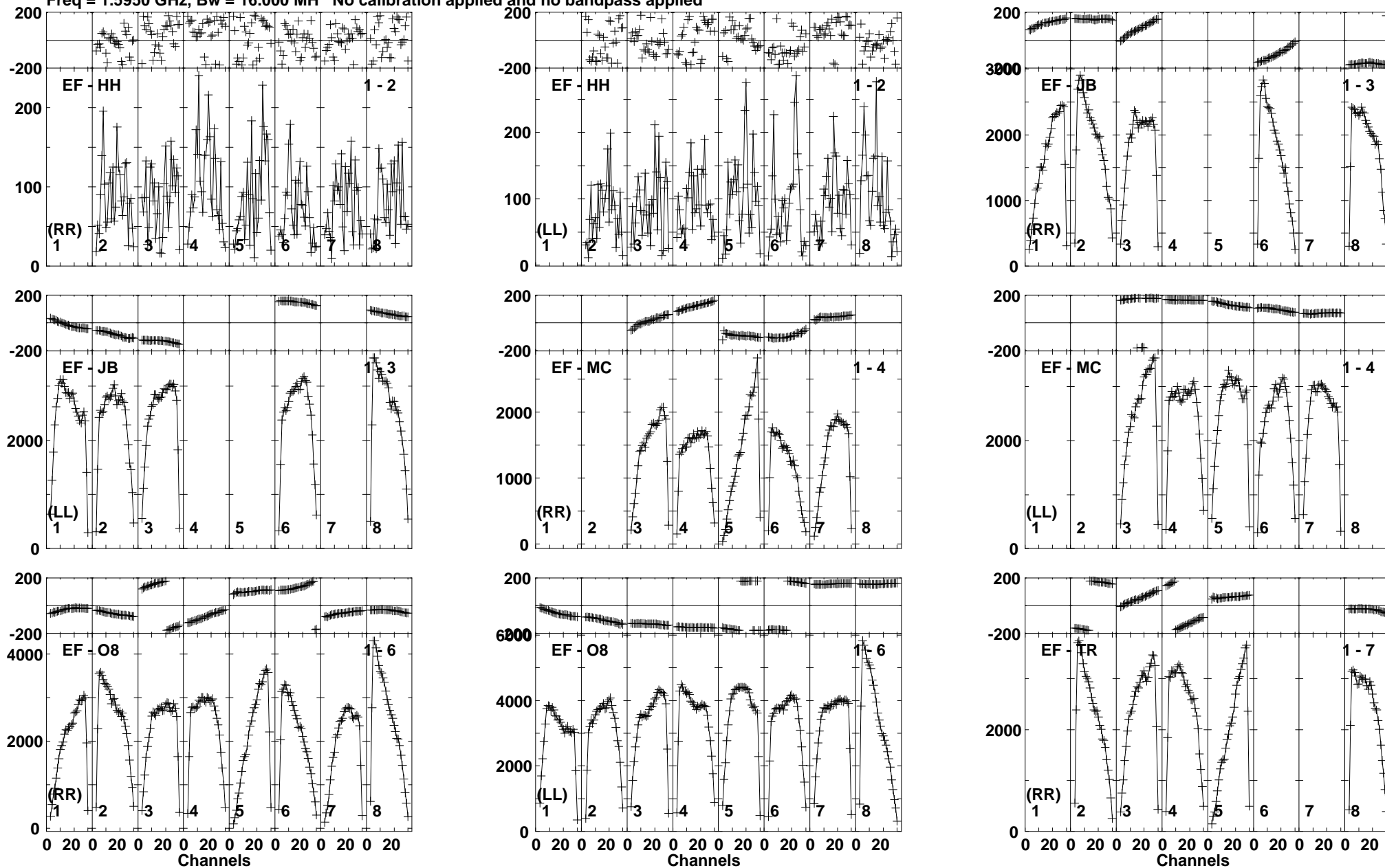
Lower frame: Micro Ampl Jy Top frame: Phas deg Vector averaged cross-power spectrum Baseline: EF (01) - HH (02) Timerange: 01/01:17:52 to 01/01:21:18
