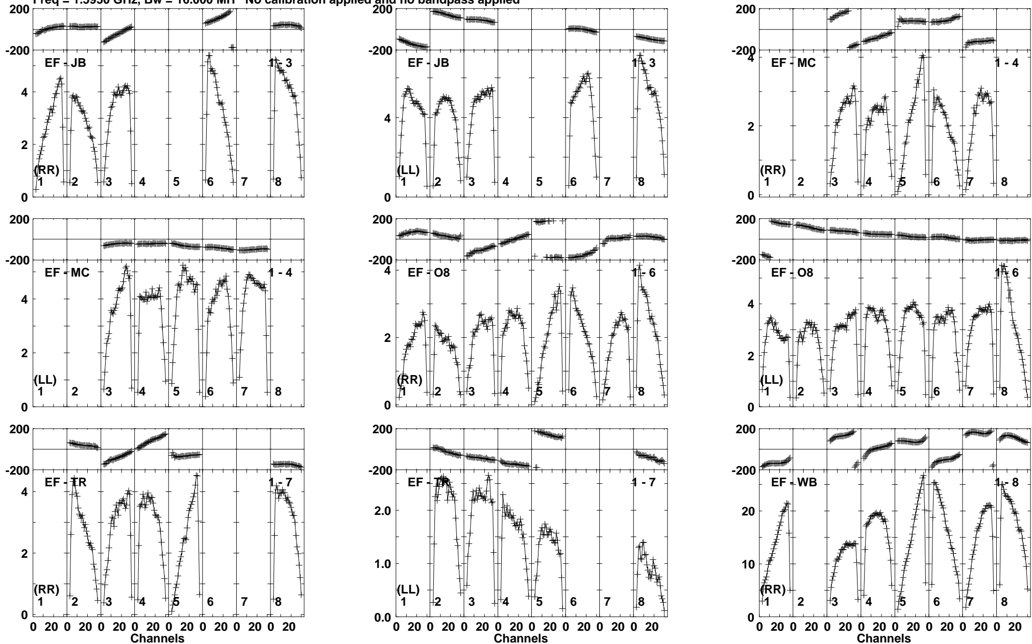
Lower frame: Milli Ampl Jy Top frame: Phas deg Vector averaged cross-power spectrum Baseline: EF (01) - JB (03) Timerange: 01/05:14:02 to 01/05:14:58
