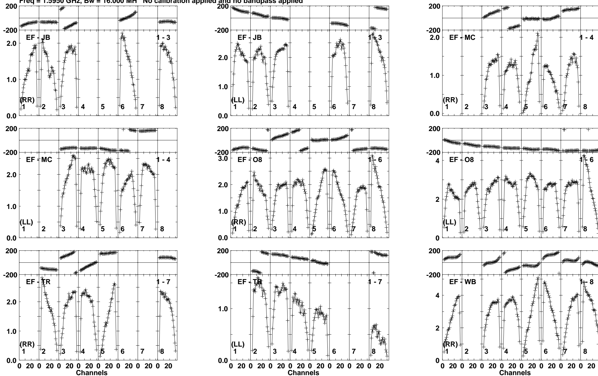
Lower frame: Milli Ampl Jy Top frame: Phas deg Vector averaged cross-power spectrum Baseline: EF (01) - JB (03) Timerange: 01/04:49:52 to 01/04:53:18
