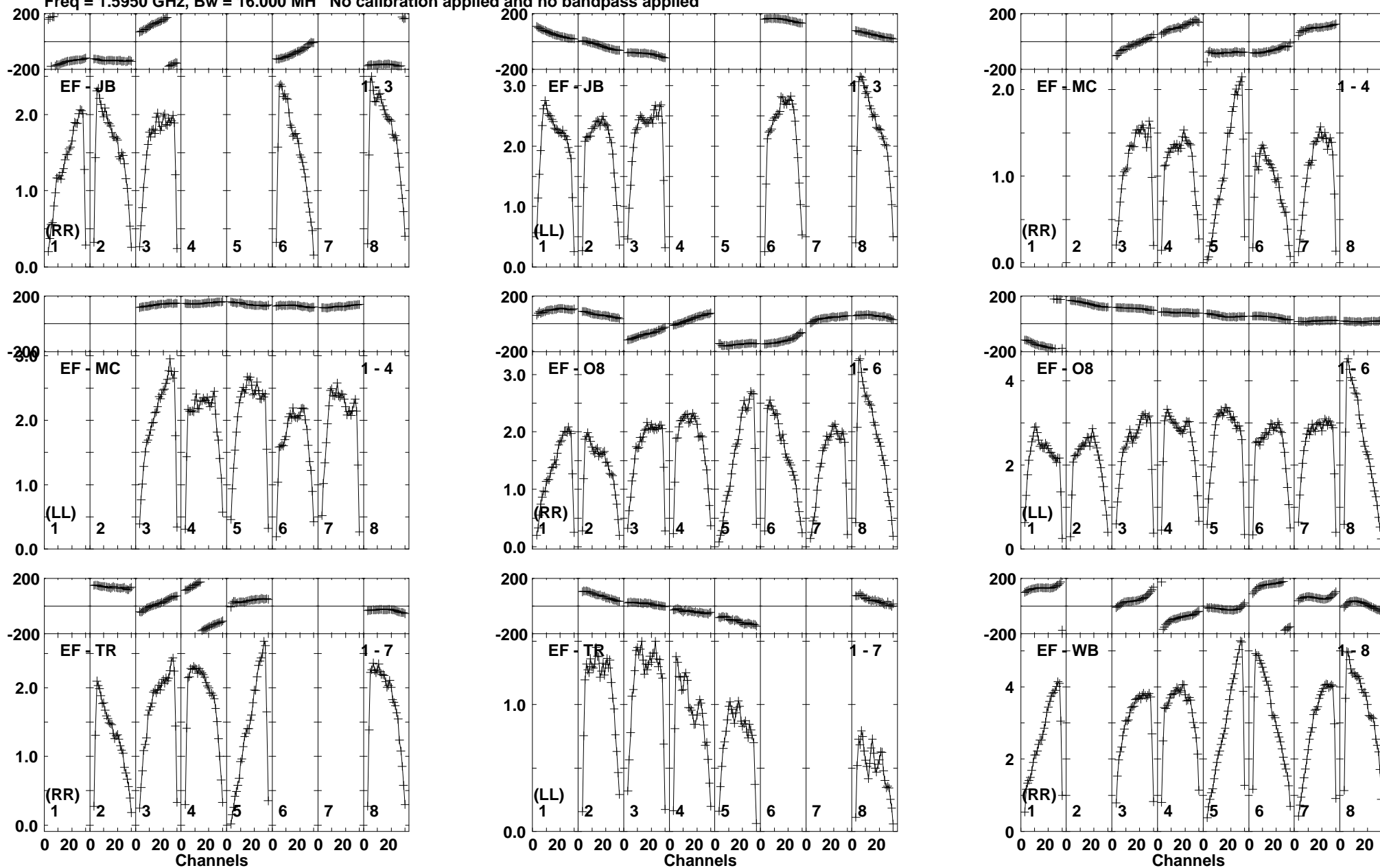
Lower frame: Milli Ampl Jy Top frame: Phas deg Vector averaged cross-power spectrum Baseline: EF (01) - JB (03) Timerange: 01/06:29:52 to 01/06:33:18
