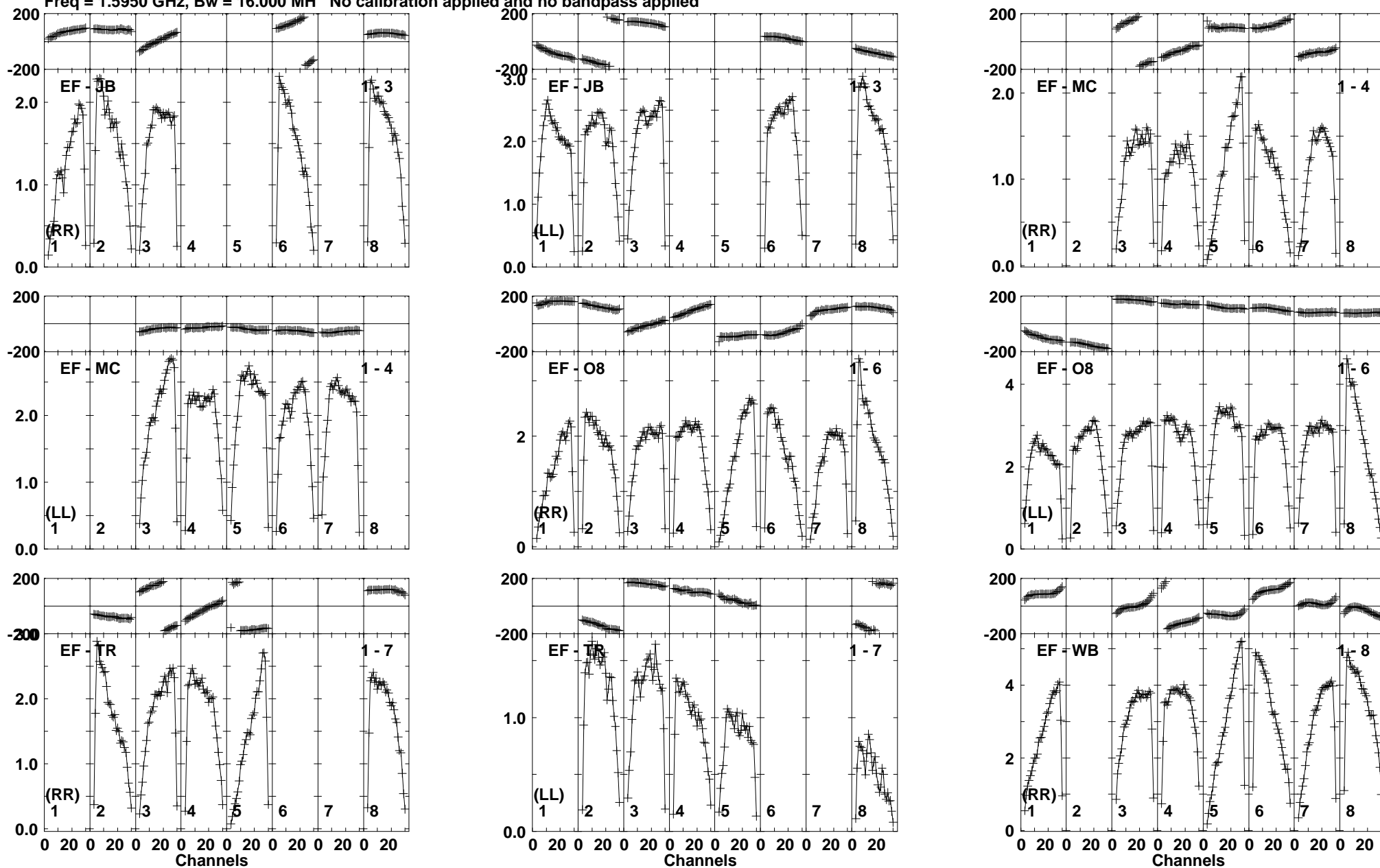
Lower frame: Milli Ampl Jy Top frame: Phas deg Vector averaged cross-power spectrum Baseline: EF (01) - JB (03) Timerange: 01/06:15:02 to 01/06:18:28
