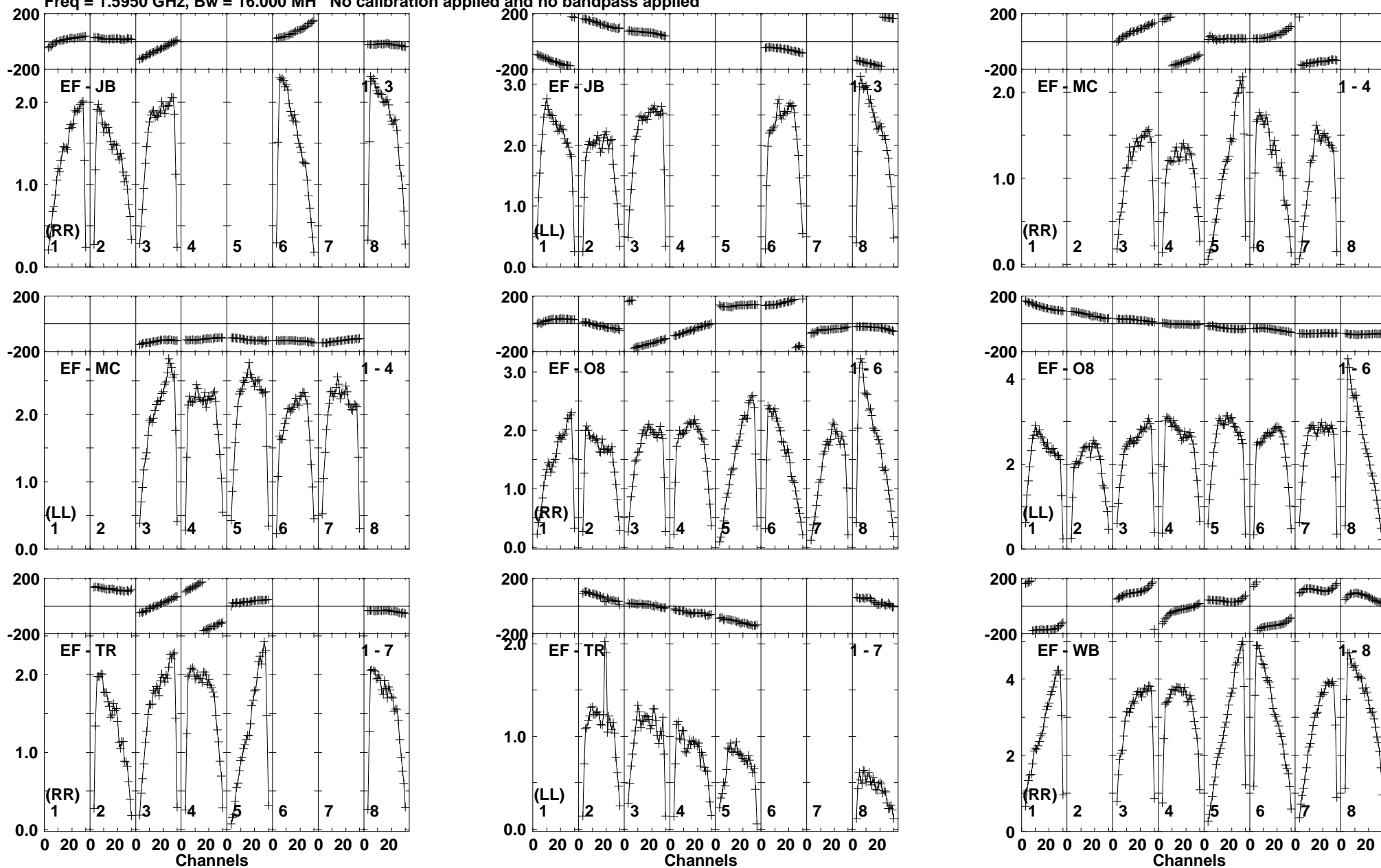
Lower frame: Milli Ampl Jy Top frame: Phas deg Vector averaged cross-power spectrum Baseline: EF (01) - JB (03) Timerange: 01/07:29:52 to 01/07:33:18
