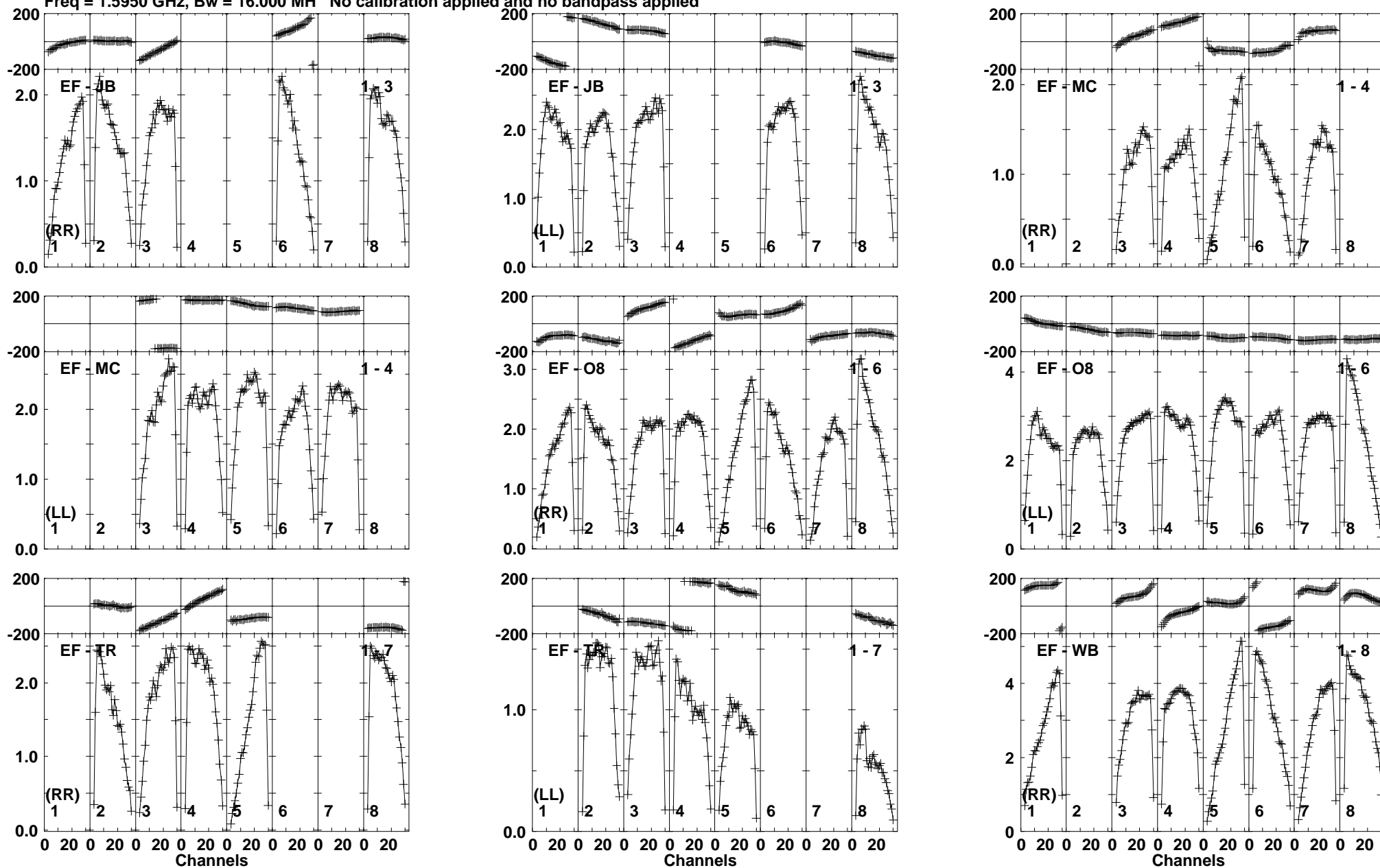
Lower frame: Milli Ampl Jy Top frame: Phas deg Vector averaged cross-power spectrum Baseline: EF (01) - JB (03) Timerange: 01/03:59:52 to 01/04:03:18
