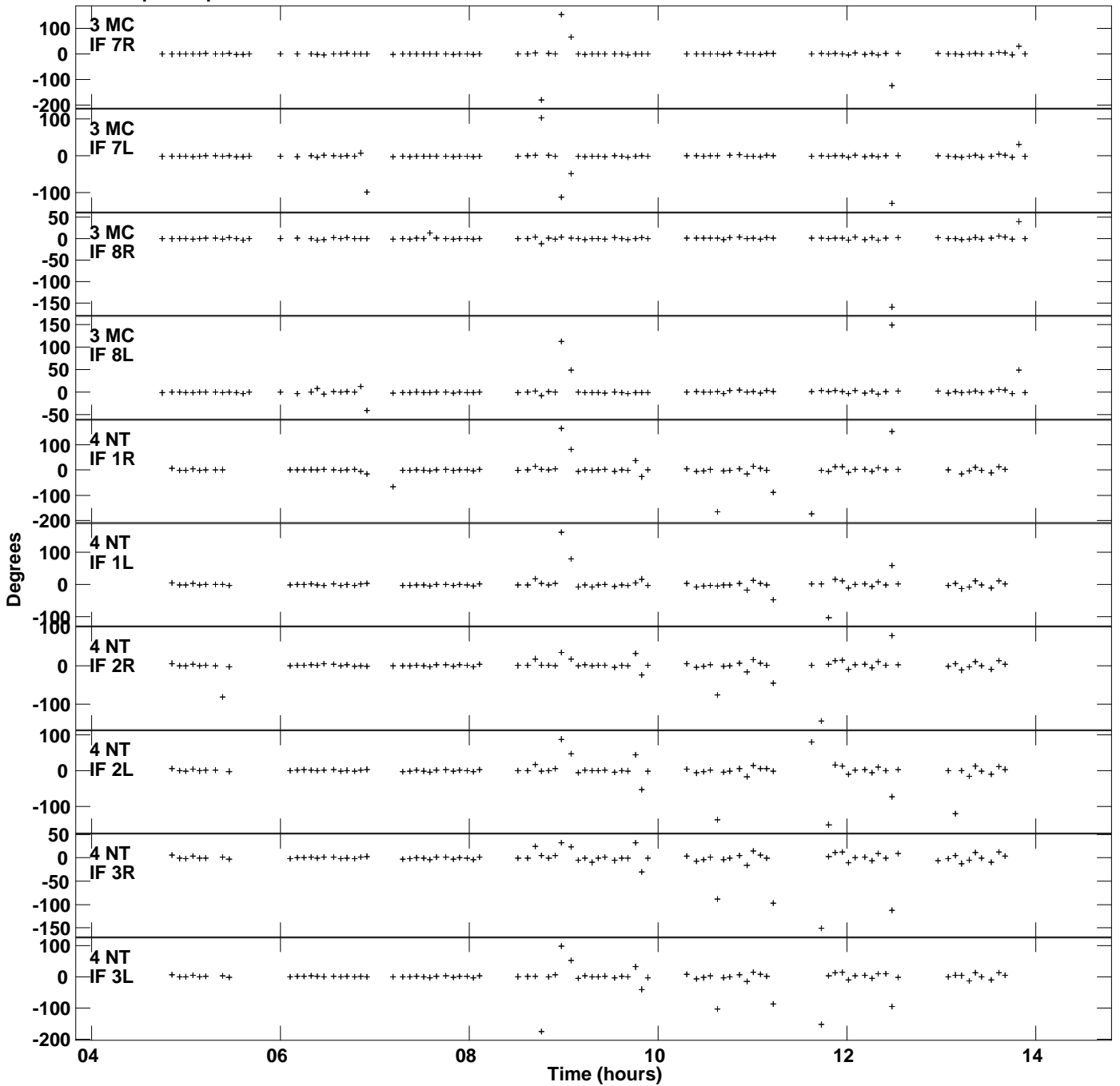
Plot file version 4 created 24-APR-2017 15:40:13 Gain phs vs UTC time for J2007+4029.MULTI.1 SN 1 Rpol & Lpol IF 1 - 8
