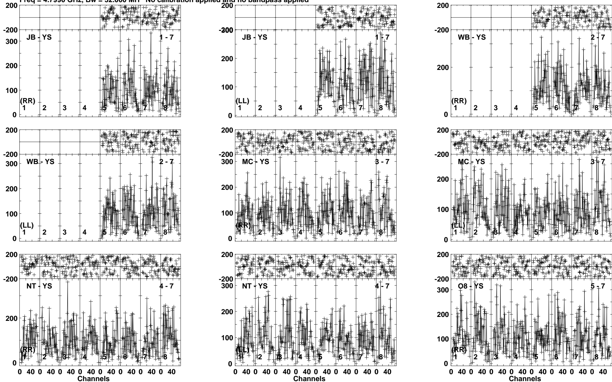
Lower frame: Micro Ampl Jy Top frame: Phas deg Vector averaged cross-power spectrum Baseline: JB (01) - YS (07) Timerange: 00:12:08:01 to 00:12:10:29
