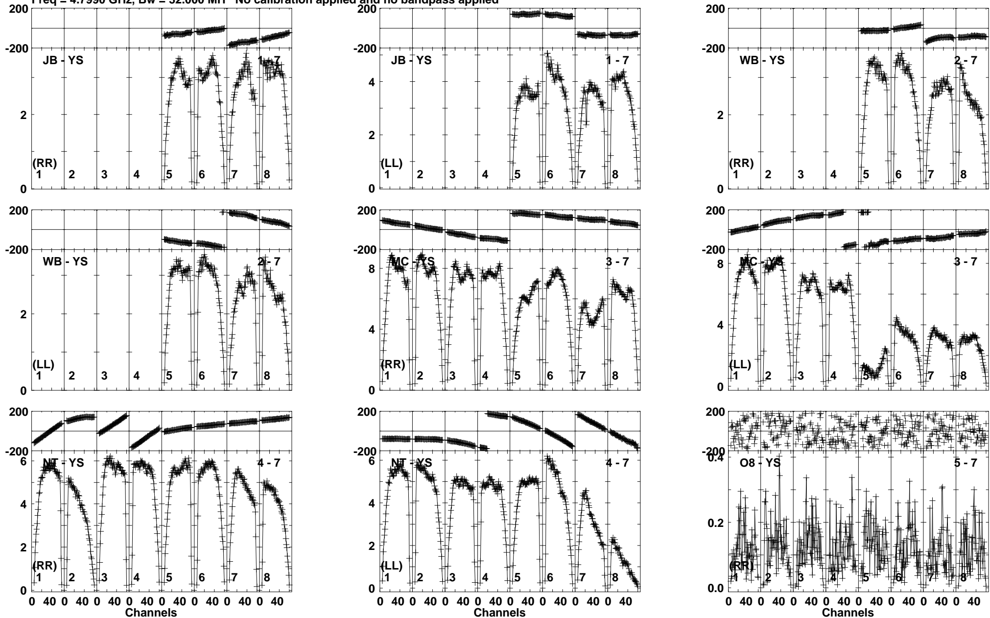
Lower frame: Milli Ampl Jy Top frame: Phas deg Vector averaged cross-power spectrum Baseline: JB (01) - YS (07) Timerange: 00/06:18:51 to 00/06:20:19
