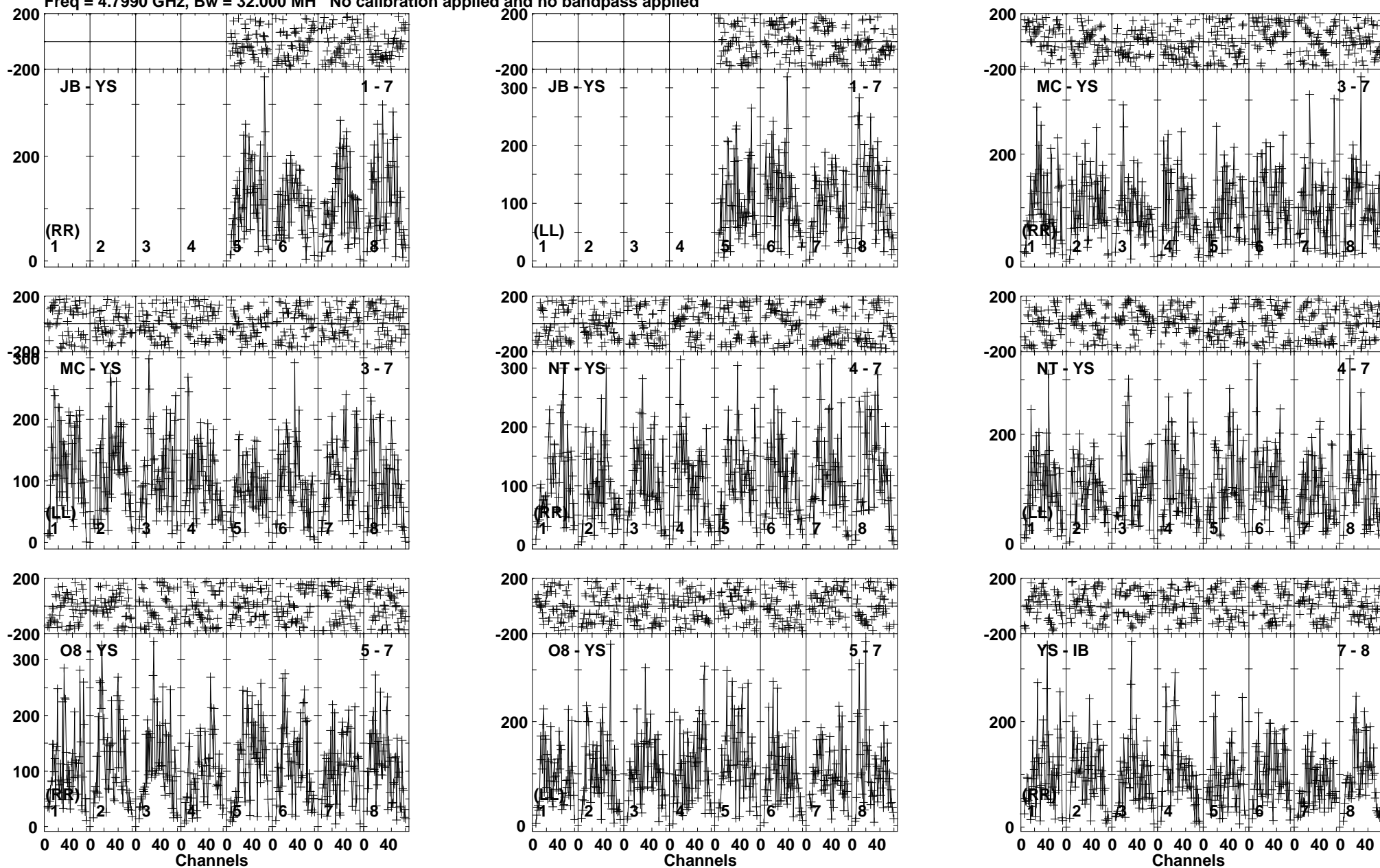
Lower frame: Micro Ampl Jy Top frame: Phas deg Vector averaged cross-power spectrum Baseline: JB (01) - YS (07) Timerange: 00/13:22:21 to 00/13:24:49
