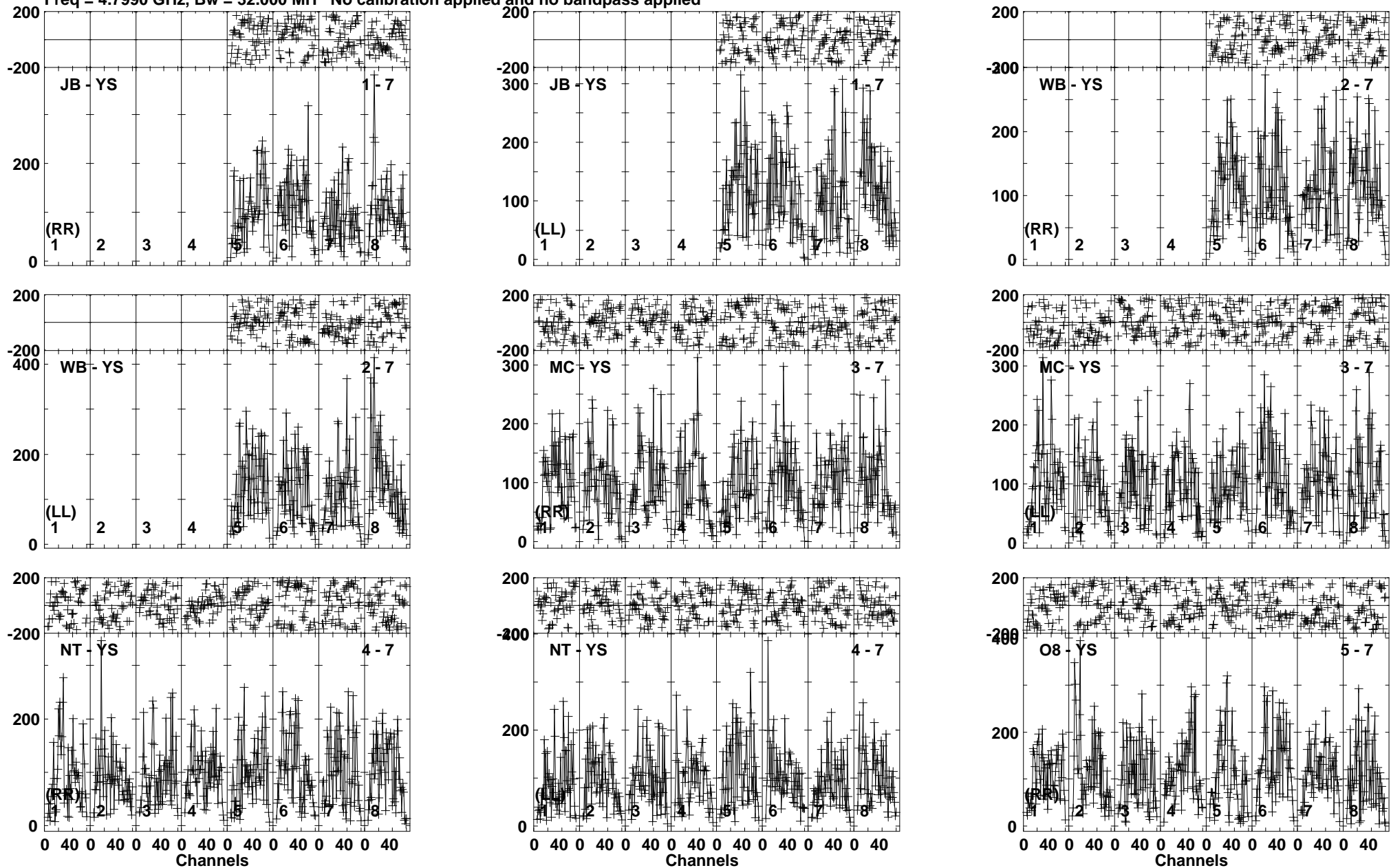
Lower frame: Micro Ampl Jy Top frame: Phas deg Vector averaged cross-power spectrum Baseline: JB (01) - YS (07) Timerange: 00:12:16:41 to 00:12:19:09
