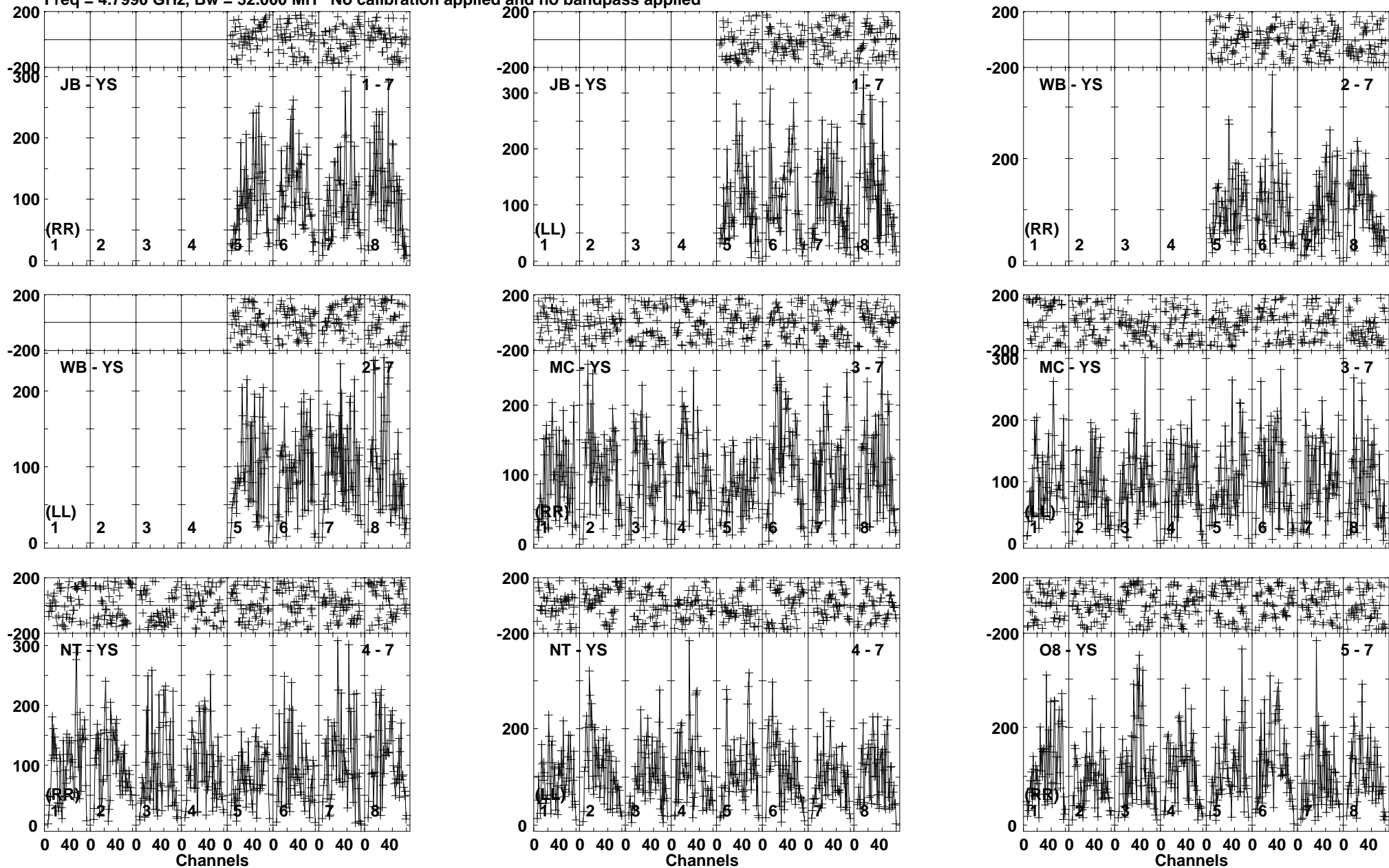
Lower frame: Micro Ampl Jy Top frame: Phas deg Vector averaged cross-power spectrum Baseline: JB (01) - YS (07) Timerange: 00/12:25:21 to 00/12:27:49
