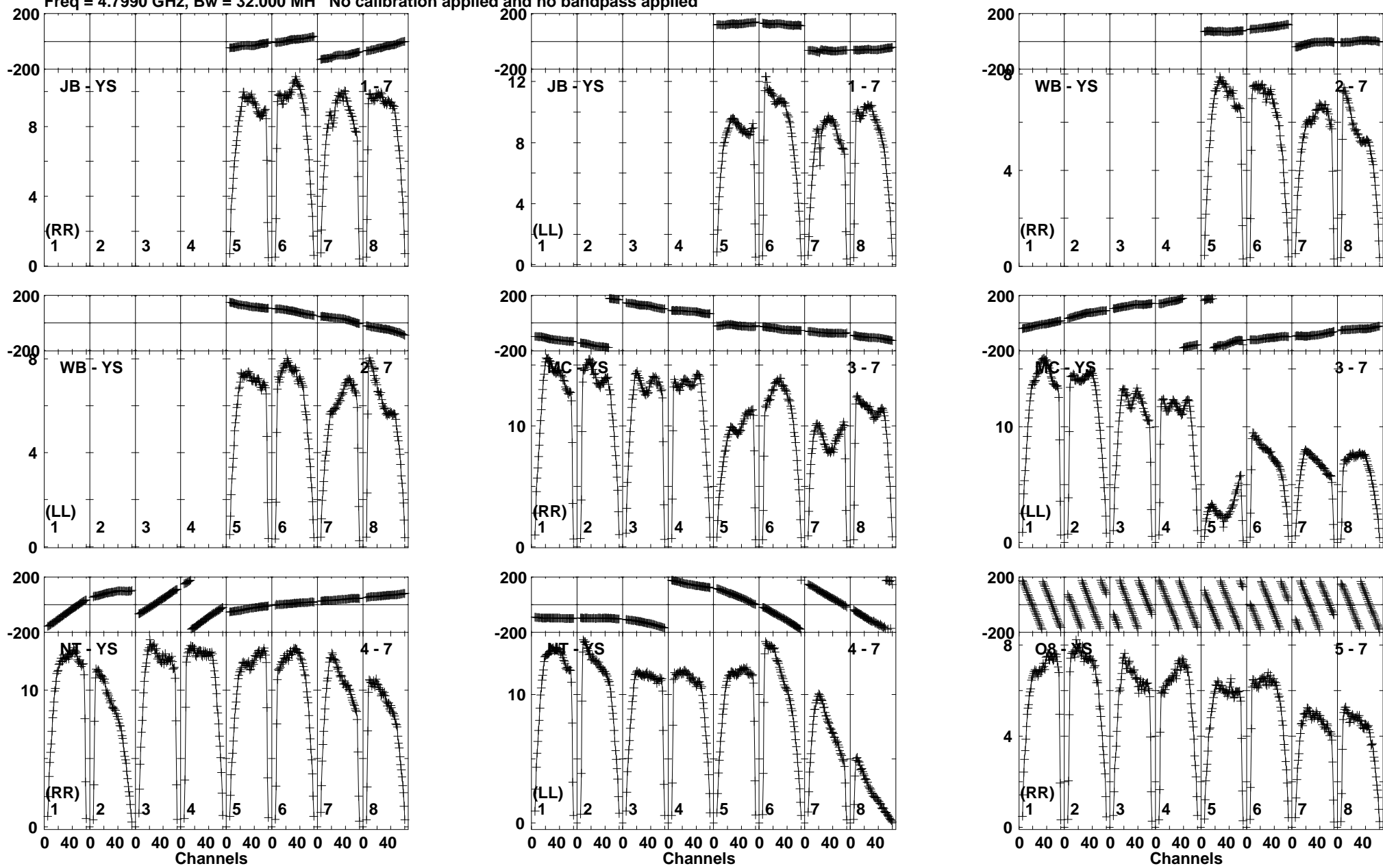
Lower frame: Milli Ampl Jy Top frame: Phas deg Vector averaged cross-power spectrum Baseline: JB (01) - YS (07) Timerange: 00/11:39:00 to 00/11:40:29
