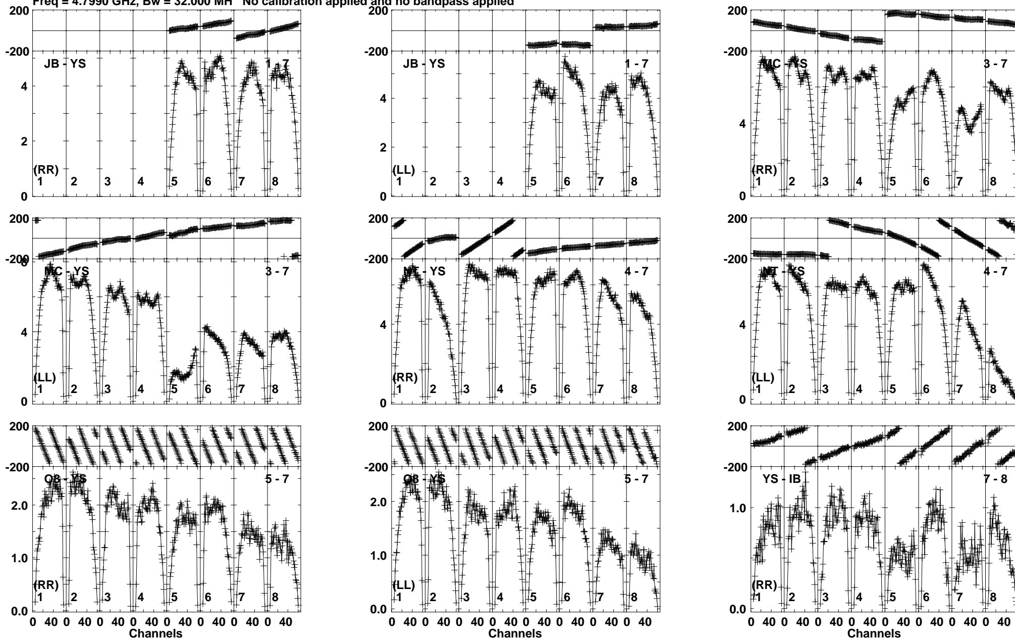
Lower frame: Milli Ampl Jy Top frame: Phas deg Vector averaged cross-power spectrum Baseline: JB (01) - YS (07) Timerange: 00/13:24:51 to 00/13:26:19
