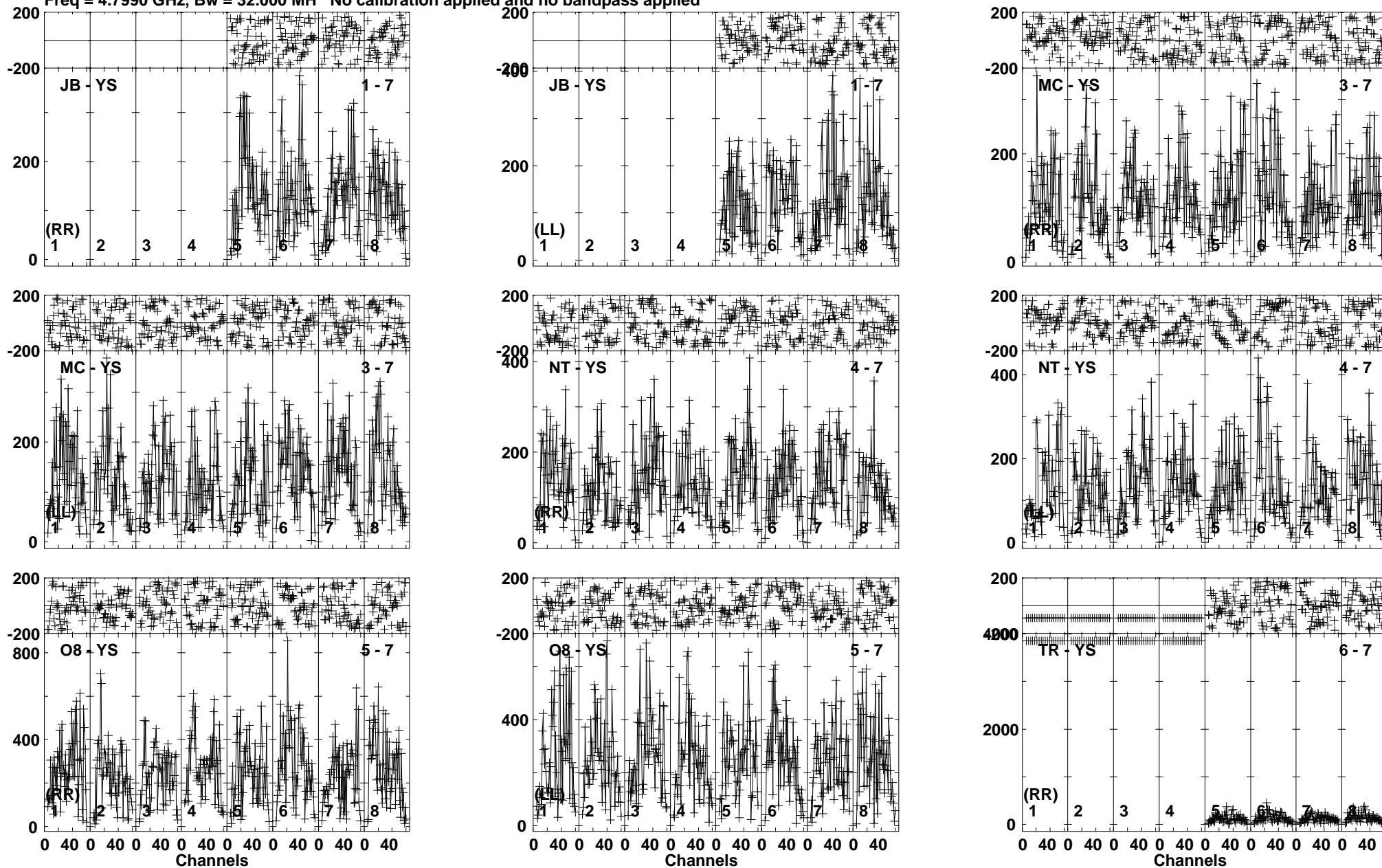
Lower frame: Micro Ampl Jy Top frame: Phas deg Vector averaged cross-power spectrum Baseline: JB (01) - YS (07) Timerange: 00/13:01:01 to 00/13:03:30
