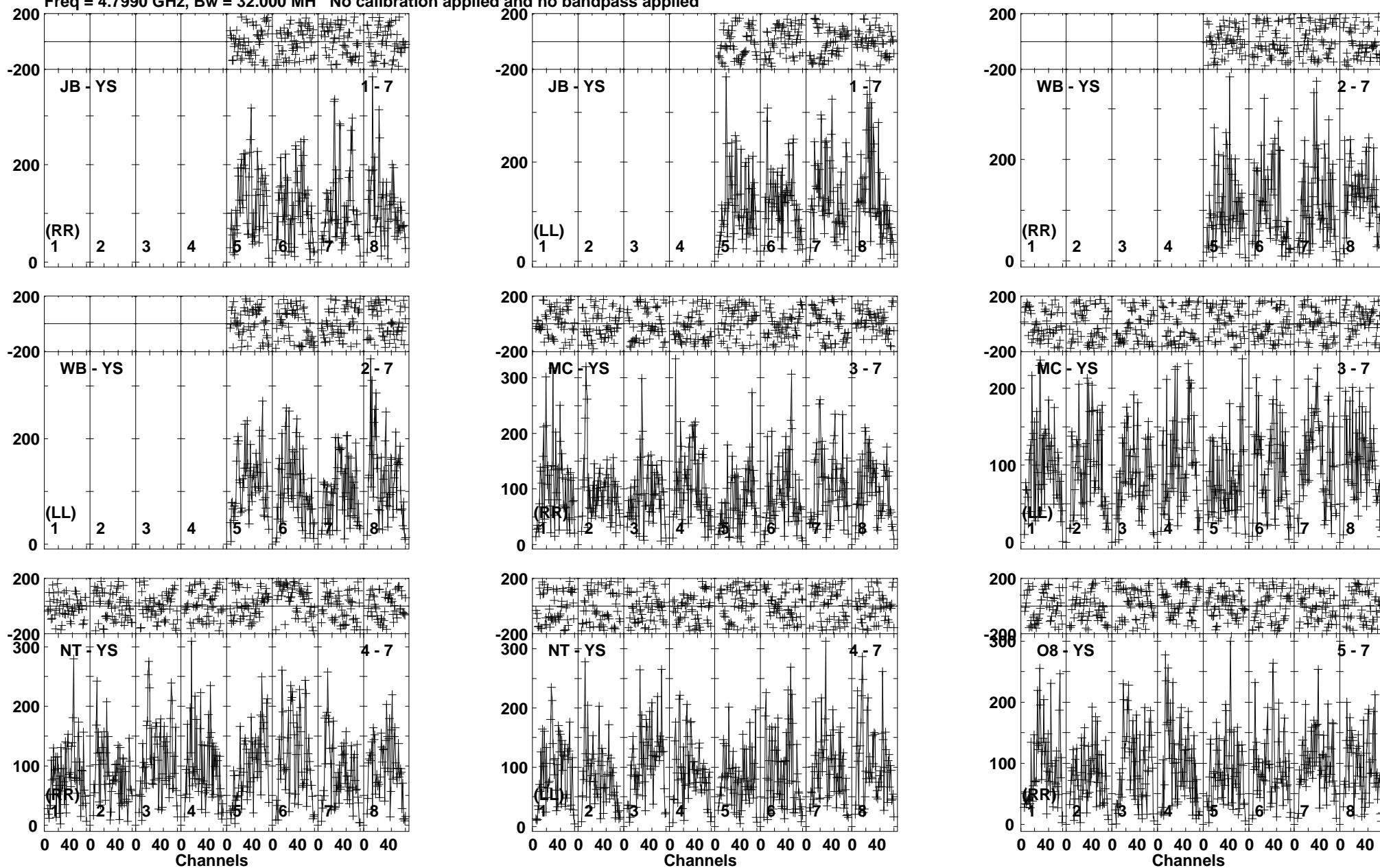
Lower frame: Micro Ampl Jy Top frame: Phas deg Vector averaged cross-power spectrum Baseline: JB (01) - YS (07) Timerange: 00/08:46:41 to 00/08:49:09
