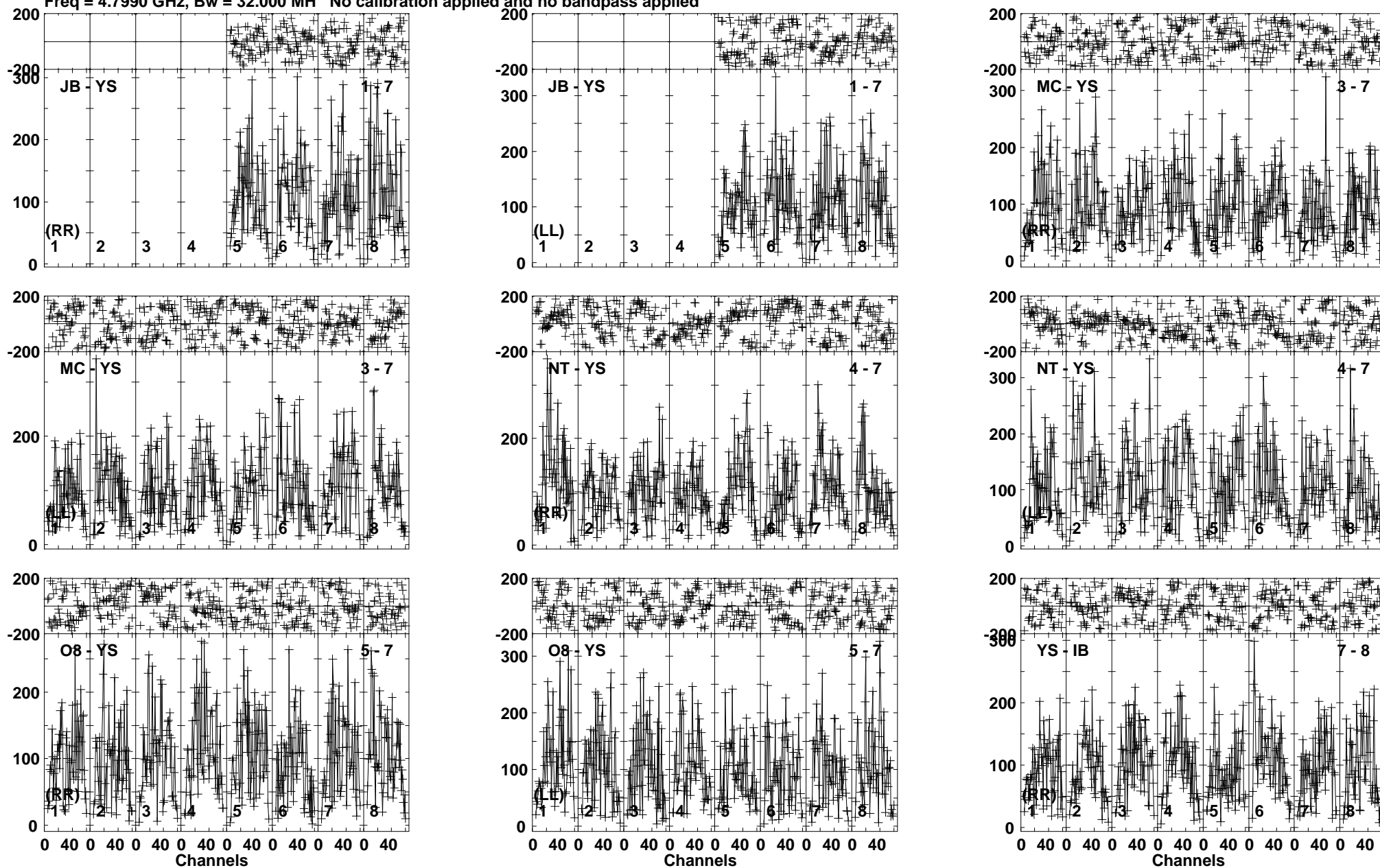
Lower frame: Micro Ampl Jy Top frame: Phas deg Vector averaged cross-power spectrum Baseline: JB (01) - YS (07) Timerange: 00/13:28:31 to 00/13:31:00
