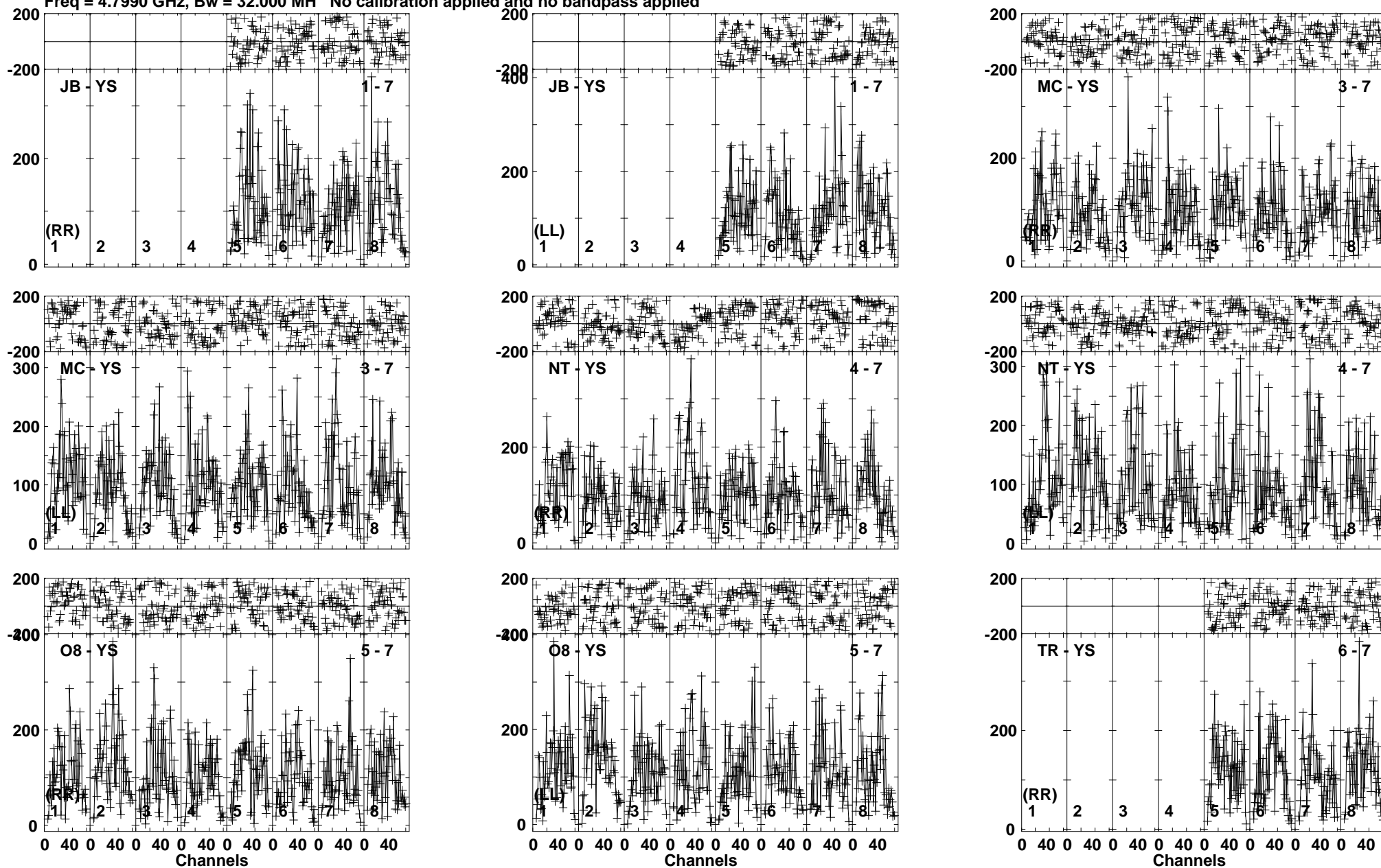
Lower frame: Micro Ampl Jy Top frame: Phas deg Vector averaged cross-power spectrum Baseline: JB (01) - YS (07) Timerange: 00/13:09:41 to 00/13:12:10
