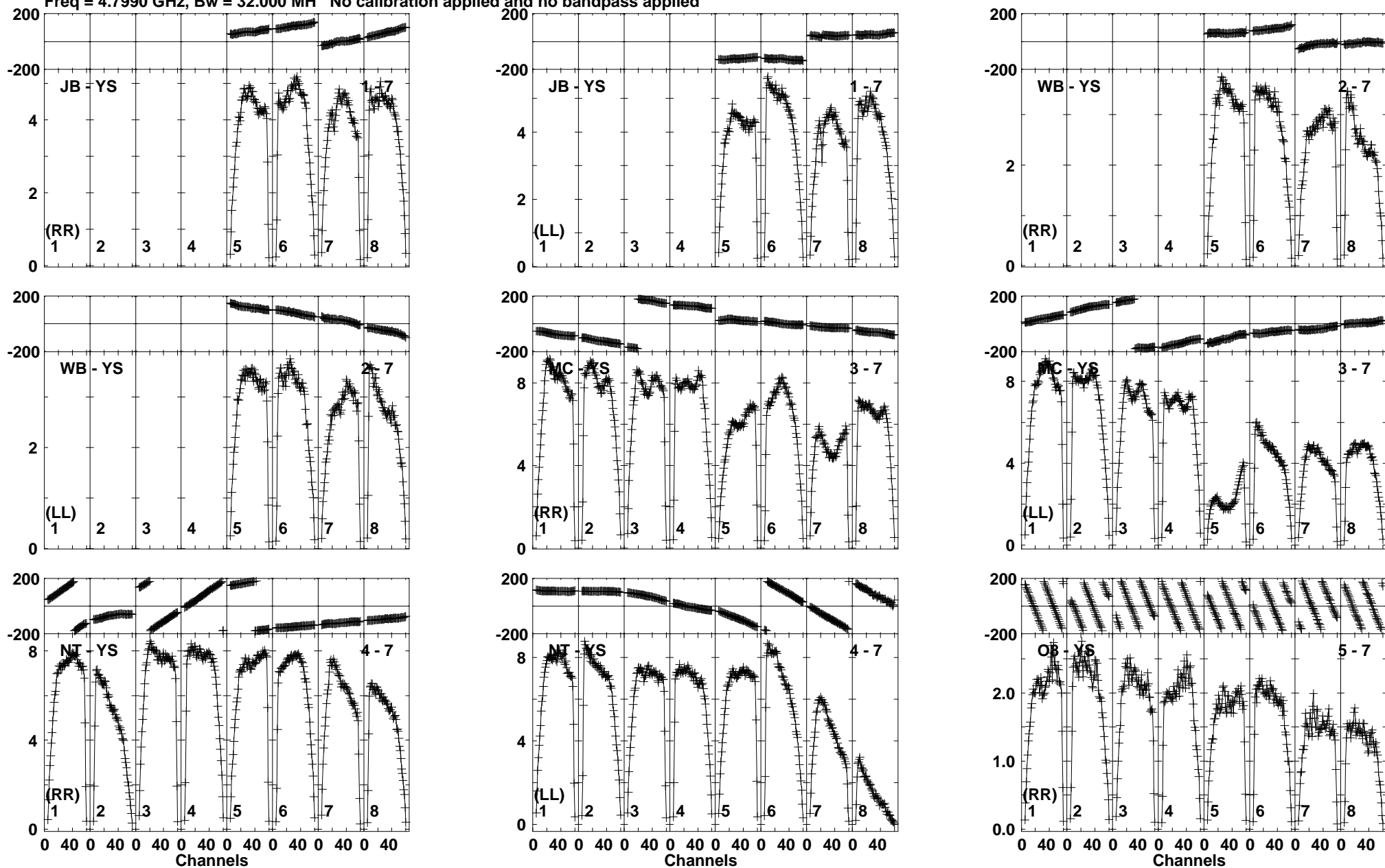
Lower frame: Milli Ampl Jy Top frame: Phas deg Vector averaged cross-power spectrum Baseline: JB (01) - YS (07) Timerange: 00/11:56:21 to 00/11:57:49
