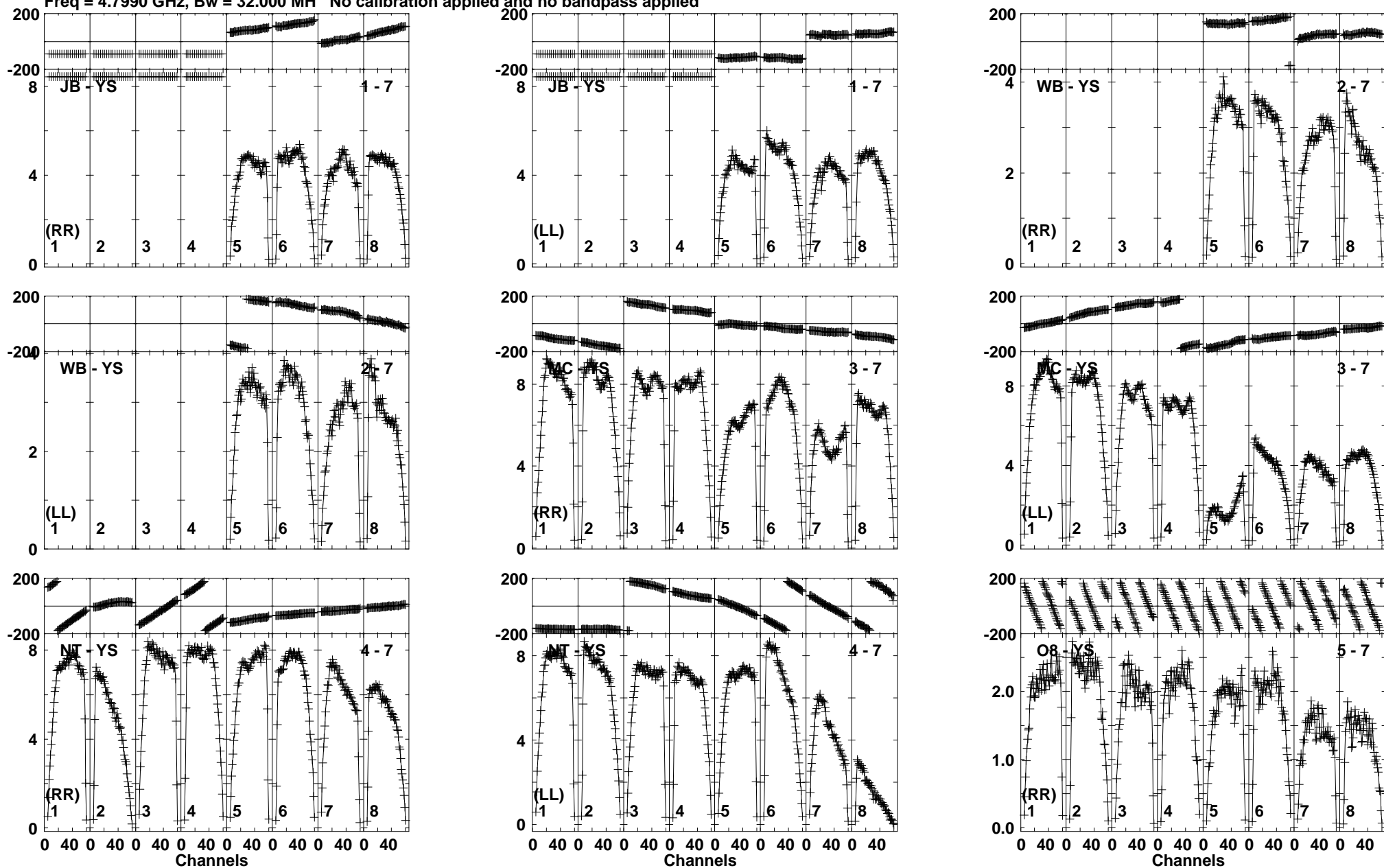
Lower frame: Milli Ampl Jy Top frame: Phas deg Vector averaged cross-power spectrum Baseline: JB (01) - YS (07) Timerange: 00/11:43:01 to 00/11:44:29
