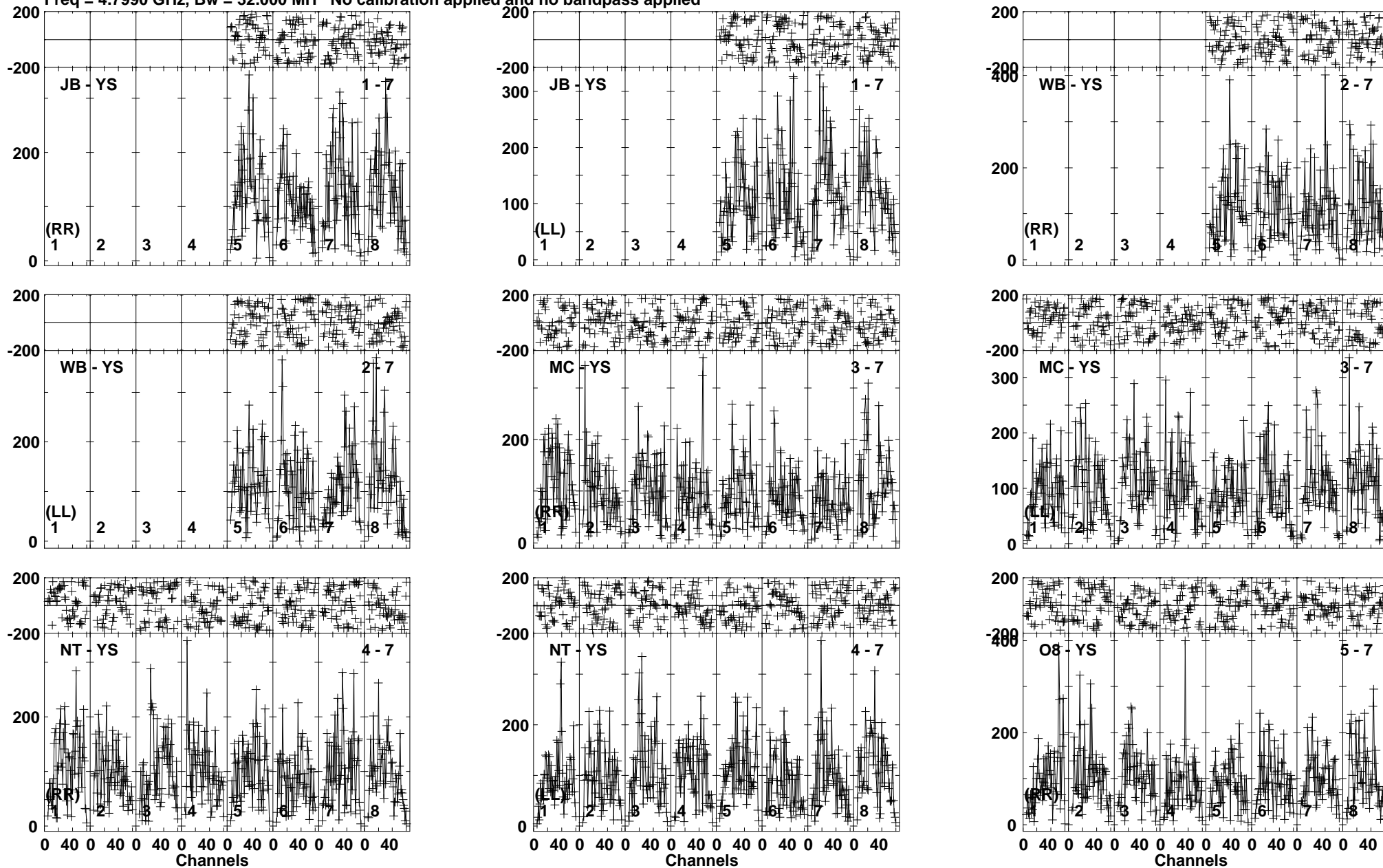
Lower frame: Micro Ampl Jy Top frame: Phas deg Vector averaged cross-power spectrum Baseline: JB (01) - YS (07) Timerange: 00/09:46:20 to 00/09:48:50
