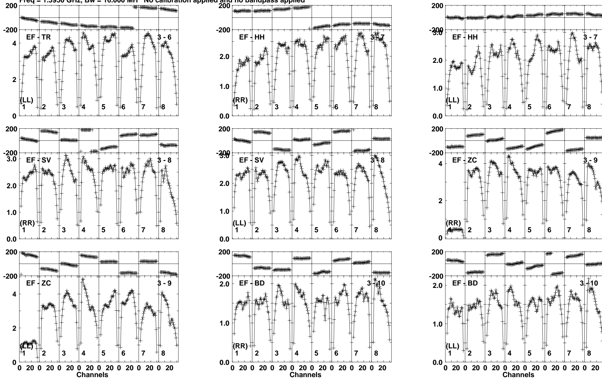
Lower frame: Milli Ampl Jy Top frame: Phas deg Vector averaged cross-power spectrum Baseline: EF (03) - TR (06) Timerange: 00/15:04:11 to 00/15:07:09
