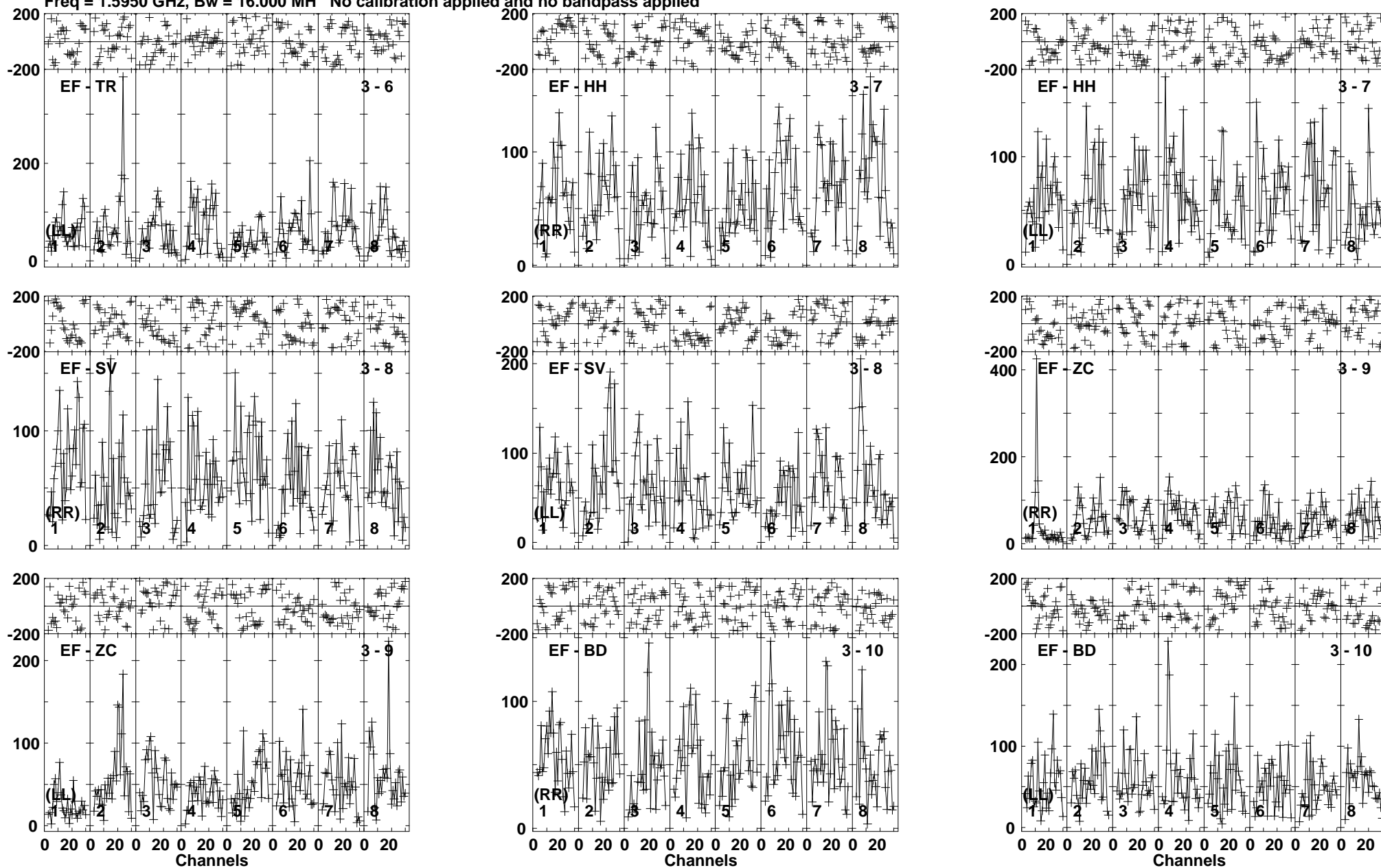
Lower frame: Micro Ampl Jy Top frame: Phas deg Vector averaged cross-power spectrum Baseline: EF (03) - TR (06) Timerange: 00/14:34:11 to 00/14:41:09
