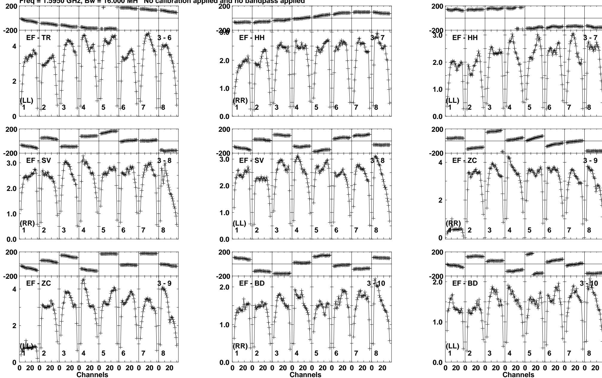
Lower frame: Milli Ampl Jy Top frame: Phas deg Vector averaged cross-power spectrum Baseline: EF (03) - TR (06) Timerange: 00/13:59:41 to 00/14:02:39
