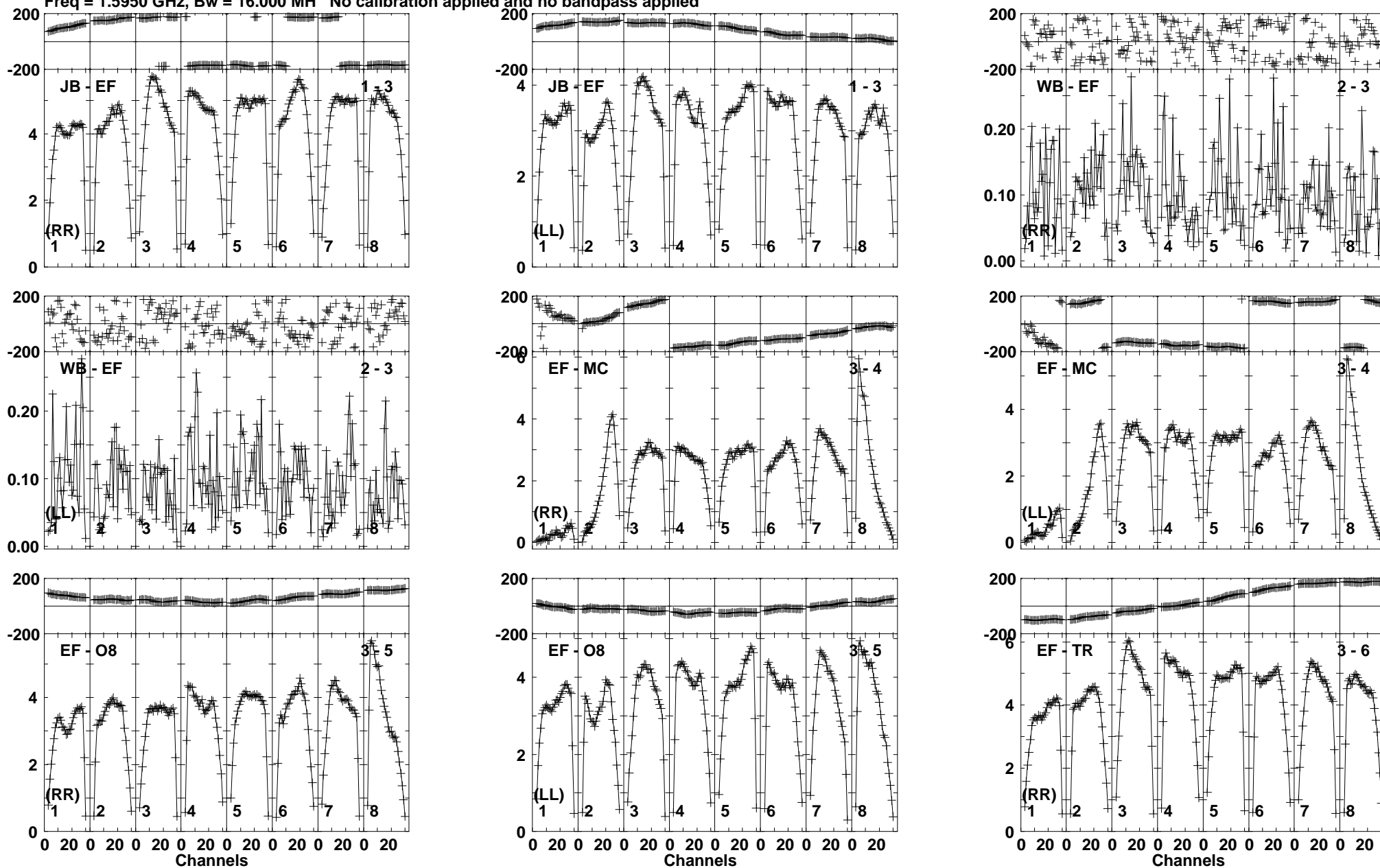
Lower frame: Milli Ampl Jy Top frame: Phas deg Vector averaged cross-power spectrum Baseline: JB (01) - EF (03) Timerange: 00/13:07:11 to 00/13:10:09
