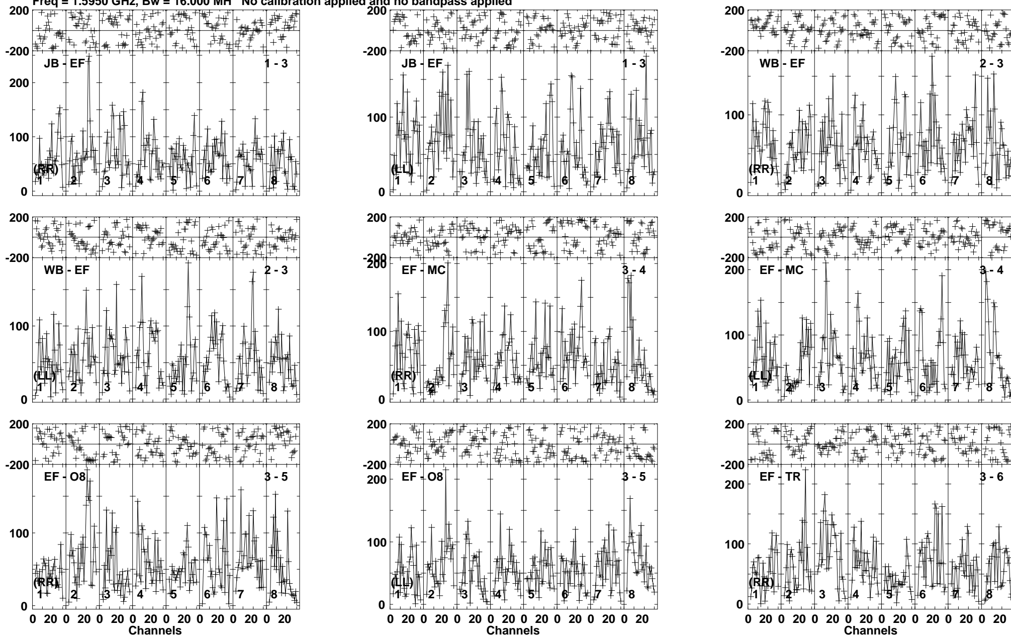
Lower frame: Micro Ampl Jy Top frame: Phas deg Vector averaged cross-power spectrum Baseline: JB (01) - EF (03) Timerange: 00/14:34:11 to 00/14:41:09
