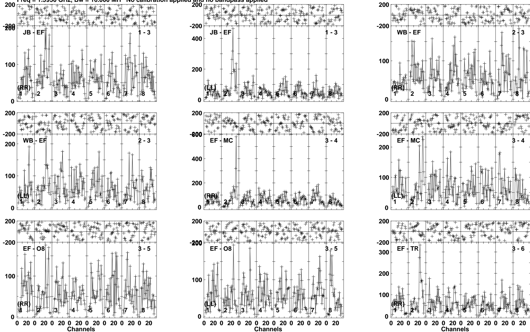
Lower frame: Micro Ampl Jy Top frame: Phas deg Vector averaged cross-power spectrum Baseline: JB (01) - EF (03) Timerange: 00/14:02:41 to 00/14:09:39
