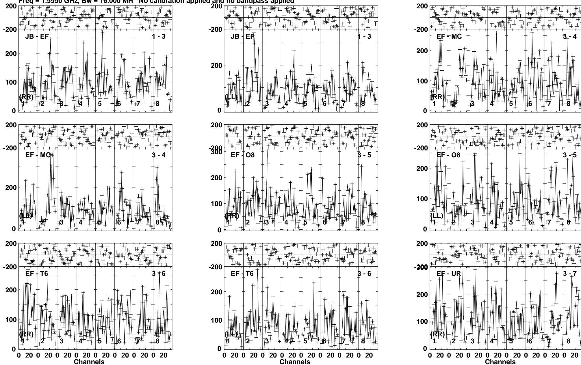
Lower frame: Micro Ampl Jy Top frame: Phas deg Vector averaged cross-power spectrum Baseline: JB (01) - EF (03) Timerange: 00/02:12:01 to 00/02:15:29
