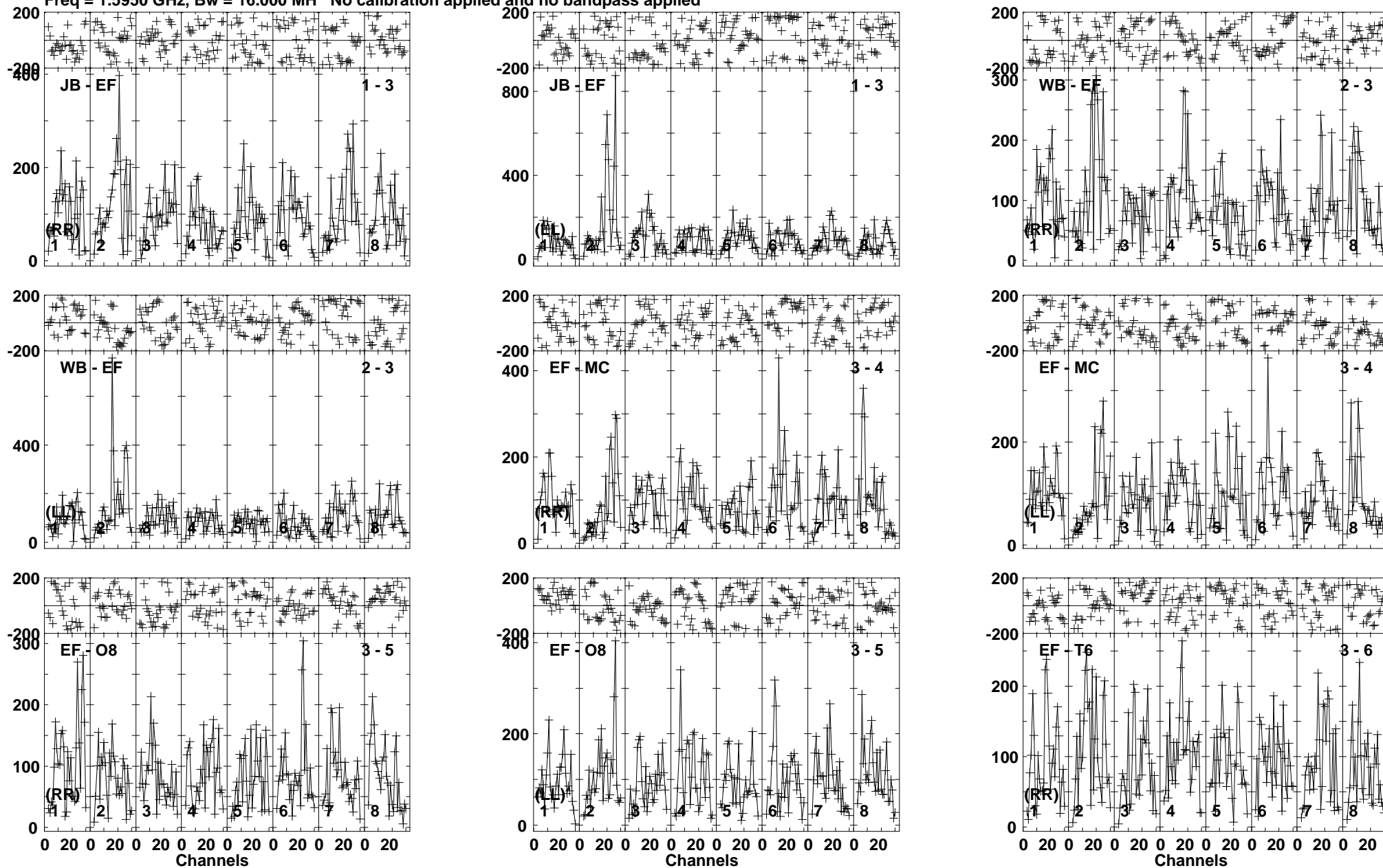
Lower frame: Micro Ampl Jy Top frame: Phas deg Vector averaged cross-power spectrum Baseline: JB (01) - EF (03) Timerange: 00/03:11:21 to 00/03:14:49
