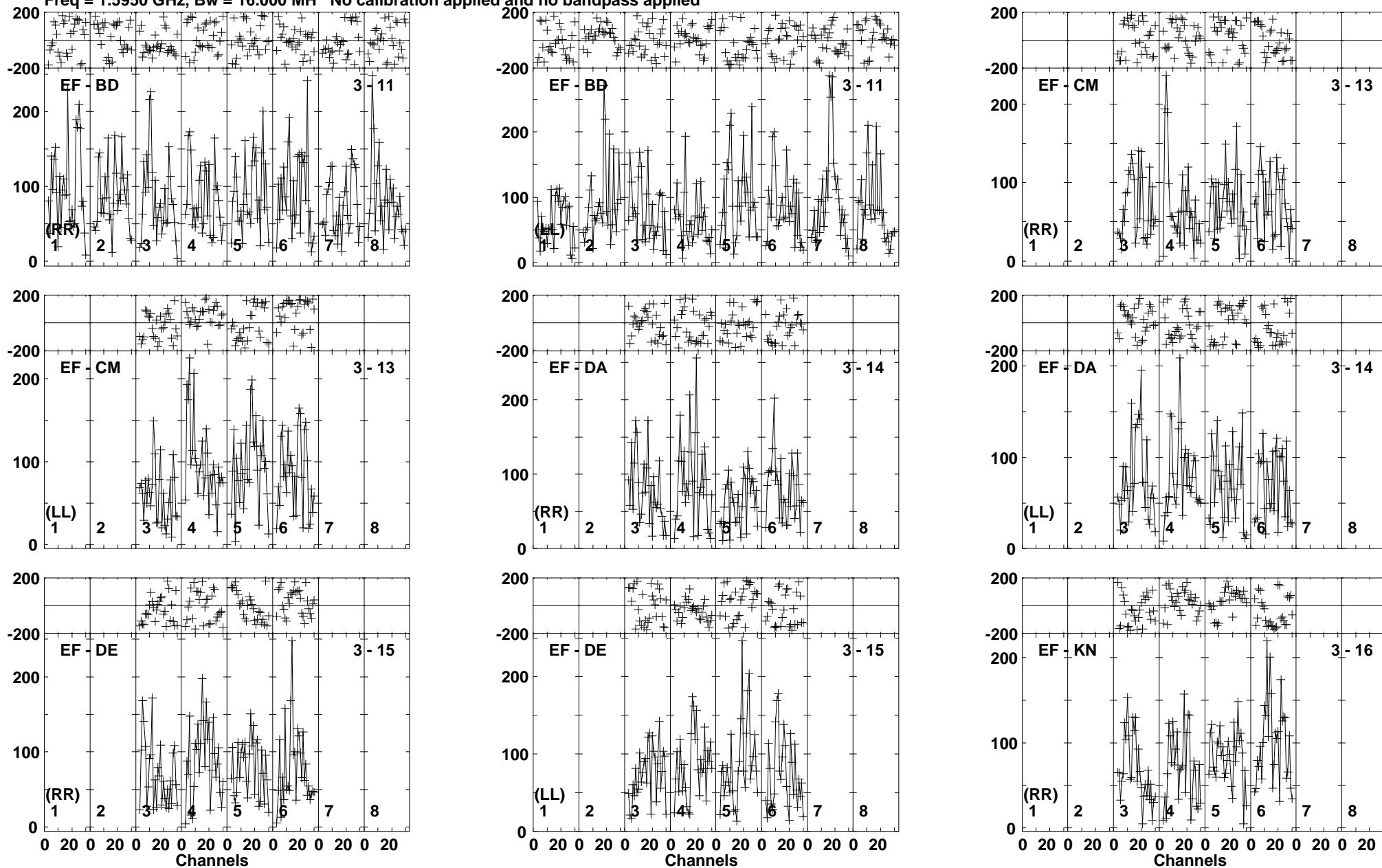
Lower frame: Micro Ampl Jy Top frame: Phas deg Vector averaged cross-power spectrum Baseline: EF (03) - BD (11) Timerange: 00/02:49:01 to 00/02:52:29
