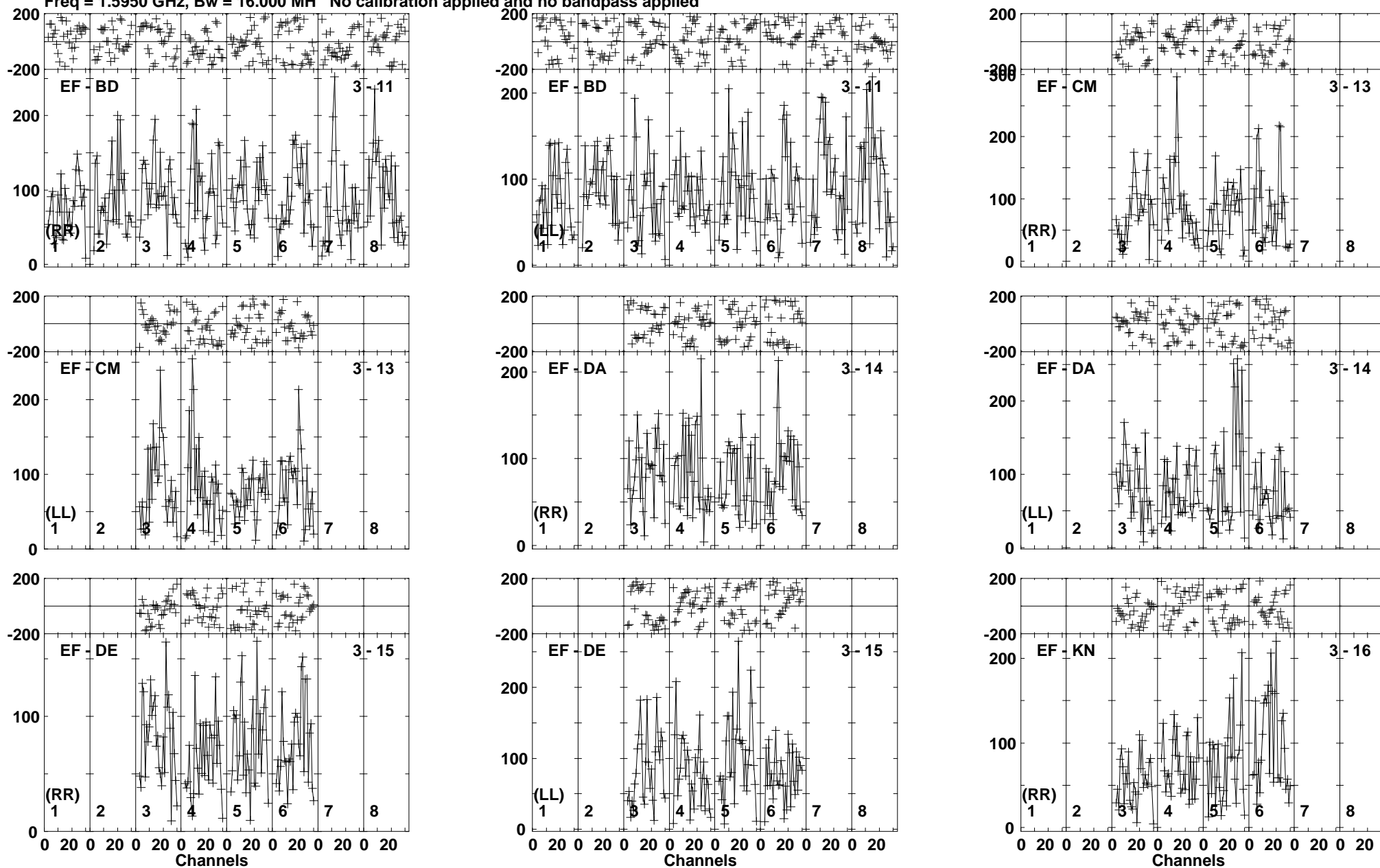
Lower frame: Micro Ampl Jy Top frame: Phas deg Vector averaged cross-power spectrum Baseline: EF (03) - BD (11) Timerange: 00/02:27:41 to 00/02:31:09
