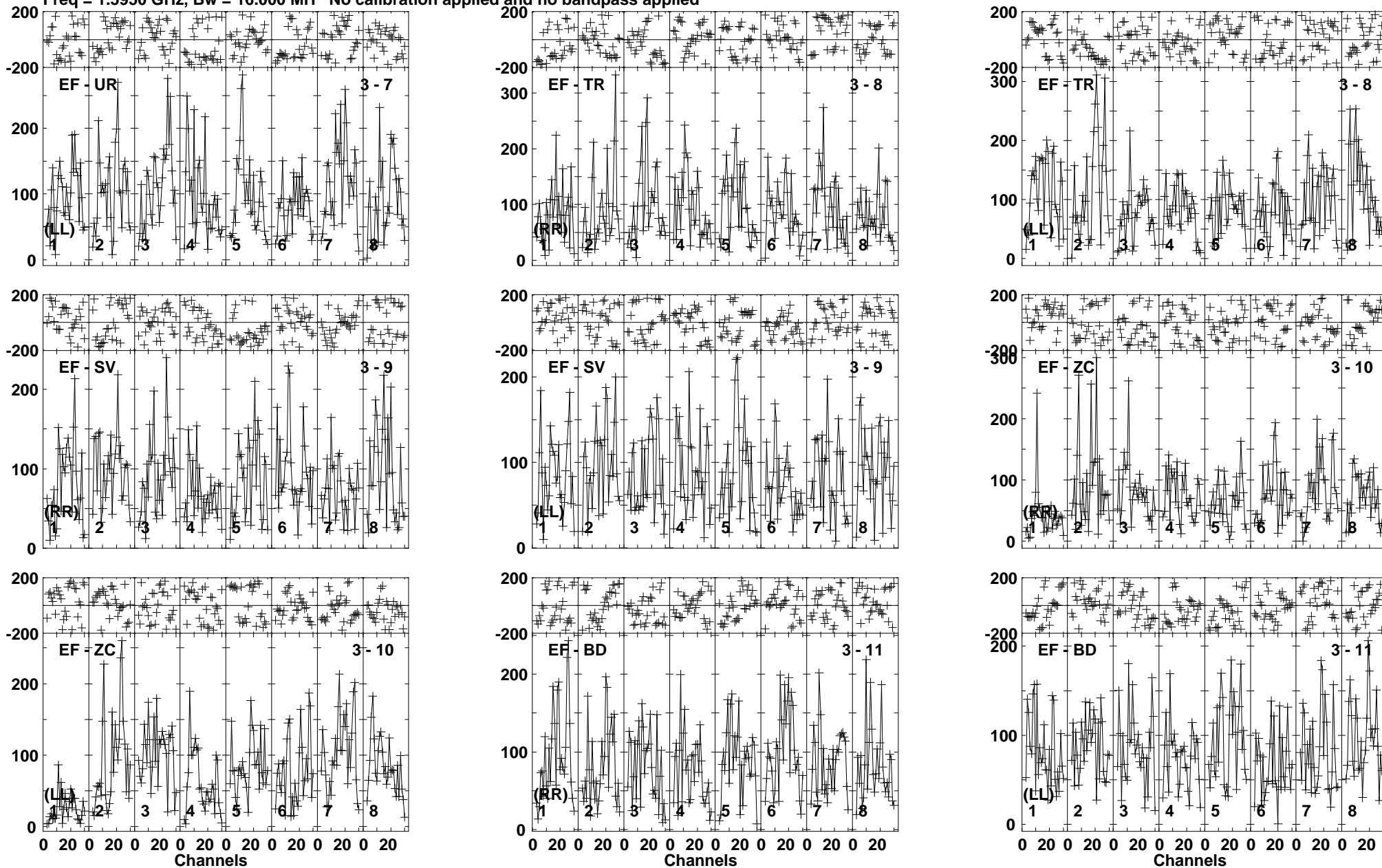
Lower frame: Micro Ampl Jy Top frame: Phas deg Vector averaged cross-power spectrum Baseline: EF (03) - UR (07) Timerange: 00/02:01:21 to 00/02:04:49
