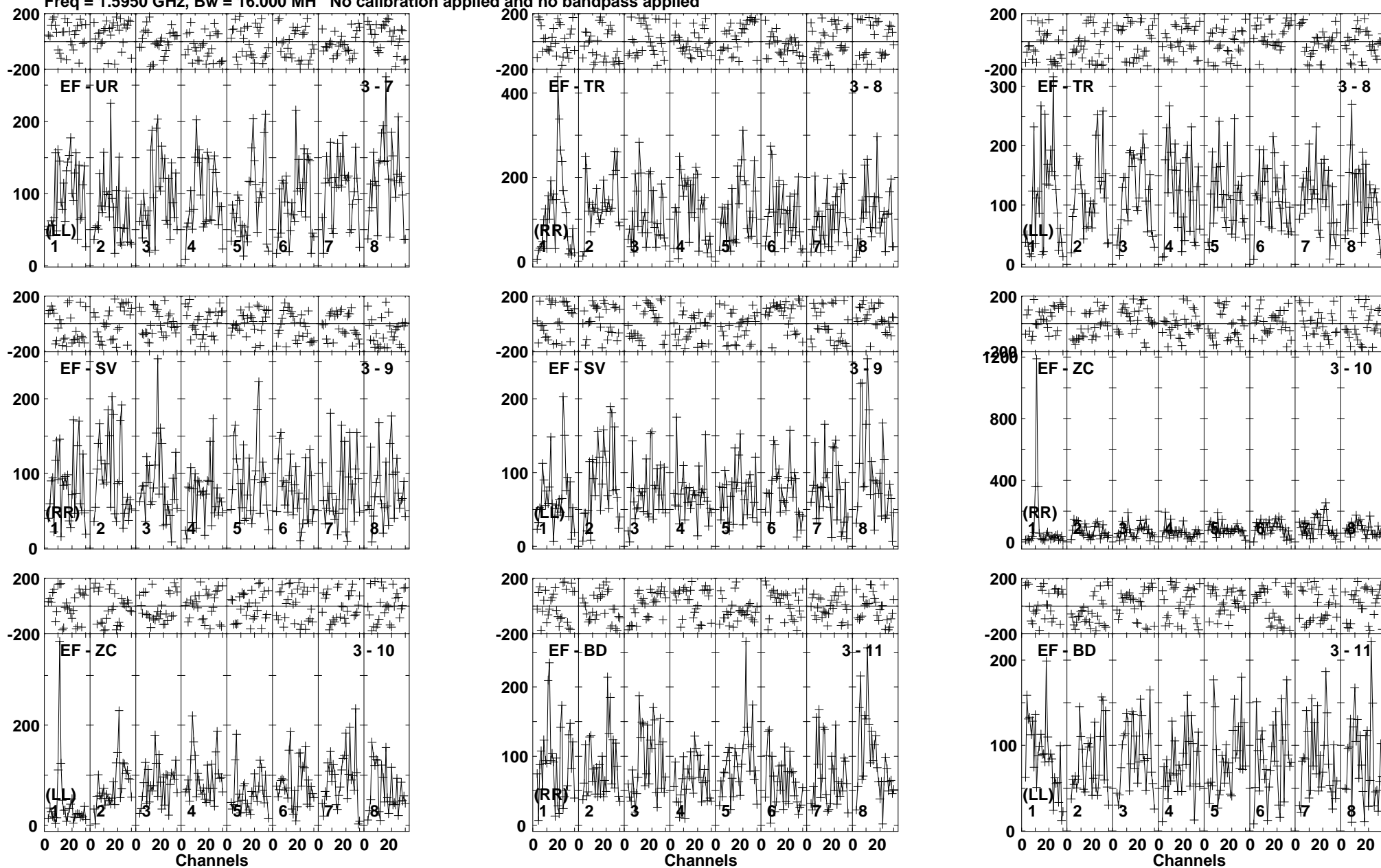
Lower frame: Micro Ampl Jy Top frame: Phas deg Vector averaged cross-power spectrum Baseline: EF (03) - UR (07) Timerange: 00/01:23:41 to 00/01:27:09
