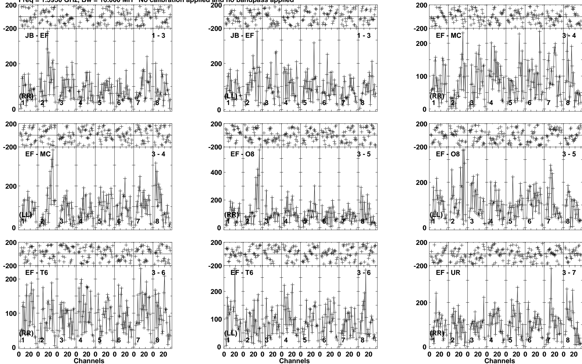
Lower frame: Micro Ampl Jy Top frame: Phas deg Vector averaged cross-power spectrum Baseline: JB (01) - EF (03) Timerange: 00/01:23:41 to 00/01:27:09
