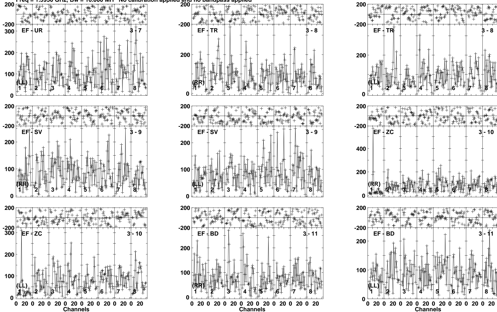
Lower frame: Micro Ampl Jy Top frame: Phas deg Vector averaged cross-power spectrum Baseline: EF (03) - UR (07) Timerange: 00/02:12:01 to 00/02:15:29
