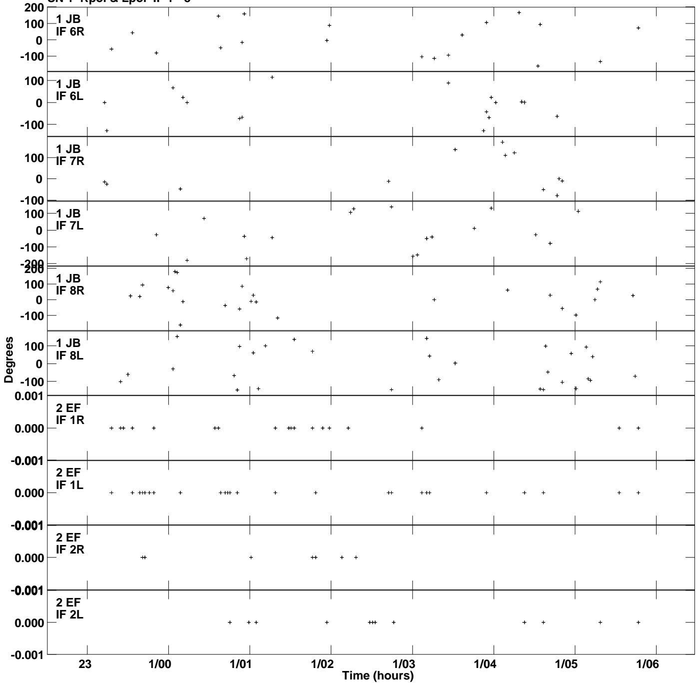
Plot file version 2 created 11-JUL-2019 09:30:03 Gain phs vs UTC time for J1134+7249.MULTI.1 SN 1 Rpol & Lpol IF 1 - 8
