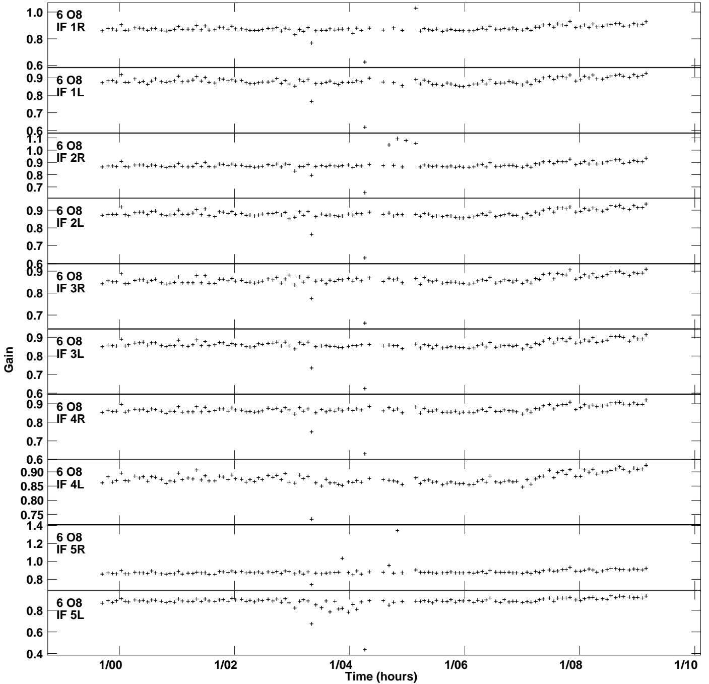
Plot file version 8 created 23-MAY-2019 14:34:38 Gain amp vs UTC time for J2007+4029.MULTI.1 SN 2 Rpol & Lpol IF 1 - 8
