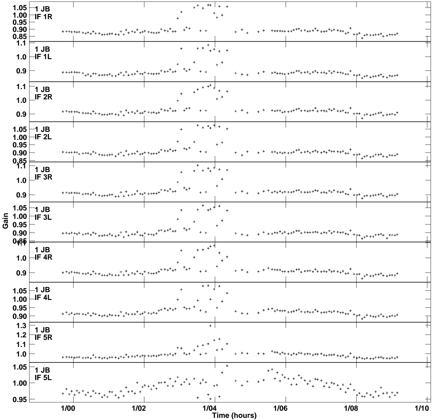
Plot file version 1 created 23-MAY-2019 14:34:38 Gain amp vs UTC time for J2007+4029.MULTI.1 SN 2 Rpol & Lpol IF 1 - 8
