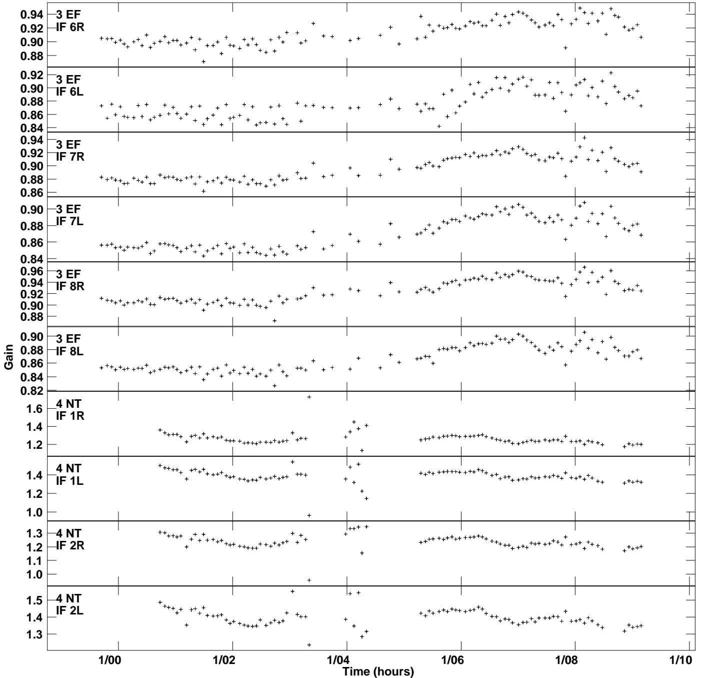
Plot file version 5 created 23-MAY-2019 14:34:38 Gain amp vs UTC time for J2007+4029.MULTI.1 SN 2 Rpol & Lpol IF 1 - 8
