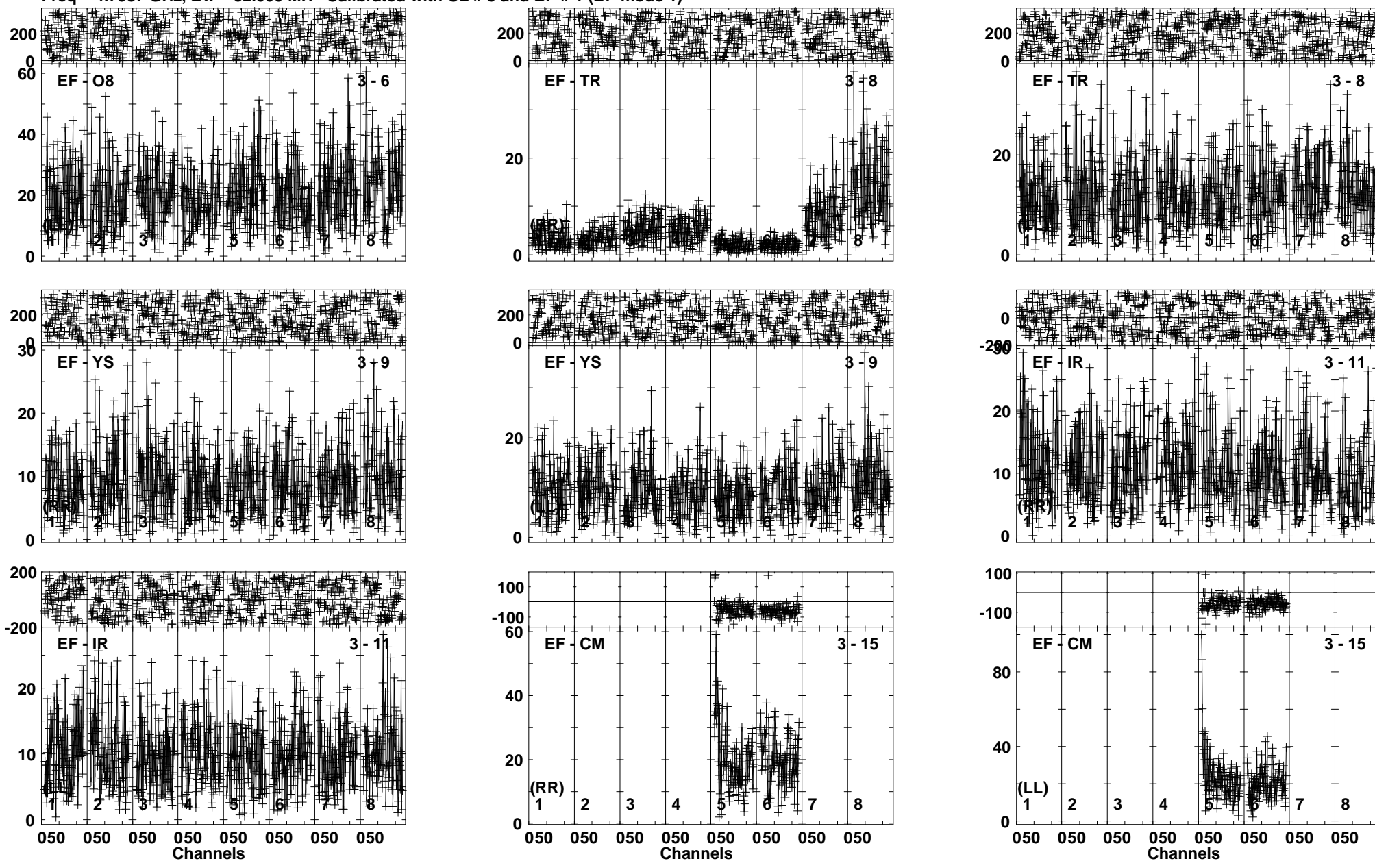
Lower frame: Milli Ampl Jy Top frame: Phas deg Vector averaged cross-power spectrum Baseline: EF (03) - O8 (06) Timerange: 01/06:50:50 to 01/06:53:20
