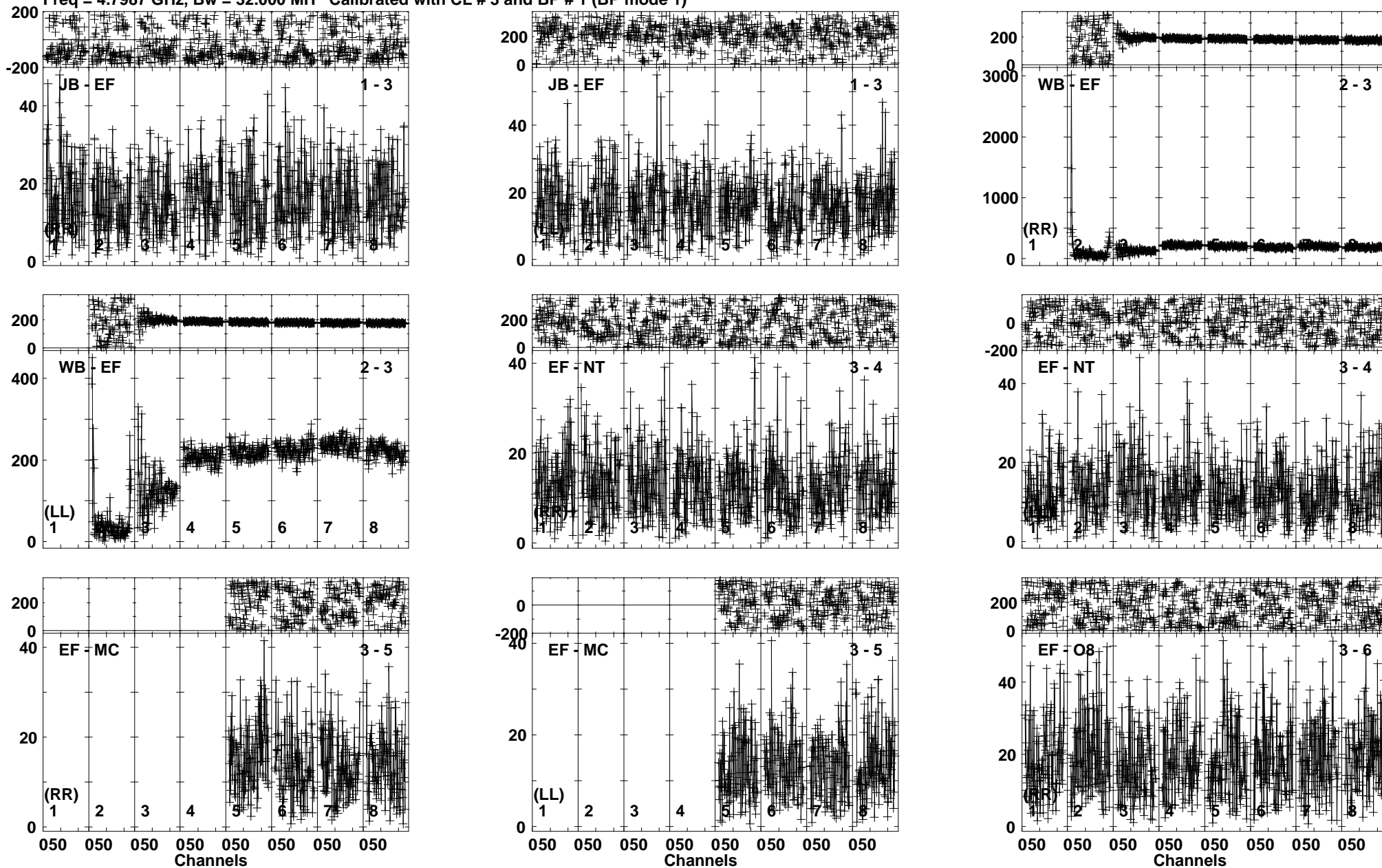
Lower frame: Milli Ampl Jy Top frame: Phas deg Vector averaged cross-power spectrum Baseline: JB (01) - EF (03) Timerange: 01/05:51:11 to 01/05:53:39
