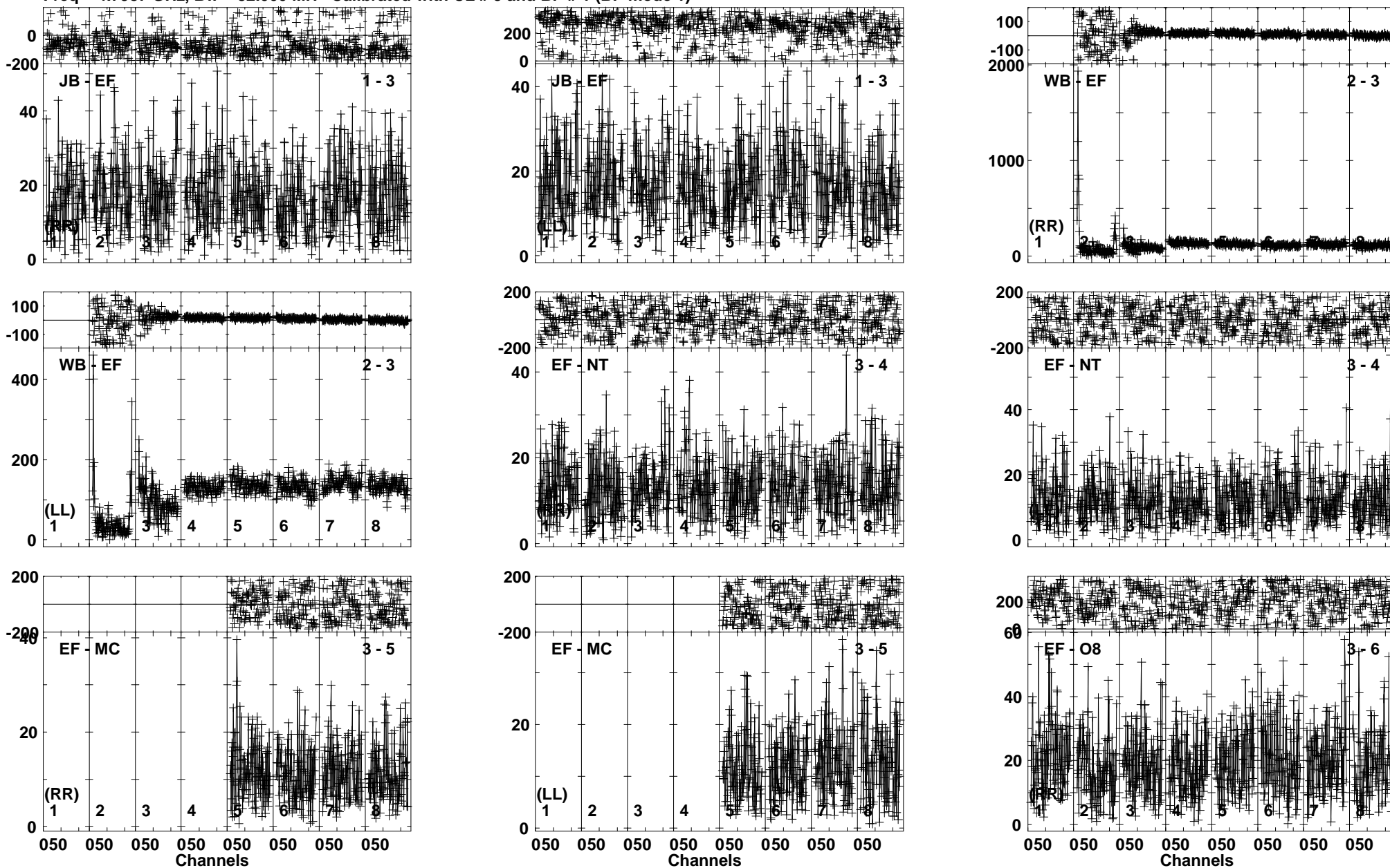
Lower frame: Milli Ampl Jy Top frame: Phas deg Vector averaged cross-power spectrum Baseline: JB (01) - EF (03) Timerange: 01/02:49:31 to 01/02:51:59
