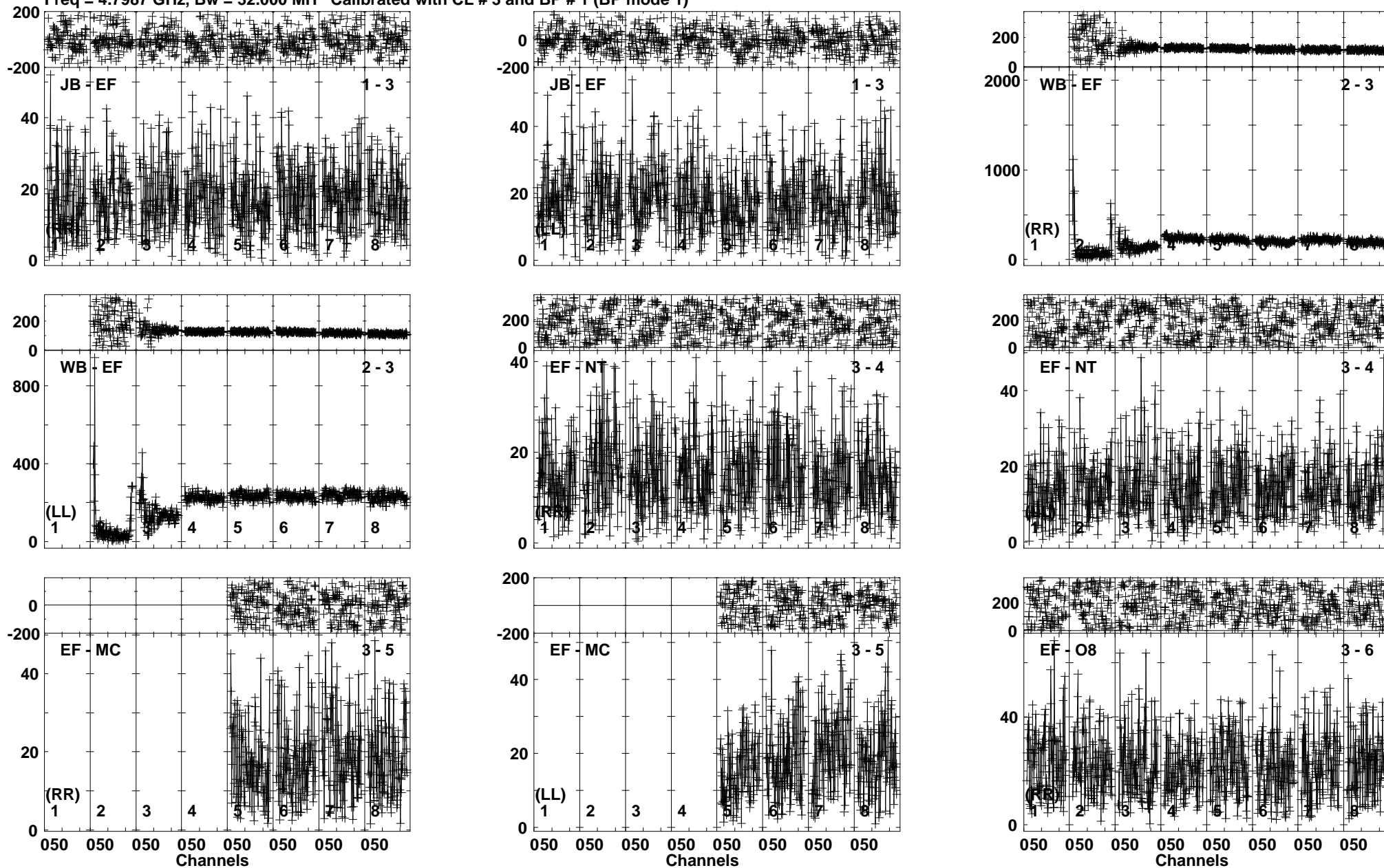
Lower frame: Milli Ampl Jy Top frame: Phas deg Vector averaged cross-power spectrum Baseline: JB (01) - EF (03) Timerange: 01/05:18:31 to 01/05:21:00
