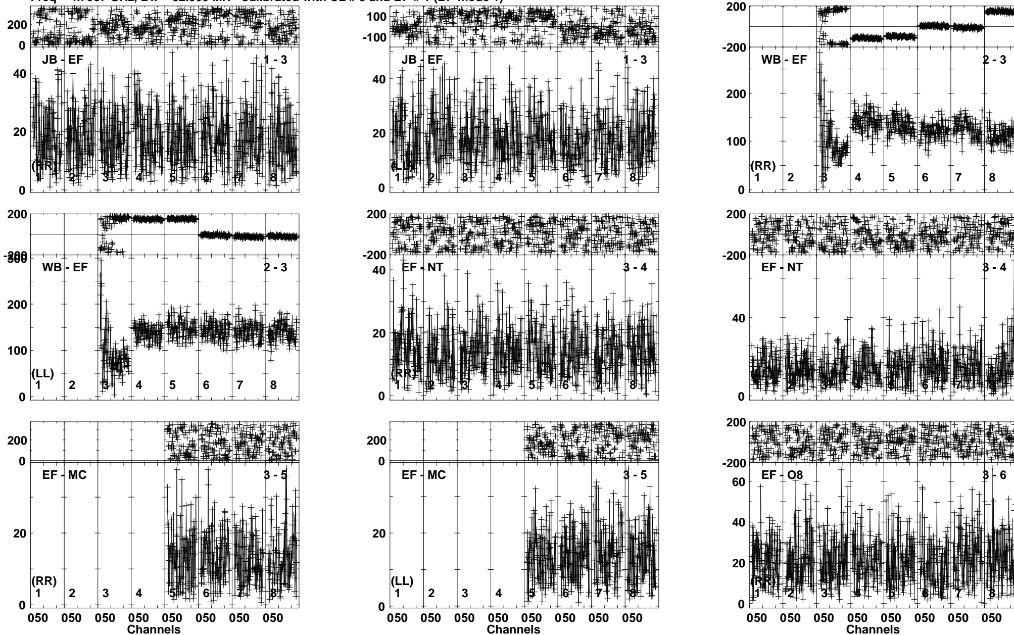
Lower frame: Milli Ampl Jy Top frame: Phas deg Vector averaged cross-power spectrum Baseline: JB (01) - EF (03) Timerange: 01/02:59:41 to 01/03:02:09
