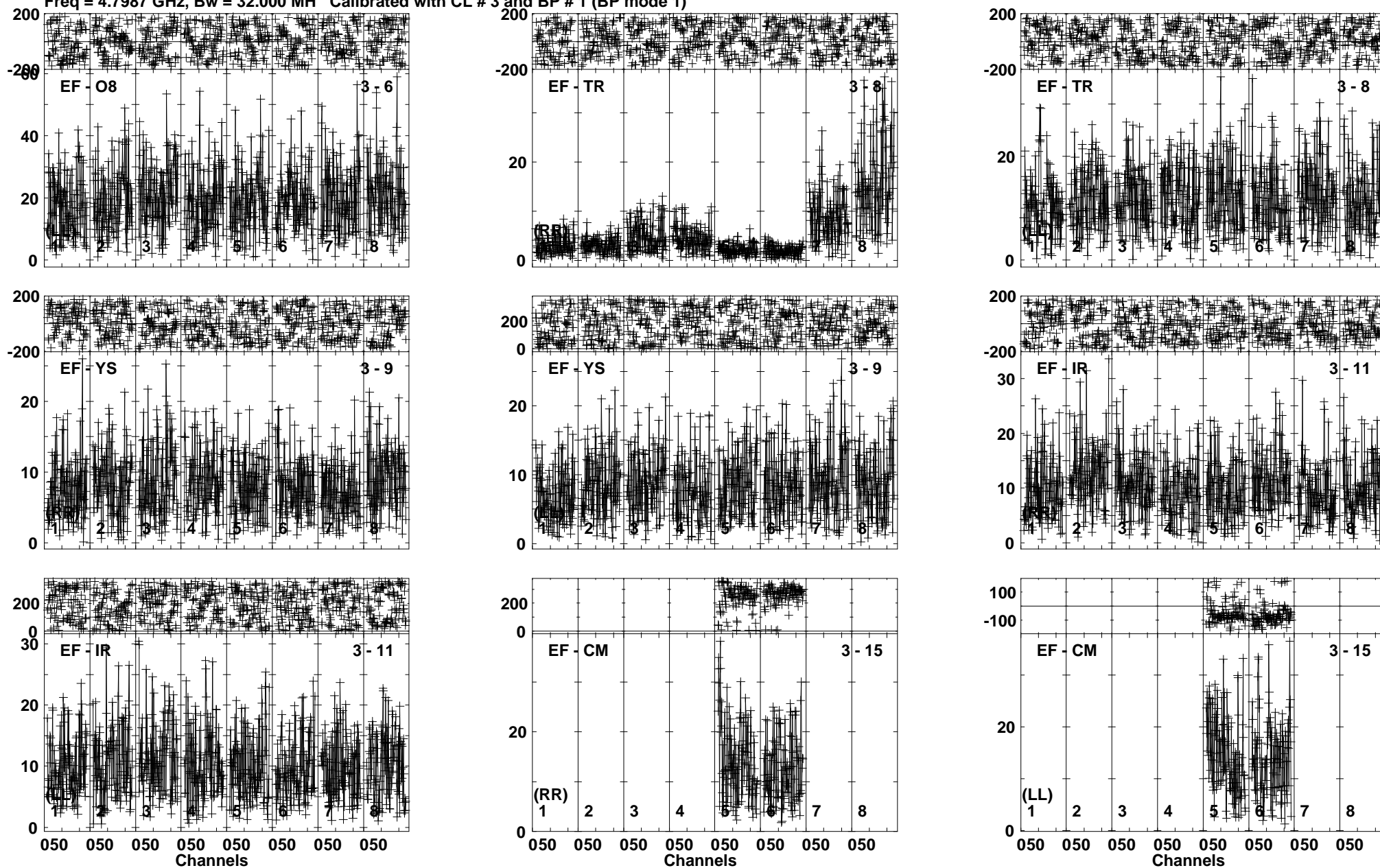
Lower frame: Milli Ampl Jy Top frame: Phas deg Vector averaged cross-power spectrum Baseline: EF (03) - O8 (06) Timerange: 01/07:56:40 to 01/07:59:10
