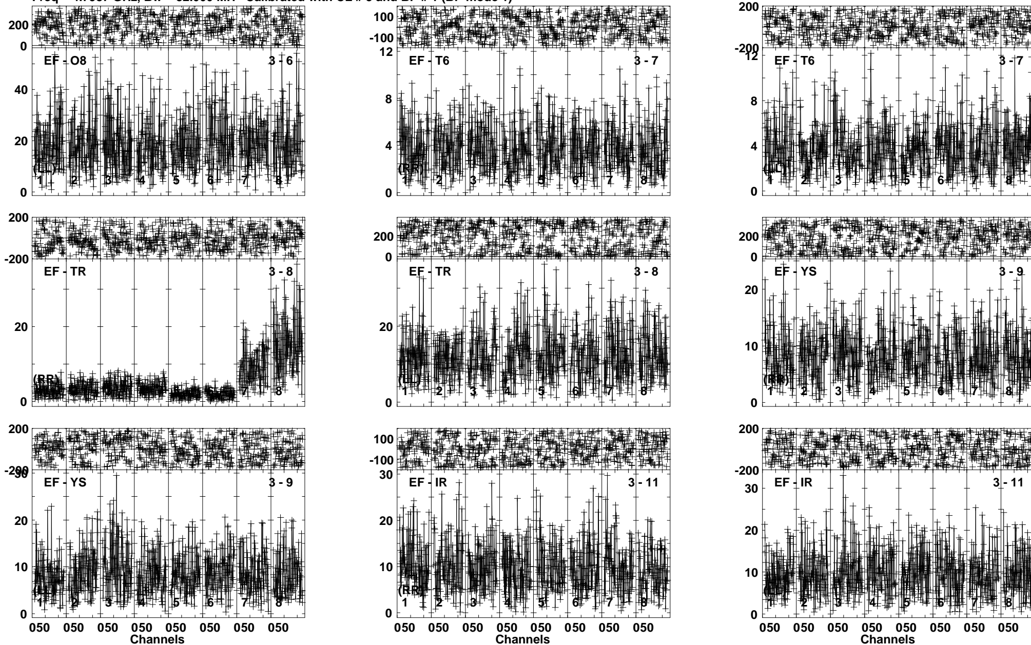
Lower frame: Milli Ampl Jy Top frame: Phas deg Vector averaged cross-power spectrum Baseline: EF (03) - O8 (06) Timerange: 01/01:53:51 to 01/01:56:19
