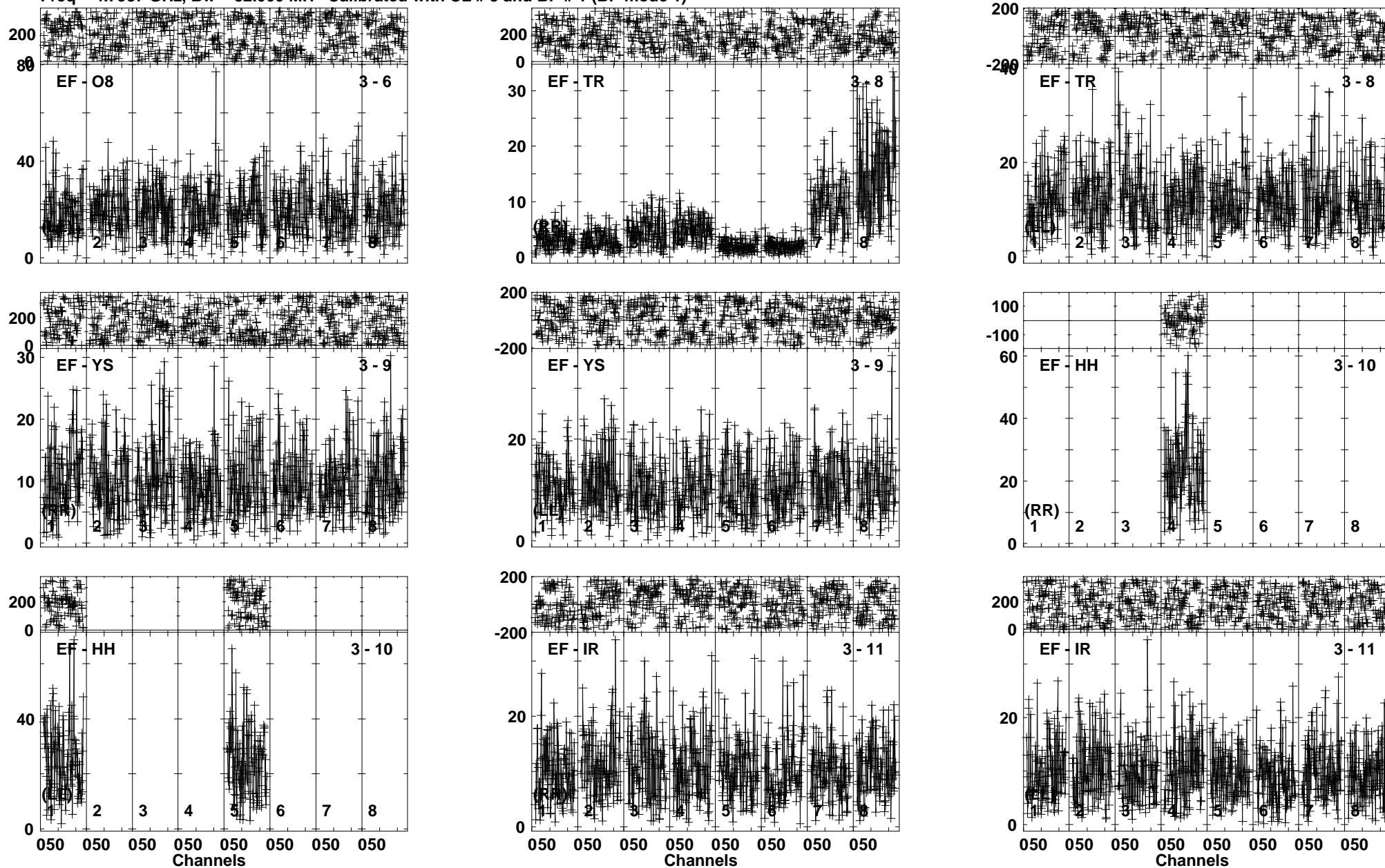
Lower frame: Milli Ampl Jy Top frame: Phas deg Vector averaged cross-power spectrum Baseline: EF (03) - O8 (06) Timerange: 01/05:46:20 to 01/05:48:50
