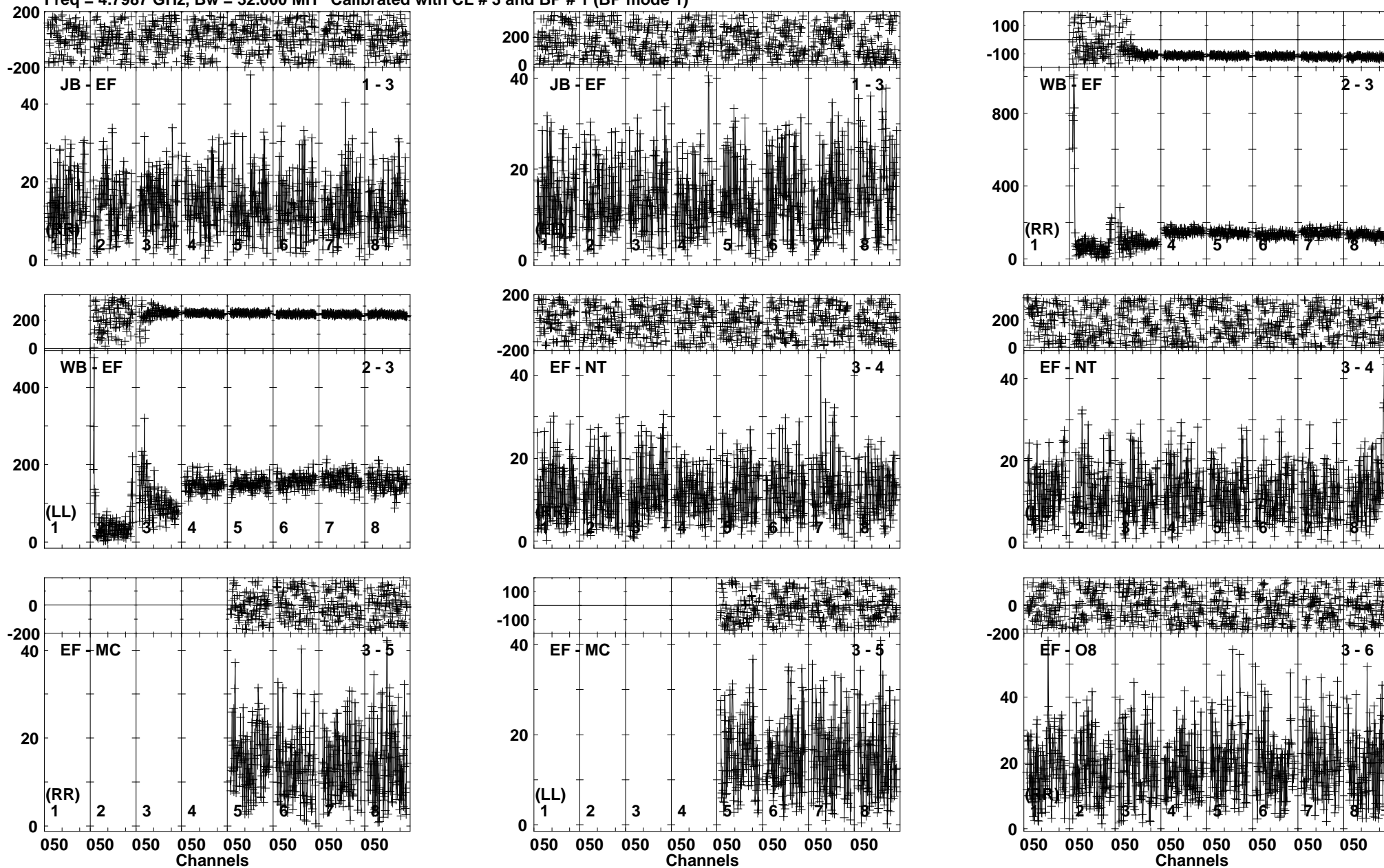
Lower frame: Milli Ampl Jy Top frame: Phas deg Vector averaged cross-power spectrum Baseline: JB (01) - EF (03) Timerange: 01/06:29:11 to 01/06:31:39
