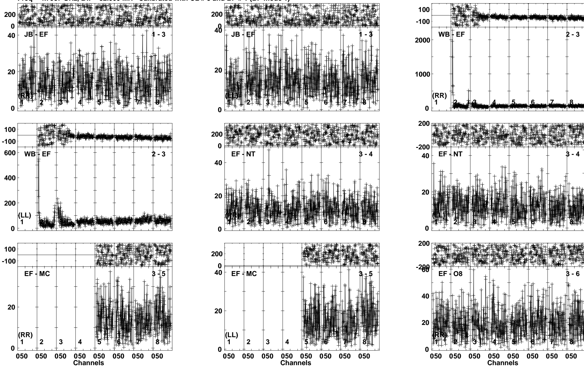
Lower frame: Milli Ampl Jy Top frame: Phas deg Vector averaged cross-power spectrum Baseline: JB (01) - EF (03) Timerange: 01/07:52:41 to 01/07:55:10
