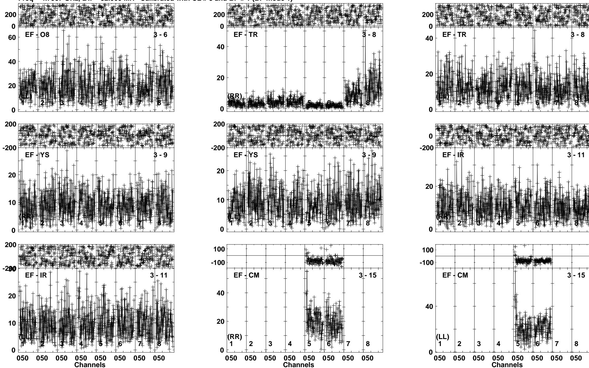
Lower frame: Milli Ampl Jy Top frame: Phas deg Vector averaged cross-power spectrum Baseline: EF (03) - O8 (06) Timerange: 01/06:57:01 to 01/06:59:29
