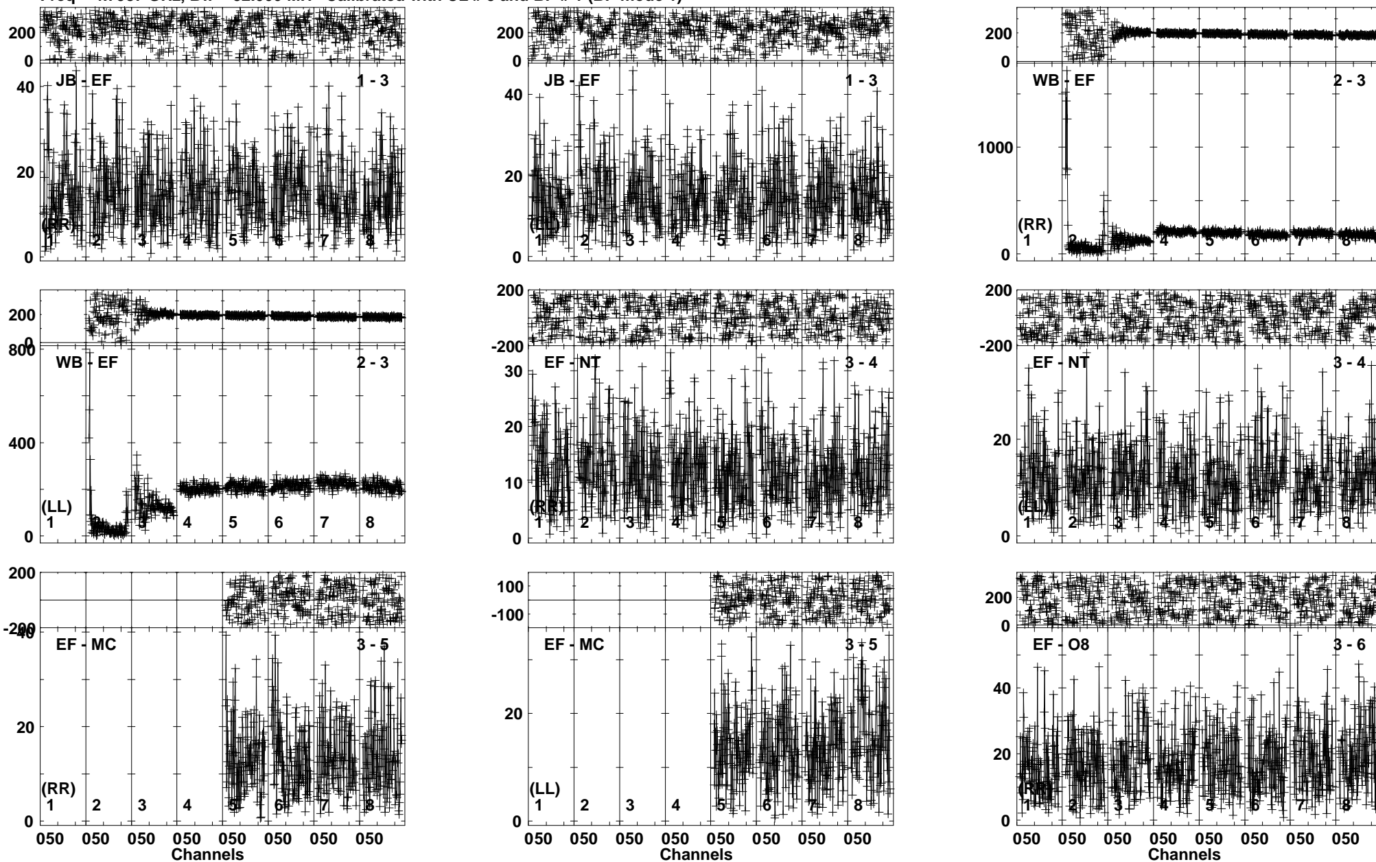
Lower frame: Milli Ampl Jy Top frame: Phas deg Vector averaged cross-power spectrum Baseline: JB (01) - EF (03) Timerange: 01/05:55:10 to 01/05:57:40
