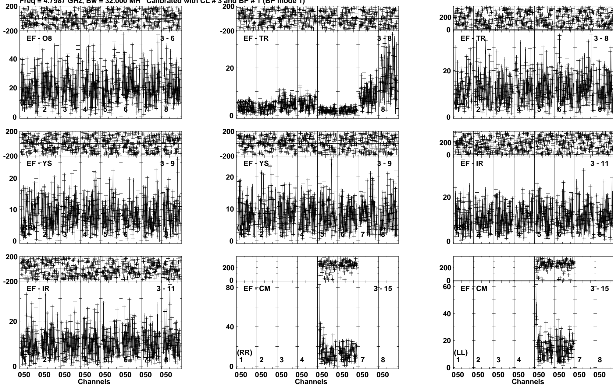
Lower frame: Milli Ampl Jy Top frame: Phas deg Vector averaged cross-power spectrum Baseline: EF (03) - O8 (06) Timerange: 01/08:01:30 to 01/08:04:00
