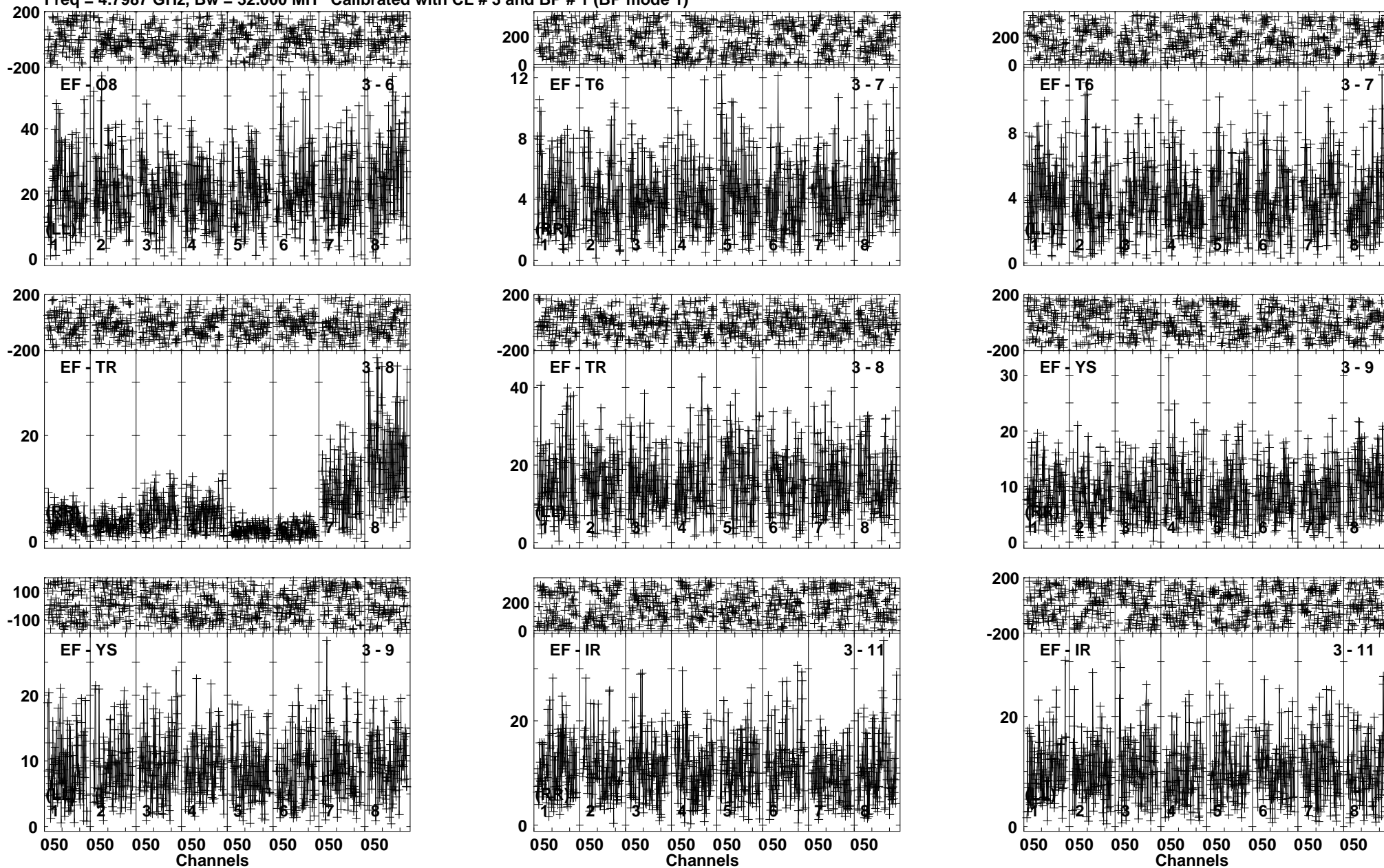
Lower frame: Milli Ampl Jy Top frame: Phas deg Vector averaged cross-power spectrum Baseline: EF (03) - O8 (06) Timerange: 01/01:08:20 to 01/01:10:50
