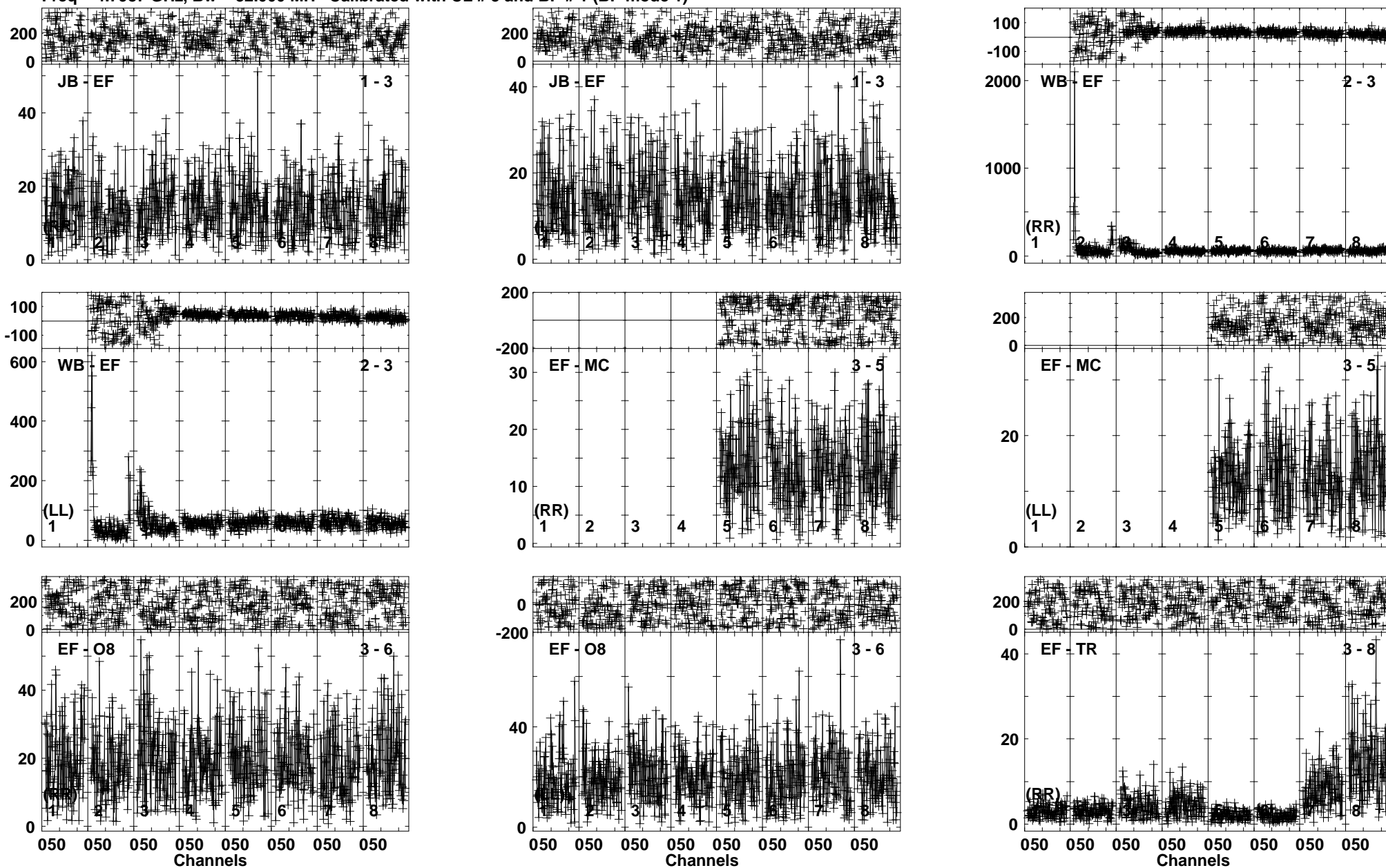
Lower frame: Milli Ampl Jy Top frame: Phas deg Vector averaged cross-power spectrum Baseline: JB (01) - EF (03) Timerange: 01/08:29:20 to 01/08:31:50
