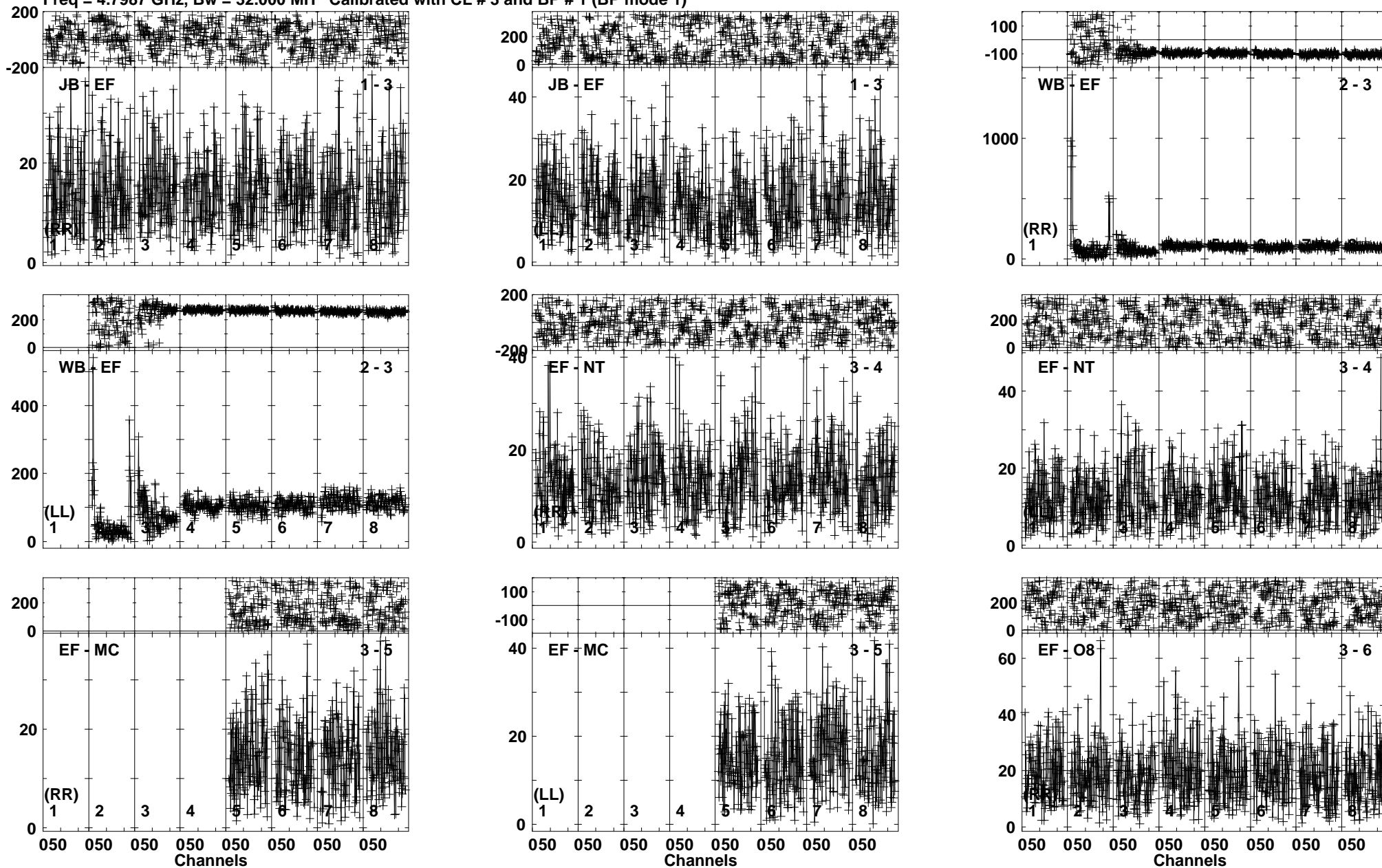
Lower frame: Milli Ampl Jy Top frame: Phas deg Vector averaged cross-power spectrum Baseline: JB (01) - EF (03) Timerange: 01/06:50:50 to 01/06:53:20
