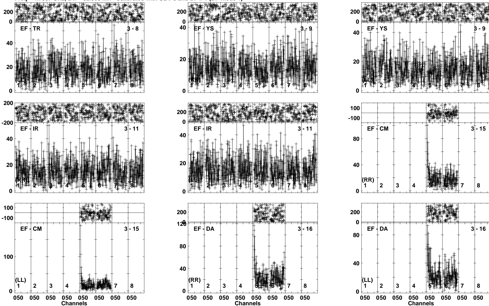
Lower frame: Milli Ampl Jy Top frame: Phas deg Vector averaged cross-power spectrum Baseline: EF (03) - TR (08) Timerange: 01/04:55:31 to 01/04:57:59
