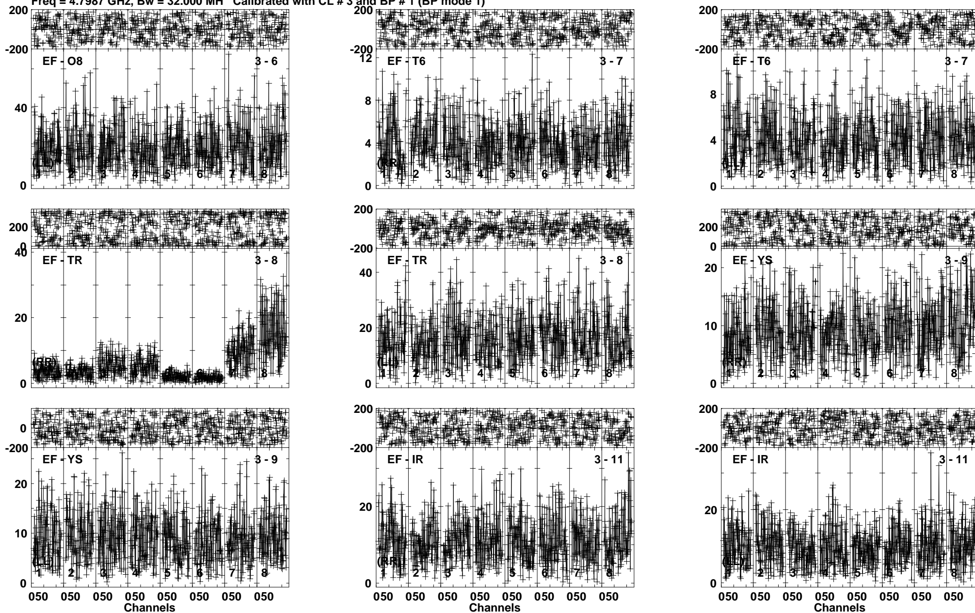
Lower frame: Milli Ampl Jy Top frame: Phas deg Vector averaged cross-power spectrum Baseline: EF (03) - O8 (06) Timerange: 01/01:12:21 to 01/01:14:49
