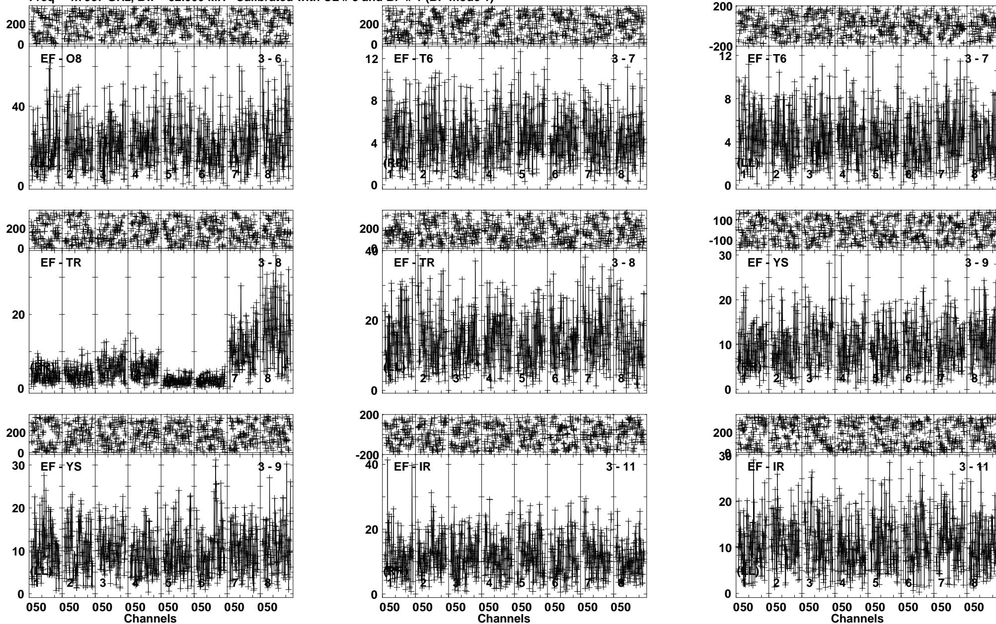
Lower frame: Milli Ampl Jy Top frame: Phas deg Vector averaged cross-power spectrum Baseline: EF (03) - O8 (06) Timerange: 01/03:08:31 to 01/03:10:59
