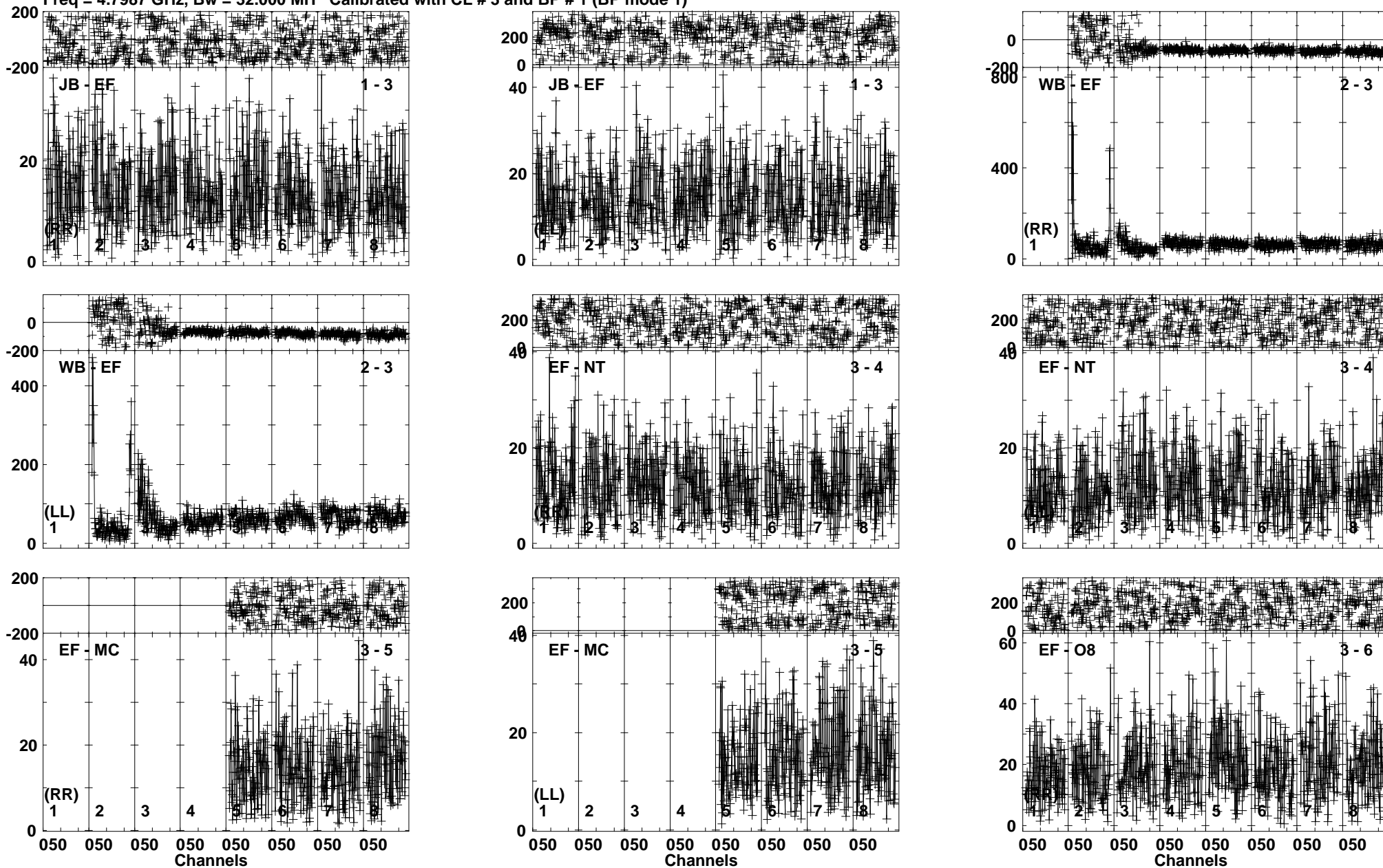
Lower frame: Milli Ampl Jy Top frame: Phas deg Vector averaged cross-power spectrum Baseline: JB (01) - EF (03) Timerange: 01/07:24:50 to 01/07:27:20
