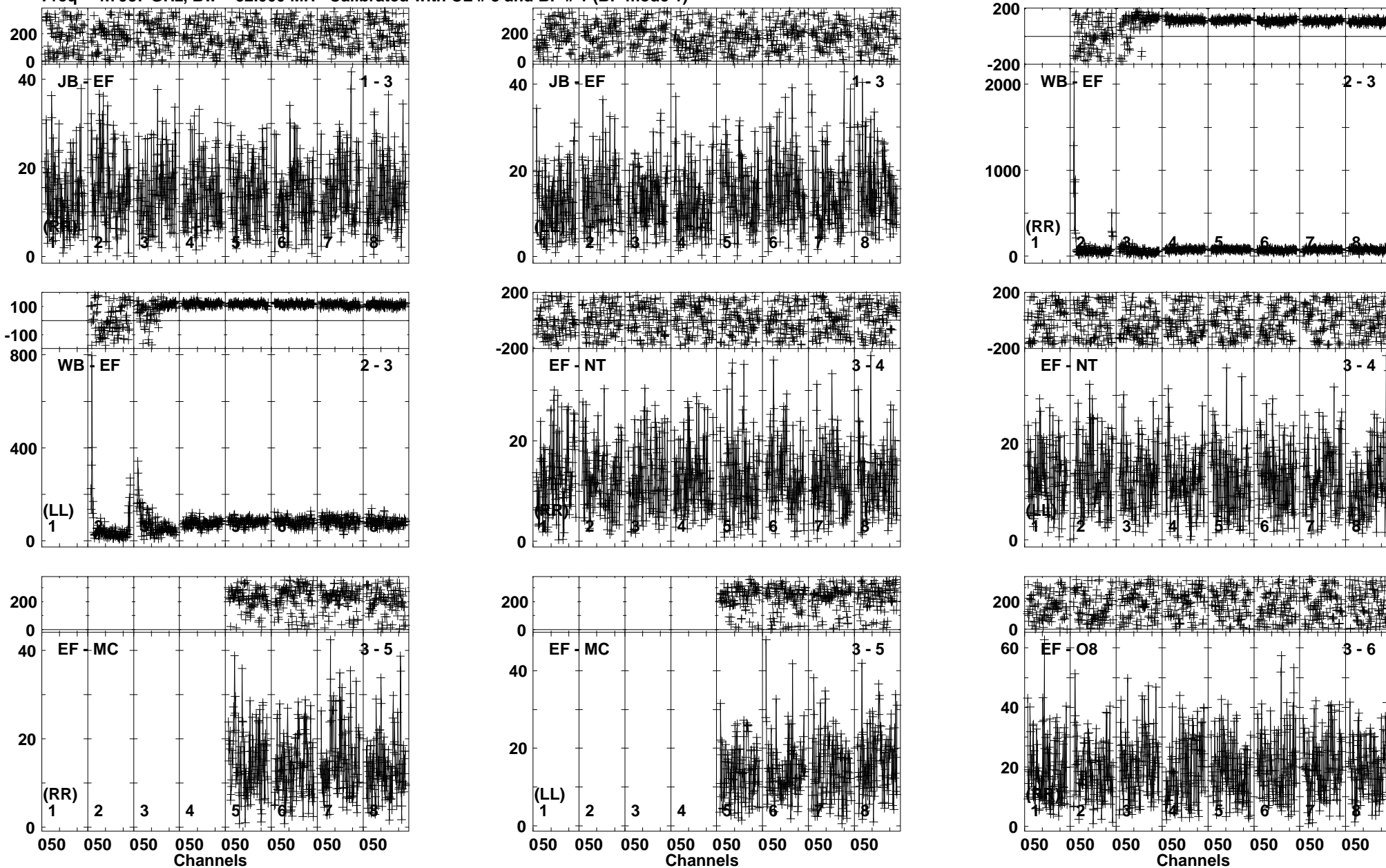
Lower frame: Milli Ampl Jy Top frame: Phas deg Vector averaged cross-power spectrum Baseline: JB (01) - EF (03) Timerange: 01/08:48:20 to 01/08:50:50
