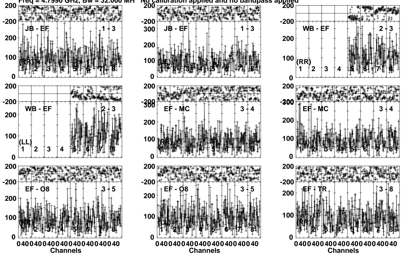
Lower frame: Micro Ampl Jy Top frame: Phas deg Vector averaged cross-power spectrum Several baselines displayed Timerange: 00/11:46:46 to 00/11:49:44
