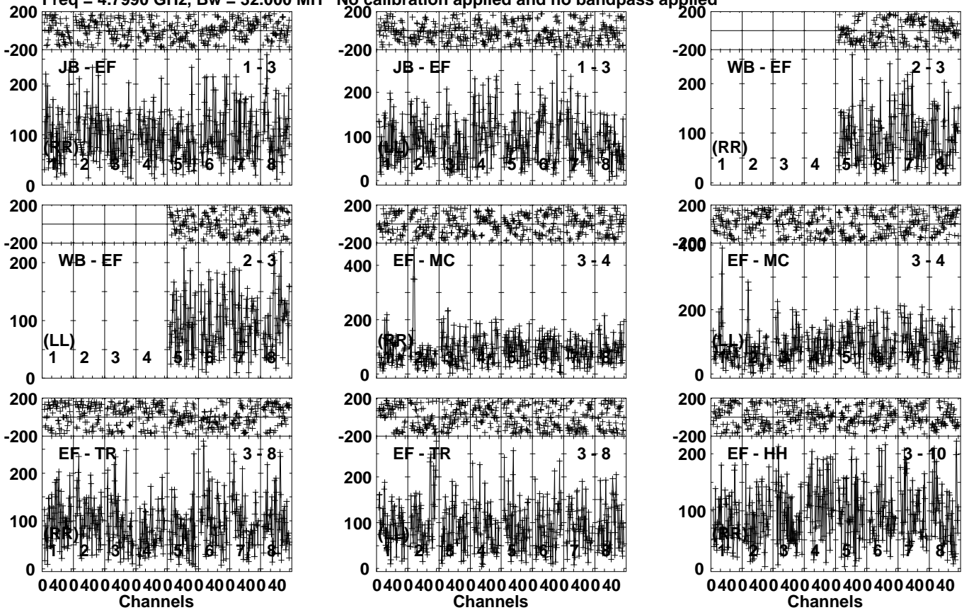
Lower frame: Micro Ampl Jy Top frame: Phas deg Vector averaged cross-power spectrum Several baselines displayed Timerange: 00/13:36:51 to 00/13:39:49
