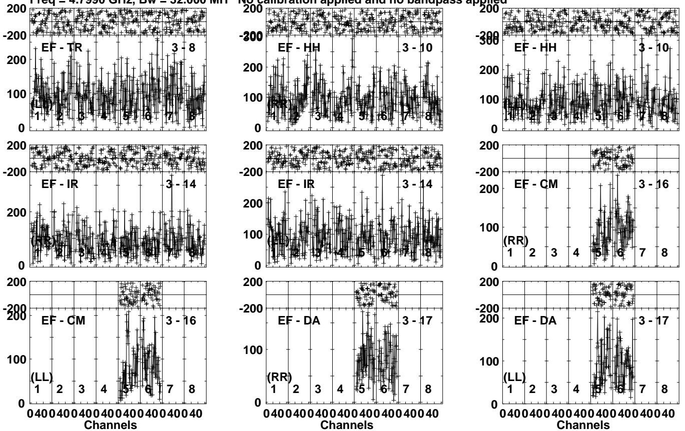
Lower frame: Micro Ampl Jy Top frame: Phas deg Vector averaged cross-power spectrum Several baselines displayed Timerange: 00/13:05:21 to 00/13:08:19
