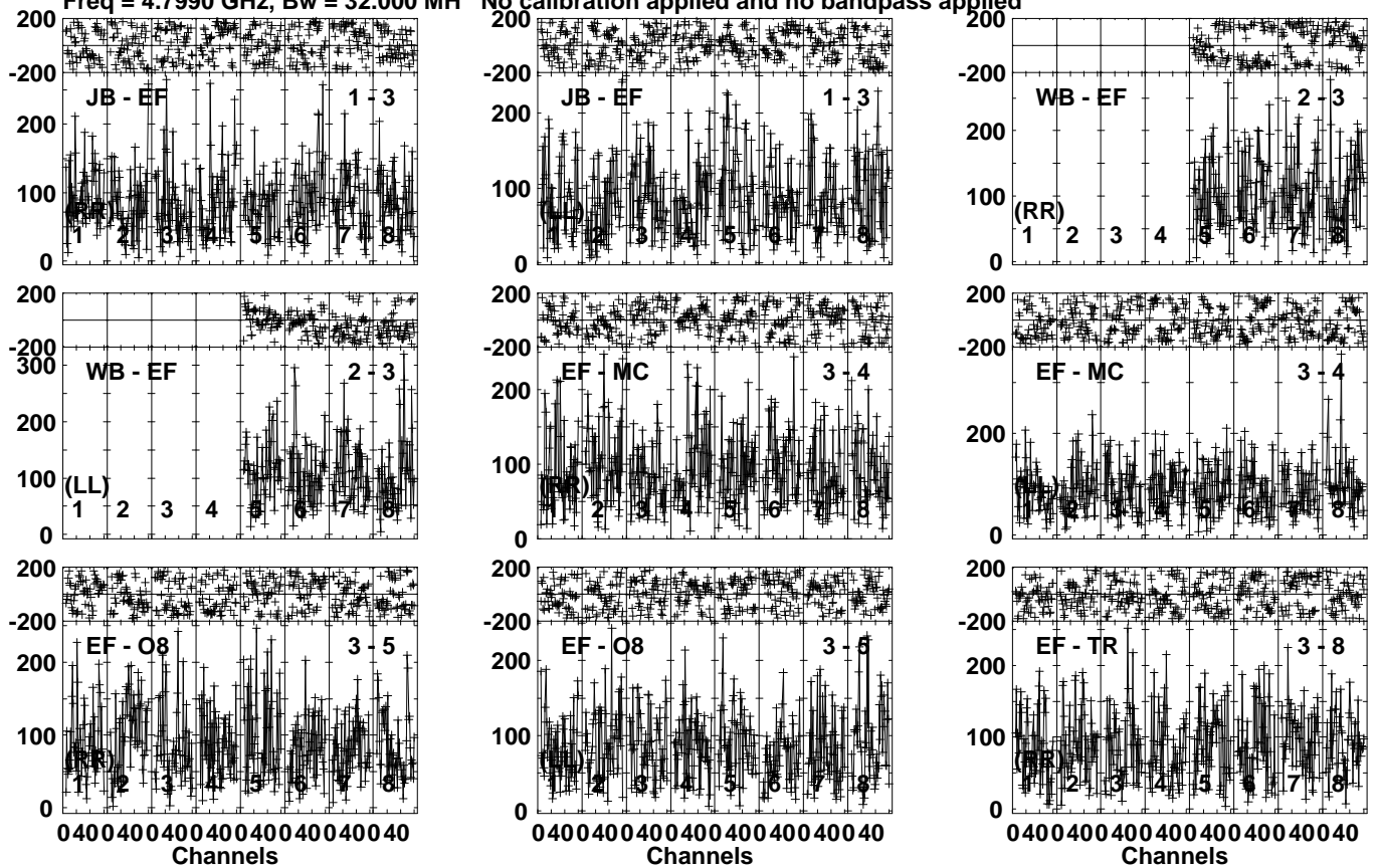
Lower frame: Micro Ampl Jy Top frame: Phas deg Vector averaged cross-power spectrum Several baselines displayed Timerange: 00/11:57:16 to 00/12:00:14
