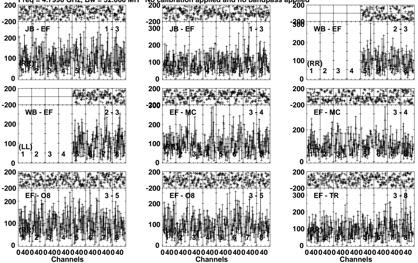
Lower frame: Micro Ampl Jy Top frame: Phas deg Vector averaged cross-power spectrum Several baselines displayed Timerange: 00/08:12:31 to 00/08:15:29
