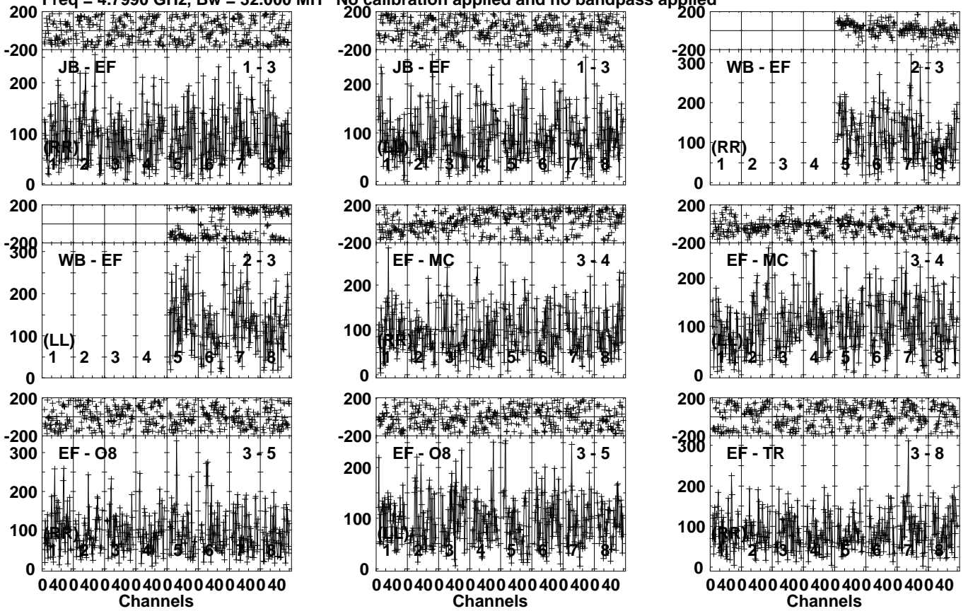
Lower frame: Micro Ampl Jy Top frame: Phas deg Vector averaged cross-power spectrum Several baselines displayed Timerange: 00/09:47:01 to 00/09:49:59
