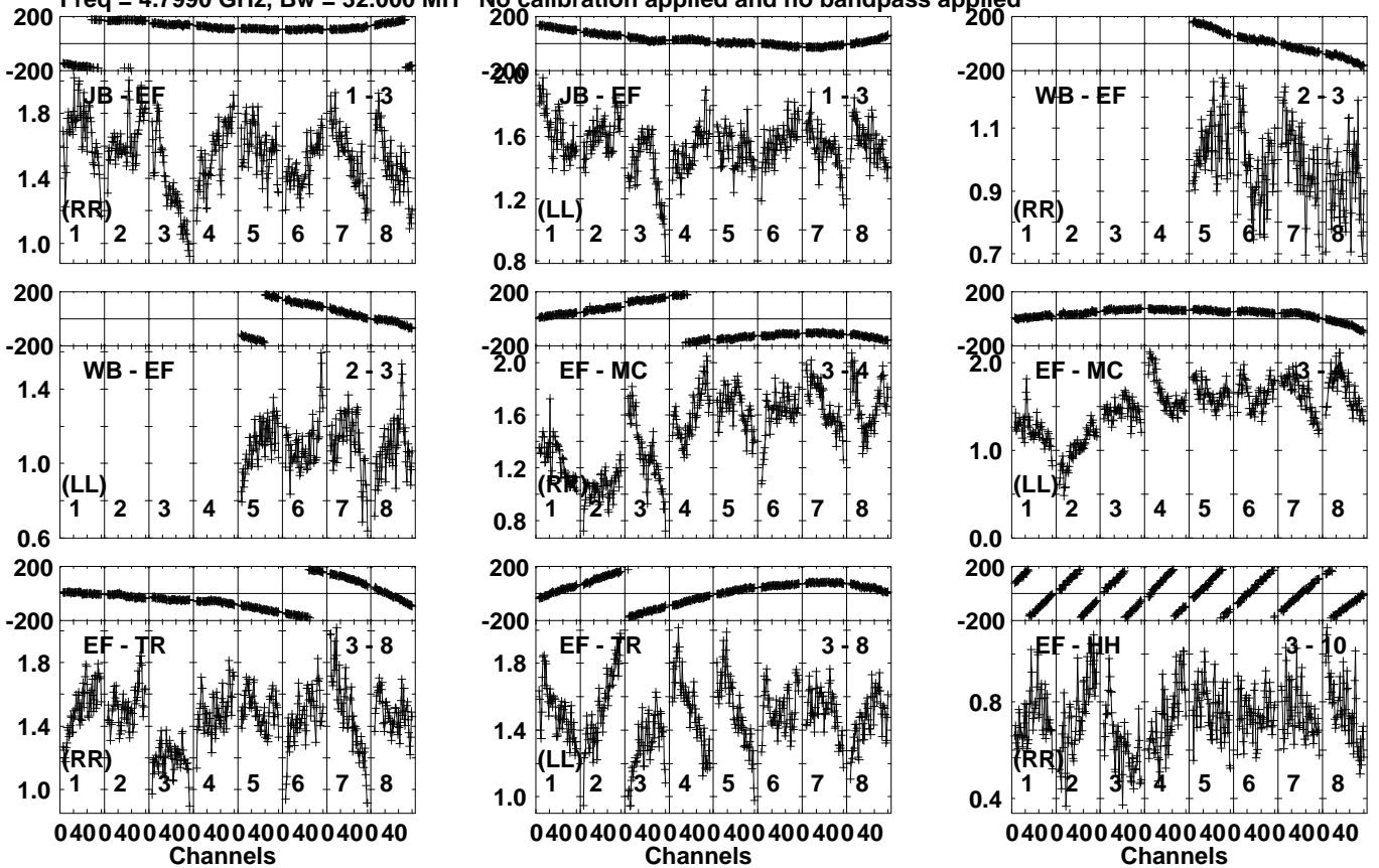
Lower frame: Milli Ampl Jy Top frame: Phas deg Vector averaged cross-power spectrum Several baselines displayed Timerange: 00/13:55:51 to 00/13:57:49
