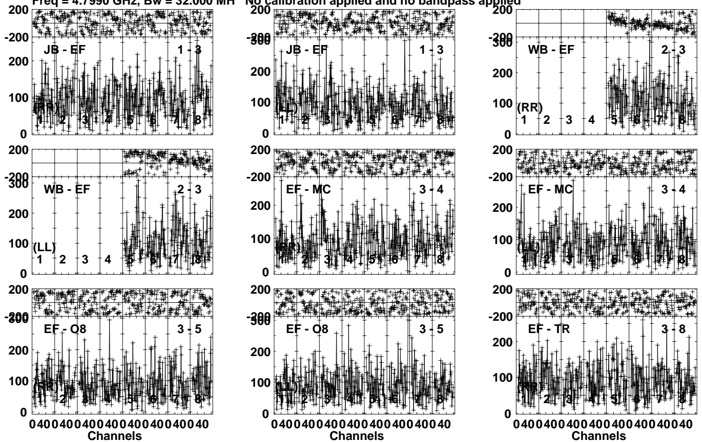
Lower frame: Micro Ampl Jy Top frame: Phas deg Vector averaged cross-power spectrum Several baselines displayed Timerange: 00/11:41:46 to 00/11:44:44
