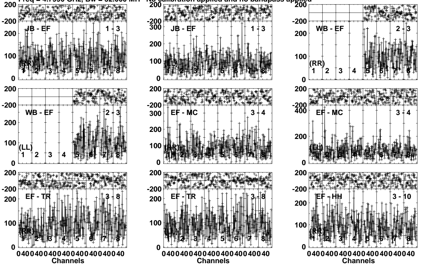
Lower frame: Micro Ampl Jy Top frame: Phas deg Vector averaged cross-power spectrum Several baselines displayed Timerange: 00/13:47:21 to 00/13:50:19
