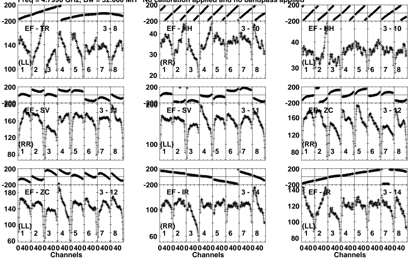
Lower frame: Milli Ampl Jy Top frame: Phas deg Vector averaged cross-power spectrum Several baselines displayed Timerange: 00/12:34:36 to 00/12:39:34
