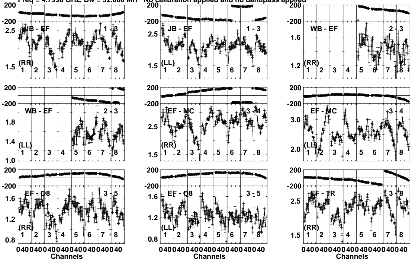
Lower frame: Milli Ampl Jy Top frame: Phas deg Vector averaged cross-power spectrum Several baselines displayed Timerange: 00/10:58:31 to 00/11:00:29
