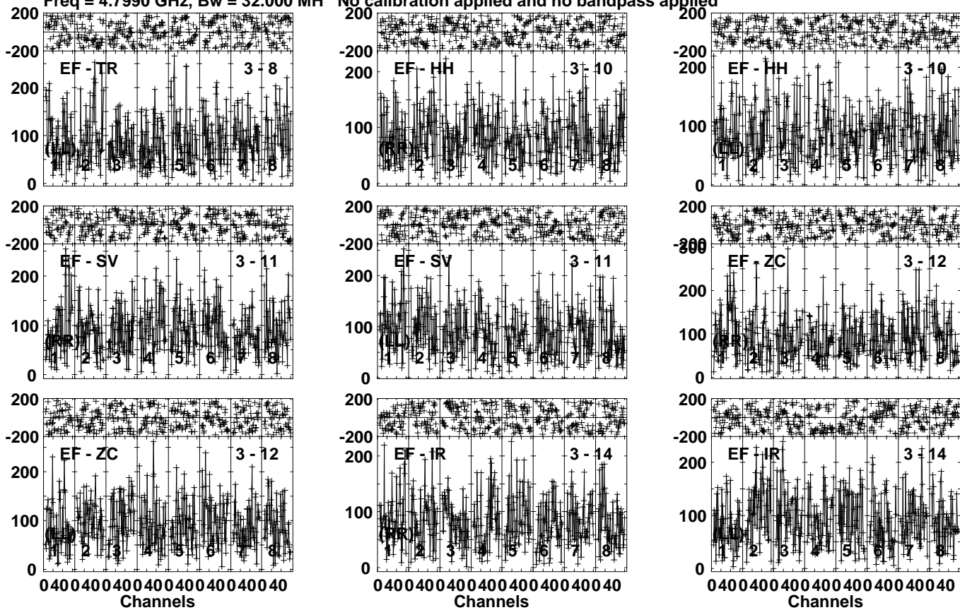
Lower frame: Micro Ampl Jy Top frame: Phas deg Vector averaged cross-power spectrum Several baselines displayed Timerange: 00/09:20:31 to 00/09:23:29
