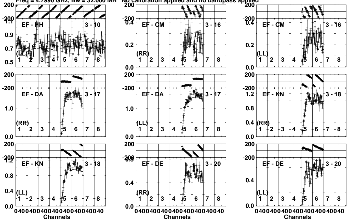
Lower frame: Milli Ampl Jy Top frame: Phas deg Vector averaged cross-power spectrum Several baselines displayed Timerange: 00/13:50:51 to 00/13:52:49
