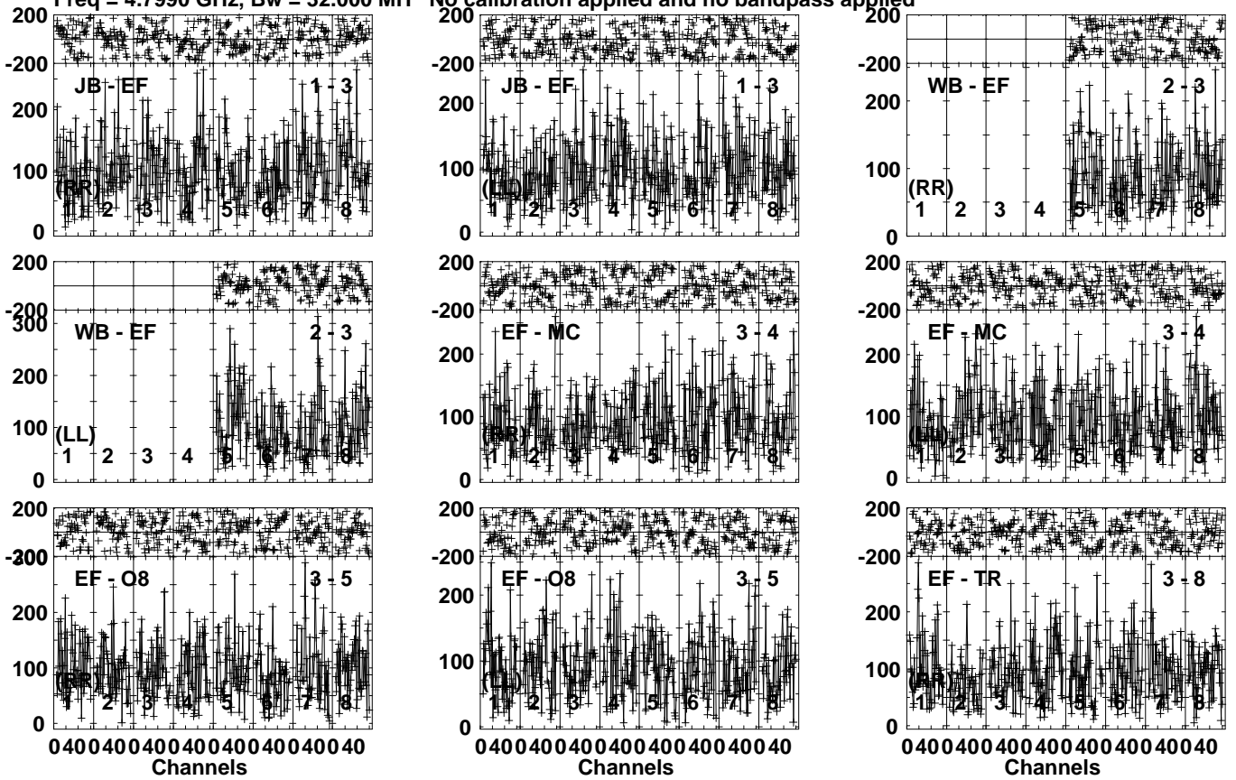
Lower frame: Micro Ampl Jy Top frame: Phas deg Vector averaged cross-power spectrum Several baselines displayed Timerange: 00/08:02:01 to 00/08:04:59
