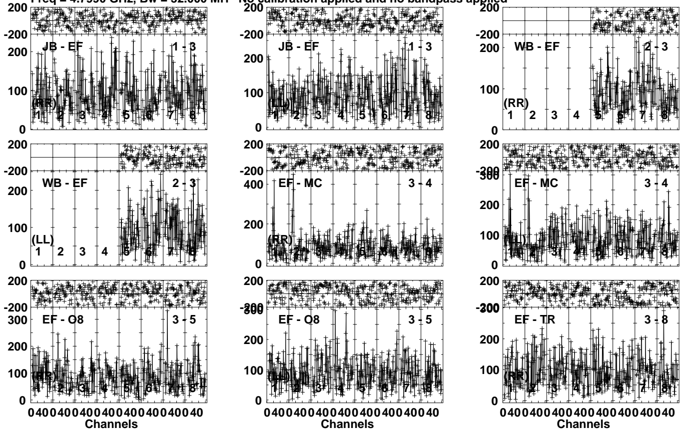
Lower frame: Micro Ampl Jy Top frame: Phas deg Vector averaged cross-power spectrum Several baselines displayed Timerange: 00/13:26:21 to 00/13:29:19
