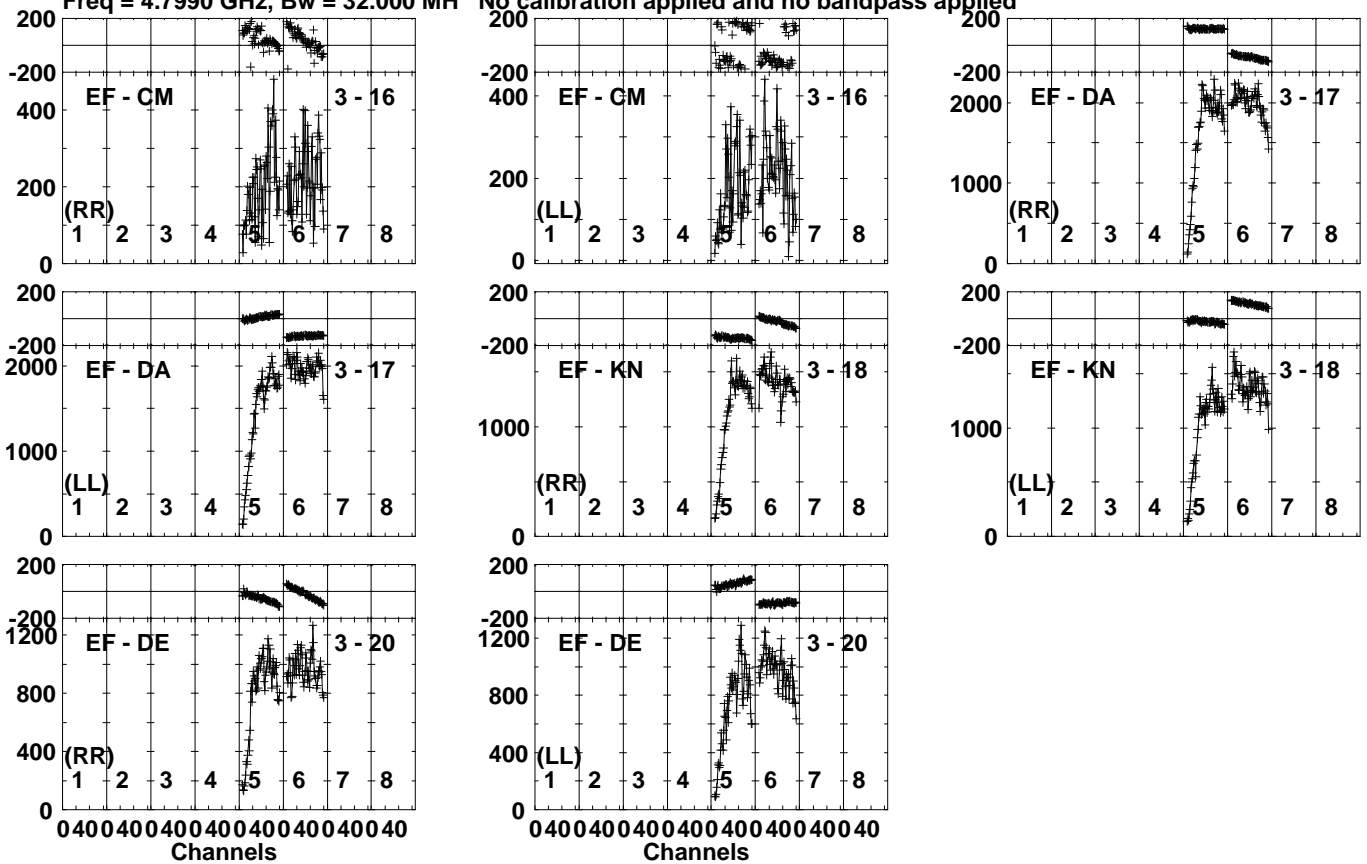
Lower frame: Micro Ampl Jy Top frame: Phas deg Vector averaged cross-power spectrum Several baselines displayed Timerange: 00/10:21:31 to 00/10:23:29
