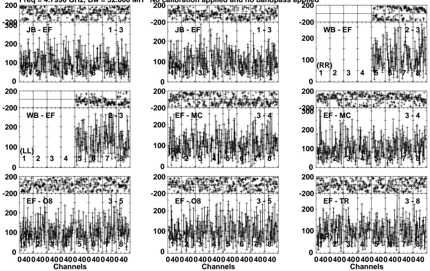
Lower frame: Micro Ampl Jy Top frame: Phas deg Vector averaged cross-power spectrum Several baselines displayed Timerange: 00/11:05:31 to 00/11:08:29
