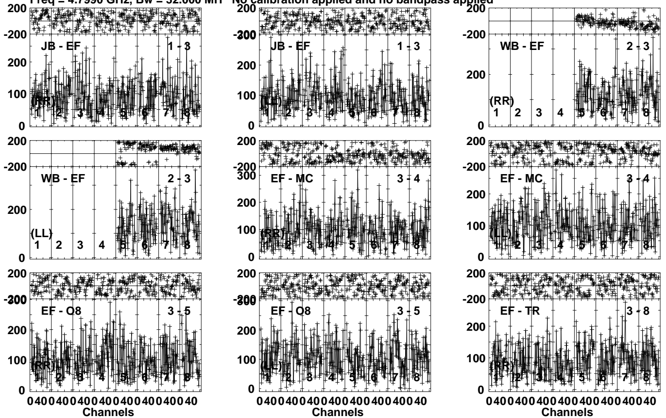
Lower frame: Micro Ampl Jy Top frame: Phas deg Vector averaged cross-power spectrum Several baselines displayed Timerange: 00/10:50:01 to 00/10:52:59
