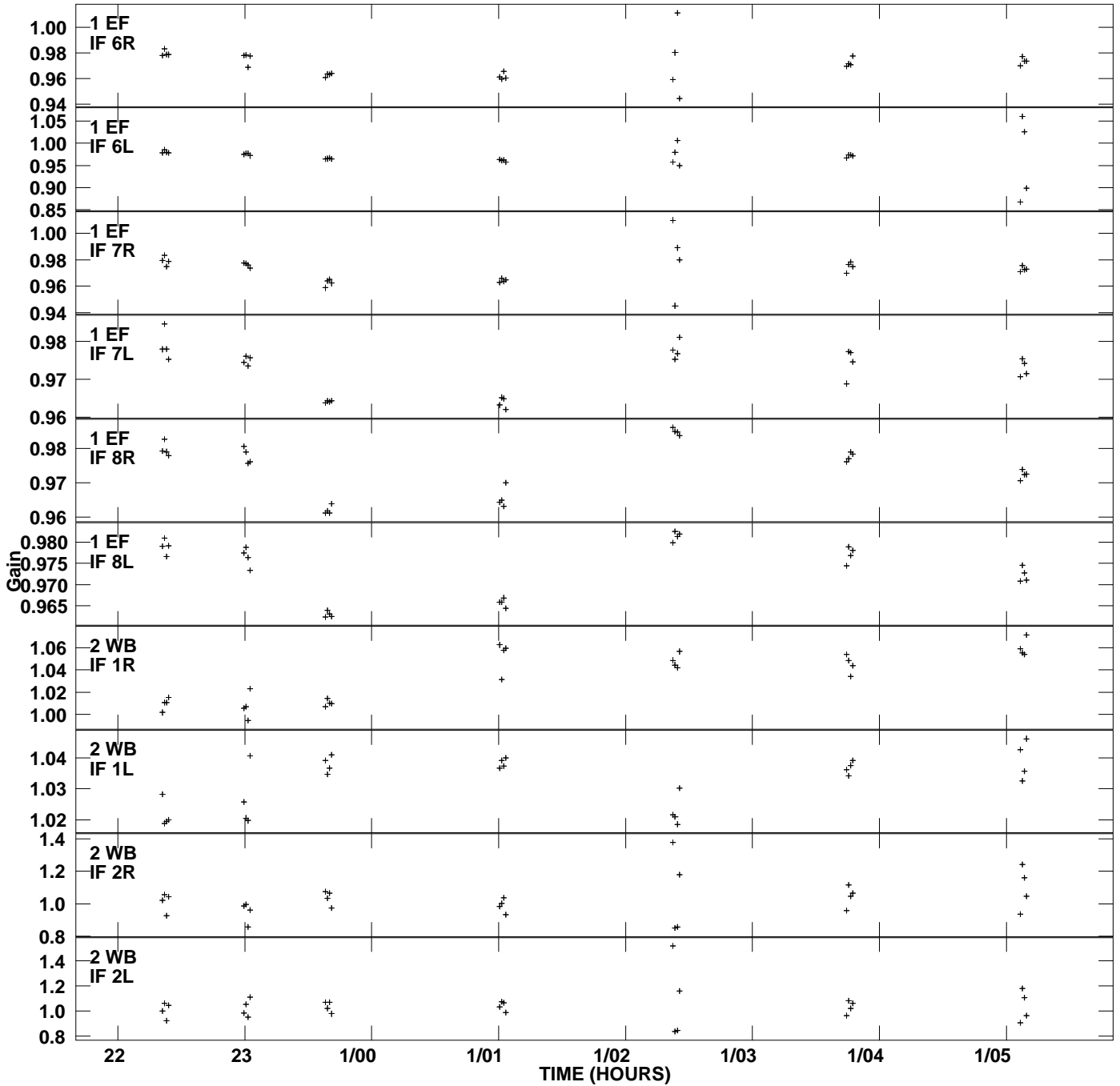
Plot file version 2 created 17-JUL-2014 15:03:54 Gain amp vs UTC time for J1256.MULTI.1 SN 4 Rpol & Lpol IF 1 - 8
